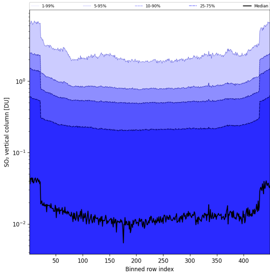
Figure 85: Along track statistics of “SO 2 vertical column” for 2025-08-10 to 2025-08-11
