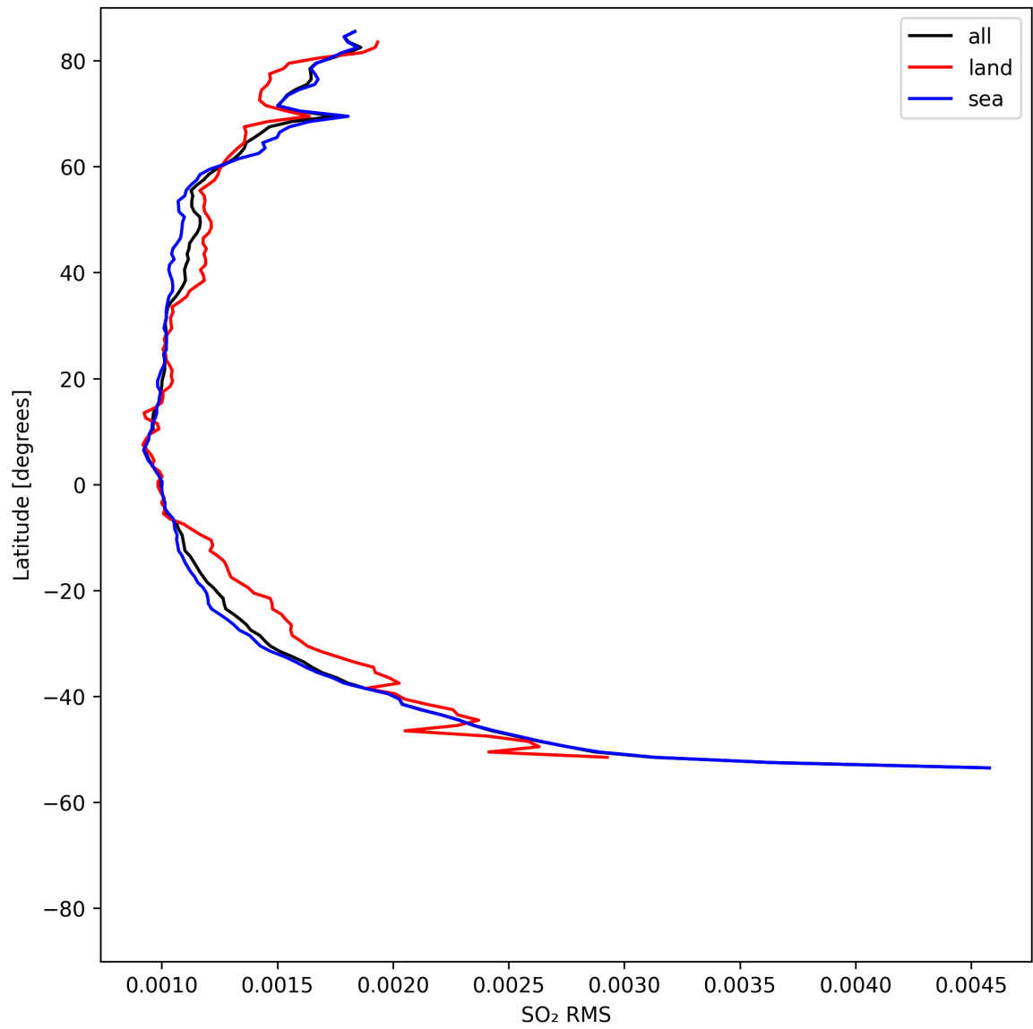
Figure 52: Zonal average of “SO 2 RMS” for 2025-08-10 to 2025-08-11.
