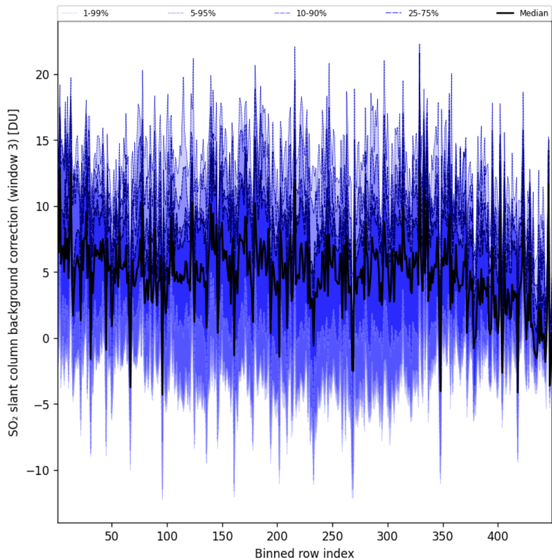
Figure 101: Along track statistics of “SO 2 slant column background correction (window 3)” for 2025-08-10 to 2025-08-11
