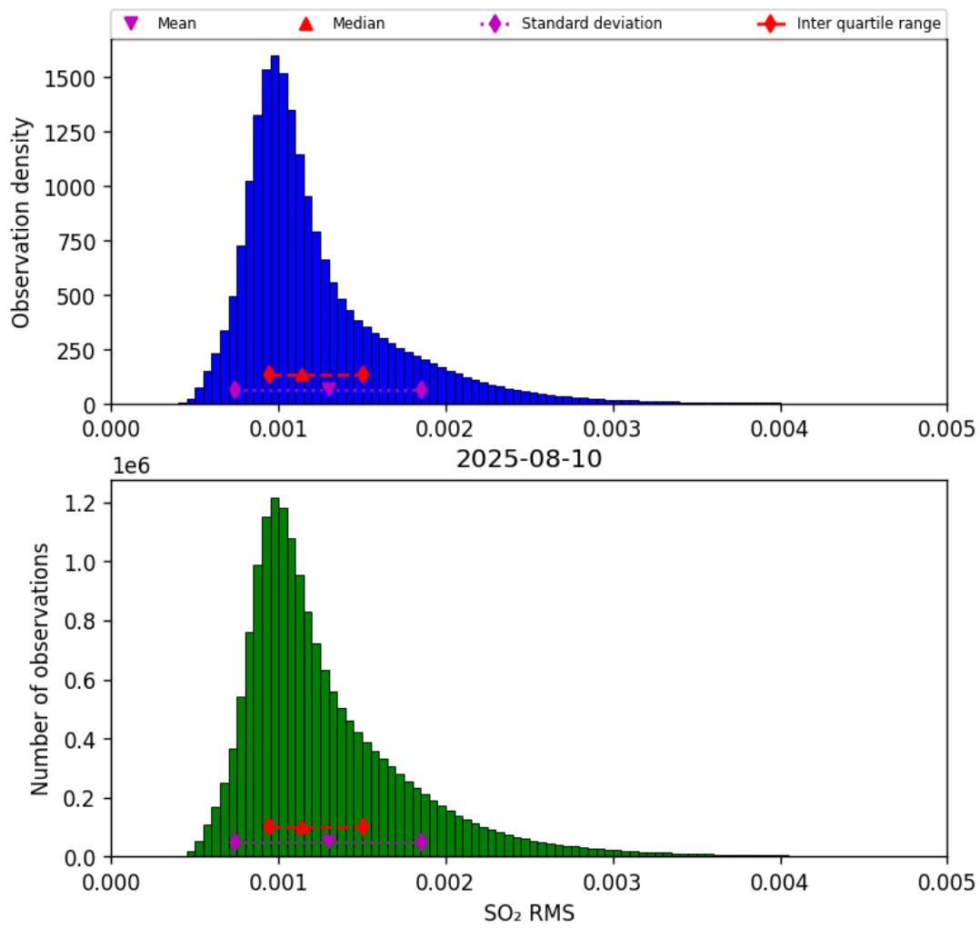
Figure 79: Histogram of “SO 2 RMS” for 2025-08-10 to 2025-08-11
