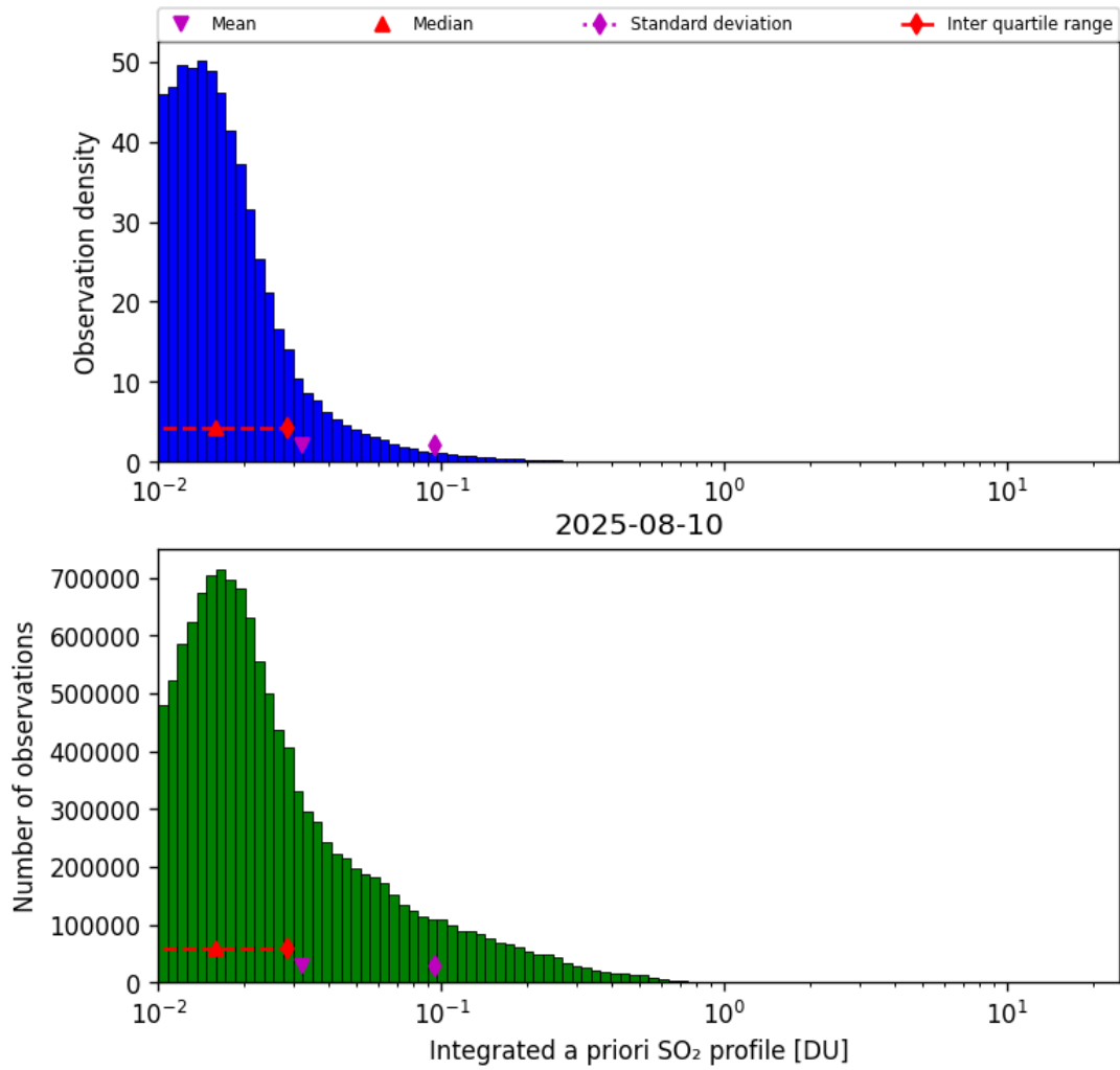
Figure 76: Histogram of “Integrated a priori SO 2 profile” for 2025-08-10 to 2025-08-11
