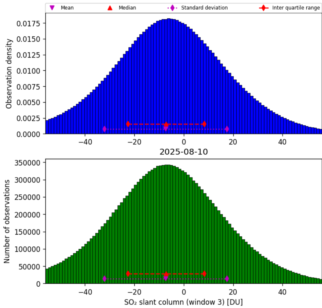
Figure 71: Histogram of “SO 2 slant column (window 3)” for 2025-08-10 to 2025-08-11
