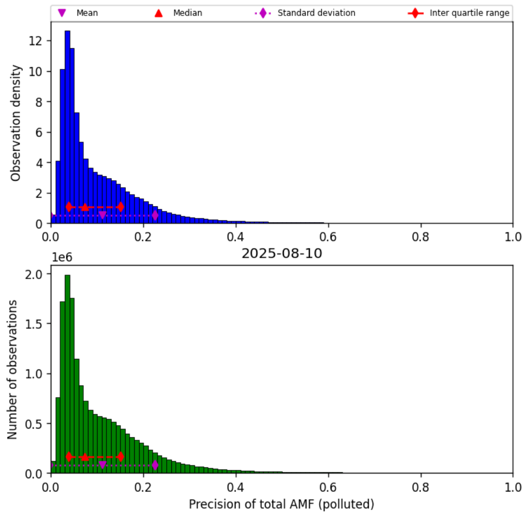
Figure 81: Histogram of “Precision of total AMF (polluted)” for 2025-08-10 to 2025-08-11
