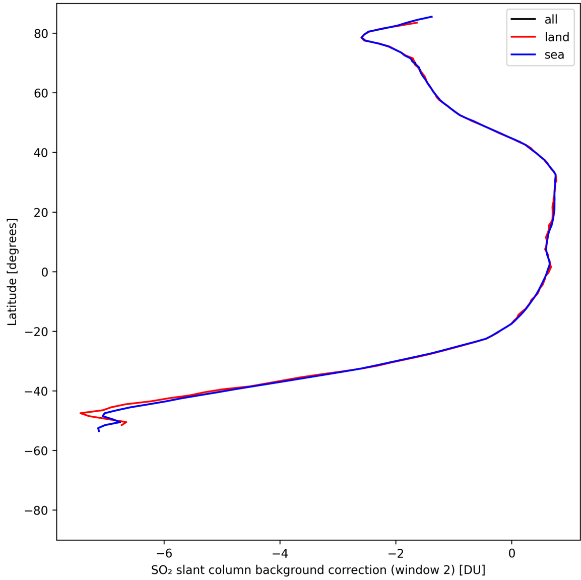
Figure 43: Zonal average of “SO 2 slant column background correction (window 2)” for 2025-08-10 to 2025-08-11.
