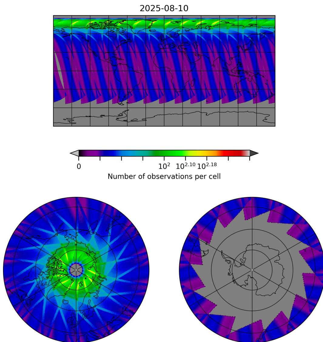
Figure 29: Map of the number of observations for 2025-08-10 to 2025-08-11
