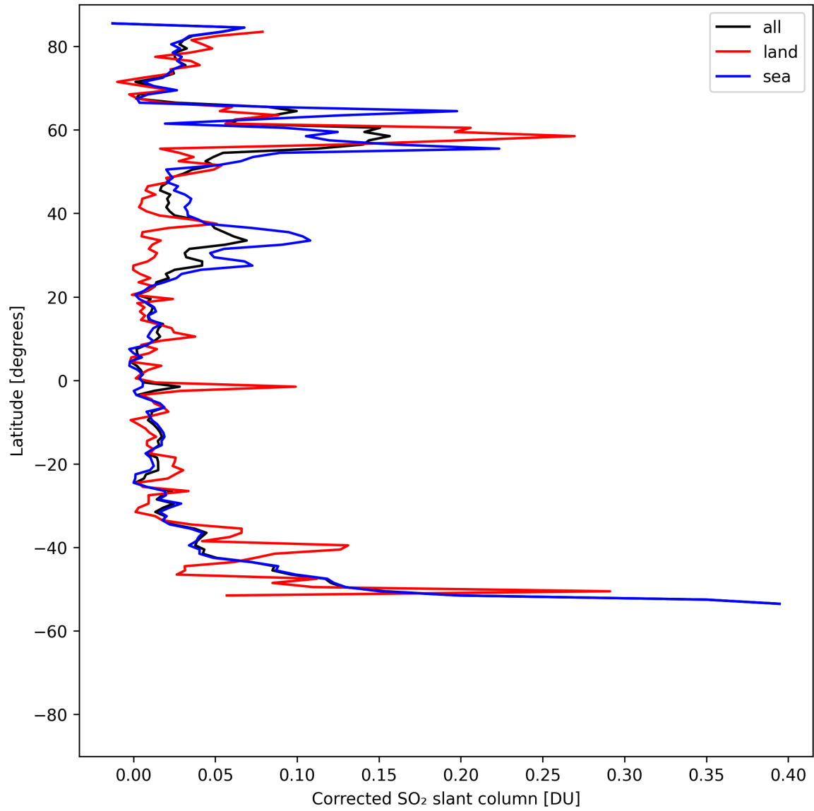
Figure 33: Zonal average of “Corrected SO 2 slant column” for 2025-08-10 to 2025-08-11.
