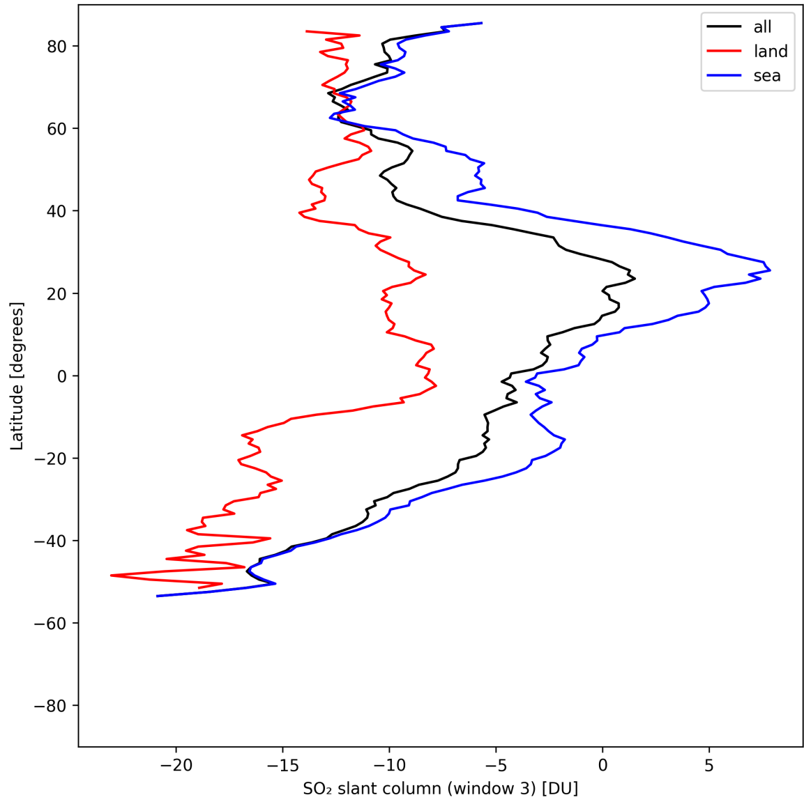
Figure 44: Zonal average of “SO 2 slant column (window 3)” for 2025-08-10 to 2025-08-11.
