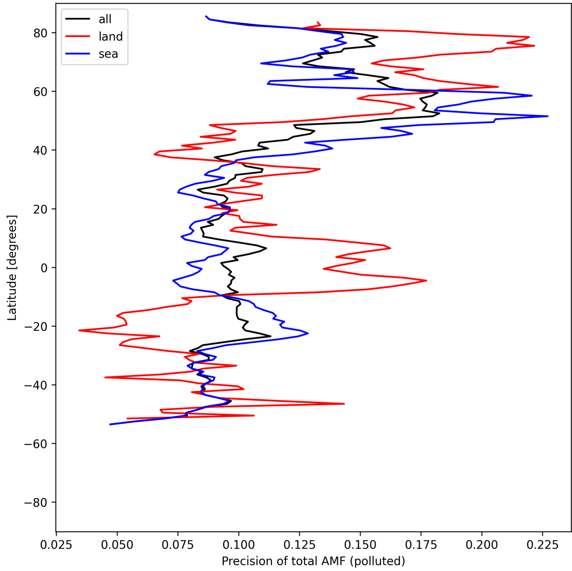
Figure 54: Zonal average of “Precision of total AMF (polluted)” for 2025-08-10 to 2025-08-11.
