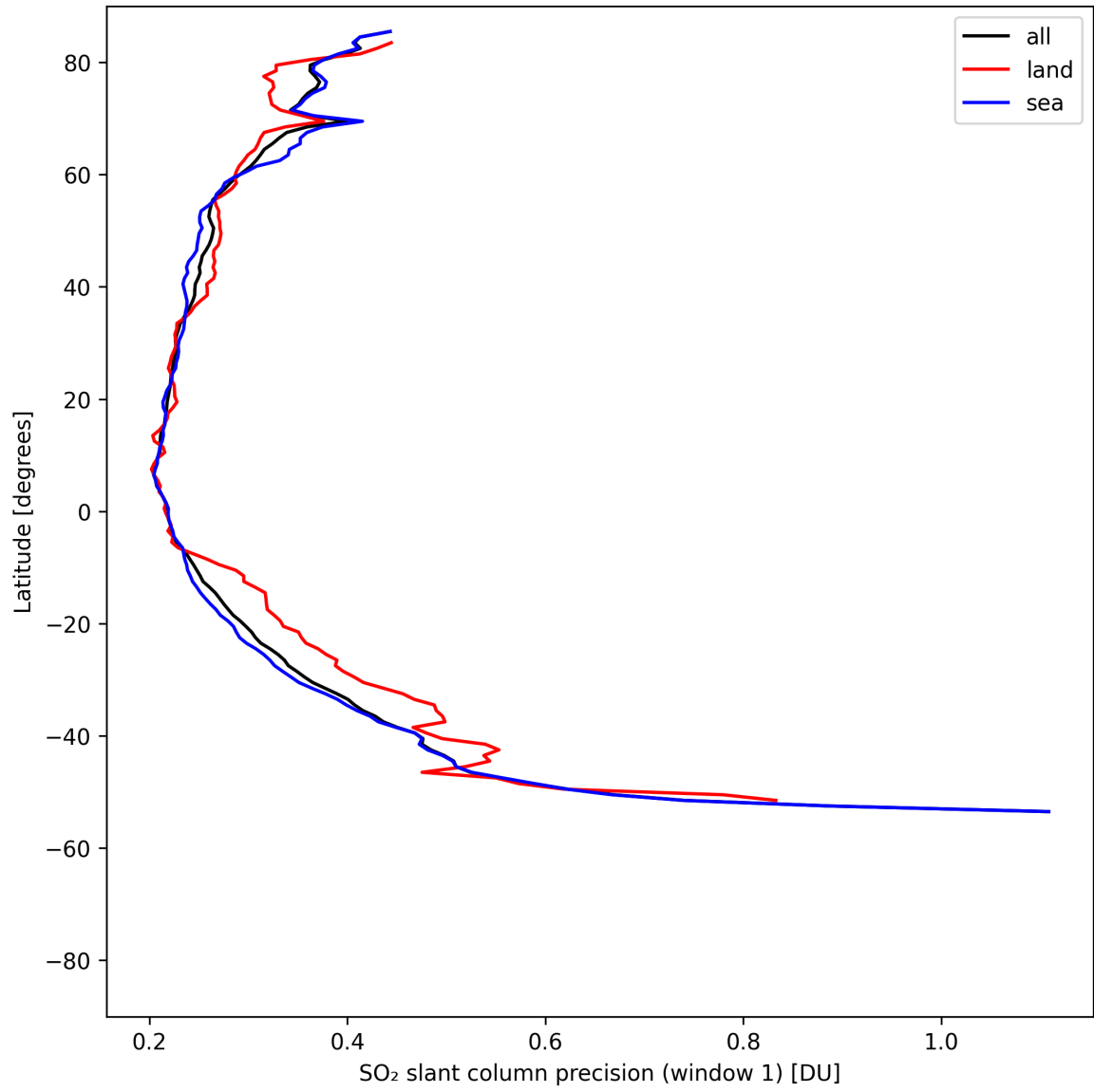
Figure 37: Zonal average of “SO 2 slant column precision (window 1)” for 2025-08-10 to 2025-08-11.
