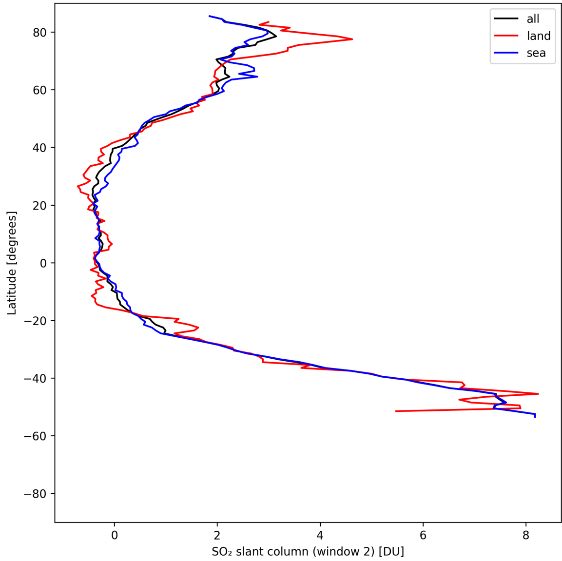
Figure 40: Zonal average of “SO 2 slant column (window 2)” for 2025-08-10 to 2025-08-11.
