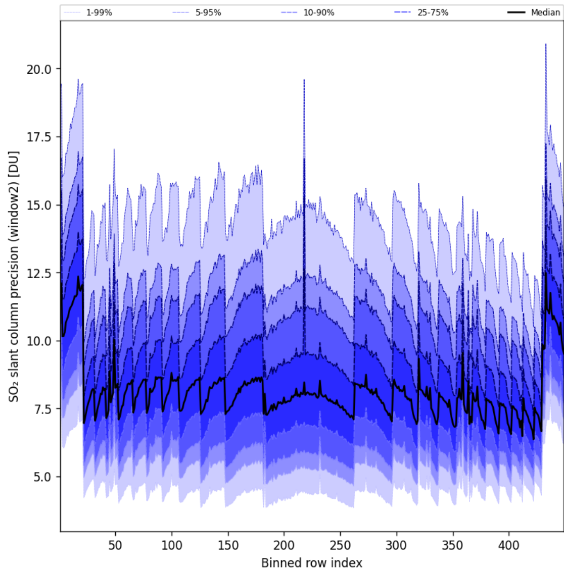
Figure 95: Along track statistics of “SO 2 slant column precision (window2)” for 2025-08-10 to 2025-08-11
