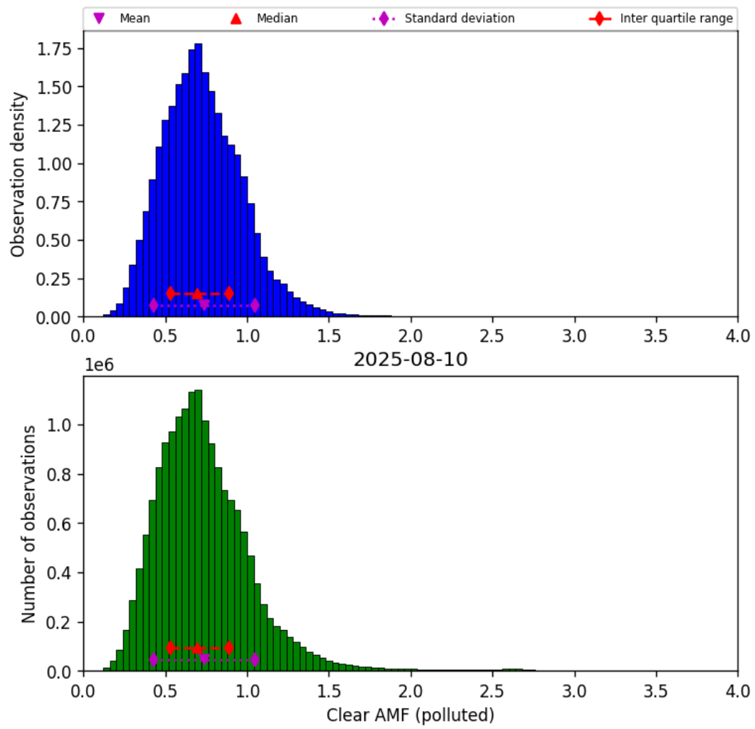
Figure 82: Histogram of “Clear AMF (polluted)” for 2025-08-10 to 2025-08-11
