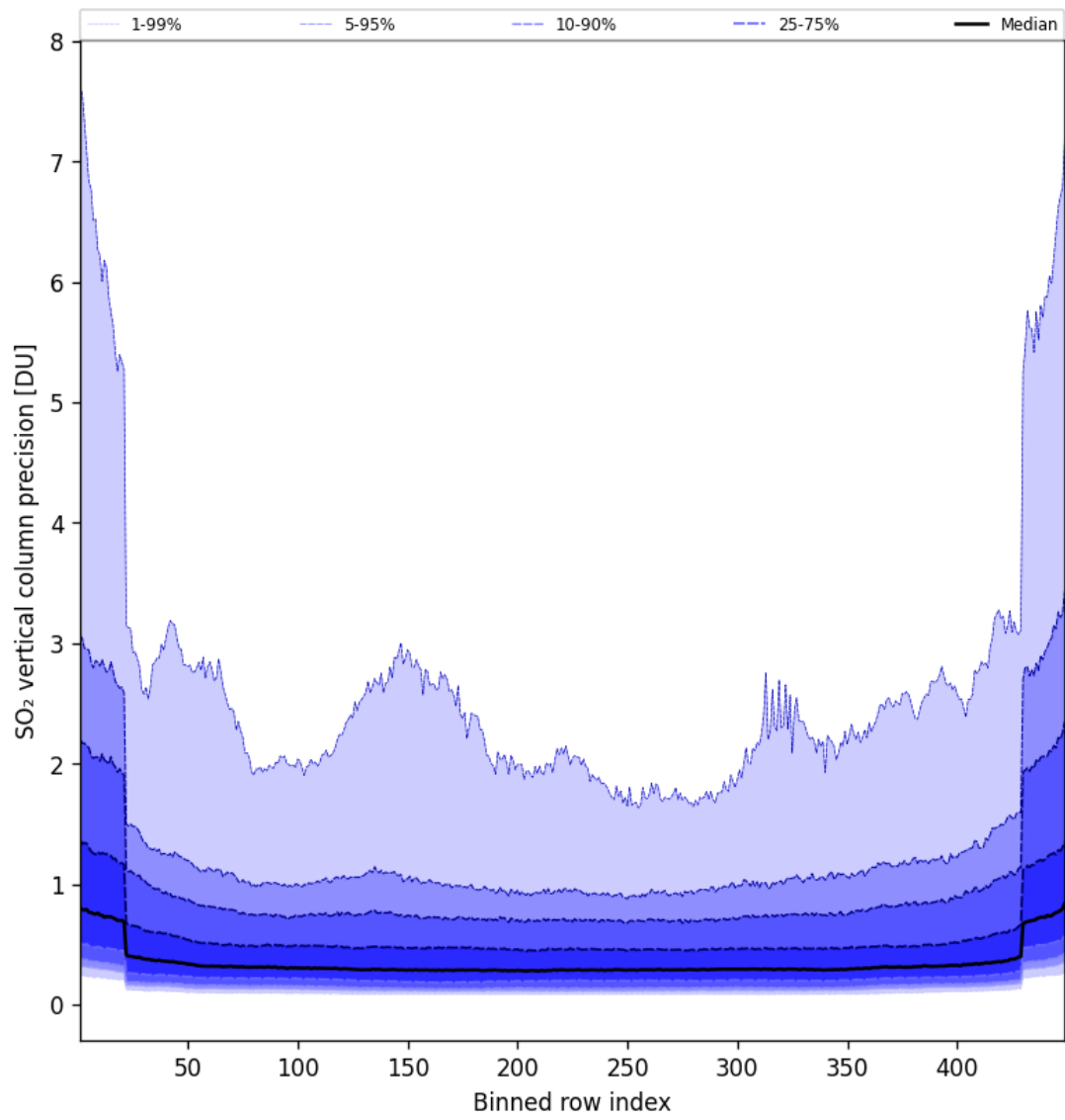
Figure 86: Along track statistics of “SO 2 vertical column precision” for 2025-08-10 to 2025-08-11
