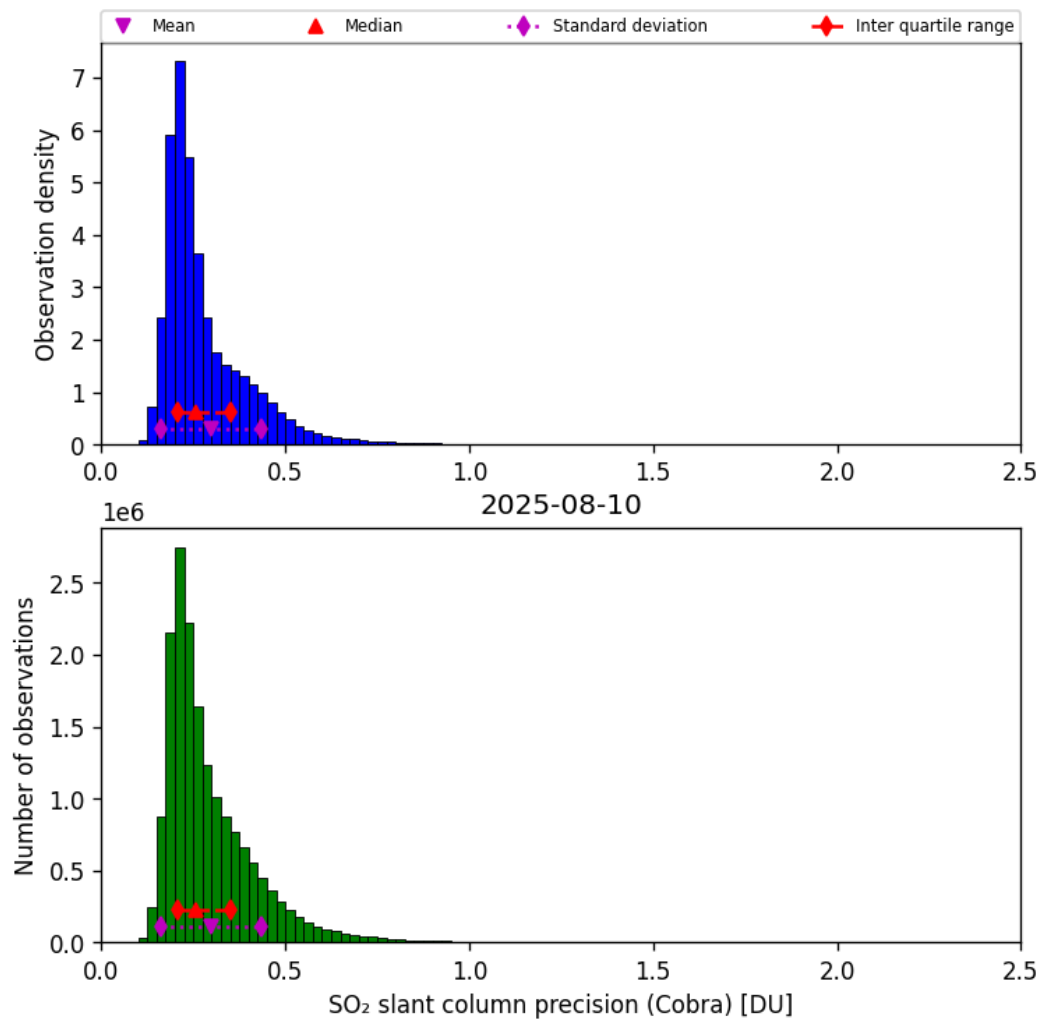
Figure 62: Histogram of “SO 2 slant column precision (Cobra)” for 2025-08-10 to 2025-08-11
