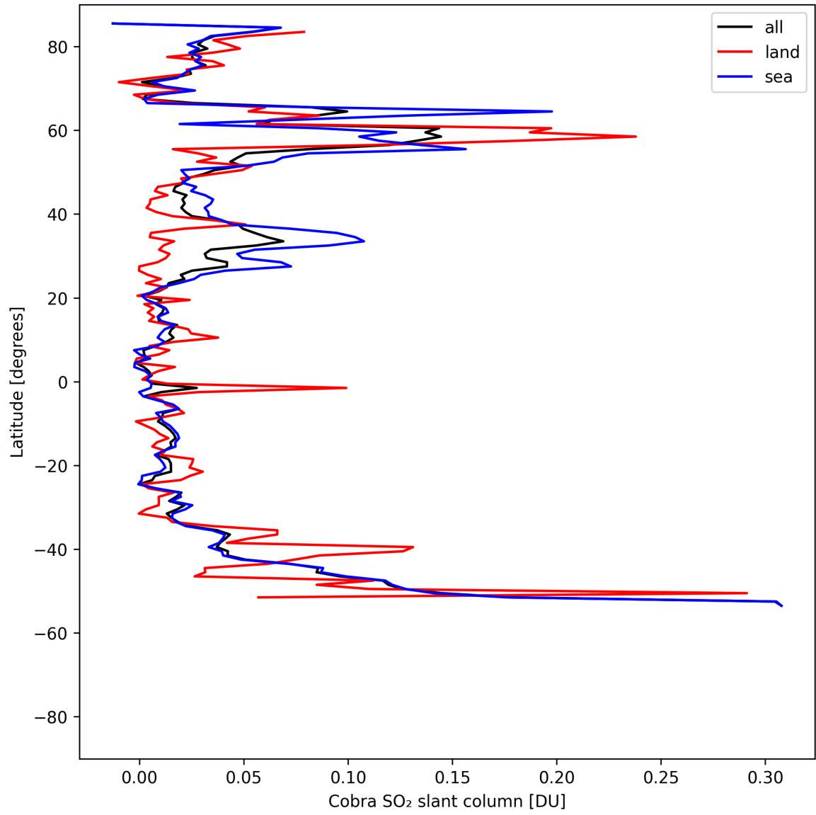
Figure 34: Zonal average of “Cobra SO 2 slant column” for 2025-08-10 to 2025-08-11.
