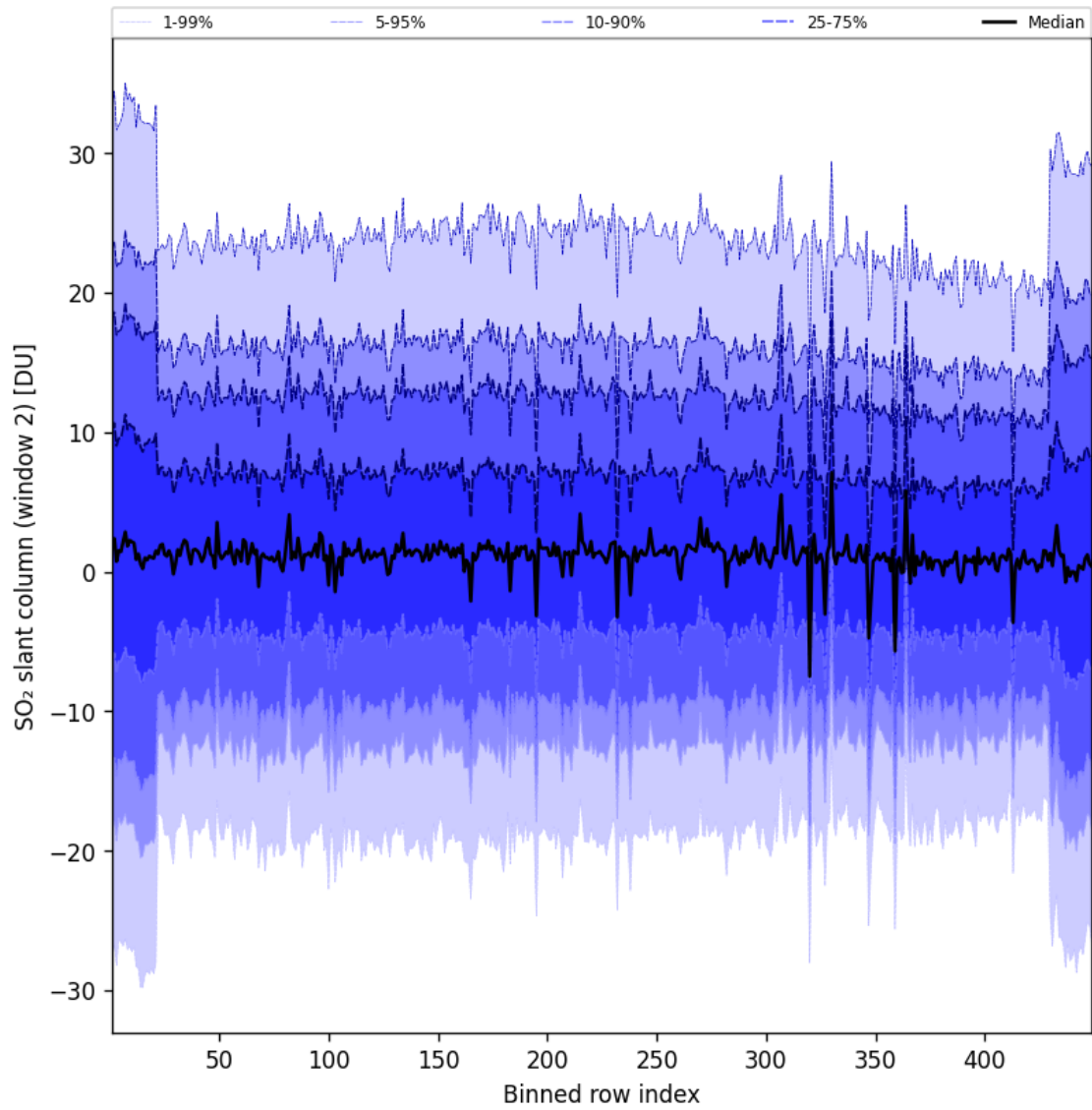
Figure 94: Along track statistics of “SO 2 slant column (window 2)” for 2025-08-10 to 2025-08-11
