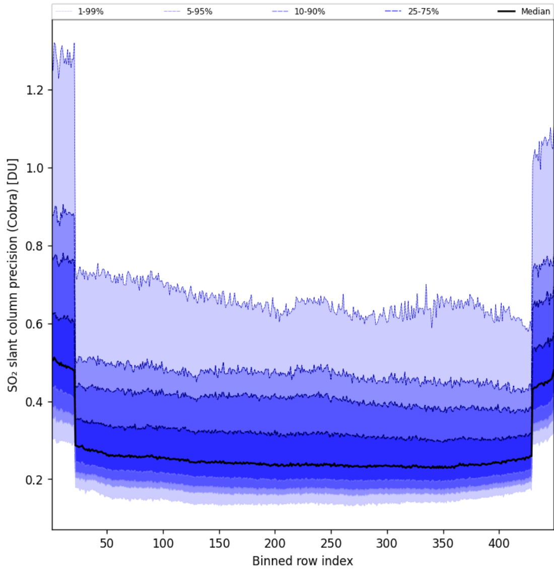
Figure 89: Along track statistics of “SO 2 slant column precision (Cobra)” for 2025-08-10 to 2025-08-11
