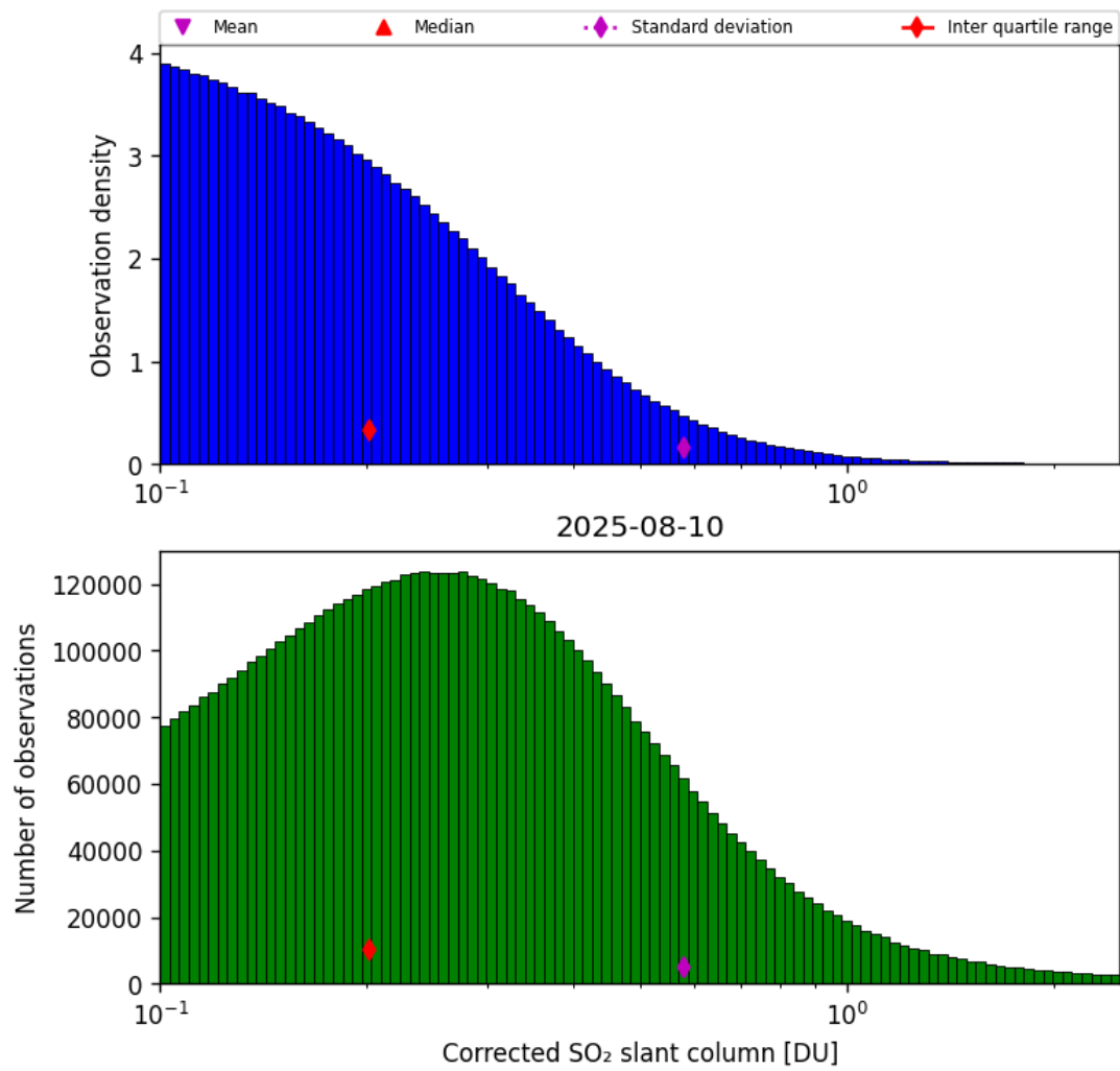
Figure 60: Histogram of “Corrected SO 2 slant column” for 2025-08-10 to 2025-08-11
