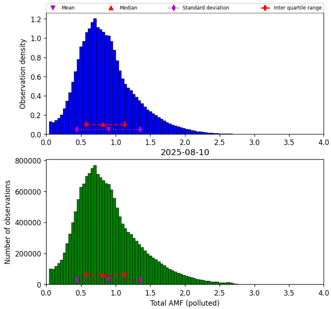
Figure 80: Histogram of “Total AMF (polluted)” for 2025-08-10 to 2025-08-11
