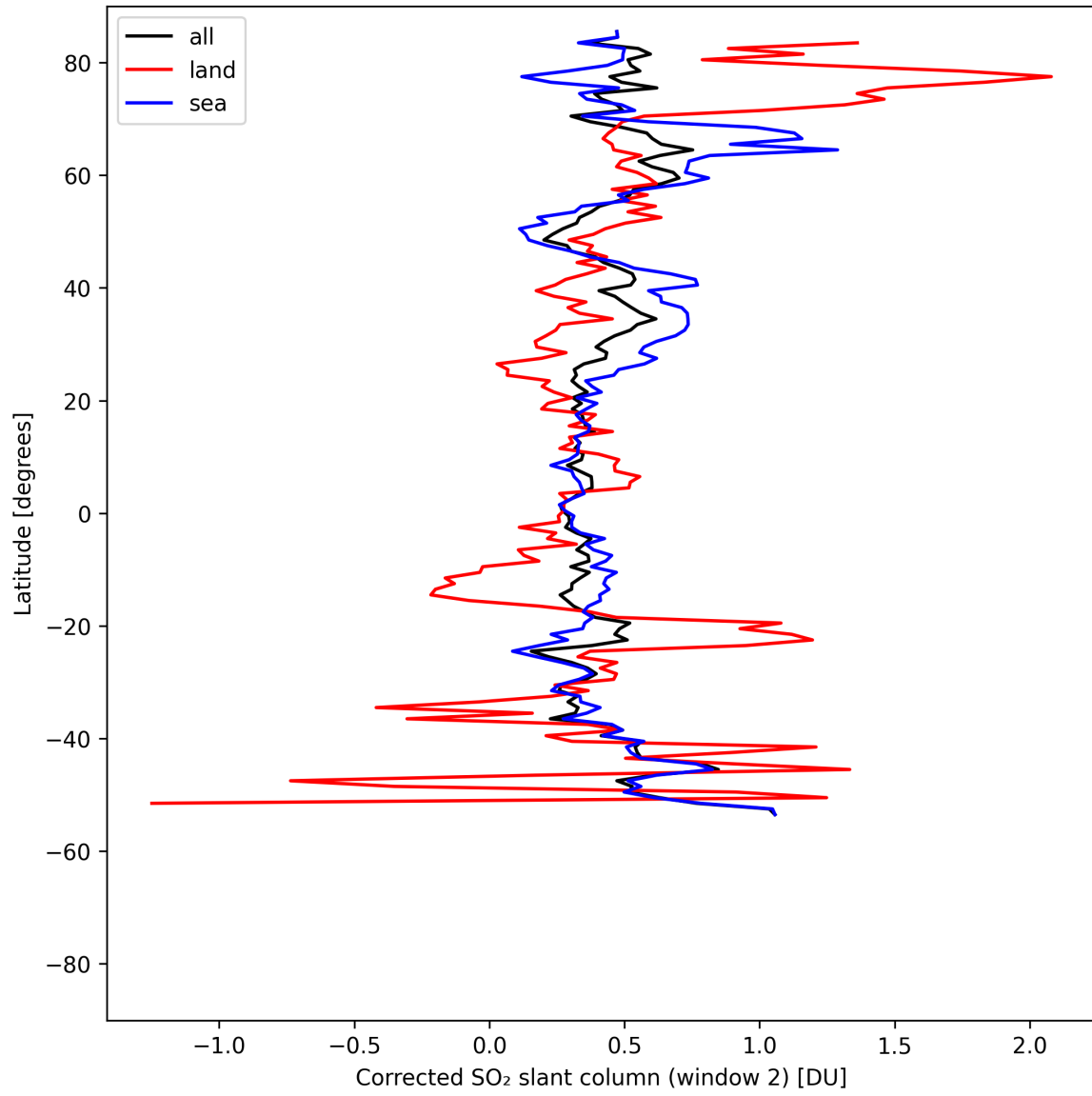
Figure 42: Zonal average of “Corrected SO 2 slant column (window 2)” for 2025-08-10 to 2025-08-11.
