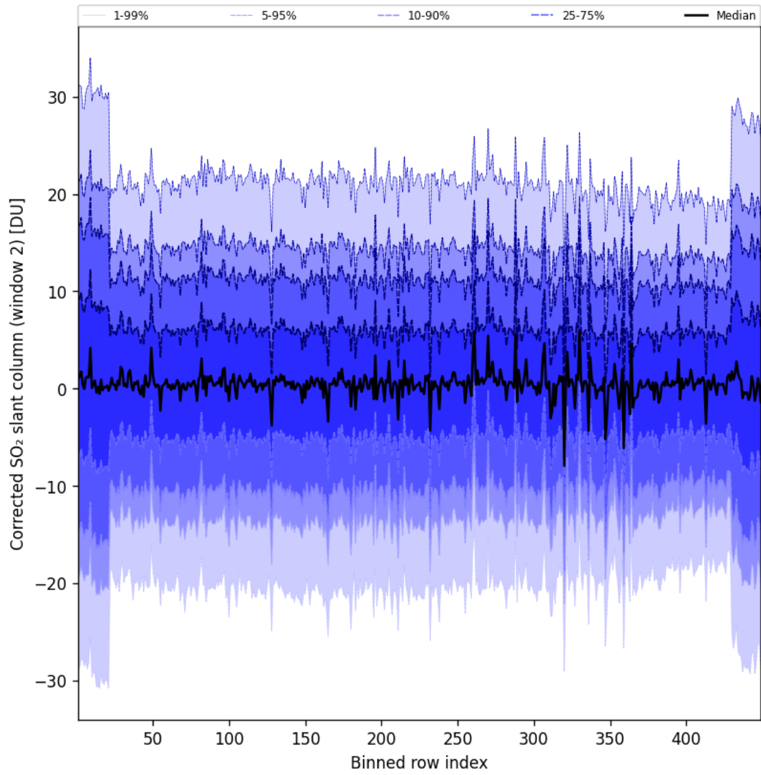
Figure 96: Along track statistics of “Corrected SO 2 slant column (window 2)” for 2025-08-10 to 2025-08-11
