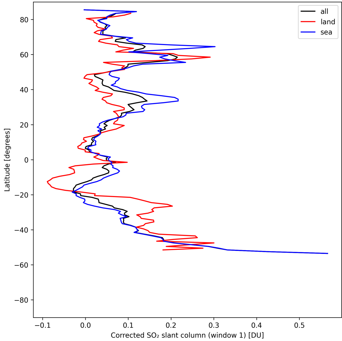
Figure 38: Zonal average of “Corrected SO 2 slant column (window 1)” for 2025-08-10 to 2025-08-11.
