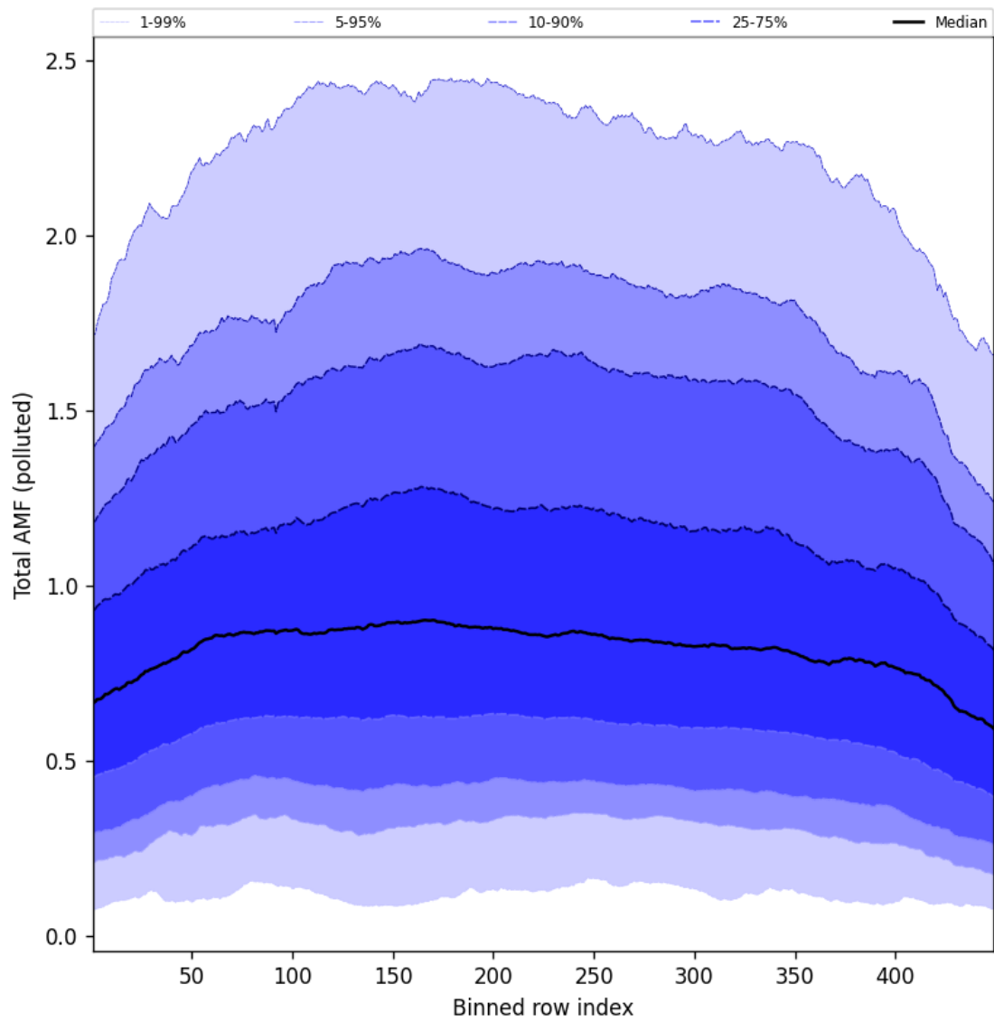
Figure 107: Along track statistics of “Total AMF (polluted)” for 2025-08-10 to 2025-08-11
