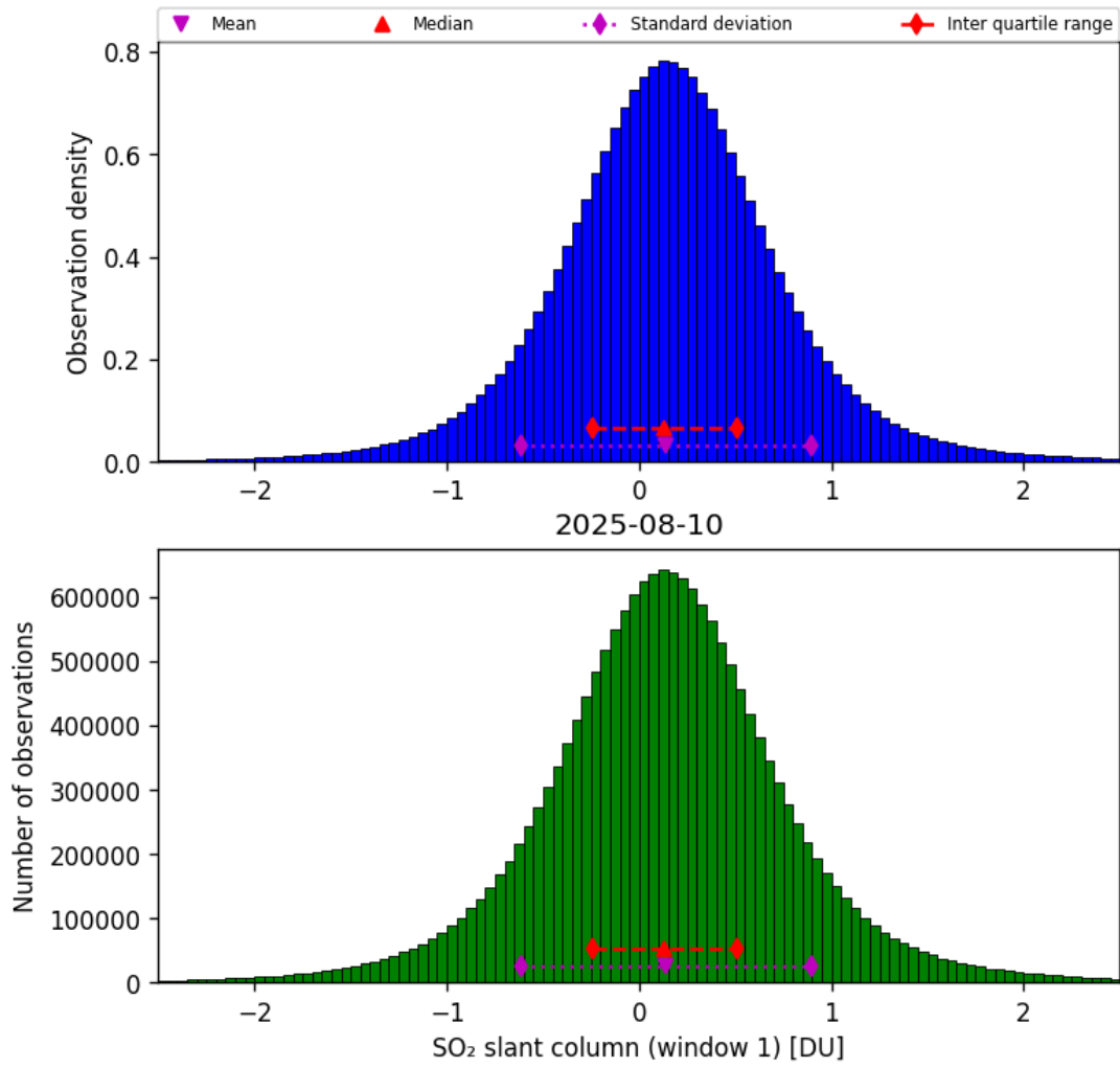
Figure 63: Histogram of “SO 2 slant column (window 1)” for 2025-08-10 to 2025-08-11
