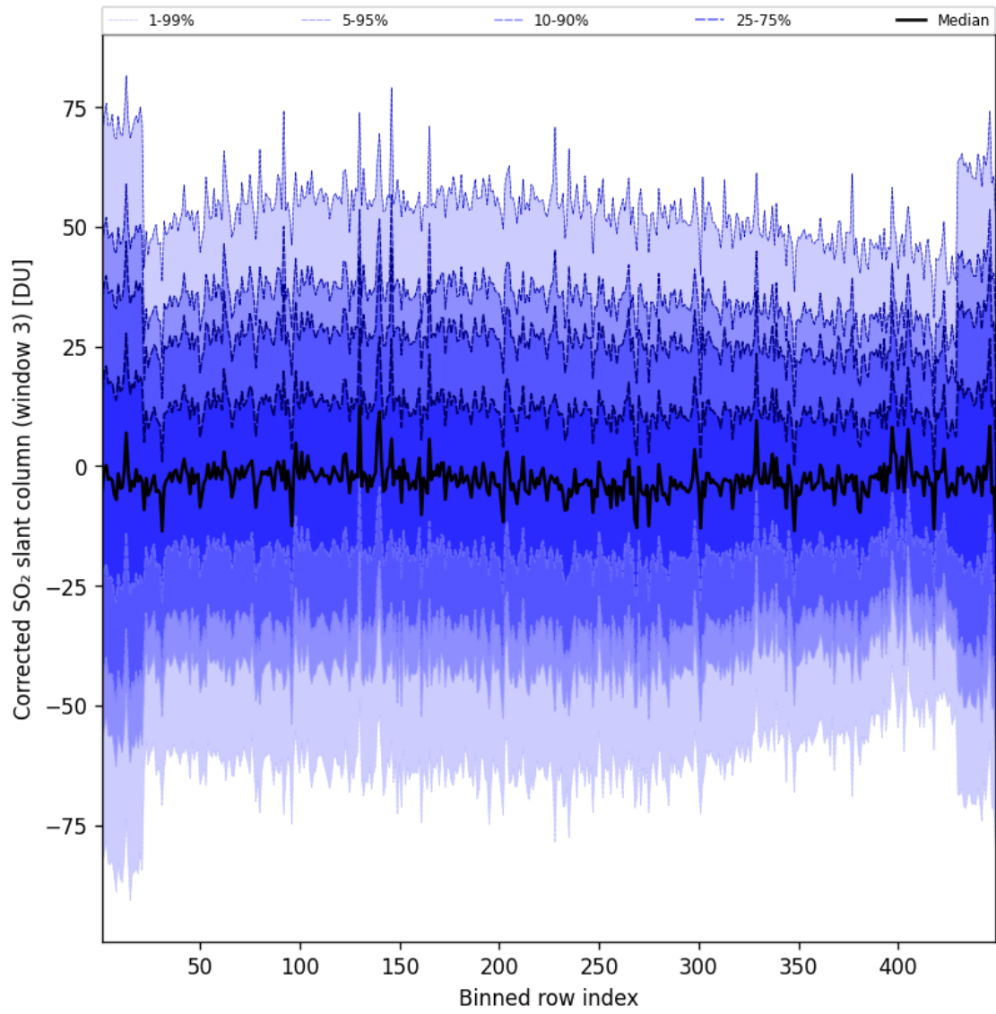
Figure 100: Along track statistics of “Corrected SO 2 slant column (window 3)” for 2025-08-10 to 2025-08-11
