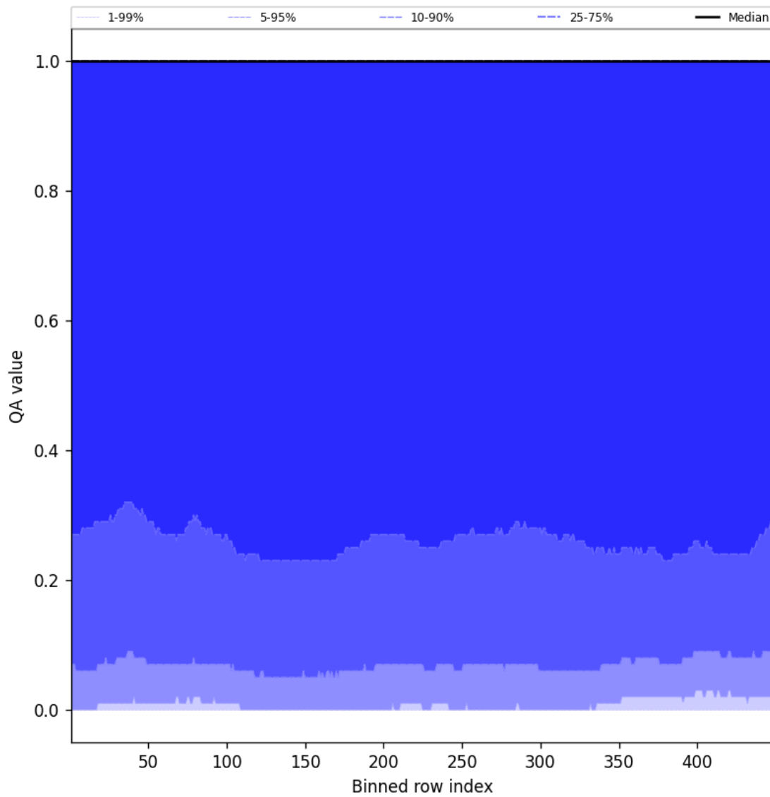
Figure 84: Along track statistics of “QA value” for 2025-08-10 to 2025-08-11
