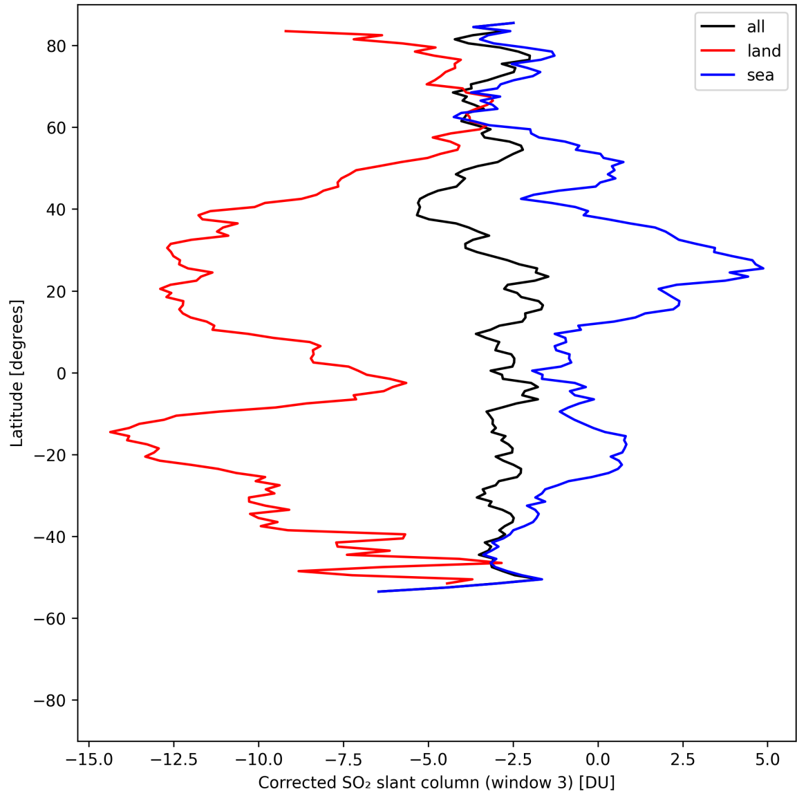
Figure 46: Zonal average of “Corrected SO 2 slant column (window 3)” for 2025-08-10 to 2025-08-11.
