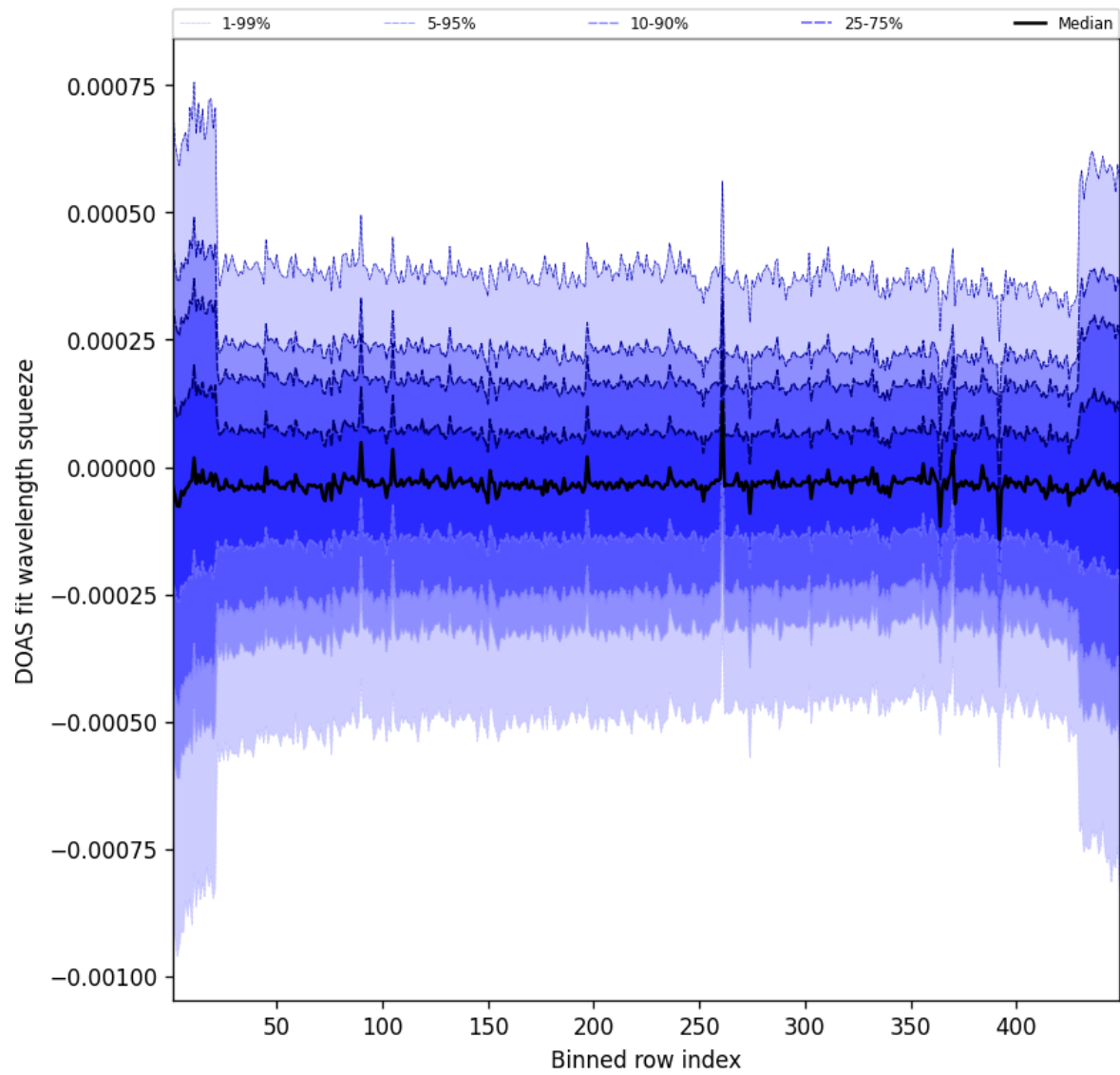
Figure 105: Along track statistics of “DOAS fit wavelength squeeze” for 2025-08-10 to 2025-08-11
