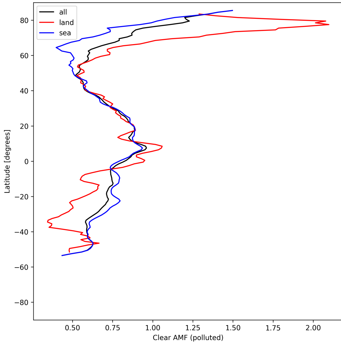
Figure 55: Zonal average of “Clear AMF (polluted)” for 2025-08-10 to 2025-08-11.
