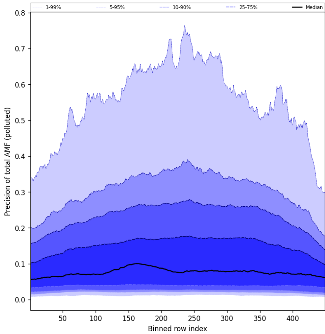
Figure 108: Along track statistics of “Precision of total AMF (polluted)” for 2025-08-10 to 2025-08-11
