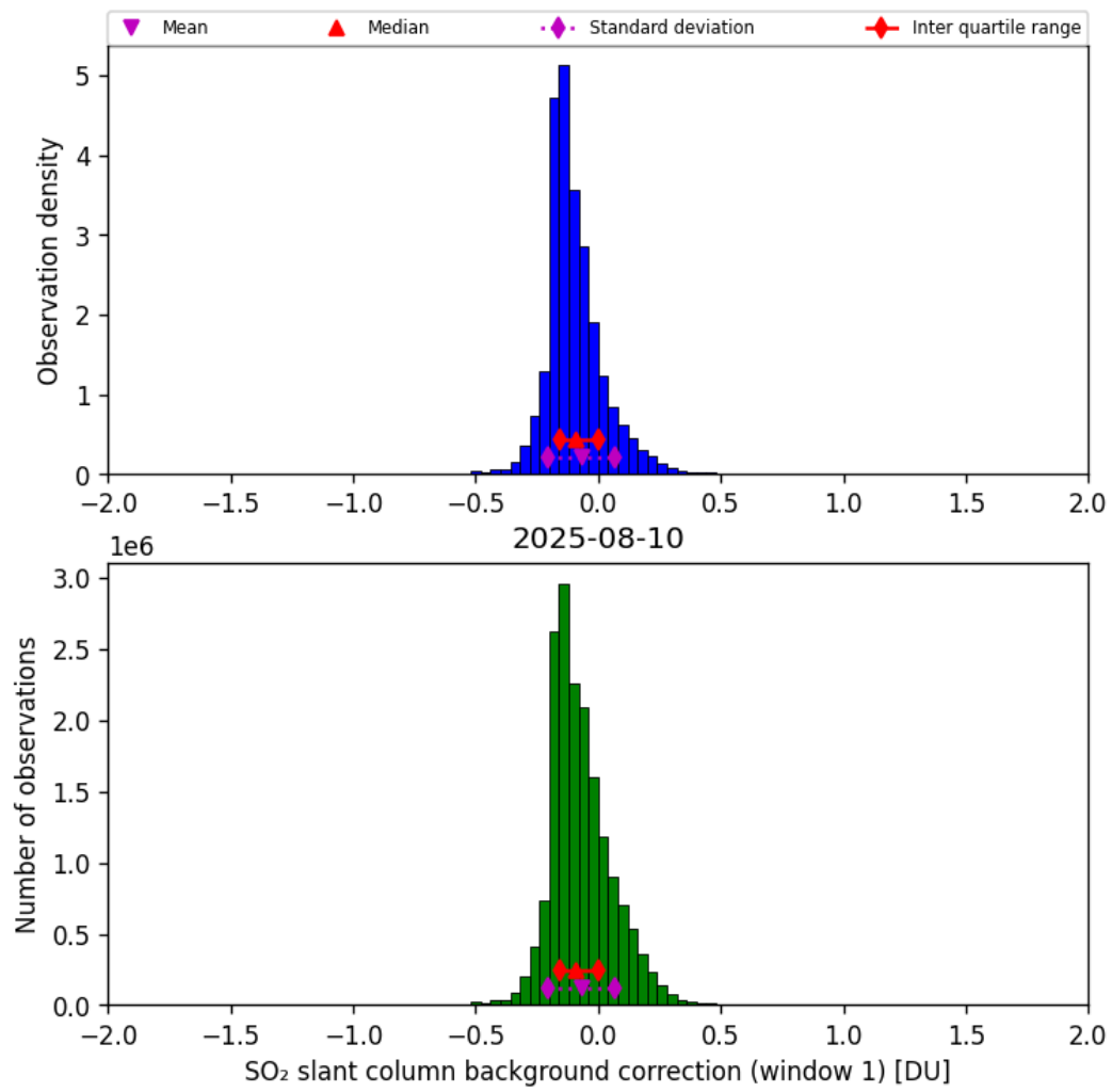
Figure 66: Histogram of “SO 2 slant column background correction (window 1)” for 2025-08-10 to 2025-08-11
