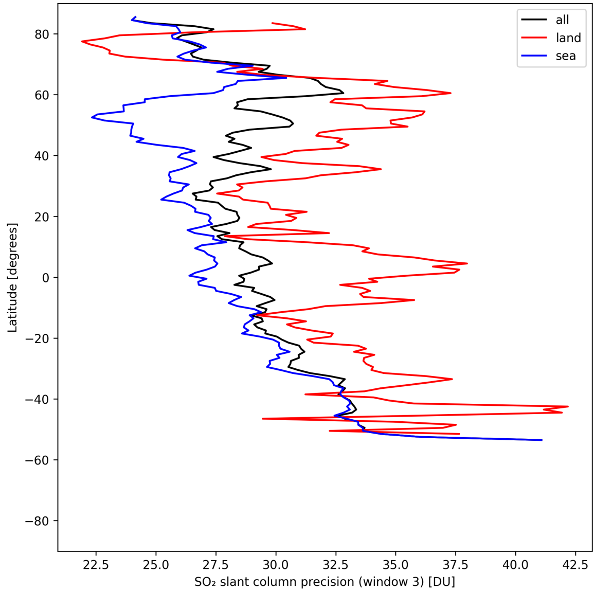
Figure 45: Zonal average of “SO 2 slant column precision (window 3)” for 2025-08-10 to 2025-08-11.
