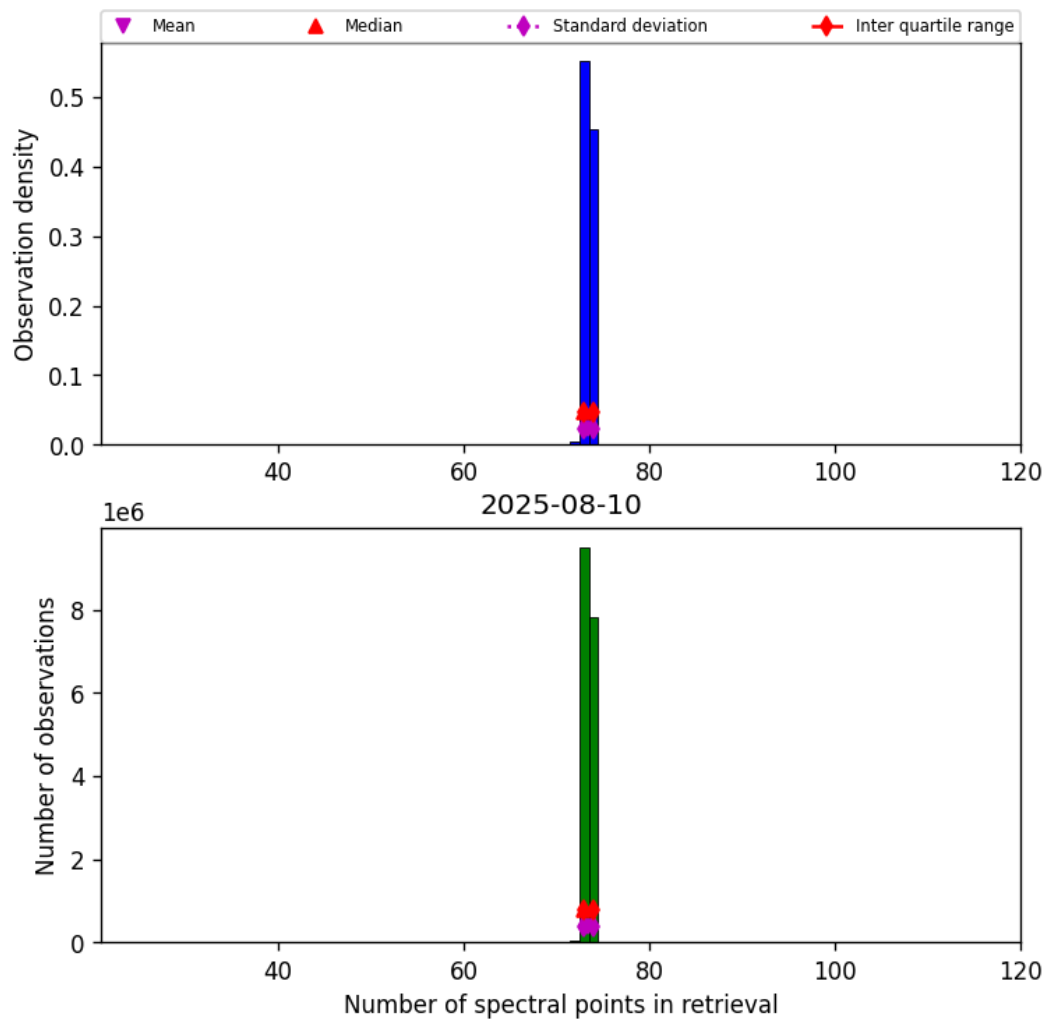
Figure 83: Histogram of “Number of spectral points in retrieval” for 2025-08-10 to 2025-08-11
