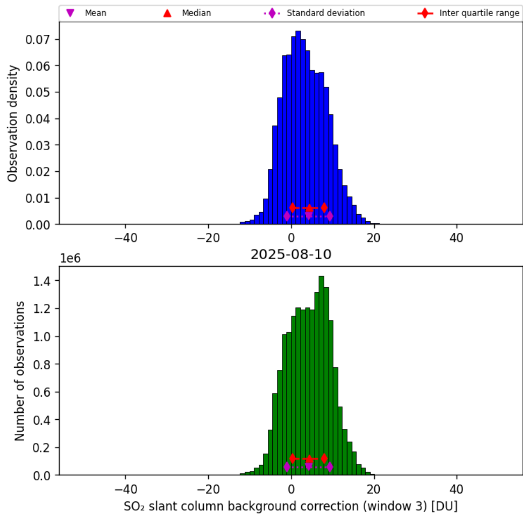
Figure 74: Histogram of “SO 2 slant column background correction (window 3)” for 2025-08-10 to 2025-08-11
