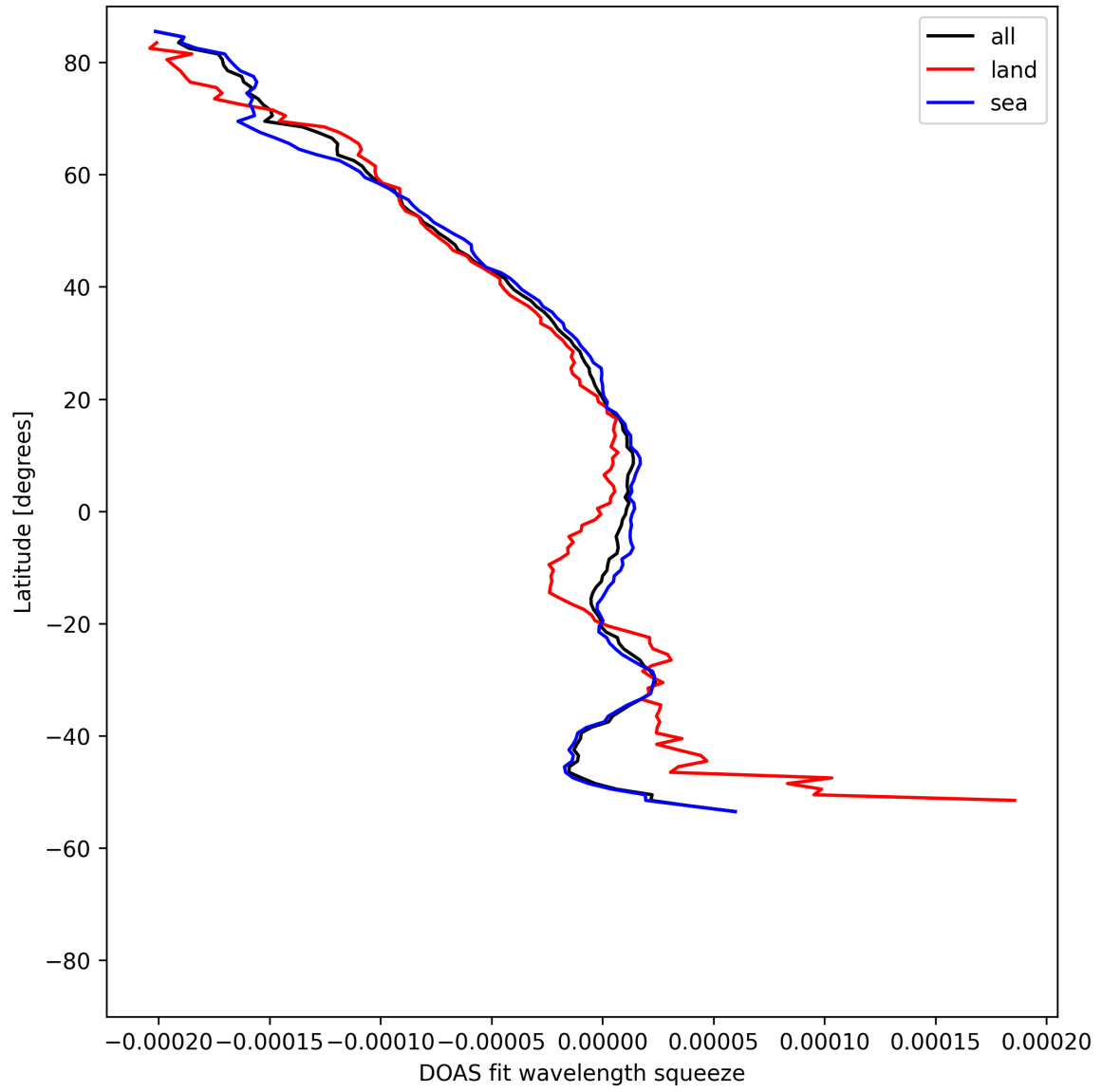
Figure 51: Zonal average of "DOAS fit wavelength squeeze" for 2025-08-10 to 2025-08-11.
