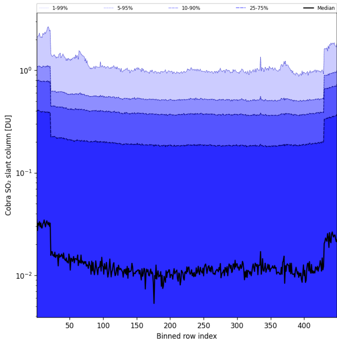
Figure 88: Along track statistics of “Cobra SO 2 slant column” for 2025-08-10 to 2025-08-11
