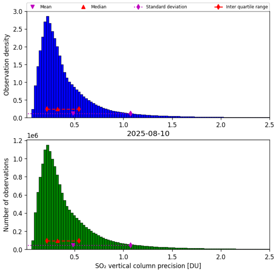
Figure 59: Histogram of “SO 2 vertical column precision” for 2025-08-10 to 2025-08-11
