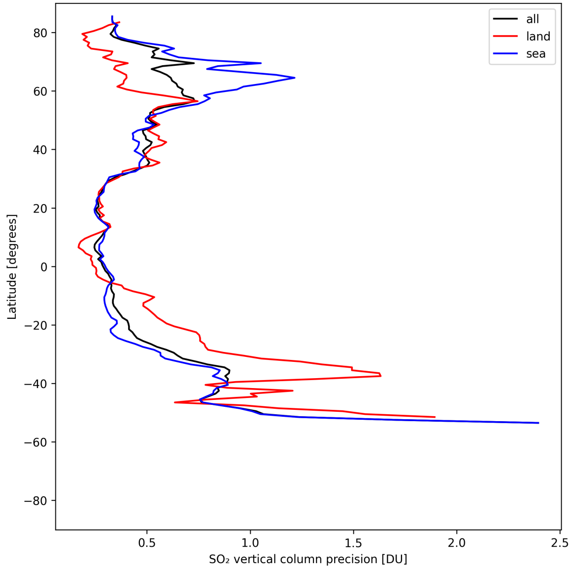
Figure 32: Zonal average of “SO 2 vertical column precision” for 2025-08-10 to 2025-08-11.
