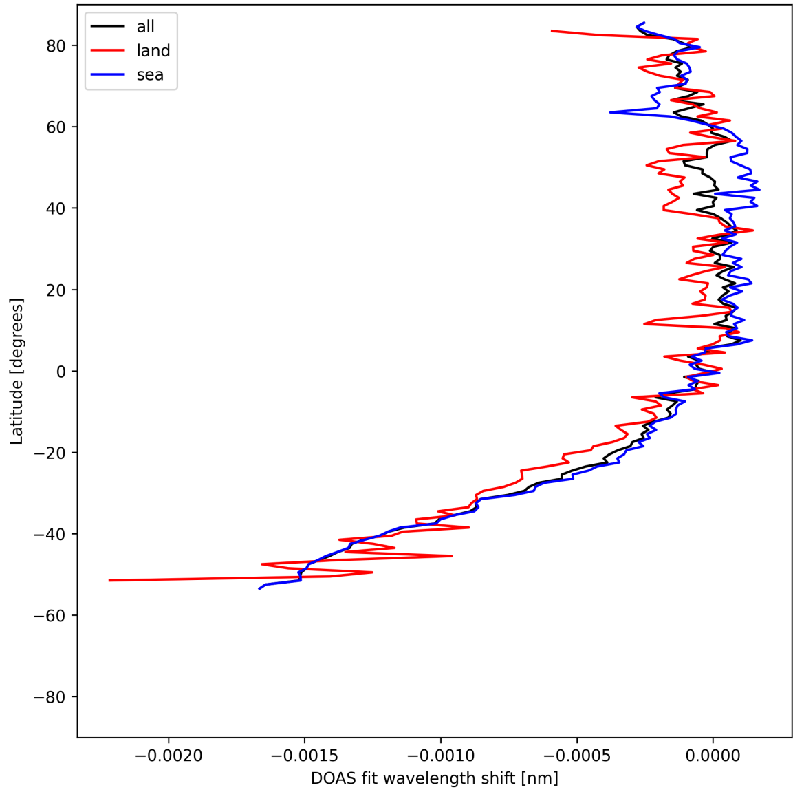
Figure 50: Zonal average of “DOAS fit wavelength shift” for 2025-08-10 to 2025-08-11.
