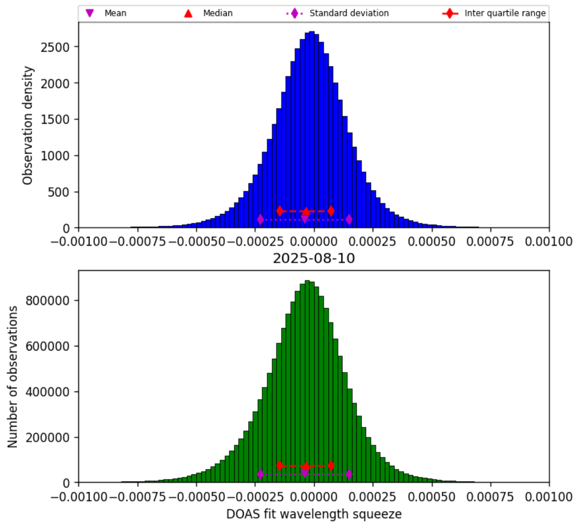
Figure 78: Histogram of “DOAS fit wavelength squeeze” for 2025-08-10 to 2025-08-11
