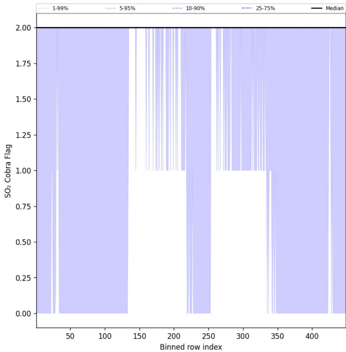
Figure 102: Along track statistics of “SO 2 Cobra Flag” for 2025-08-10 to 2025-08-11
