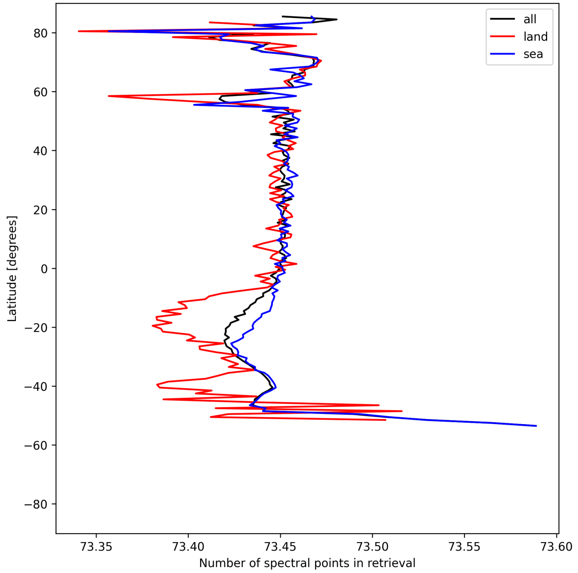
Figure 56: Zonal average of “Number of spectral points in retrieval” for 2025-08-10 to 2025-08-11.
