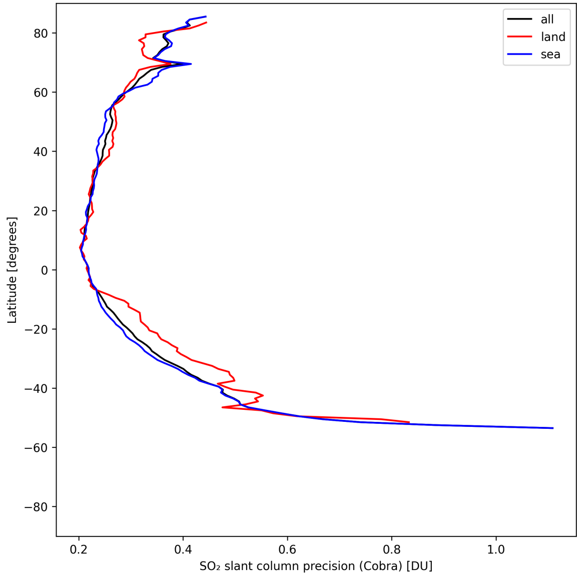
Figure 35: Zonal average of “SO 2 slant column precision (Cobra)” for 2025-08-10 to 2025-08-11.
