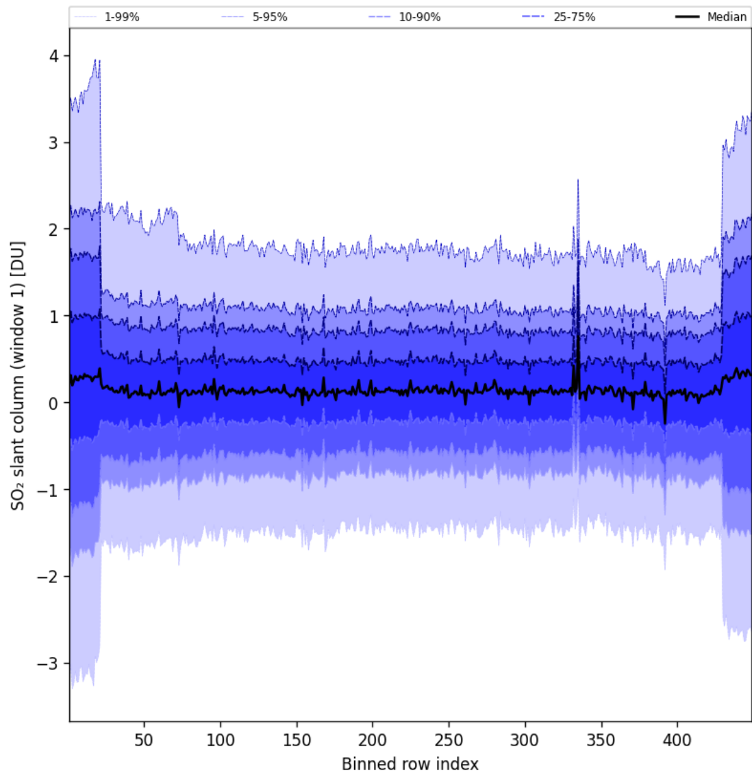
Figure 90: Along track statistics of “SO 2 slant column (window 1)” for 2025-08-10 to 2025-08-11
