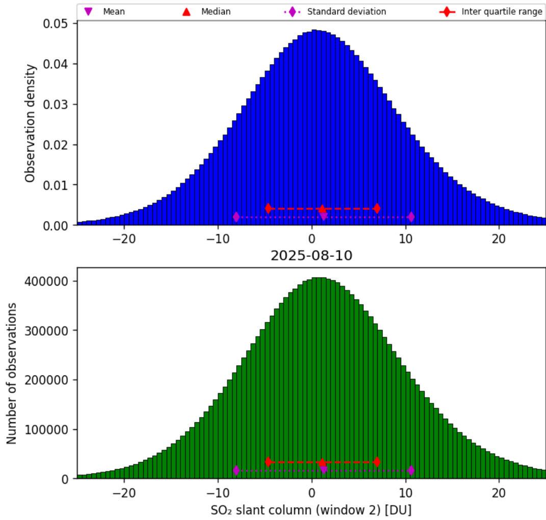
Figure 67: Histogram of “SO 2 slant column (window 2)” for 2025-08-10 to 2025-08-11
