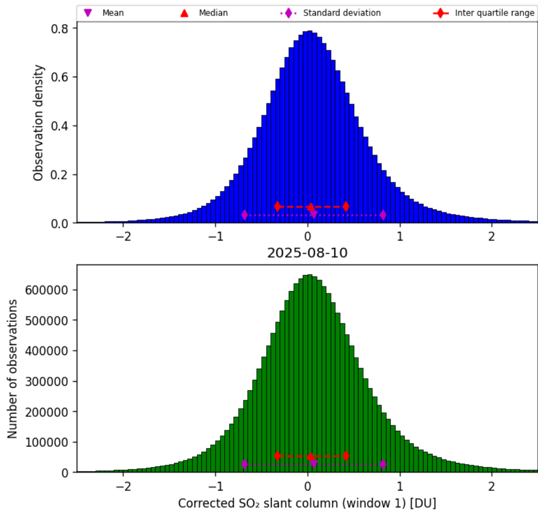
Figure 65: Histogram of “Corrected SO 2 slant column (window 1)” for 2025-08-10 to 2025-08-11
