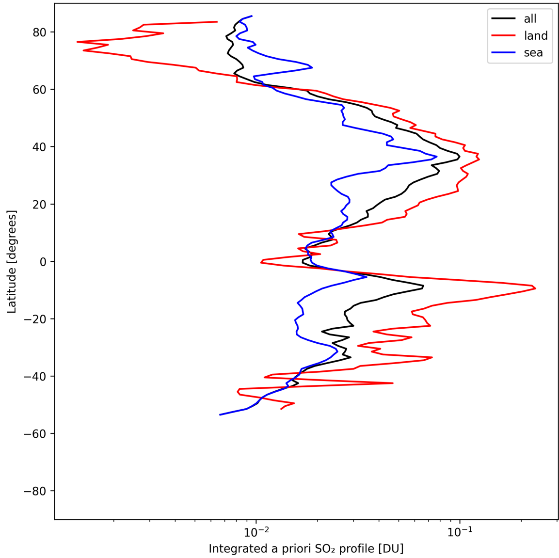
Figure 49: Zonal average of “Integrated a priori SO 2 profile” for 2025-08-10 to 2025-08-11.
