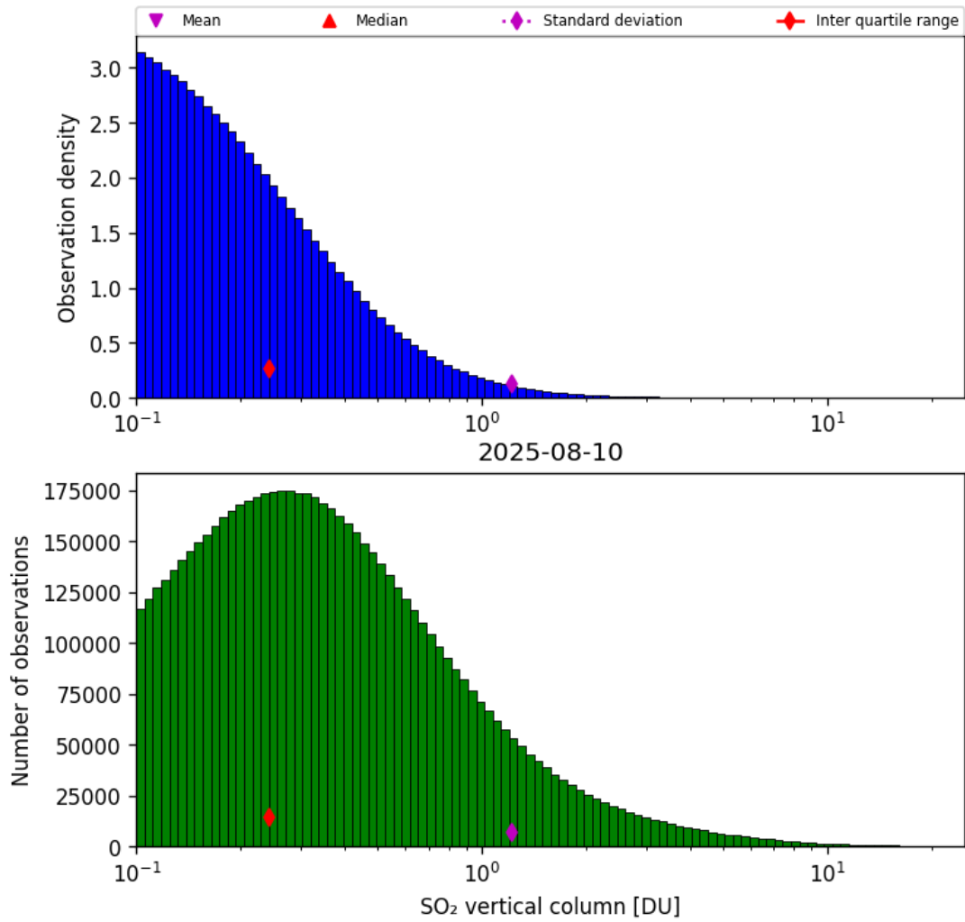
Figure 58: Histogram of “SO 2 vertical column” for 2025-08-10 to 2025-08-11
