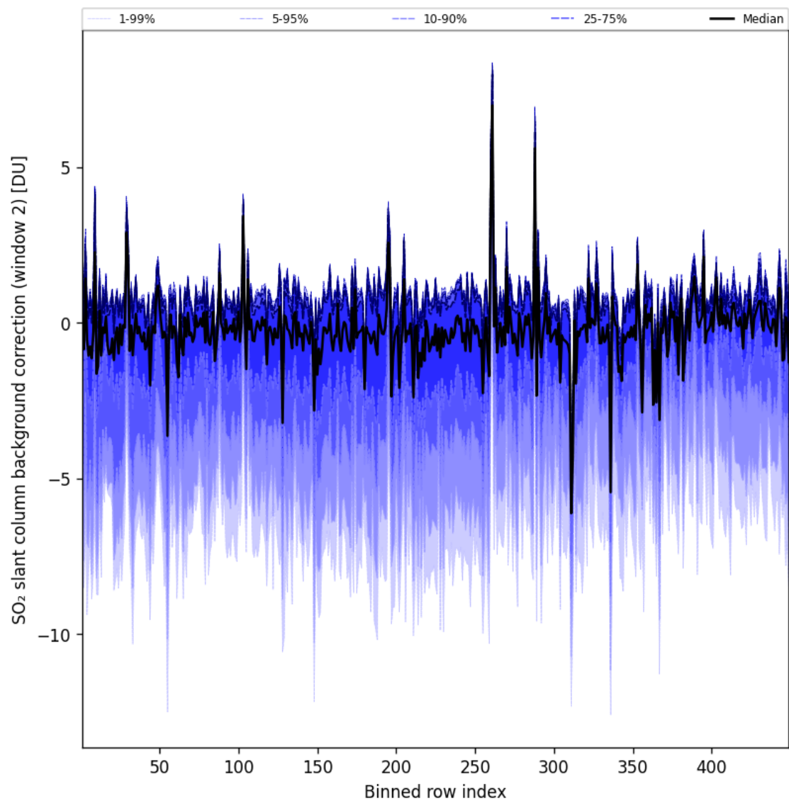
Figure 97: Along track statistics of “SO 2 slant column background correction (window 2)” for 2025-08-10 to 2025-08-11
