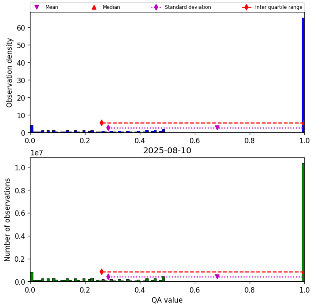
Figure 57: Histogram of “QA value” for 2025-08-10 to 2025-08-11
