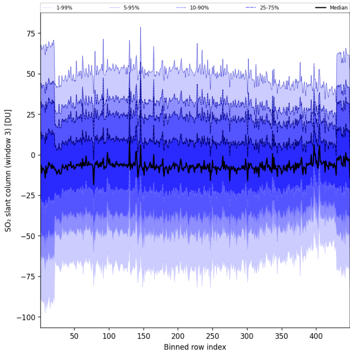
Figure 98: Along track statistics of “SO 2 slant column (window 3)” for 2025-08-10 to 2025-08-11
