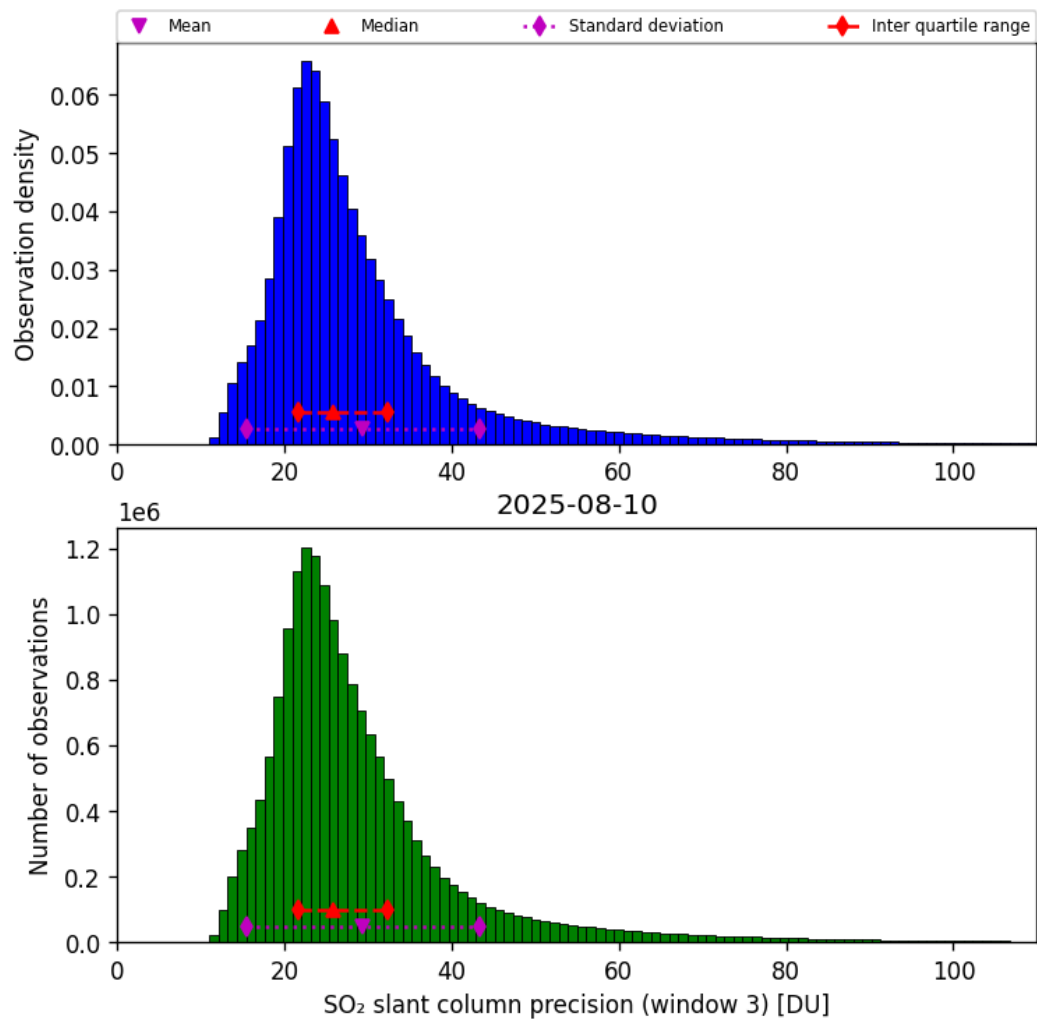
Figure 72: Histogram of “SO 2 slant column precision (window 3)” for 2025-08-10 to 2025-08-11
