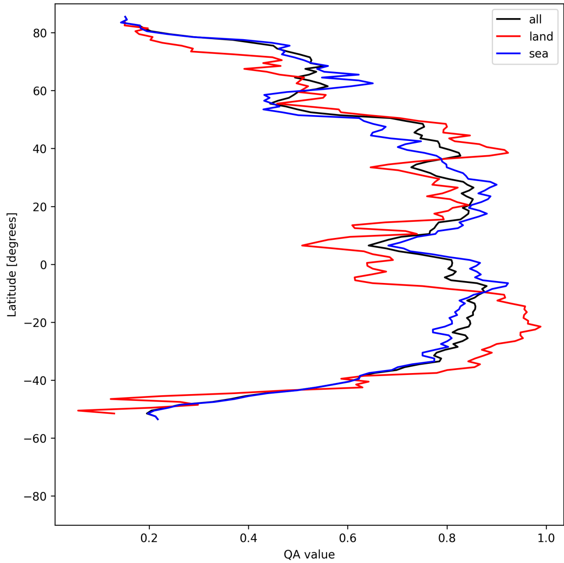
Figure 30: Zonal average of “QA value” for 2025-08-10 to 2025-08-11.
