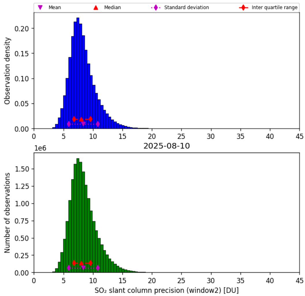
Figure 68: Histogram of “SO 2 slant column precision (window2)” for 2025-08-10 to 2025-08-11
