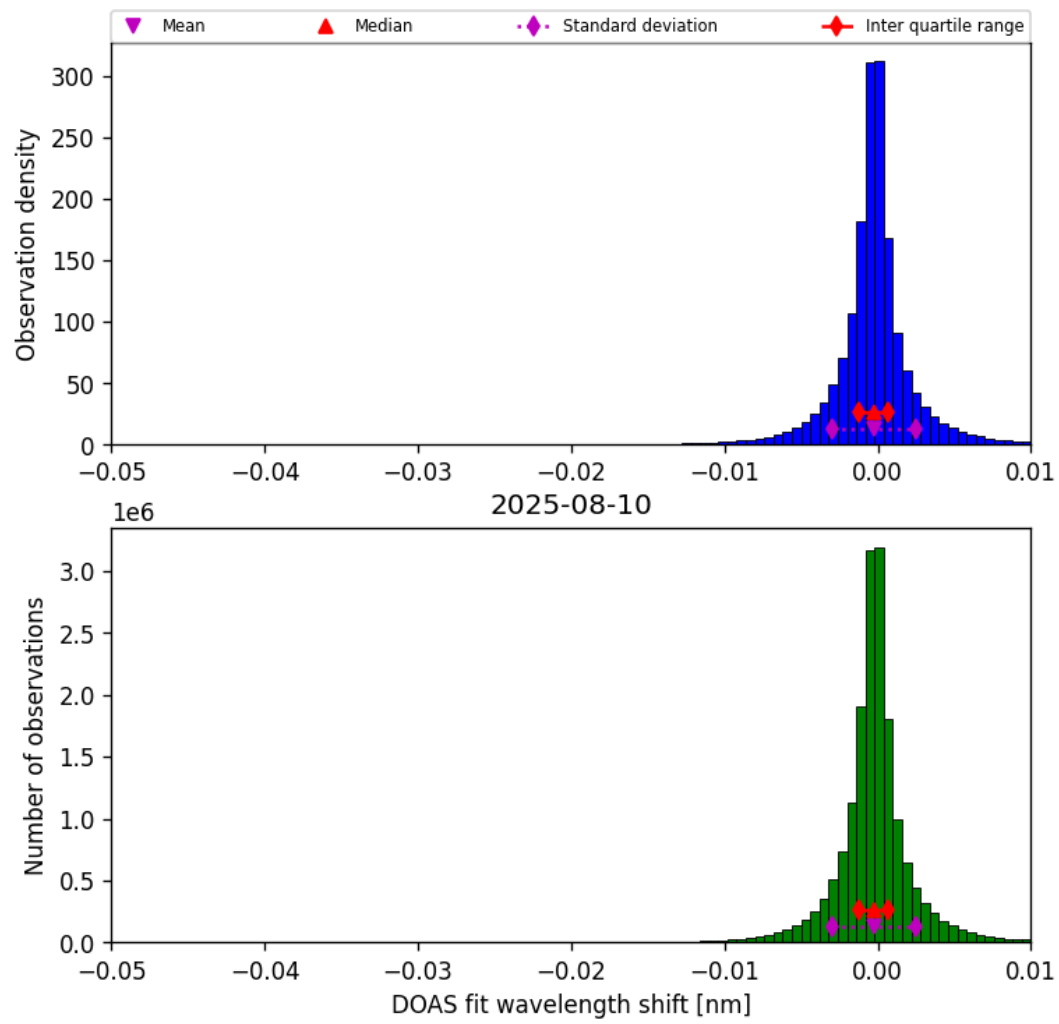
Figure 77: Histogram of “DOAS fit wavelength shift” for 2025-08-10 to 2025-08-11
