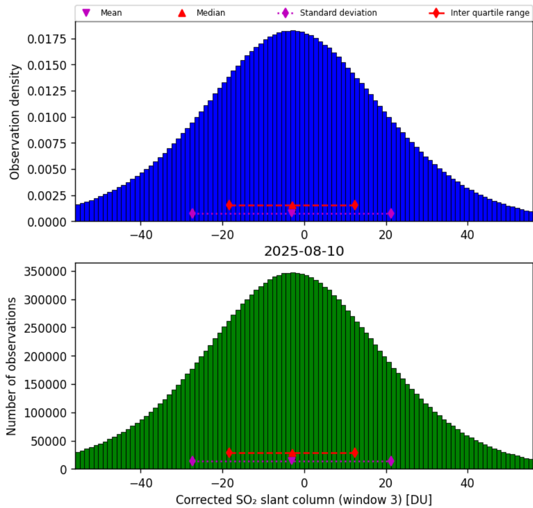
Figure 73: Histogram of “Corrected SO 2 slant column (window 3)” for 2025-08-10 to 2025-08-11
