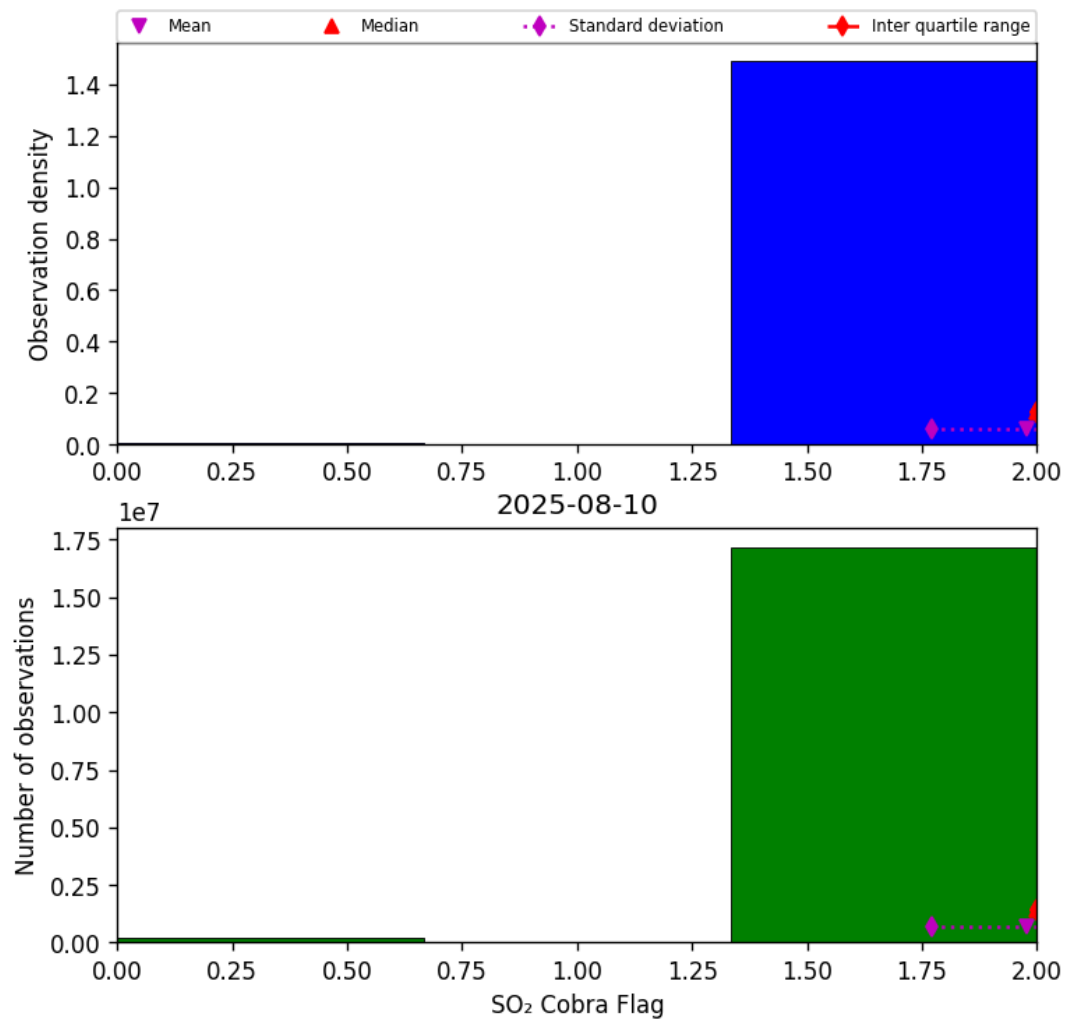
Figure 75: Histogram of “SO 2 Cobra Flag” for 2025-08-10 to 2025-08-11
