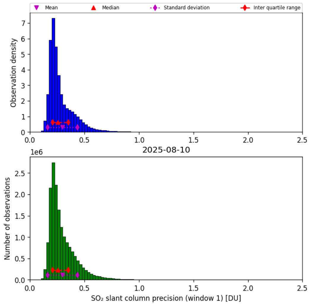
Figure 64: Histogram of “SO 2 slant column precision (window 1)” for 2025-08-10 to 2025-08-11
