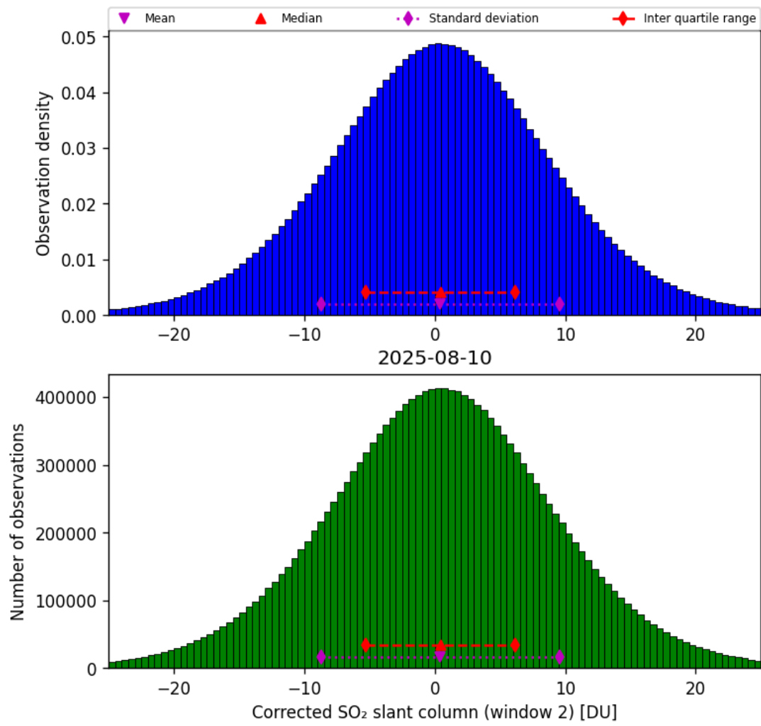
Figure 69: Histogram of “Corrected SO 2 slant column (window 2)” for 2025-08-10 to 2025-08-11
