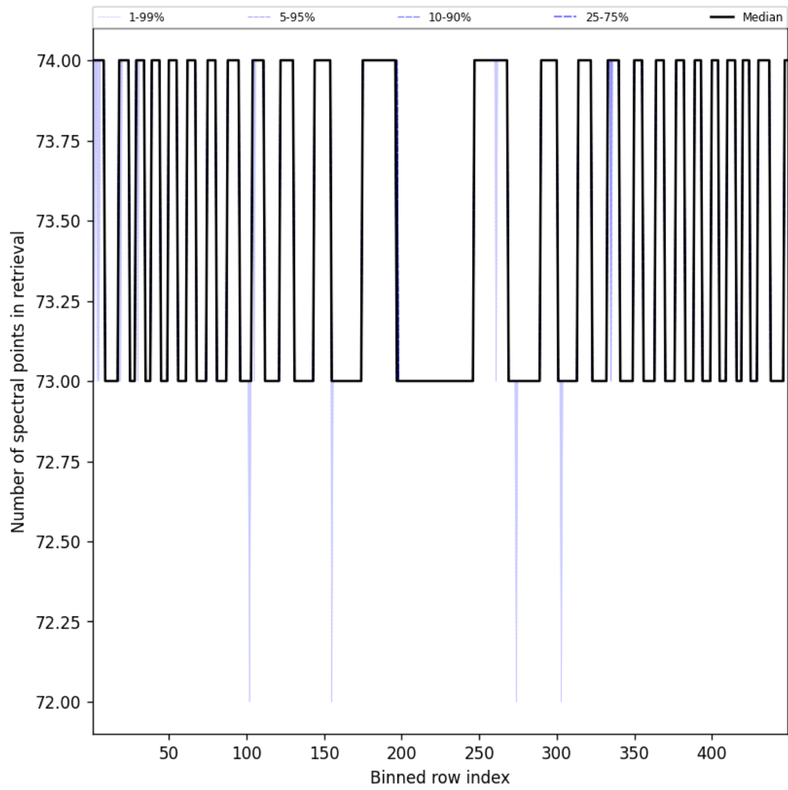
Figure 110: Along track statistics of “Number of spectral points in retrieval” for 2025-08-10 to 2025-08-11
