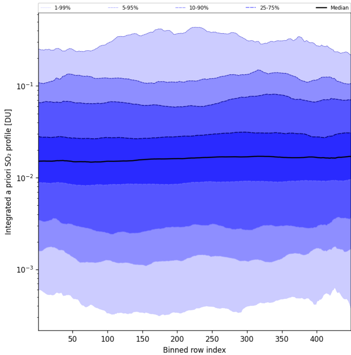
Figure 103: Along track statistics of “Integrated a priori SO 2 profile” for 2025-08-10 to 2025-08-11
