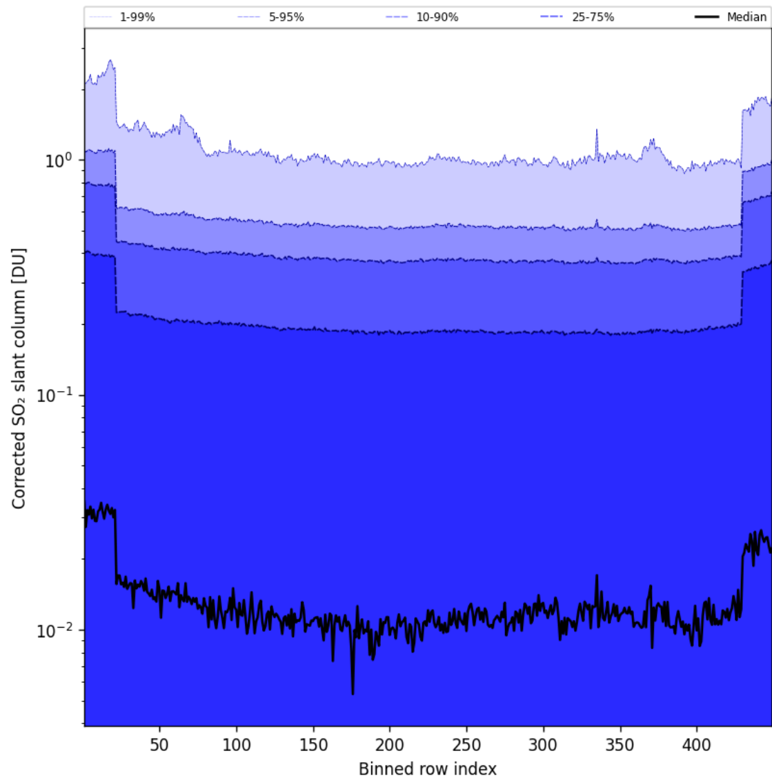
Figure 87: Along track statistics of “Corrected SO 2 slant column” for 2025-08-10 to 2025-08-11
