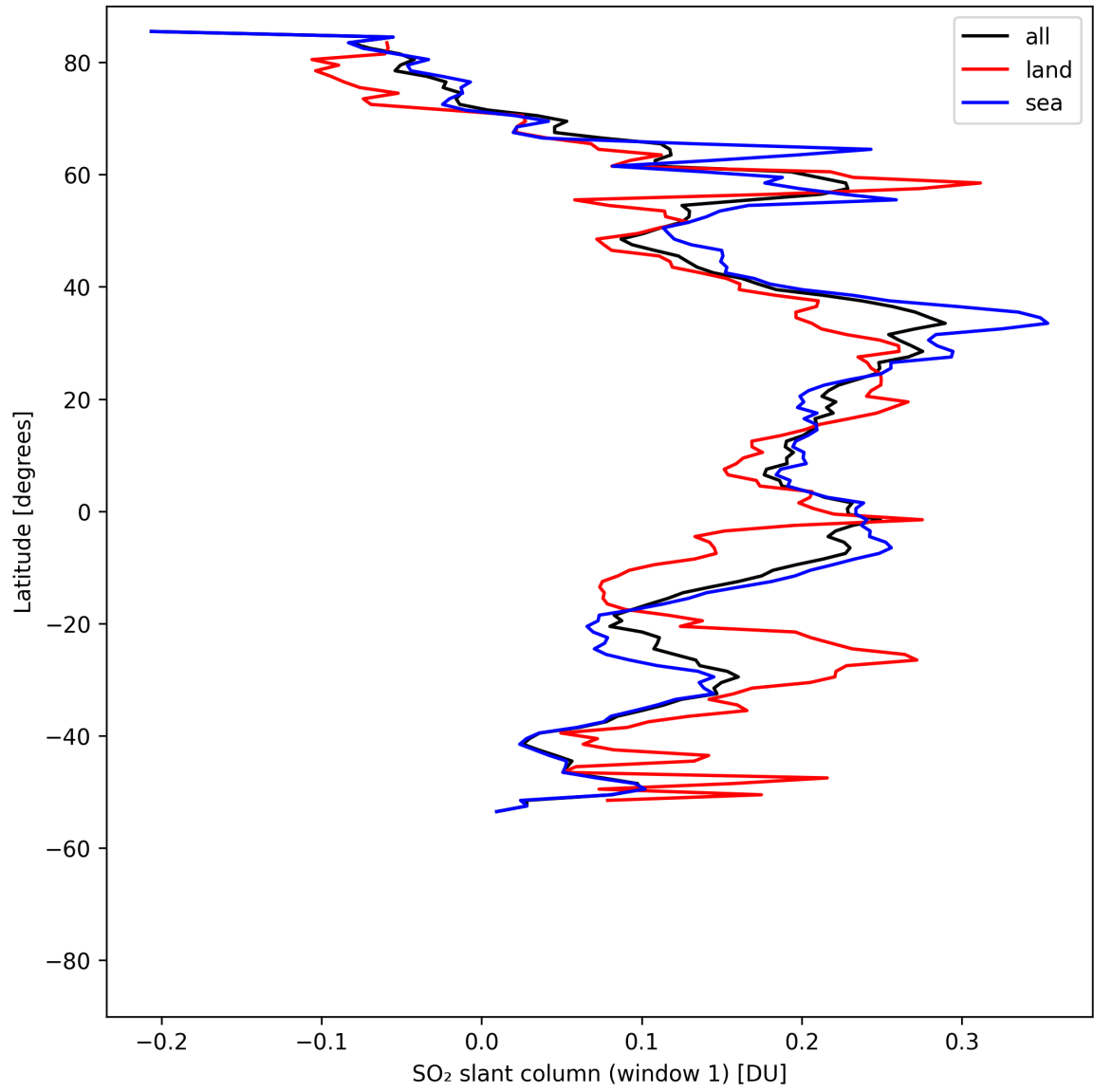
Figure 36: Zonal average of “SO 2 slant column (window 1)” for 2025-08-10 to 2025-08-11.
