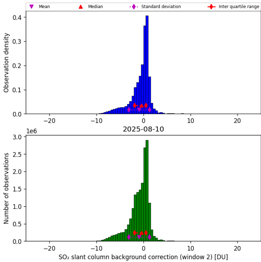
Figure 70: Histogram of “SO 2 slant column background correction (window 2)” for 2025-08-10 to 2025-08-11
