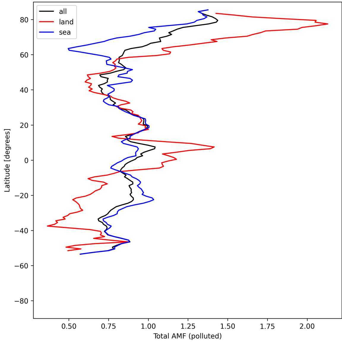
Figure 53: Zonal average of “Total AMF (polluted)” for 2025-08-10 to 2025-08-11.
