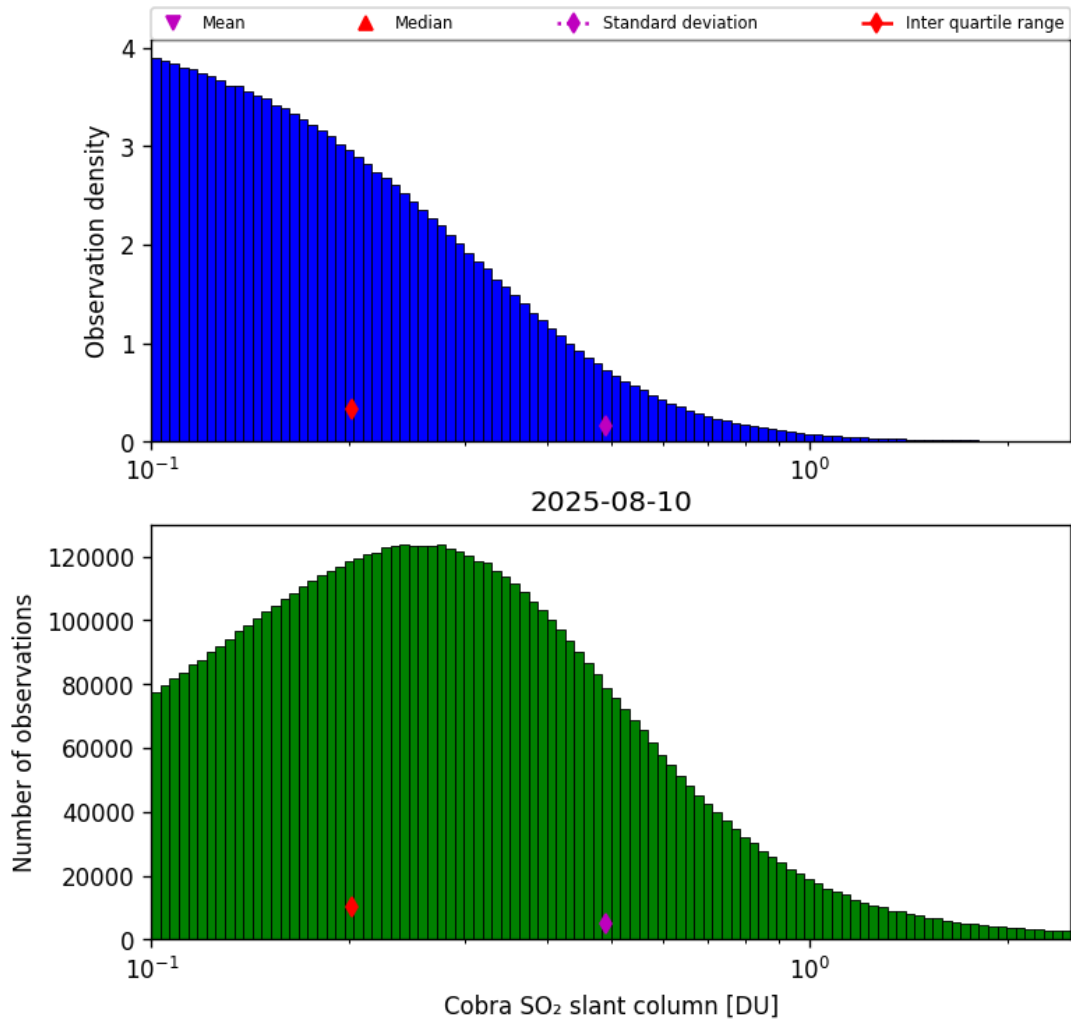
Figure 61: Histogram of “Cobra SO 2 slant column” for 2025-08-10 to 2025-08-11
