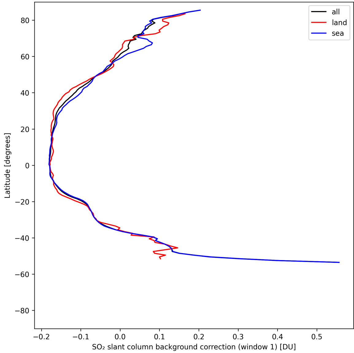
Figure 39: Zonal average of "SO 2 slant column background correction (window 1)" for 2025-08-10 to 2025-08-11.
