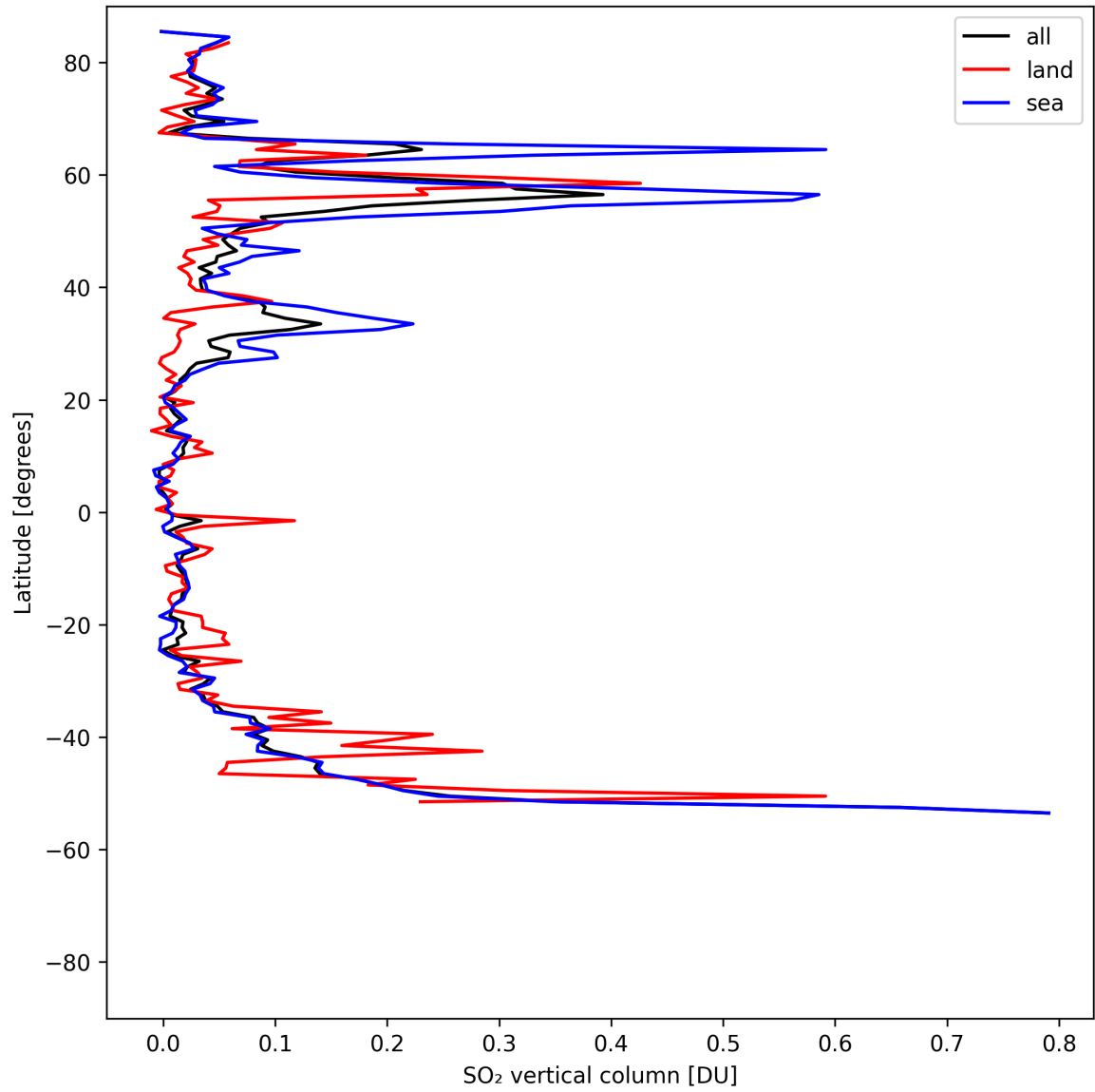
Figure 31: Zonal average of “SO 2 vertical column” for 2025-08-10 to 2025-08-11.
