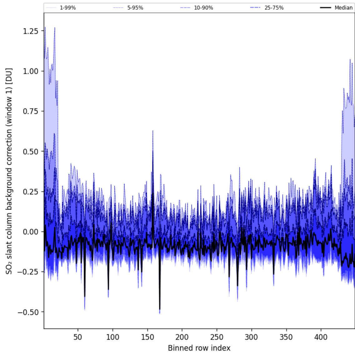
Figure 93: Along track statistics of “SO 2 slant column background correction (window 1)” for 2025-08-10 to 2025-08-11
