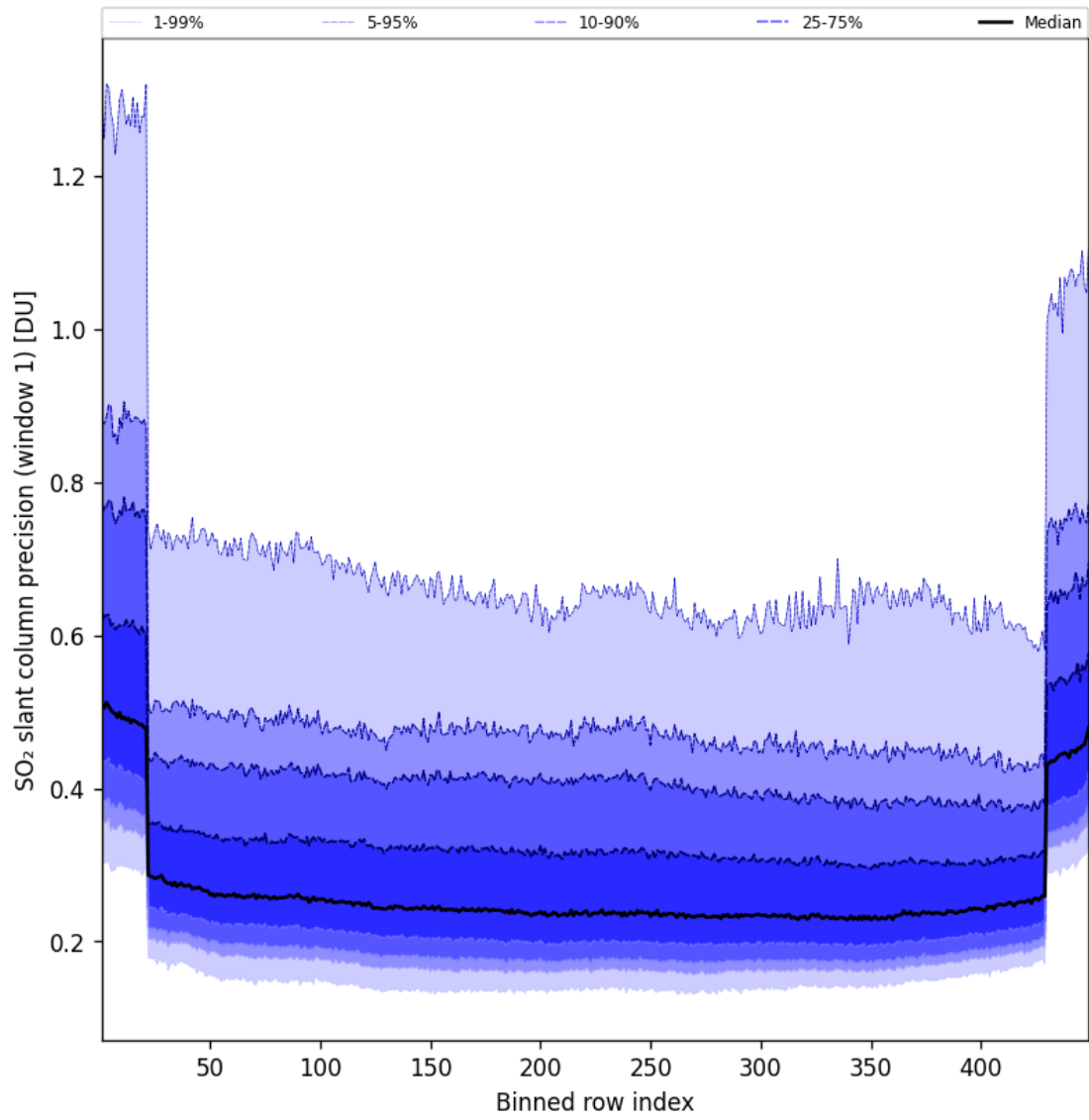
Figure 91: Along track statistics of “SO 2 slant column precision (window 1)” for 2025-08-10 to 2025-08-11
