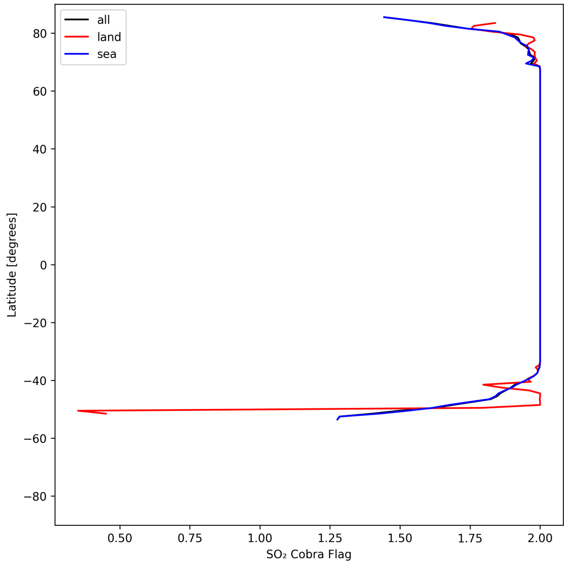
Figure 48: Zonal average of "SO 2 Cobra Flag" for 2025-08-10 to 2025-08-11.
