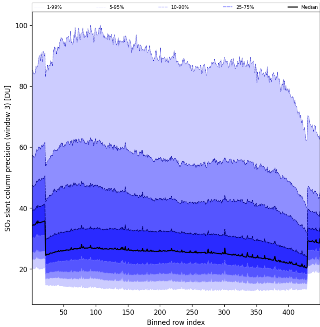
Figure 99: Along track statistics of “SO 2 slant column precision (window 3)” for 2025-08-10 to 2025-08-11
