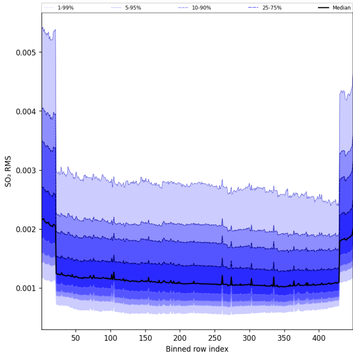
Figure 106: Along track statistics of “SO 2 RMS” for 2025-08-10 to 2025-08-11
