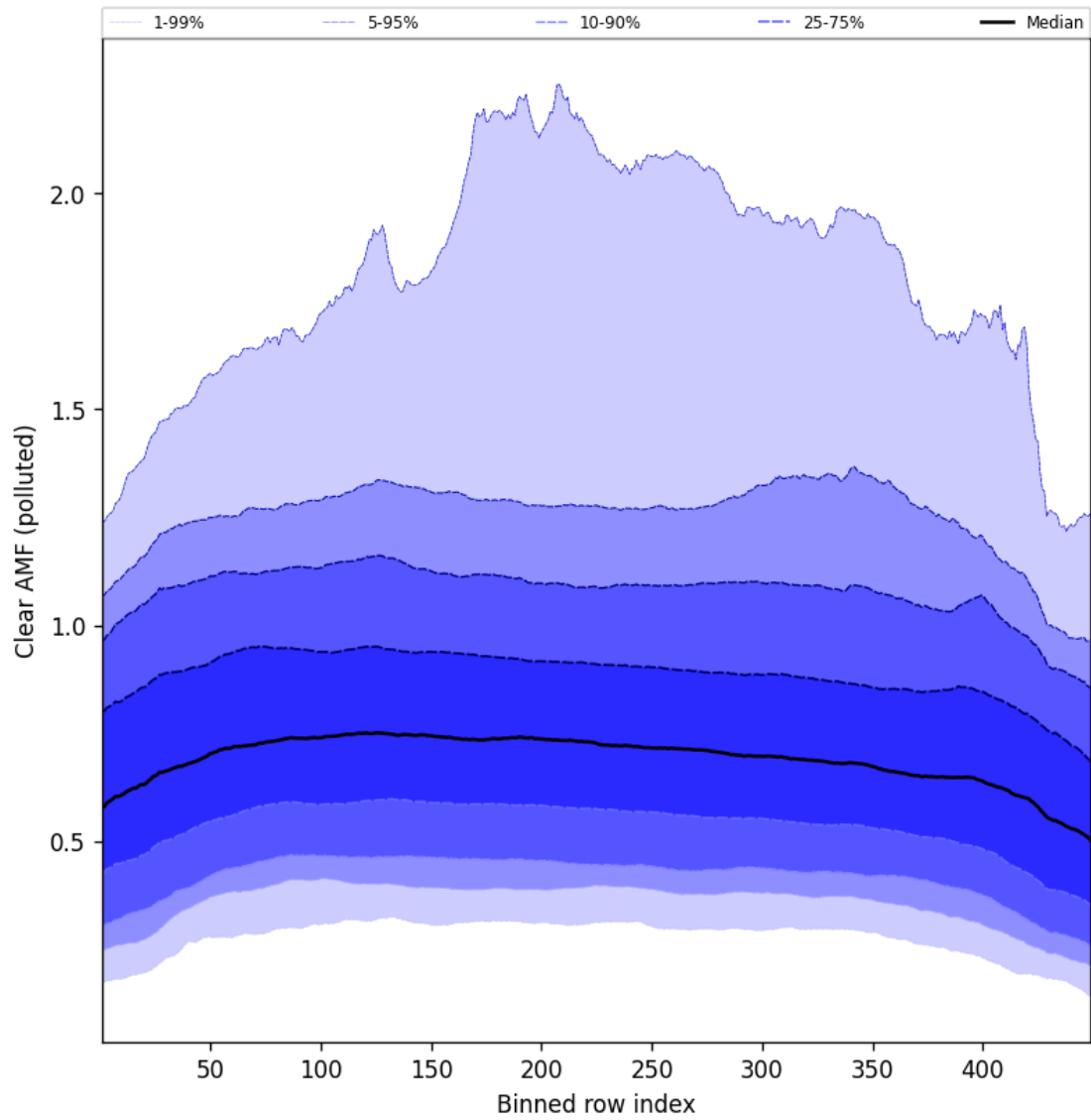
Figure 109: Along track statistics of “Clear AMF (polluted)” for 2025-08-10 to 2025-08-11
