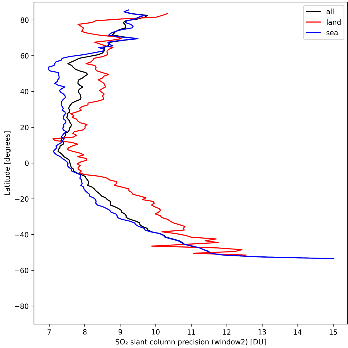
Figure 41: Zonal average of “SO 2 slant column precision (window2)” for 2025-08-10 to 2025-08-11.
