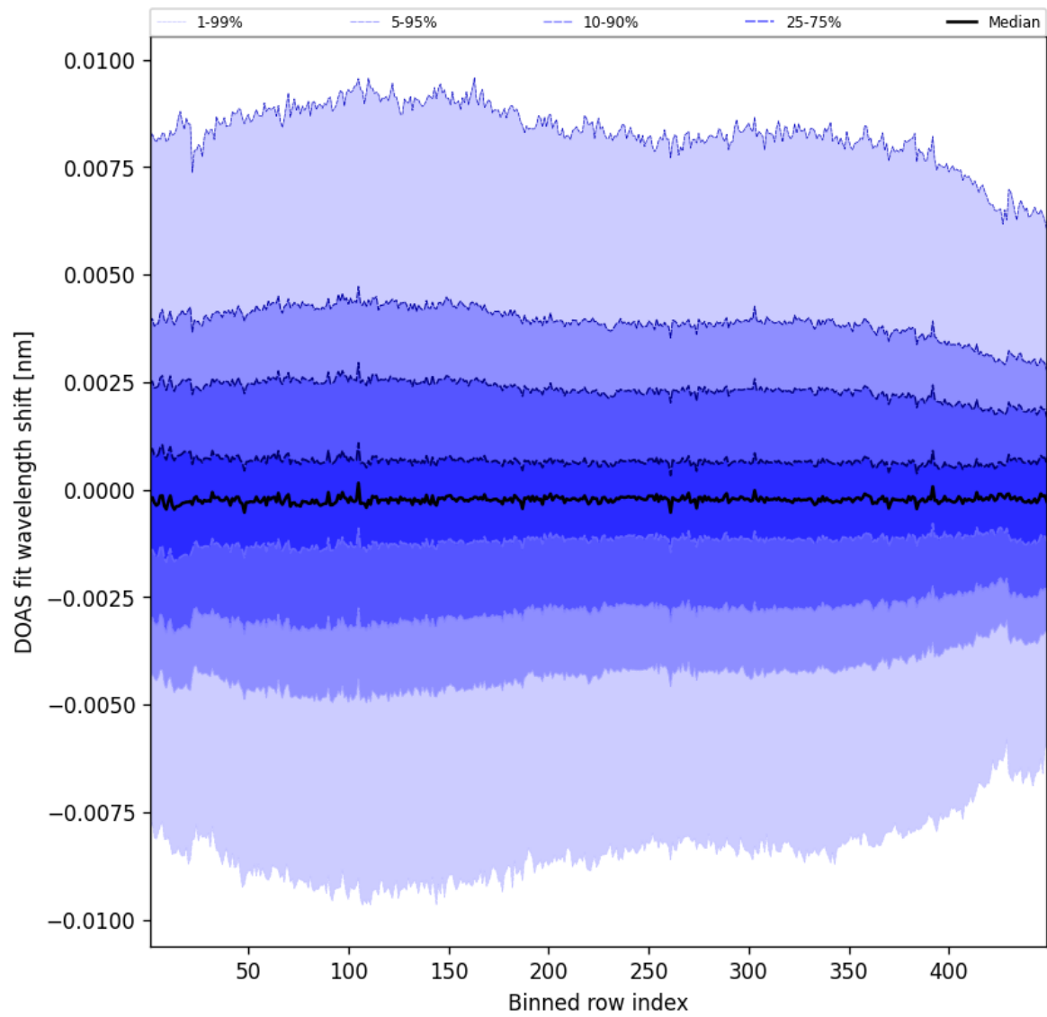
Figure 104: Along track statistics of “DOAS fit wavelength shift” for 2025-08-10 to 2025-08-11
