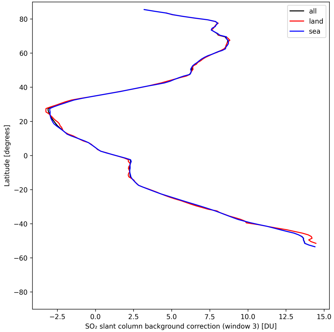
Figure 47: Zonal average of “SO 2 slant column background correction (window 3)” for 2025-08-10 to 2025-08-11.
