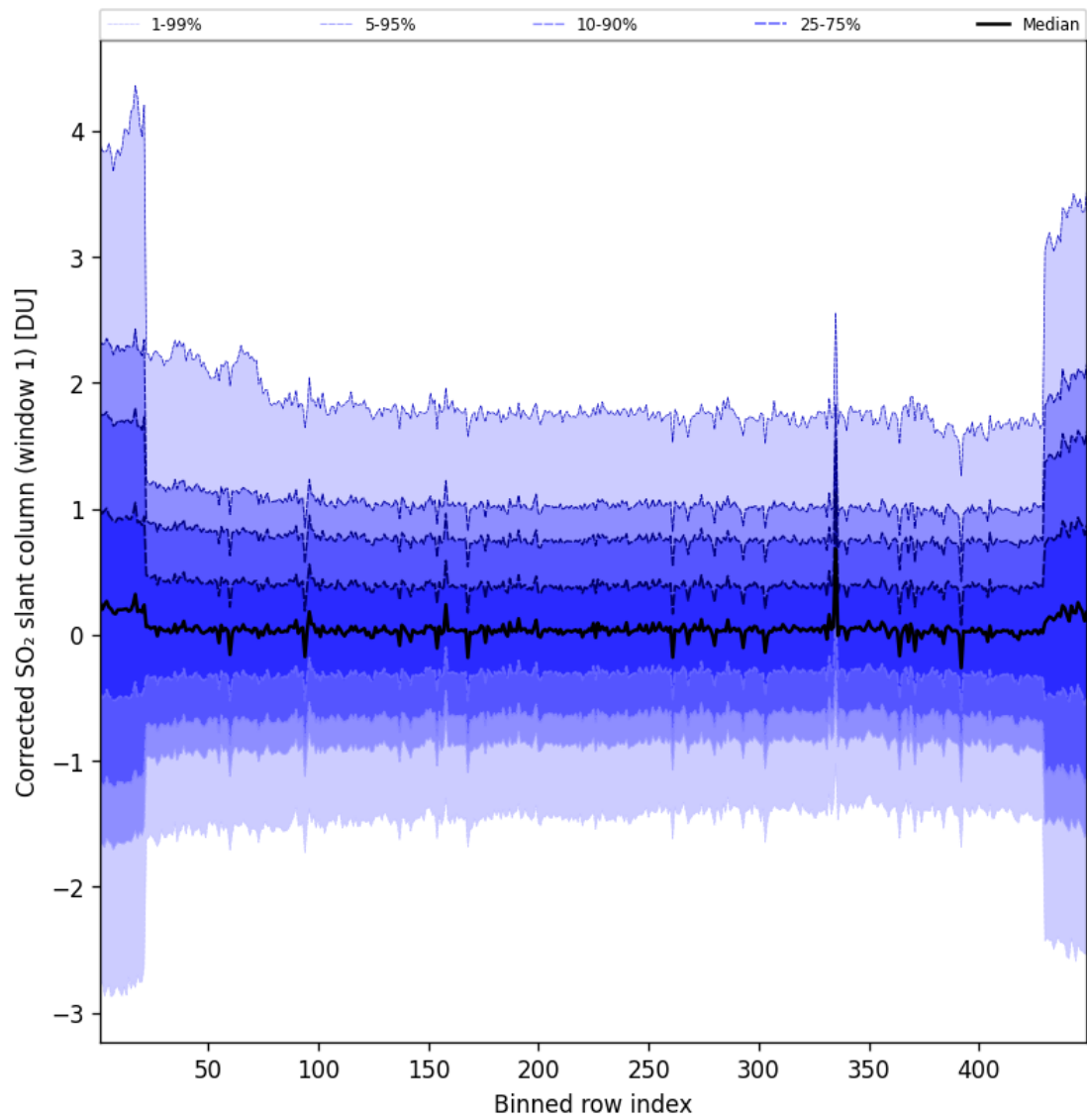
Figure 92: Along track statistics of “Corrected SO 2 slant column (window 1)” for 2025-08-10 to 2025-08-11
