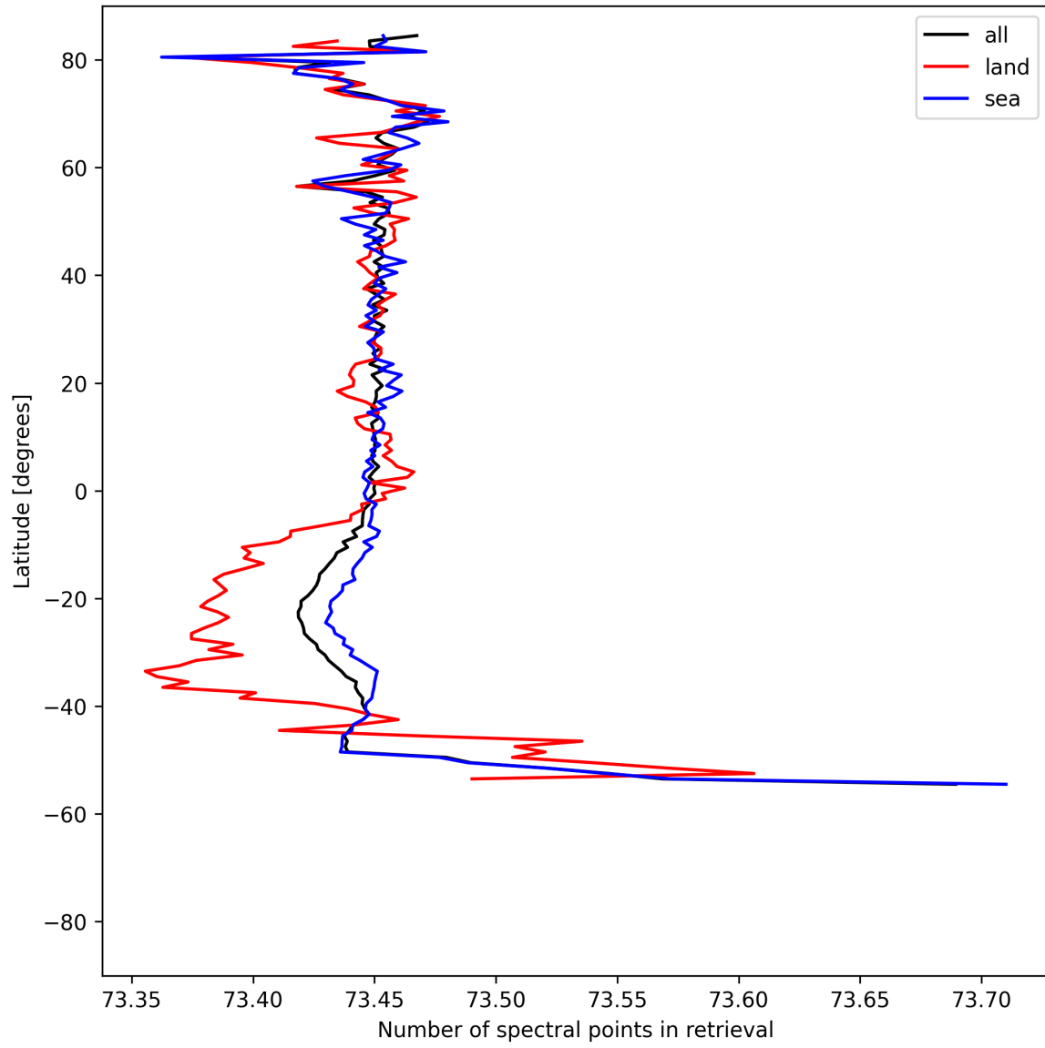
Figure 56: Zonal average of “Number of spectral points in retrieval” for 2025-08-12 to 2025-08-12.
