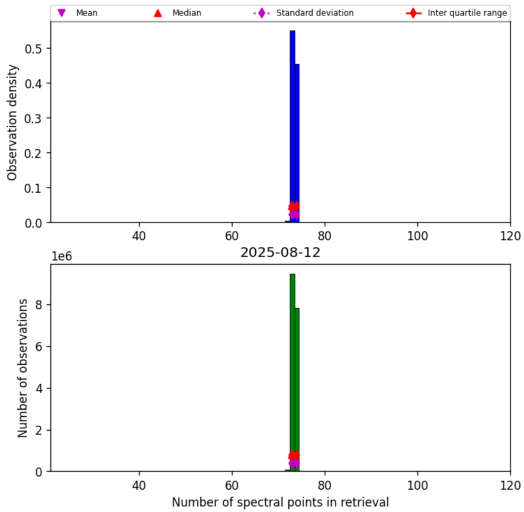
Figure 83: Histogram of “Number of spectral points in retrieval” for 2025-08-12 to 2025-08-12
