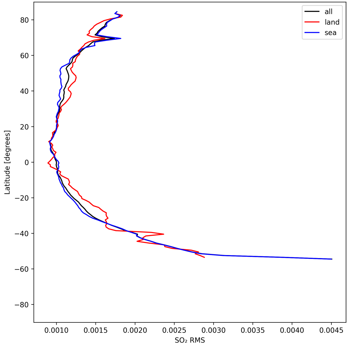
Figure 52: Zonal average of “SO 2 RMS” for 2025-08-12 to 2025-08-12.
