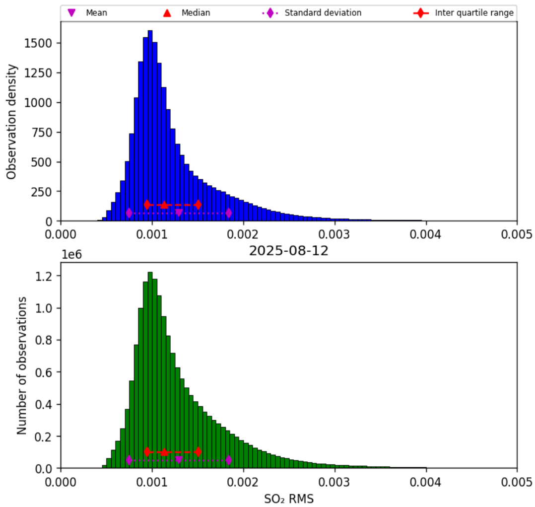
Figure 79: Histogram of “SO 2 RMS” for 2025-08-12 to 2025-08-12
