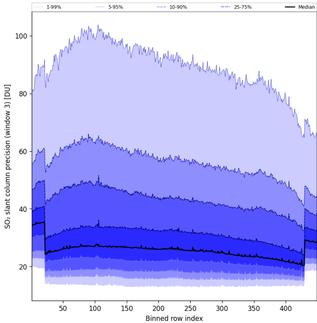
Figure 99: Along track statistics of “SO 2 slant column precision (window 3)” for 2025-08-12 to 2025-08-12
