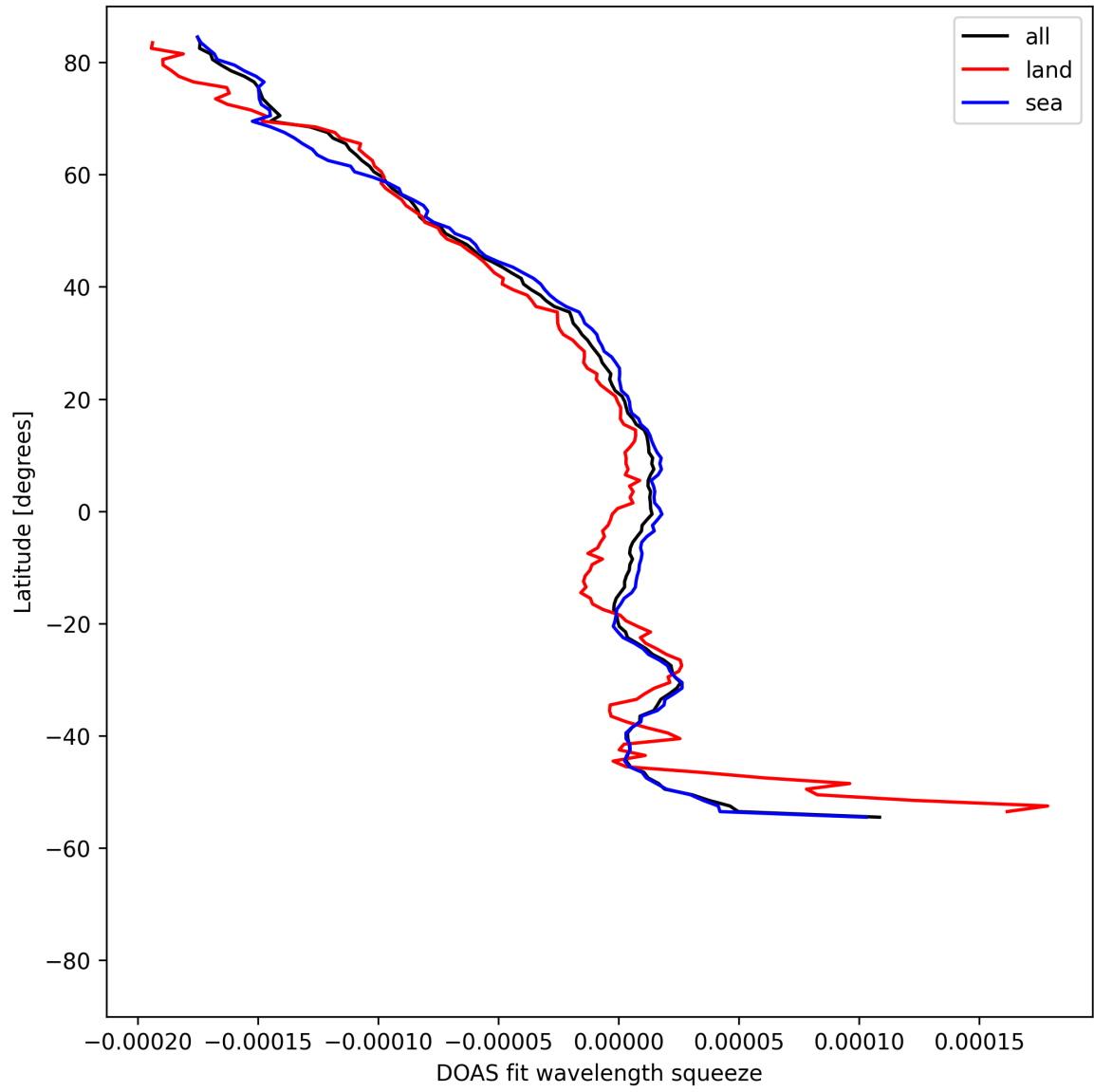
Figure 51: Zonal average of “DOAS fit wavelength squeeze” for 2025-08-12 to 2025-08-12.
