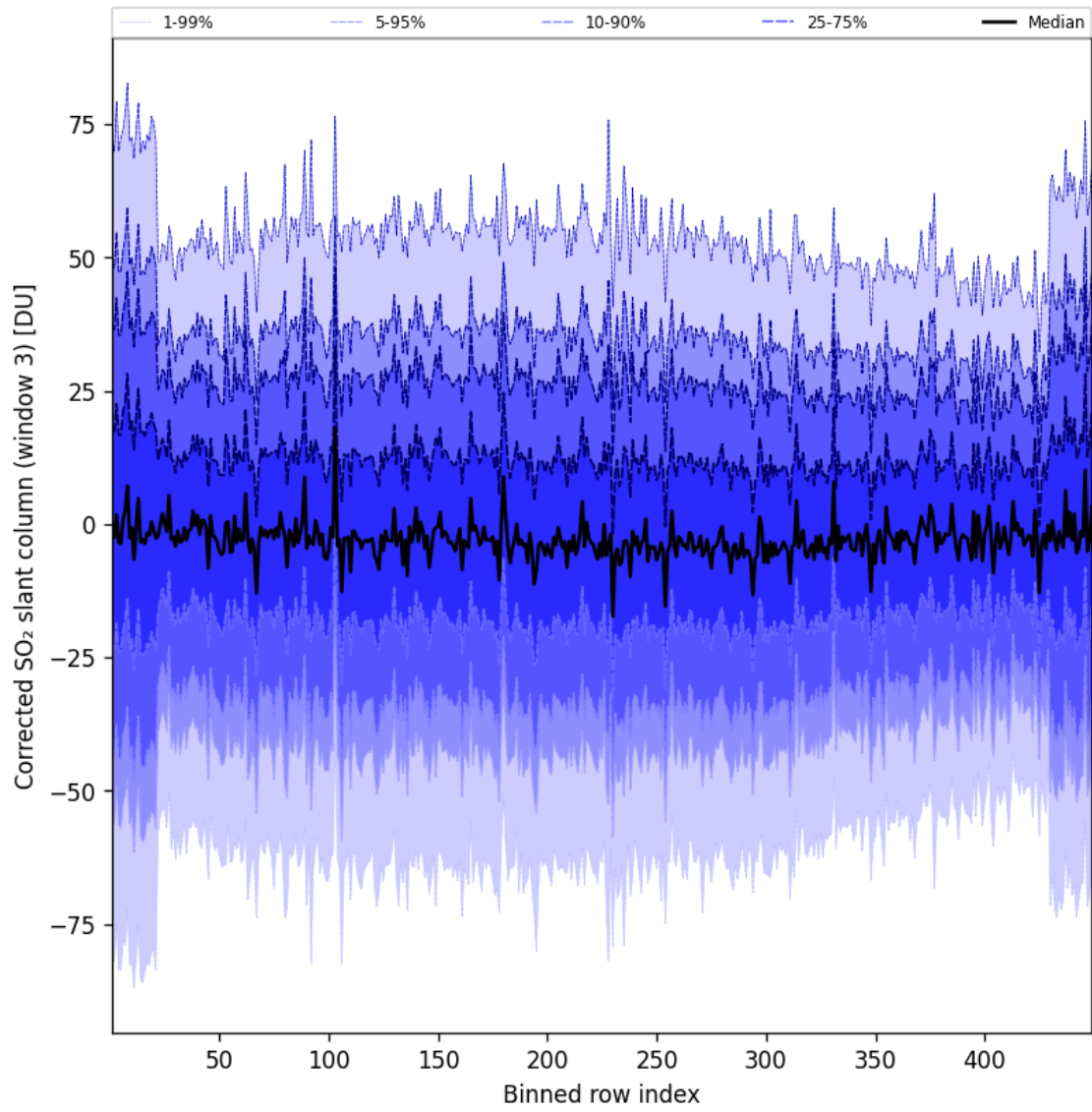
Figure 100: Along track statistics of “Corrected SO 2 slant column (window 3)” for 2025-08-12 to 2025-08-12
