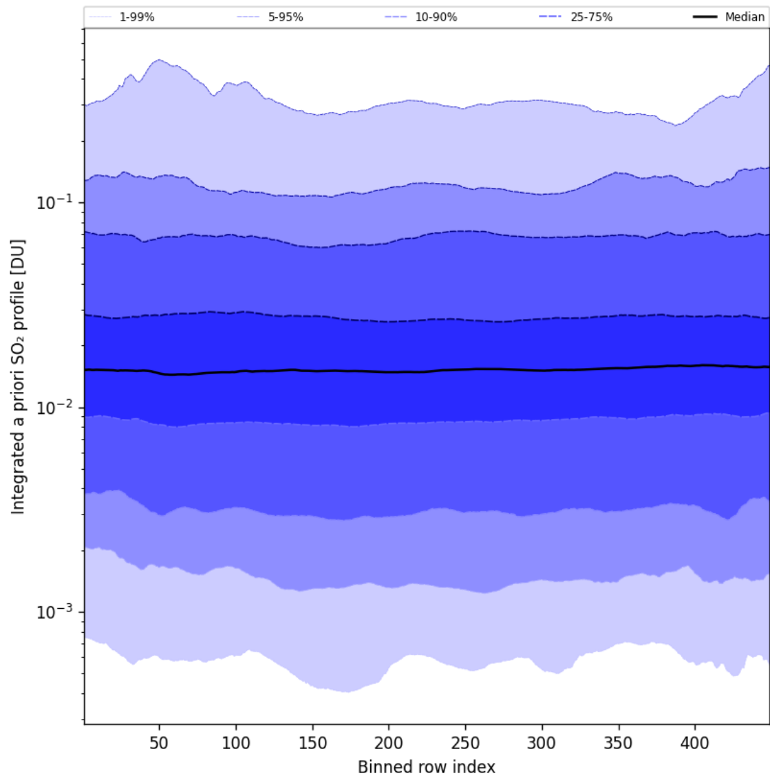
Figure 103: Along track statistics of “Integrated a priori SO 2 profile” for 2025-08-12 to 2025-08-12
