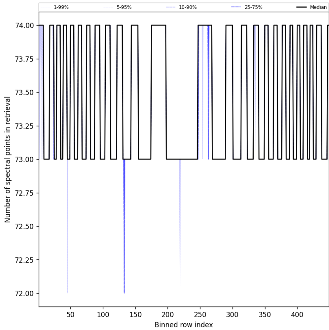
Figure 110: Along track statistics of “Number of spectral points in retrieval” for 2025-08-12 to 2025-08-12
