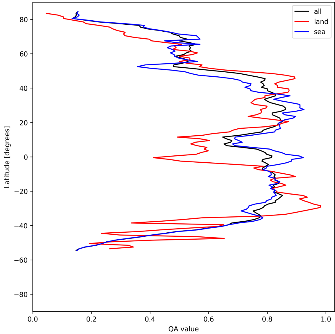
Figure 30: Zonal average of “QA value” for 2025-08-12 to 2025-08-12.
