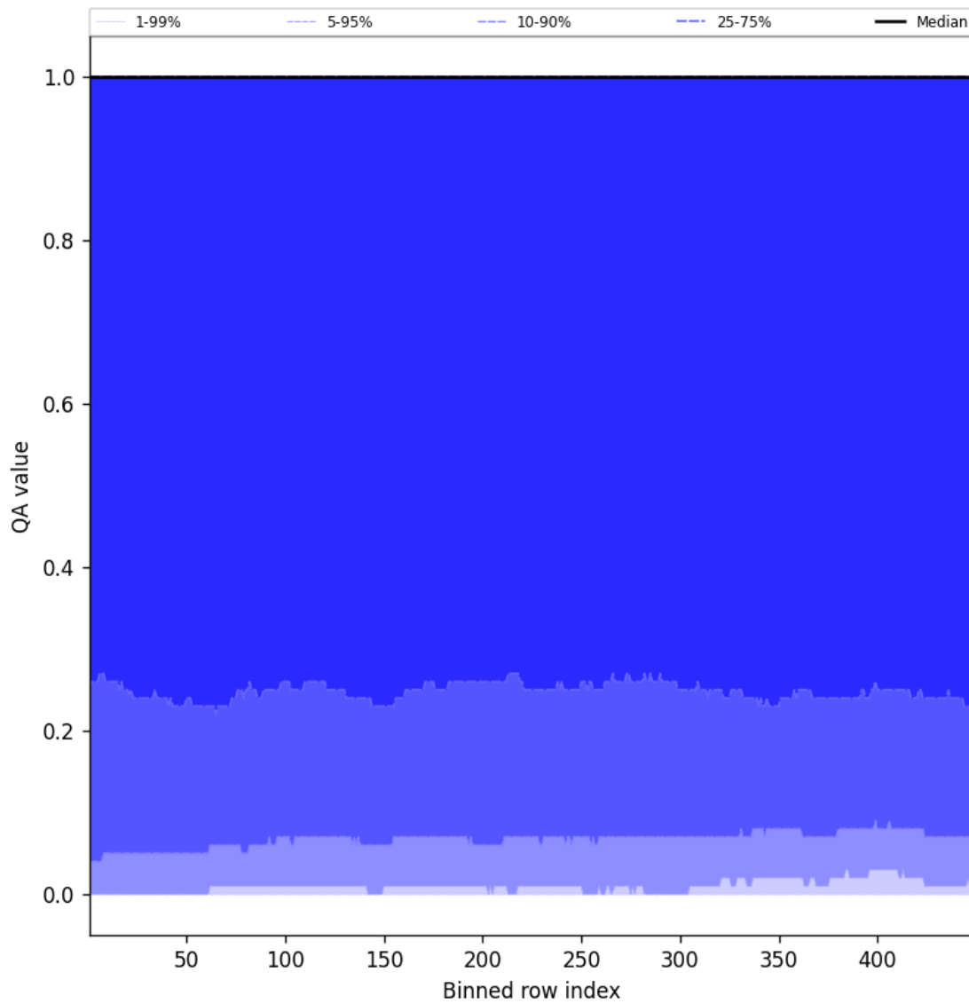
Figure 84: Along track statistics of “QA value” for 2025-08-12 to 2025-08-12
