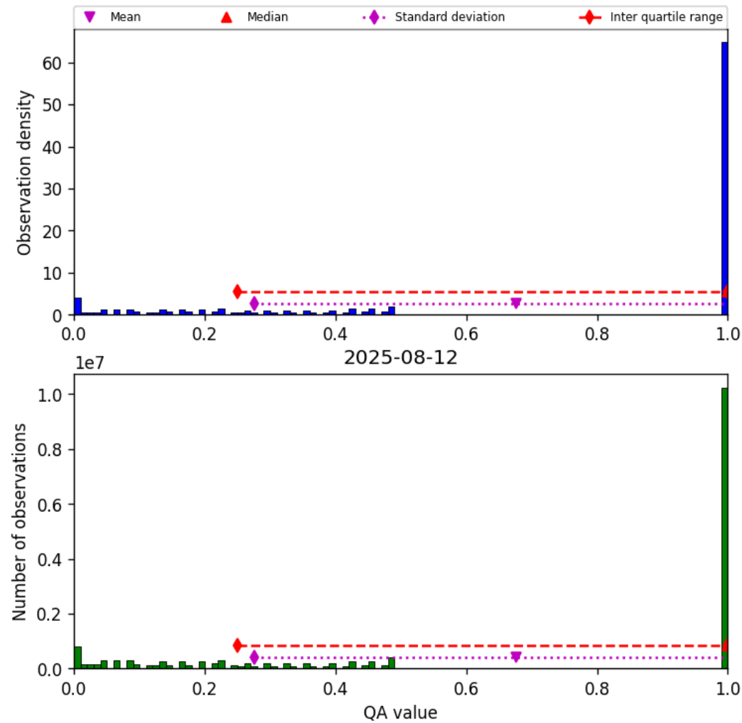
Figure 57: Histogram of “QA value” for 2025-08-12 to 2025-08-12
