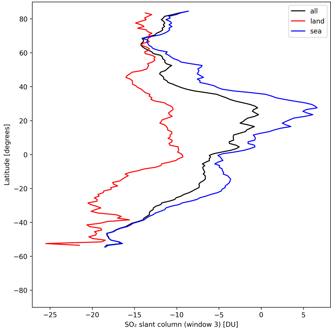
Figure 44: Zonal average of “SO 2 slant column (window 3)” for 2025-08-12 to 2025-08-12.
