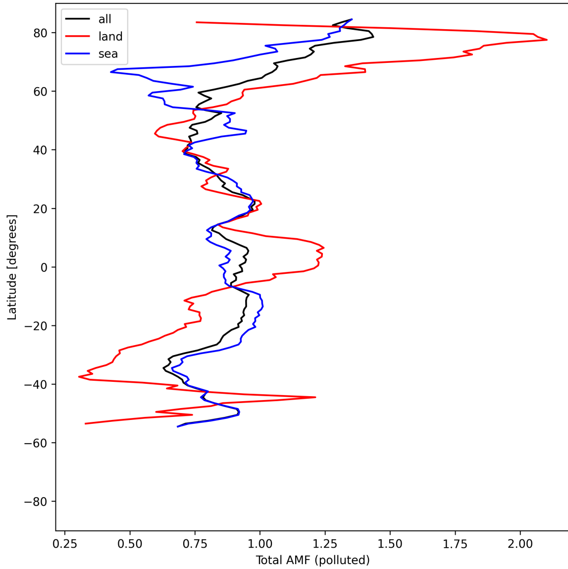
Figure 53: Zonal average of “Total AMF (polluted)” for 2025-08-12 to 2025-08-12.
