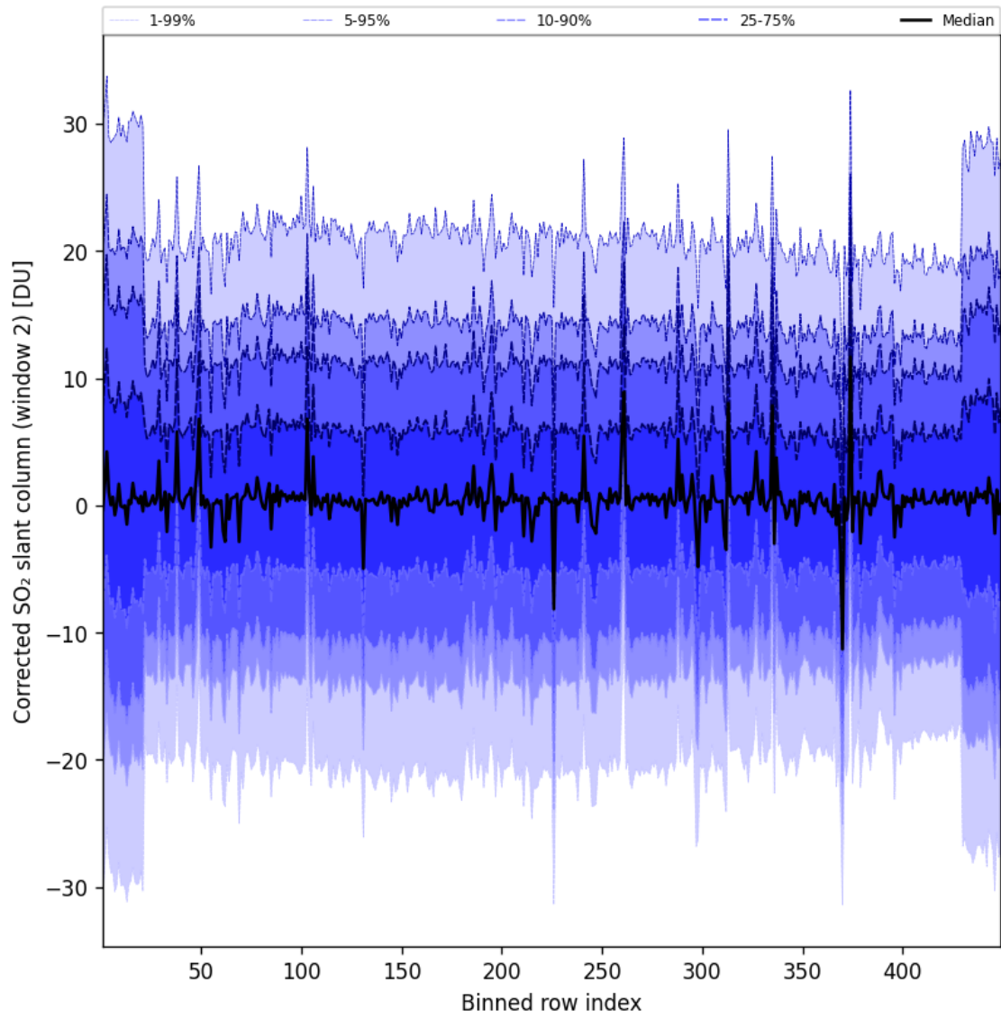
Figure 96: Along track statistics of “Corrected SO 2 slant column (window 2)” for 2025-08-12 to 2025-08-12
