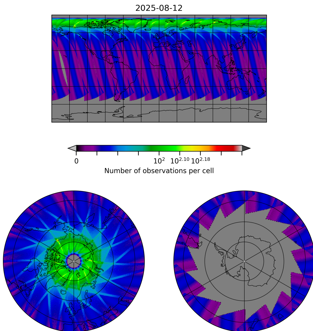
Figure 29: Map of the number of observations for 2025-08-12 to 2025-08-12
