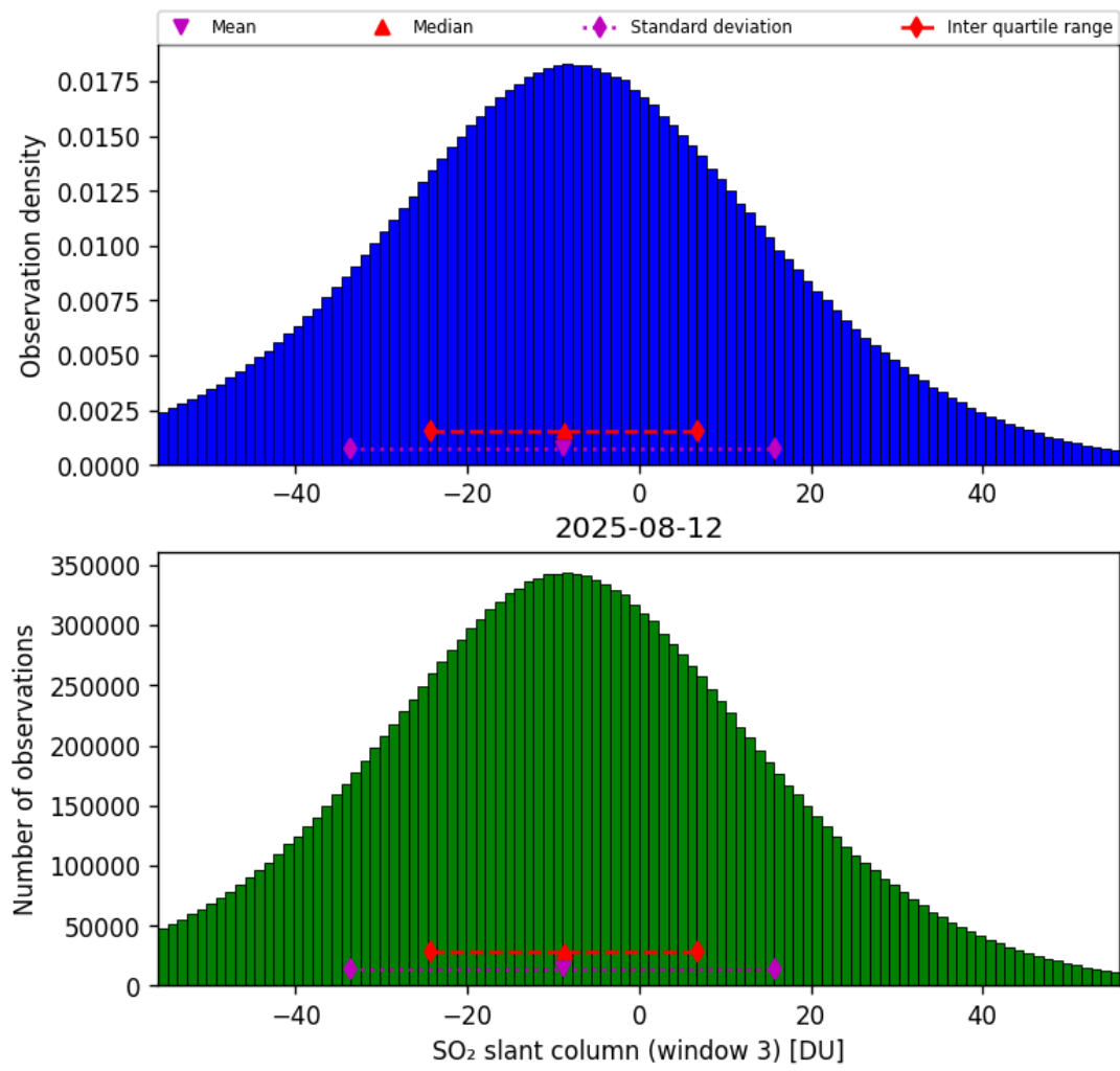
Figure 71: Histogram of “SO 2 slant column (window 3)” for 2025-08-12 to 2025-08-12
