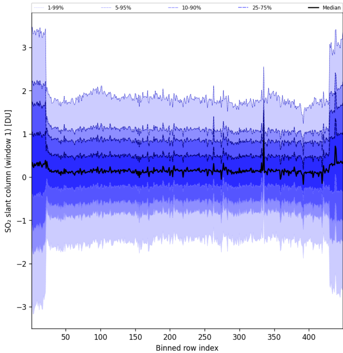
Figure 90: Along track statistics of “SO 2 slant column (window 1)” for 2025-08-12 to 2025-08-12
