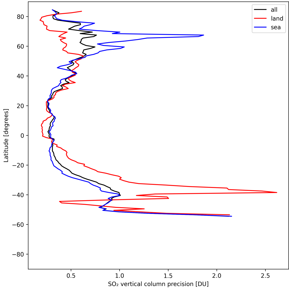
Figure 32: Zonal average of “SO 2 vertical column precision” for 2025-08-12 to 2025-08-12.
