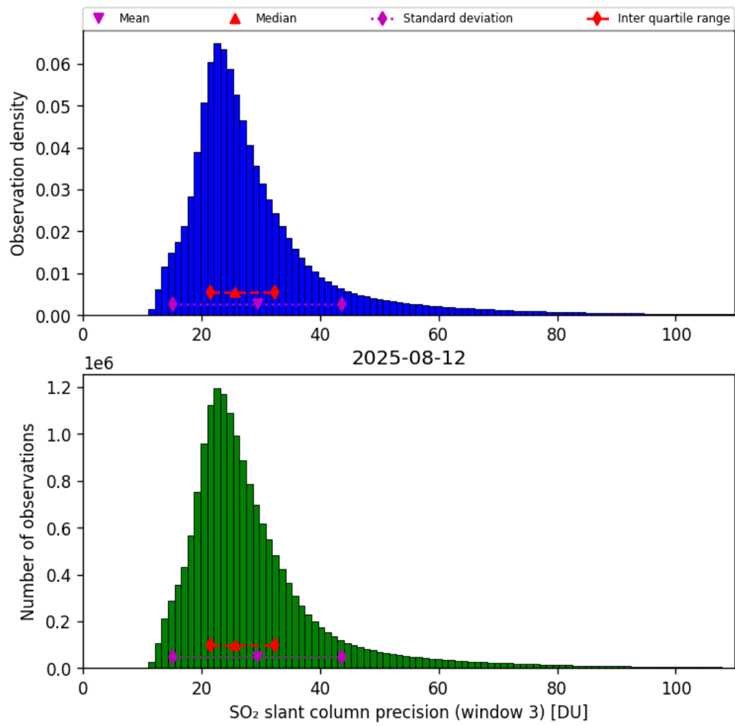
Figure 72: Histogram of “SO 2 slant column precision (window 3)” for 2025-08-12 to 2025-08-12
