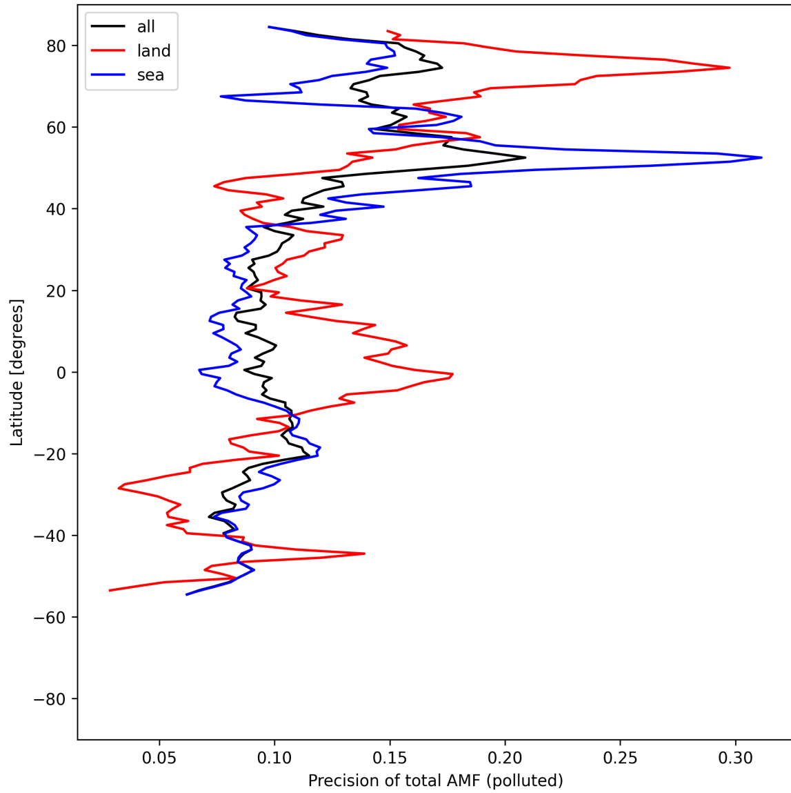
Figure 54: Zonal average of “Precision of total AMF (polluted)” for 2025-08-12 to 2025-08-12.
