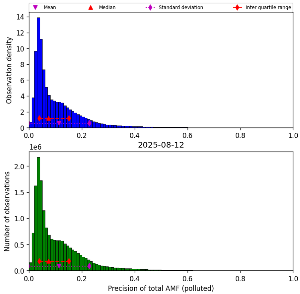
Figure 81: Histogram of “Precision of total AMF (polluted)” for 2025-08-12 to 2025-08-12
