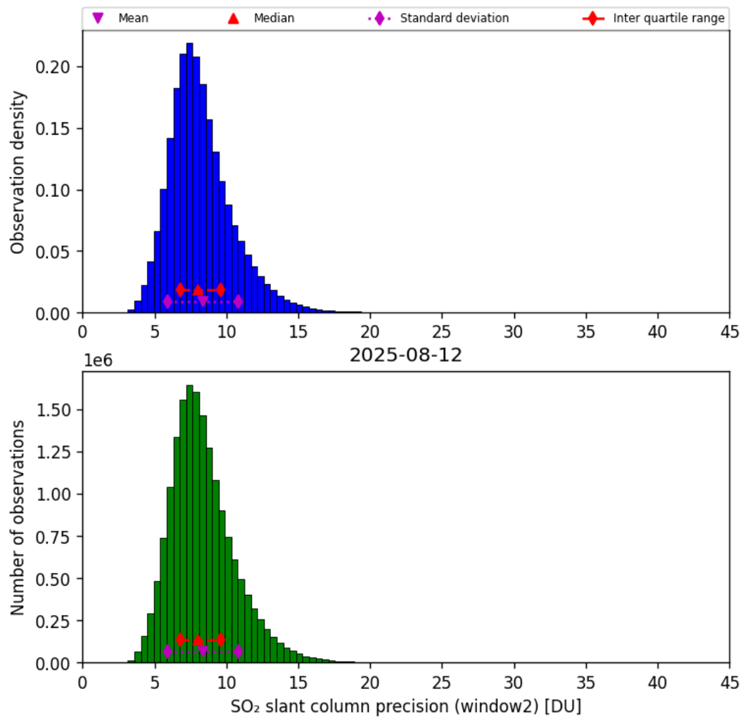
Figure 68: Histogram of “SO 2 slant column precision (window2)” for 2025-08-12 to 2025-08-12
