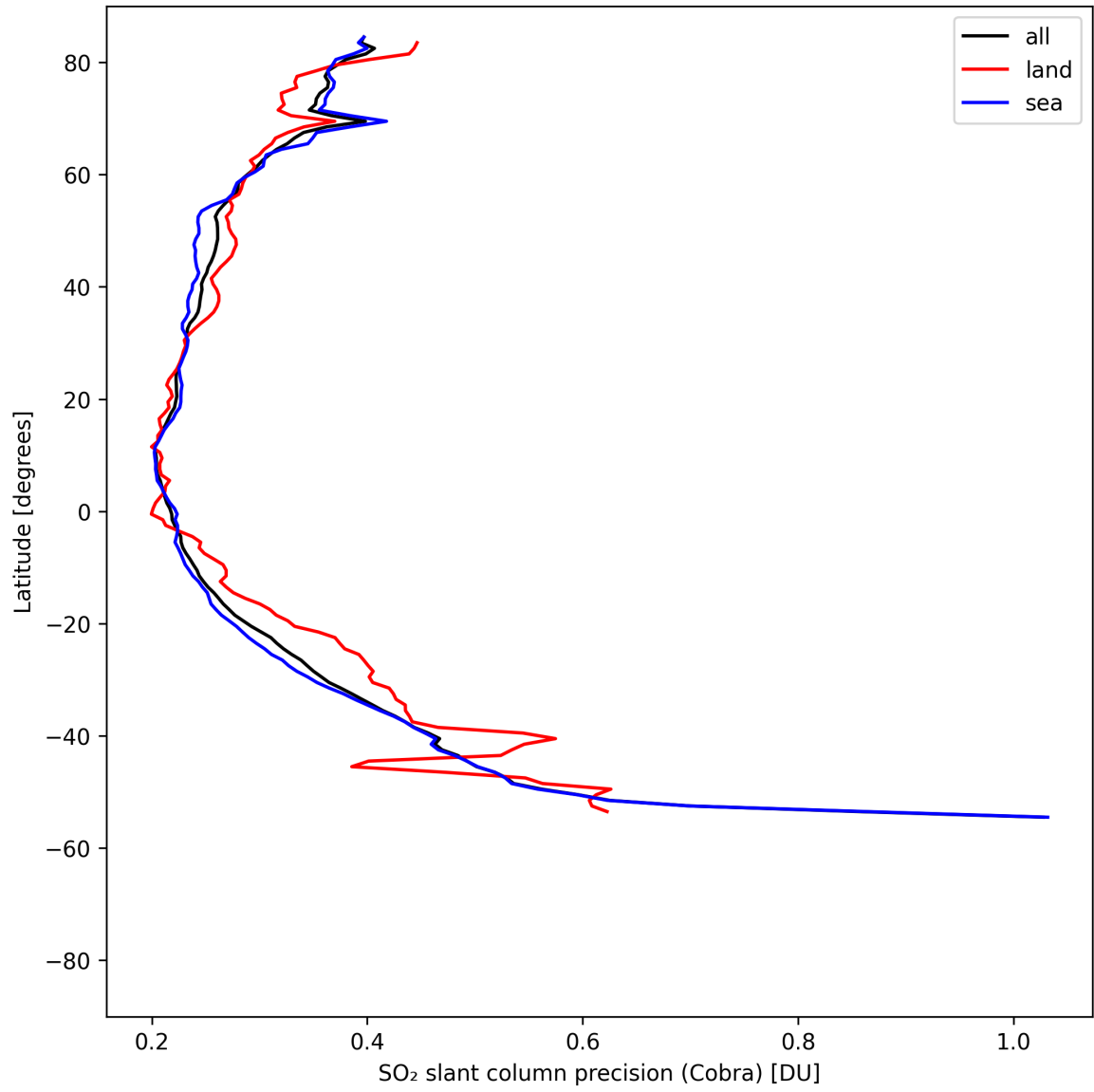
Figure 35: Zonal average of “SO 2 slant column precision (Cobra)” for 2025-08-12 to 2025-08-12.
