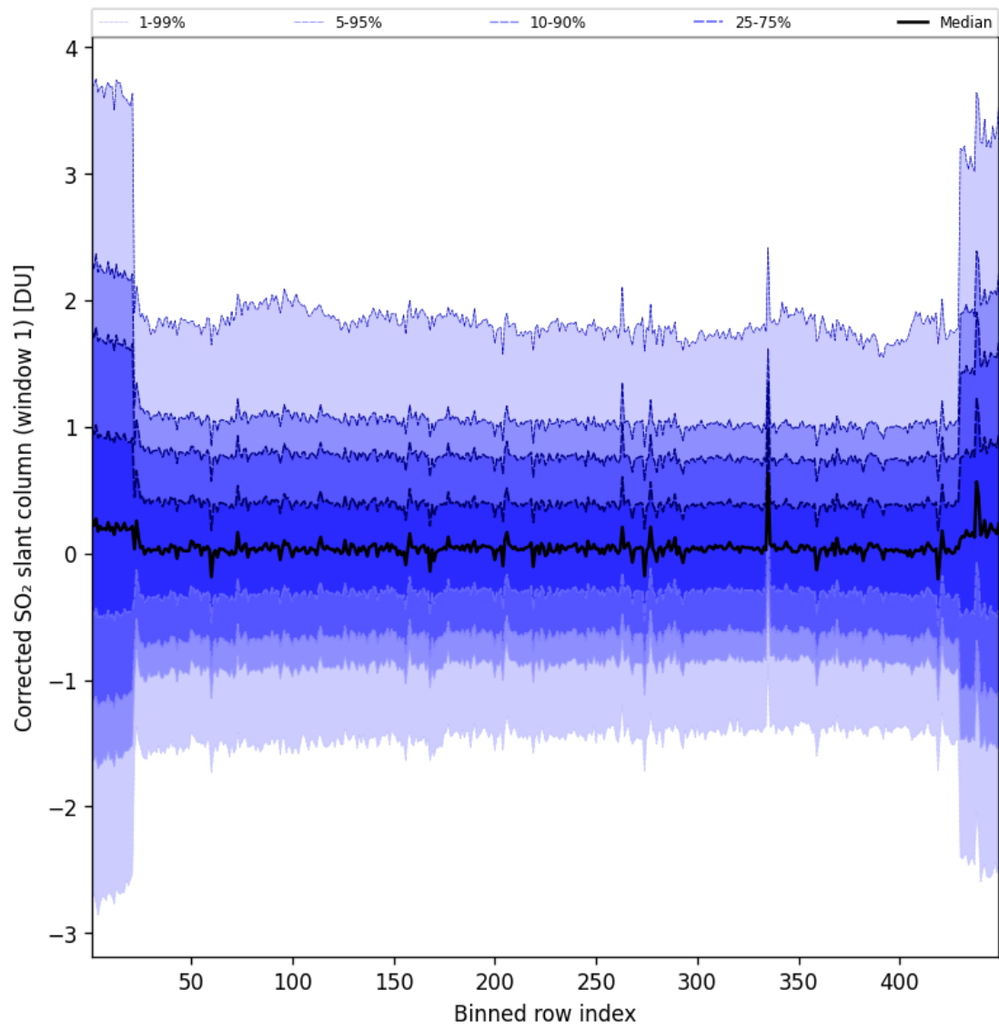
Figure 92: Along track statistics of “Corrected SO 2 slant column (window 1)” for 2025-08-12 to 2025-08-12
