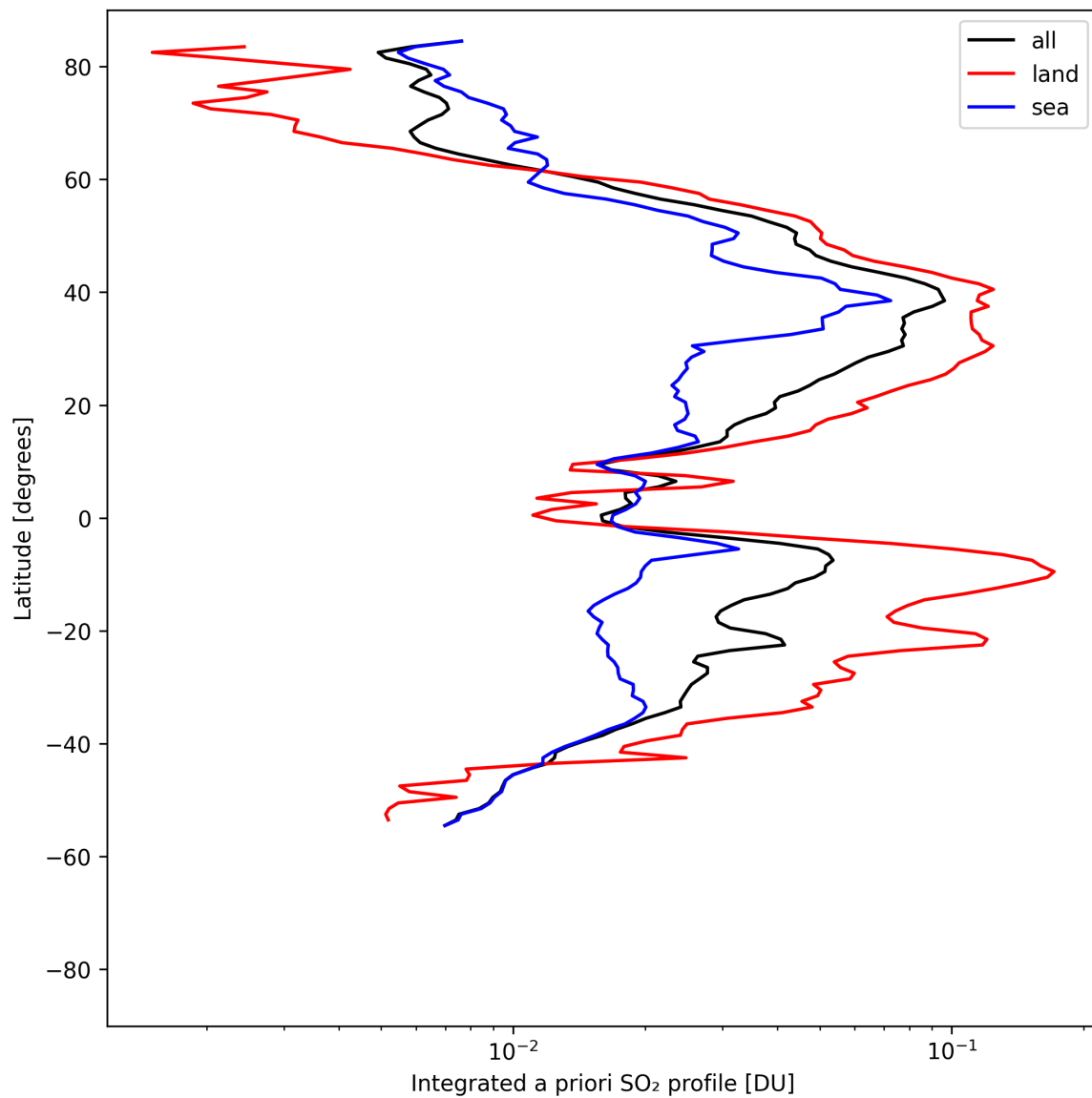
Figure 49: Zonal average of “Integrated a priori SO 2 profile” for 2025-08-12 to 2025-08-12.
