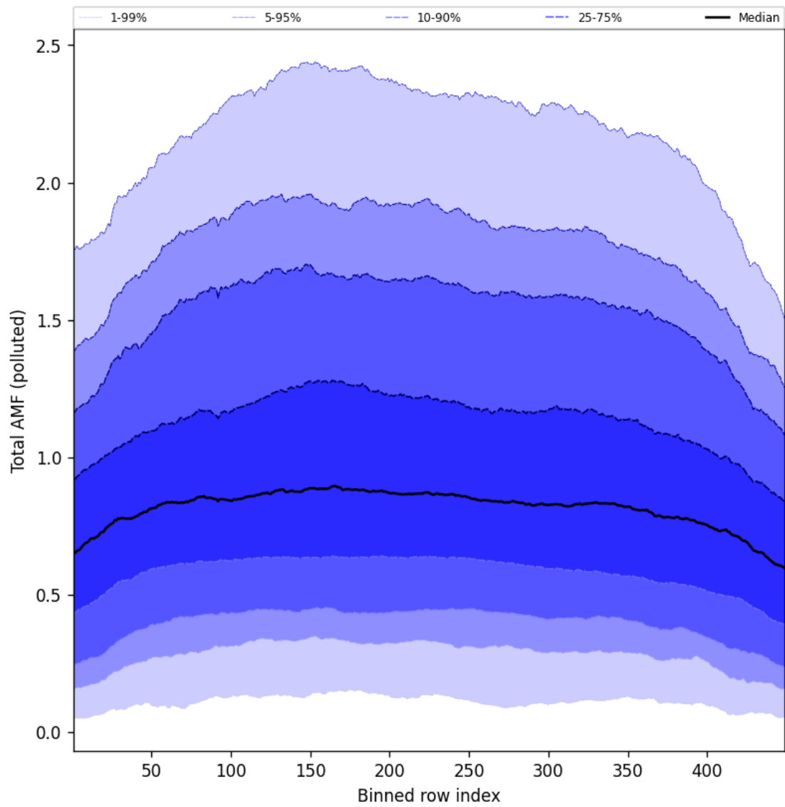
Figure 107: Along track statistics of “Total AMF (polluted)” for 2025-08-12 to 2025-08-12
