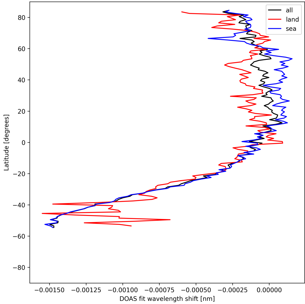
Figure 50: Zonal average of “DOAS fit wavelength shift” for 2025-08-12 to 2025-08-12.
