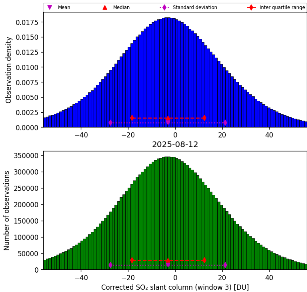
Figure 73: Histogram of “Corrected SO 2 slant column (window 3)” for 2025-08-12 to 2025-08-12
