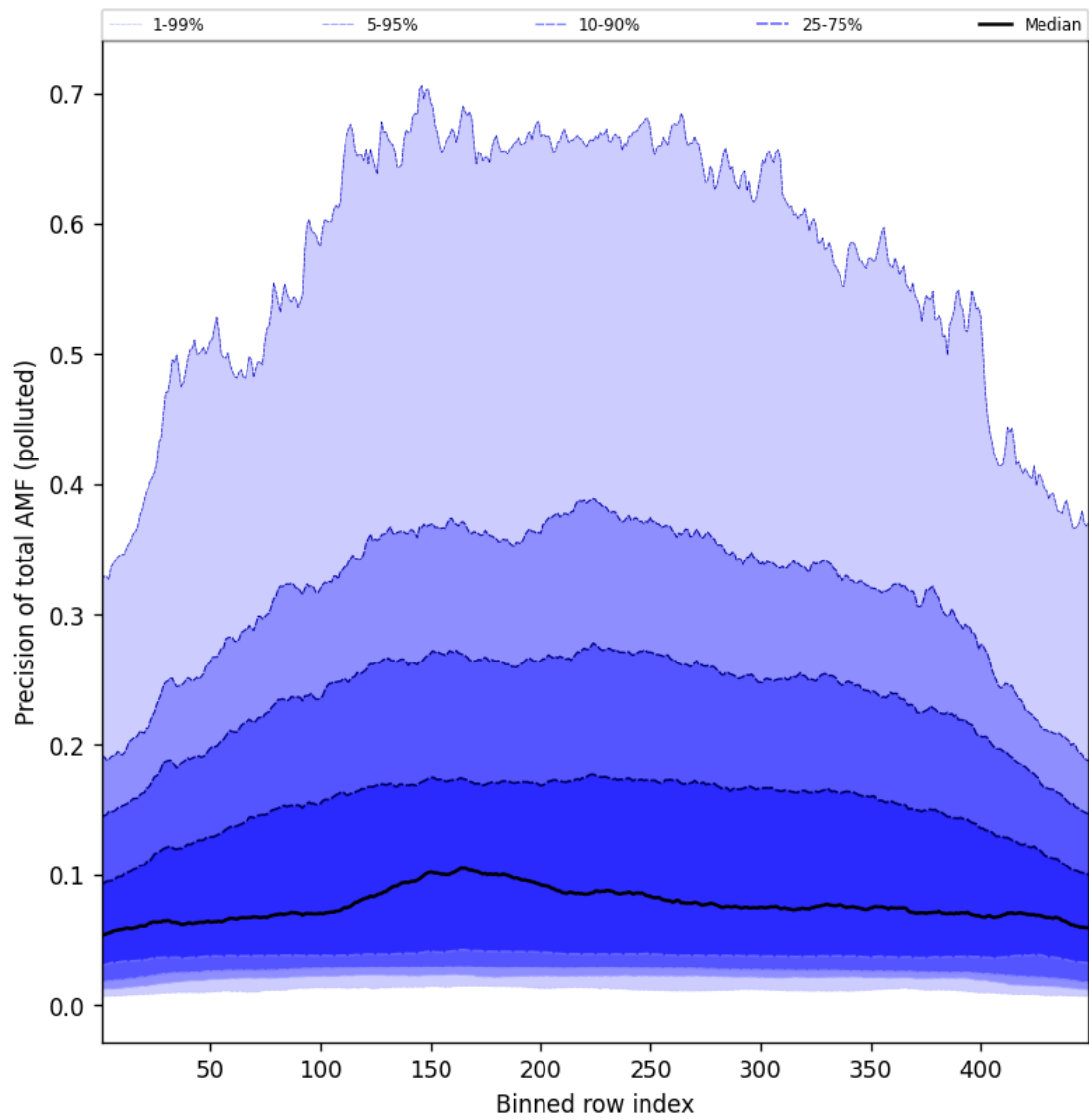
Figure 108: Along track statistics of “Precision of total AMF (polluted)” for 2025-08-12 to 2025-08-12
