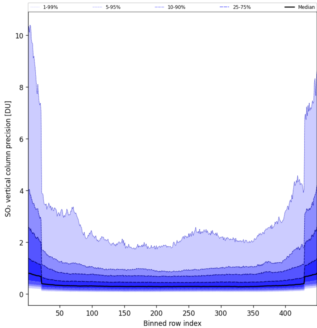
Figure 86: Along track statistics of “SO 2 vertical column precision” for 2025-08-12 to 2025-08-12
