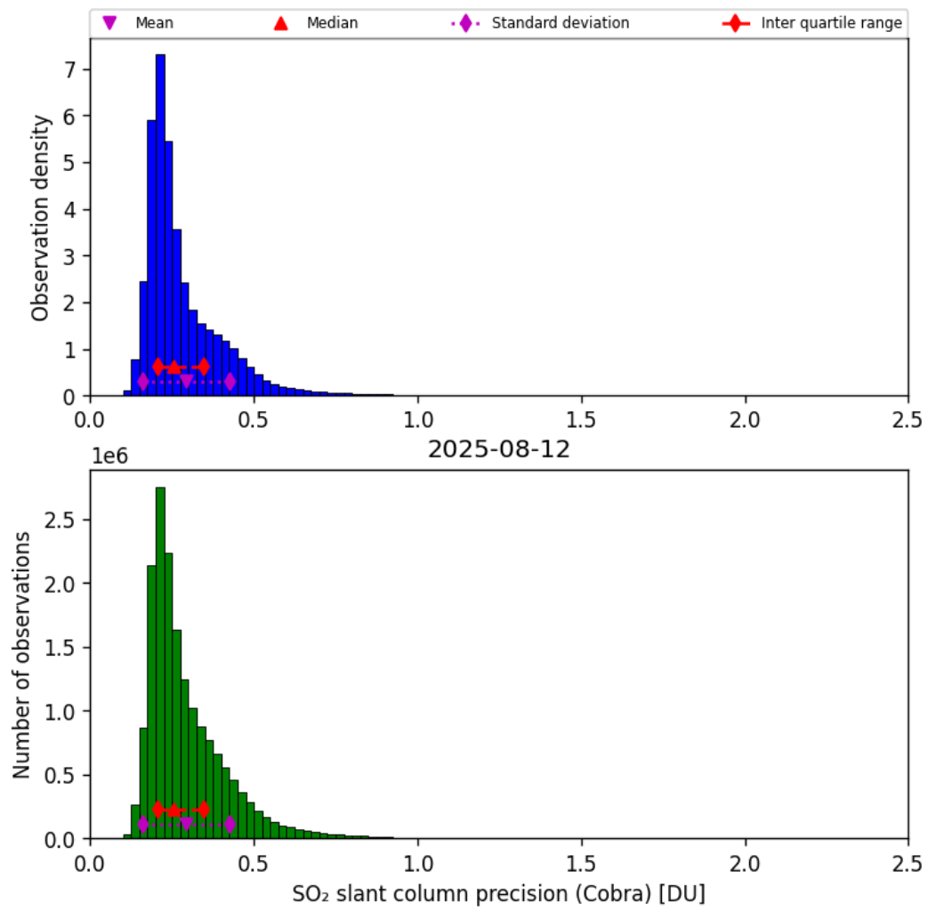
Figure 62: Histogram of “SO 2 slant column precision (Cobra)” for 2025-08-12 to 2025-08-12
