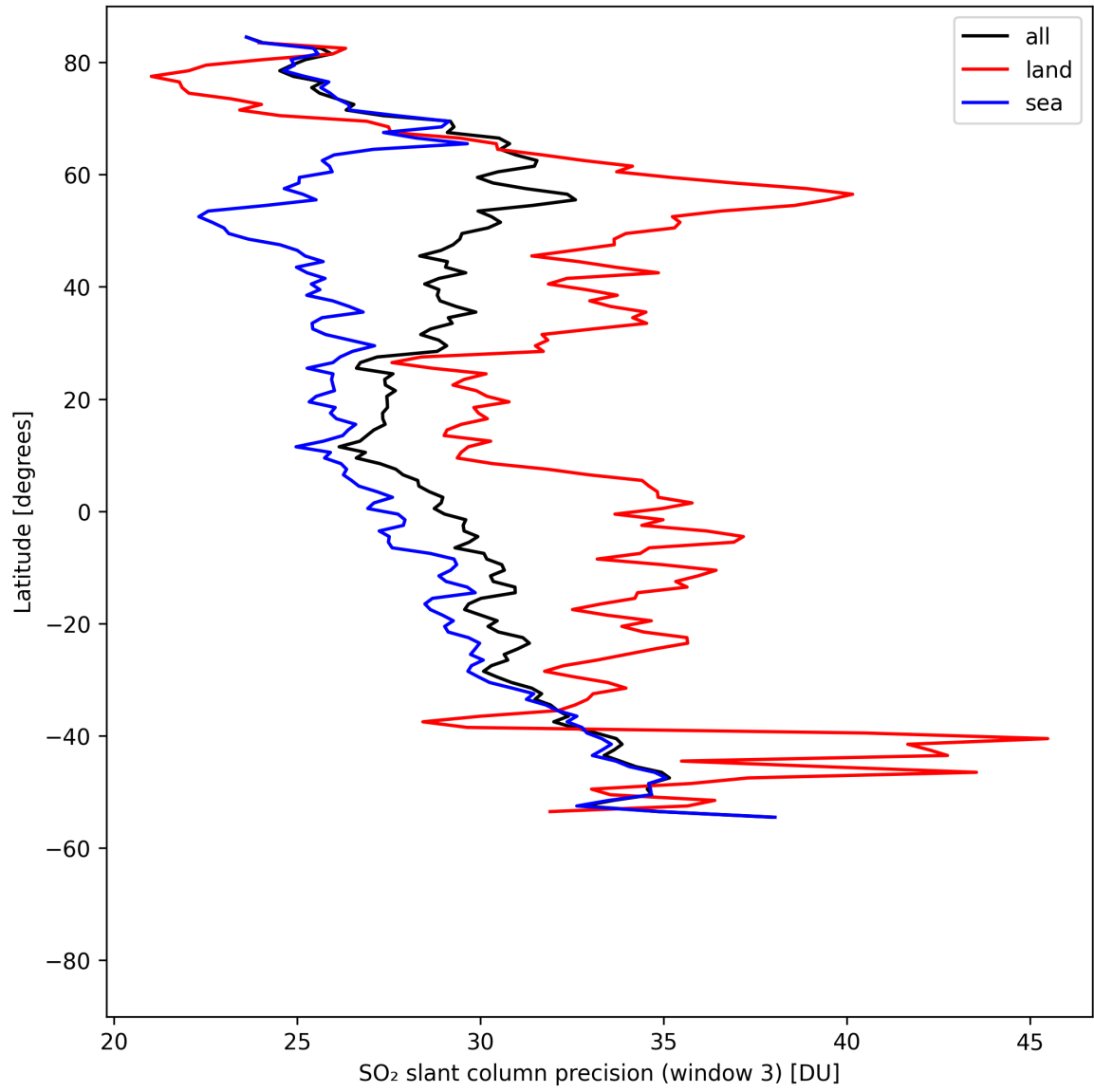
Figure 45: Zonal average of “SO 2 slant column precision (window 3)” for 2025-08-12 to 2025-08-12.
