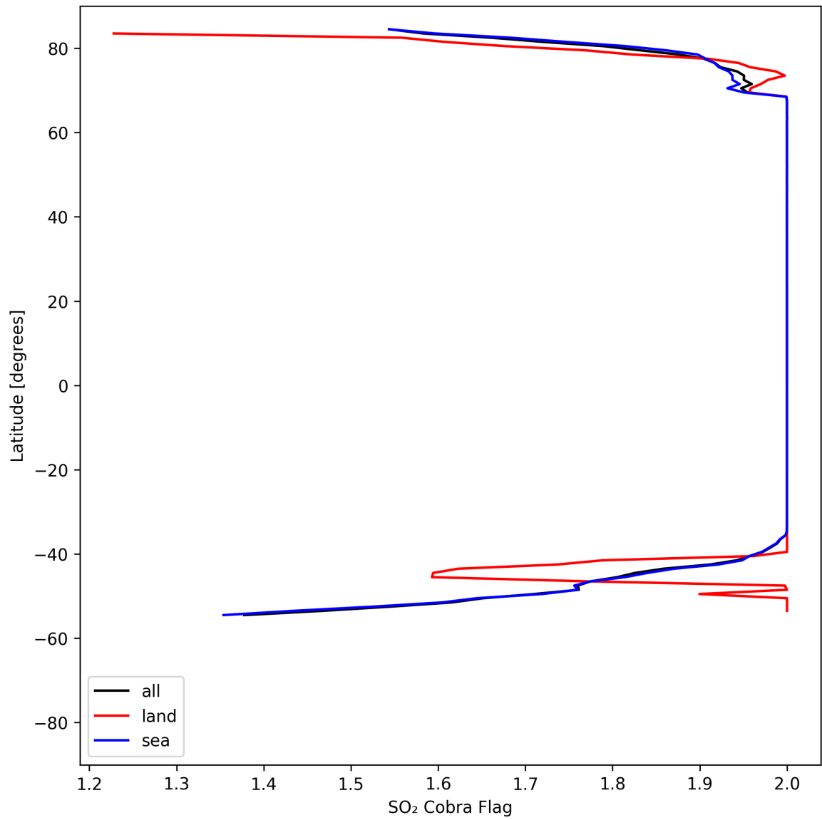
Figure 48: Zonal average of “SO 2 Cobra Flag” for 2025-08-12 to 2025-08-12.
