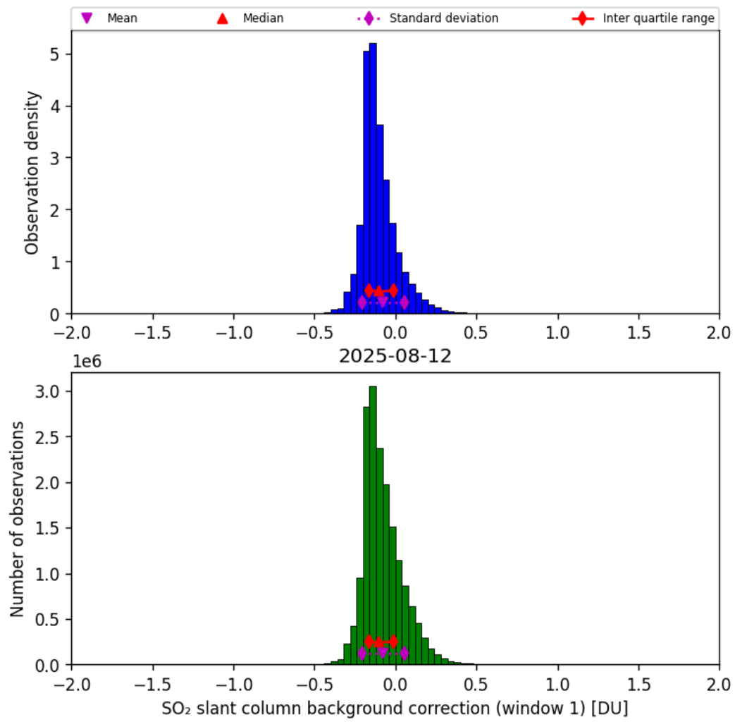
Figure 66: Histogram of “SO 2 slant column background correction (window 1)” for 2025-08-12 to 2025-08-12
