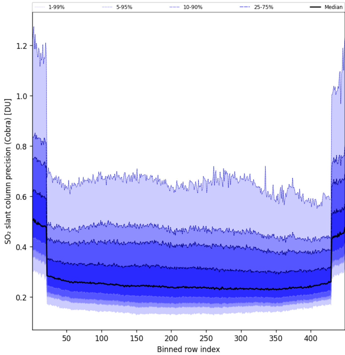
Figure 89: Along track statistics of “SO 2 slant column precision (Cobra)” for 2025-08-12 to 2025-08-12
