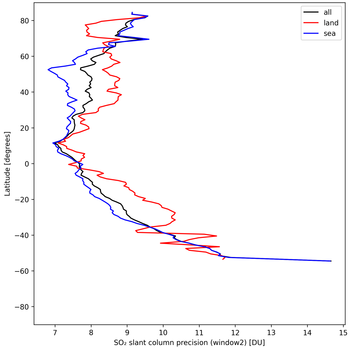
Figure 41: Zonal average of “SO 2 slant column precision (window2)” for 2025-08-12 to 2025-08-12.
