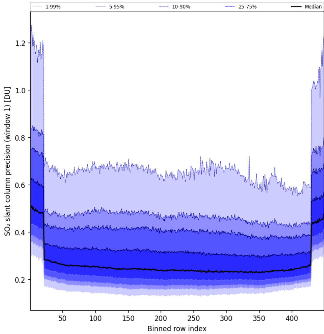
Figure 91: Along track statistics of “SO 2 slant column precision (window 1)” for 2025-08-12 to 2025-08-12
