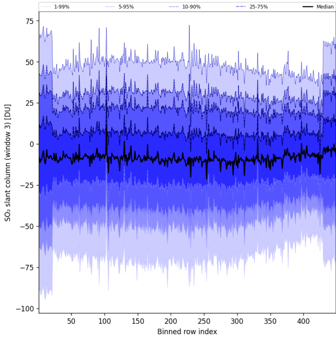
Figure 98: Along track statistics of “SO 2 slant column (window 3)” for 2025-08-12 to 2025-08-12
