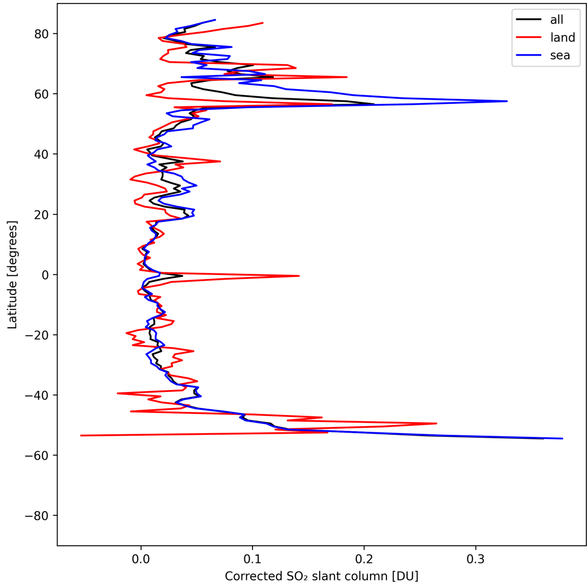
Figure 33: Zonal average of “Corrected SO 2 slant column” for 2025-08-12 to 2025-08-12.
