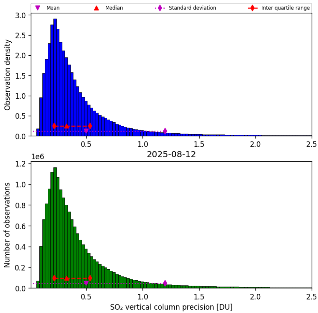
Figure 59: Histogram of “SO 2 vertical column precision” for 2025-08-12 to 2025-08-12
