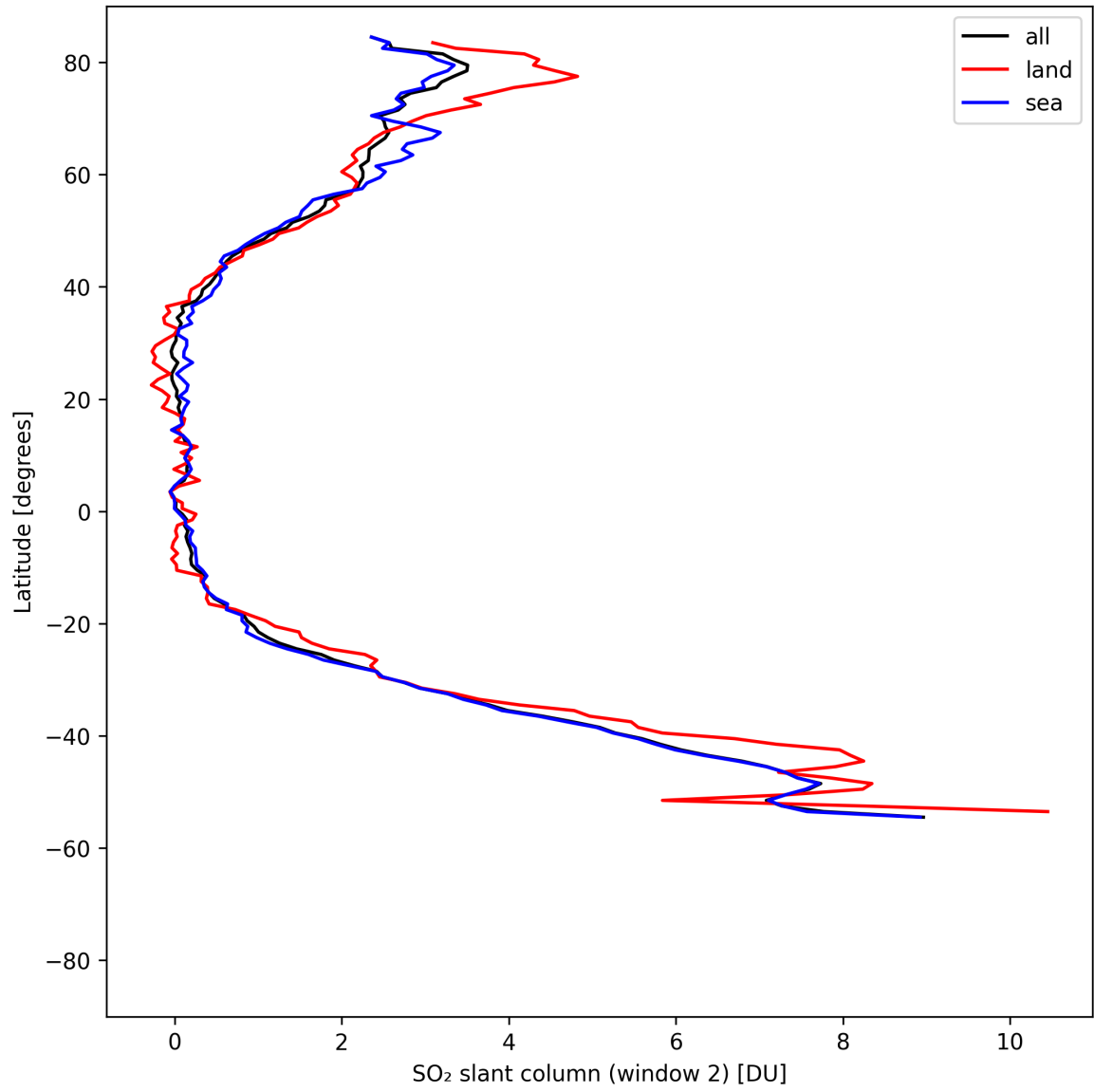
Figure 40: Zonal average of “SO 2 slant column (window 2)” for 2025-08-12 to 2025-08-12.
