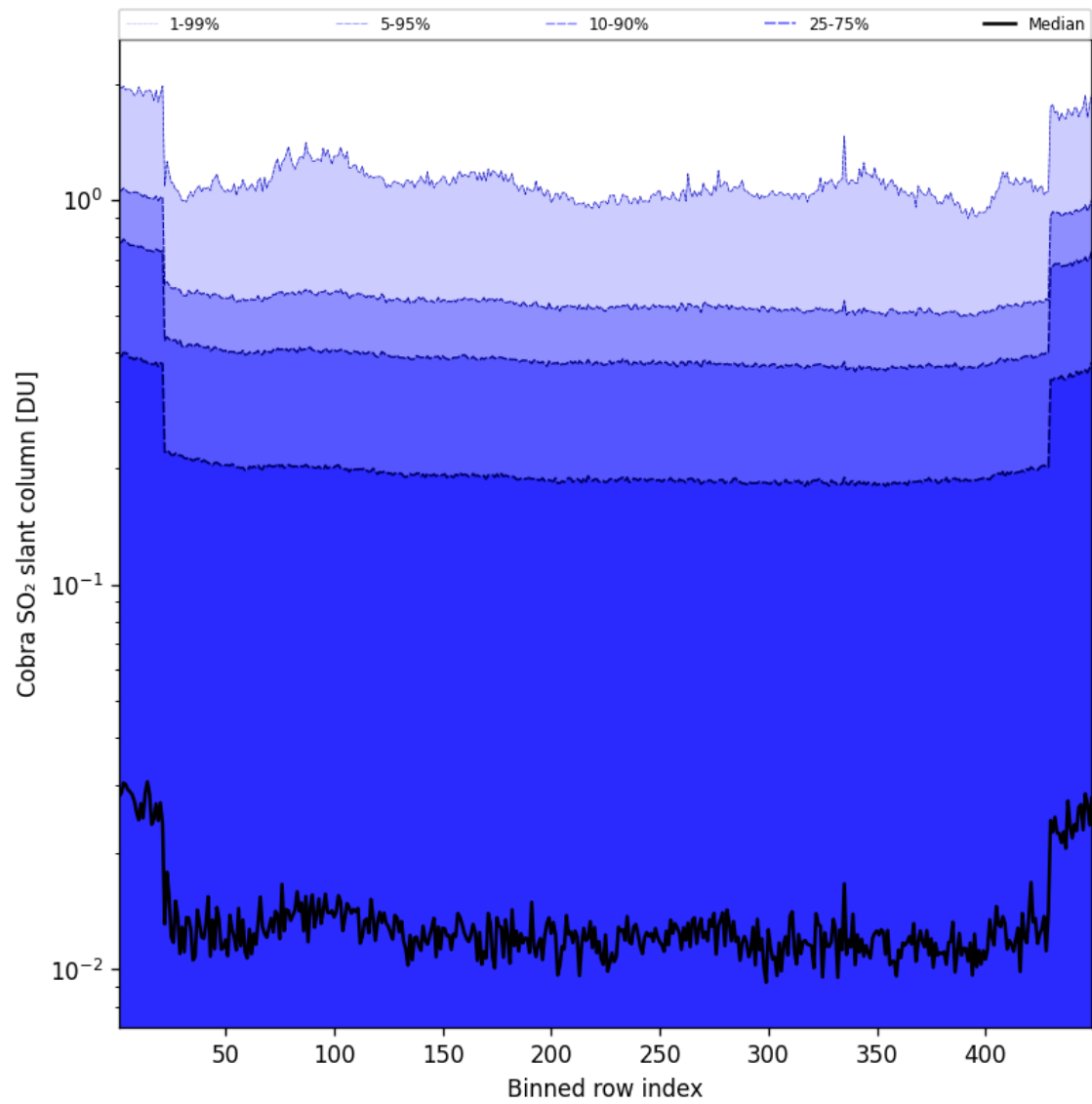
Figure 88: Along track statistics of “Cobra SO 2 slant column” for 2025-08-12 to 2025-08-12
