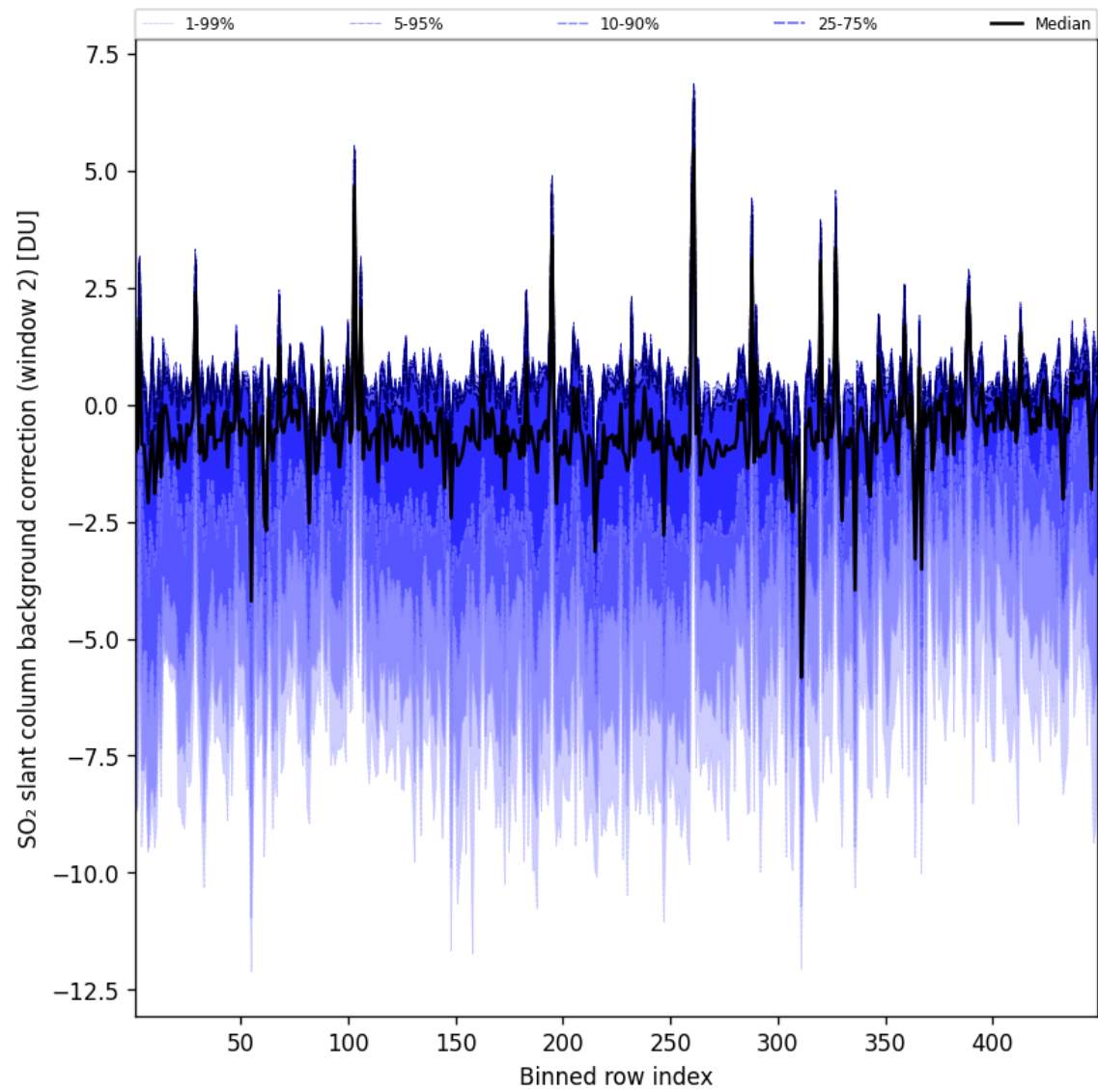
Figure 97: Along track statistics of “SO 2 slant column background correction (window 2)” for 2025-08-12 to 2025-08-12
