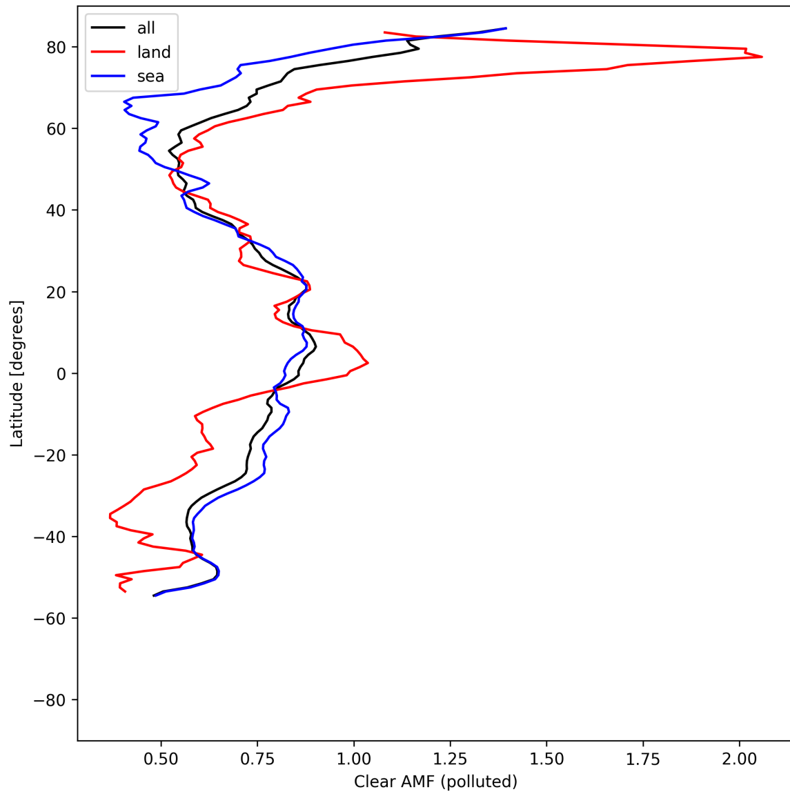
Figure 55: Zonal average of “Clear AMF (polluted)” for 2025-08-12 to 2025-08-12.
