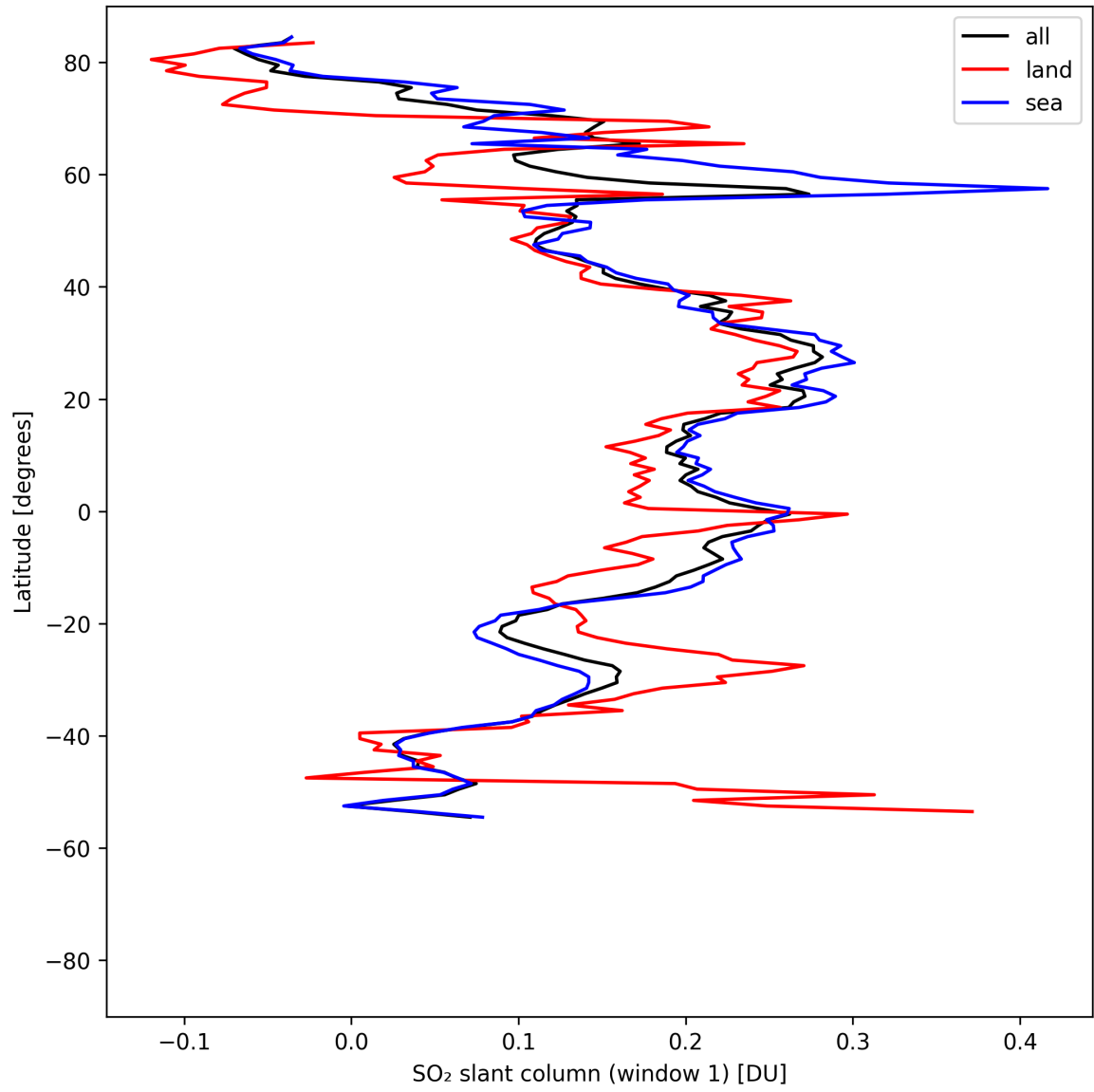
Figure 36: Zonal average of “SO 2 slant column (window 1)” for 2025-08-12 to 2025-08-12.
