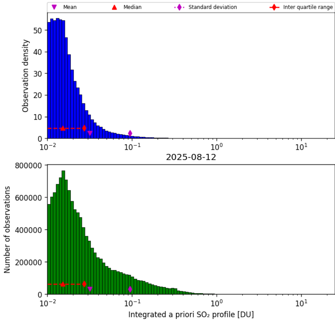
Figure 76: Histogram of “Integrated a priori SO 2 profile” for 2025-08-12 to 2025-08-12
