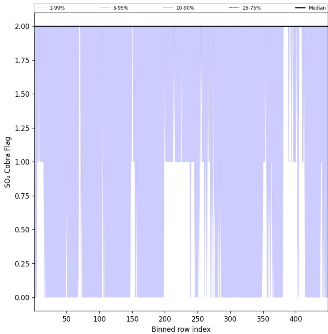
Figure 102: Along track statistics of “SO 2 Cobra Flag” for 2025-08-12 to 2025-08-12
