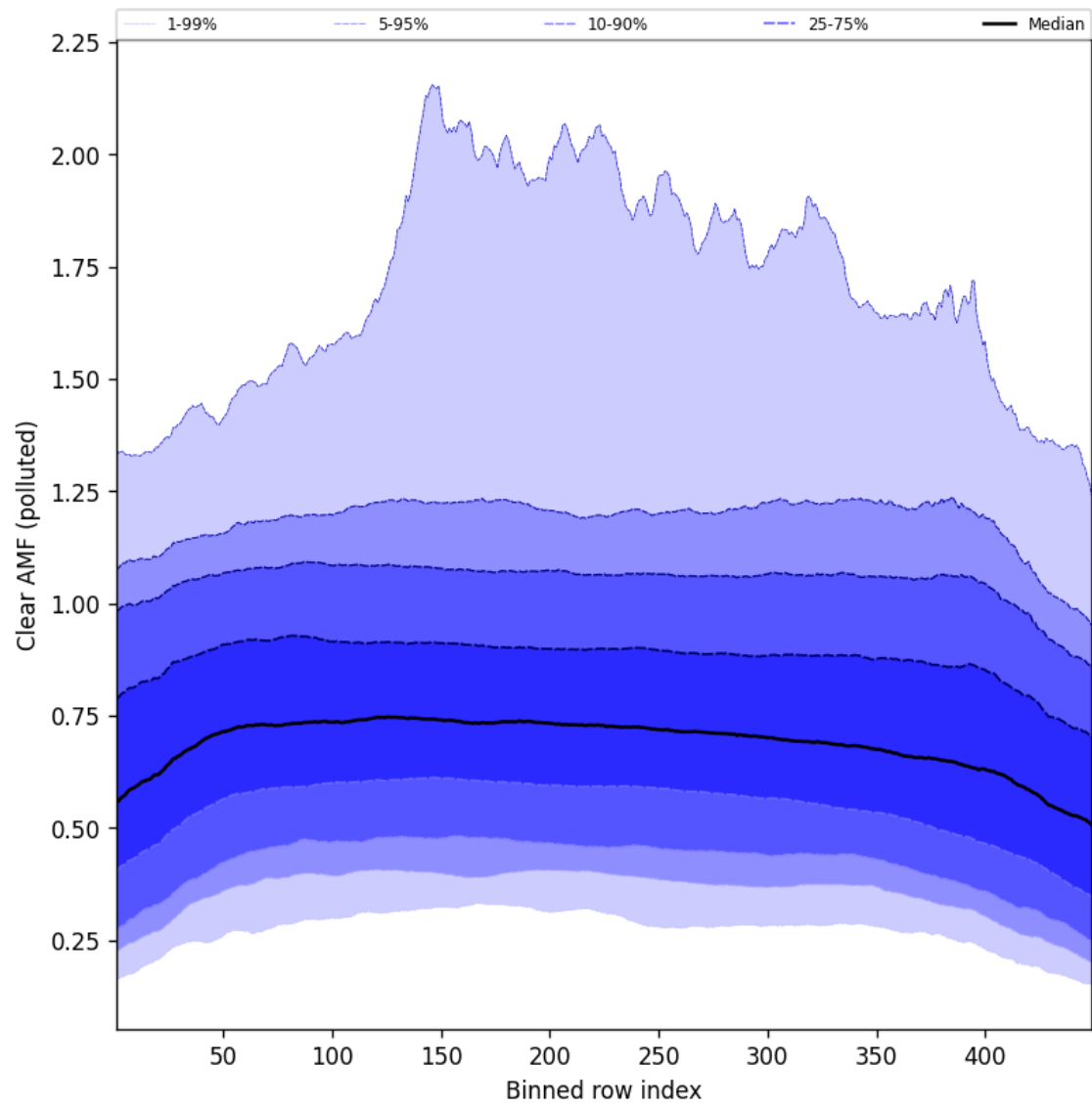
Figure 109: Along track statistics of “Clear AMF (polluted)” for 2025-08-12 to 2025-08-12
