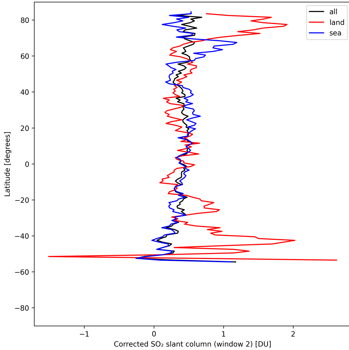
Figure 42: Zonal average of “Corrected SO 2 slant column (window 2)” for 2025-08-12 to 2025-08-12.
