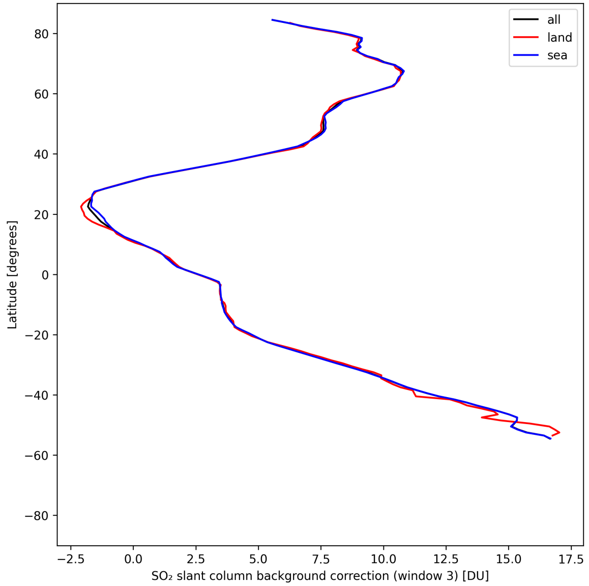
Figure 47: Zonal average of “SO 2 slant column background correction (window 3)” for 2025-08-12 to 2025-08-12.
