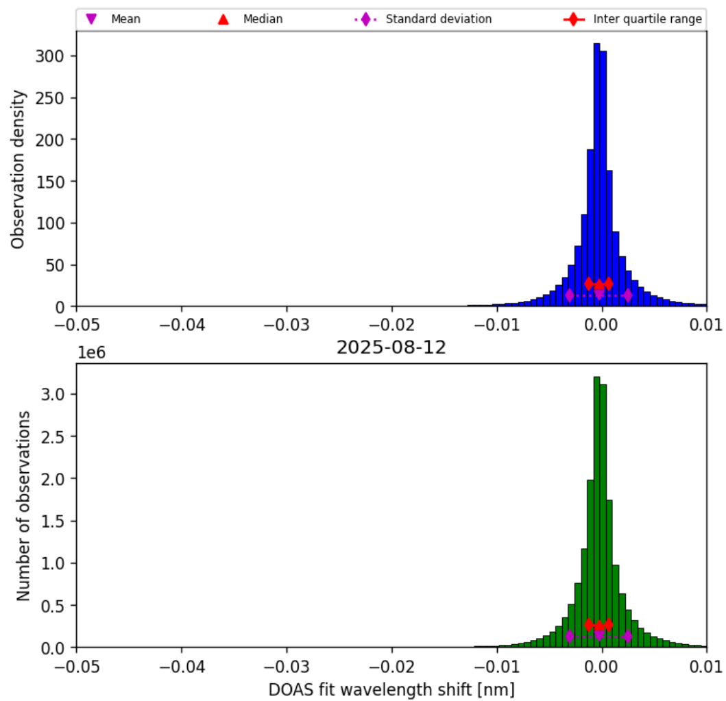
Figure 77: Histogram of “DOAS fit wavelength shift” for 2025-08-12 to 2025-08-12
