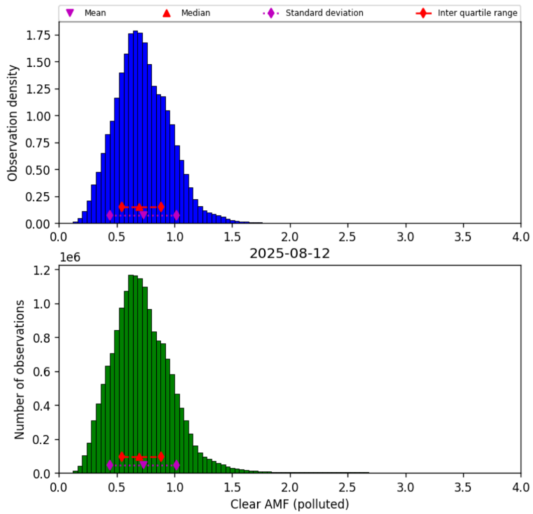
Figure 82: Histogram of “Clear AMF (polluted)” for 2025-08-12 to 2025-08-12
