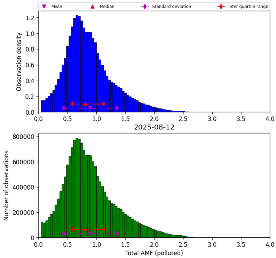
Figure 80: Histogram of “Total AMF (polluted)” for 2025-08-12 to 2025-08-12
