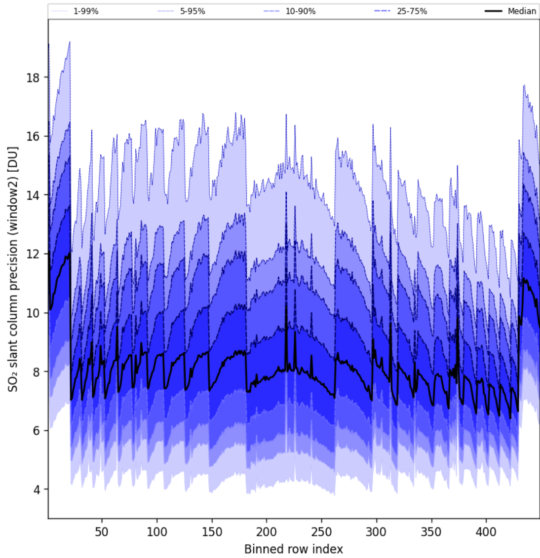
Figure 95: Along track statistics of “SO 2 slant column precision (window2)” for 2025-08-12 to 2025-08-12
