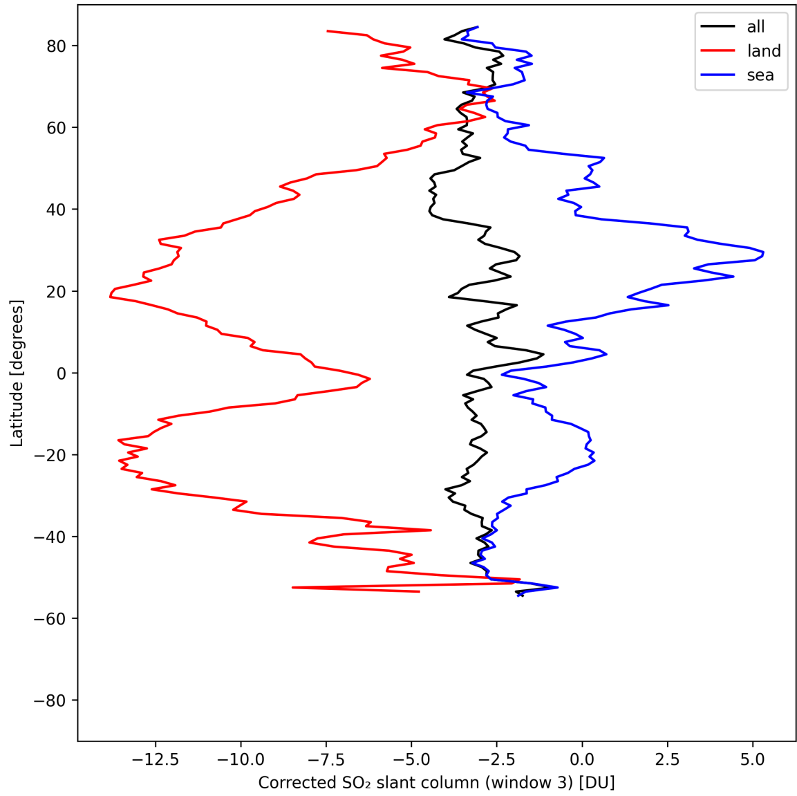
Figure 46: Zonal average of “Corrected SO 2 slant column (window 3)” for 2025-08-12 to 2025-08-12.
