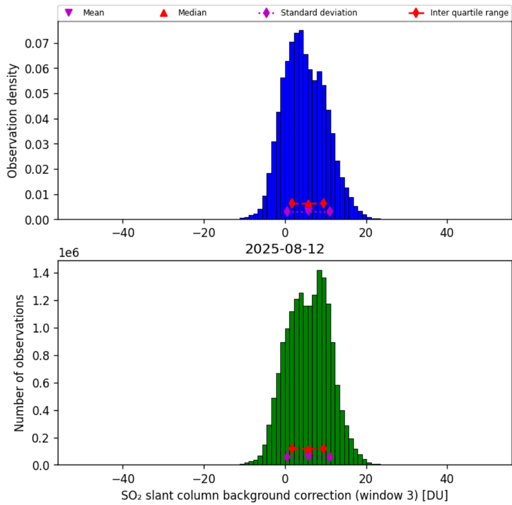
Figure 74: Histogram of “SO 2 slant column background correction (window 3)” for 2025-08-12 to 2025-08-12
