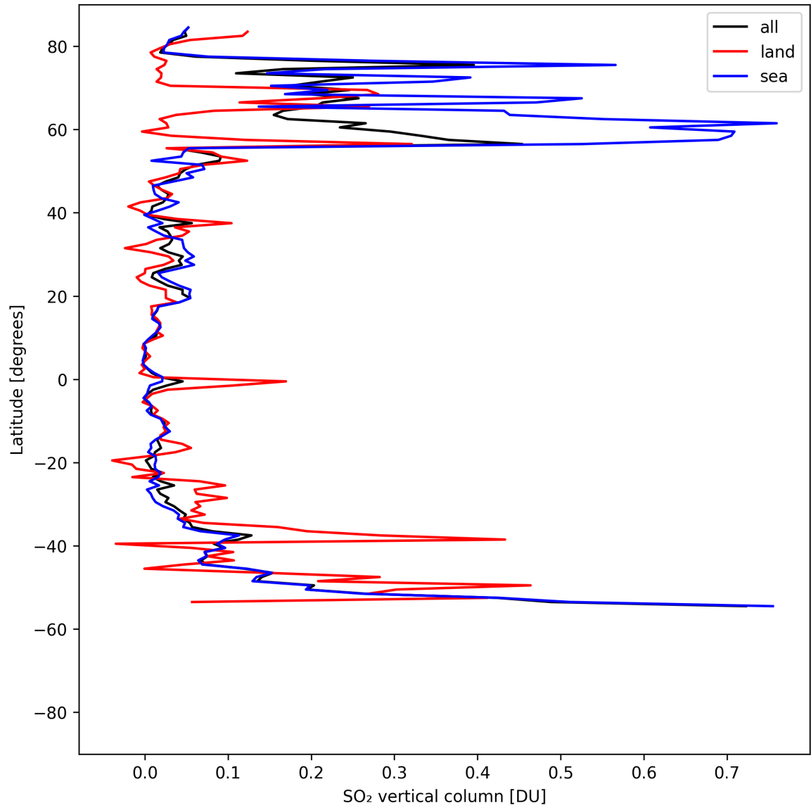
Figure 31: Zonal average of “SO 2 vertical column” for 2025-08-12 to 2025-08-12.
