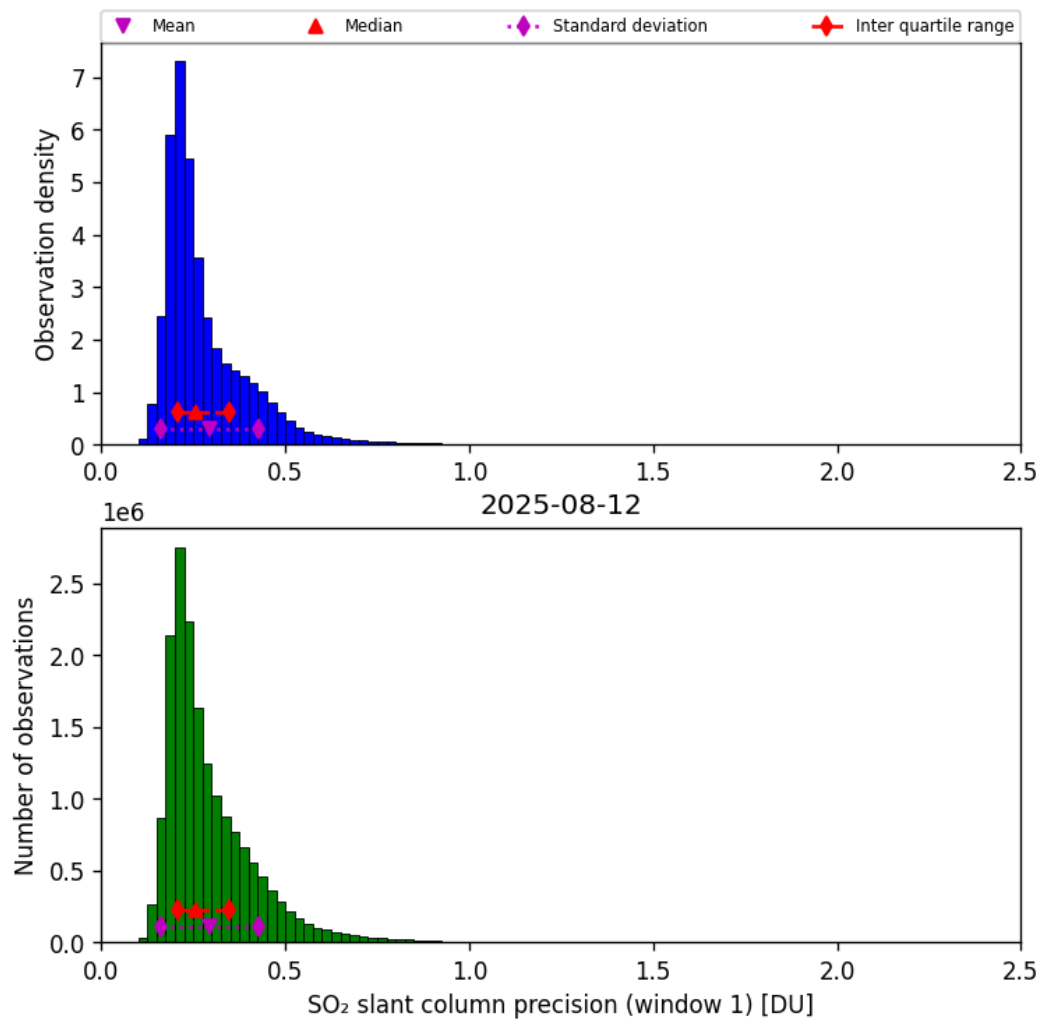
Figure 64: Histogram of “SO 2 slant column precision (window 1)” for 2025-08-12 to 2025-08-12
