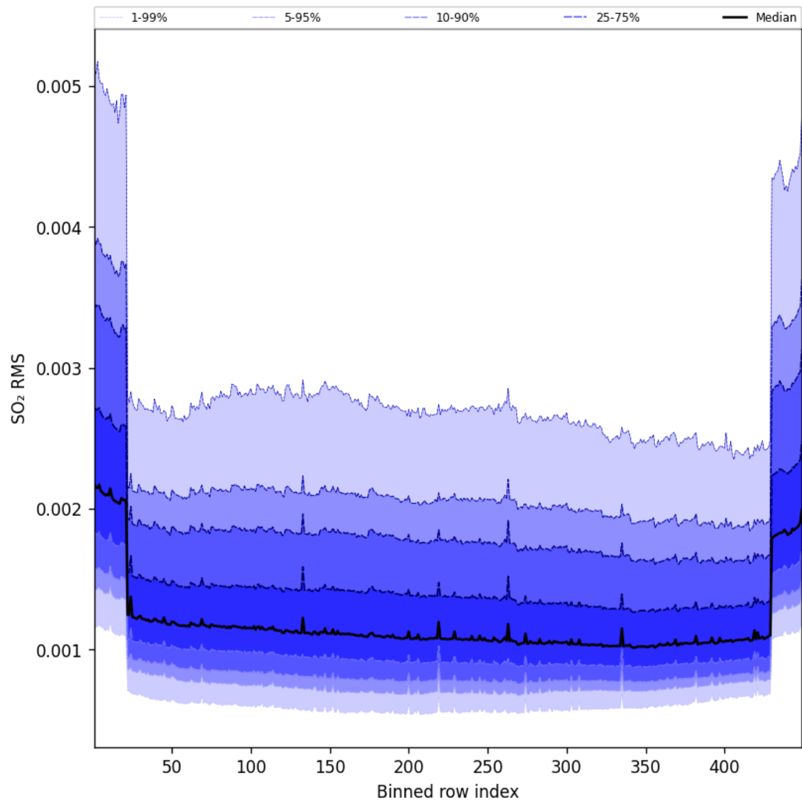
Figure 106: Along track statistics of “SO 2 RMS” for 2025-08-12 to 2025-08-12
