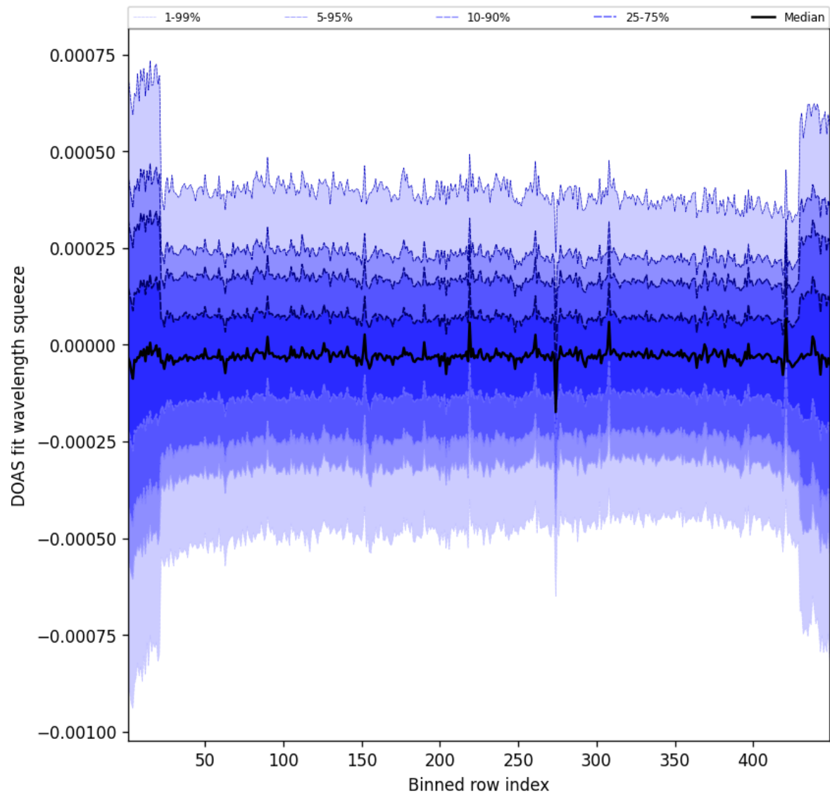
Figure 105: Along track statistics of “DOAS fit wavelength squeeze” for 2025-08-12 to 2025-08-12
