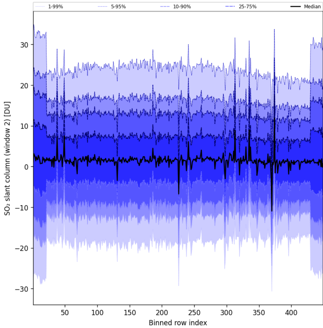
Figure 94: Along track statistics of “SO 2 slant column (window 2)” for 2025-08-12 to 2025-08-12
