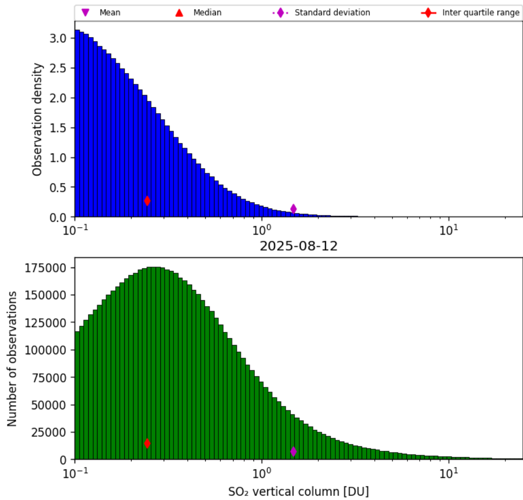
Figure 58: Histogram of “SO 2 vertical column” for 2025-08-12 to 2025-08-12
