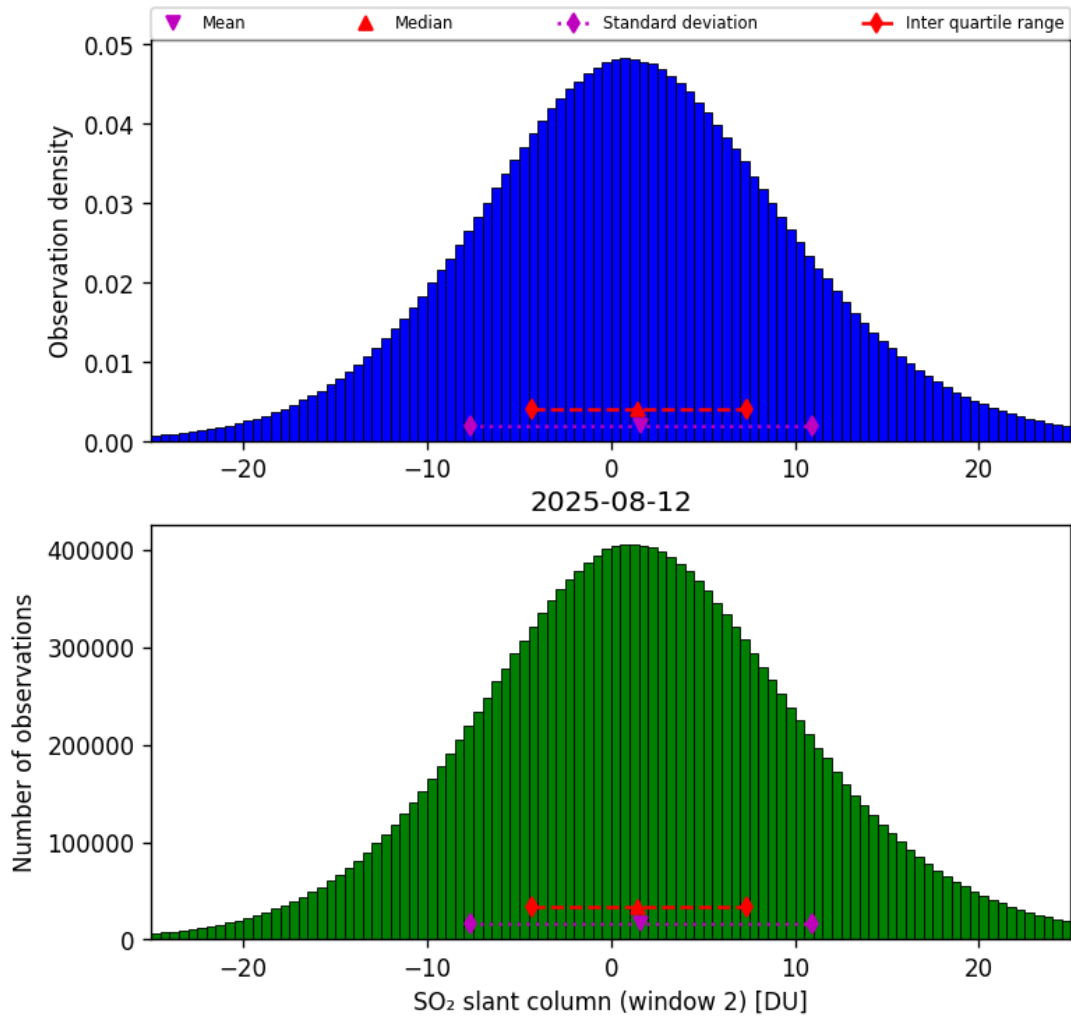
Figure 67: Histogram of “SO 2 slant column (window 2)” for 2025-08-12 to 2025-08-12
