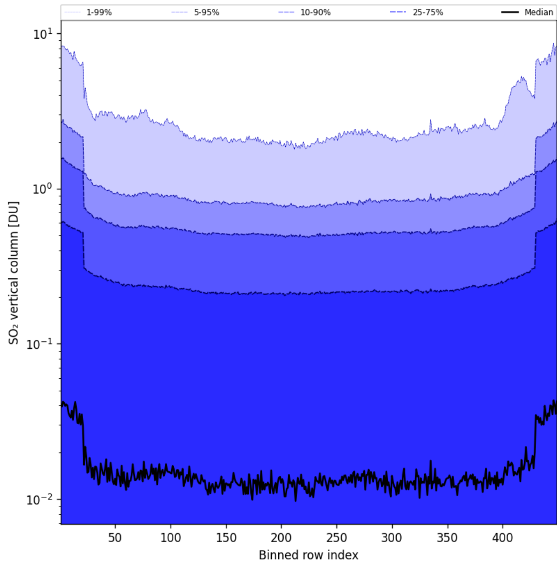
Figure 85: Along track statistics of “SO 2 vertical column” for 2025-08-12 to 2025-08-12
