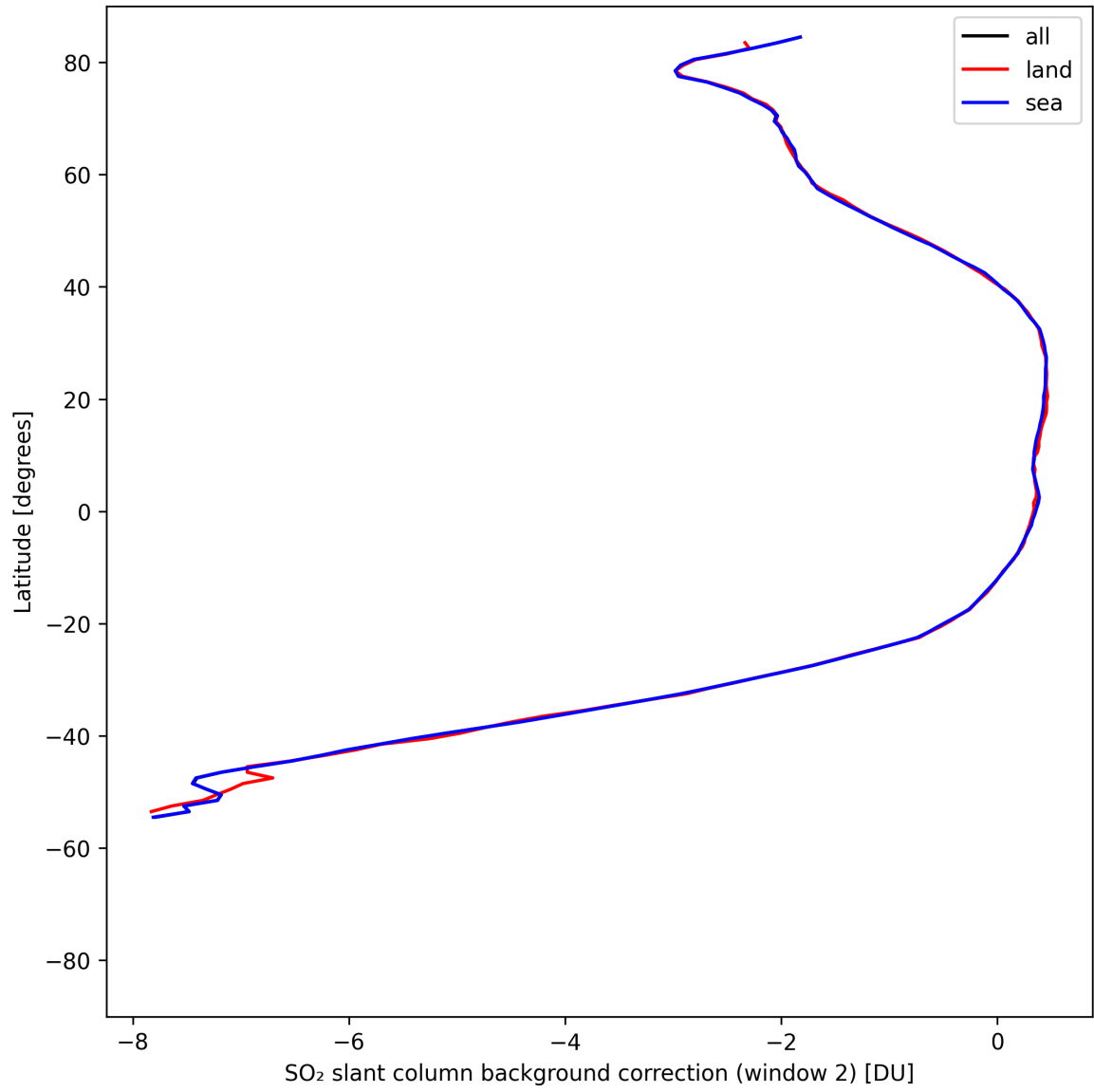
Figure 43: Zonal average of “SO 2 slant column background correction (window 2)” for 2025-08-12 to 2025-08-12.
