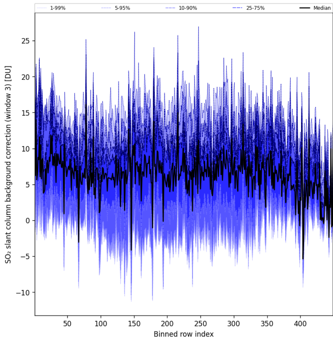
Figure 101: Along track statistics of "SO 2 slant column background correction (window 3)" for 2025-08-12 to 2025-08-12
