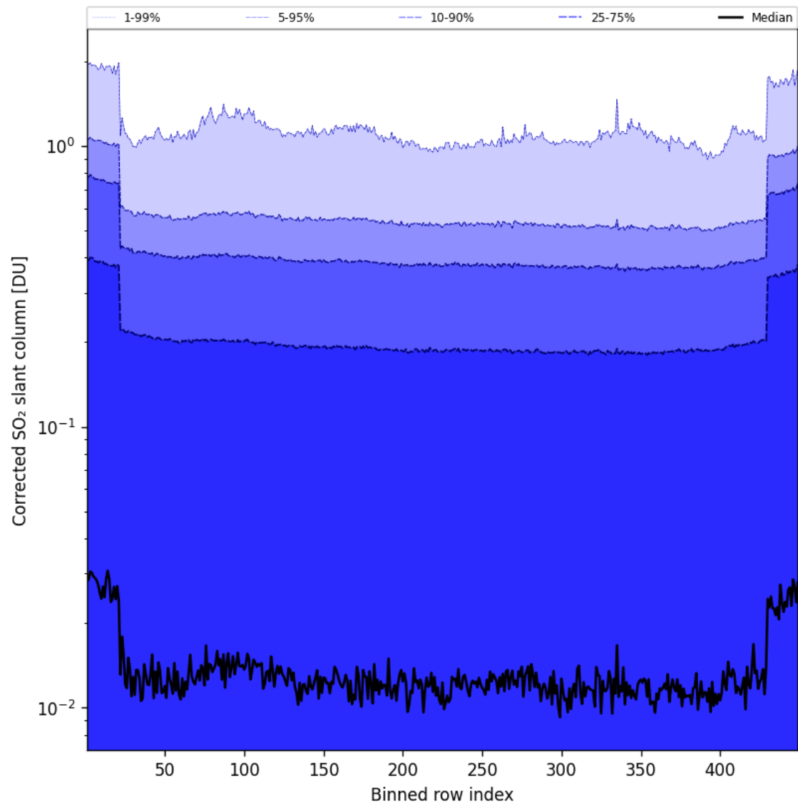
Figure 87: Along track statistics of “Corrected SO 2 slant column” for 2025-08-12 to 2025-08-12
