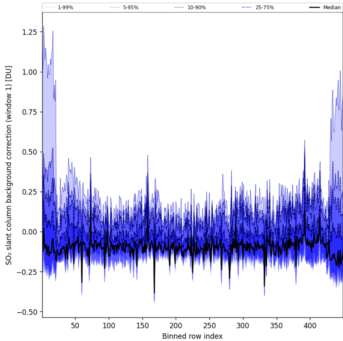
Figure 93: Along track statistics of “SO 2 slant column background correction (window 1)” for 2025-08-12 to 2025-08-12
