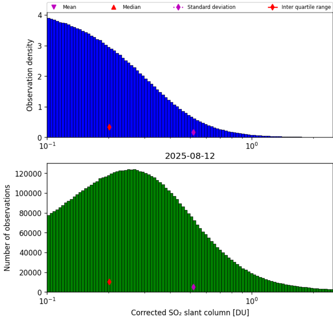
Figure 60: Histogram of “Corrected SO 2 slant column” for 2025-08-12 to 2025-08-12
