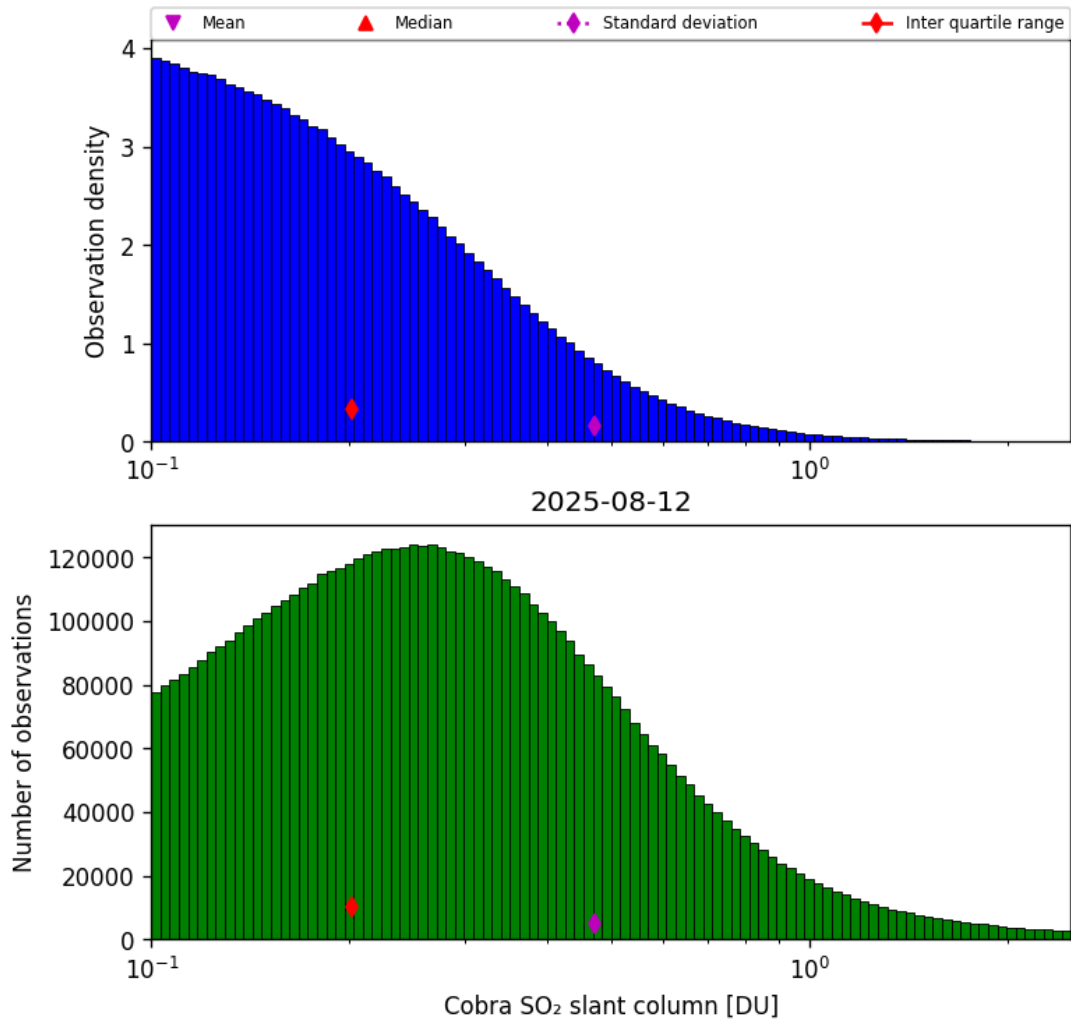
Figure 61: Histogram of “Cobra SO 2 slant column” for 2025-08-12 to 2025-08-12
