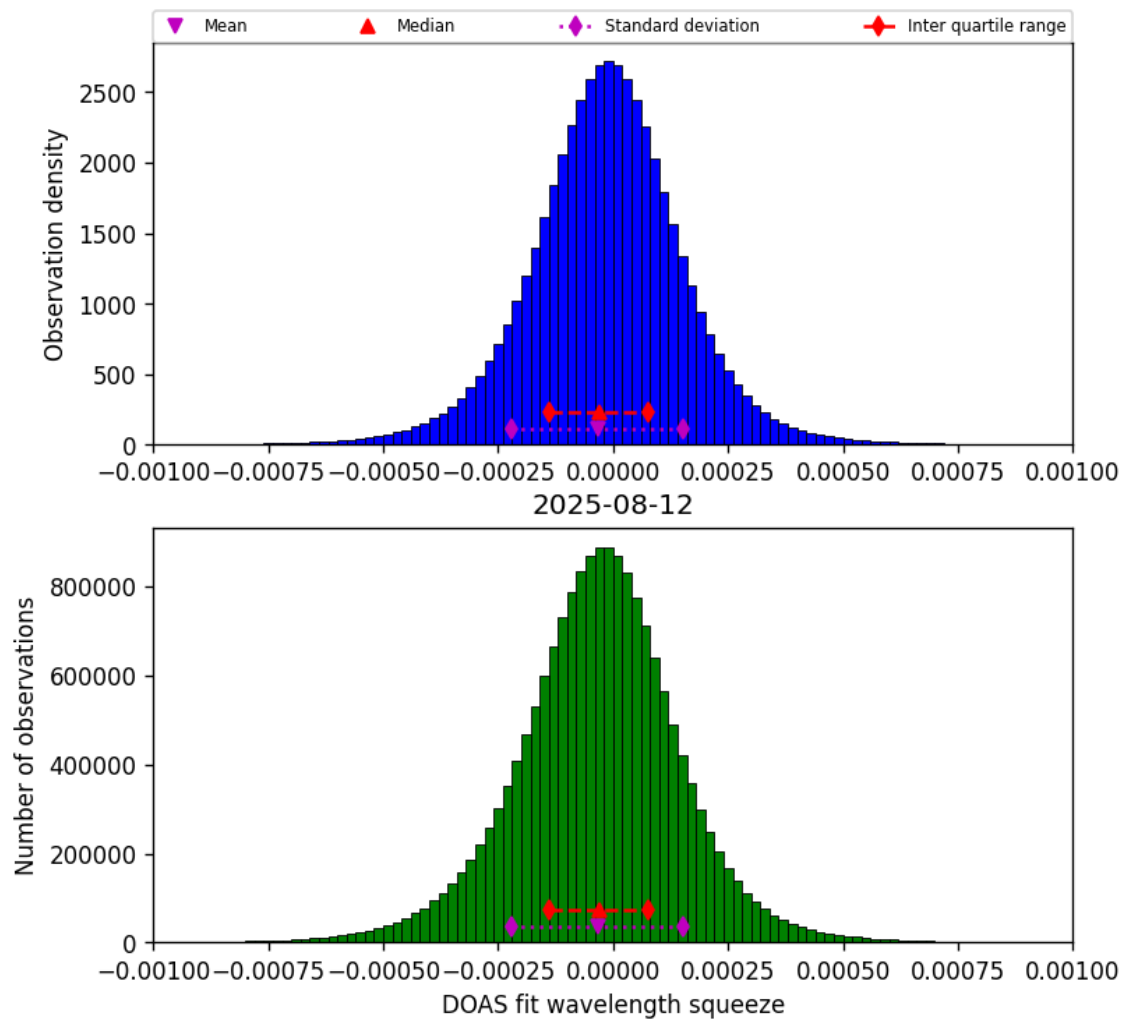
Figure 78: Histogram of “DOAS fit wavelength squeeze” for 2025-08-12 to 2025-08-12
