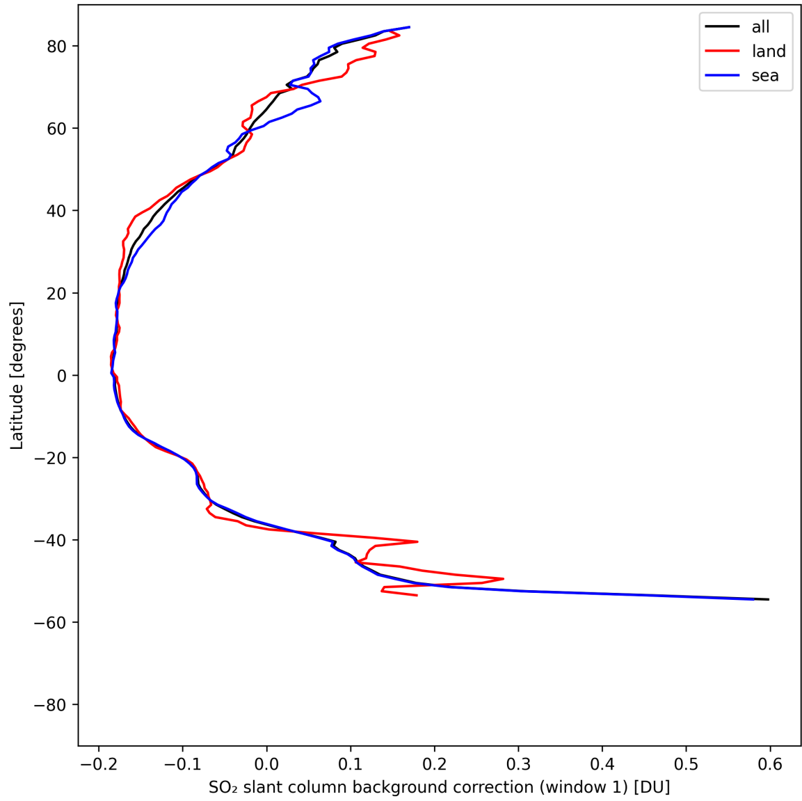
Figure 39: Zonal average of "SO 2 slant column background correction (window 1)" for 2025-08-12 to 2025-08-12.
