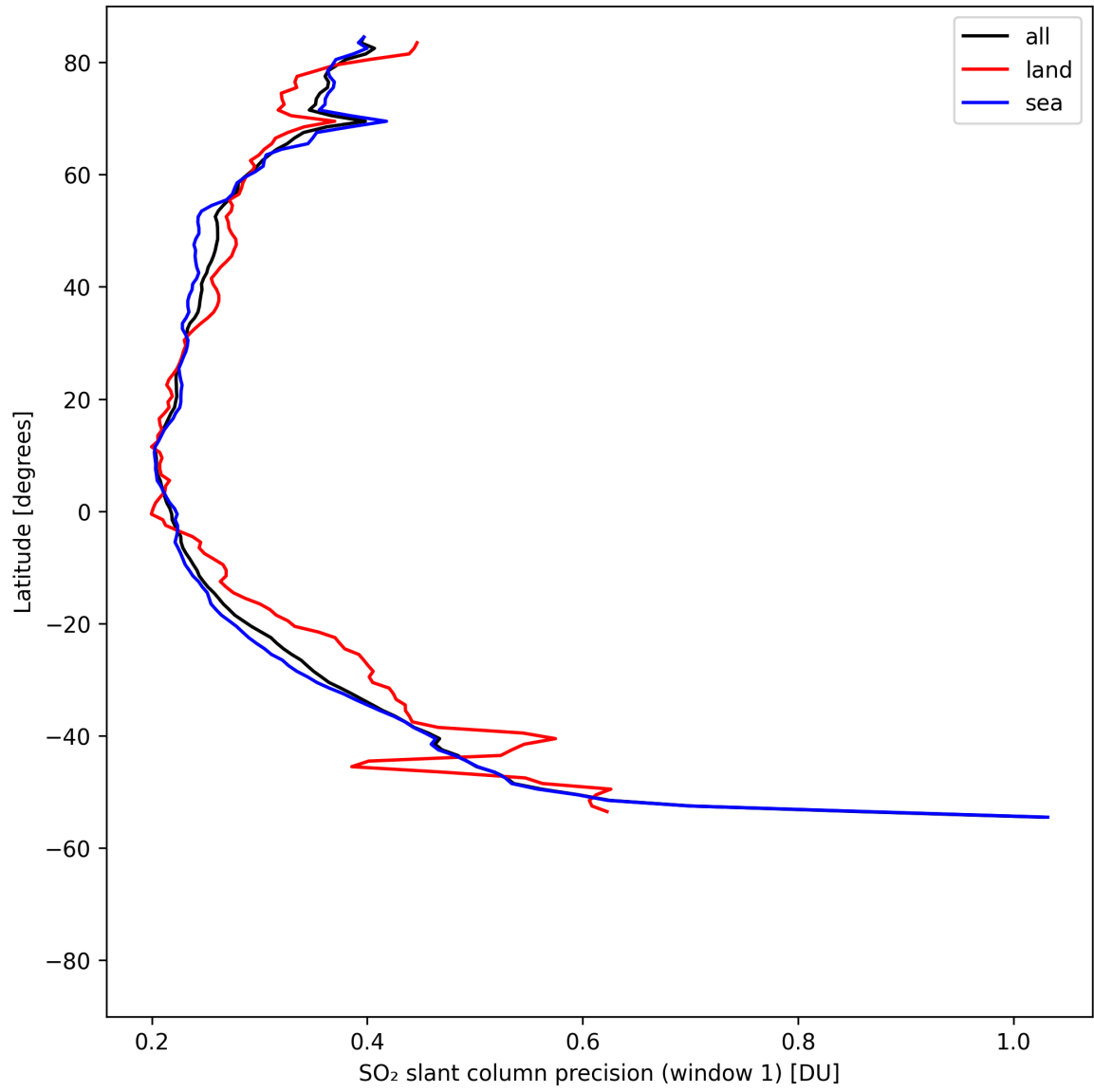
Figure 37: Zonal average of “SO 2 slant column precision (window 1)” for 2025-08-12 to 2025-08-12.
