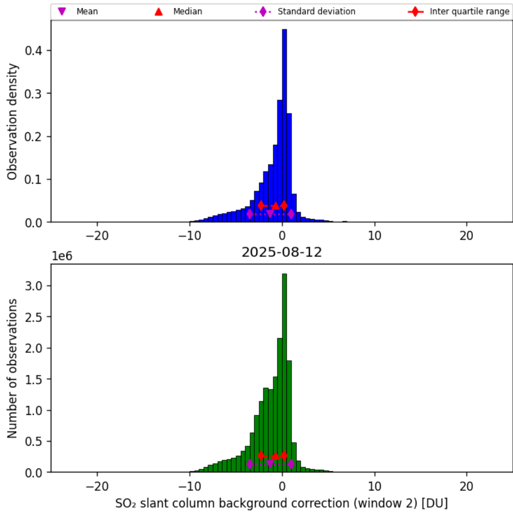
Figure 70: Histogram of “SO 2 slant column background correction (window 2)” for 2025-08-12 to 2025-08-12
