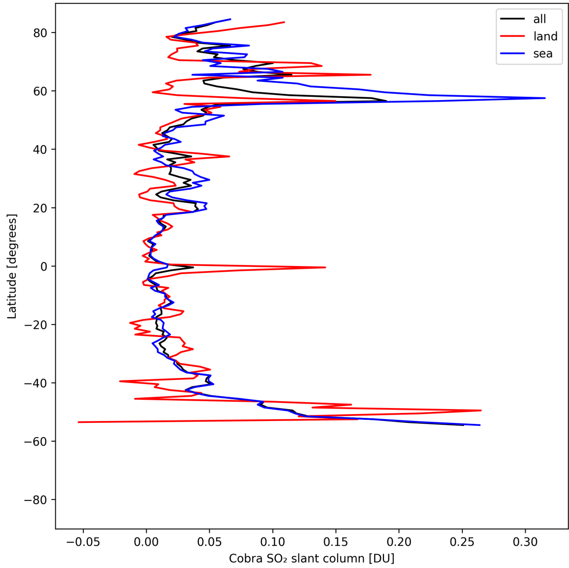
Figure 34: Zonal average of “Cobra SO 2 slant column” for 2025-08-12 to 2025-08-12.
