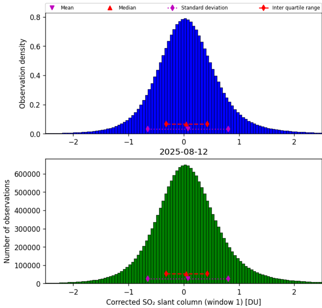
Figure 65: Histogram of “Corrected SO 2 slant column (window 1)” for 2025-08-12 to 2025-08-12
