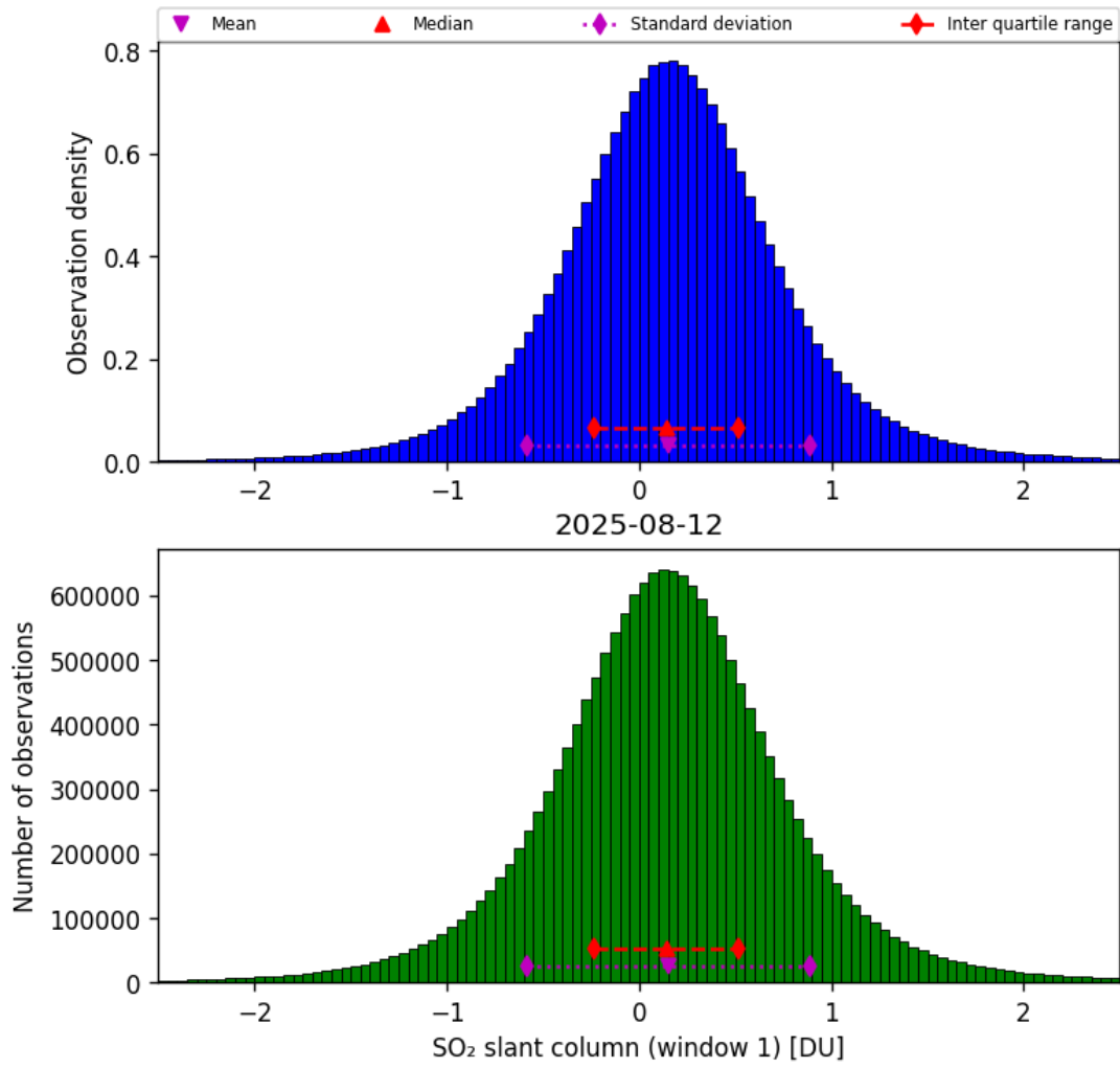
Figure 63: Histogram of “SO 2 slant column (window 1)” for 2025-08-12 to 2025-08-12
