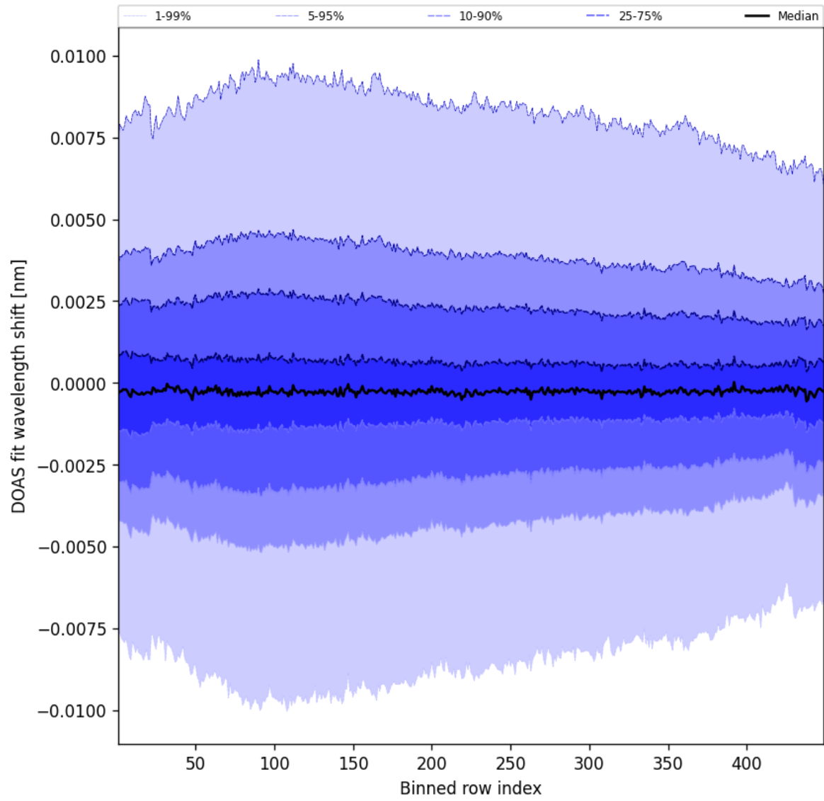
Figure 104: Along track statistics of “DOAS fit wavelength shift” for 2025-08-12 to 2025-08-12
