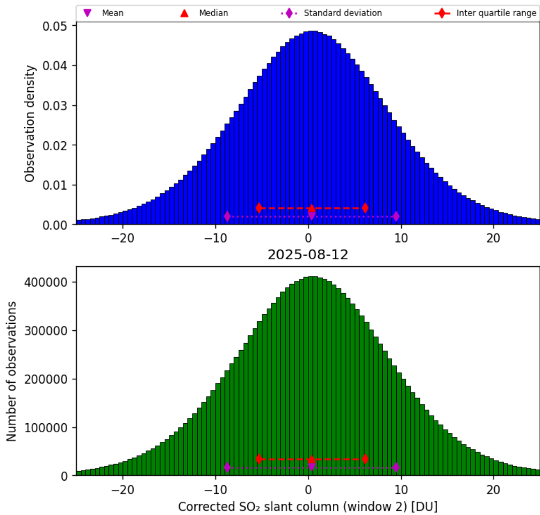
Figure 69: Histogram of “Corrected SO 2 slant column (window 2)” for 2025-08-12 to 2025-08-12
