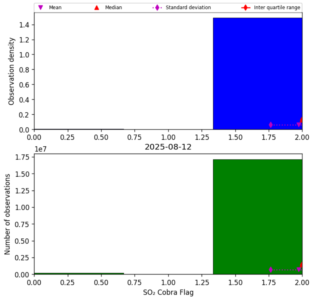
Figure 75: Histogram of “SO 2 Cobra Flag” for 2025-08-12 to 2025-08-12
