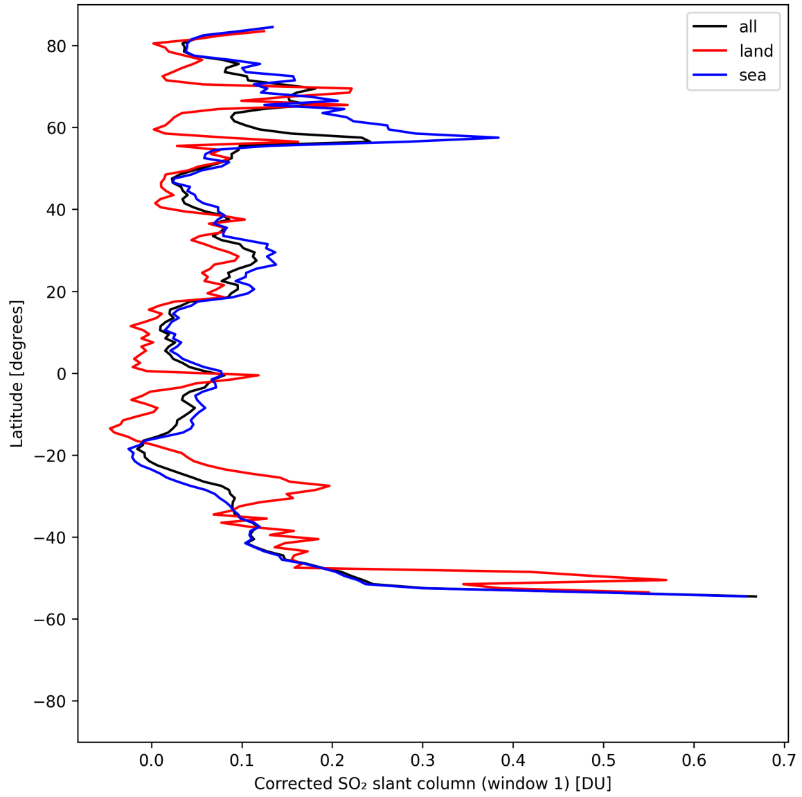
Figure 38: Zonal average of “Corrected SO 2 slant column (window 1)” for 2025-08-12 to 2025-08-12.
