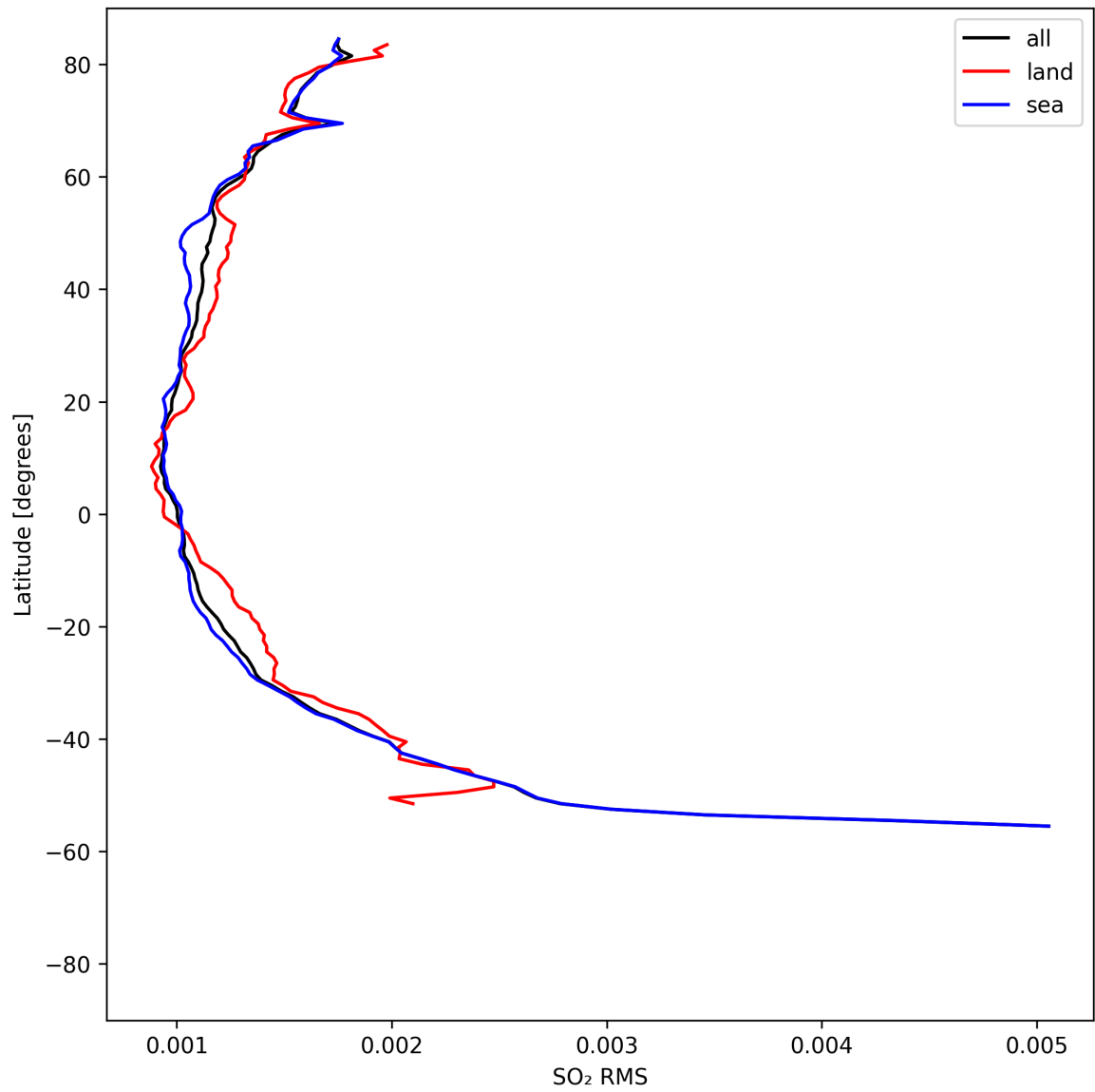
Figure 52: Zonal average of “SO 2 RMS” for 2025-08-14 to 2025-08-15.
