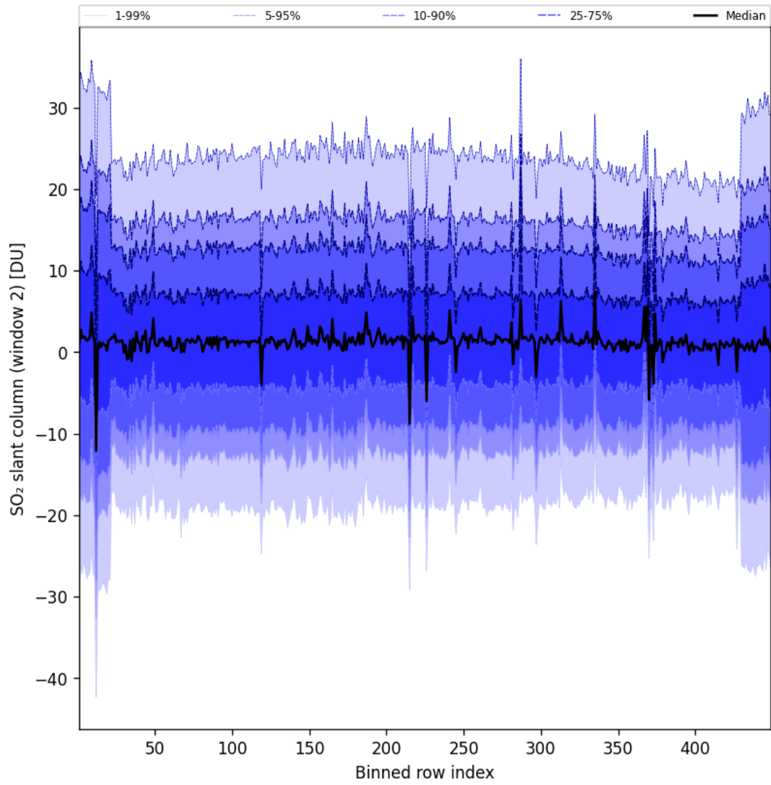
Figure 94: Along track statistics of “SO 2 slant column (window 2)” for 2025-08-14 to 2025-08-15
