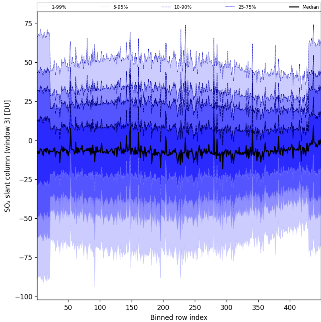
Figure 98: Along track statistics of “SO 2 slant column (window 3)” for 2025-08-14 to 2025-08-15
