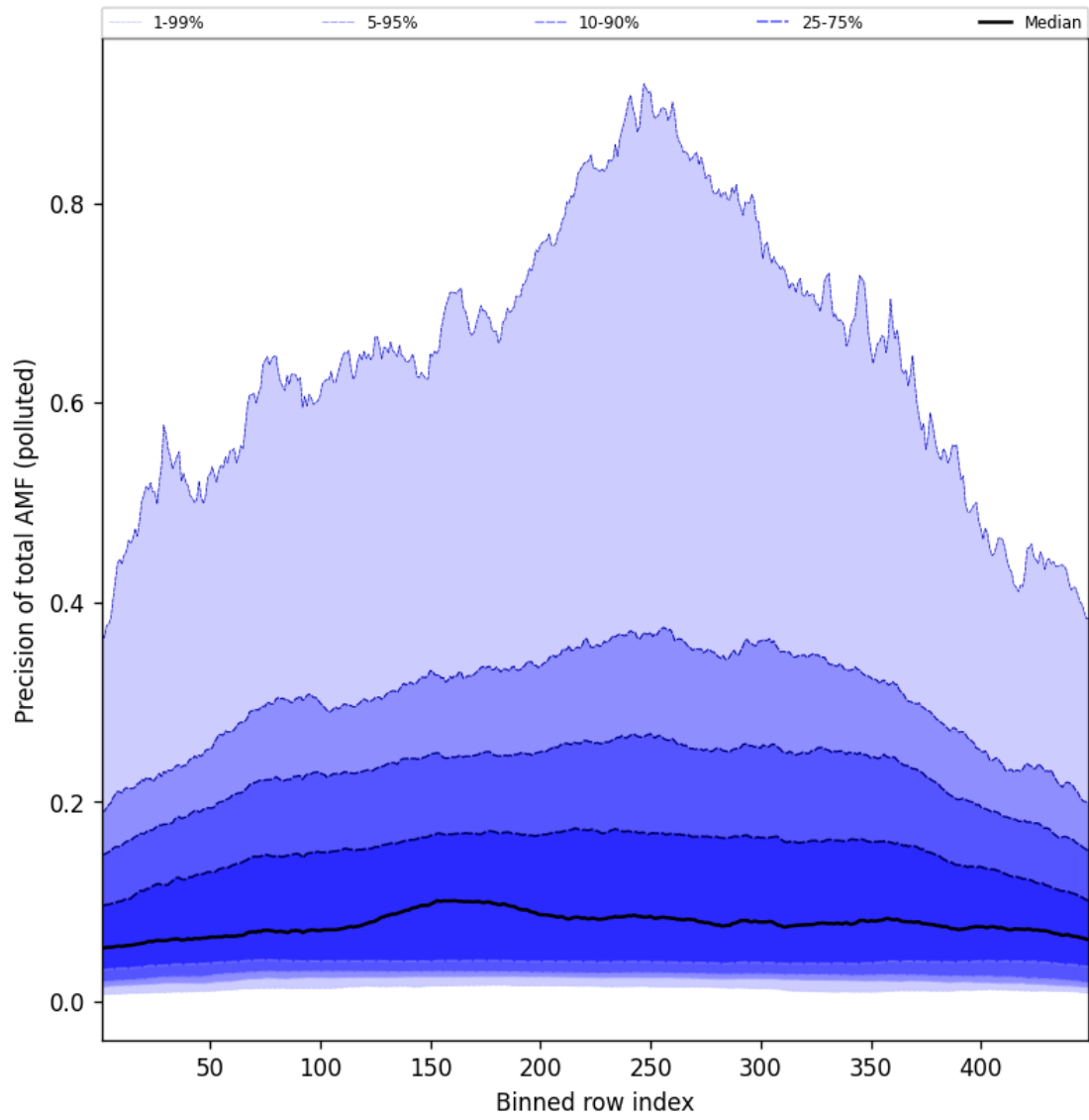
Figure 108: Along track statistics of “Precision of total AMF (polluted)” for 2025-08-14 to 2025-08-15
