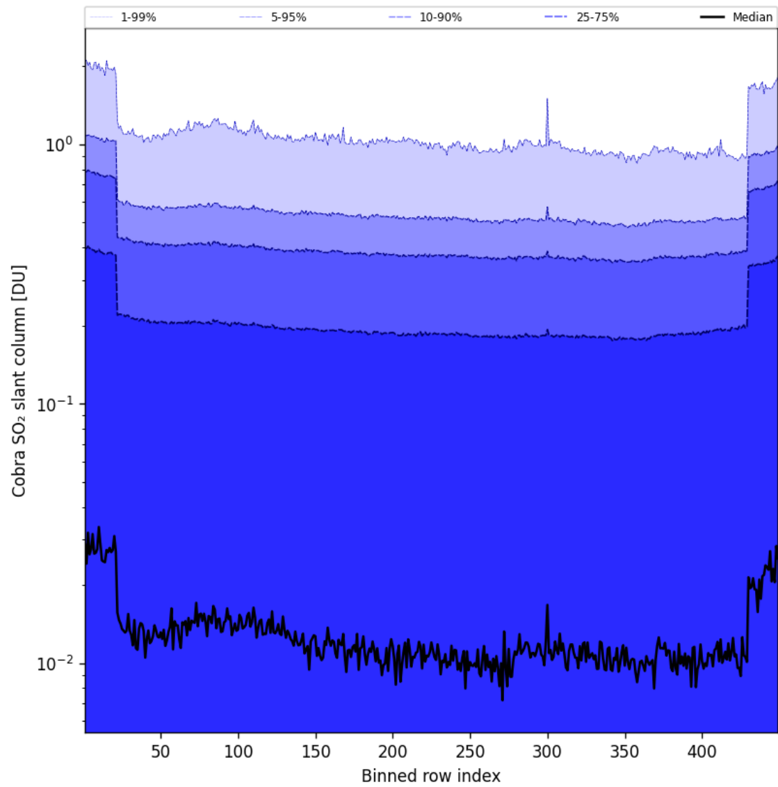
Figure 88: Along track statistics of “Cobra SO 2 slant column” for 2025-08-14 to 2025-08-15
