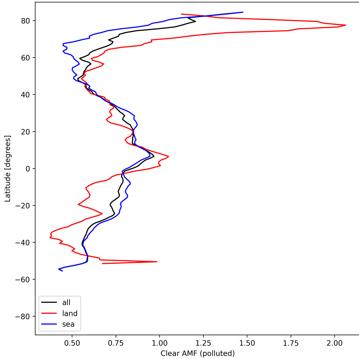
Figure 55: Zonal average of “Clear AMF (polluted)” for 2025-08-14 to 2025-08-15.
