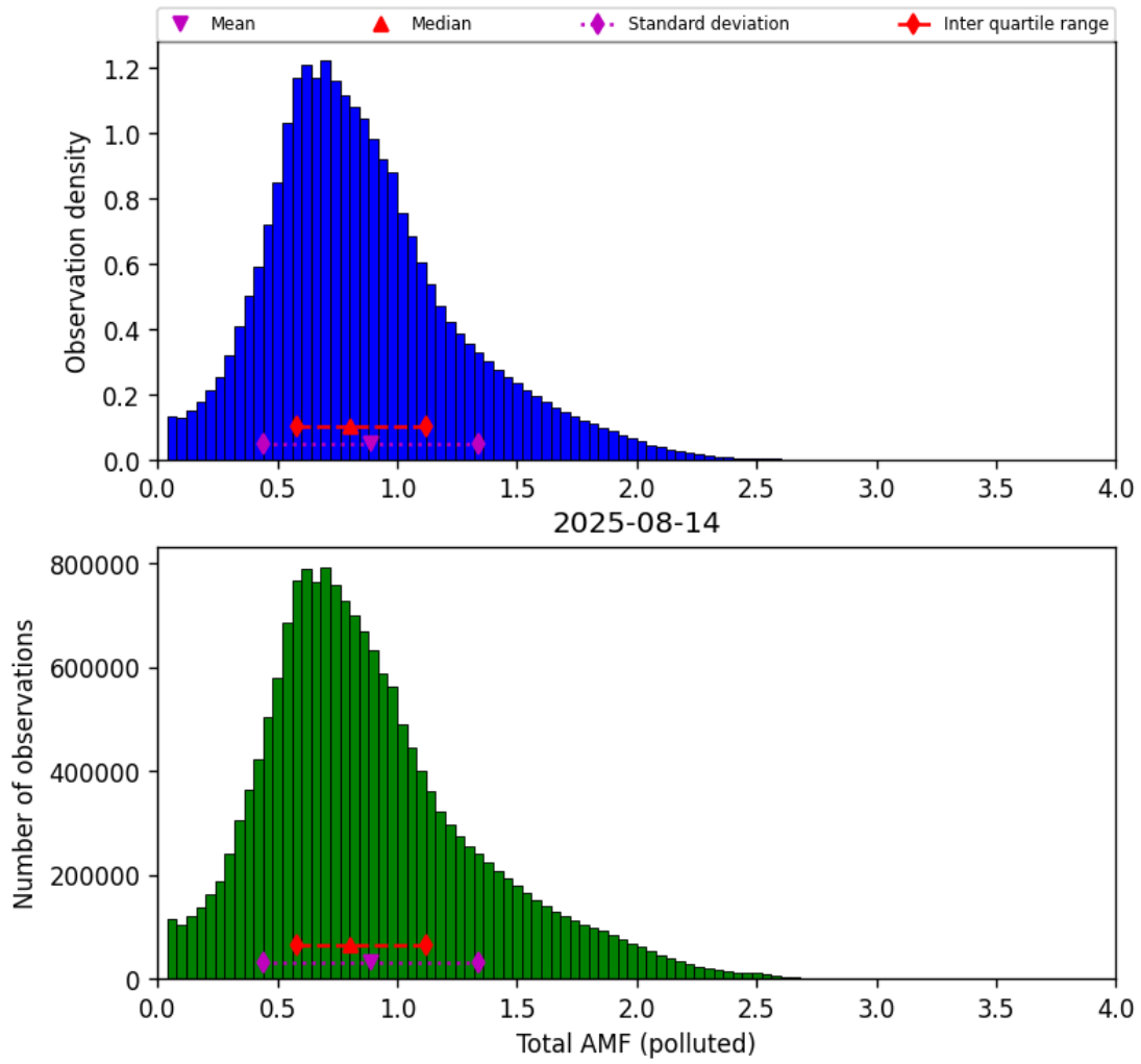
Figure 80: Histogram of “Total AMF (polluted)” for 2025-08-14 to 2025-08-15
