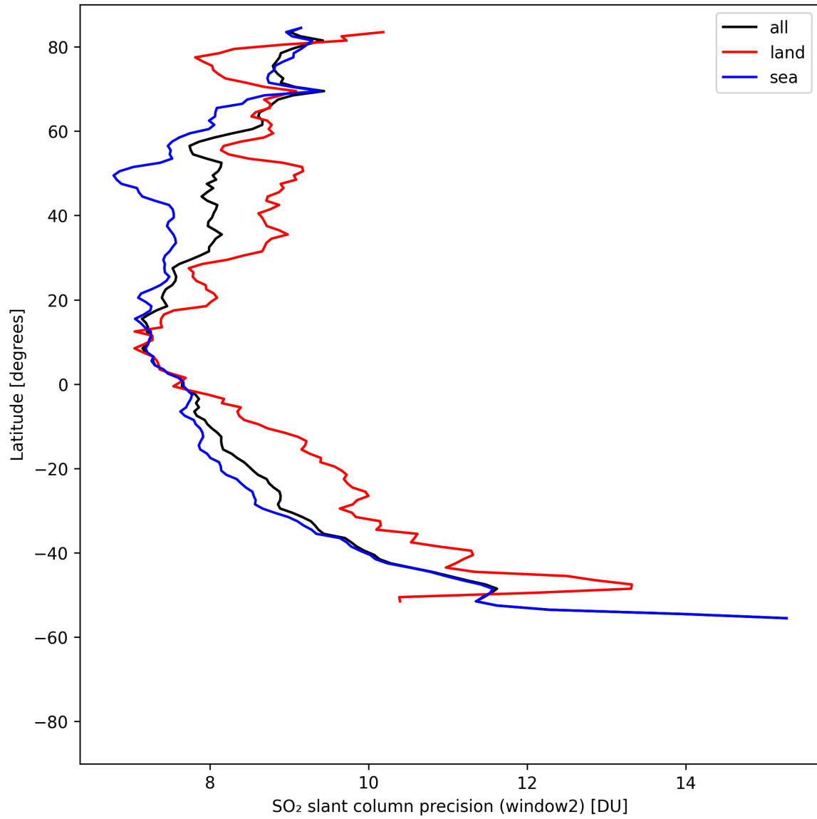
Figure 41: Zonal average of “SO 2 slant column precision (window2)” for 2025-08-14 to 2025-08-15.
