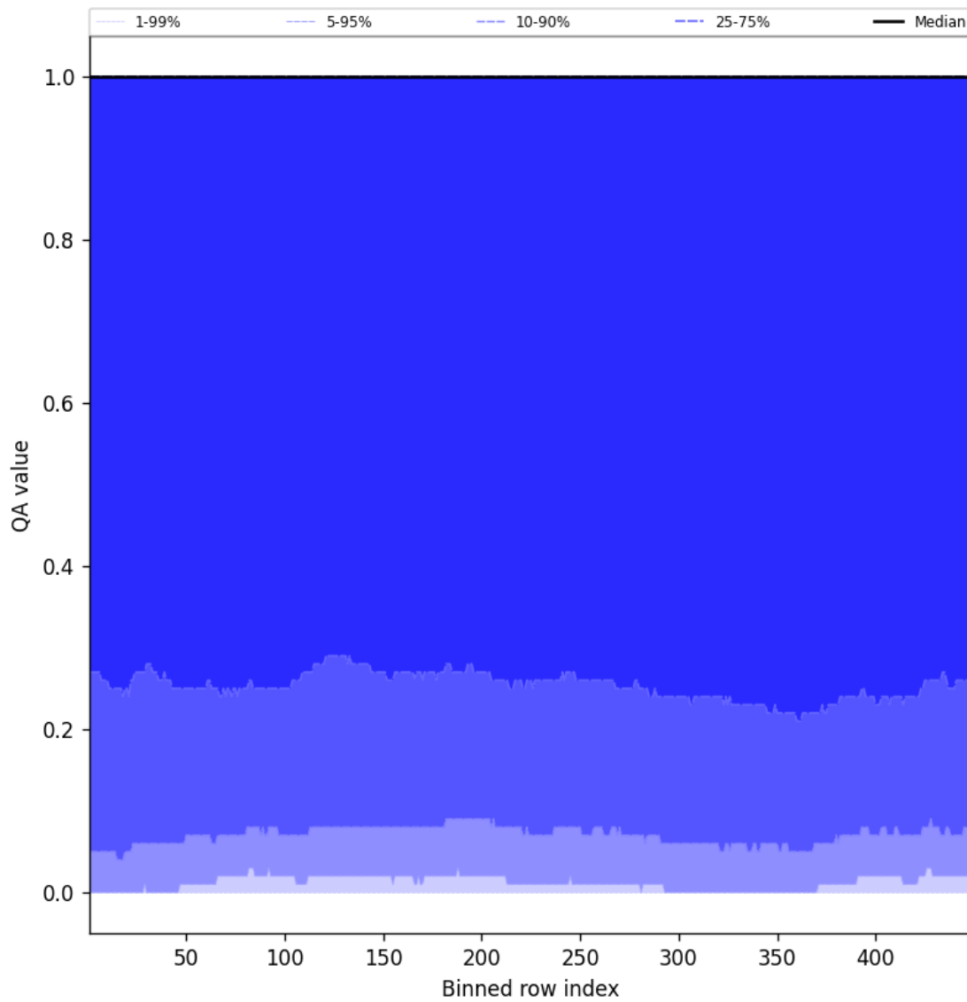
Figure 84: Along track statistics of “QA value” for 2025-08-14 to 2025-08-15
