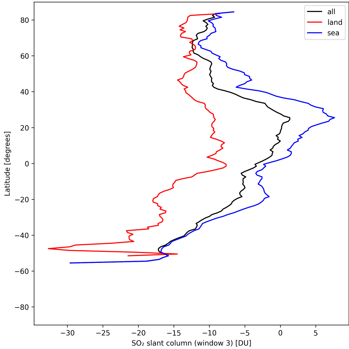
Figure 44: Zonal average of “SO 2 slant column (window 3)” for 2025-08-14 to 2025-08-15.
