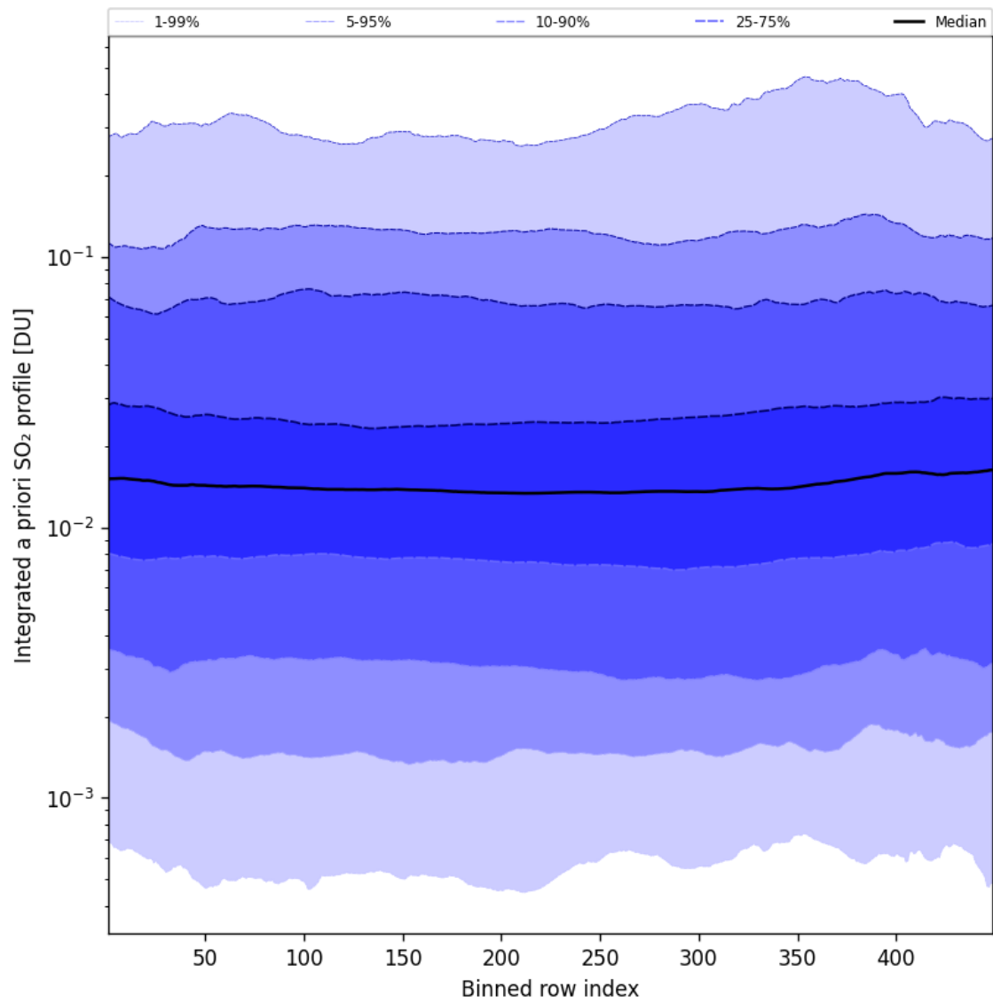
Figure 103: Along track statistics of “Integrated a priori SO 2 profile” for 2025-08-14 to 2025-08-15
