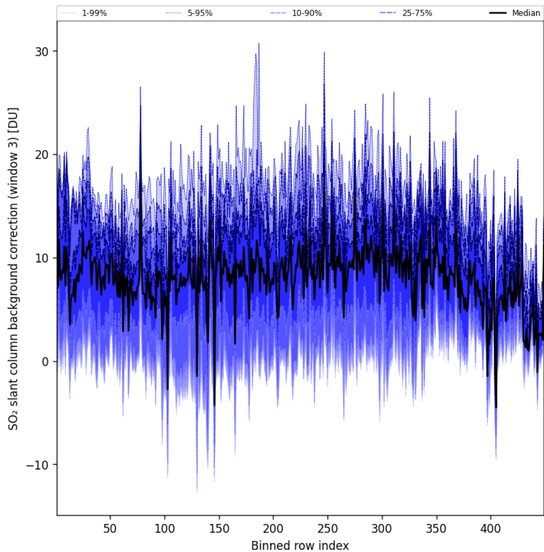
Figure 101: Along track statistics of “SO 2 slant column background correction (window 3)” for 2025-08-14 to 2025-08-15
