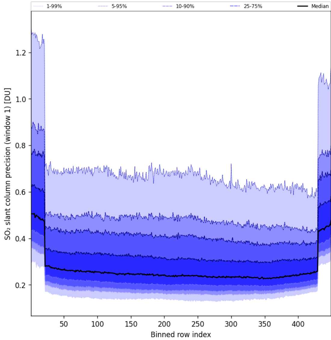
Figure 91: Along track statistics of “SO 2 slant column precision (window 1)” for 2025-08-14 to 2025-08-15
