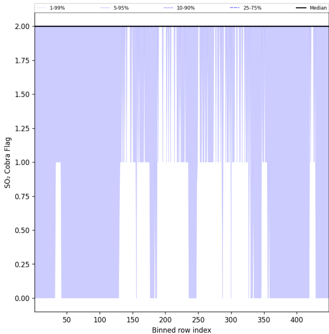
Figure 102: Along track statistics of “SO 2 Cobra Flag” for 2025-08-14 to 2025-08-15
