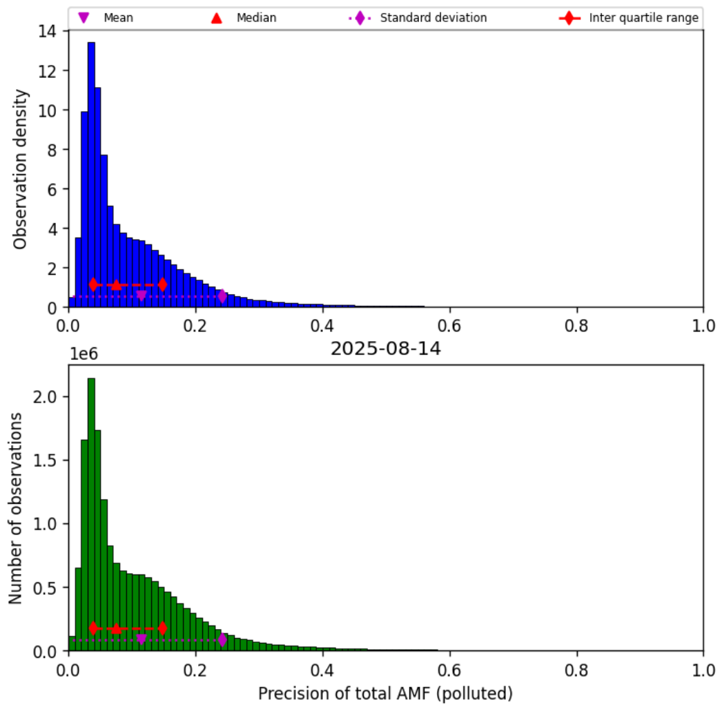
Figure 81: Histogram of “Precision of total AMF (polluted)” for 2025-08-14 to 2025-08-15
