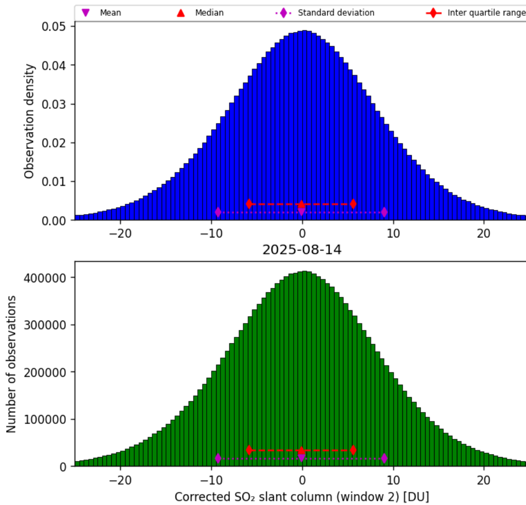
Figure 69: Histogram of “Corrected SO 2 slant column (window 2)” for 2025-08-14 to 2025-08-15
