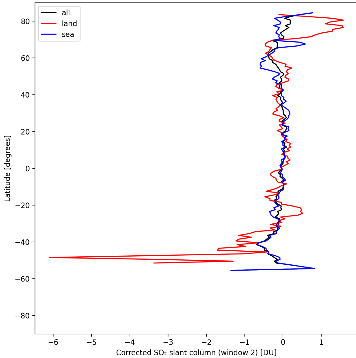
Figure 42: Zonal average of “Corrected SO 2 slant column (window 2)” for 2025-08-14 to 2025-08-15.
