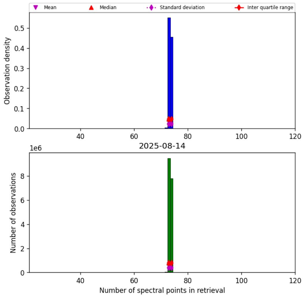
Figure 83: Histogram of “Number of spectral points in retrieval” for 2025-08-14 to 2025-08-15
