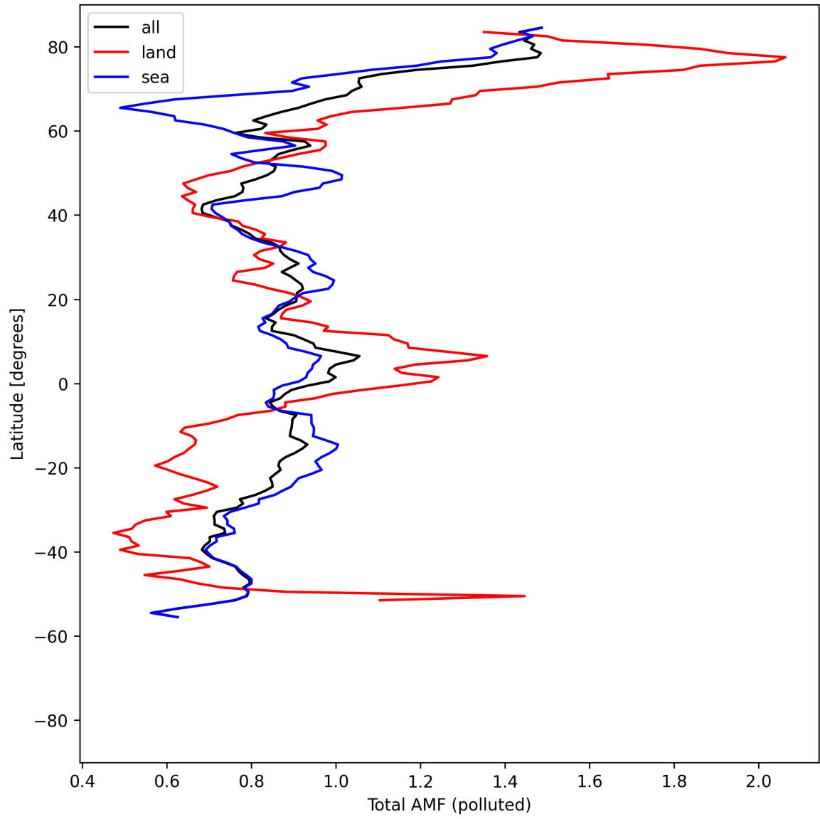
Figure 53: Zonal average of “Total AMF (polluted)” for 2025-08-14 to 2025-08-15.
