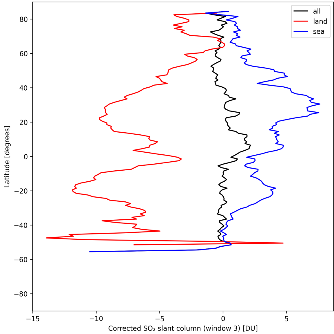
Figure 46: Zonal average of “Corrected SO 2 slant column (window 3)” for 2025-08-14 to 2025-08-15.
