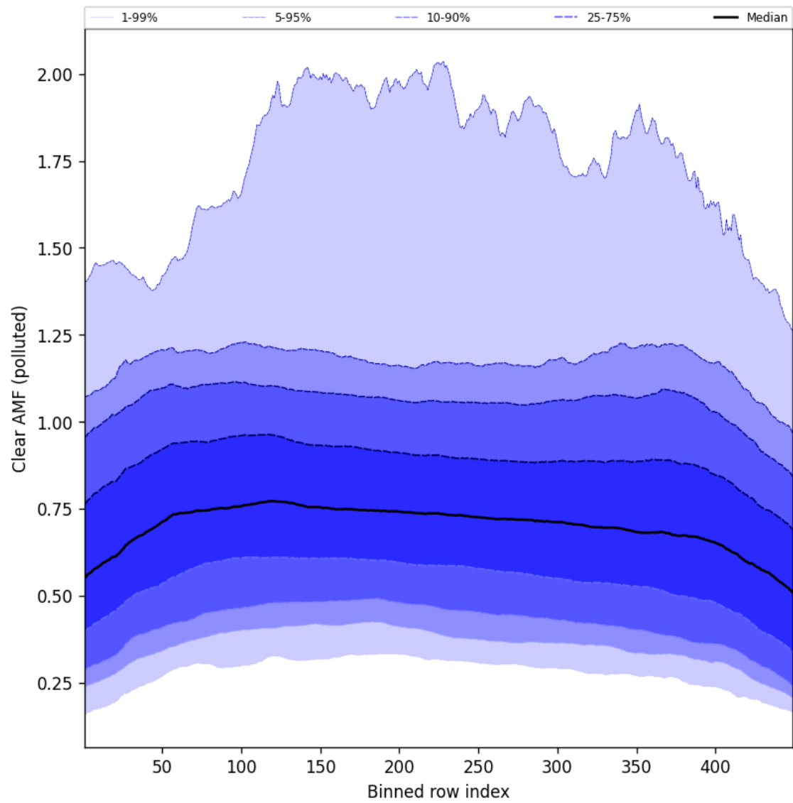
Figure 109: Along track statistics of "Clear AMF (polluted)" for 2025-08-14 to 2025-08-15
