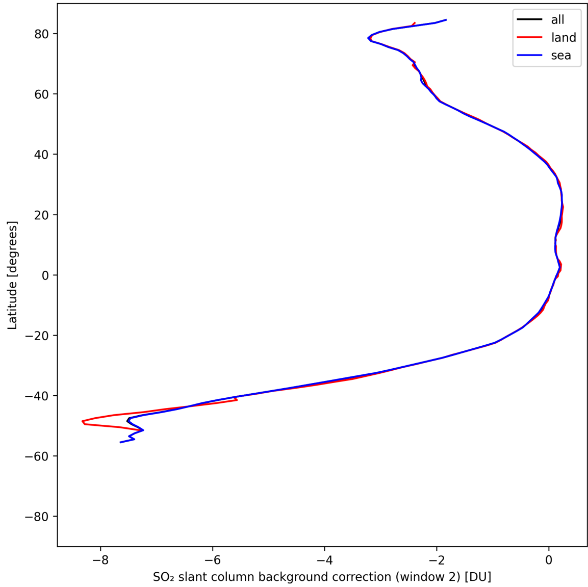
Figure 43: Zonal average of “SO 2 slant column background correction (window 2)” for 2025-08-14 to 2025-08-15.
