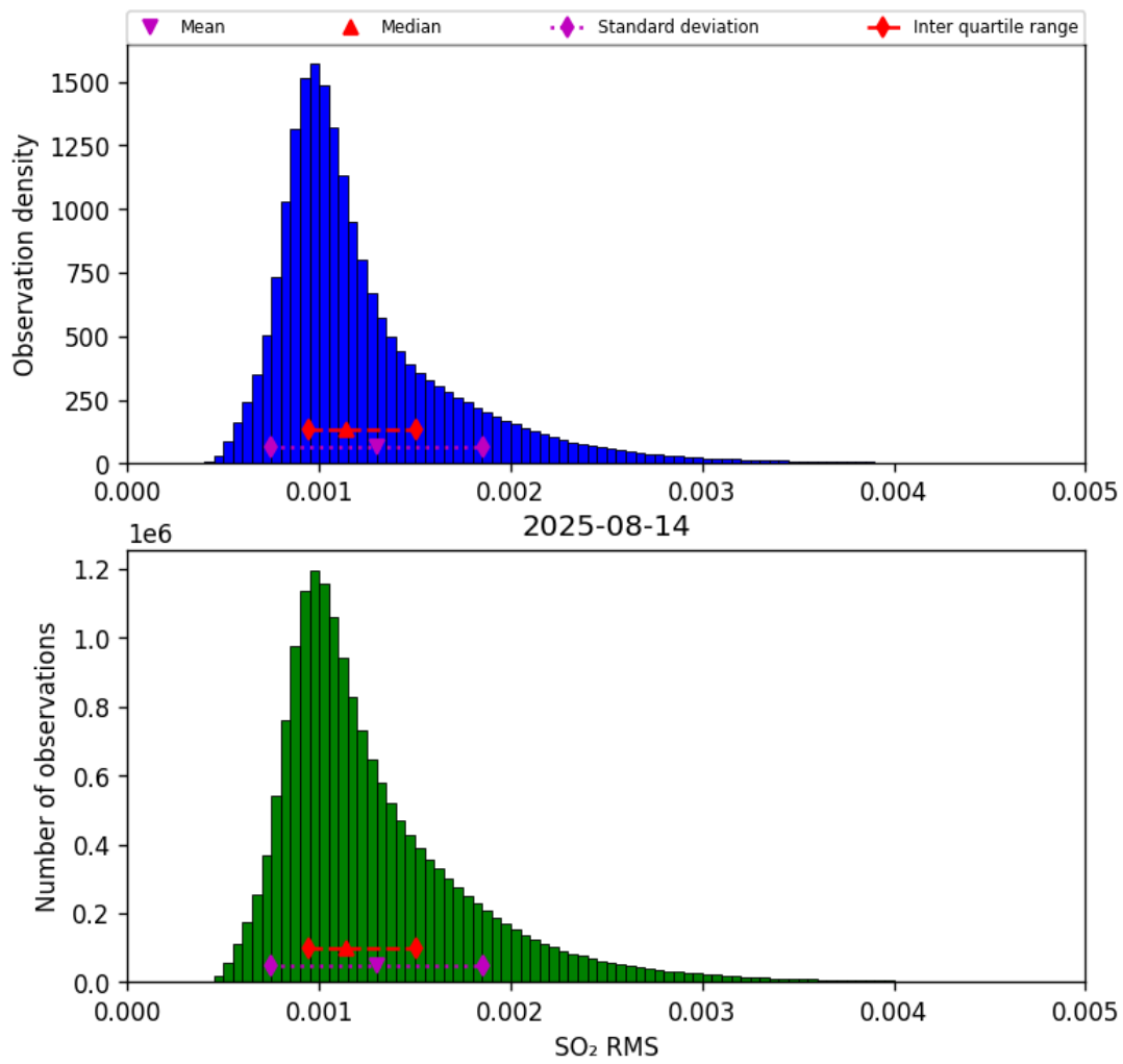
Figure 79: Histogram of "SO 2 RMS" for 2025-08-14 to 2025-08-15
