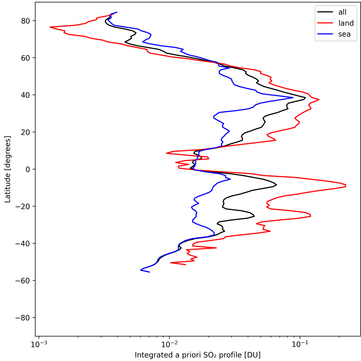
Figure 49: Zonal average of “Integrated a priori SO 2 profile” for 2025-08-14 to 2025-08-15.
