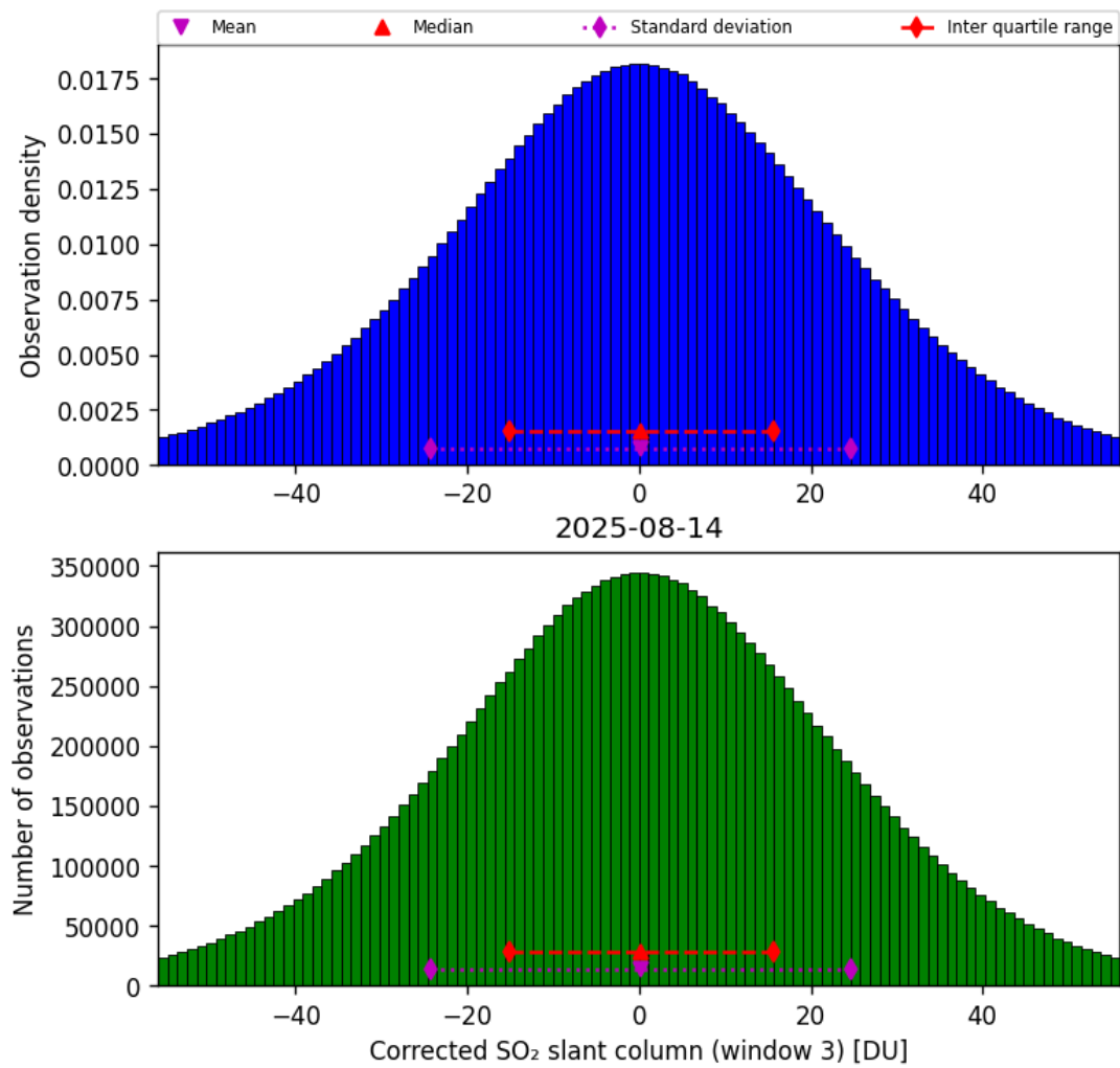
Figure 73: Histogram of “Corrected SO 2 slant column (window 3)” for 2025-08-14 to 2025-08-15
