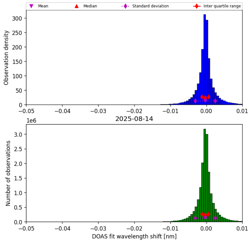
Figure 77: Histogram of “DOAS fit wavelength shift” for 2025-08-14 to 2025-08-15
