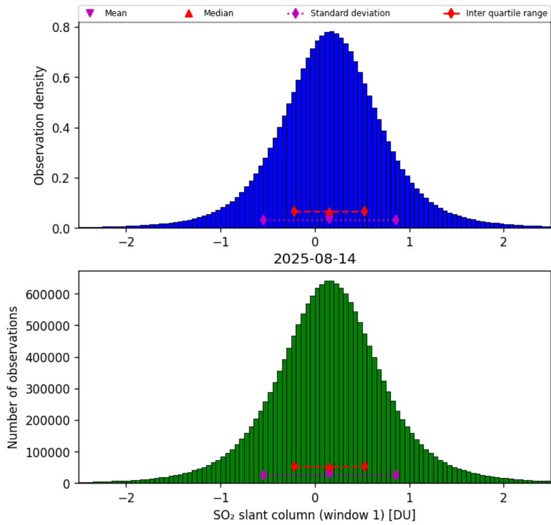
Figure 63: Histogram of “SO 2 slant column (window 1)” for 2025-08-14 to 2025-08-15
