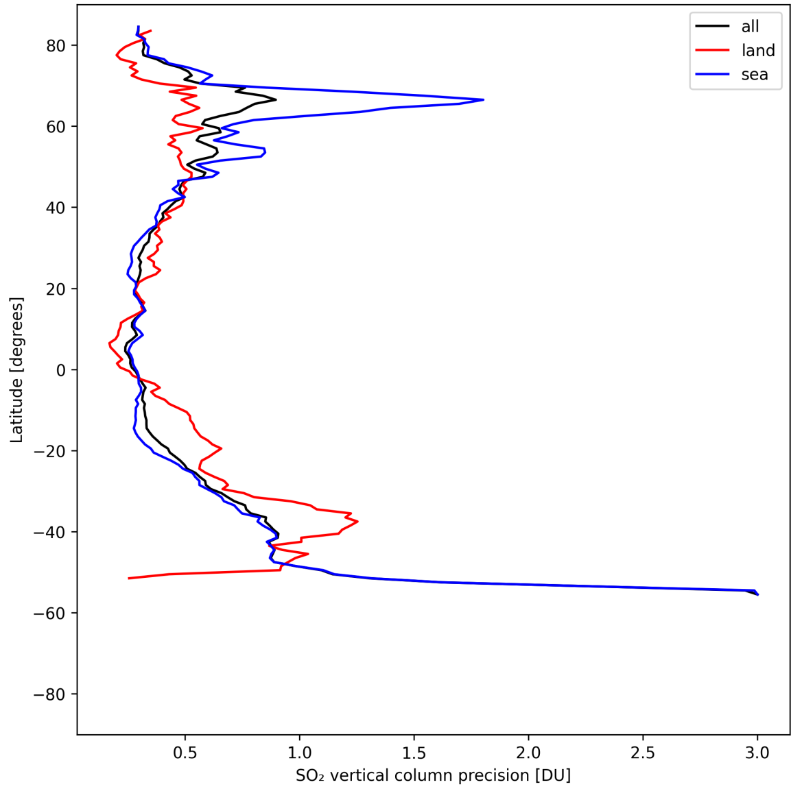
Figure 32: Zonal average of “SO 2 vertical column precision” for 2025-08-14 to 2025-08-15.
