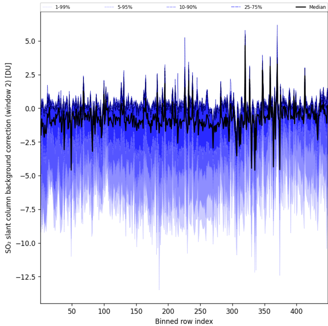
Figure 97: Along track statistics of “SO 2 slant column background correction (window 2)” for 2025-08-14 to 2025-08-15
