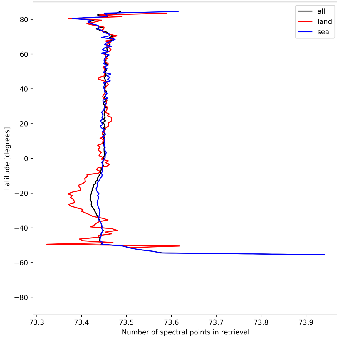
Figure 56: Zonal average of “Number of spectral points in retrieval” for 2025-08-14 to 2025-08-15.
