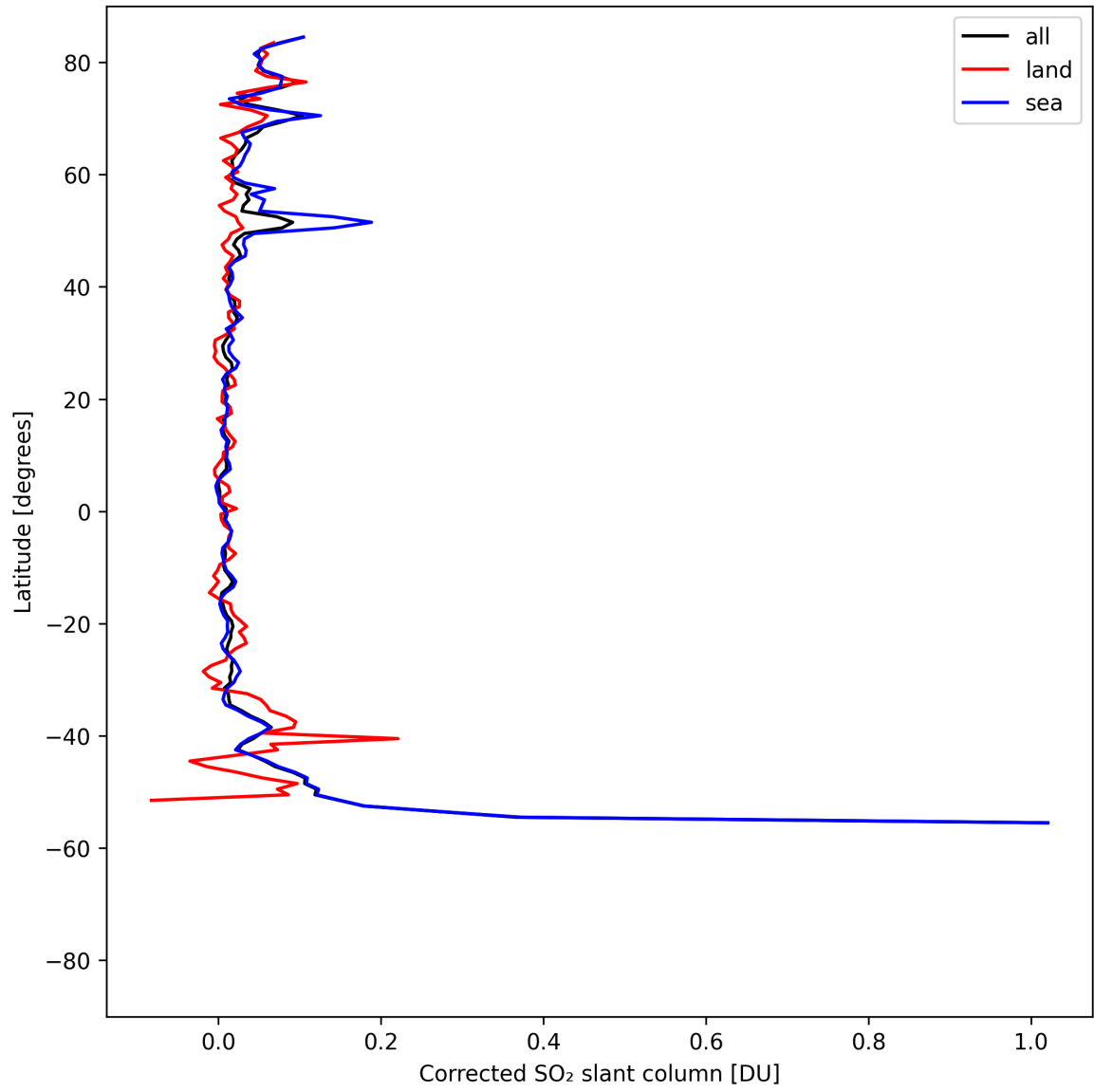
Figure 33: Zonal average of “Corrected SO 2 slant column” for 2025-08-14 to 2025-08-15.
