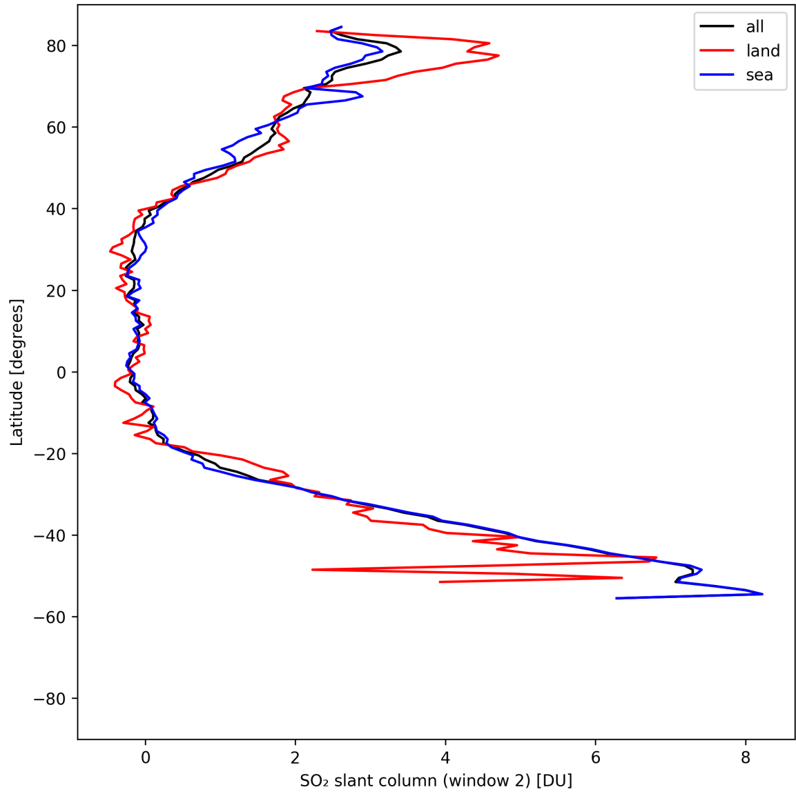
Figure 40: Zonal average of “SO 2 slant column (window 2)” for 2025-08-14 to 2025-08-15.
