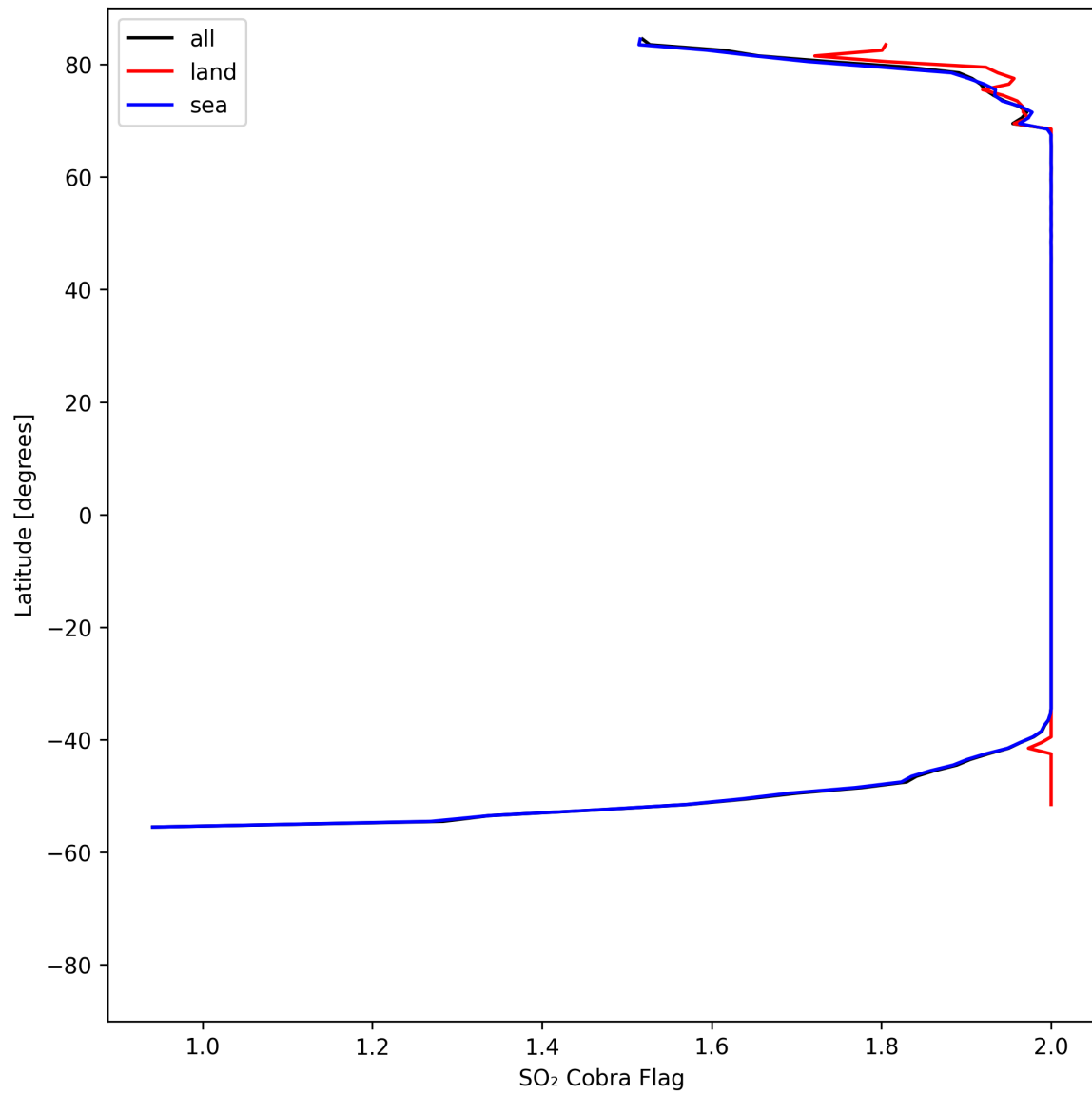
Figure 48: Zonal average of "SO 2 Cobra Flag" for 2025-08-14 to 2025-08-15.
