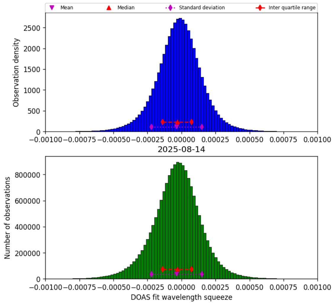
Figure 78: Histogram of “DOAS fit wavelength squeeze” for 2025-08-14 to 2025-08-15
