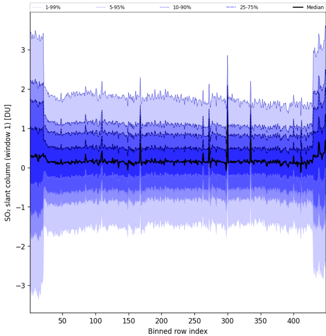
Figure 90: Along track statistics of “SO 2 slant column (window 1)” for 2025-08-14 to 2025-08-15
