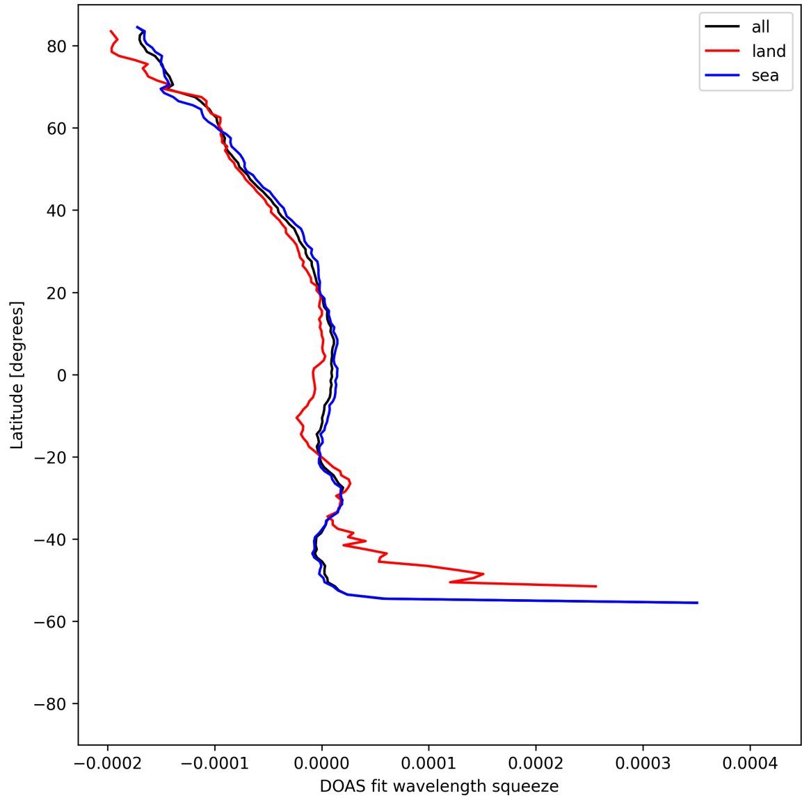
Figure 51: Zonal average of “DOAS fit wavelength squeeze” for 2025-08-14 to 2025-08-15.
