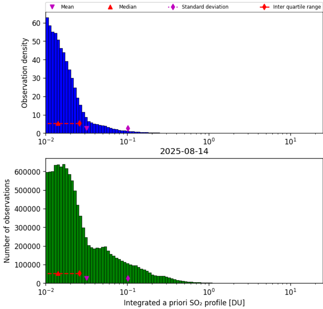
Figure 76: Histogram of “Integrated a priori SO 2 profile” for 2025-08-14 to 2025-08-15
