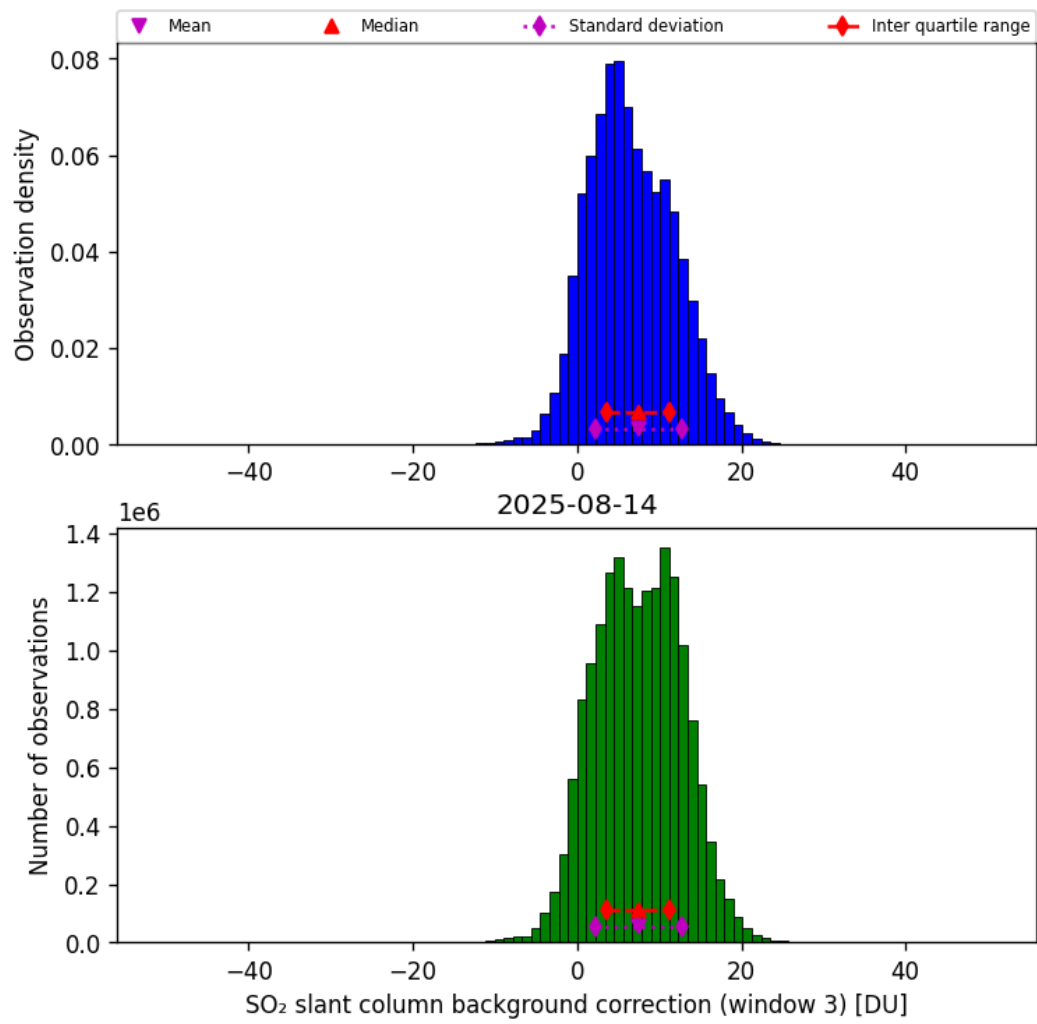
Figure 74: Histogram of “SO 2 slant column background correction (window 3)” for 2025-08-14 to 2025-08-15
