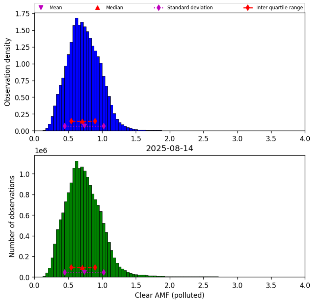
Figure 82: Histogram of “Clear AMF (polluted)” for 2025-08-14 to 2025-08-15
