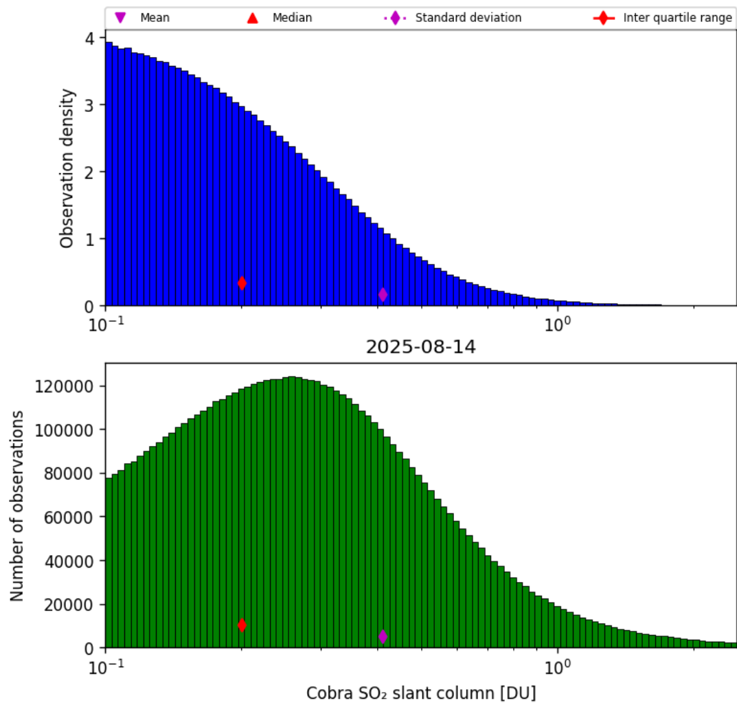
Figure 61: Histogram of “Cobra SO 2 slant column” for 2025-08-14 to 2025-08-15
