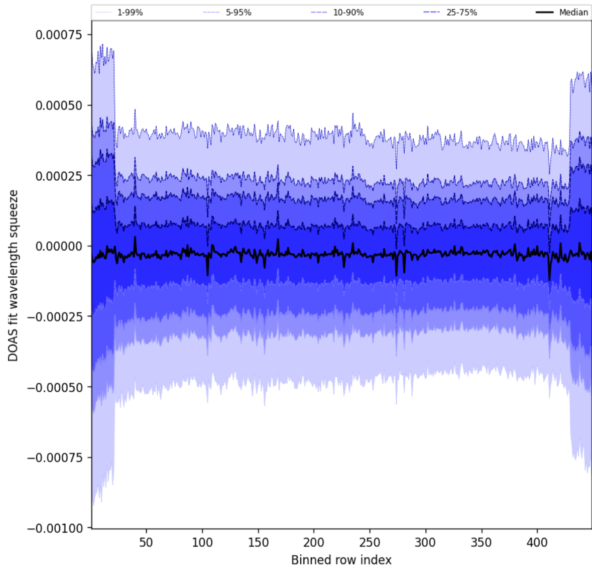
Figure 105: Along track statistics of “DOAS fit wavelength squeeze” for 2025-08-14 to 2025-08-15
