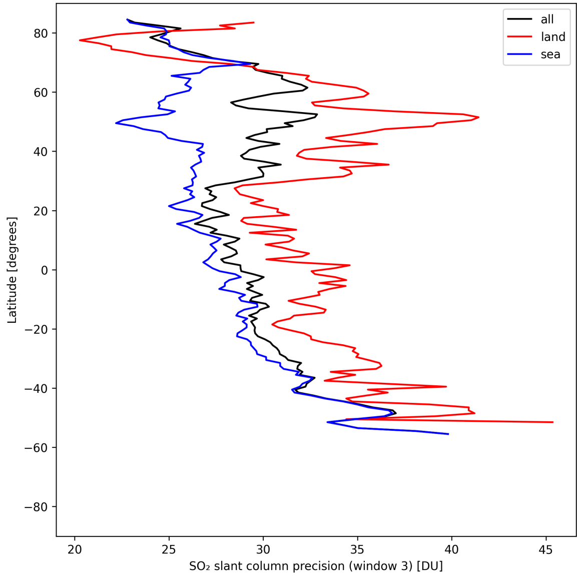
Figure 45: Zonal average of “SO 2 slant column precision (window 3)” for 2025-08-14 to 2025-08-15.
