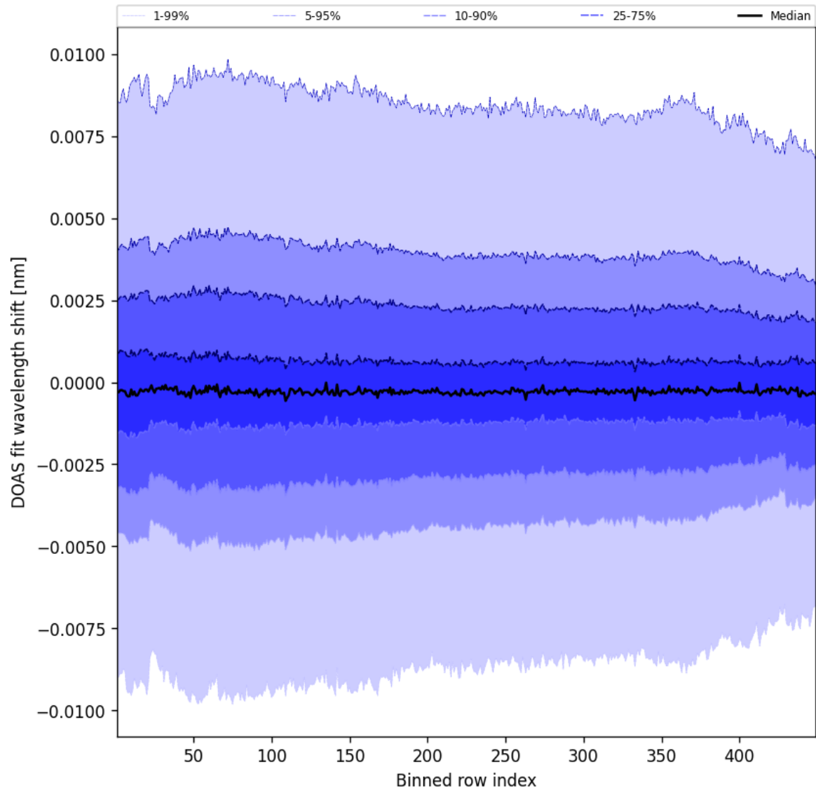
Figure 104: Along track statistics of “DOAS fit wavelength shift” for 2025-08-14 to 2025-08-15
