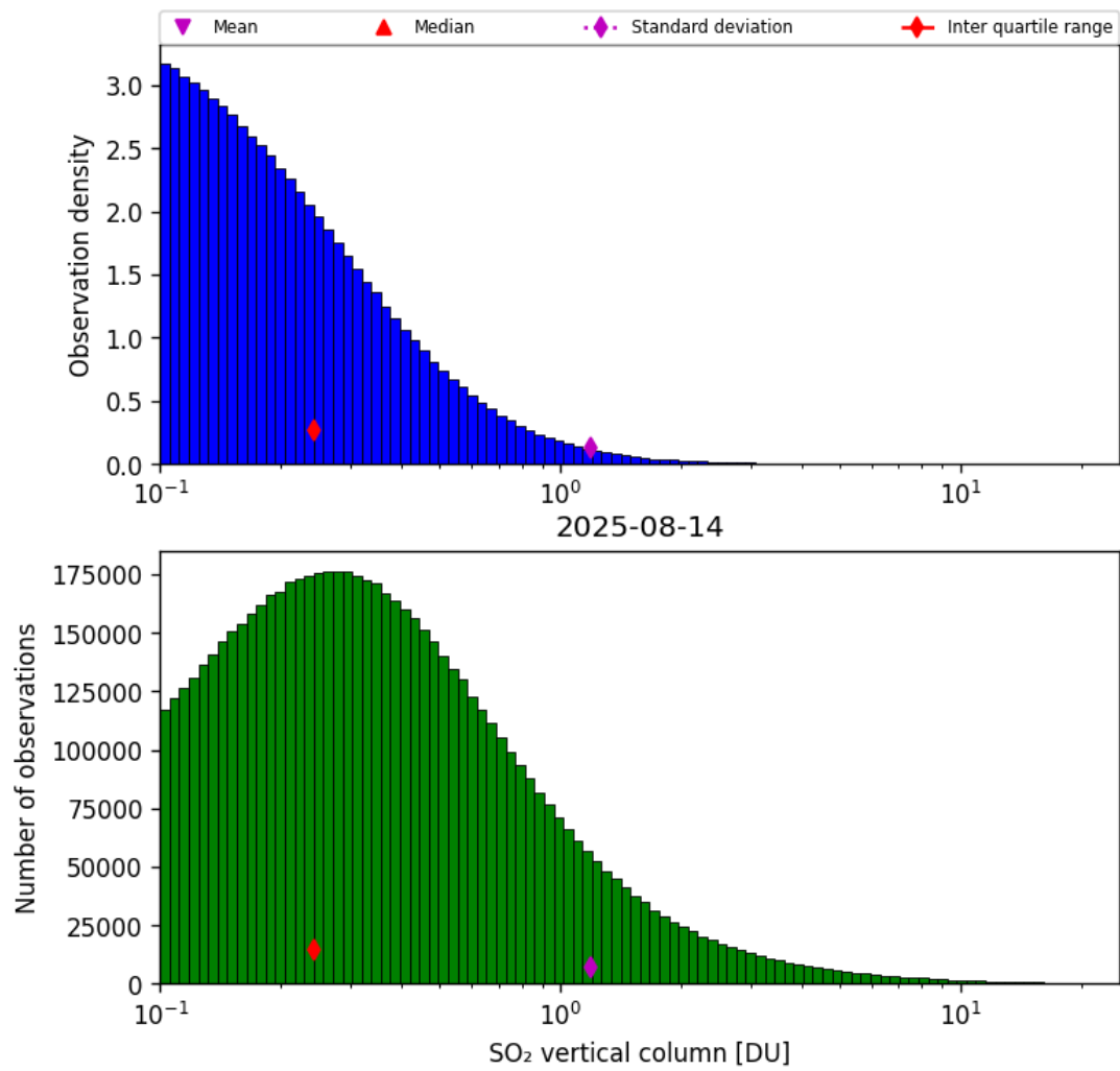
Figure 58: Histogram of “SO 2 vertical column” for 2025-08-14 to 2025-08-15
