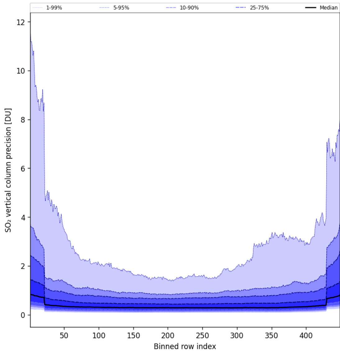
Figure 86: Along track statistics of “SO 2 vertical column precision” for 2025-08-14 to 2025-08-15
