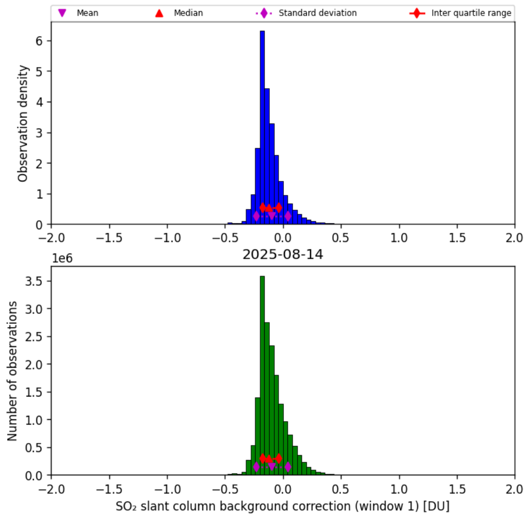
Figure 66: Histogram of “SO 2 slant column background correction (window 1)” for 2025-08-14 to 2025-08-15
