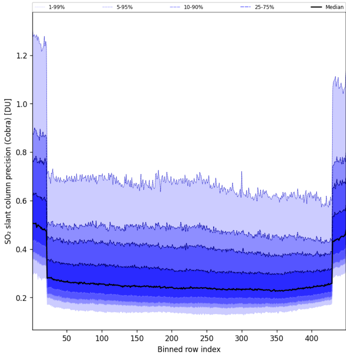
Figure 89: Along track statistics of “SO 2 slant column precision (Cobra)” for 2025-08-14 to 2025-08-15
