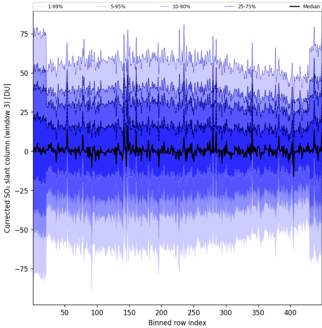
Figure 100: Along track statistics of “Corrected SO 2 slant column (window 3)” for 2025-08-14 to 2025-08-15
