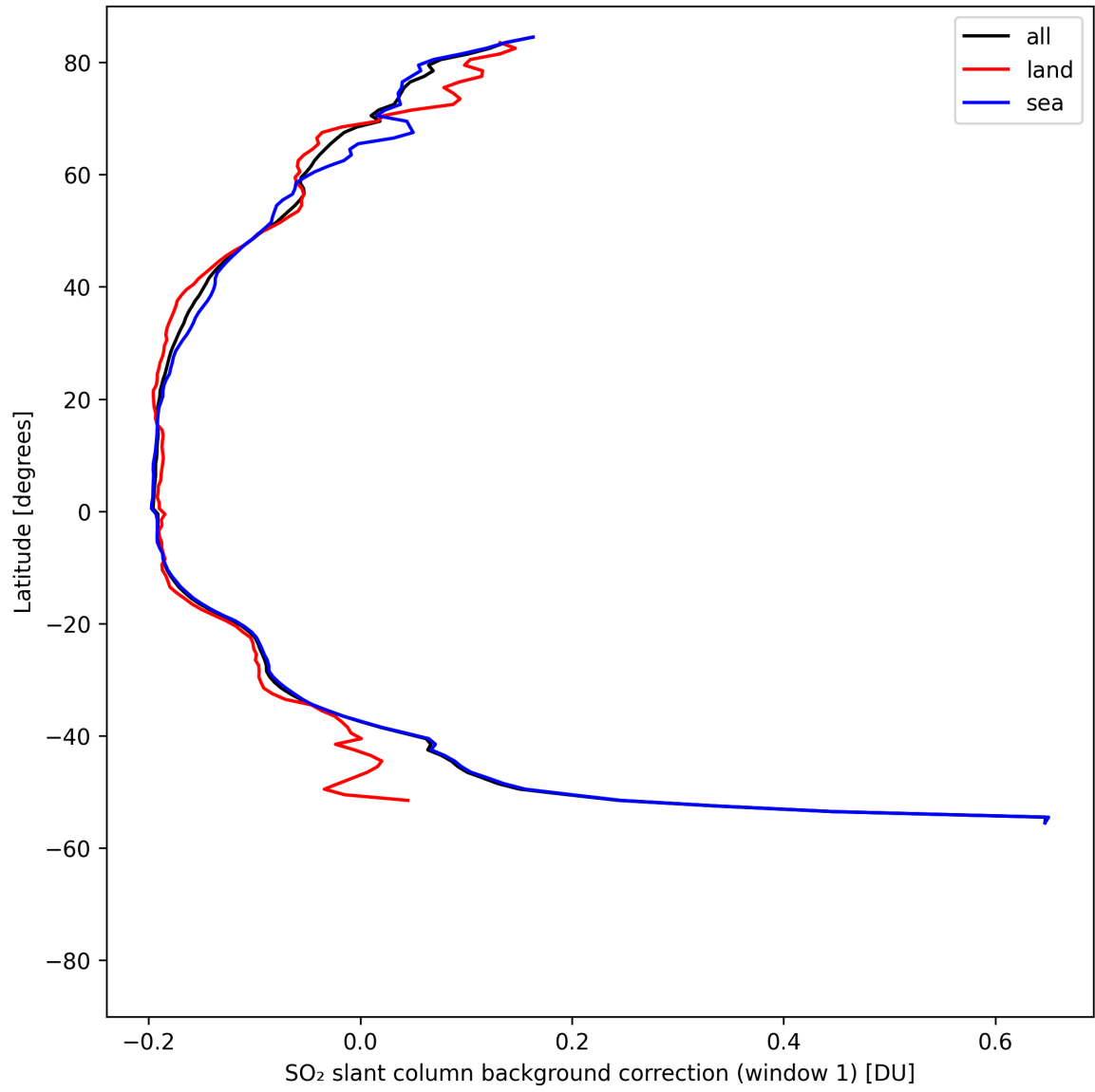
Figure 39: Zonal average of "SO 2 slant column background correction (window 1)" for 2025-08-14 to 2025-08-15.
