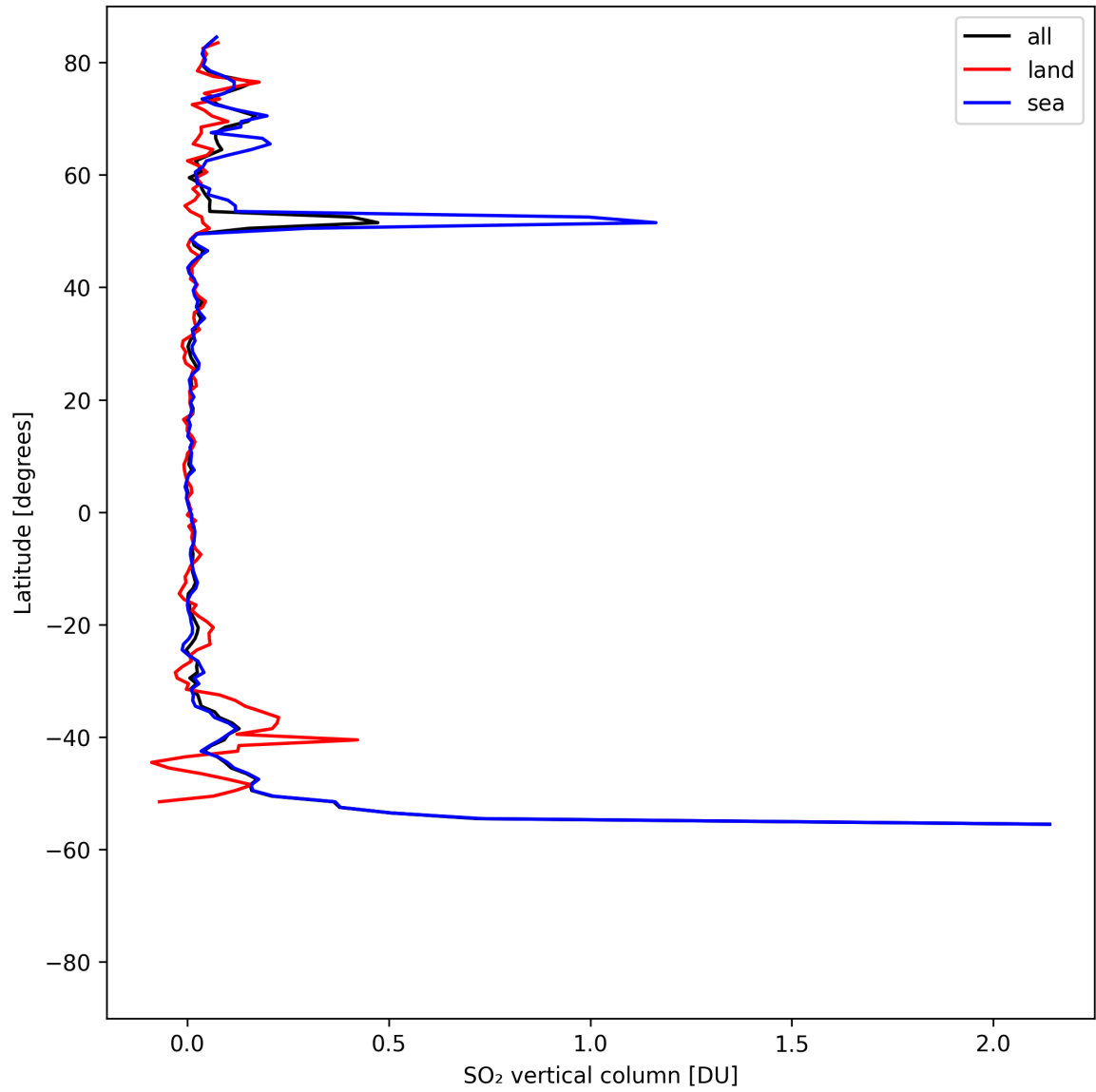
Figure 31: Zonal average of “SO 2 vertical column” for 2025-08-14 to 2025-08-15.
