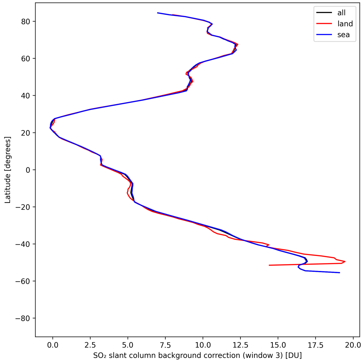
Figure 47: Zonal average of “SO 2 slant column background correction (window 3)” for 2025-08-14 to 2025-08-15.
