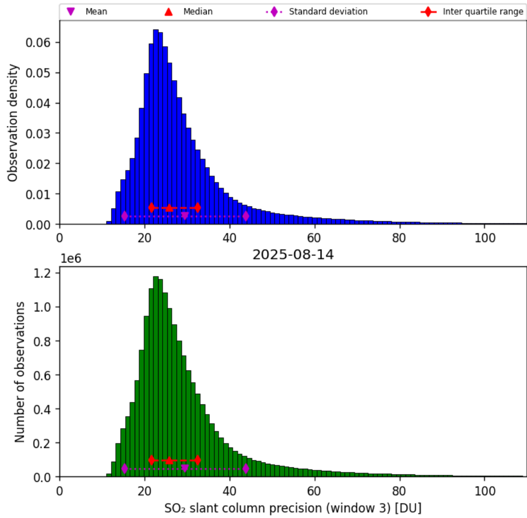
Figure 72: Histogram of “SO 2 slant column precision (window 3)” for 2025-08-14 to 2025-08-15
