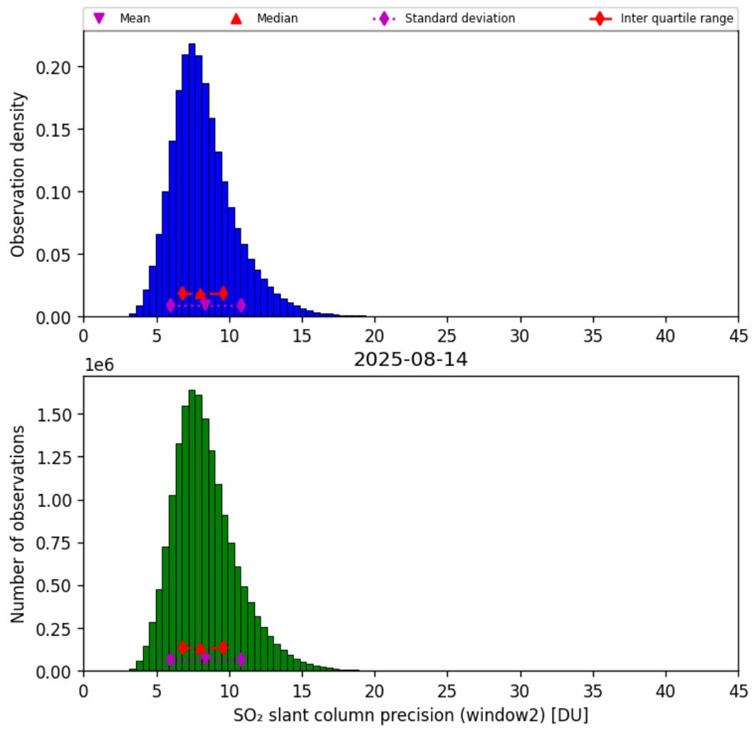
Figure 68: Histogram of “SO 2 slant column precision (window2)” for 2025-08-14 to 2025-08-15
