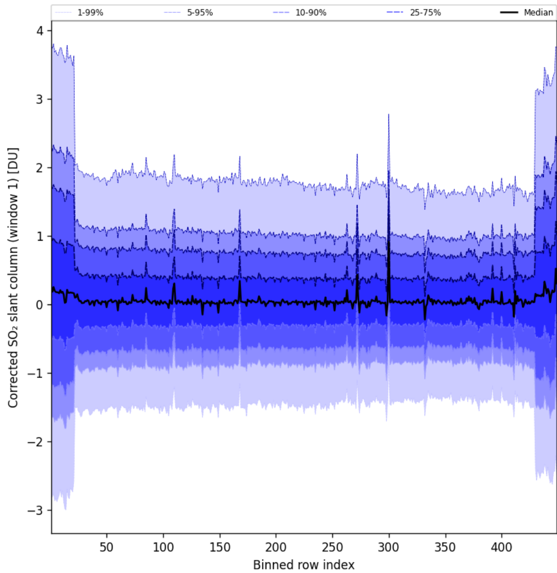
Figure 92: Along track statistics of “Corrected SO 2 slant column (window 1)” for 2025-08-14 to 2025-08-15
