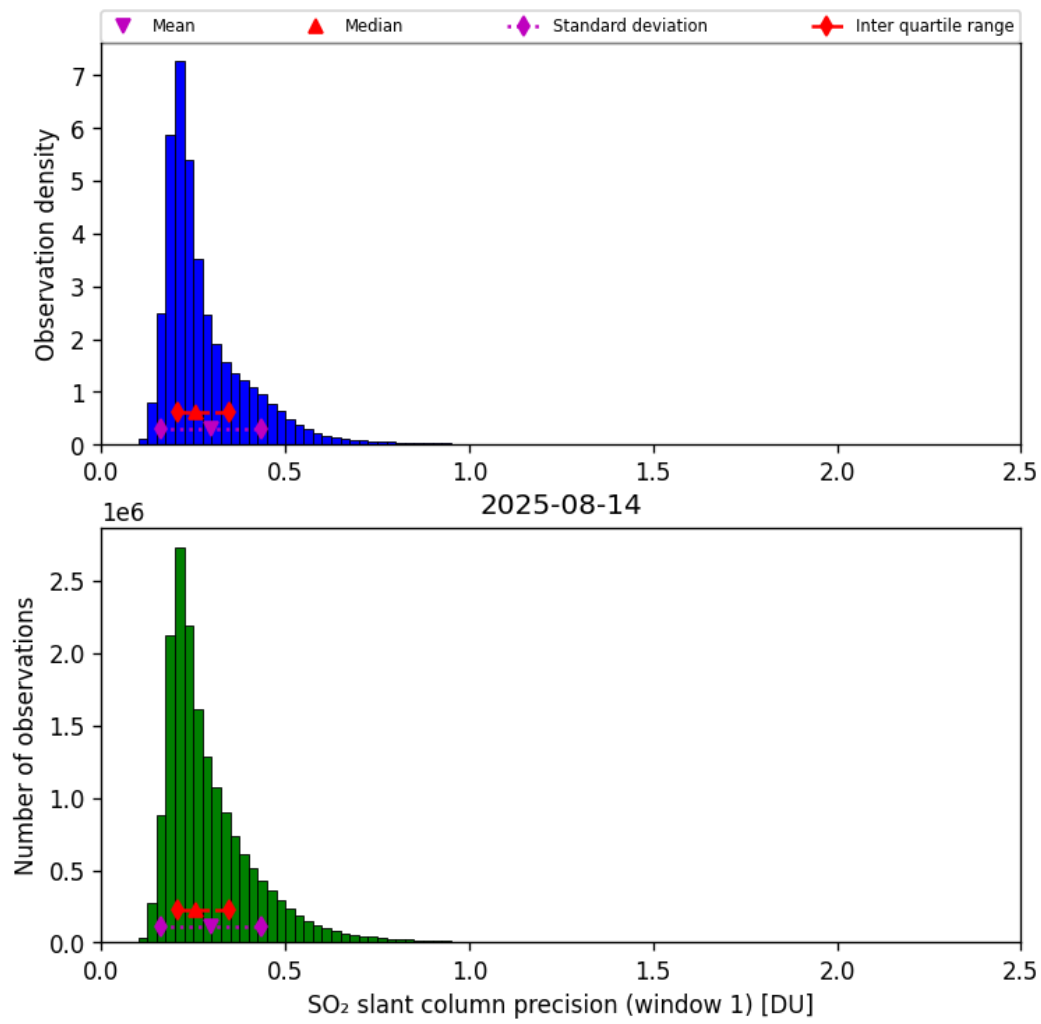
Figure 64: Histogram of “SO 2 slant column precision (window 1)” for 2025-08-14 to 2025-08-15
