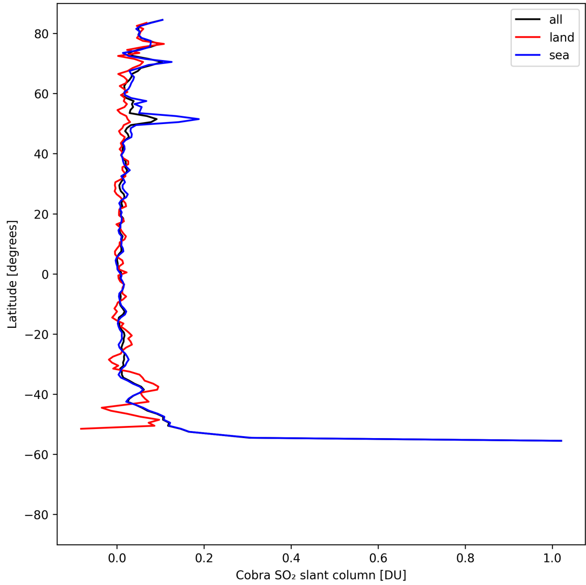
Figure 34: Zonal average of “Cobra SO 2 slant column” for 2025-08-14 to 2025-08-15.
