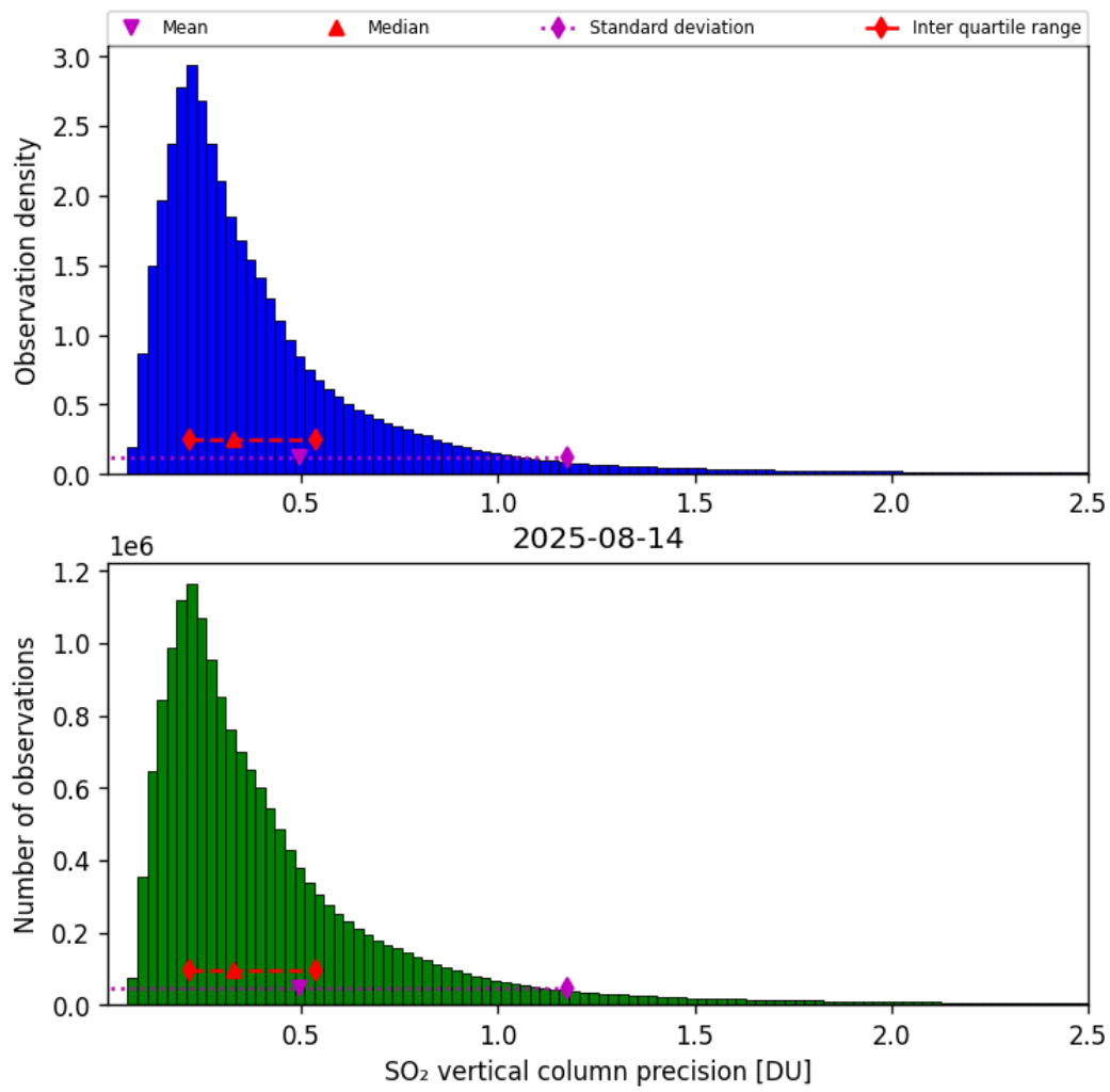
Figure 59: Histogram of “SO 2 vertical column precision” for 2025-08-14 to 2025-08-15
