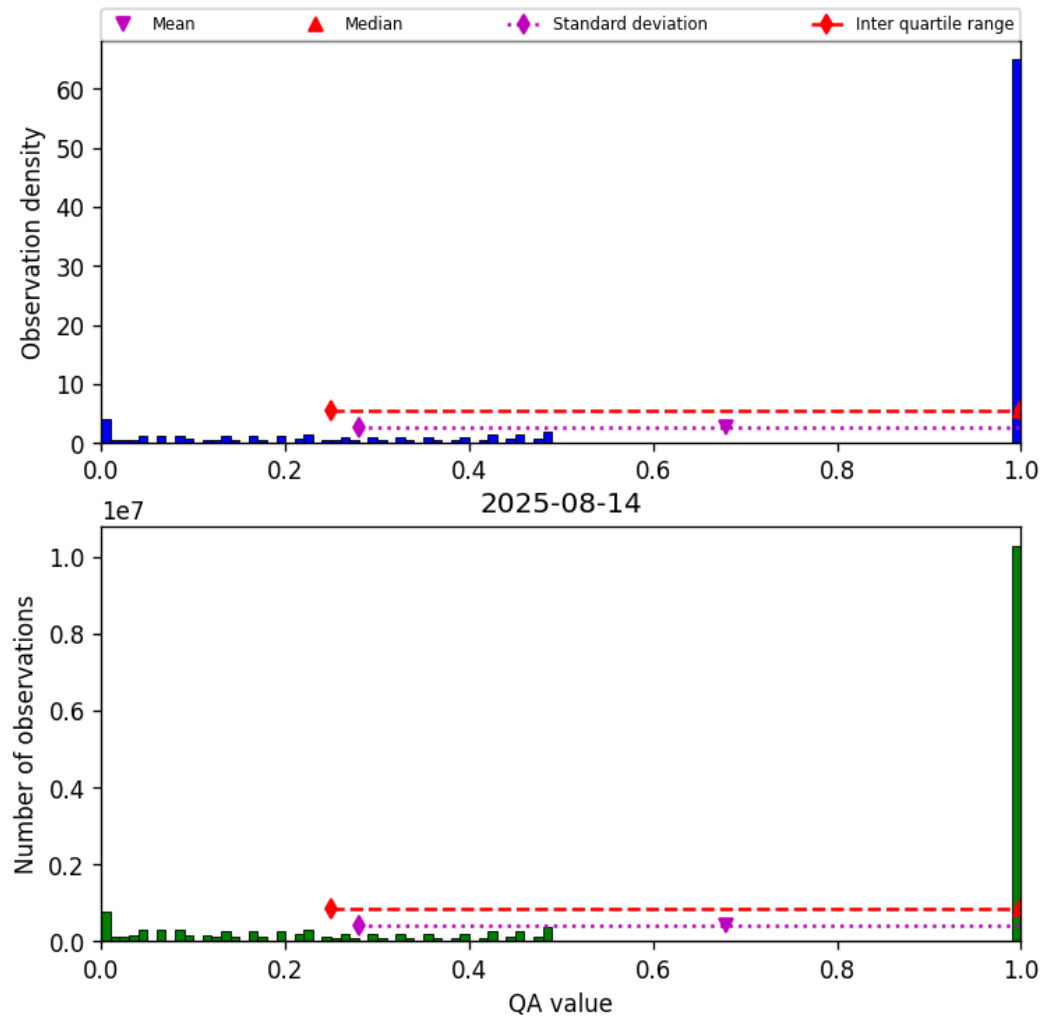
Figure 57: Histogram of “QA value” for 2025-08-14 to 2025-08-15
