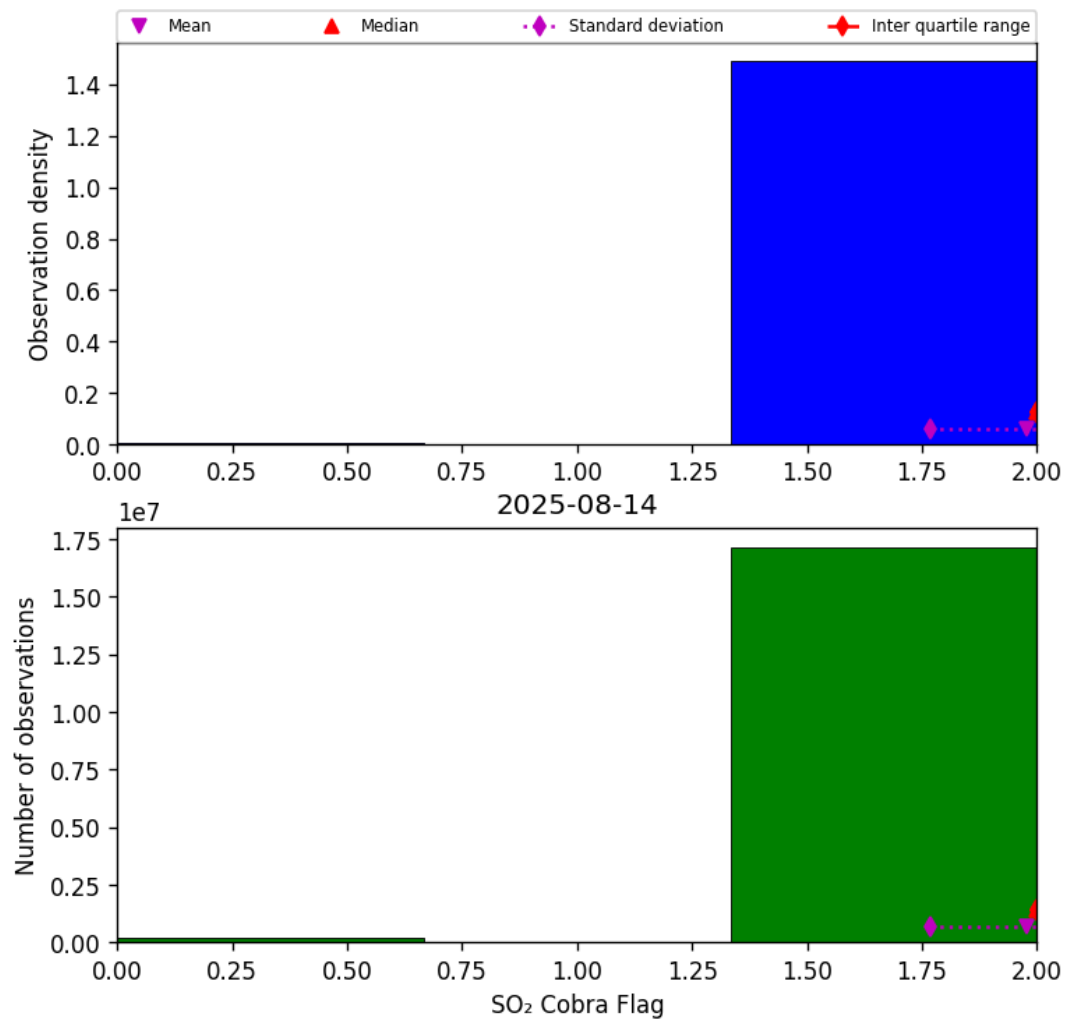
Figure 75: Histogram of “SO 2 Cobra Flag” for 2025-08-14 to 2025-08-15
