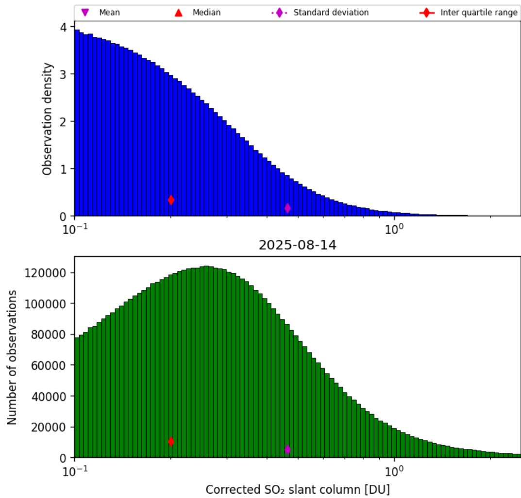
Figure 60: Histogram of "Corrected SO 2 slant column" for 2025-08-14 to 2025-08-15
