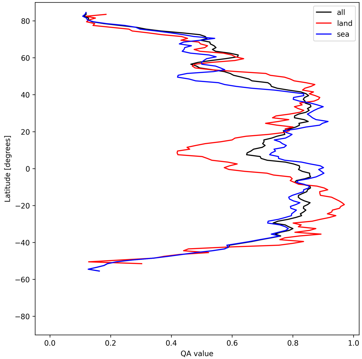
Figure 30: Zonal average of “QA value” for 2025-08-14 to 2025-08-15.
