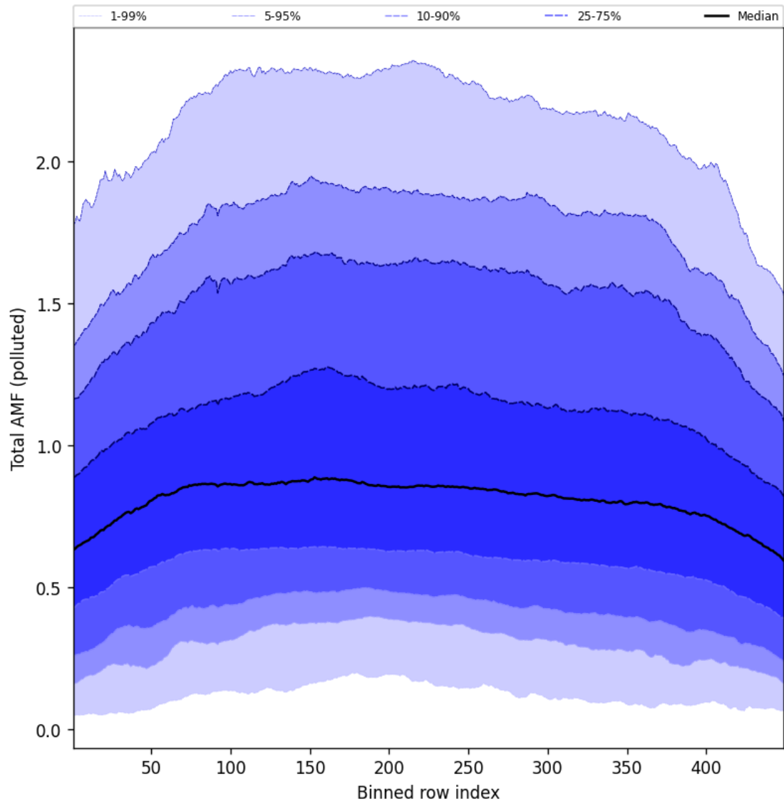
Figure 107: Along track statistics of “Total AMF (polluted)” for 2025-08-14 to 2025-08-15
