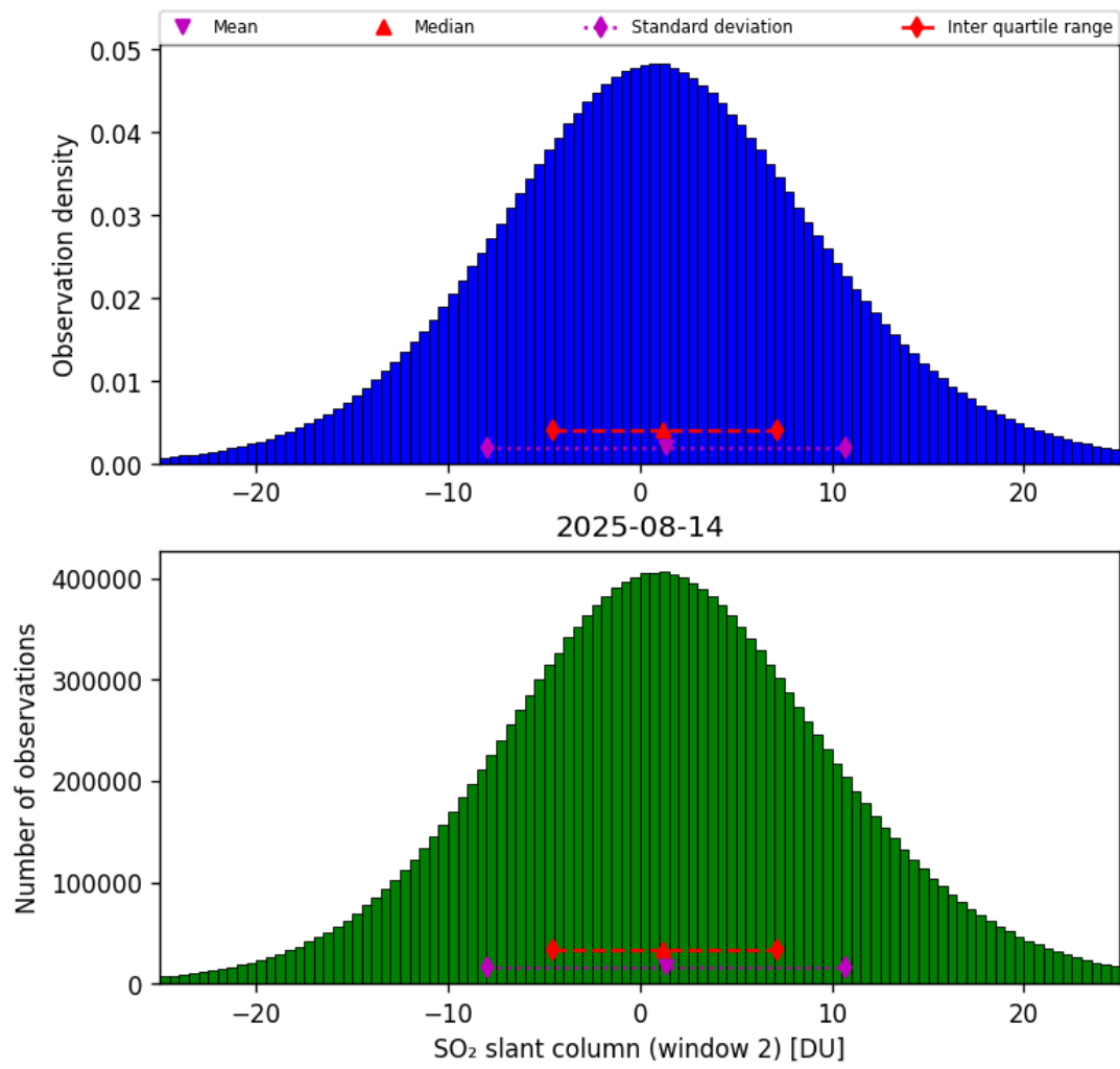
Figure 67: Histogram of “SO 2 slant column (window 2)” for 2025-08-14 to 2025-08-15
