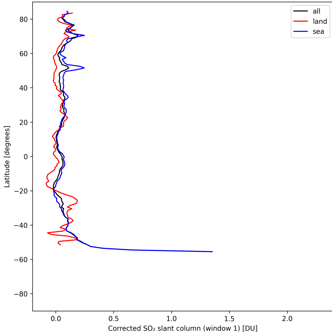
Figure 38: Zonal average of “Corrected SO 2 slant column (window 1)” for 2025-08-14 to 2025-08-15.
