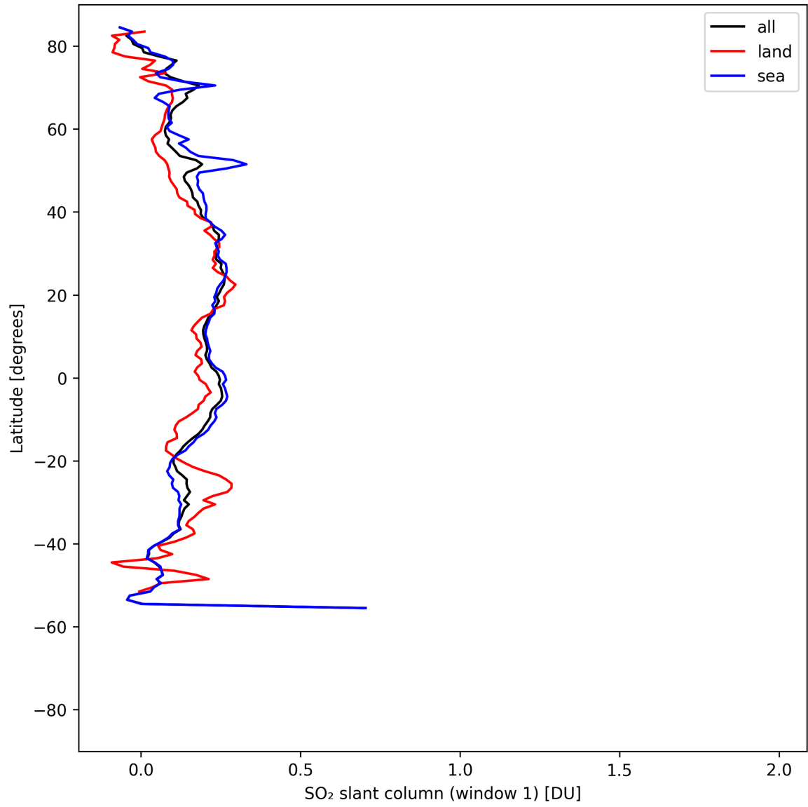
Figure 36: Zonal average of “SO 2 slant column (window 1)” for 2025-08-14 to 2025-08-15.
