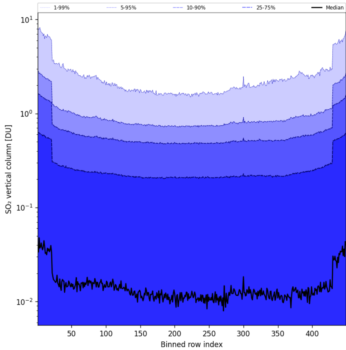
Figure 85: Along track statistics of “SO 2 vertical column” for 2025-08-14 to 2025-08-15
