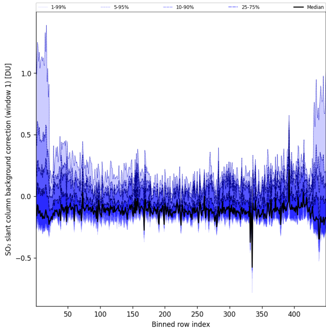
Figure 93: Along track statistics of “SO 2 slant column background correction (window 1)” for 2025-08-14 to 2025-08-15
