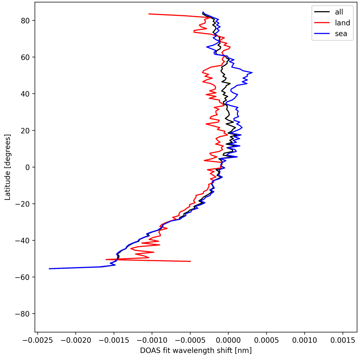
Figure 50: Zonal average of “DOAS fit wavelength shift” for 2025-08-14 to 2025-08-15.
