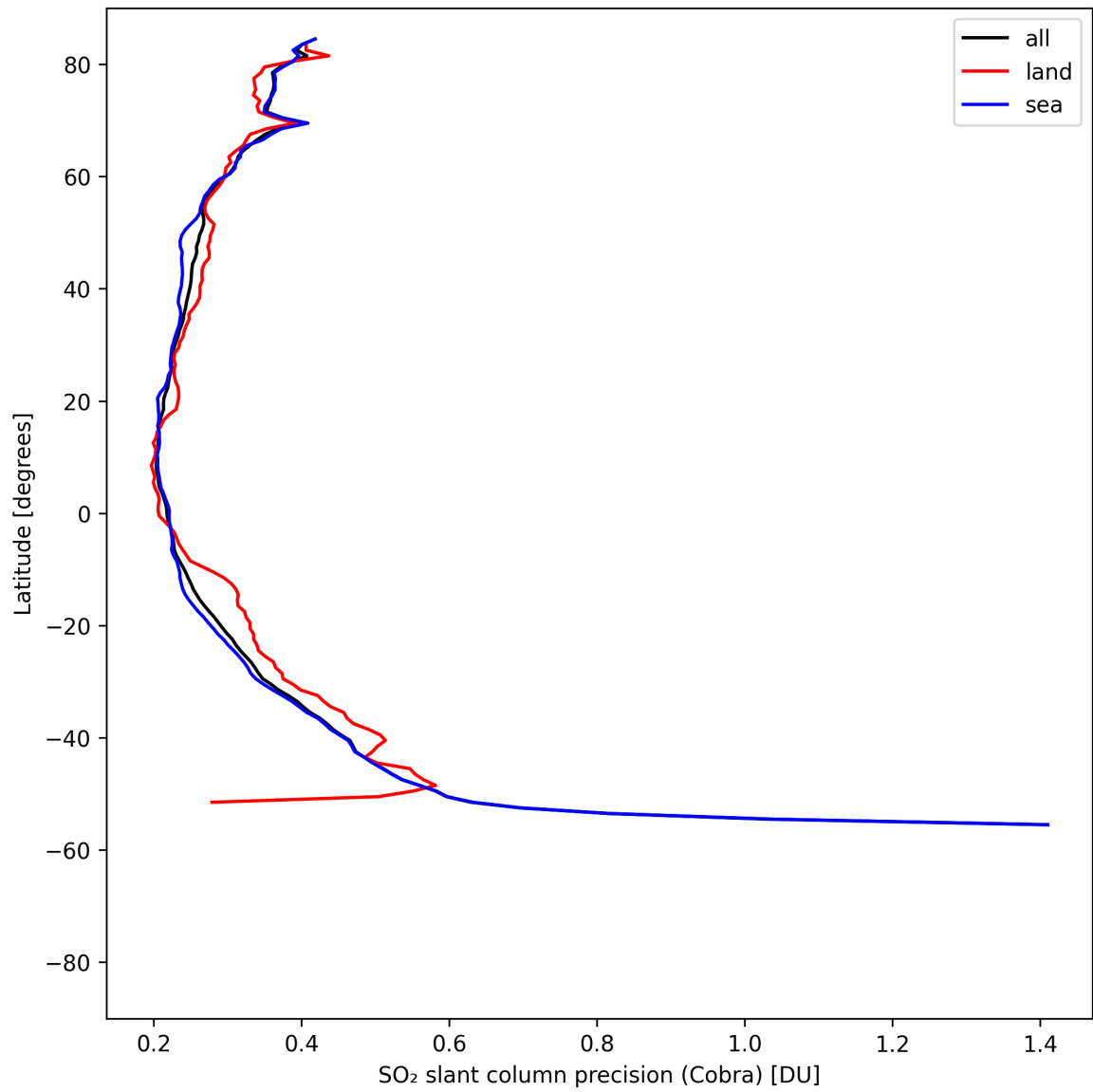
Figure 35: Zonal average of “SO 2 slant column precision (Cobra)” for 2025-08-14 to 2025-08-15.
