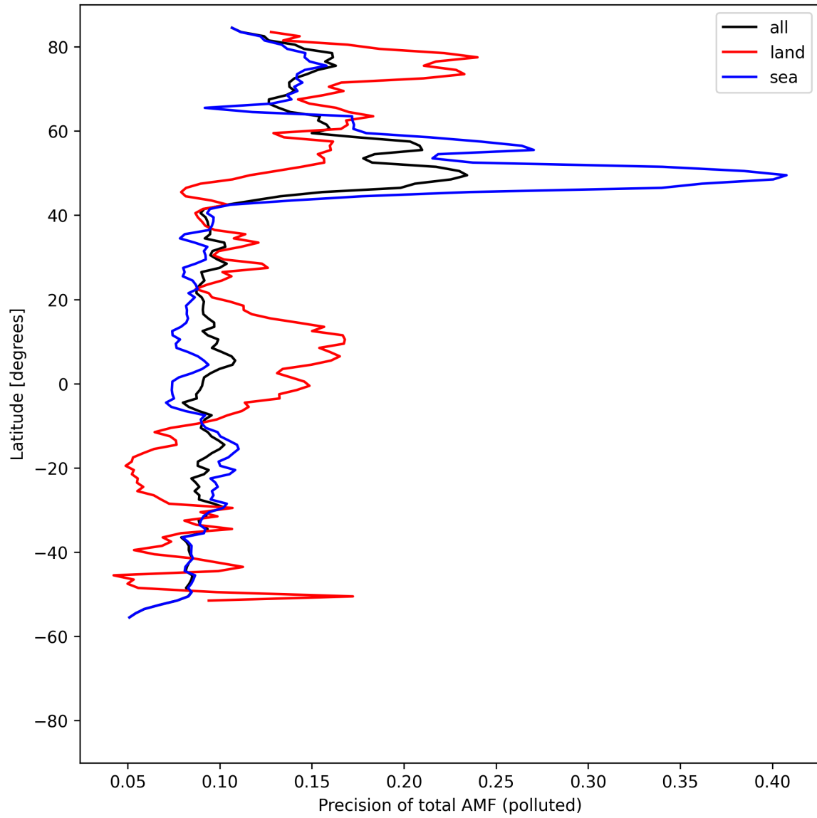
Figure 54: Zonal average of “Precision of total AMF (polluted)” for 2025-08-14 to 2025-08-15.
