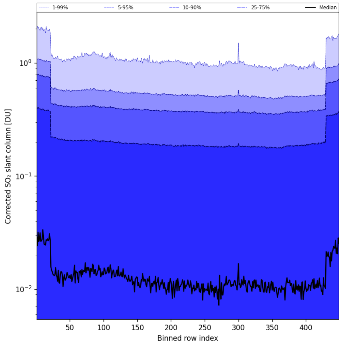
Figure 87: Along track statistics of “Corrected SO 2 slant column” for 2025-08-14 to 2025-08-15
