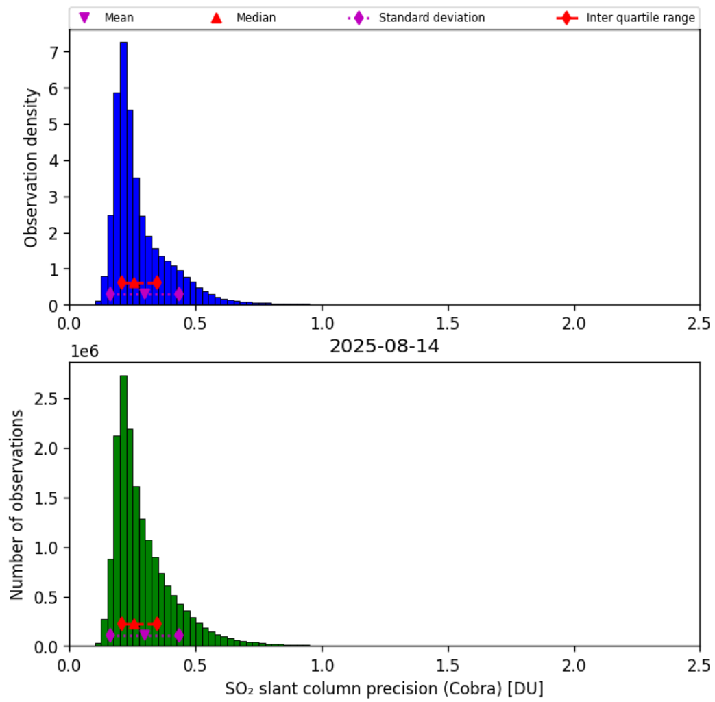
Figure 62: Histogram of “SO 2 slant column precision (Cobra)” for 2025-08-14 to 2025-08-15
