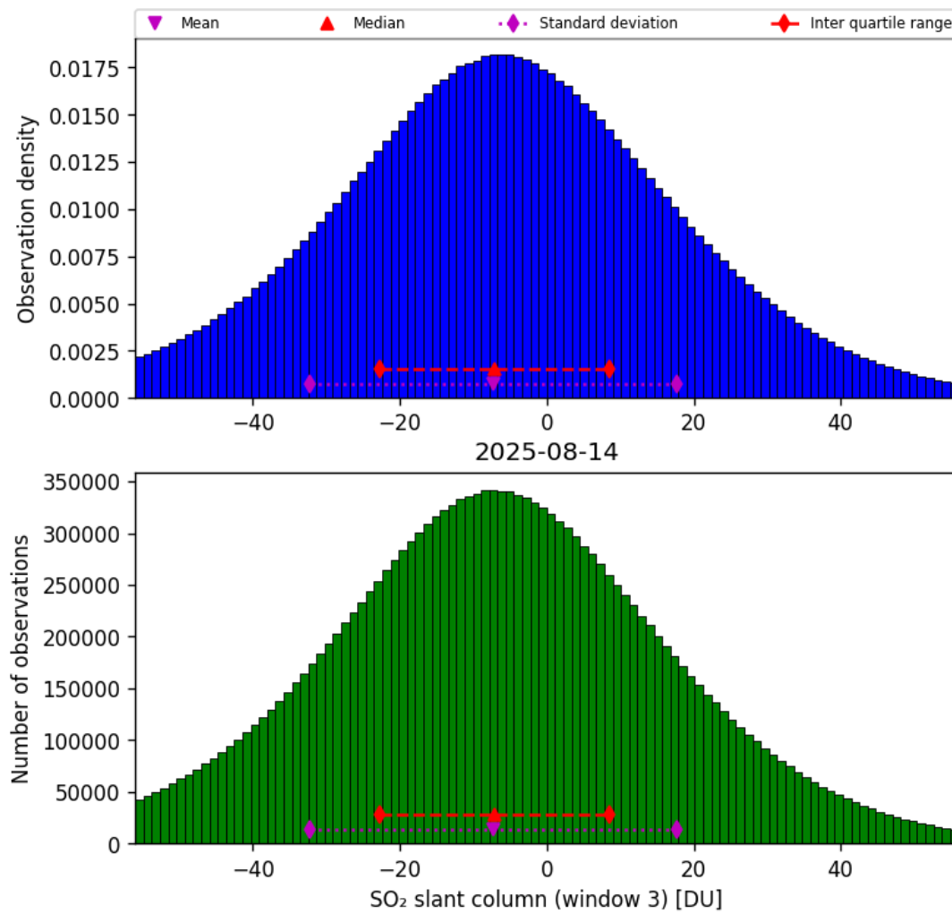
Figure 71: Histogram of “SO 2 slant column (window 3)” for 2025-08-14 to 2025-08-15
