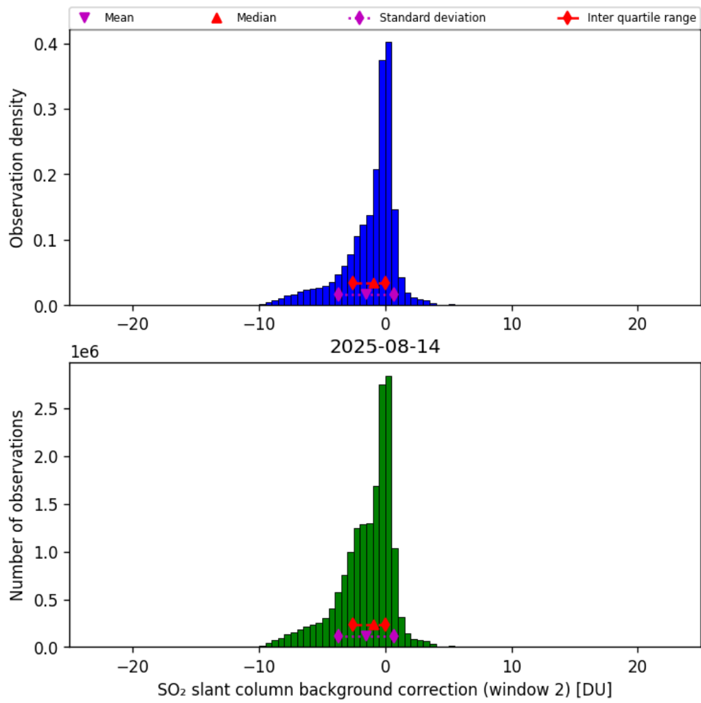
Figure 70: Histogram of “SO 2 slant column background correction (window 2)” for 2025-08-14 to 2025-08-15
