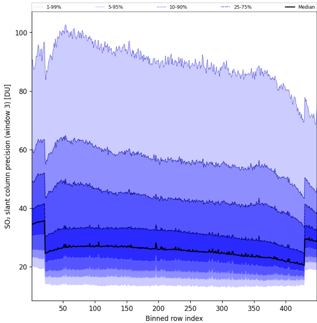
Figure 99: Along track statistics of “SO 2 slant column precision (window 3)” for 2025-08-14 to 2025-08-15
