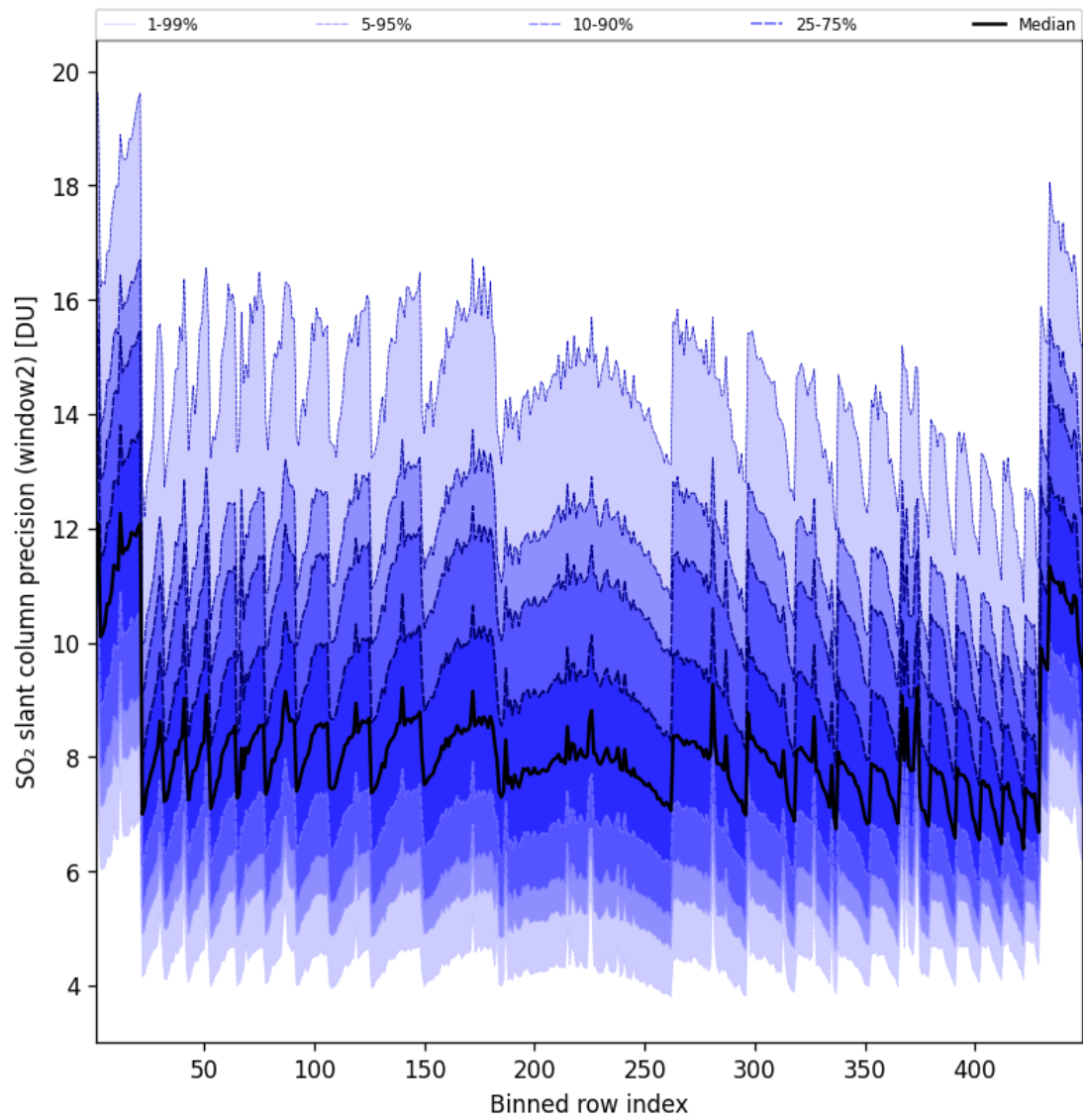
Figure 95: Along track statistics of “SO 2 slant column precision (window2)” for 2025-08-14 to 2025-08-15
