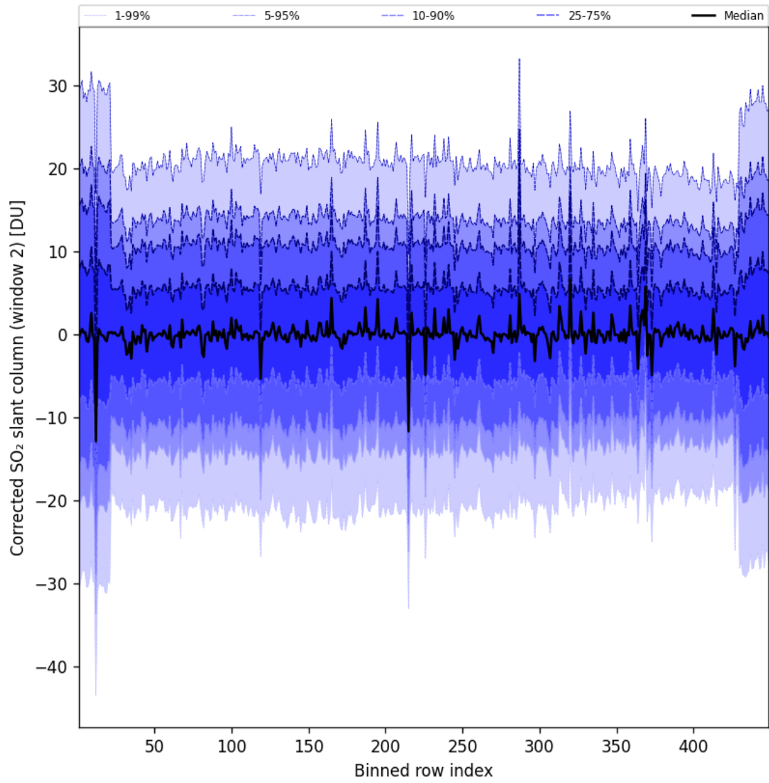
Figure 96: Along track statistics of “Corrected SO 2 slant column (window 2)” for 2025-08-14 to 2025-08-15
