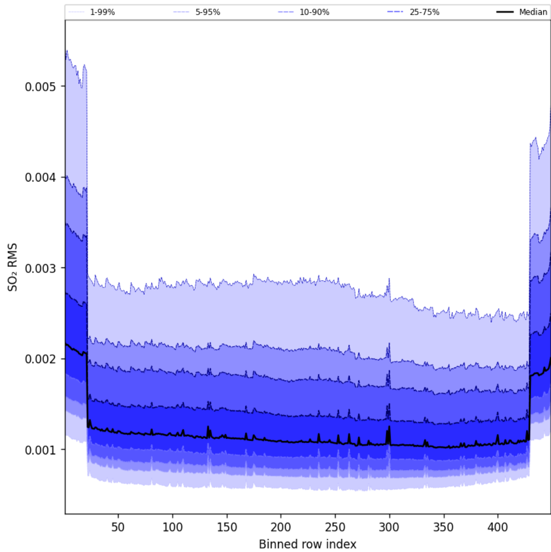
Figure 106: Along track statistics of “SO 2 RMS” for 2025-08-14 to 2025-08-15
