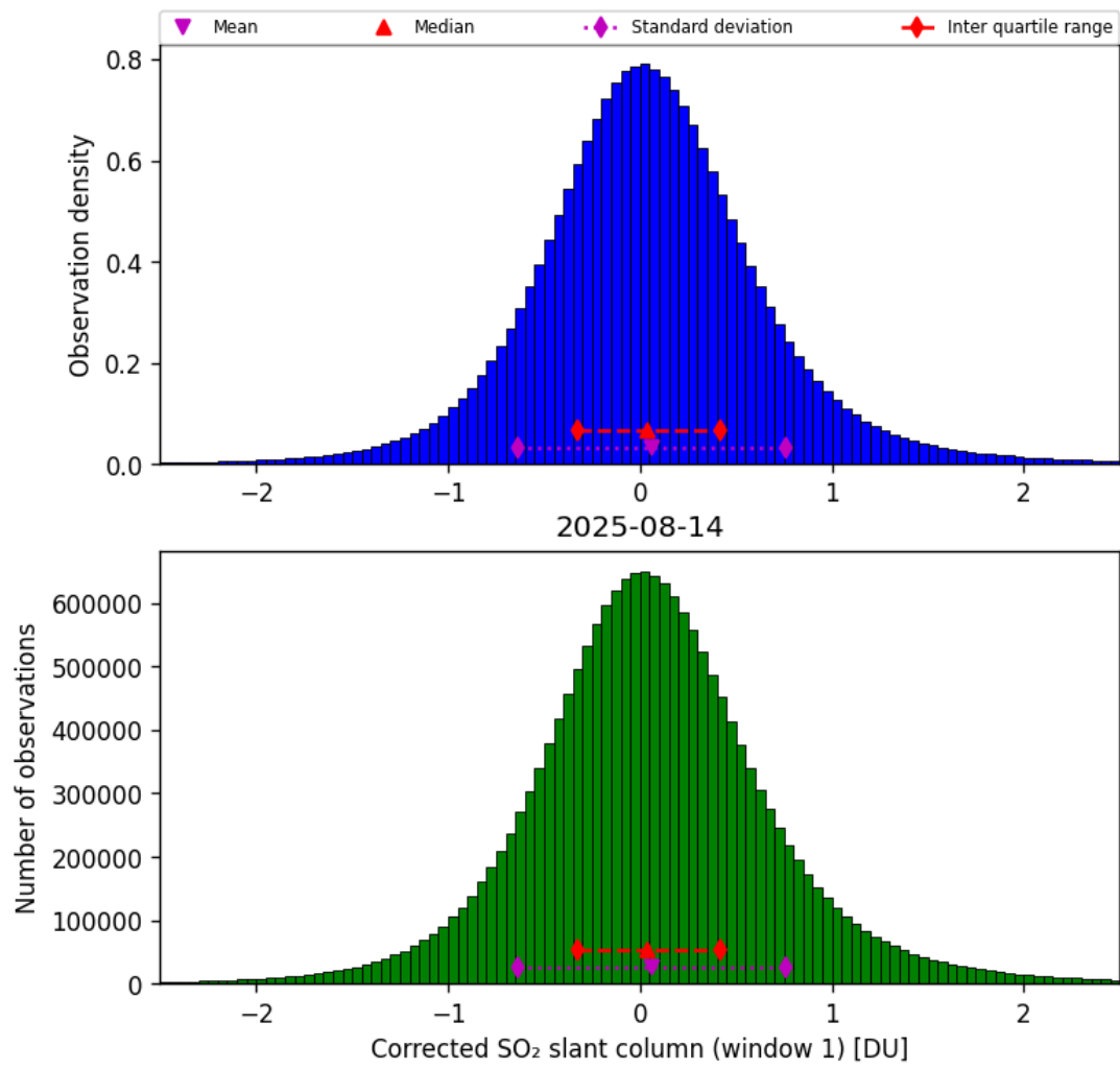
Figure 65: Histogram of “Corrected SO 2 slant column (window 1)” for 2025-08-14 to 2025-08-15
