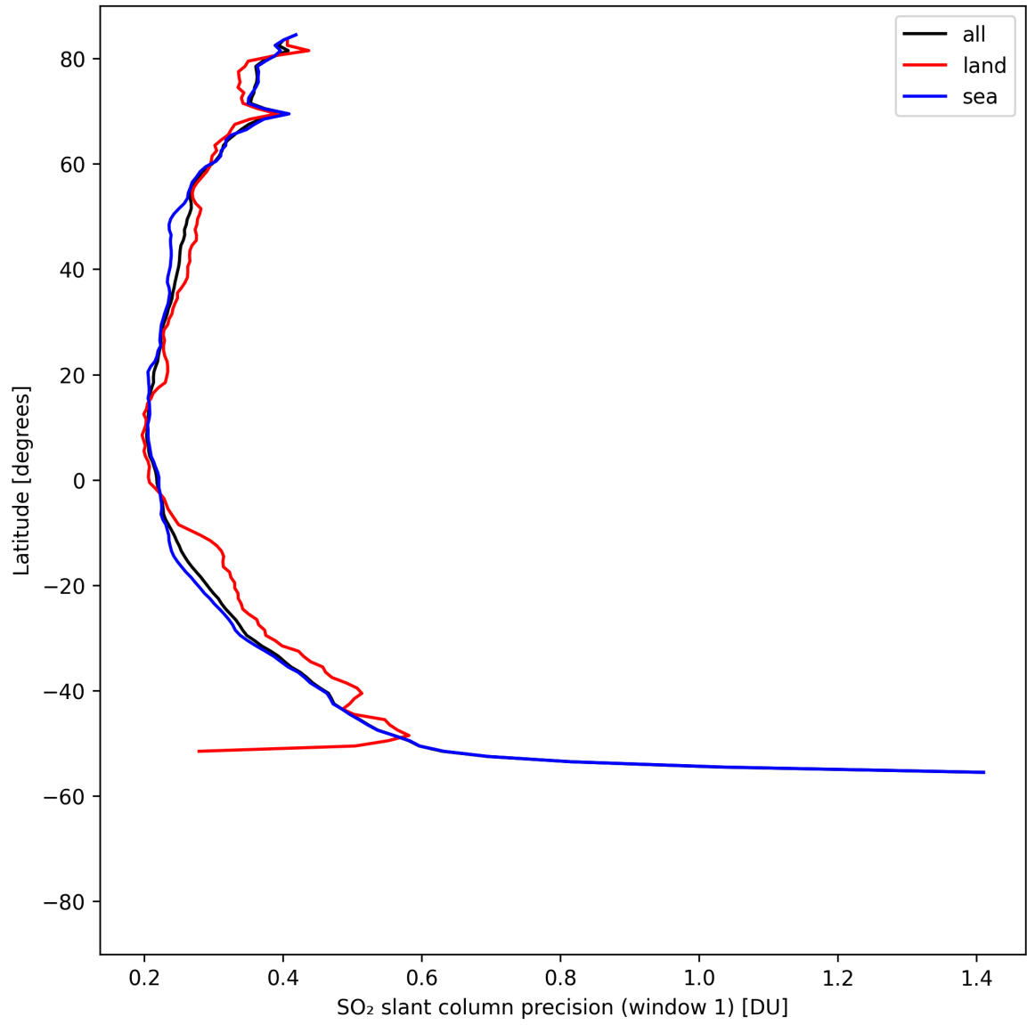
Figure 37: Zonal average of “SO 2 slant column precision (window 1)” for 2025-08-14 to 2025-08-15.
