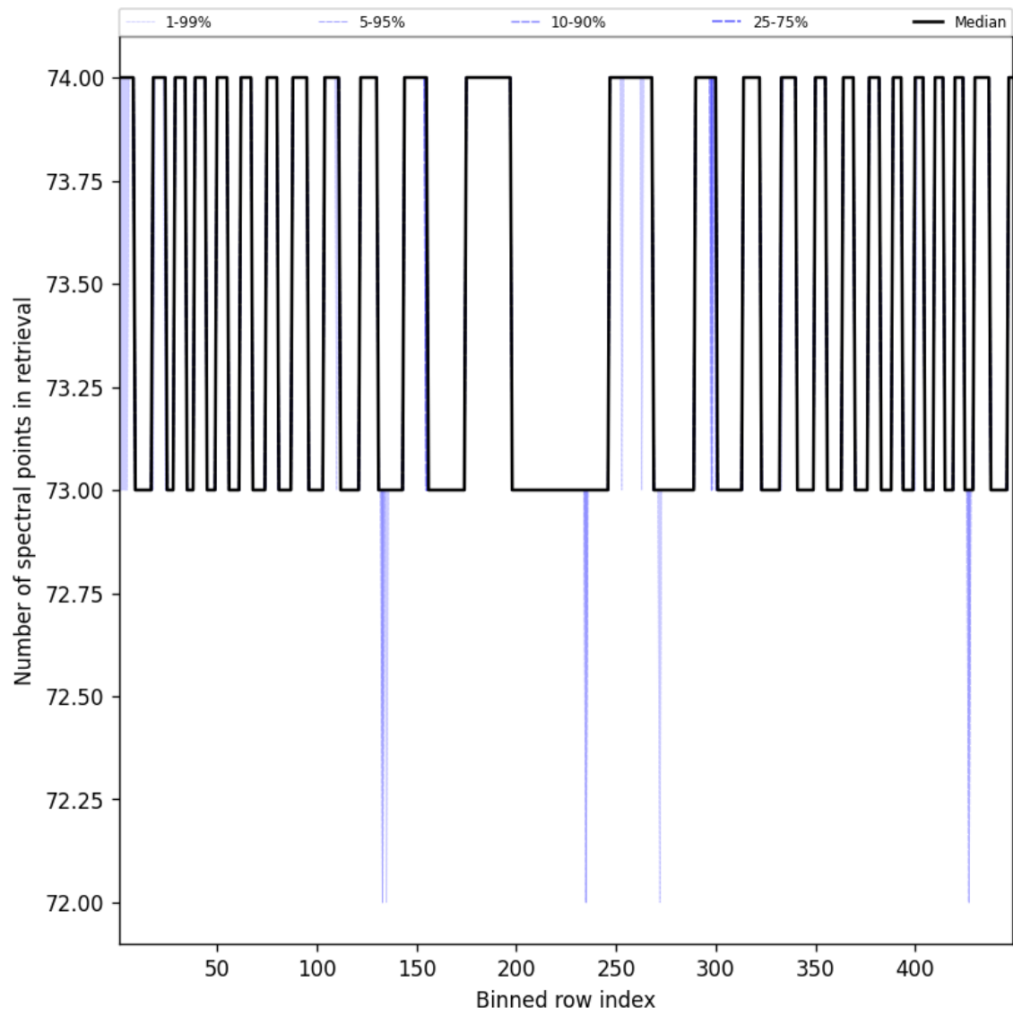
Figure 110: Along track statistics of “Number of spectral points in retrieval” for 2025-08-14 to 2025-08-15
