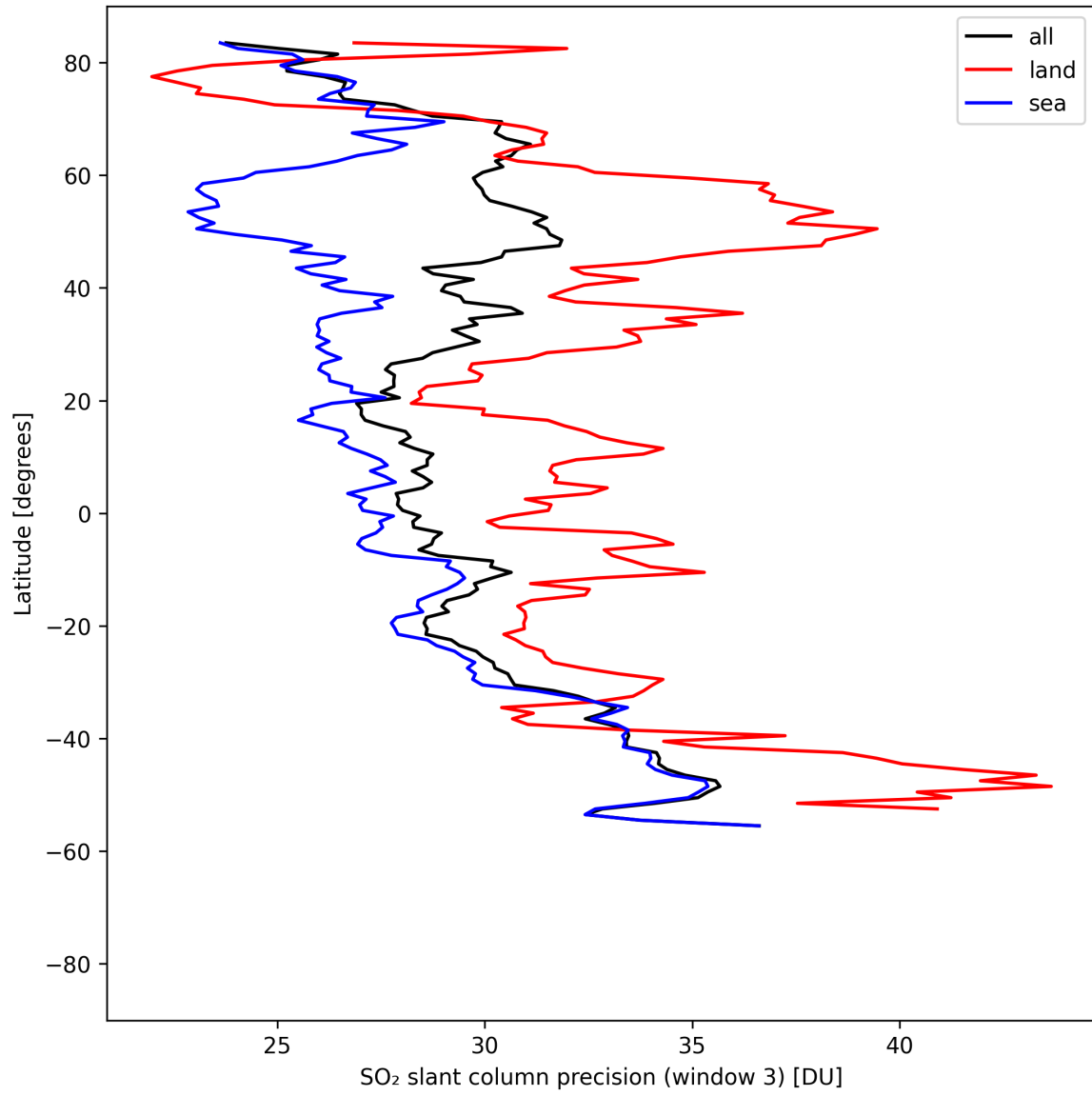
Figure 45: Zonal average of “SO 2 slant column precision (window 3)” for 2025-08-15 to 2025-08-16.
