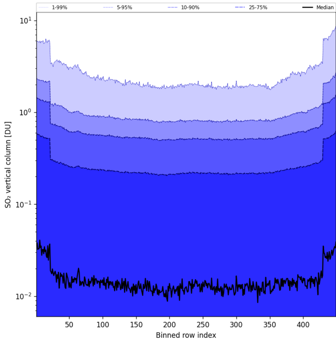
Figure 85: Along track statistics of “SO 2 vertical column” for 2025-08-15 to 2025-08-16
