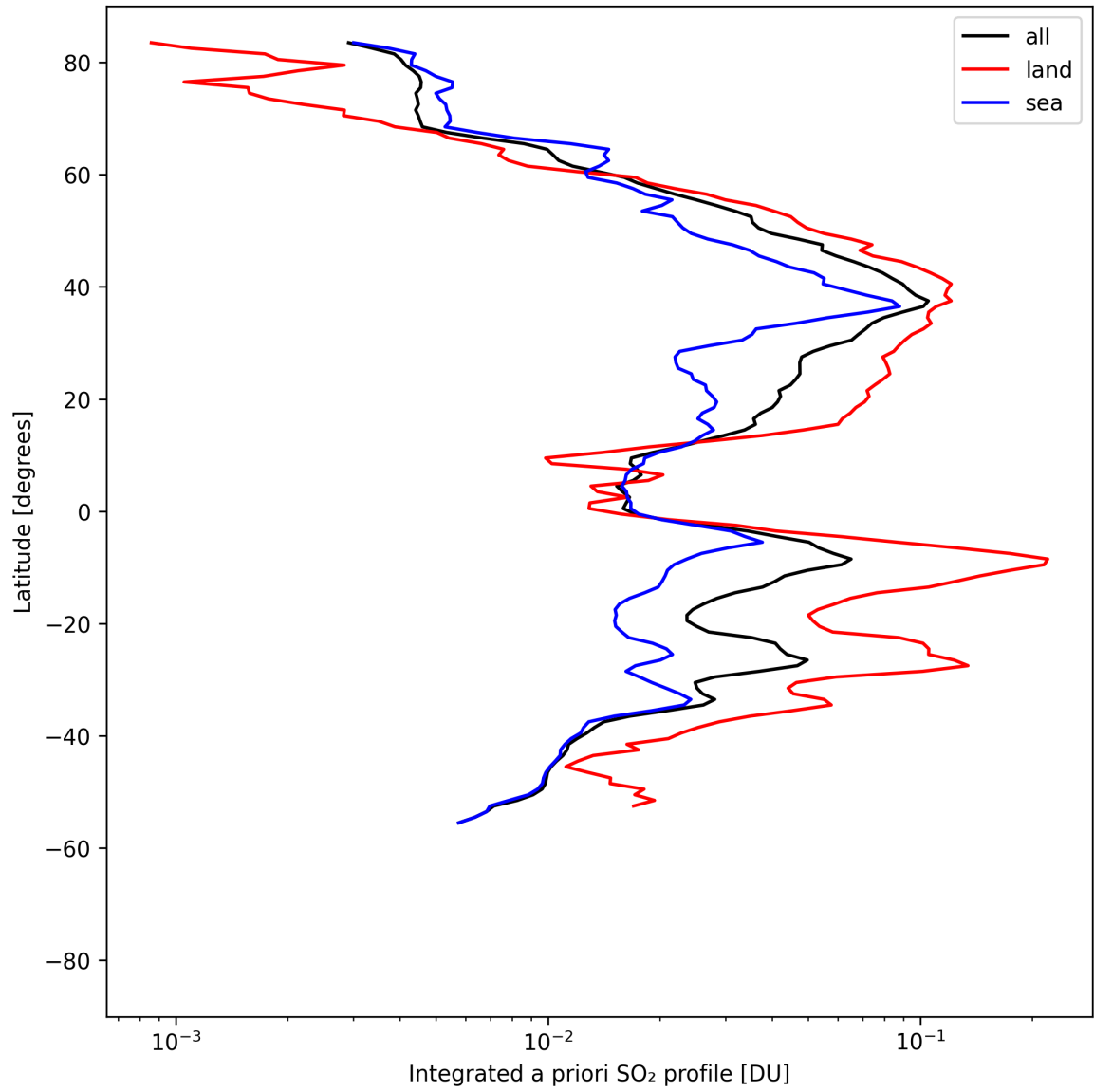
Figure 49: Zonal average of “Integrated a priori SO 2 profile” for 2025-08-15 to 2025-08-16.
