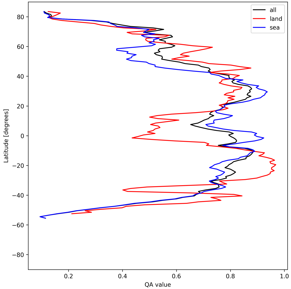
Figure 30: Zonal average of “QA value” for 2025-08-15 to 2025-08-16.
