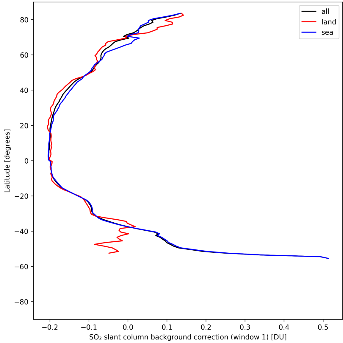
Figure 39: Zonal average of “SO 2 slant column background correction (window 1)” for 2025-08-15 to 2025-08-16.
