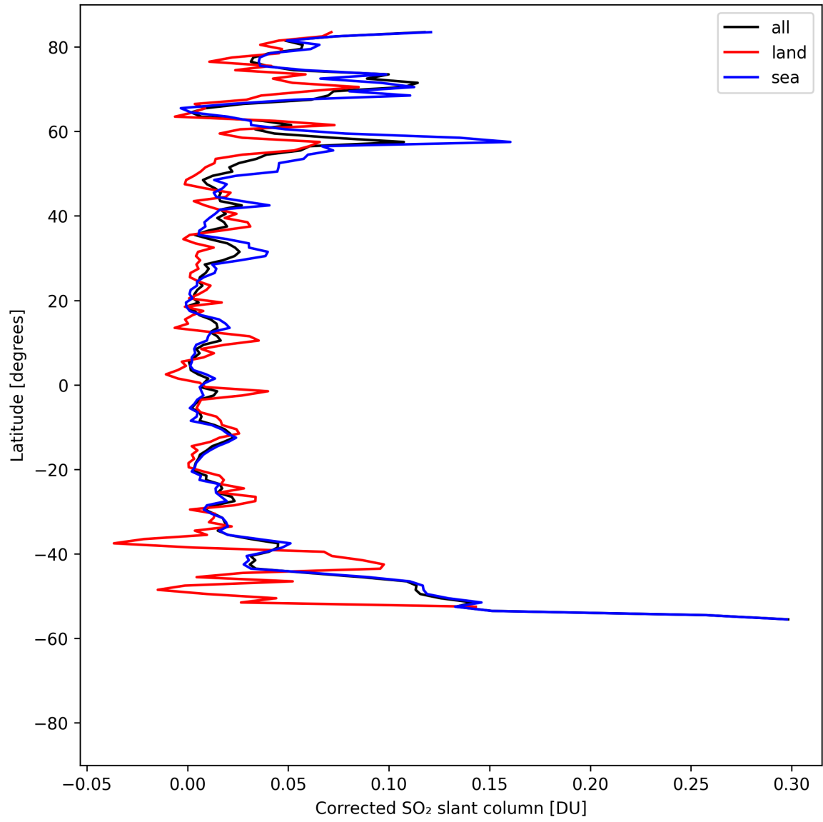
Figure 33: Zonal average of “Corrected SO 2 slant column” for 2025-08-15 to 2025-08-16.
