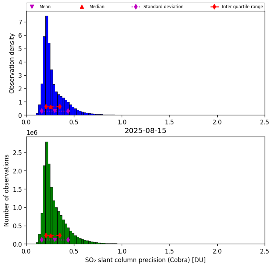
Figure 62: Histogram of “SO 2 slant column precision (Cobra)” for 2025-08-15 to 2025-08-16
