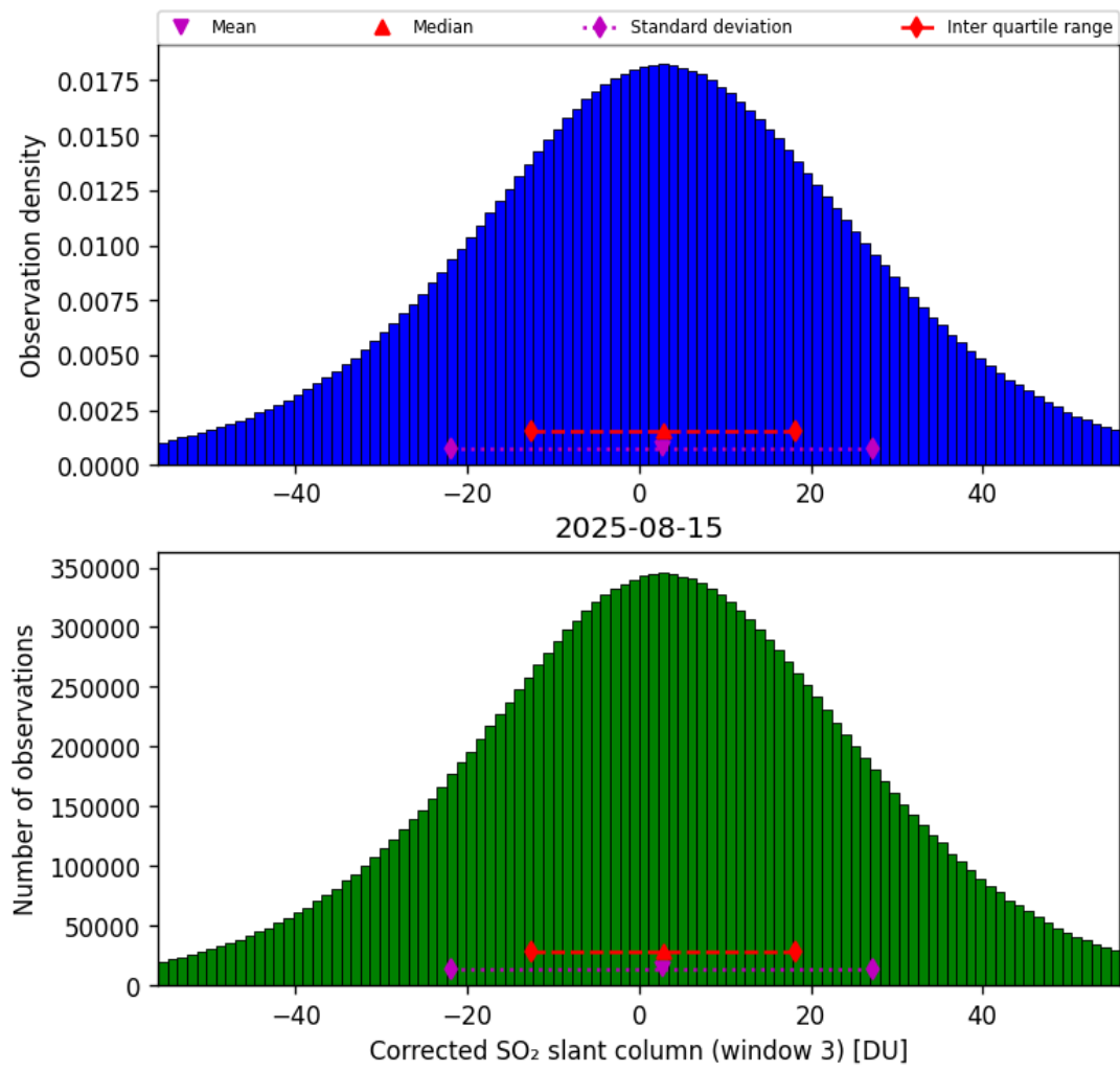
Figure 73: Histogram of “Corrected SO 2 slant column (window 3)” for 2025-08-15 to 2025-08-16
