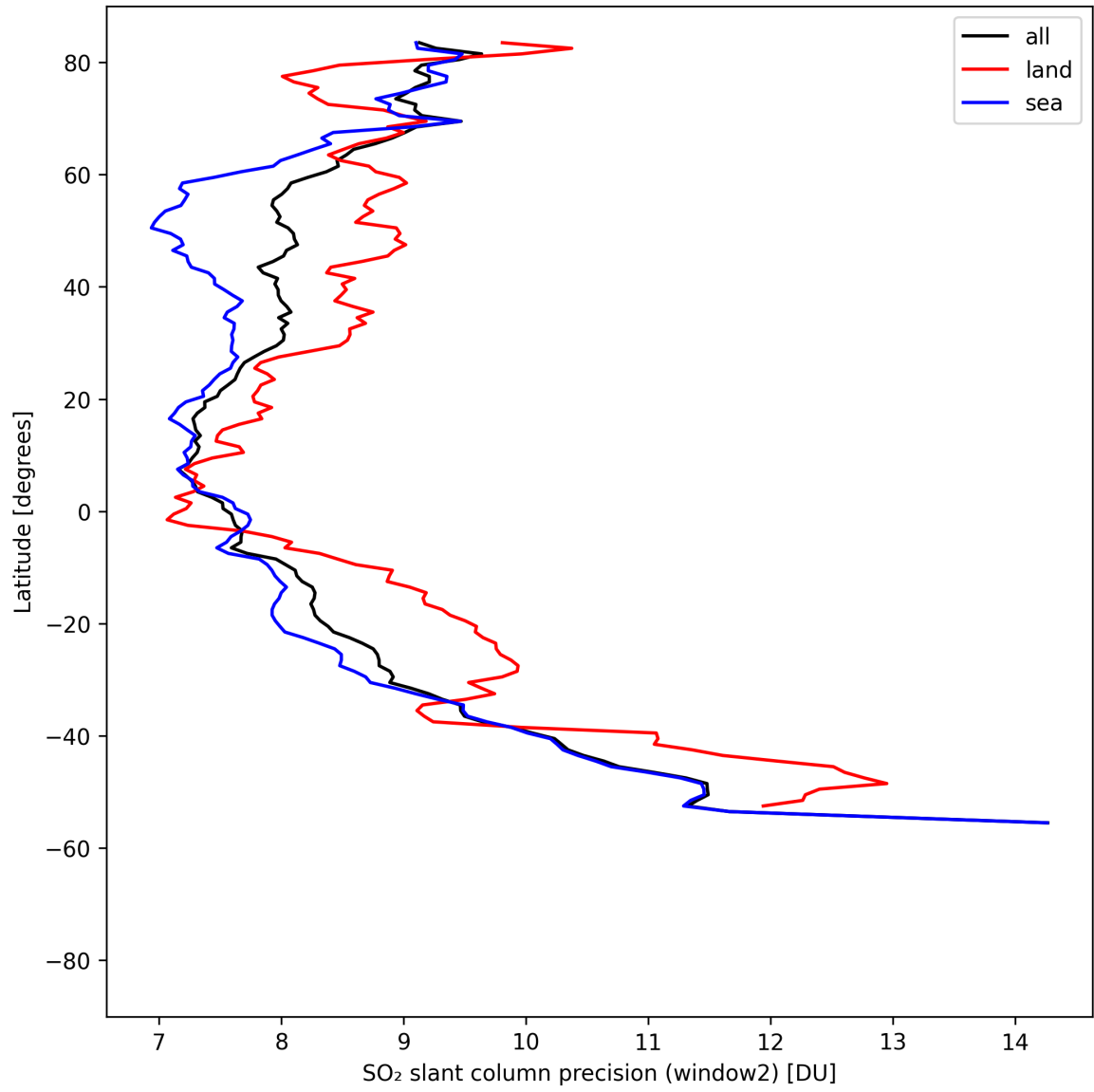
Figure 41: Zonal average of “SO 2 slant column precision (window2)” for 2025-08-15 to 2025-08-16.
