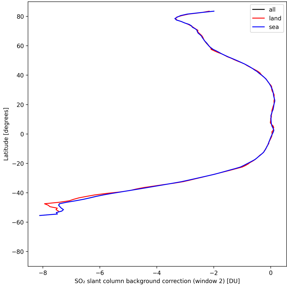
Figure 43: Zonal average of “SO 2 slant column background correction (window 2)” for 2025-08-15 to 2025-08-16.
