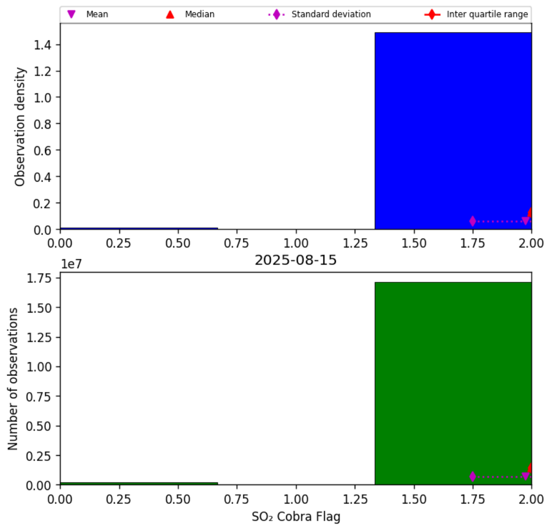
Figure 75: Histogram of “SO 2 Cobra Flag” for 2025-08-15 to 2025-08-16
