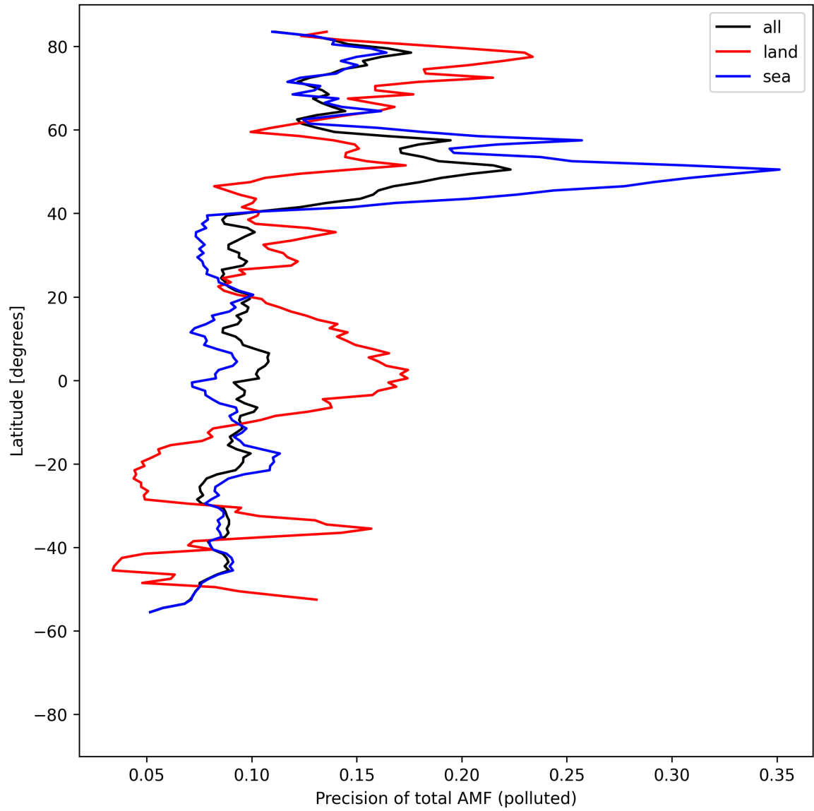
Figure 54: Zonal average of “Precision of total AMF (polluted)” for 2025-08-15 to 2025-08-16.
