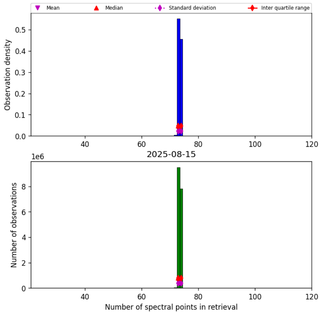
Figure 83: Histogram of “Number of spectral points in retrieval” for 2025-08-15 to 2025-08-16
