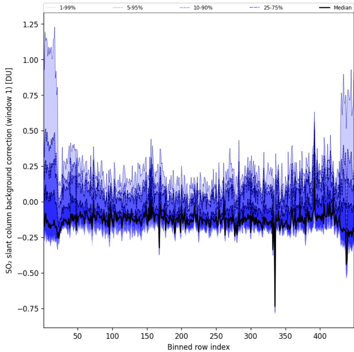
Figure 93: Along track statistics of “SO 2 slant column background correction (window 1)” for 2025-08-15 to 2025-08-16
