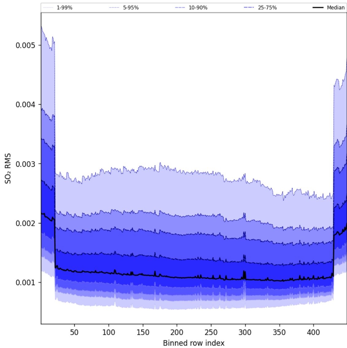
Figure 106: Along track statistics of “SO 2 RMS” for 2025-08-15 to 2025-08-16
