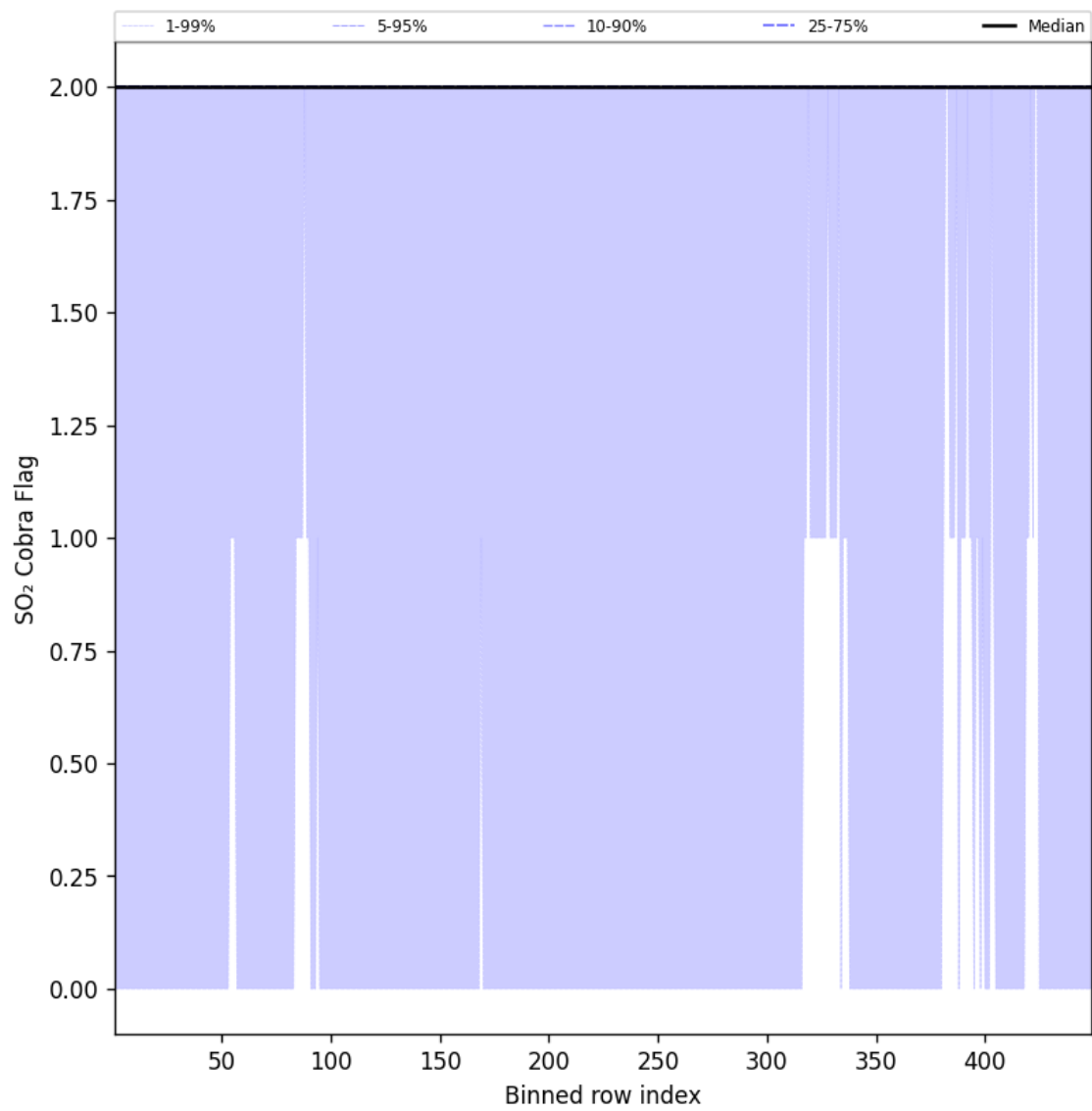
Figure 102: Along track statistics of “SO 2 Cobra Flag” for 2025-08-15 to 2025-08-16
