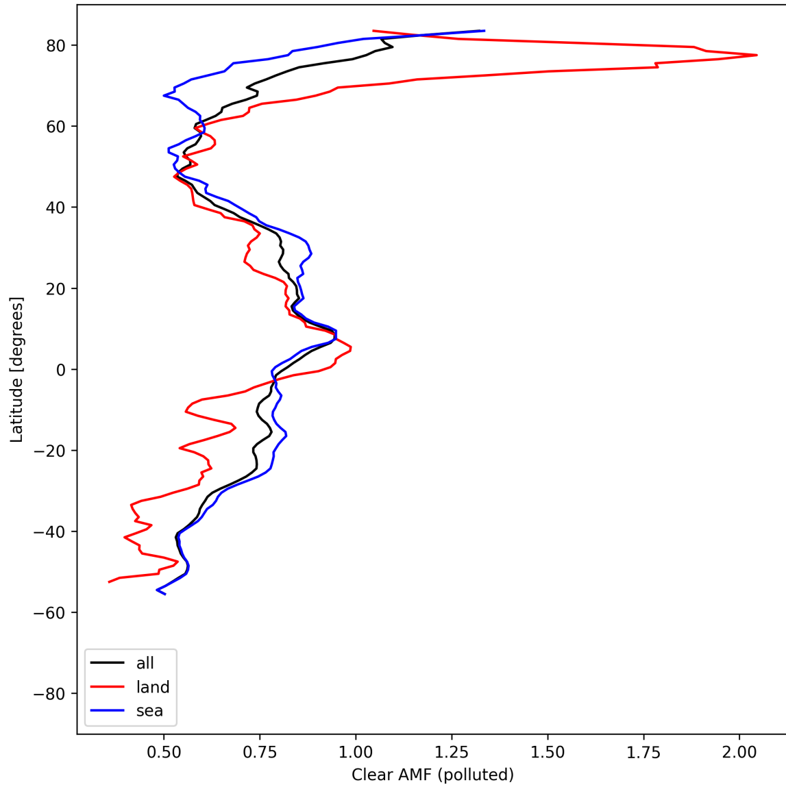
Figure 55: Zonal average of “Clear AMF (polluted)” for 2025-08-15 to 2025-08-16.
