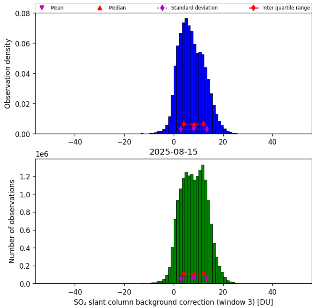
Figure 74: Histogram of “SO 2 slant column background correction (window 3)” for 2025-08-15 to 2025-08-16
