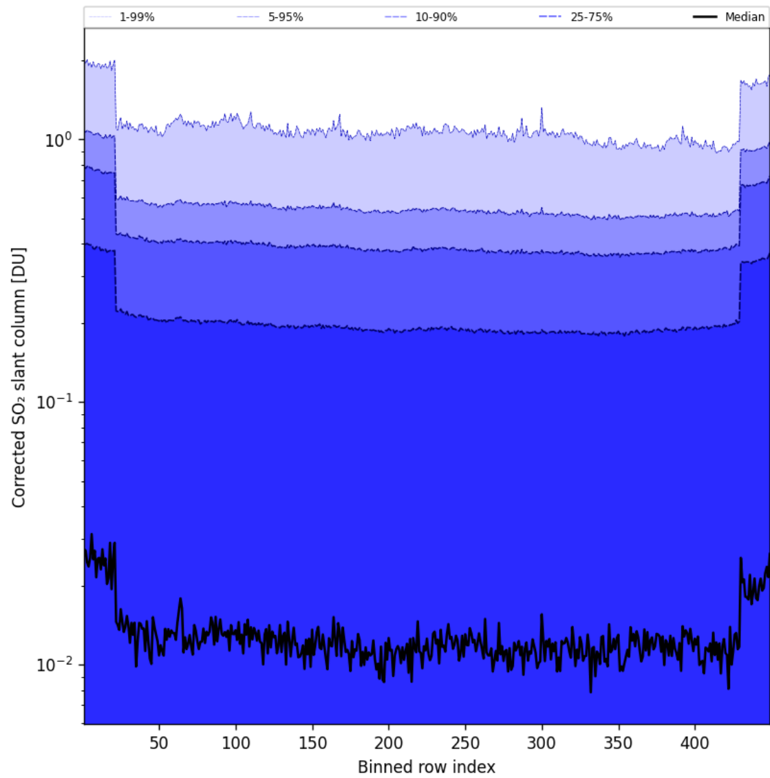
Figure 87: Along track statistics of “Corrected SO 2 slant column” for 2025-08-15 to 2025-08-16
