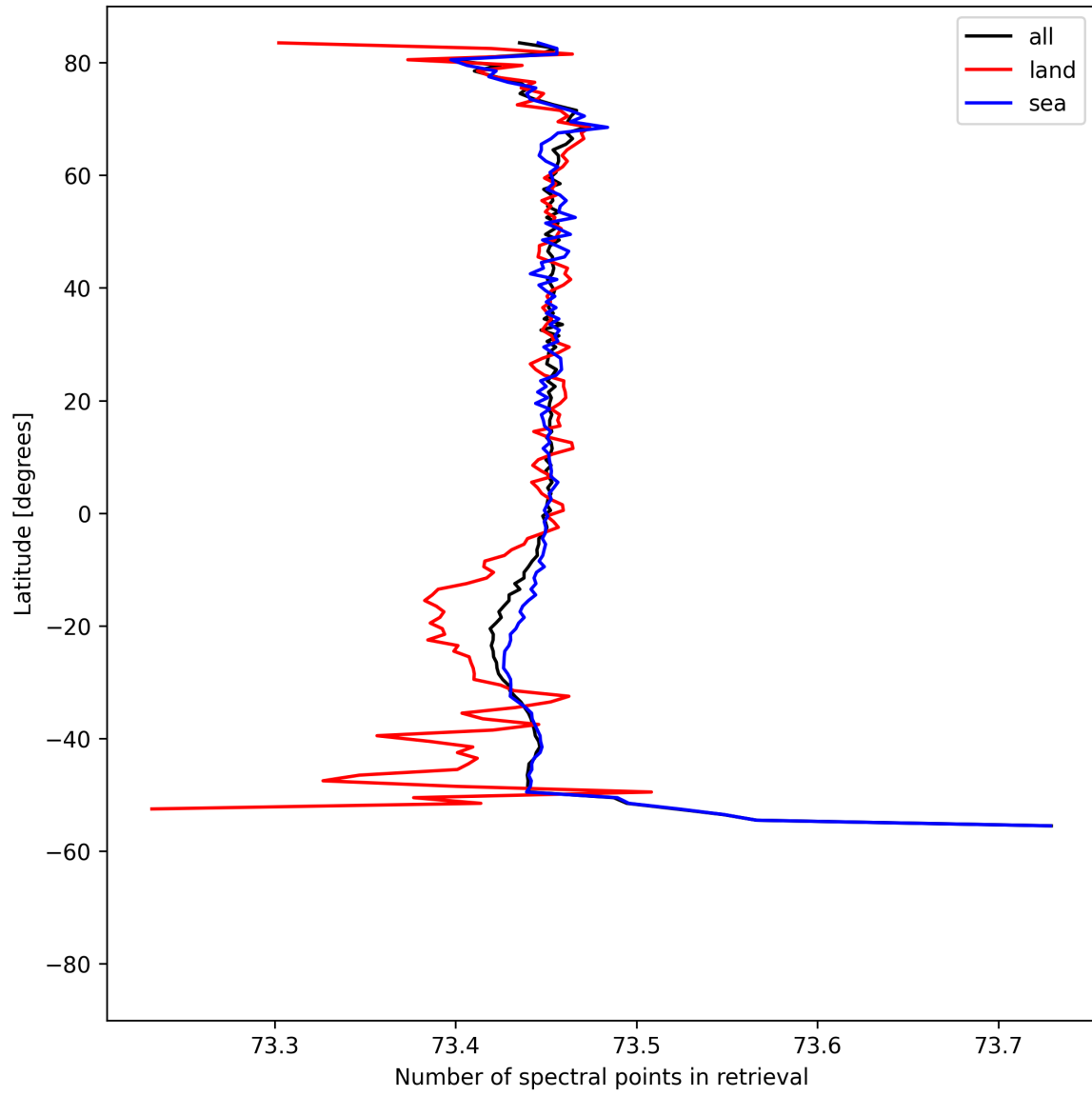
Figure 56: Zonal average of “Number of spectral points in retrieval” for 2025-08-15 to 2025-08-16.
