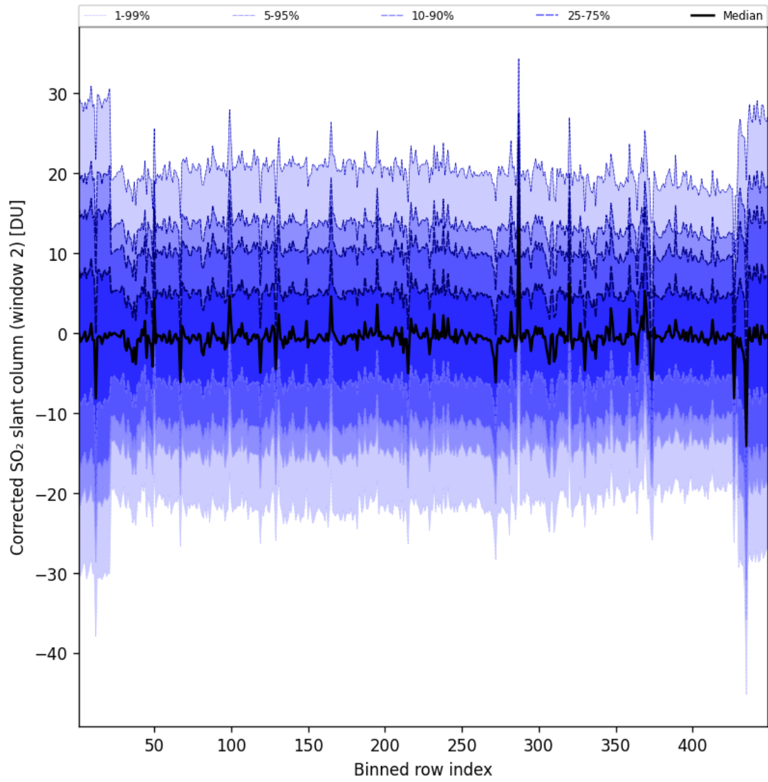
Figure 96: Along track statistics of “Corrected SO 2 slant column (window 2)” for 2025-08-15 to 2025-08-16
