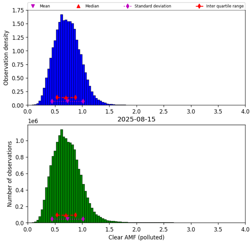
Figure 82: Histogram of “Clear AMF (polluted)” for 2025-08-15 to 2025-08-16
