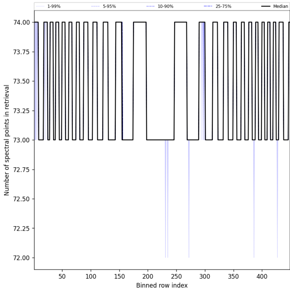
Figure 110: Along track statistics of “Number of spectral points in retrieval” for 2025-08-15 to 2025-08-16
