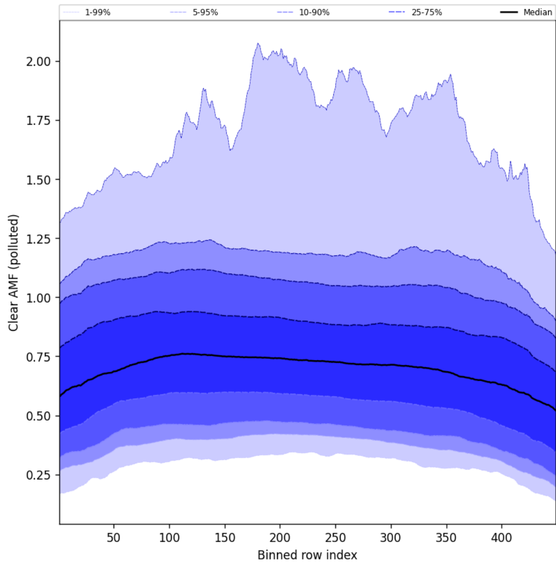
Figure 109: Along track statistics of “Clear AMF (polluted)” for 2025-08-15 to 2025-08-16
