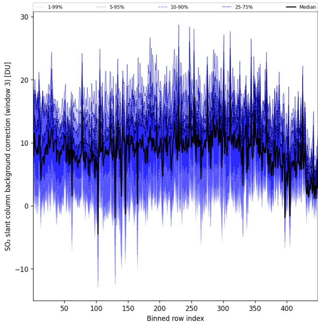
Figure 101: Along track statistics of “SO 2 slant column background correction (window 3)” for 2025-08-15 to 2025-08-16
