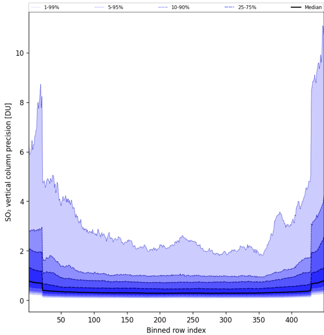
Figure 86: Along track statistics of “SO 2 vertical column precision” for 2025-08-15 to 2025-08-16
