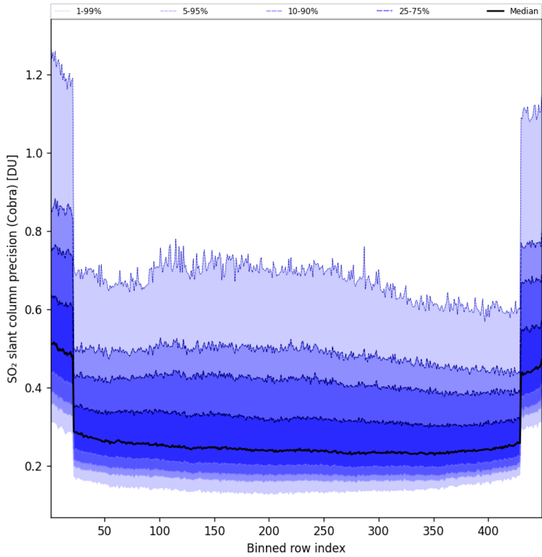
Figure 89: Along track statistics of “SO 2 slant column precision (Cobra)” for 2025-08-15 to 2025-08-16
