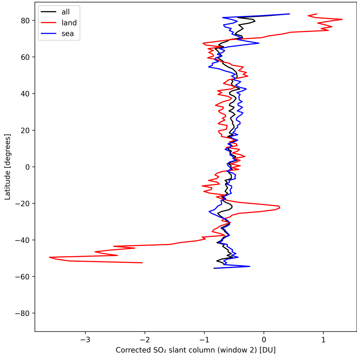
Figure 42: Zonal average of "Corrected SO 2 slant column (window 2)" for 2025-08-15 to 2025-08-16.
