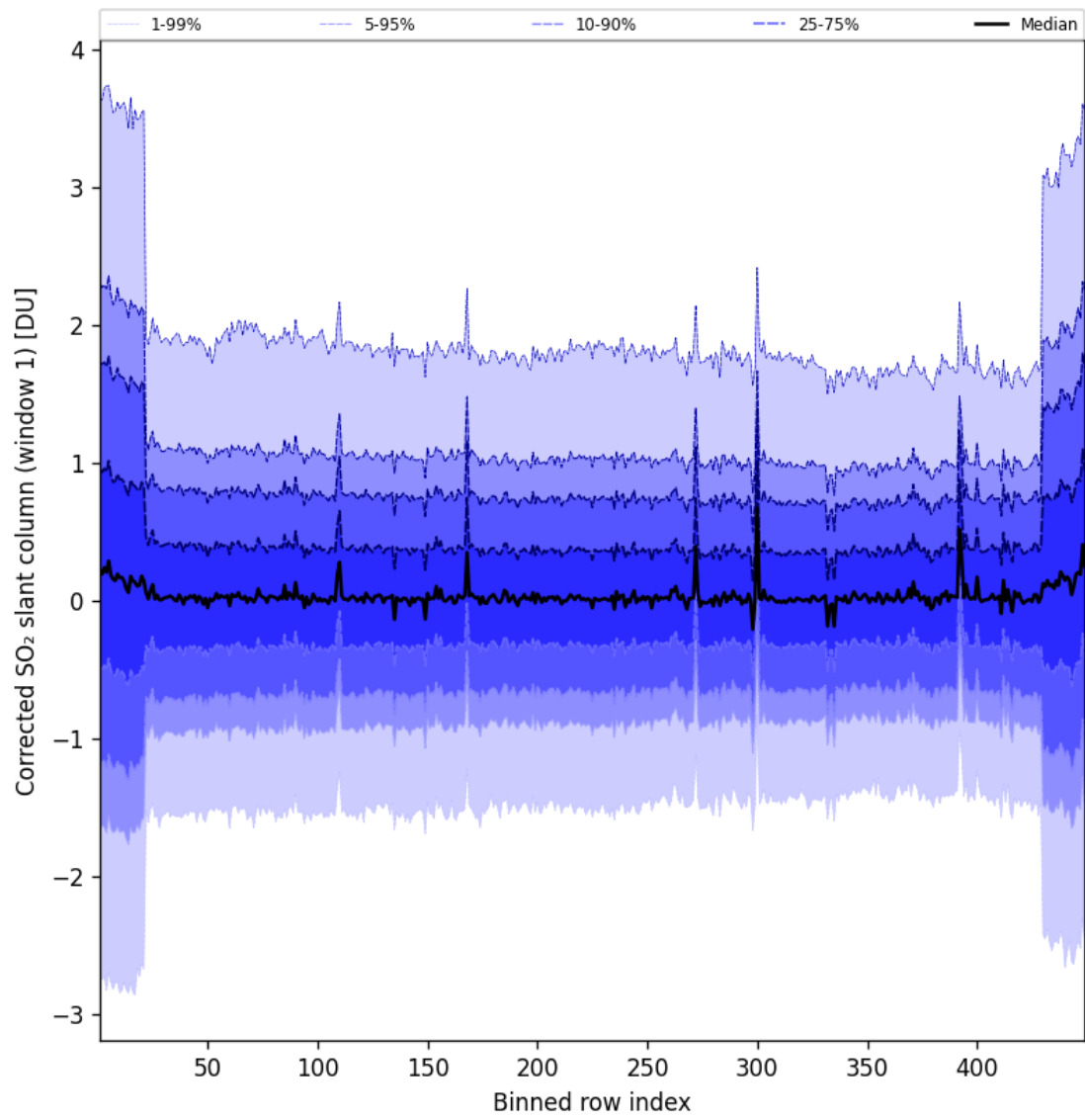
Figure 92: Along track statistics of “Corrected SO 2 slant column (window 1)” for 2025-08-15 to 2025-08-16
