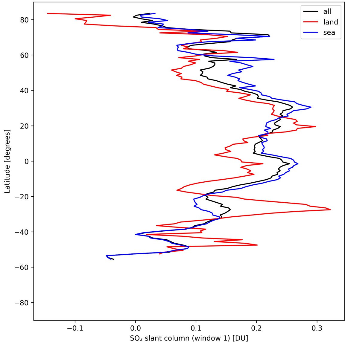
Figure 36: Zonal average of “SO 2 slant column (window 1)” for 2025-08-15 to 2025-08-16.
