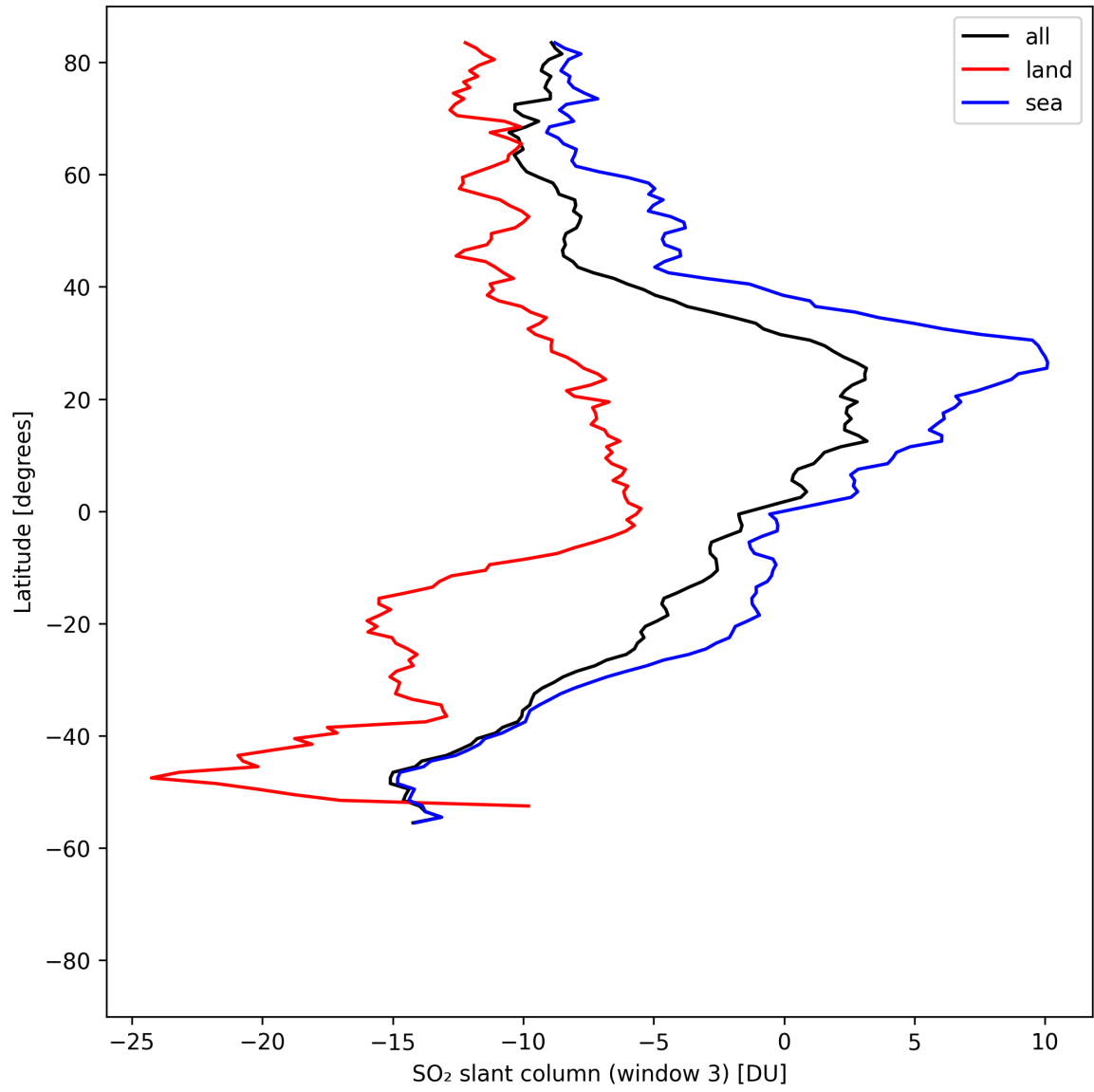
Figure 44: Zonal average of “SO 2 slant column (window 3)” for 2025-08-15 to 2025-08-16.
