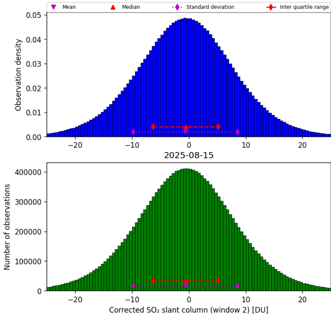
Figure 69: Histogram of “Corrected SO 2 slant column (window 2)” for 2025-08-15 to 2025-08-16
