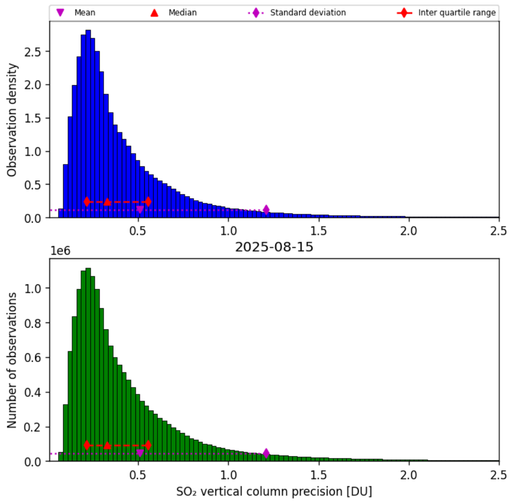
Figure 59: Histogram of “SO 2 vertical column precision” for 2025-08-15 to 2025-08-16
