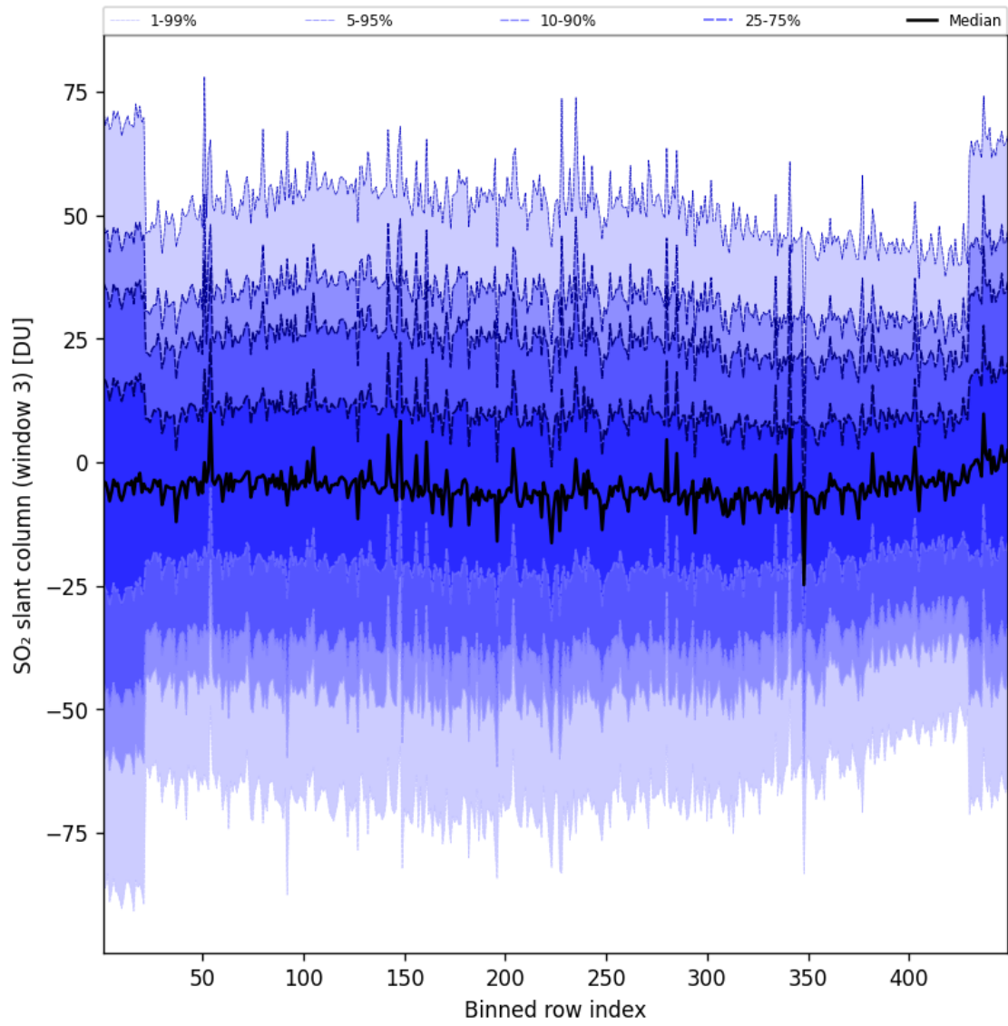
Figure 98: Along track statistics of “SO 2 slant column (window 3)” for 2025-08-15 to 2025-08-16
