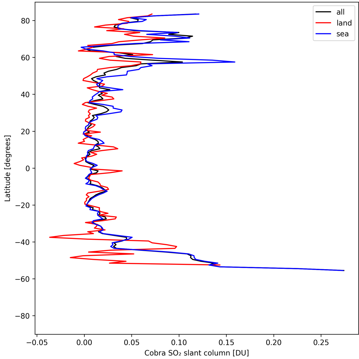
Figure 34: Zonal average of “Cobra SO 2 slant column” for 2025-08-15 to 2025-08-16.
