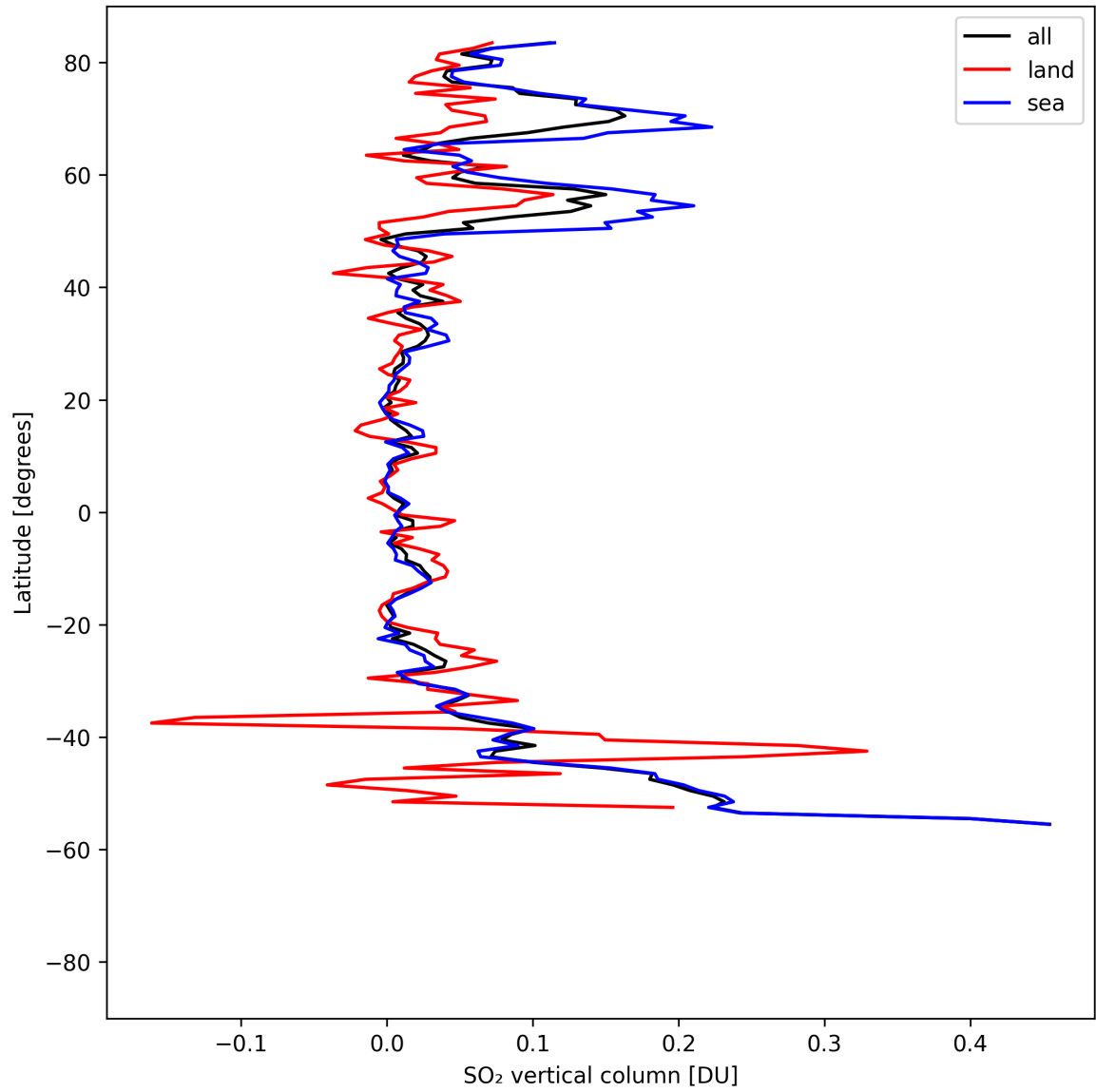
Figure 31: Zonal average of “SO 2 vertical column” for 2025-08-15 to 2025-08-16.
