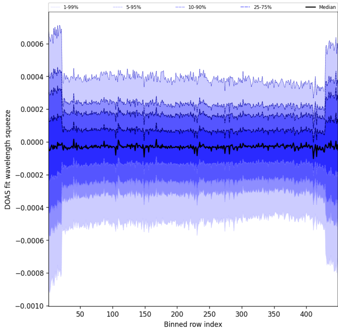
Figure 105: Along track statistics of “DOAS fit wavelength squeeze” for 2025-08-15 to 2025-08-16
