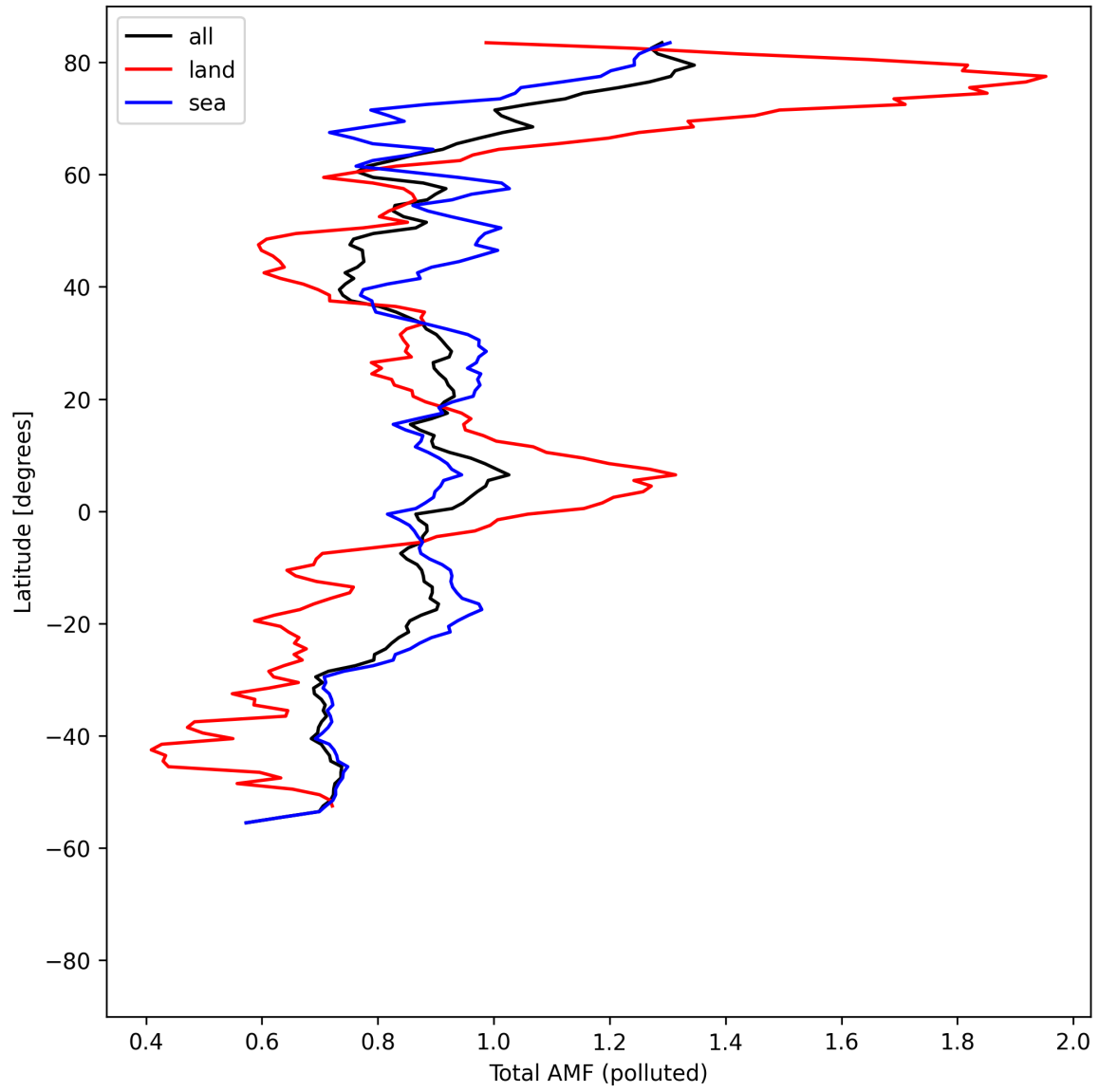
Figure 53: Zonal average of “Total AMF (polluted)” for 2025-08-15 to 2025-08-16.
