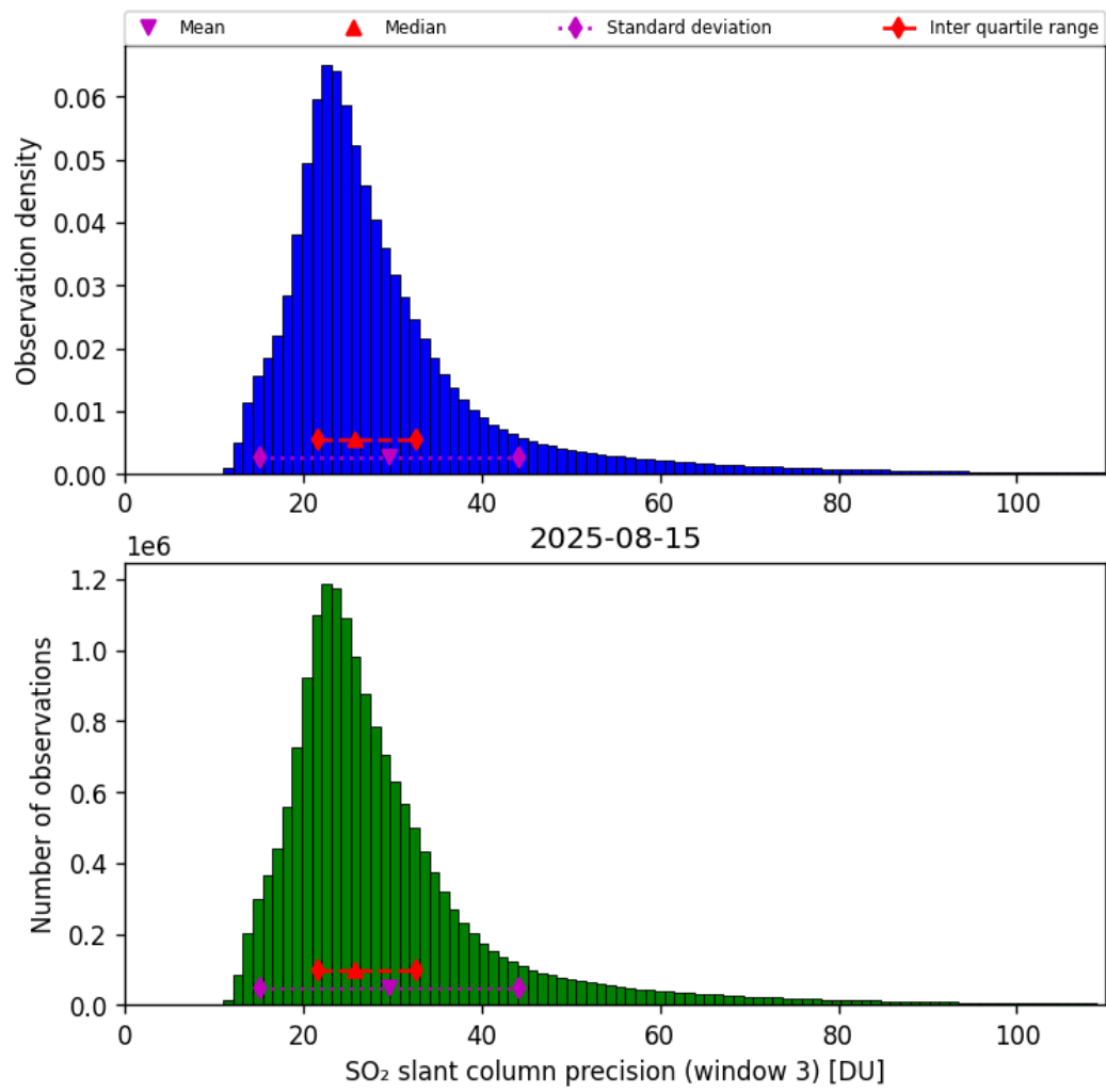
Figure 72: Histogram of “SO 2 slant column precision (window 3)” for 2025-08-15 to 2025-08-16
