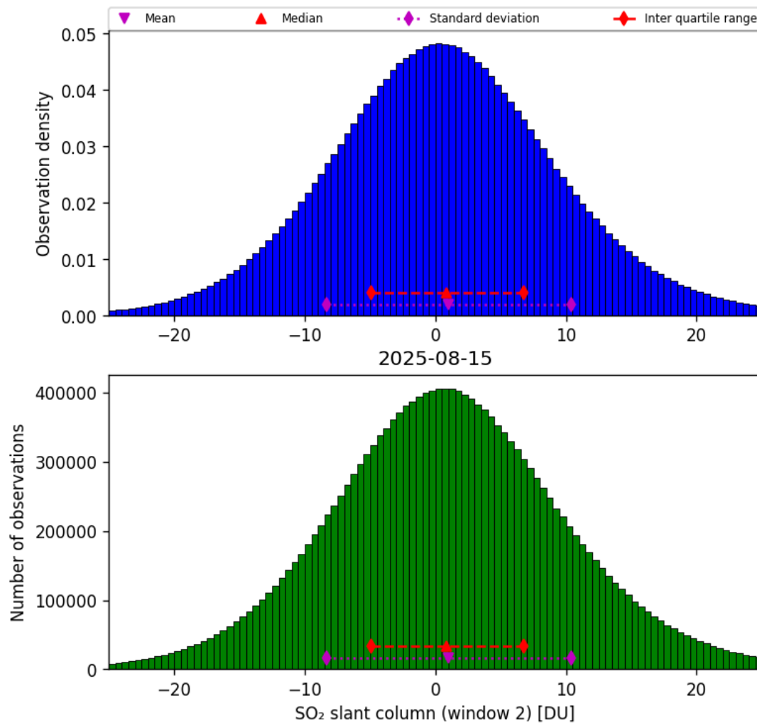
Figure 67: Histogram of “SO 2 slant column (window 2)” for 2025-08-15 to 2025-08-16
