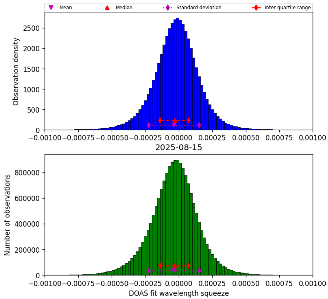
Figure 78: Histogram of “DOAS fit wavelength squeeze” for 2025-08-15 to 2025-08-16
