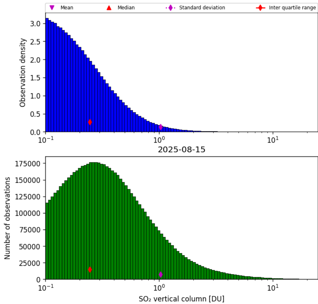
Figure 58: Histogram of “SO 2 vertical column” for 2025-08-15 to 2025-08-16
