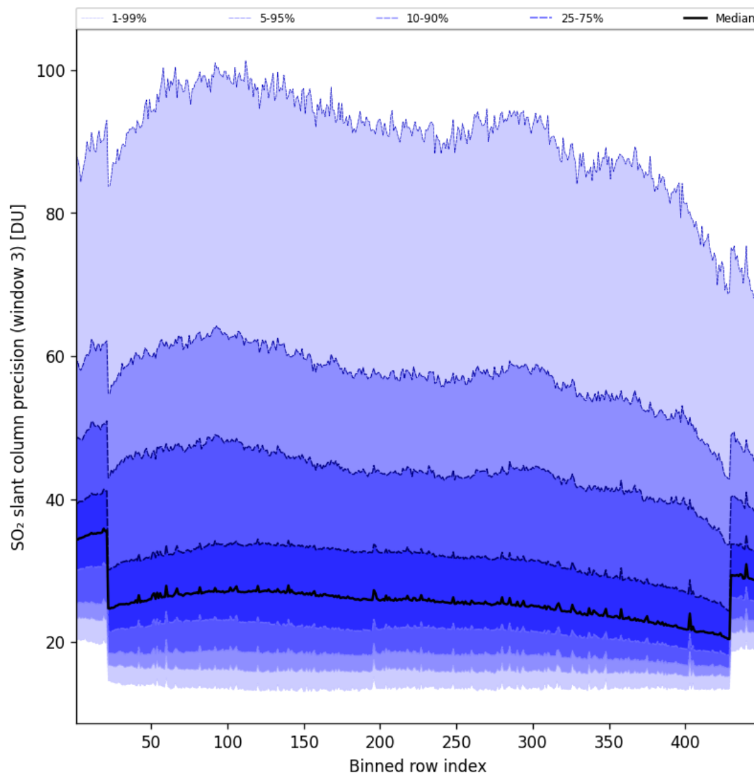
Figure 99: Along track statistics of “SO 2 slant column precision (window 3)” for 2025-08-15 to 2025-08-16
