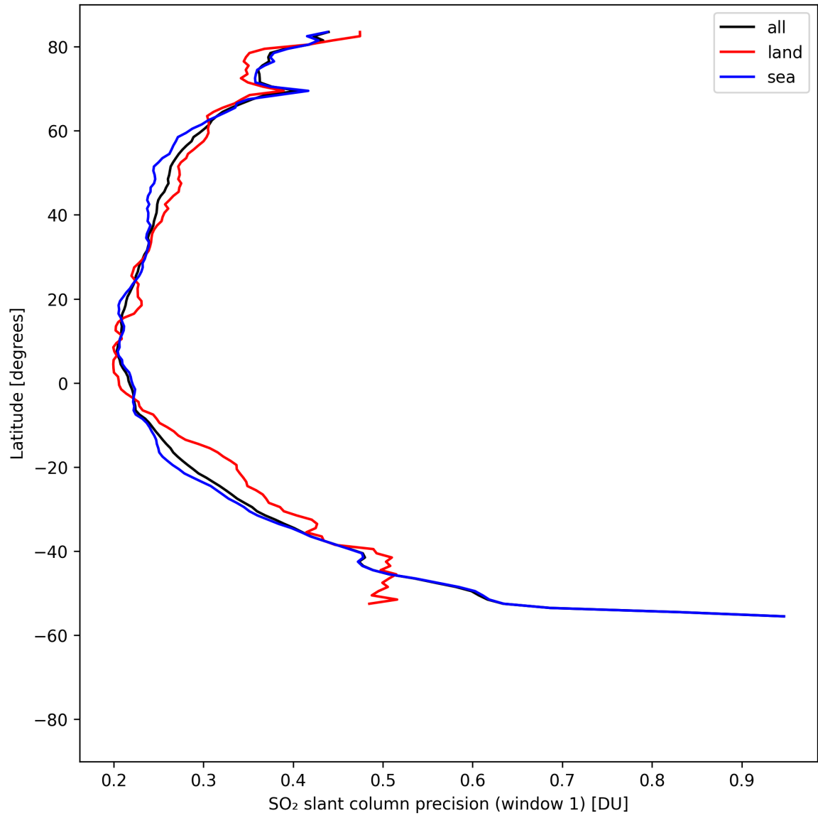
Figure 37: Zonal average of “SO 2 slant column precision (window 1)” for 2025-08-15 to 2025-08-16.
