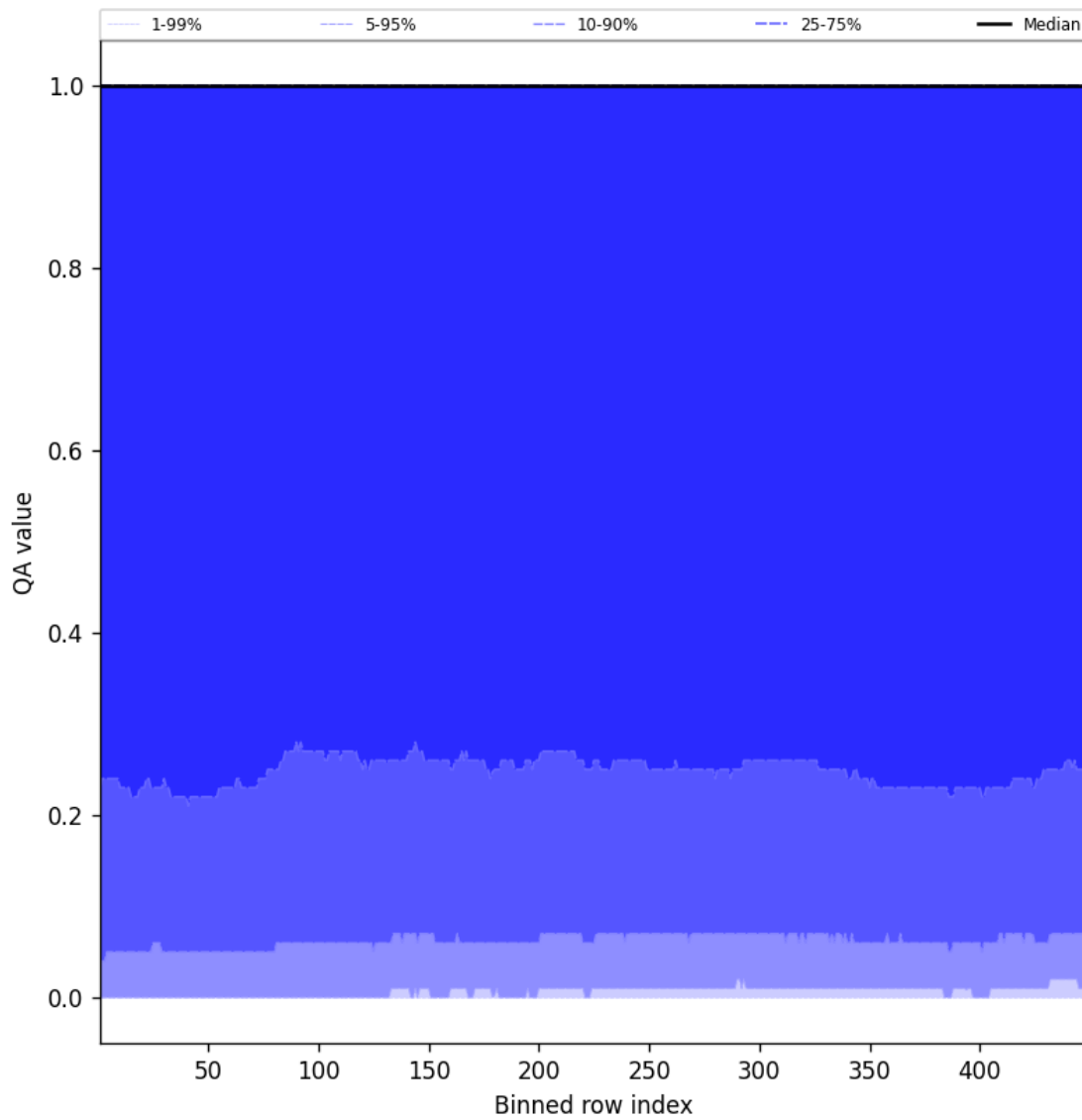
Figure 84: Along track statistics of “QA value” for 2025-08-15 to 2025-08-16
