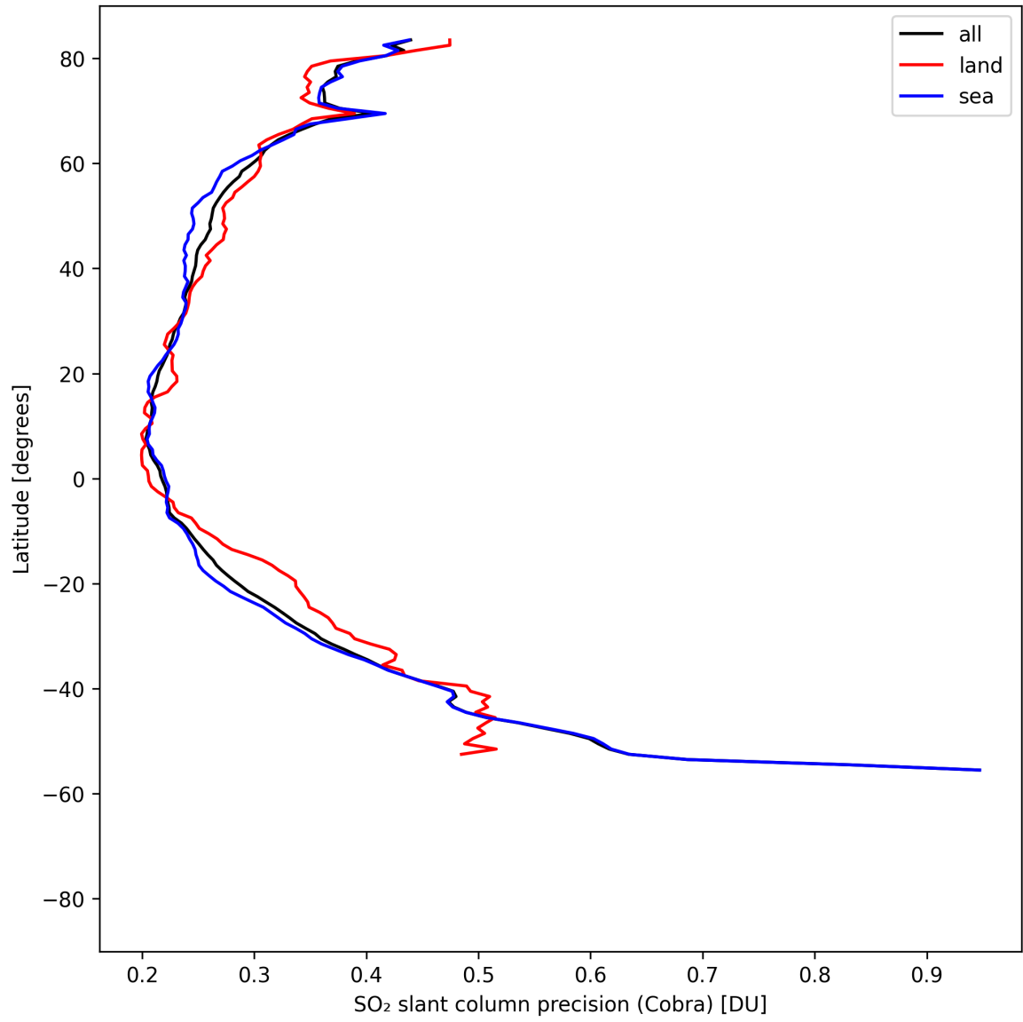
Figure 35: Zonal average of “SO 2 slant column precision (Cobra)” for 2025-08-15 to 2025-08-16.
