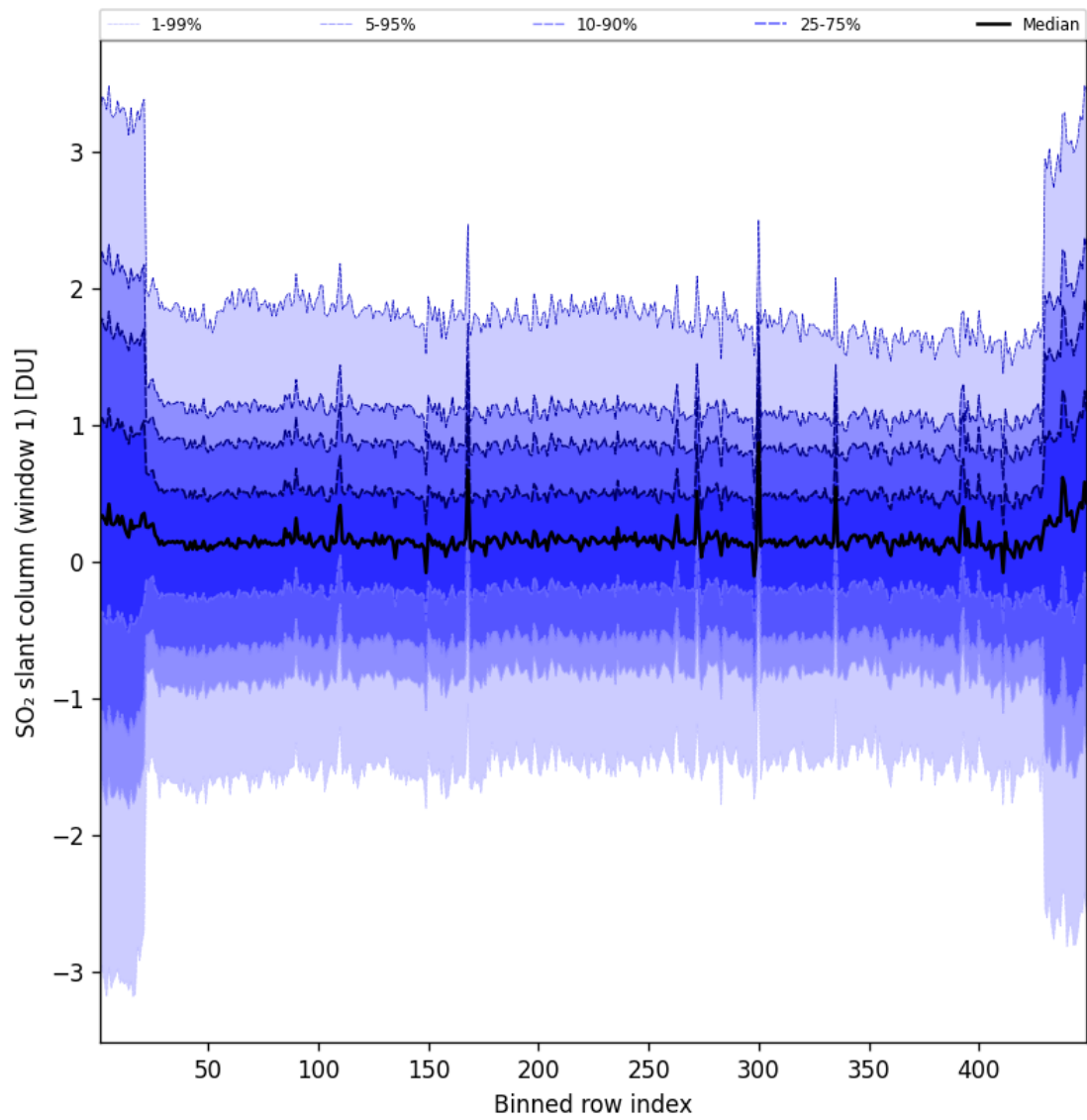
Figure 90: Along track statistics of “SO 2 slant column (window 1)” for 2025-08-15 to 2025-08-16
