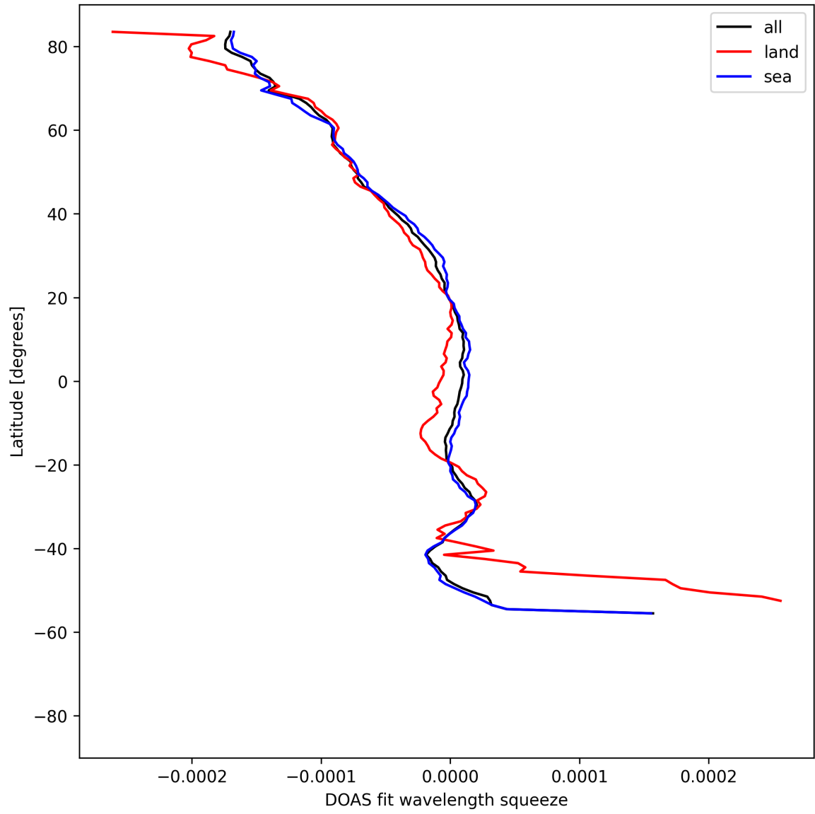
Figure 51: Zonal average of “DOAS fit wavelength squeeze” for 2025-08-15 to 2025-08-16.
