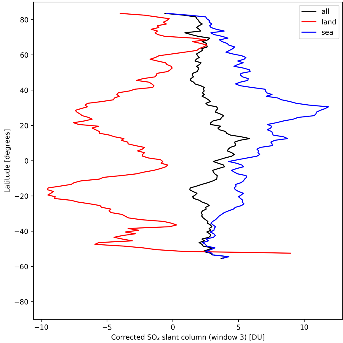
Figure 46: Zonal average of “Corrected SO 2 slant column (window 3)” for 2025-08-15 to 2025-08-16.
