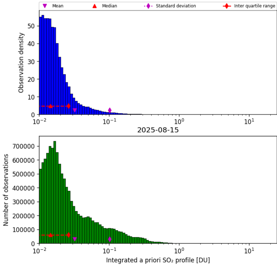
Figure 76: Histogram of “Integrated a priori SO 2 profile” for 2025-08-15 to 2025-08-16
