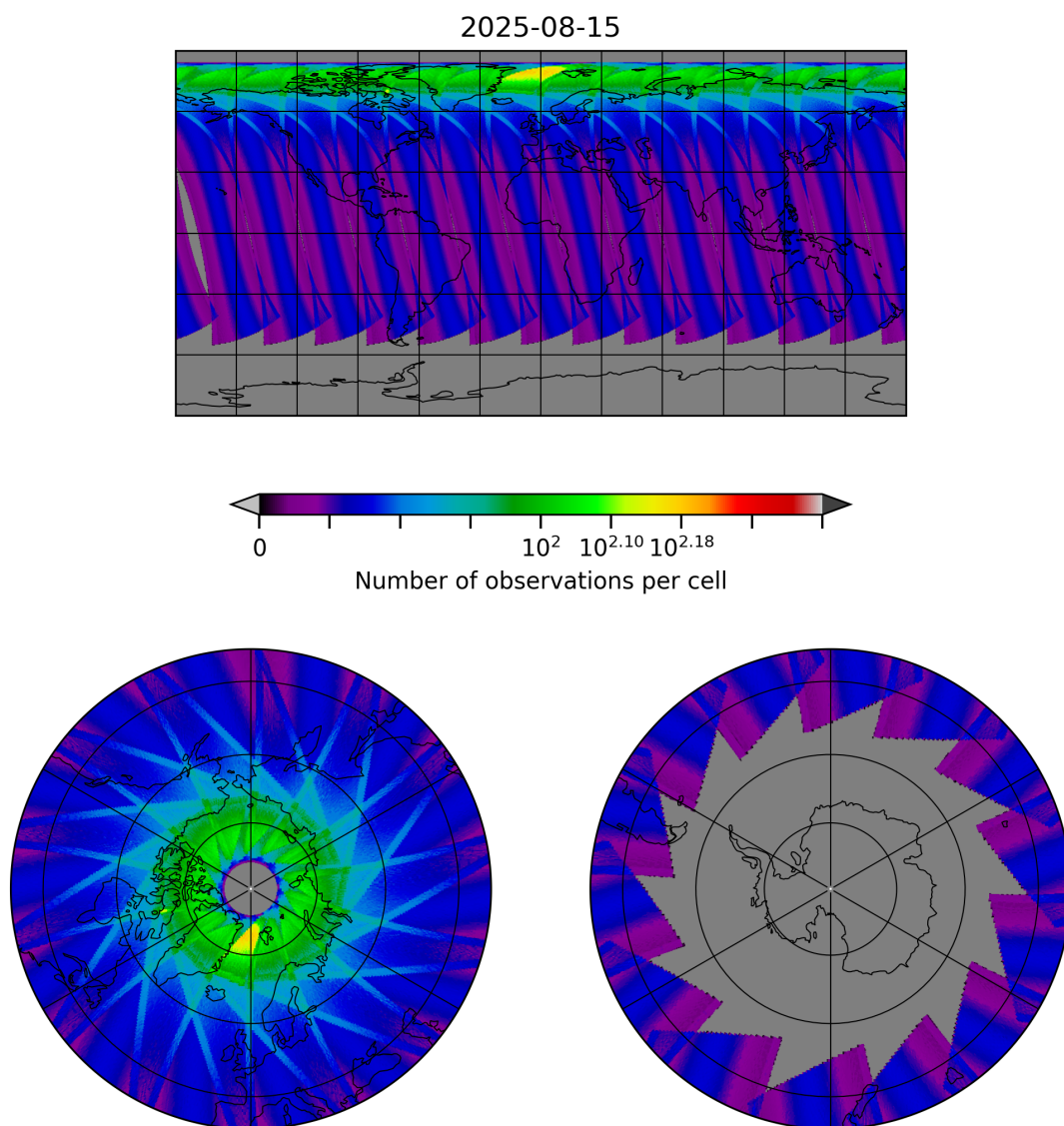
Figure 29: Map of the number of observations for 2025-08-15 to 2025-08-16
