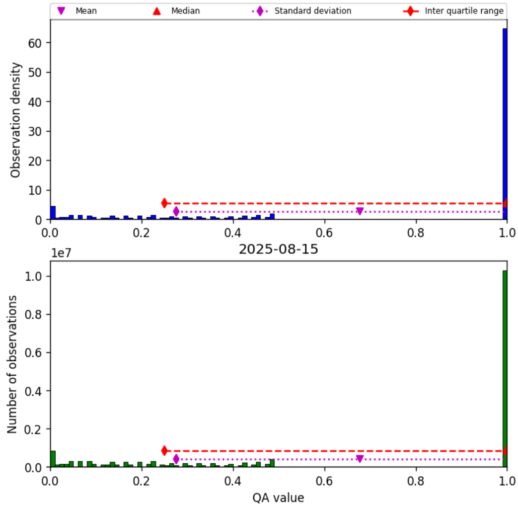
Figure 57: Histogram of “QA value” for 2025-08-15 to 2025-08-16
