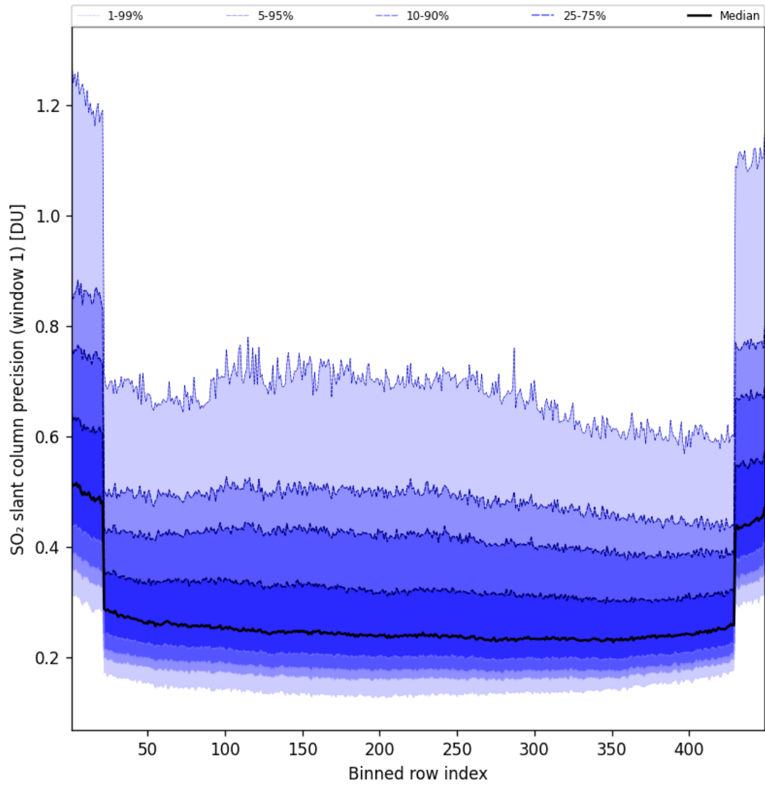
Figure 91: Along track statistics of “SO 2 slant column precision (window 1)” for 2025-08-15 to 2025-08-16
