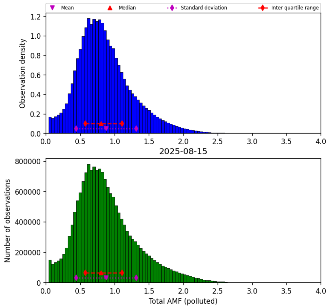
Figure 80: Histogram of “Total AMF (polluted)” for 2025-08-15 to 2025-08-16
