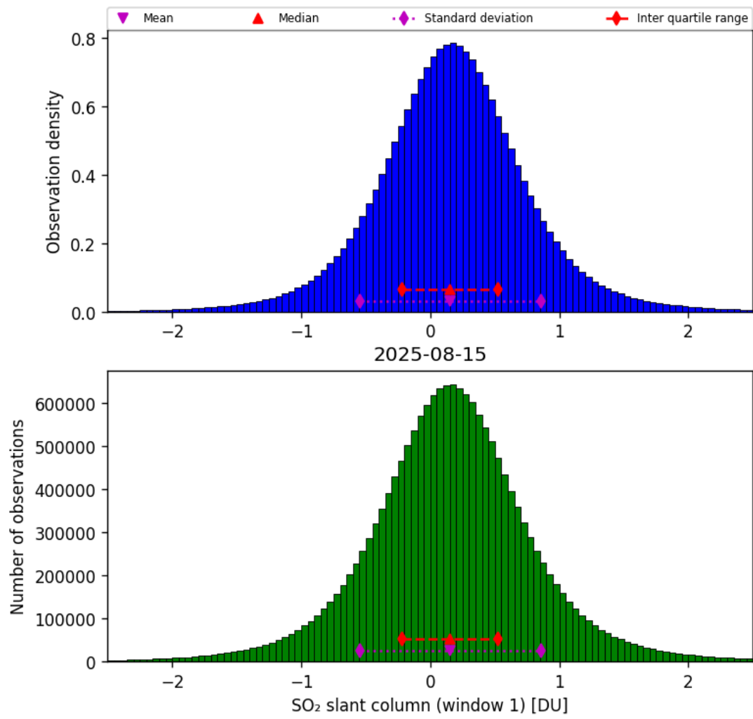
Figure 63: Histogram of “SO 2 slant column (window 1)” for 2025-08-15 to 2025-08-16
