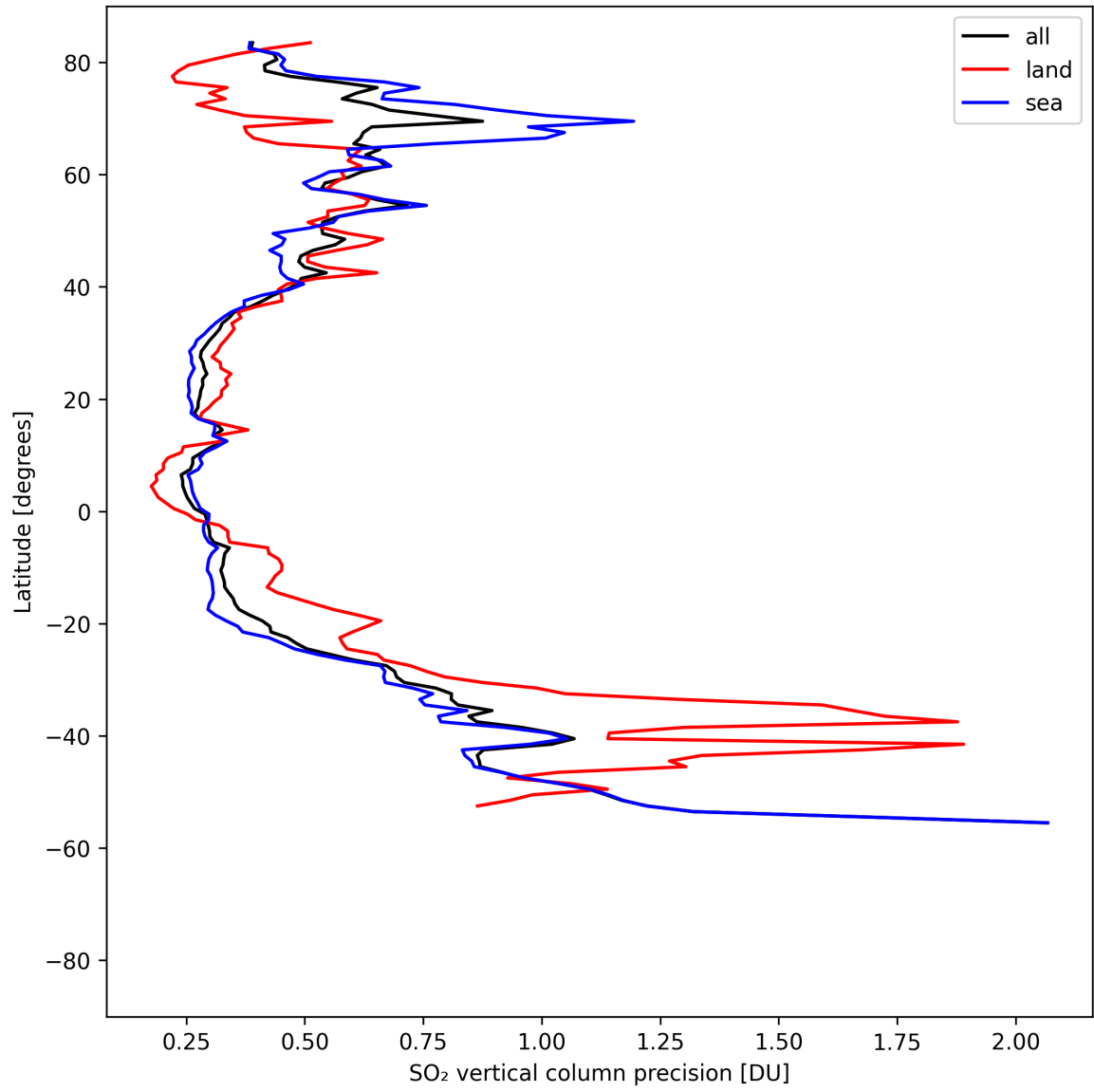
Figure 32: Zonal average of “SO 2 vertical column precision” for 2025-08-15 to 2025-08-16.
