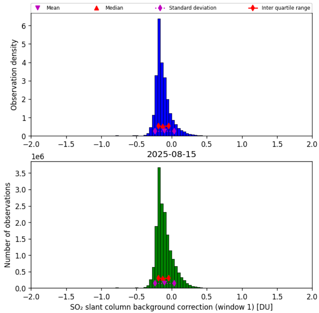
Figure 66: Histogram of “SO 2 slant column background correction (window 1)” for 2025-08-15 to 2025-08-16
