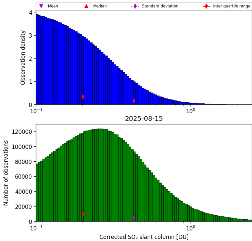
Figure 60: Histogram of “Corrected SO 2 slant column” for 2025-08-15 to 2025-08-16
