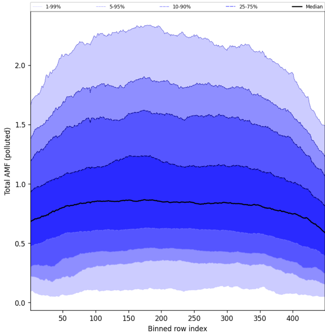
Figure 107: Along track statistics of “Total AMF (polluted)” for 2025-08-15 to 2025-08-16
