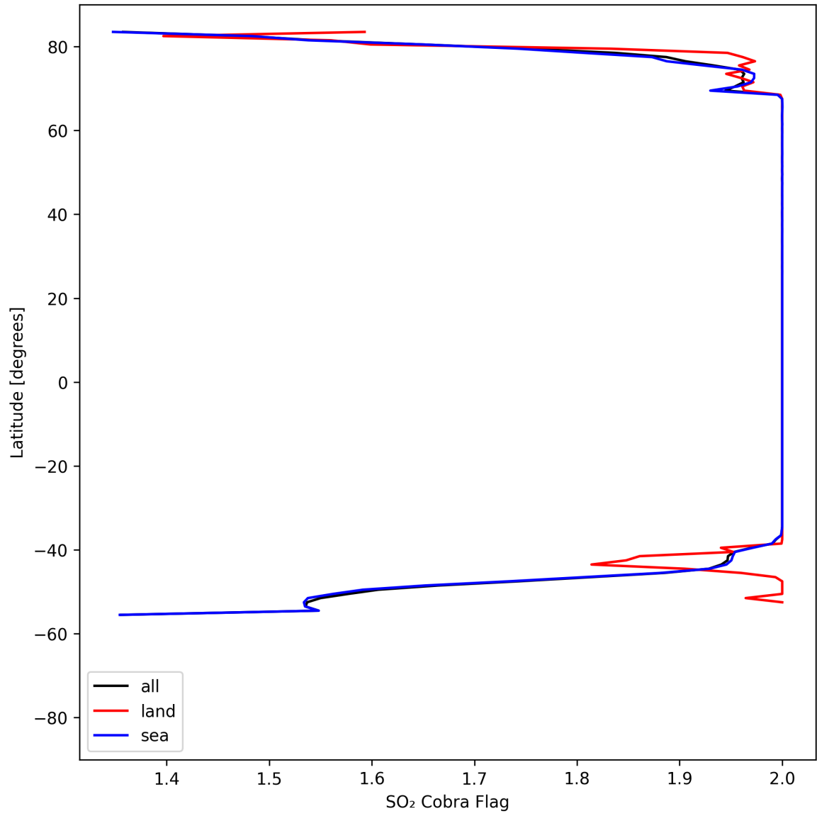
Figure 48: Zonal average of "SO 2 Cobra Flag" for 2025-08-15 to 2025-08-16.
