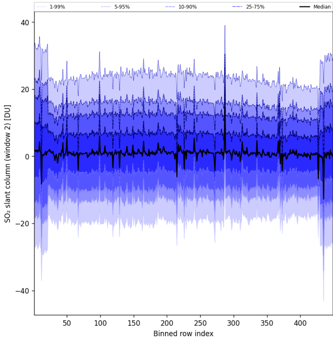
Figure 94: Along track statistics of “SO 2 slant column (window 2)” for 2025-08-15 to 2025-08-16
