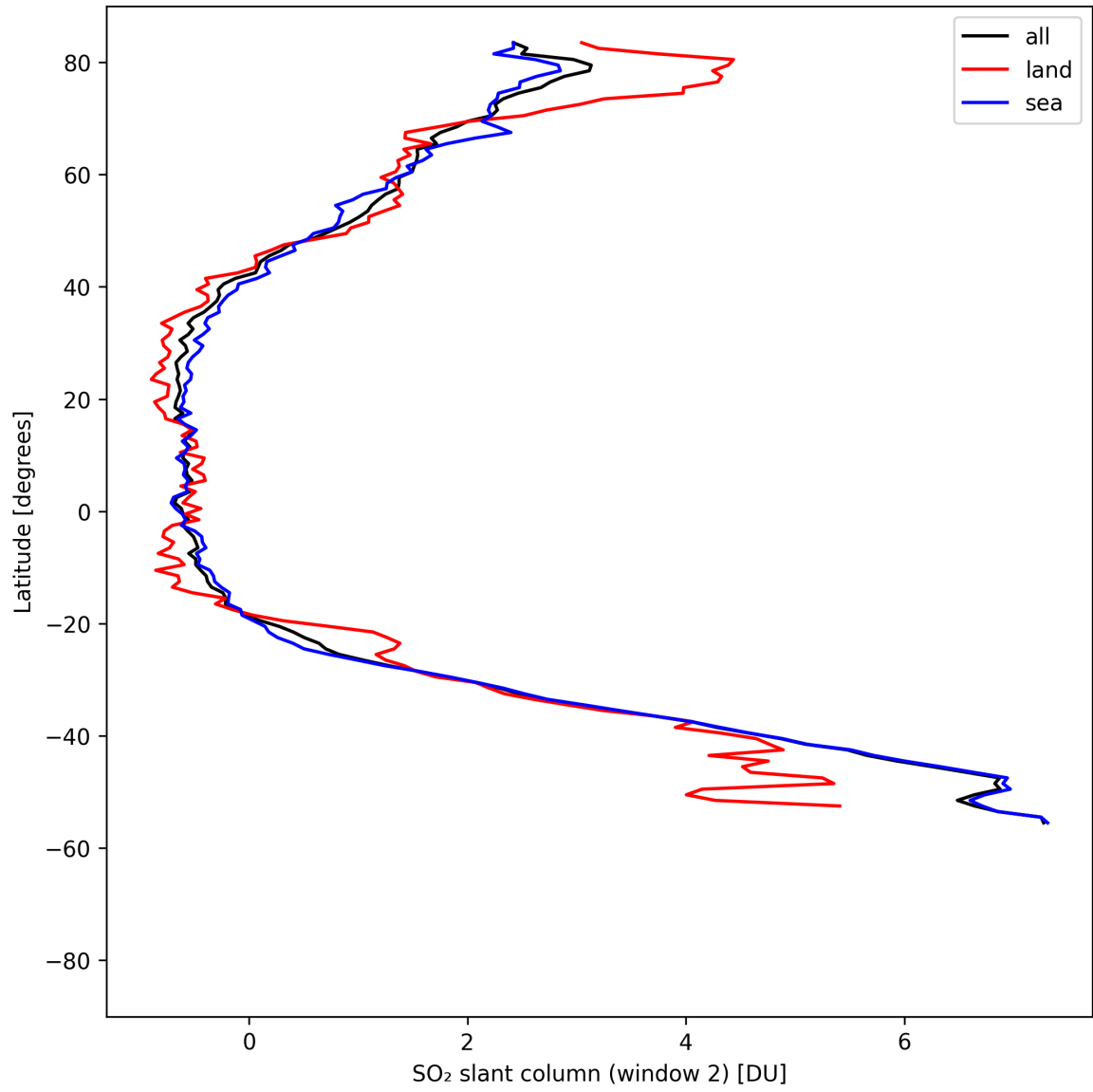
Figure 40: Zonal average of “SO 2 slant column (window 2)” for 2025-08-15 to 2025-08-16.
