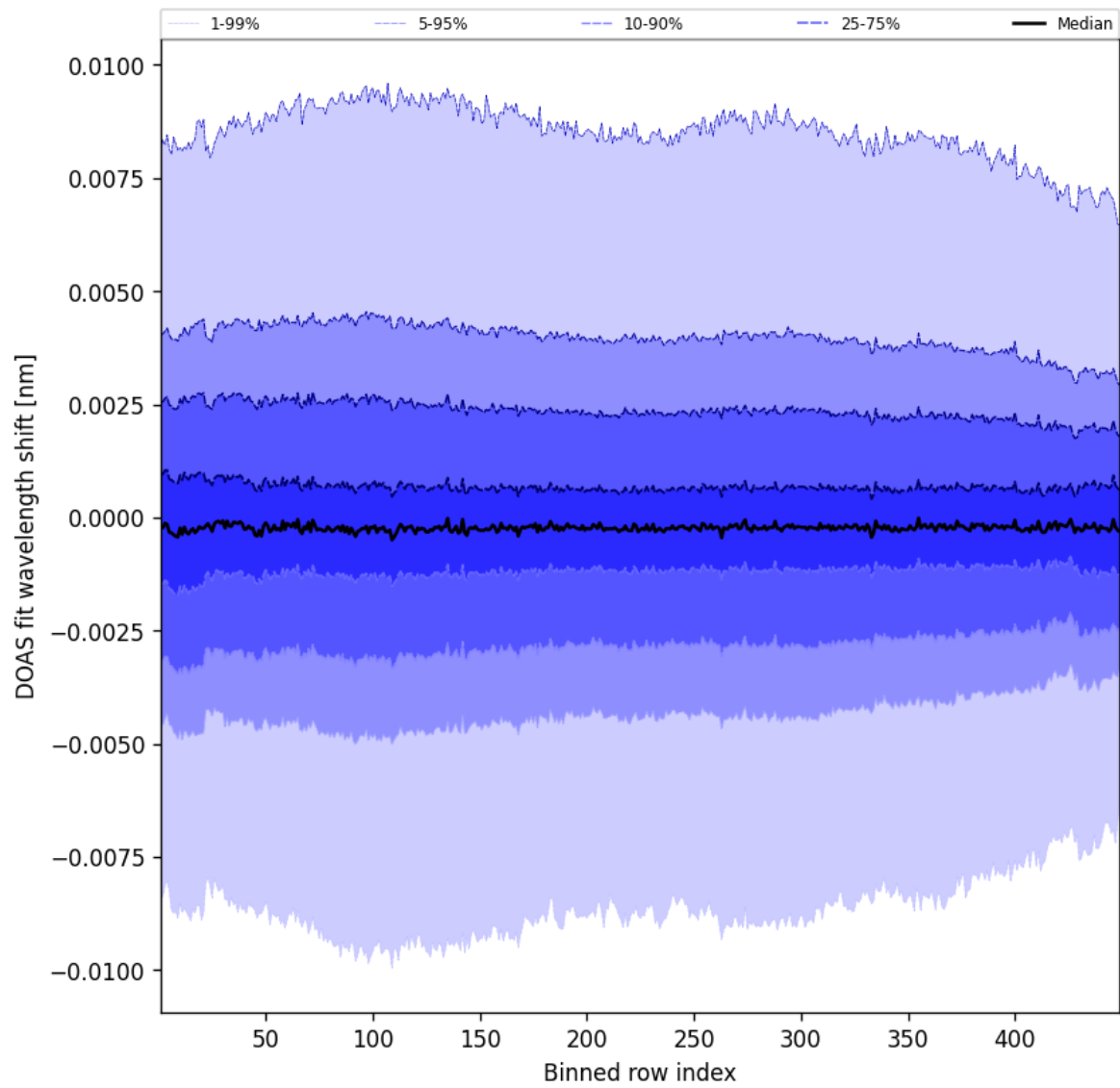
Figure 104: Along track statistics of “DOAS fit wavelength shift” for 2025-08-15 to 2025-08-16
