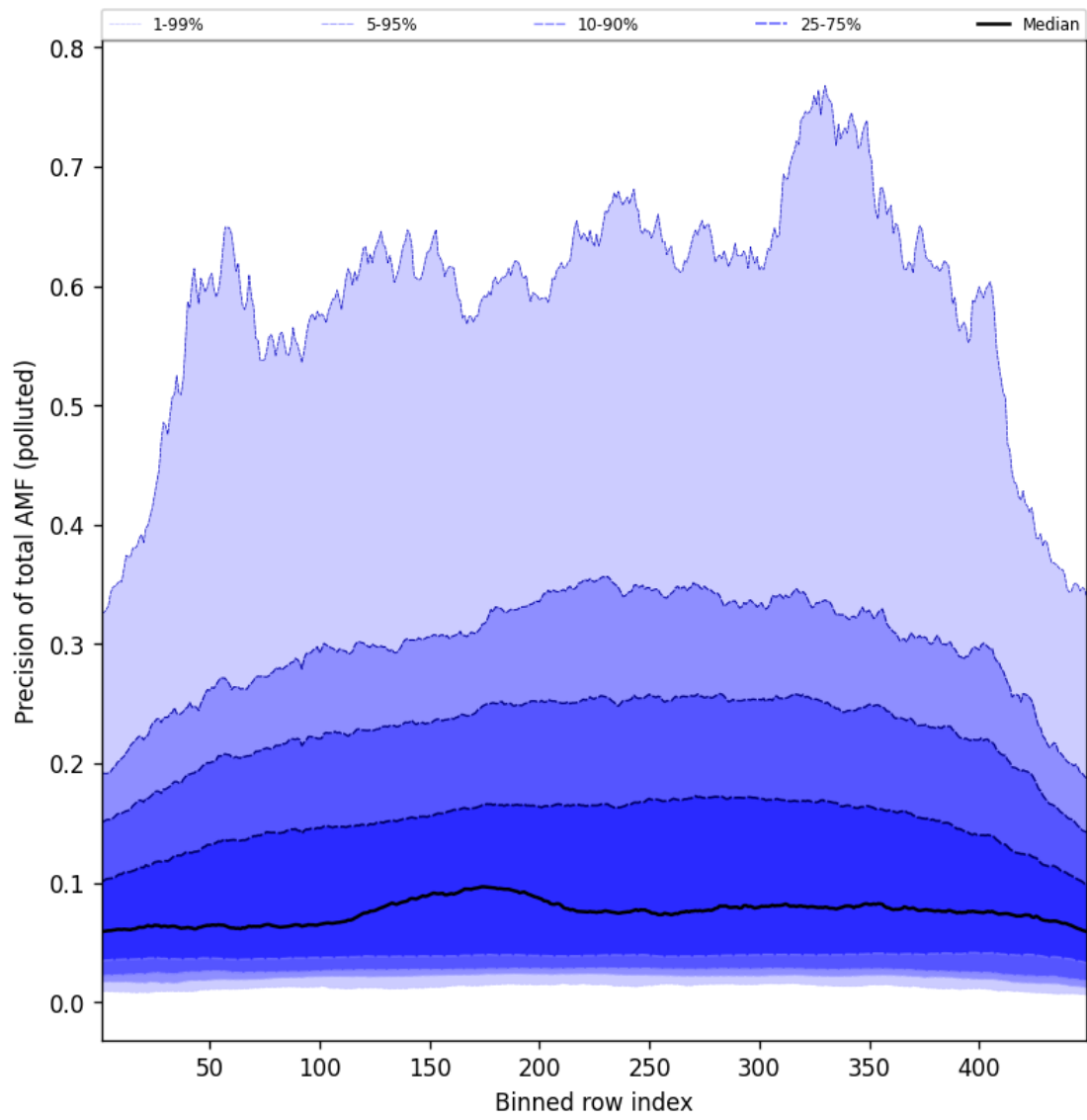
Figure 108: Along track statistics of “Precision of total AMF (polluted)” for 2025-08-15 to 2025-08-16
