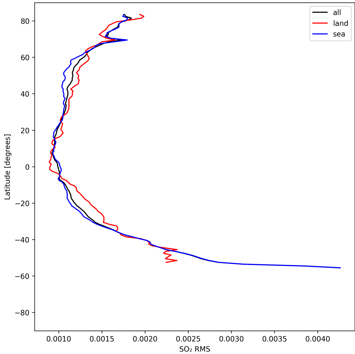
Figure 52: Zonal average of “SO 2 RMS” for 2025-08-15 to 2025-08-16.
