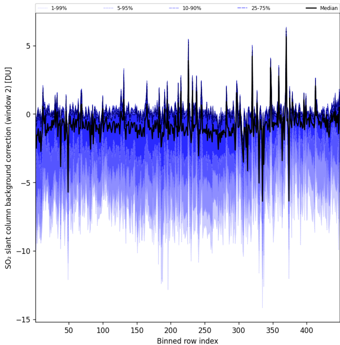
Figure 97: Along track statistics of “SO 2 slant column background correction (window 2)” for 2025-08-15 to 2025-08-16
