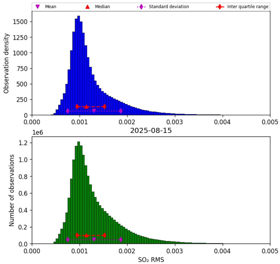
Figure 79: Histogram of “SO 2 RMS” for 2025-08-15 to 2025-08-16
