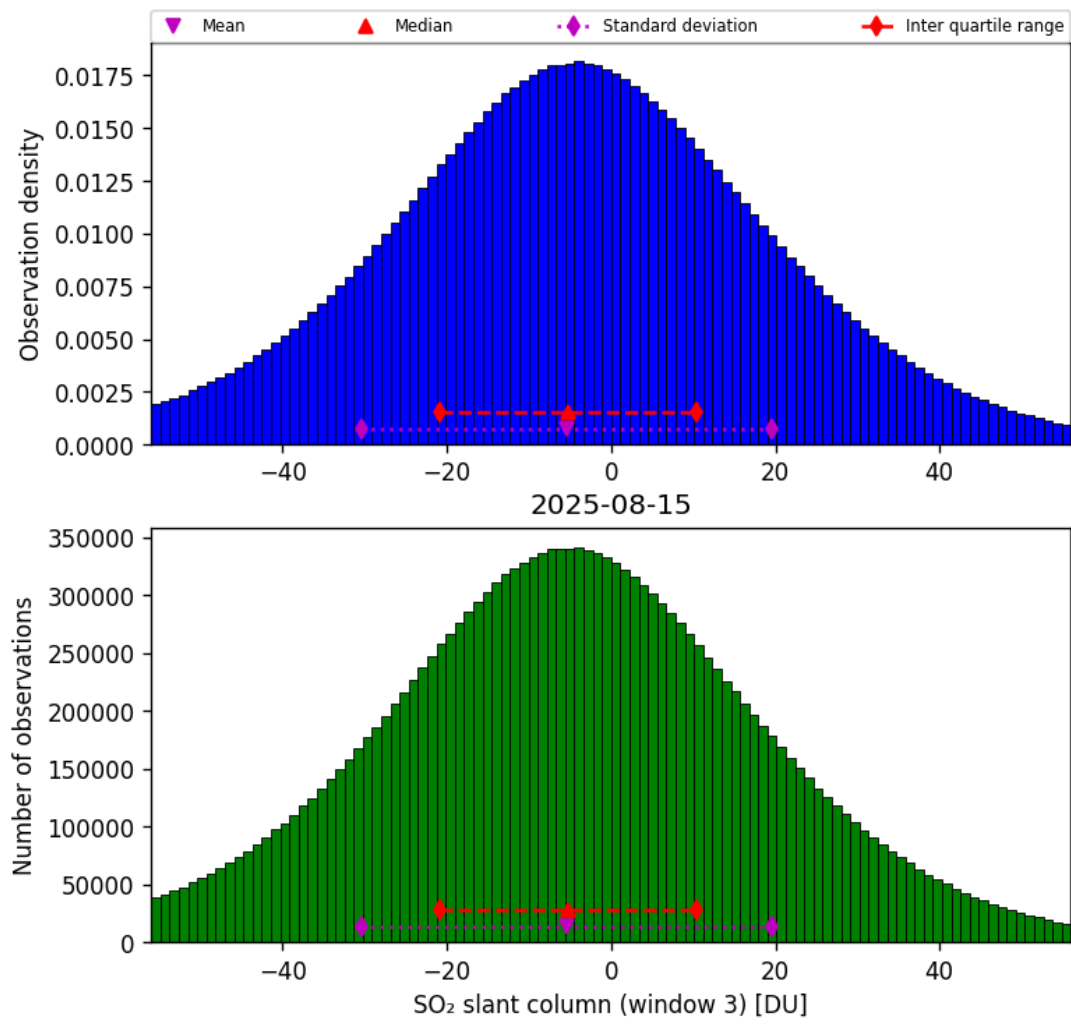
Figure 71: Histogram of “SO 2 slant column (window 3)” for 2025-08-15 to 2025-08-16
