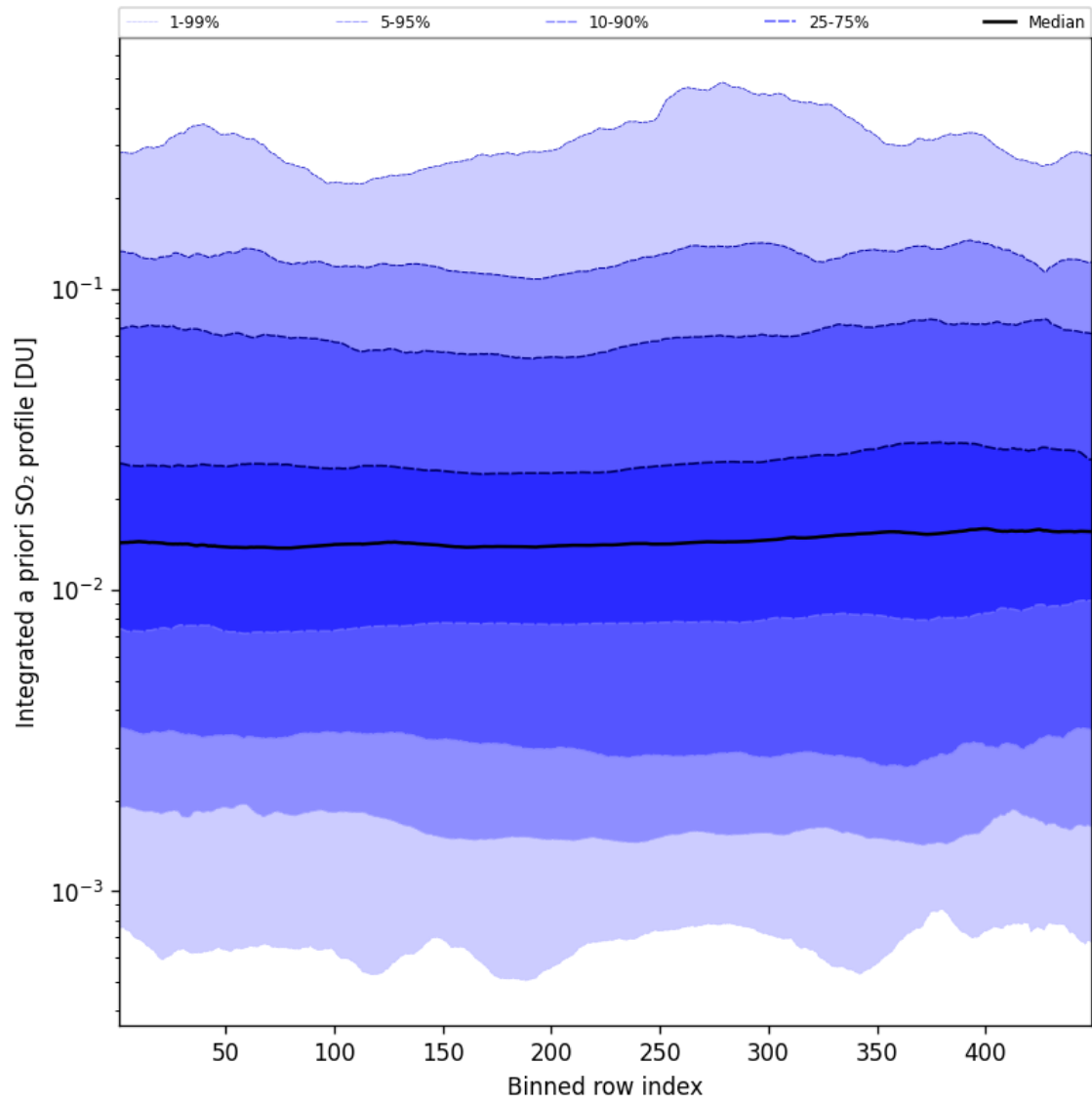
Figure 103: Along track statistics of “Integrated a priori SO 2 profile” for 2025-08-15 to 2025-08-16
