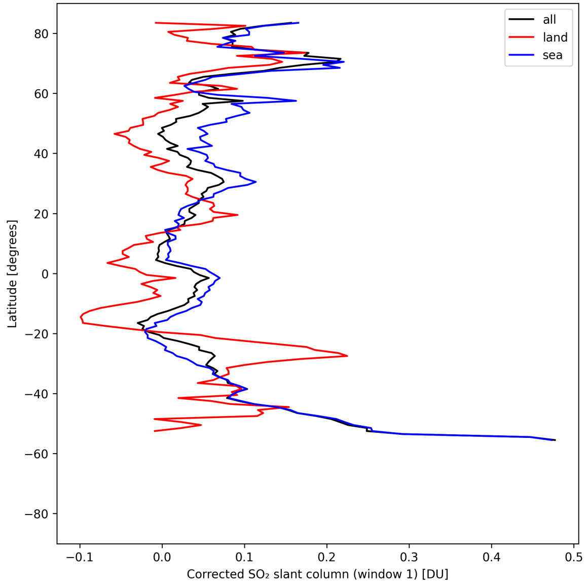
Figure 38: Zonal average of “Corrected SO 2 slant column (window 1)” for 2025-08-15 to 2025-08-16.
