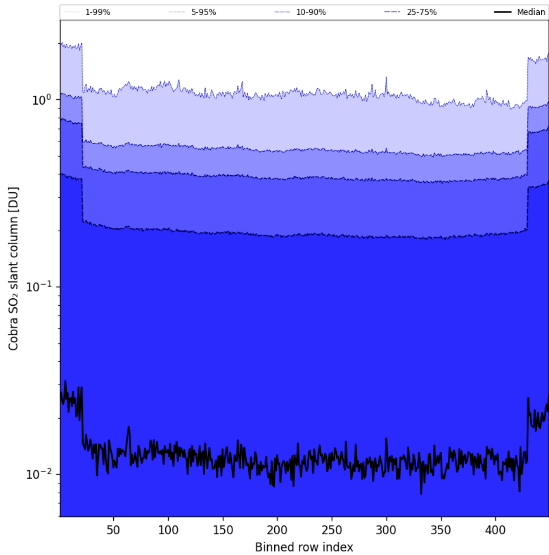
Figure 88: Along track statistics of "Cobra SO 2 slant column" for 2025-08-15 to 2025-08-16
