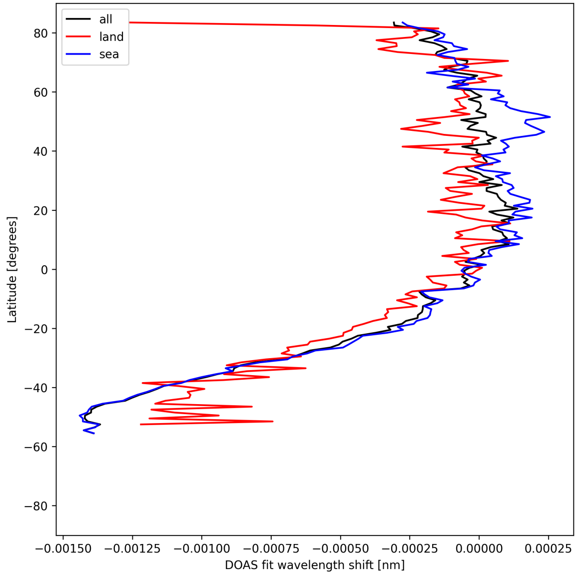
Figure 50: Zonal average of “DOAS fit wavelength shift” for 2025-08-15 to 2025-08-16.
