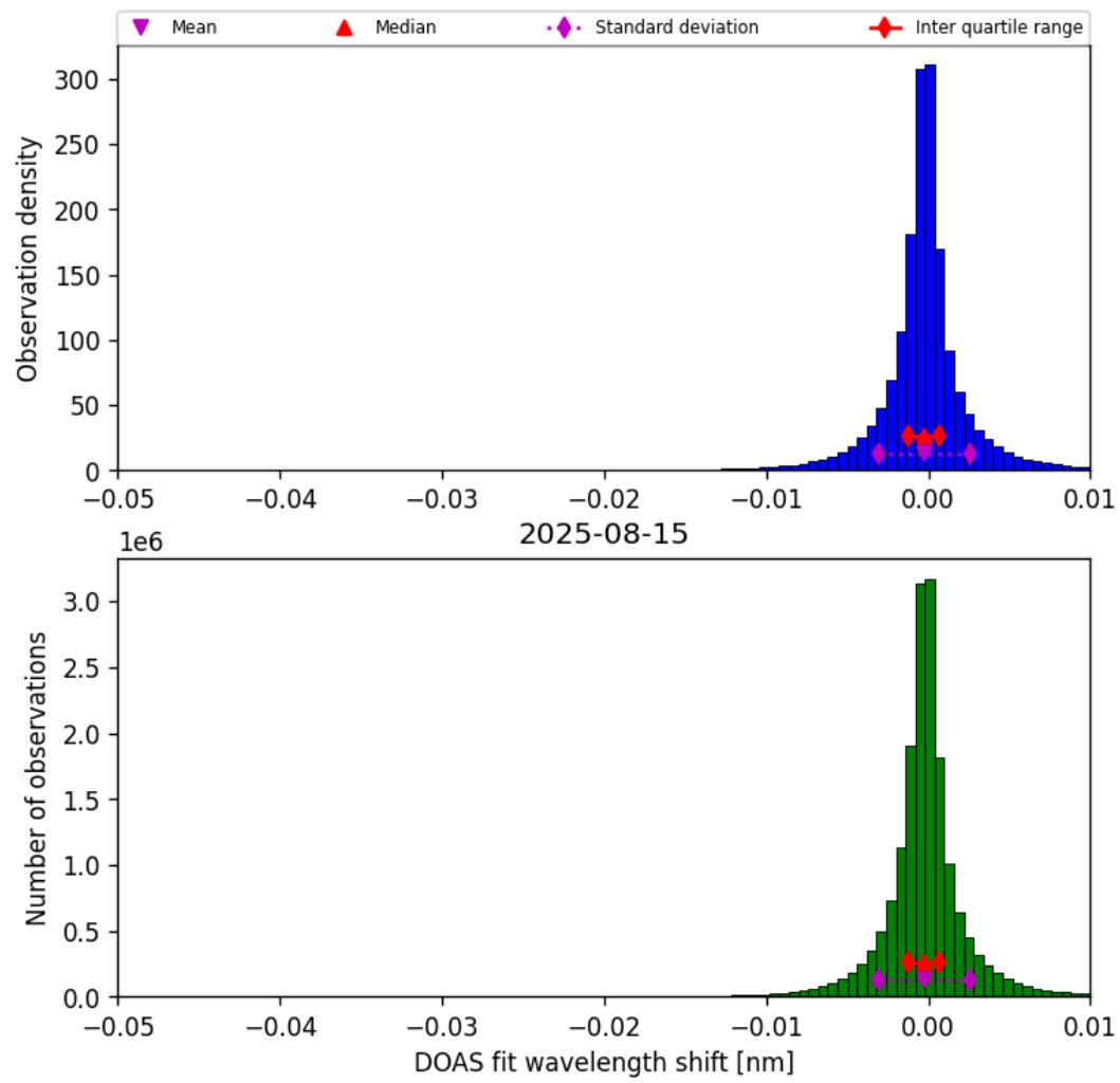
Figure 77: Histogram of “DOAS fit wavelength shift” for 2025-08-15 to 2025-08-16
