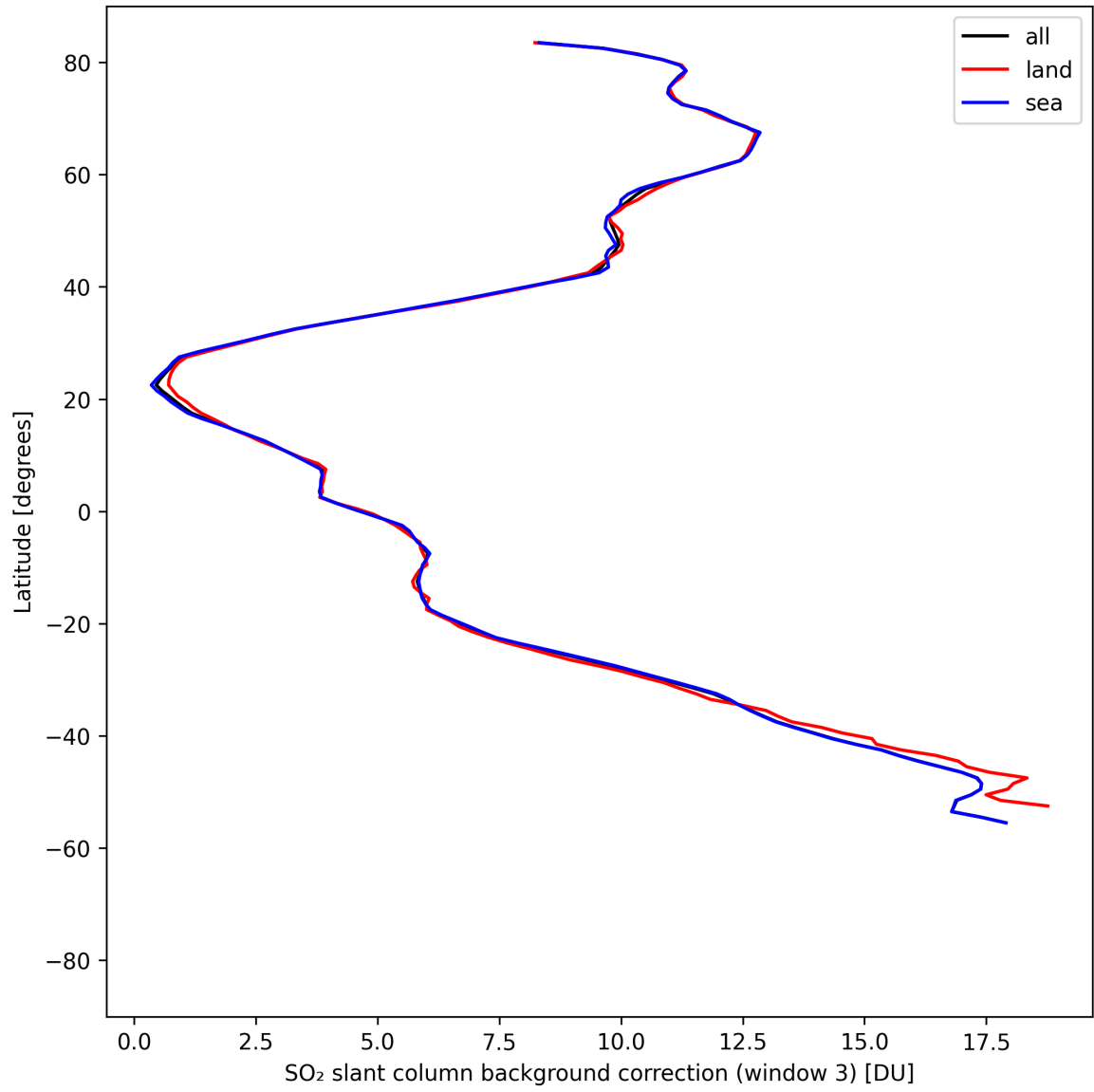
Figure 47: Zonal average of “SO 2 slant column background correction (window 3)” for 2025-08-15 to 2025-08-16.
