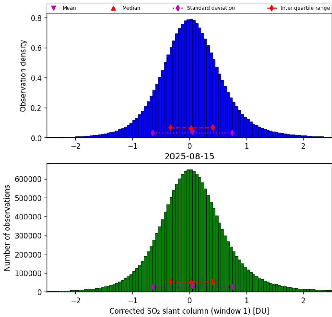
Figure 65: Histogram of “Corrected SO 2 slant column (window 1)” for 2025-08-15 to 2025-08-16
