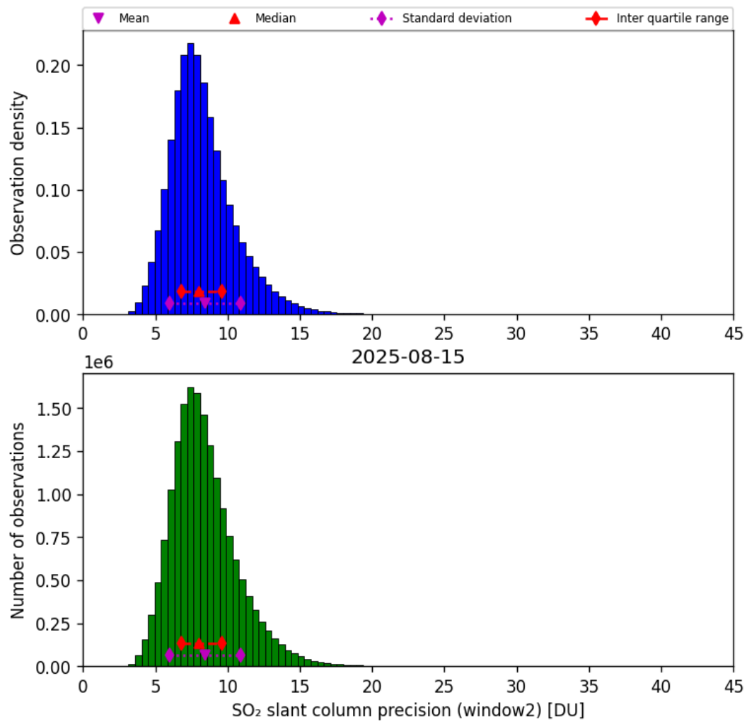
Figure 68: Histogram of “SO 2 slant column precision (window2)” for 2025-08-15 to 2025-08-16
