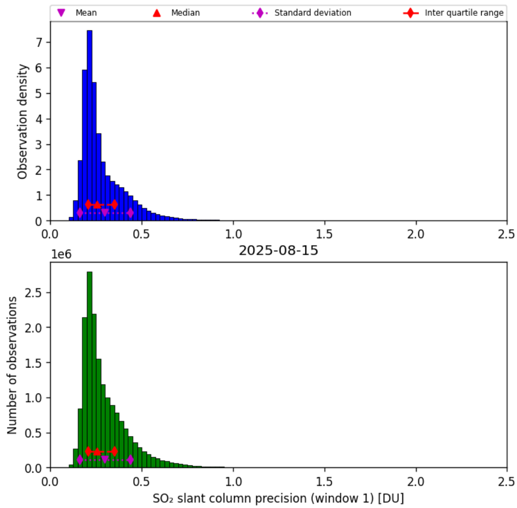
Figure 64: Histogram of “SO 2 slant column precision (window 1)” for 2025-08-15 to 2025-08-16
