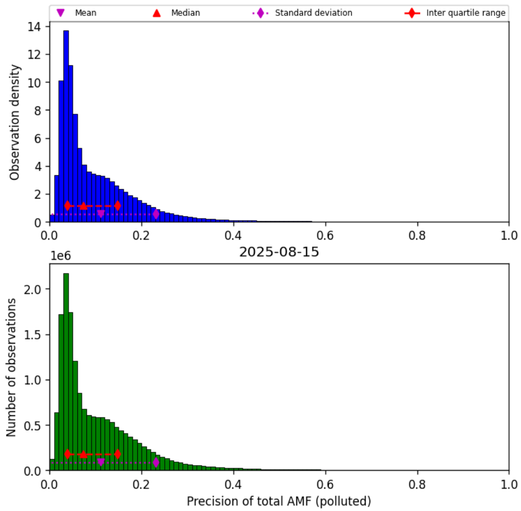
Figure 81: Histogram of “Precision of total AMF (polluted)” for 2025-08-15 to 2025-08-16
