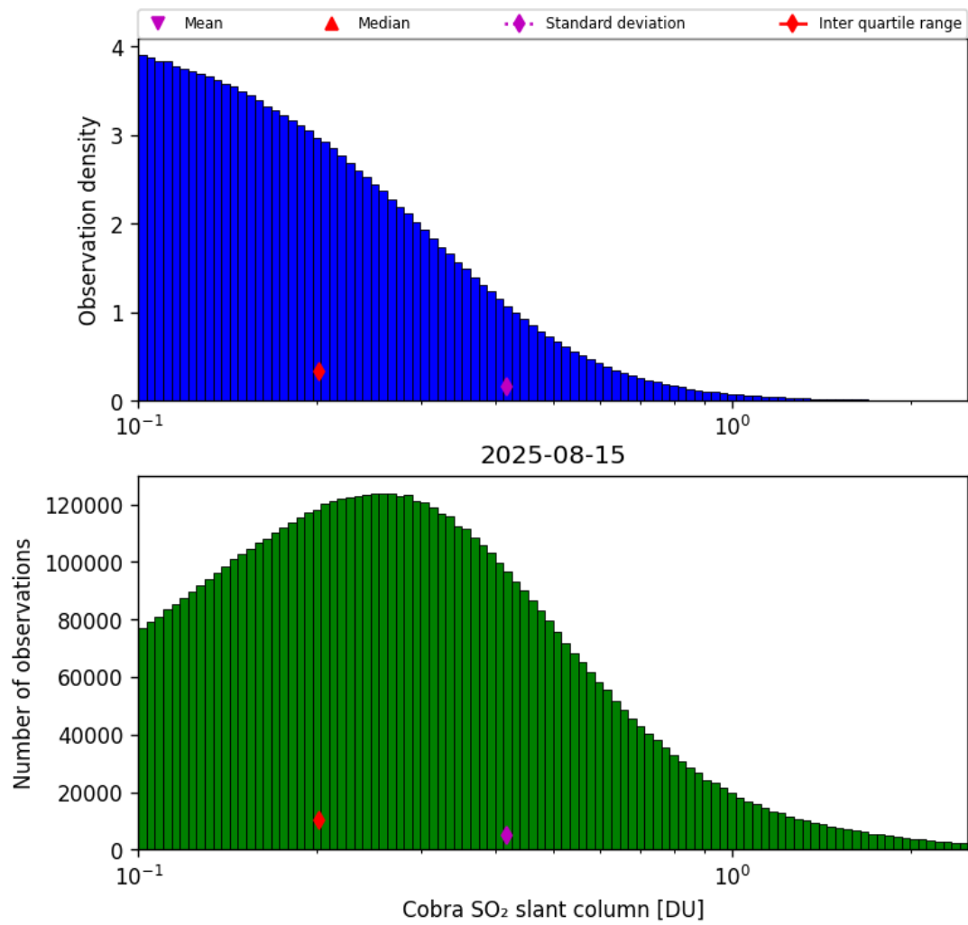
Figure 61: Histogram of “Cobra SO 2 slant column” for 2025-08-15 to 2025-08-16
