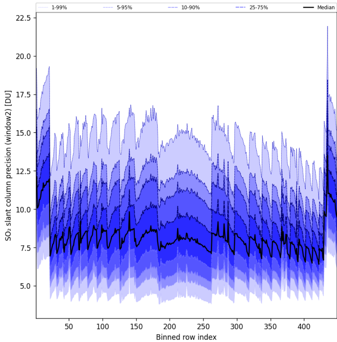
Figure 95: Along track statistics of “SO 2 slant column precision (window2)” for 2025-08-15 to 2025-08-16
