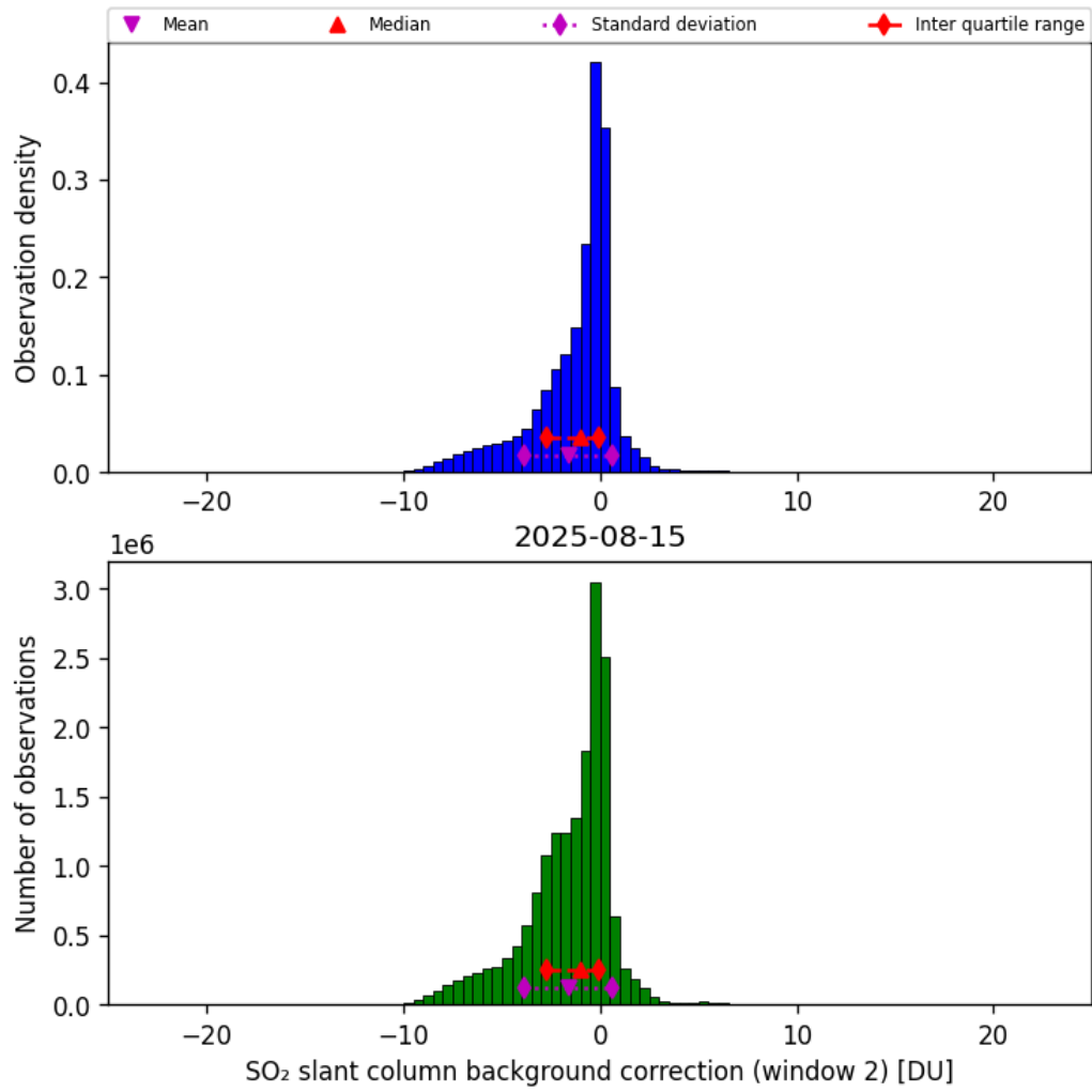
Figure 70: Histogram of “SO 2 slant column background correction (window 2)” for 2025-08-15 to 2025-08-16
