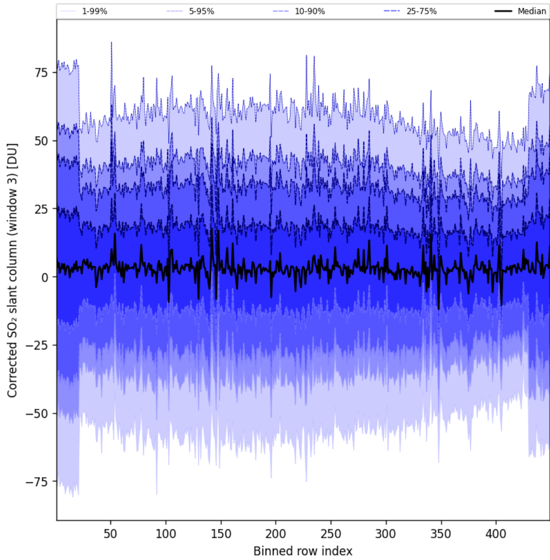
Figure 100: Along track statistics of “Corrected SO 2 slant column (window 3)” for 2025-08-15 to 2025-08-16
