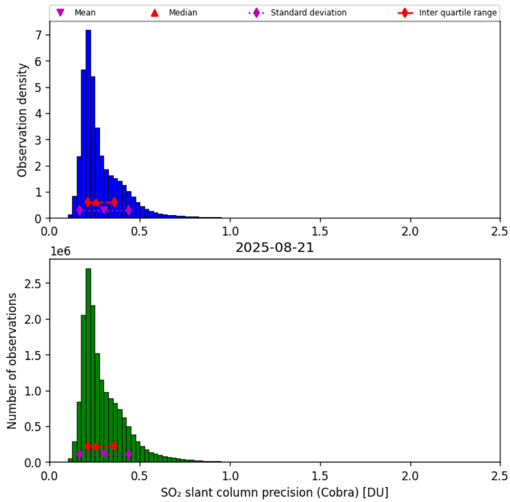
Figure 62: Histogram of “SO 2 slant column precision (Cobra)” for 2025-08-21 to 2025-08-22
