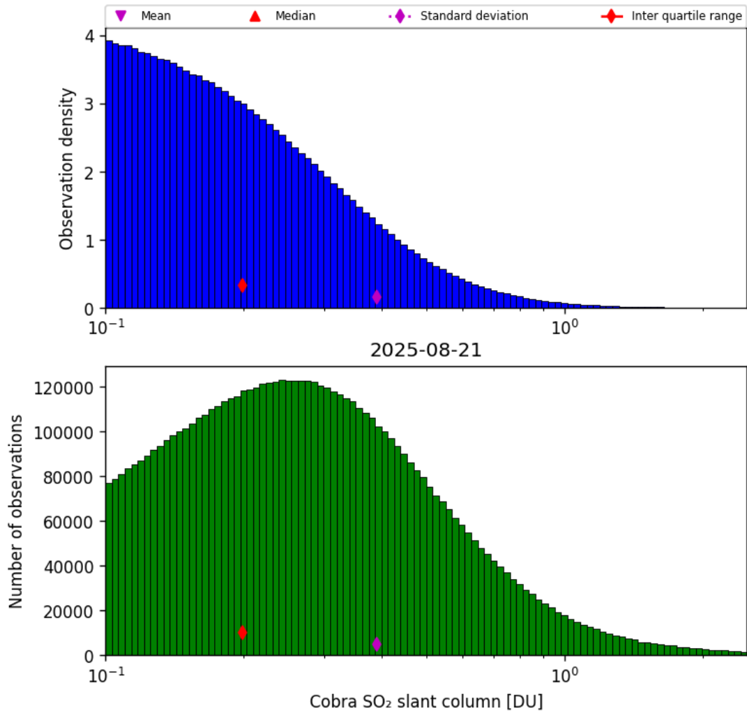
Figure 61: Histogram of “Cobra SO 2 slant column” for 2025-08-21 to 2025-08-22
