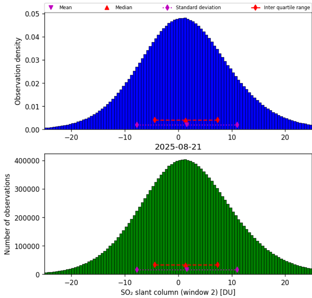
Figure 67: Histogram of “SO 2 slant column (window 2)” for 2025-08-21 to 2025-08-22
