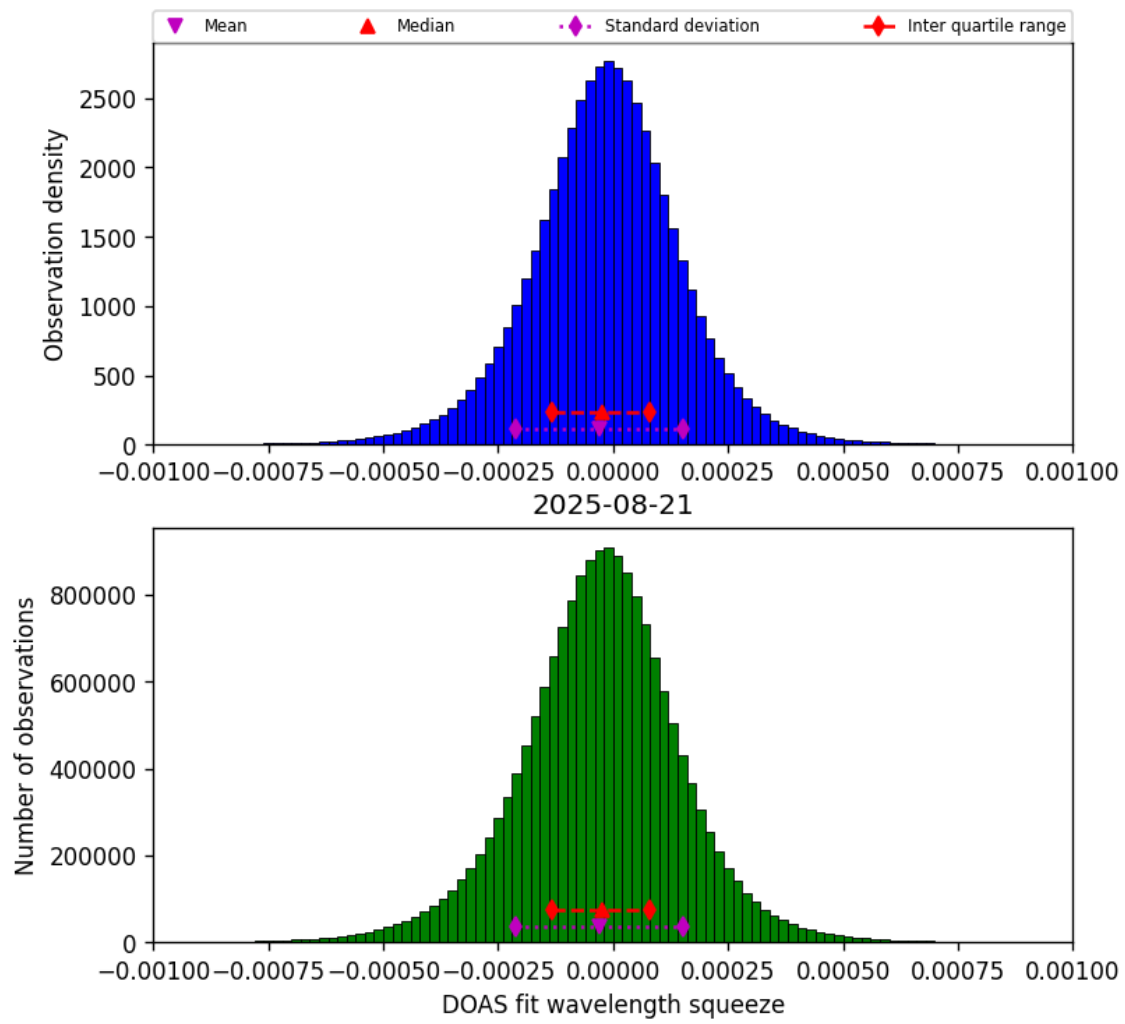
Figure 78: Histogram of “DOAS fit wavelength squeeze” for 2025-08-21 to 2025-08-22
