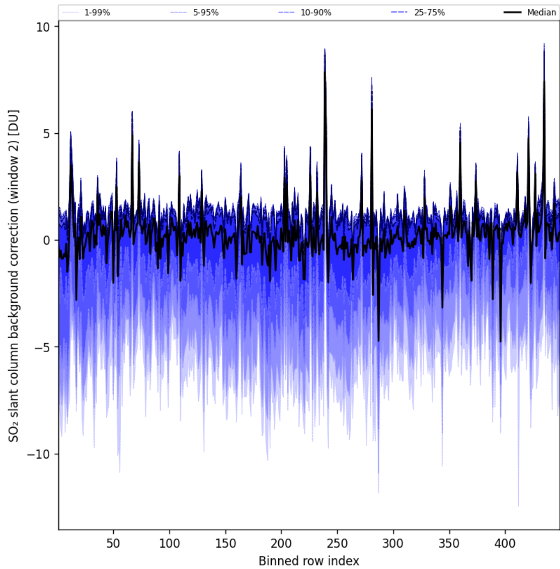
Figure 97: Along track statistics of “SO 2 slant column background correction (window 2)” for 2025-08-21 to 2025-08-22
