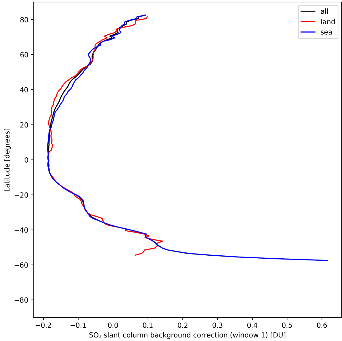
Figure 39: Zonal average of “SO 2 slant column background correction (window 1)” for 2025-08-21 to 2025-08-22.
