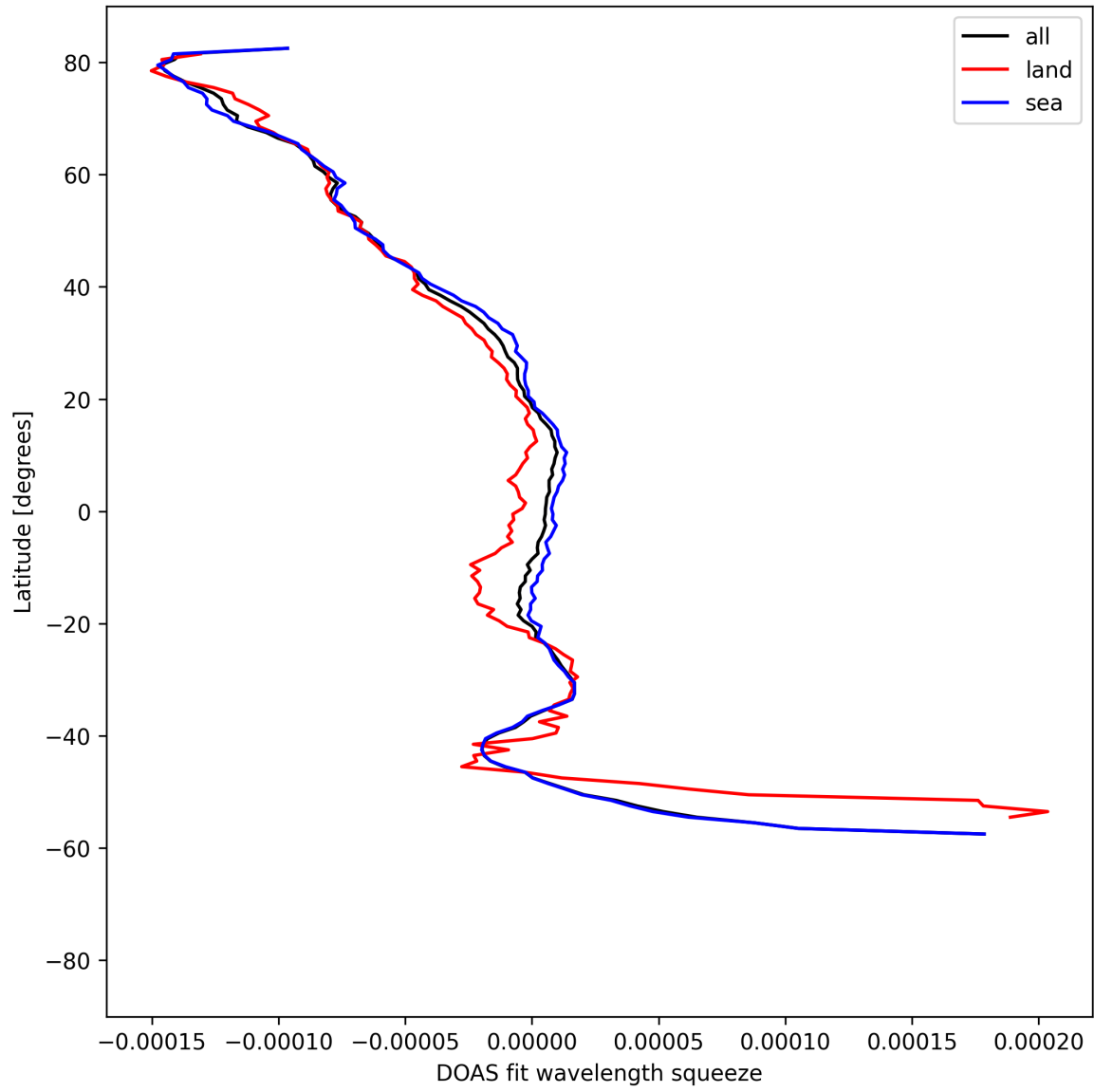
Figure 51: Zonal average of “DOAS fit wavelength squeeze” for 2025-08-21 to 2025-08-22.
