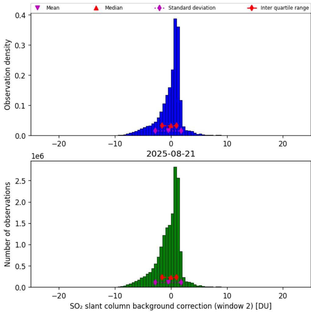
Figure 70: Histogram of “SO 2 slant column background correction (window 2)” for 2025-08-21 to 2025-08-22
