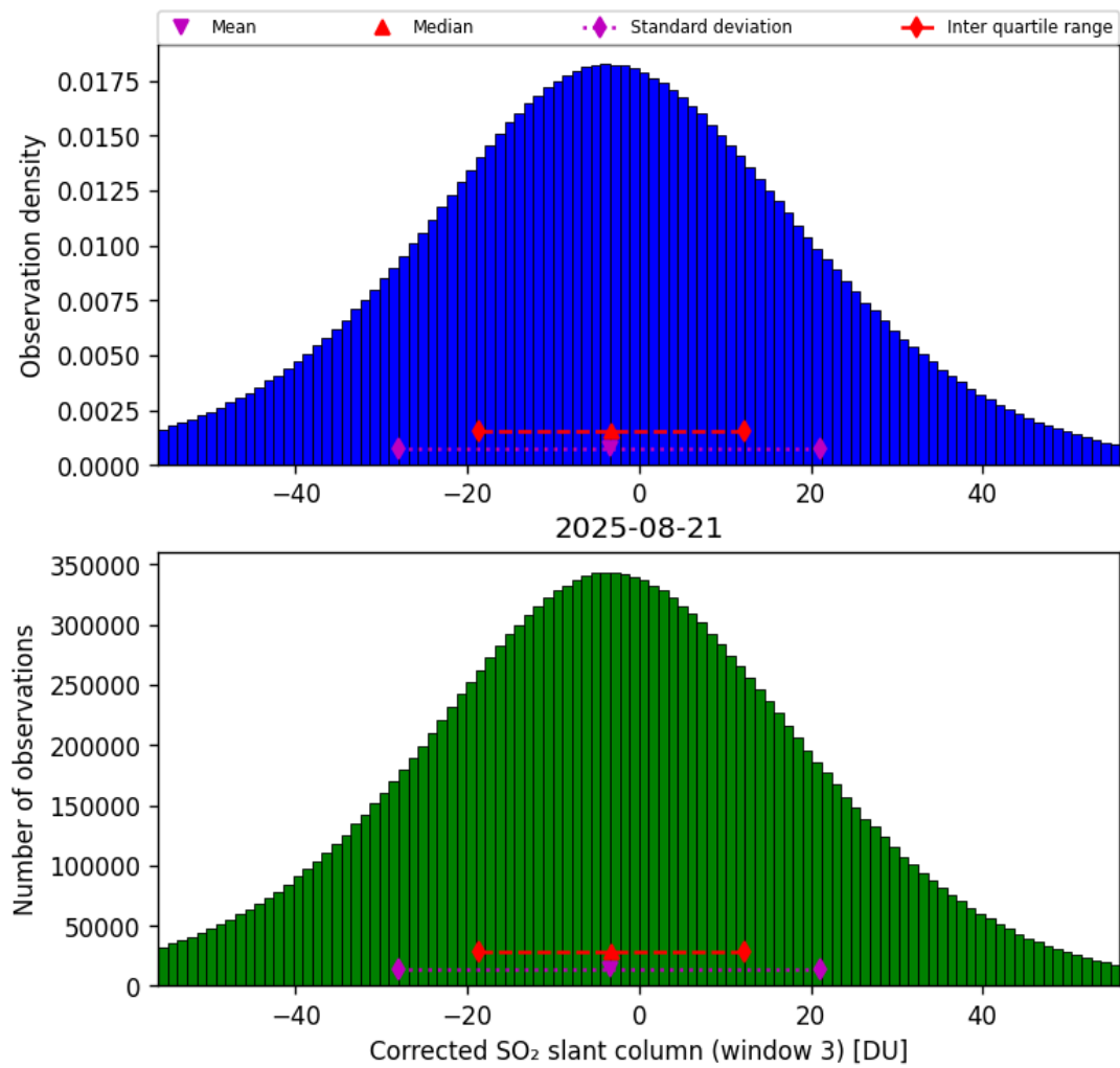
Figure 73: Histogram of “Corrected SO 2 slant column (window 3)” for 2025-08-21 to 2025-08-22
