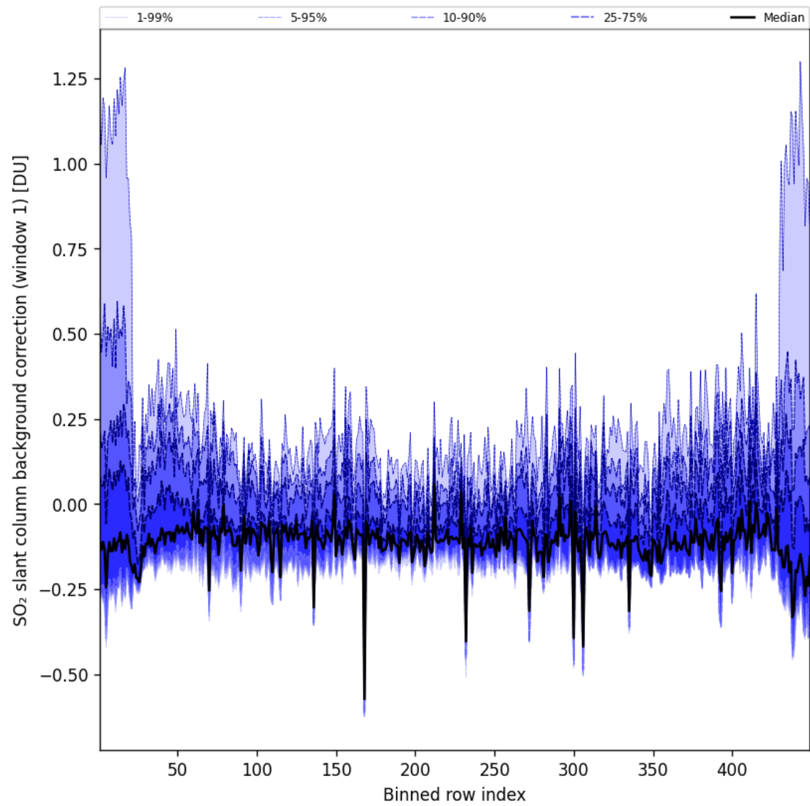
Figure 93: Along track statistics of “SO 2 slant column background correction (window 1)” for 2025-08-21 to 2025-08-22
