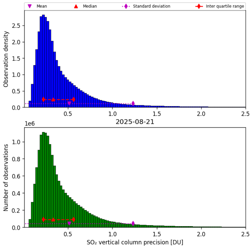
Figure 59: Histogram of “SO 2 vertical column precision” for 2025-08-21 to 2025-08-22
