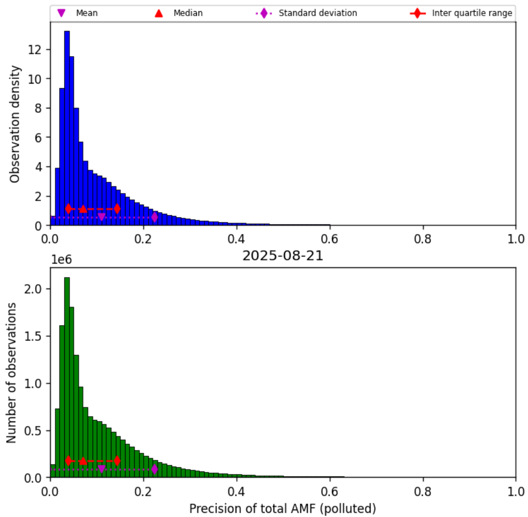
Figure 81: Histogram of “Precision of total AMF (polluted)” for 2025-08-21 to 2025-08-22
