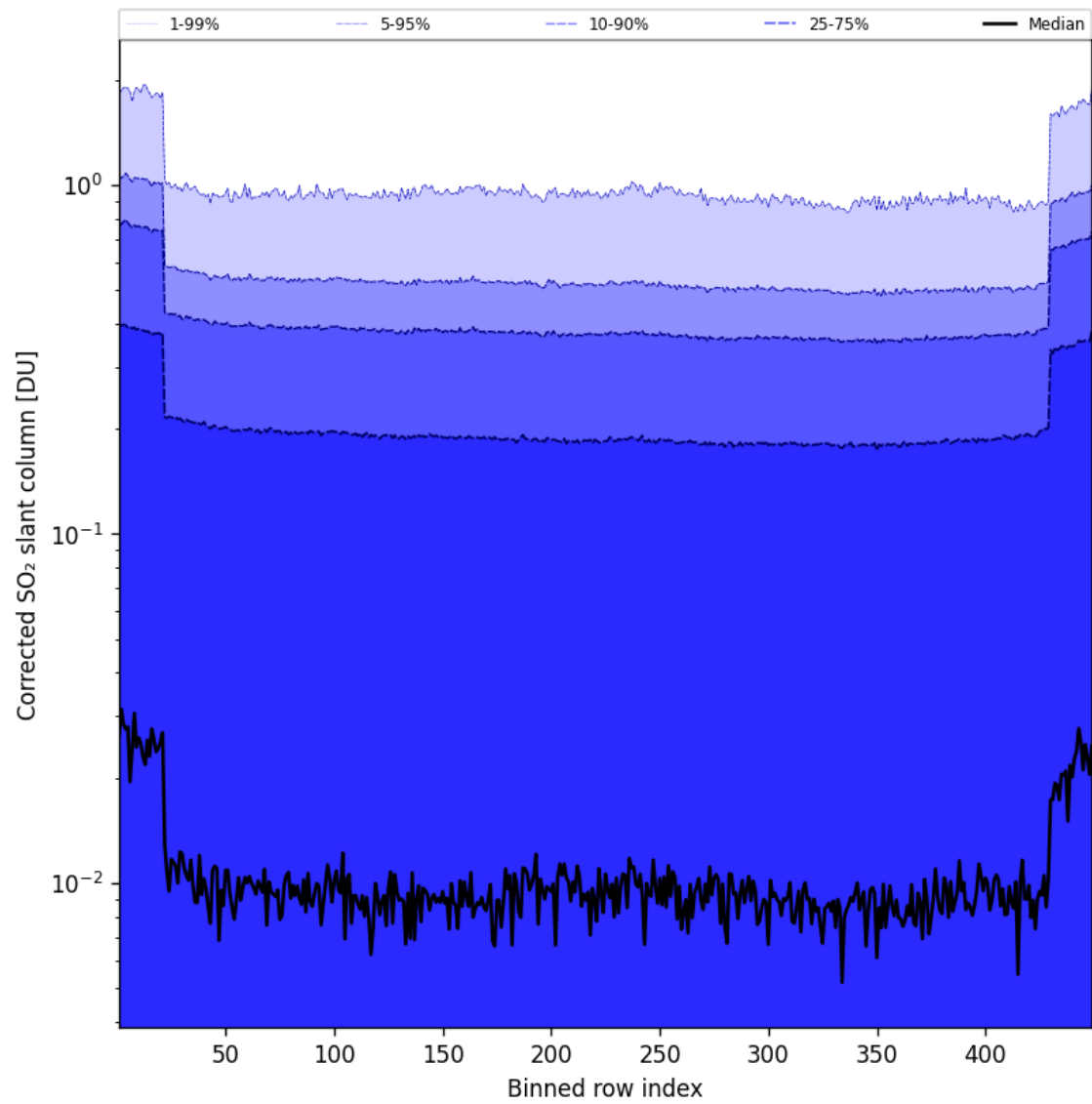
Figure 87: Along track statistics of “Corrected SO 2 slant column” for 2025-08-21 to 2025-08-22
