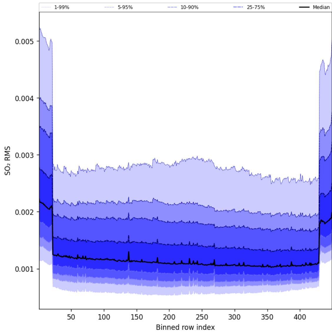
Figure 106: Along track statistics of “SO 2 RMS” for 2025-08-21 to 2025-08-22
