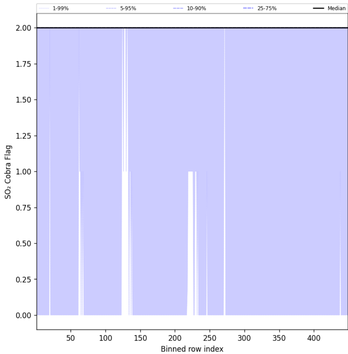
Figure 102: Along track statistics of "SO 2 Cobra Flag" for 2025-08-21 to 2025-08-22
