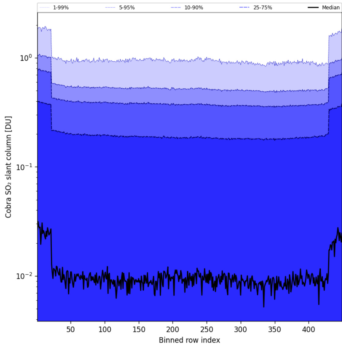
Figure 88: Along track statistics of “Cobra SO 2 slant column” for 2025-08-21 to 2025-08-22
