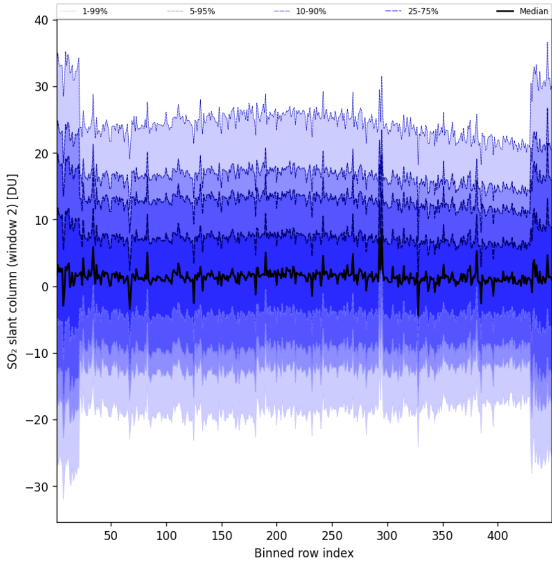
Figure 94: Along track statistics of "SO 2 slant column (window 2)" for 2025-08-21 to 2025-08-22
