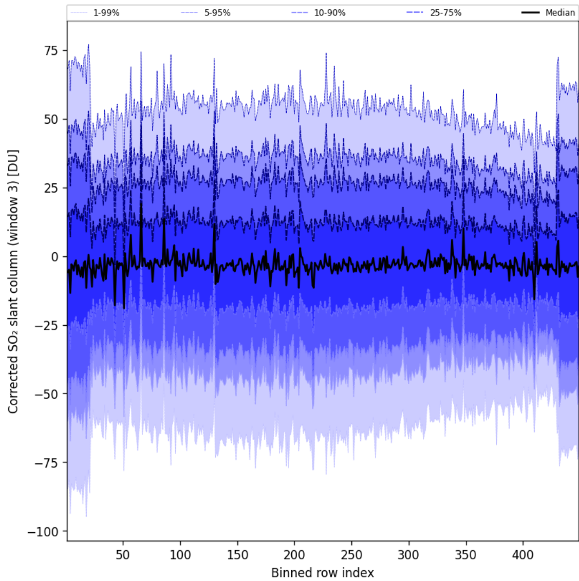
Figure 100: Along track statistics of “Corrected SO 2 slant column (window 3)” for 2025-08-21 to 2025-08-22
