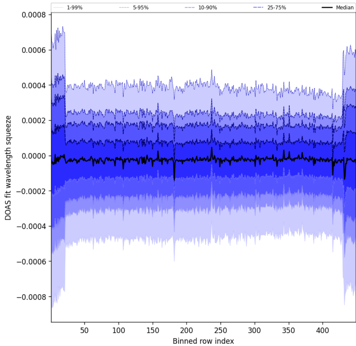
Figure 105: Along track statistics of “DOAS fit wavelength squeeze” for 2025-08-21 to 2025-08-22
