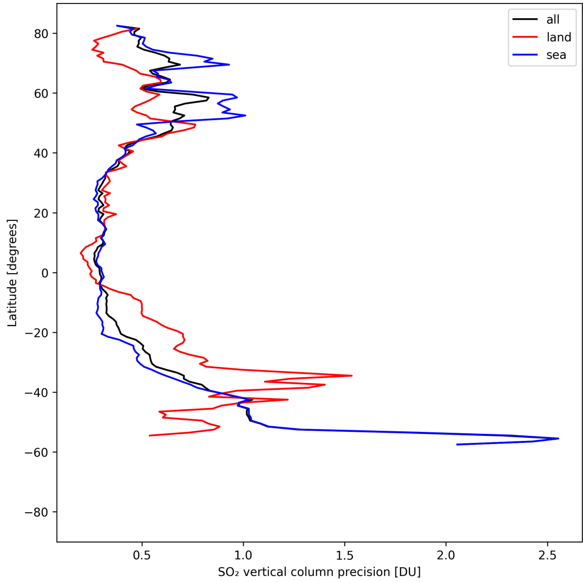
Figure 32: Zonal average of “SO 2 vertical column precision” for 2025-08-21 to 2025-08-22.
