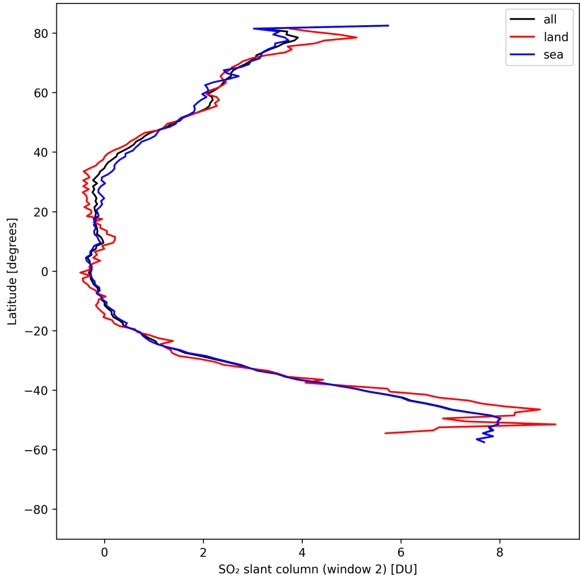
Figure 40: Zonal average of “SO 2 slant column (window 2)” for 2025-08-21 to 2025-08-22.
