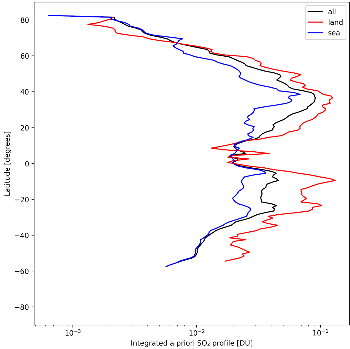
Figure 49: Zonal average of “Integrated a priori SO 2 profile” for 2025-08-21 to 2025-08-22.
