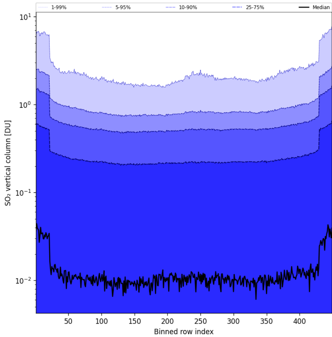
Figure 85: Along track statistics of “SO 2 vertical column” for 2025-08-21 to 2025-08-22
