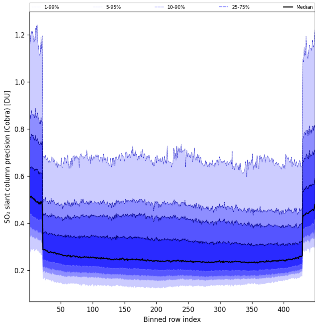
Figure 89: Along track statistics of “SO 2 slant column precision (Cobra)” for 2025-08-21 to 2025-08-22
