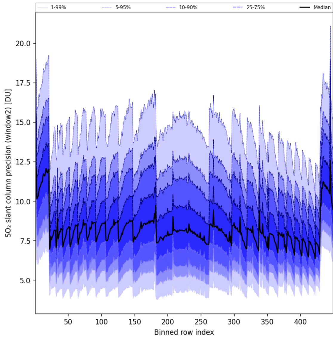
Figure 95: Along track statistics of “SO 2 slant column precision (window2)” for 2025-08-21 to 2025-08-22
