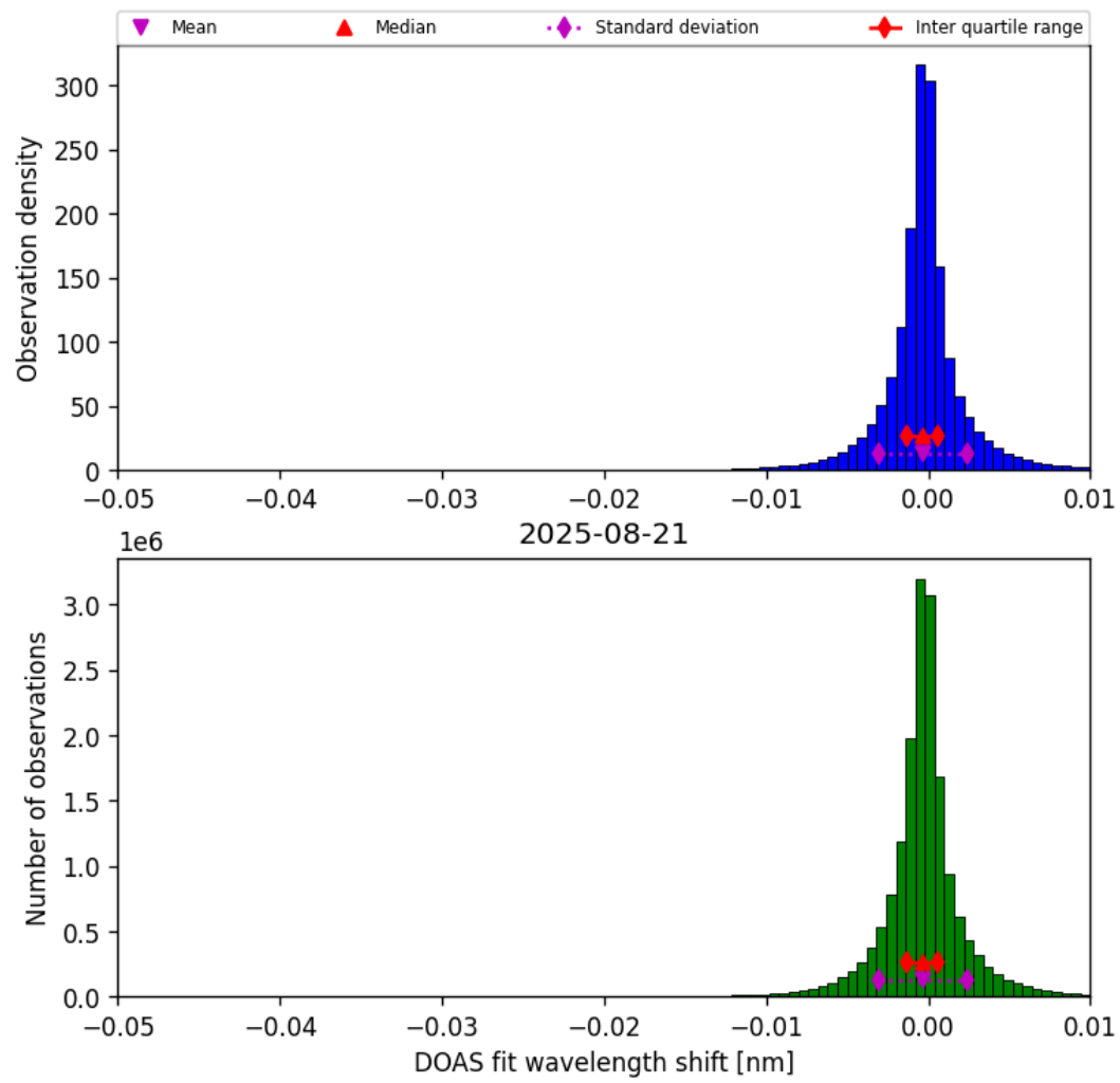
Figure 77: Histogram of “DOAS fit wavelength shift” for 2025-08-21 to 2025-08-22
