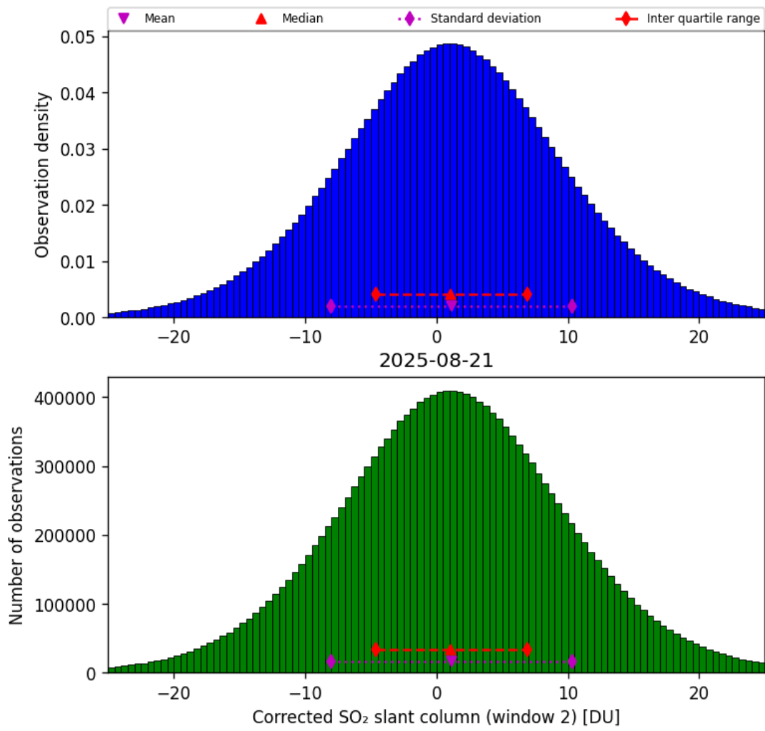
Figure 69: Histogram of “Corrected SO 2 slant column (window 2)” for 2025-08-21 to 2025-08-22
