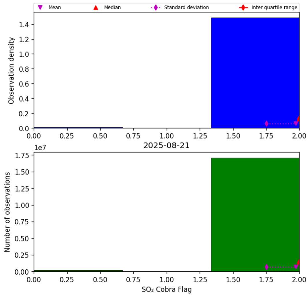
Figure 75: Histogram of “SO 2 Cobra Flag” for 2025-08-21 to 2025-08-22
