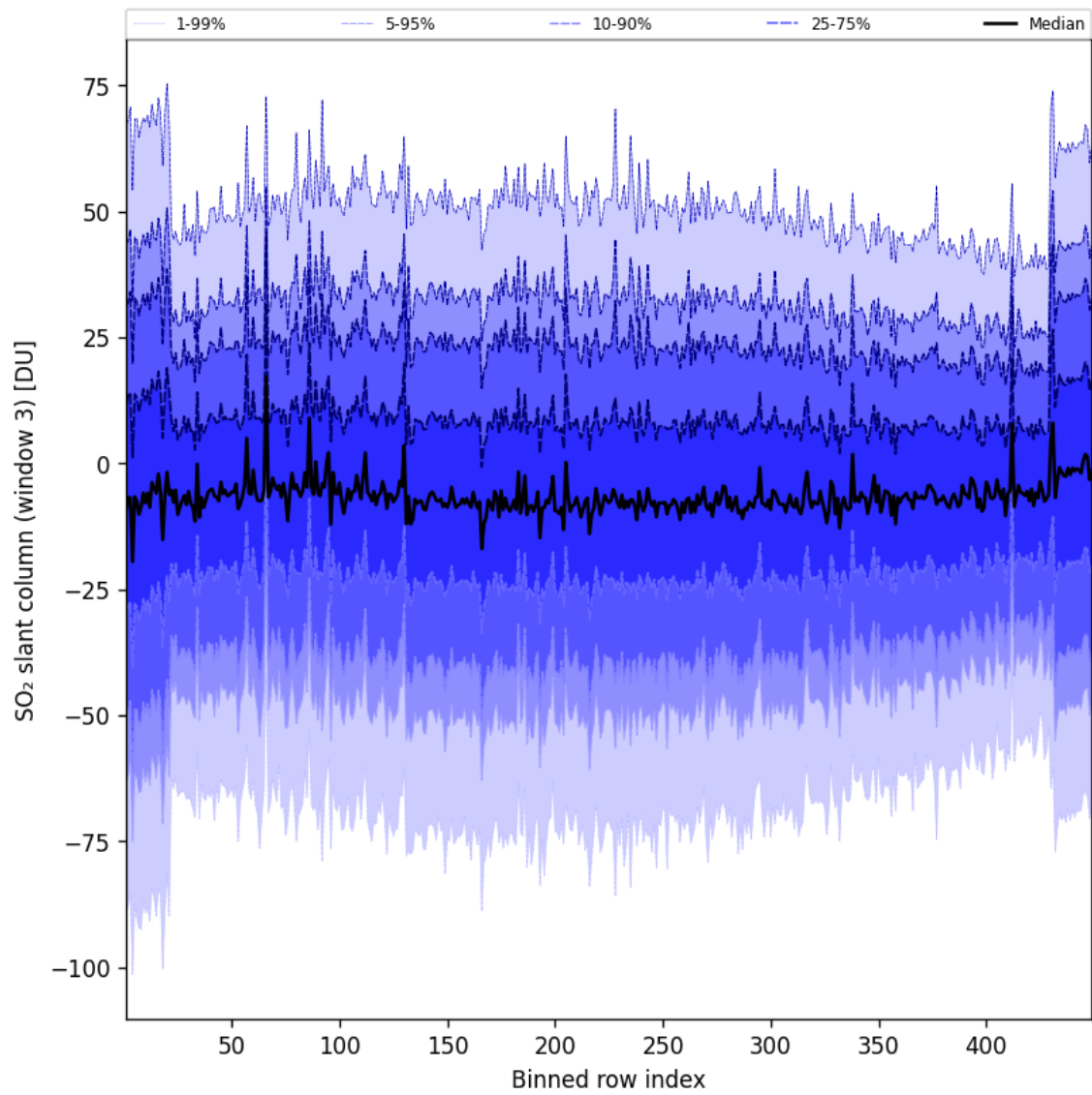
Figure 98: Along track statistics of “SO 2 slant column (window 3)” for 2025-08-21 to 2025-08-22
