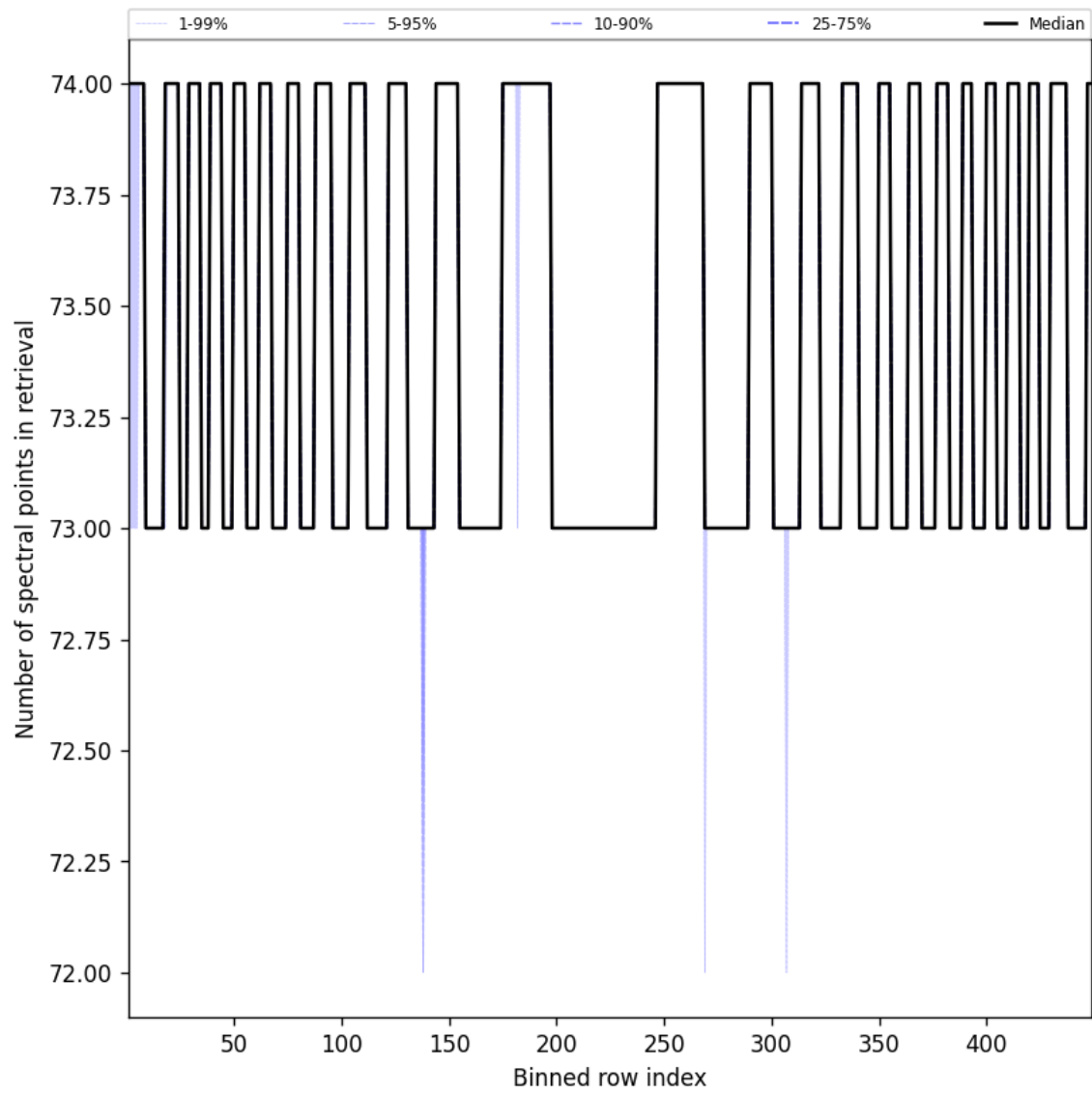
Figure 110: Along track statistics of “Number of spectral points in retrieval” for 2025-08-21 to 2025-08-22
