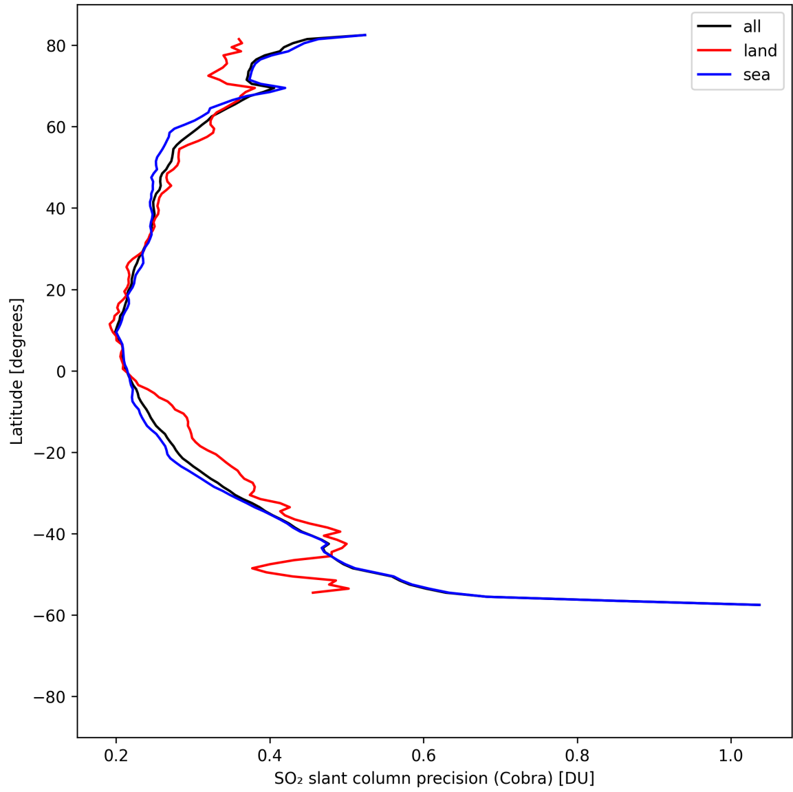
Figure 35: Zonal average of “SO 2 slant column precision (Cobra)” for 2025-08-21 to 2025-08-22.
