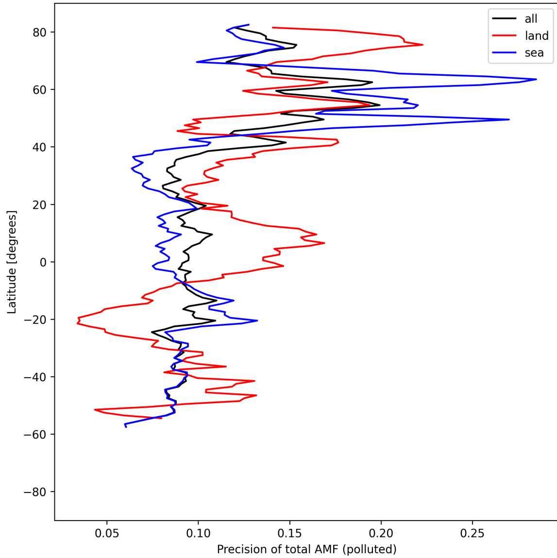
Figure 54: Zonal average of “Precision of total AMF (polluted)” for 2025-08-21 to 2025-08-22.
