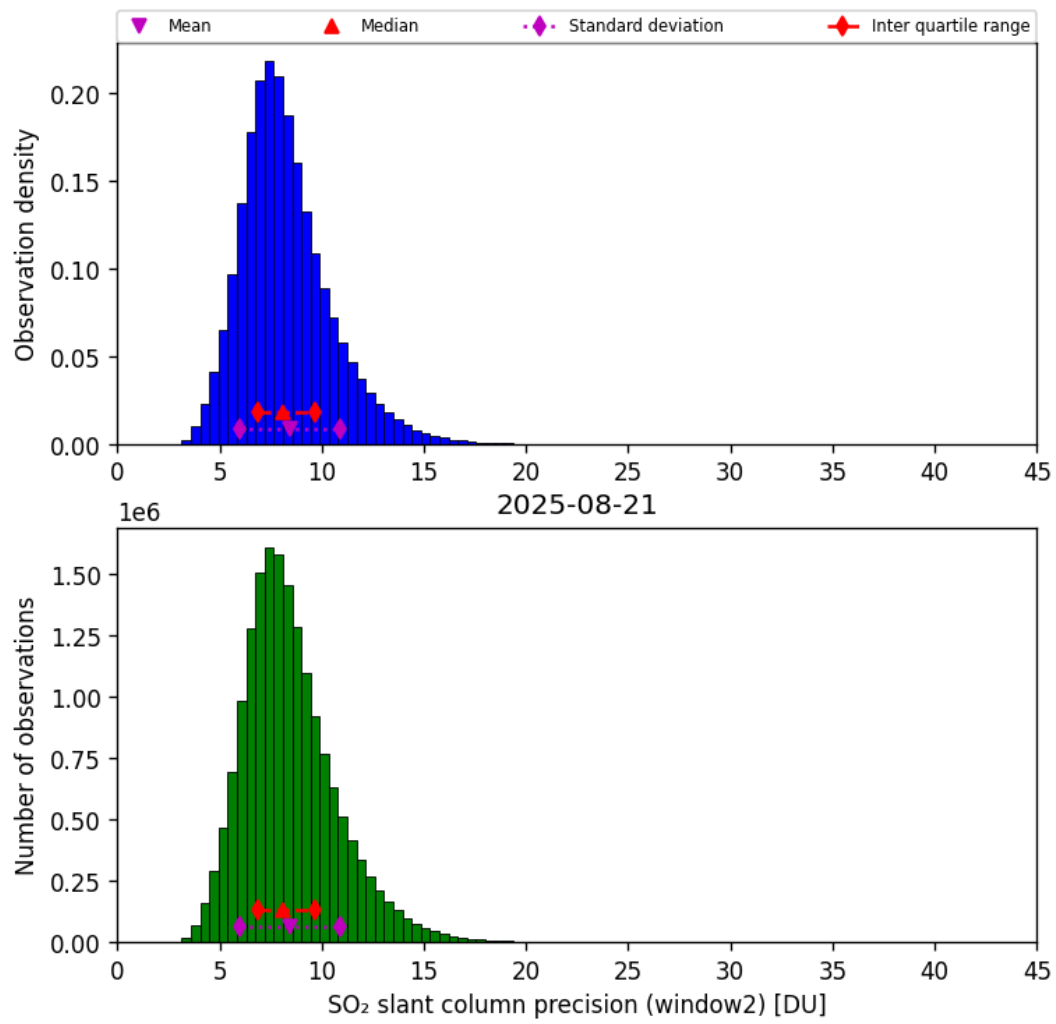
Figure 68: Histogram of “SO 2 slant column precision (window2)” for 2025-08-21 to 2025-08-22
