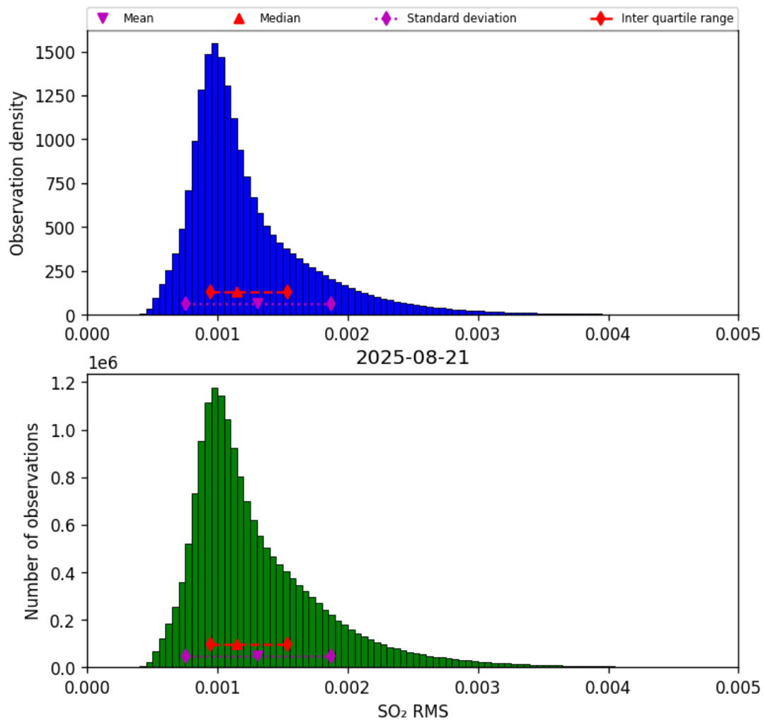
Figure 79: Histogram of "SO 2 RMS" for 2025-08-21 to 2025-08-22
