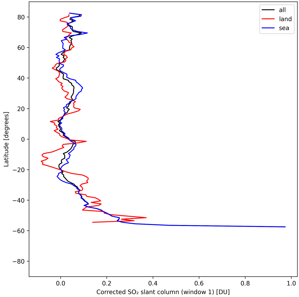
Figure 38: Zonal average of “Corrected SO 2 slant column (window 1)” for 2025-08-21 to 2025-08-22.
