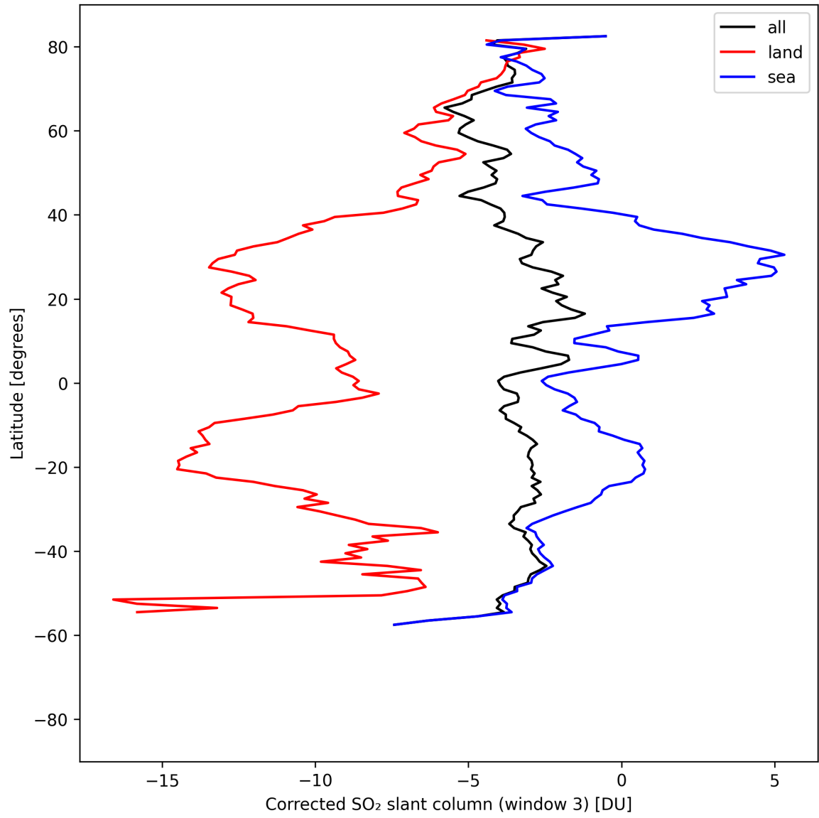
Figure 46: Zonal average of “Corrected SO 2 slant column (window 3)” for 2025-08-21 to 2025-08-22.
