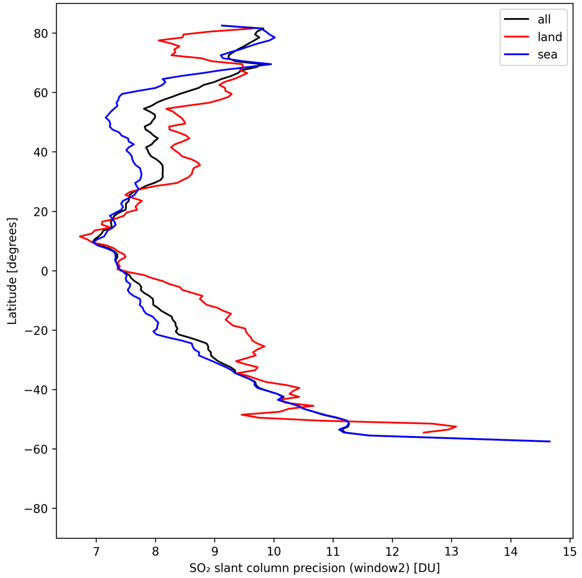
Figure 41: Zonal average of “SO 2 slant column precision (window2)” for 2025-08-21 to 2025-08-22.
