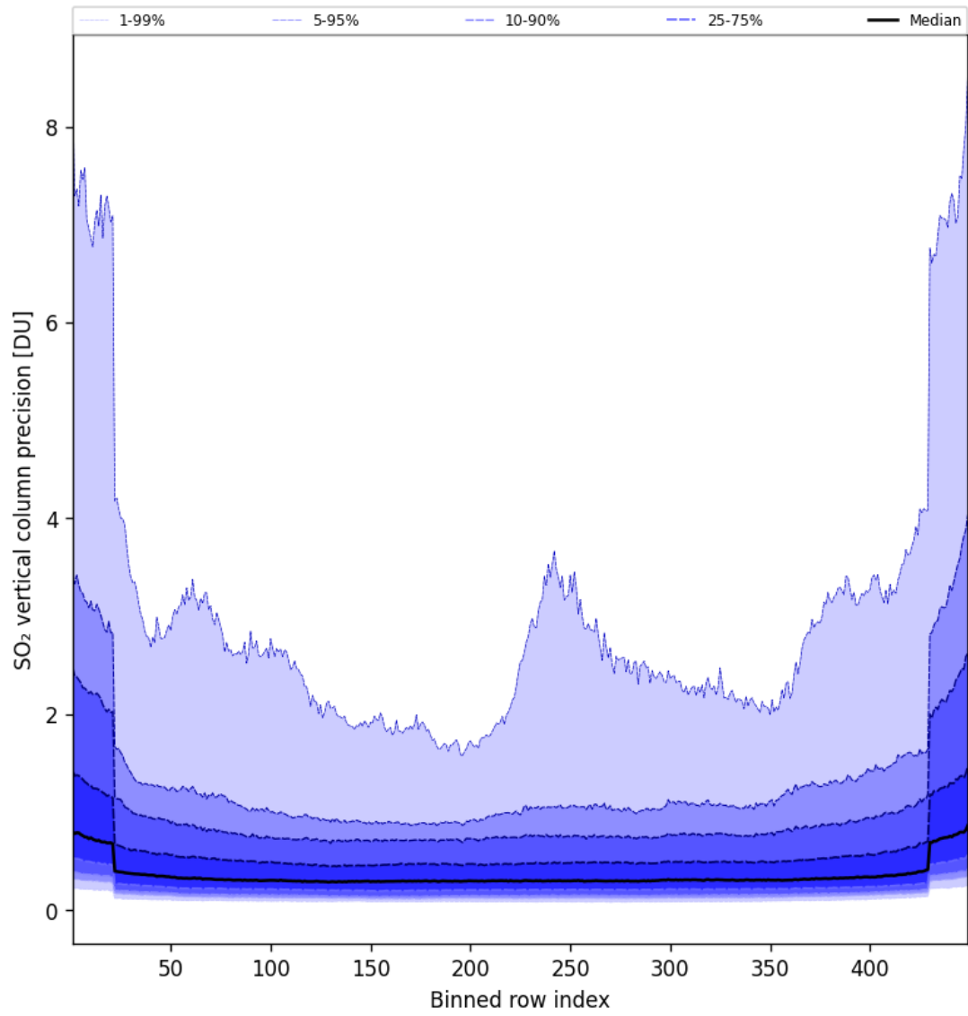
Figure 86: Along track statistics of “SO 2 vertical column precision” for 2025-08-21 to 2025-08-22
