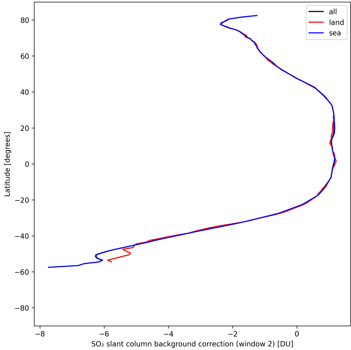
Figure 43: Zonal average of “SO 2 slant column background correction (window 2)” for 2025-08-21 to 2025-08-22.
