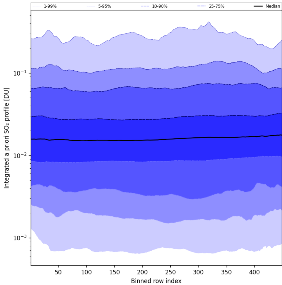
Figure 103: Along track statistics of “Integrated a priori SO 2 profile” for 2025-08-21 to 2025-08-22
