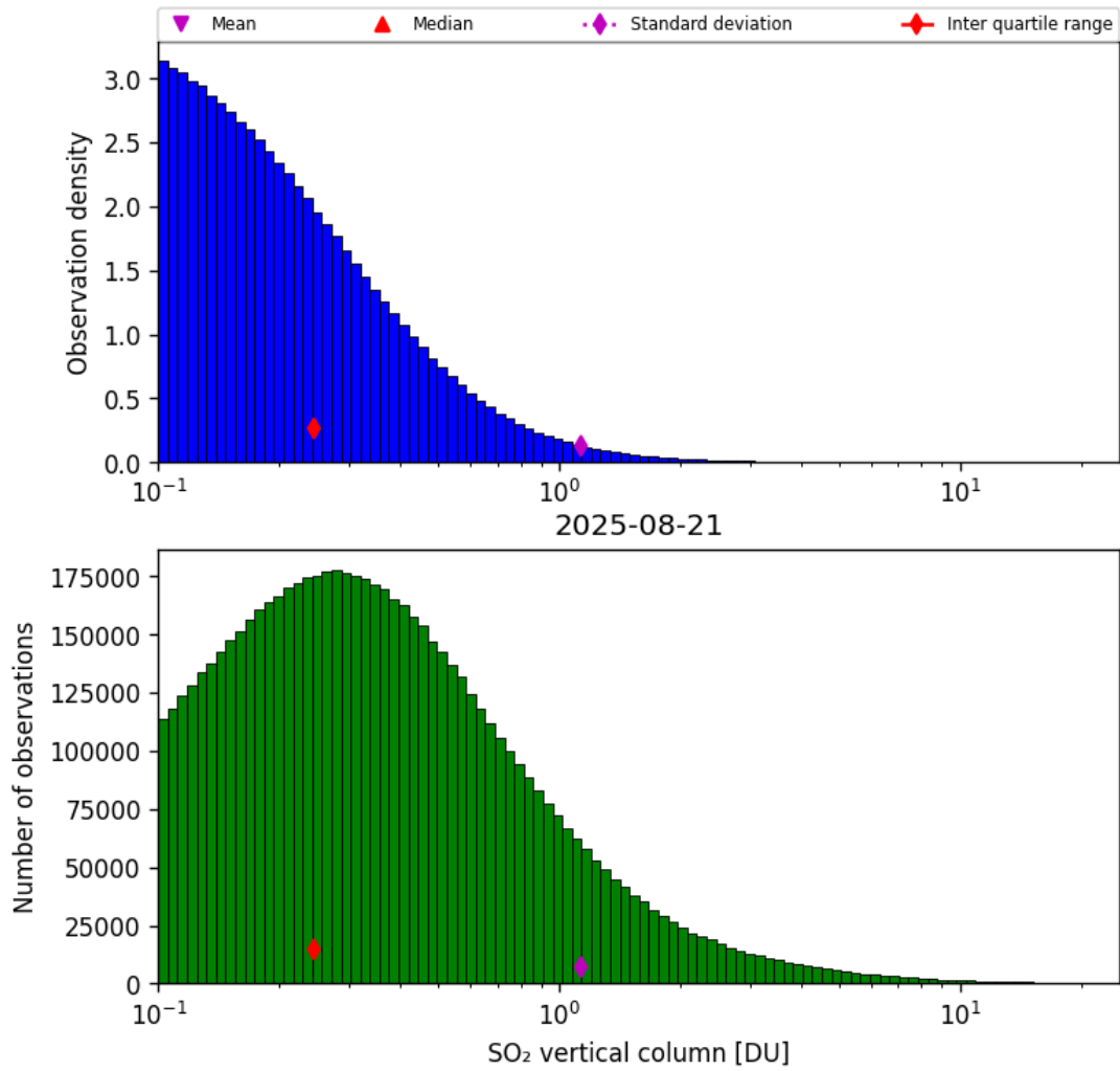
Figure 58: Histogram of “SO 2 vertical column” for 2025-08-21 to 2025-08-22
