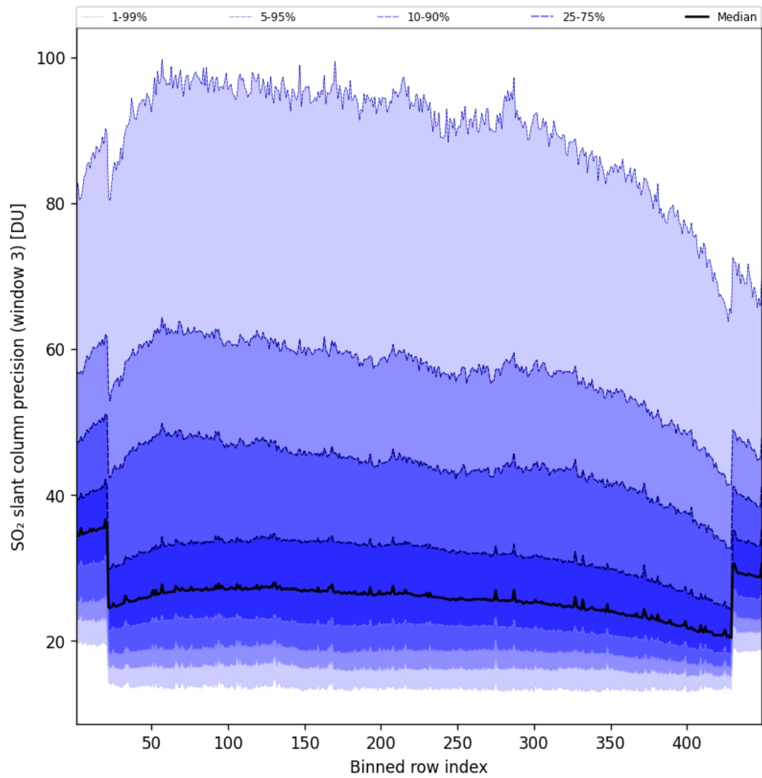
Figure 99: Along track statistics of “SO 2 slant column precision (window 3)” for 2025-08-21 to 2025-08-22
