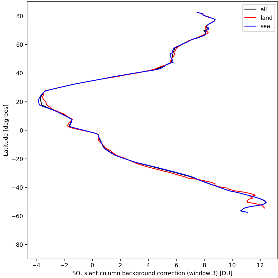
Figure 47: Zonal average of “SO 2 slant column background correction (window 3)” for 2025-08-21 to 2025-08-22.
