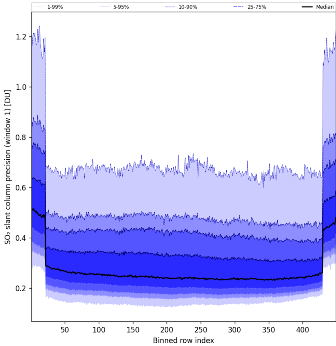
Figure 91: Along track statistics of “SO 2 slant column precision (window 1)” for 2025-08-21 to 2025-08-22
