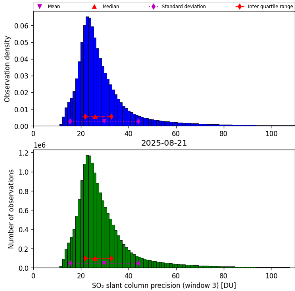
Figure 72: Histogram of “SO 2 slant column precision (window 3)” for 2025-08-21 to 2025-08-22
