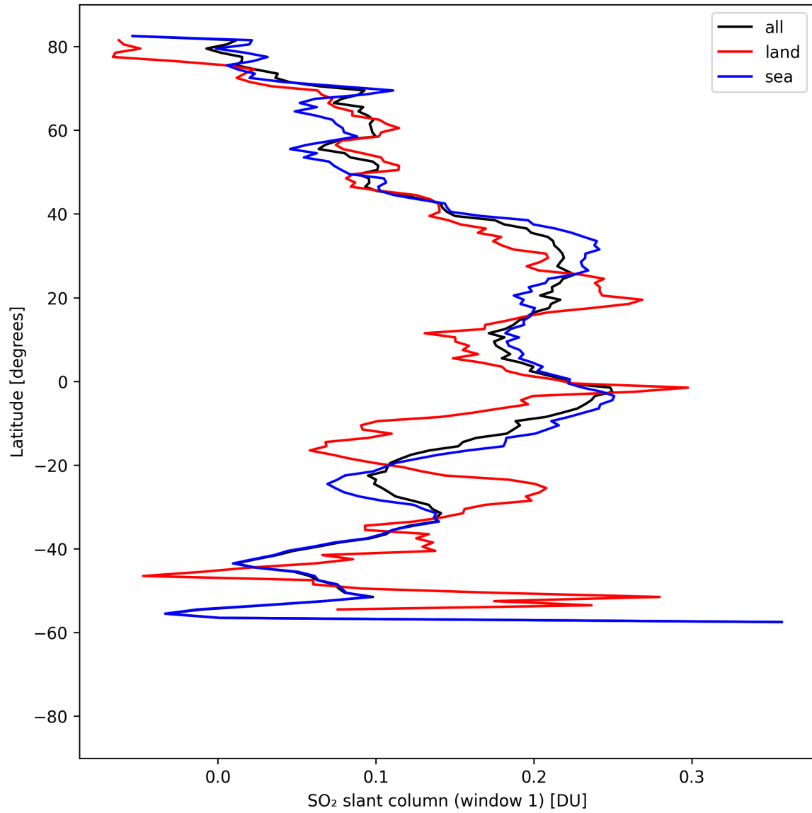
Figure 36: Zonal average of “SO 2 slant column (window 1)” for 2025-08-21 to 2025-08-22.
