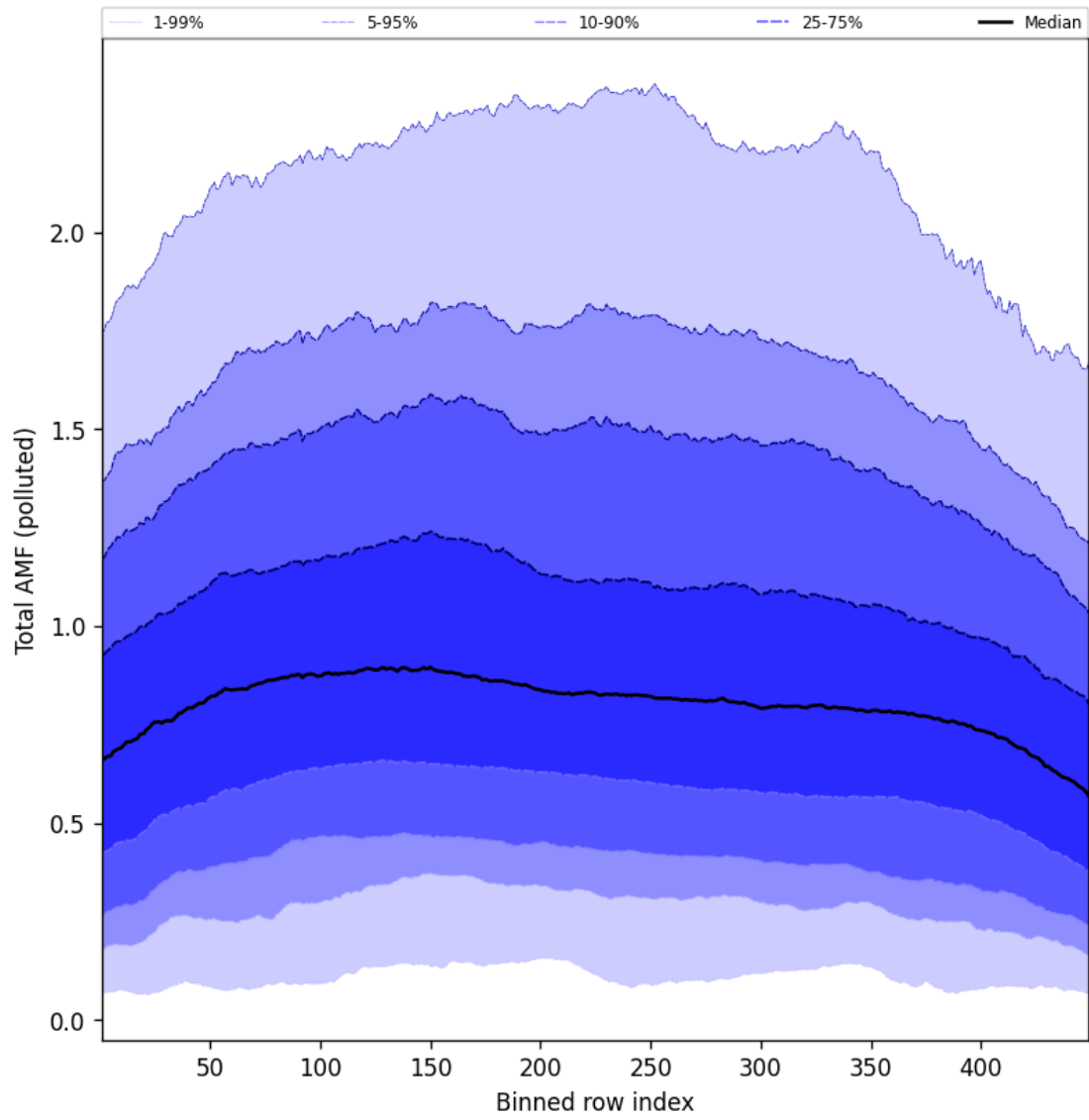
Figure 107: Along track statistics of “Total AMF (polluted)” for 2025-08-21 to 2025-08-22
