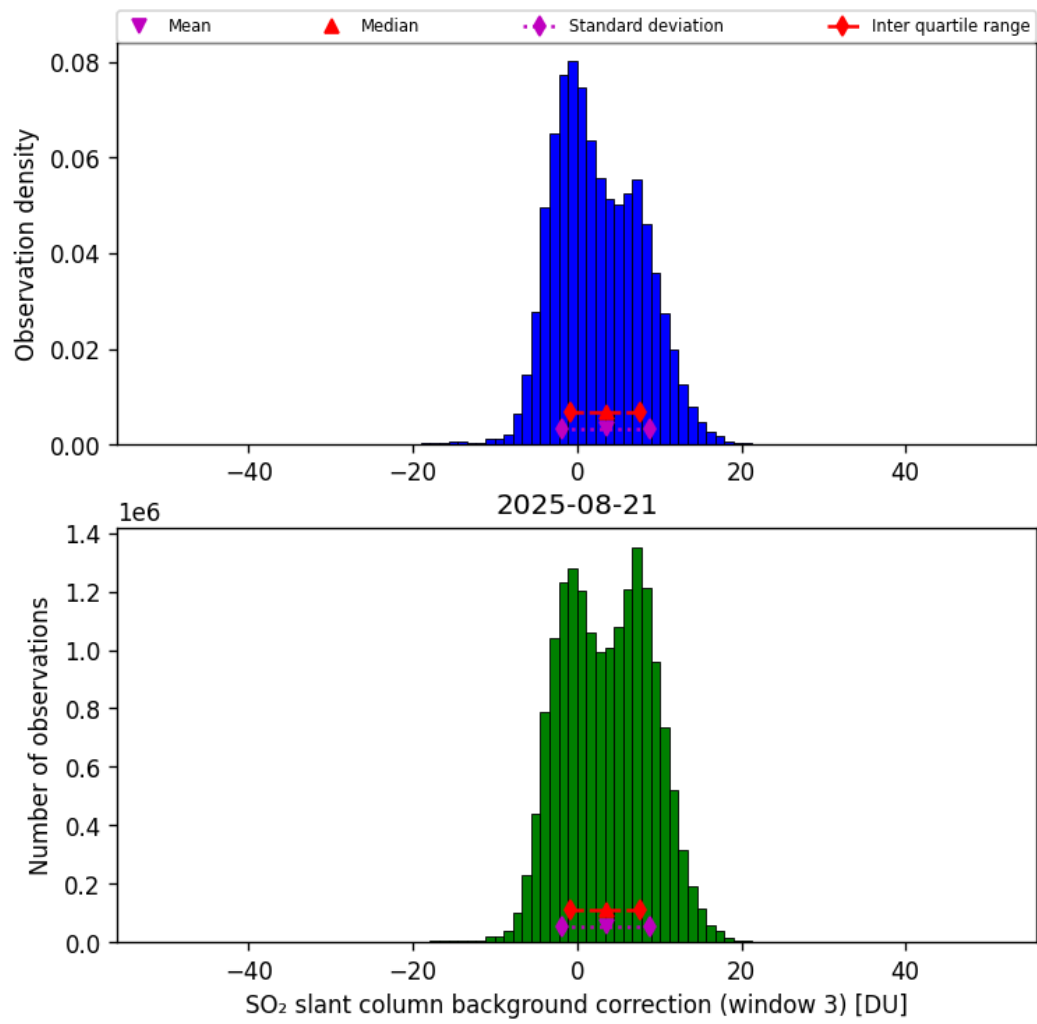
Figure 74: Histogram of “SO 2 slant column background correction (window 3)” for 2025-08-21 to 2025-08-22
