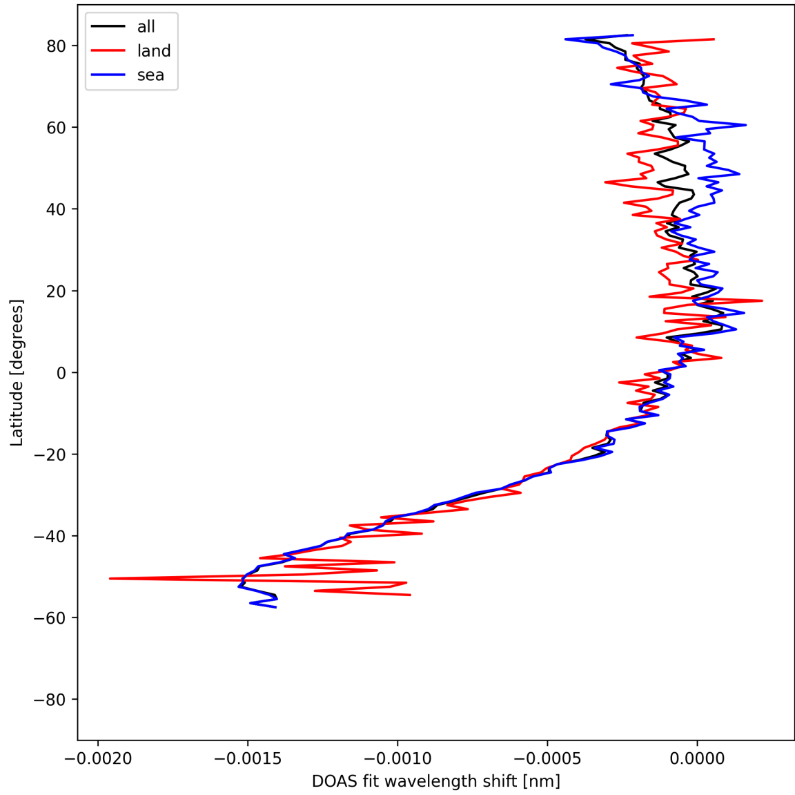
Figure 50: Zonal average of “DOAS fit wavelength shift” for 2025-08-21 to 2025-08-22.
