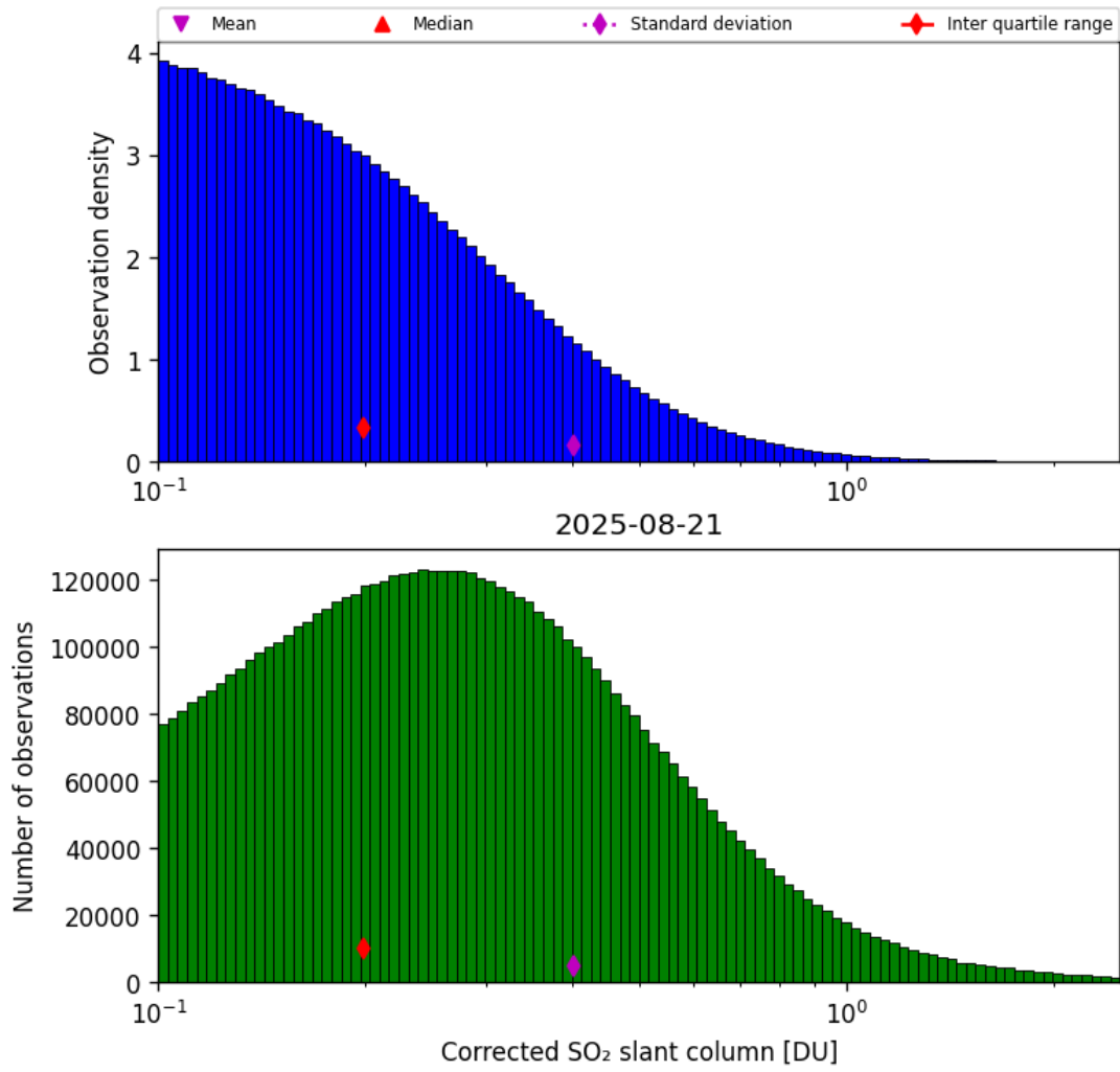
Figure 60: Histogram of “Corrected SO 2 slant column” for 2025-08-21 to 2025-08-22
