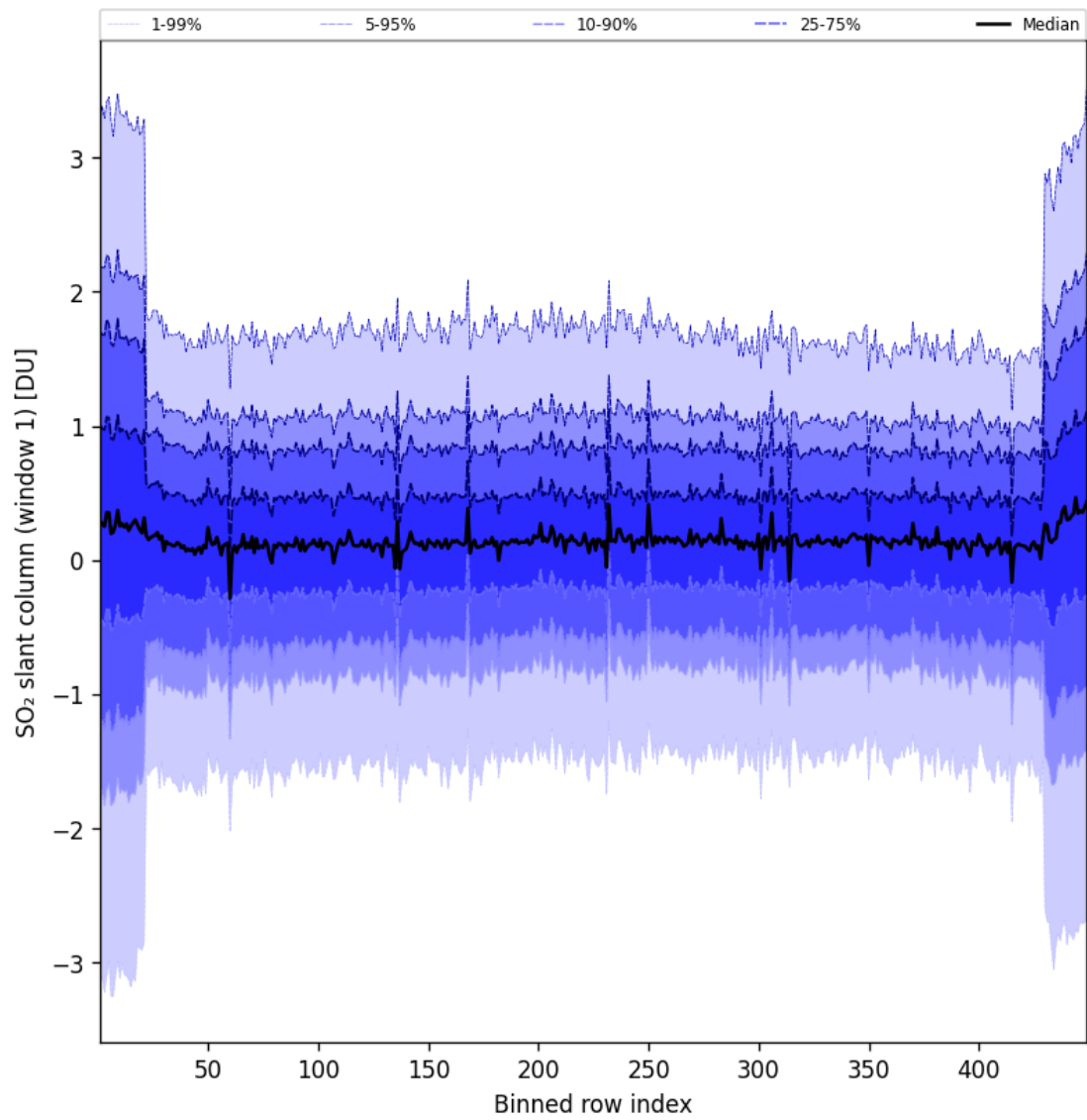
Figure 90: Along track statistics of “SO 2 slant column (window 1)” for 2025-08-21 to 2025-08-22
