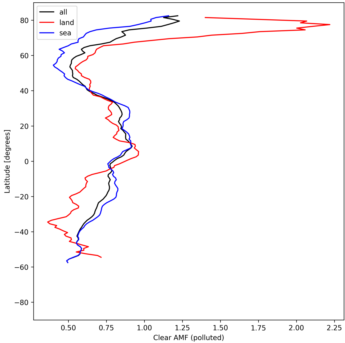
Figure 55: Zonal average of “Clear AMF (polluted)” for 2025-08-21 to 2025-08-22.
