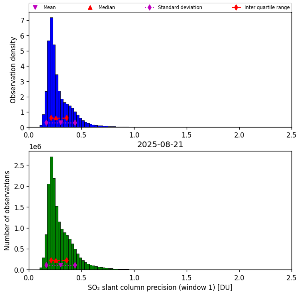
Figure 64: Histogram of “SO 2 slant column precision (window 1)” for 2025-08-21 to 2025-08-22
