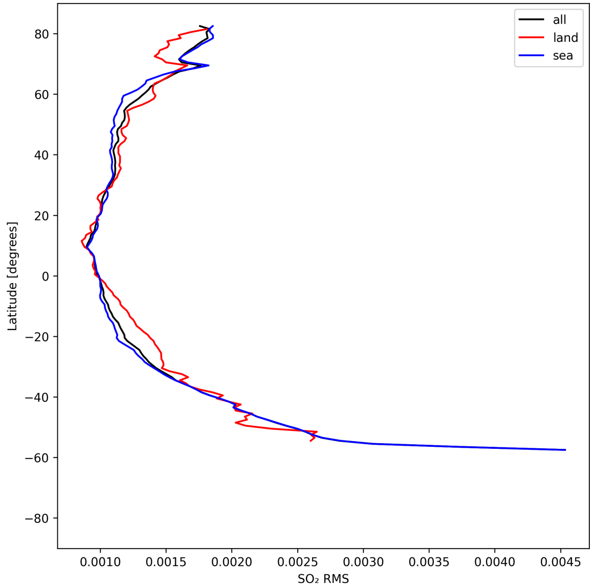
Figure 52: Zonal average of “SO 2 RMS” for 2025-08-21 to 2025-08-22.
