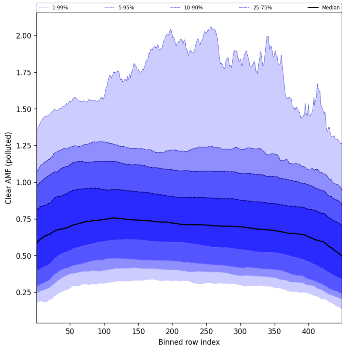
Figure 109: Along track statistics of “Clear AMF (polluted)” for 2025-08-21 to 2025-08-22
