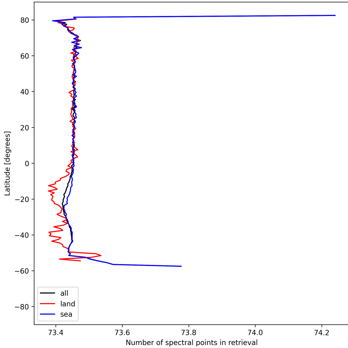
Figure 56: Zonal average of “Number of spectral points in retrieval” for 2025-08-21 to 2025-08-22.
