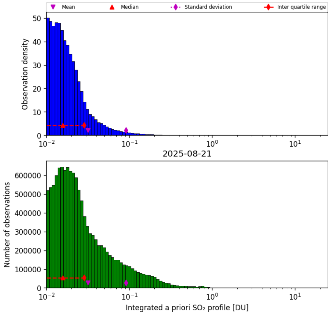
Figure 76: Histogram of “Integrated a priori SO 2 profile” for 2025-08-21 to 2025-08-22
