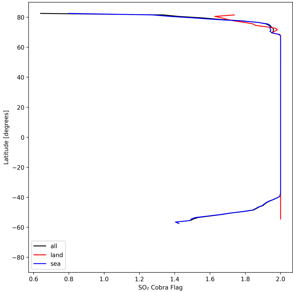
Figure 48: Zonal average of “SO 2 Cobra Flag” for 2025-08-21 to 2025-08-22.
