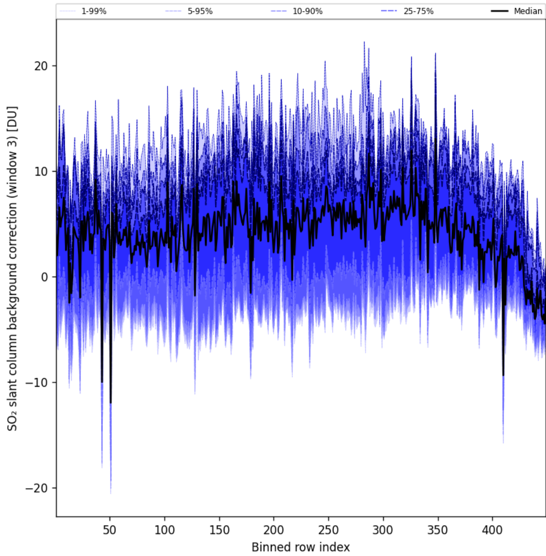
Figure 101: Along track statistics of “SO 2 slant column background correction (window 3)” for 2025-08-21 to 2025-08-22
