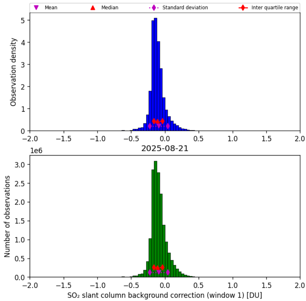
Figure 66: Histogram of “SO 2 slant column background correction (window 1)” for 2025-08-21 to 2025-08-22
