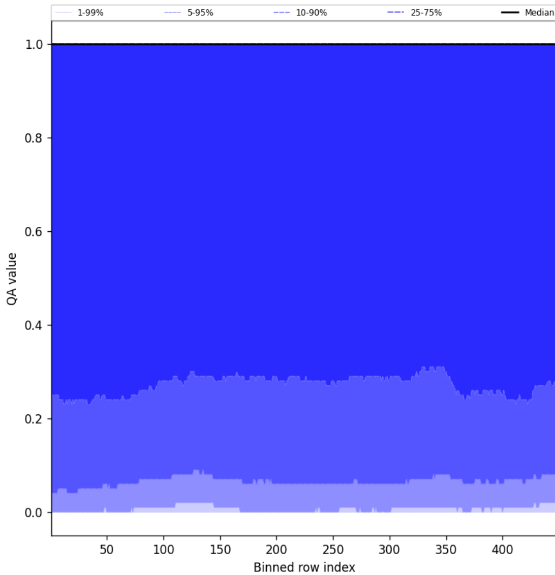
Figure 84: Along track statistics of “QA value” for 2025-08-21 to 2025-08-22
