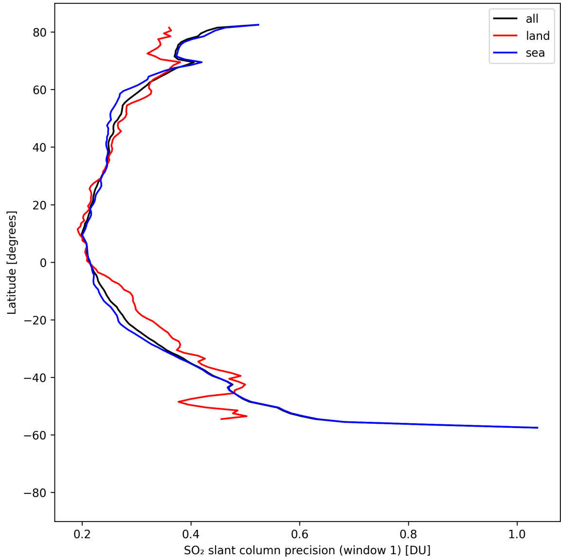
Figure 37: Zonal average of “SO 2 slant column precision (window 1)” for 2025-08-21 to 2025-08-22.
