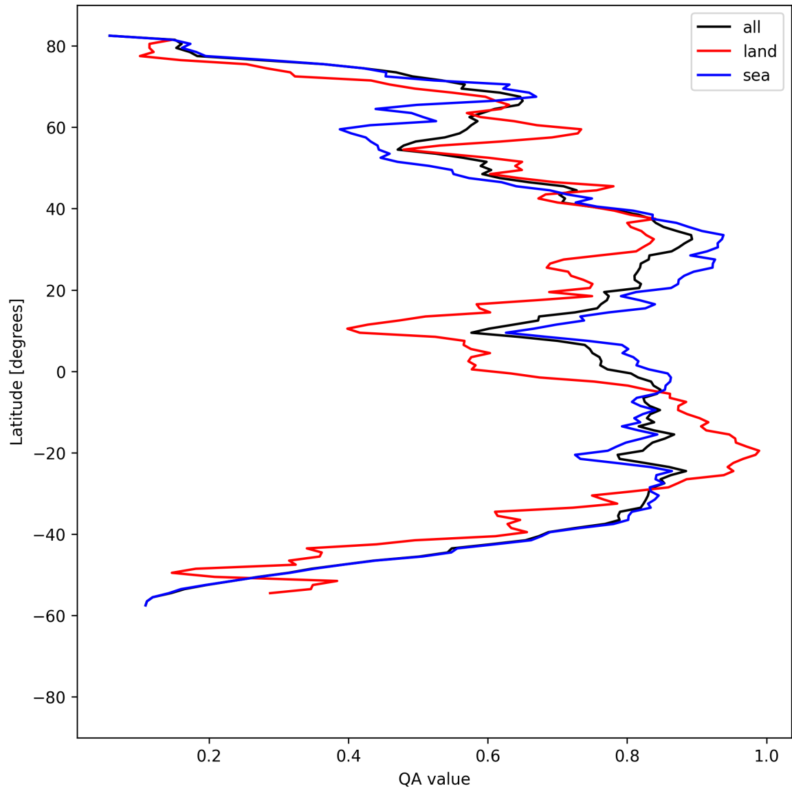
Figure 30: Zonal average of “QA value” for 2025-08-21 to 2025-08-22.
