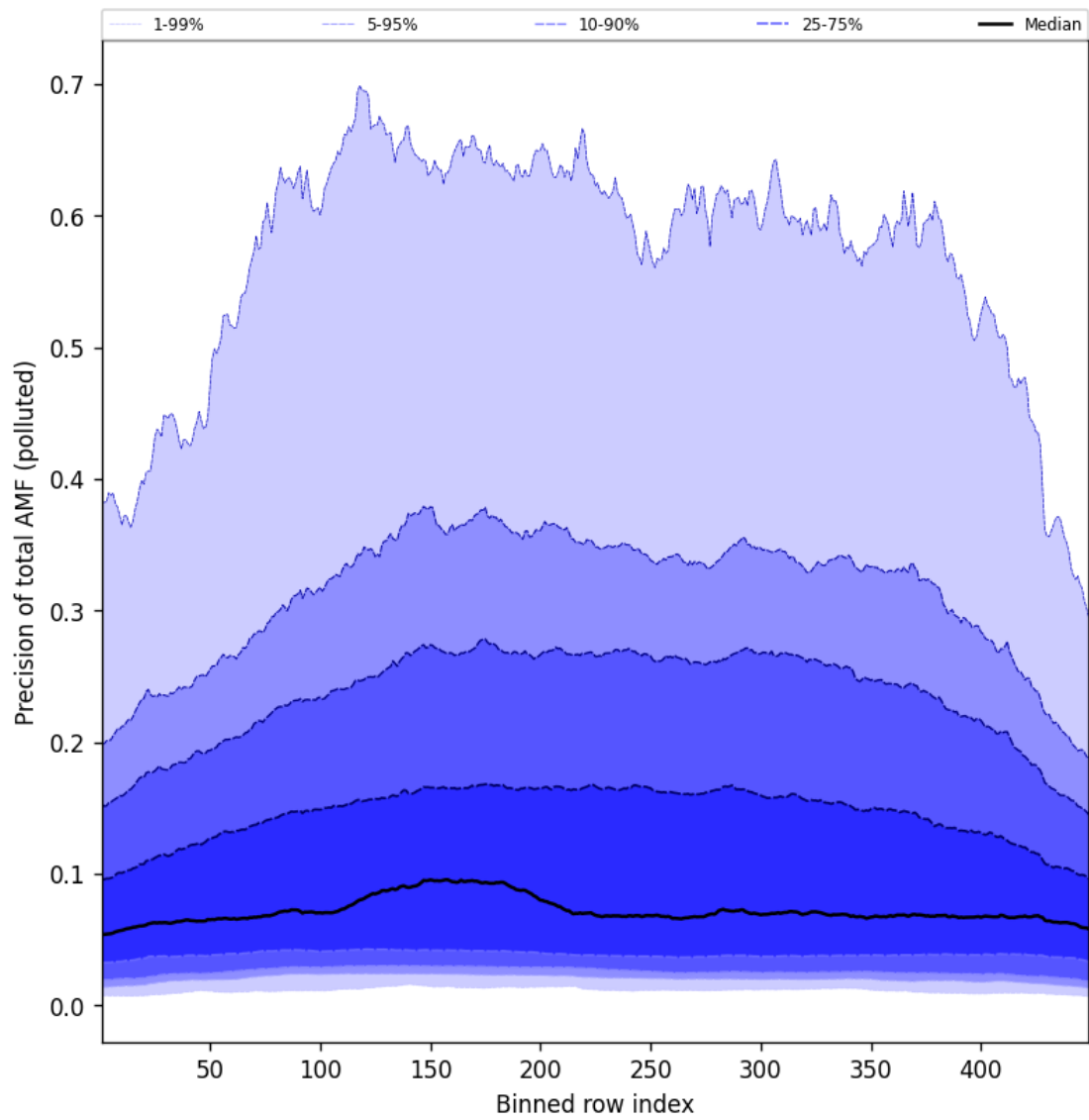
Figure 108: Along track statistics of “Precision of total AMF (polluted)” for 2025-08-21 to 2025-08-22
