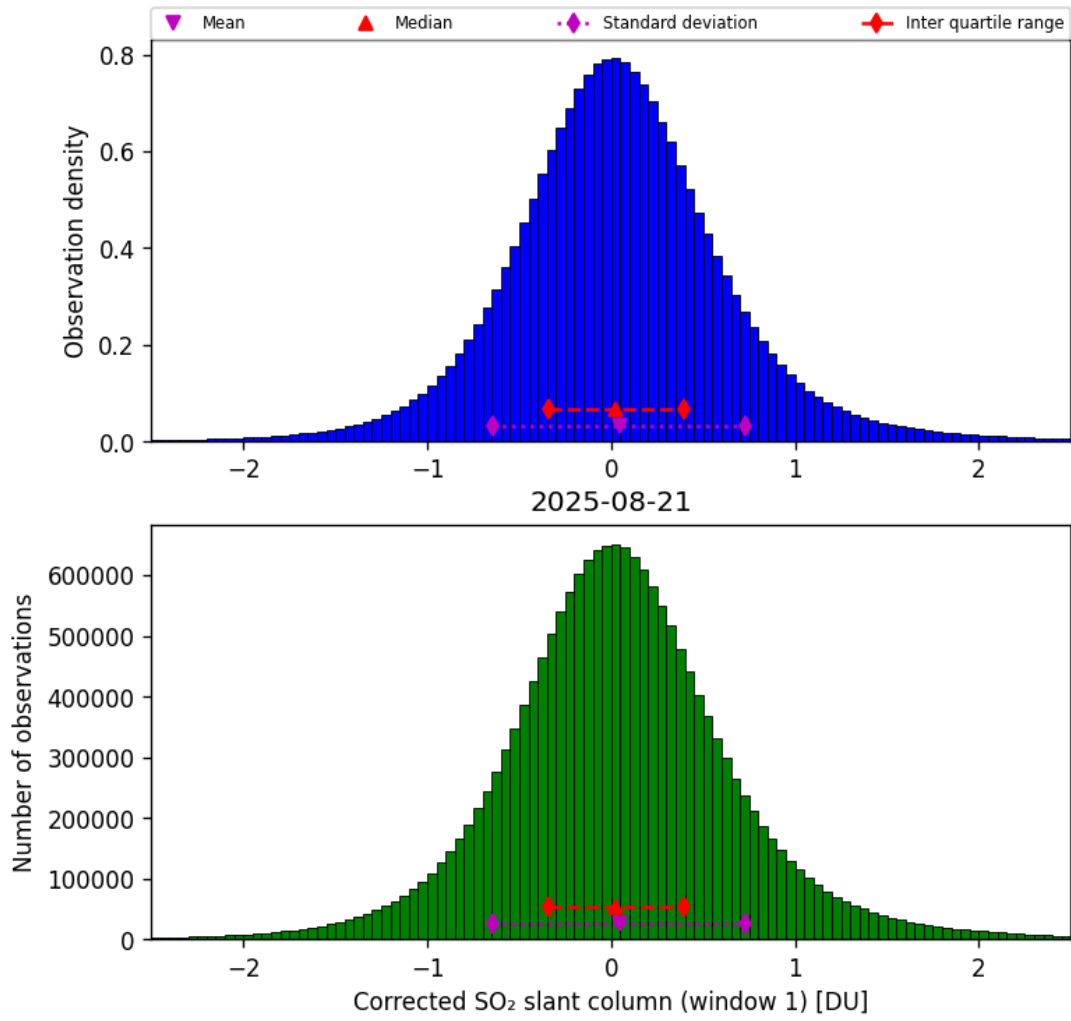
Figure 65: Histogram of “Corrected SO 2 slant column (window 1)” for 2025-08-21 to 2025-08-22
