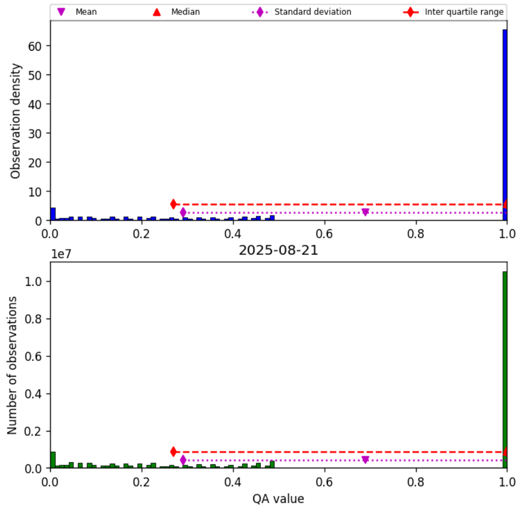
Figure 57: Histogram of “QA value” for 2025-08-21 to 2025-08-22
