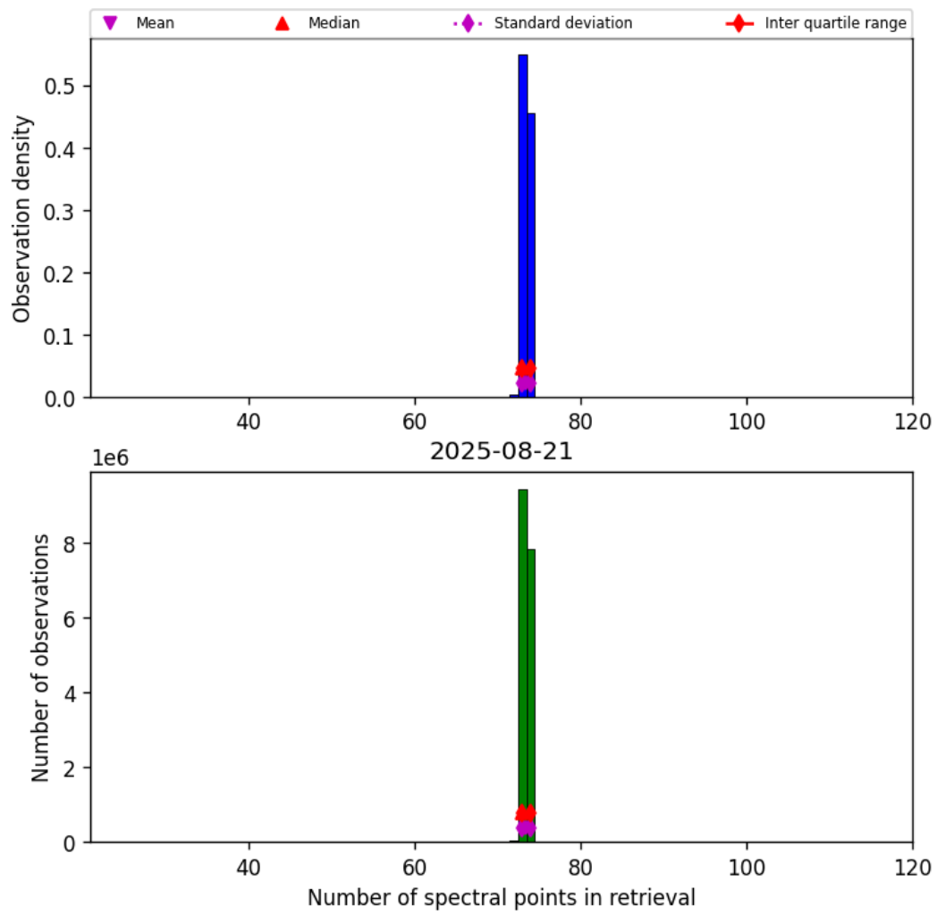
Figure 83: Histogram of “Number of spectral points in retrieval” for 2025-08-21 to 2025-08-22
