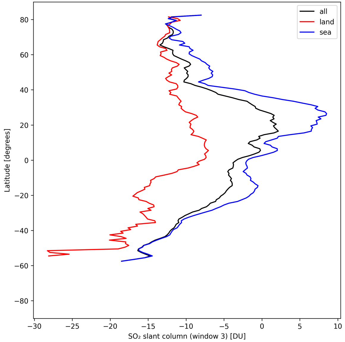
Figure 44: Zonal average of “SO 2 slant column (window 3)” for 2025-08-21 to 2025-08-22.
