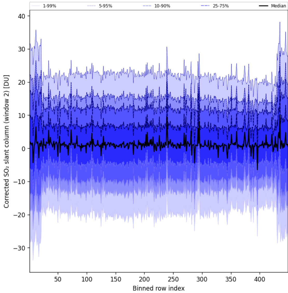
Figure 96: Along track statistics of “Corrected SO 2 slant column (window 2)” for 2025-08-21 to 2025-08-22
