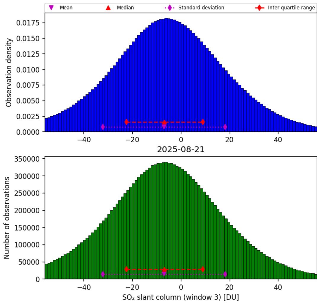
Figure 71: Histogram of “SO 2 slant column (window 3)” for 2025-08-21 to 2025-08-22
