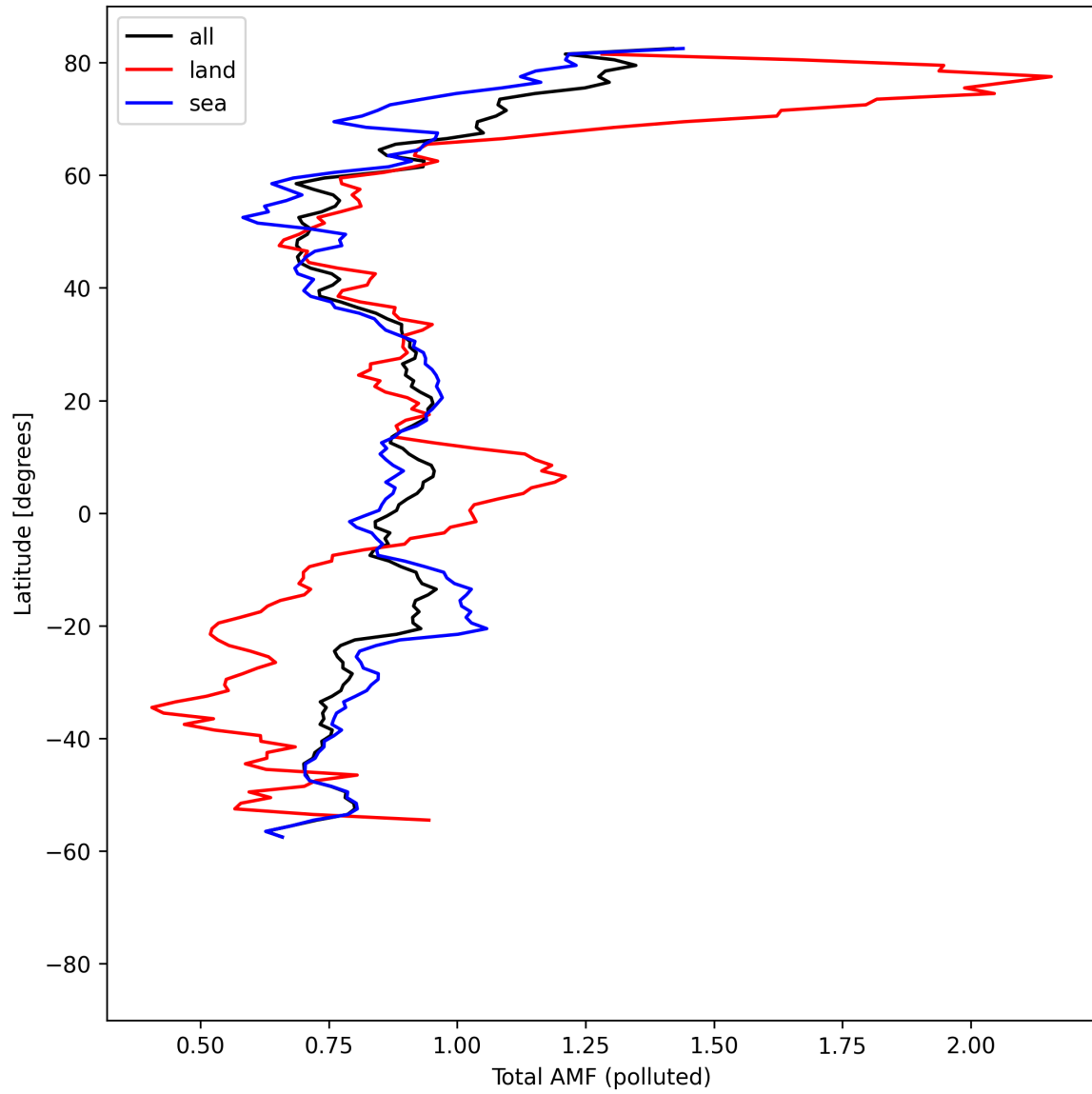
Figure 53: Zonal average of “Total AMF (polluted)” for 2025-08-21 to 2025-08-22.
