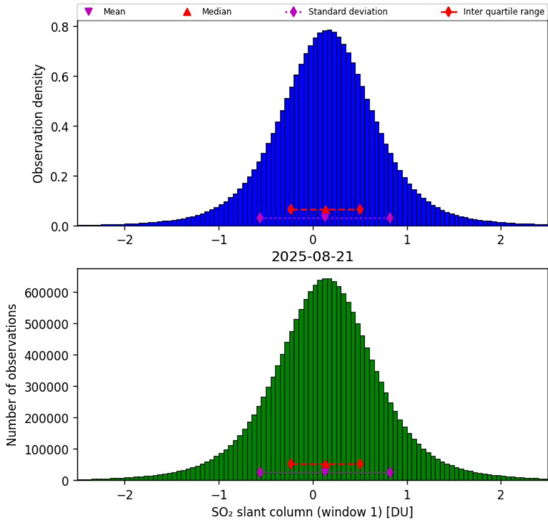
Figure 63: Histogram of “SO 2 slant column (window 1)” for 2025-08-21 to 2025-08-22
