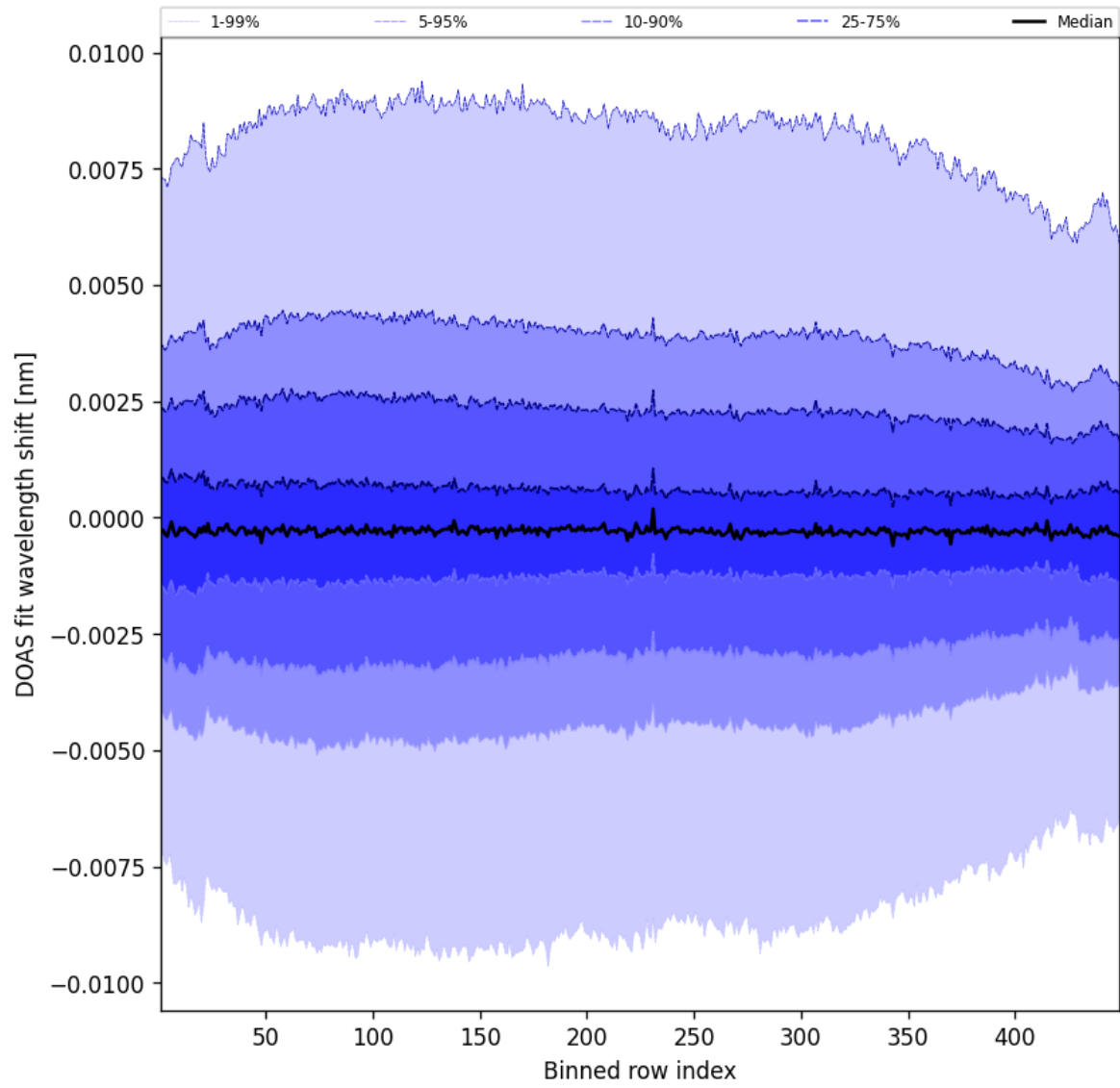
Figure 104: Along track statistics of “DOAS fit wavelength shift” for 2025-08-21 to 2025-08-22
