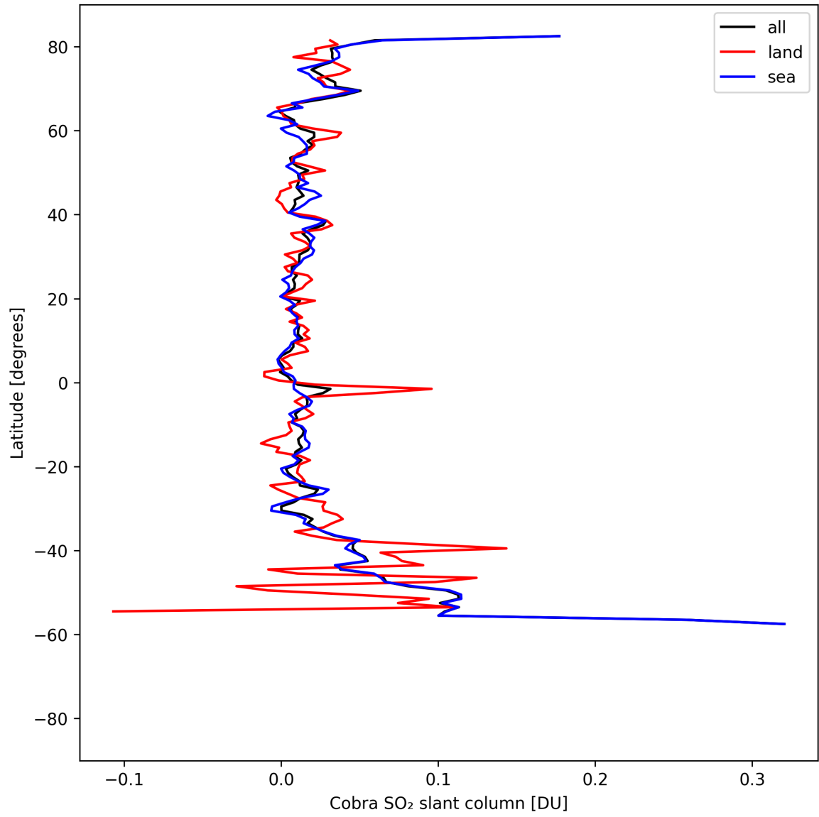
Figure 34: Zonal average of “Cobra SO 2 slant column” for 2025-08-21 to 2025-08-22.
