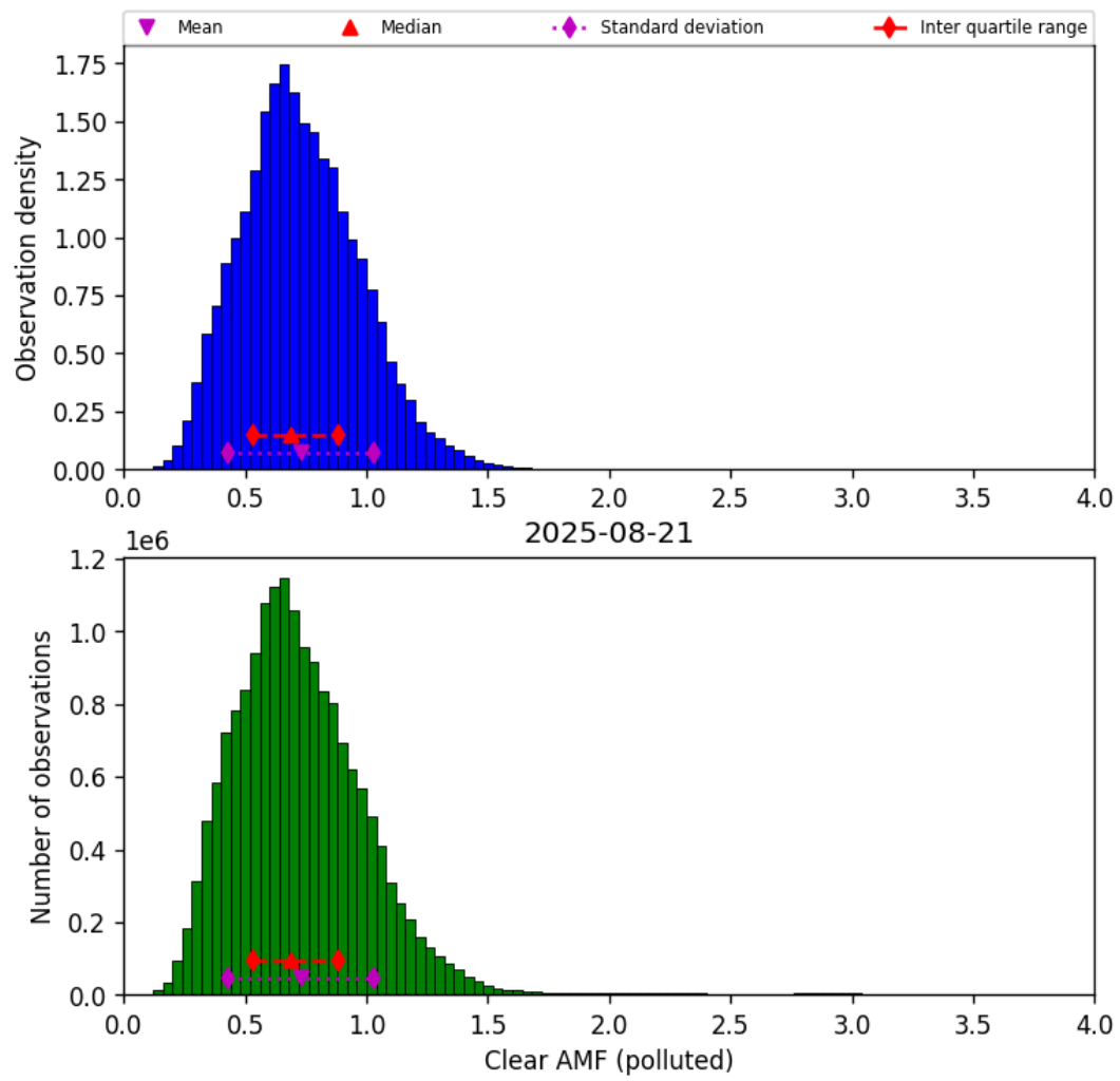
Figure 82: Histogram of “Clear AMF (polluted)” for 2025-08-21 to 2025-08-22
