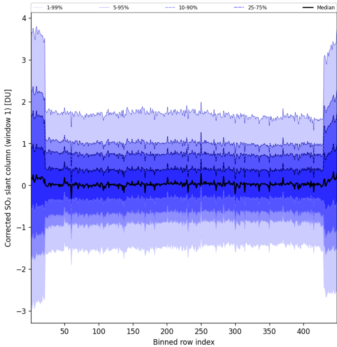
Figure 92: Along track statistics of “Corrected SO 2 slant column (window 1)” for 2025-08-21 to 2025-08-22
