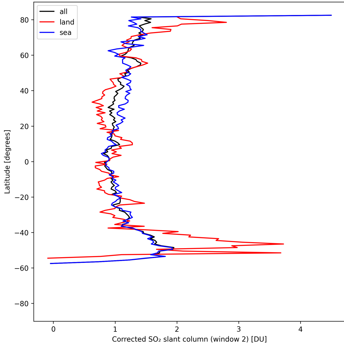
Figure 42: Zonal average of "Corrected SO 2 slant column (window 2)" for 2025-08-21 to 2025-08-22.
