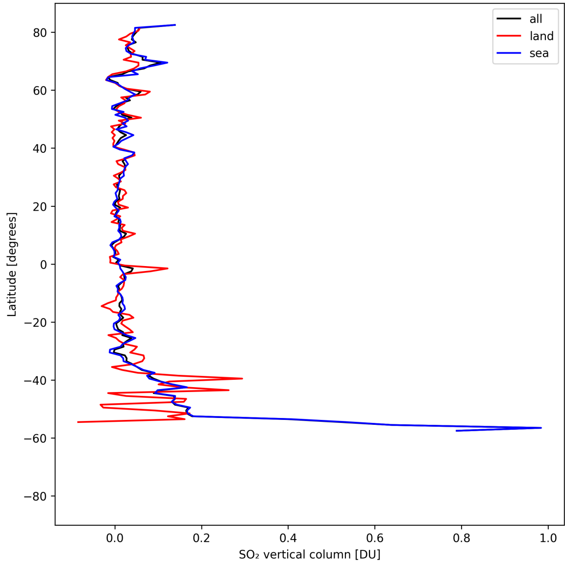
Figure 31: Zonal average of “SO 2 vertical column” for 2025-08-21 to 2025-08-22.
