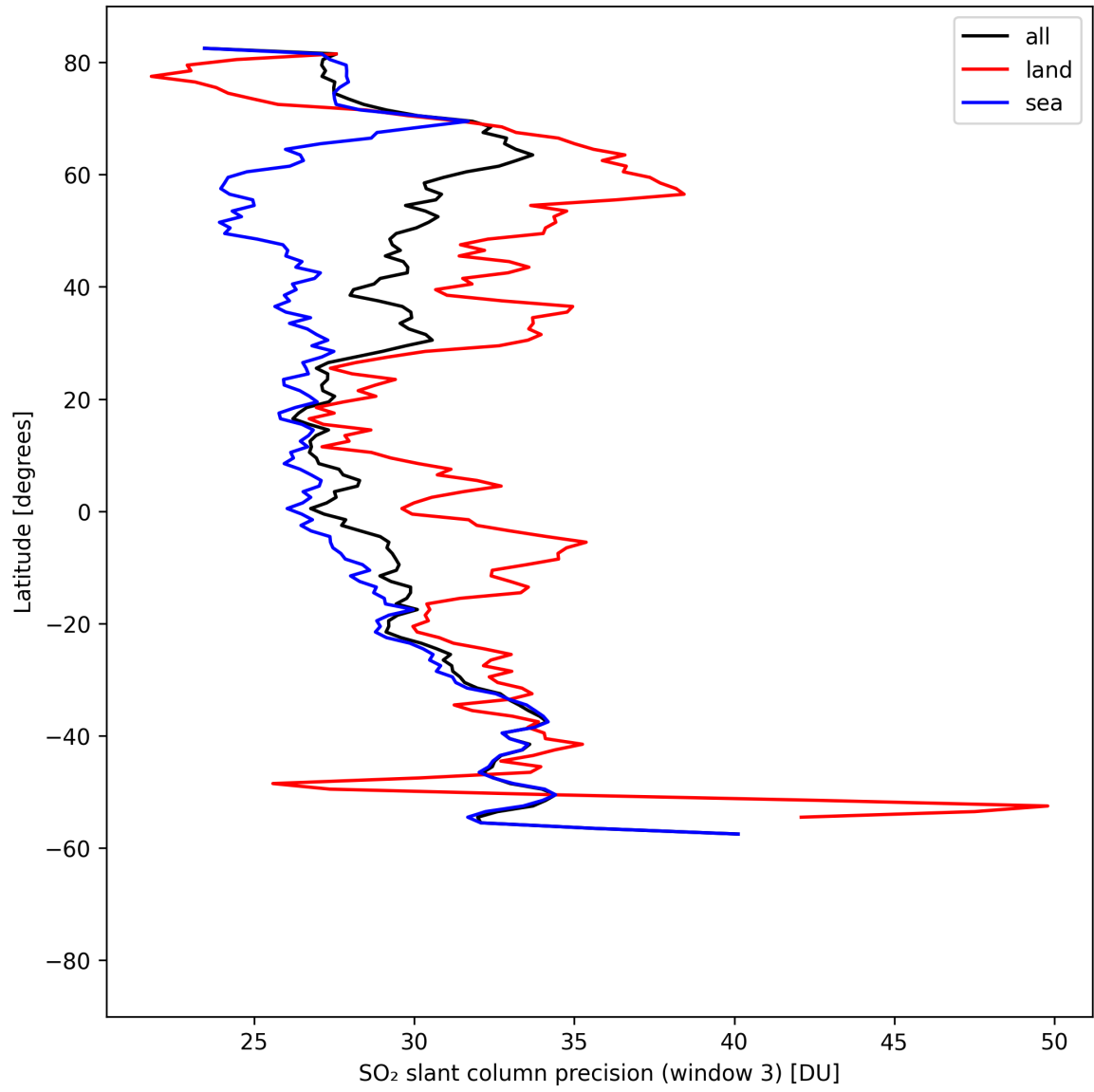
Figure 45: Zonal average of “SO 2 slant column precision (window 3)” for 2025-08-21 to 2025-08-22.
