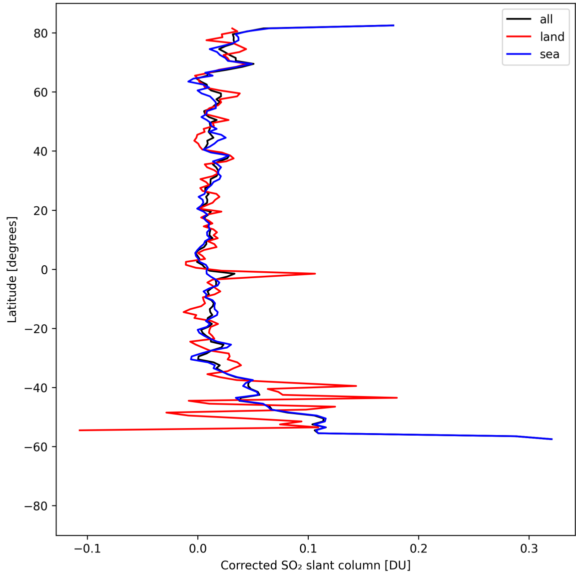
Figure 33: Zonal average of “Corrected SO 2 slant column” for 2025-08-21 to 2025-08-22.
