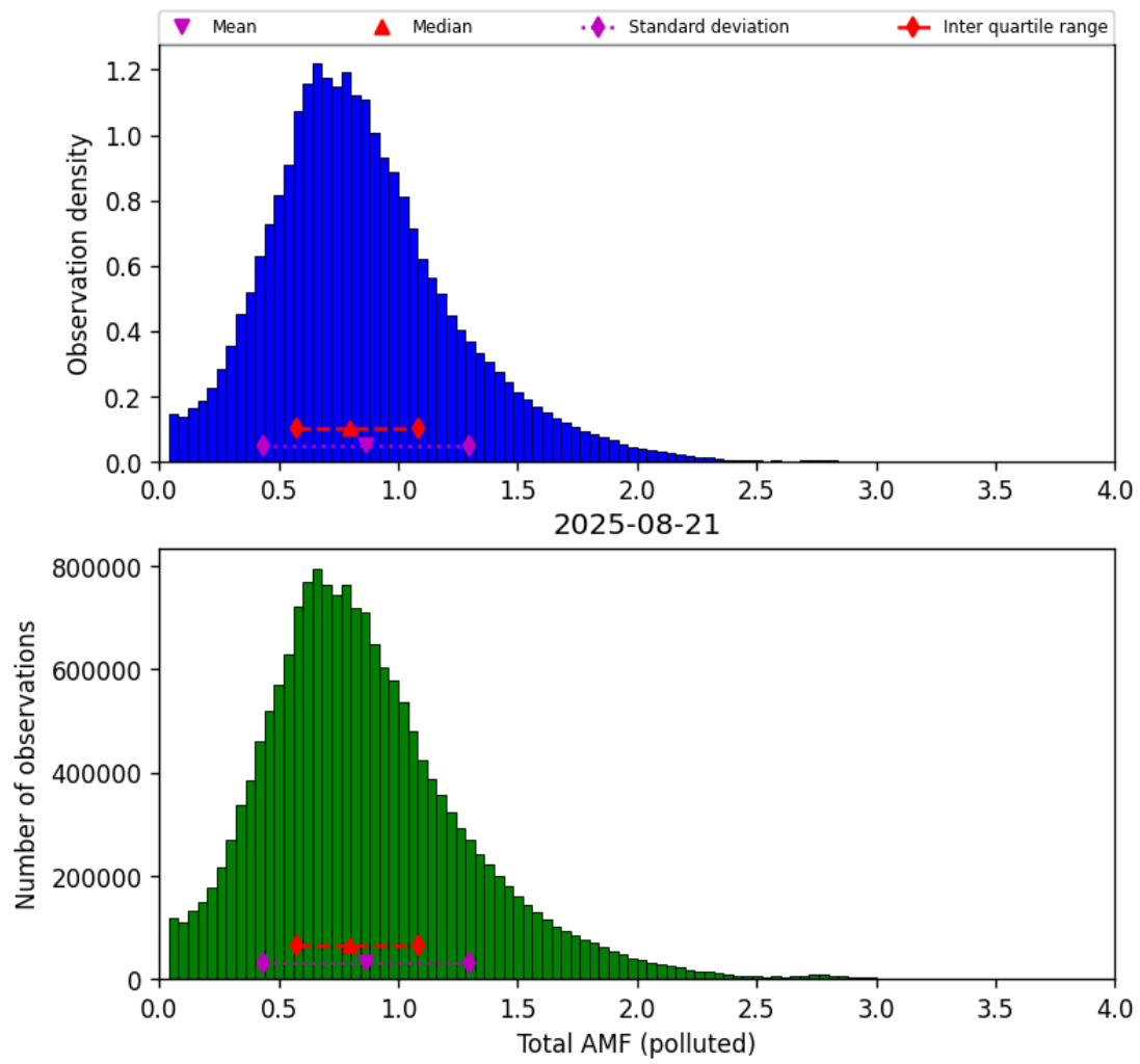
Figure 80: Histogram of “Total AMF (polluted)” for 2025-08-21 to 2025-08-22
