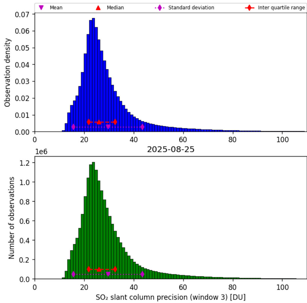
Figure 72: Histogram of “SO 2 slant column precision (window 3)” for 2025-08-25 to 2025-08-26
