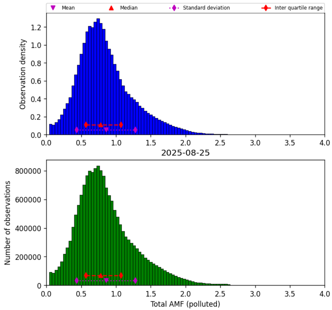
Figure 80: Histogram of “Total AMF (polluted)” for 2025-08-25 to 2025-08-26
