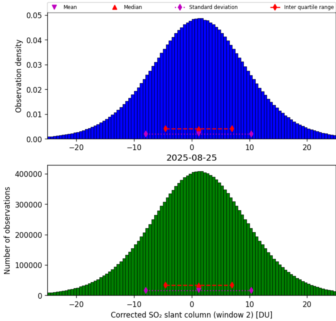
Figure 69: Histogram of “Corrected SO 2 slant column (window 2)” for 2025-08-25 to 2025-08-26
