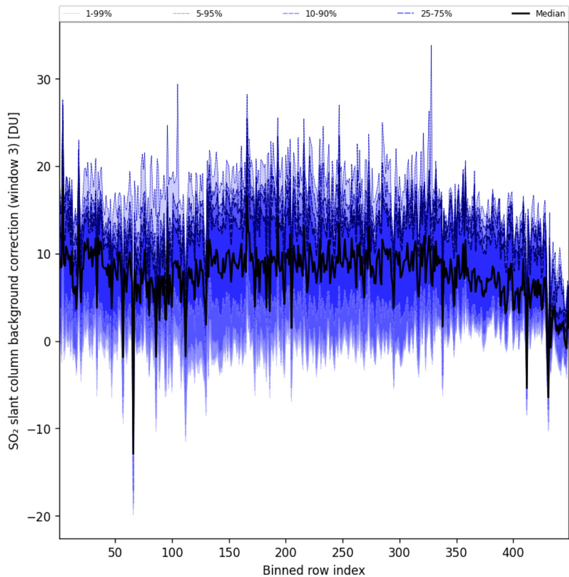
Figure 101: Along track statistics of “SO 2 slant column background correction (window 3)” for 2025-08-25 to 2025-08-26
