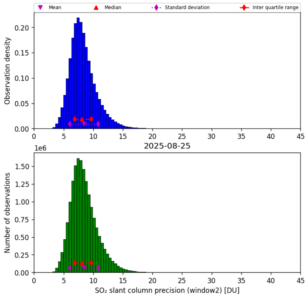
Figure 68: Histogram of “SO 2 slant column precision (window2)” for 2025-08-25 to 2025-08-26
