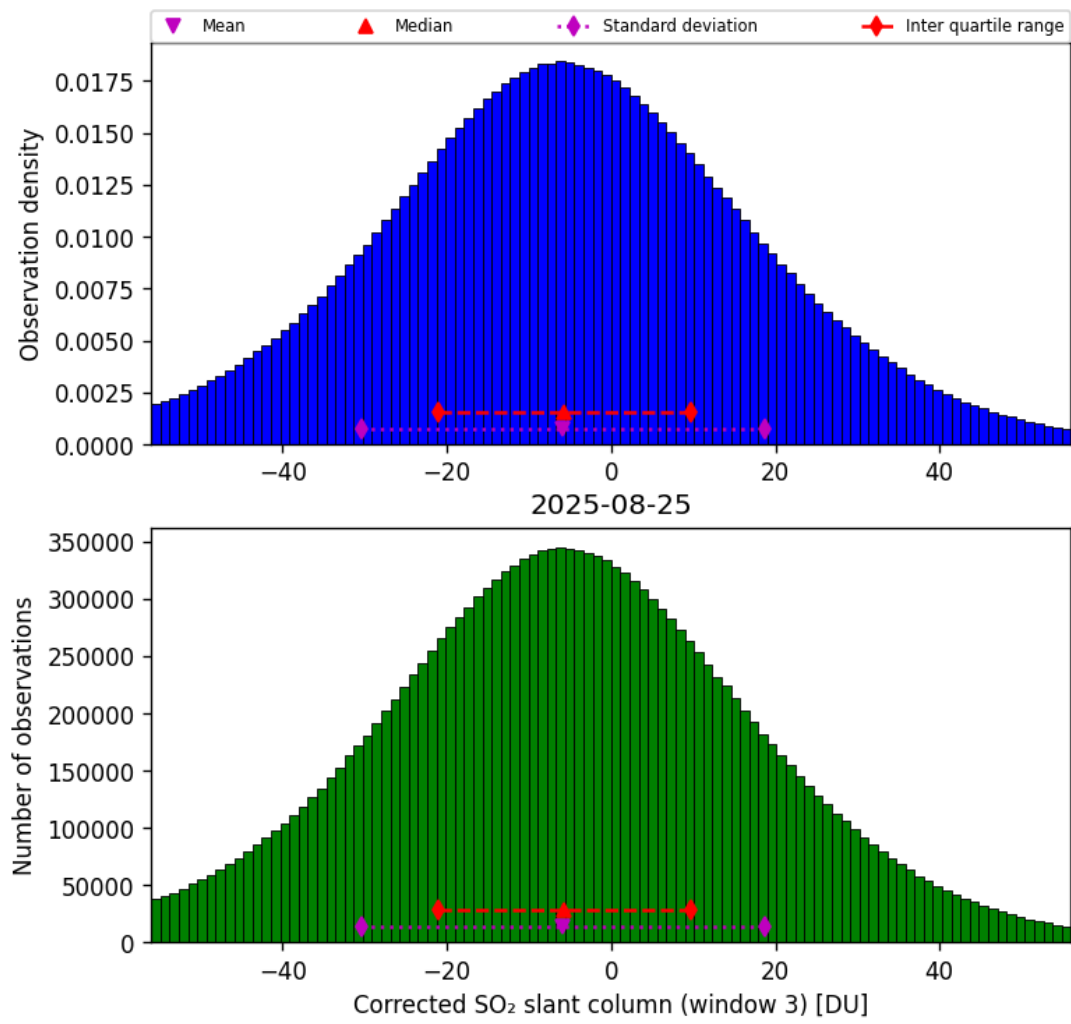
Figure 73: Histogram of “Corrected SO 2 slant column (window 3)” for 2025-08-25 to 2025-08-26
