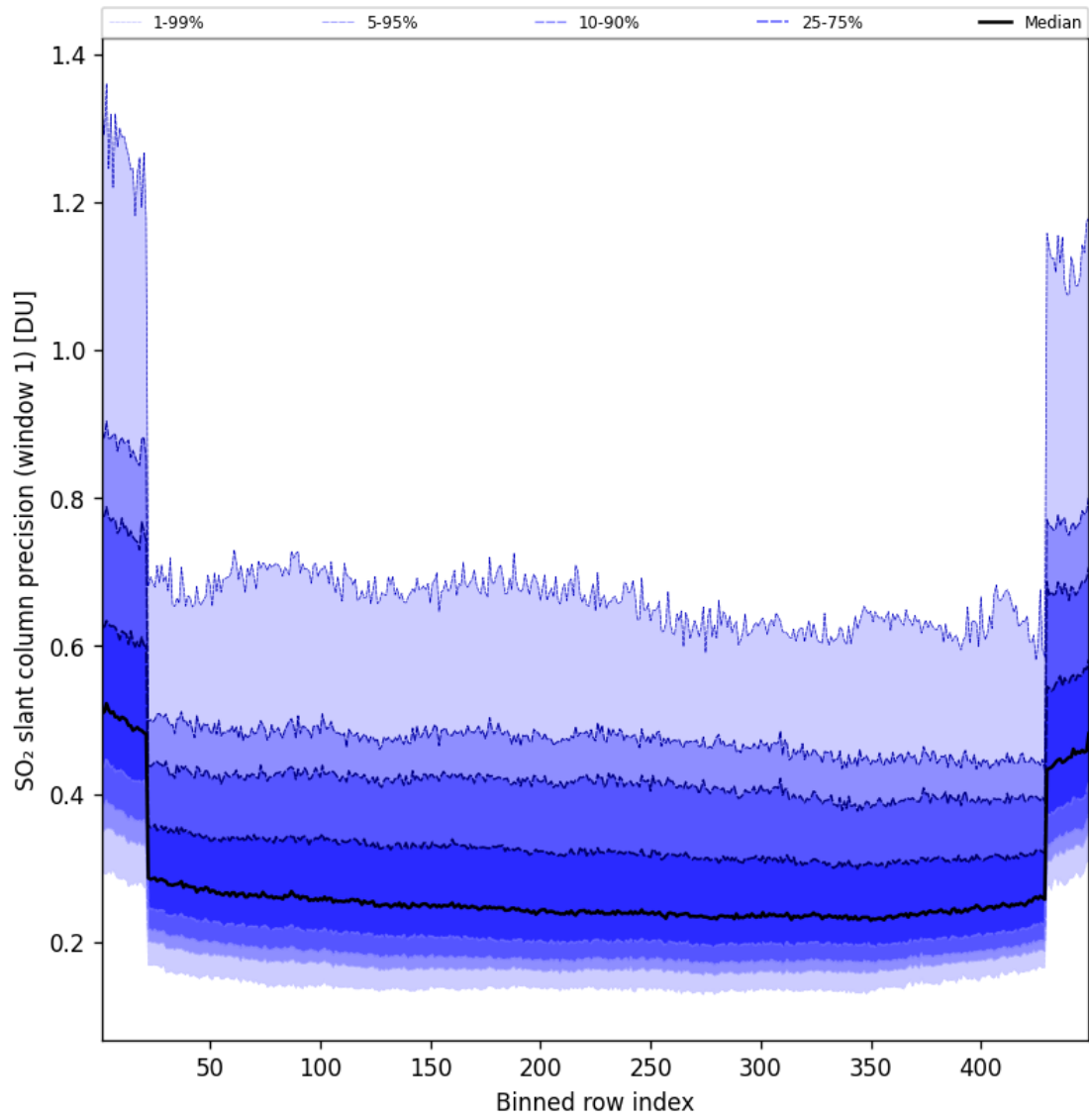
Figure 91: Along track statistics of “SO 2 slant column precision (window 1)” for 2025-08-25 to 2025-08-26
