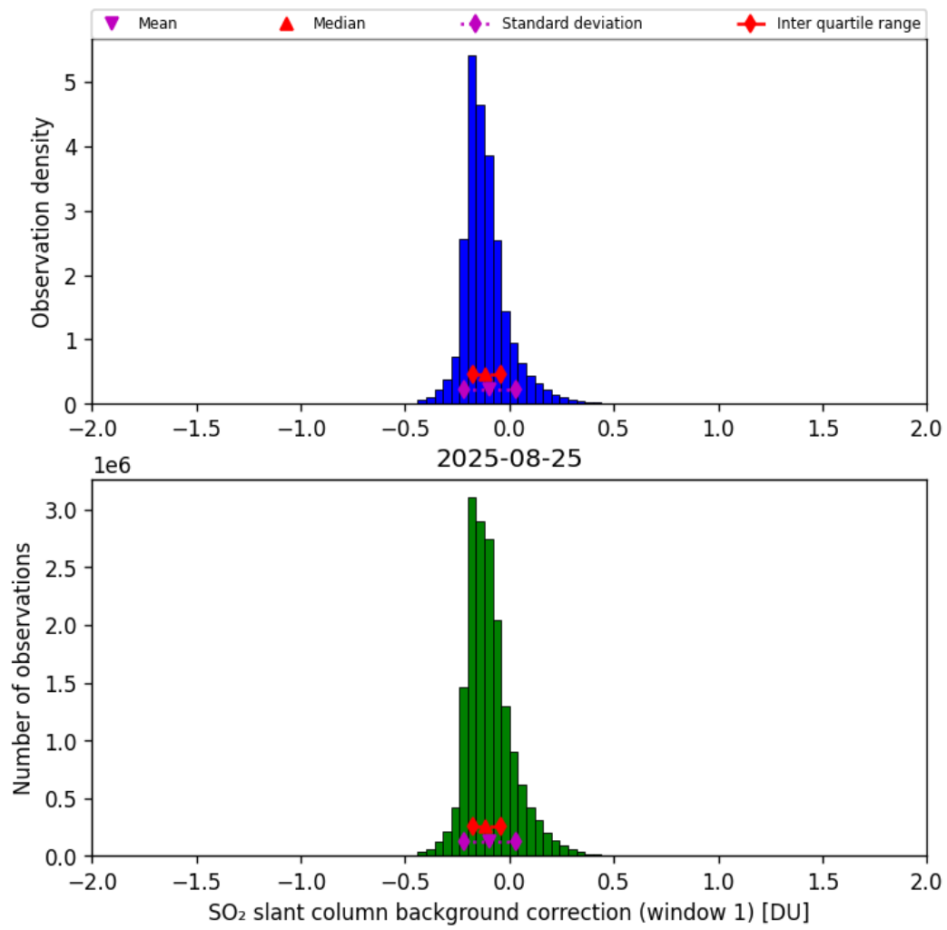
Figure 66: Histogram of “SO 2 slant column background correction (window 1)” for 2025-08-25 to 2025-08-26
