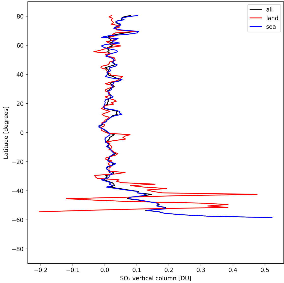
Figure 31: Zonal average of “SO 2 vertical column” for 2025-08-25 to 2025-08-26.
