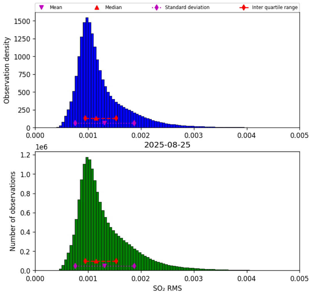
Figure 79: Histogram of "SO 2 RMS" for 2025-08-25 to 2025-08-26
