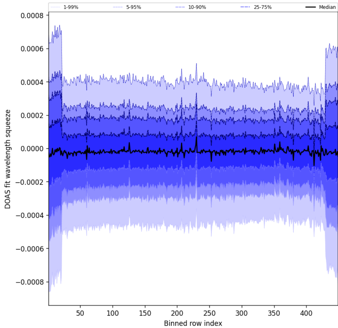
Figure 105: Along track statistics of “DOAS fit wavelength squeeze” for 2025-08-25 to 2025-08-26
