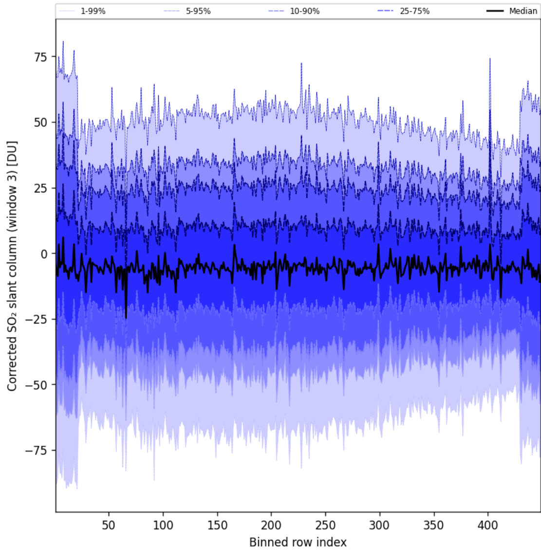
Figure 100: Along track statistics of “Corrected SO 2 slant column (window 3)” for 2025-08-25 to 2025-08-26
