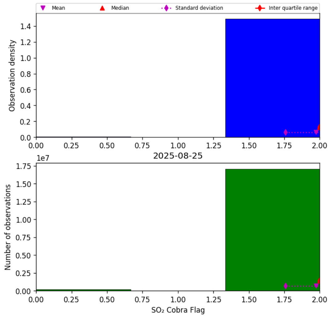
Figure 75: Histogram of "SO 2 Cobra Flag" for 2025-08-25 to 2025-08-26
