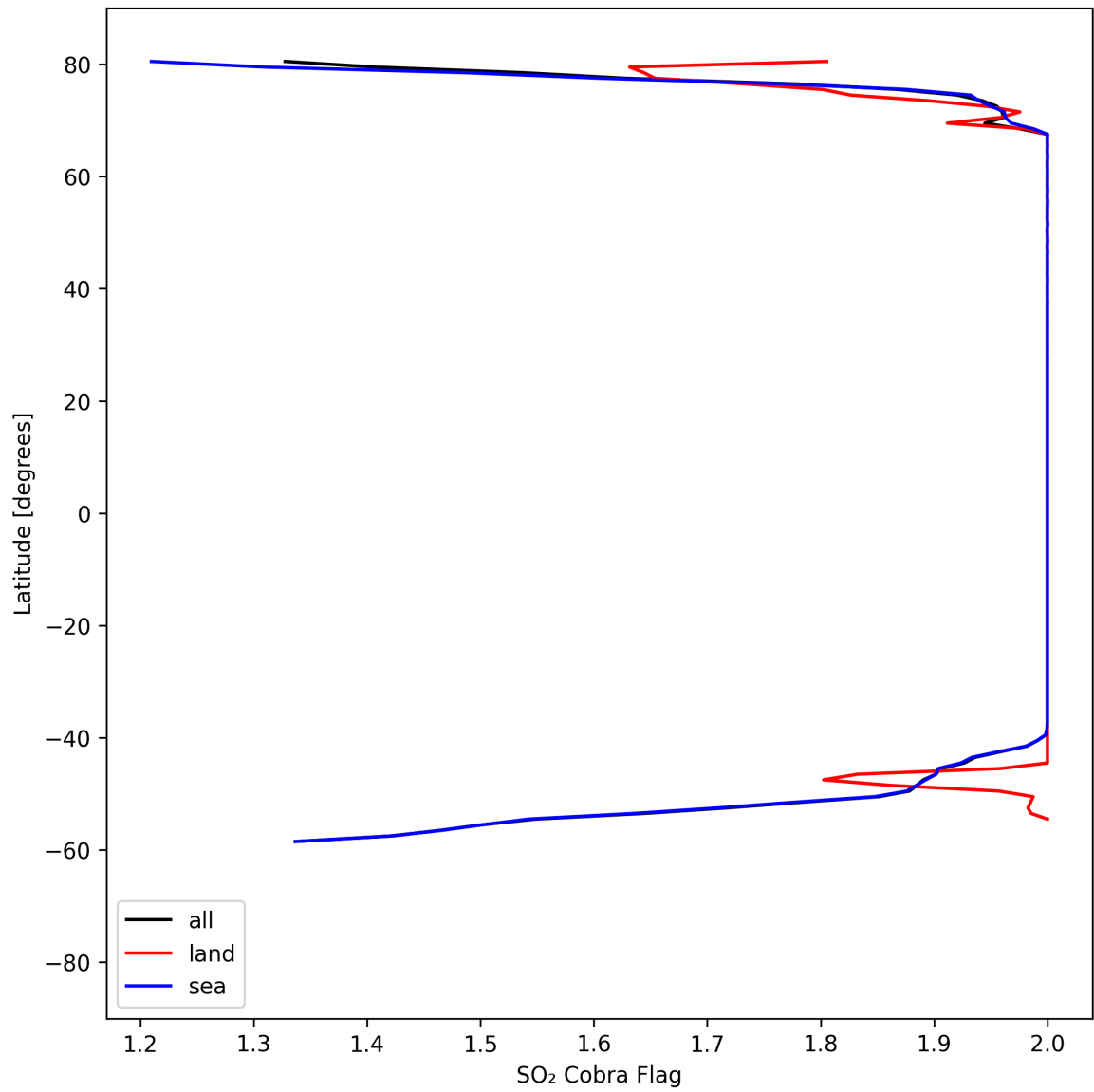
Figure 48: Zonal average of "SO 2 Cobra Flag" for 2025-08-25 to 2025-08-26.
