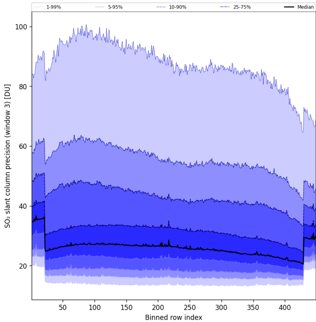
Figure 99: Along track statistics of “SO 2 slant column precision (window 3)” for 2025-08-25 to 2025-08-26
