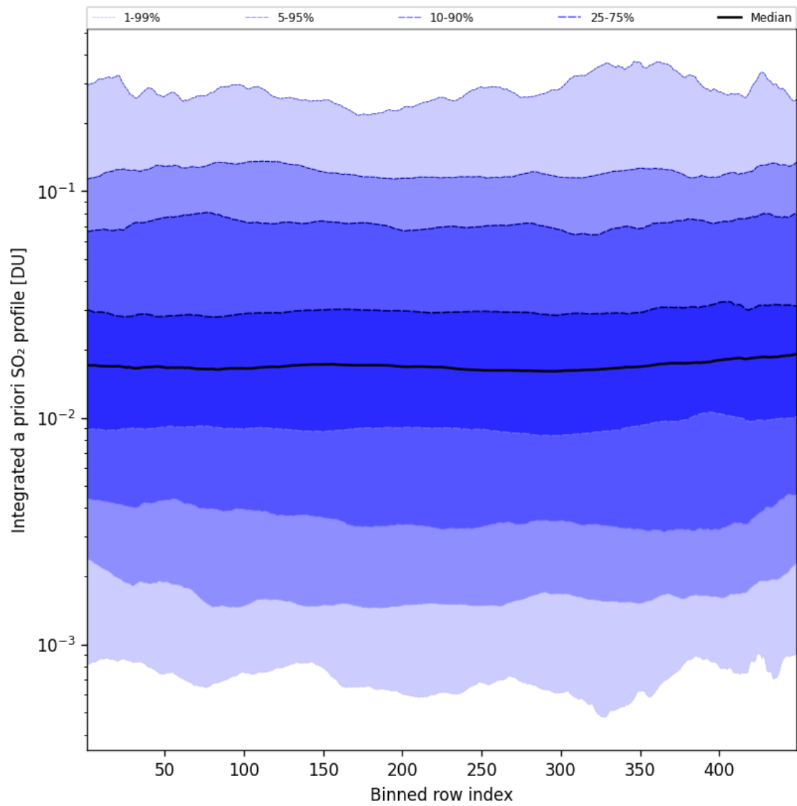
Figure 103: Along track statistics of “Integrated a priori SO 2 profile” for 2025-08-25 to 2025-08-26
