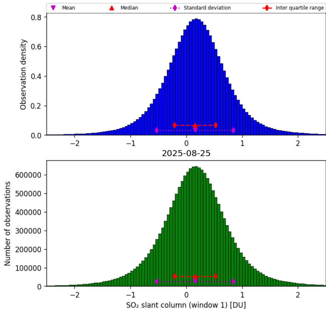
Figure 63: Histogram of “SO 2 slant column (window 1)” for 2025-08-25 to 2025-08-26
