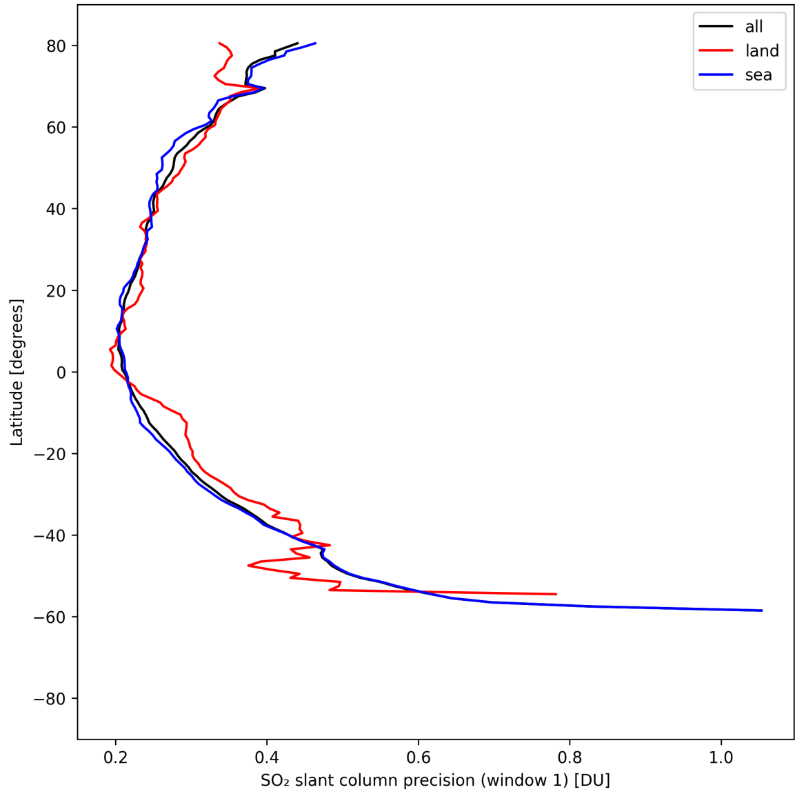
Figure 37: Zonal average of “SO 2 slant column precision (window 1)” for 2025-08-25 to 2025-08-26.
