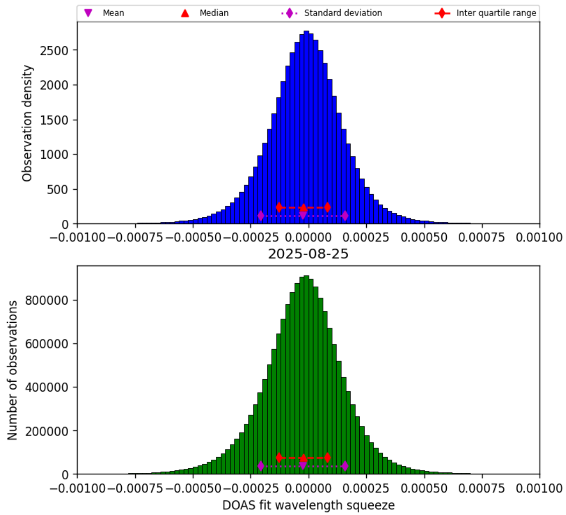
Figure 78: Histogram of “DOAS fit wavelength squeeze” for 2025-08-25 to 2025-08-26
