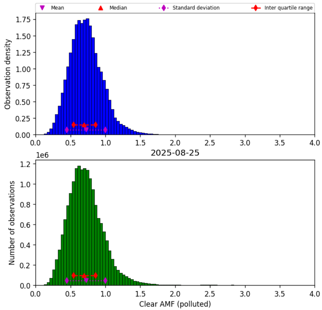
Figure 82: Histogram of “Clear AMF (polluted)” for 2025-08-25 to 2025-08-26
