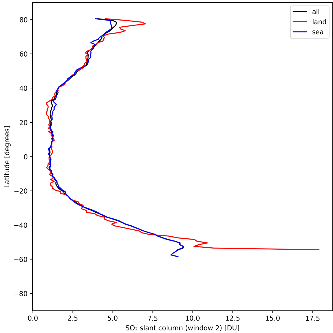
Figure 40: Zonal average of “SO 2 slant column (window 2)” for 2025-08-25 to 2025-08-26.
