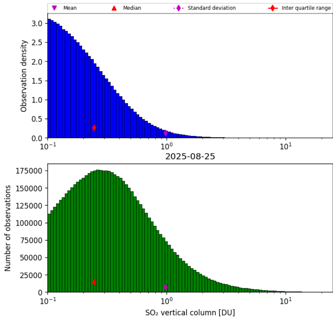
Figure 58: Histogram of “SO 2 vertical column” for 2025-08-25 to 2025-08-26
