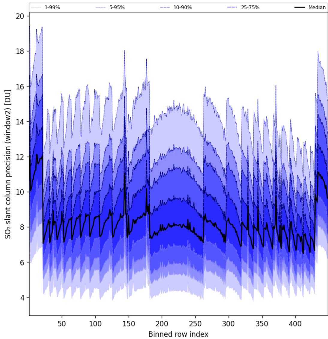
Figure 95: Along track statistics of “SO 2 slant column precision (window2)” for 2025-08-25 to 2025-08-26
