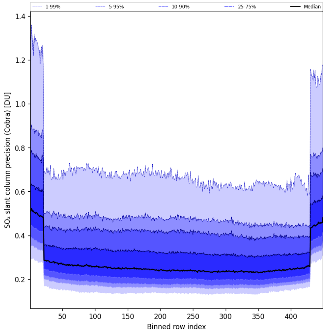
Figure 89: Along track statistics of “SO 2 slant column precision (Cobra)” for 2025-08-25 to 2025-08-26
