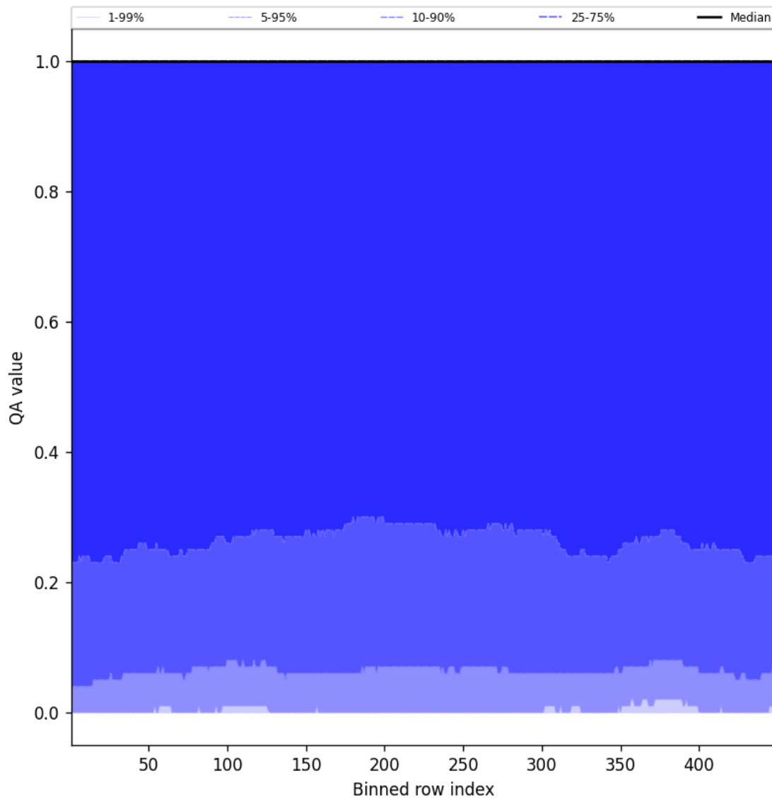
Figure 84: Along track statistics of “QA value” for 2025-08-25 to 2025-08-26
