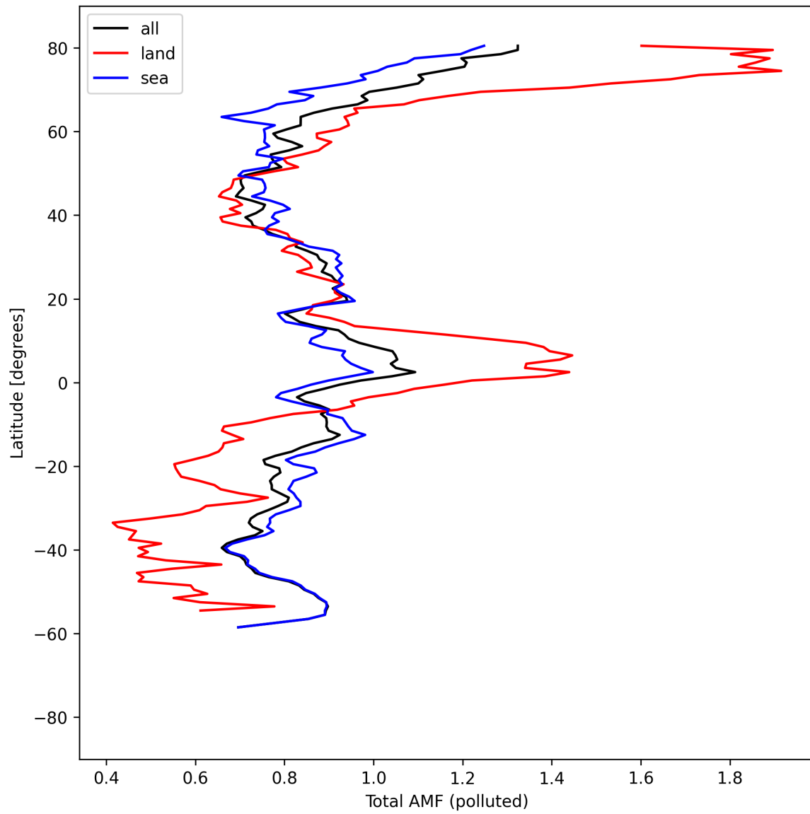
Figure 53: Zonal average of “Total AMF (polluted)” for 2025-08-25 to 2025-08-26.
