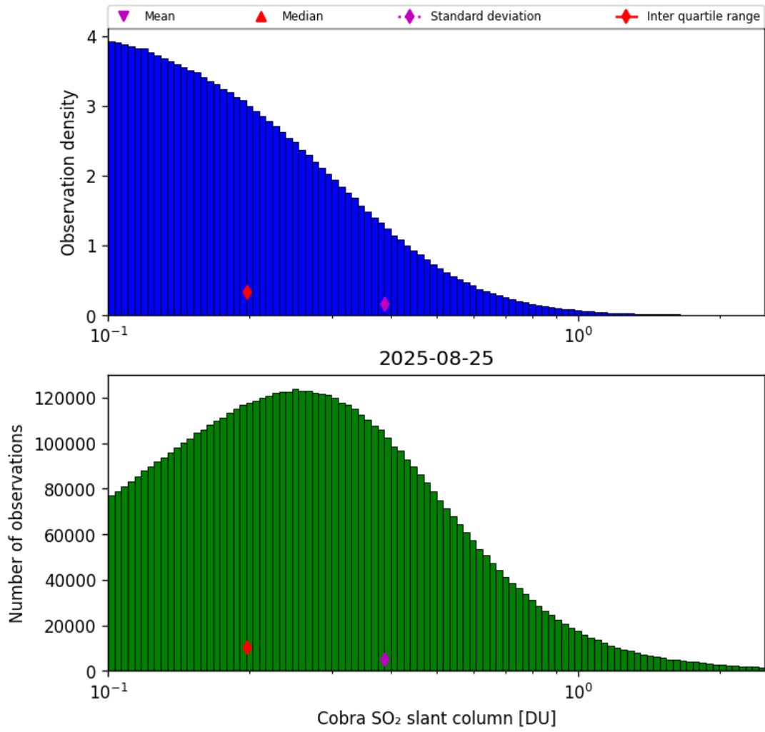
Figure 61: Histogram of “Cobra SO 2 slant column” for 2025-08-25 to 2025-08-26
