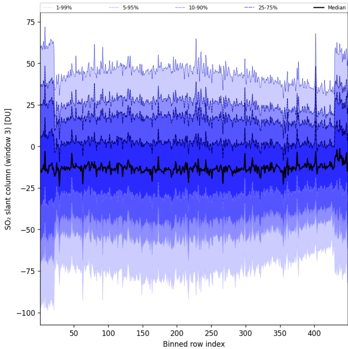
Figure 98: Along track statistics of “SO 2 slant column (window 3)” for 2025-08-25 to 2025-08-26
