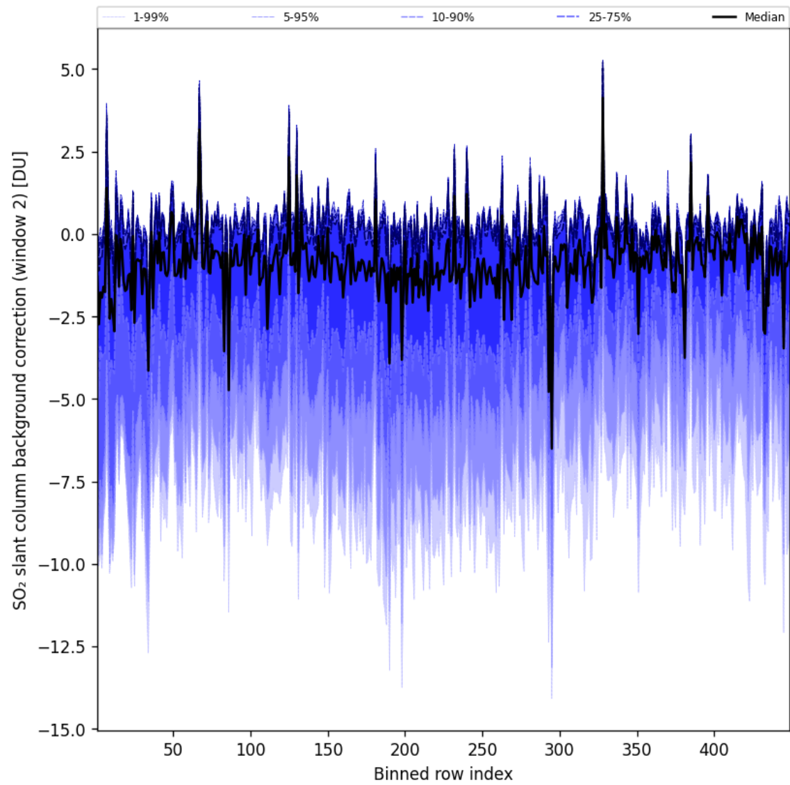
Figure 97: Along track statistics of “SO 2 slant column background correction (window 2)” for 2025-08-25 to 2025-08-26
