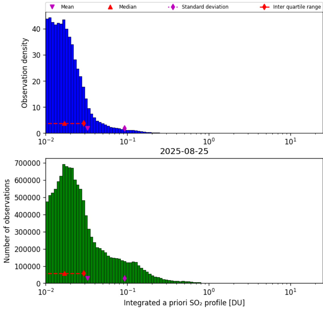
Figure 76: Histogram of “Integrated a priori SO 2 profile” for 2025-08-25 to 2025-08-26
