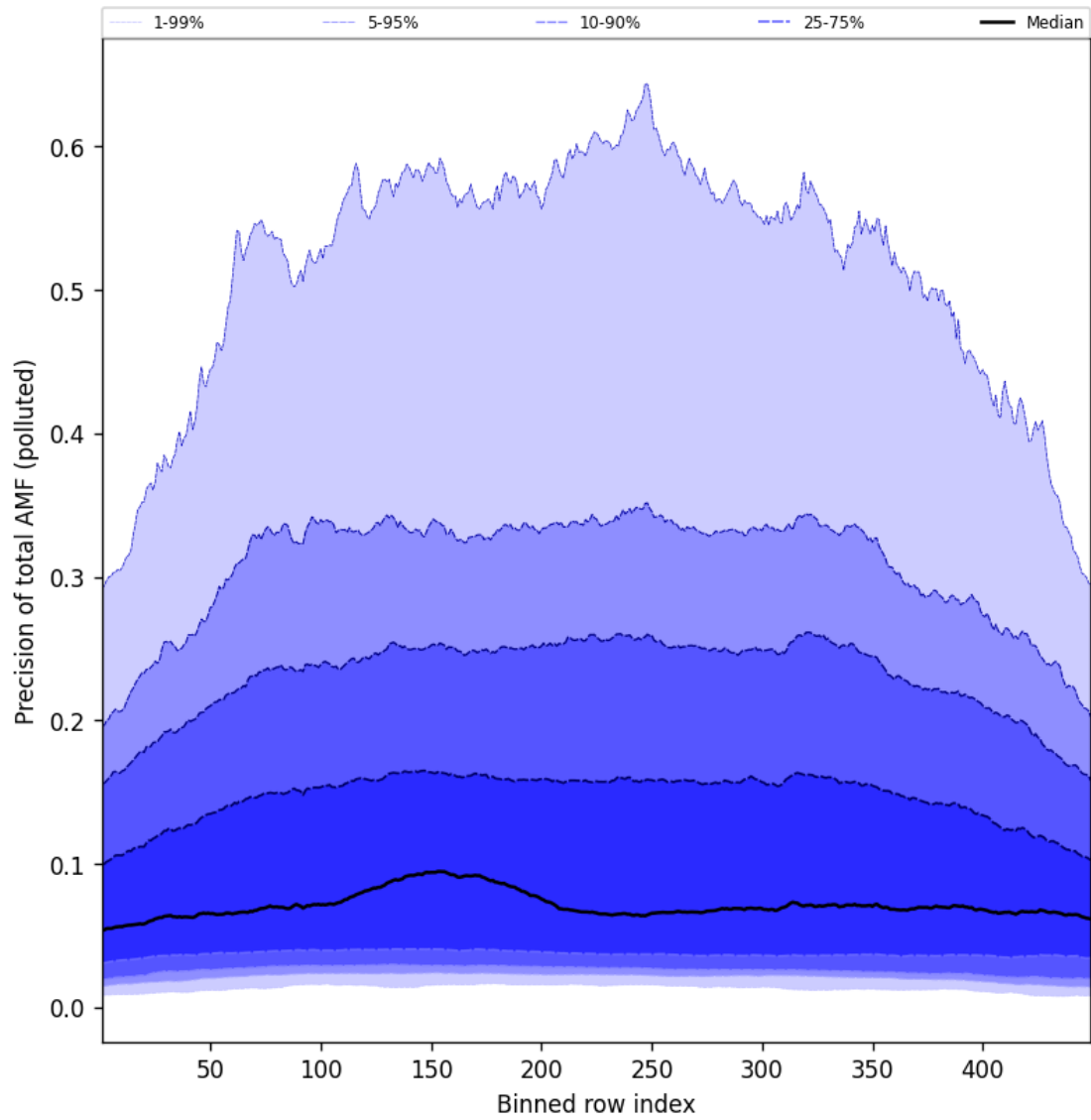
Figure 108: Along track statistics of “Precision of total AMF (polluted)” for 2025-08-25 to 2025-08-26
