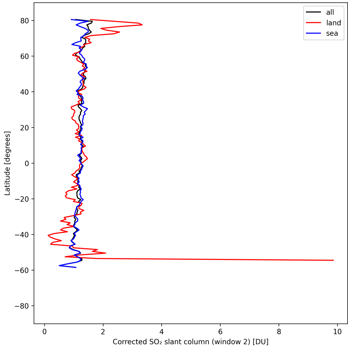
Figure 42: Zonal average of “Corrected SO 2 slant column (window 2)” for 2025-08-25 to 2025-08-26.
