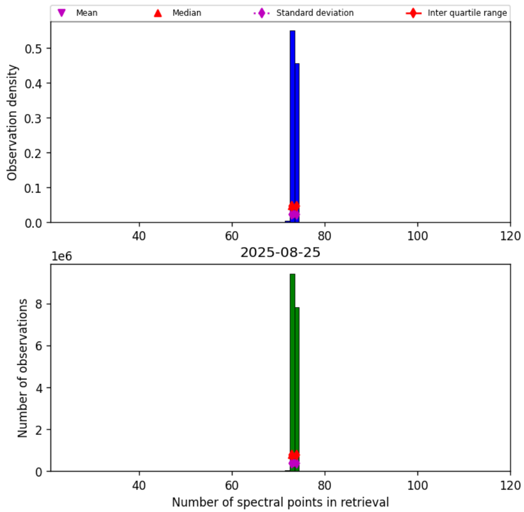
Figure 83: Histogram of “Number of spectral points in retrieval” for 2025-08-25 to 2025-08-26
