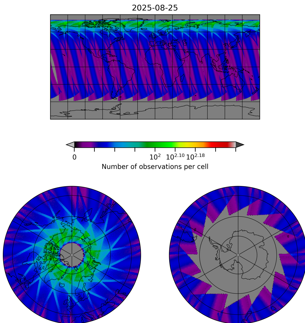
Figure 29: Map of the number of observations for 2025-08-25 to 2025-08-26
