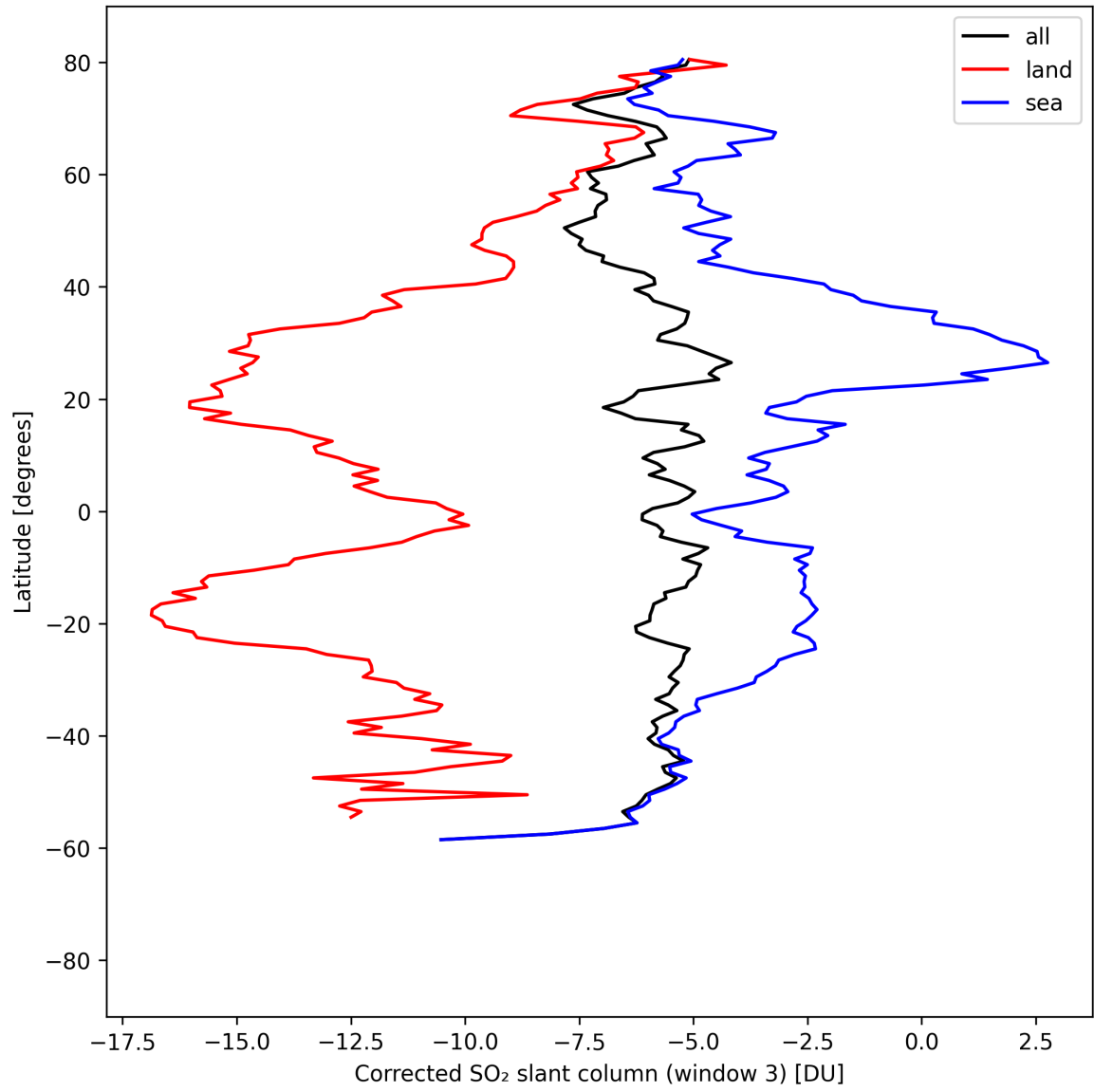
Figure 46: Zonal average of “Corrected SO 2 slant column (window 3)” for 2025-08-25 to 2025-08-26.
