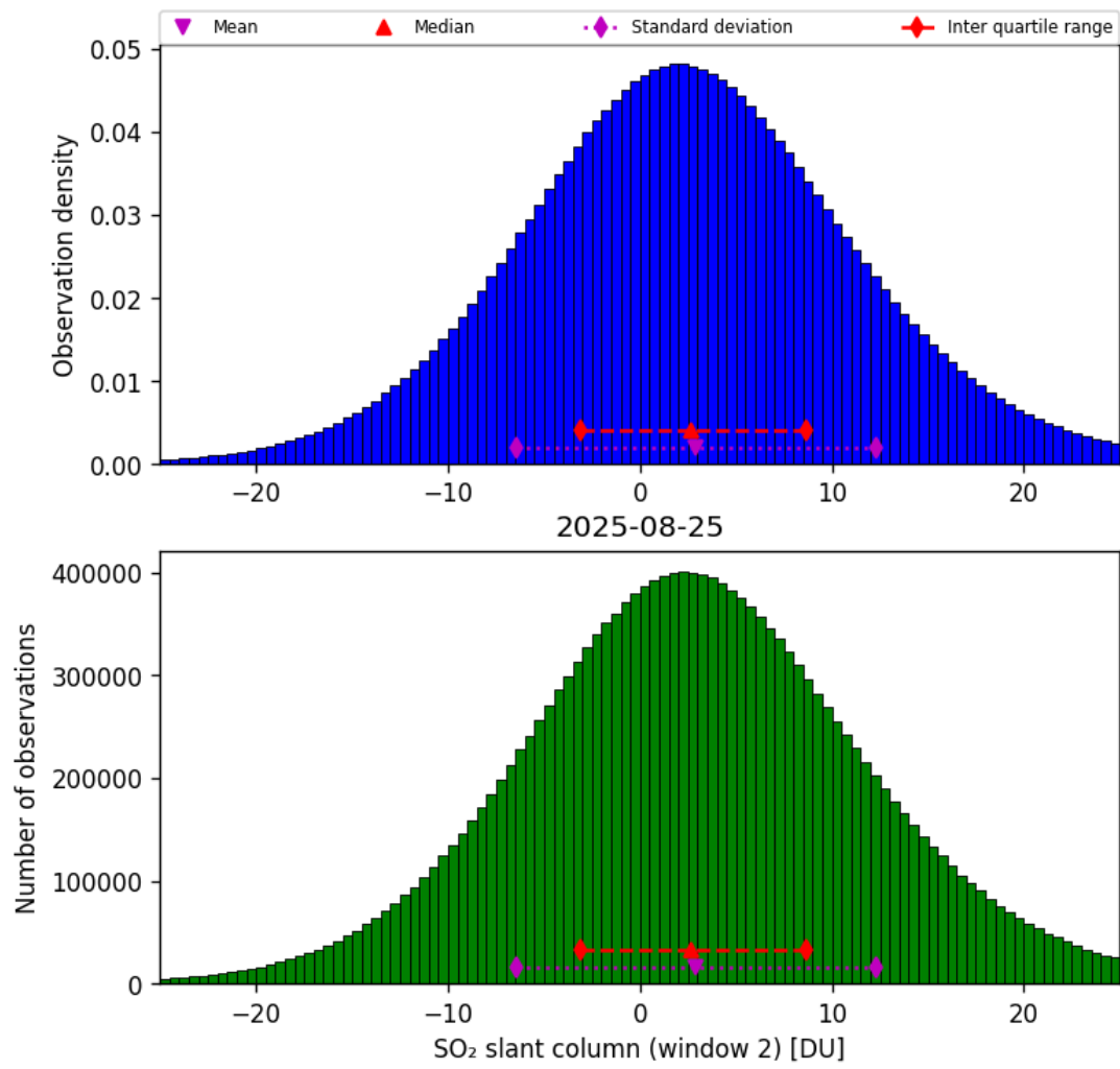
Figure 67: Histogram of “SO 2 slant column (window 2)” for 2025-08-25 to 2025-08-26
