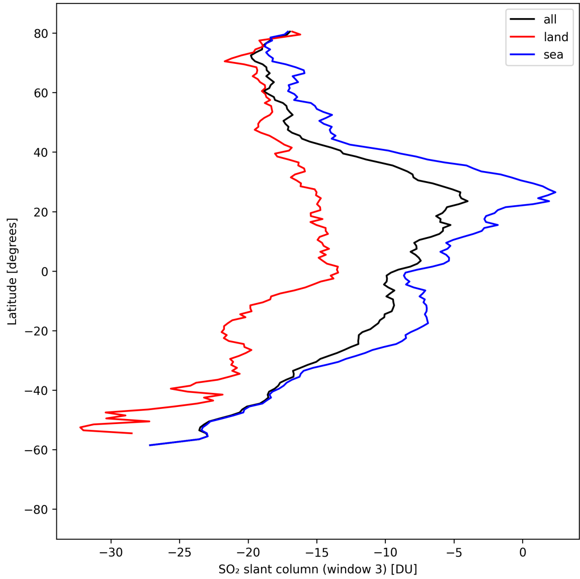
Figure 44: Zonal average of “SO 2 slant column (window 3)” for 2025-08-25 to 2025-08-26.
