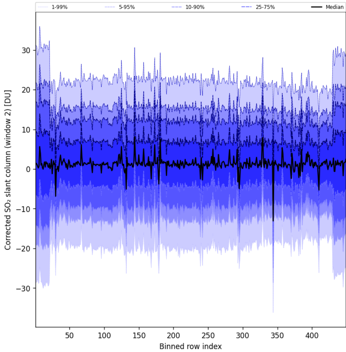
Figure 96: Along track statistics of “Corrected SO 2 slant column (window 2)” for 2025-08-25 to 2025-08-26
