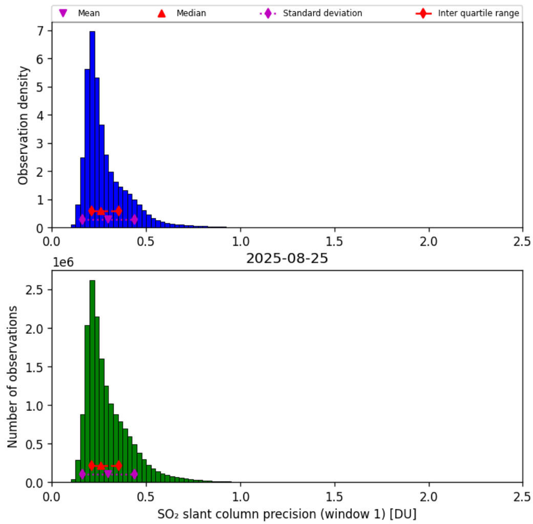
Figure 64: Histogram of “SO 2 slant column precision (window 1)” for 2025-08-25 to 2025-08-26
