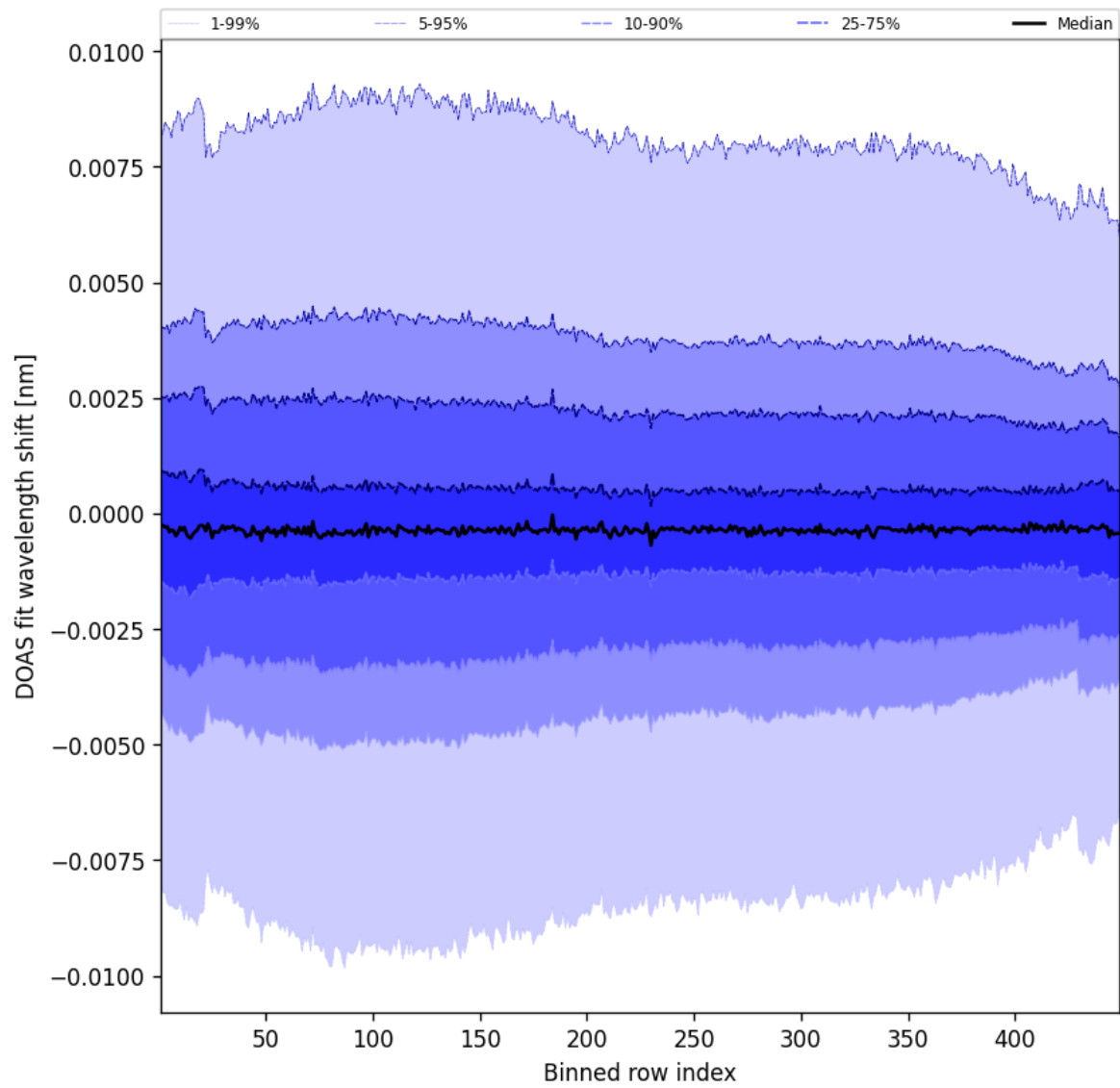
Figure 104: Along track statistics of “DOAS fit wavelength shift” for 2025-08-25 to 2025-08-26
