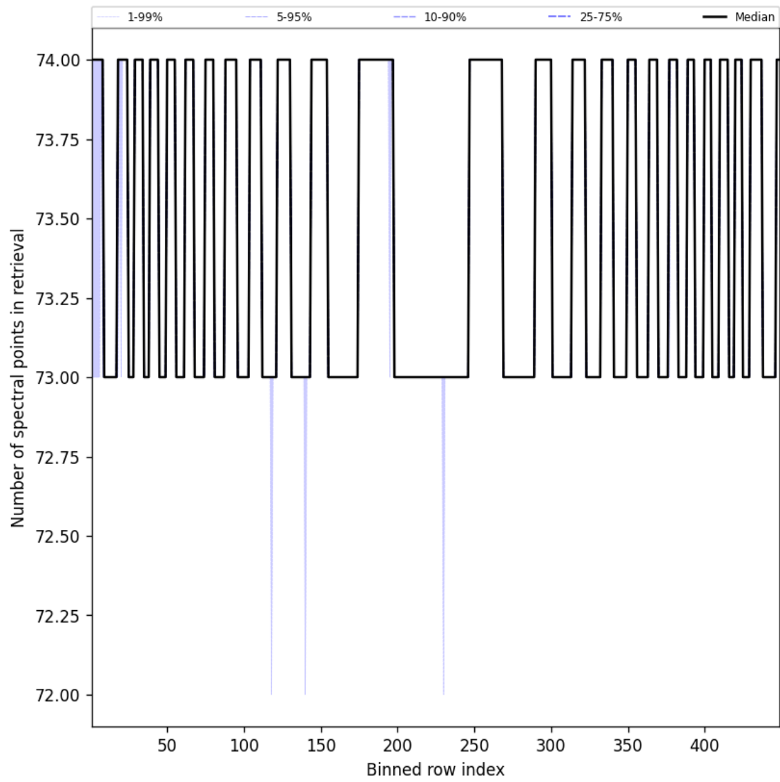
Figure 110: Along track statistics of “Number of spectral points in retrieval” for 2025-08-25 to 2025-08-26
