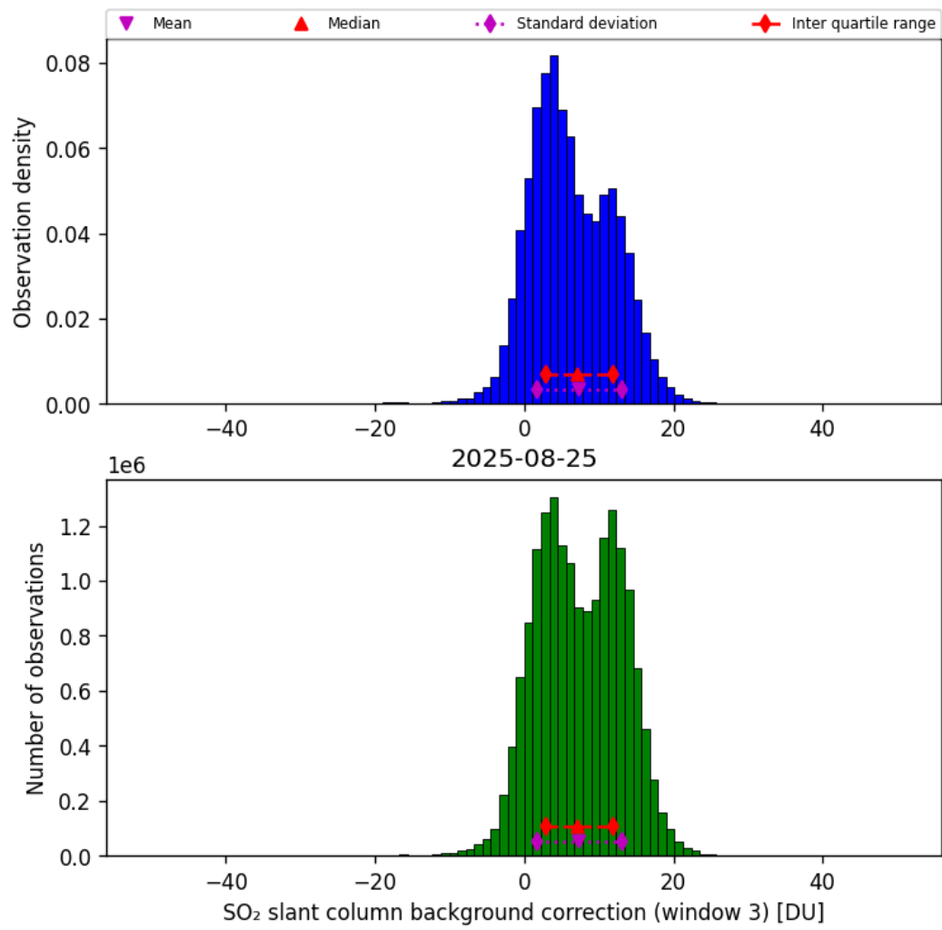
Figure 74: Histogram of “SO 2 slant column background correction (window 3)” for 2025-08-25 to 2025-08-26
