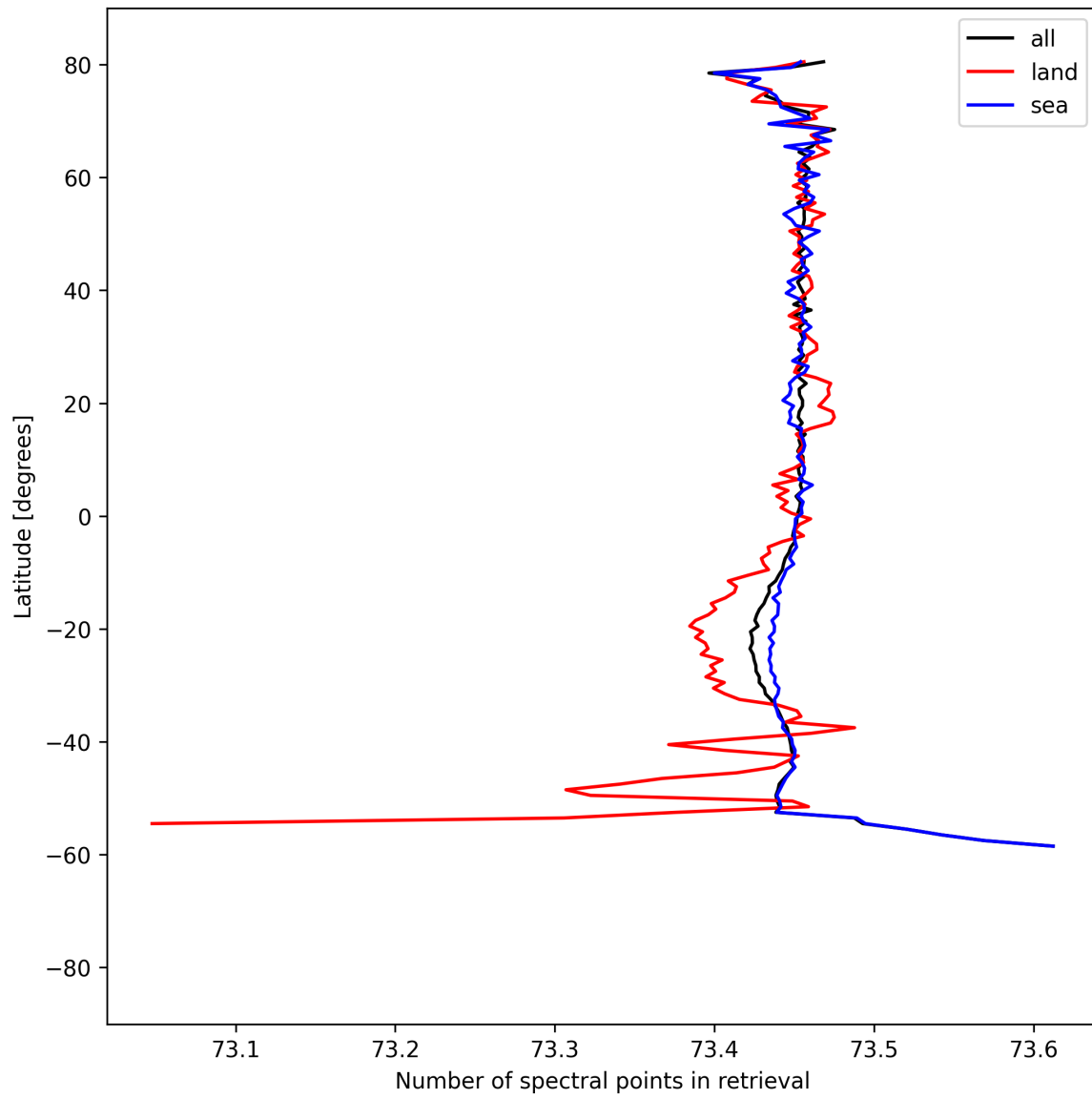
Figure 56: Zonal average of “Number of spectral points in retrieval” for 2025-08-25 to 2025-08-26.
