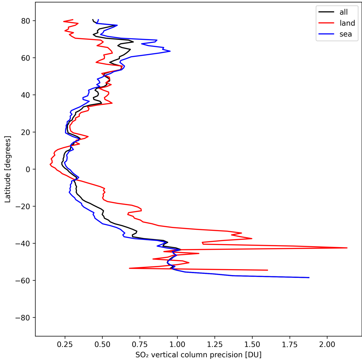
Figure 32: Zonal average of “SO 2 vertical column precision” for 2025-08-25 to 2025-08-26.
