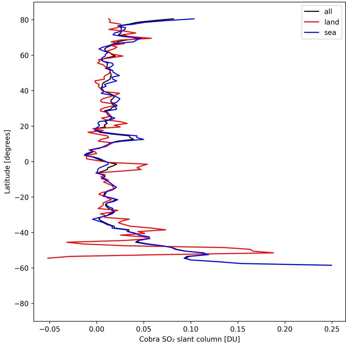
Figure 34: Zonal average of “Cobra SO 2 slant column” for 2025-08-25 to 2025-08-26.
