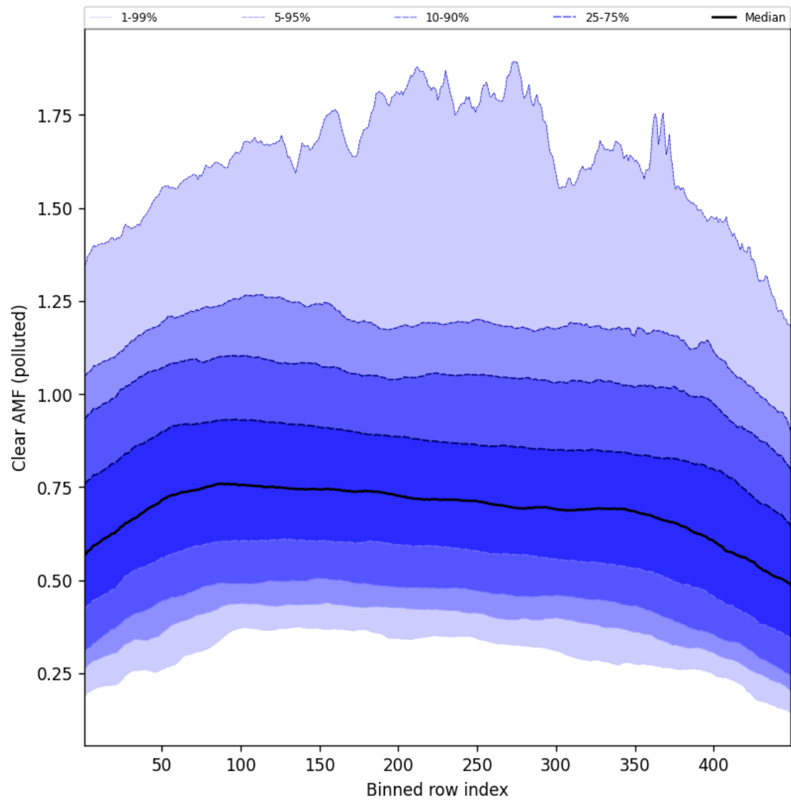
Figure 109: Along track statistics of “Clear AMF (polluted)” for 2025-08-25 to 2025-08-26
