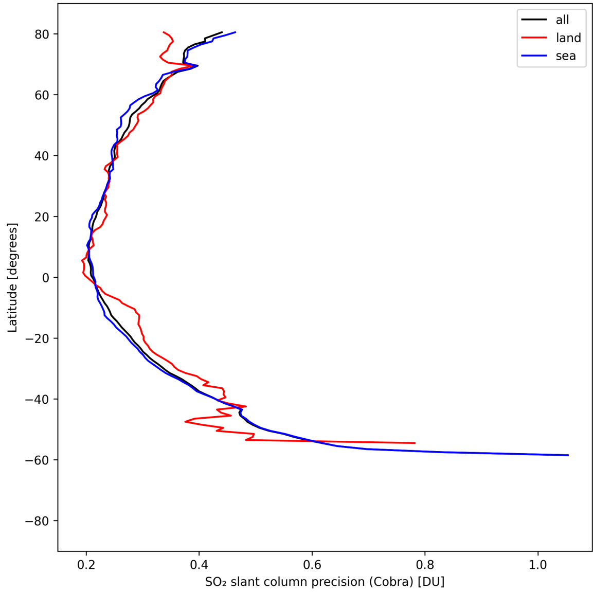
Figure 35: Zonal average of “SO 2 slant column precision (Cobra)” for 2025-08-25 to 2025-08-26.
