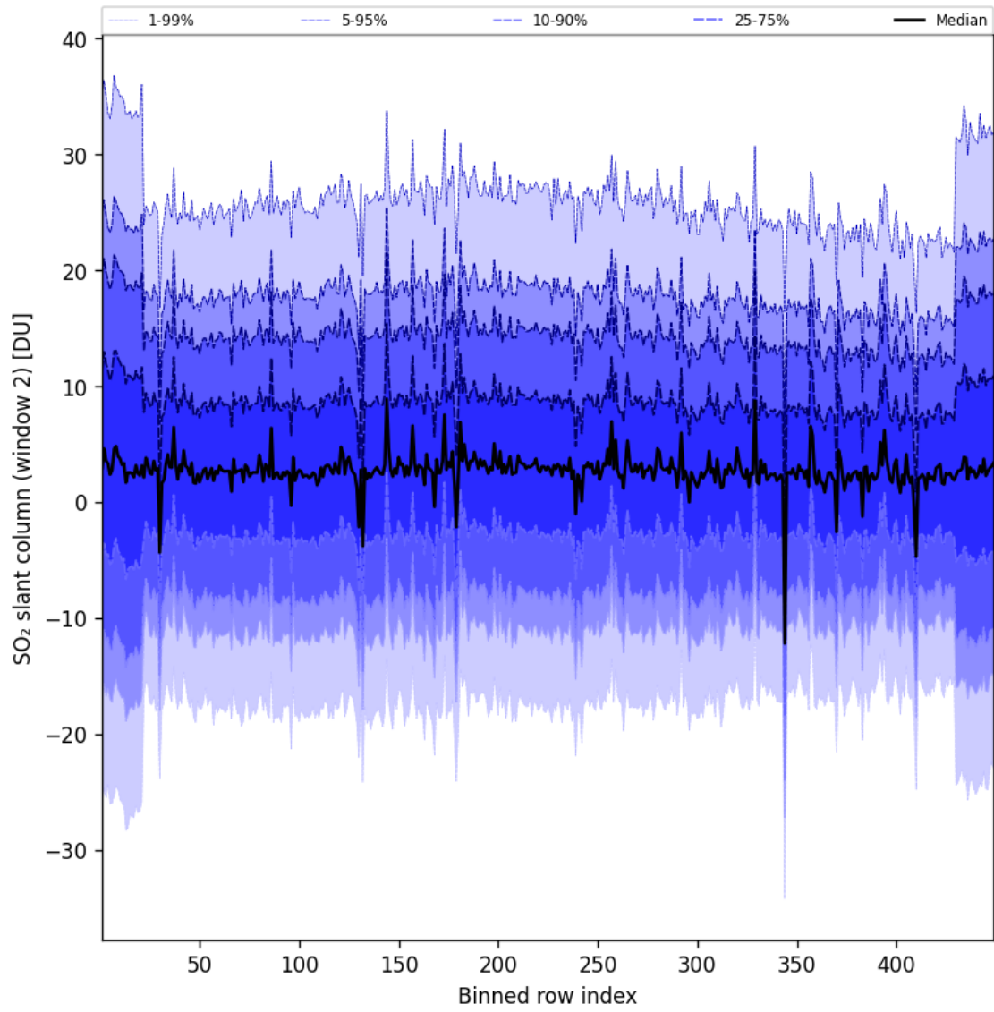
Figure 94: Along track statistics of “SO 2 slant column (window 2)” for 2025-08-25 to 2025-08-26
