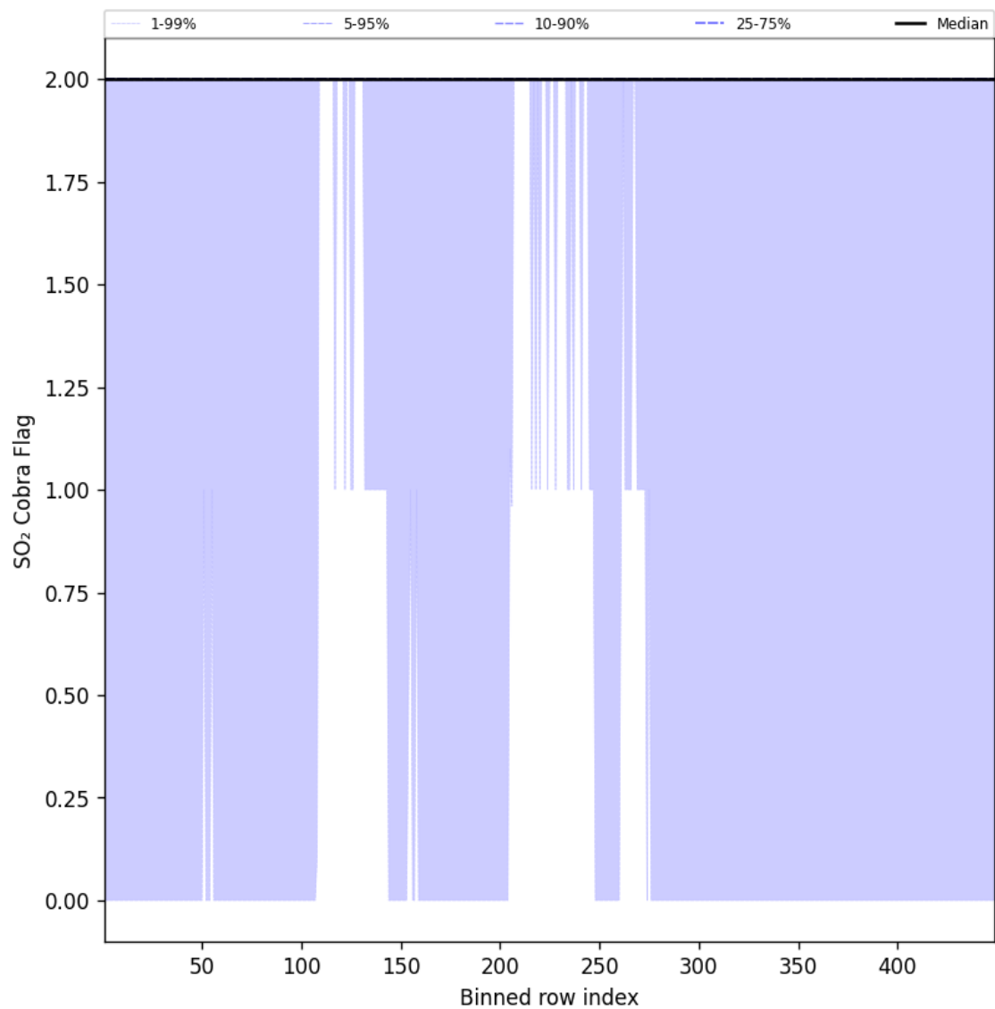
Figure 102: Along track statistics of “SO 2 Cobra Flag” for 2025-08-25 to 2025-08-26
