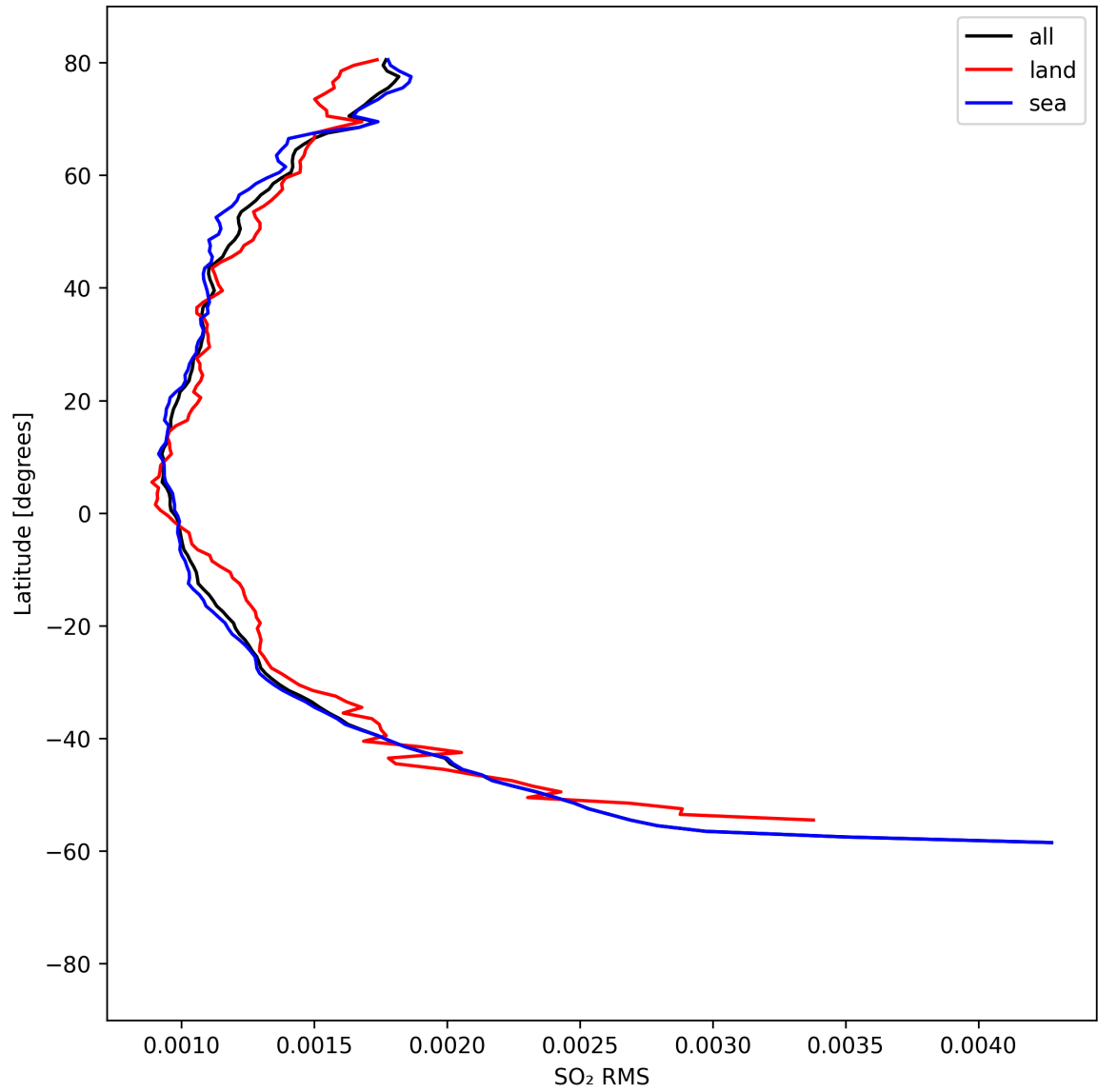
Figure 52: Zonal average of “SO 2 RMS” for 2025-08-25 to 2025-08-26.
