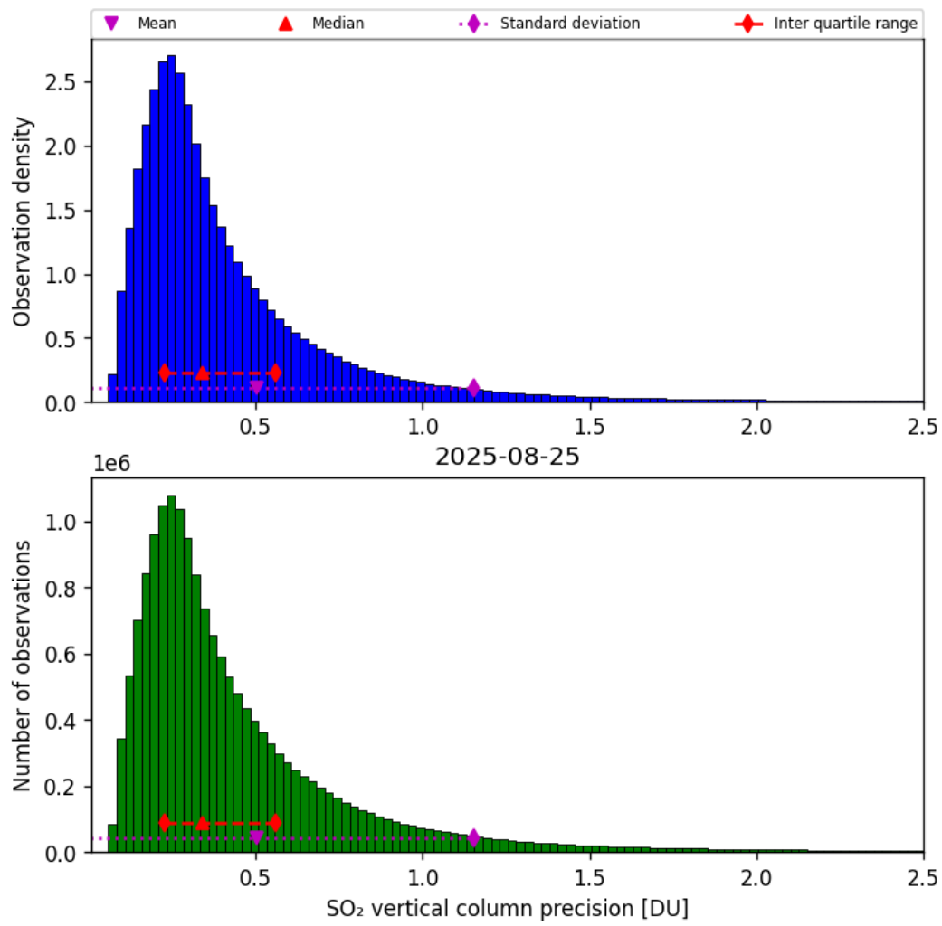
Figure 59: Histogram of “SO 2 vertical column precision” for 2025-08-25 to 2025-08-26
