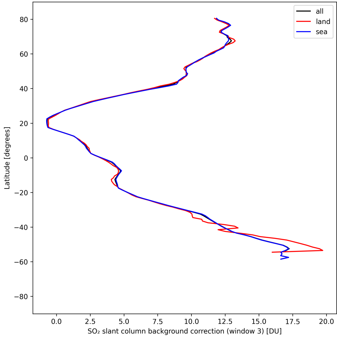
Figure 47: Zonal average of “SO 2 slant column background correction (window 3)” for 2025-08-25 to 2025-08-26.
