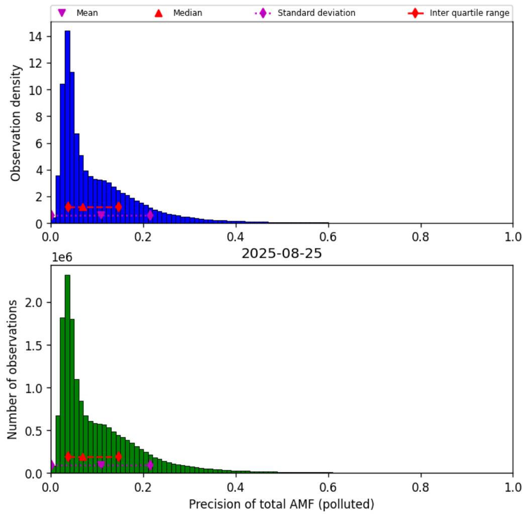
Figure 81: Histogram of “Precision of total AMF (polluted)” for 2025-08-25 to 2025-08-26
