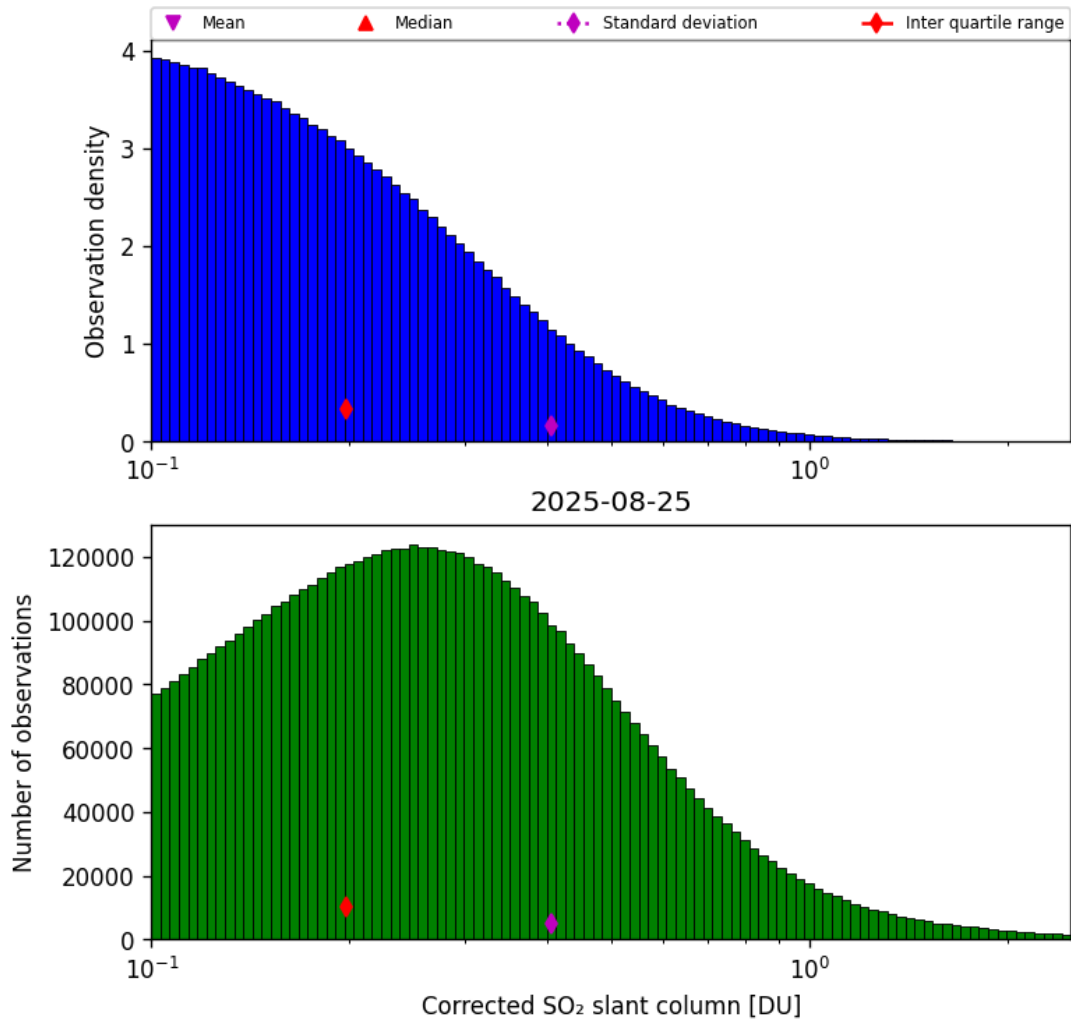
Figure 60: Histogram of “Corrected SO 2 slant column” for 2025-08-25 to 2025-08-26
