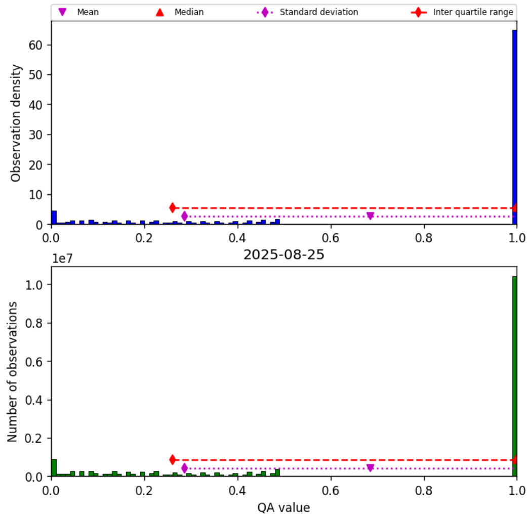
Figure 57: Histogram of “QA value” for 2025-08-25 to 2025-08-26
