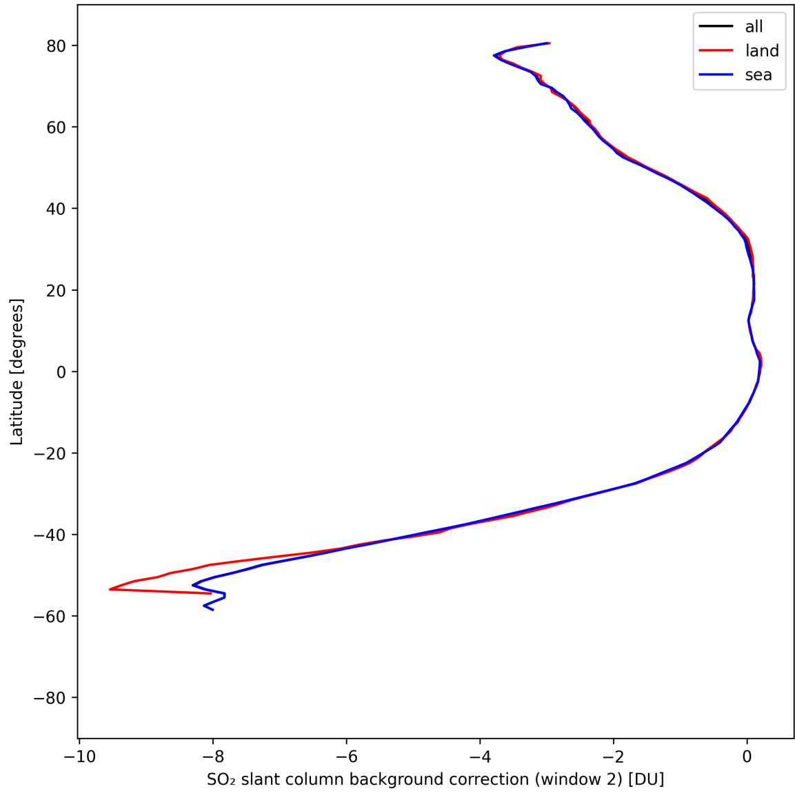
Figure 43: Zonal average of “SO 2 slant column background correction (window 2)” for 2025-08-25 to 2025-08-26.
