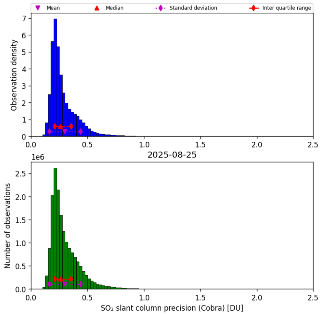
Figure 62: Histogram of “SO 2 slant column precision (Cobra)” for 2025-08-25 to 2025-08-26
