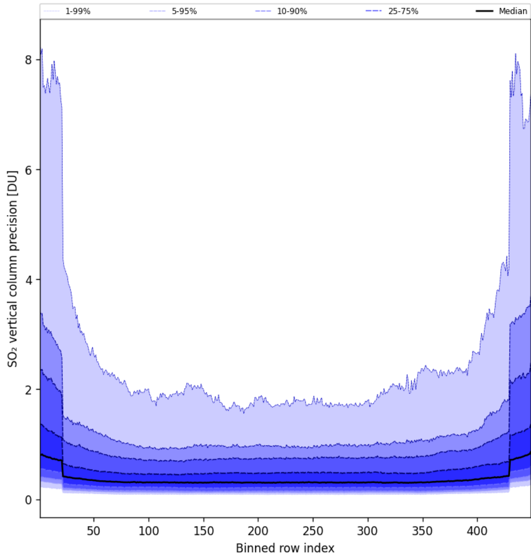
Figure 86: Along track statistics of “SO 2 vertical column precision” for 2025-08-25 to 2025-08-26
