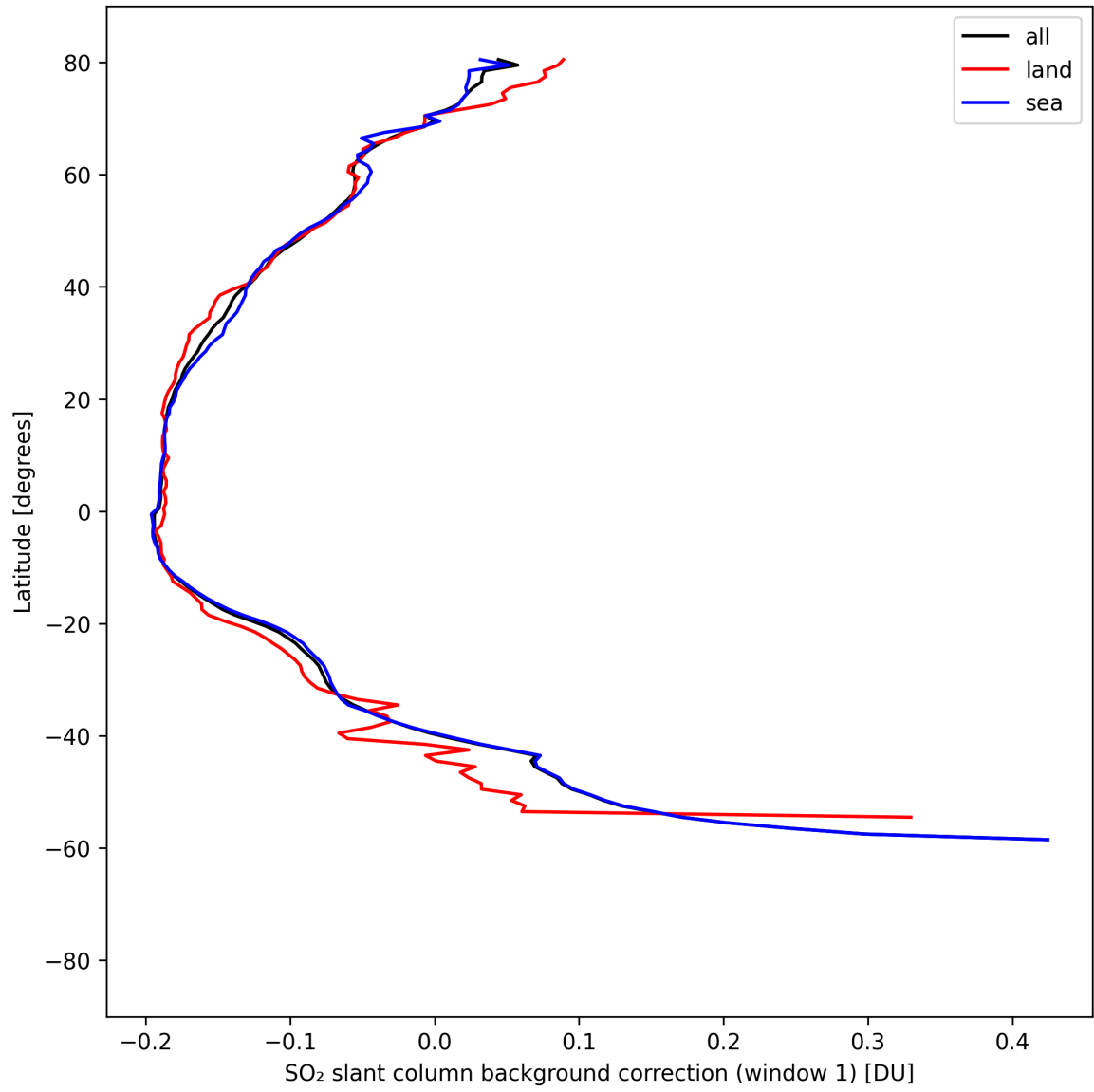
Figure 39: Zonal average of “SO 2 slant column background correction (window 1)” for 2025-08-25 to 2025-08-26.
