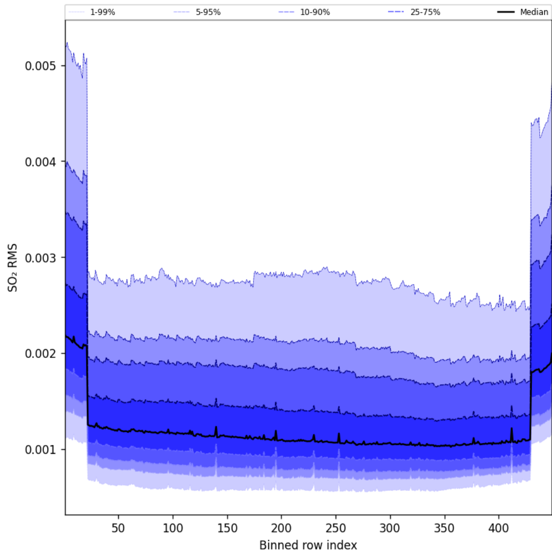
Figure 106: Along track statistics of “SO 2 RMS” for 2025-08-25 to 2025-08-26
