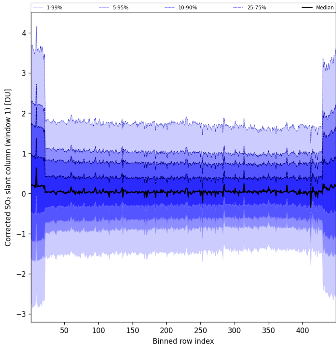
Figure 92: Along track statistics of “Corrected SO 2 slant column (window 1)” for 2025-08-25 to 2025-08-26
