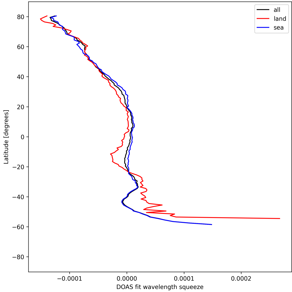
Figure 51: Zonal average of “DOAS fit wavelength squeeze” for 2025-08-25 to 2025-08-26.
