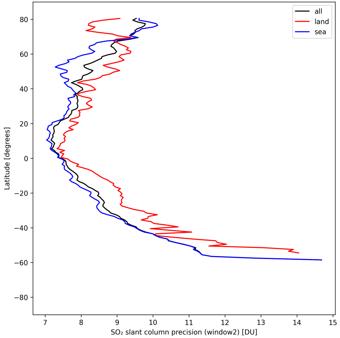
Figure 41: Zonal average of “SO 2 slant column precision (window2)” for 2025-08-25 to 2025-08-26.
