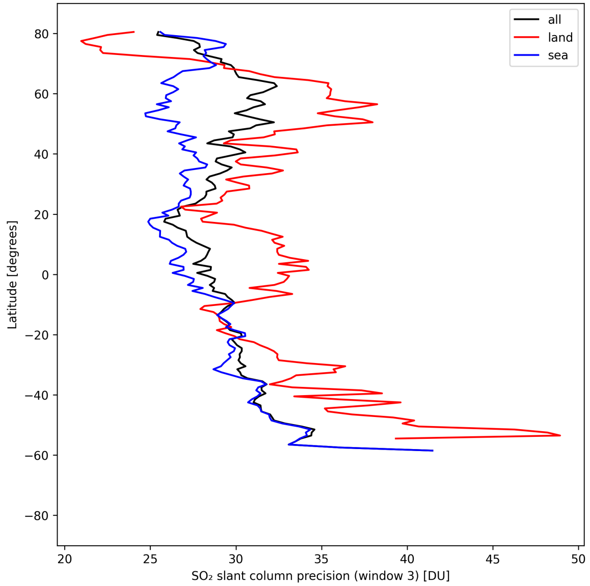
Figure 45: Zonal average of “SO 2 slant column precision (window 3)” for 2025-08-25 to 2025-08-26.
