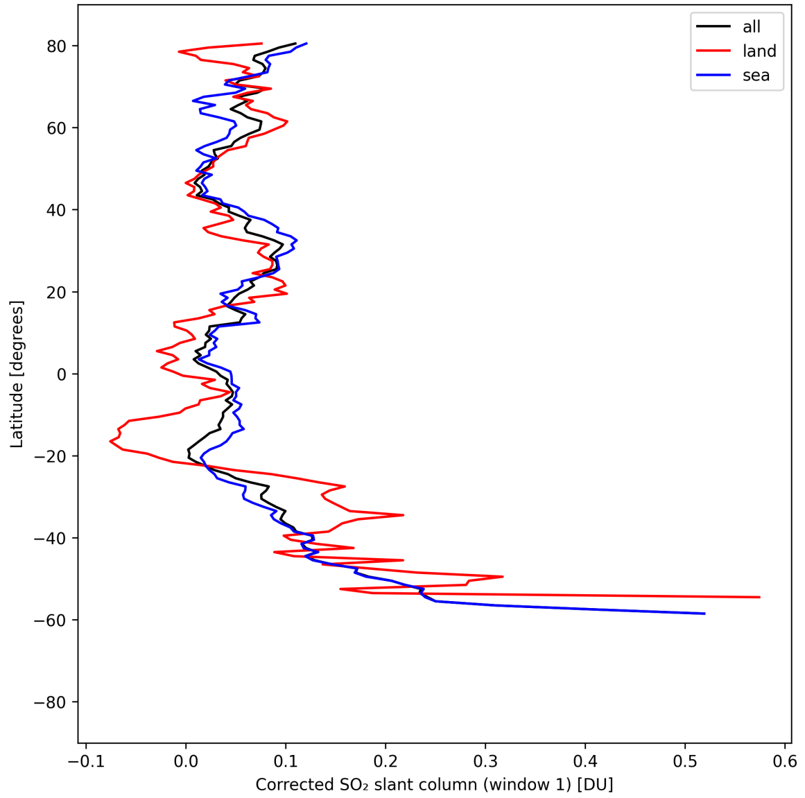
Figure 38: Zonal average of “Corrected SO 2 slant column (window 1)” for 2025-08-25 to 2025-08-26.
