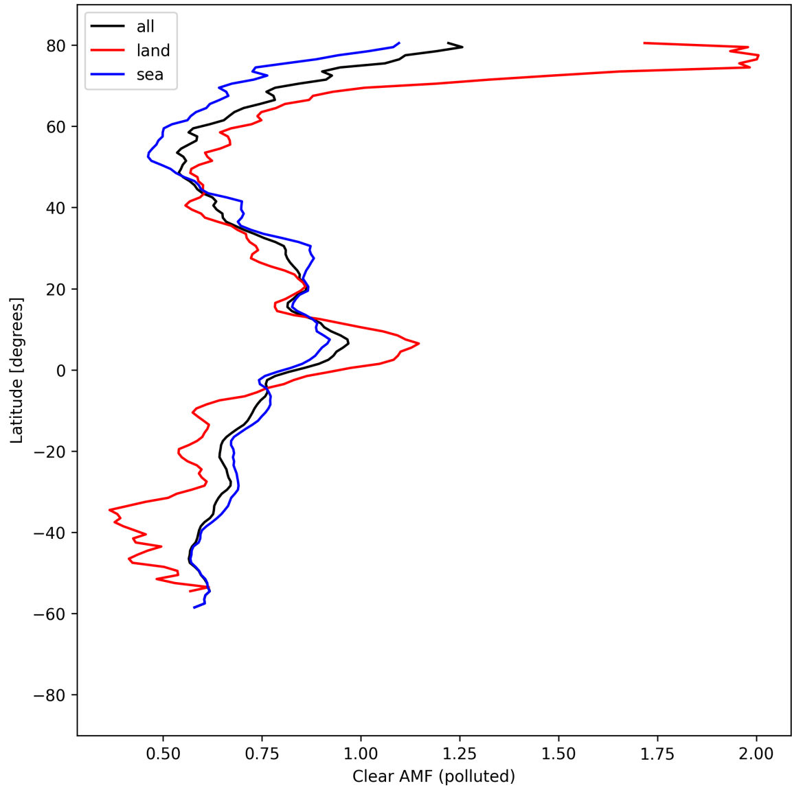
Figure 55: Zonal average of “Clear AMF (polluted)” for 2025-08-25 to 2025-08-26.
