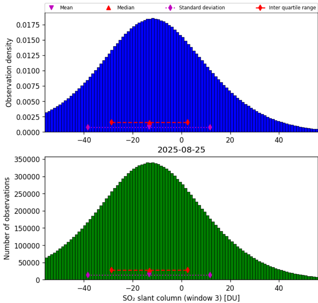
Figure 71: Histogram of “SO 2 slant column (window 3)” for 2025-08-25 to 2025-08-26
