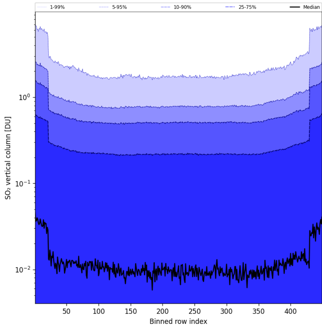
Figure 85: Along track statistics of “SO 2 vertical column” for 2025-08-25 to 2025-08-26
