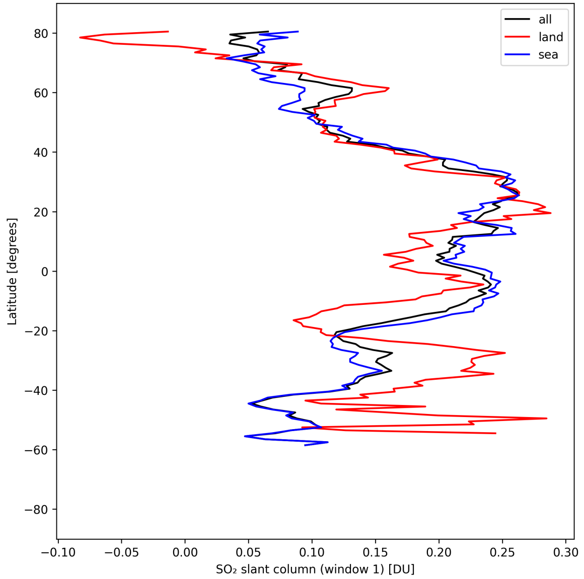
Figure 36: Zonal average of “SO 2 slant column (window 1)” for 2025-08-25 to 2025-08-26.
