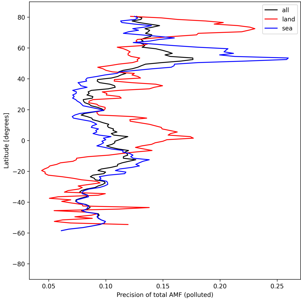
Figure 54: Zonal average of “Precision of total AMF (polluted)” for 2025-08-25 to 2025-08-26.
