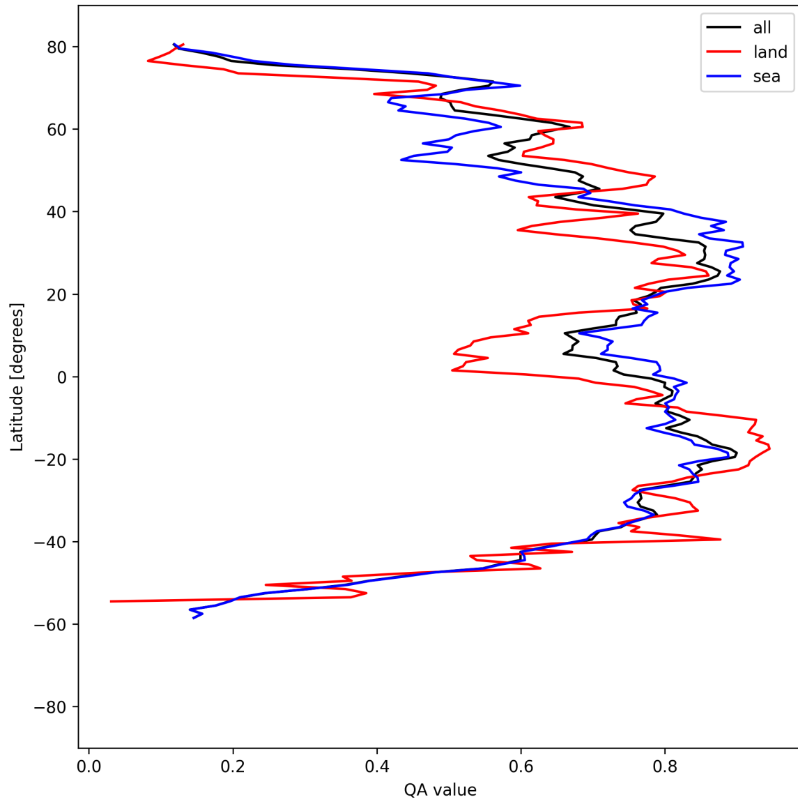
Figure 30: Zonal average of “QA value” for 2025-08-25 to 2025-08-26.
