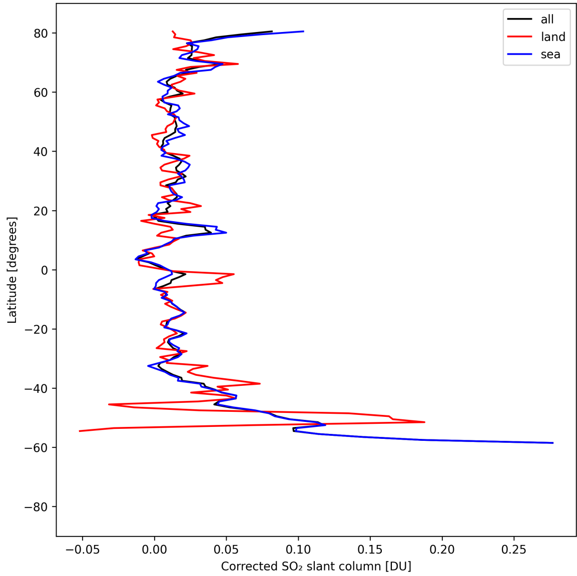
Figure 33: Zonal average of “Corrected SO 2 slant column” for 2025-08-25 to 2025-08-26.
