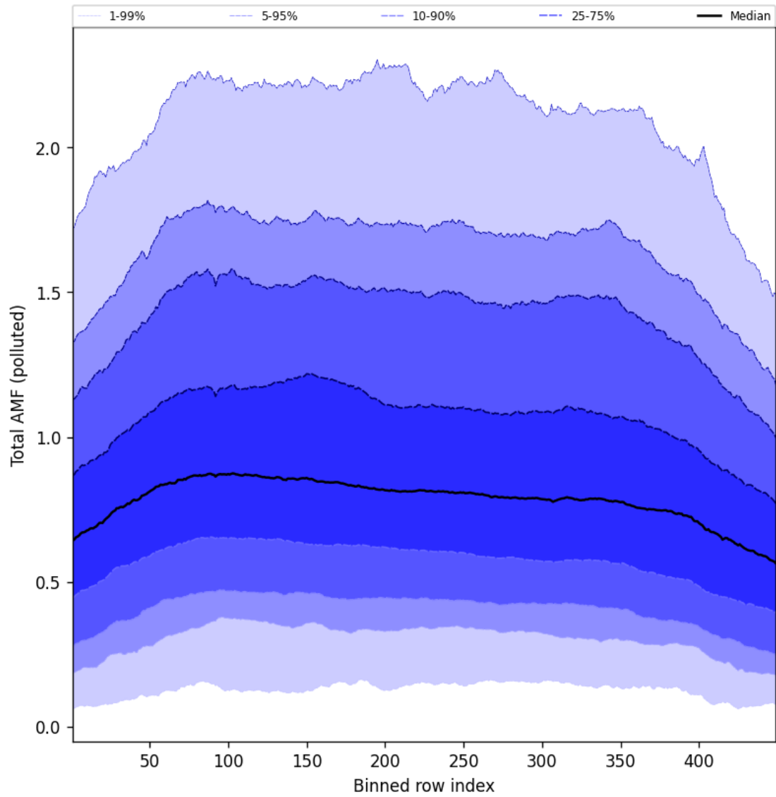
Figure 107: Along track statistics of “Total AMF (polluted)” for 2025-08-25 to 2025-08-26
