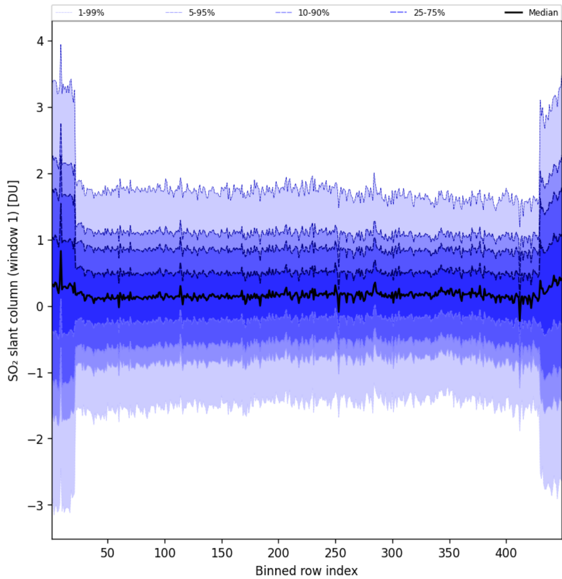
Figure 90: Along track statistics of “SO 2 slant column (window 1)” for 2025-08-25 to 2025-08-26
