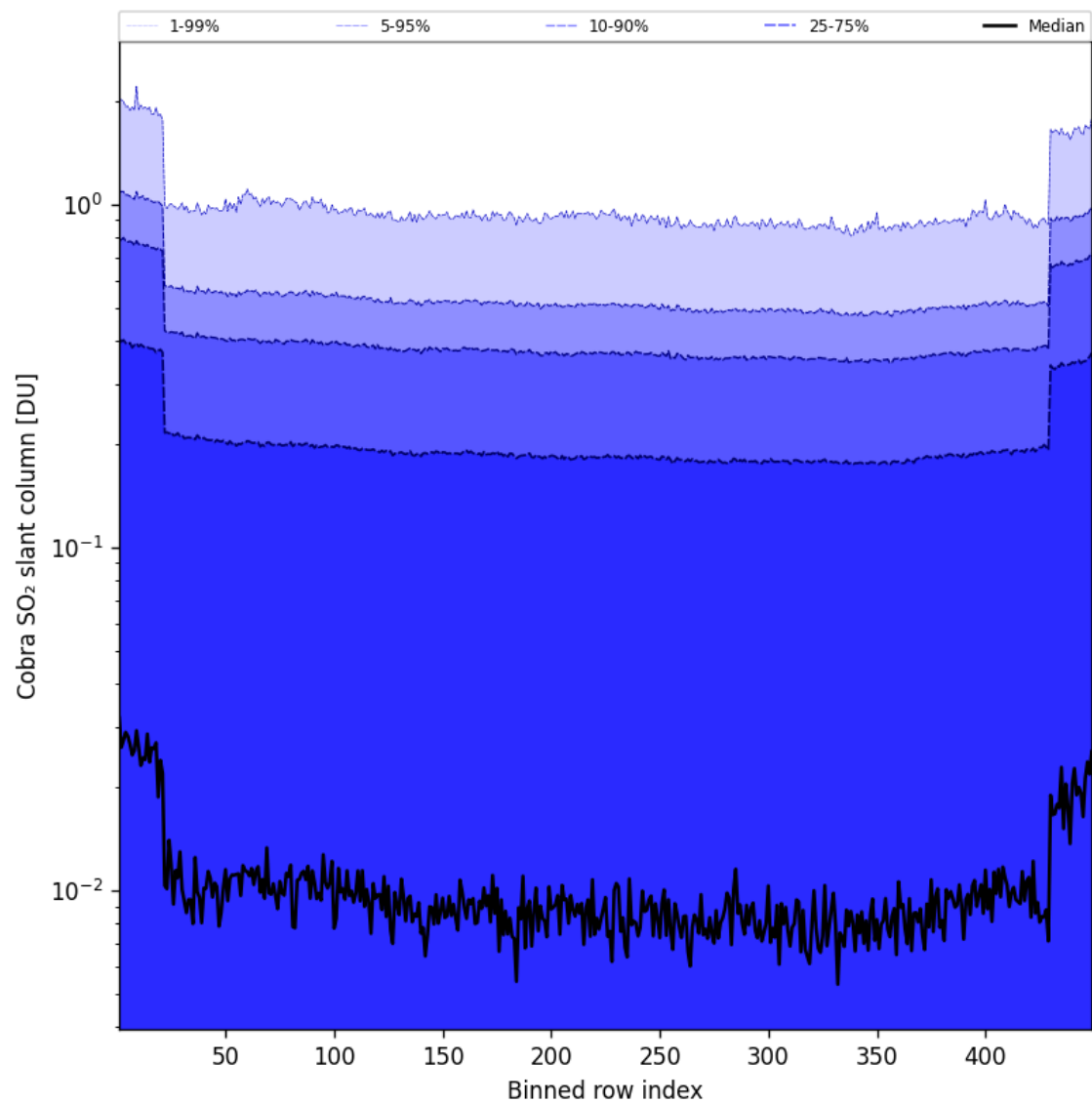
Figure 88: Along track statistics of “Cobra SO 2 slant column” for 2025-08-25 to 2025-08-26
