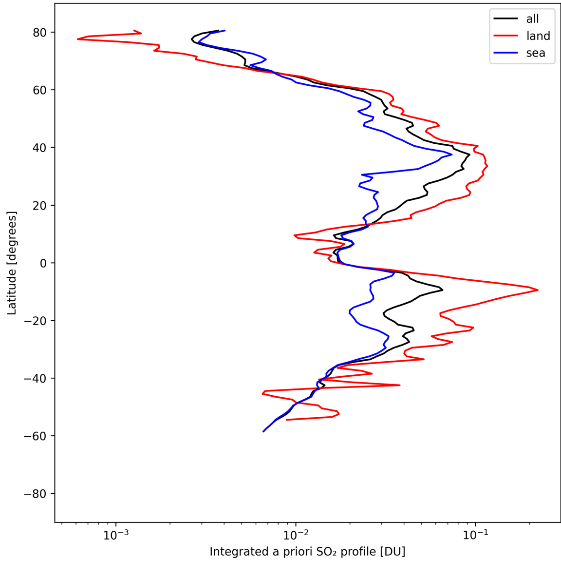
Figure 49: Zonal average of “Integrated a priori SO 2 profile” for 2025-08-25 to 2025-08-26.
