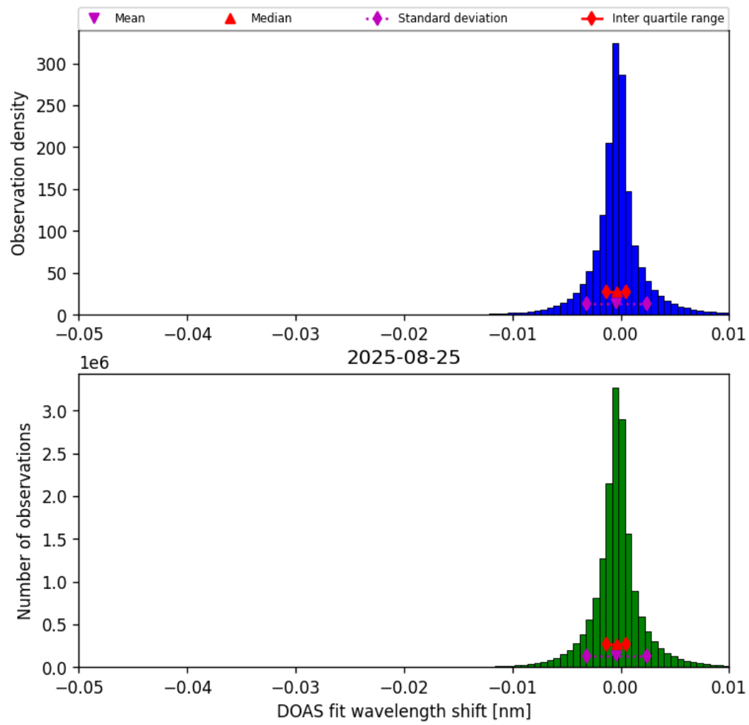
Figure 77: Histogram of “DOAS fit wavelength shift” for 2025-08-25 to 2025-08-26
