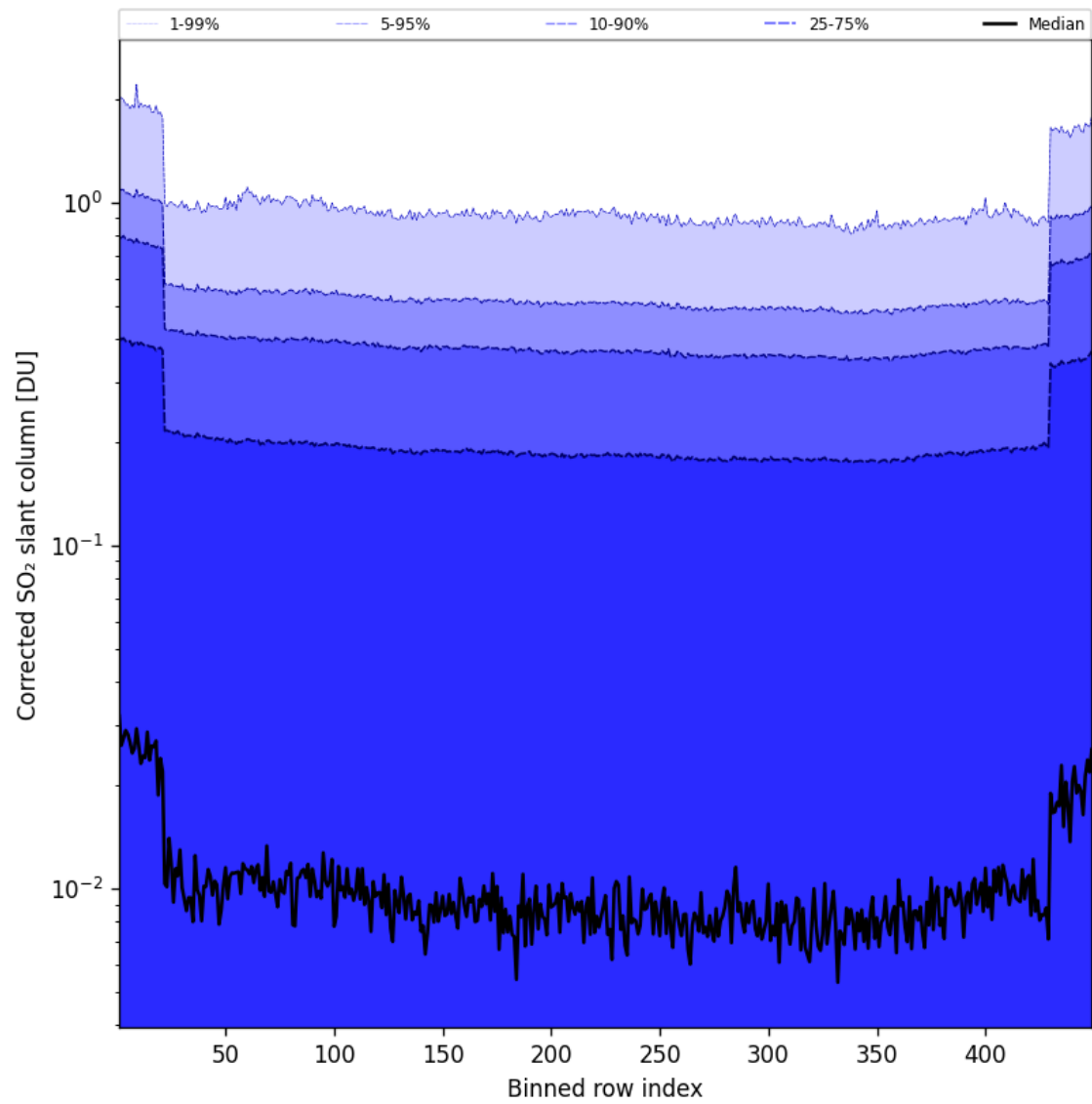
Figure 87: Along track statistics of “Corrected SO 2 slant column” for 2025-08-25 to 2025-08-26
