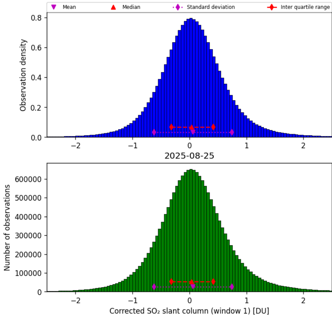
Figure 65: Histogram of “Corrected SO 2 slant column (window 1)” for 2025-08-25 to 2025-08-26
