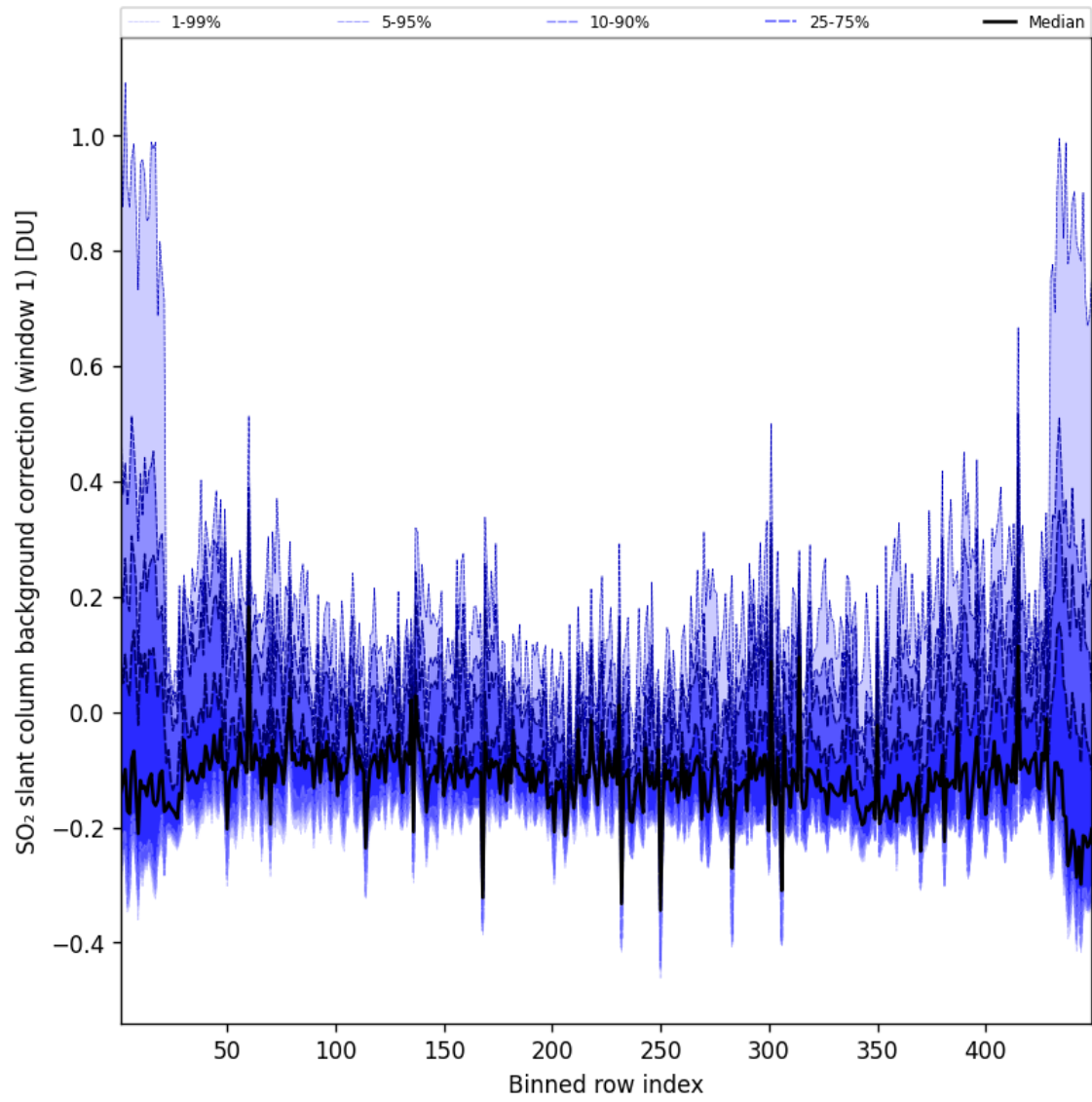
Figure 93: Along track statistics of “SO 2 slant column background correction (window 1)” for 2025-08-25 to 2025-08-26
