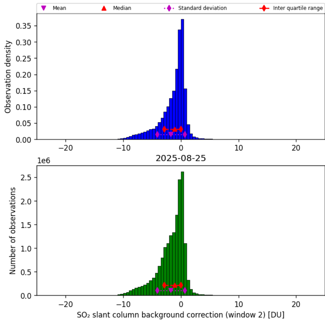
Figure 70: Histogram of “SO 2 slant column background correction (window 2)” for 2025-08-25 to 2025-08-26
