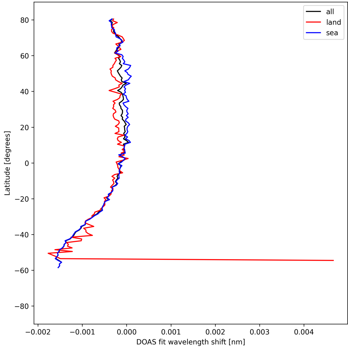
Figure 50: Zonal average of “DOAS fit wavelength shift” for 2025-08-25 to 2025-08-26.
