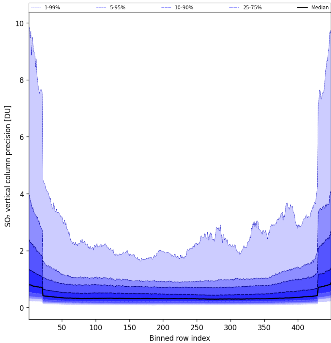
Figure 86: Along track statistics of "SO 2 vertical column precision" for 2025-08-28 to 2025-08-28
