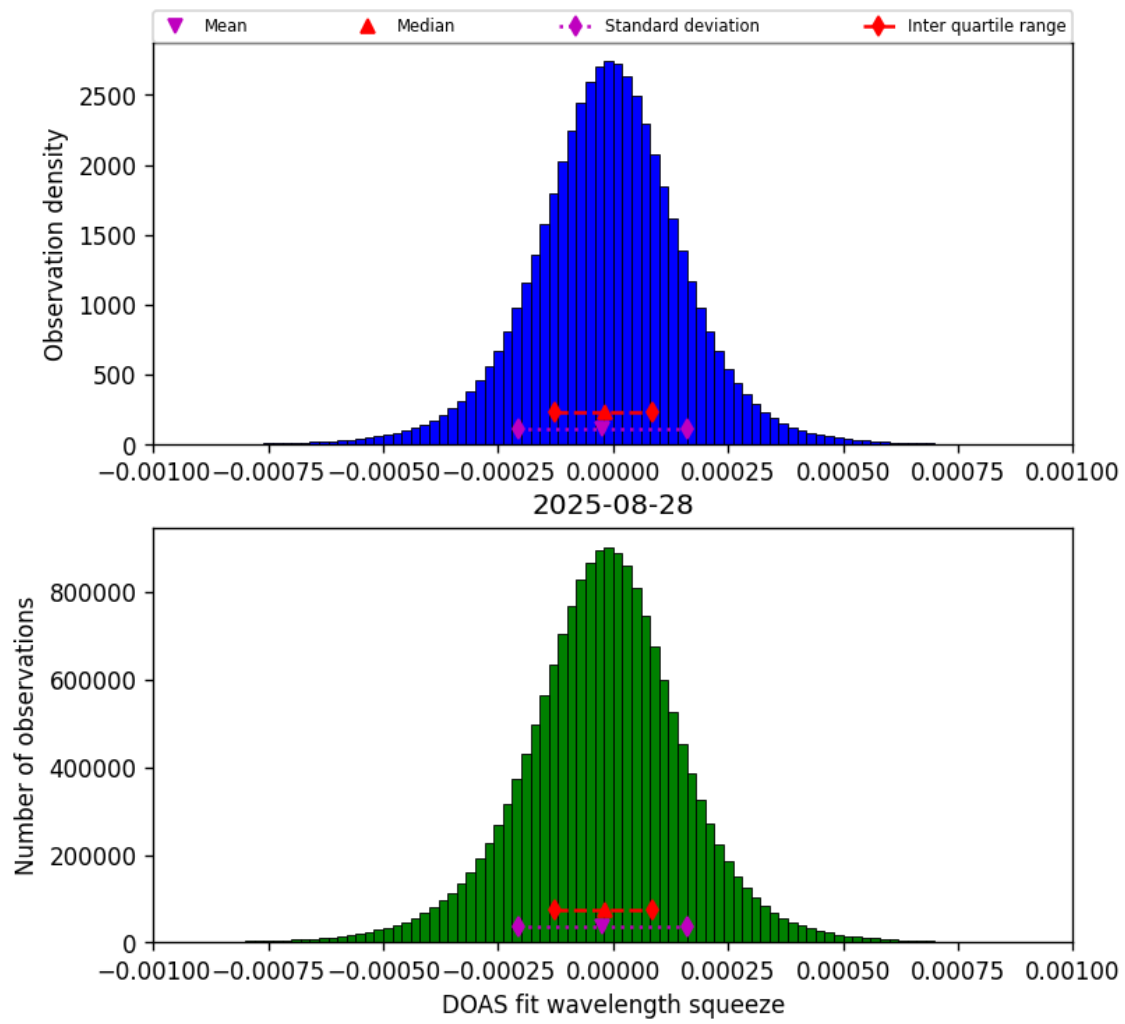
Figure 78: Histogram of “DOAS fit wavelength squeeze” for 2025-08-28 to 2025-08-28
