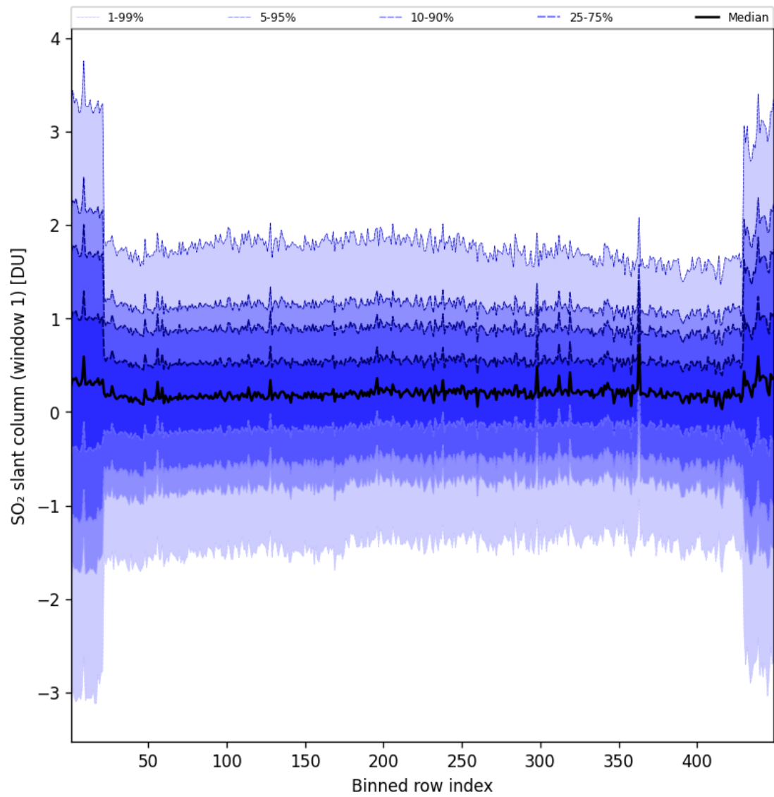
Figure 90: Along track statistics of “SO 2 slant column (window 1)” for 2025-08-28 to 2025-08-28
