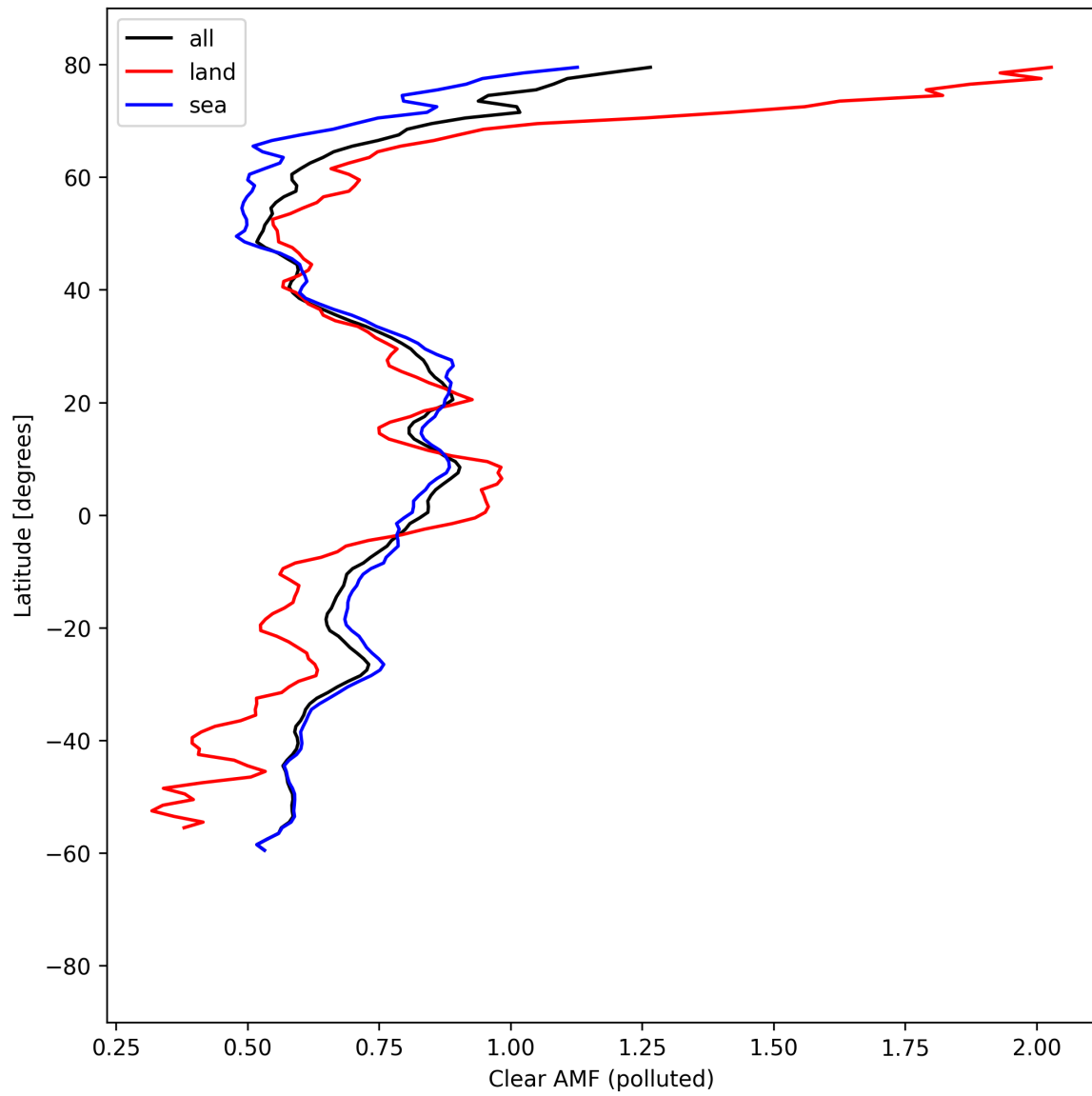
Figure 55: Zonal average of “Clear AMF (polluted)” for 2025-08-28 to 2025-08-28.
