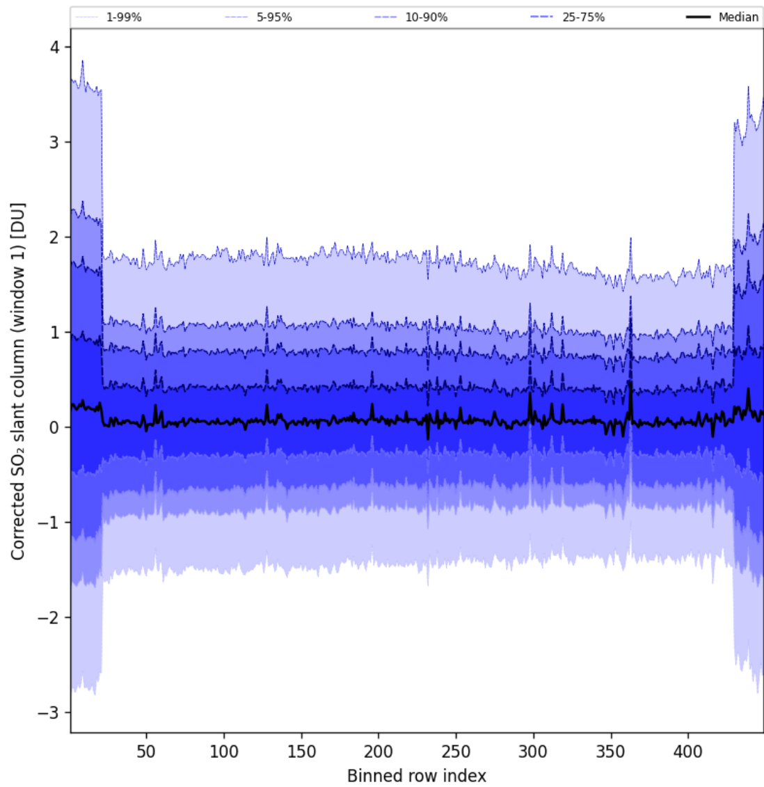
Figure 92: Along track statistics of “Corrected SO 2 slant column (window 1)” for 2025-08-28 to 2025-08-28
