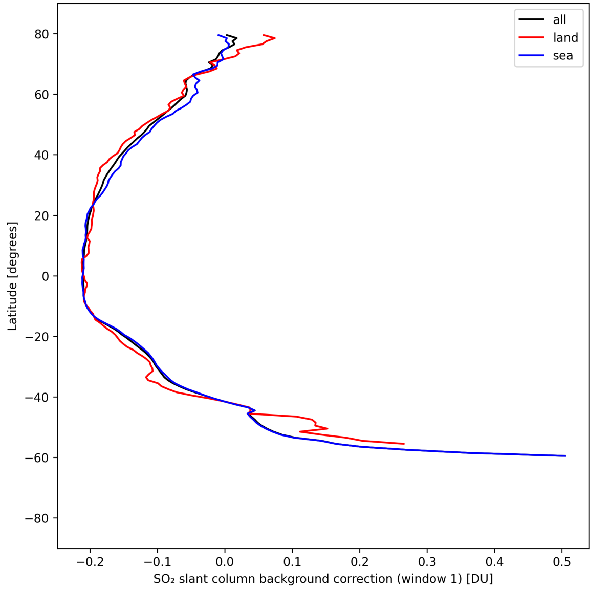
Figure 39: Zonal average of “SO 2 slant column background correction (window 1)” for 2025-08-28 to 2025-08-28.
