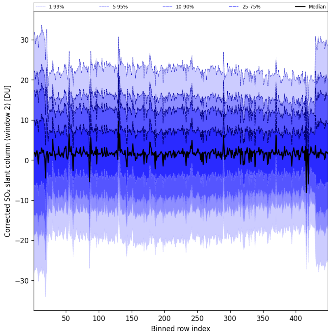
Figure 96: Along track statistics of “Corrected SO 2 slant column (window 2)” for 2025-08-28 to 2025-08-28
