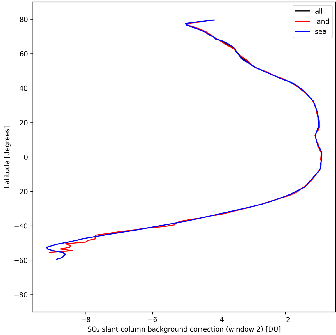
Figure 43: Zonal average of “SO 2 slant column background correction (window 2)” for 2025-08-28 to 2025-08-28.
