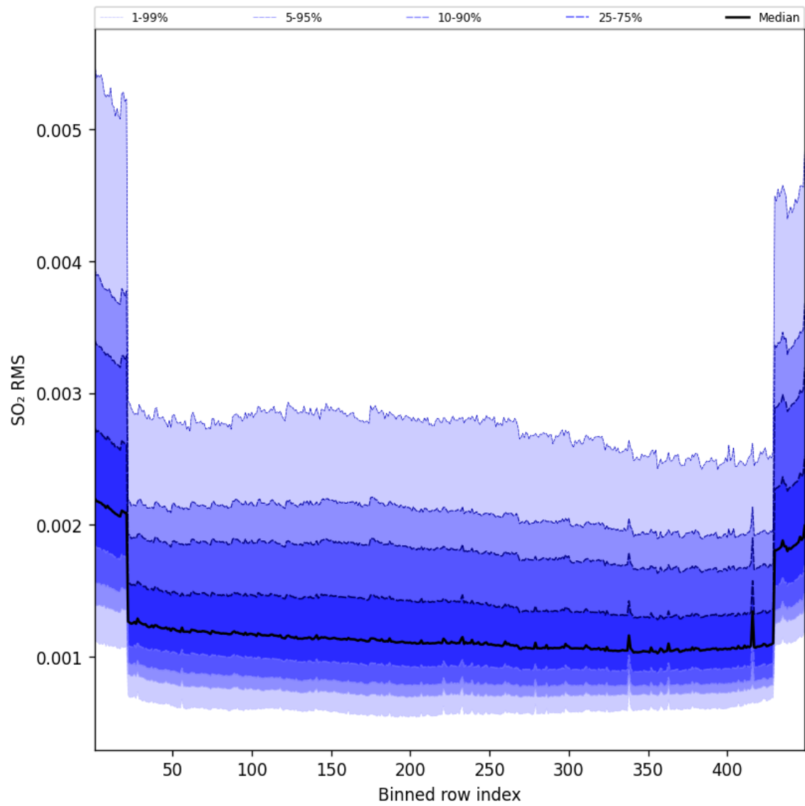
Figure 106: Along track statistics of “SO 2 RMS” for 2025-08-28 to 2025-08-28
