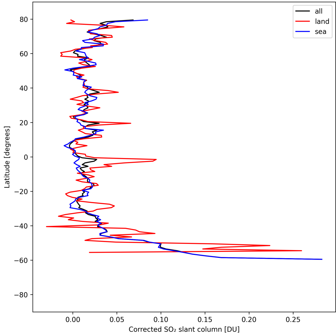
Figure 33: Zonal average of “Corrected SO 2 slant column” for 2025-08-28 to 2025-08-28.
