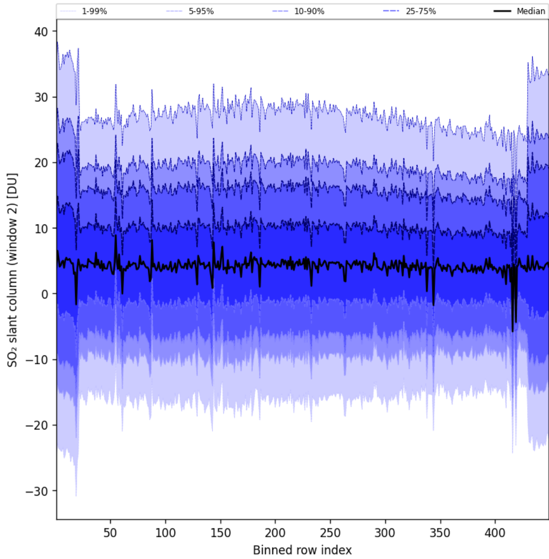
Figure 94: Along track statistics of “SO 2 slant column (window 2)” for 2025-08-28 to 2025-08-28
