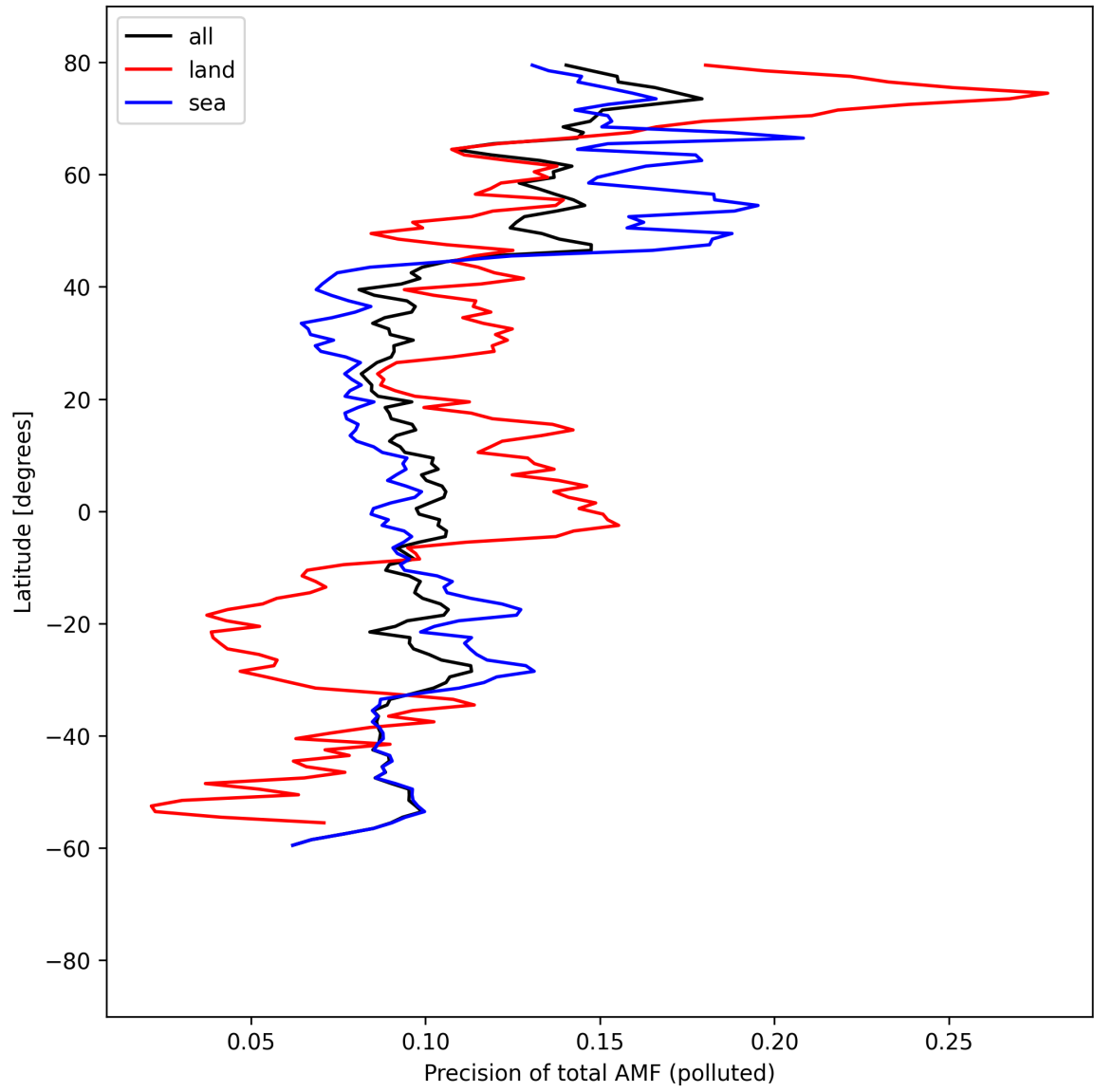
Figure 54: Zonal average of “Precision of total AMF (polluted)” for 2025-08-28 to 2025-08-28.
