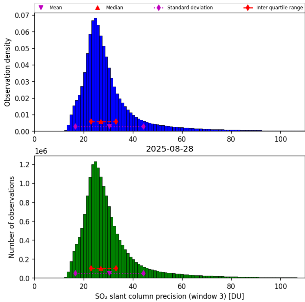
Figure 72: Histogram of “SO 2 slant column precision (window 3)” for 2025-08-28 to 2025-08-28
