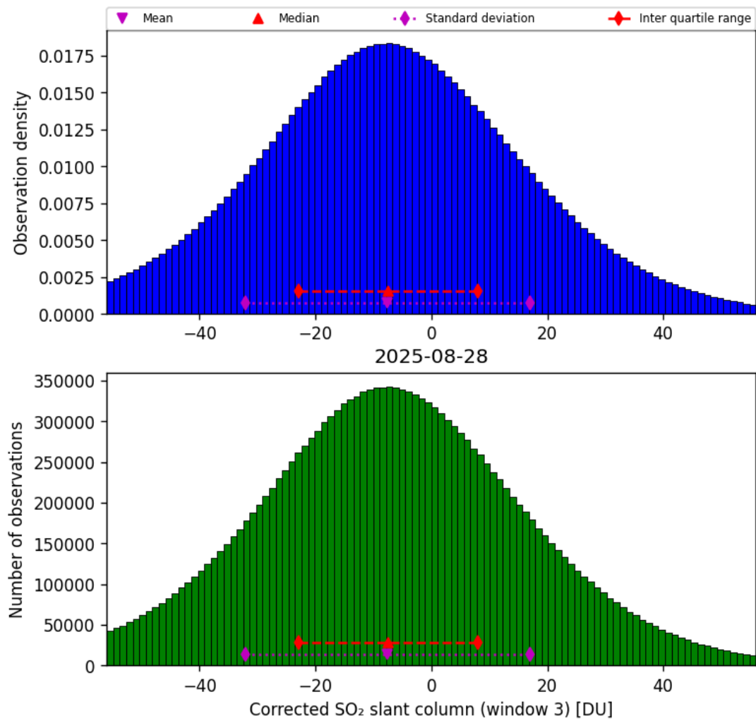
Figure 73: Histogram of “Corrected SO 2 slant column (window 3)” for 2025-08-28 to 2025-08-28
