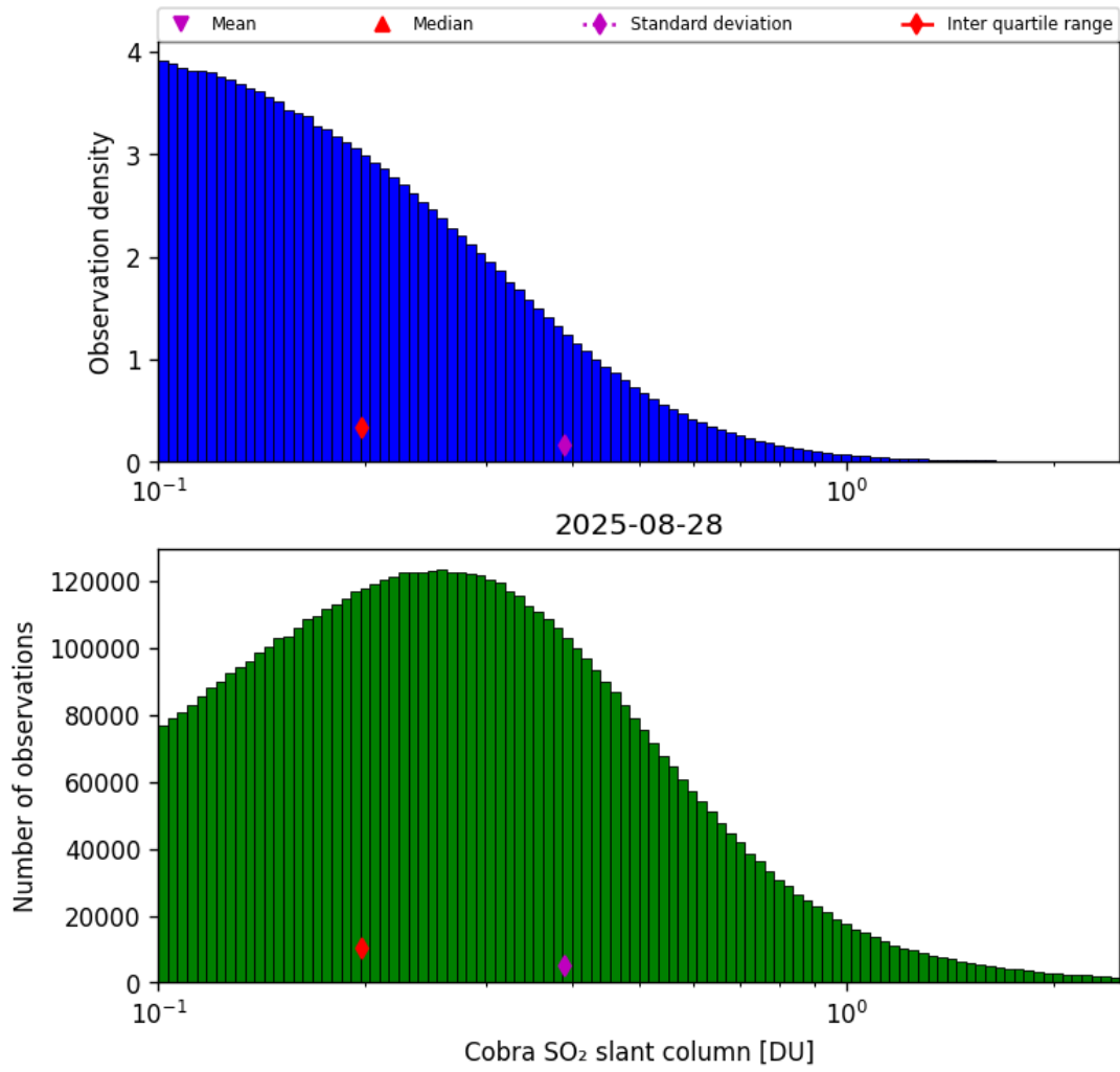
Figure 61: Histogram of “Cobra SO 2 slant column” for 2025-08-28 to 2025-08-28
