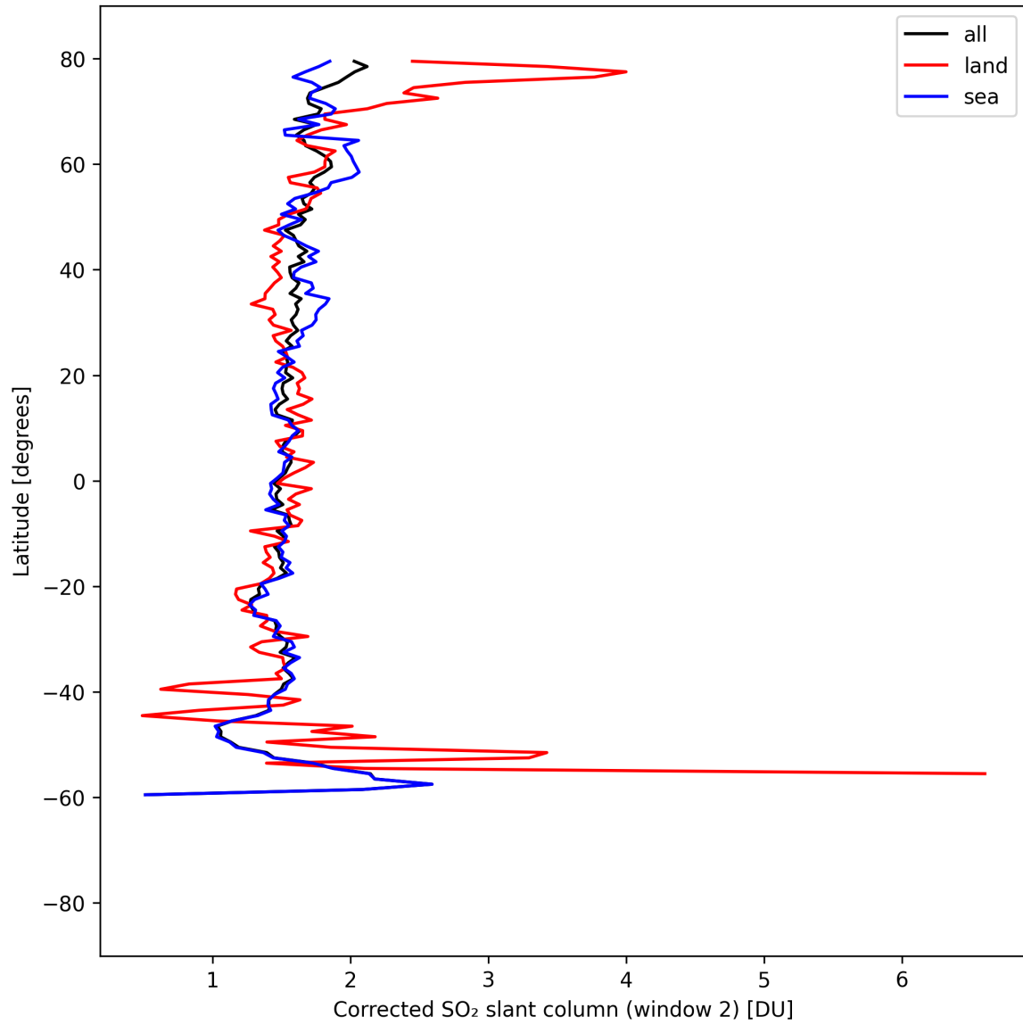
Figure 42: Zonal average of “Corrected SO 2 slant column (window 2)” for 2025-08-28 to 2025-08-28.
