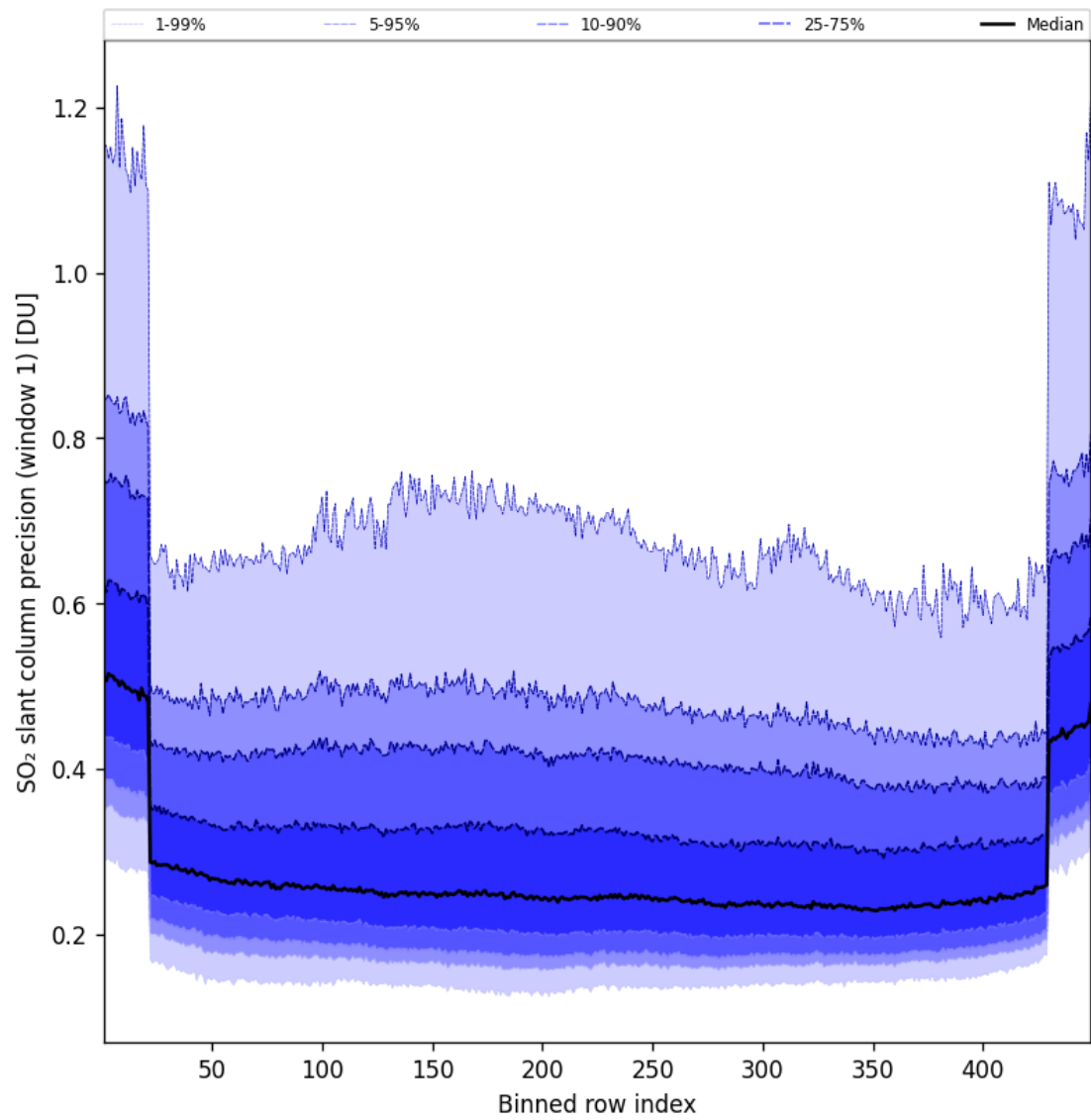
Figure 91: Along track statistics of “SO 2 slant column precision (window 1)” for 2025-08-28 to 2025-08-28
