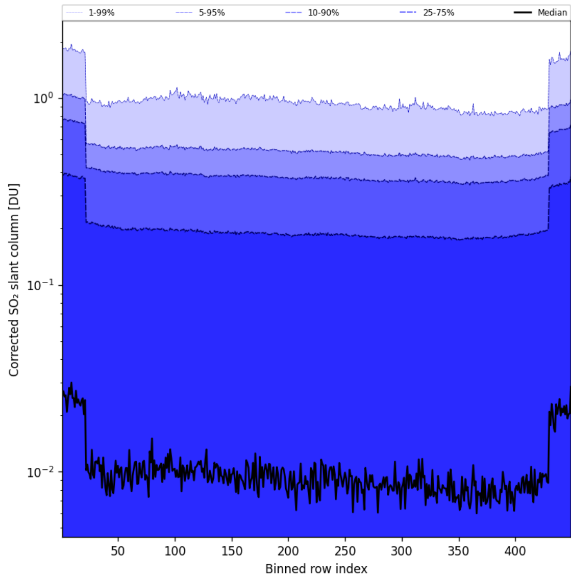
Figure 87: Along track statistics of "Corrected SO 2 slant column" for 2025-08-28 to 2025-08-28
