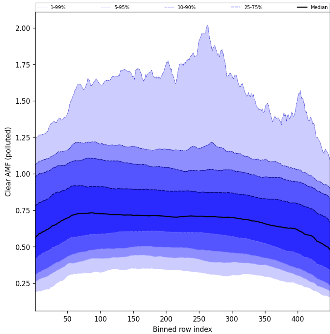
Figure 109: Along track statistics of “Clear AMF (polluted)” for 2025-08-28 to 2025-08-28
