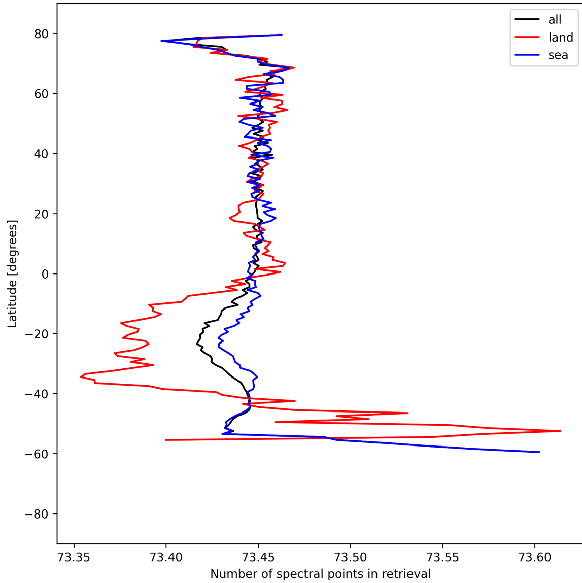
Figure 56: Zonal average of “Number of spectral points in retrieval” for 2025-08-28 to 2025-08-28.
