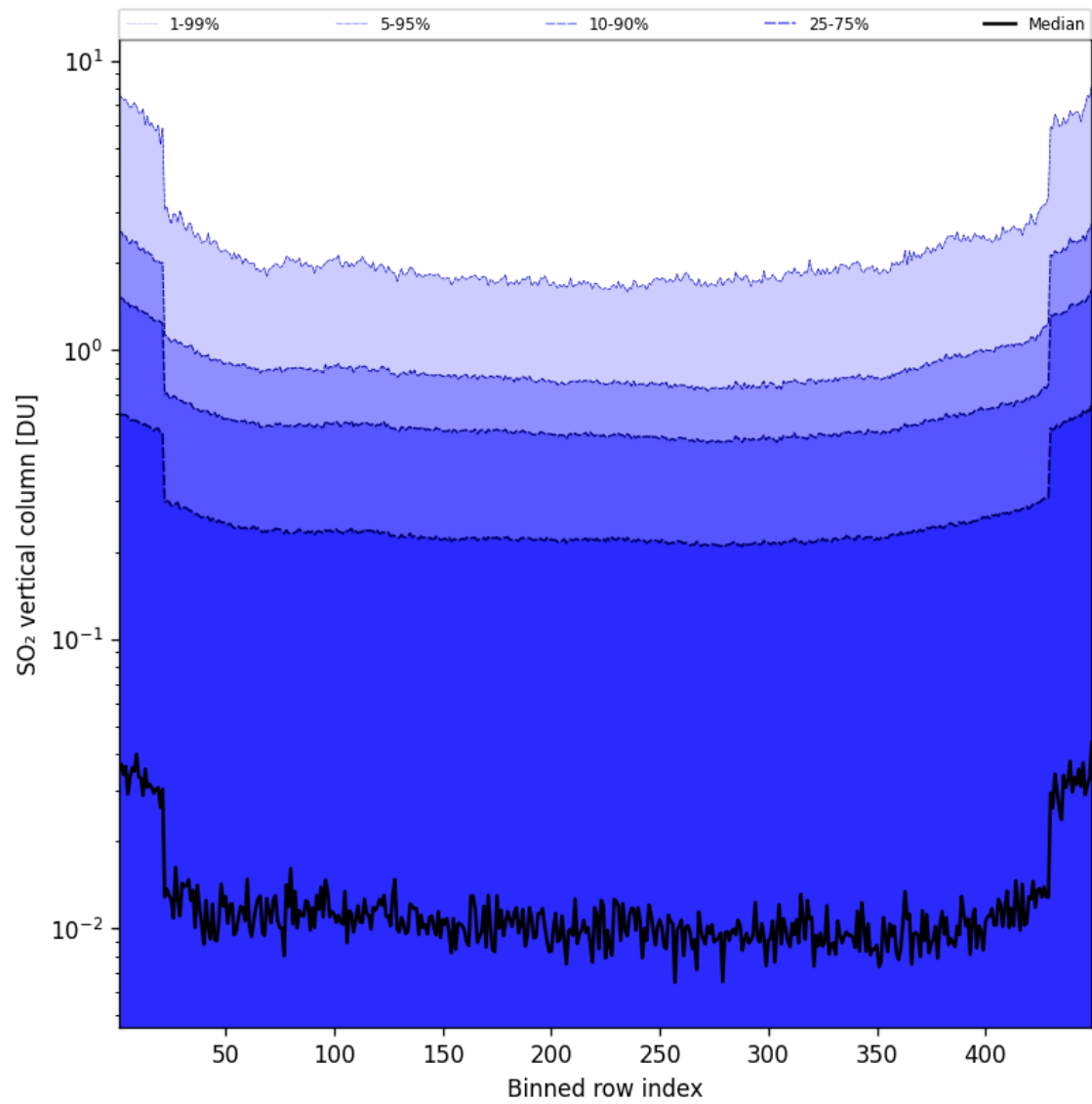
Figure 85: Along track statistics of “SO 2 vertical column” for 2025-08-28 to 2025-08-28
