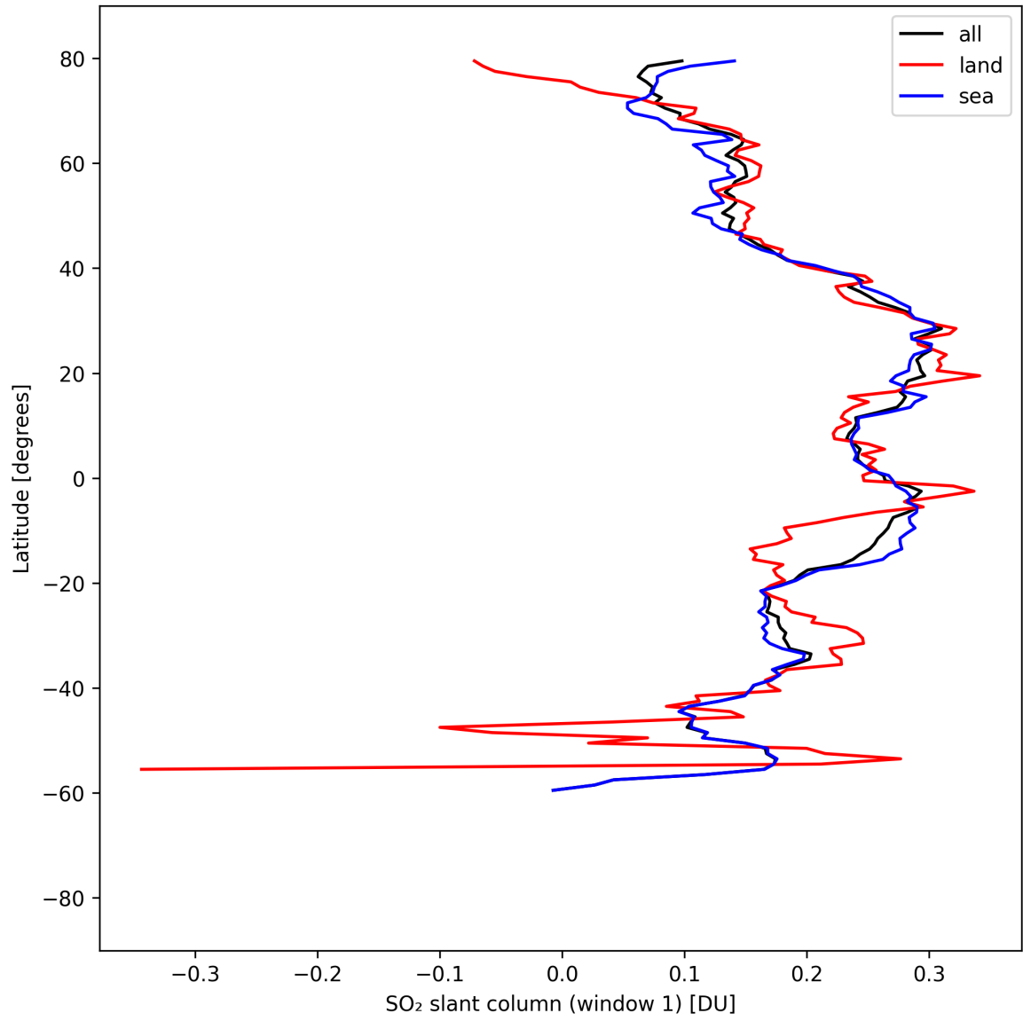
Figure 36: Zonal average of “SO 2 slant column (window 1)” for 2025-08-28 to 2025-08-28.
