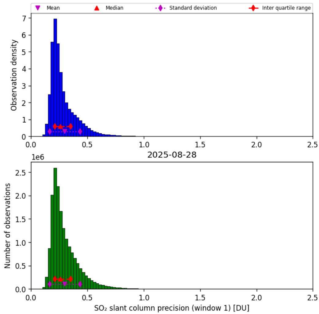
Figure 64: Histogram of “SO 2 slant column precision (window 1)” for 2025-08-28 to 2025-08-28
