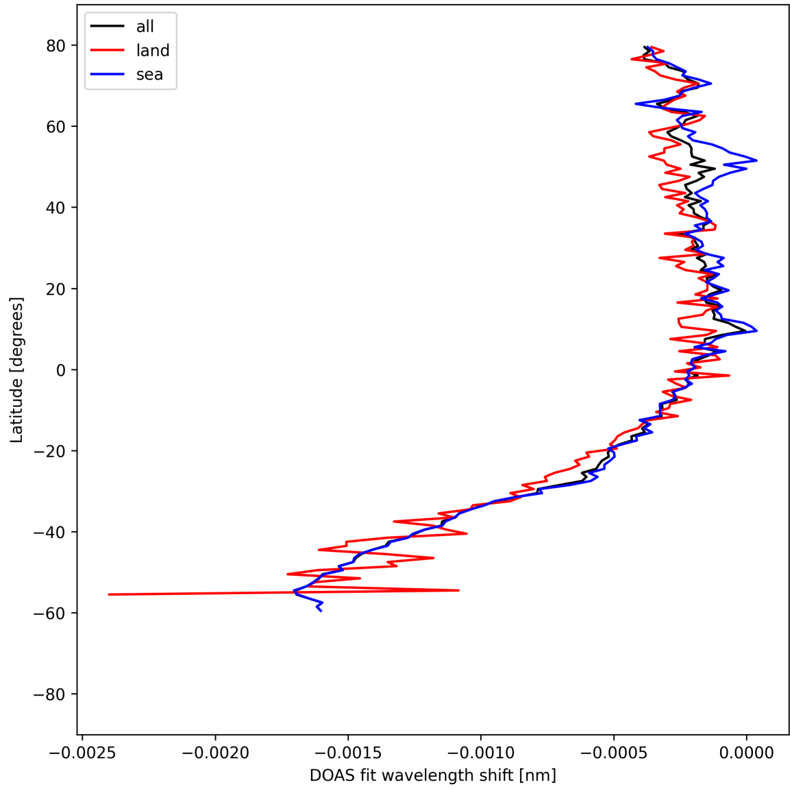
Figure 50: Zonal average of “DOAS fit wavelength shift” for 2025-08-28 to 2025-08-28.
