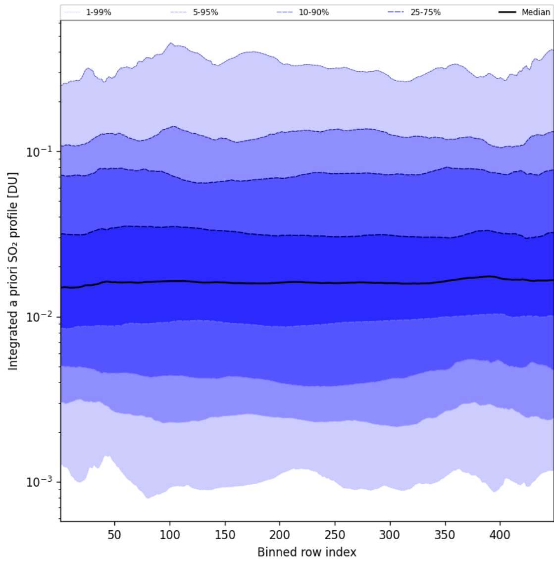
Figure 103: Along track statistics of “Integrated a priori SO 2 profile” for 2025-08-28 to 2025-08-28
