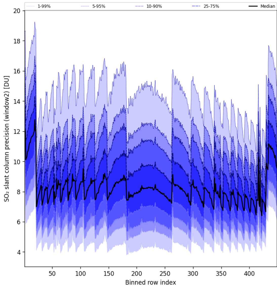
Figure 95: Along track statistics of “SO 2 slant column precision (window2)” for 2025-08-28 to 2025-08-28
