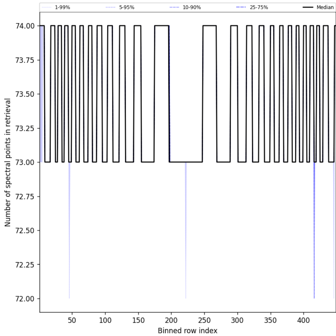
Figure 110: Along track statistics of “Number of spectral points in retrieval” for 2025-08-28 to 2025-08-28
