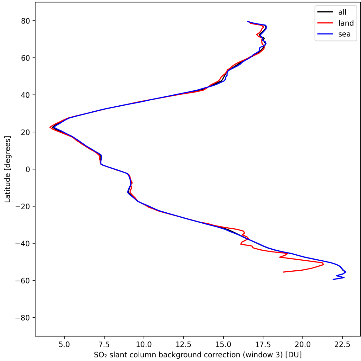
Figure 47: Zonal average of “SO 2 slant column background correction (window 3)” for 2025-08-28 to 2025-08-28.
