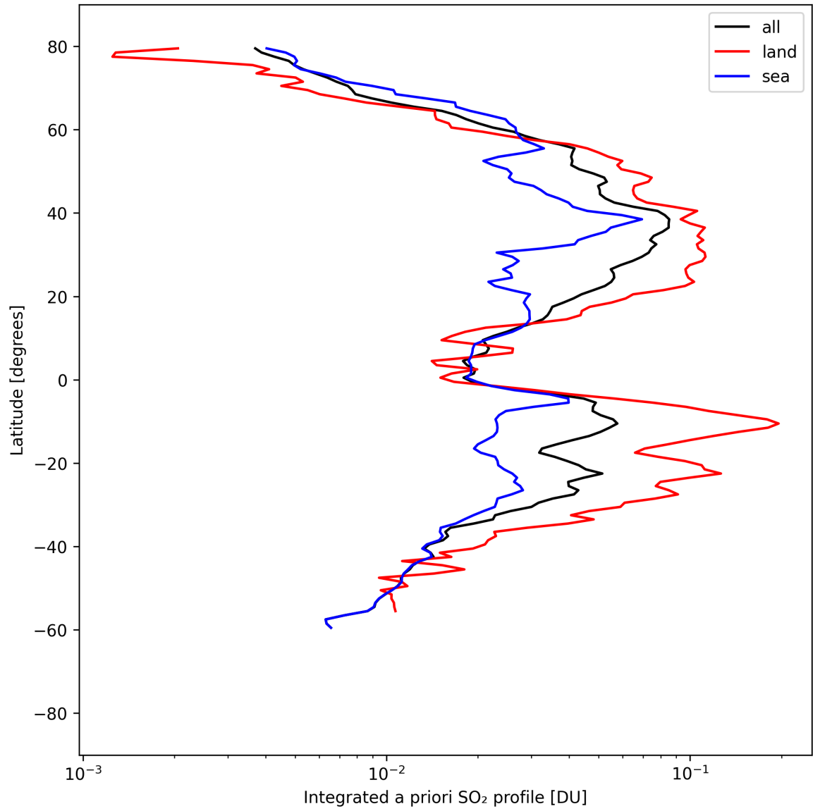
Figure 49: Zonal average of “Integrated a priori SO 2 profile” for 2025-08-28 to 2025-08-28.
