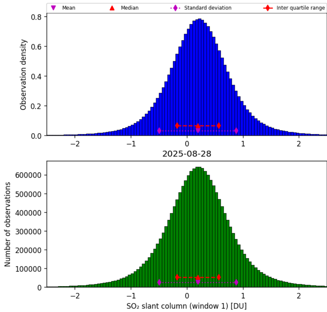
Figure 63: Histogram of “SO 2 slant column (window 1)” for 2025-08-28 to 2025-08-28
