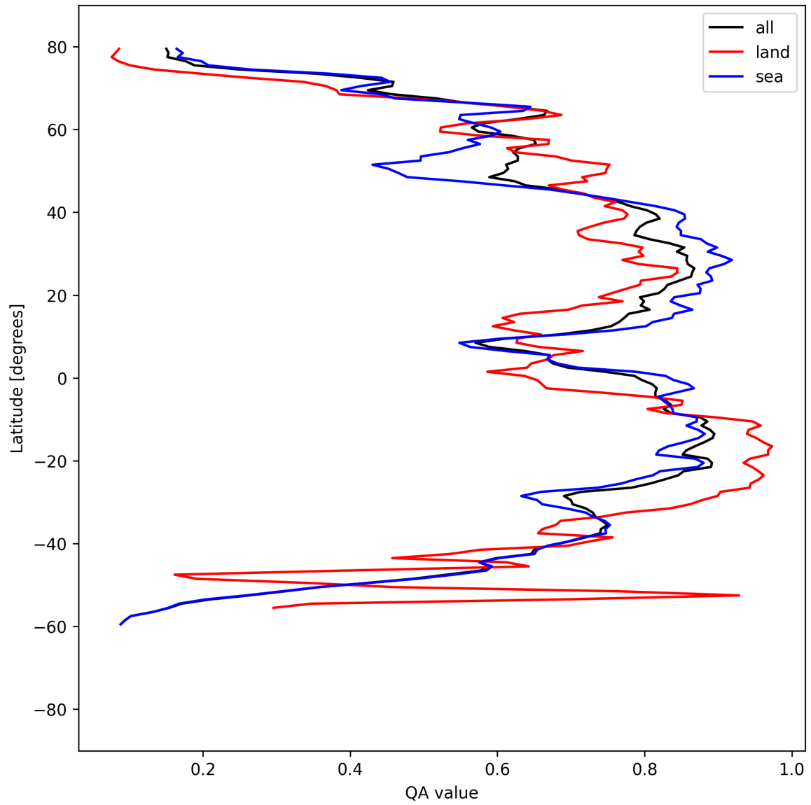
Figure 30: Zonal average of “QA value” for 2025-08-28 to 2025-08-28.
