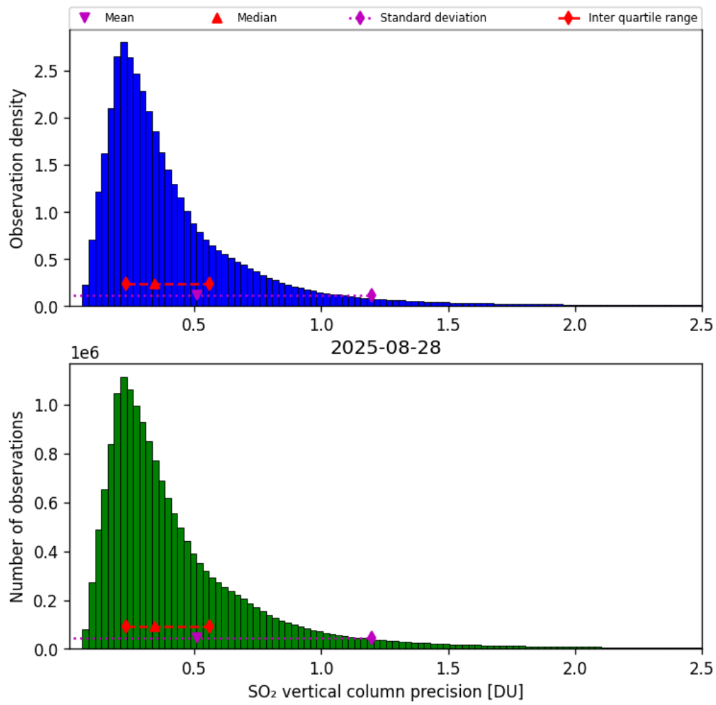
Figure 59: Histogram of “SO 2 vertical column precision” for 2025-08-28 to 2025-08-28
