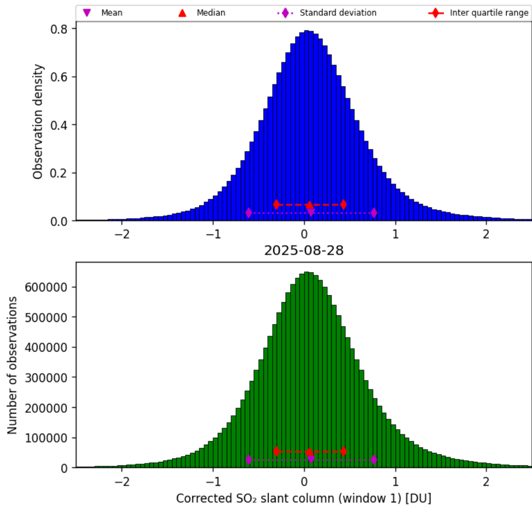
Figure 65: Histogram of “Corrected SO 2 slant column (window 1)” for 2025-08-28 to 2025-08-28
