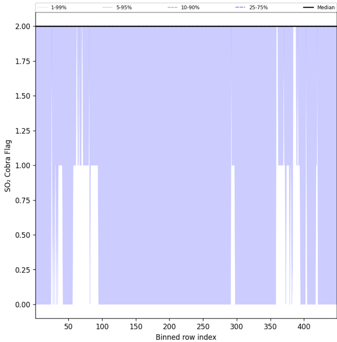
Figure 102: Along track statistics of “SO 2 Cobra Flag” for 2025-08-28 to 2025-08-28
