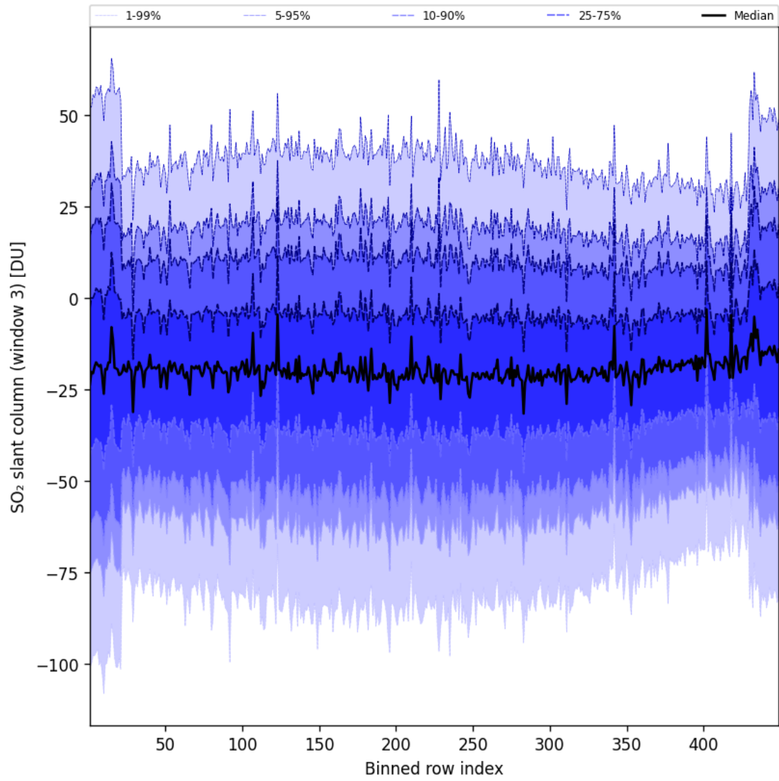
Figure 98: Along track statistics of “SO 2 slant column (window 3)” for 2025-08-28 to 2025-08-28
