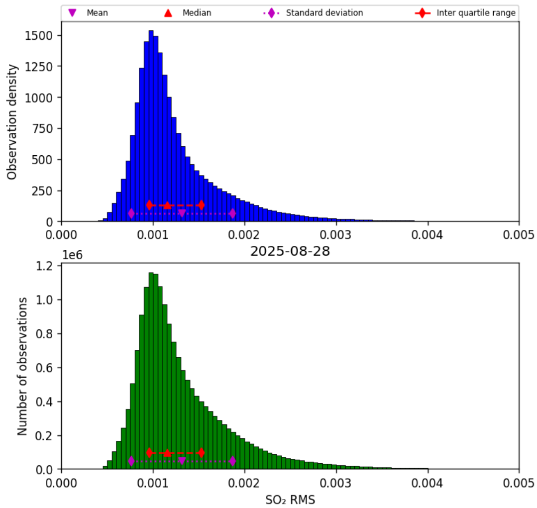
Figure 79: Histogram of “SO 2 RMS” for 2025-08-28 to 2025-08-28
