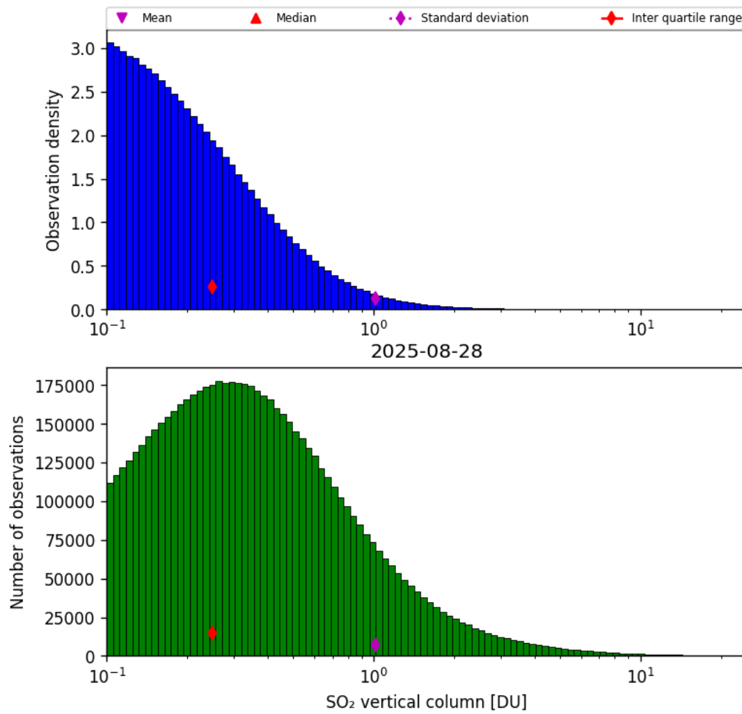
Figure 58: Histogram of “SO 2 vertical column” for 2025-08-28 to 2025-08-28
