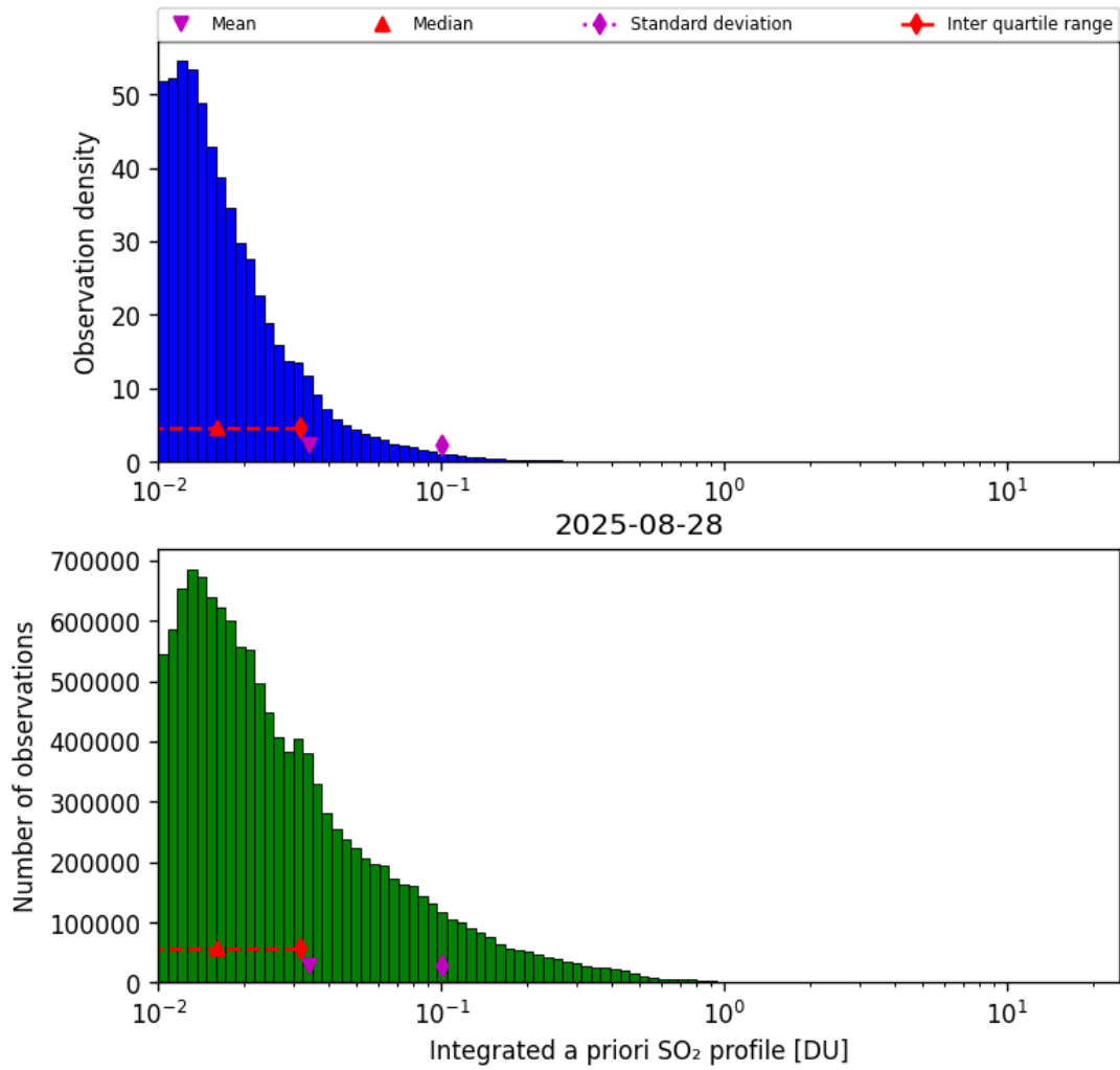
Figure 76: Histogram of “Integrated a priori SO 2 profile” for 2025-08-28 to 2025-08-28
