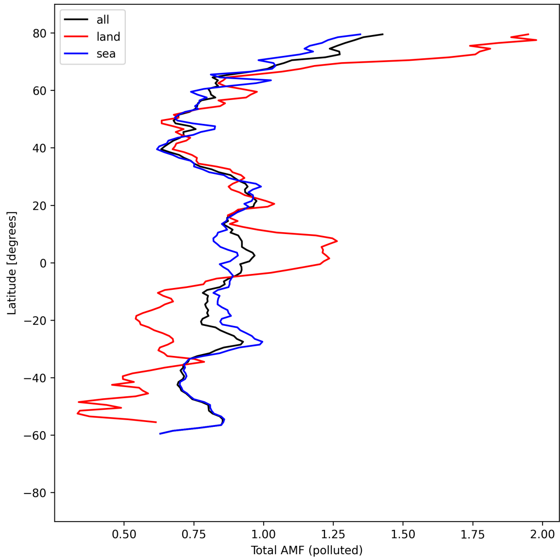
Figure 53: Zonal average of “Total AMF (polluted)” for 2025-08-28 to 2025-08-28.
