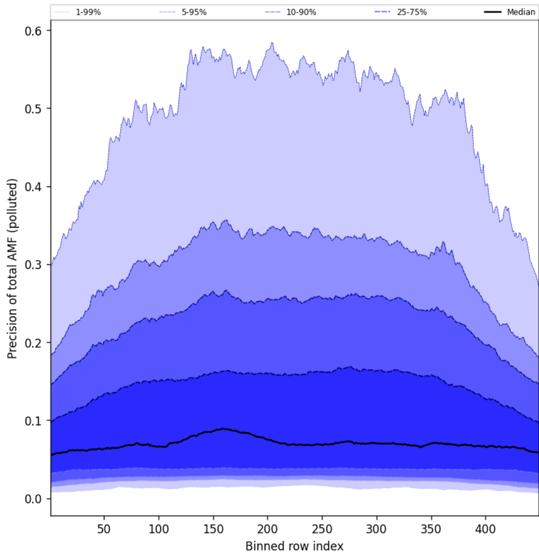
Figure 108: Along track statistics of “Precision of total AMF (polluted)” for 2025-08-28 to 2025-08-28
