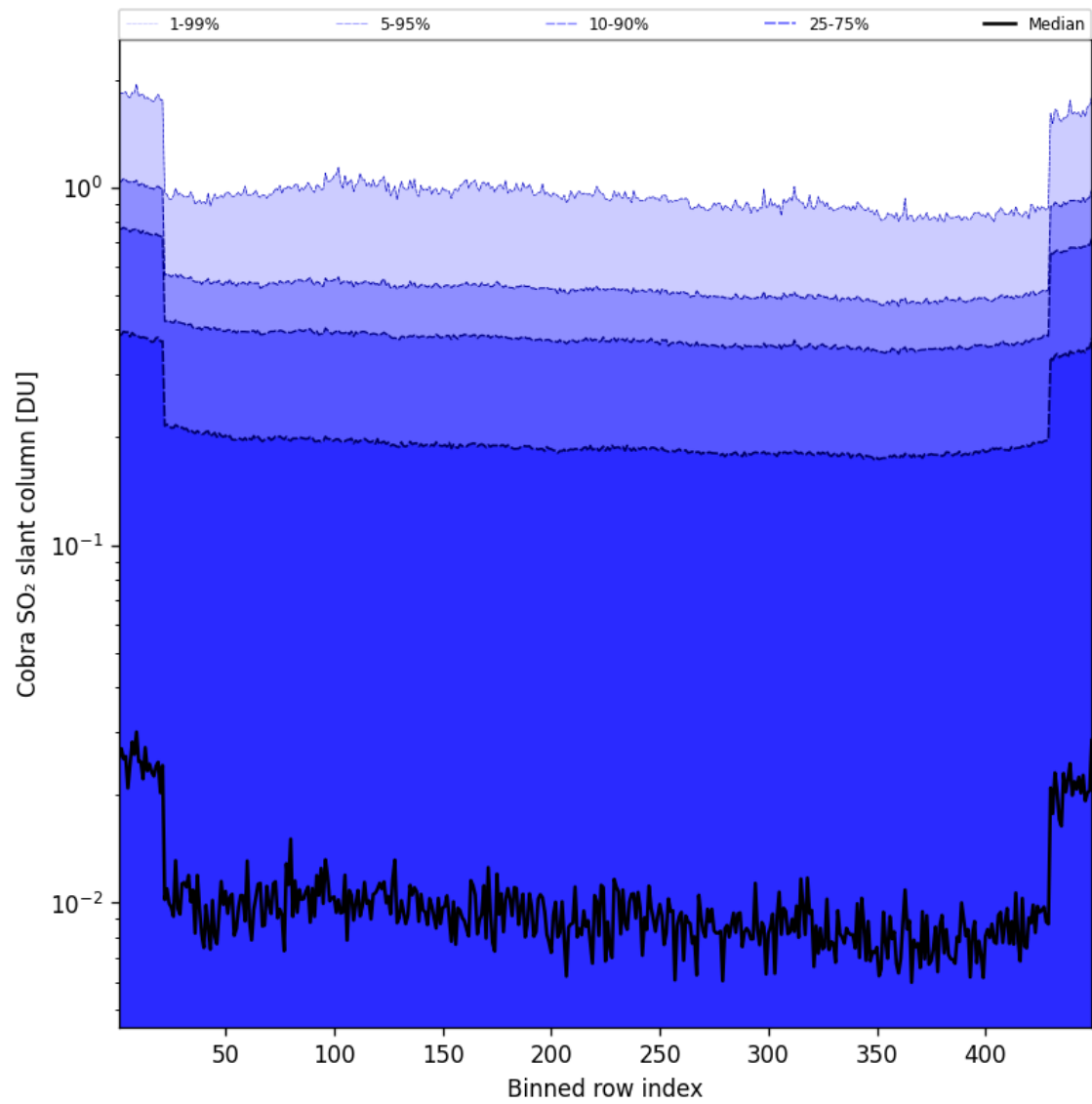
Figure 88: Along track statistics of “Cobra SO 2 slant column” for 2025-08-28 to 2025-08-28
