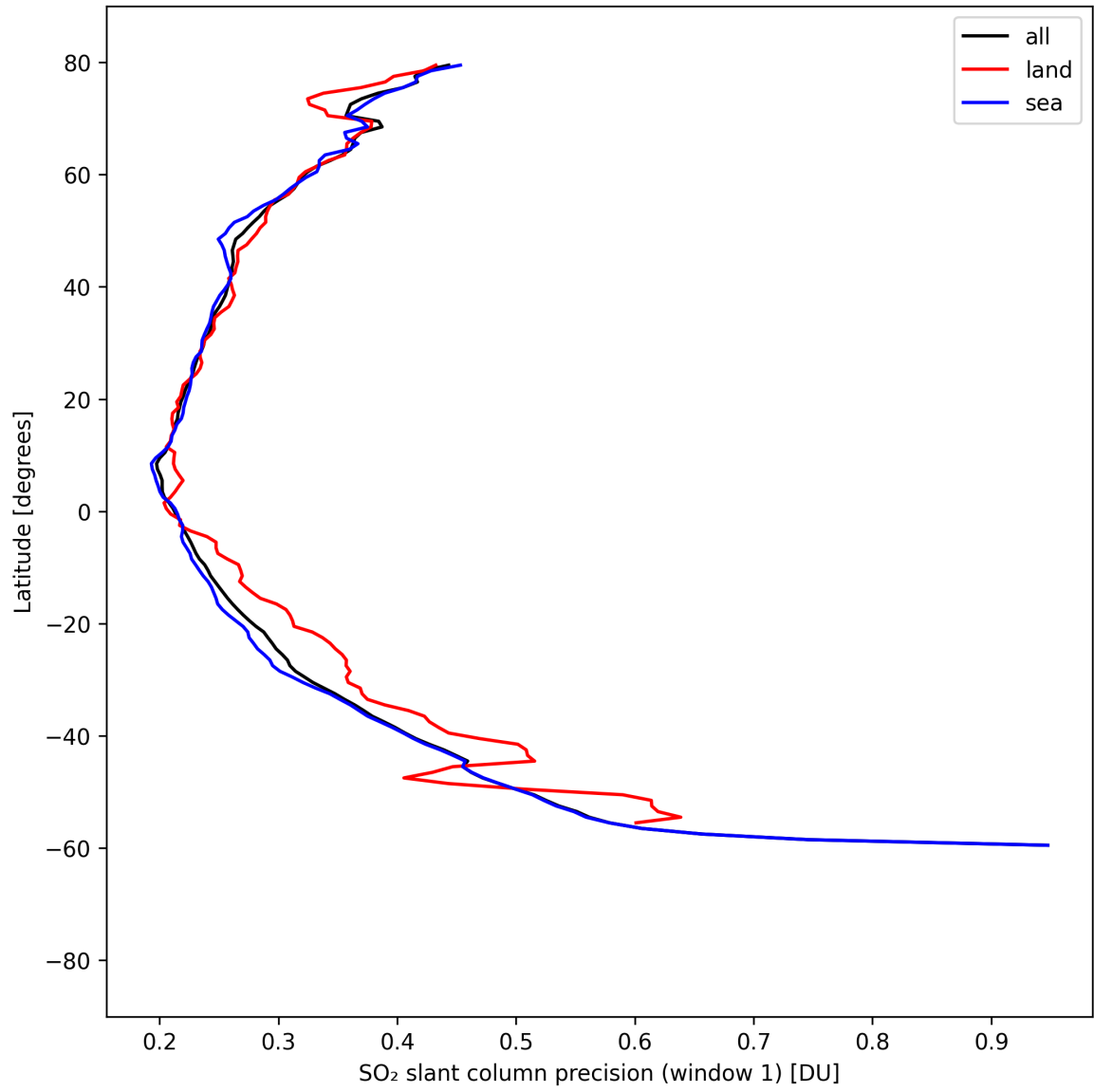
Figure 37: Zonal average of “SO 2 slant column precision (window 1)” for 2025-08-28 to 2025-08-28.
