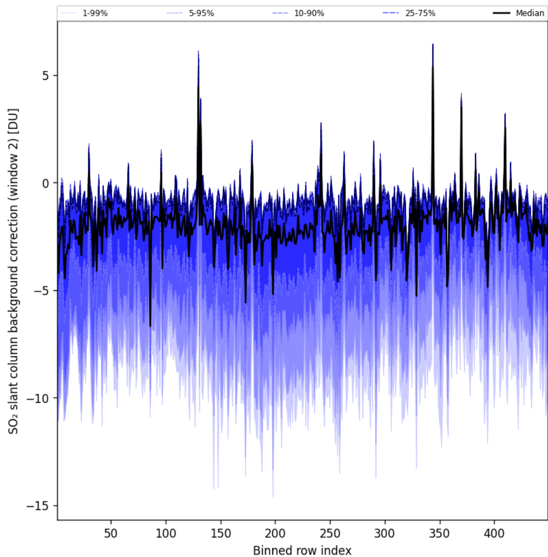
Figure 97: Along track statistics of “SO 2 slant column background correction (window 2)” for 2025-08-28 to 2025-08-28
