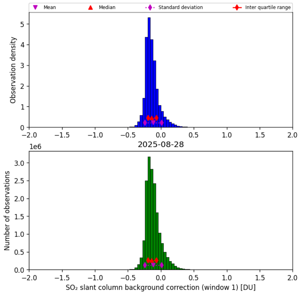
Figure 66: Histogram of “SO 2 slant column background correction (window 1)” for 2025-08-28 to 2025-08-28
