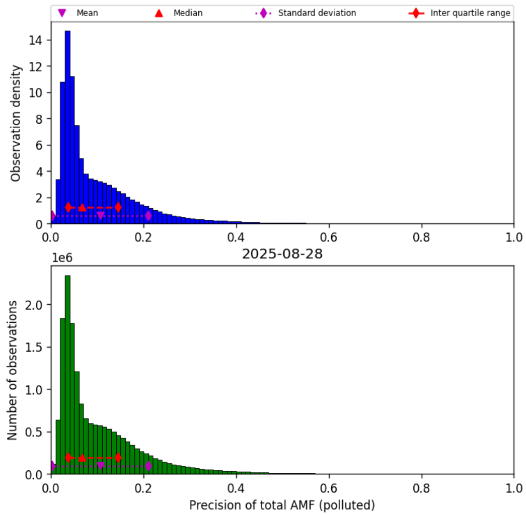
Figure 81: Histogram of “Precision of total AMF (polluted)” for 2025-08-28 to 2025-08-28
