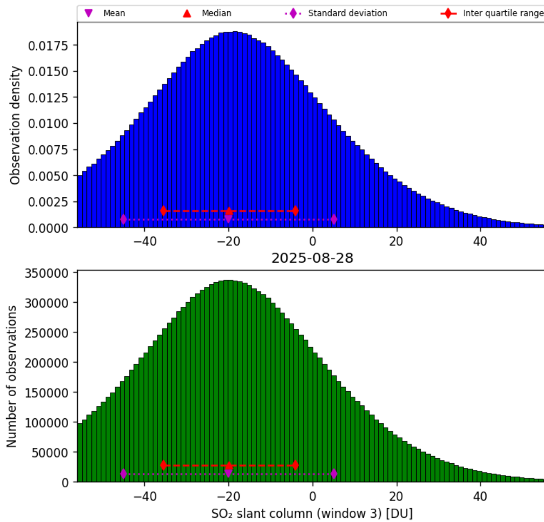
Figure 71: Histogram of “SO 2 slant column (window 3)” for 2025-08-28 to 2025-08-28
