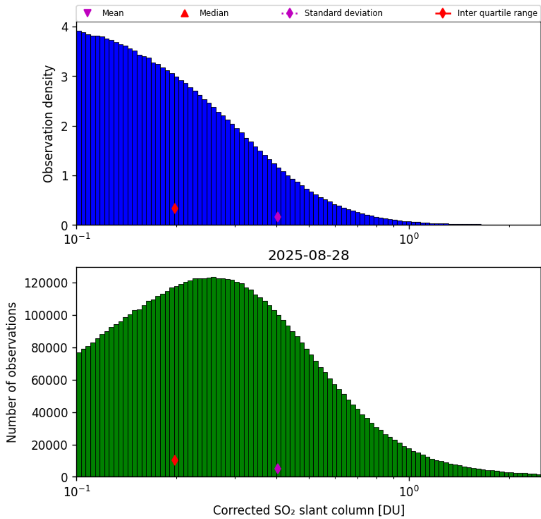
Figure 60: Histogram of “Corrected SO 2 slant column” for 2025-08-28 to 2025-08-28
