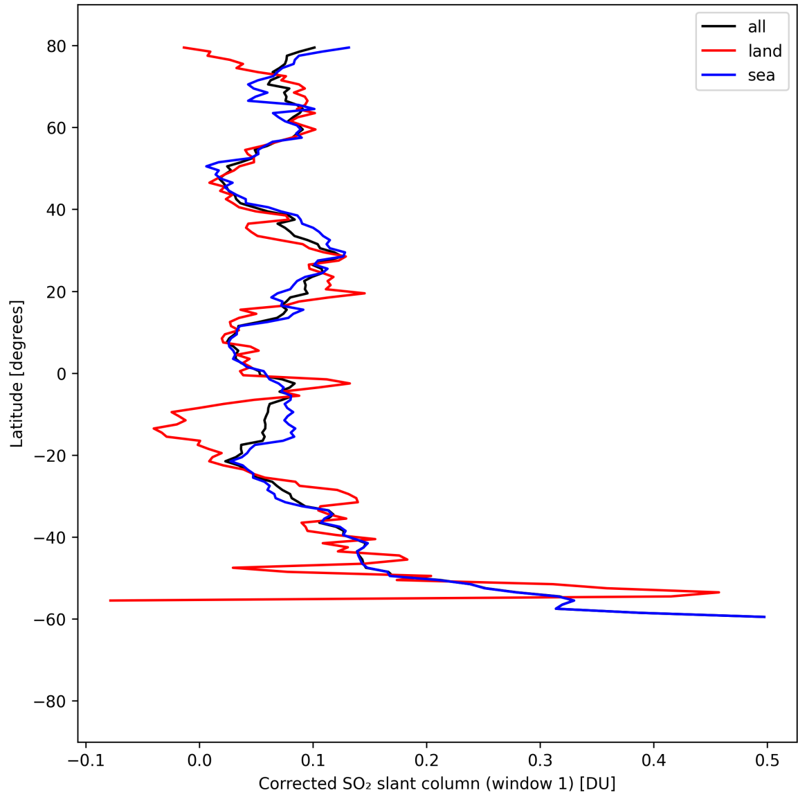
Figure 38: Zonal average of “Corrected SO 2 slant column (window 1)” for 2025-08-28 to 2025-08-28.
