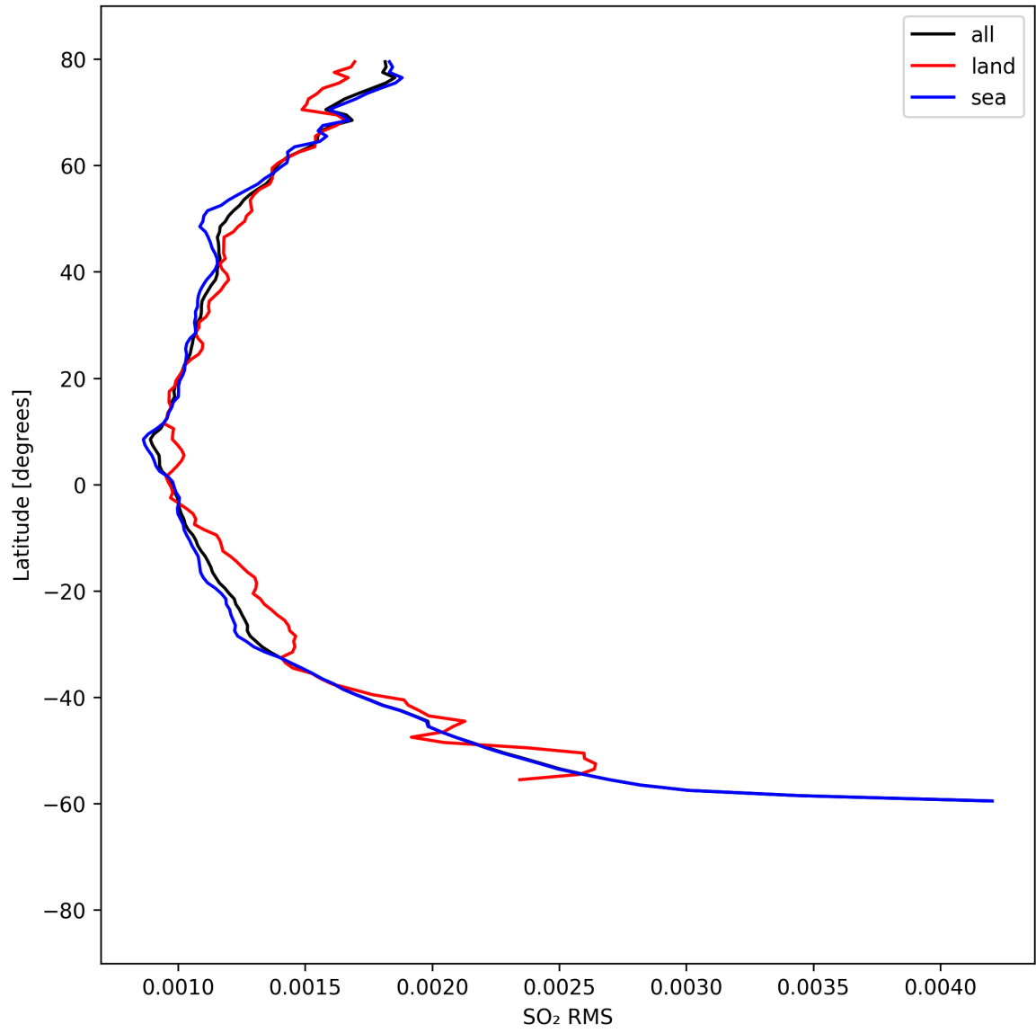
Figure 52: Zonal average of “SO 2 RMS” for 2025-08-28 to 2025-08-28.
