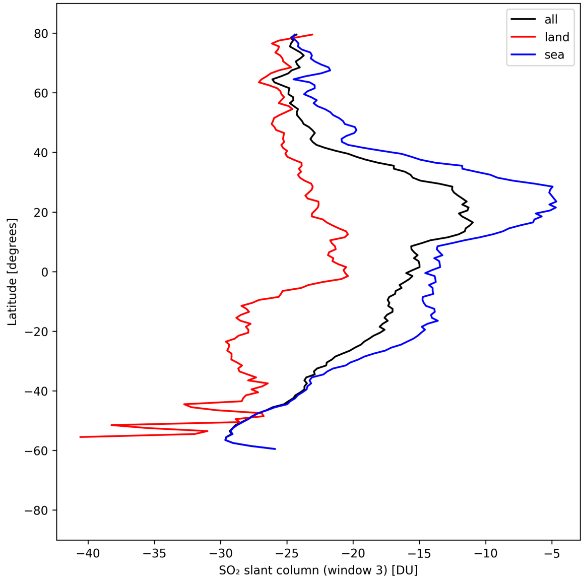
Figure 44: Zonal average of “SO 2 slant column (window 3)” for 2025-08-28 to 2025-08-28.
