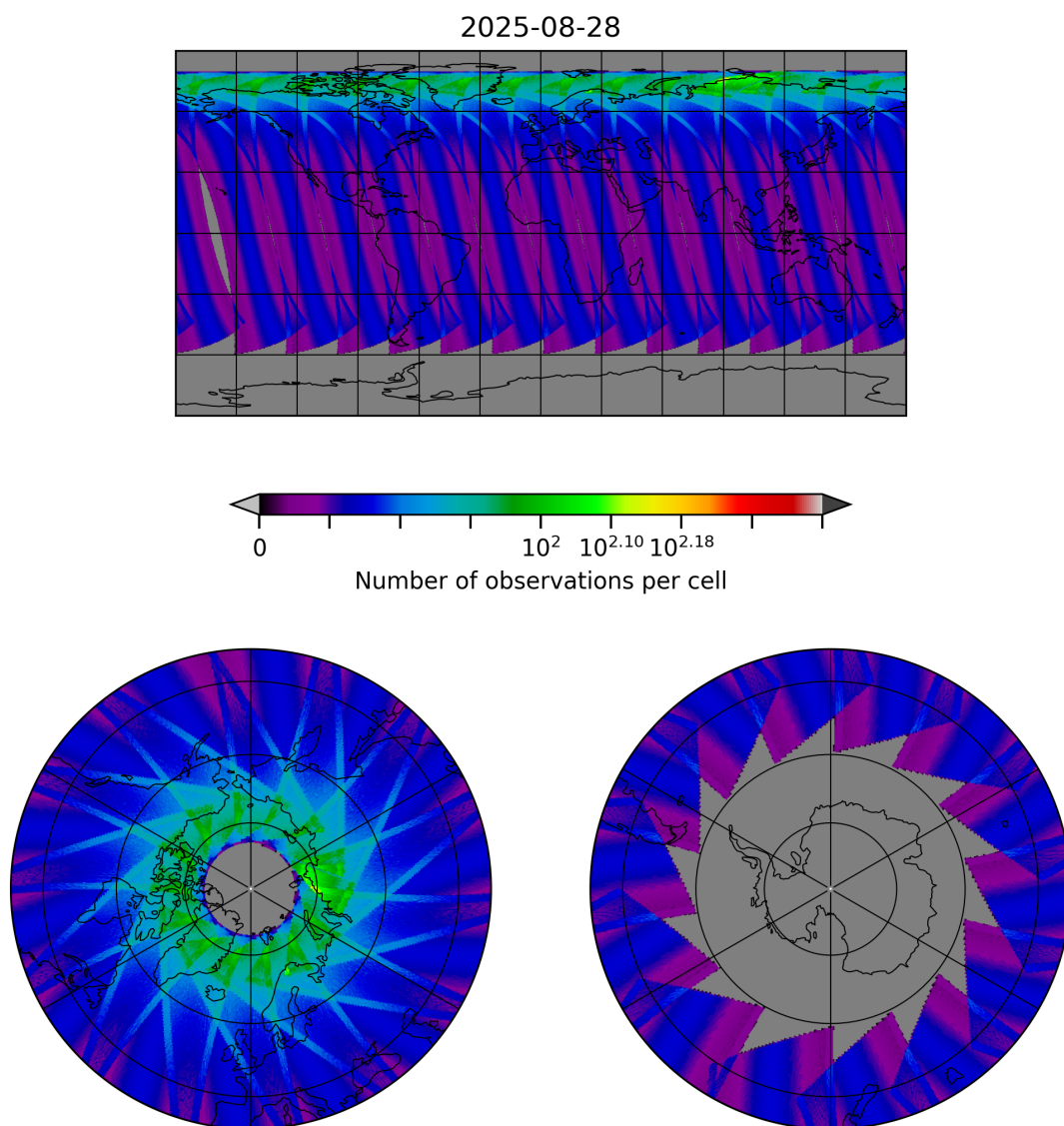
Figure 29: Map of the number of observations for 2025-08-28 to 2025-08-28
