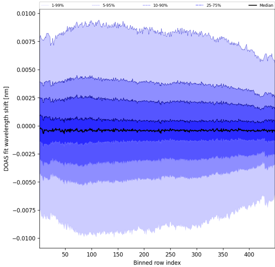
Figure 104: Along track statistics of “DOAS fit wavelength shift” for 2025-08-28 to 2025-08-28
