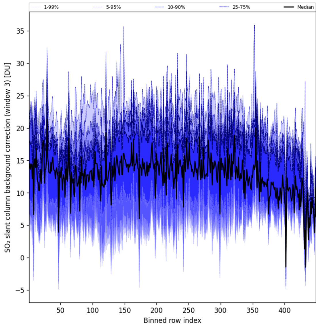
Figure 101: Along track statistics of “SO 2 slant column background correction (window 3)” for 2025-08-28 to 2025-08-28
