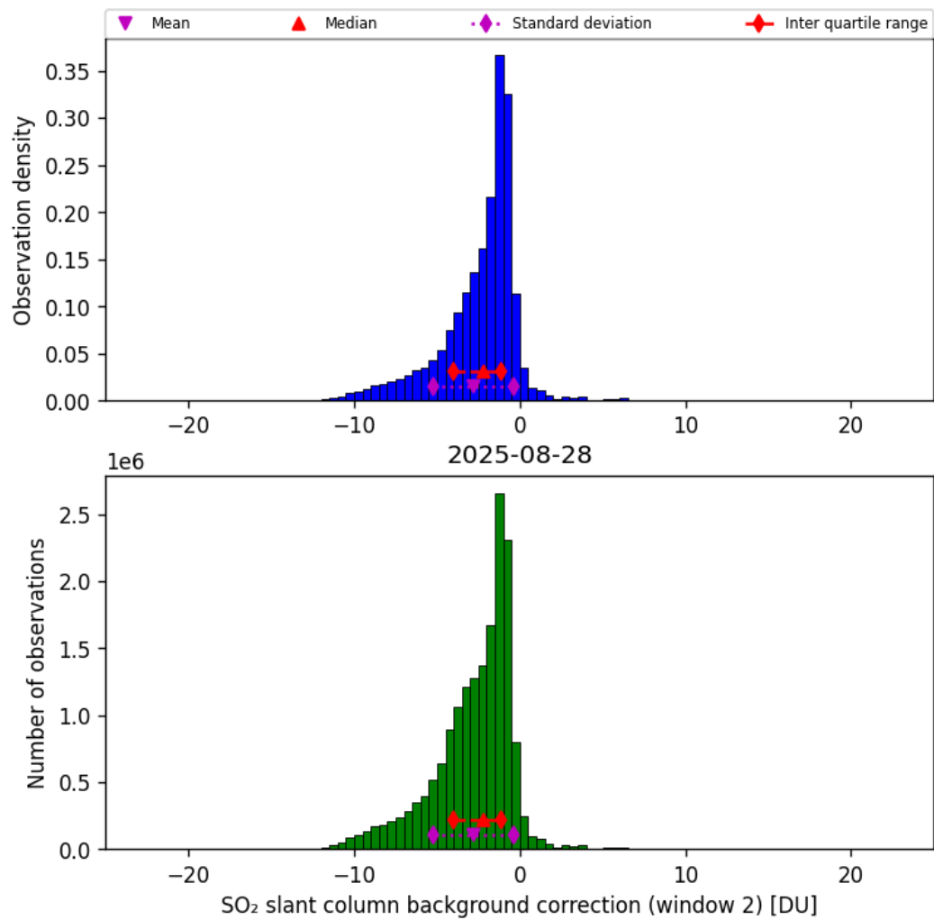
Figure 70: Histogram of “SO 2 slant column background correction (window 2)” for 2025-08-28 to 2025-08-28
