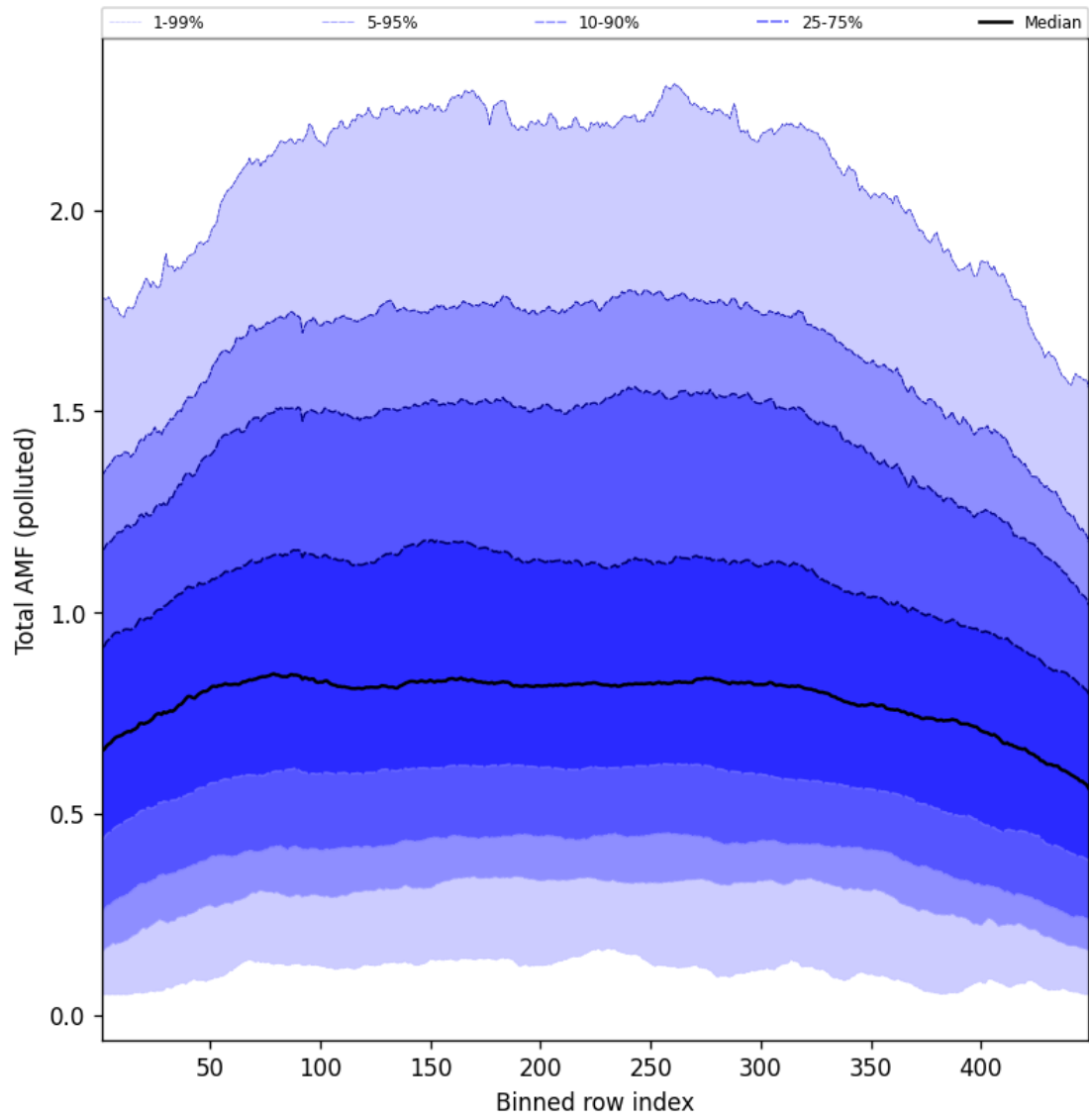
Figure 107: Along track statistics of “Total AMF (polluted)” for 2025-08-28 to 2025-08-28
