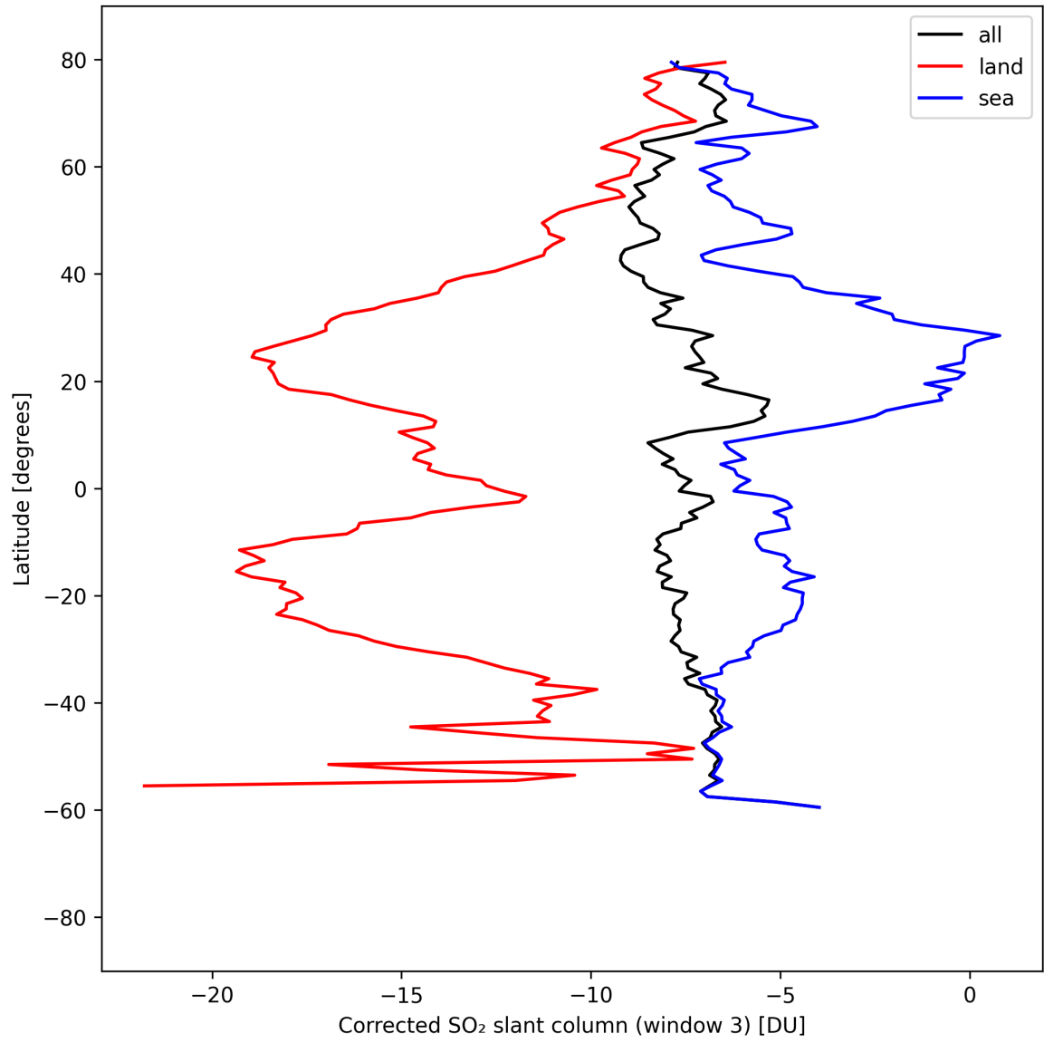
Figure 46: Zonal average of “Corrected SO 2 slant column (window 3)” for 2025-08-28 to 2025-08-28.
