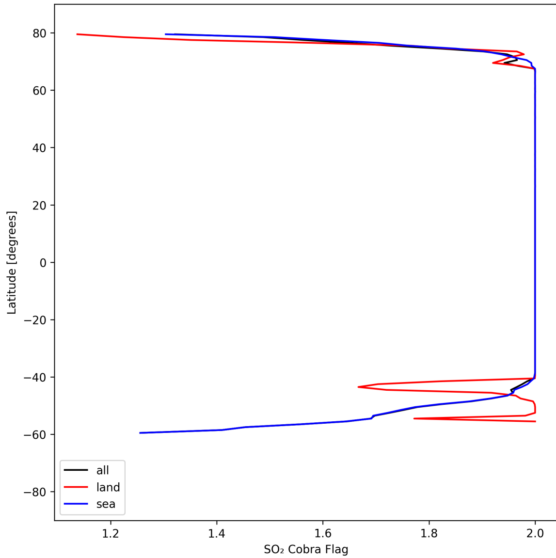
Figure 48: Zonal average of "SO 2 Cobra Flag" for 2025-08-28 to 2025-08-28.
