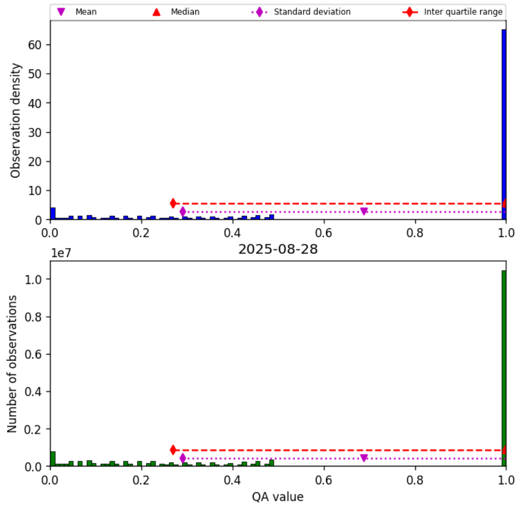
Figure 57: Histogram of “QA value” for 2025-08-28 to 2025-08-28
