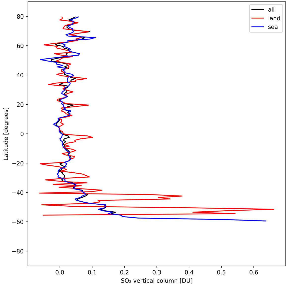
Figure 31: Zonal average of “SO 2 vertical column” for 2025-08-28 to 2025-08-28.
