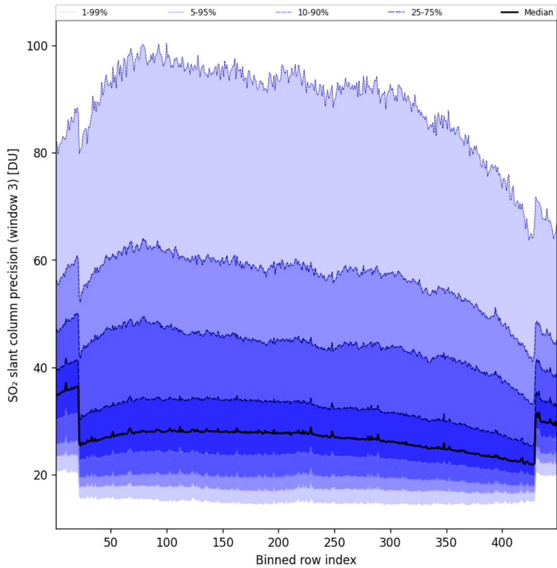
Figure 99: Along track statistics of “SO 2 slant column precision (window 3)” for 2025-08-28 to 2025-08-28
