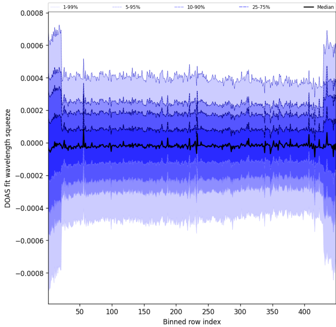
Figure 105: Along track statistics of “DOAS fit wavelength squeeze” for 2025-08-28 to 2025-08-28
