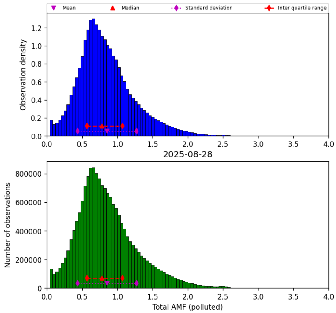
Figure 80: Histogram of “Total AMF (polluted)” for 2025-08-28 to 2025-08-28
