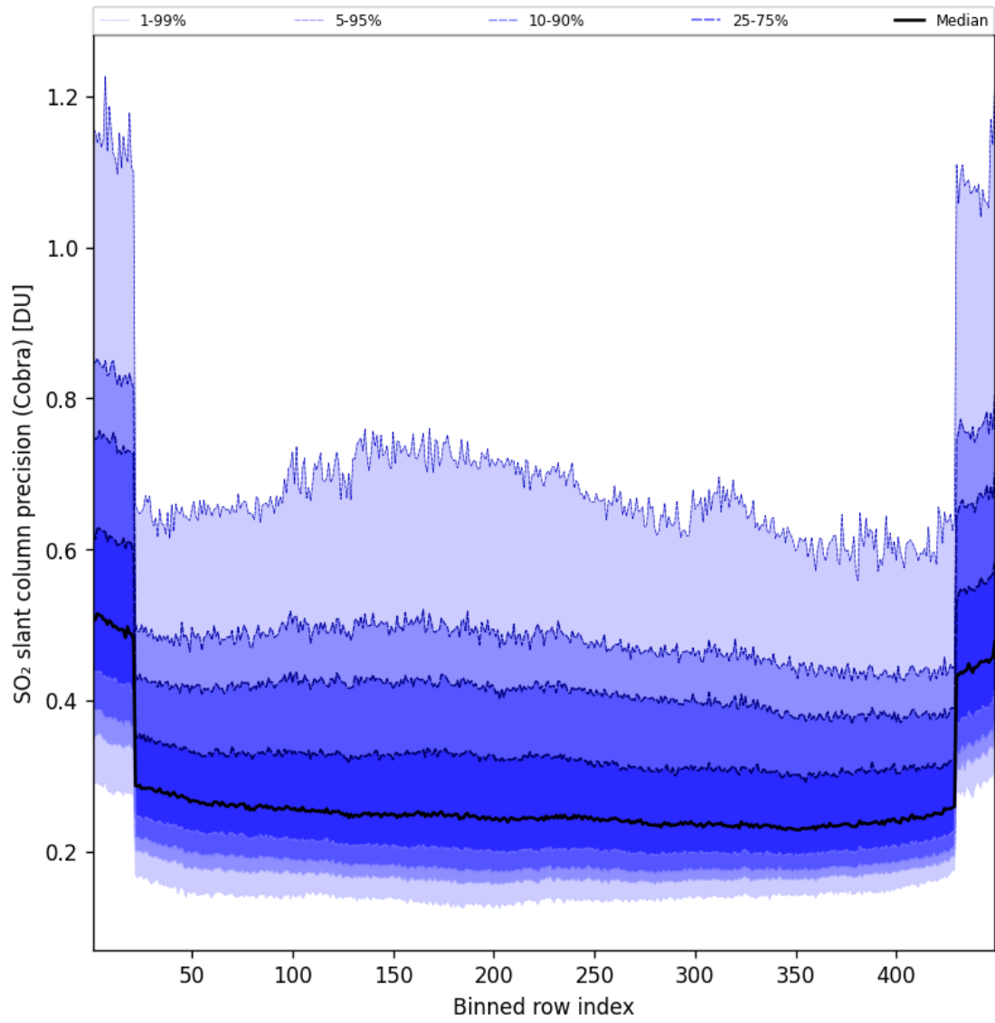
Figure 89: Along track statistics of “SO 2 slant column precision (Cobra)” for 2025-08-28 to 2025-08-28
