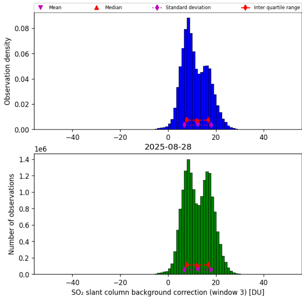
Figure 74: Histogram of “SO 2 slant column background correction (window 3)” for 2025-08-28 to 2025-08-28
