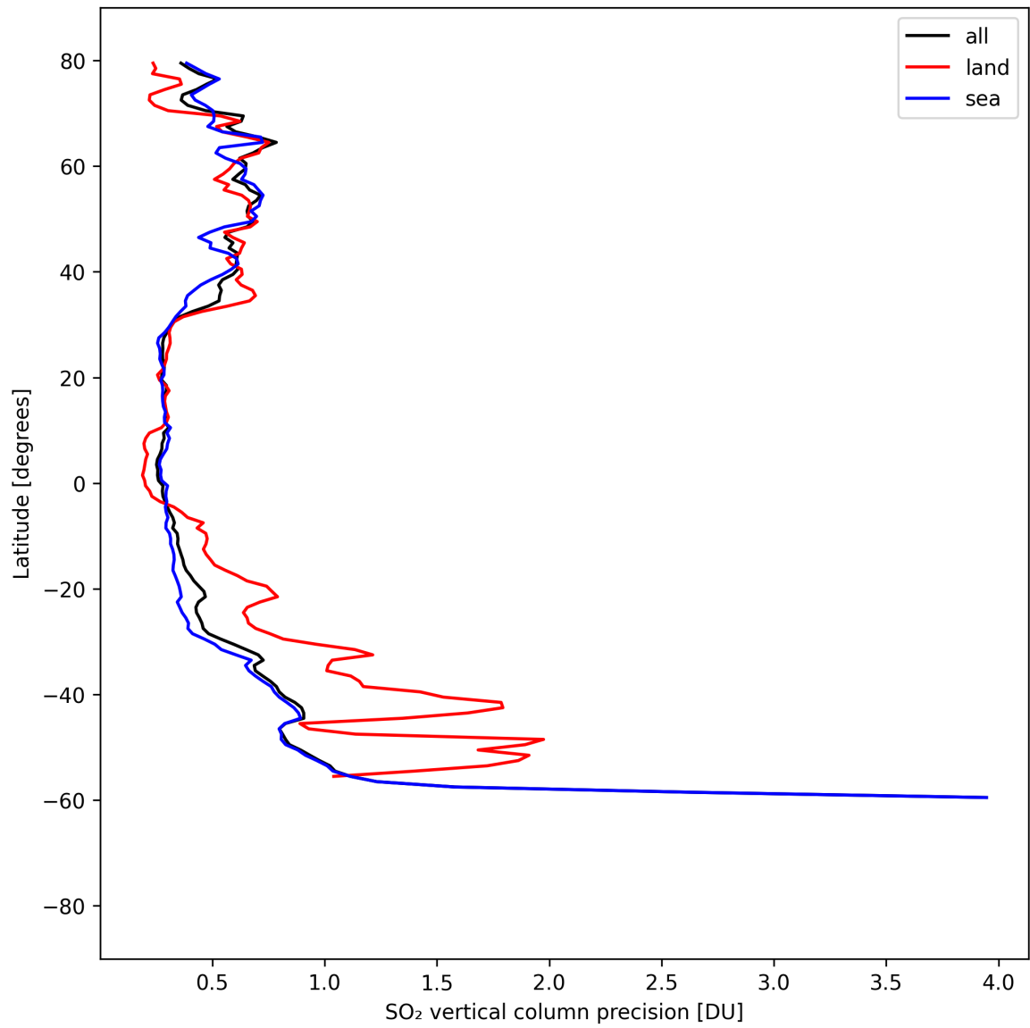
Figure 32: Zonal average of “SO 2 vertical column precision” for 2025-08-28 to 2025-08-28.
