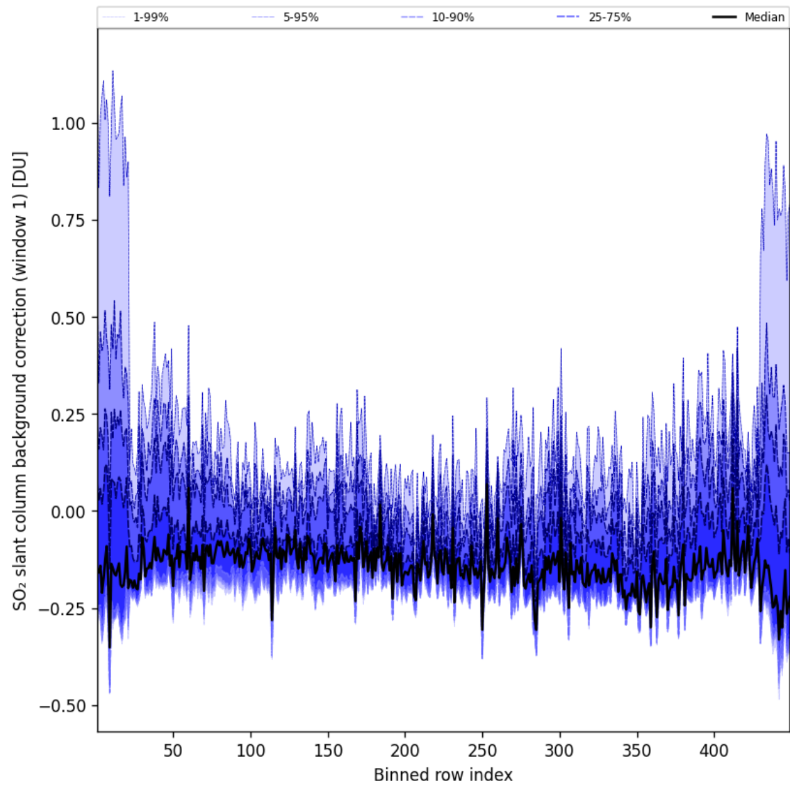
Figure 93: Along track statistics of “SO 2 slant column background correction (window 1)” for 2025-08-28 to 2025-08-28
