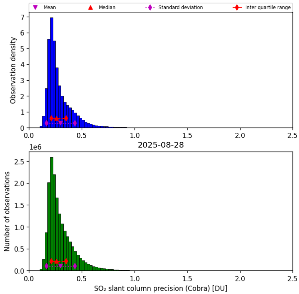
Figure 62: Histogram of “SO 2 slant column precision (Cobra)” for 2025-08-28 to 2025-08-28
