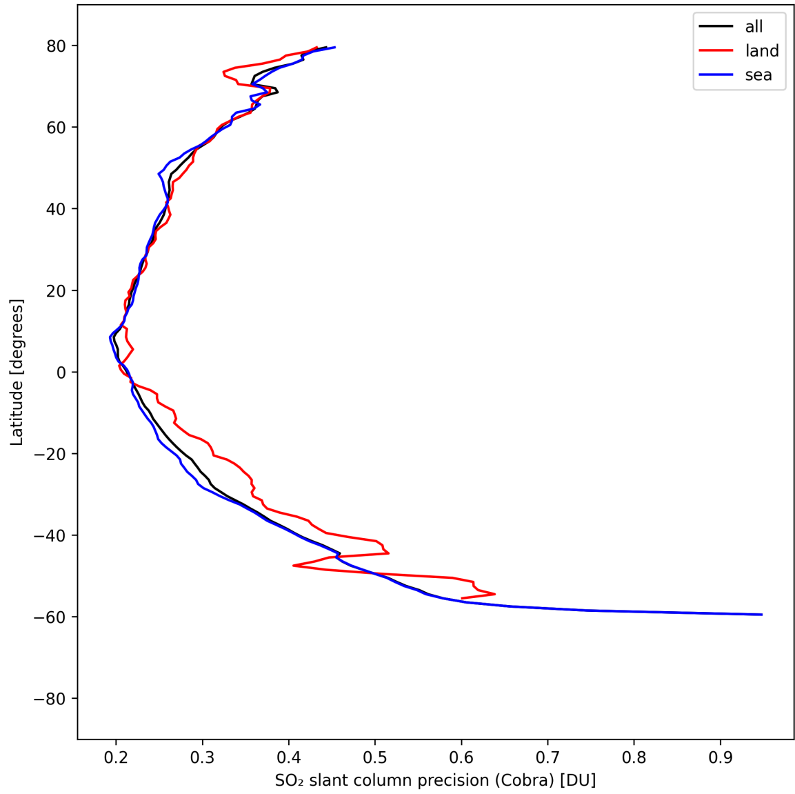
Figure 35: Zonal average of “SO 2 slant column precision (Cobra)” for 2025-08-28 to 2025-08-28.
