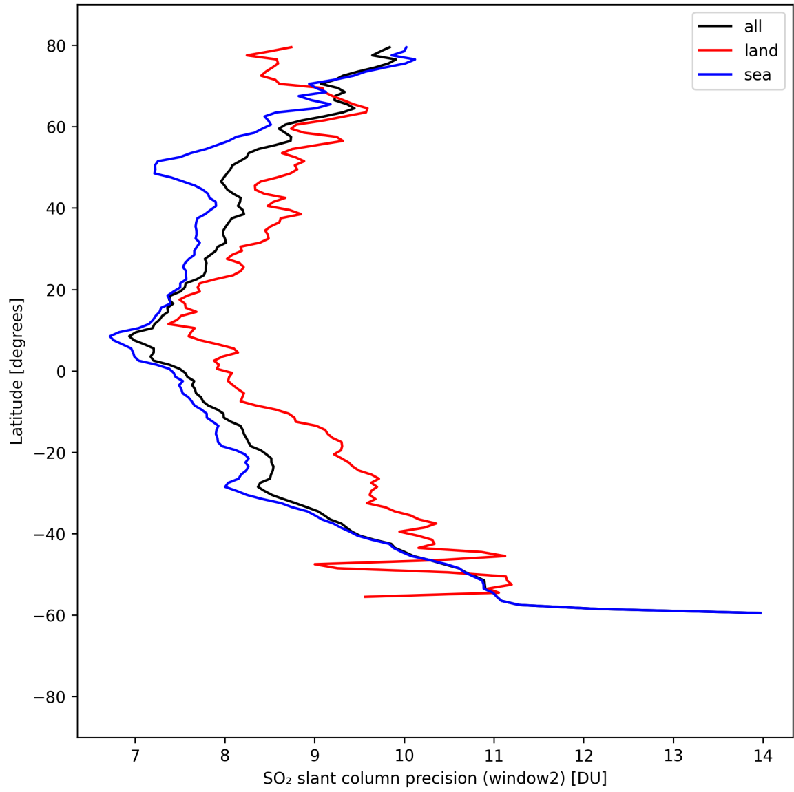
Figure 41: Zonal average of “SO 2 slant column precision (window2)” for 2025-08-28 to 2025-08-28.
