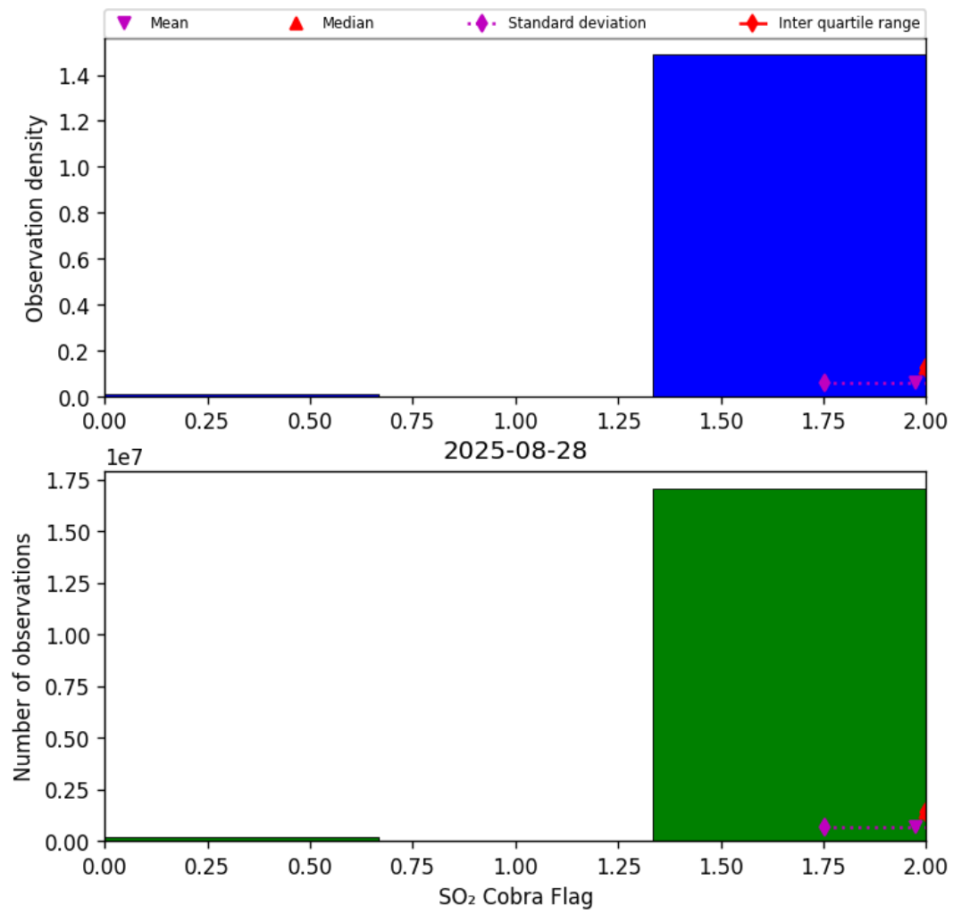
Figure 75: Histogram of “SO 2 Cobra Flag” for 2025-08-28 to 2025-08-28
