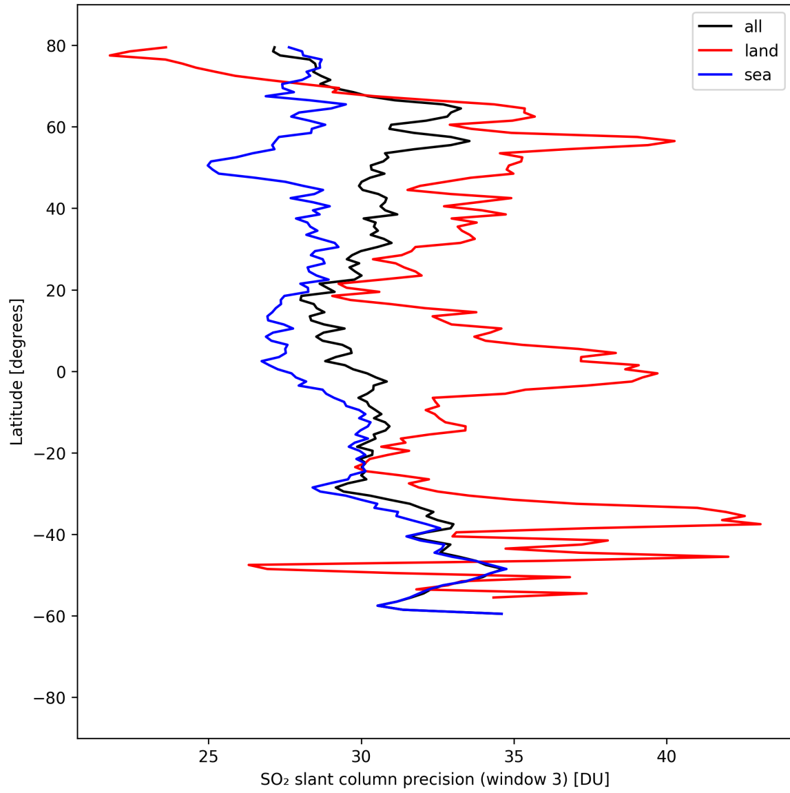
Figure 45: Zonal average of “SO 2 slant column precision (window 3)” for 2025-08-28 to 2025-08-28.
