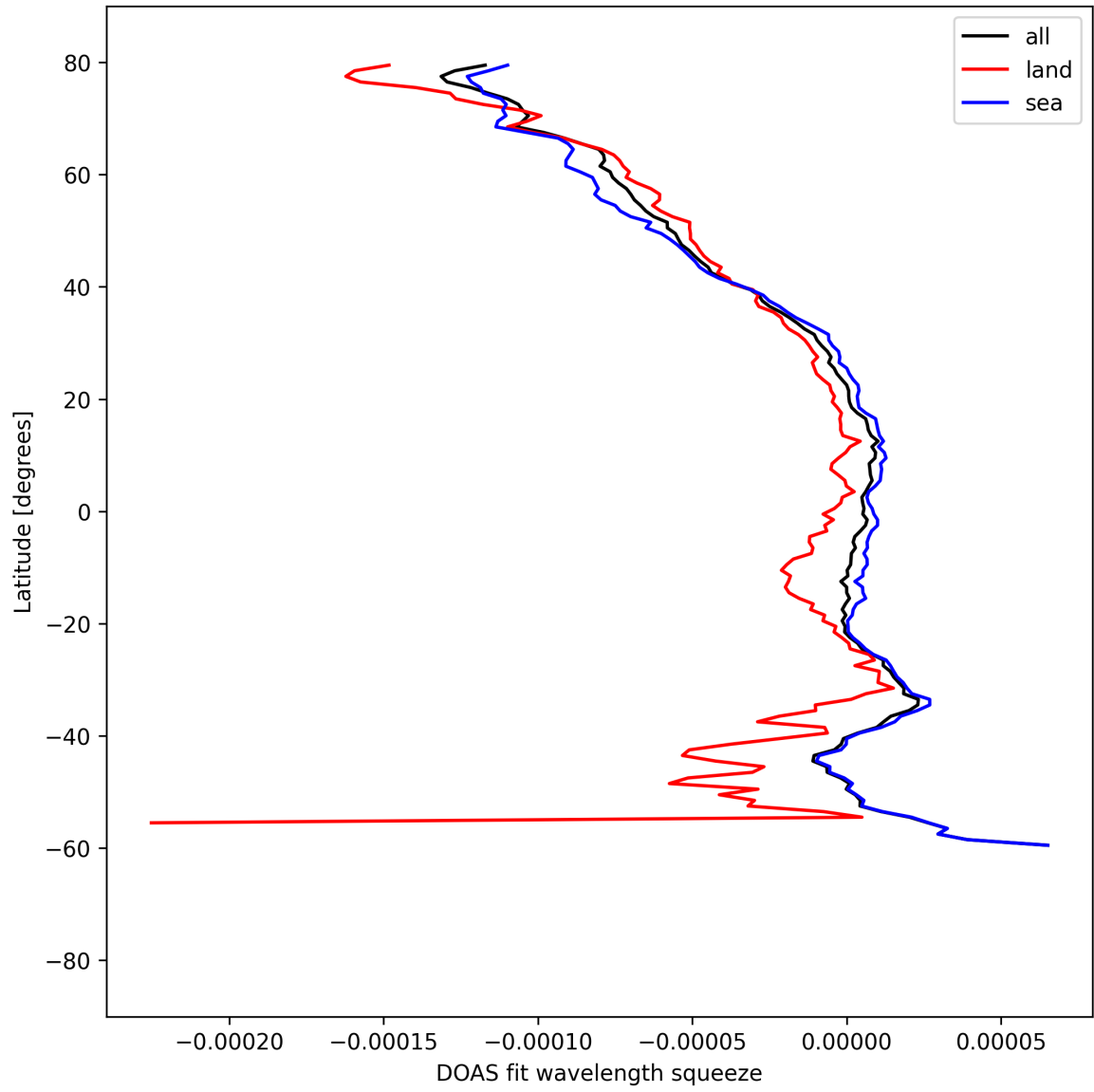
Figure 51: Zonal average of “DOAS fit wavelength squeeze” for 2025-08-28 to 2025-08-28.
