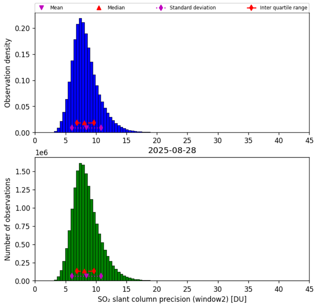
Figure 68: Histogram of “SO 2 slant column precision (window2)” for 2025-08-28 to 2025-08-28
