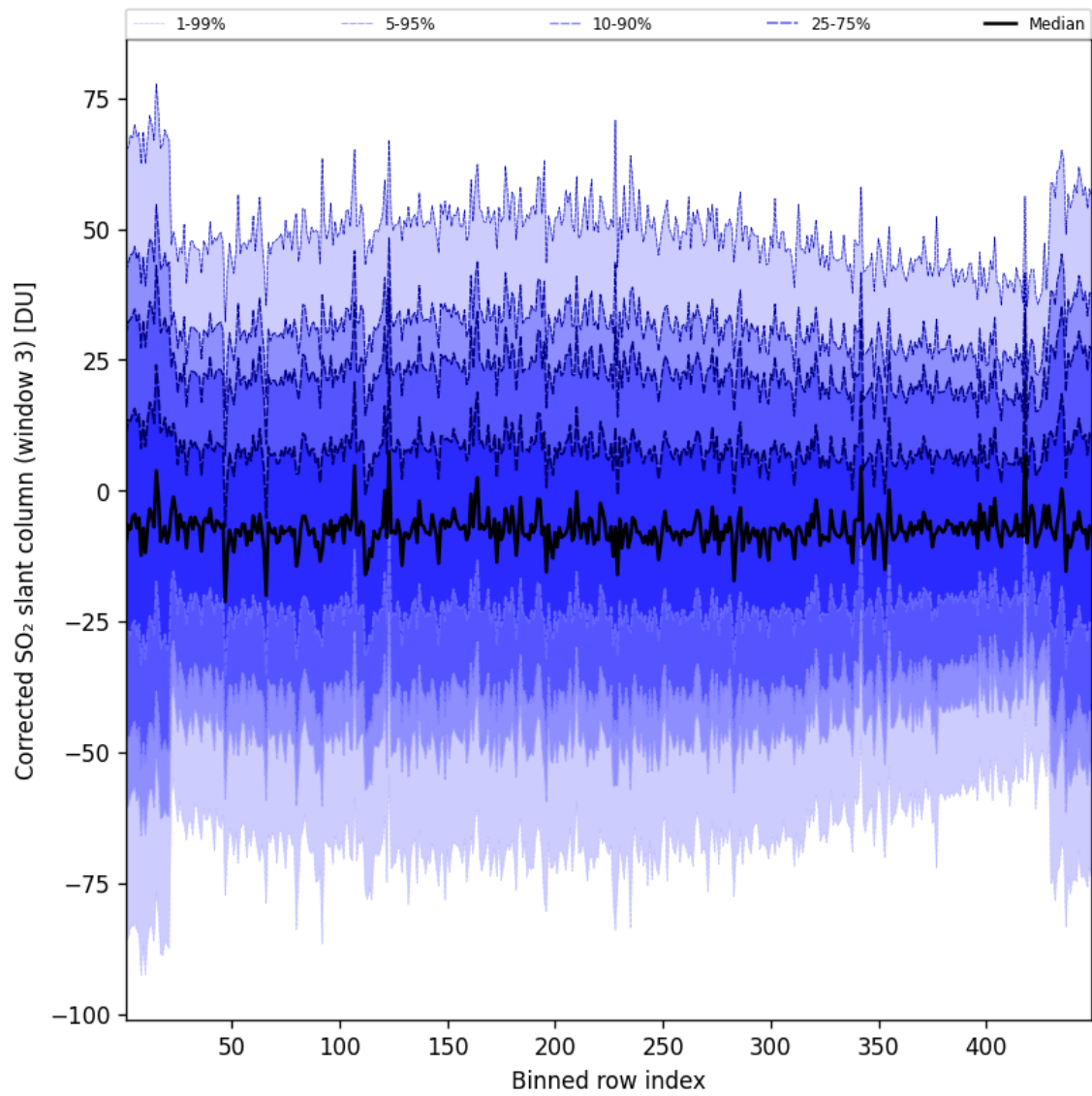
Figure 100: Along track statistics of “Corrected SO 2 slant column (window 3)” for 2025-08-28 to 2025-08-28
