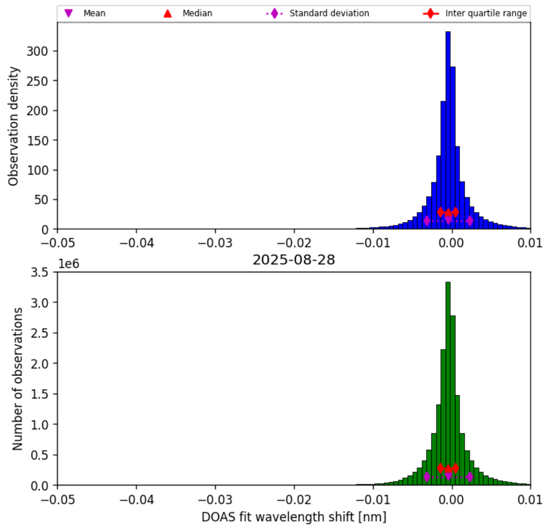
Figure 77: Histogram of “DOAS fit wavelength shift” for 2025-08-28 to 2025-08-28
