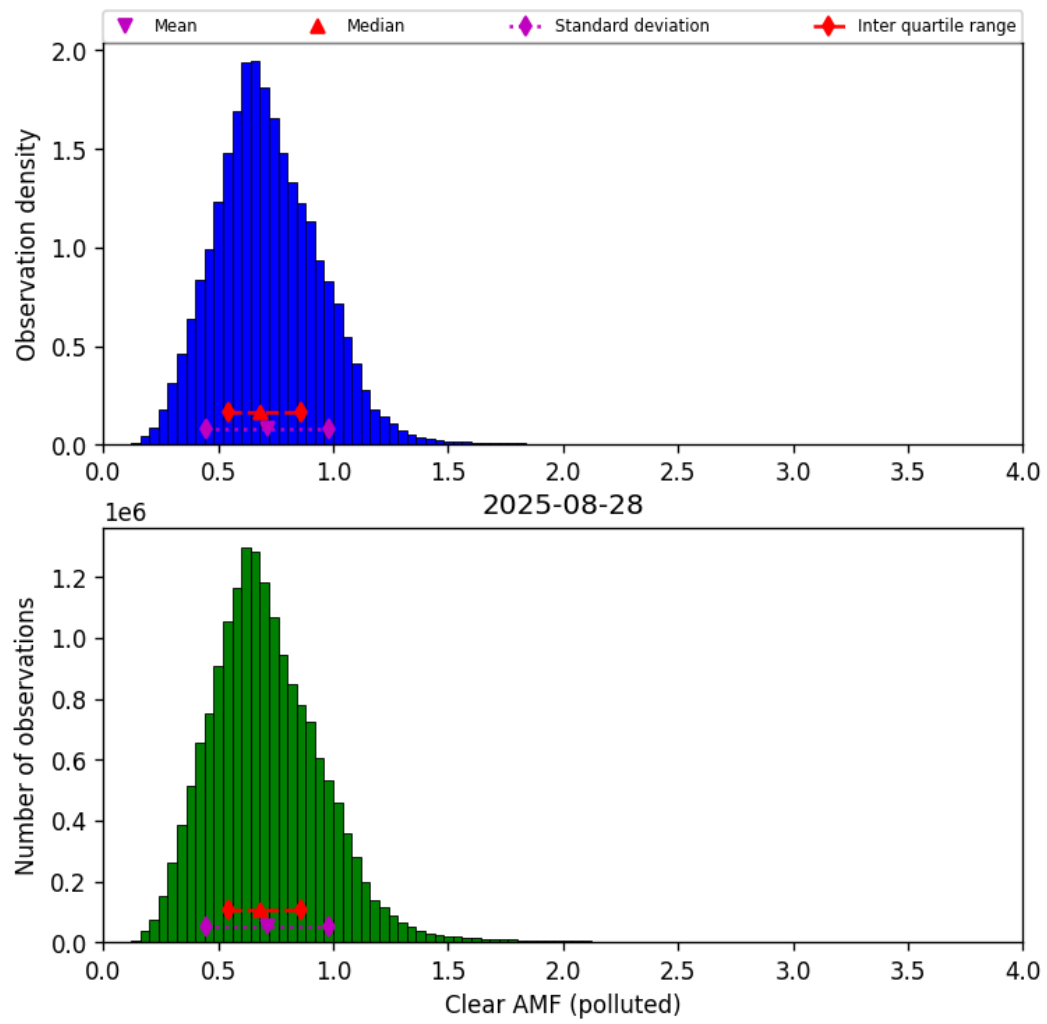
Figure 82: Histogram of “Clear AMF (polluted)” for 2025-08-28 to 2025-08-28
