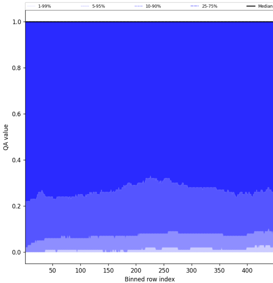
Figure 84: Along track statistics of “QA value” for 2025-08-28 to 2025-08-28
