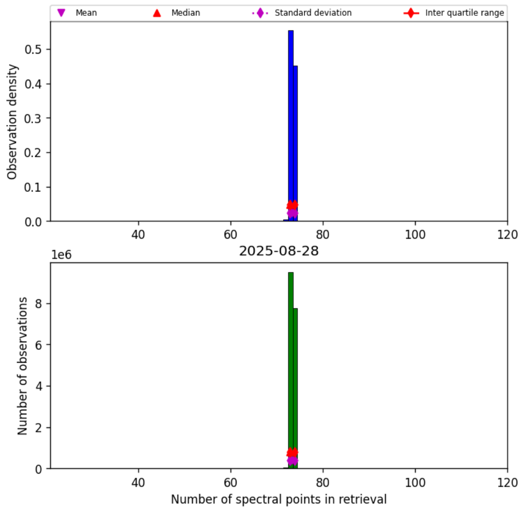
Figure 83: Histogram of “Number of spectral points in retrieval” for 2025-08-28 to 2025-08-28
