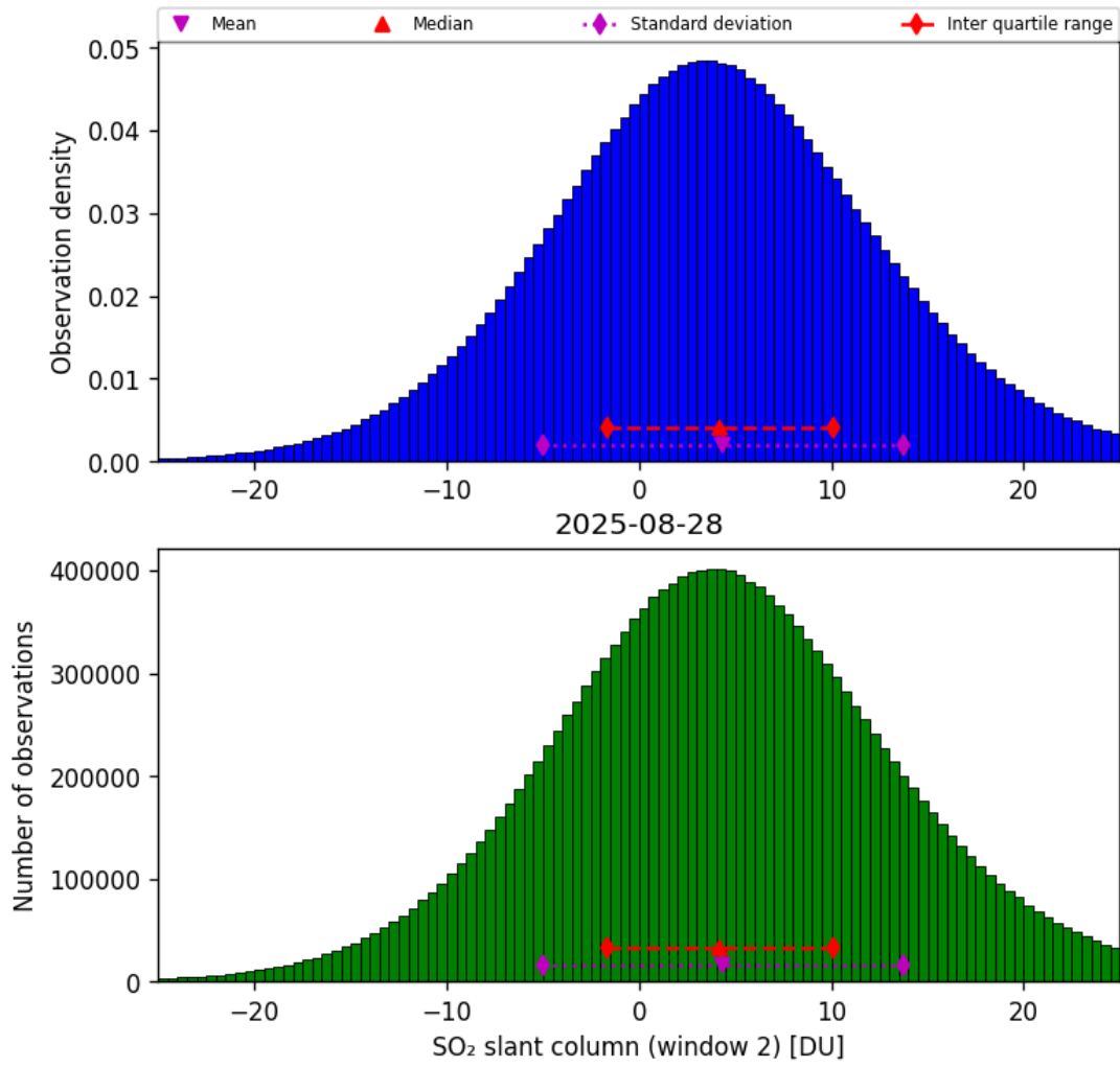
Figure 67: Histogram of “SO 2 slant column (window 2)” for 2025-08-28 to 2025-08-28
