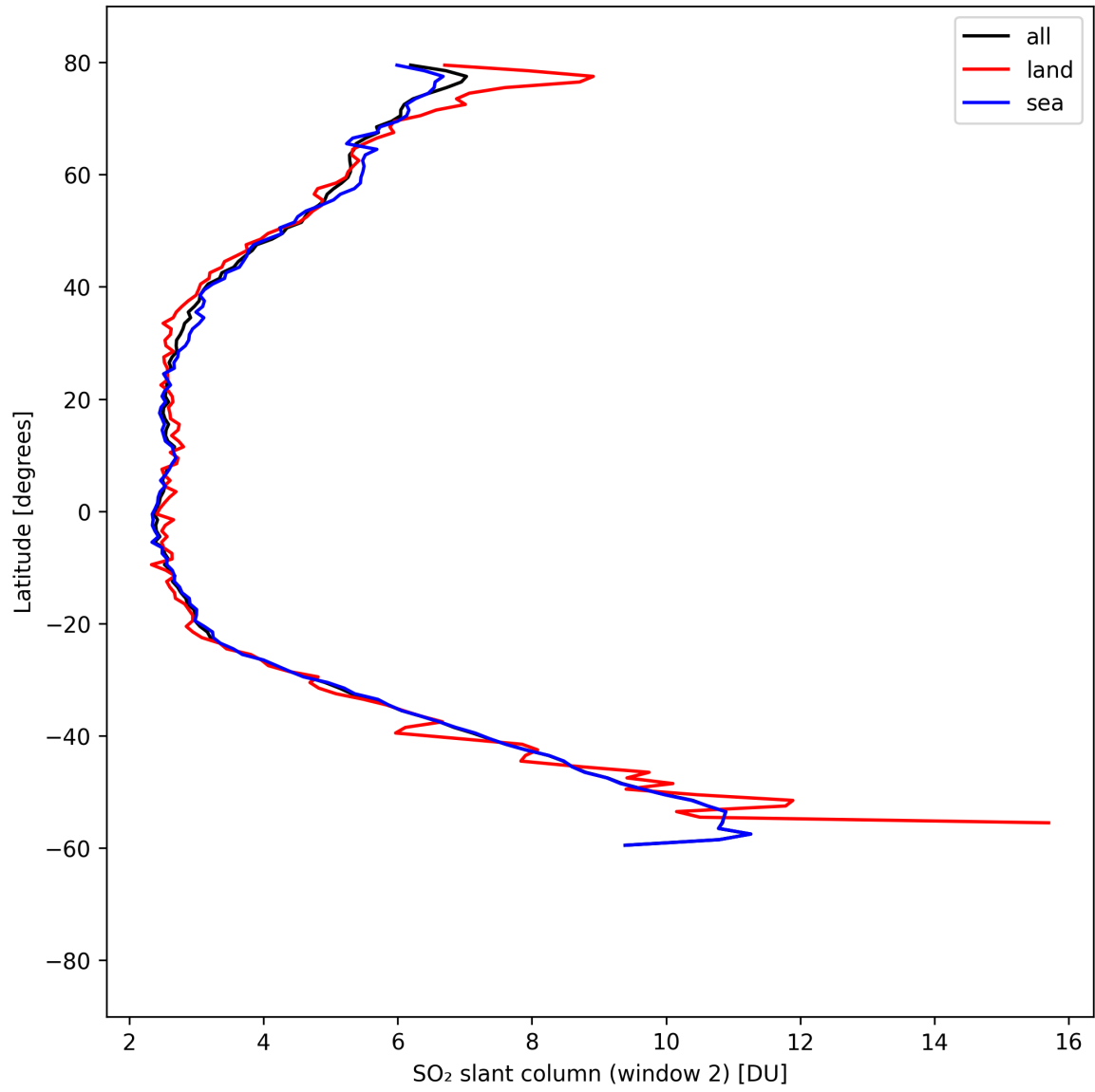
Figure 40: Zonal average of “SO 2 slant column (window 2)” for 2025-08-28 to 2025-08-28.
