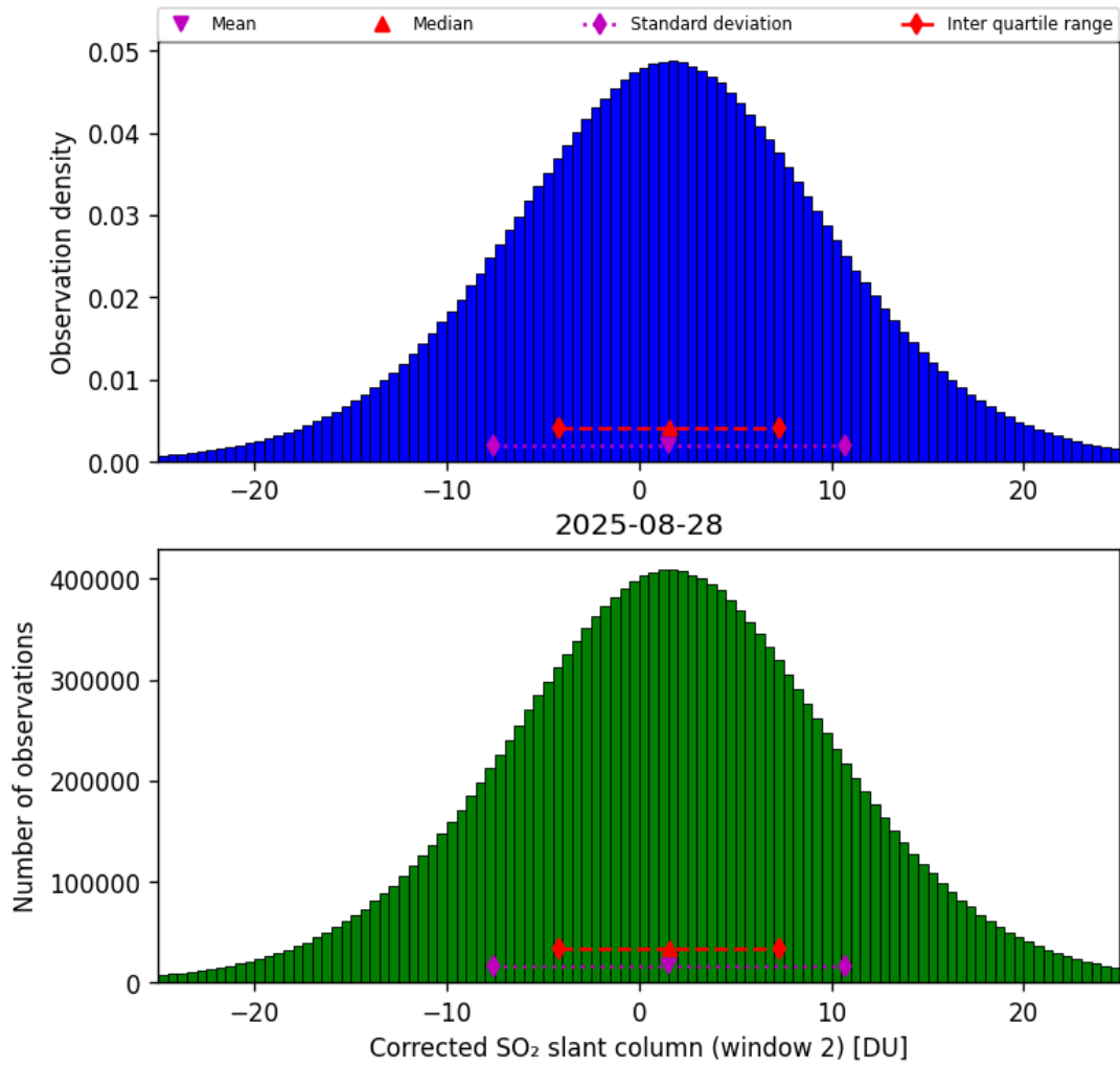
Figure 69: Histogram of “Corrected SO 2 slant column (window 2)” for 2025-08-28 to 2025-08-28
