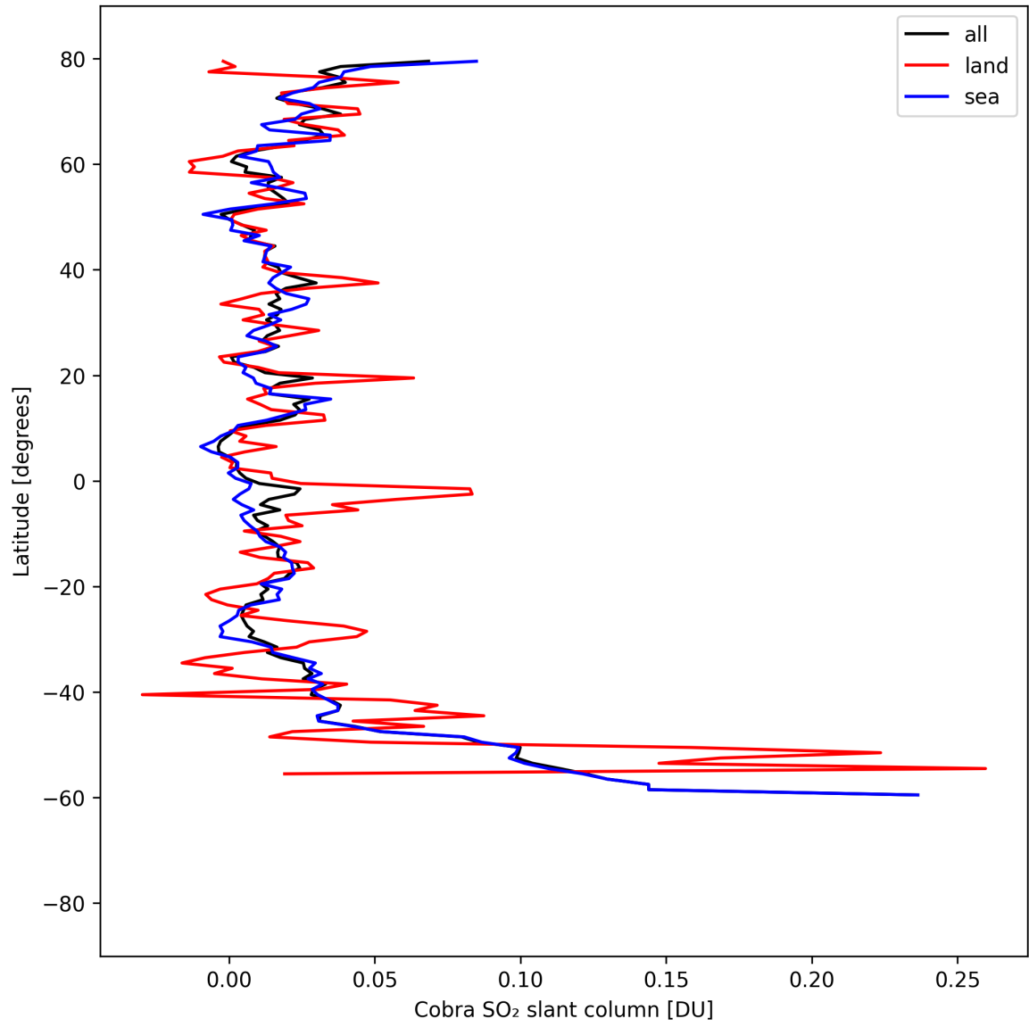
Figure 34: Zonal average of “Cobra SO 2 slant column” for 2025-08-28 to 2025-08-28.
