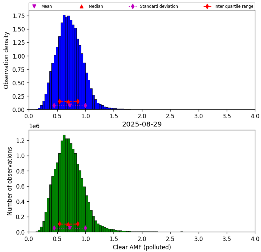
Figure 82: Histogram of "Clear AMF (polluted)" for 2025-08-29 to 2025-08-30
