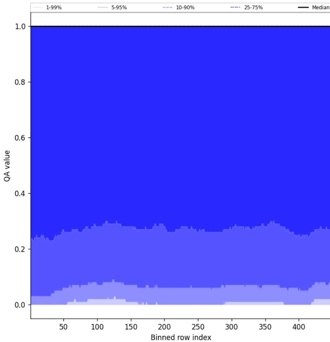
Figure 84: Along track statistics of “QA value” for 2025-08-29 to 2025-08-30
