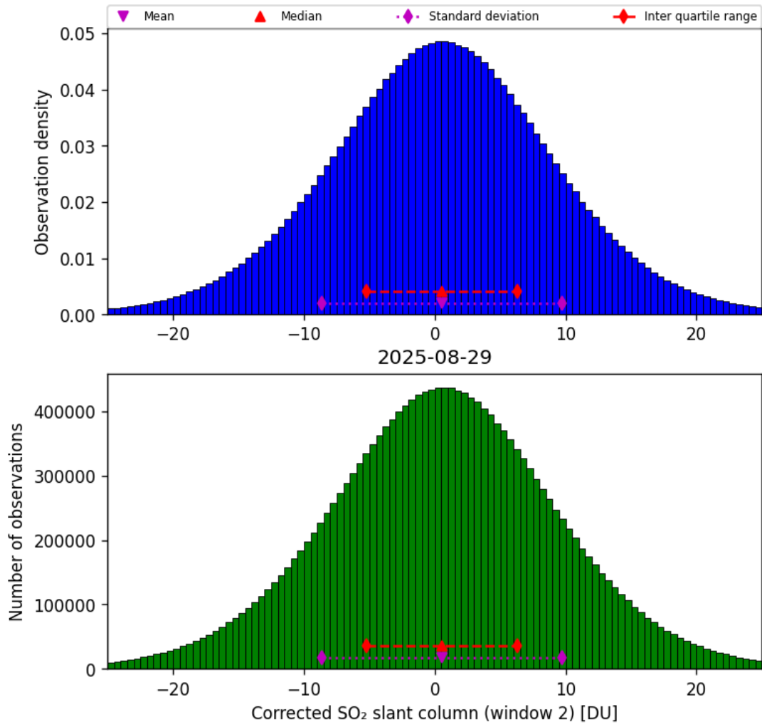
Figure 69: Histogram of “Corrected SO 2 slant column (window 2)” for 2025-08-29 to 2025-08-30
