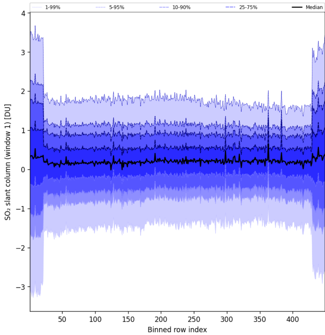
Figure 90: Along track statistics of “SO 2 slant column (window 1)” for 2025-08-29 to 2025-08-30
