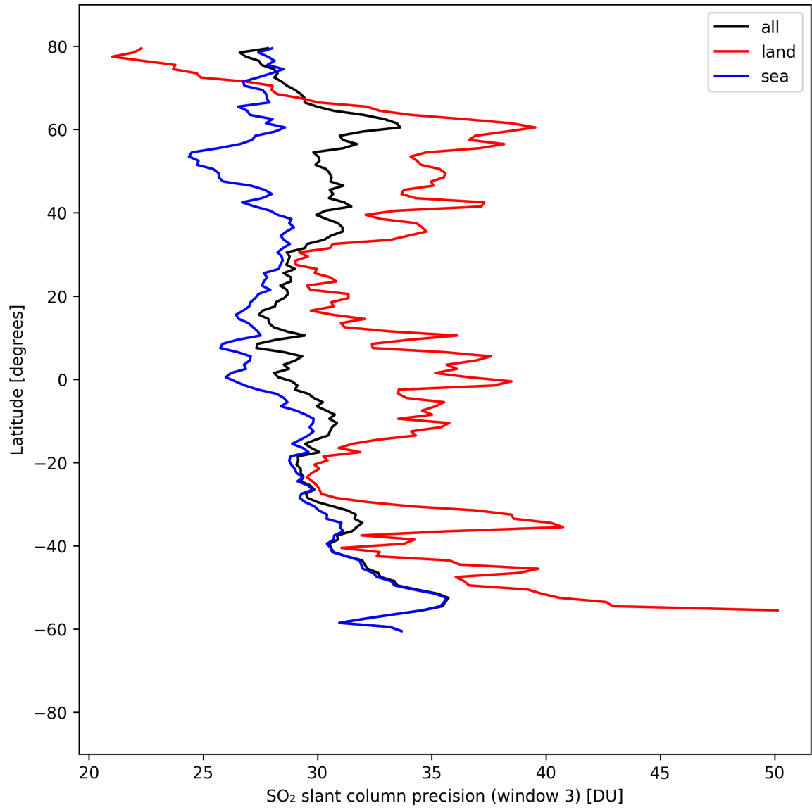
Figure 45: Zonal average of “SO 2 slant column precision (window 3)” for 2025-08-29 to 2025-08-30.
