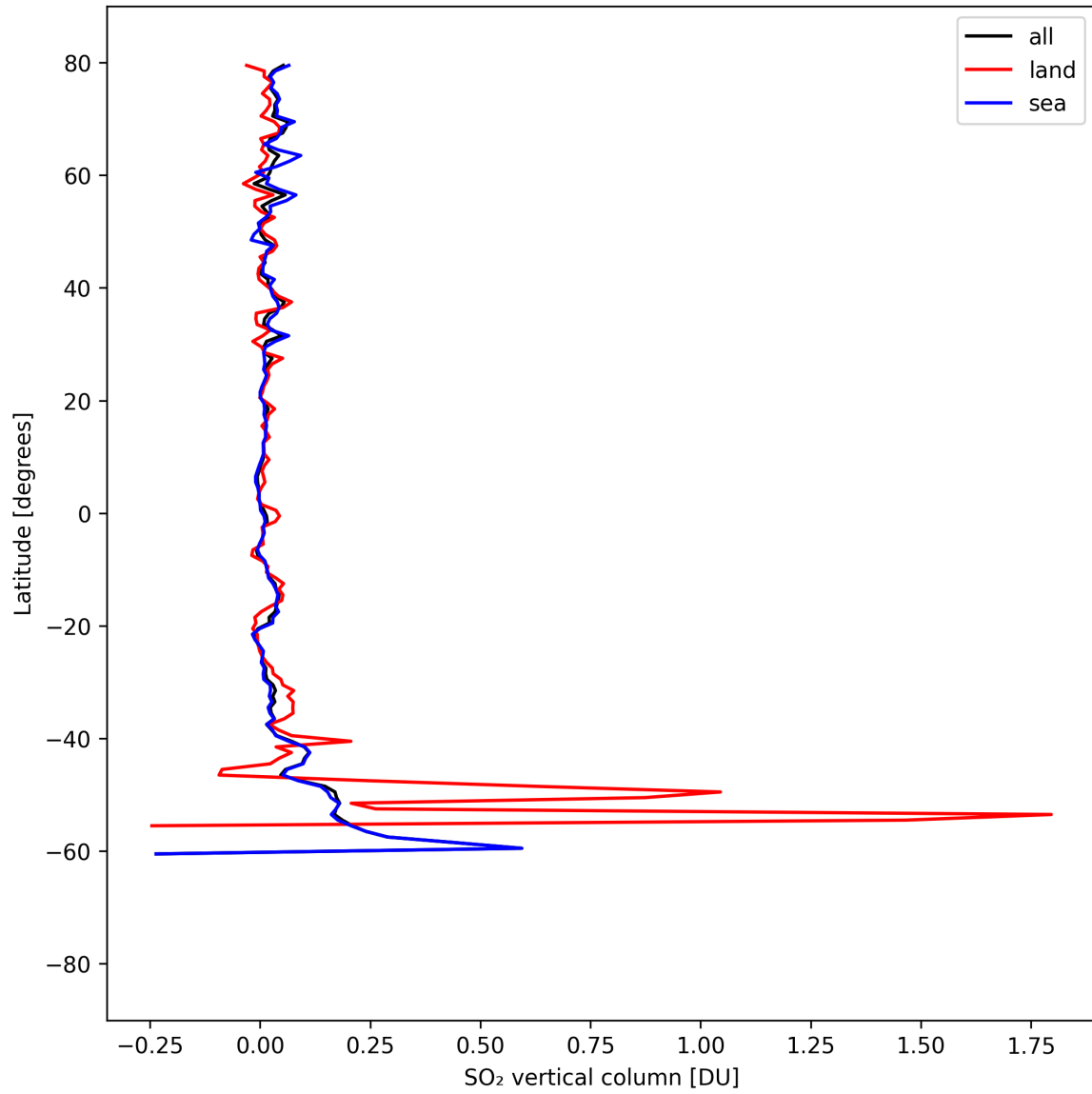
Figure 31: Zonal average of “SO 2 vertical column” for 2025-08-29 to 2025-08-30.
