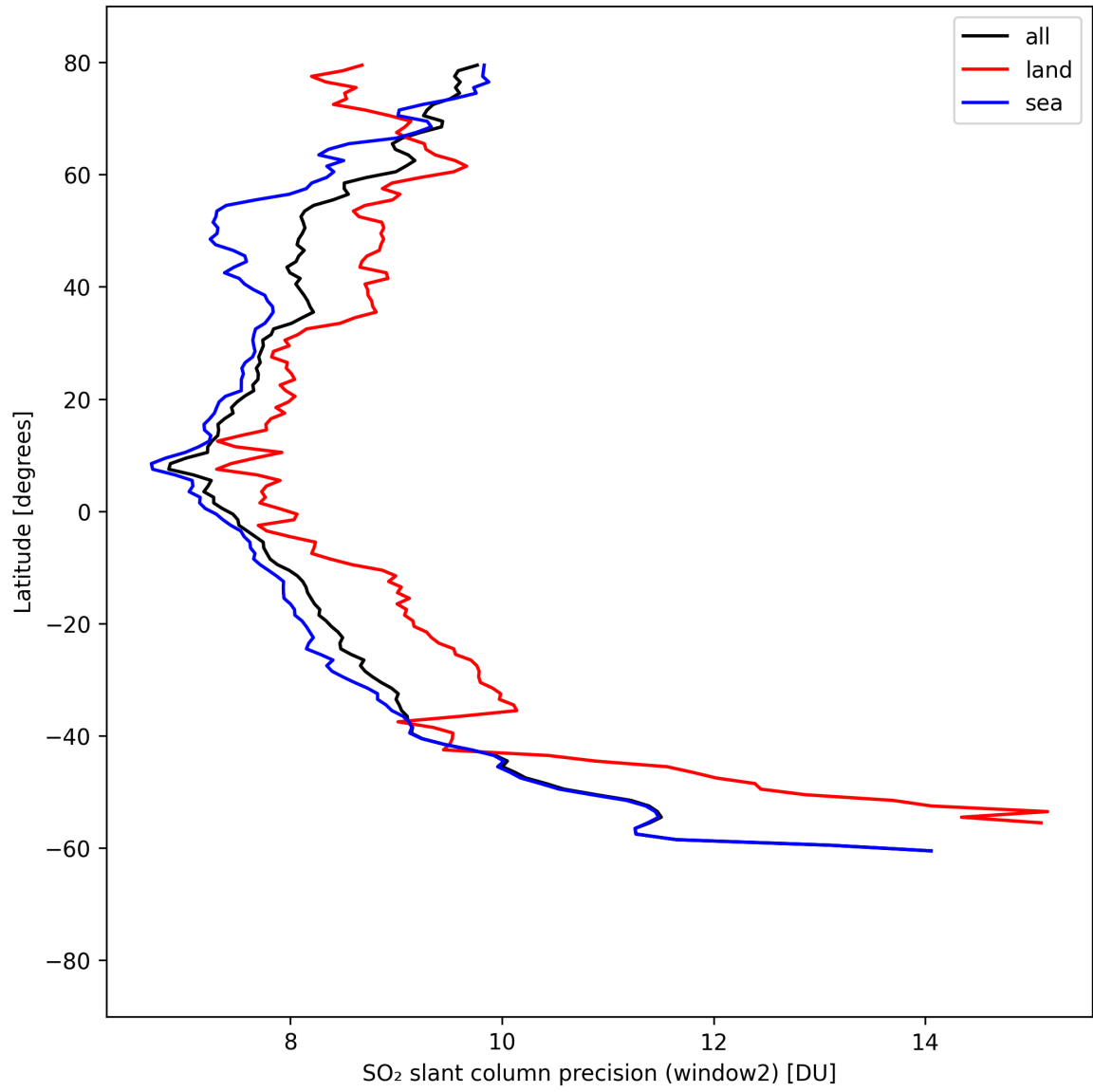
Figure 41: Zonal average of “SO 2 slant column precision (window2)” for 2025-08-29 to 2025-08-30.
