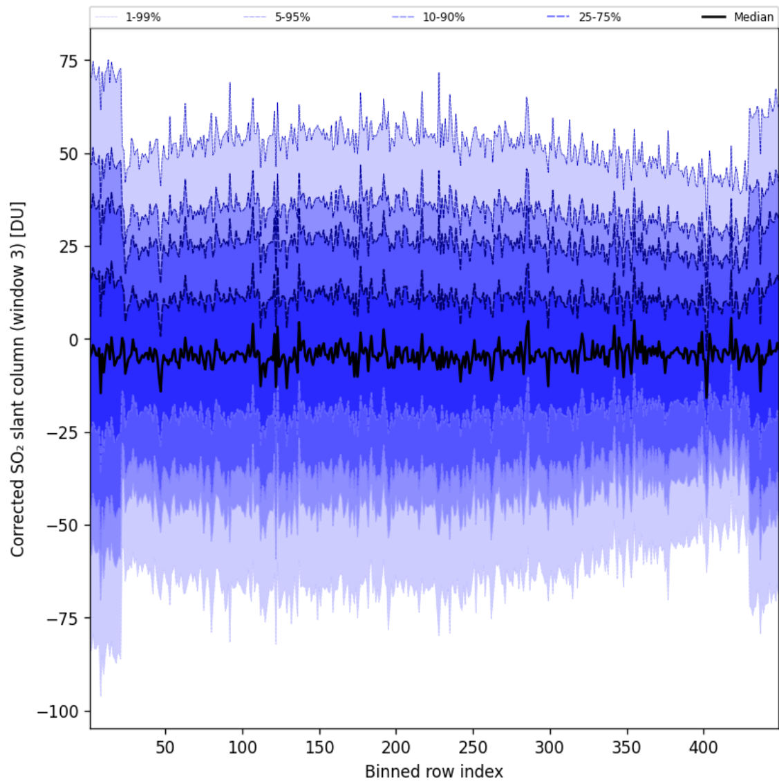
Figure 100: Along track statistics of “Corrected SO 2 slant column (window 3)” for 2025-08-29 to 2025-08-30
