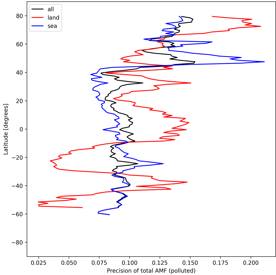
Figure 54: Zonal average of “Precision of total AMF (polluted)” for 2025-08-29 to 2025-08-30.
