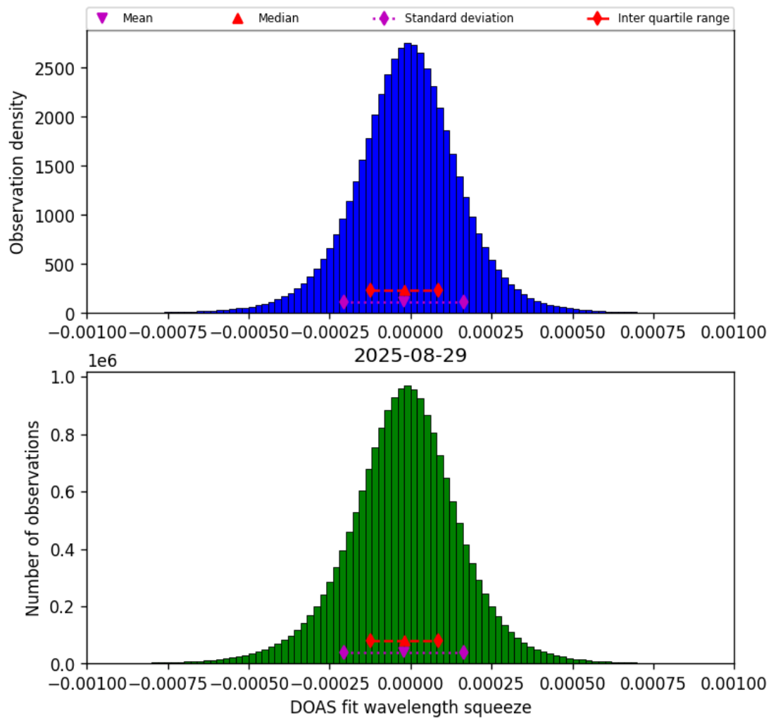
Figure 78: Histogram of “DOAS fit wavelength squeeze” for 2025-08-29 to 2025-08-30
