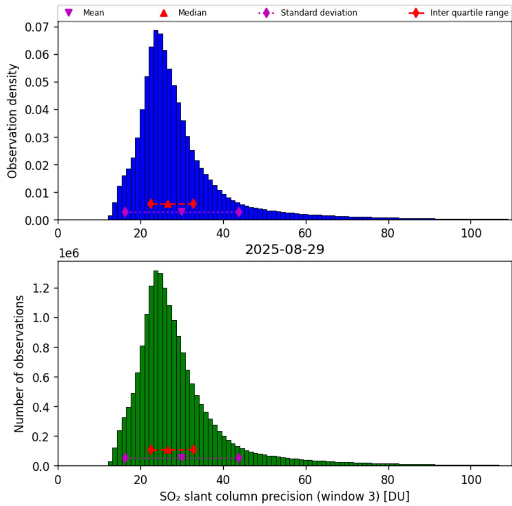
Figure 72: Histogram of “SO 2 slant column precision (window 3)” for 2025-08-29 to 2025-08-30
