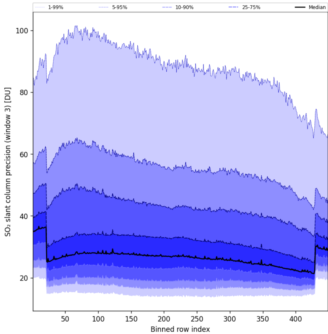
Figure 99: Along track statistics of “SO 2 slant column precision (window 3)” for 2025-08-29 to 2025-08-30
