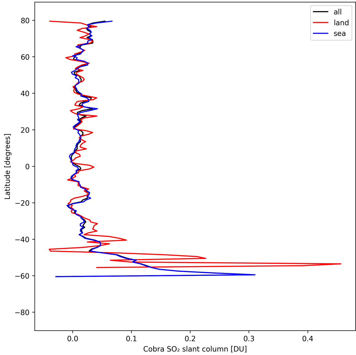
Figure 34: Zonal average of “Cobra SO 2 slant column” for 2025-08-29 to 2025-08-30.
