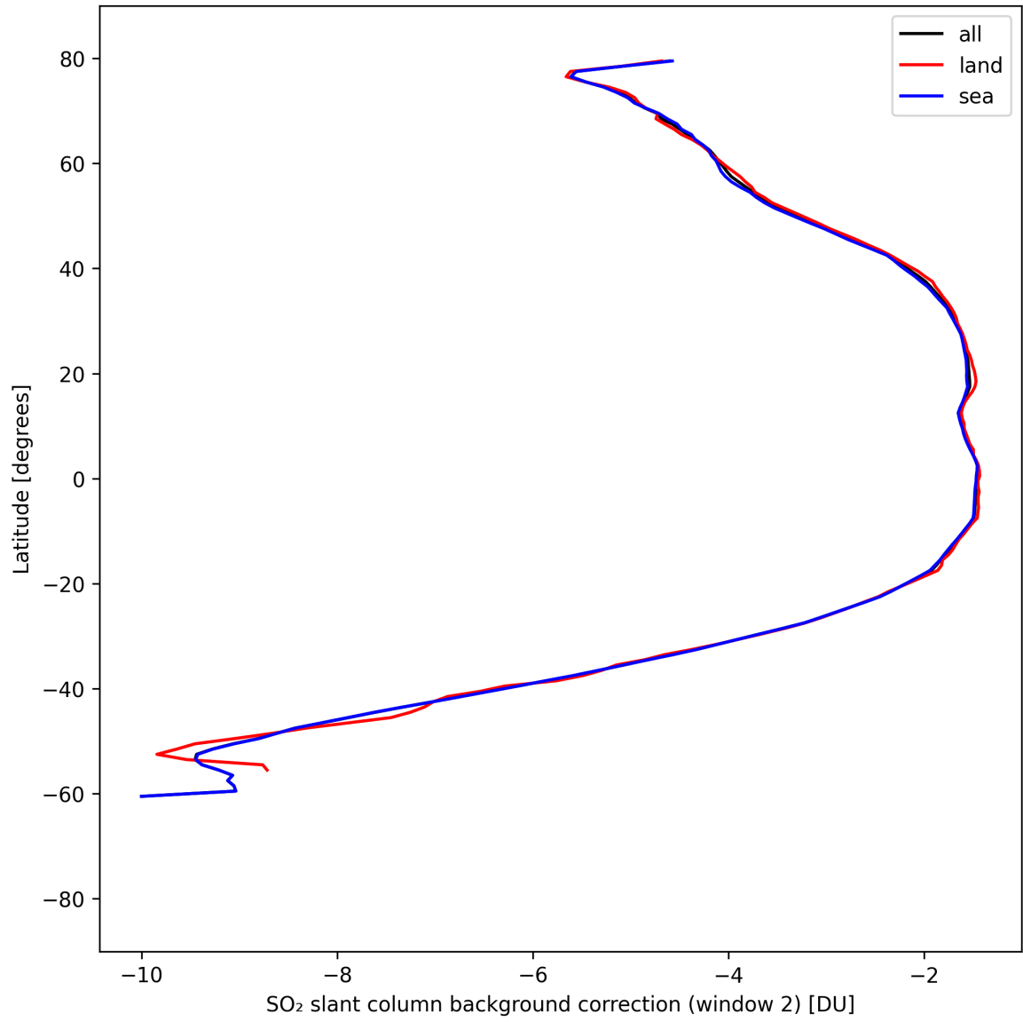
Figure 43: Zonal average of “SO 2 slant column background correction (window 2)” for 2025-08-29 to 2025-08-30.
