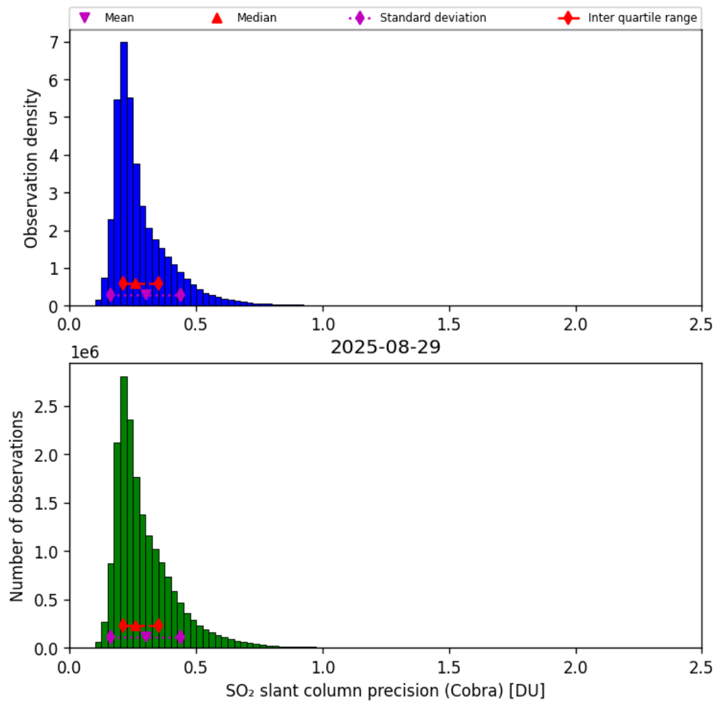
Figure 62: Histogram of “SO 2 slant column precision (Cobra)” for 2025-08-29 to 2025-08-30
