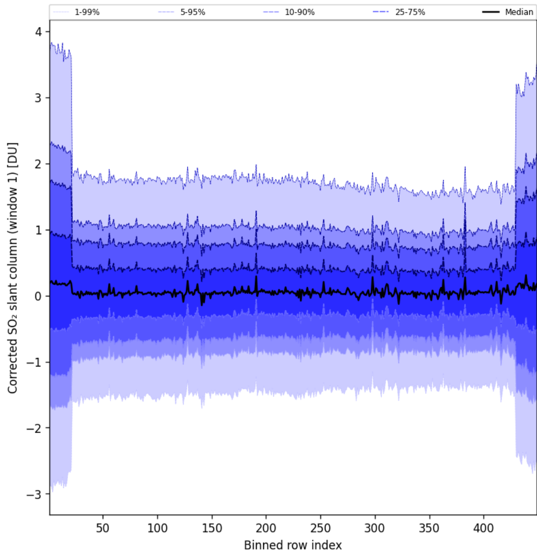
Figure 92: Along track statistics of “Corrected SO 2 slant column (window 1)” for 2025-08-29 to 2025-08-30
