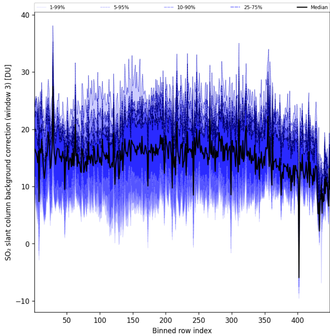
Figure 101: Along track statistics of “SO 2 slant column background correction (window 3)” for 2025-08-29 to 2025-08-30
