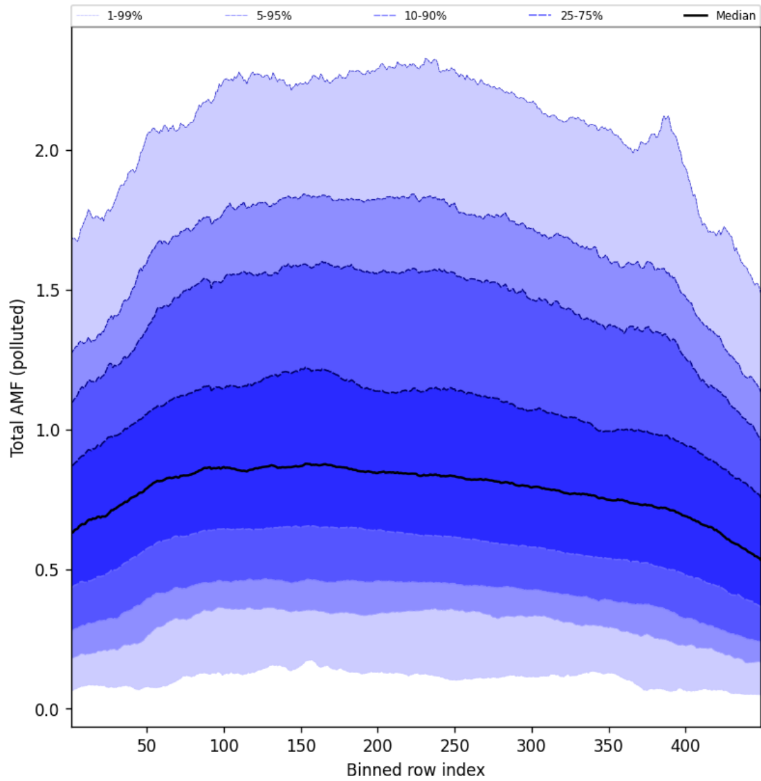
Figure 107: Along track statistics of “Total AMF (polluted)” for 2025-08-29 to 2025-08-30
