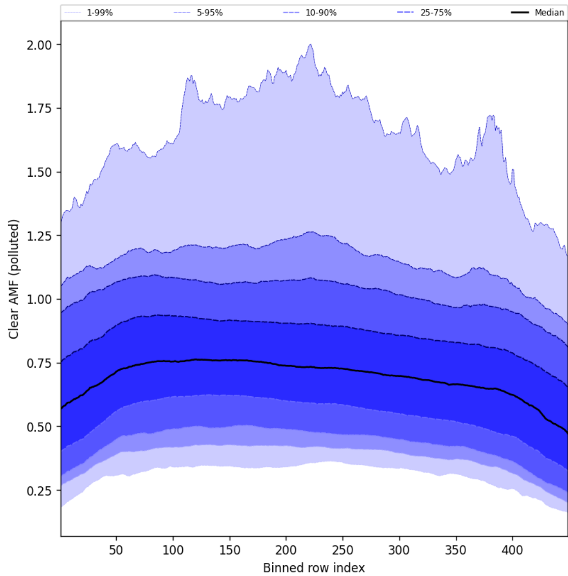
Figure 109: Along track statistics of “Clear AMF (polluted)” for 2025-08-29 to 2025-08-30
