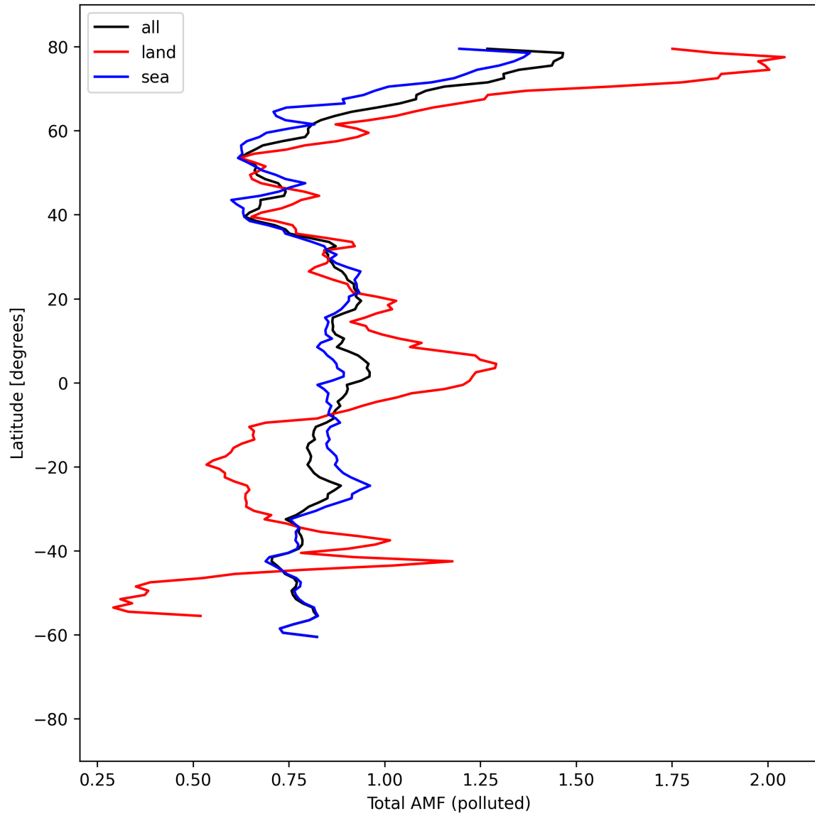
Figure 53: Zonal average of “Total AMF (polluted)” for 2025-08-29 to 2025-08-30.
