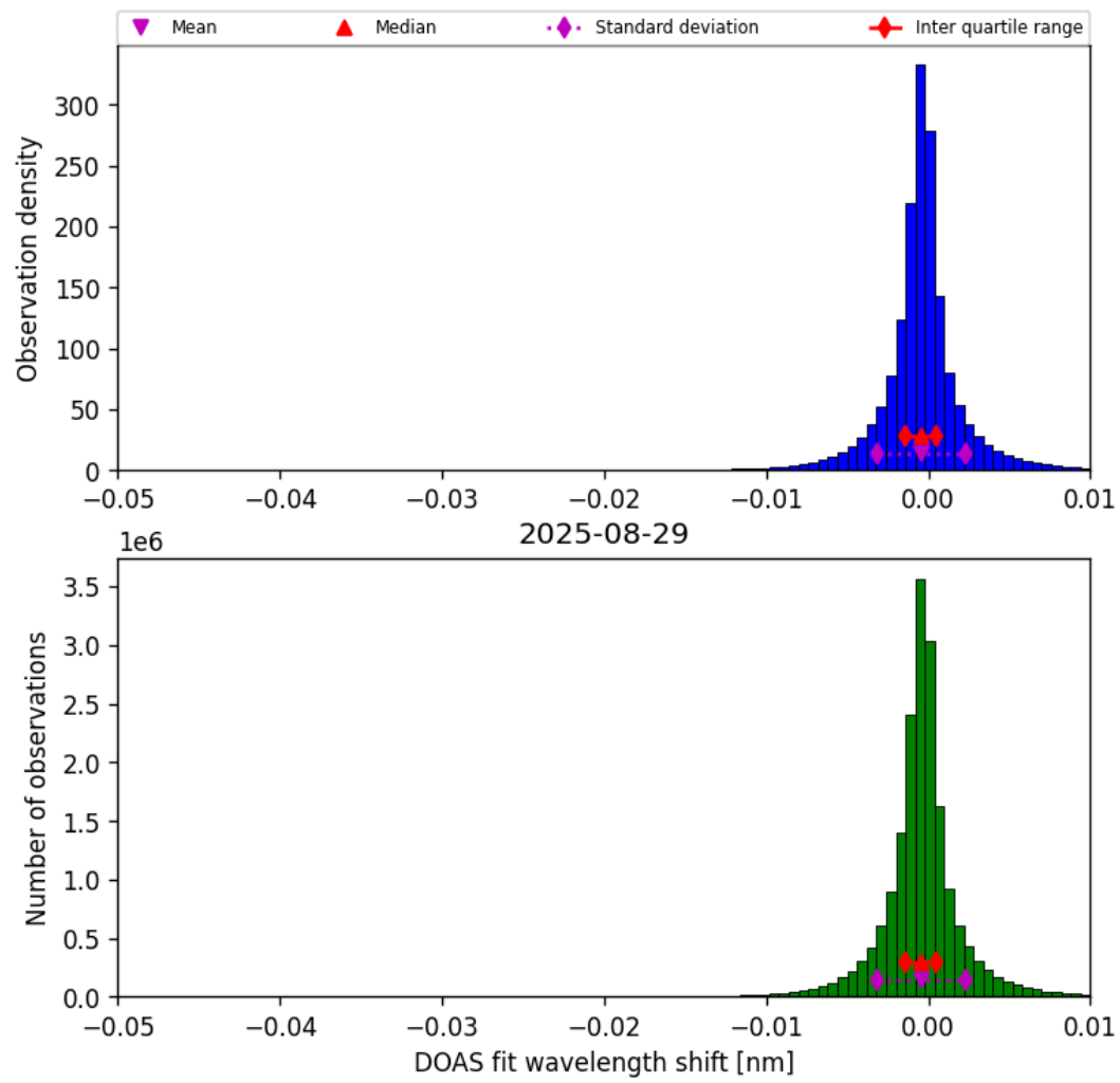
Figure 77: Histogram of “DOAS fit wavelength shift” for 2025-08-29 to 2025-08-30
