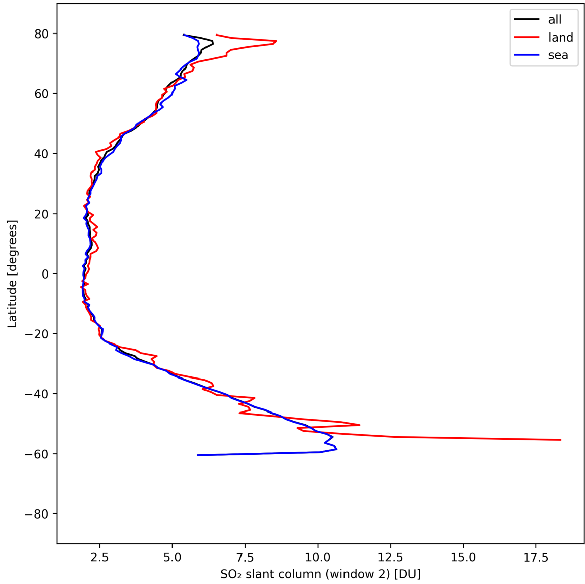
Figure 40: Zonal average of “SO 2 slant column (window 2)” for 2025-08-29 to 2025-08-30.
