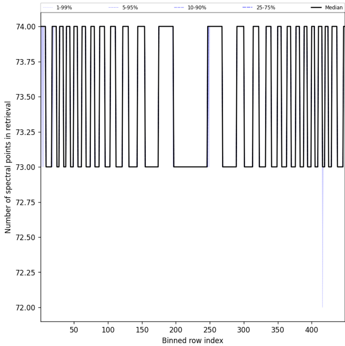
Figure 110: Along track statistics of “Number of spectral points in retrieval” for 2025-08-29 to 2025-08-30
