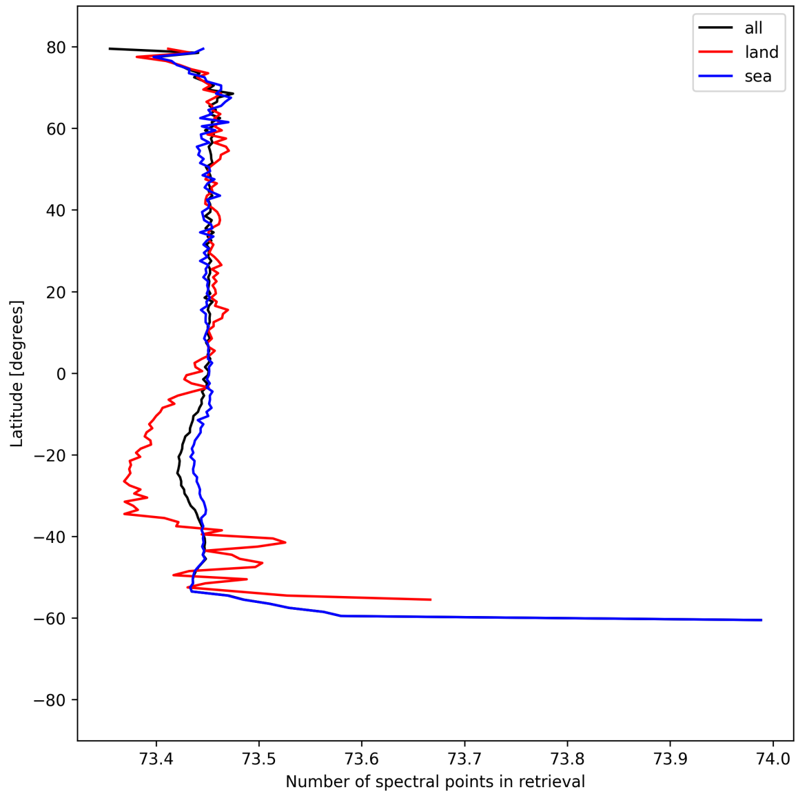
Figure 56: Zonal average of “Number of spectral points in retrieval” for 2025-08-29 to 2025-08-30.
