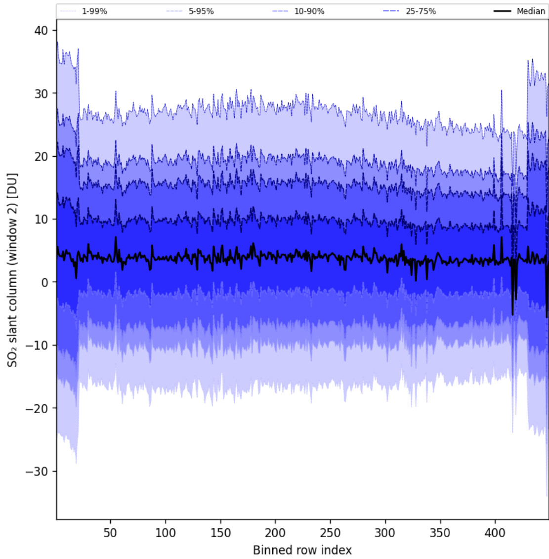
Figure 94: Along track statistics of “SO 2 slant column (window 2)” for 2025-08-29 to 2025-08-30
