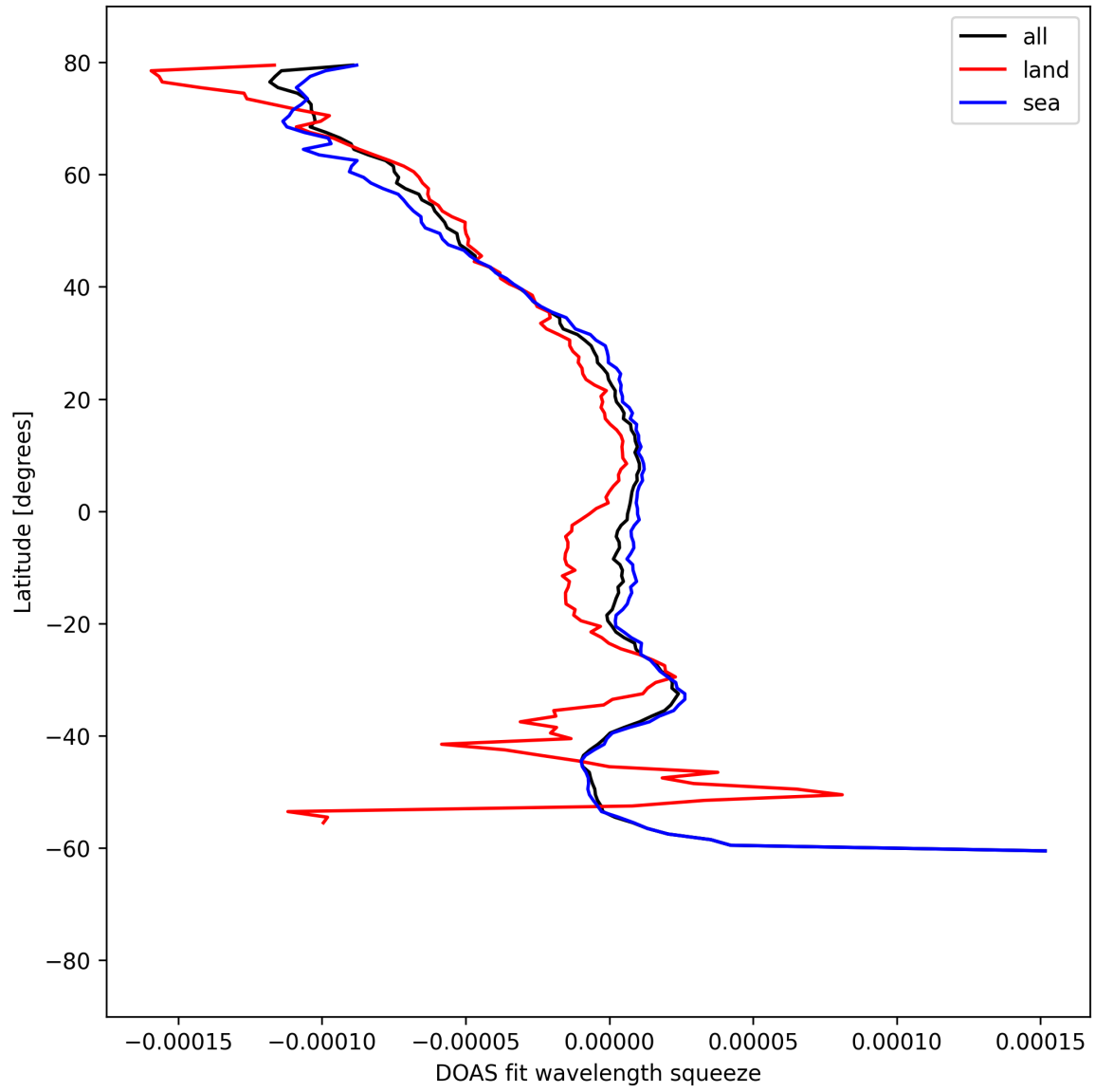
Figure 51: Zonal average of "DOAS fit wavelength squeeze" for 2025-08-29 to 2025-08-30.
