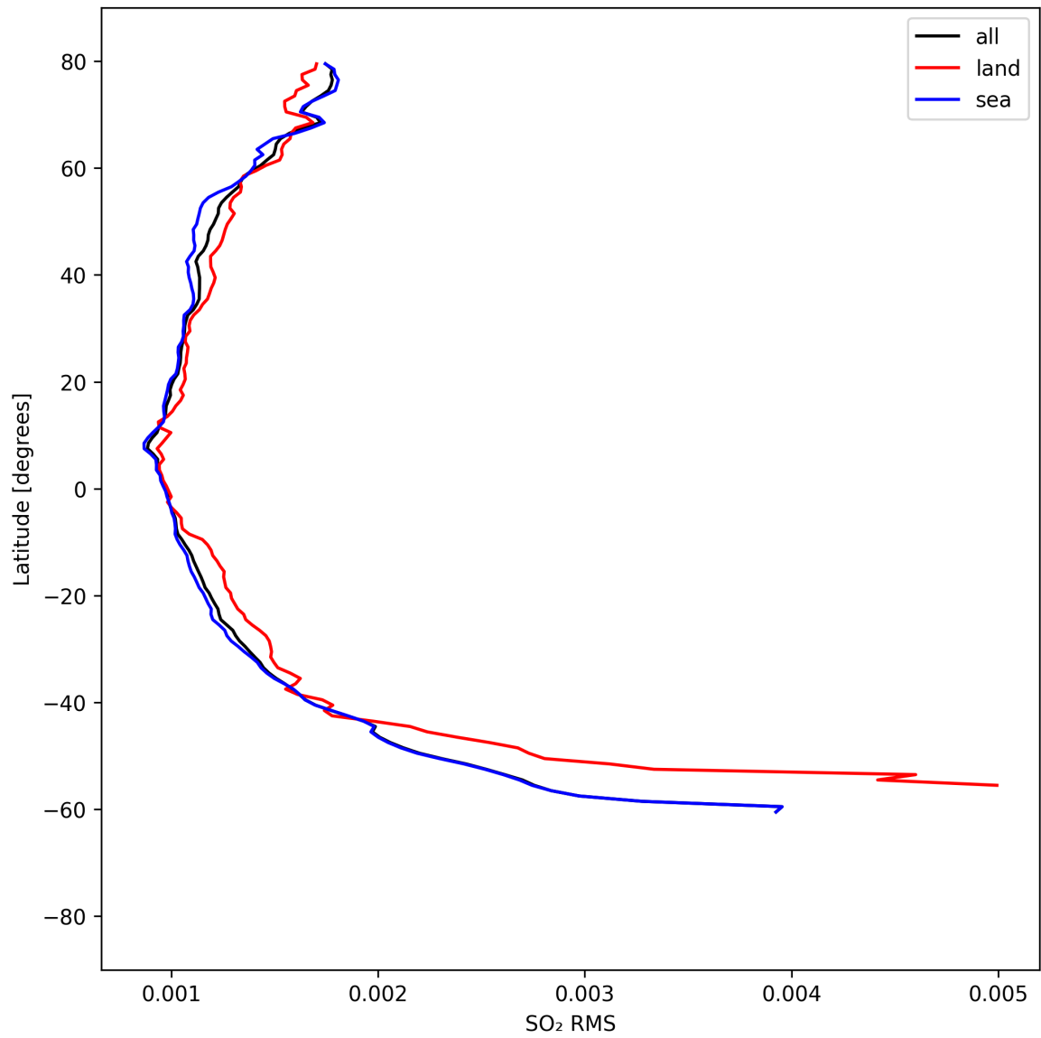
Figure 52: Zonal average of “SO 2 RMS” for 2025-08-29 to 2025-08-30.
