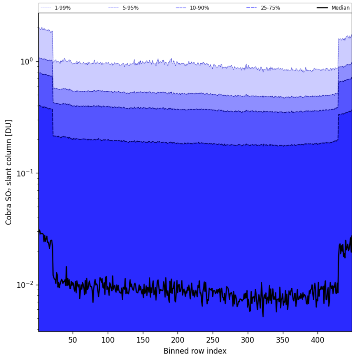
Figure 88: Along track statistics of “Cobra SO 2 slant column” for 2025-08-29 to 2025-08-30
