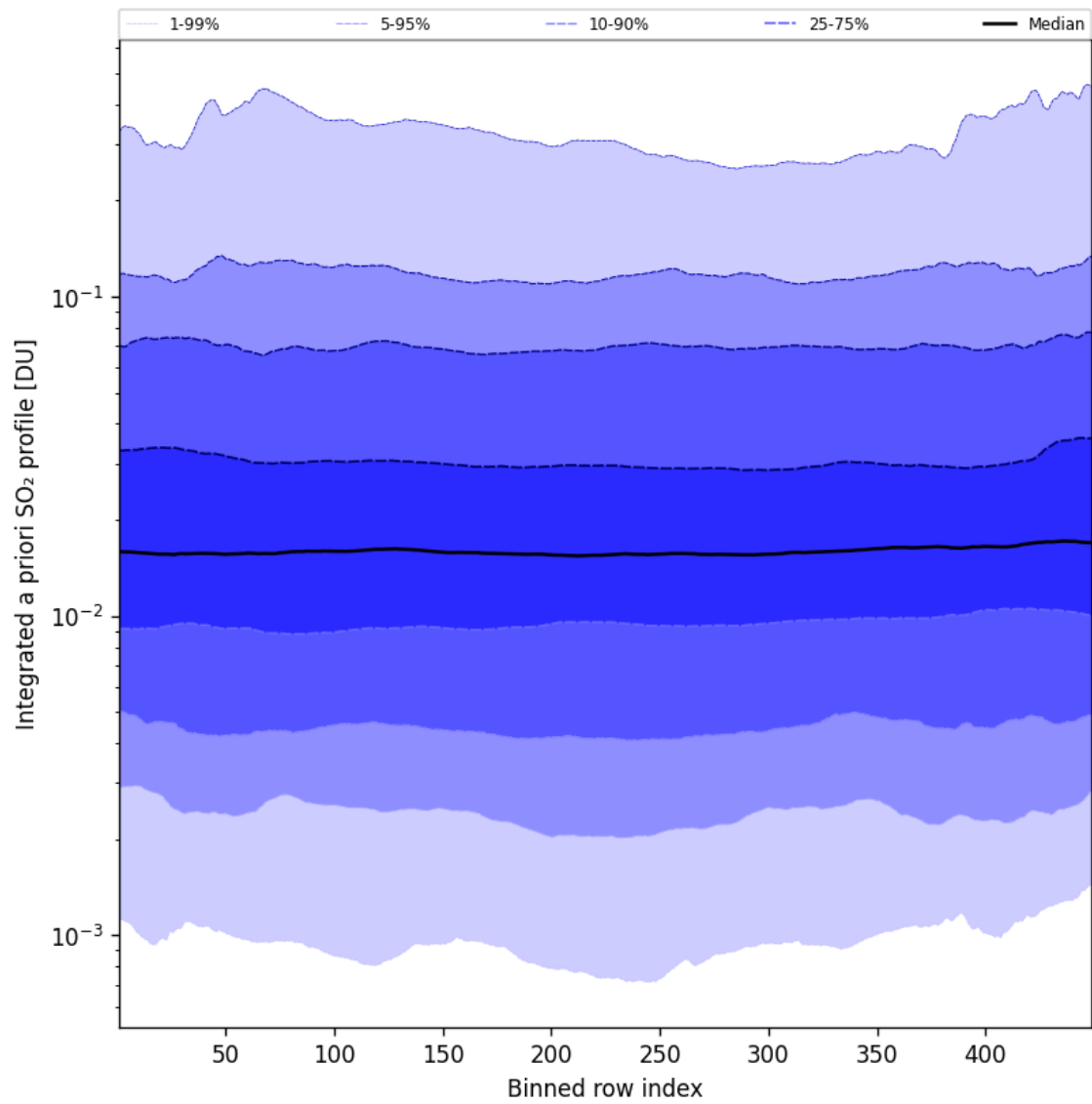
Figure 103: Along track statistics of “Integrated a priori SO 2 profile” for 2025-08-29 to 2025-08-30
