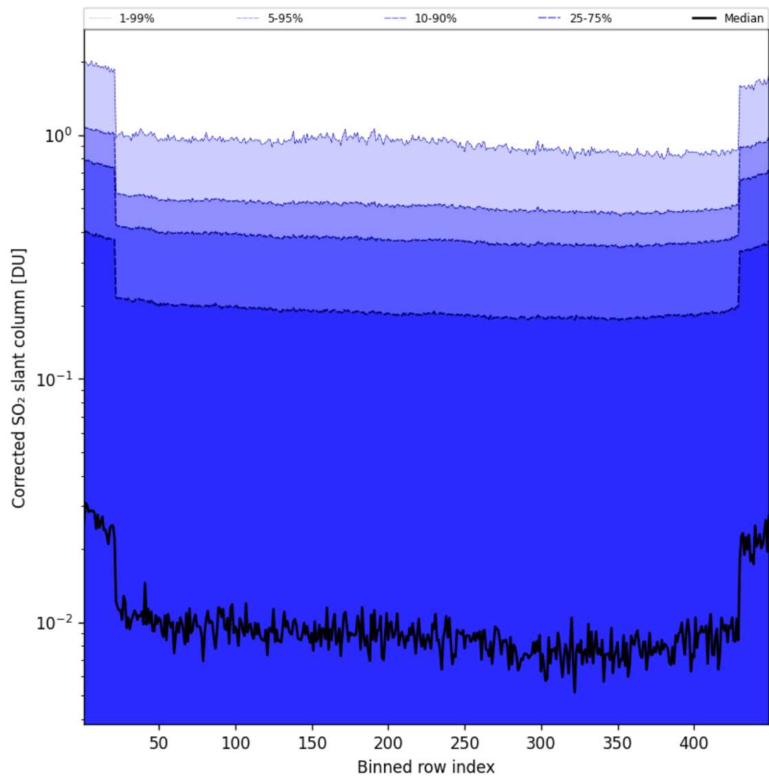
Figure 87: Along track statistics of "Corrected SO 2 slant column" for 2025-08-29 to 2025-08-30
