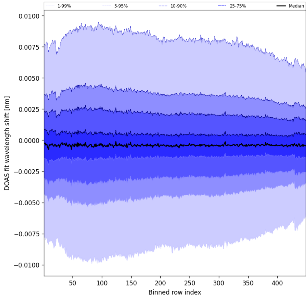
Figure 104: Along track statistics of “DOAS fit wavelength shift” for 2025-08-29 to 2025-08-30
