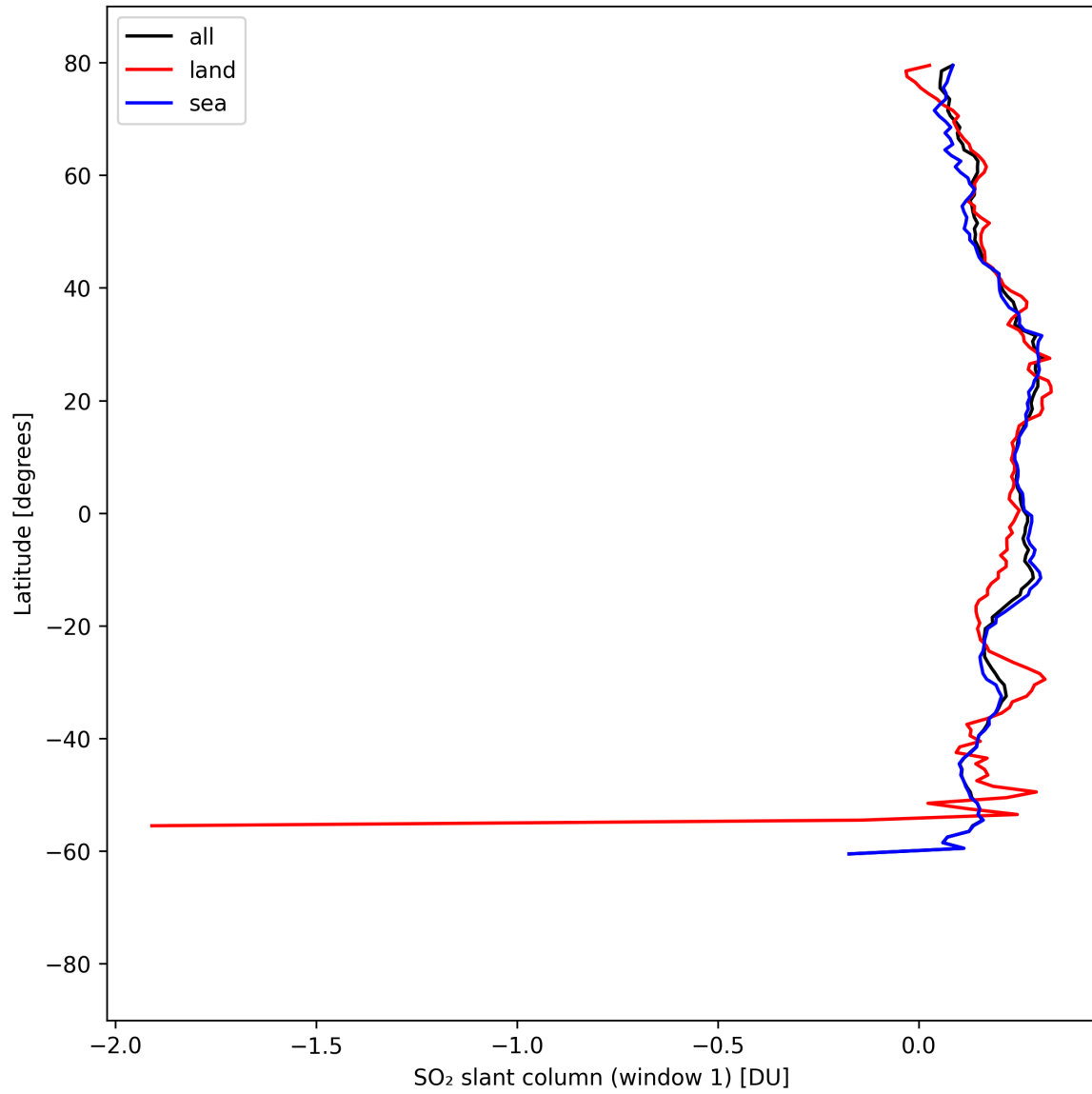
Figure 36: Zonal average of “SO 2 slant column (window 1)” for 2025-08-29 to 2025-08-30.
