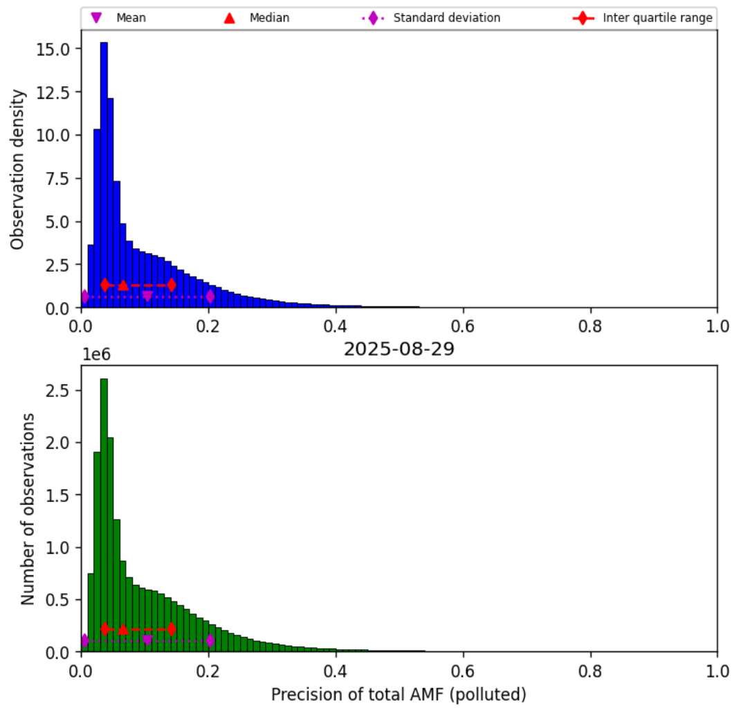
Figure 81: Histogram of “Precision of total AMF (polluted)” for 2025-08-29 to 2025-08-30
