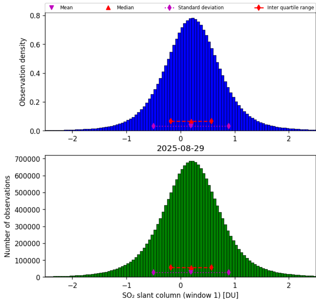
Figure 63: Histogram of “SO 2 slant column (window 1)” for 2025-08-29 to 2025-08-30
