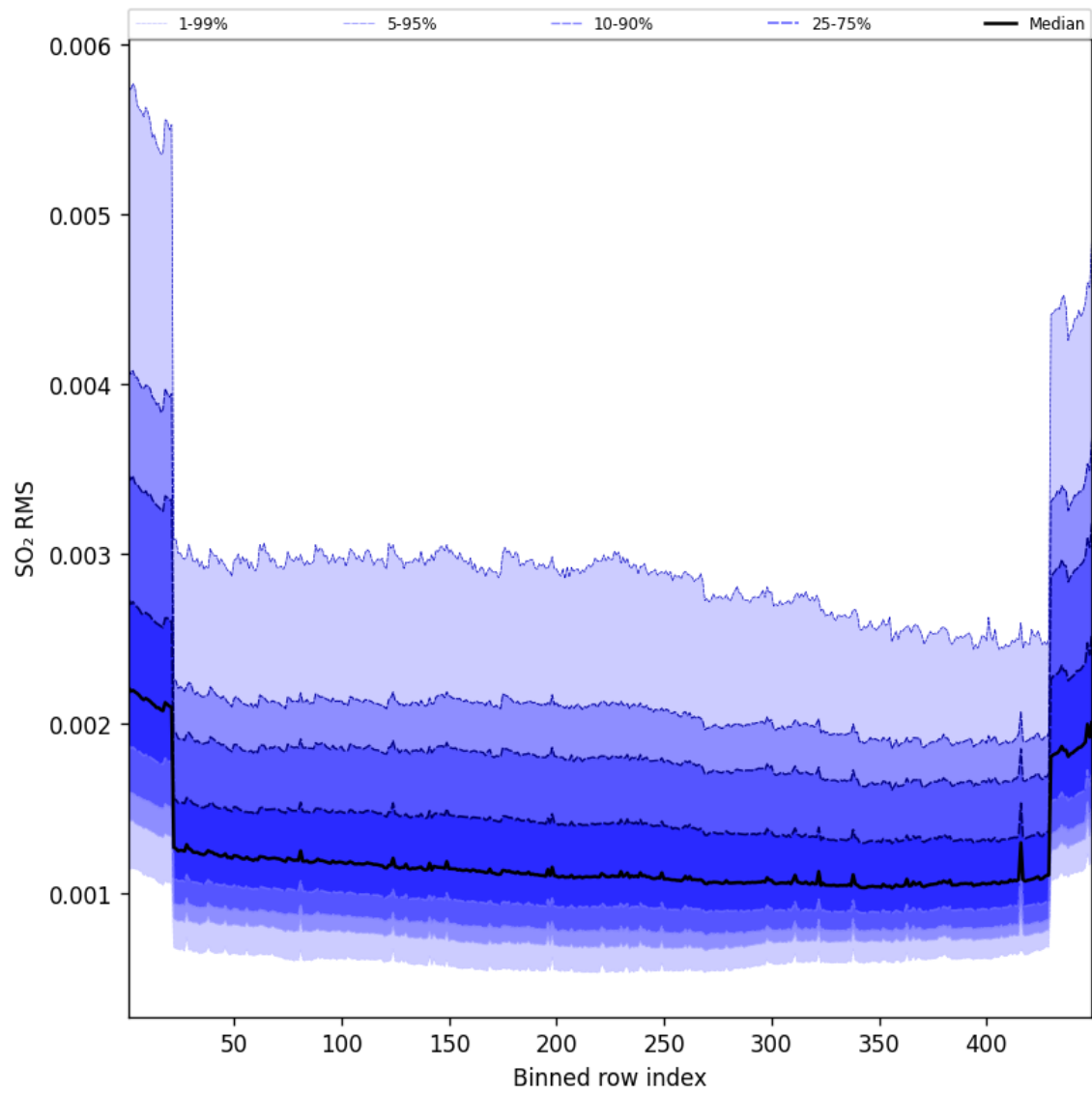
Figure 106: Along track statistics of “SO 2 RMS” for 2025-08-29 to 2025-08-30
