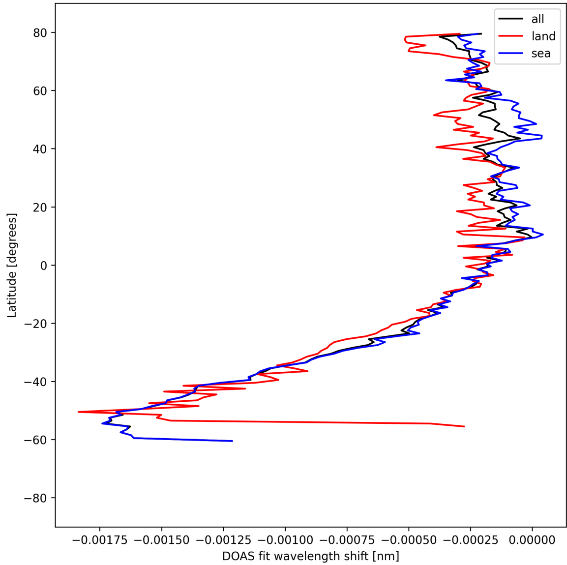
Figure 50: Zonal average of “DOAS fit wavelength shift” for 2025-08-29 to 2025-08-30.
