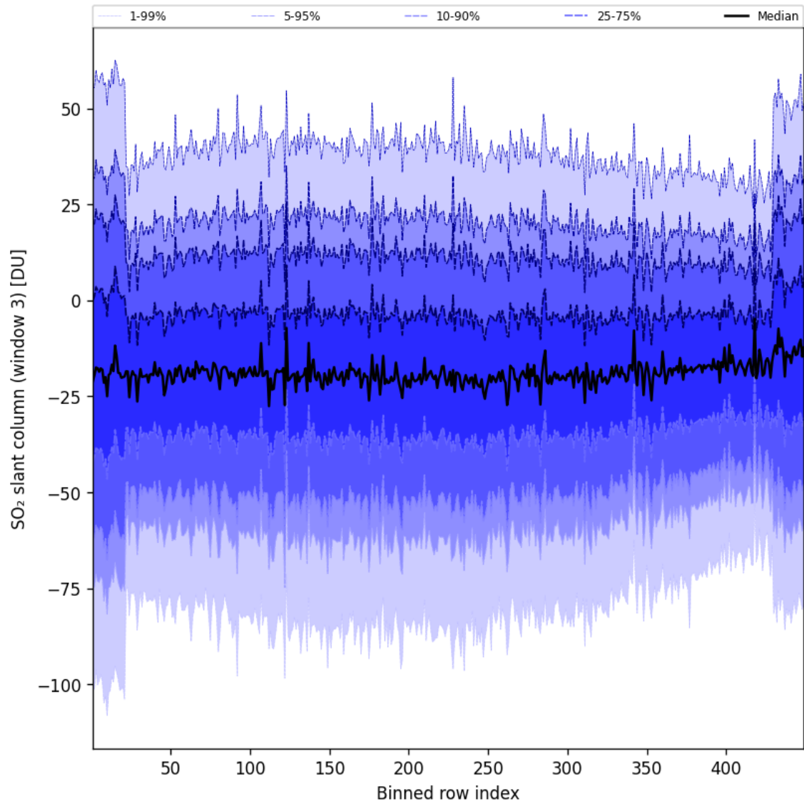
Figure 98: Along track statistics of “SO 2 slant column (window 3)” for 2025-08-29 to 2025-08-30
