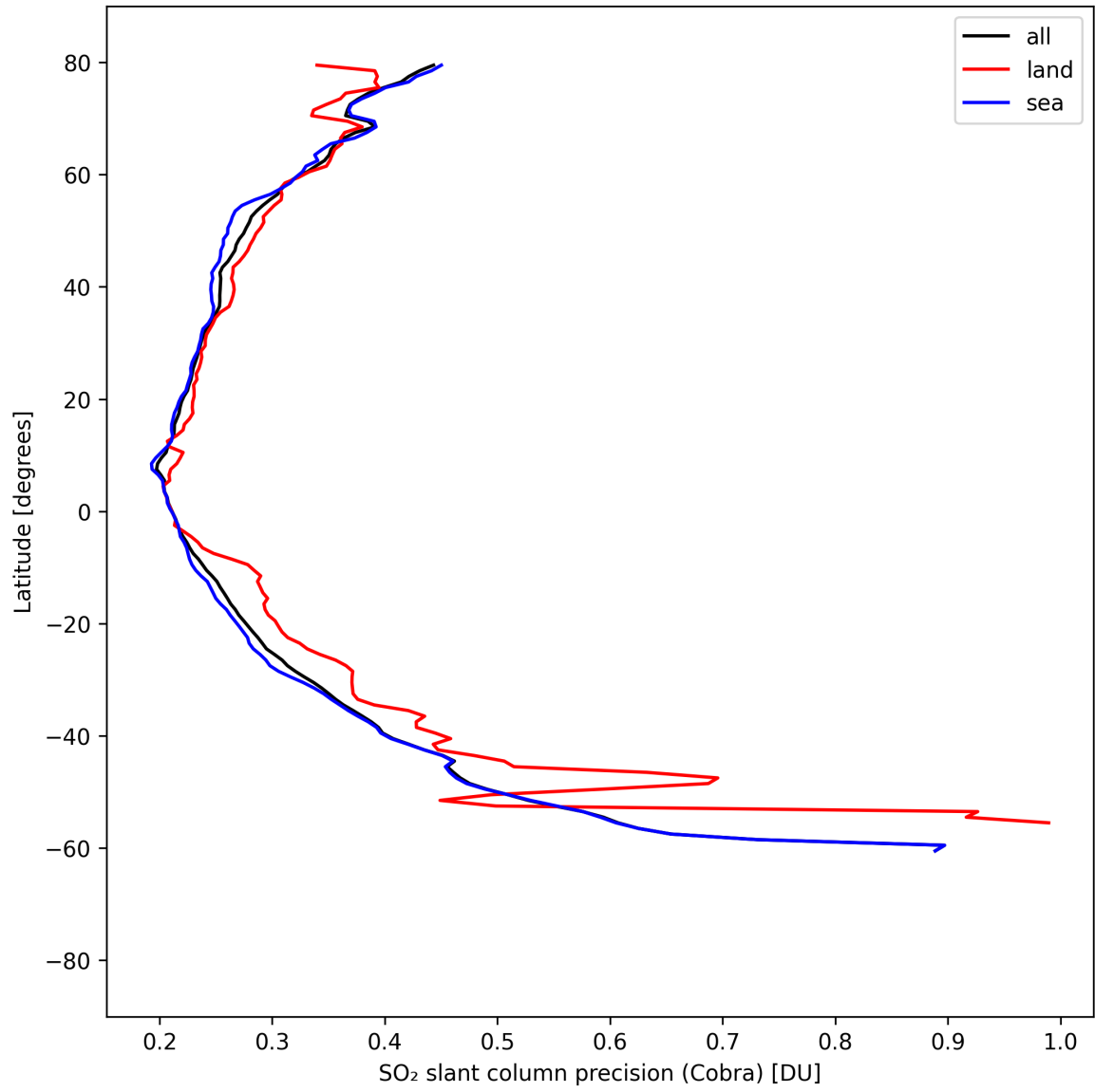
Figure 35: Zonal average of “SO 2 slant column precision (Cobra)” for 2025-08-29 to 2025-08-30.
