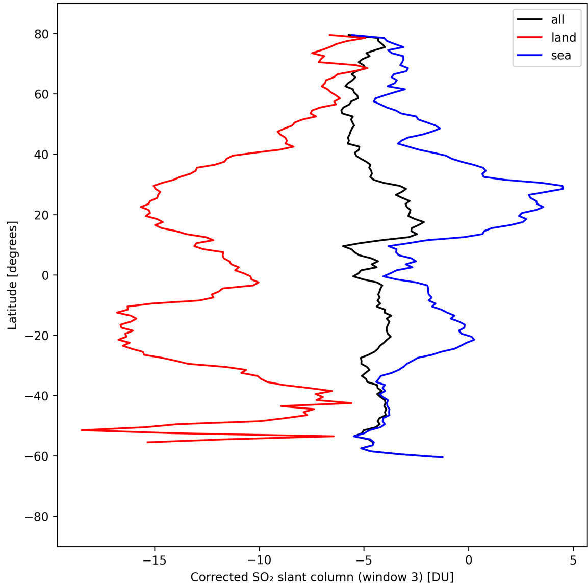
Figure 46: Zonal average of “Corrected SO 2 slant column (window 3)” for 2025-08-29 to 2025-08-30.
