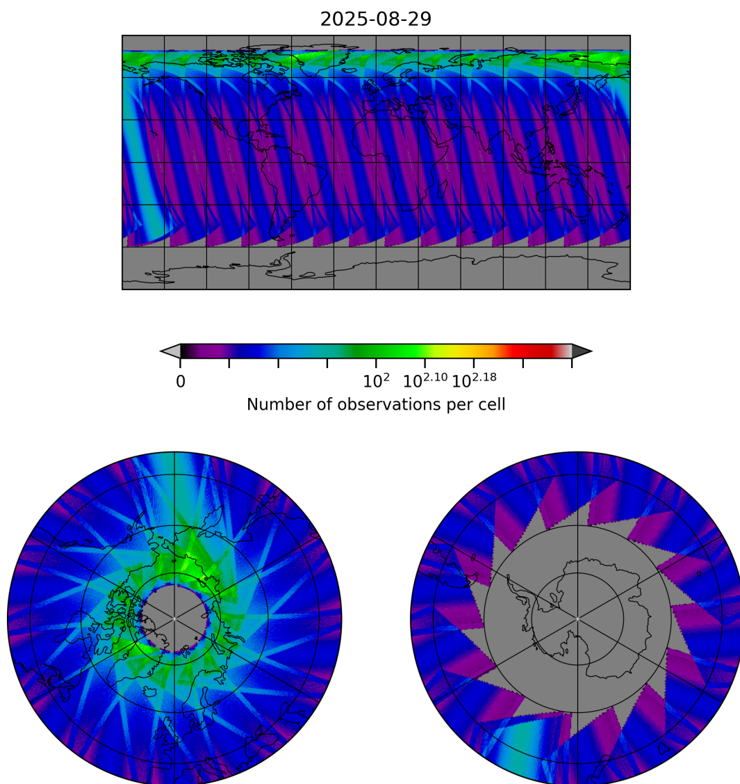
Figure 29: Map of the number of observations for 2025-08-29 to 2025-08-30
