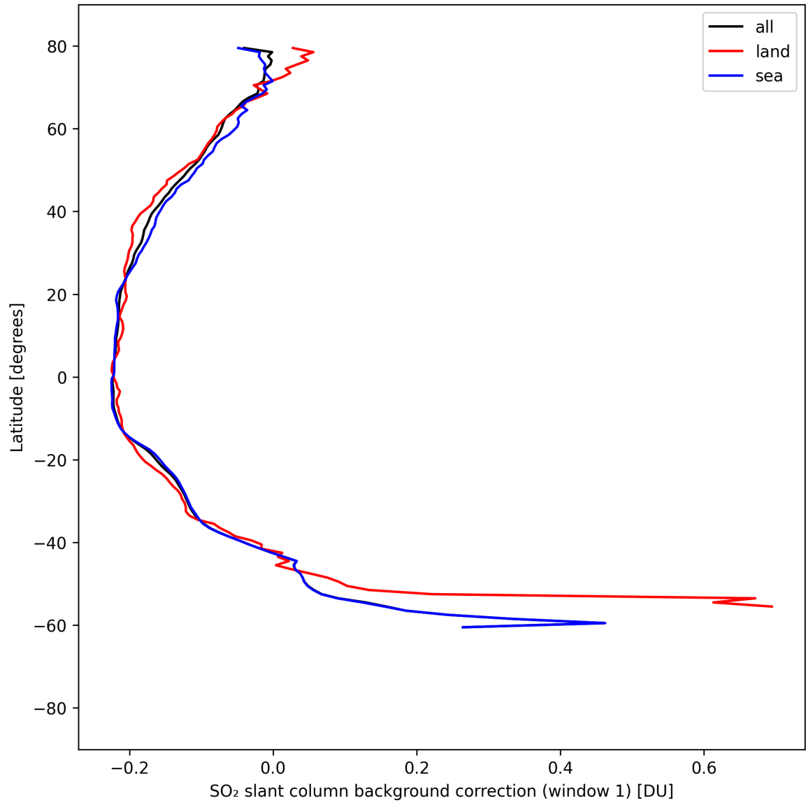
Figure 39: Zonal average of “SO 2 slant column background correction (window 1)” for 2025-08-29 to 2025-08-30.
