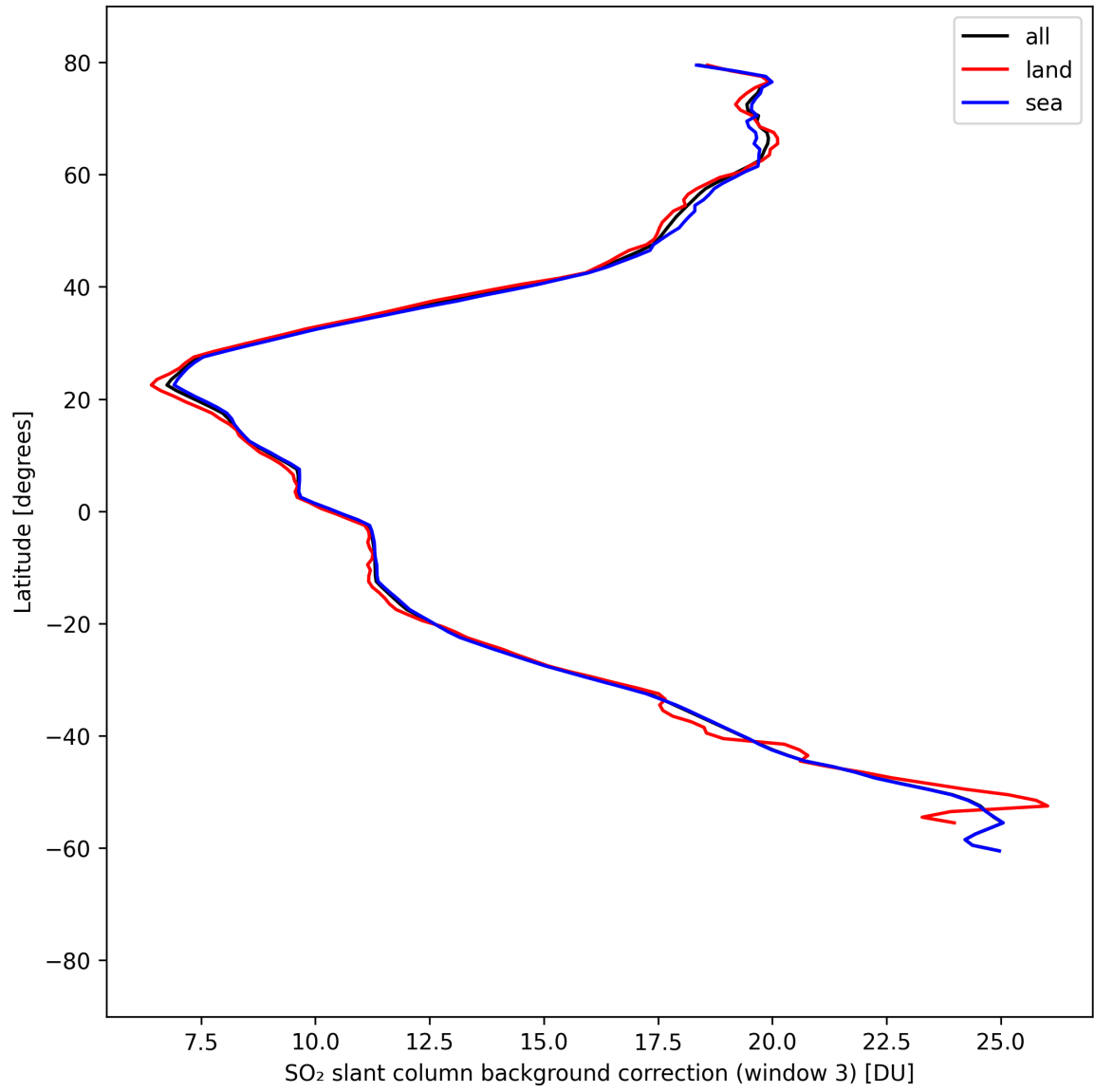
Figure 47: Zonal average of “SO 2 slant column background correction (window 3)” for 2025-08-29 to 2025-08-30.
