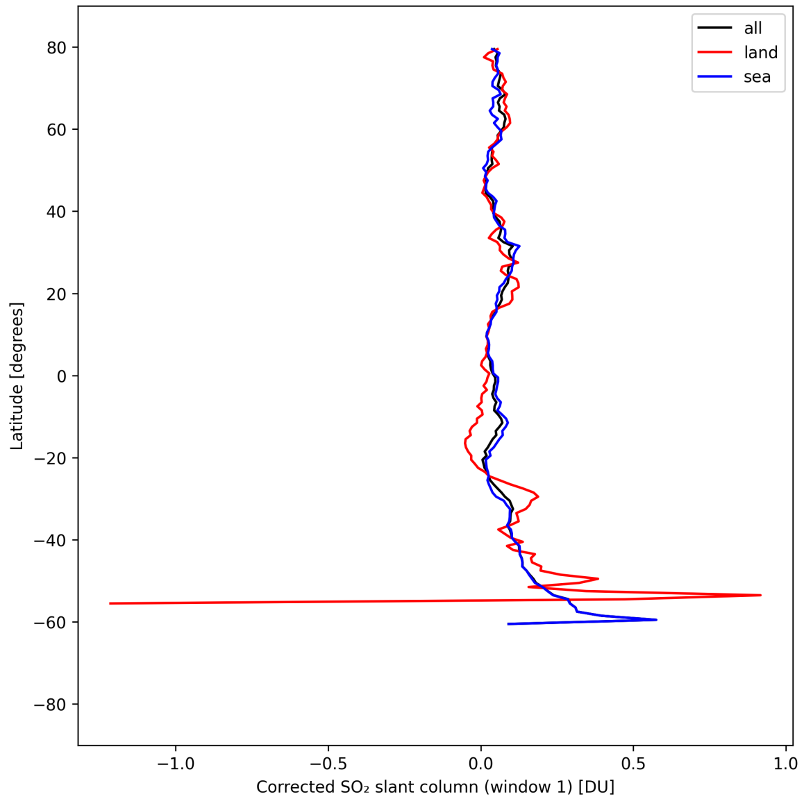
Figure 38: Zonal average of “Corrected SO 2 slant column (window 1)” for 2025-08-29 to 2025-08-30.
