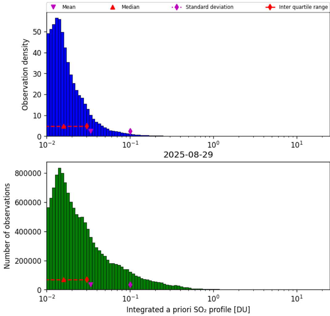
Figure 76: Histogram of “Integrated a priori SO 2 profile” for 2025-08-29 to 2025-08-30
