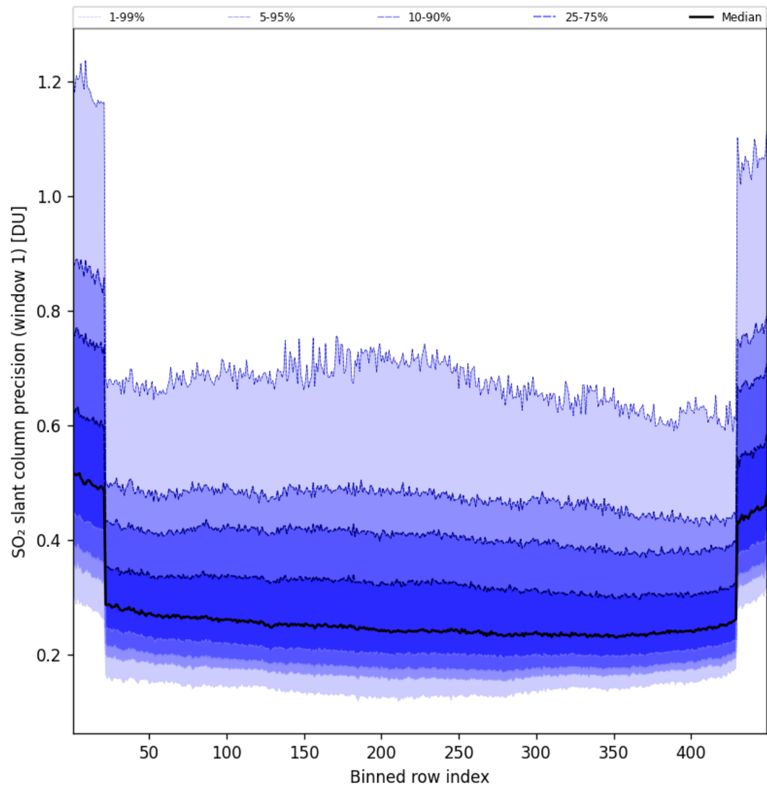
Figure 91: Along track statistics of “SO 2 slant column precision (window 1)” for 2025-08-29 to 2025-08-30
