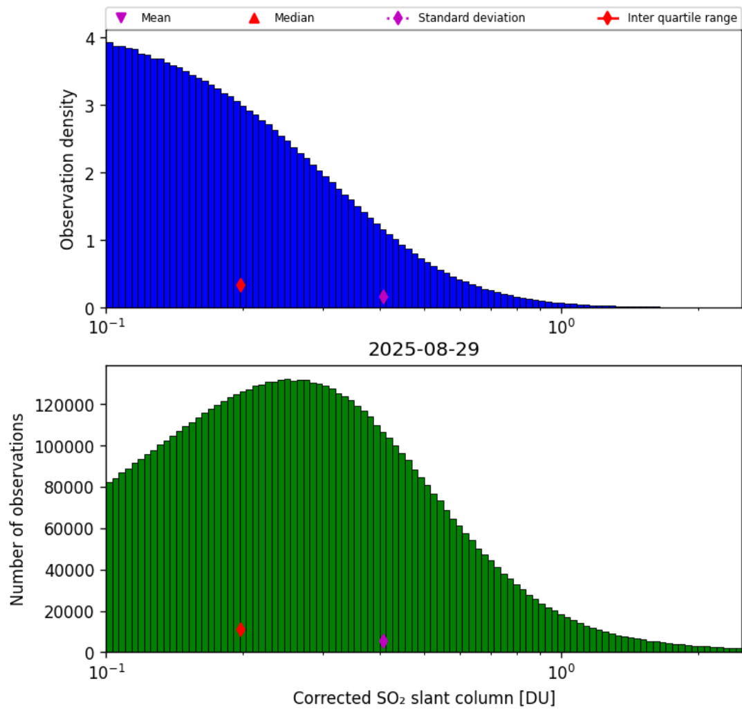
Figure 60: Histogram of “Corrected SO 2 slant column” for 2025-08-29 to 2025-08-30
