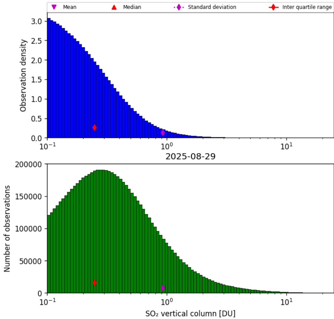
Figure 58: Histogram of “SO 2 vertical column” for 2025-08-29 to 2025-08-30
