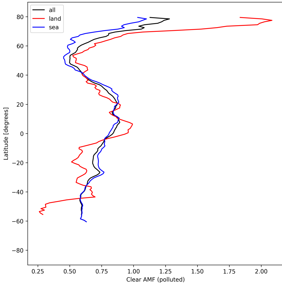
Figure 55: Zonal average of “Clear AMF (polluted)” for 2025-08-29 to 2025-08-30.
