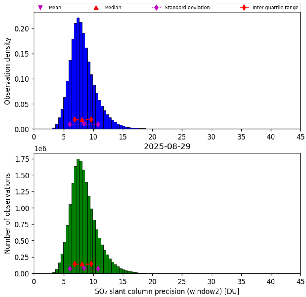
Figure 68: Histogram of “SO 2 slant column precision (window2)” for 2025-08-29 to 2025-08-30
