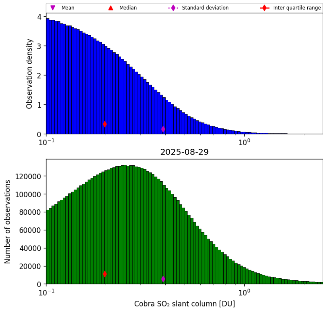
Figure 61: Histogram of “Cobra SO 2 slant column” for 2025-08-29 to 2025-08-30
