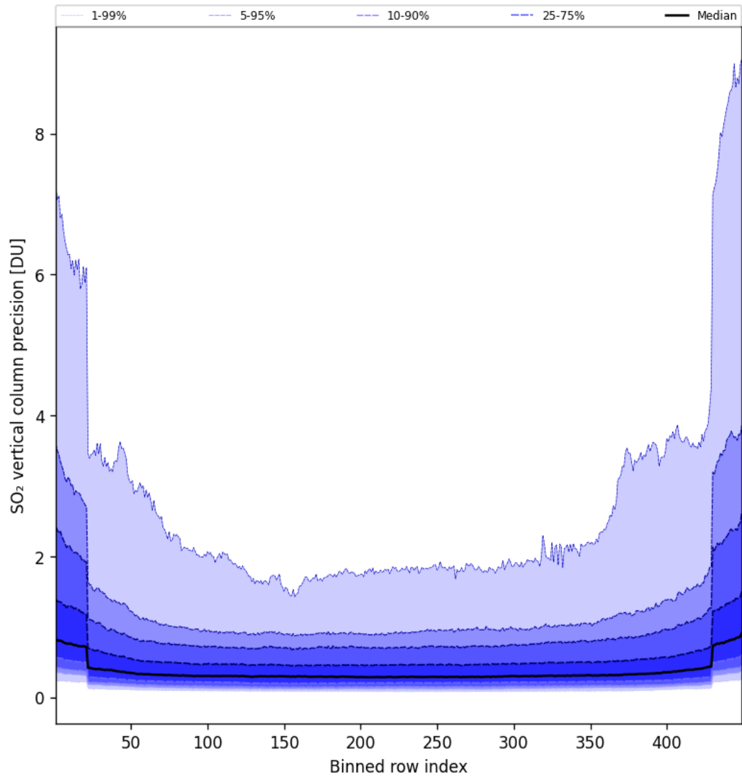
Figure 86: Along track statistics of “SO 2 vertical column precision” for 2025-08-29 to 2025-08-30
