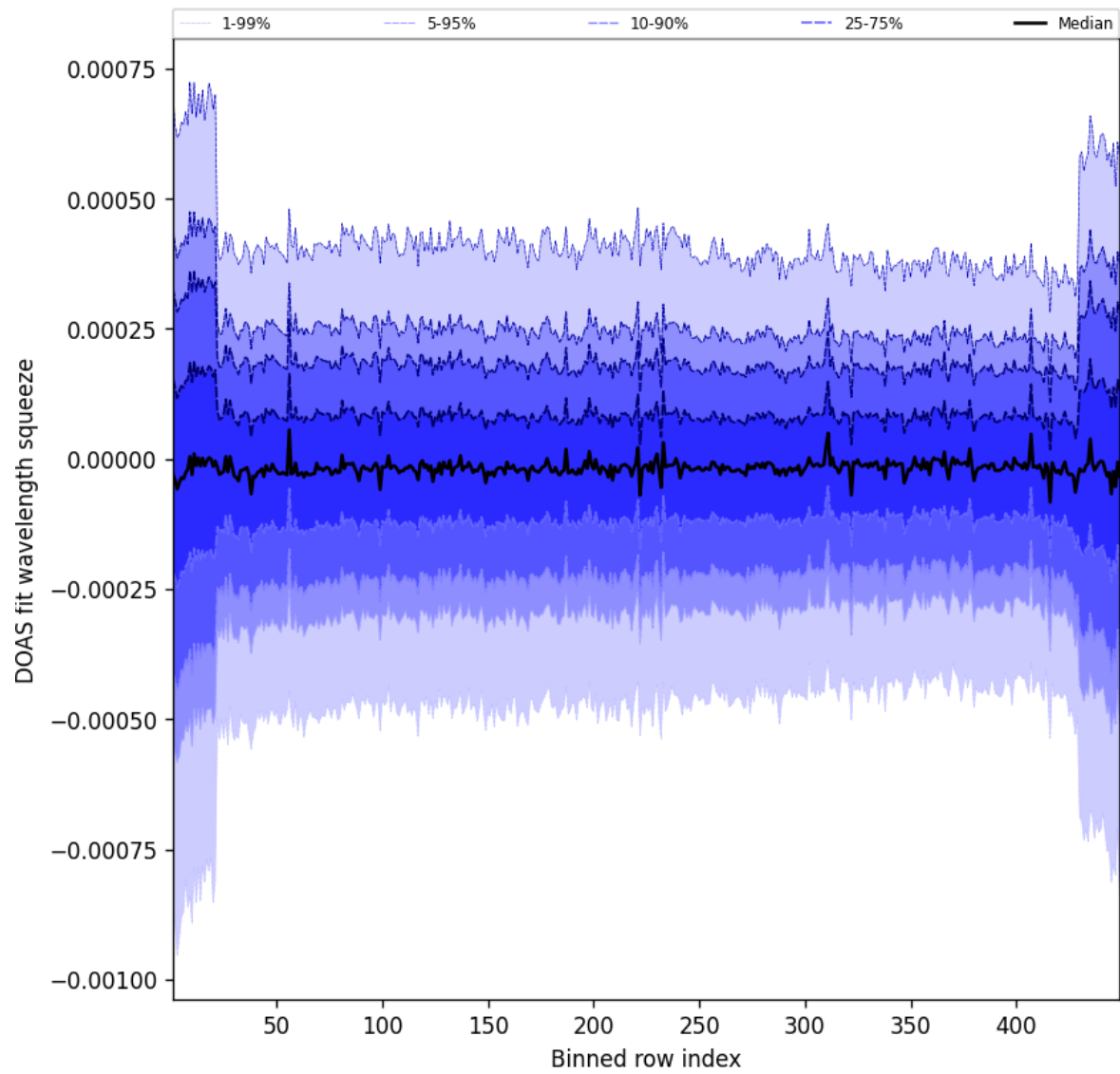
Figure 105: Along track statistics of “DOAS fit wavelength squeeze” for 2025-08-29 to 2025-08-30
