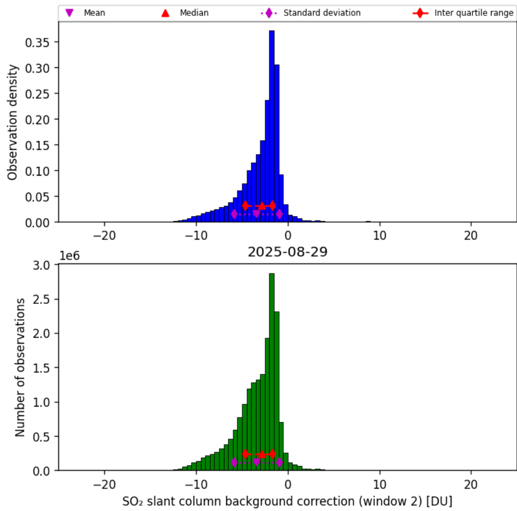
Figure 70: Histogram of “SO 2 slant column background correction (window 2)” for 2025-08-29 to 2025-08-30
