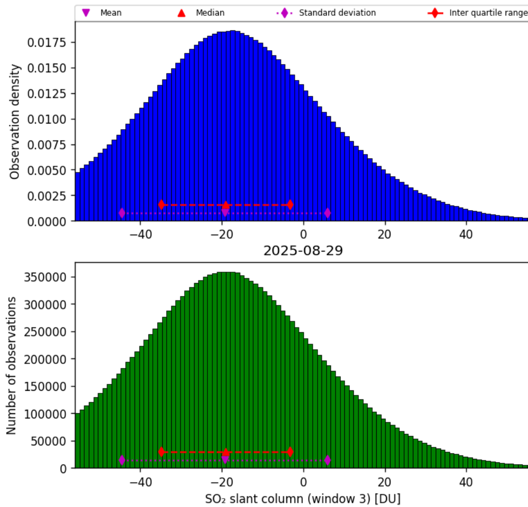
Figure 71: Histogram of “SO 2 slant column (window 3)” for 2025-08-29 to 2025-08-30
