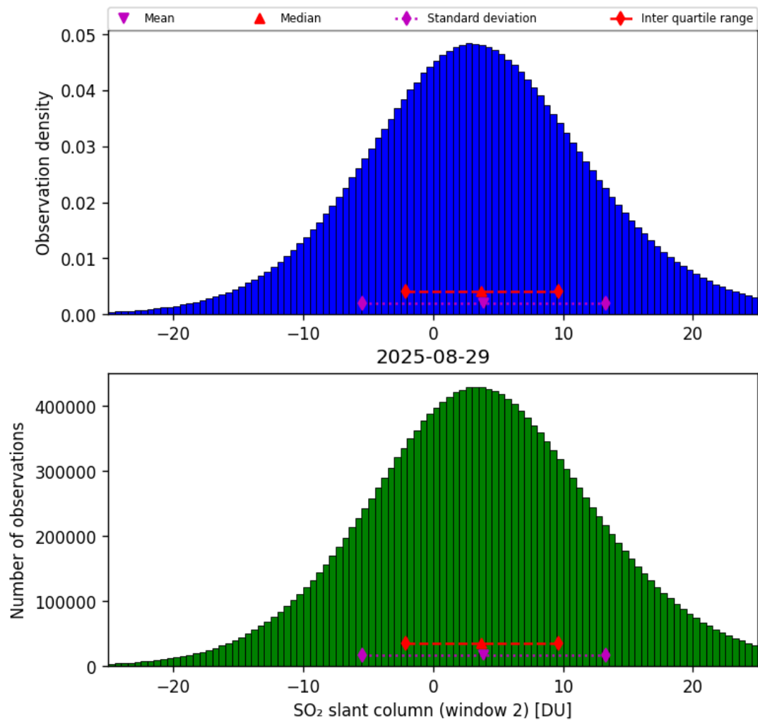
Figure 67: Histogram of “SO 2 slant column (window 2)” for 2025-08-29 to 2025-08-30
