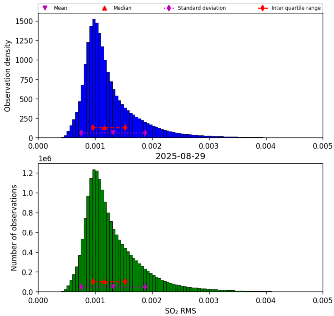
Figure 79: Histogram of “SO 2 RMS” for 2025-08-29 to 2025-08-30
