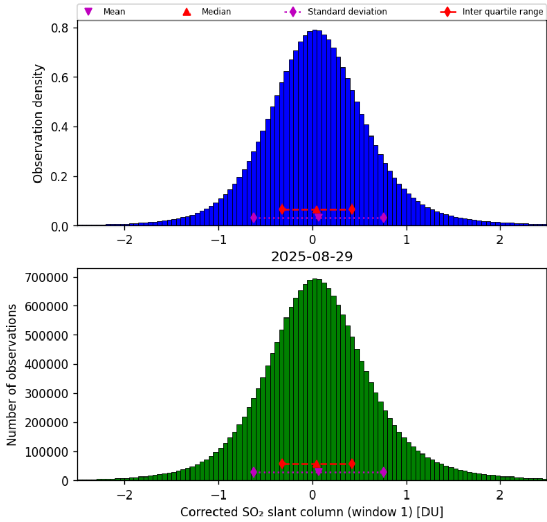
Figure 65: Histogram of “Corrected SO 2 slant column (window 1)” for 2025-08-29 to 2025-08-30
