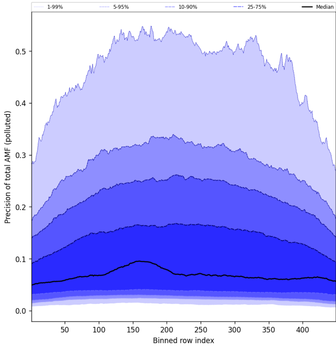
Figure 108: Along track statistics of “Precision of total AMF (polluted)” for 2025-08-29 to 2025-08-30
