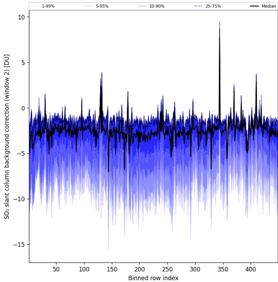
Figure 97: Along track statistics of “SO 2 slant column background correction (window 2)” for 2025-08-29 to 2025-08-30
