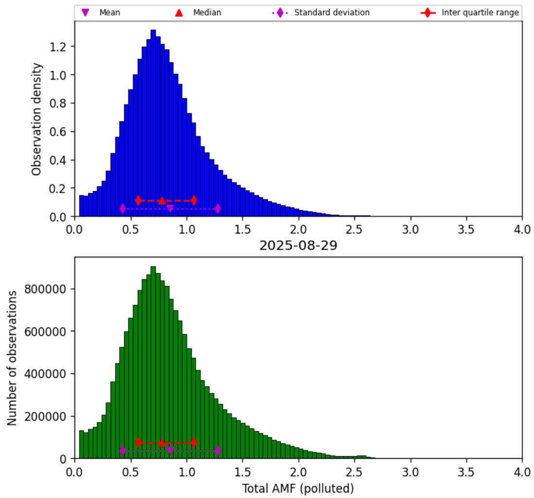
Figure 80: Histogram of “Total AMF (polluted)” for 2025-08-29 to 2025-08-30
