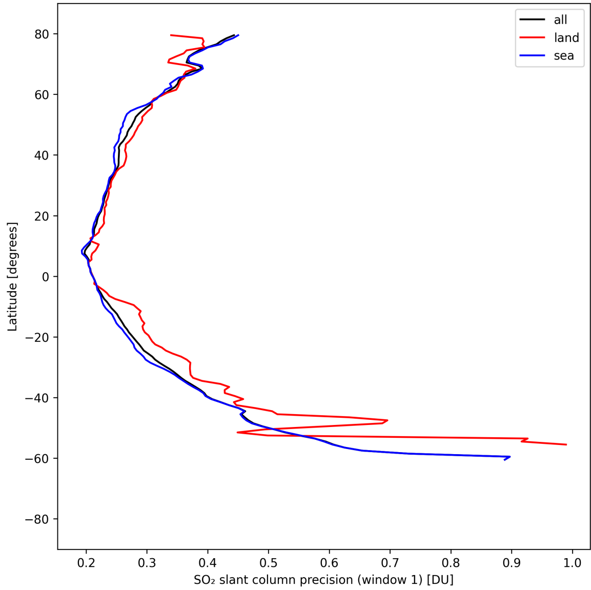
Figure 37: Zonal average of “SO 2 slant column precision (window 1)” for 2025-08-29 to 2025-08-30.
