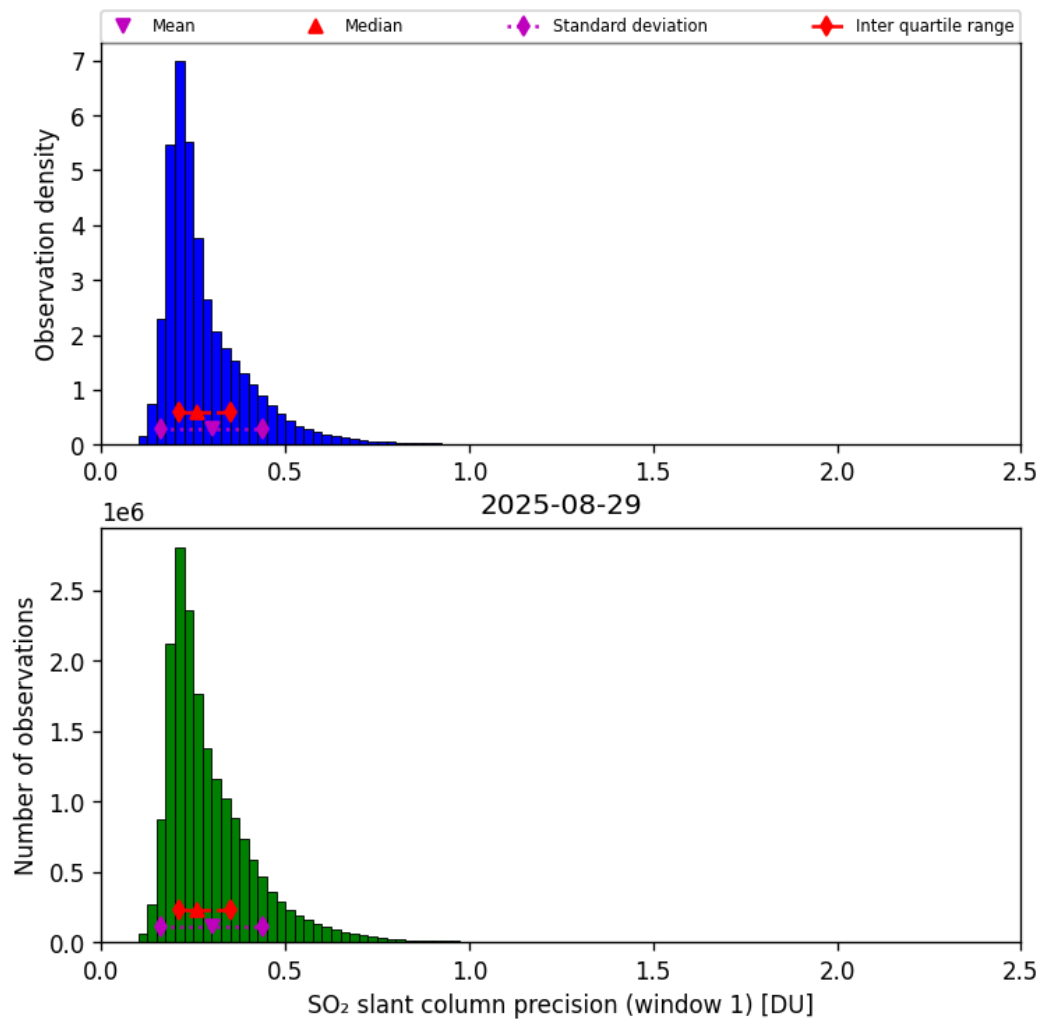
Figure 64: Histogram of “SO 2 slant column precision (window 1)” for 2025-08-29 to 2025-08-30
