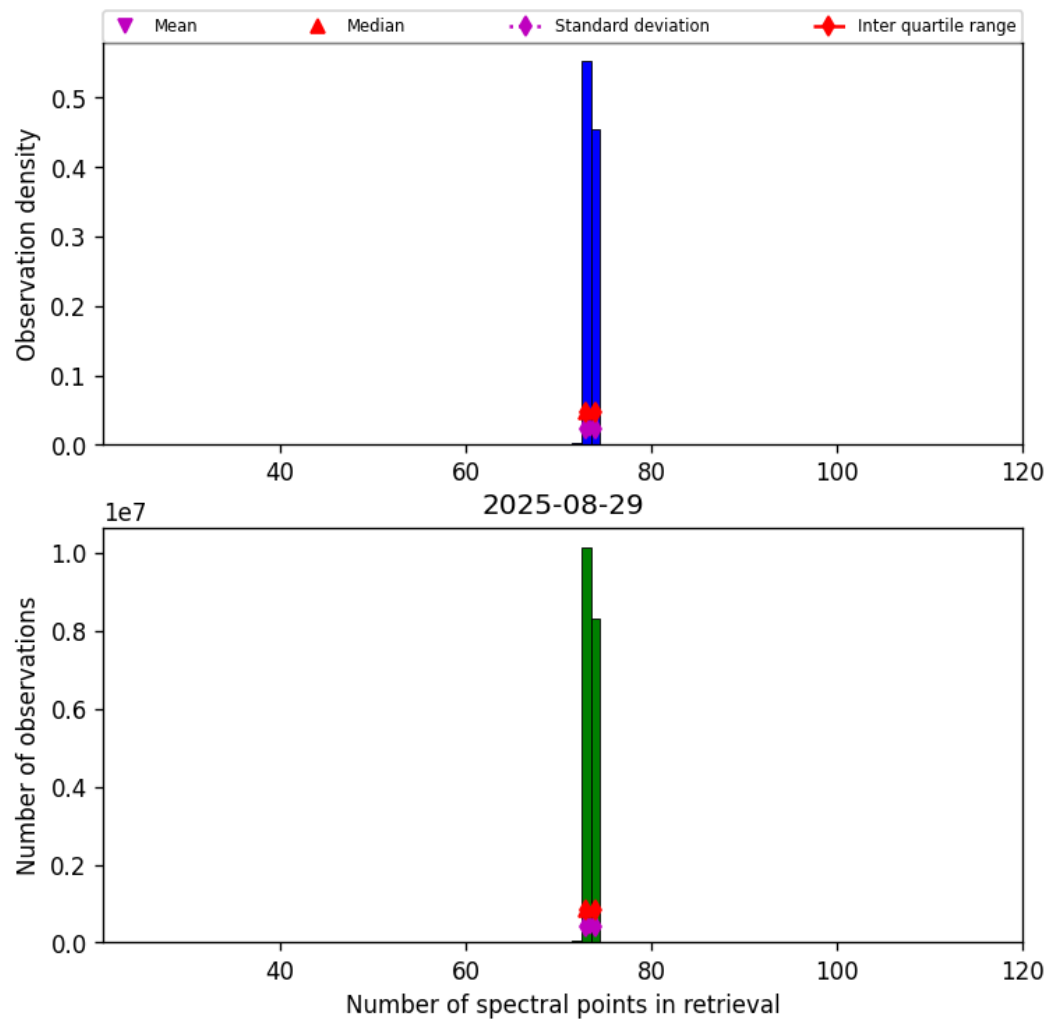
Figure 83: Histogram of “Number of spectral points in retrieval” for 2025-08-29 to 2025-08-30
