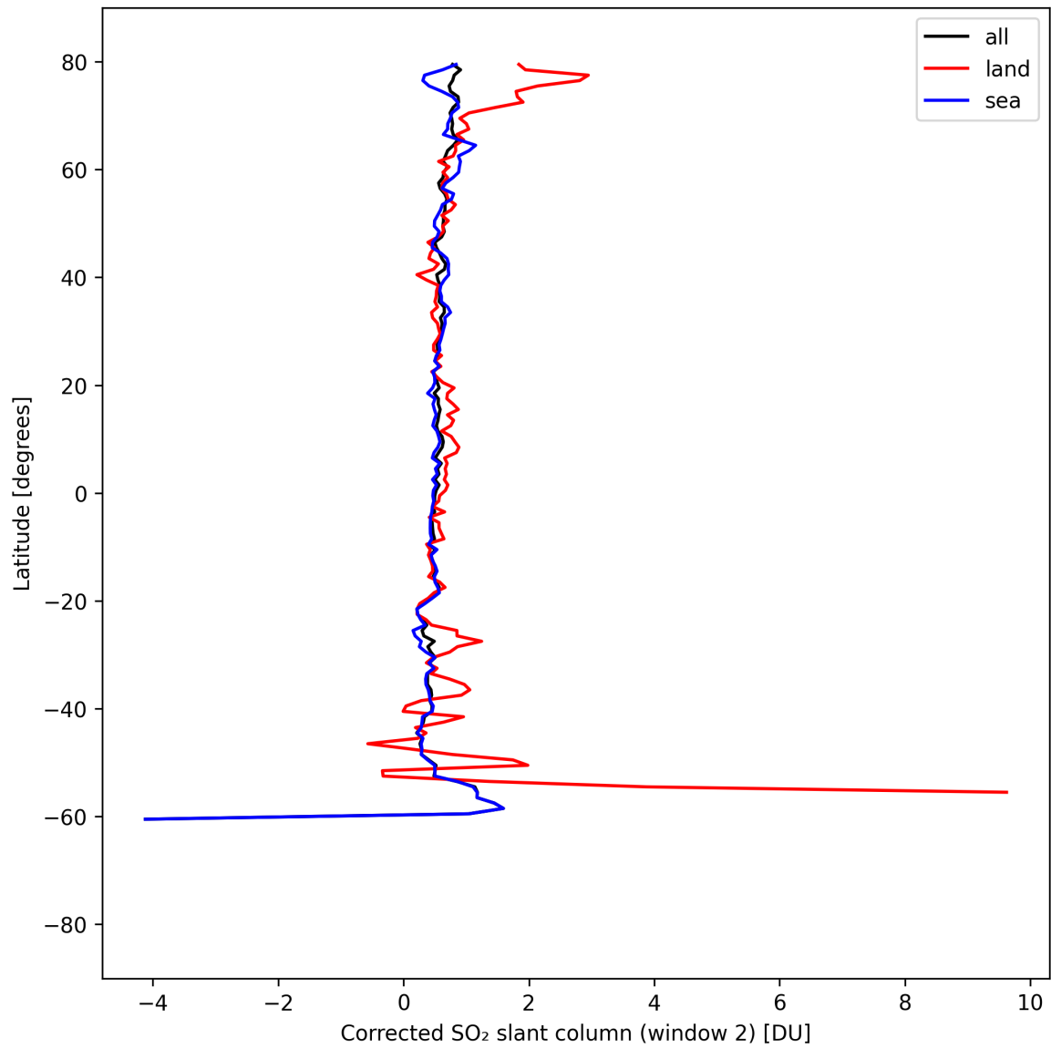
Figure 42: Zonal average of “Corrected SO 2 slant column (window 2)” for 2025-08-29 to 2025-08-30.
