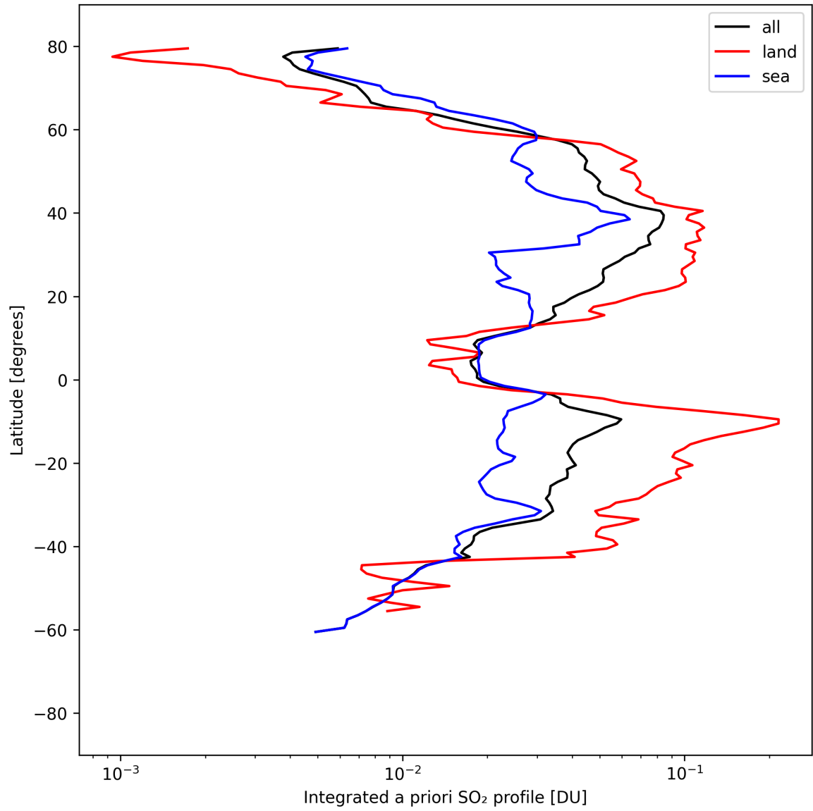
Figure 49: Zonal average of “Integrated a priori SO 2 profile” for 2025-08-29 to 2025-08-30.
