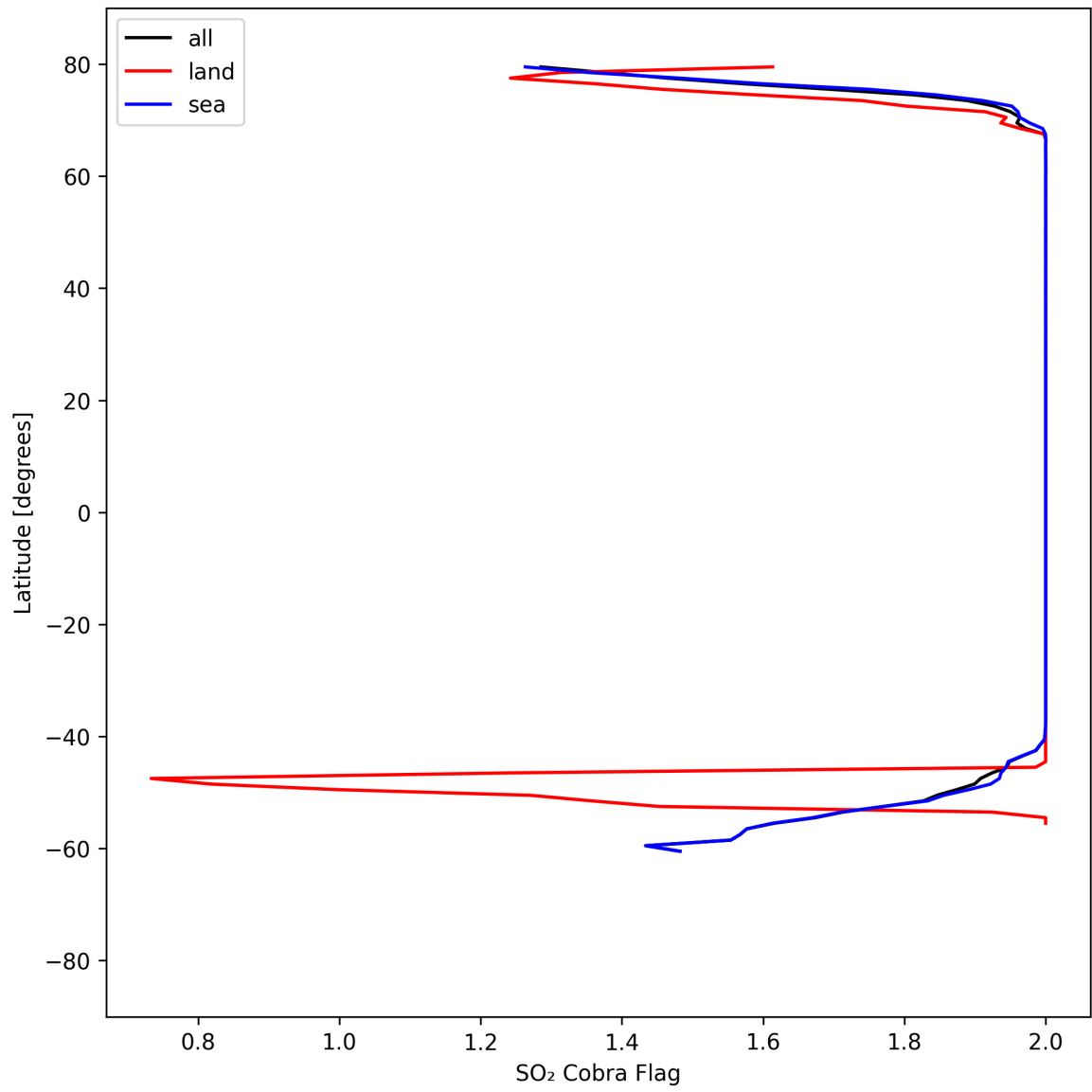
Figure 48: Zonal average of "SO 2 Cobra Flag" for 2025-08-29 to 2025-08-30.
