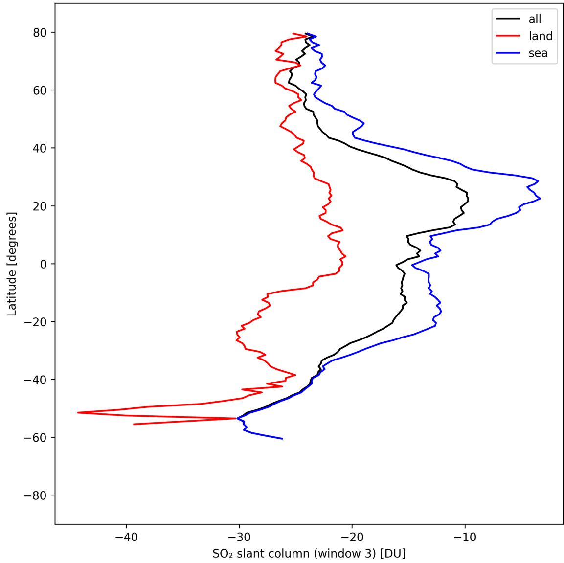
Figure 44: Zonal average of “SO 2 slant column (window 3)” for 2025-08-29 to 2025-08-30.
