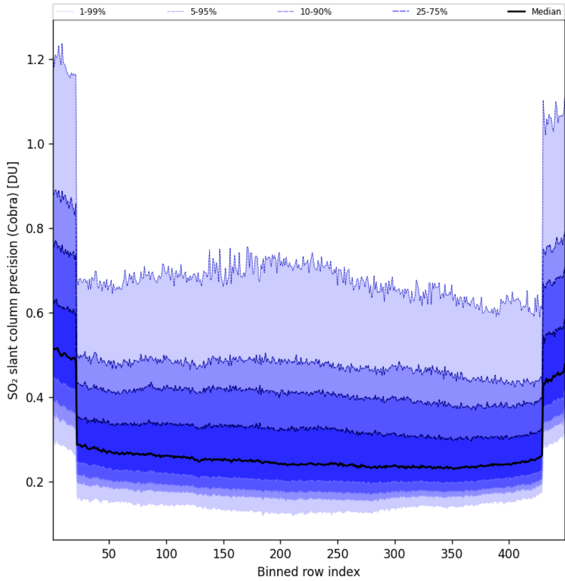
Figure 89: Along track statistics of “SO 2 slant column precision (Cobra)” for 2025-08-29 to 2025-08-30
