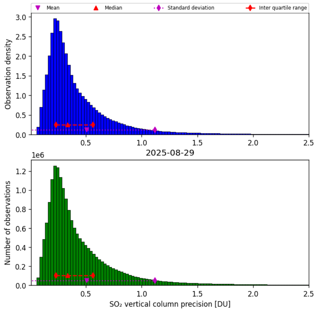
Figure 59: Histogram of “SO 2 vertical column precision” for 2025-08-29 to 2025-08-30
