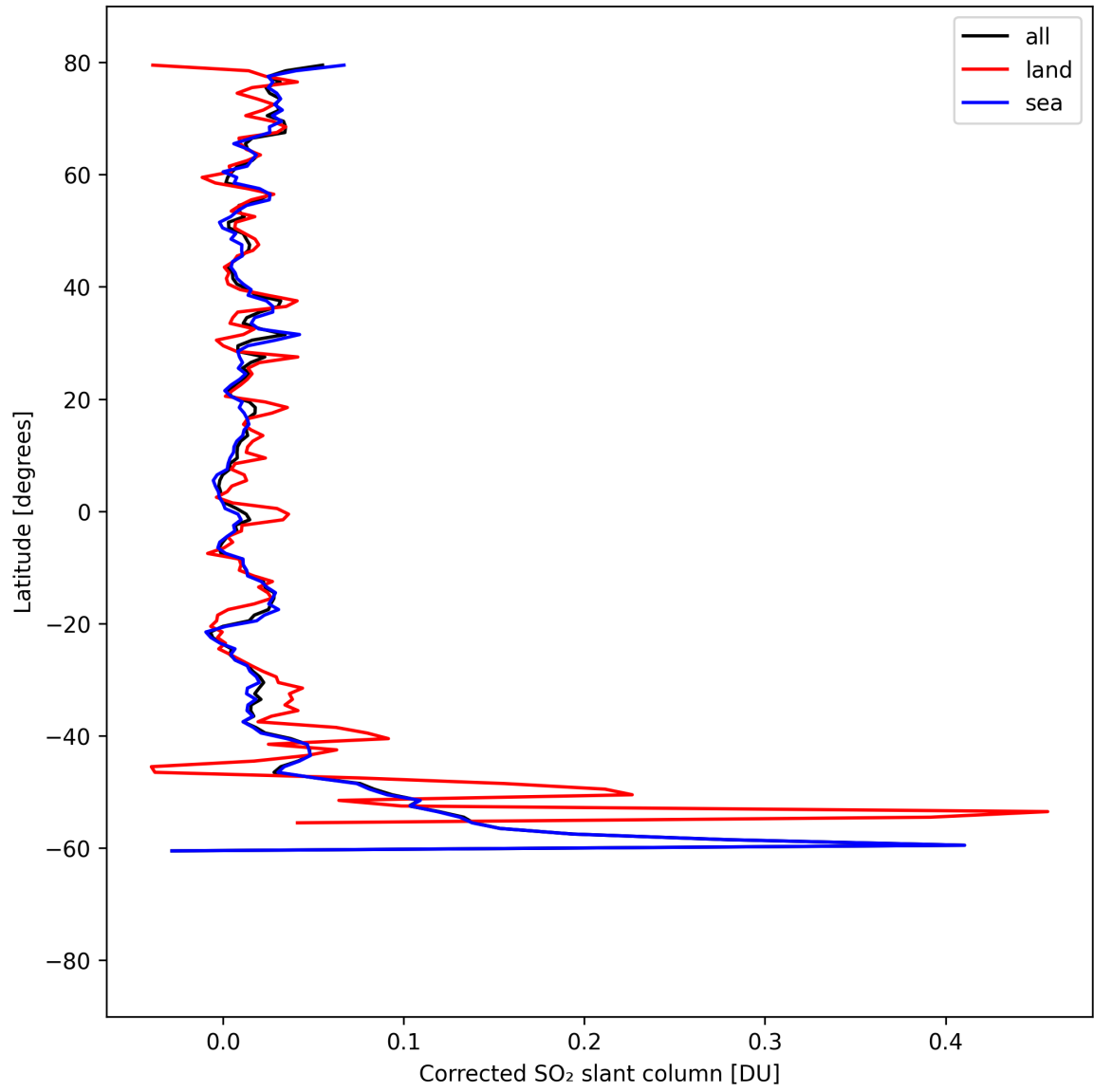
Figure 33: Zonal average of “Corrected SO 2 slant column” for 2025-08-29 to 2025-08-30.
