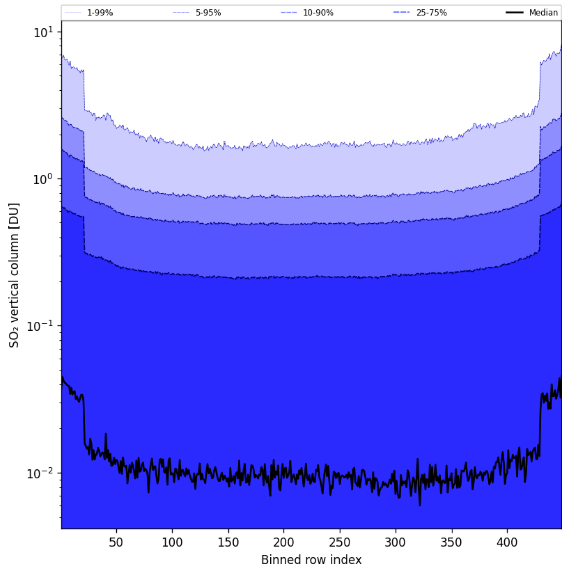
Figure 85: Along track statistics of “SO 2 vertical column” for 2025-08-29 to 2025-08-30
