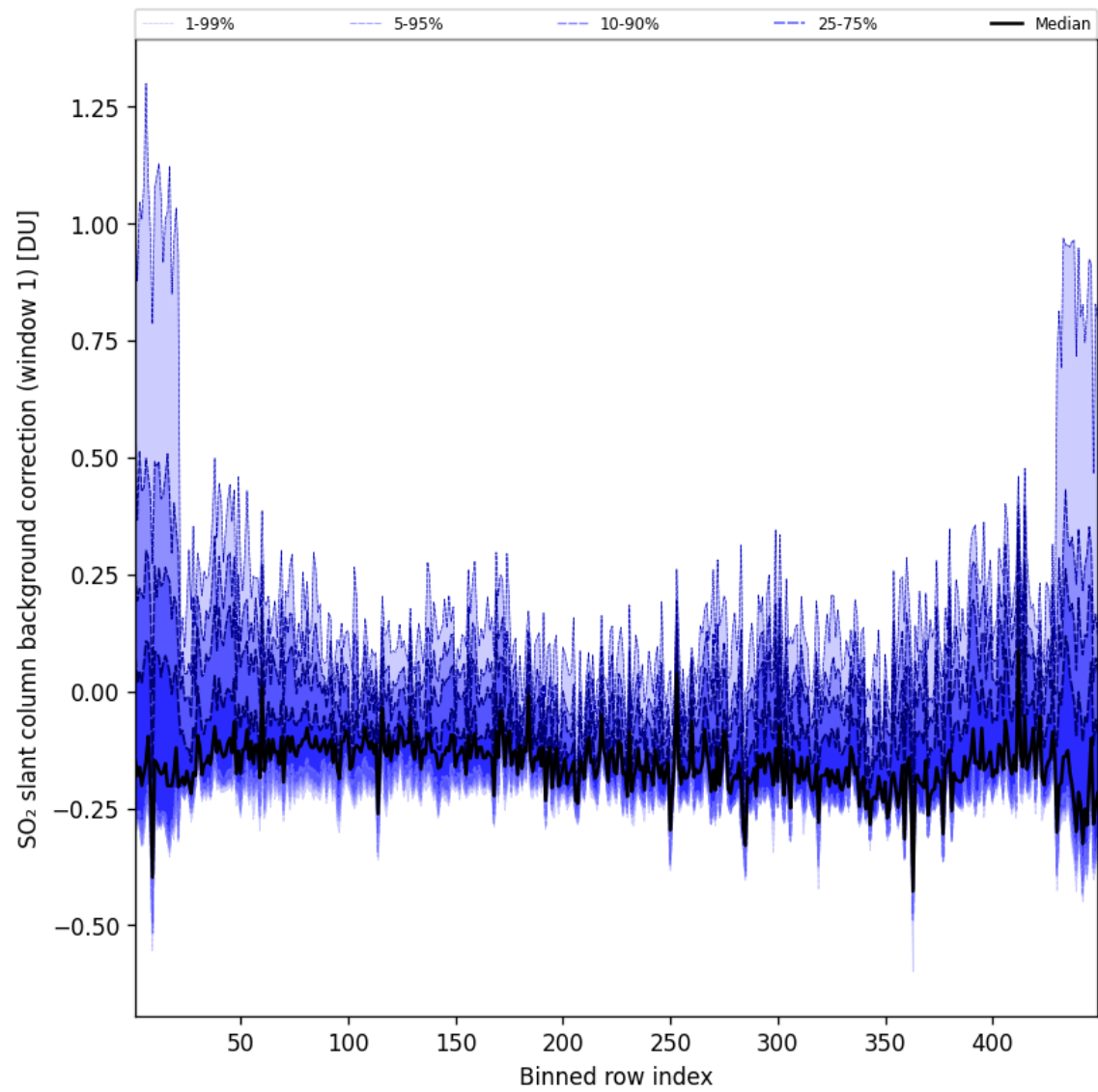
Figure 93: Along track statistics of “SO 2 slant column background correction (window 1)” for 2025-08-29 to 2025-08-30
