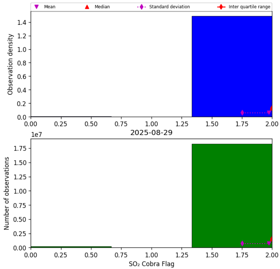
Figure 75: Histogram of “SO 2 Cobra Flag” for 2025-08-29 to 2025-08-30
