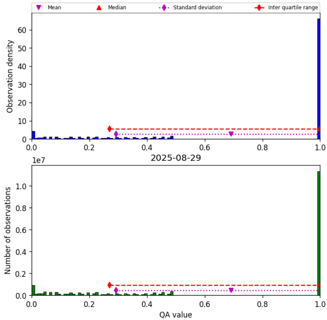
Figure 57: Histogram of “QA value” for 2025-08-29 to 2025-08-30
