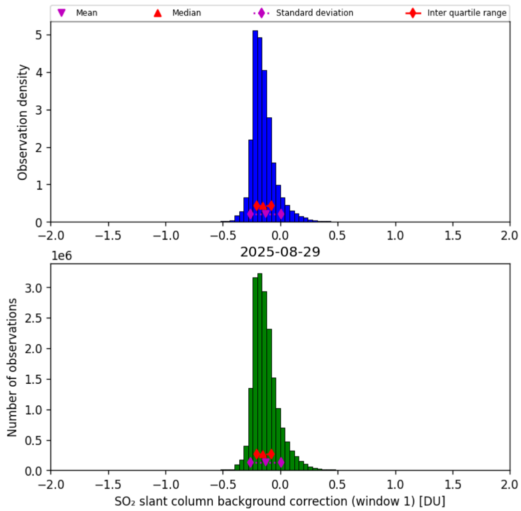
Figure 66: Histogram of “SO 2 slant column background correction (window 1)” for 2025-08-29 to 2025-08-30
