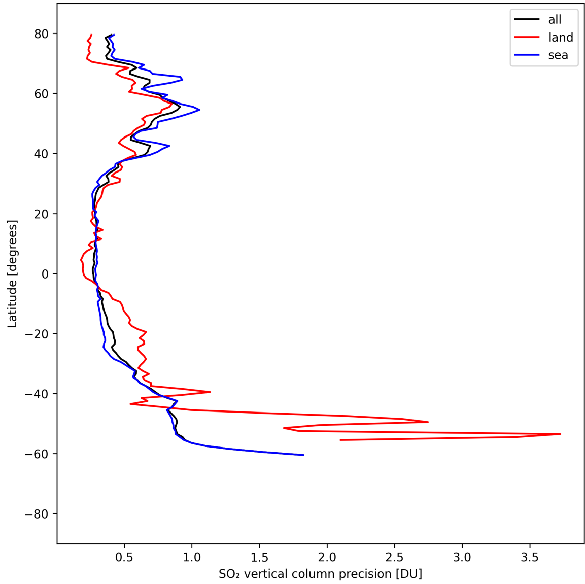
Figure 32: Zonal average of “SO 2 vertical column precision” for 2025-08-29 to 2025-08-30.
