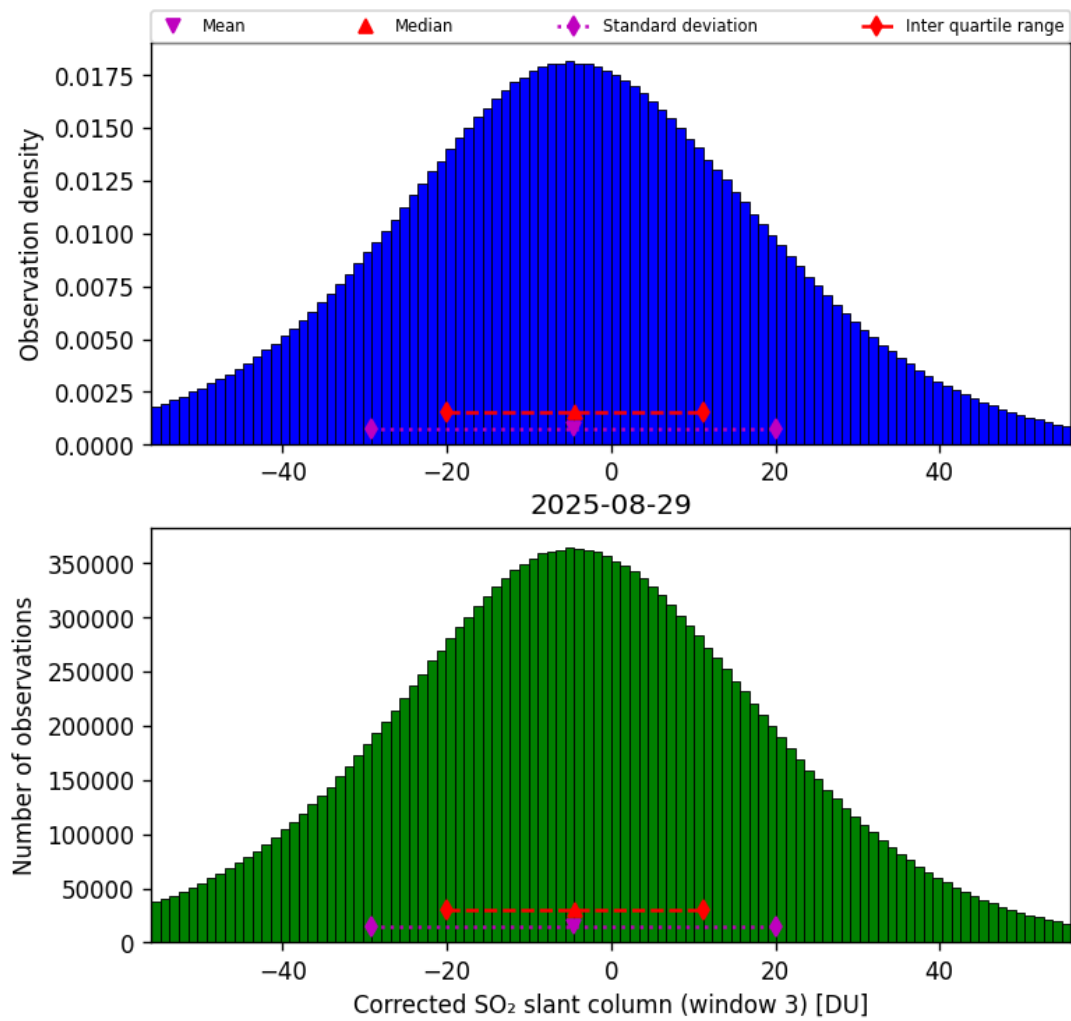
Figure 73: Histogram of “Corrected SO 2 slant column (window 3)” for 2025-08-29 to 2025-08-30
