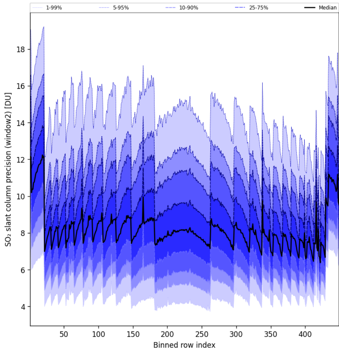
Figure 95: Along track statistics of “SO 2 slant column precision (window2)” for 2025-08-29 to 2025-08-30
