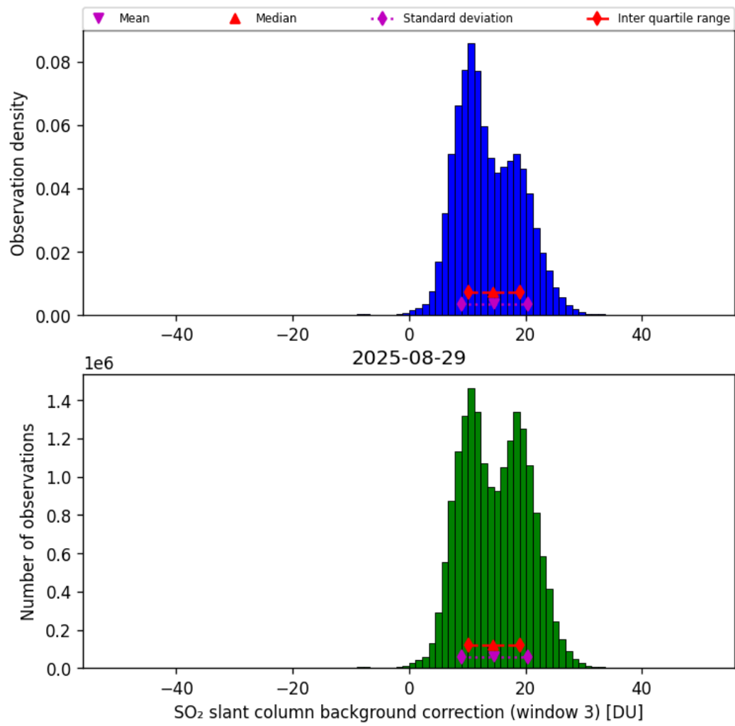
Figure 74: Histogram of “SO 2 slant column background correction (window 3)” for 2025-08-29 to 2025-08-30
