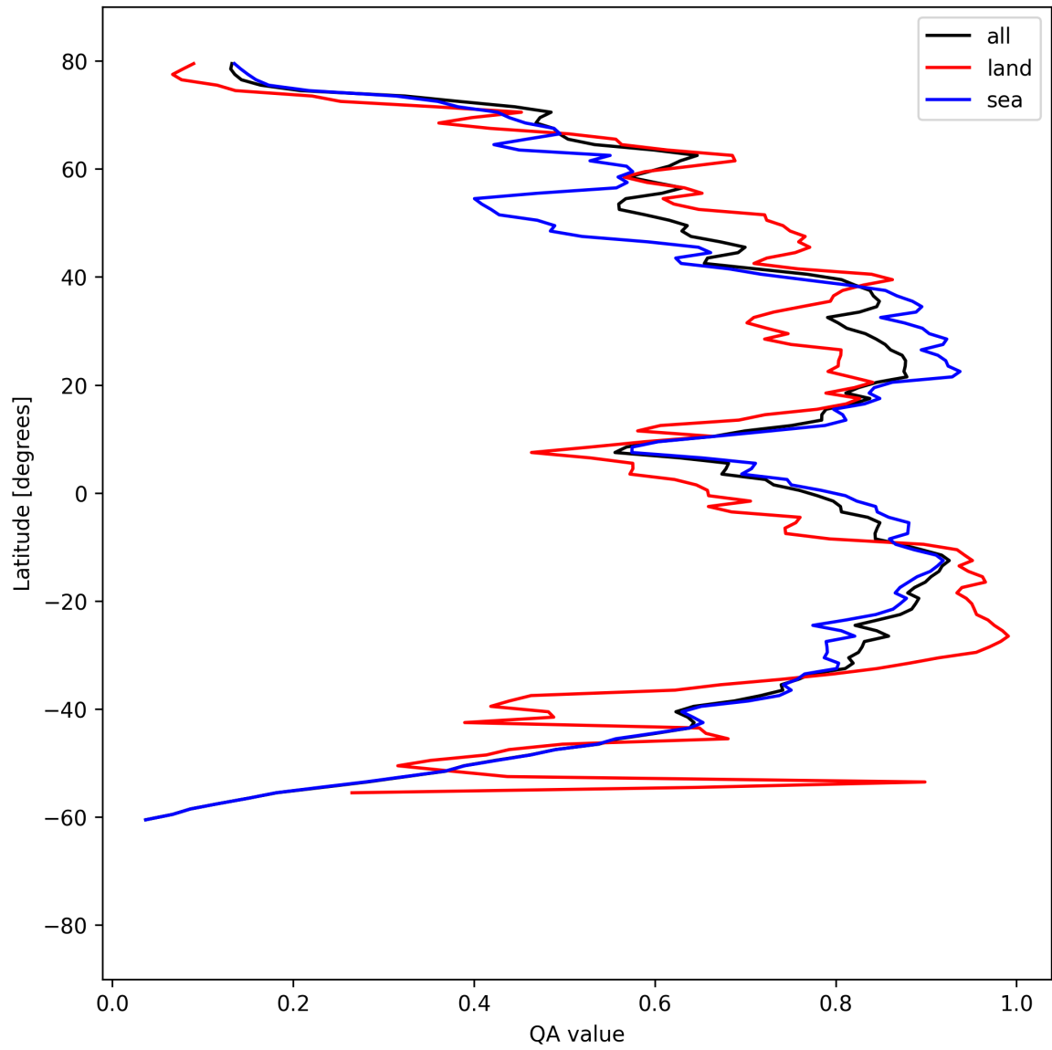
Figure 30: Zonal average of “QA value” for 2025-08-29 to 2025-08-30.
