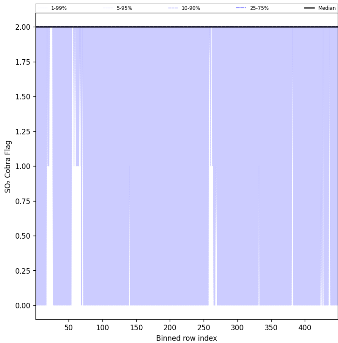
Figure 102: Along track statistics of "SO 2 Cobra Flag" for 2025-08-29 to 2025-08-30
