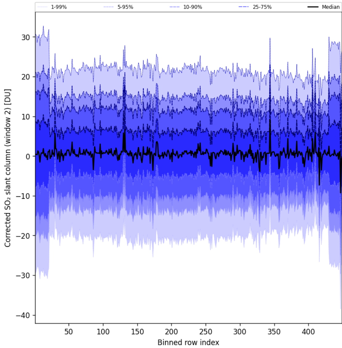
Figure 96: Along track statistics of “Corrected SO 2 slant column (window 2)” for 2025-08-29 to 2025-08-30
