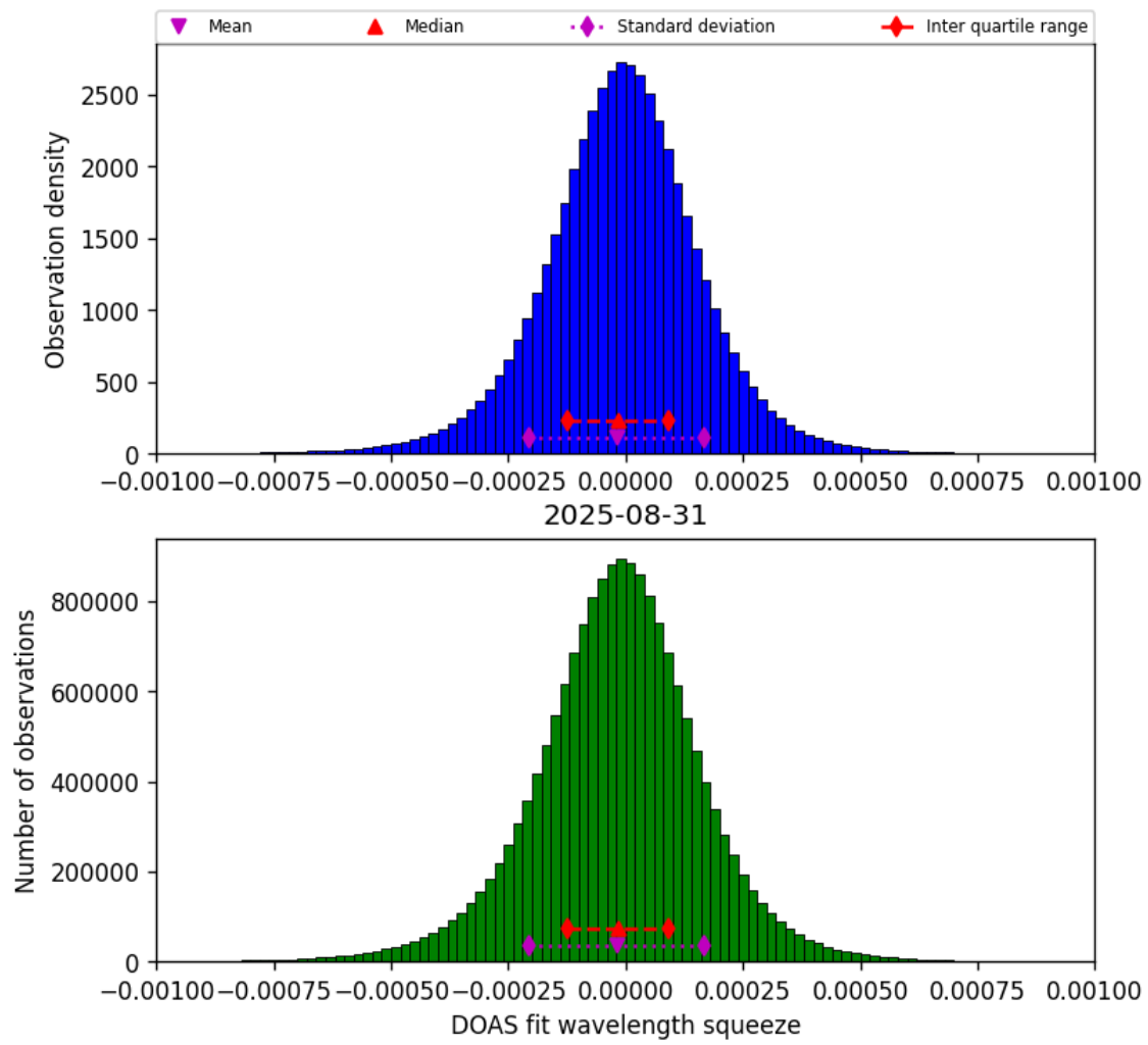
Figure 78: Histogram of “DOAS fit wavelength squeeze” for 2025-08-31 to 2025-09-01
