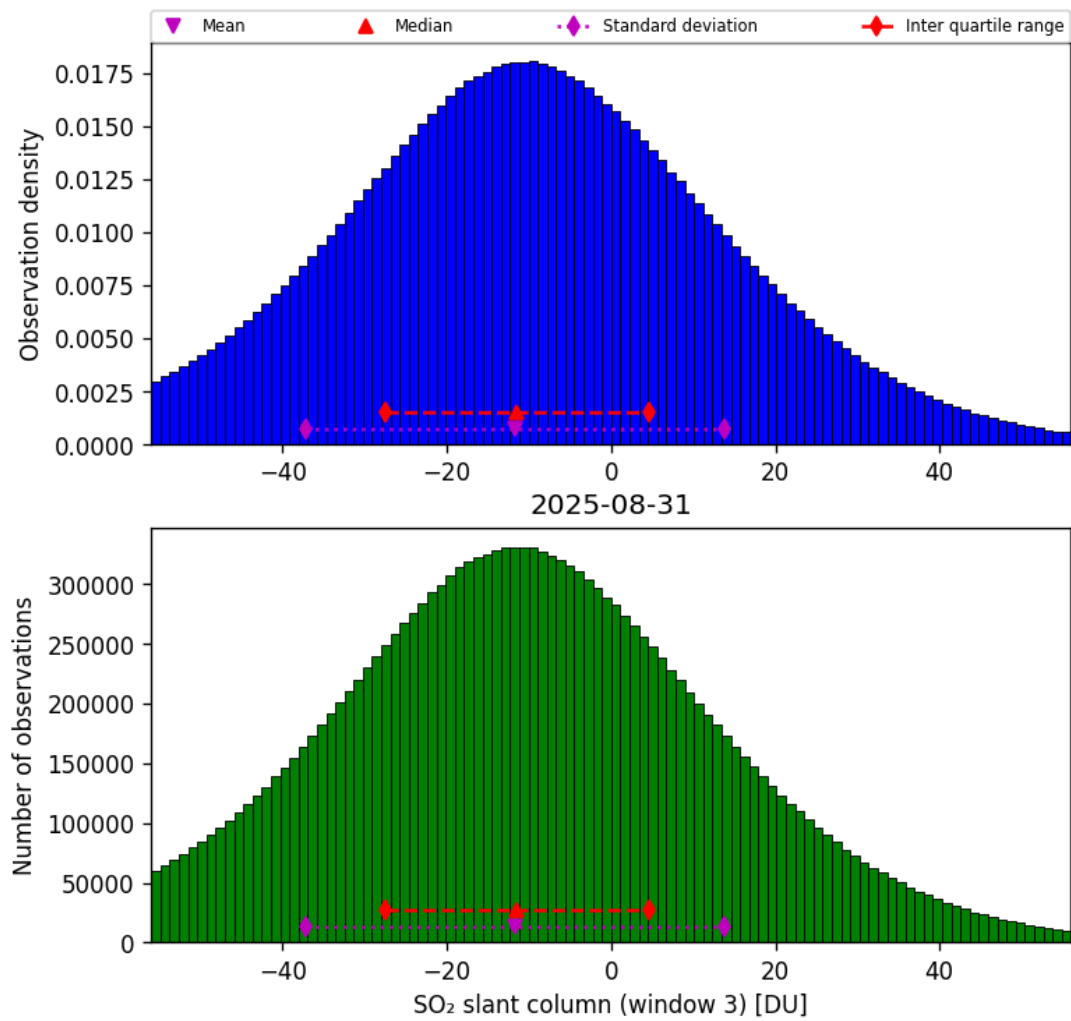
Figure 71: Histogram of “SO 2 slant column (window 3)” for 2025-08-31 to 2025-09-01
