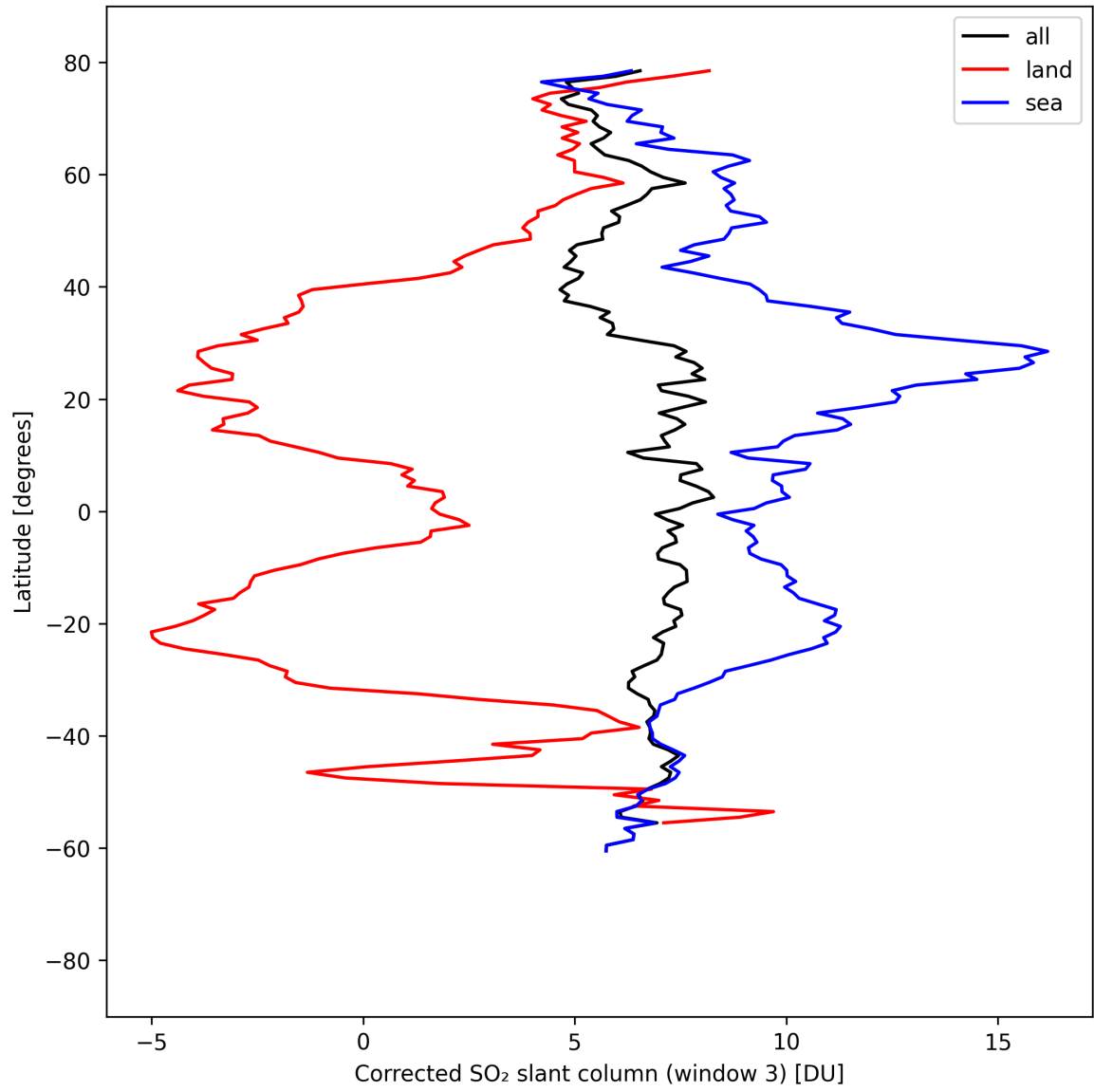
Figure 46: Zonal average of “Corrected SO 2 slant column (window 3)” for 2025-08-31 to 2025-09-01.
