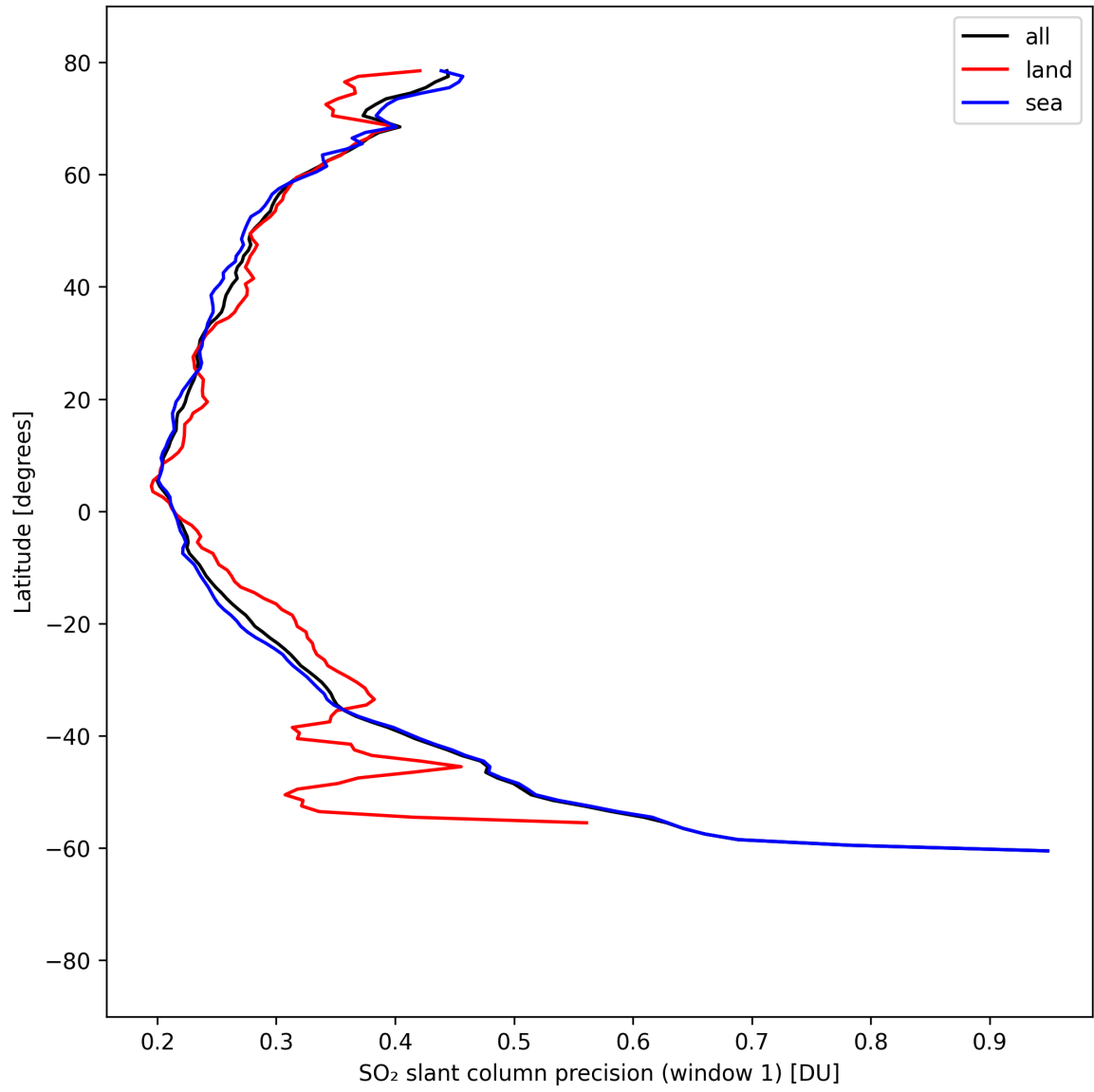
Figure 37: Zonal average of “SO 2 slant column precision (window 1)” for 2025-08-31 to 2025-09-01.
