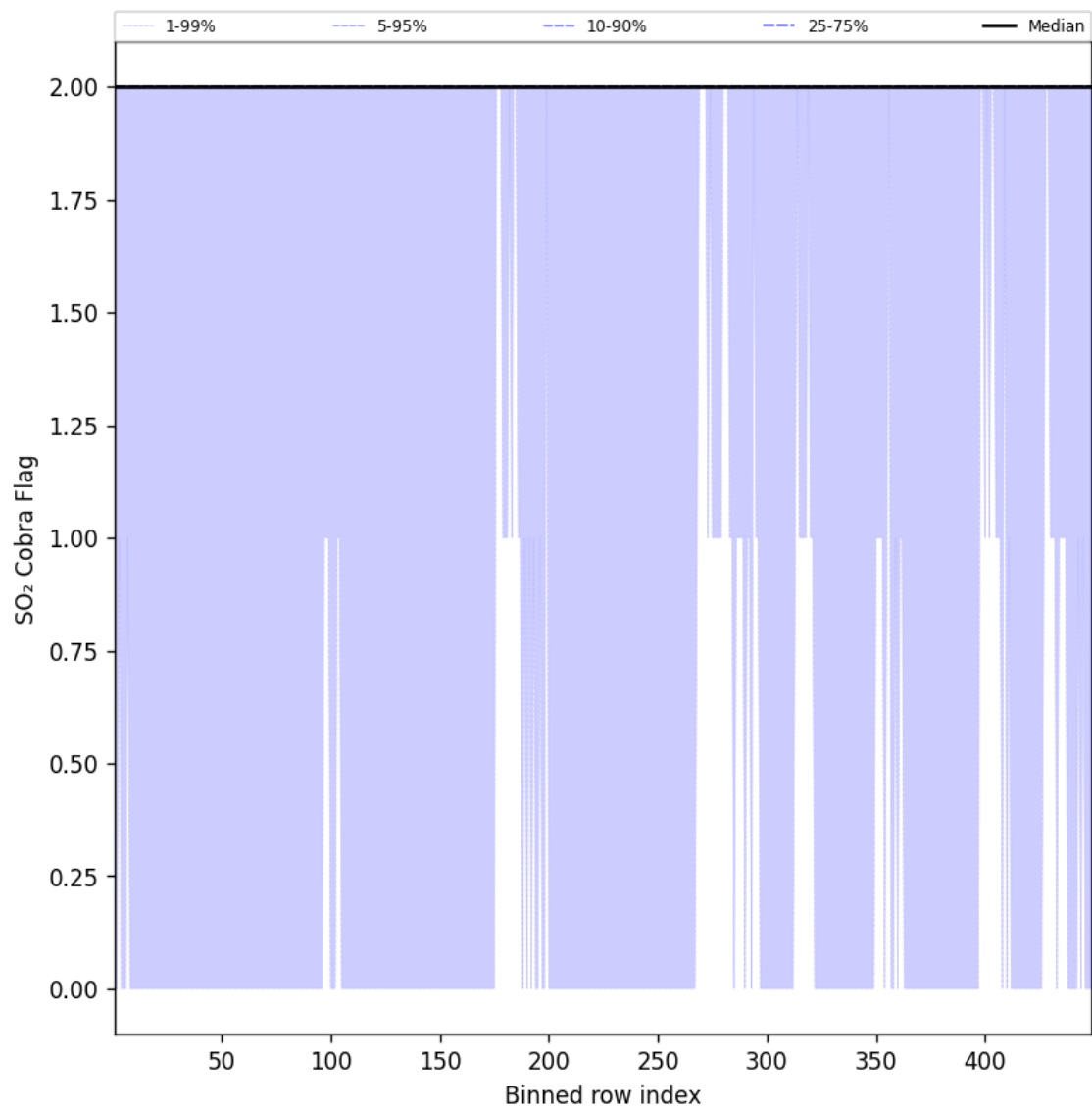
Figure 102: Along track statistics of “SO 2 Cobra Flag” for 2025-08-31 to 2025-09-01
