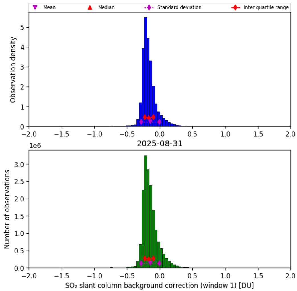
Figure 66: Histogram of “SO 2 slant column background correction (window 1)” for 2025-08-31 to 2025-09-01
