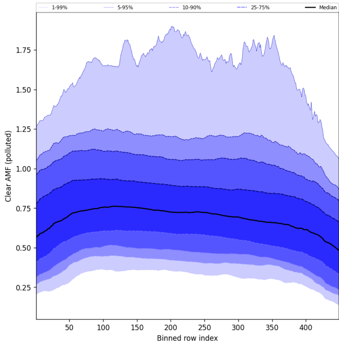
Figure 109: Along track statistics of “Clear AMF (polluted)” for 2025-08-31 to 2025-09-01
