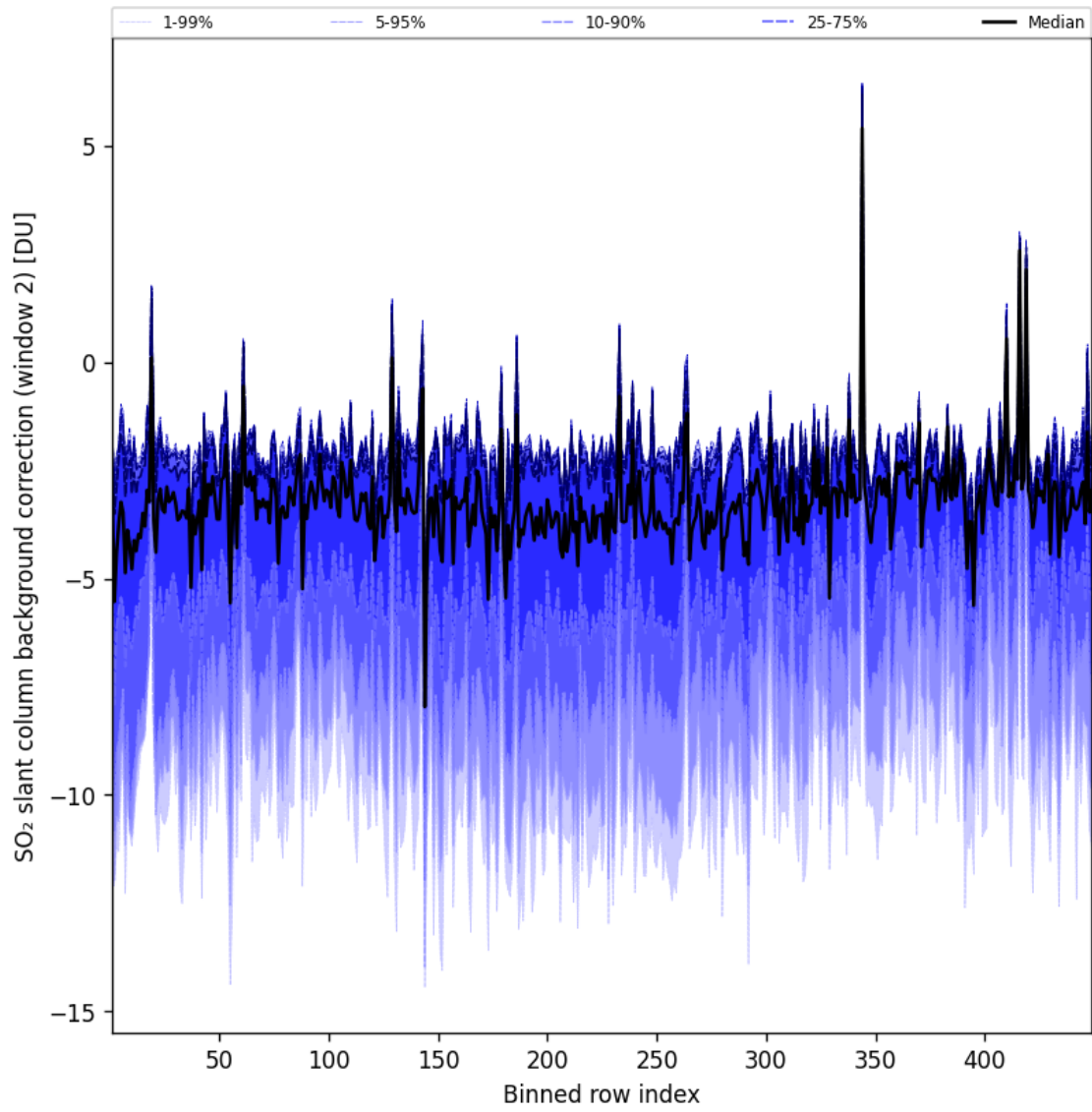
Figure 97: Along track statistics of “SO 2 slant column background correction (window 2)” for 2025-08-31 to 2025-09-01
