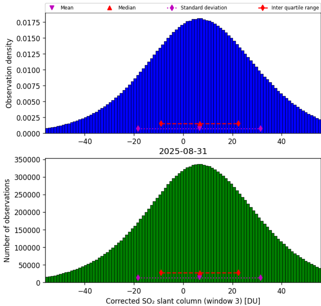
Figure 73: Histogram of “Corrected SO 2 slant column (window 3)” for 2025-08-31 to 2025-09-01
