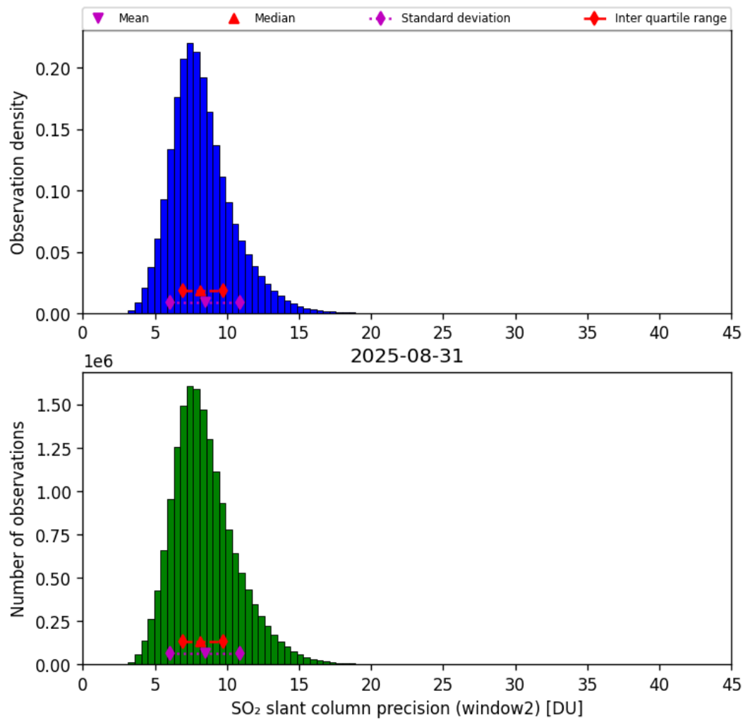
Figure 68: Histogram of “SO 2 slant column precision (window2)” for 2025-08-31 to 2025-09-01
