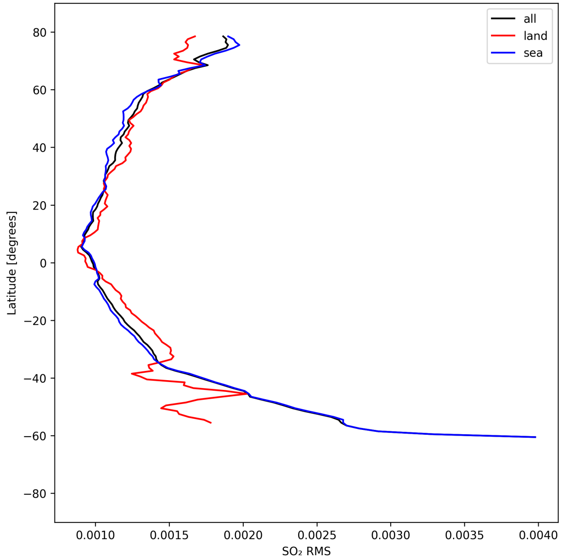
Figure 52: Zonal average of “SO 2 RMS” for 2025-08-31 to 2025-09-01.
