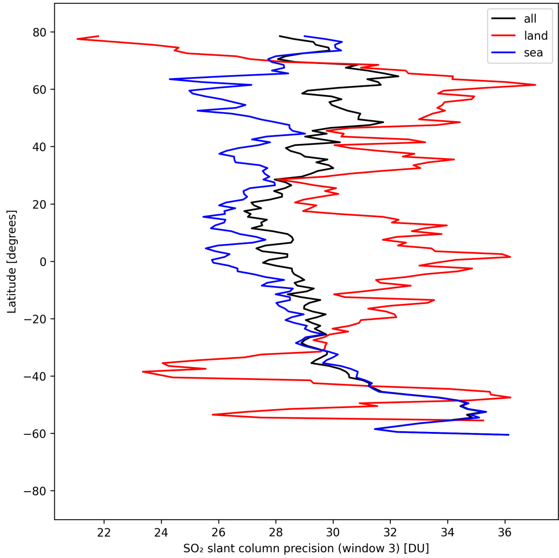
Figure 45: Zonal average of “SO 2 slant column precision (window 3)” for 2025-08-31 to 2025-09-01.
