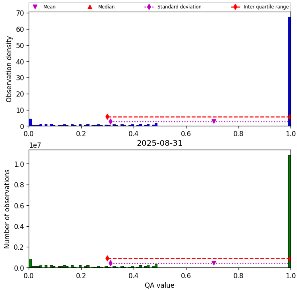
Figure 57: Histogram of “QA value” for 2025-08-31 to 2025-09-01
