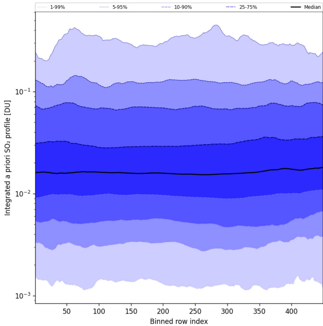
Figure 103: Along track statistics of “Integrated a priori SO 2 profile” for 2025-08-31 to 2025-09-01
