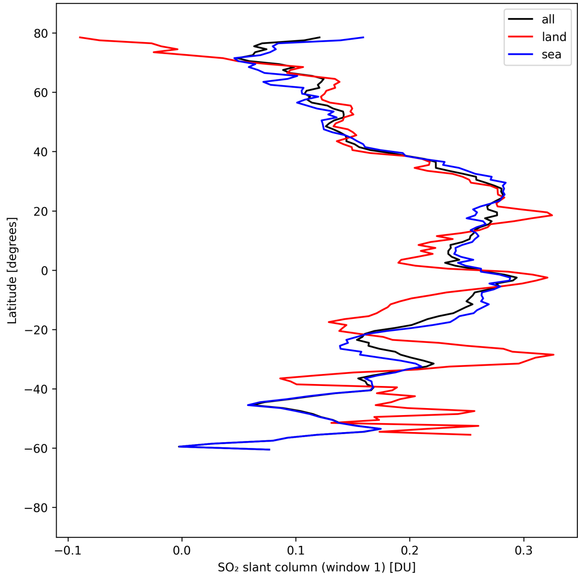
Figure 36: Zonal average of “SO 2 slant column (window 1)” for 2025-08-31 to 2025-09-01.
