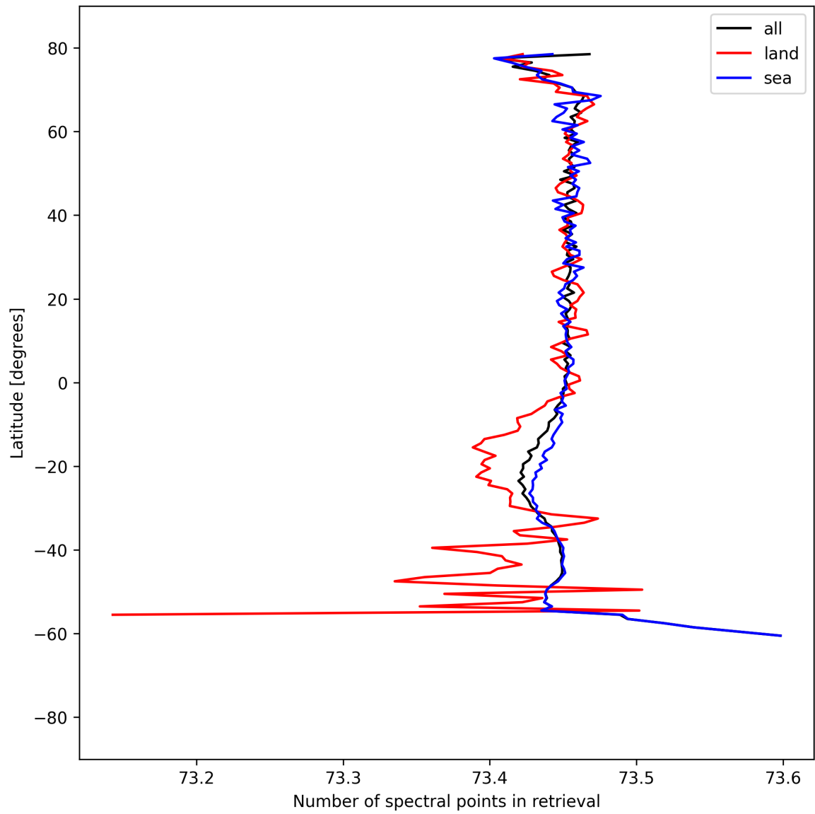
Figure 56: Zonal average of “Number of spectral points in retrieval” for 2025-08-31 to 2025-09-01.
