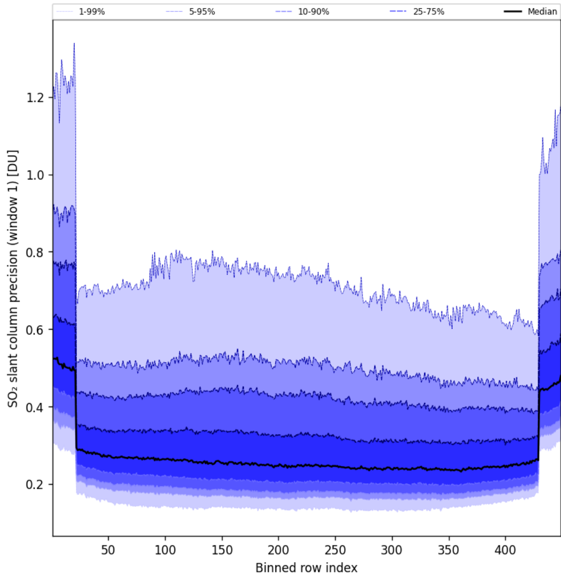
Figure 91: Along track statistics of "SO 2 slant column precision (window 1)" for 2025-08-31 to 2025-09-01
