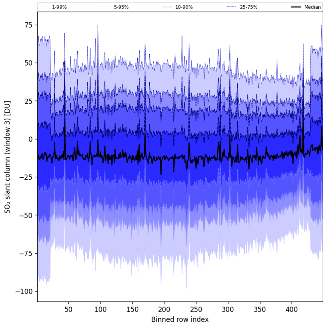
Figure 98: Along track statistics of “SO 2 slant column (window 3)” for 2025-08-31 to 2025-09-01
