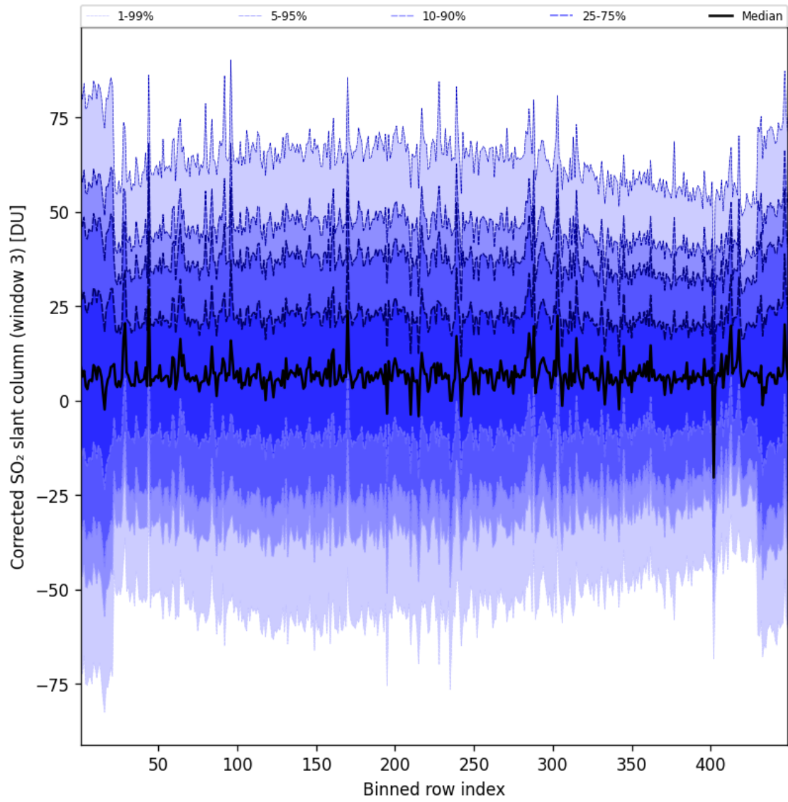
Figure 100: Along track statistics of “Corrected SO 2 slant column (window 3)” for 2025-08-31 to 2025-09-01
