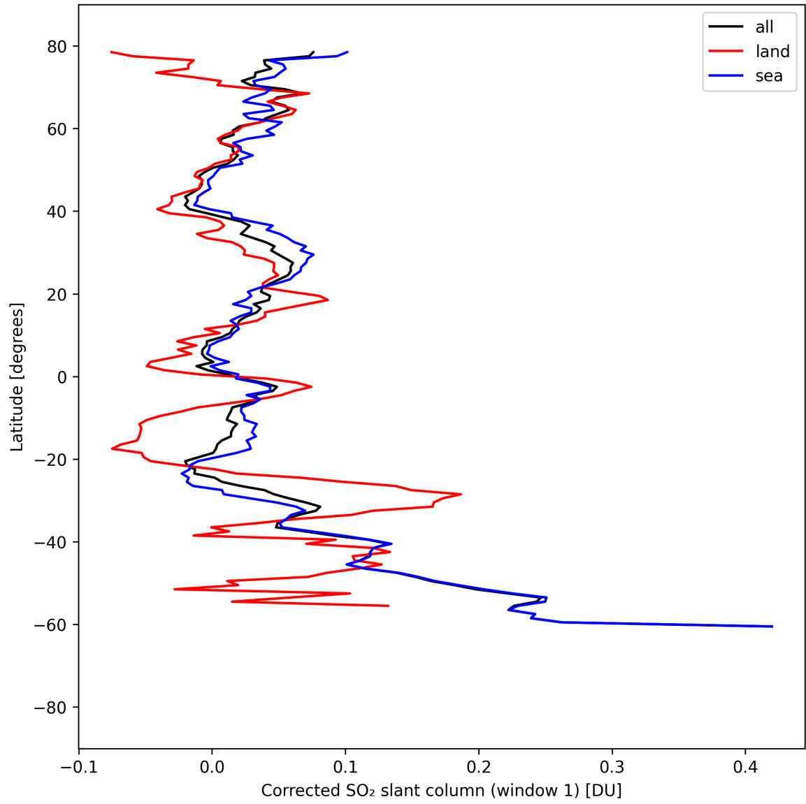
Figure 38: Zonal average of “Corrected SO 2 slant column (window 1)” for 2025-08-31 to 2025-09-01.
