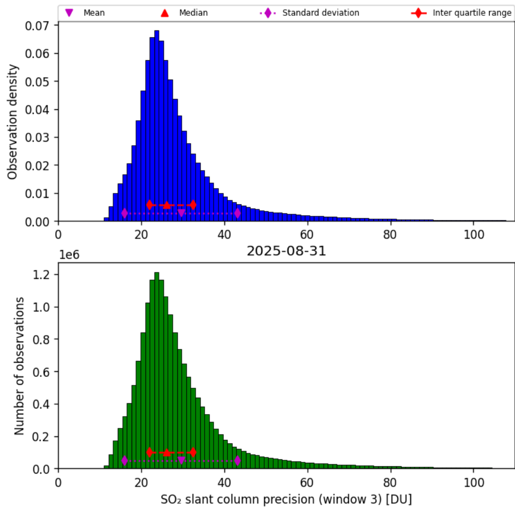
Figure 72: Histogram of “SO 2 slant column precision (window 3)” for 2025-08-31 to 2025-09-01
