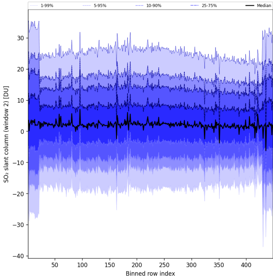
Figure 94: Along track statistics of “SO 2 slant column (window 2)” for 2025-08-31 to 2025-09-01
