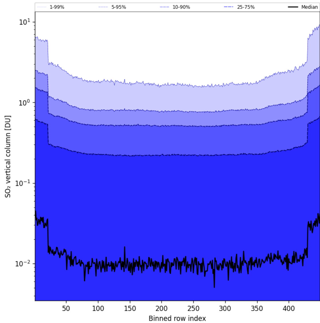
Figure 85: Along track statistics of “SO 2 vertical column” for 2025-08-31 to 2025-09-01
