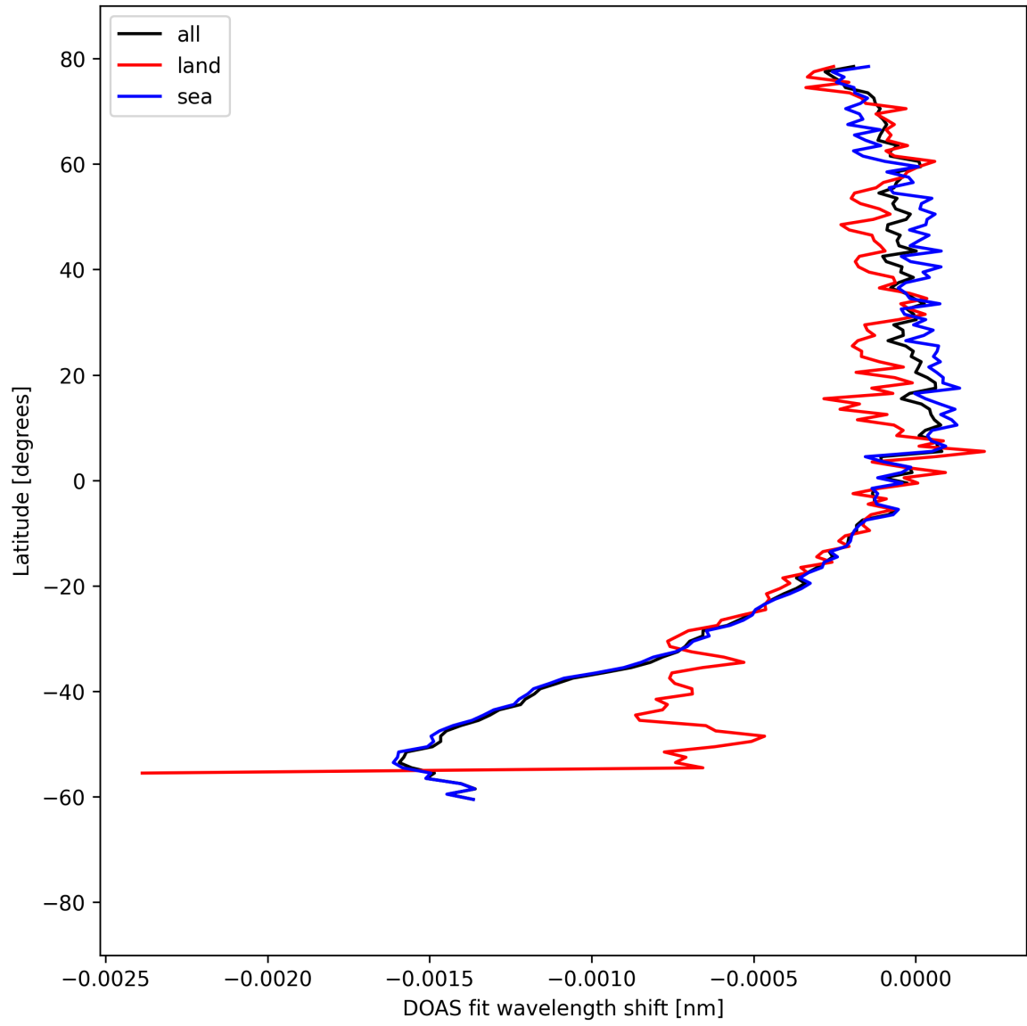
Figure 50: Zonal average of “DOAS fit wavelength shift” for 2025-08-31 to 2025-09-01.
