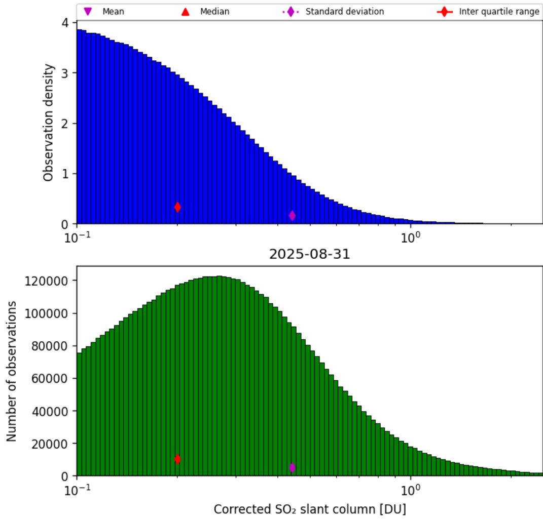
Figure 60: Histogram of “Corrected SO 2 slant column” for 2025-08-31 to 2025-09-01
