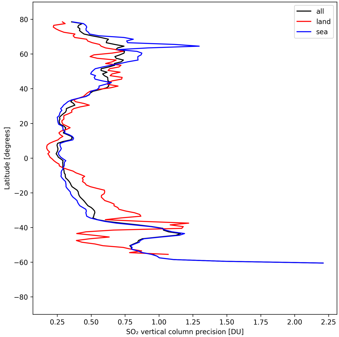
Figure 32: Zonal average of “SO 2 vertical column precision” for 2025-08-31 to 2025-09-01.
