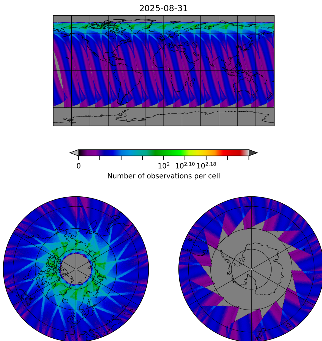
Figure 29: Map of the number of observations for 2025-08-31 to 2025-09-01
