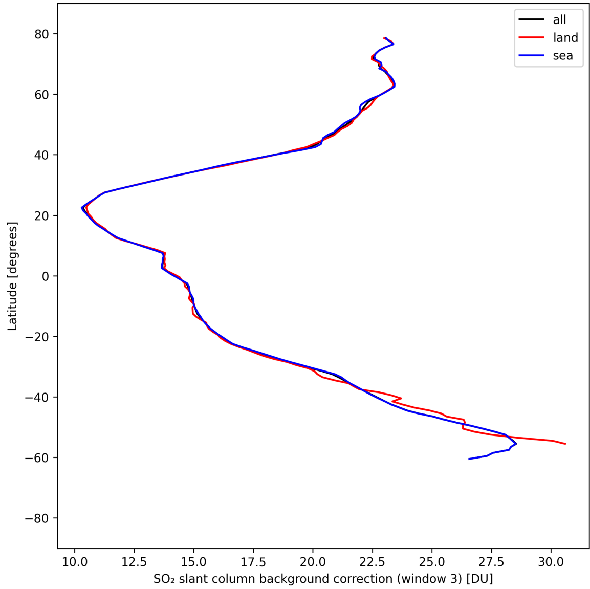
Figure 47: Zonal average of “SO 2 slant column background correction (window 3)” for 2025-08-31 to 2025-09-01.
