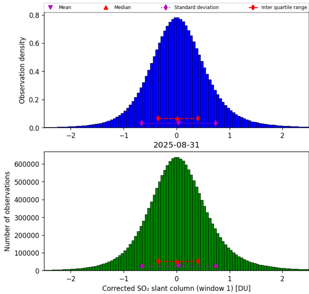
Figure 65: Histogram of “Corrected SO 2 slant column (window 1)” for 2025-08-31 to 2025-09-01
