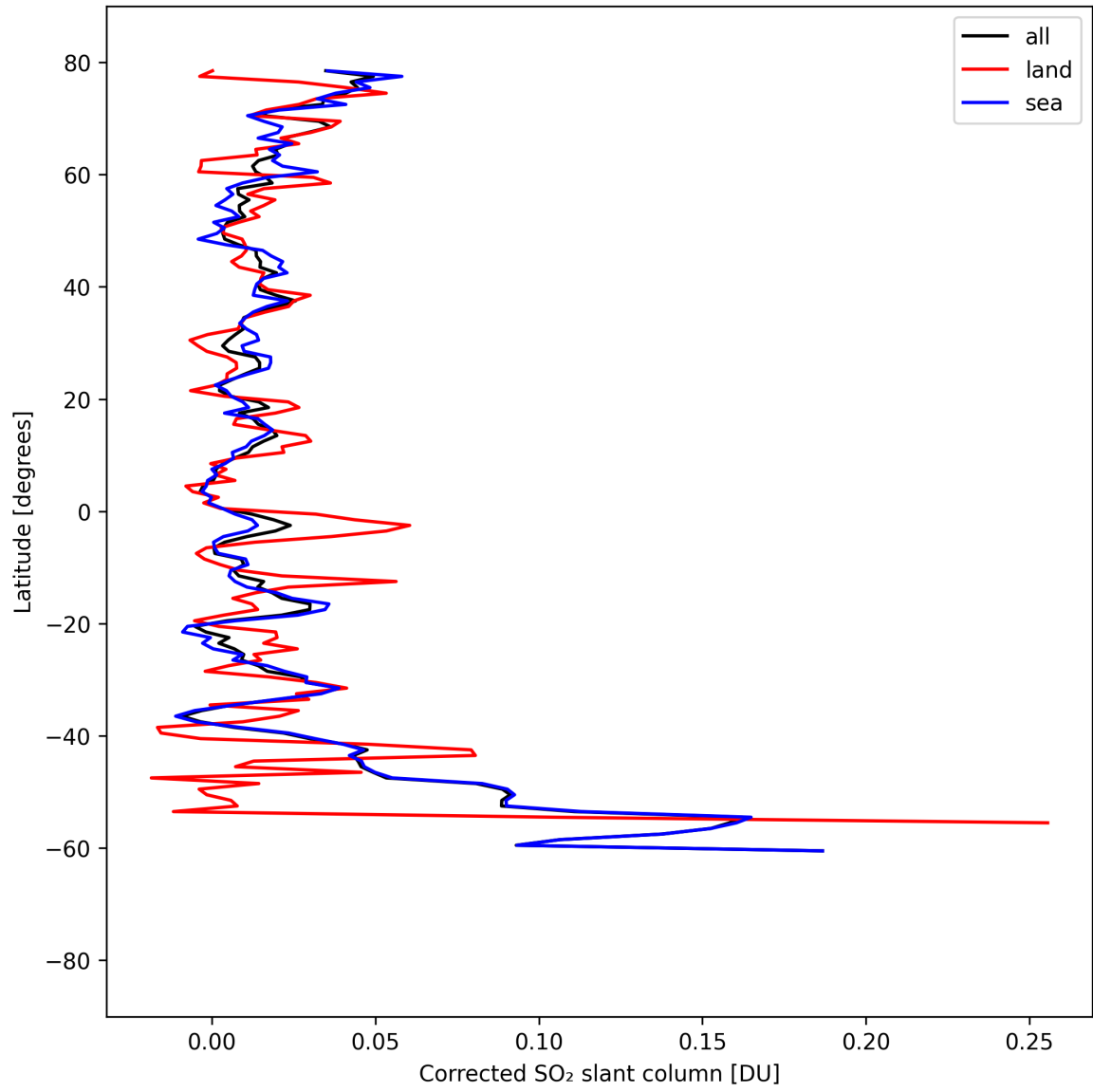
Figure 33: Zonal average of “Corrected SO 2 slant column” for 2025-08-31 to 2025-09-01.
