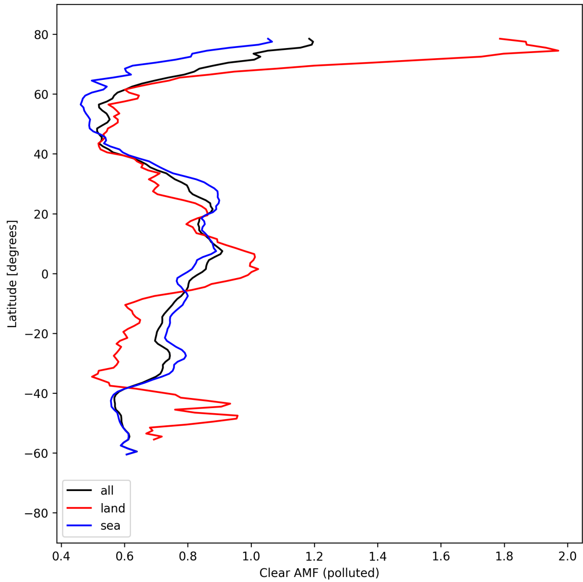
Figure 55: Zonal average of “Clear AMF (polluted)” for 2025-08-31 to 2025-09-01.
