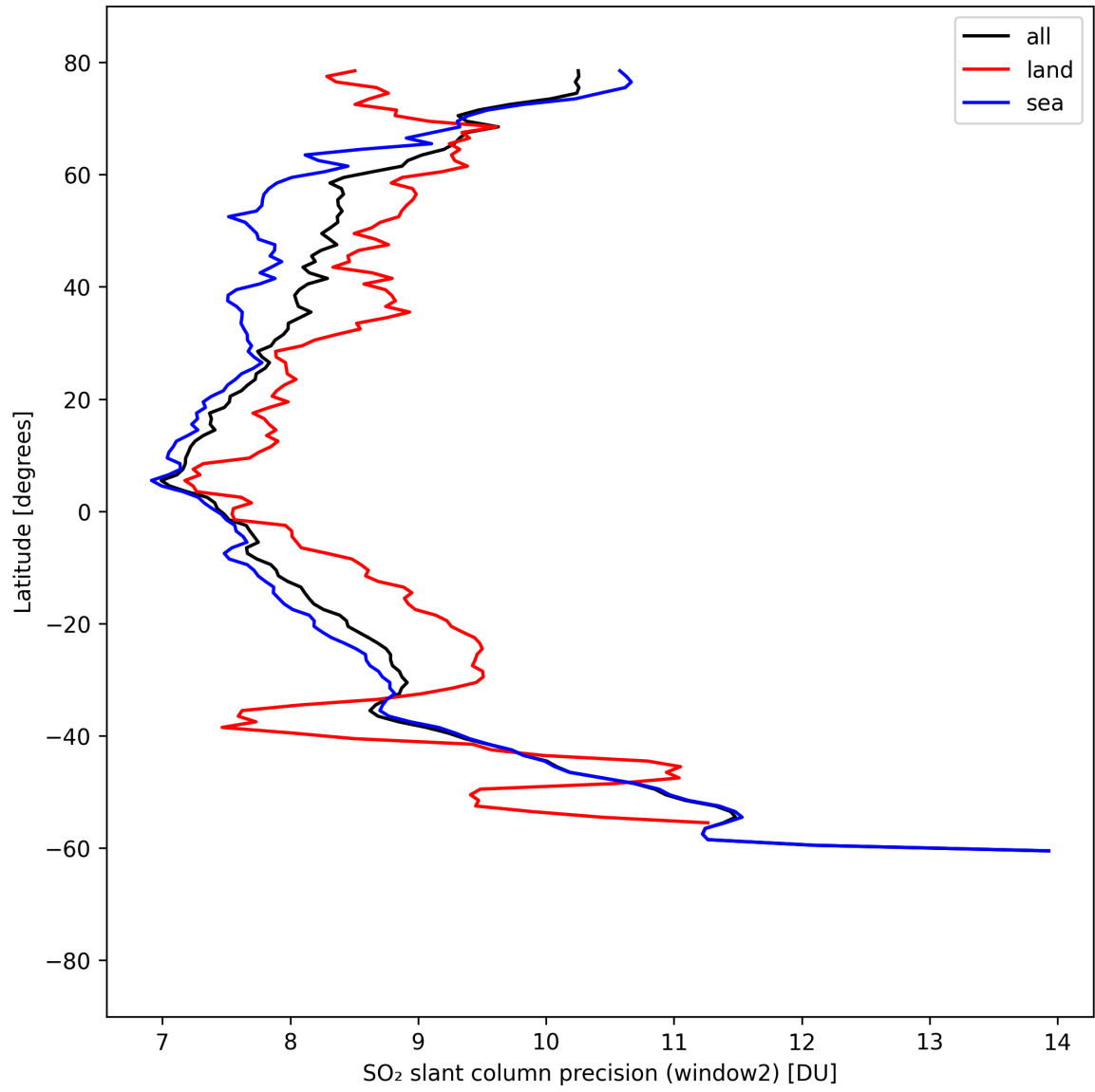
Figure 41: Zonal average of “SO 2 slant column precision (window2)” for 2025-08-31 to 2025-09-01.
