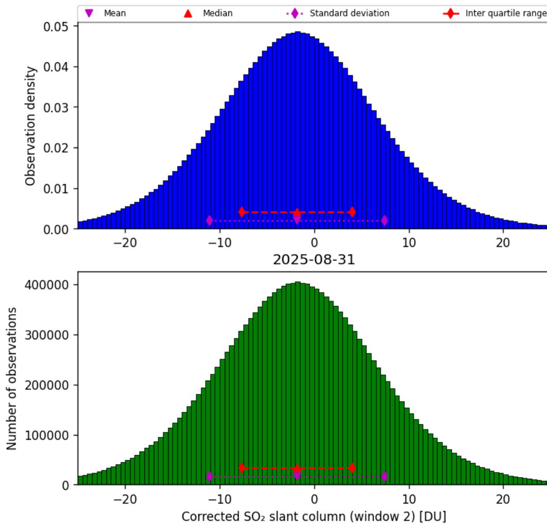
Figure 69: Histogram of “Corrected SO 2 slant column (window 2)” for 2025-08-31 to 2025-09-01
