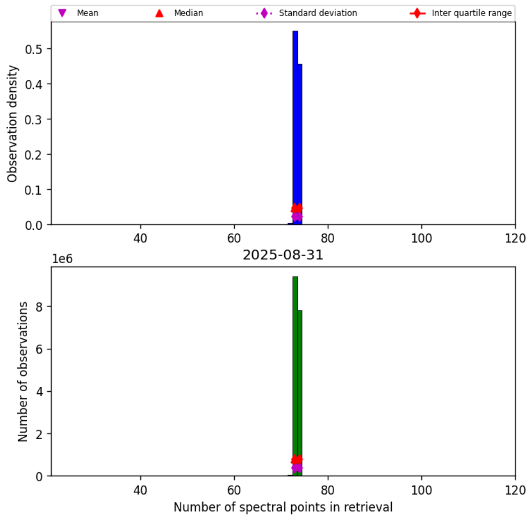
Figure 83: Histogram of “Number of spectral points in retrieval” for 2025-08-31 to 2025-09-01
