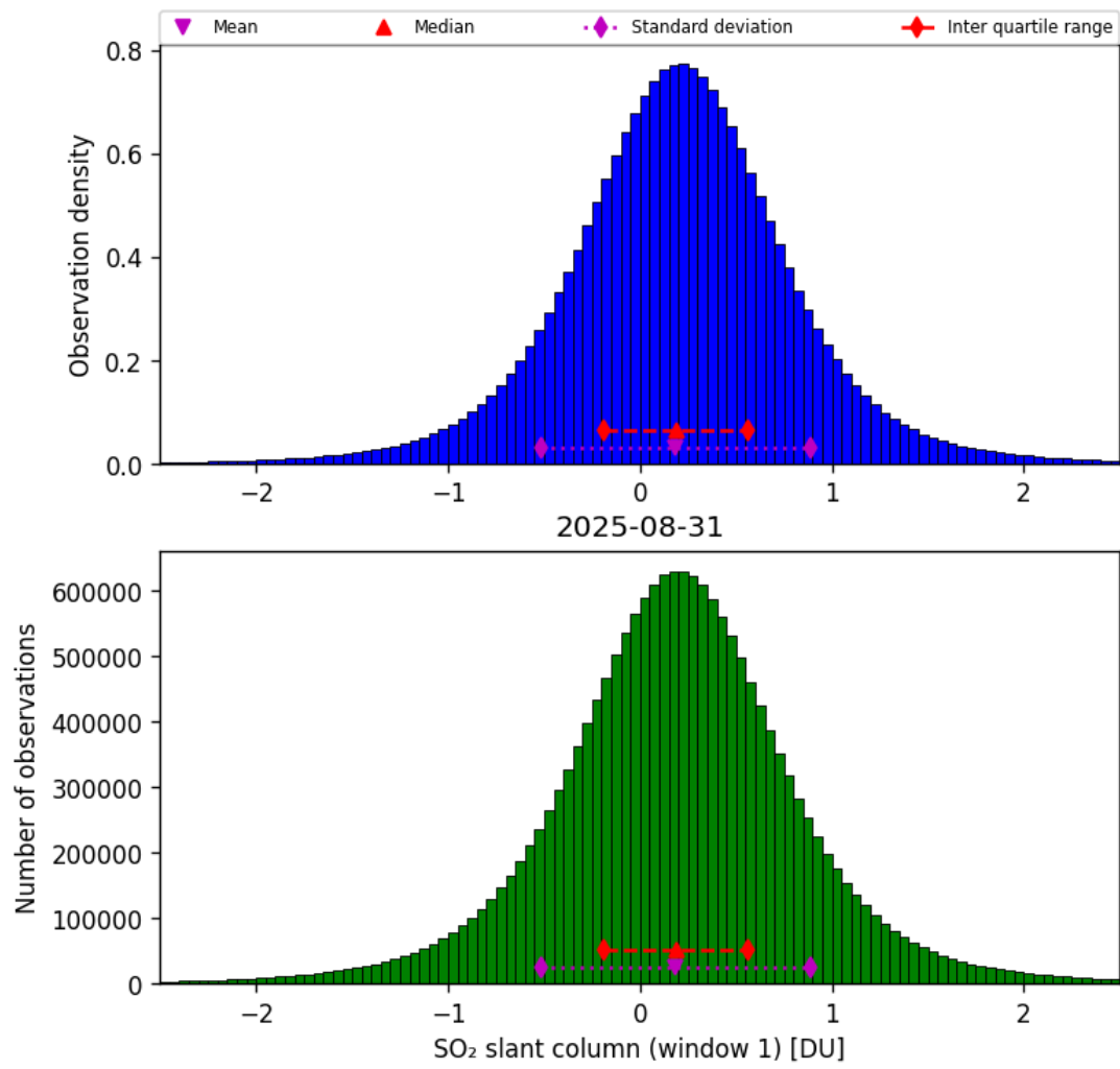
Figure 63: Histogram of “SO 2 slant column (window 1)” for 2025-08-31 to 2025-09-01
