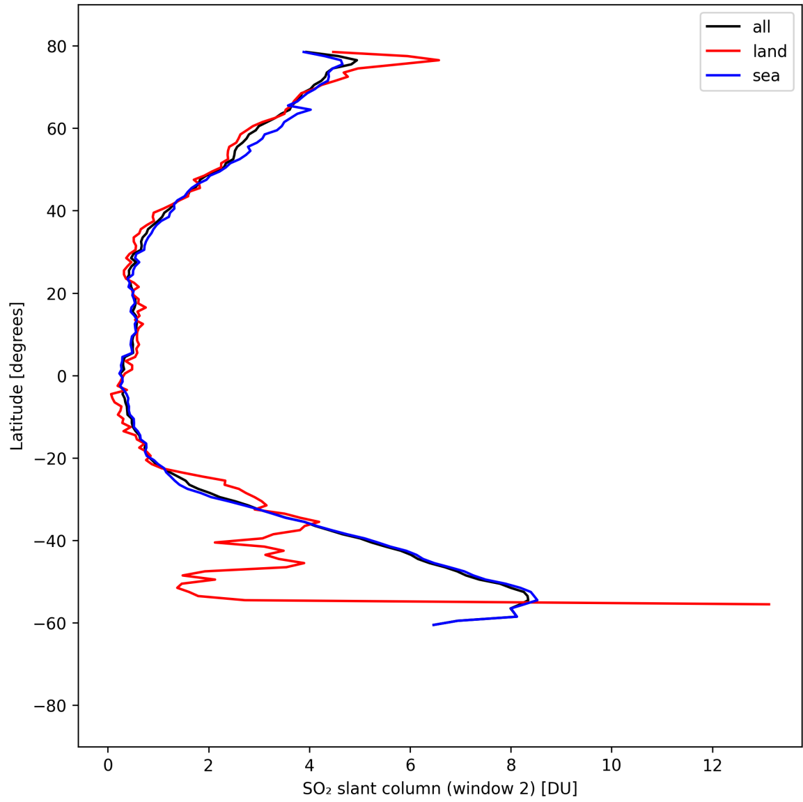
Figure 40: Zonal average of “SO 2 slant column (window 2)” for 2025-08-31 to 2025-09-01.
