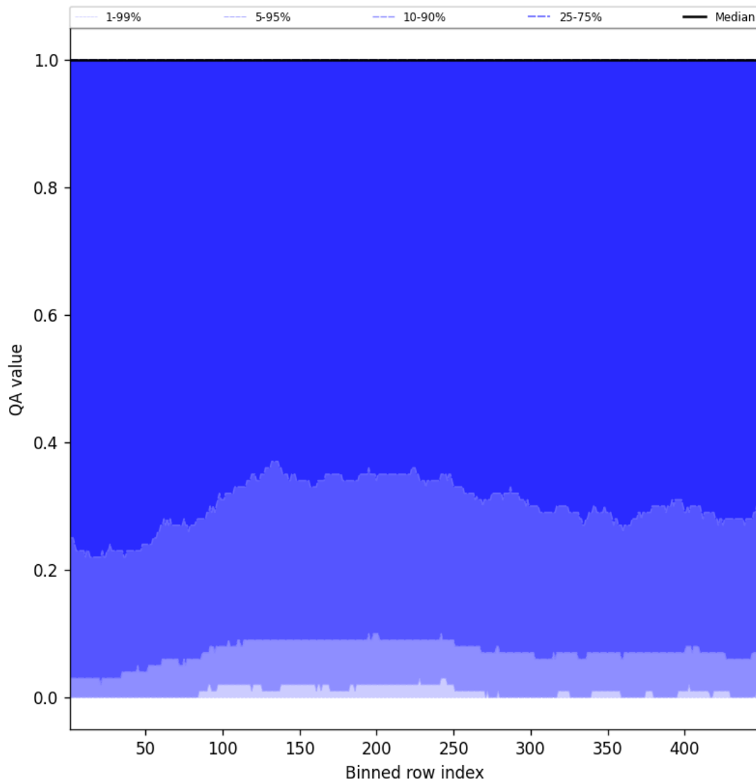
Figure 84: Along track statistics of “QA value” for 2025-08-31 to 2025-09-01
