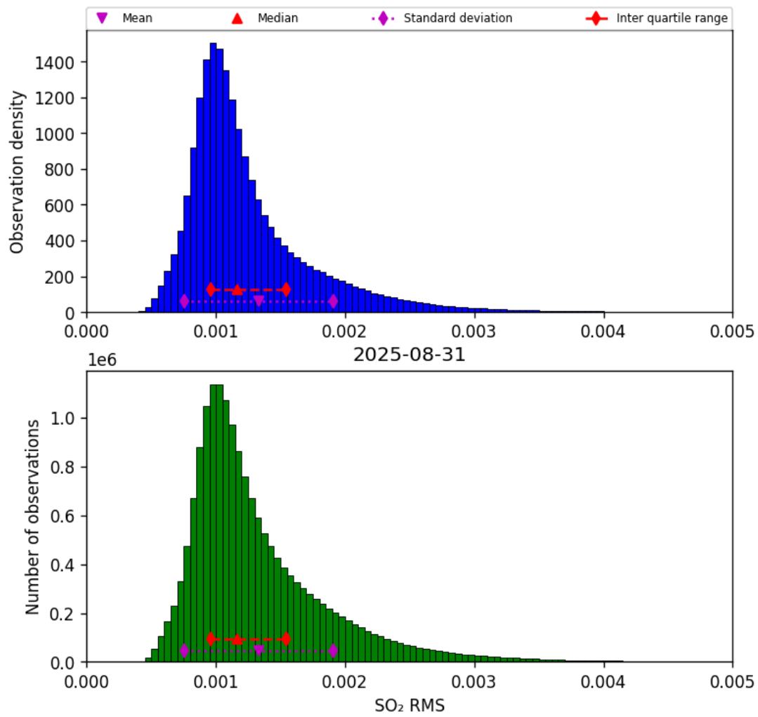
Figure 79: Histogram of “SO 2 RMS” for 2025-08-31 to 2025-09-01
