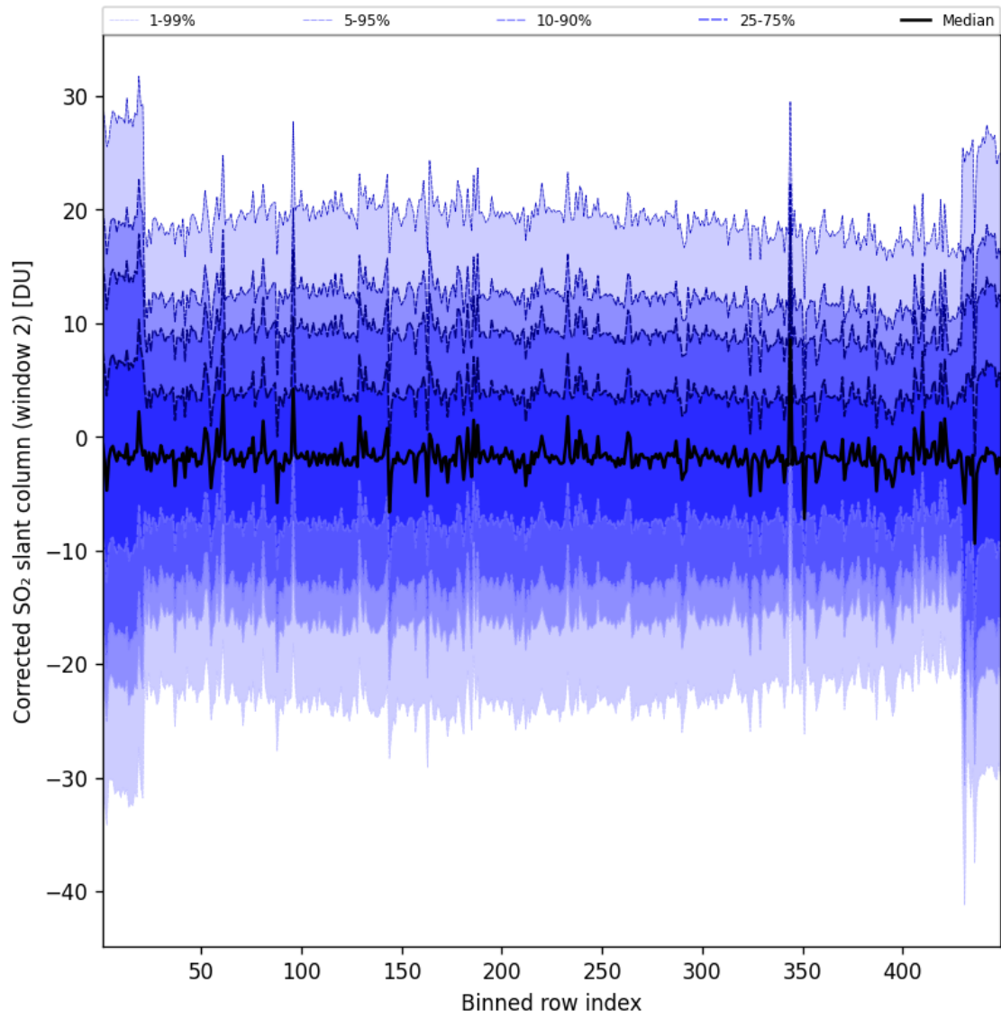
Figure 96: Along track statistics of “Corrected SO 2 slant column (window 2)” for 2025-08-31 to 2025-09-01
