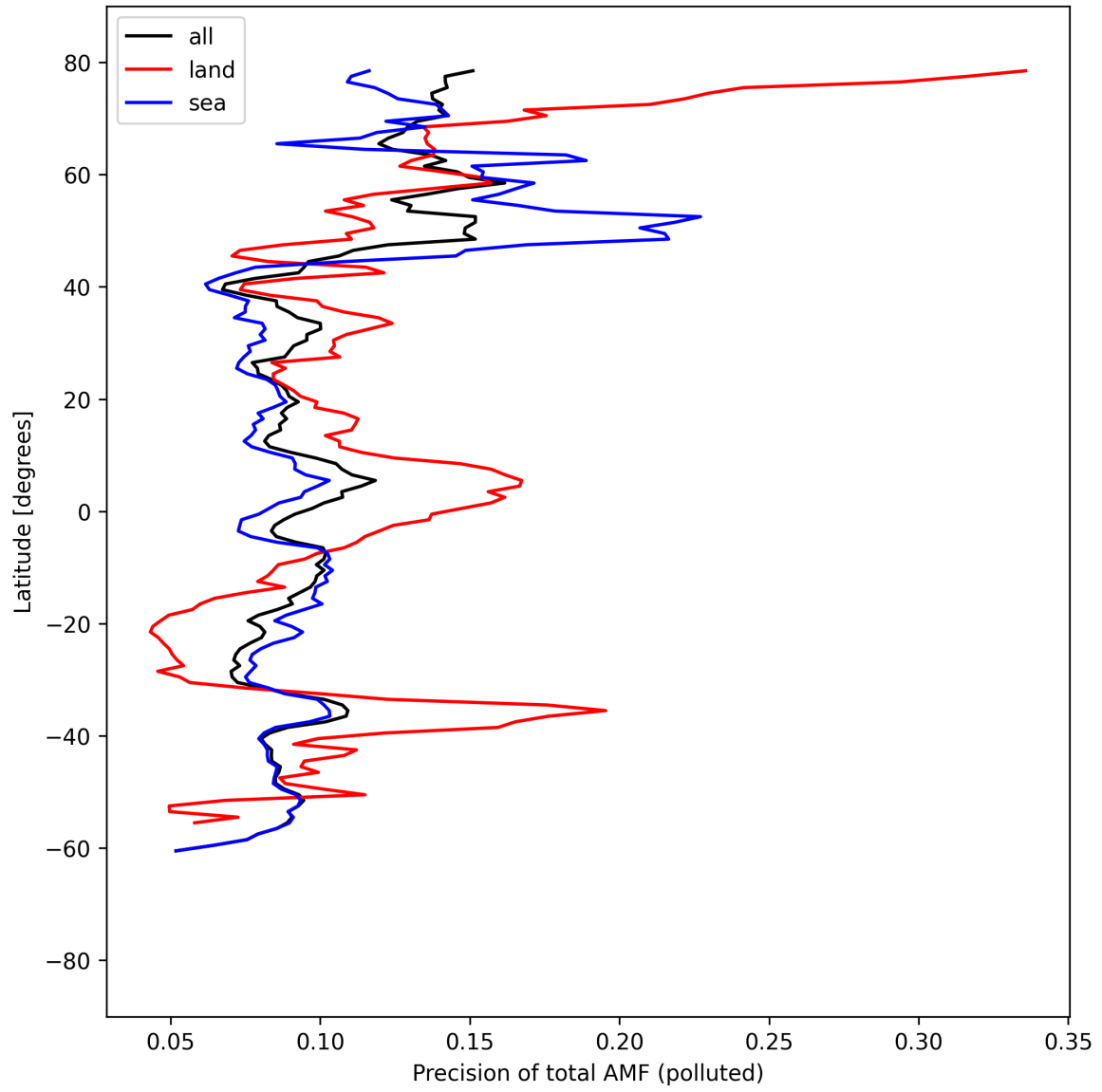
Figure 54: Zonal average of “Precision of total AMF (polluted)” for 2025-08-31 to 2025-09-01.
