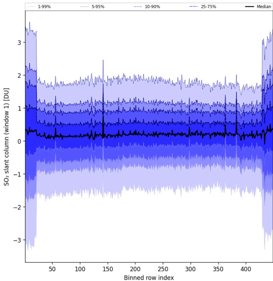
Figure 90: Along track statistics of “SO 2 slant column (window 1)” for 2025-08-31 to 2025-09-01
