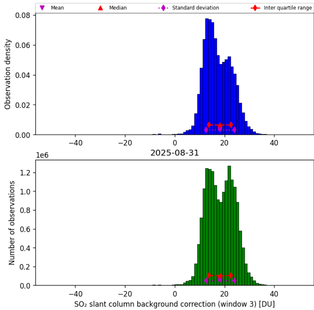
Figure 74: Histogram of “SO 2 slant column background correction (window 3)” for 2025-08-31 to 2025-09-01
