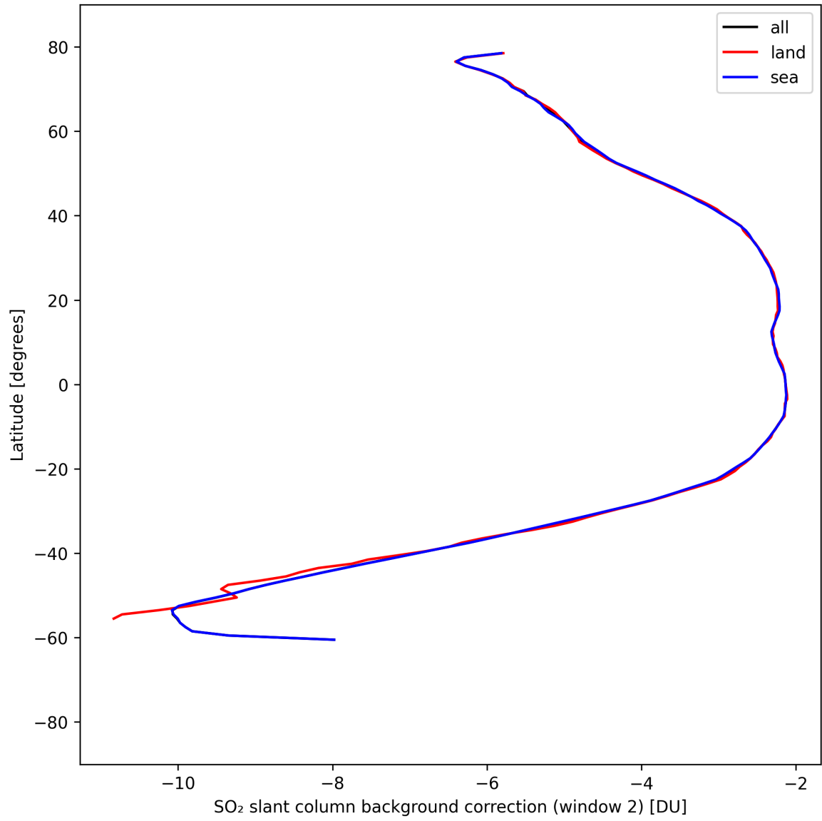
Figure 43: Zonal average of “SO 2 slant column background correction (window 2)” for 2025-08-31 to 2025-09-01.
