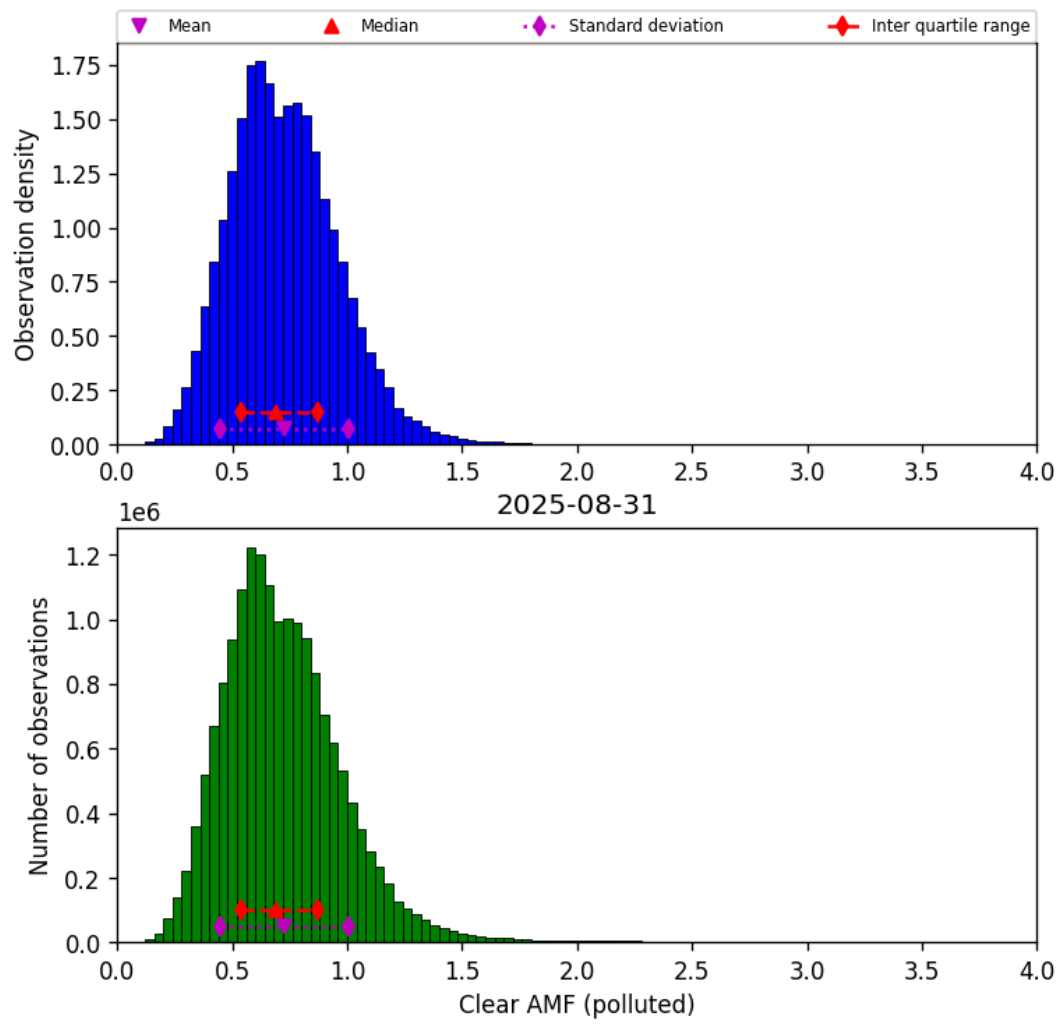
Figure 82: Histogram of “Clear AMF (polluted)” for 2025-08-31 to 2025-09-01
