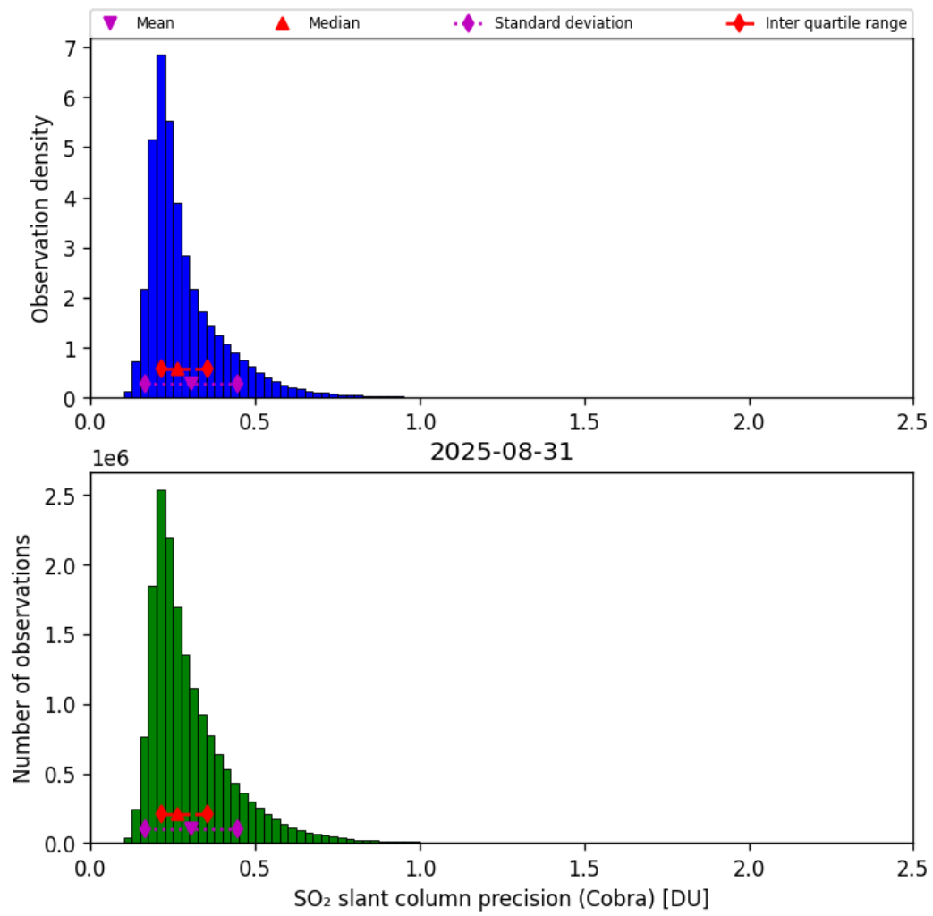
Figure 62: Histogram of “SO 2 slant column precision (Cobra)” for 2025-08-31 to 2025-09-01
