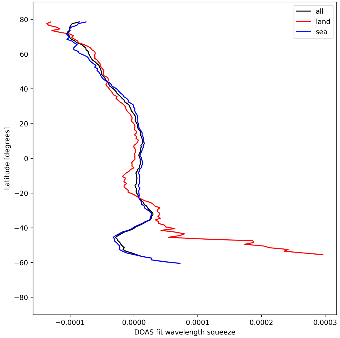
Figure 51: Zonal average of “DOAS fit wavelength squeeze” for 2025-08-31 to 2025-09-01.
