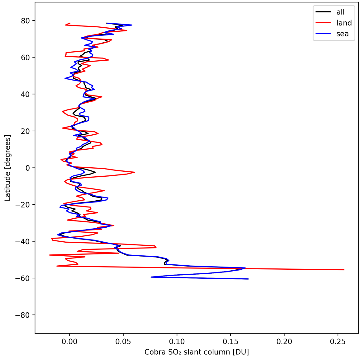
Figure 34: Zonal average of “Cobra SO 2 slant column” for 2025-08-31 to 2025-09-01.
