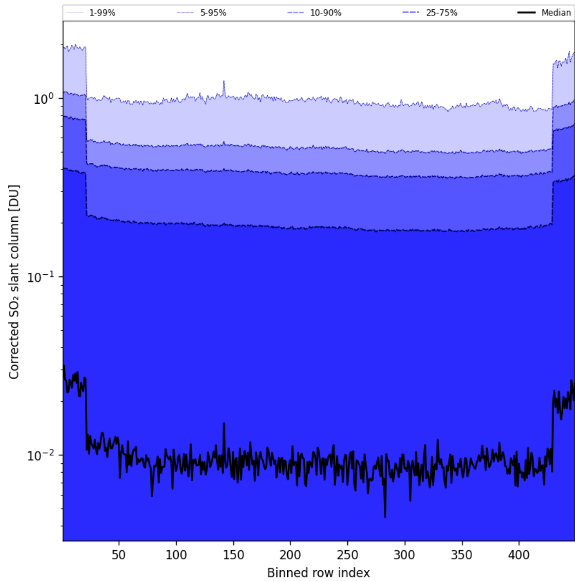
Figure 87: Along track statistics of “Corrected SO 2 slant column” for 2025-08-31 to 2025-09-01
