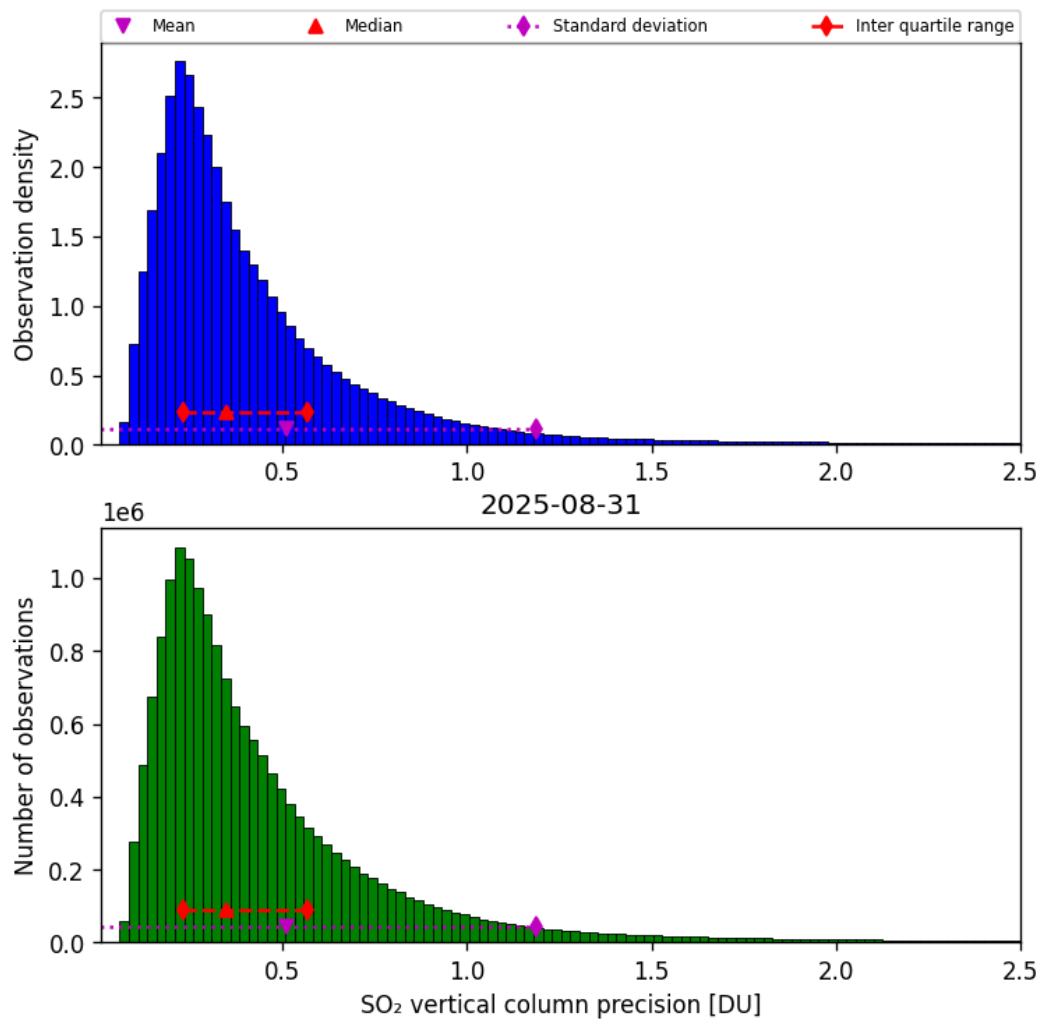
Figure 59: Histogram of “SO 2 vertical column precision” for 2025-08-31 to 2025-09-01
