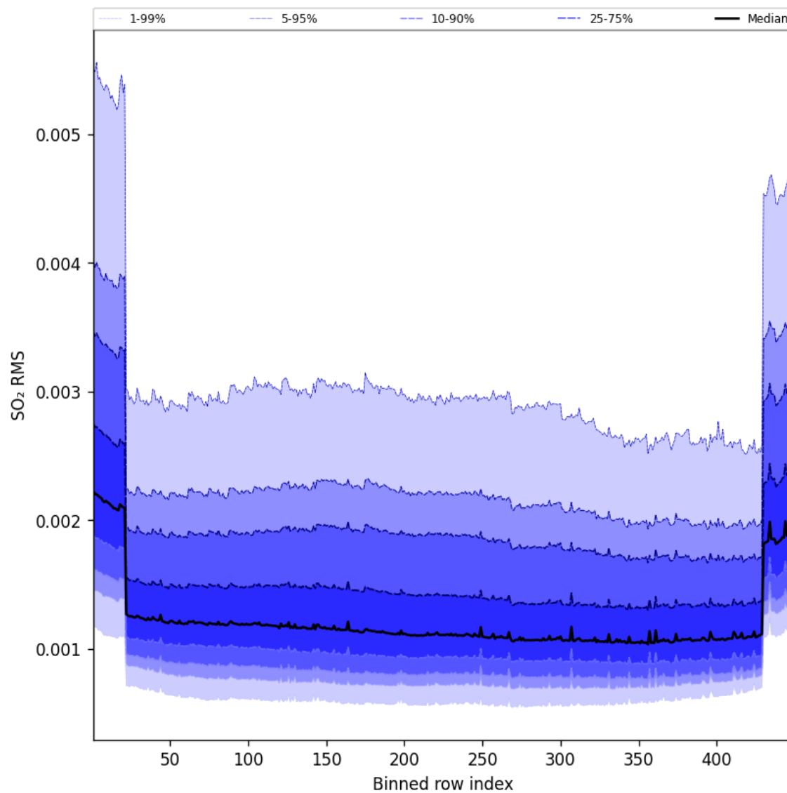
Figure 106: Along track statistics of “SO 2 RMS” for 2025-08-31 to 2025-09-01
