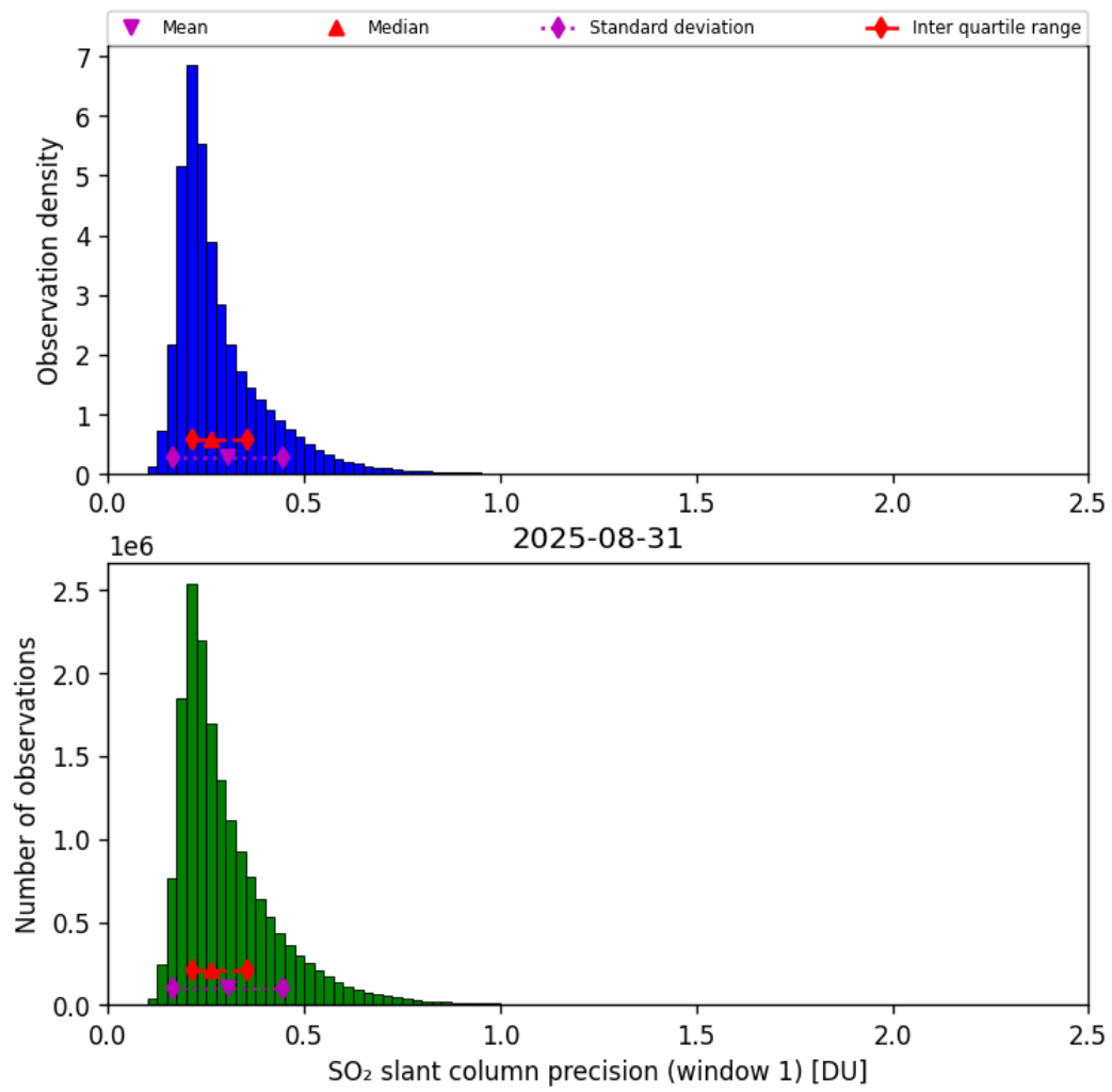
Figure 64: Histogram of “SO 2 slant column precision (window 1)” for 2025-08-31 to 2025-09-01
