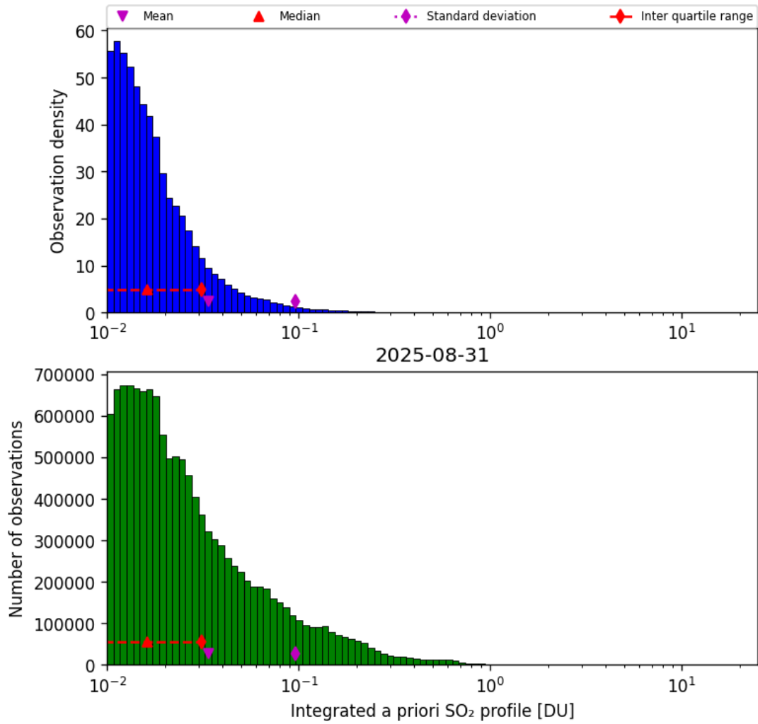
Figure 76: Histogram of “Integrated a priori SO 2 profile” for 2025-08-31 to 2025-09-01
