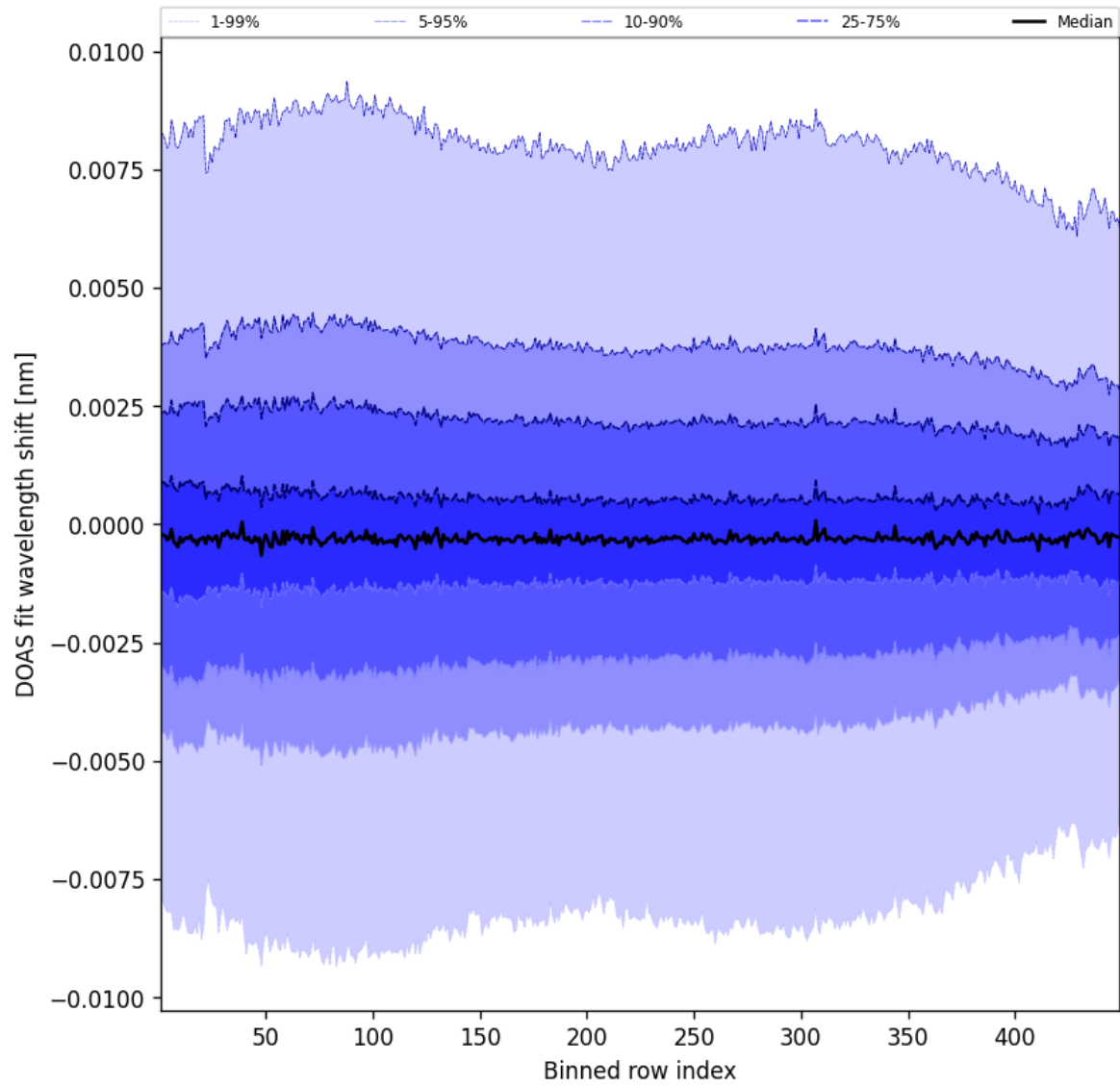
Figure 104: Along track statistics of “DOAS fit wavelength shift” for 2025-08-31 to 2025-09-01
