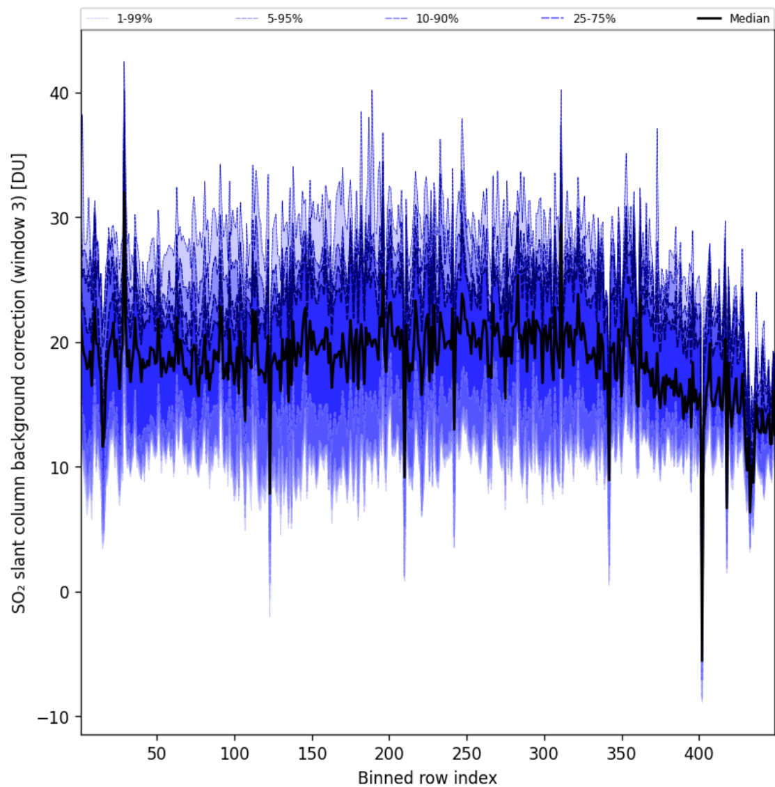
Figure 101: Along track statistics of “SO 2 slant column background correction (window 3)” for 2025-08-31 to 2025-09-01
