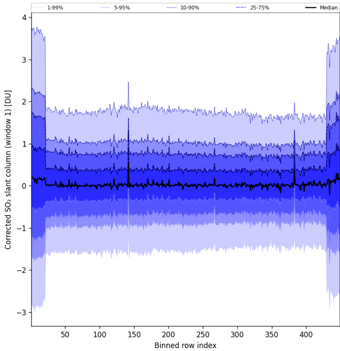
Figure 92: Along track statistics of “Corrected SO 2 slant column (window 1)” for 2025-08-31 to 2025-09-01
