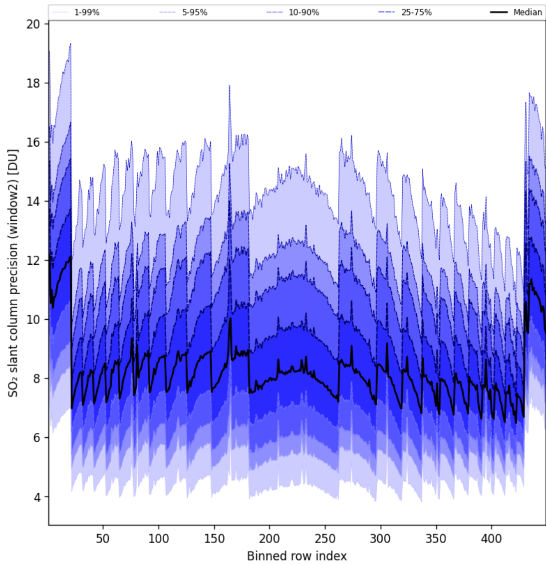
Figure 95: Along track statistics of “SO 2 slant column precision (window2)” for 2025-08-31 to 2025-09-01
