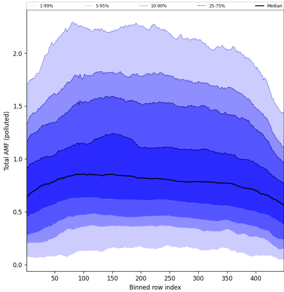
Figure 107: Along track statistics of “Total AMF (polluted)” for 2025-08-31 to 2025-09-01
