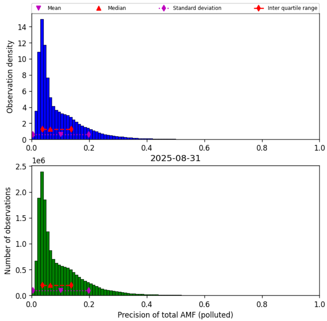
Figure 81: Histogram of “Precision of total AMF (polluted)” for 2025-08-31 to 2025-09-01
