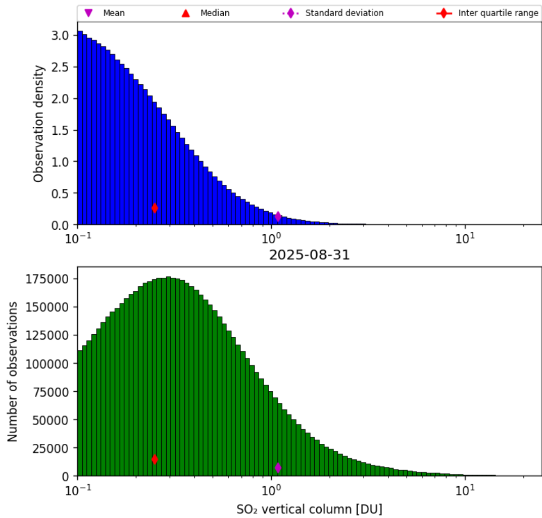
Figure 58: Histogram of “SO 2 vertical column” for 2025-08-31 to 2025-09-01
