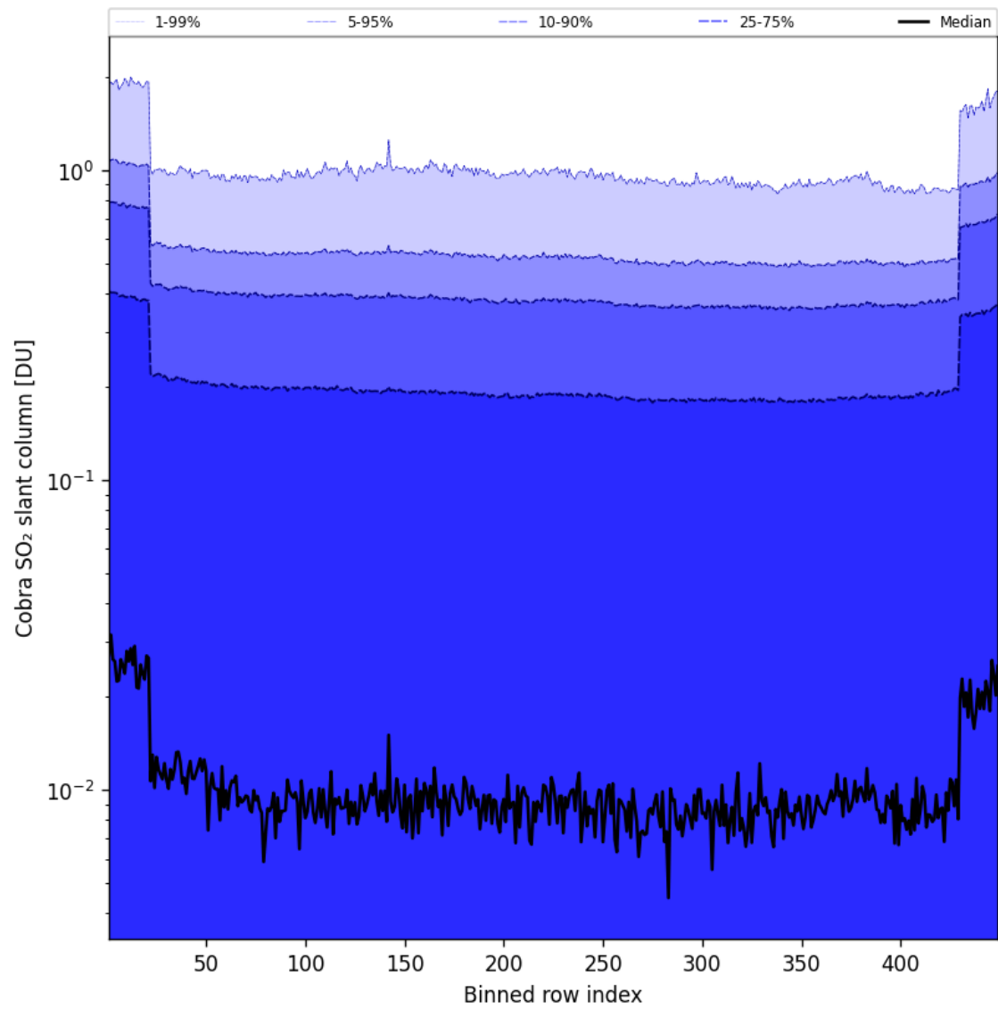
Figure 88: Along track statistics of “Cobra SO 2 slant column” for 2025-08-31 to 2025-09-01
