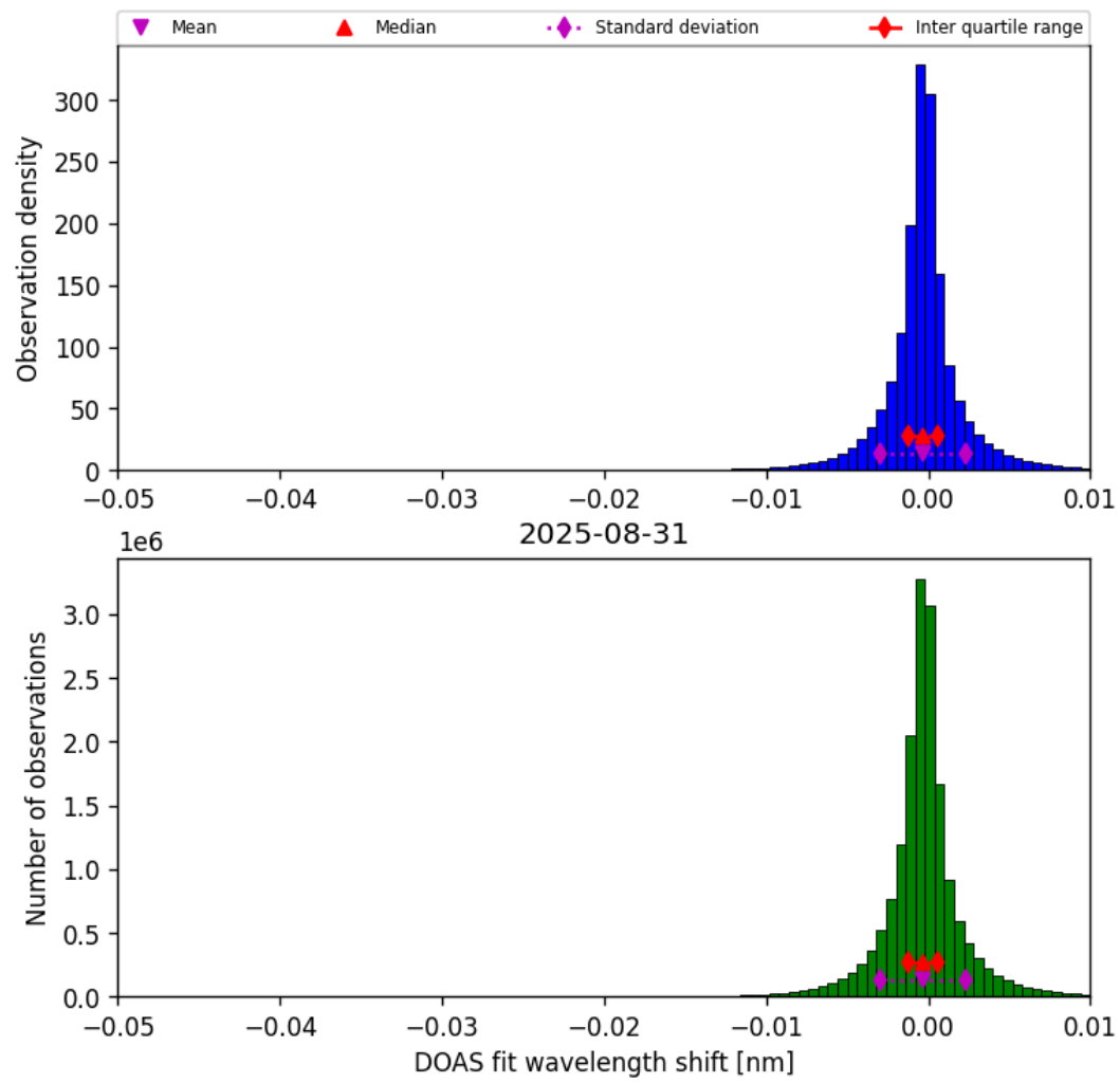
Figure 77: Histogram of “DOAS fit wavelength shift” for 2025-08-31 to 2025-09-01
