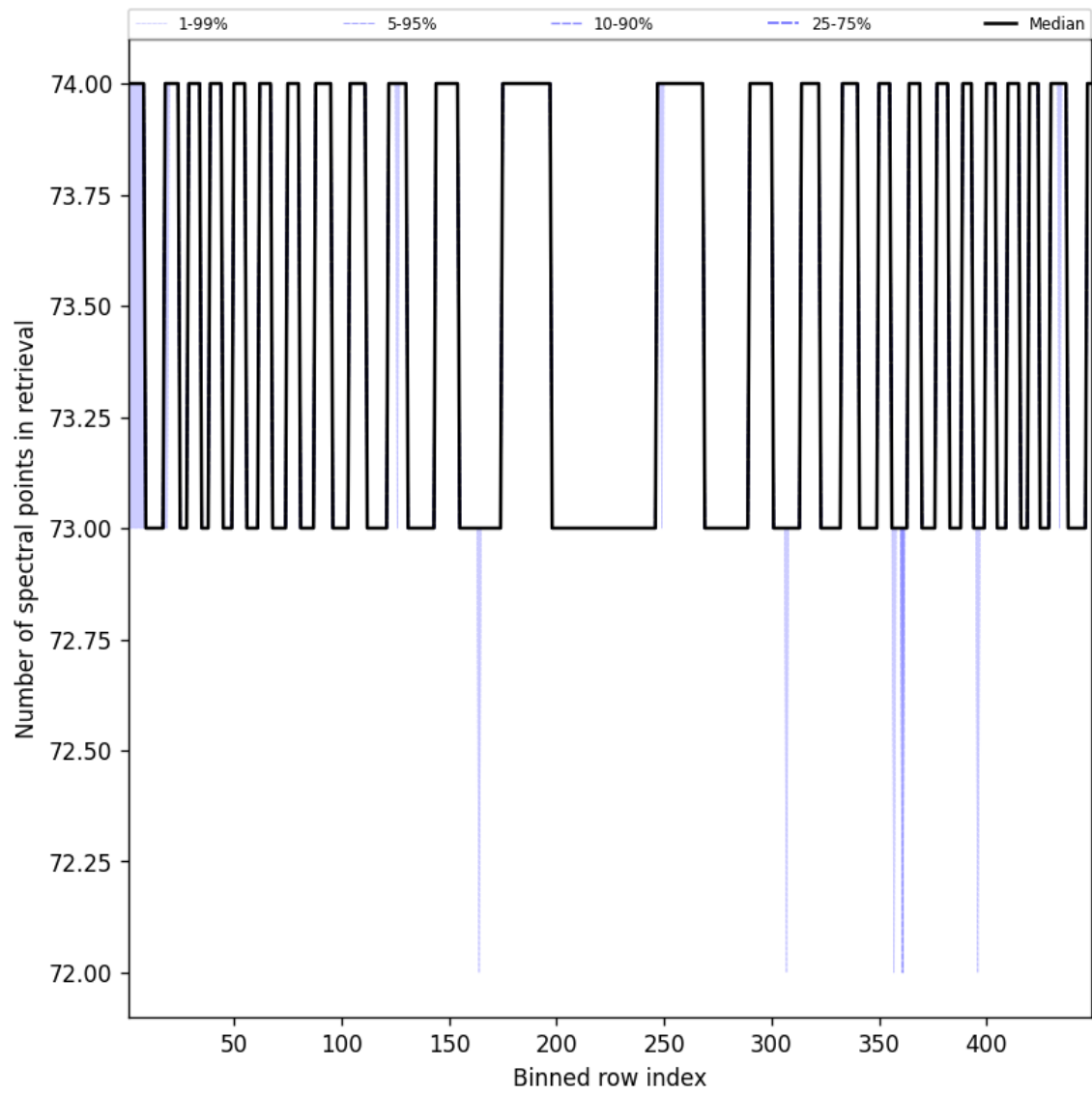
Figure 110: Along track statistics of “Number of spectral points in retrieval” for 2025-08-31 to 2025-09-01
