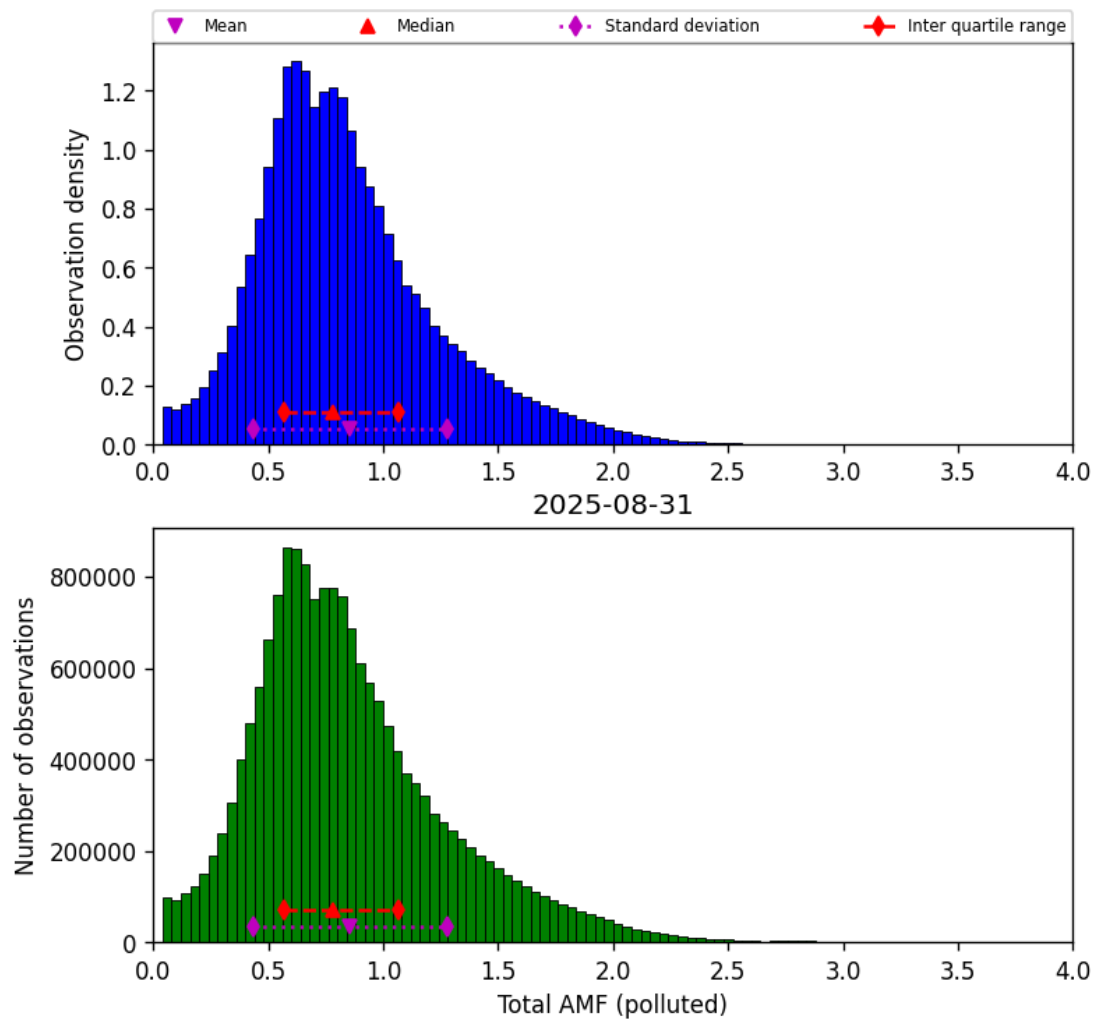
Figure 80: Histogram of “Total AMF (polluted)” for 2025-08-31 to 2025-09-01
