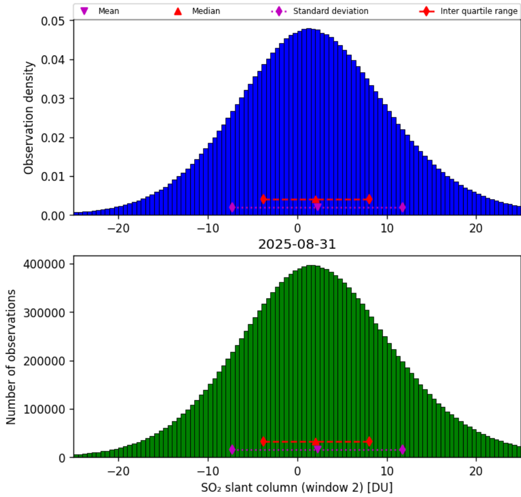
Figure 67: Histogram of “SO 2 slant column (window 2)” for 2025-08-31 to 2025-09-01
