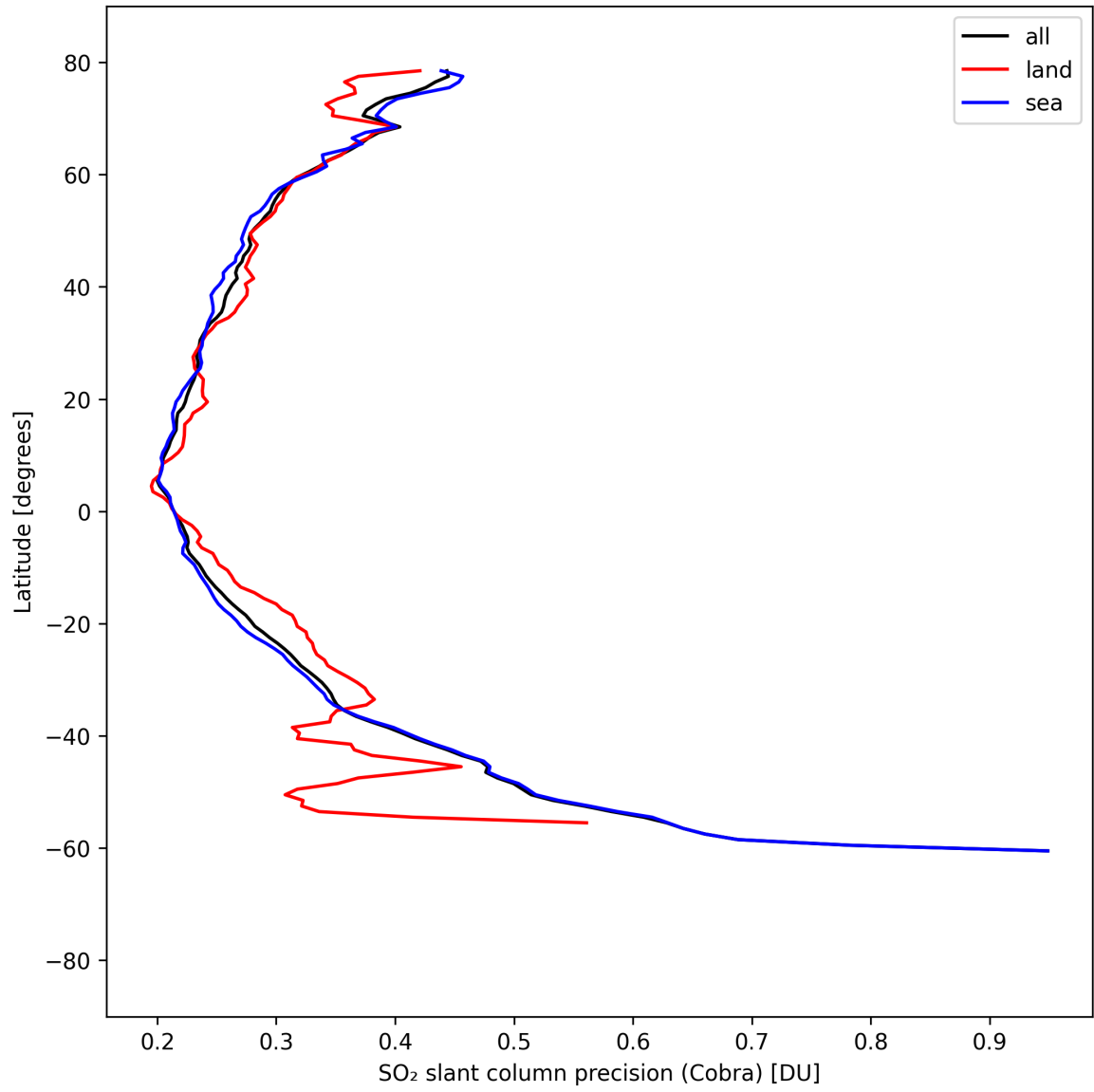
Figure 35: Zonal average of “SO 2 slant column precision (Cobra)” for 2025-08-31 to 2025-09-01.
