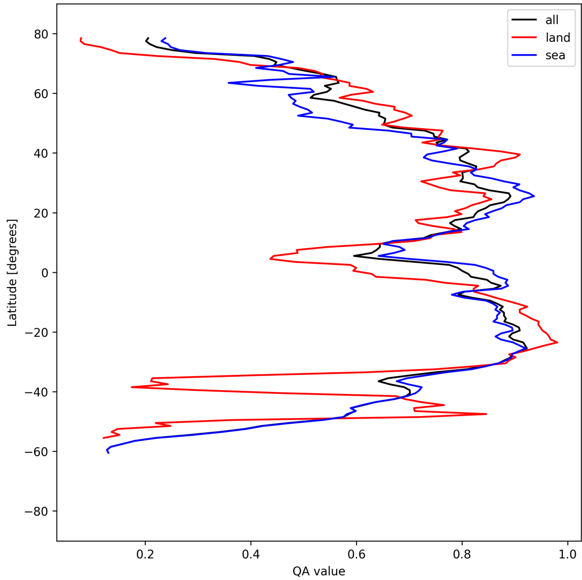
Figure 30: Zonal average of “QA value” for 2025-08-31 to 2025-09-01.
