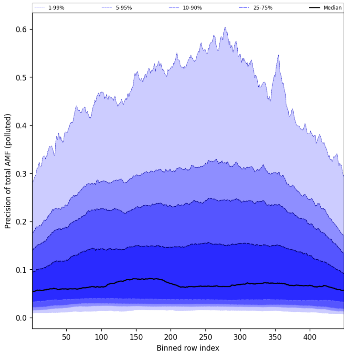
Figure 108: Along track statistics of “Precision of total AMF (polluted)” for 2025-08-31 to 2025-09-01
