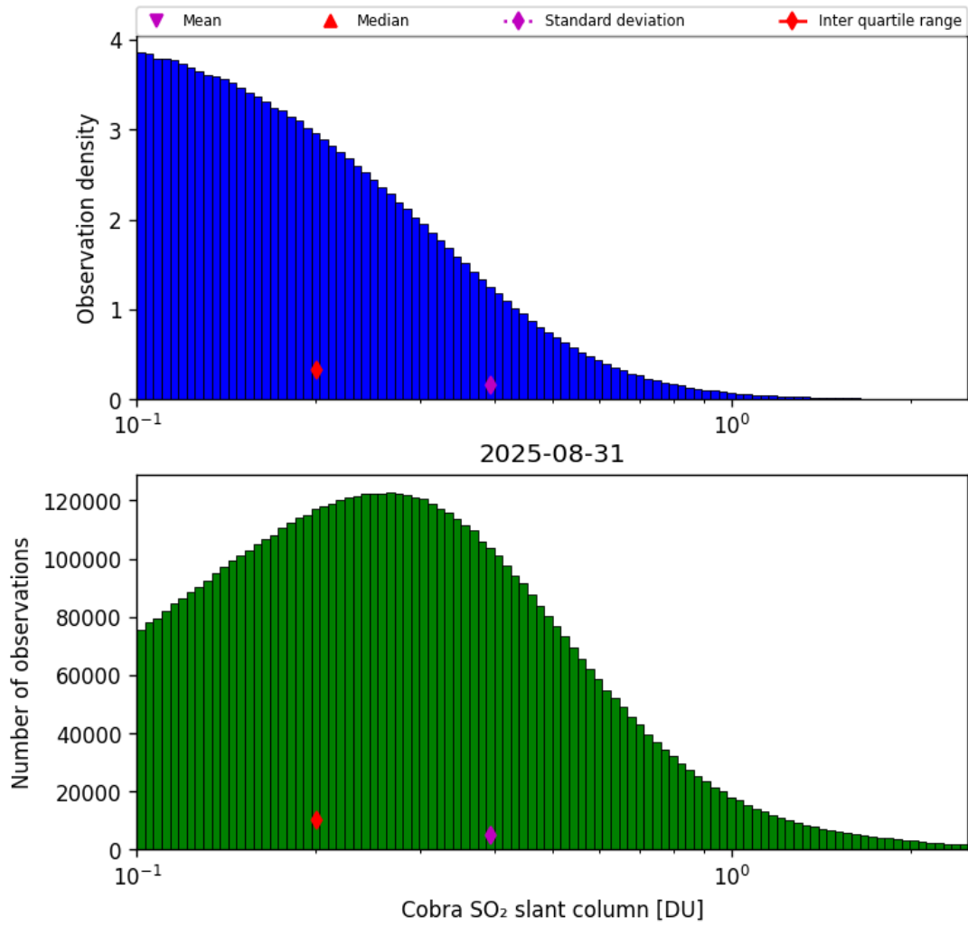
Figure 61: Histogram of “Cobra SO 2 slant column” for 2025-08-31 to 2025-09-01
