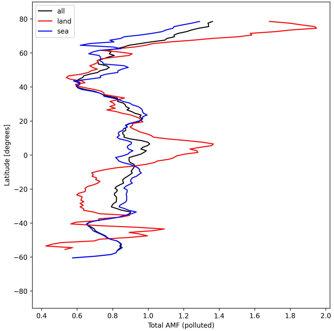
Figure 53: Zonal average of “Total AMF (polluted)” for 2025-08-31 to 2025-09-01.
