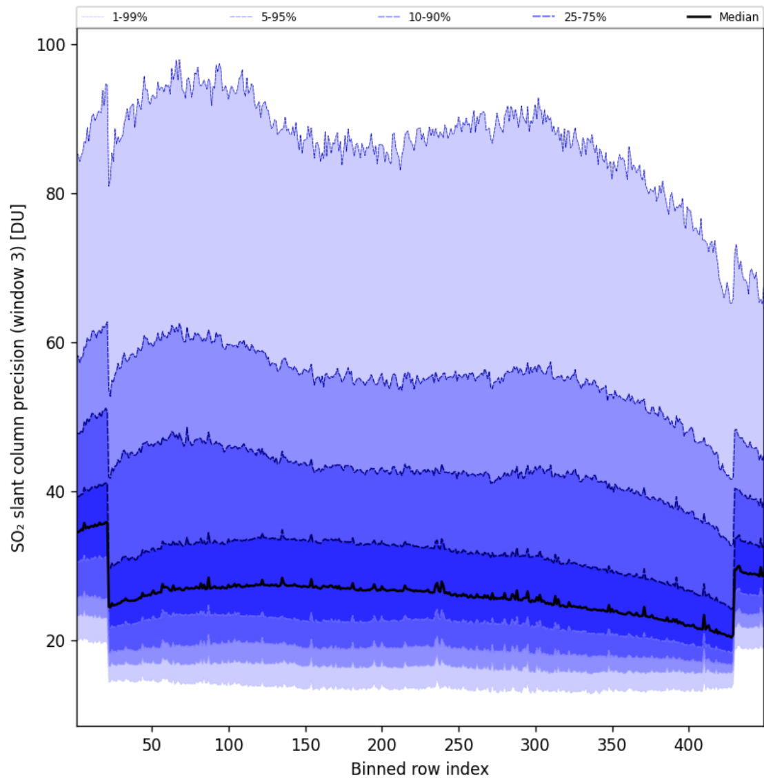
Figure 99: Along track statistics of “SO 2 slant column precision (window 3)” for 2025-08-31 to 2025-09-01
