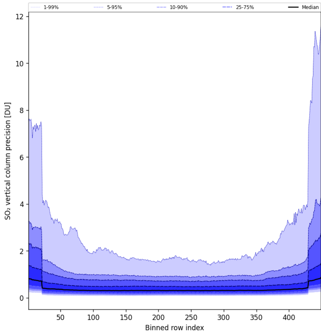
Figure 86: Along track statistics of “SO 2 vertical column precision” for 2025-08-31 to 2025-09-01
