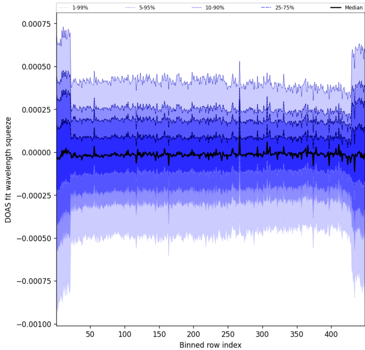
Figure 105: Along track statistics of “DOAS fit wavelength squeeze” for 2025-08-31 to 2025-09-01
