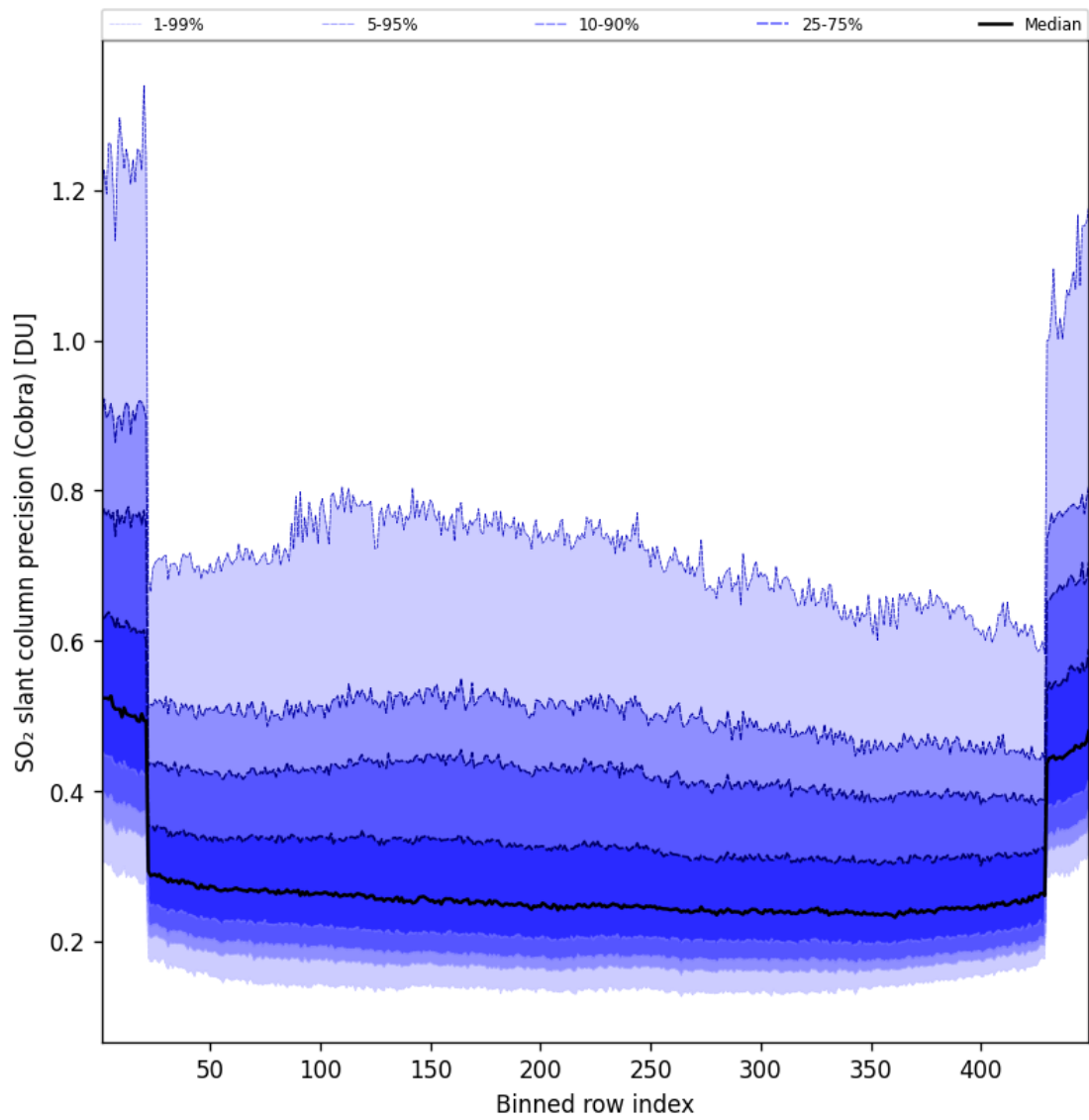
Figure 89: Along track statistics of “SO 2 slant column precision (Cobra)” for 2025-08-31 to 2025-09-01
