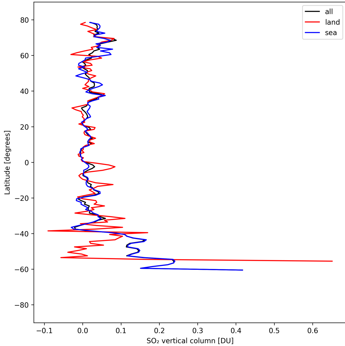
Figure 31: Zonal average of “SO 2 vertical column” for 2025-08-31 to 2025-09-01.
