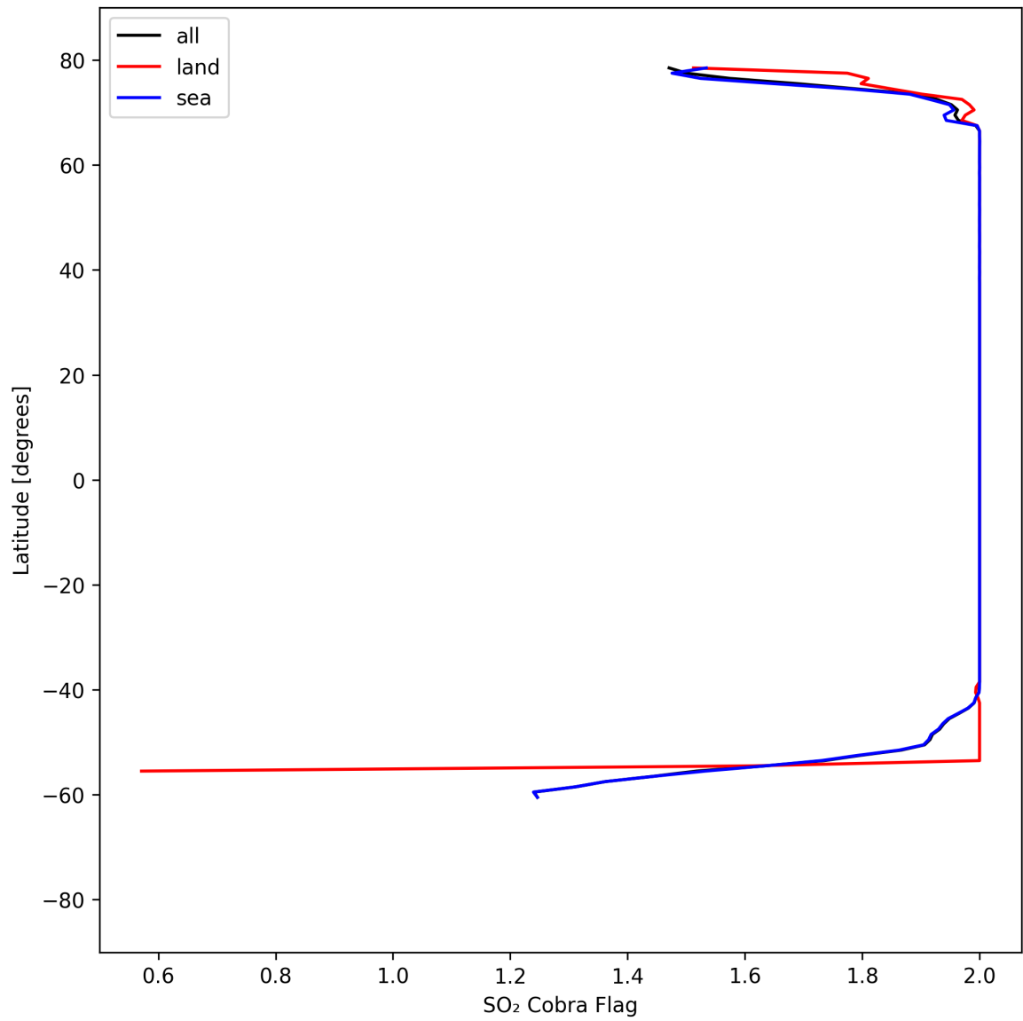
Figure 48: Zonal average of "SO 2 Cobra Flag" for 2025-08-31 to 2025-09-01.
