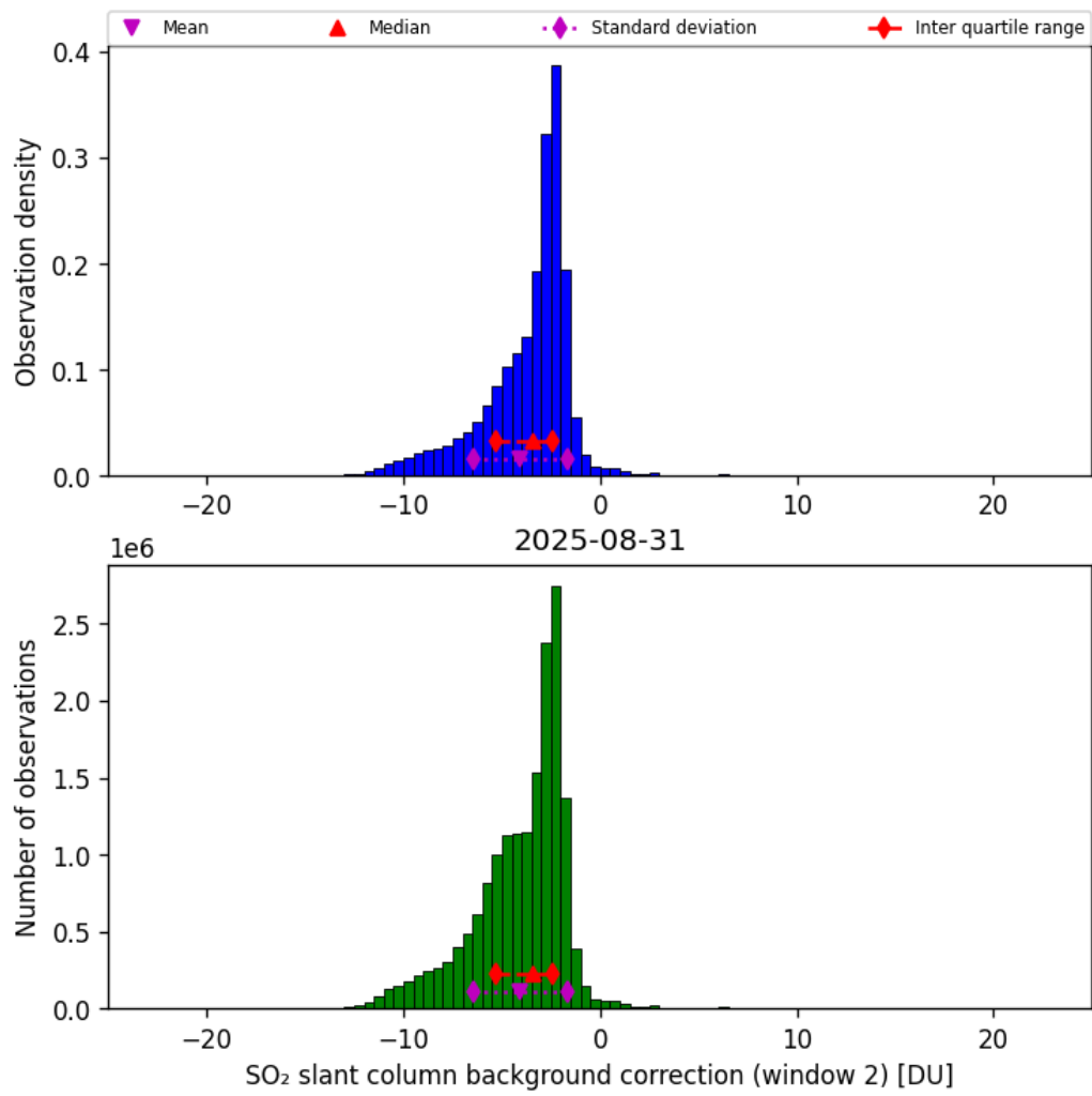
Figure 70: Histogram of “SO 2 slant column background correction (window 2)” for 2025-08-31 to 2025-09-01
