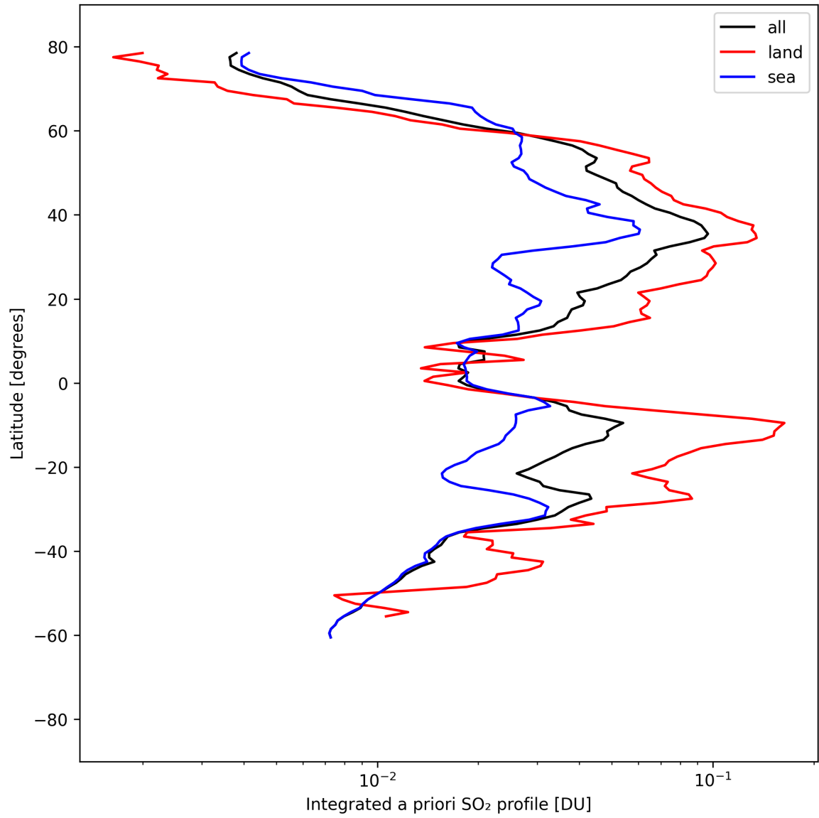
Figure 49: Zonal average of “Integrated a priori SO 2 profile” for 2025-08-31 to 2025-09-01.
