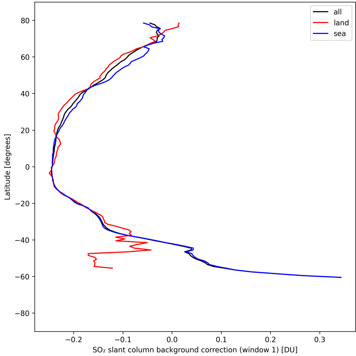
Figure 39: Zonal average of “SO 2 slant column background correction (window 1)” for 2025-08-31 to 2025-09-01.
