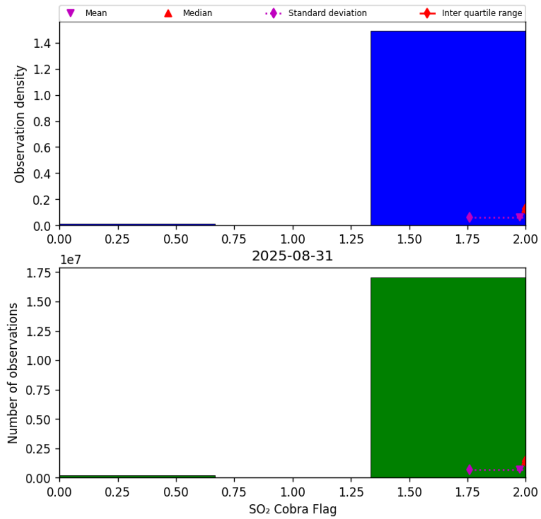
Figure 75: Histogram of “SO 2 Cobra Flag” for 2025-08-31 to 2025-09-01
