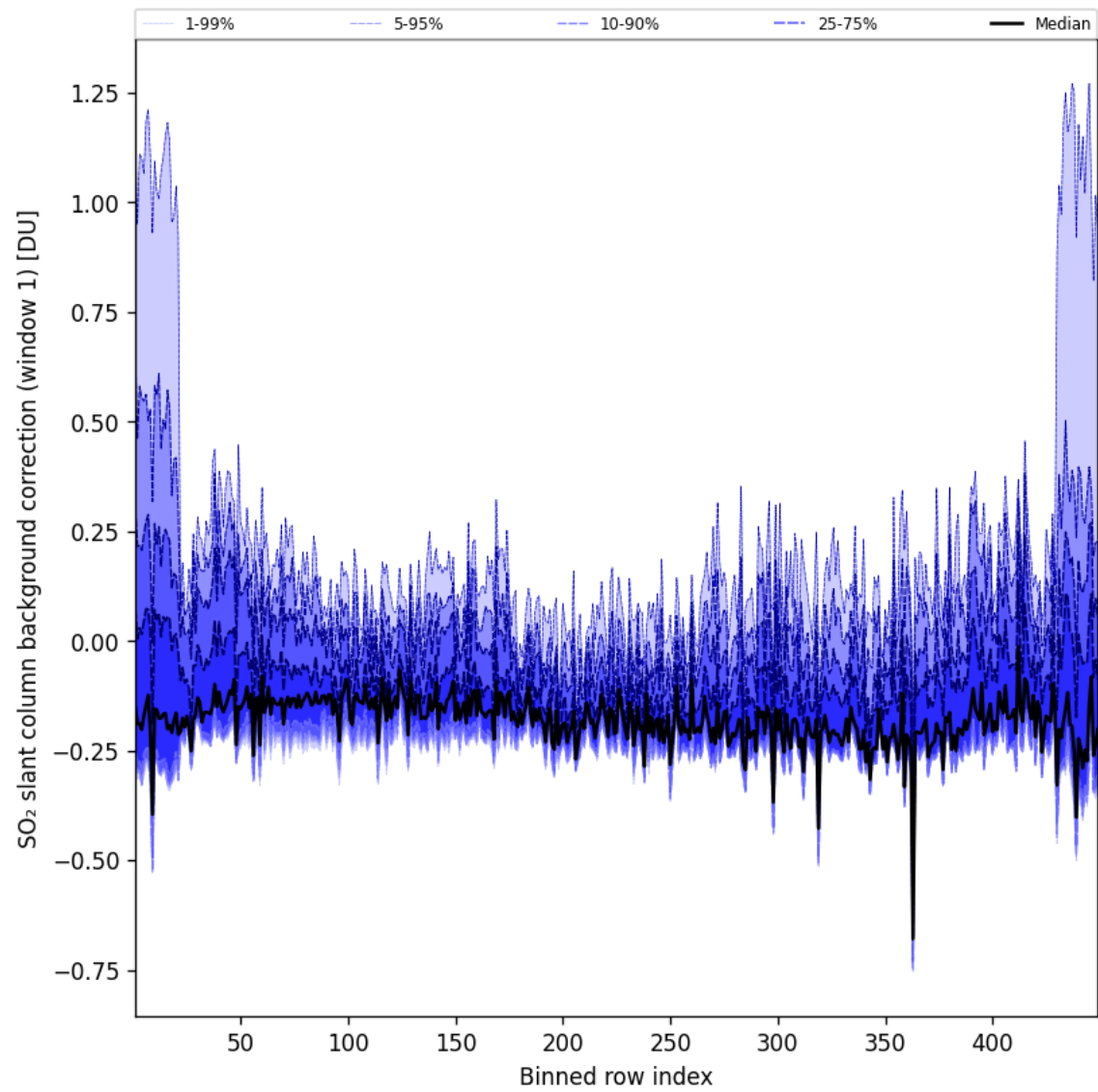
Figure 93: Along track statistics of “SO 2 slant column background correction (window 1)” for 2025-08-31 to 2025-09-01
