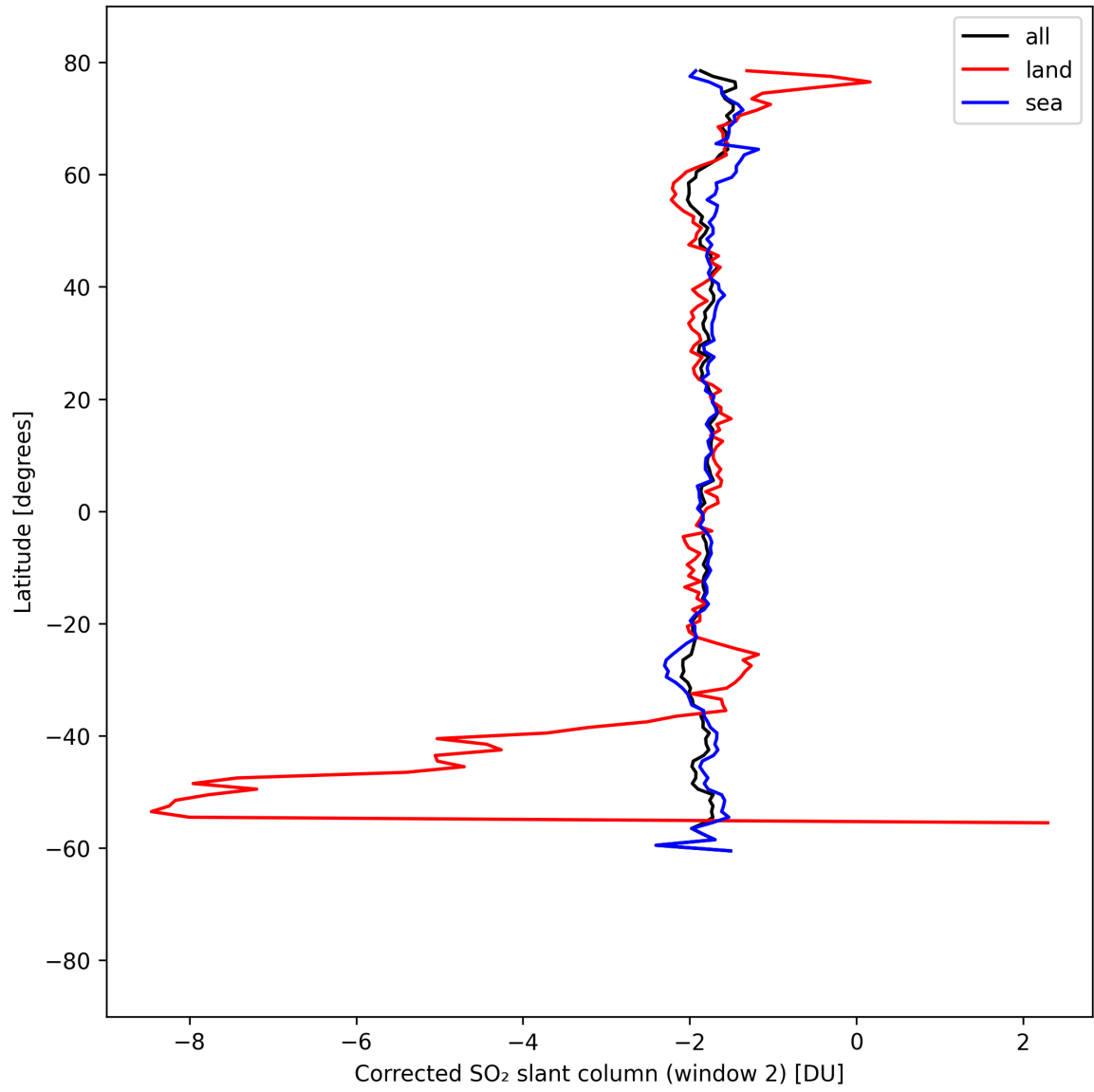
Figure 42: Zonal average of “Corrected SO 2 slant column (window 2)” for 2025-08-31 to 2025-09-01.
