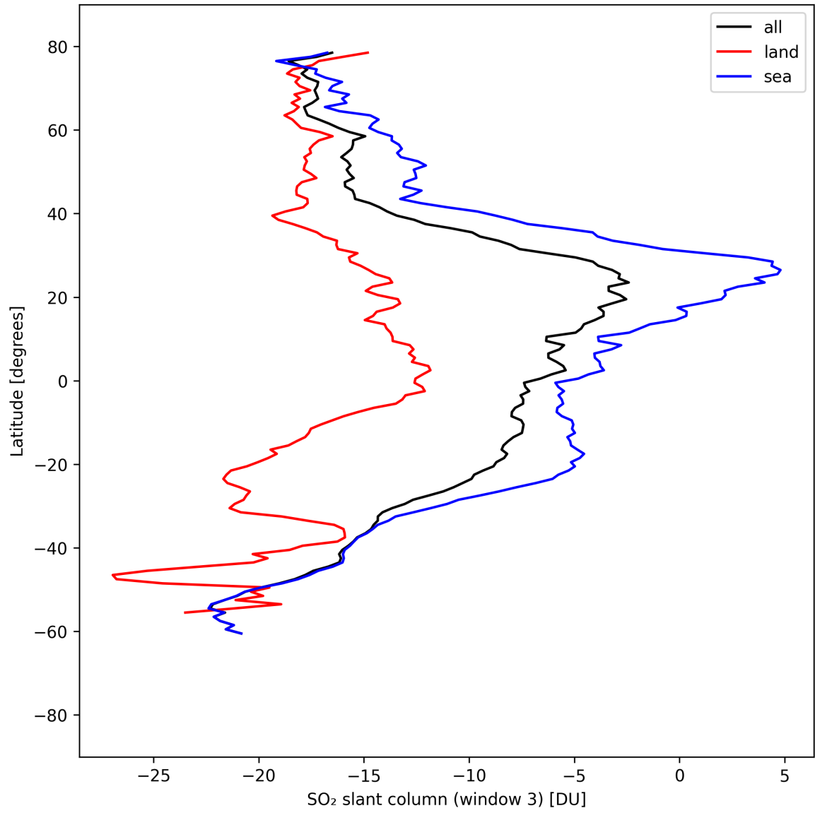
Figure 44: Zonal average of “SO 2 slant column (window 3)” for 2025-08-31 to 2025-09-01.
