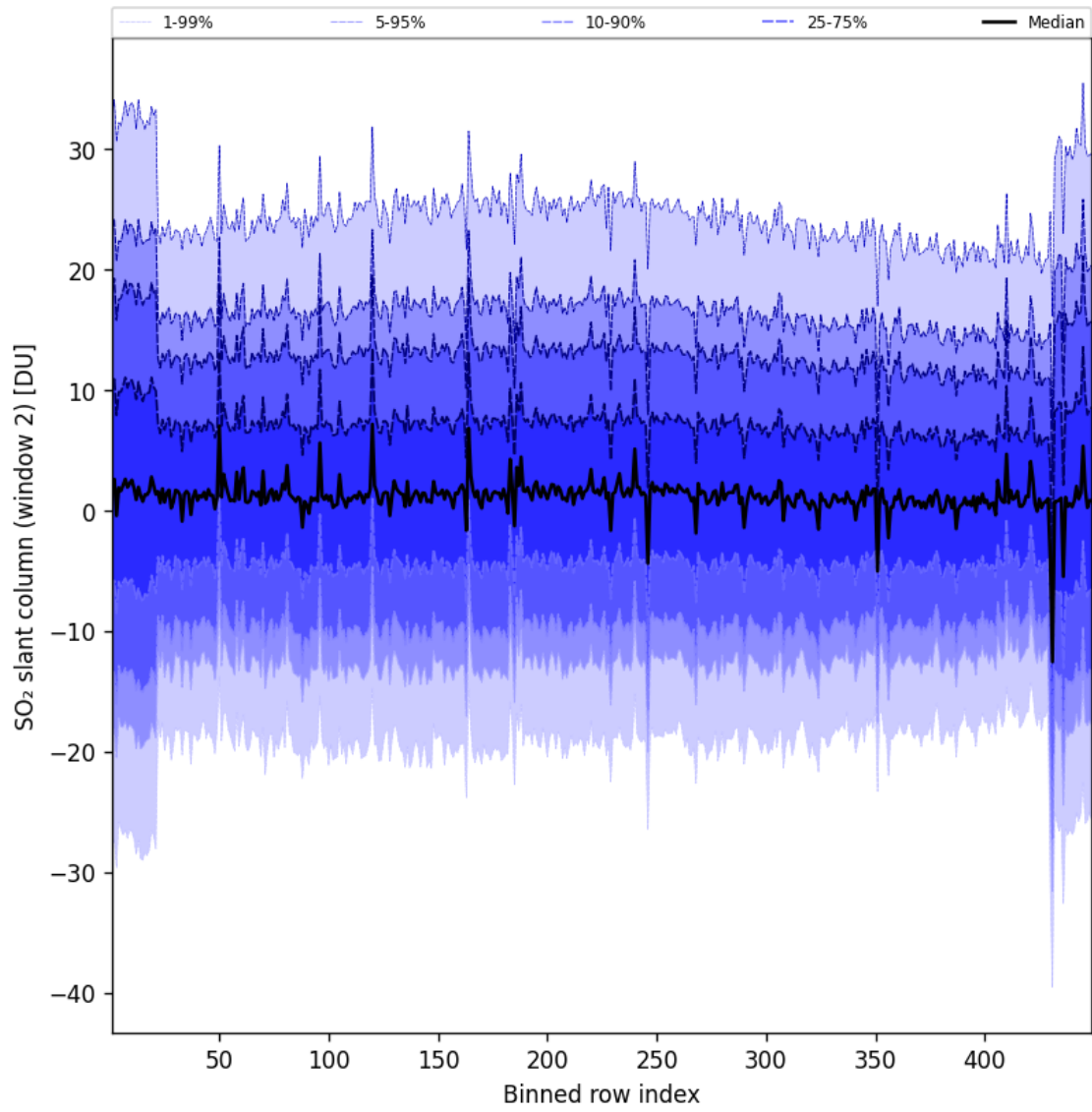
Figure 94: Along track statistics of “SO 2 slant column (window 2)” for 2025-09-01 to 2025-09-02
