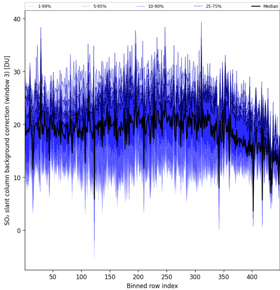
Figure 101: Along track statistics of “SO 2 slant column background correction (window 3)” for 2025-09-01 to 2025-09-02
