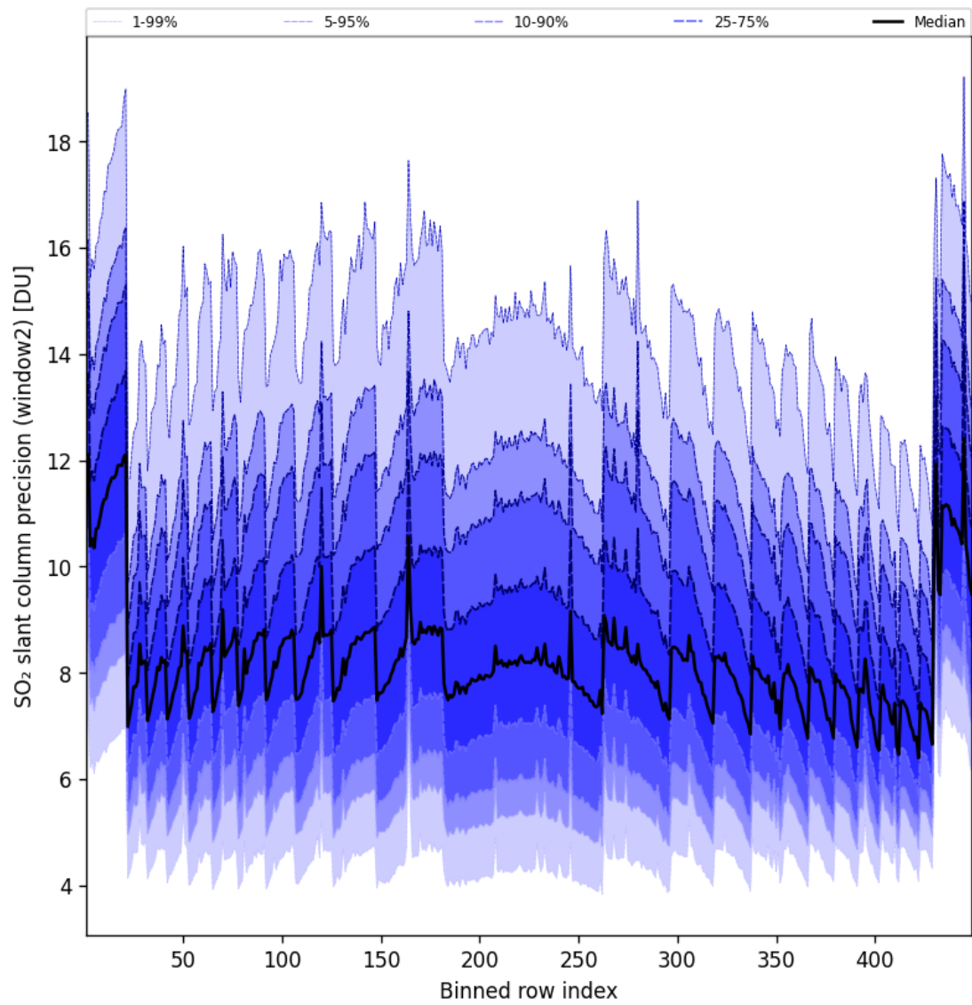
Figure 95: Along track statistics of “SO 2 slant column precision (window2)” for 2025-09-01 to 2025-09-02
