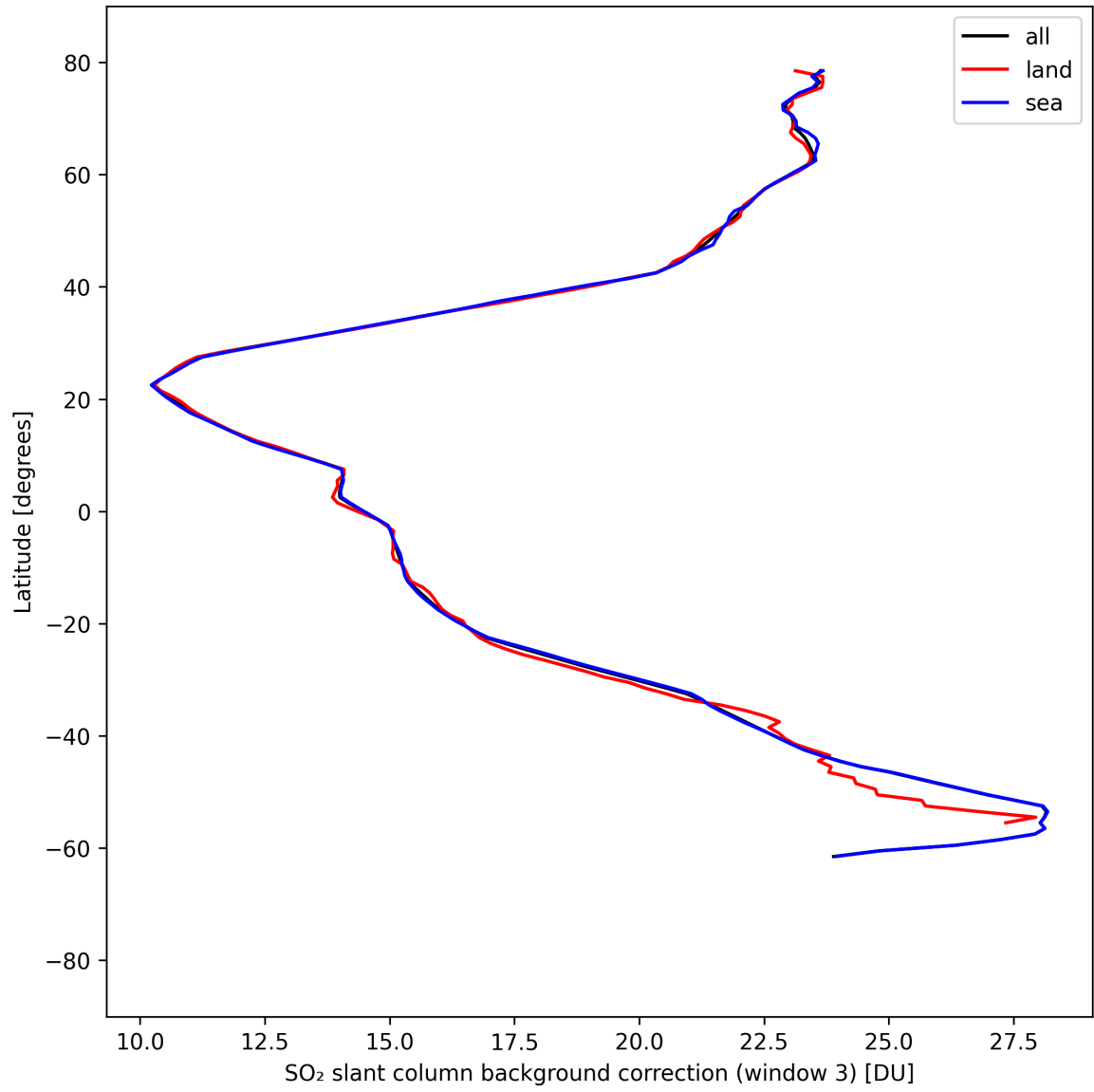
Figure 47: Zonal average of “SO 2 slant column background correction (window 3)” for 2025-09-01 to 2025-09-02.
