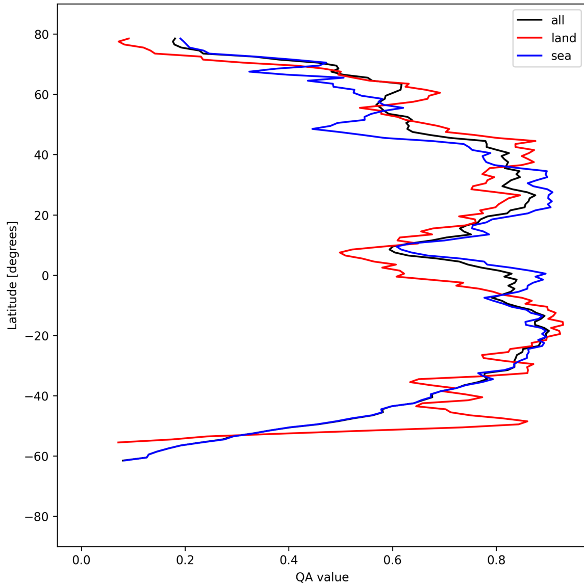
Figure 30: Zonal average of “QA value” for 2025-09-01 to 2025-09-02.
