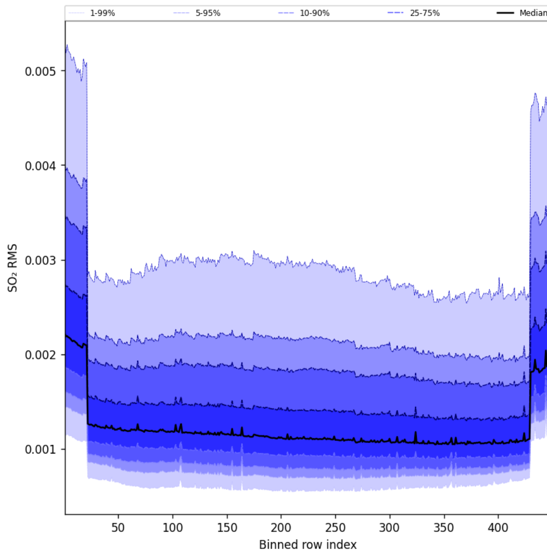
Figure 106: Along track statistics of “SO 2 RMS” for 2025-09-01 to 2025-09-02
