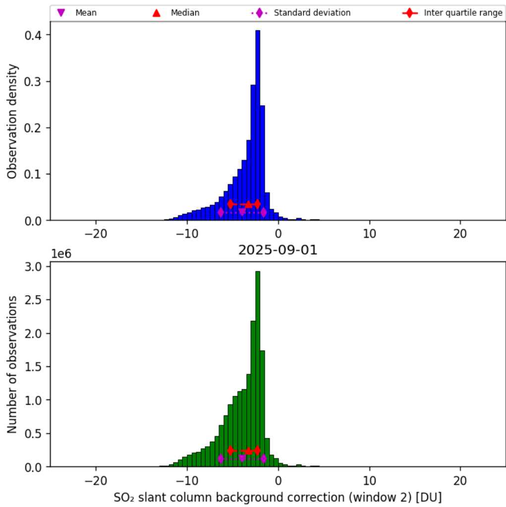
Figure 70: Histogram of “SO 2 slant column background correction (window 2)” for 2025-09-01 to 2025-09-02
