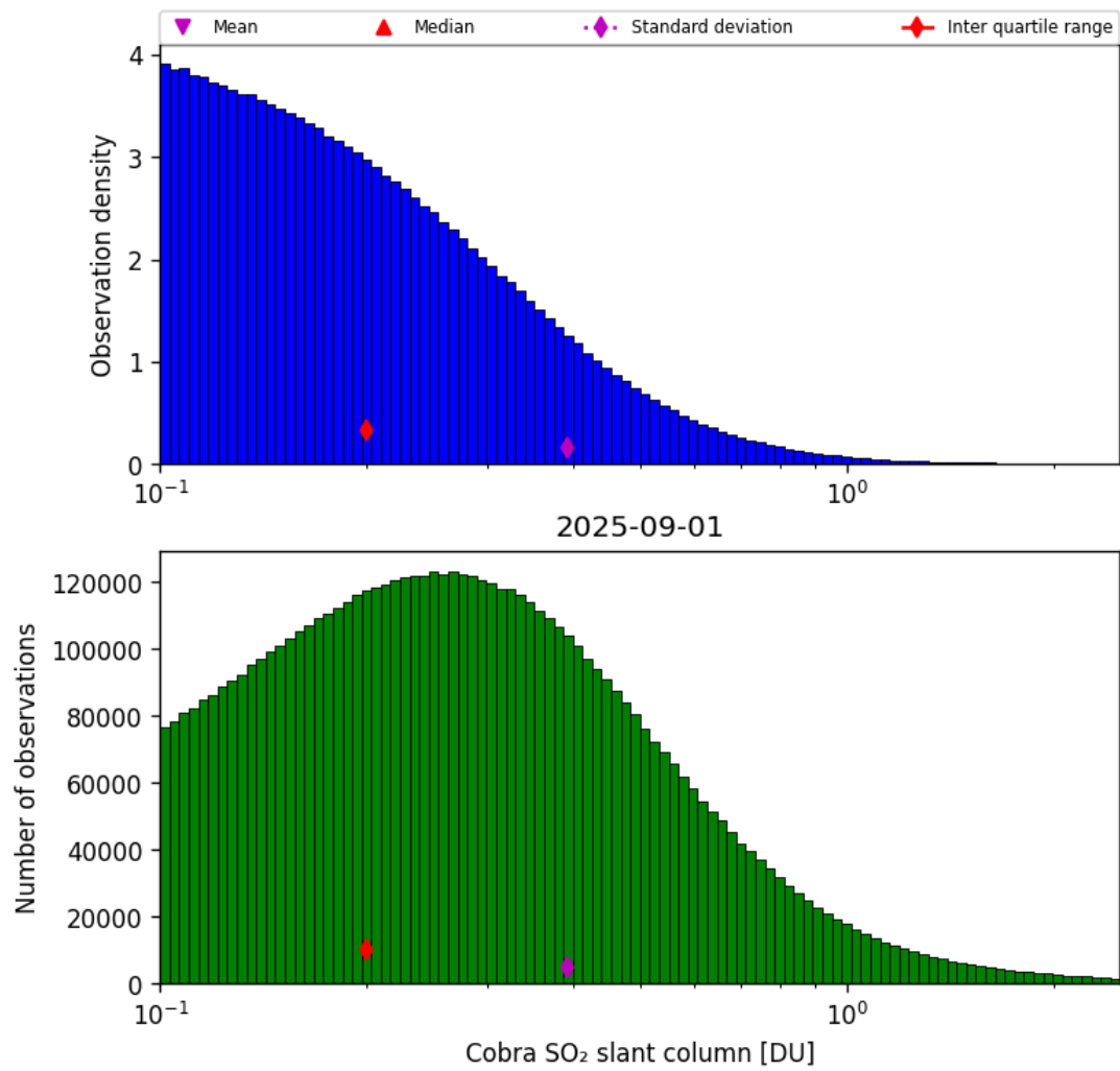
Figure 61: Histogram of “Cobra SO 2 slant column” for 2025-09-01 to 2025-09-02
