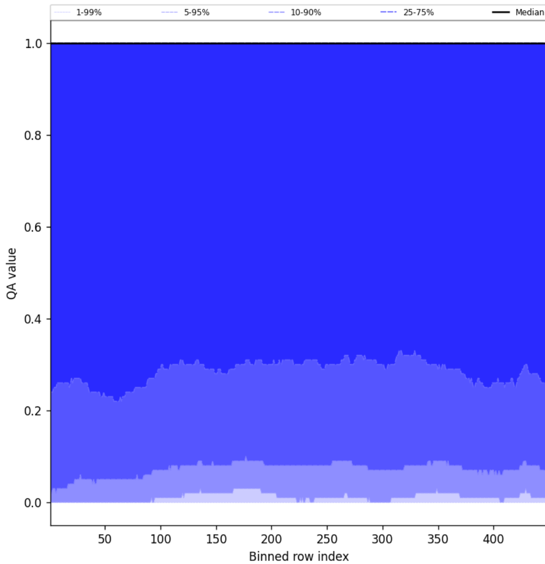
Figure 84: Along track statistics of “QA value” for 2025-09-01 to 2025-09-02
