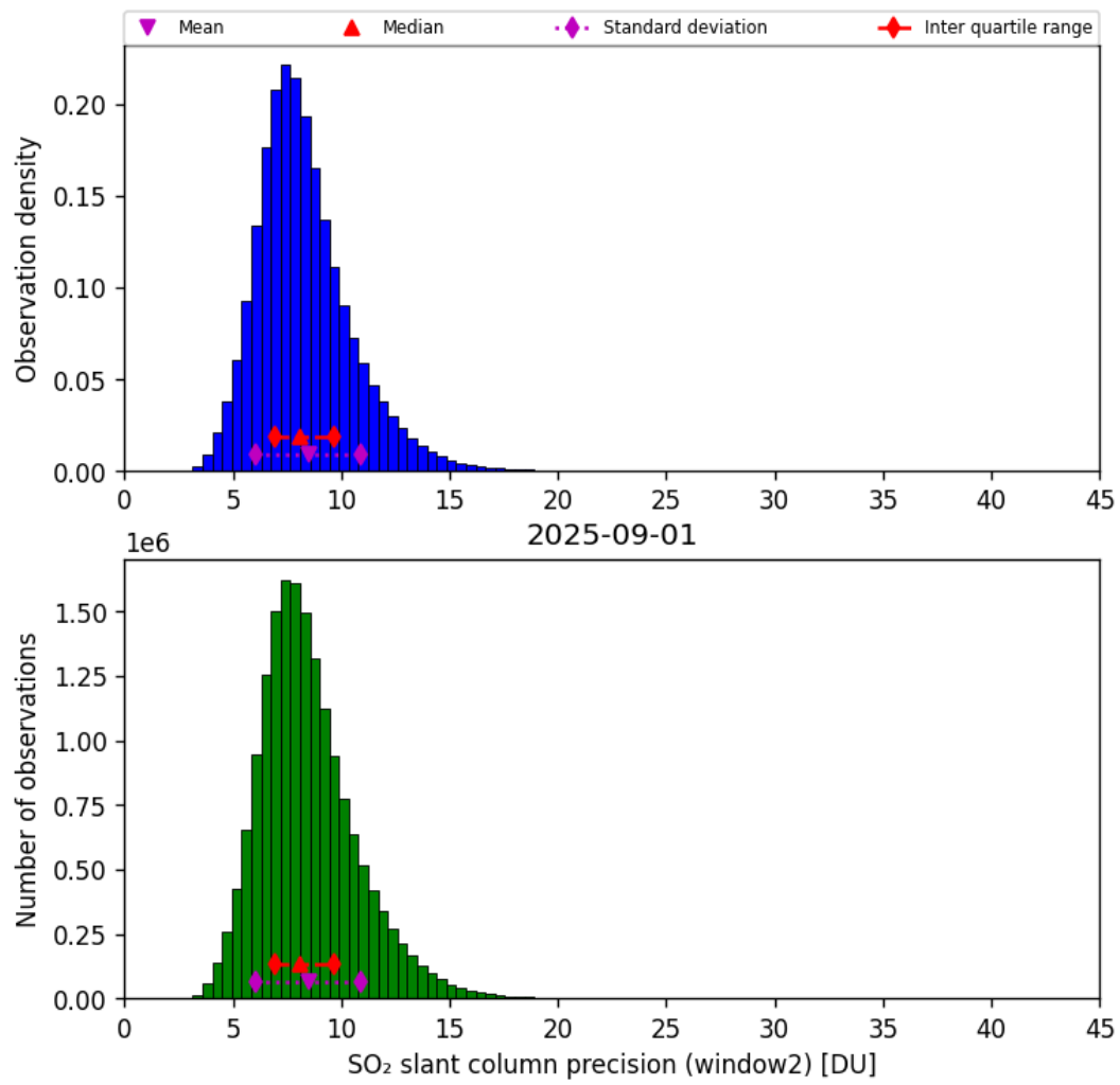
Figure 68: Histogram of “SO 2 slant column precision (window2)” for 2025-09-01 to 2025-09-02
