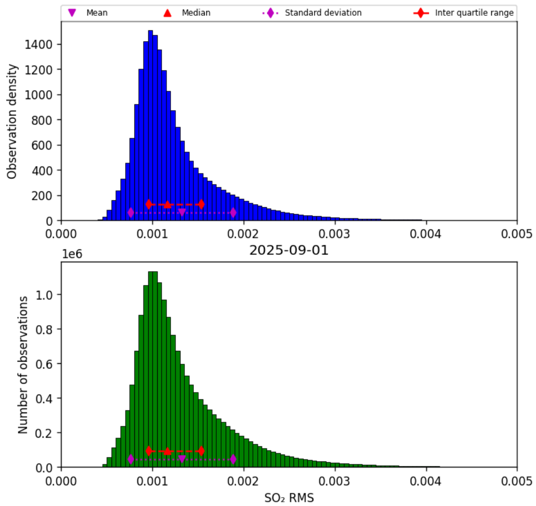
Figure 79: Histogram of “SO 2 RMS” for 2025-09-01 to 2025-09-02
