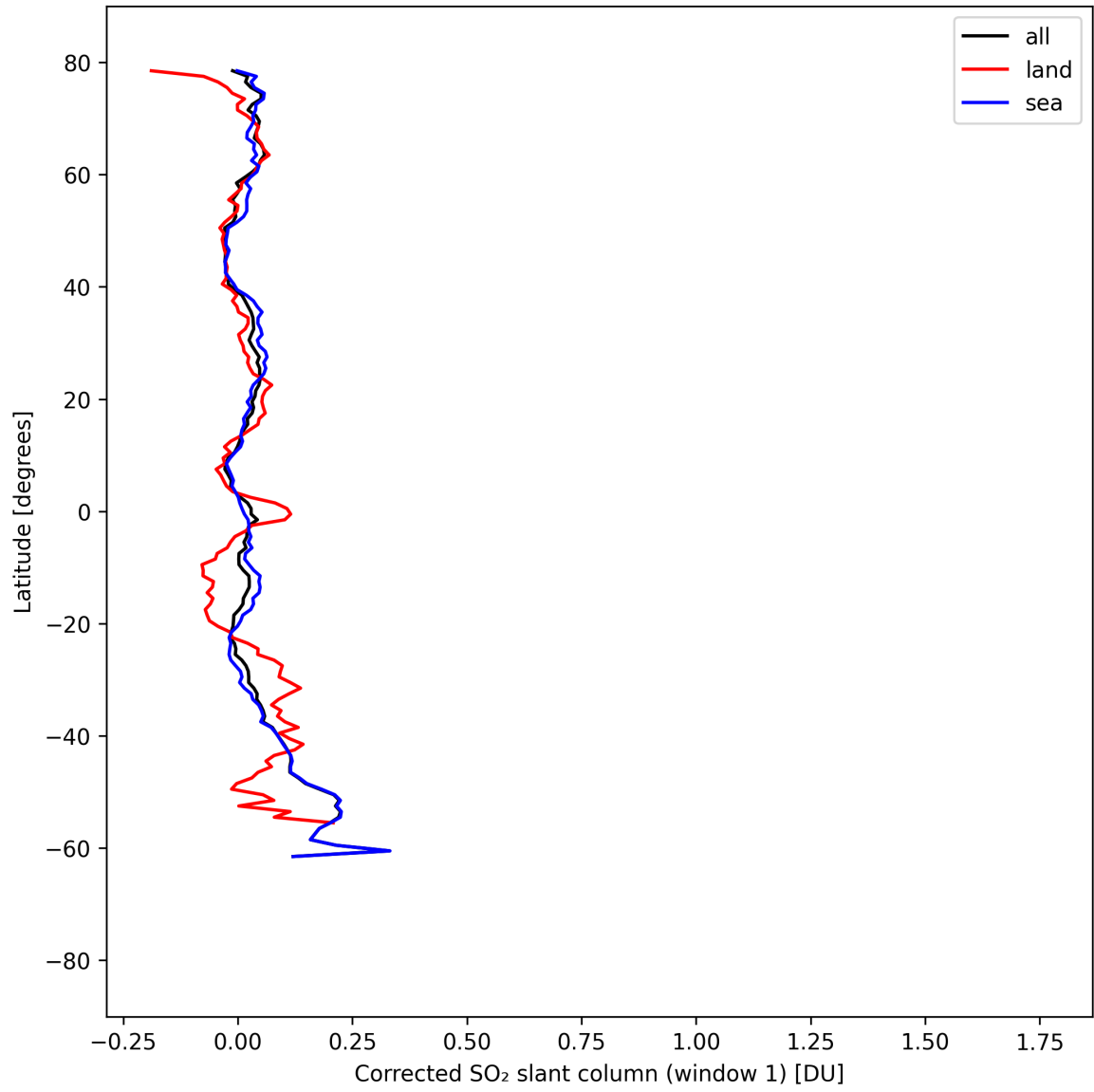
Figure 38: Zonal average of “Corrected SO 2 slant column (window 1)” for 2025-09-01 to 2025-09-02.
