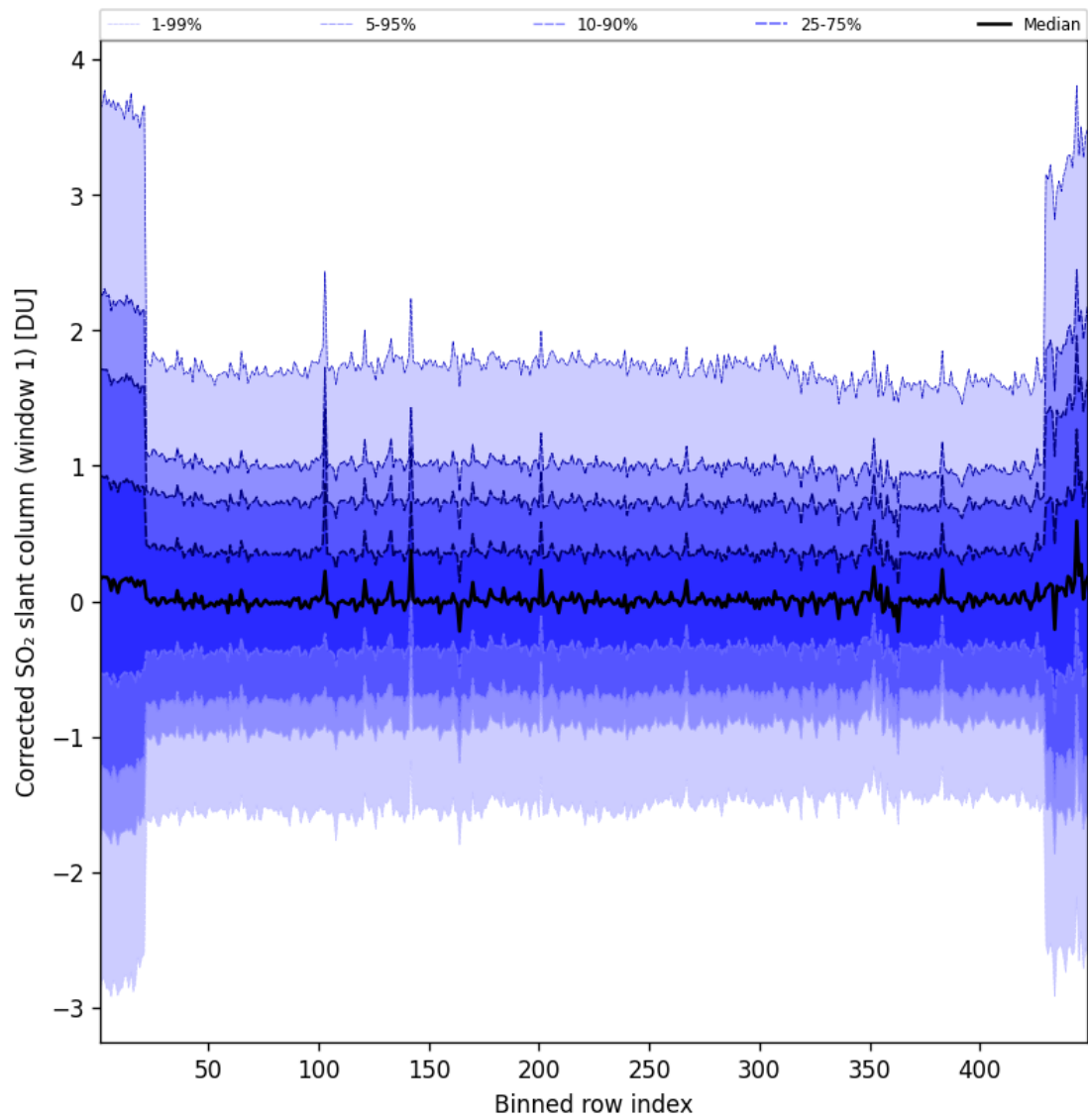
Figure 92: Along track statistics of "Corrected SO 2 slant column (window 1)" for 2025-09-01 to 2025-09-02
