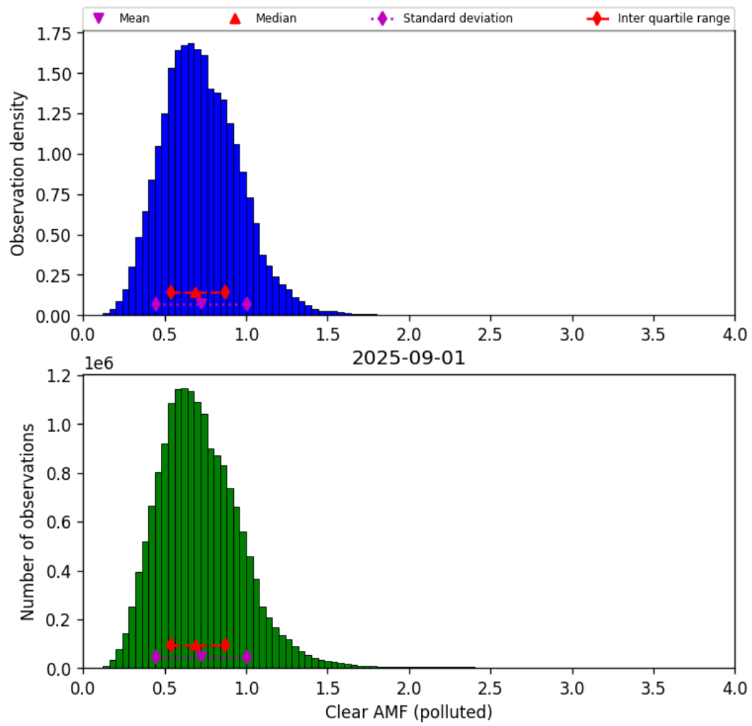
Figure 82: Histogram of “Clear AMF (polluted)” for 2025-09-01 to 2025-09-02
