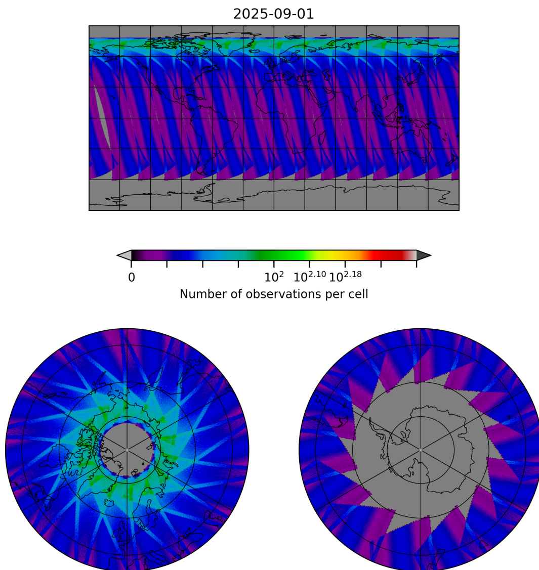
Figure 29: Map of the number of observations for 2025-09-01 to 2025-09-02
