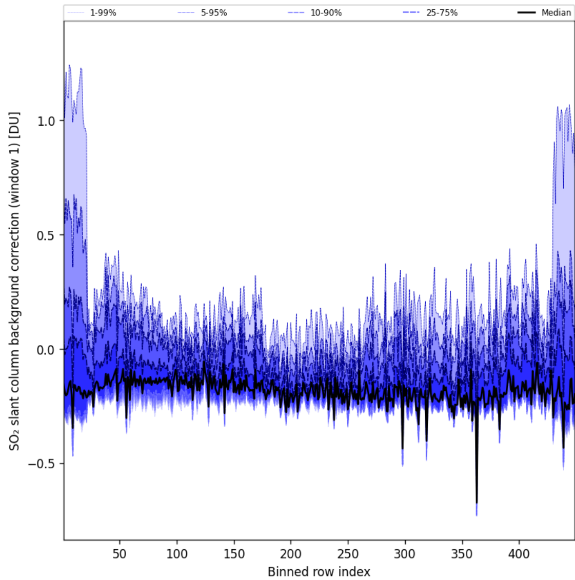
Figure 93: Along track statistics of “SO 2 slant column background correction (window 1)” for 2025-09-01 to 2025-09-02
