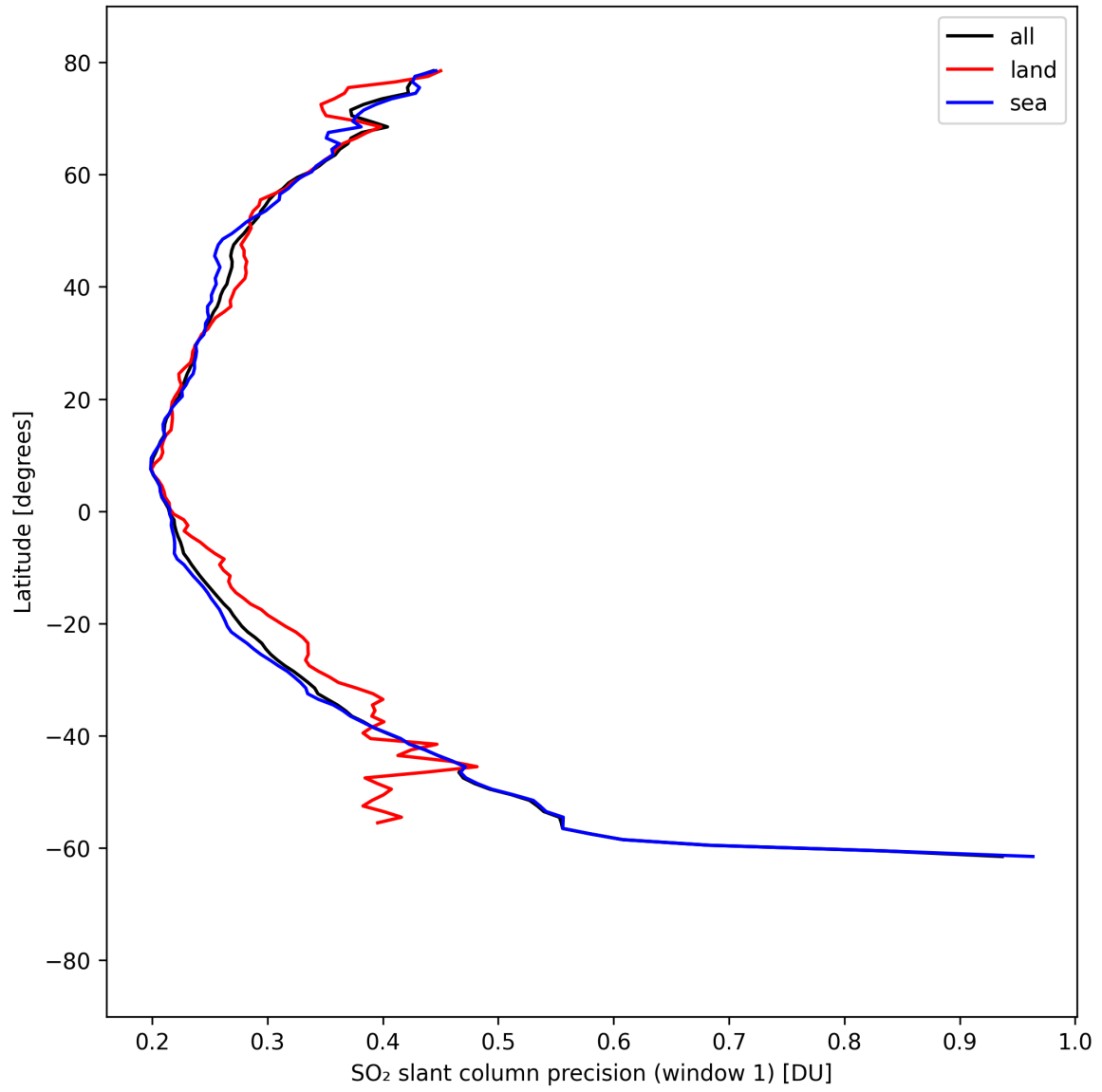
Figure 37: Zonal average of “SO 2 slant column precision (window 1)” for 2025-09-01 to 2025-09-02.
