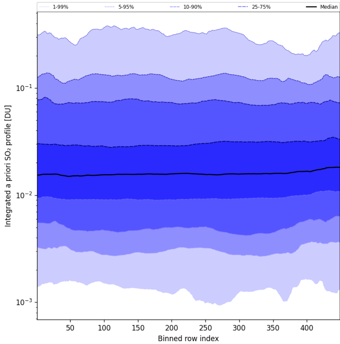
Figure 103: Along track statistics of “Integrated a priori SO 2 profile” for 2025-09-01 to 2025-09-02
