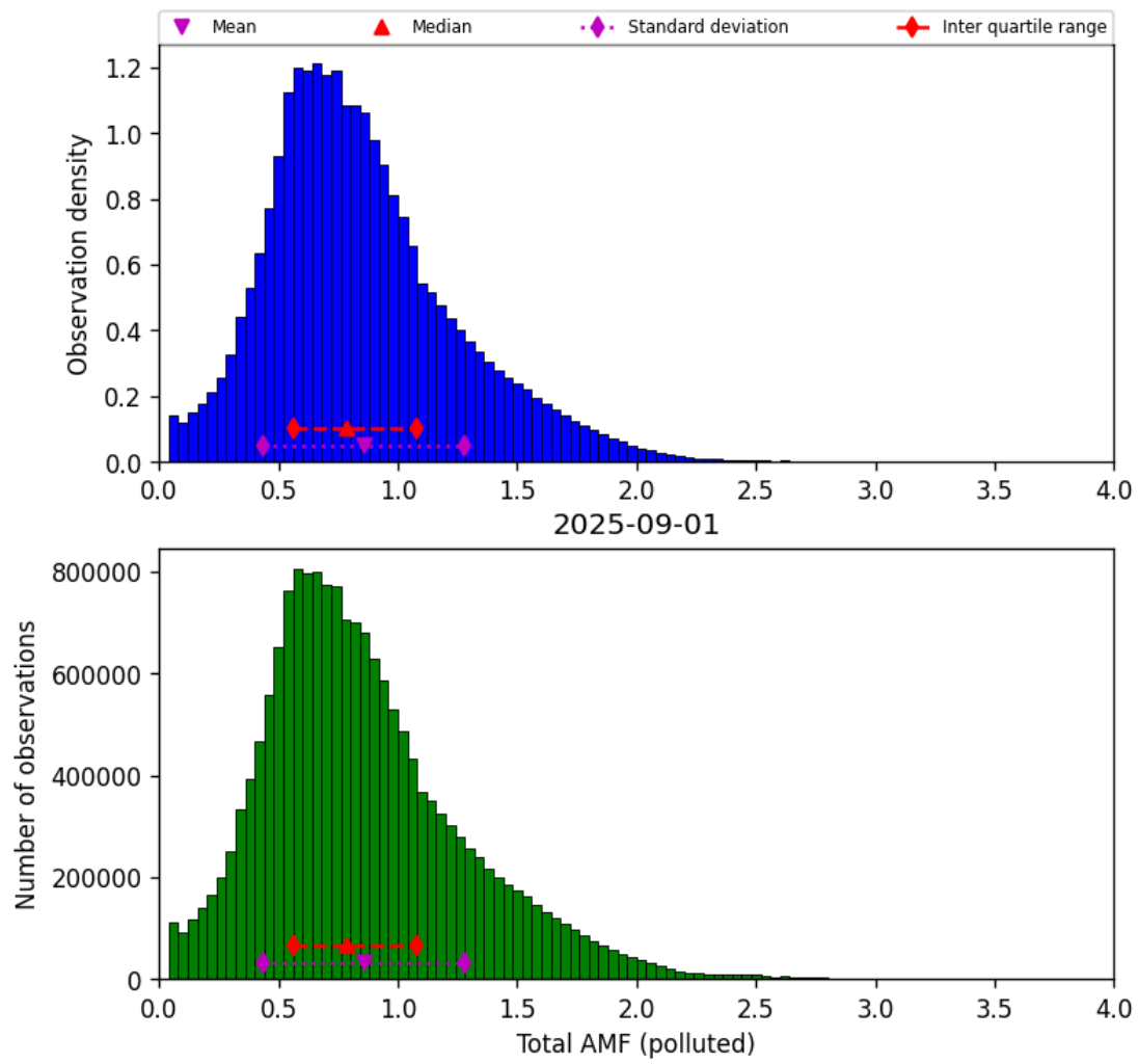
Figure 80: Histogram of “Total AMF (polluted)” for 2025-09-01 to 2025-09-02
