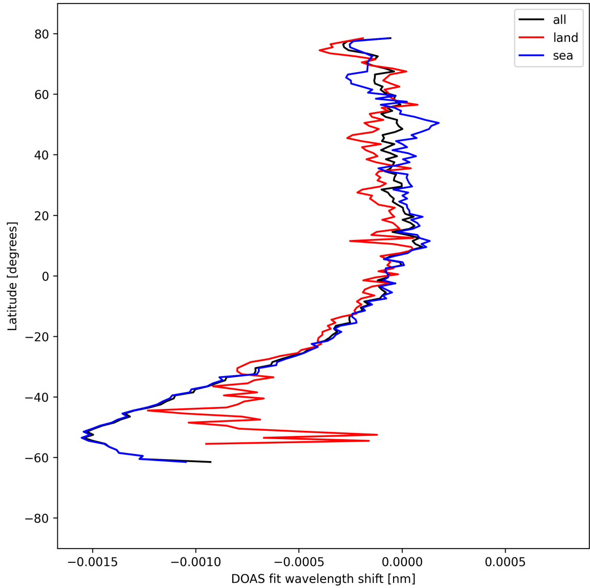
Figure 50: Zonal average of “DOAS fit wavelength shift” for 2025-09-01 to 2025-09-02.
