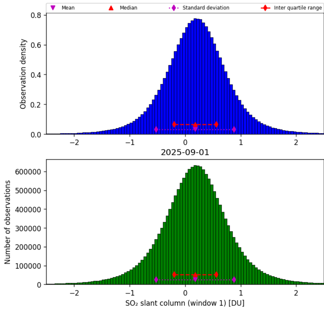
Figure 63: Histogram of “SO 2 slant column (window 1)” for 2025-09-01 to 2025-09-02
