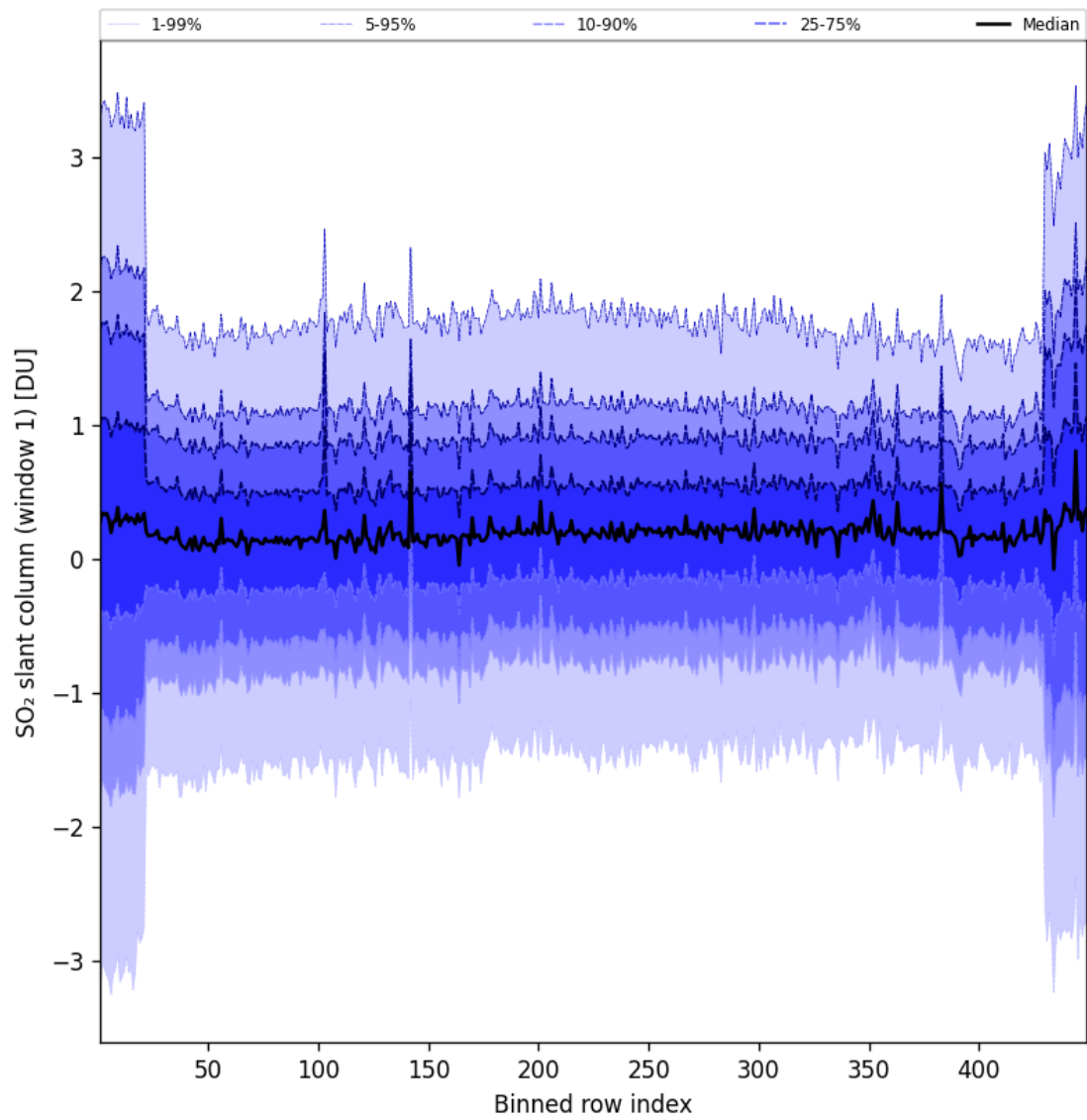
Figure 90: Along track statistics of “SO 2 slant column (window 1)” for 2025-09-01 to 2025-09-02
