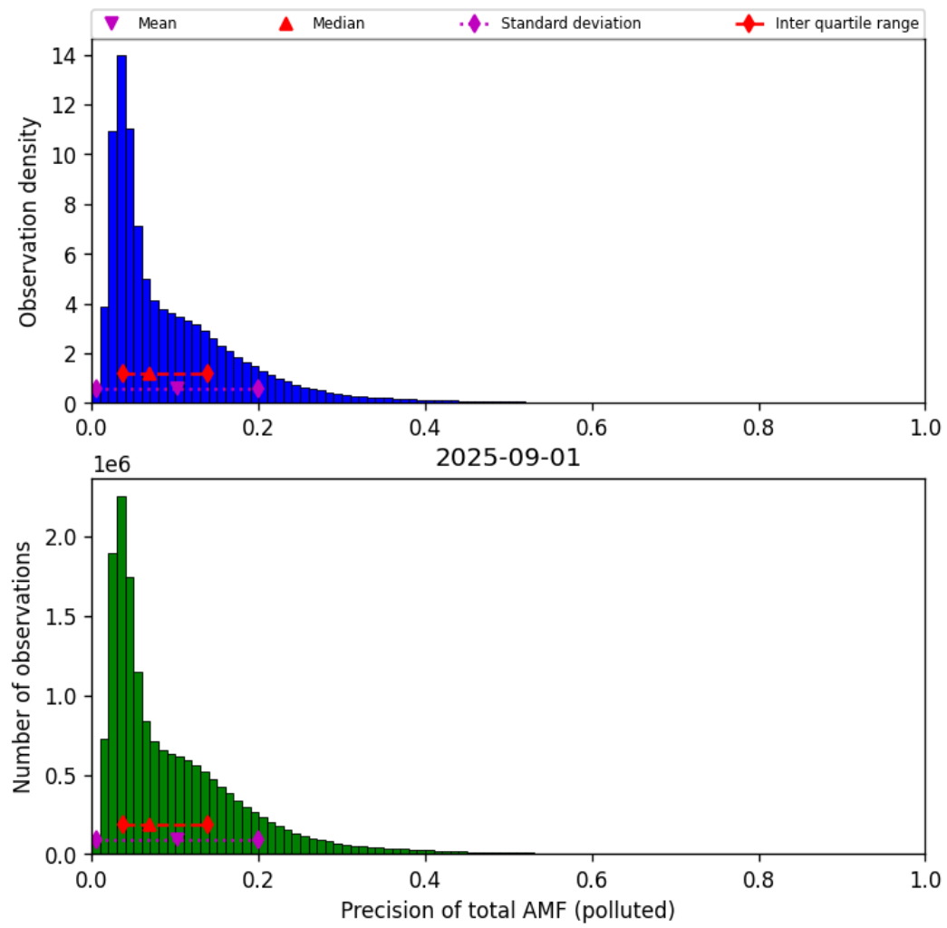
Figure 81: Histogram of “Precision of total AMF (polluted)” for 2025-09-01 to 2025-09-02
