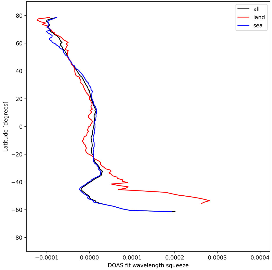
Figure 51: Zonal average of “DOAS fit wavelength squeeze” for 2025-09-01 to 2025-09-02.
