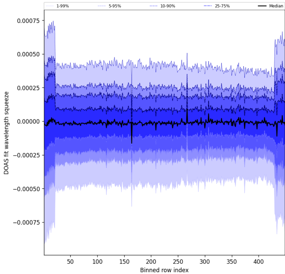
Figure 105: Along track statistics of “DOAS fit wavelength squeeze” for 2025-09-01 to 2025-09-02
