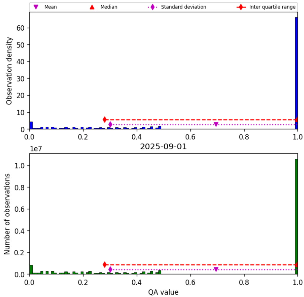
Figure 57: Histogram of “QA value” for 2025-09-01 to 2025-09-02
