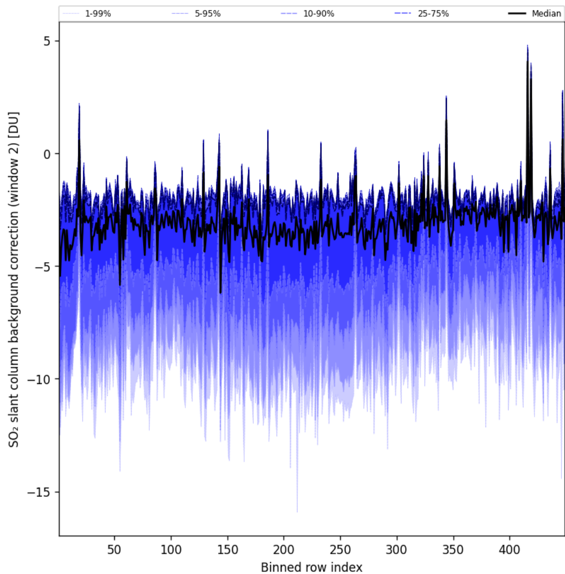
Figure 97: Along track statistics of “SO 2 slant column background correction (window 2)” for 2025-09-01 to 2025-09-02
