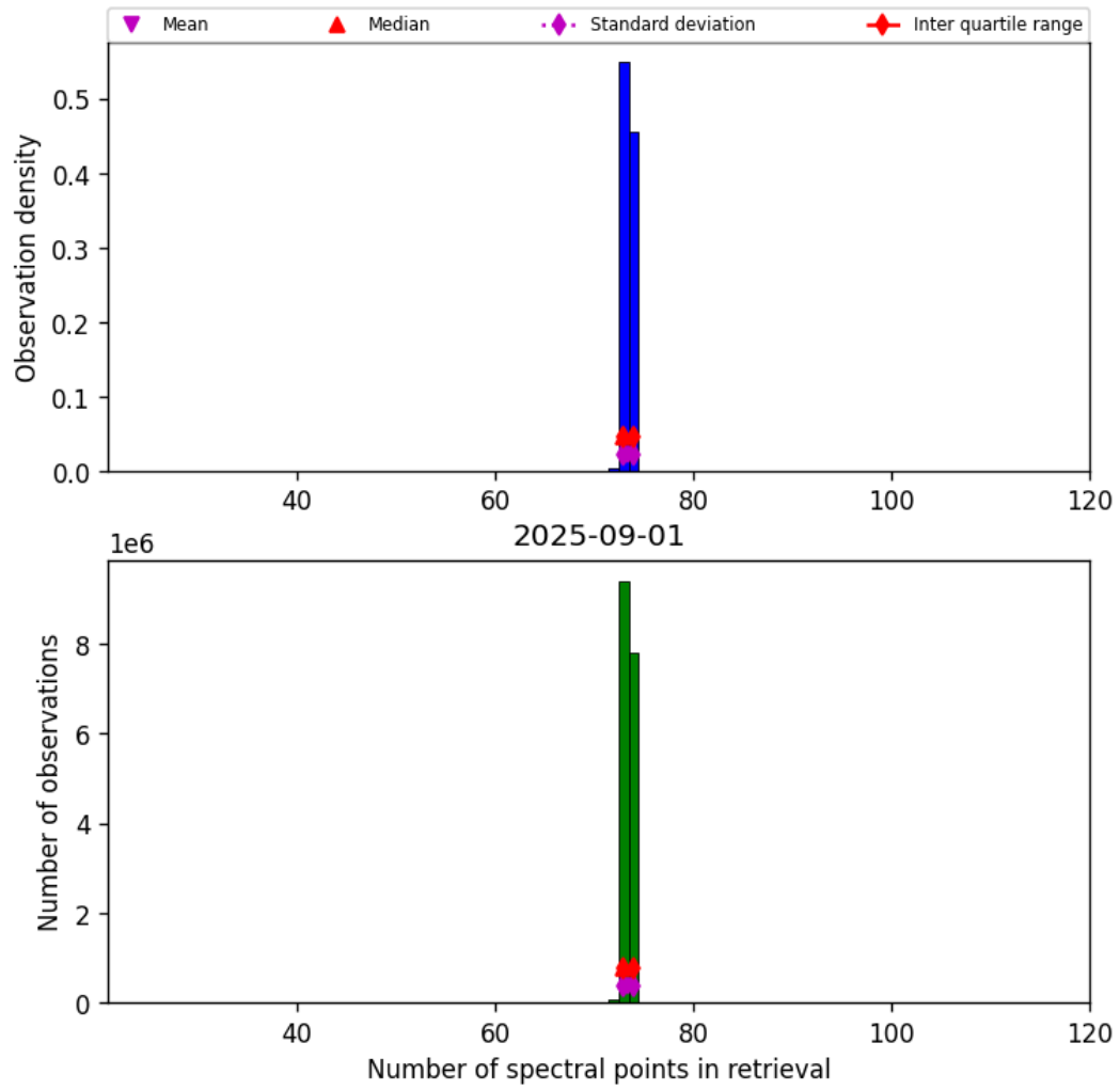
Figure 83: Histogram of “Number of spectral points in retrieval” for 2025-09-01 to 2025-09-02
