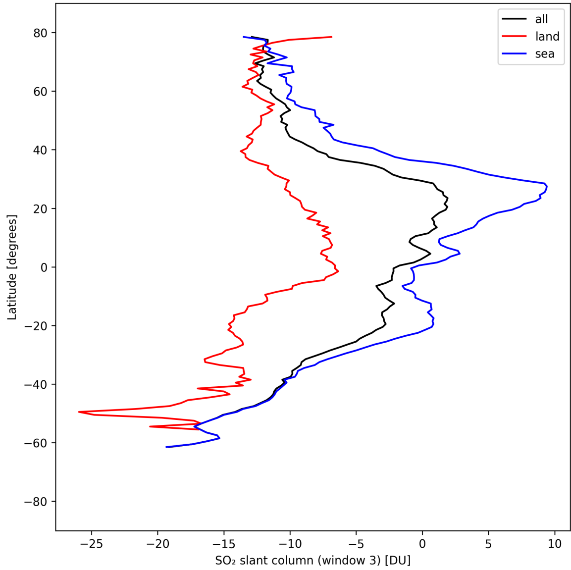
Figure 44: Zonal average of “SO 2 slant column (window 3)” for 2025-09-01 to 2025-09-02.
