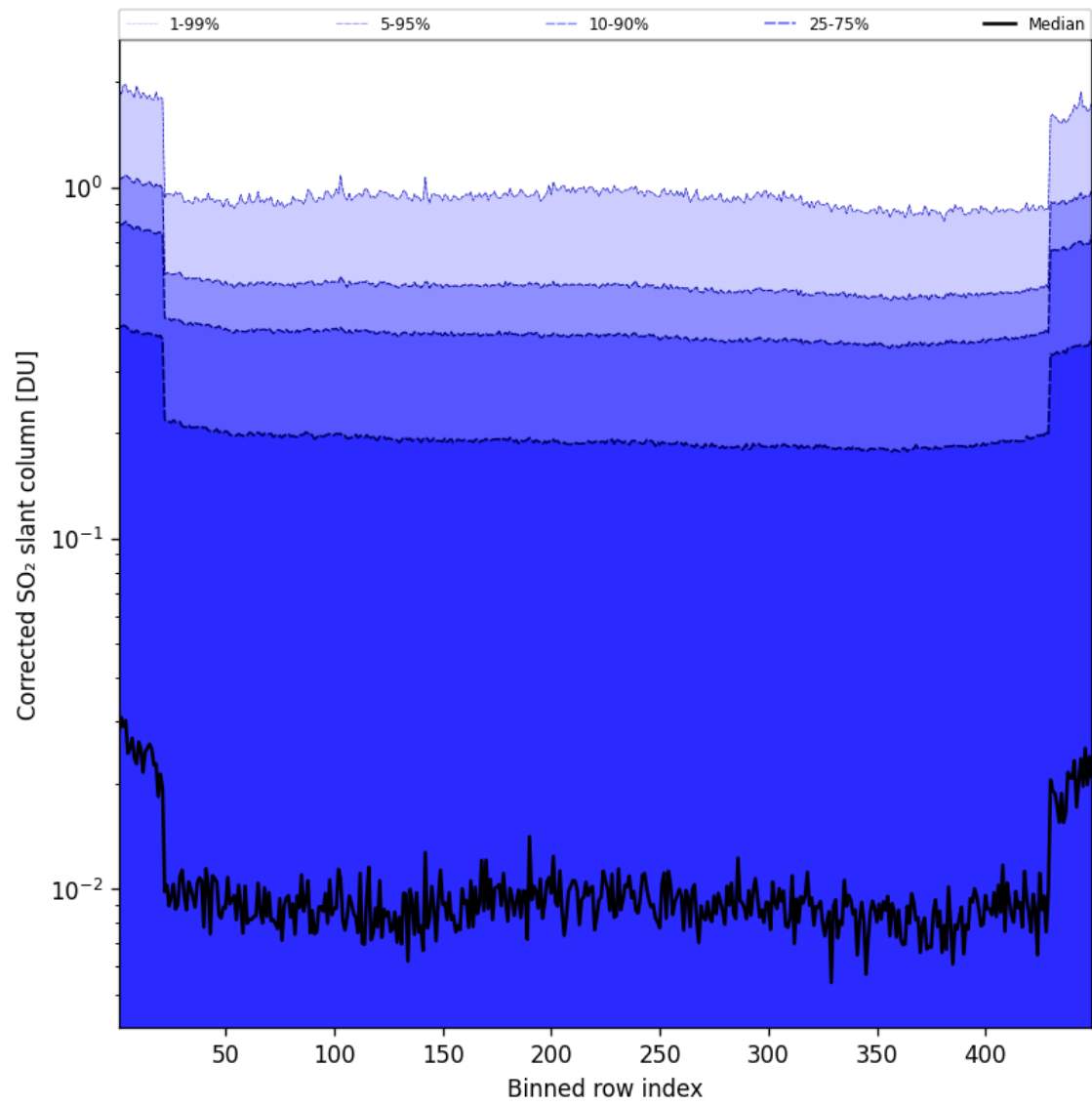
Figure 87: Along track statistics of “Corrected SO 2 slant column” for 2025-09-01 to 2025-09-02
