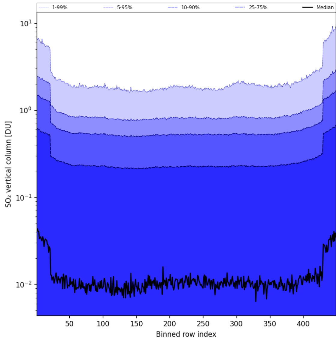
Figure 85: Along track statistics of “SO 2 vertical column” for 2025-09-01 to 2025-09-02
