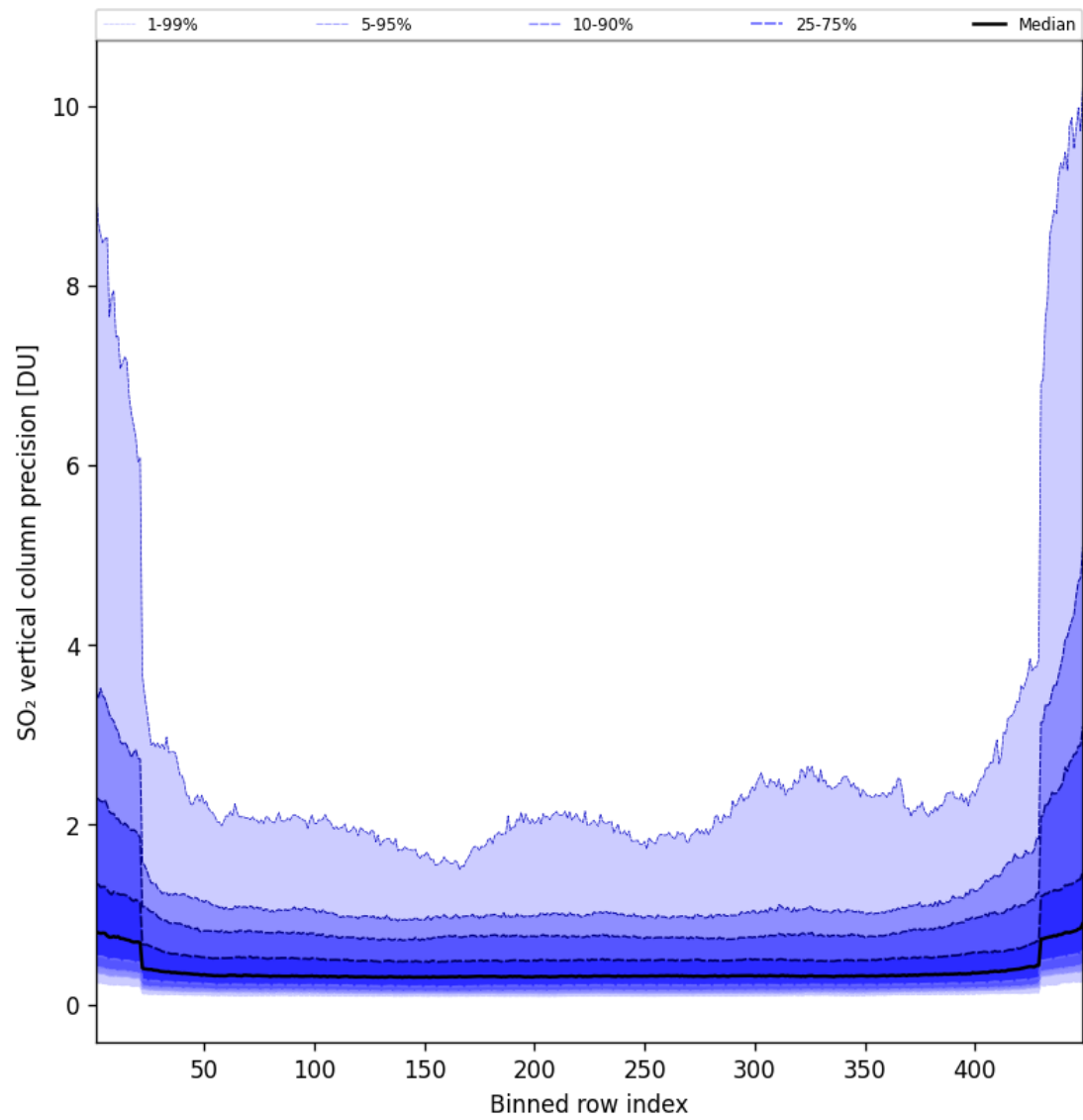
Figure 86: Along track statistics of “SO 2 vertical column precision” for 2025-09-01 to 2025-09-02
