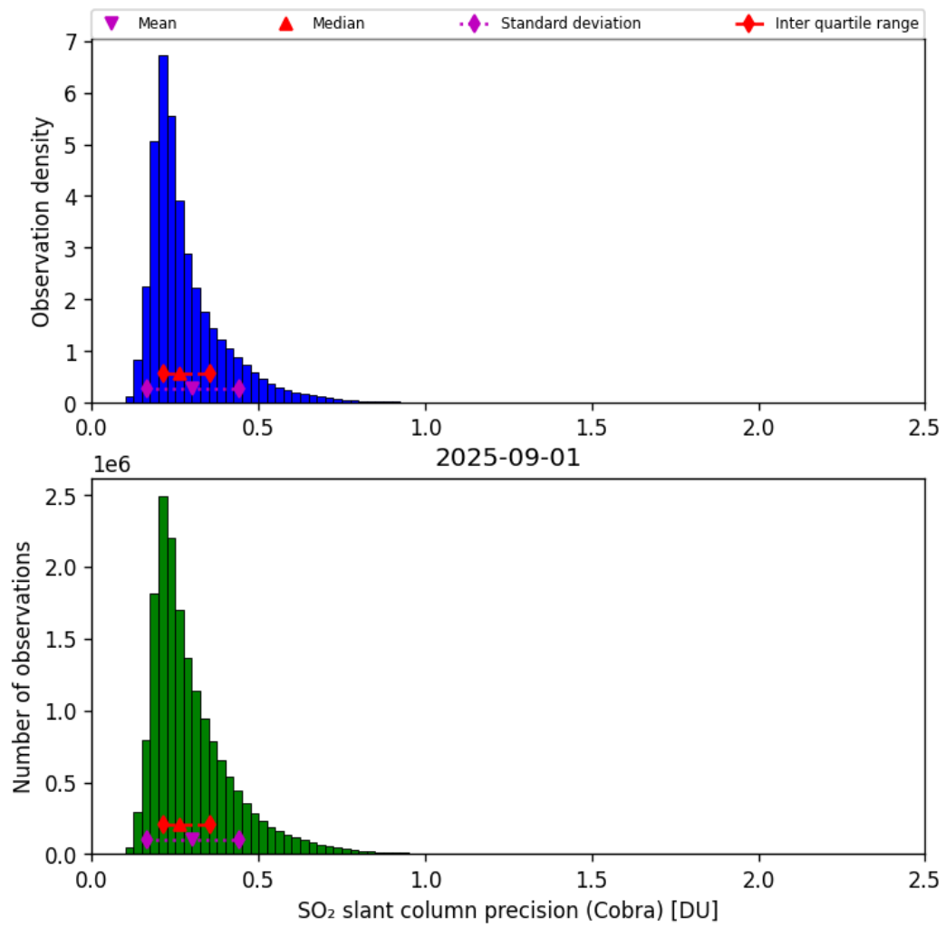
Figure 62: Histogram of “SO 2 slant column precision (Cobra)” for 2025-09-01 to 2025-09-02
