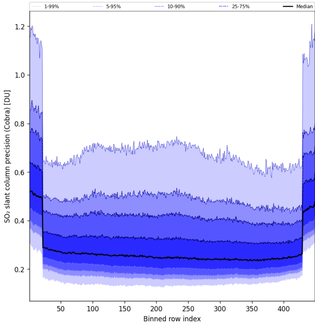
Figure 89: Along track statistics of “SO 2 slant column precision (Cobra)” for 2025-09-01 to 2025-09-02
