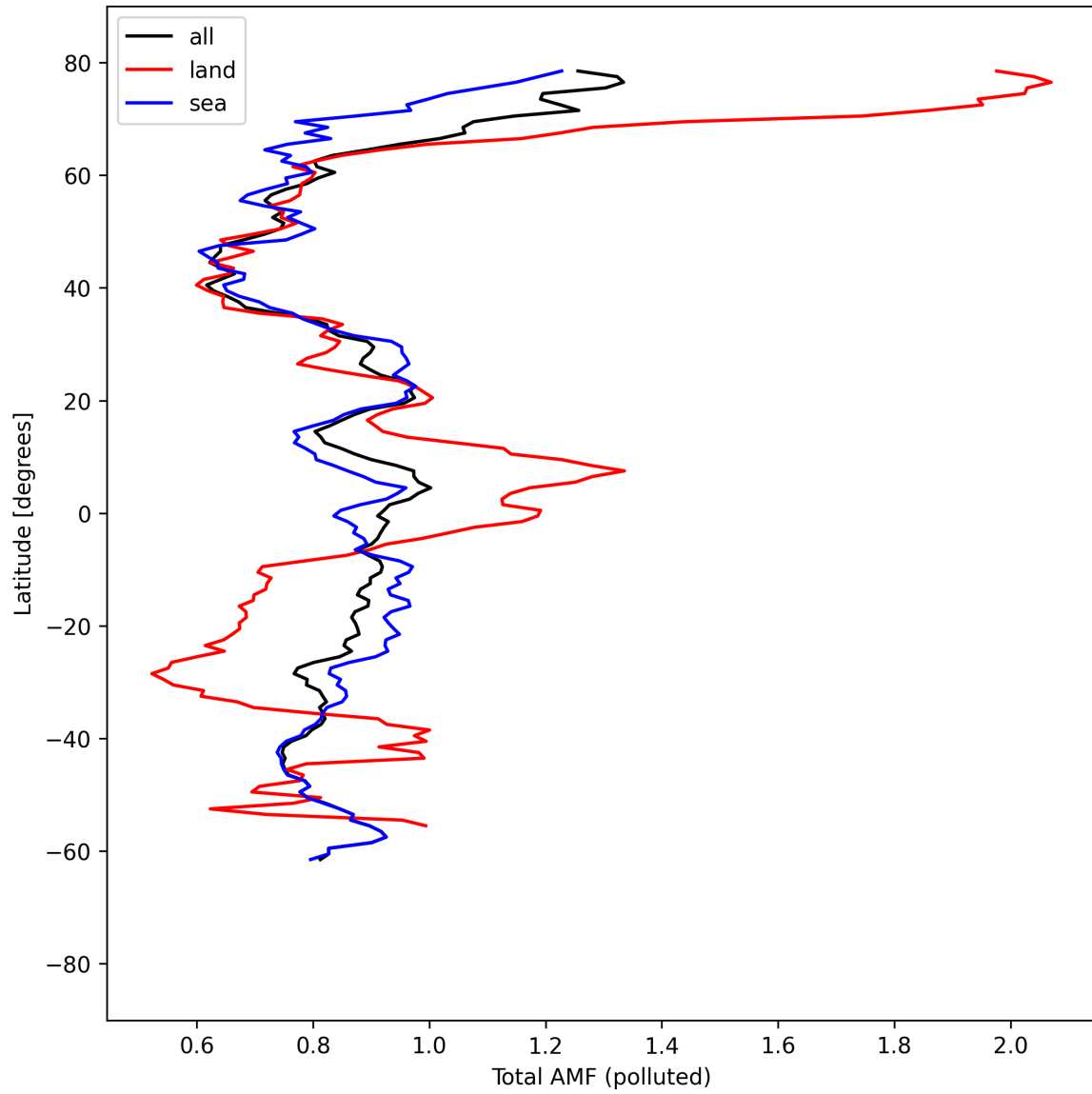
Figure 53: Zonal average of “Total AMF (polluted)” for 2025-09-01 to 2025-09-02.
