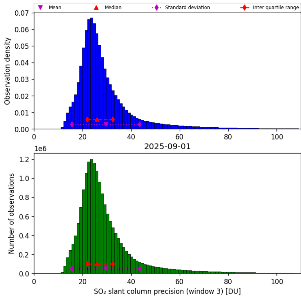
Figure 72: Histogram of “SO 2 slant column precision (window 3)” for 2025-09-01 to 2025-09-02
