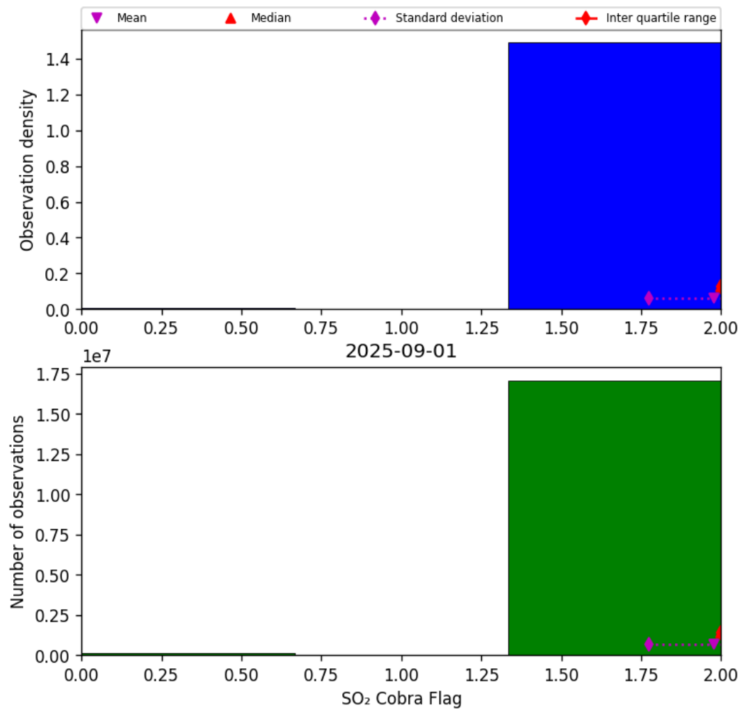
Figure 75: Histogram of "SO 2 Cobra Flag" for 2025-09-01 to 2025-09-02
