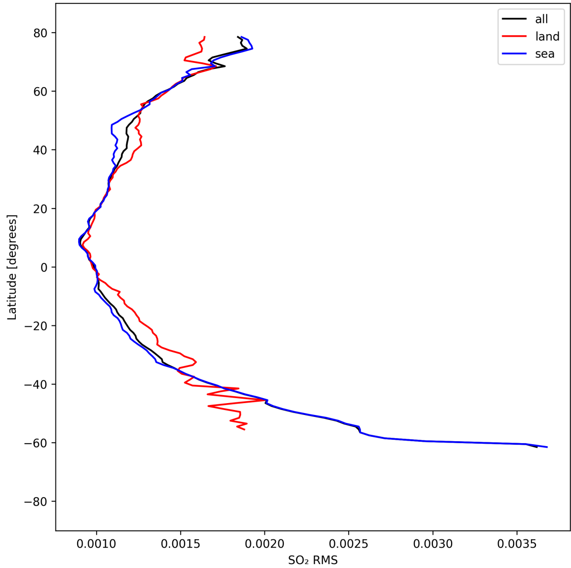
Figure 52: Zonal average of “SO 2 RMS” for 2025-09-01 to 2025-09-02.
