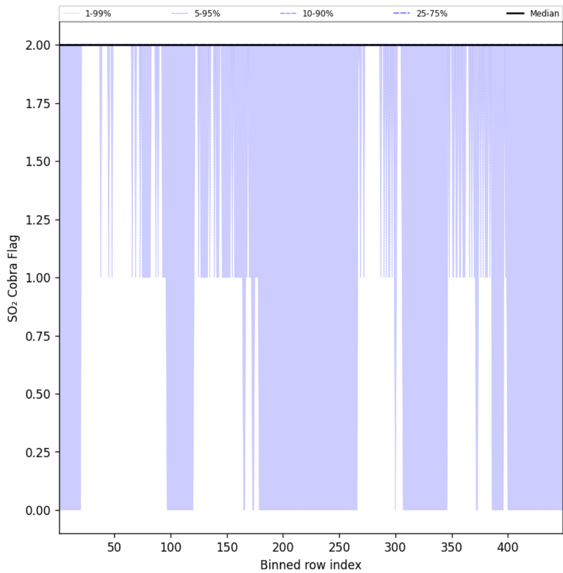
Figure 102: Along track statistics of “SO 2 Cobra Flag” for 2025-09-01 to 2025-09-02
