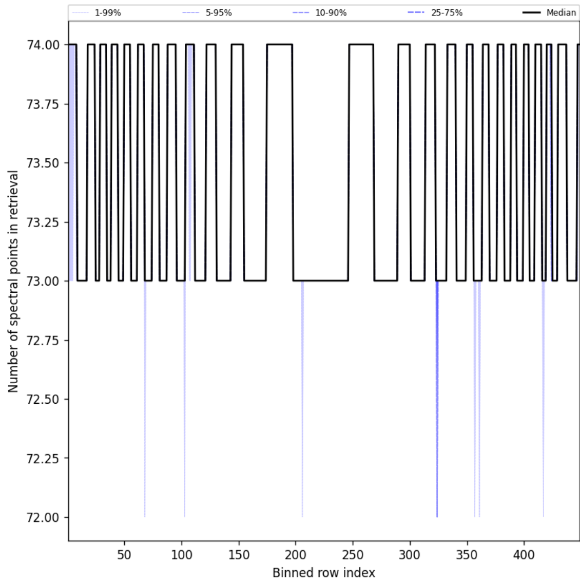
Figure 110: Along track statistics of “Number of spectral points in retrieval” for 2025-09-01 to 2025-09-02
