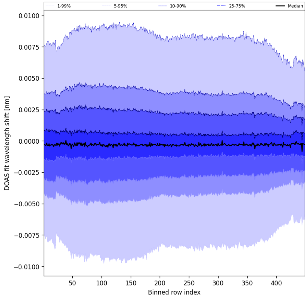
Figure 104: Along track statistics of “DOAS fit wavelength shift” for 2025-09-01 to 2025-09-02
