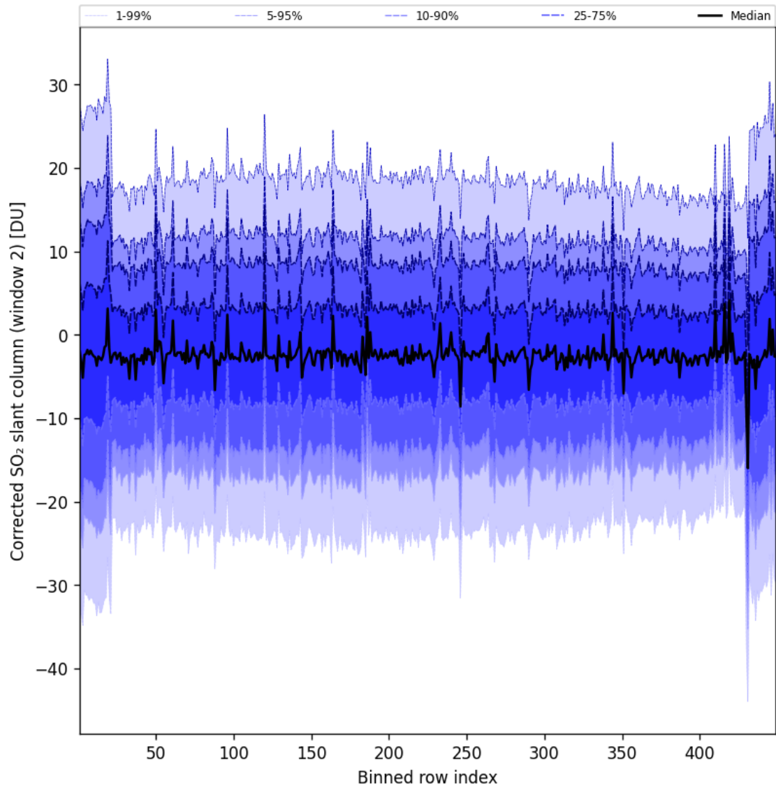
Figure 96: Along track statistics of “Corrected SO 2 slant column (window 2)” for 2025-09-01 to 2025-09-02
