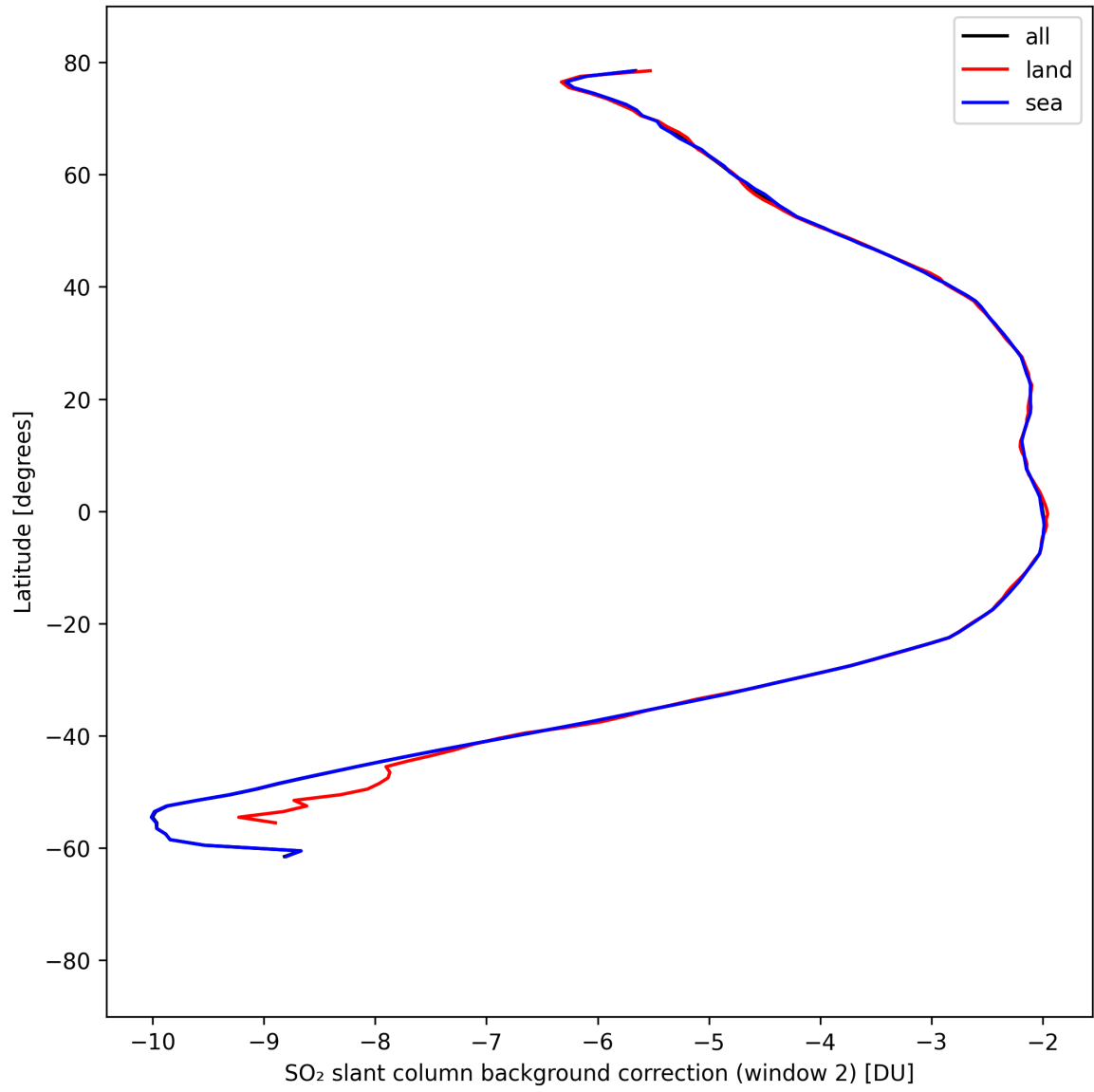
Figure 43: Zonal average of "SO 2 slant column background correction (window 2)" for 2025-09-01 to 2025-09-02.
