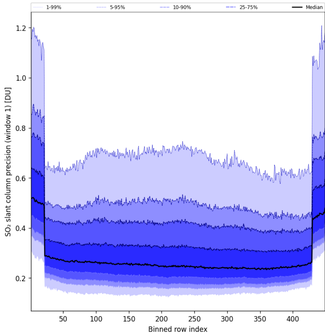
Figure 91: Along track statistics of “SO 2 slant column precision (window 1)” for 2025-09-01 to 2025-09-02
