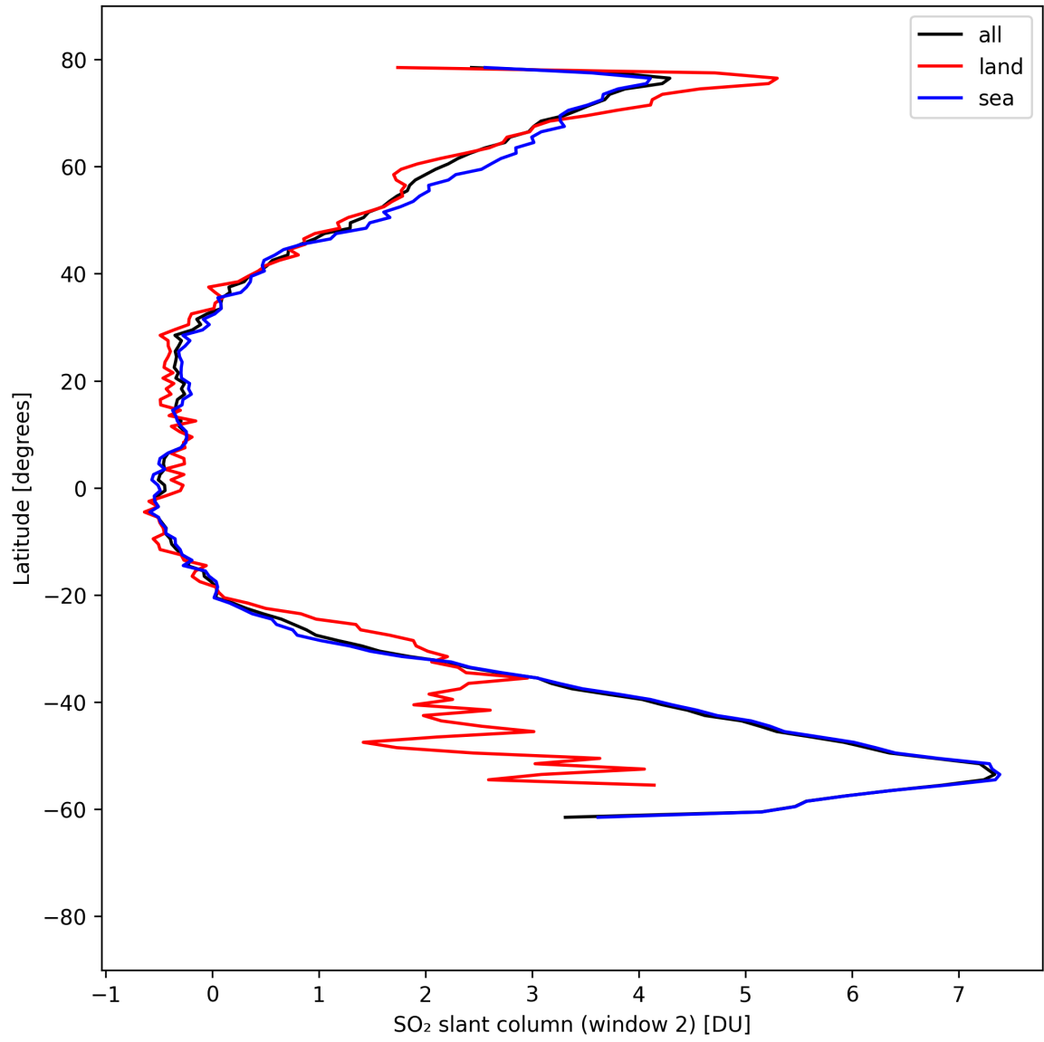
Figure 40: Zonal average of “SO 2 slant column (window 2)” for 2025-09-01 to 2025-09-02.
