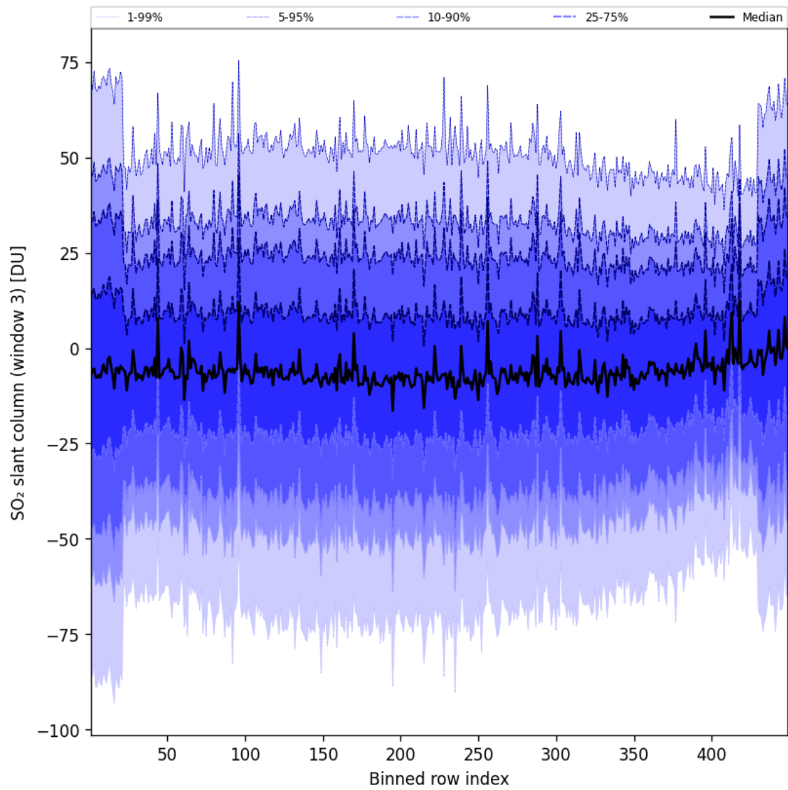
Figure 98: Along track statistics of “SO 2 slant column (window 3)” for 2025-09-01 to 2025-09-02
