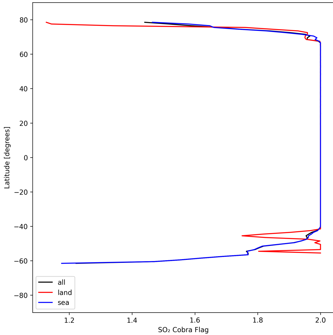
Figure 48: Zonal average of "SO 2 Cobra Flag" for 2025-09-01 to 2025-09-02.
