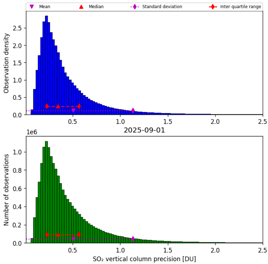
Figure 59: Histogram of “SO 2 vertical column precision” for 2025-09-01 to 2025-09-02
