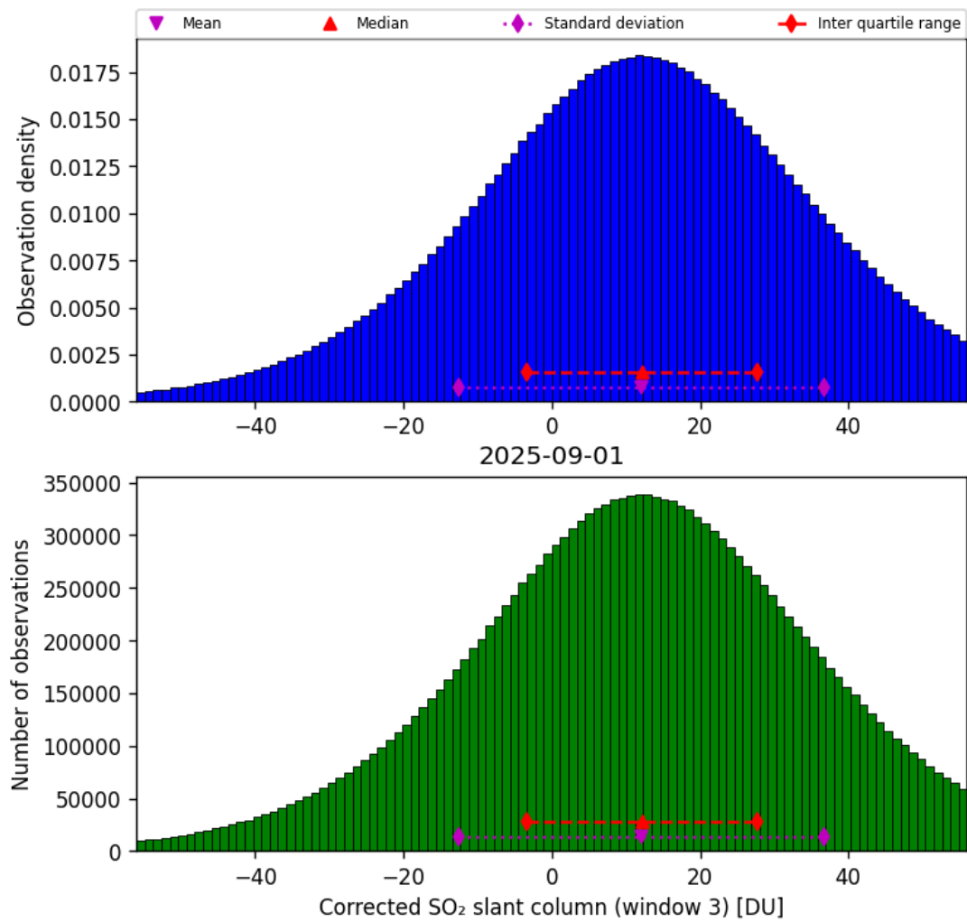
Figure 73: Histogram of “Corrected SO 2 slant column (window 3)” for 2025-09-01 to 2025-09-02
