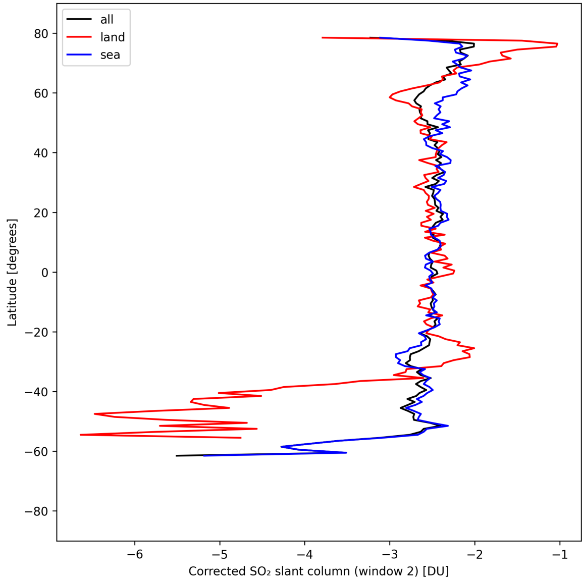
Figure 42: Zonal average of “Corrected SO 2 slant column (window 2)” for 2025-09-01 to 2025-09-02.
