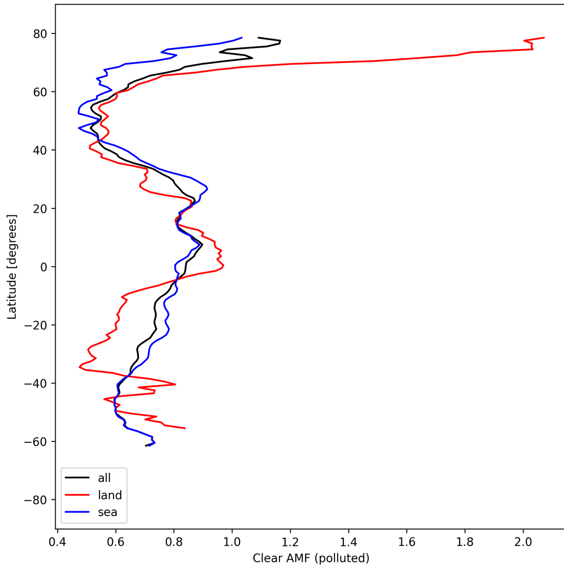
Figure 55: Zonal average of “Clear AMF (polluted)” for 2025-09-01 to 2025-09-02.
