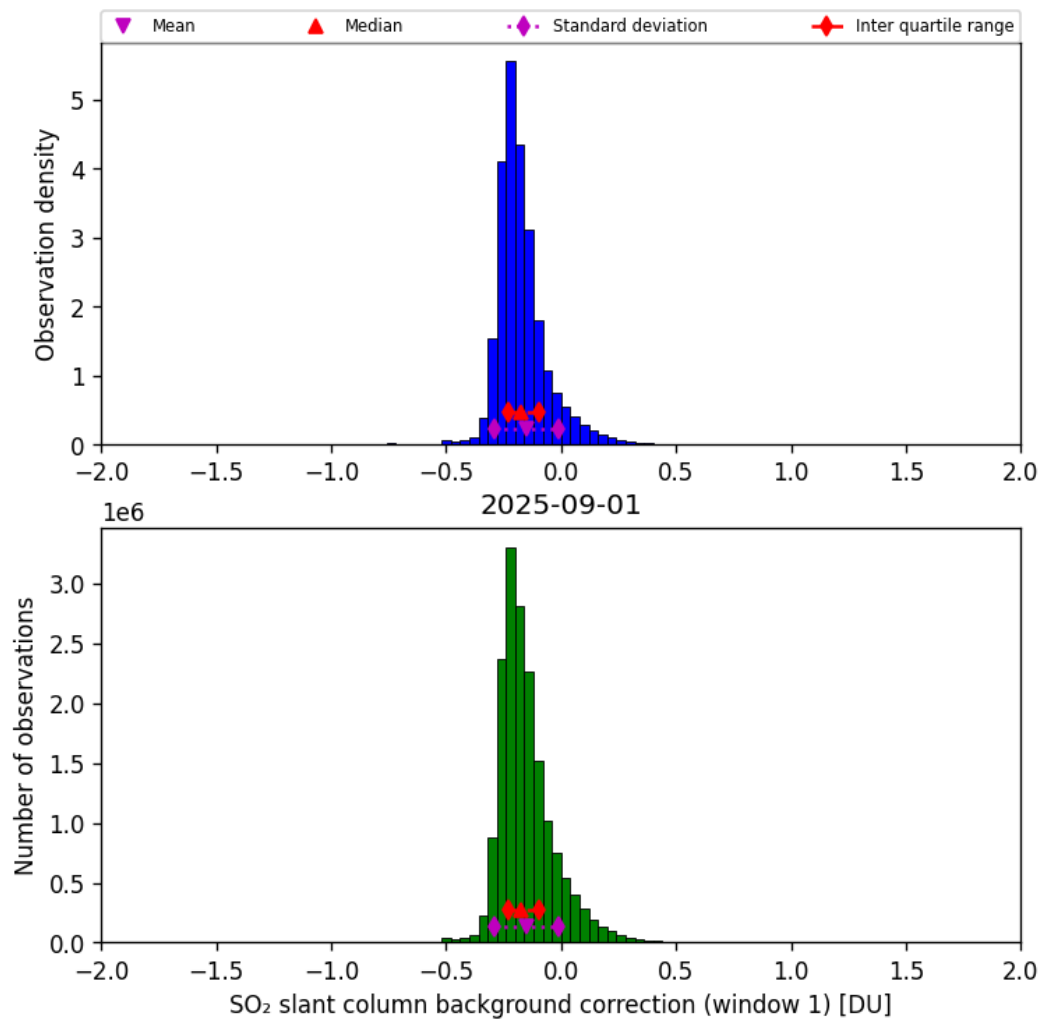
Figure 66: Histogram of “SO 2 slant column background correction (window 1)” for 2025-09-01 to 2025-09-02
