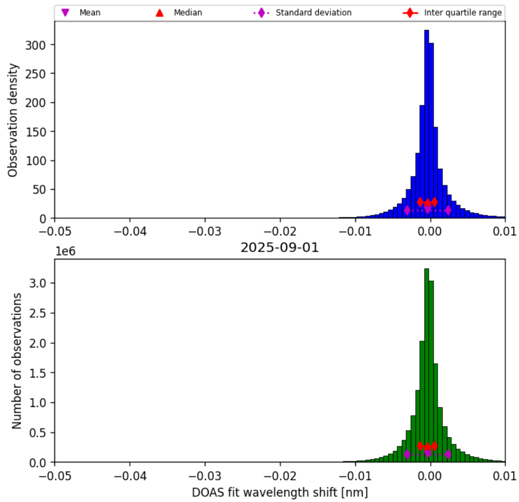
Figure 77: Histogram of “DOAS fit wavelength shift” for 2025-09-01 to 2025-09-02
