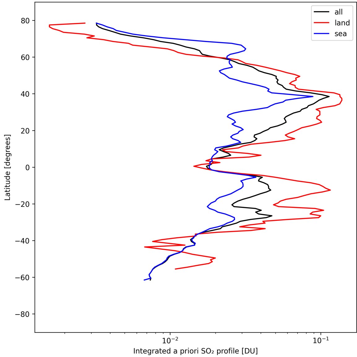
Figure 49: Zonal average of “Integrated a priori SO 2 profile” for 2025-09-01 to 2025-09-02.
