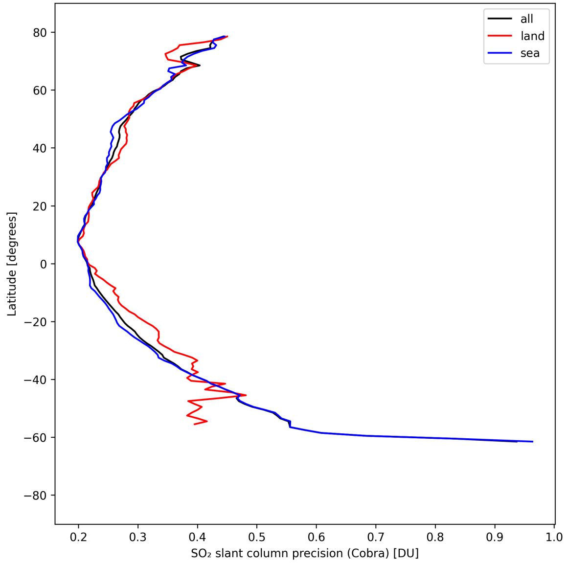
Figure 35: Zonal average of “SO 2 slant column precision (Cobra)” for 2025-09-01 to 2025-09-02.
