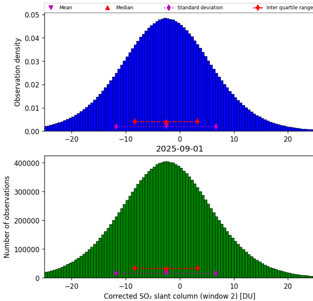
Figure 69: Histogram of “Corrected SO 2 slant column (window 2)” for 2025-09-01 to 2025-09-02
