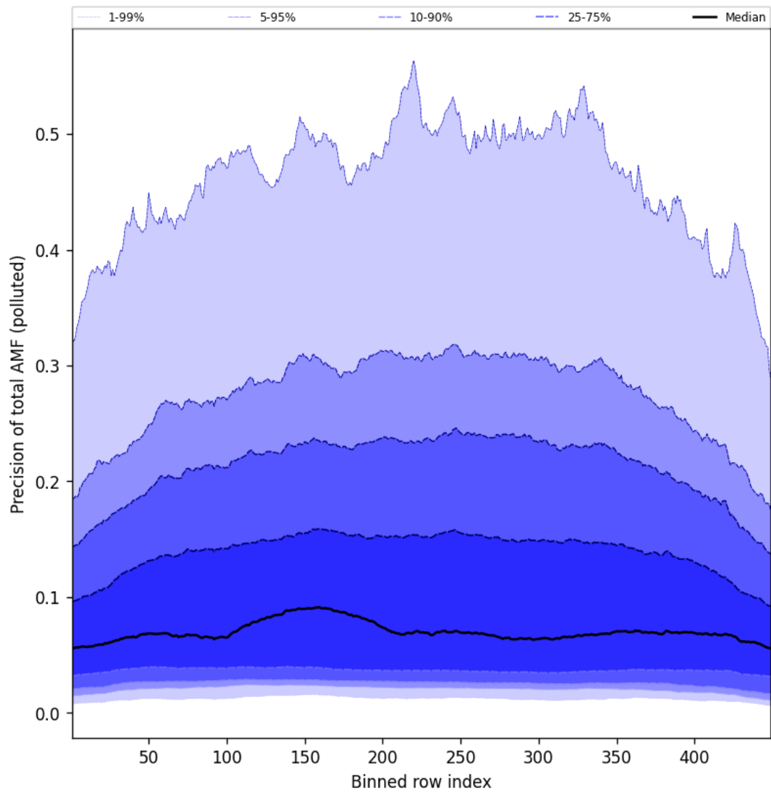
Figure 108: Along track statistics of “Precision of total AMF (polluted)” for 2025-09-01 to 2025-09-02
