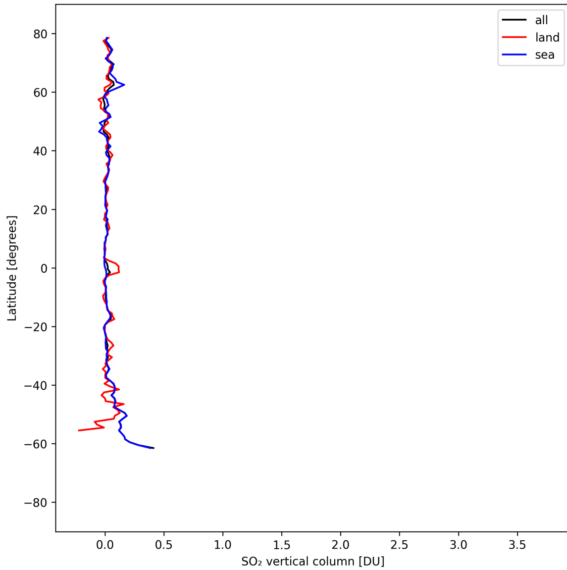
Figure 31: Zonal average of “SO 2 vertical column” for 2025-09-01 to 2025-09-02.
