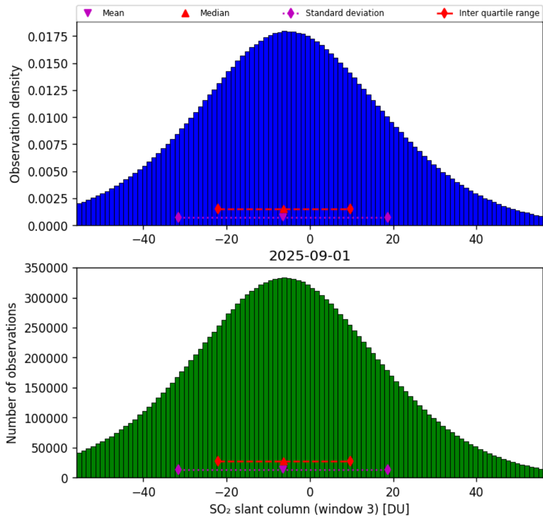
Figure 71: Histogram of “SO 2 slant column (window 3)” for 2025-09-01 to 2025-09-02
