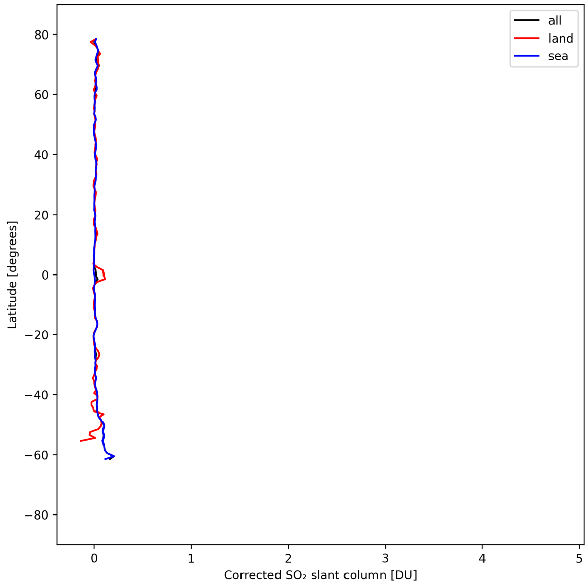
Figure 33: Zonal average of “Corrected SO 2 slant column” for 2025-09-01 to 2025-09-02.
