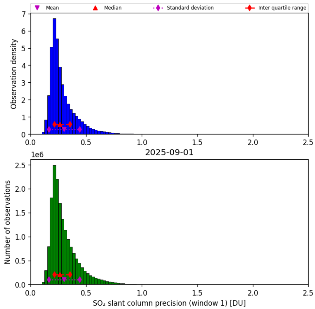
Figure 64: Histogram of “SO 2 slant column precision (window 1)” for 2025-09-01 to 2025-09-02
