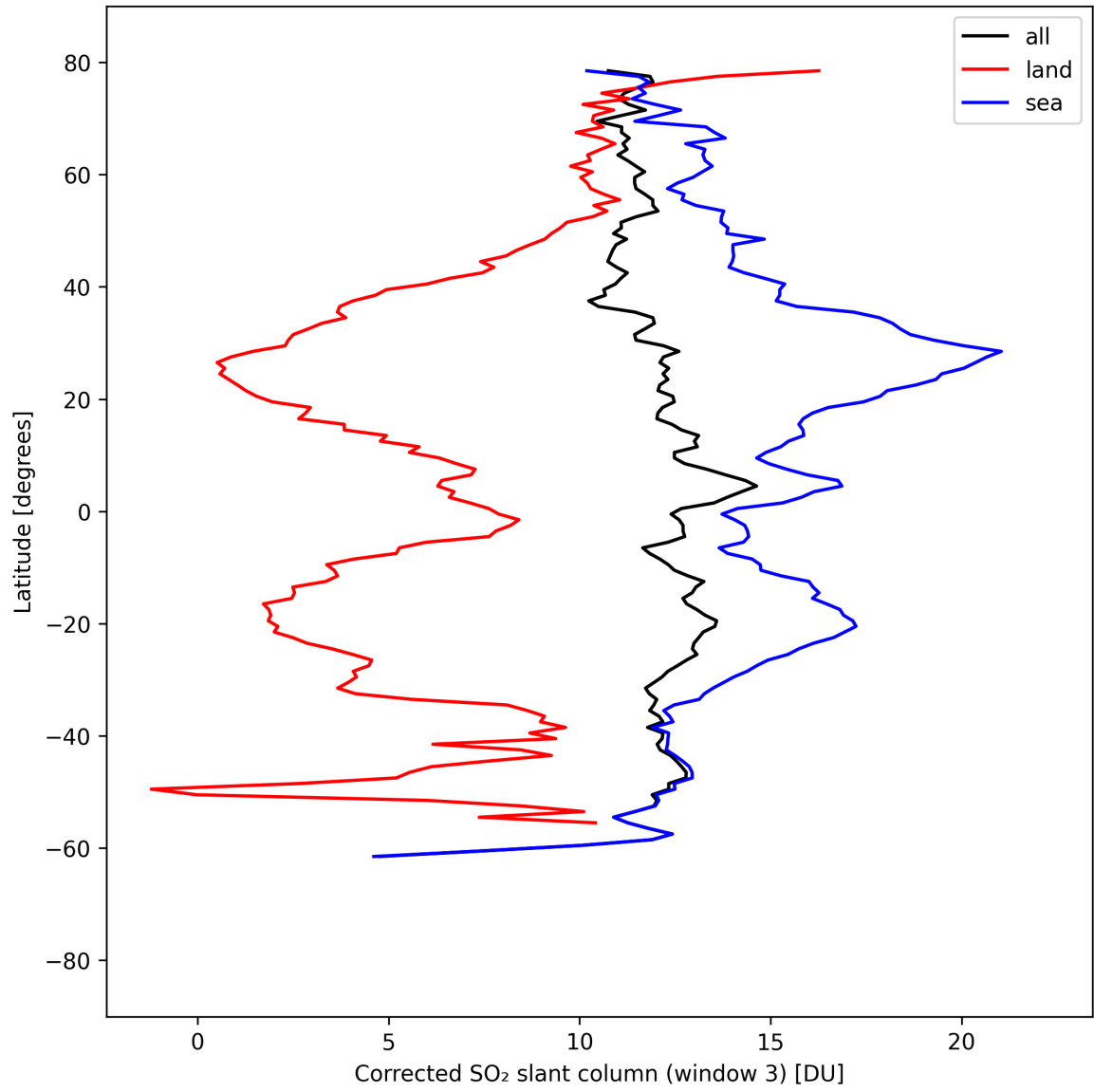
Figure 46: Zonal average of “Corrected SO 2 slant column (window 3)” for 2025-09-01 to 2025-09-02.
