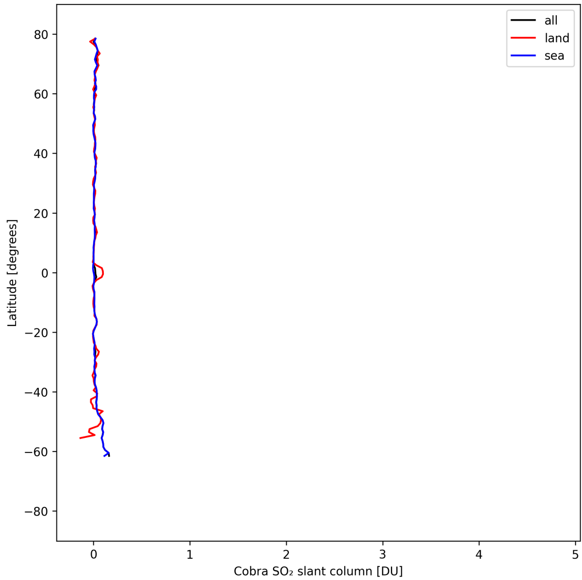
Figure 34: Zonal average of “Cobra SO 2 slant column” for 2025-09-01 to 2025-09-02.
