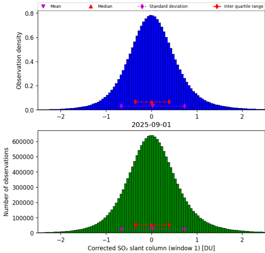
Figure 65: Histogram of “Corrected SO 2 slant column (window 1)” for 2025-09-01 to 2025-09-02
