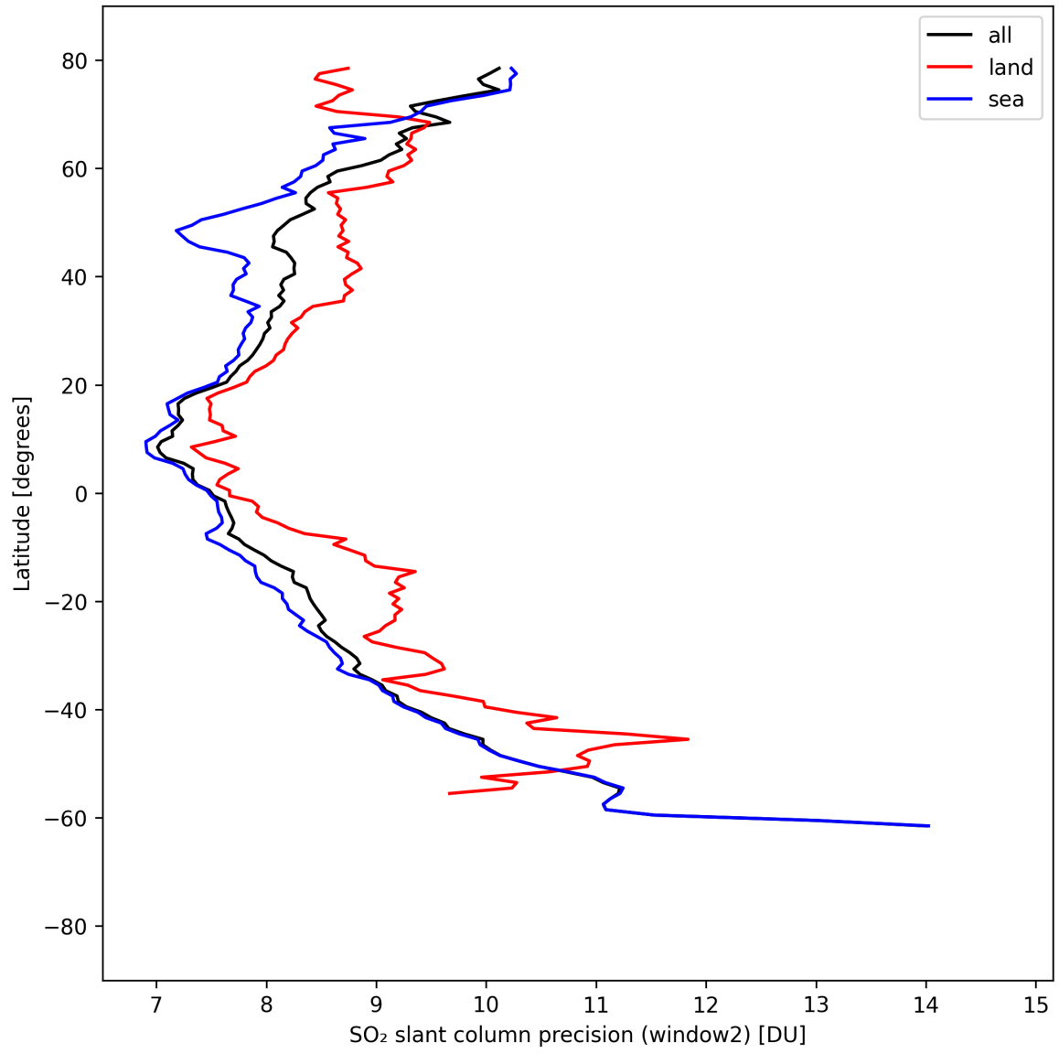
Figure 41: Zonal average of “SO 2 slant column precision (window2)” for 2025-09-01 to 2025-09-02.
