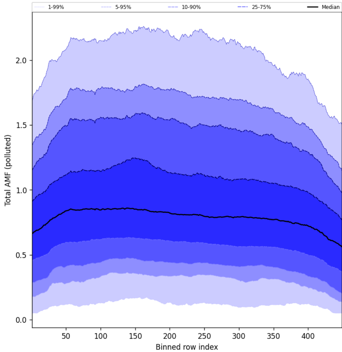
Figure 107: Along track statistics of “Total AMF (polluted)” for 2025-09-01 to 2025-09-02
