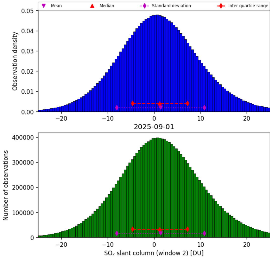
Figure 67: Histogram of “SO 2 slant column (window 2)” for 2025-09-01 to 2025-09-02
