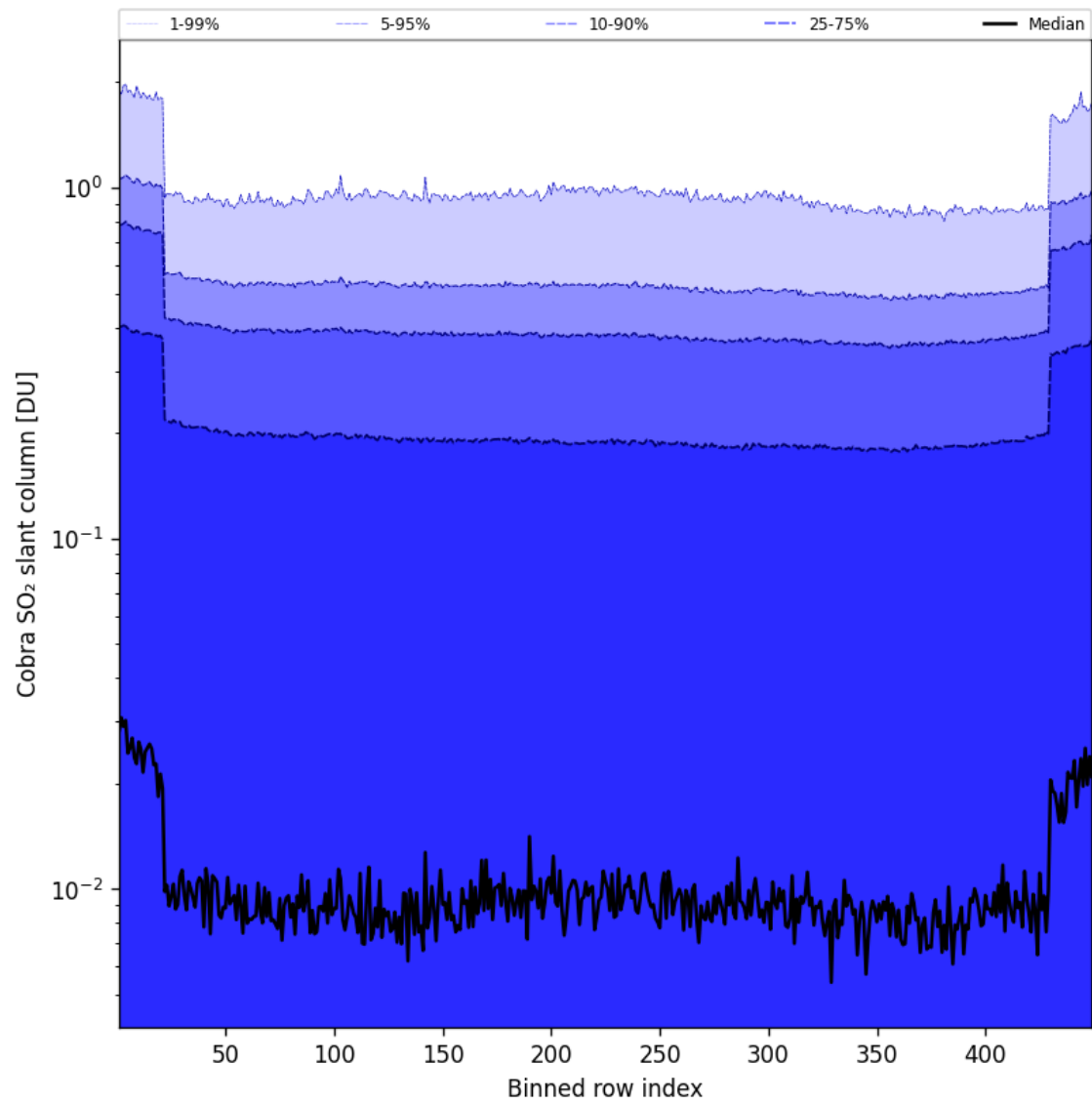
Figure 88: Along track statistics of “Cobra SO 2 slant column” for 2025-09-01 to 2025-09-02
