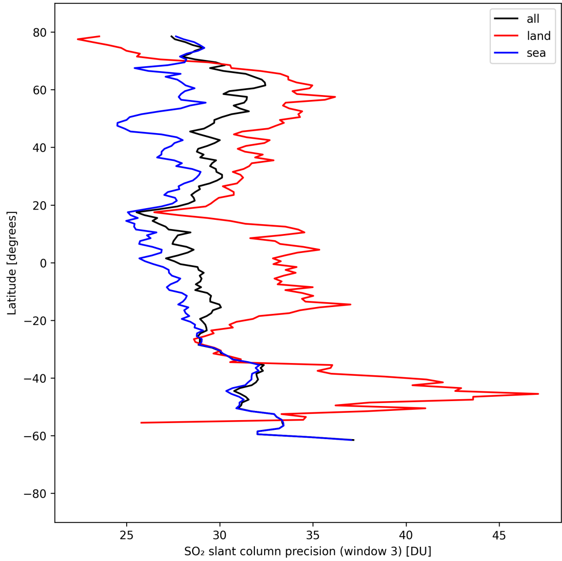
Figure 45: Zonal average of “SO 2 slant column precision (window 3)” for 2025-09-01 to 2025-09-02.
