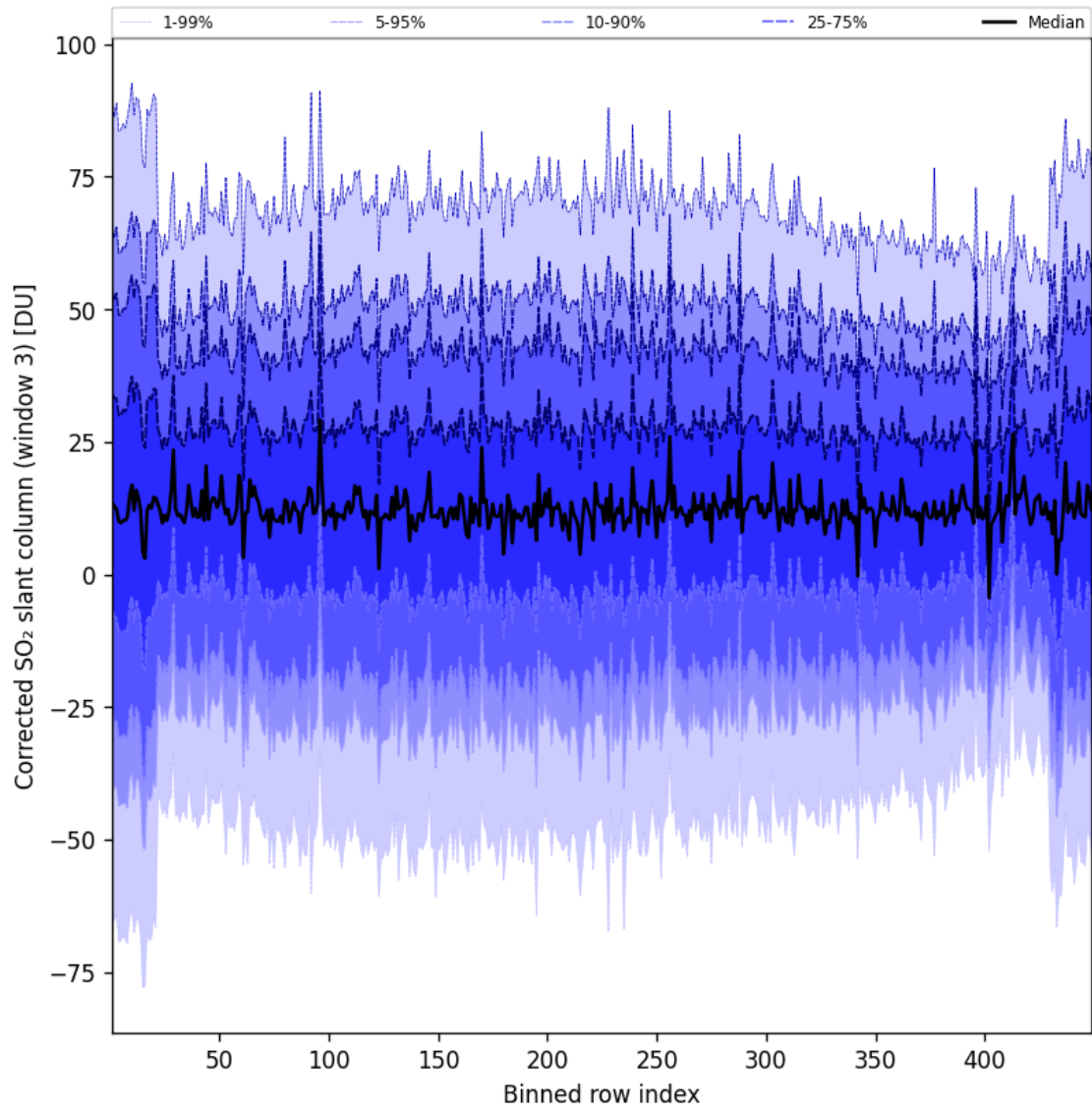
Figure 100: Along track statistics of “Corrected SO 2 slant column (window 3)” for 2025-09-01 to 2025-09-02
