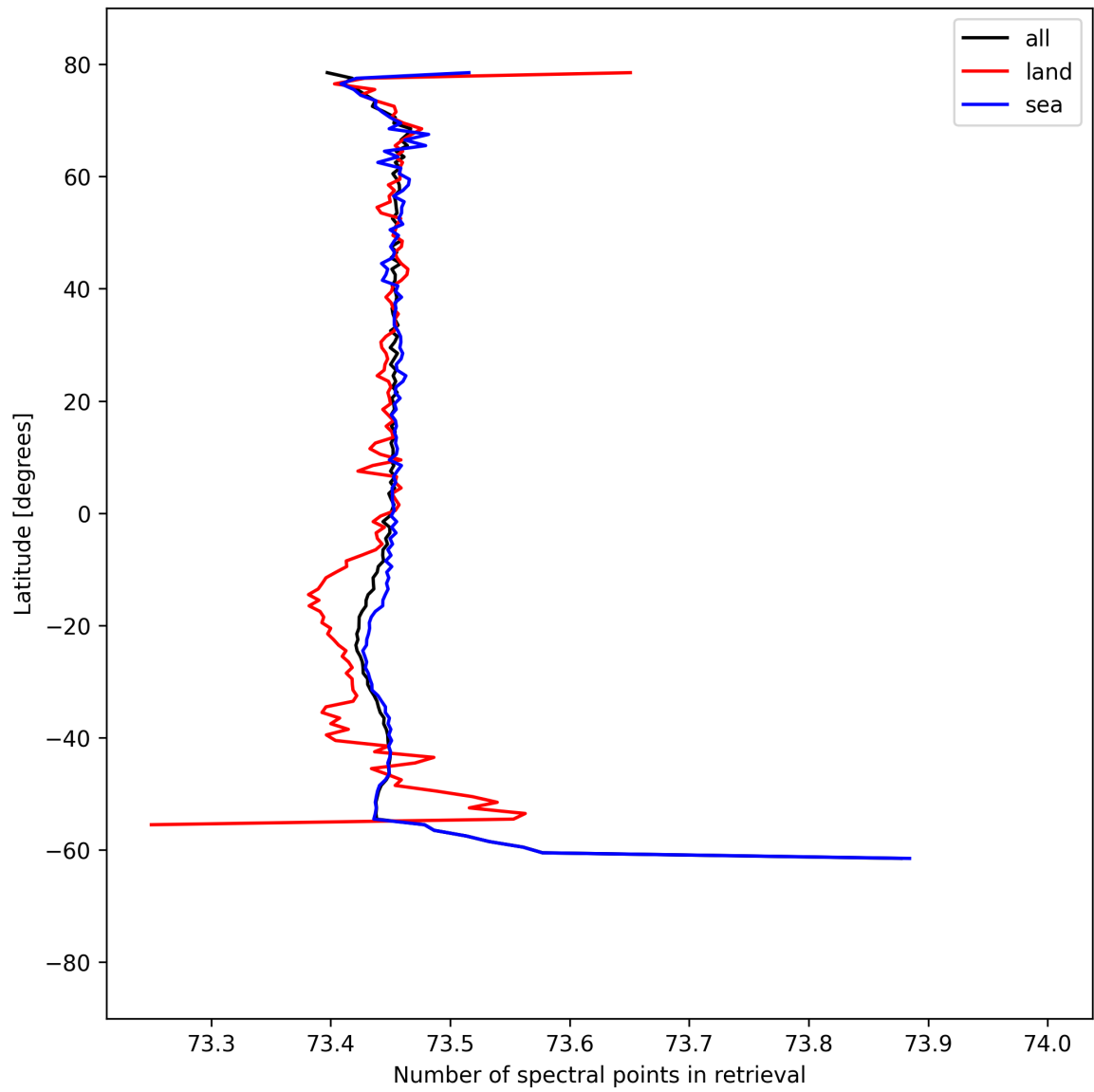
Figure 56: Zonal average of “Number of spectral points in retrieval” for 2025-09-01 to 2025-09-02.
