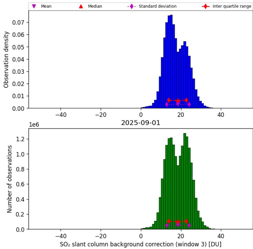
Figure 74: Histogram of “SO 2 slant column background correction (window 3)” for 2025-09-01 to 2025-09-02
