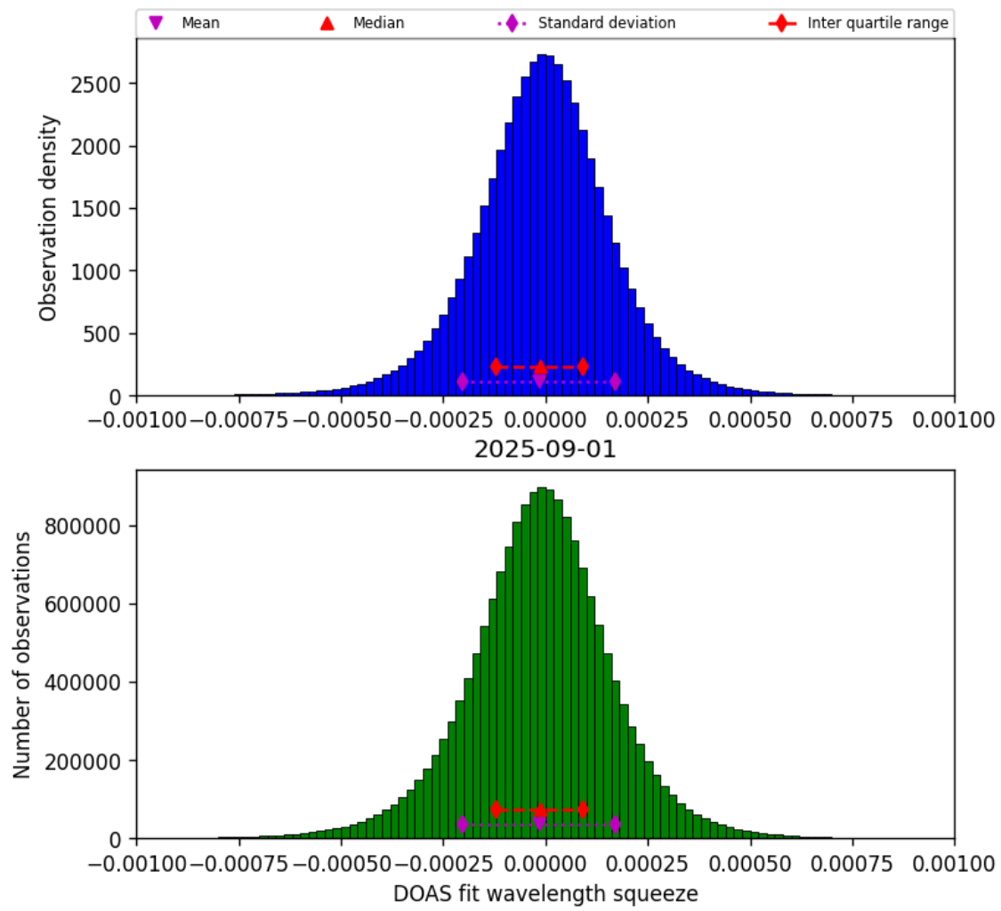
Figure 78: Histogram of “DOAS fit wavelength squeeze” for 2025-09-01 to 2025-09-02
