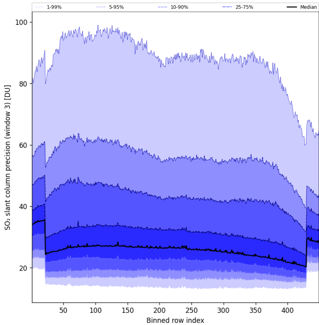
Figure 99: Along track statistics of “SO 2 slant column precision (window 3)” for 2025-09-01 to 2025-09-02
