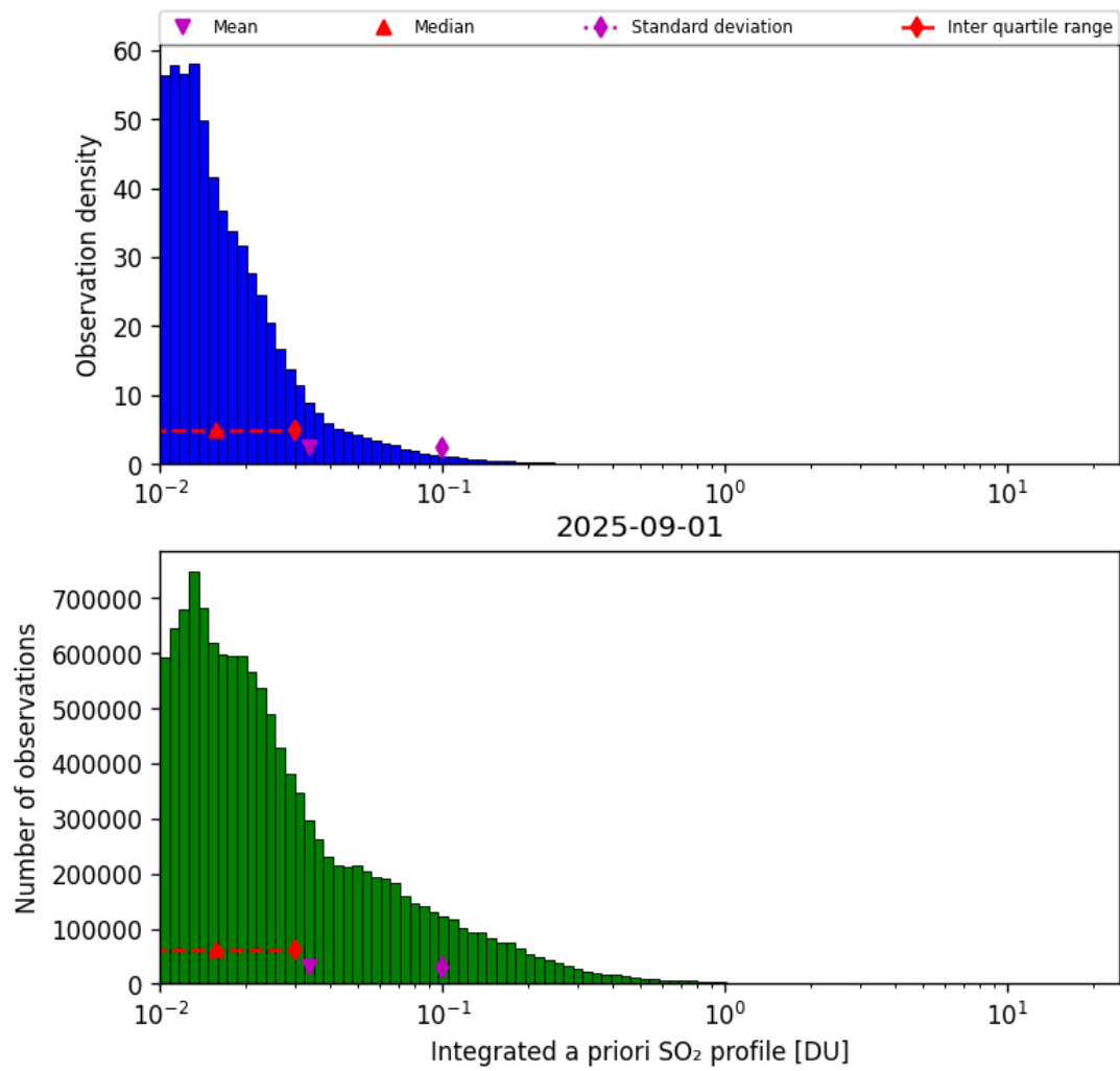
Figure 76: Histogram of “Integrated a priori SO 2 profile” for 2025-09-01 to 2025-09-02
