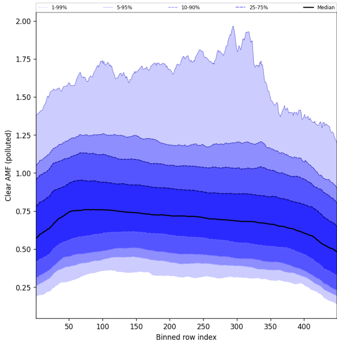
Figure 109: Along track statistics of “Clear AMF (polluted)” for 2025-09-01 to 2025-09-02
