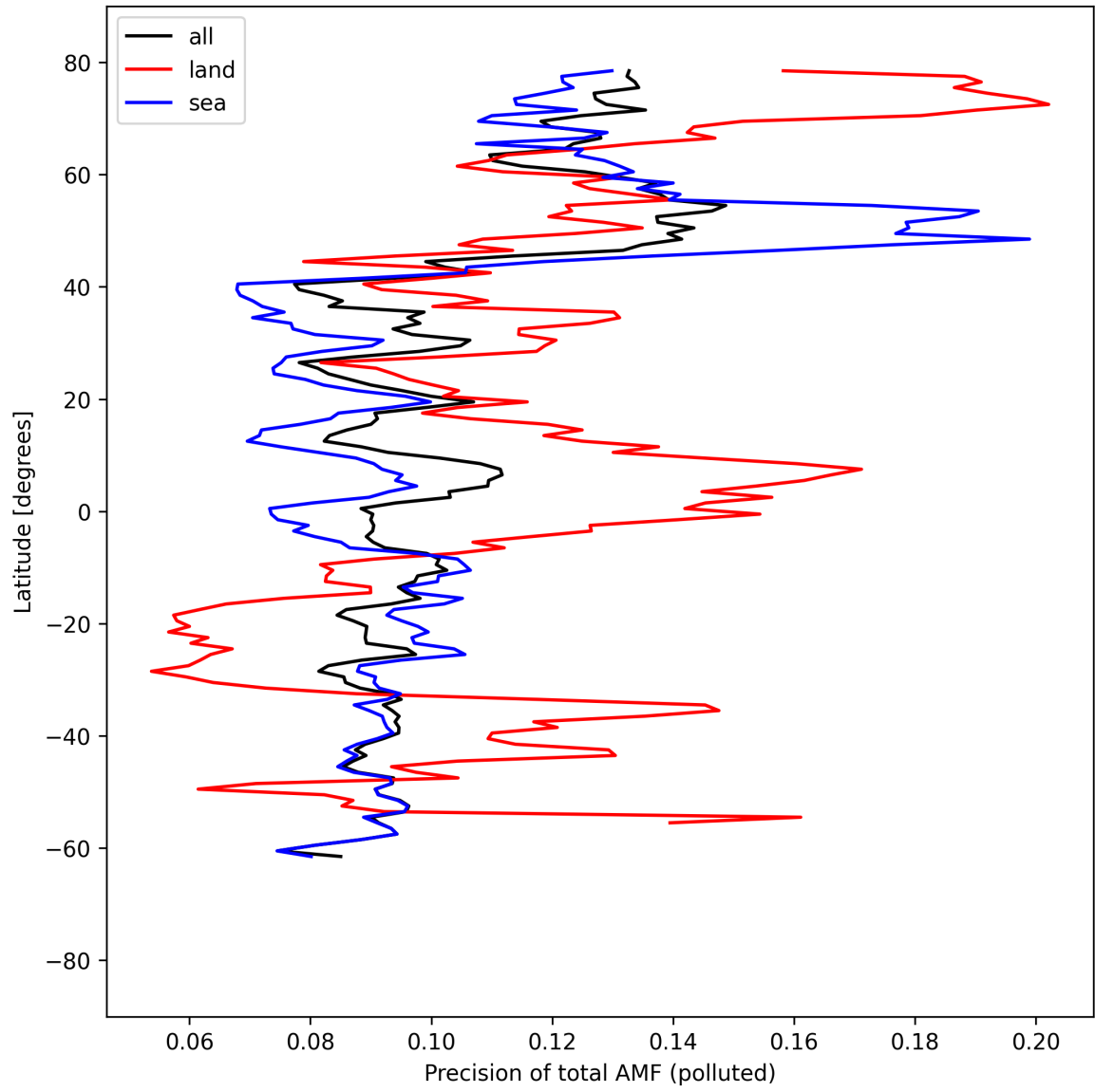
Figure 54: Zonal average of “Precision of total AMF (polluted)” for 2025-09-01 to 2025-09-02.
