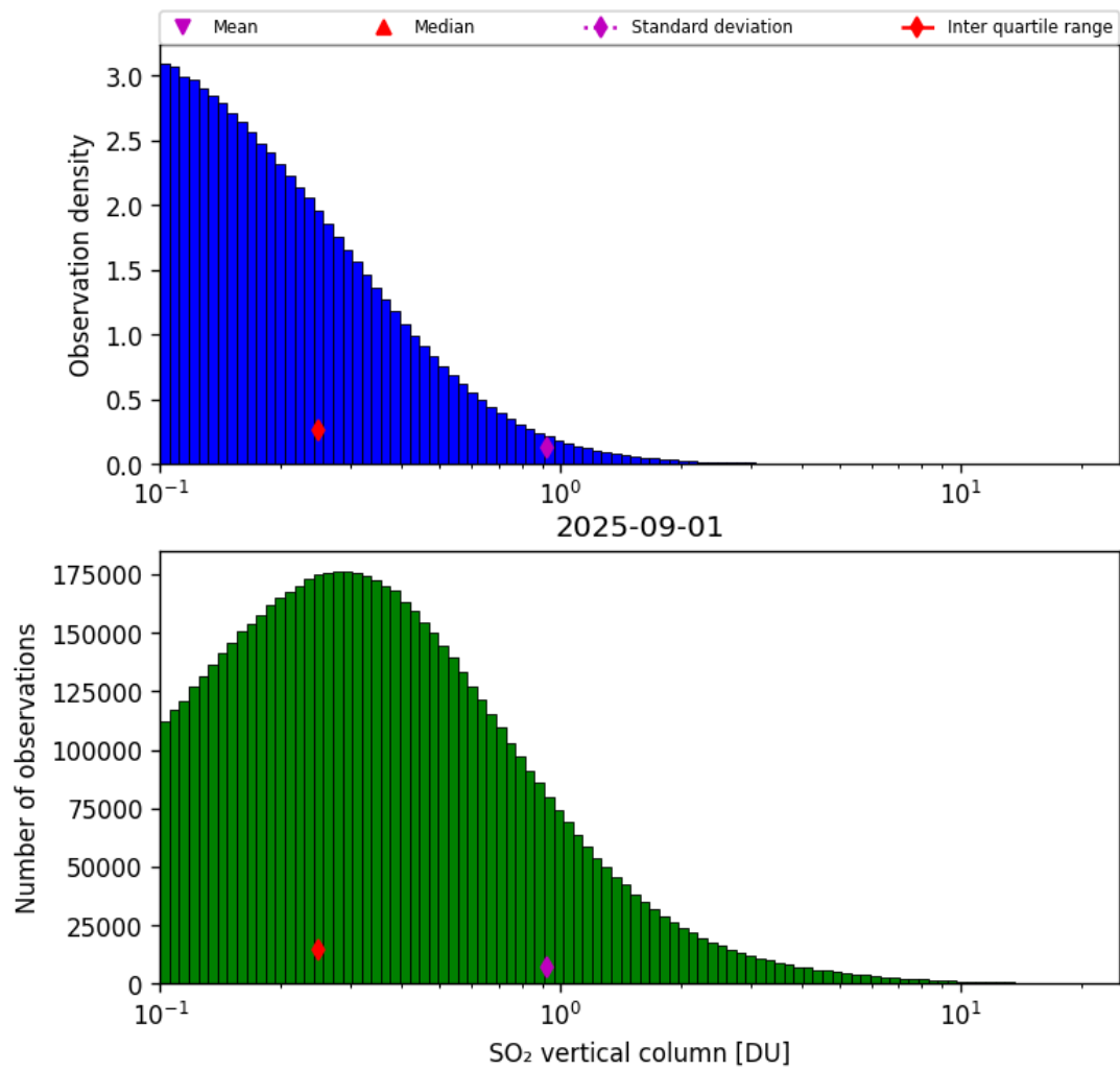
Figure 58: Histogram of “SO 2 vertical column” for 2025-09-01 to 2025-09-02
