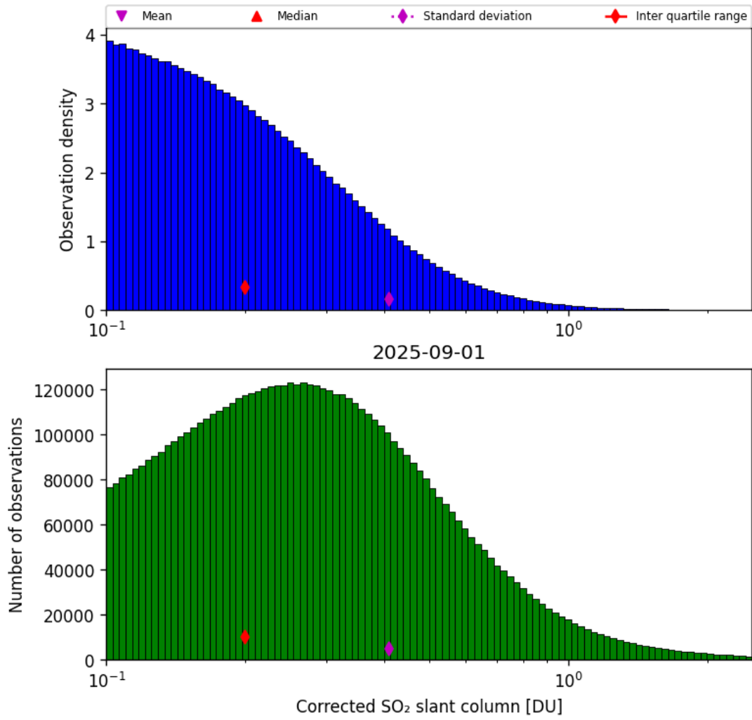
Figure 60: Histogram of “Corrected SO 2 slant column” for 2025-09-01 to 2025-09-02
