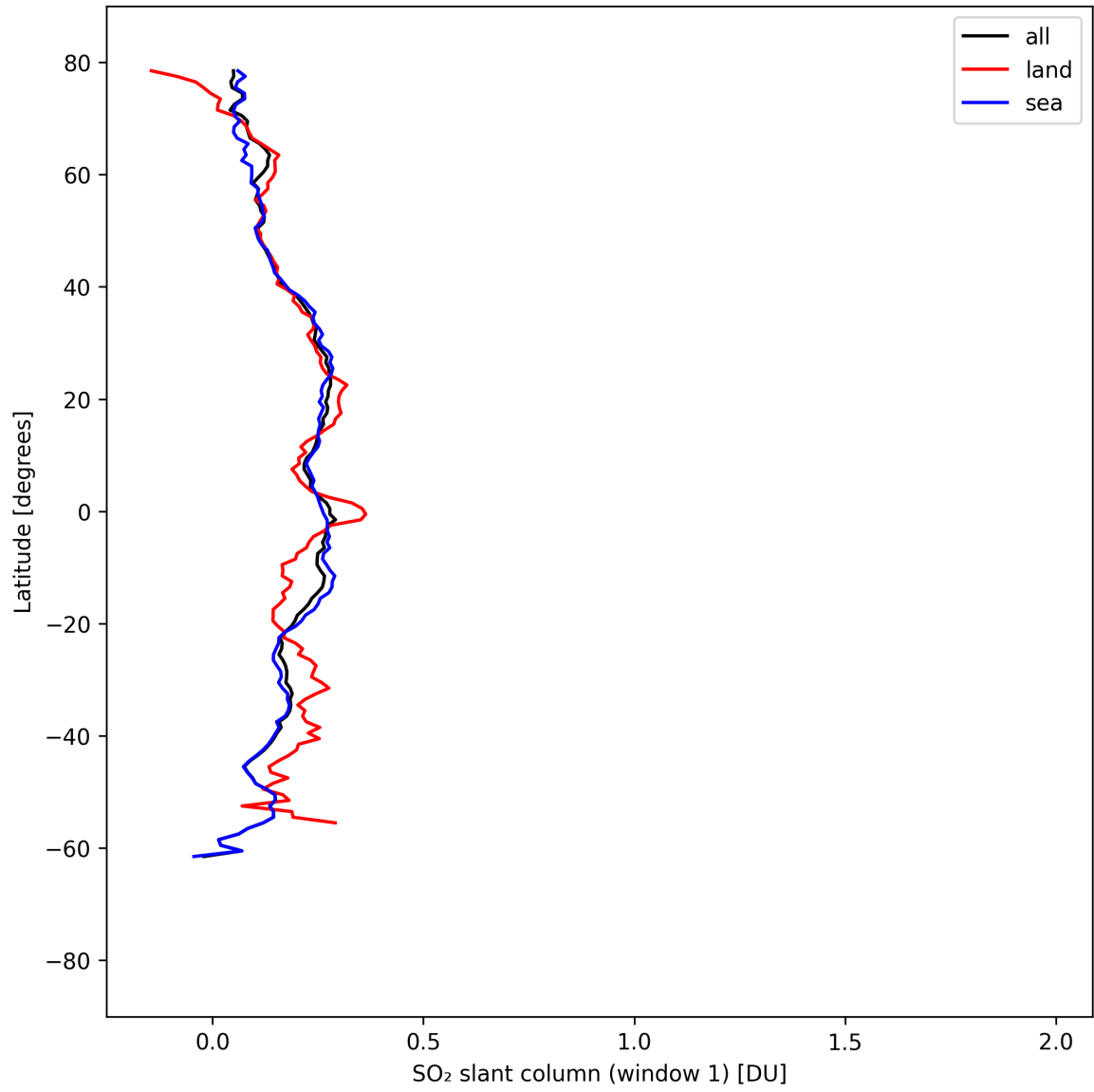
Figure 36: Zonal average of “SO 2 slant column (window 1)” for 2025-09-01 to 2025-09-02.
