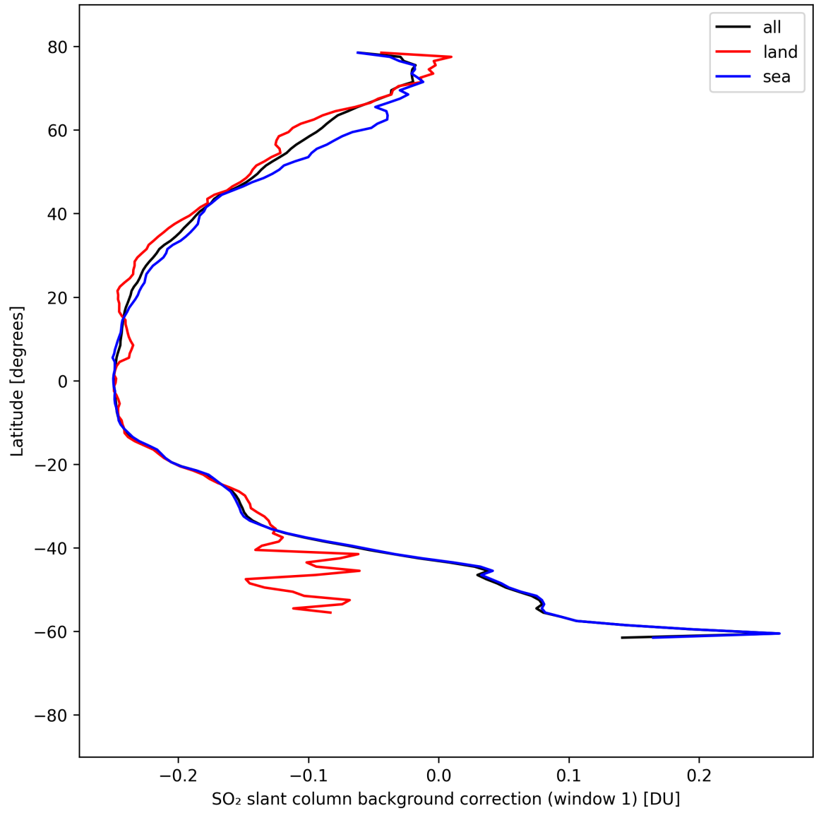
Figure 39: Zonal average of “SO 2 slant column background correction (window 1)” for 2025-09-01 to 2025-09-02.
