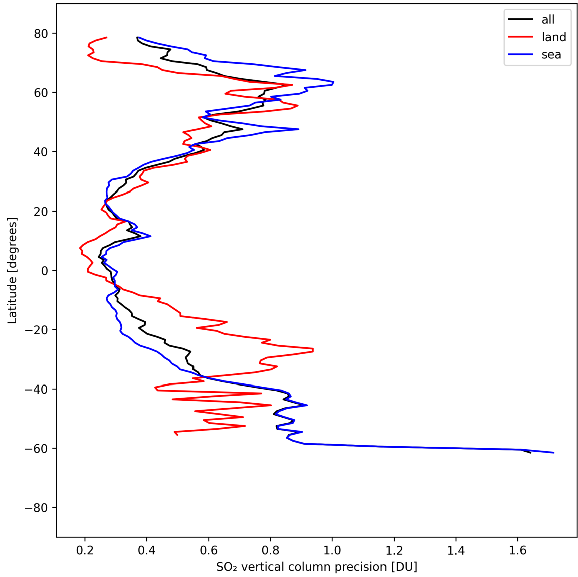
Figure 32: Zonal average of “SO 2 vertical column precision” for 2025-09-01 to 2025-09-02.
