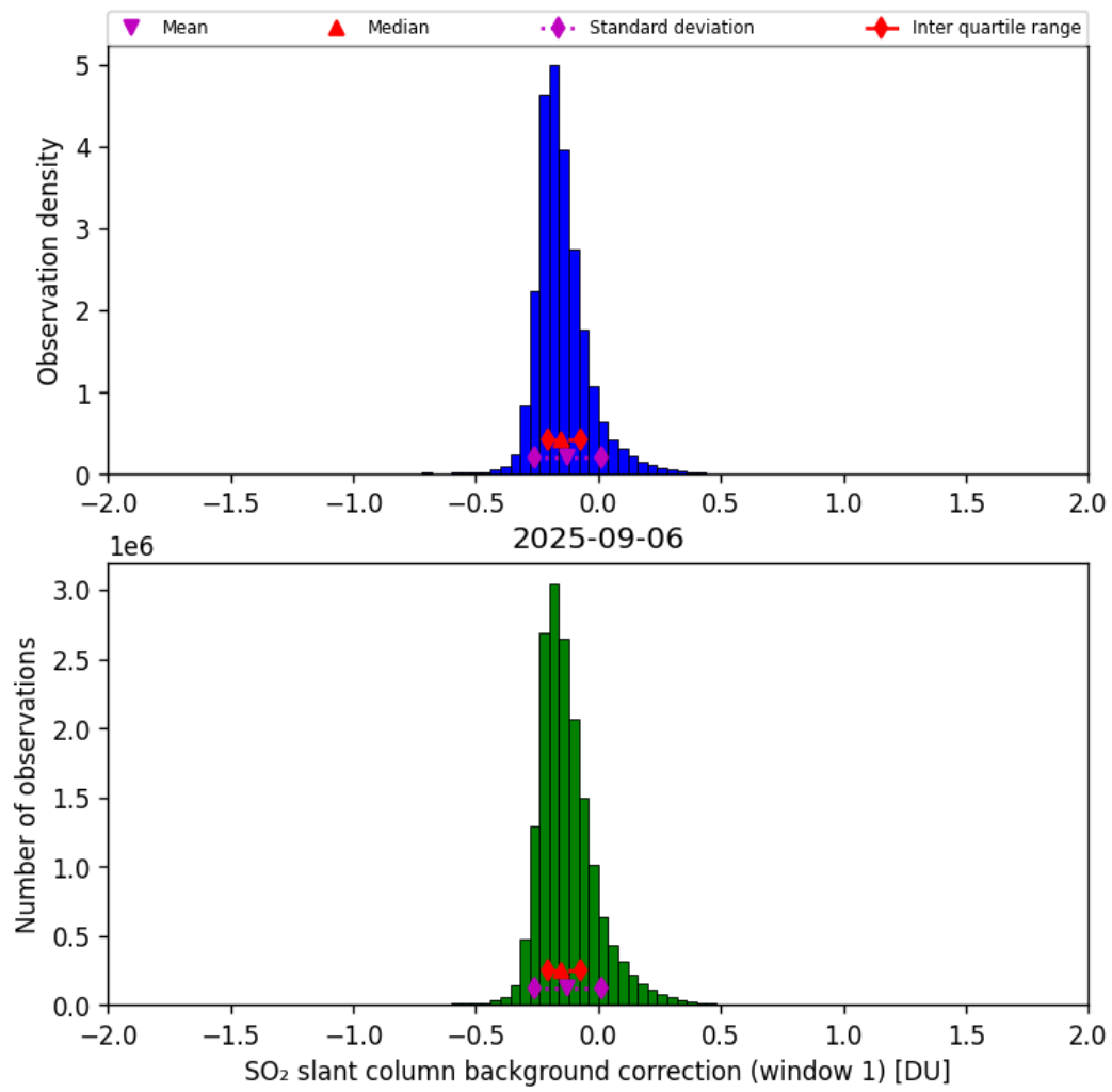
Figure 66: Histogram of “SO 2 slant column background correction (window 1)” for 2025-09-06 to 2025-09-07
