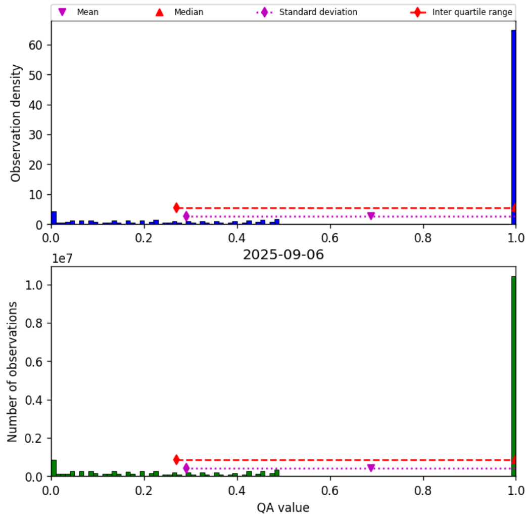
Figure 57: Histogram of “QA value” for 2025-09-06 to 2025-09-07
