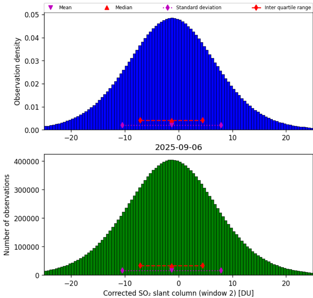
Figure 69: Histogram of “Corrected SO 2 slant column (window 2)” for 2025-09-06 to 2025-09-07
