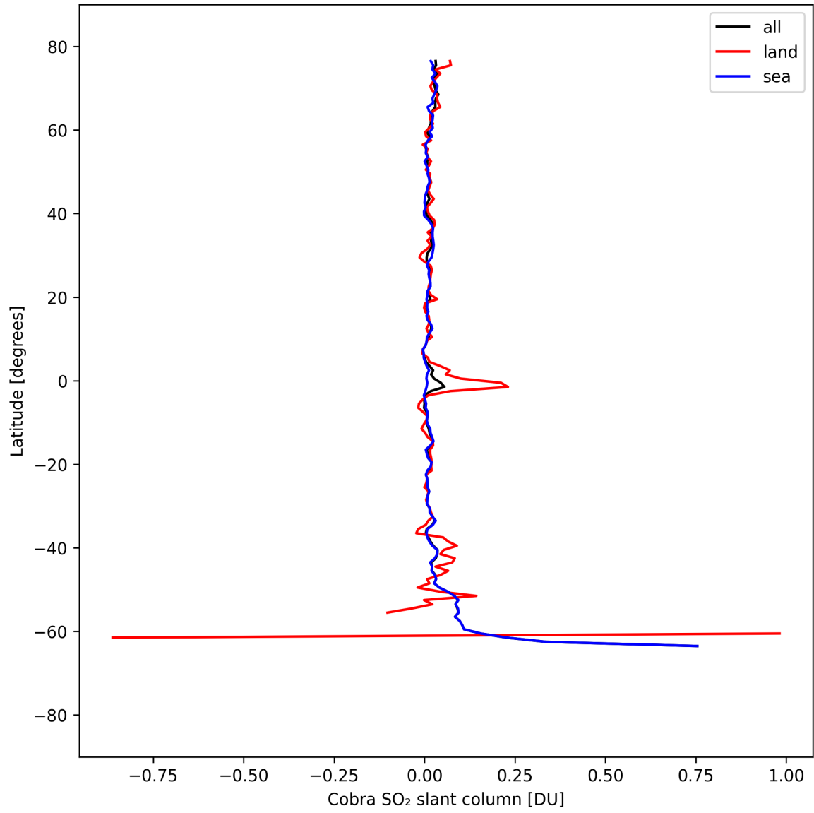
Figure 34: Zonal average of “Cobra SO 2 slant column” for 2025-09-06 to 2025-09-07.
