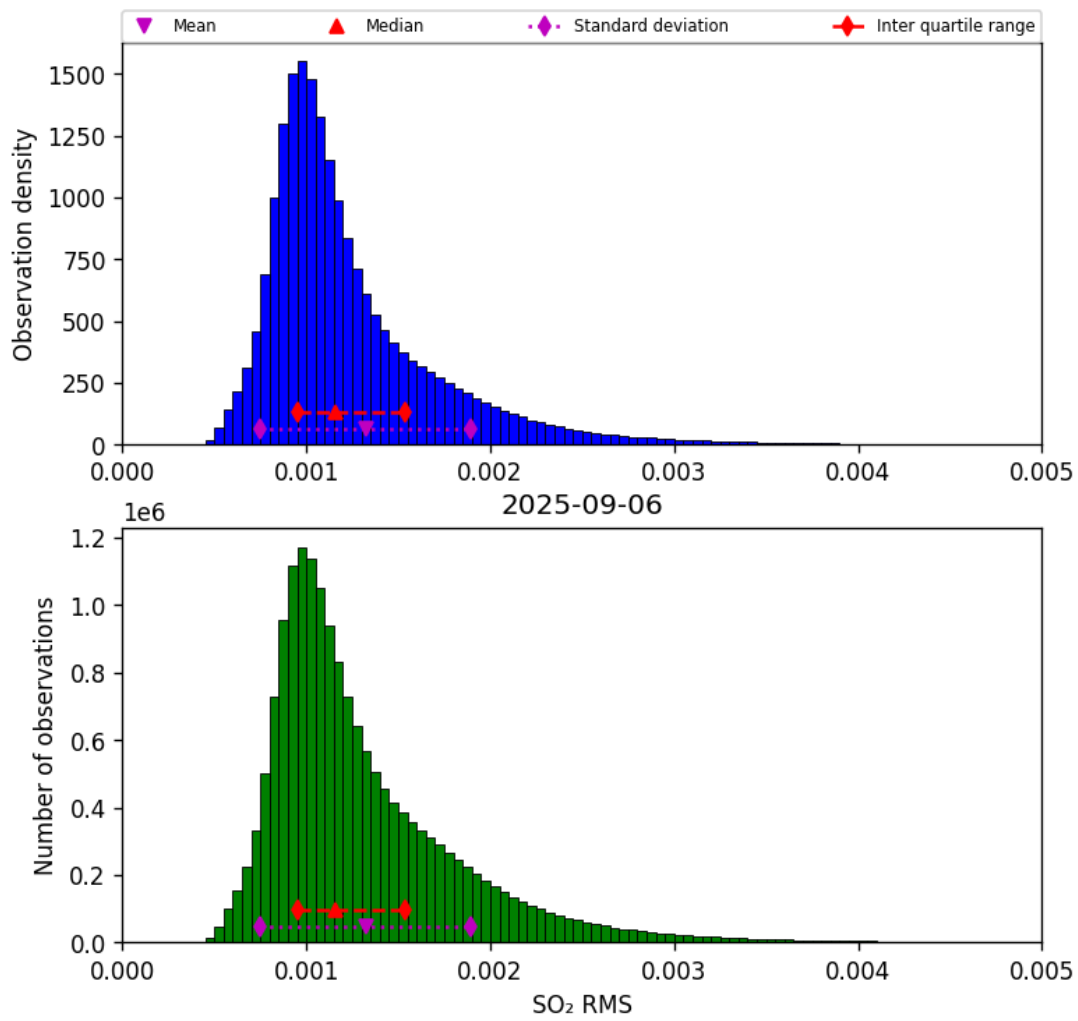
Figure 79: Histogram of "SO 2 RMS" for 2025-09-06 to 2025-09-07
