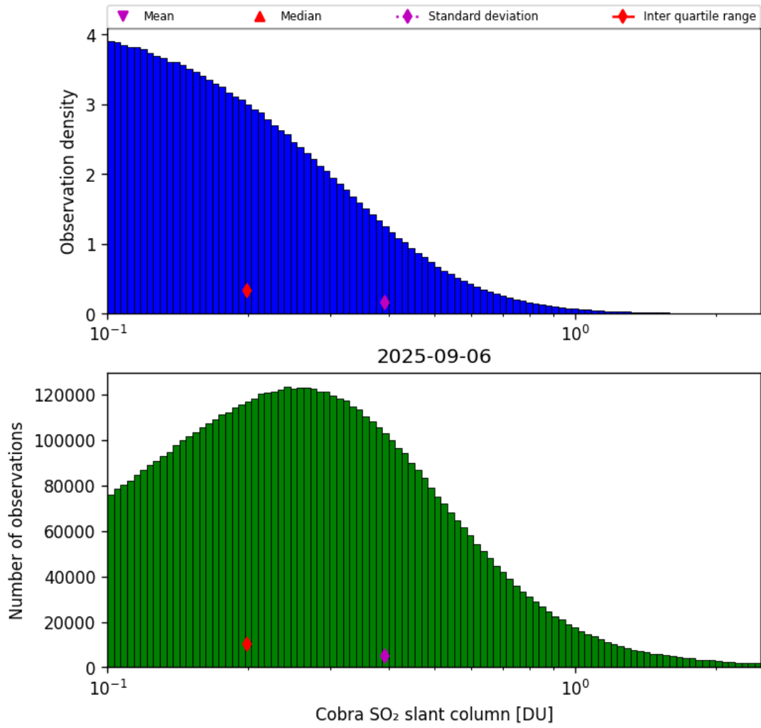
Figure 61: Histogram of “Cobra SO 2 slant column” for 2025-09-06 to 2025-09-07
