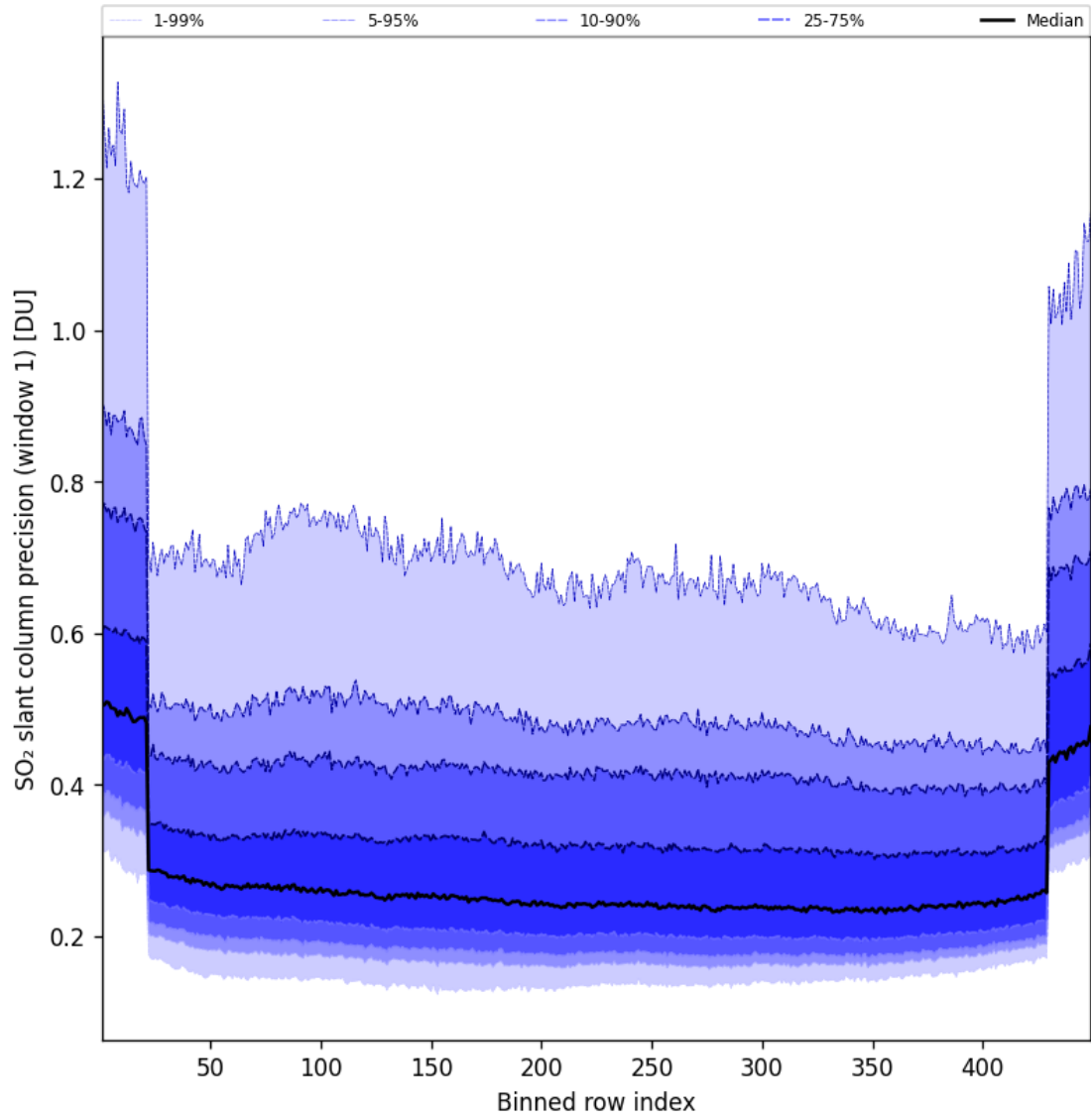
Figure 91: Along track statistics of “SO 2 slant column precision (window 1)” for 2025-09-06 to 2025-09-07
