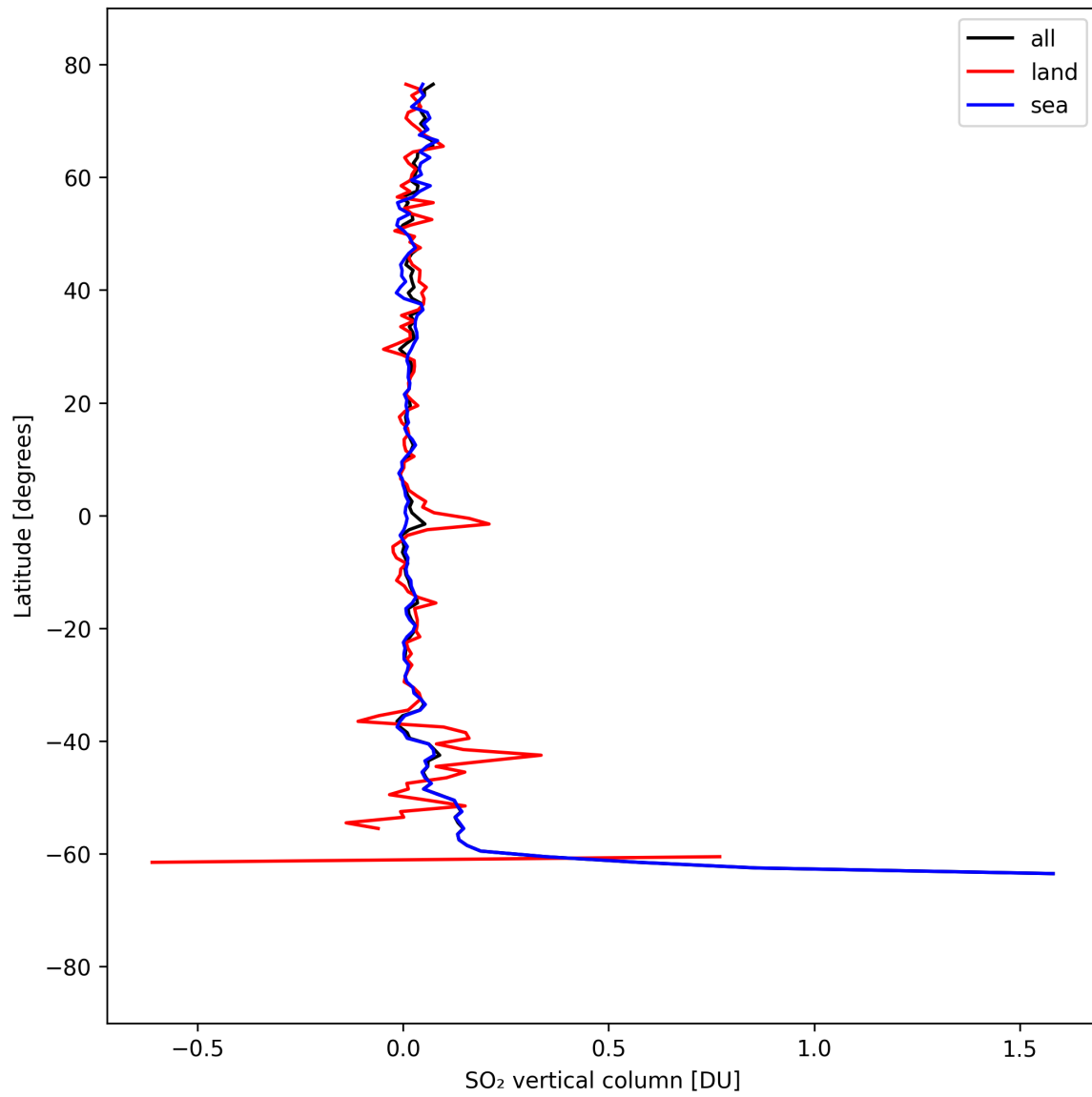
Figure 31: Zonal average of “SO 2 vertical column” for 2025-09-06 to 2025-09-07.
