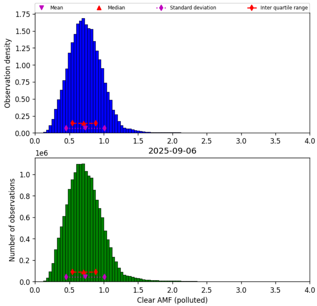
Figure 82: Histogram of “Clear AMF (polluted)” for 2025-09-06 to 2025-09-07
