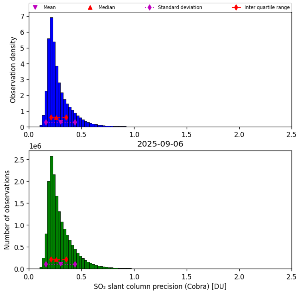
Figure 62: Histogram of “SO 2 slant column precision (Cobra)” for 2025-09-06 to 2025-09-07
