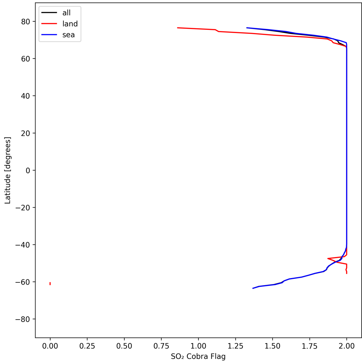
Figure 48: Zonal average of “SO 2 Cobra Flag” for 2025-09-06 to 2025-09-07.
