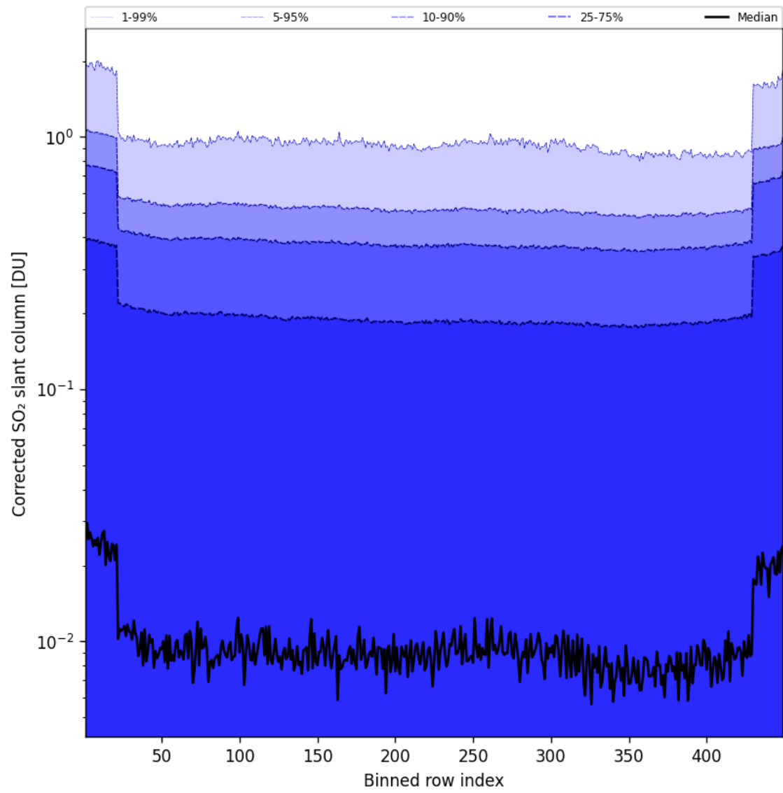
Figure 87: Along track statistics of “Corrected SO 2 slant column” for 2025-09-06 to 2025-09-07
