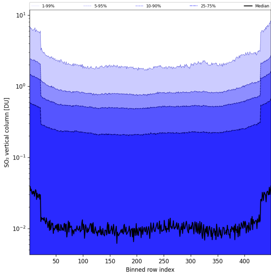
Figure 85: Along track statistics of “SO 2 vertical column” for 2025-09-06 to 2025-09-07
