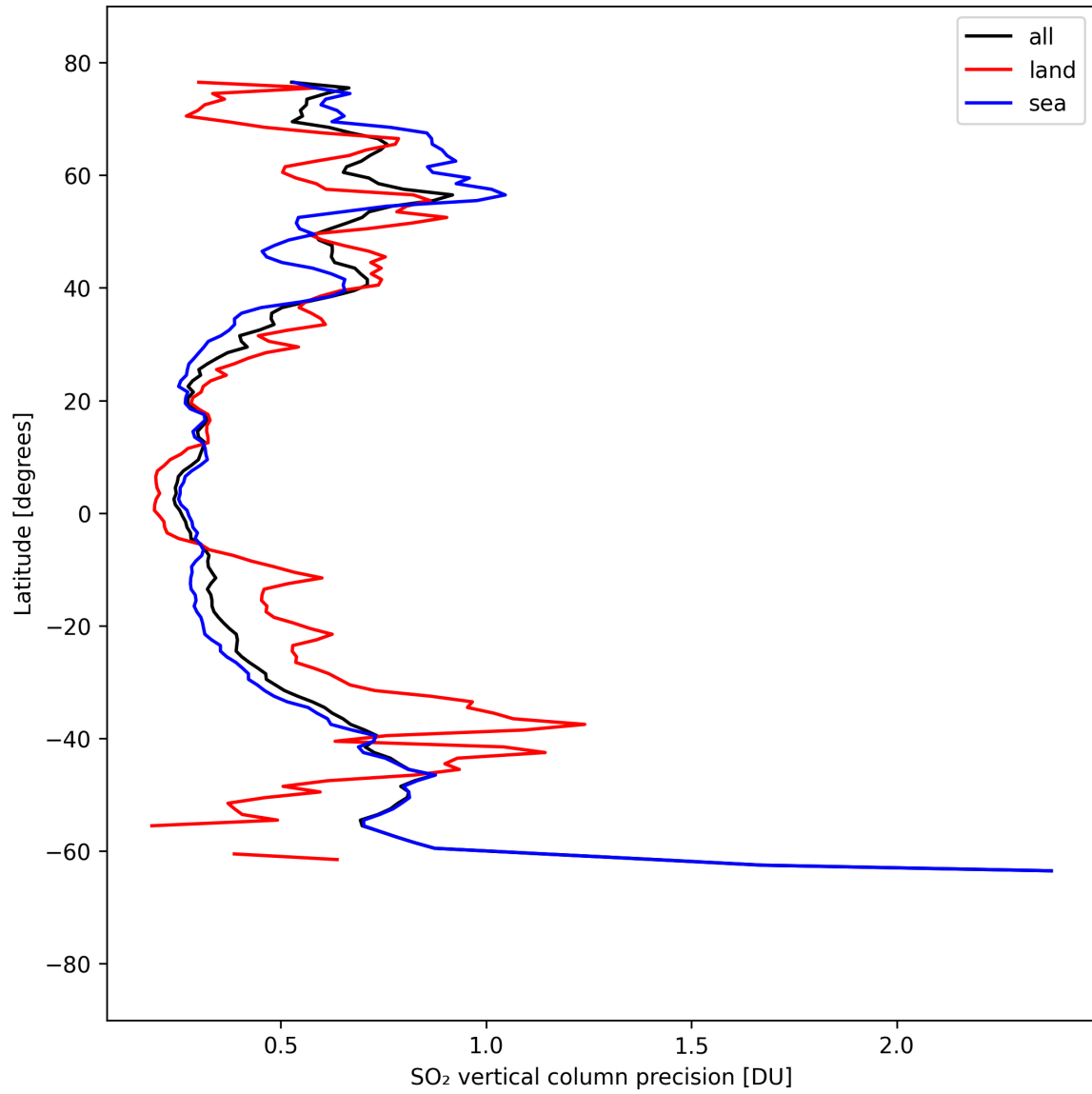
Figure 32: Zonal average of “SO 2 vertical column precision” for 2025-09-06 to 2025-09-07.
