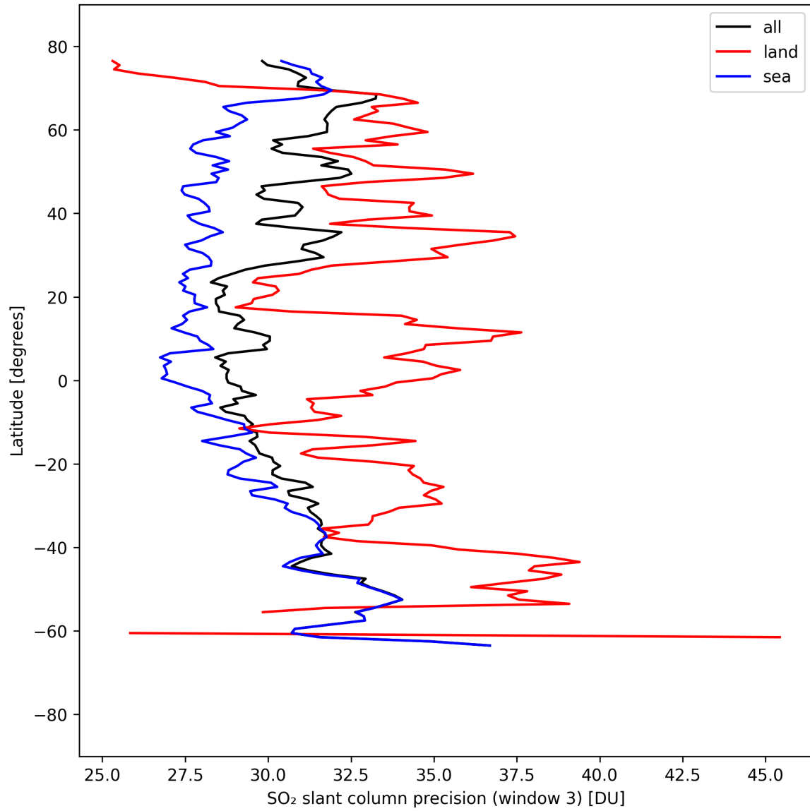
Figure 45: Zonal average of “SO 2 slant column precision (window 3)” for 2025-09-06 to 2025-09-07.
