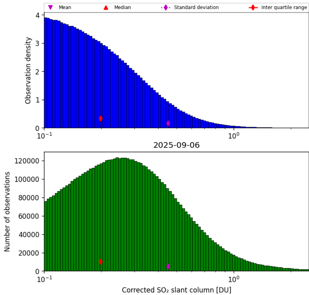
Figure 60: Histogram of “Corrected SO 2 slant column” for 2025-09-06 to 2025-09-07
