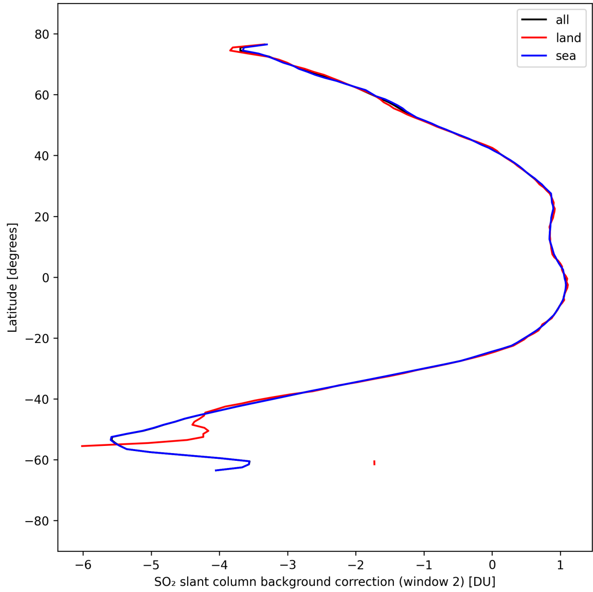
Figure 43: Zonal average of “SO 2 slant column background correction (window 2)” for 2025-09-06 to 2025-09-07.
