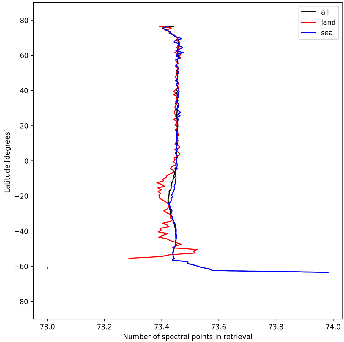
Figure 56: Zonal average of “Number of spectral points in retrieval” for 2025-09-06 to 2025-09-07.
