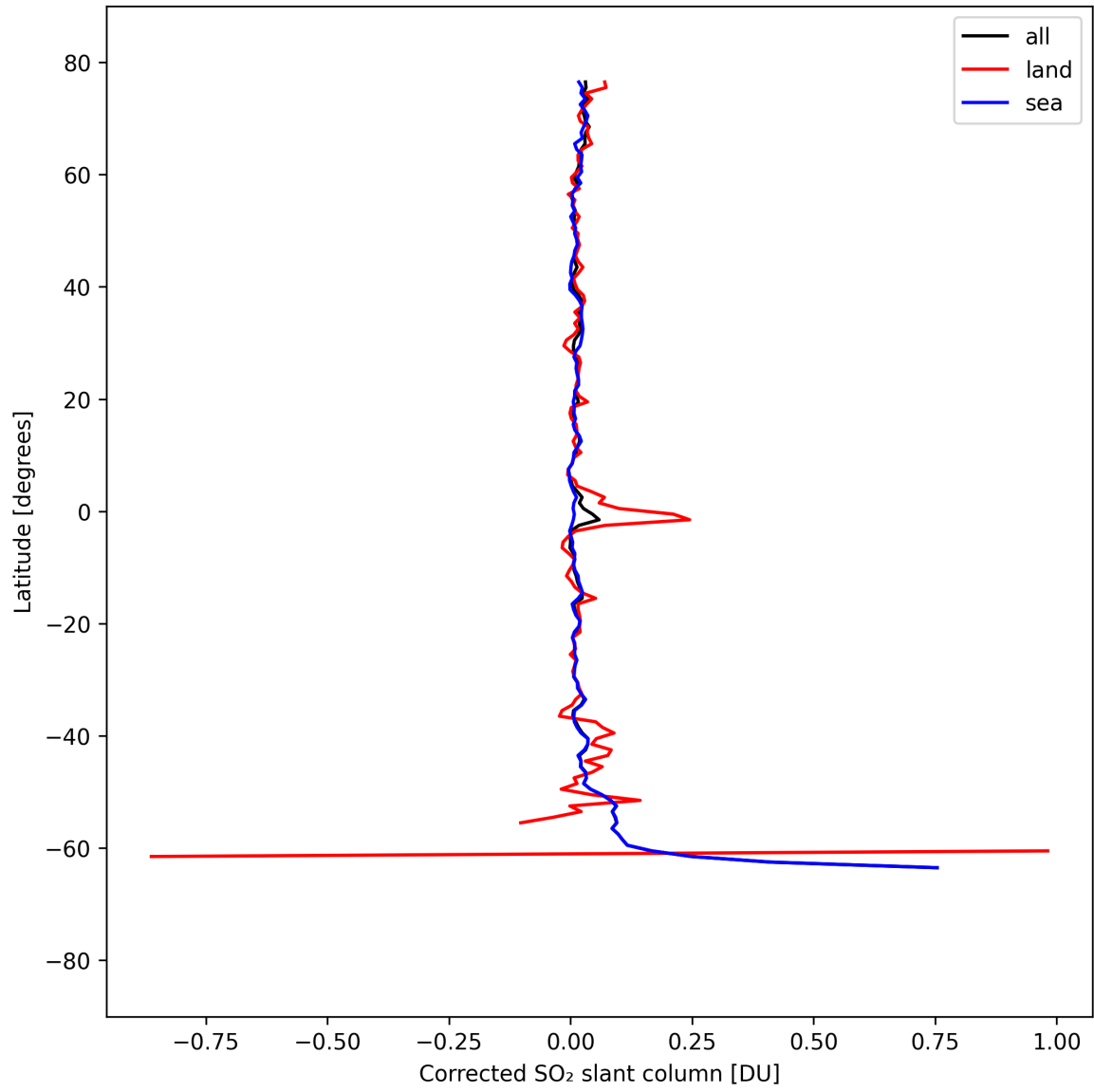
Figure 33: Zonal average of “Corrected SO 2 slant column” for 2025-09-06 to 2025-09-07.
