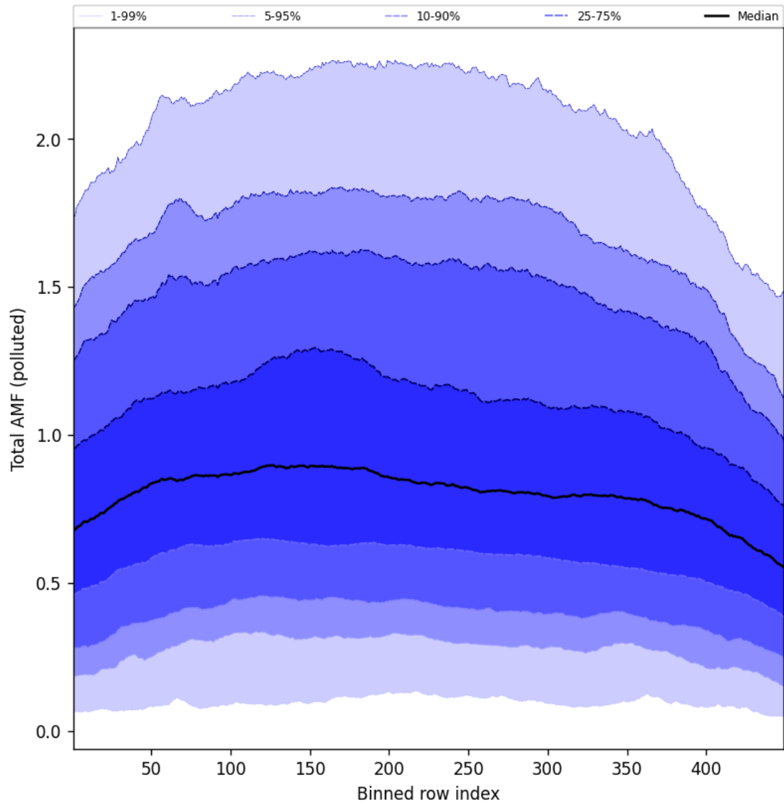
Figure 107: Along track statistics of “Total AMF (polluted)” for 2025-09-06 to 2025-09-07
