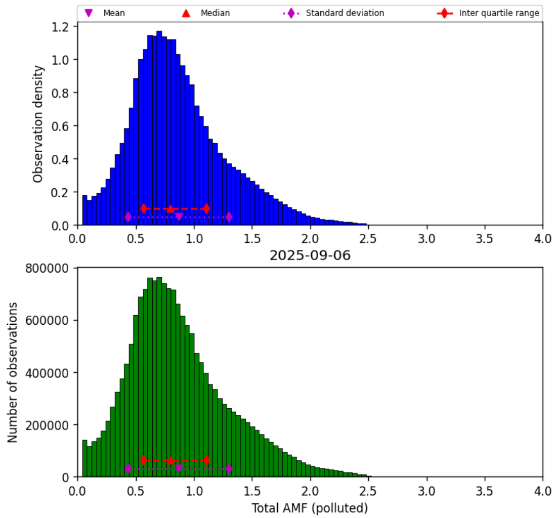
Figure 80: Histogram of “Total AMF (polluted)” for 2025-09-06 to 2025-09-07
