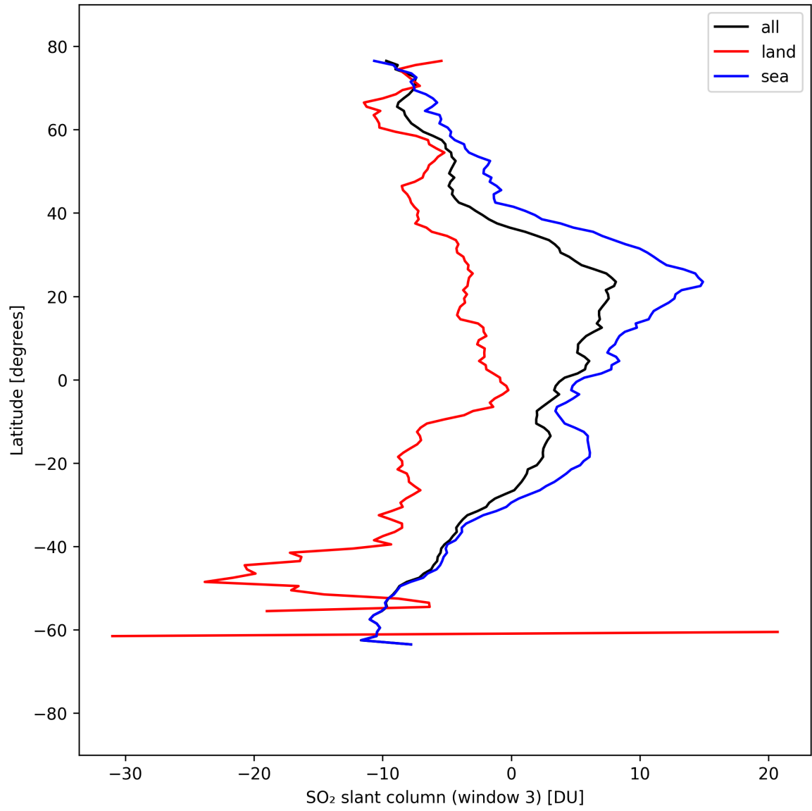
Figure 44: Zonal average of “SO 2 slant column (window 3)” for 2025-09-06 to 2025-09-07.
