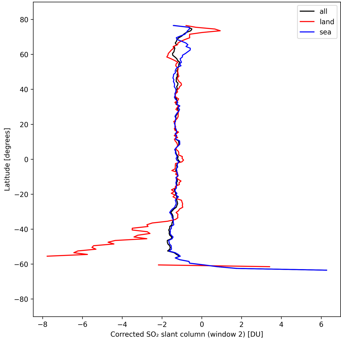
Figure 42: Zonal average of “Corrected SO 2 slant column (window 2)” for 2025-09-06 to 2025-09-07.
