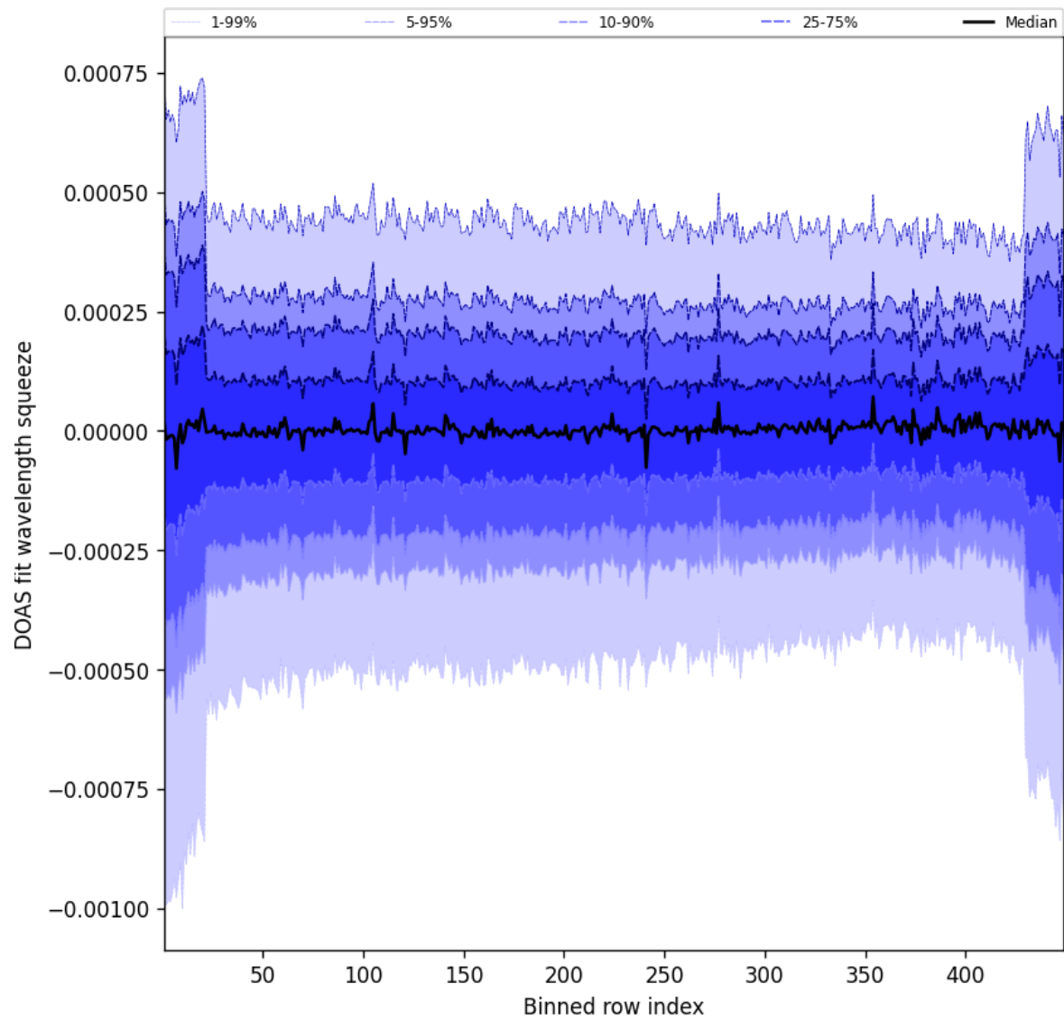
Figure 105: Along track statistics of “DOAS fit wavelength squeeze” for 2025-09-06 to 2025-09-07
