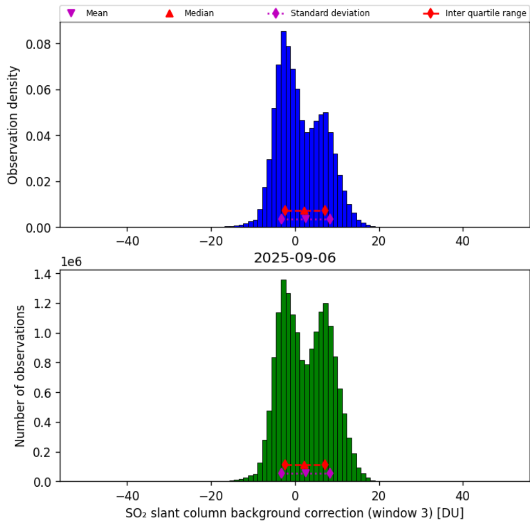
Figure 74: Histogram of “SO 2 slant column background correction (window 3)” for 2025-09-06 to 2025-09-07
