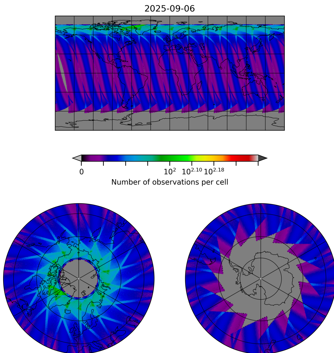
Figure 29: Map of the number of observations for 2025-09-06 to 2025-09-07
