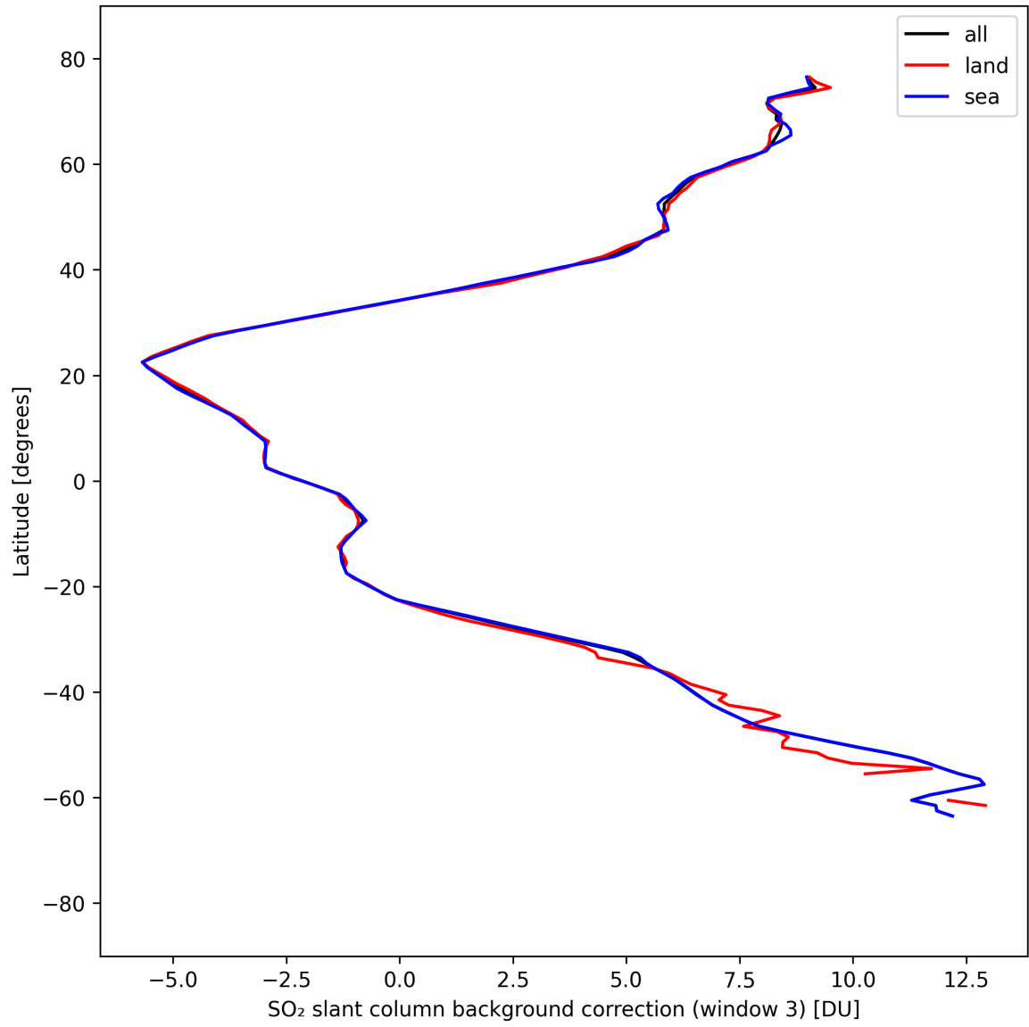
Figure 47: Zonal average of “SO 2 slant column background correction (window 3)” for 2025-09-06 to 2025-09-07.
