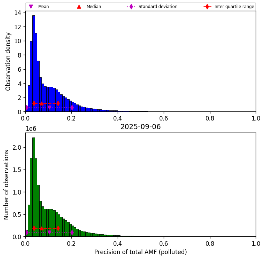
Figure 81: Histogram of “Precision of total AMF (polluted)” for 2025-09-06 to 2025-09-07
