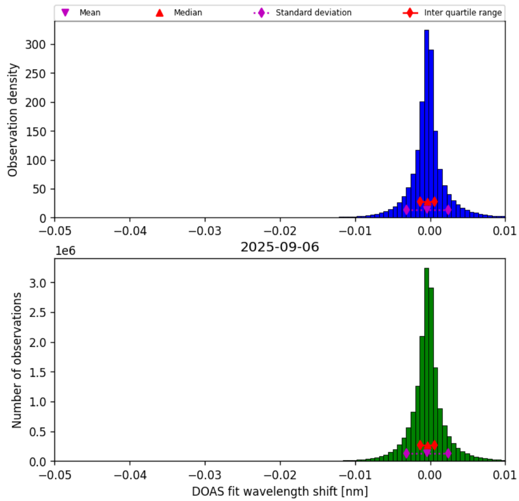
Figure 77: Histogram of “DOAS fit wavelength shift” for 2025-09-06 to 2025-09-07
