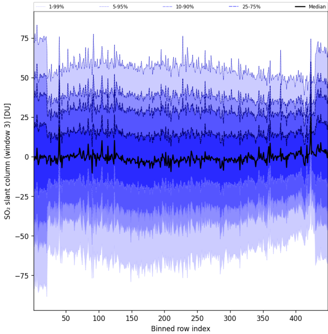
Figure 98: Along track statistics of “SO 2 slant column (window 3)” for 2025-09-06 to 2025-09-07
