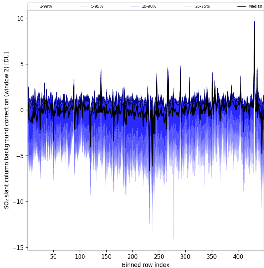
Figure 97: Along track statistics of “SO 2 slant column background correction (window 2)” for 2025-09-06 to 2025-09-07
