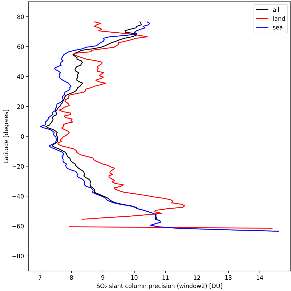
Figure 41: Zonal average of “SO 2 slant column precision (window2)” for 2025-09-06 to 2025-09-07.
