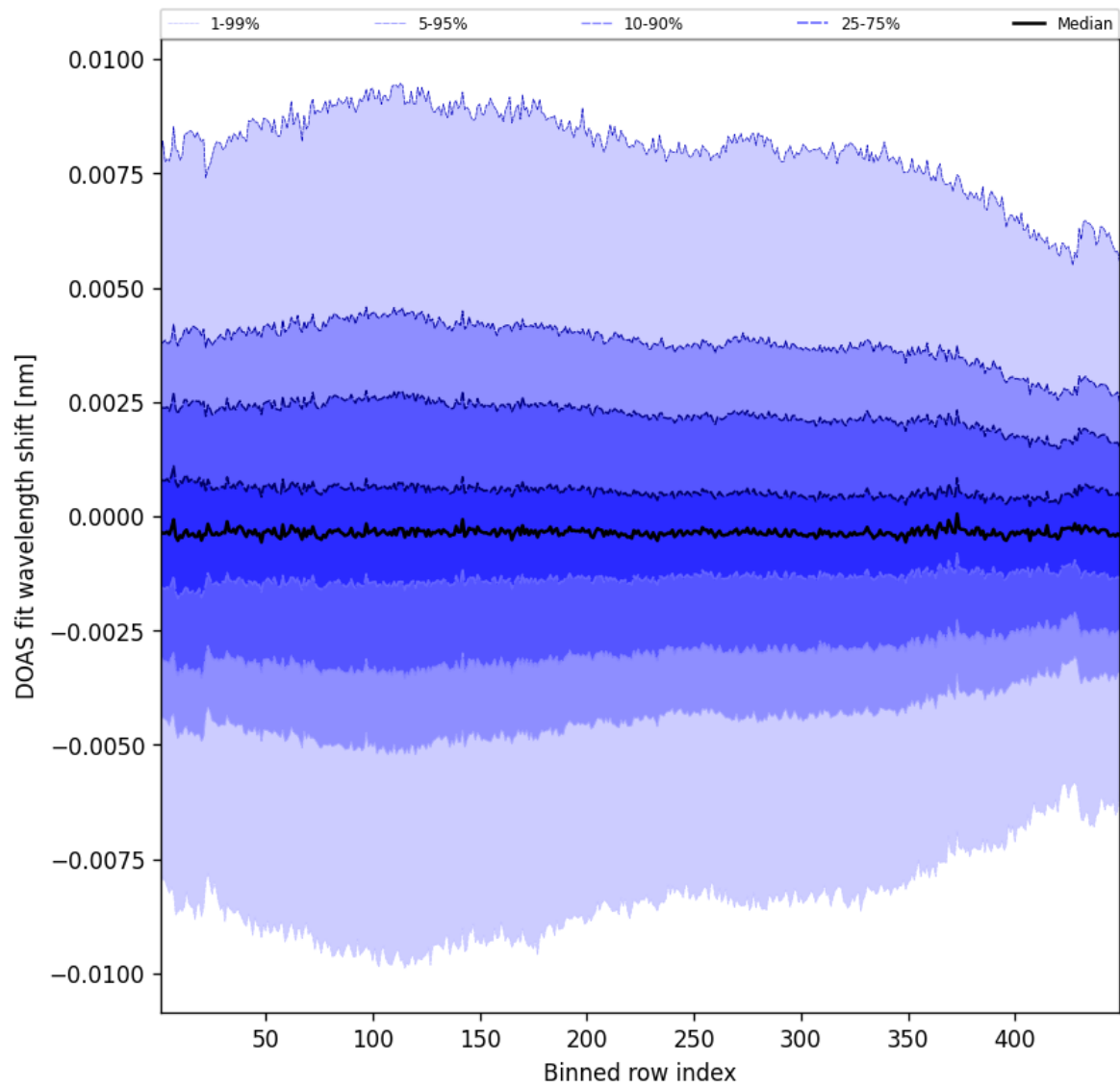
Figure 104: Along track statistics of “DOAS fit wavelength shift” for 2025-09-06 to 2025-09-07
