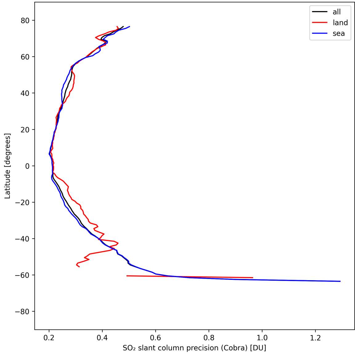
Figure 35: Zonal average of “SO 2 slant column precision (Cobra)” for 2025-09-06 to 2025-09-07.
