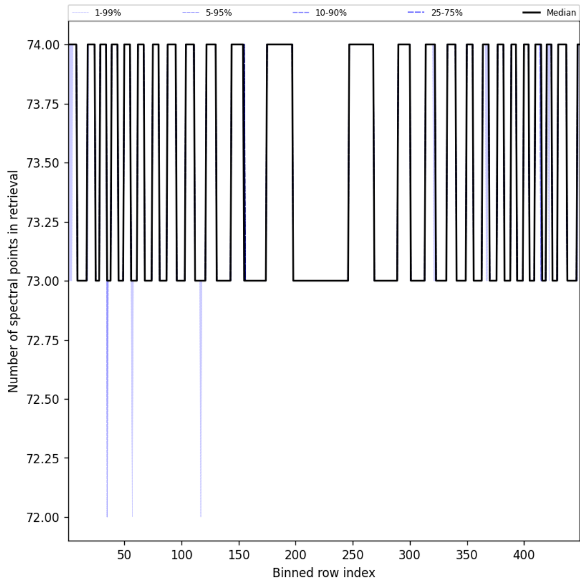
Figure 110: Along track statistics of “Number of spectral points in retrieval” for 2025-09-06 to 2025-09-07
