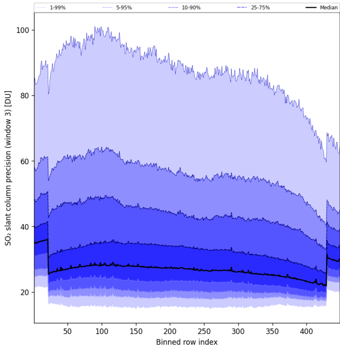
Figure 99: Along track statistics of “SO 2 slant column precision (window 3)” for 2025-09-06 to 2025-09-07
