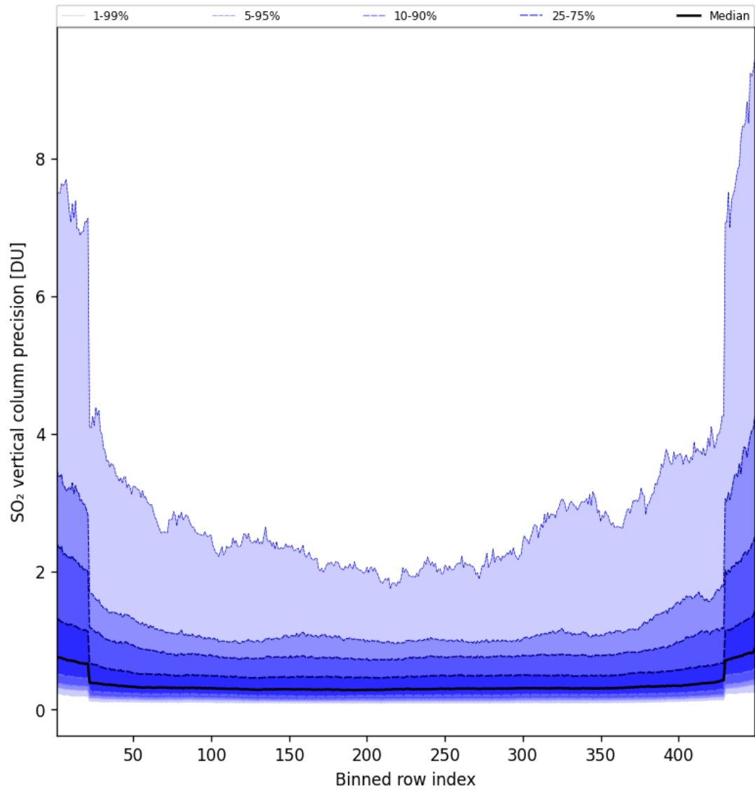
Figure 86: Along track statistics of “SO 2 vertical column precision” for 2025-09-06 to 2025-09-07
