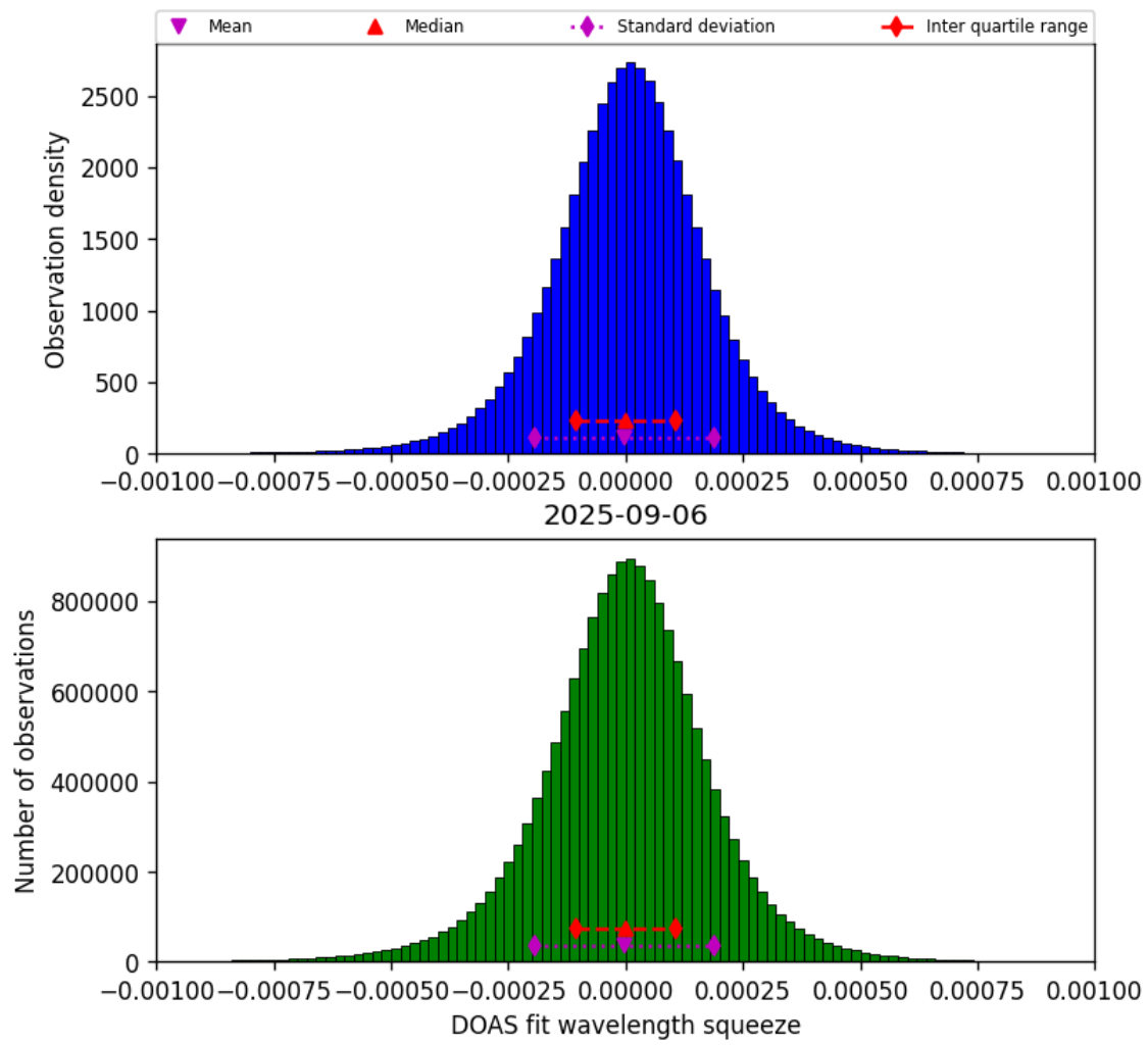
Figure 78: Histogram of “DOAS fit wavelength squeeze” for 2025-09-06 to 2025-09-07
