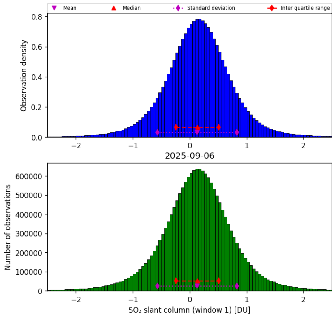
Figure 63: Histogram of “SO 2 slant column (window 1)” for 2025-09-06 to 2025-09-07
