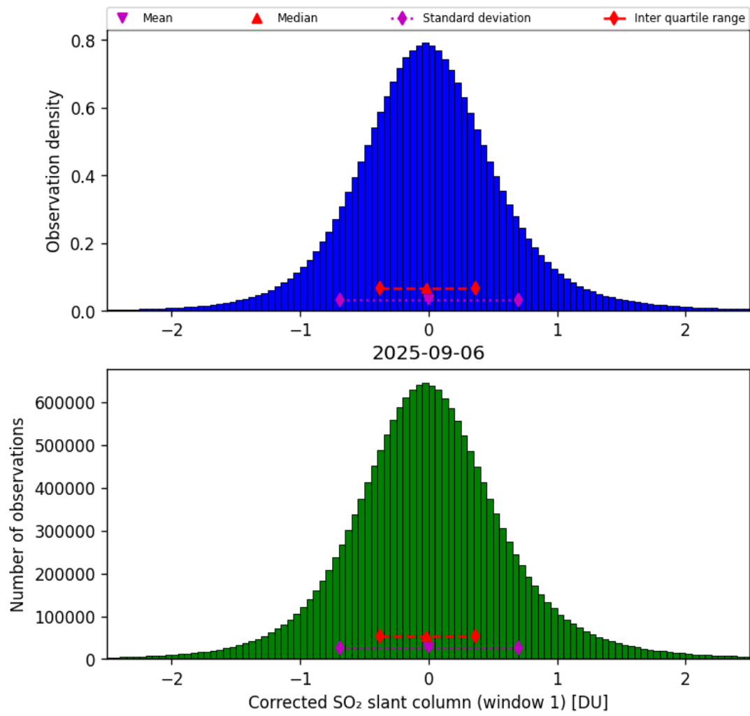
Figure 65: Histogram of “Corrected SO 2 slant column (window 1)” for 2025-09-06 to 2025-09-07
