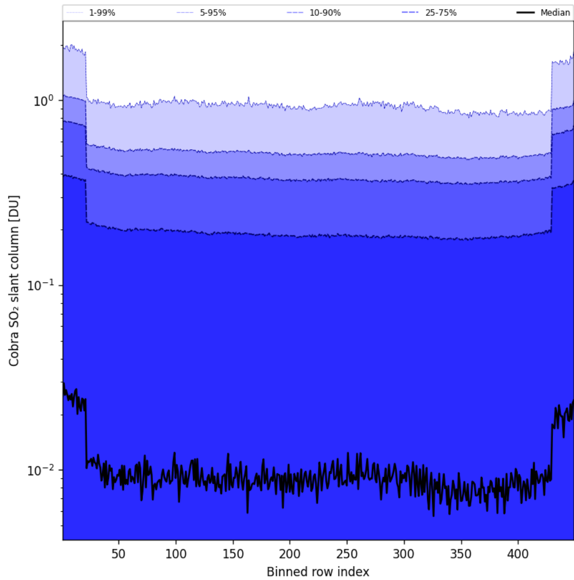
Figure 88: Along track statistics of “Cobra SO 2 slant column” for 2025-09-06 to 2025-09-07
