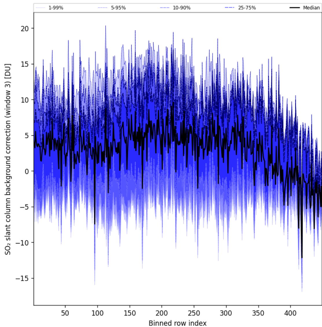
Figure 101: Along track statistics of “SO 2 slant column background correction (window 3)” for 2025-09-06 to 2025-09-07
