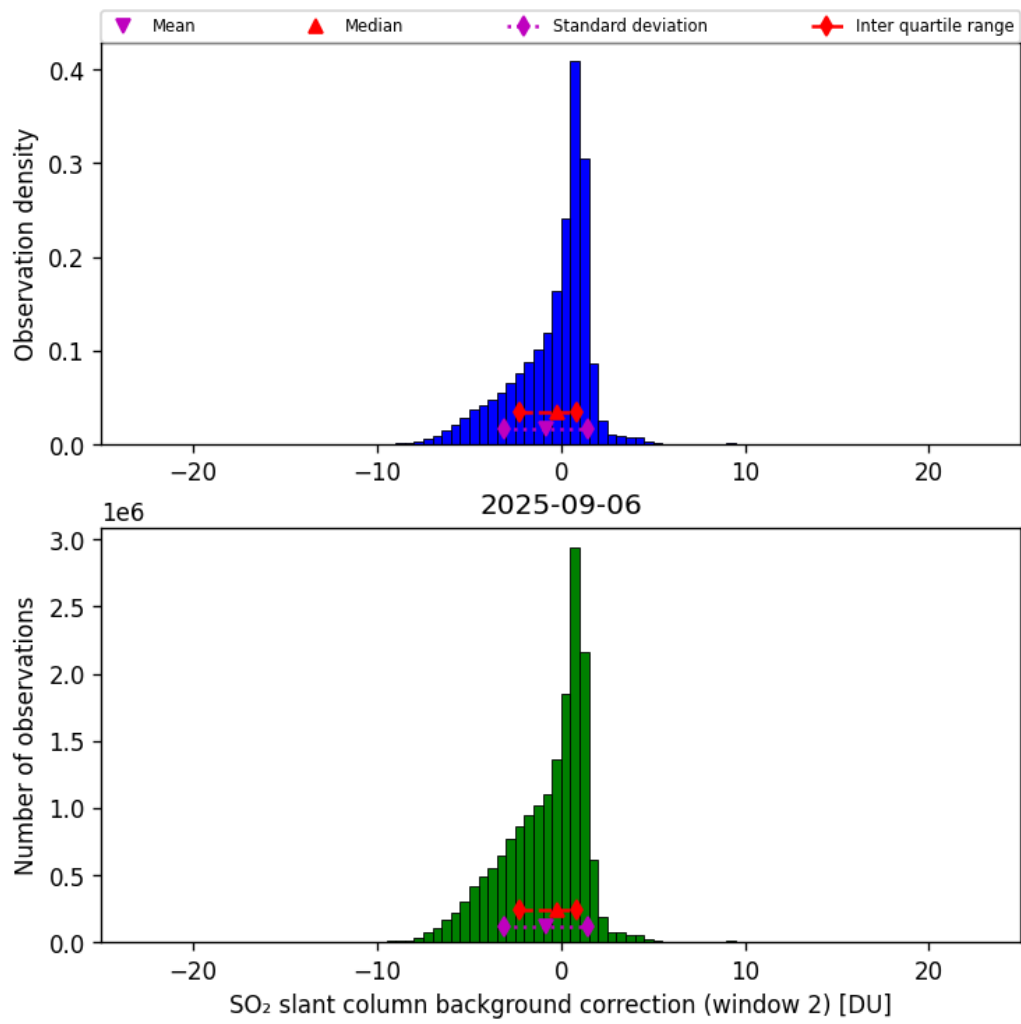
Figure 70: Histogram of “SO 2 slant column background correction (window 2)” for 2025-09-06 to 2025-09-07
