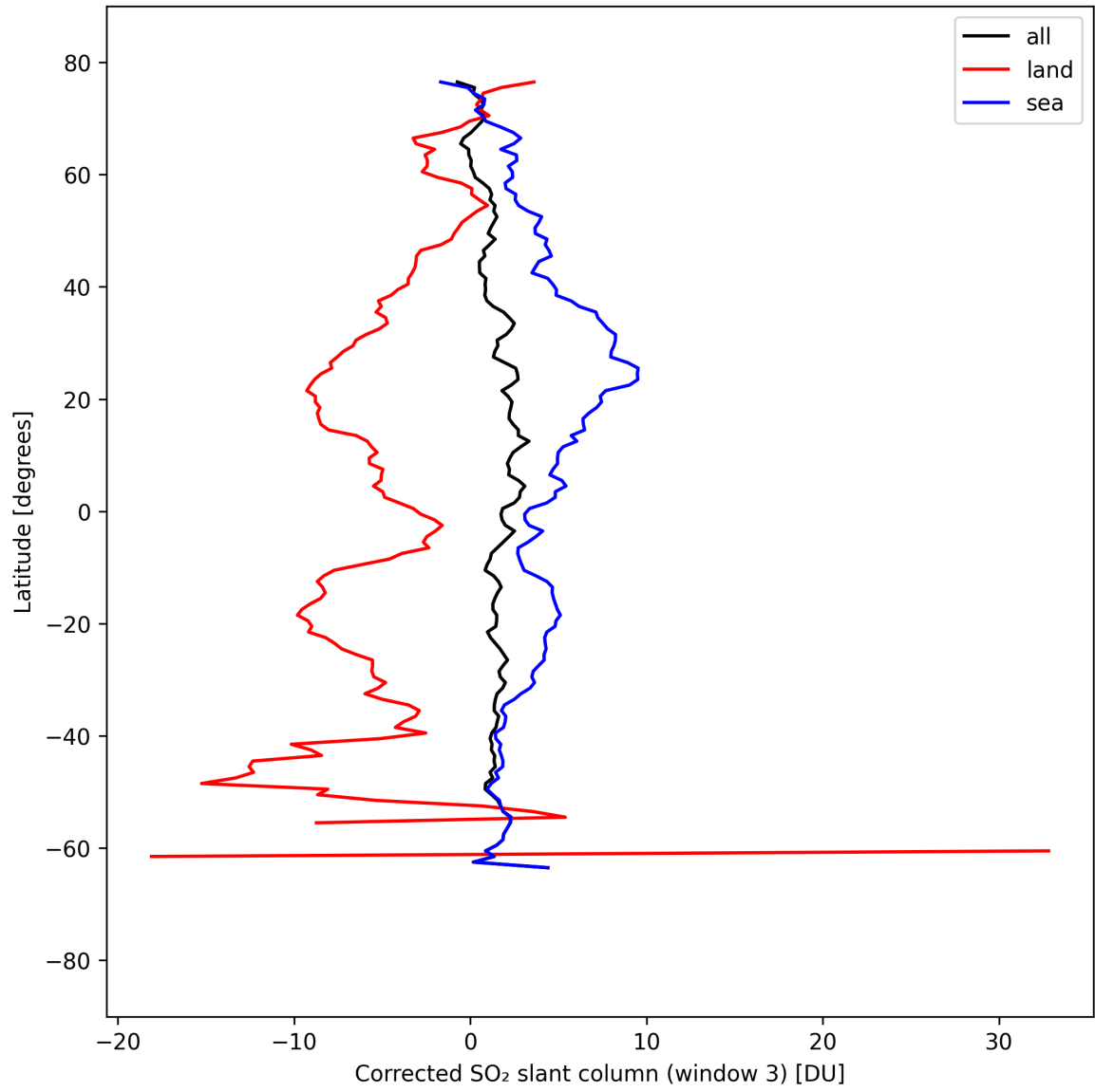
Figure 46: Zonal average of “Corrected SO 2 slant column (window 3)” for 2025-09-06 to 2025-09-07.
