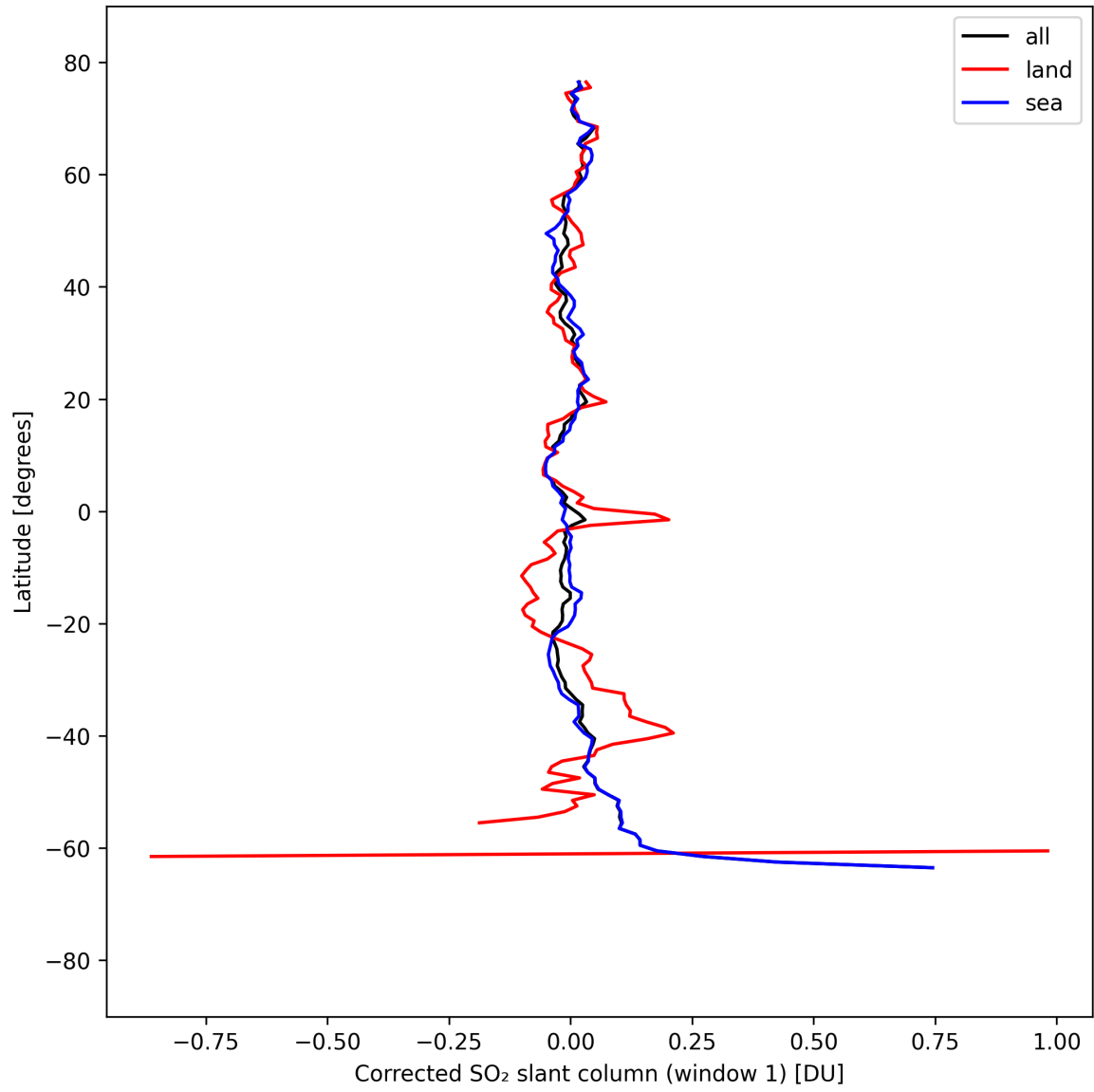
Figure 38: Zonal average of “Corrected SO 2 slant column (window 1)” for 2025-09-06 to 2025-09-07.
