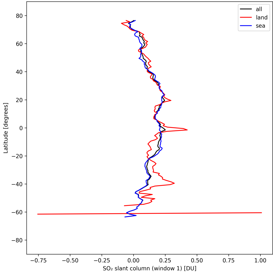
Figure 36: Zonal average of “SO 2 slant column (window 1)” for 2025-09-06 to 2025-09-07.
