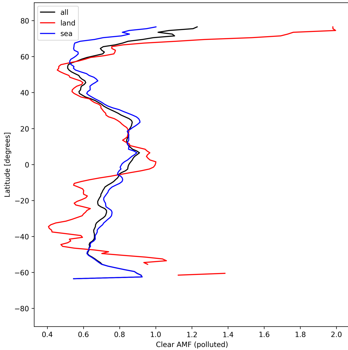
Figure 55: Zonal average of “Clear AMF (polluted)” for 2025-09-06 to 2025-09-07.
