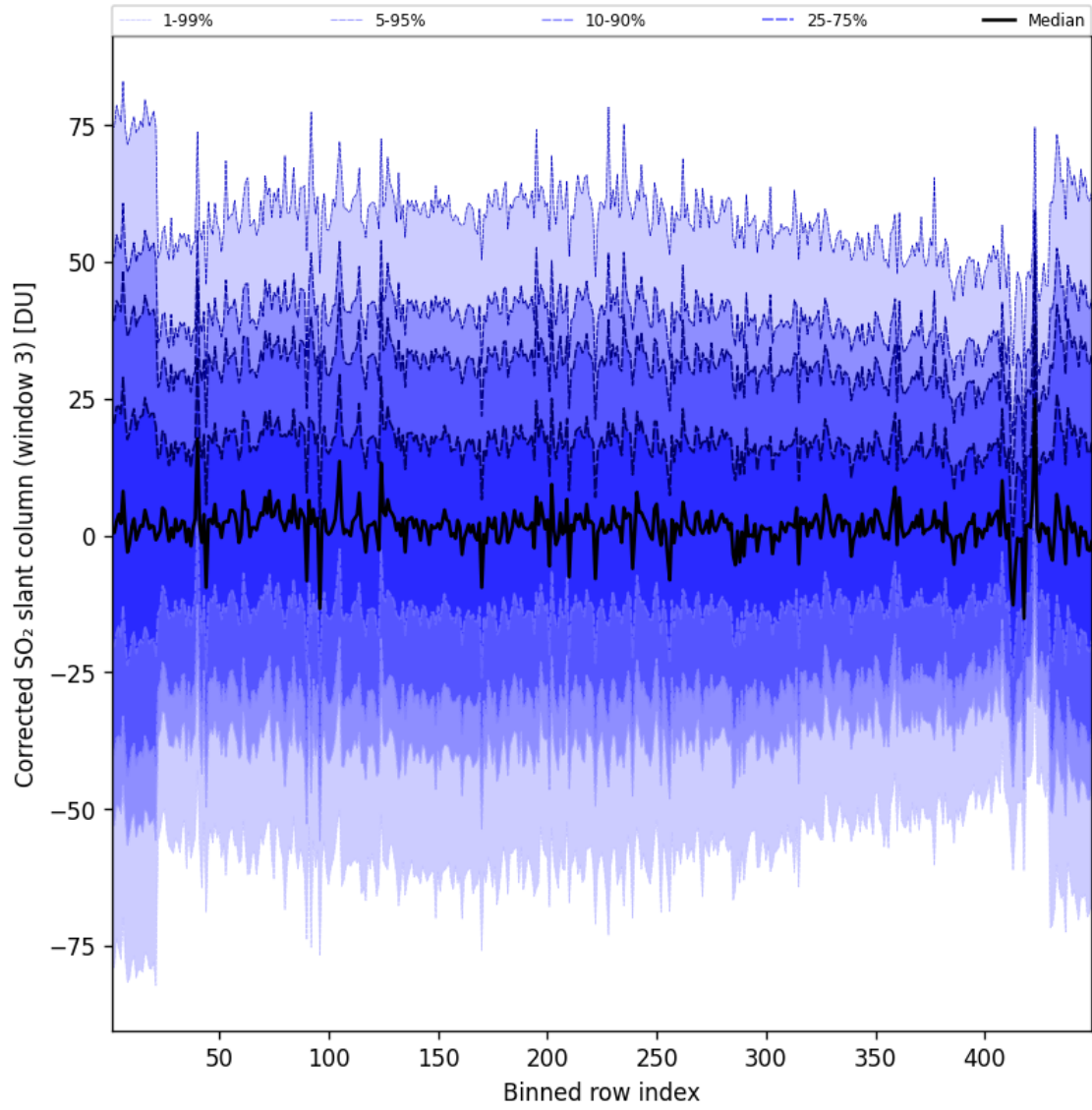
Figure 100: Along track statistics of “Corrected SO 2 slant column (window 3)” for 2025-09-06 to 2025-09-07
