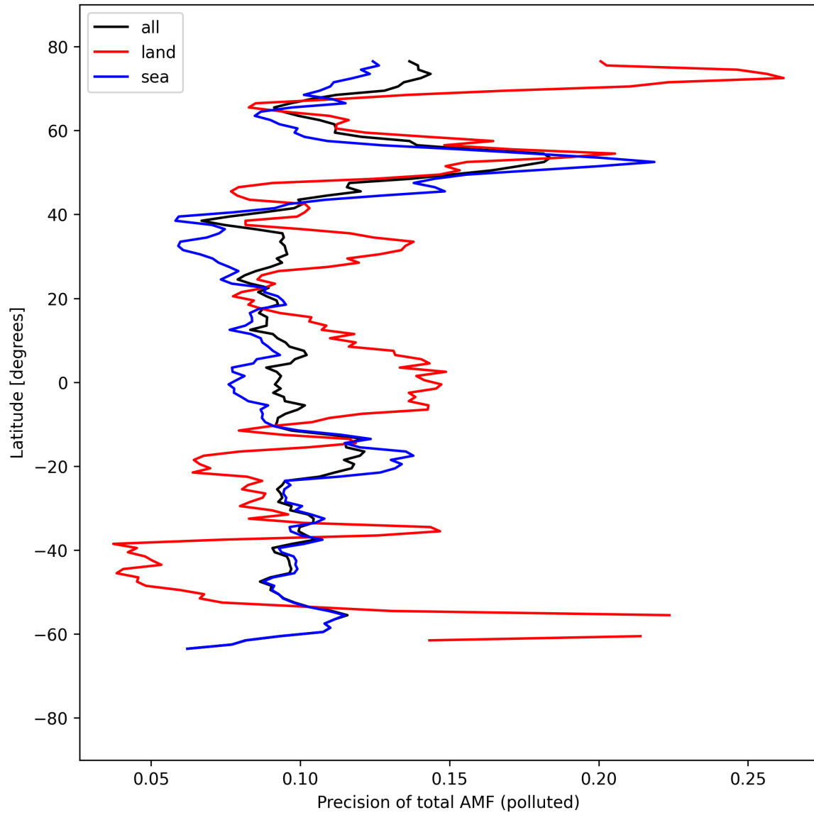
Figure 54: Zonal average of “Precision of total AMF (polluted)” for 2025-09-06 to 2025-09-07.
