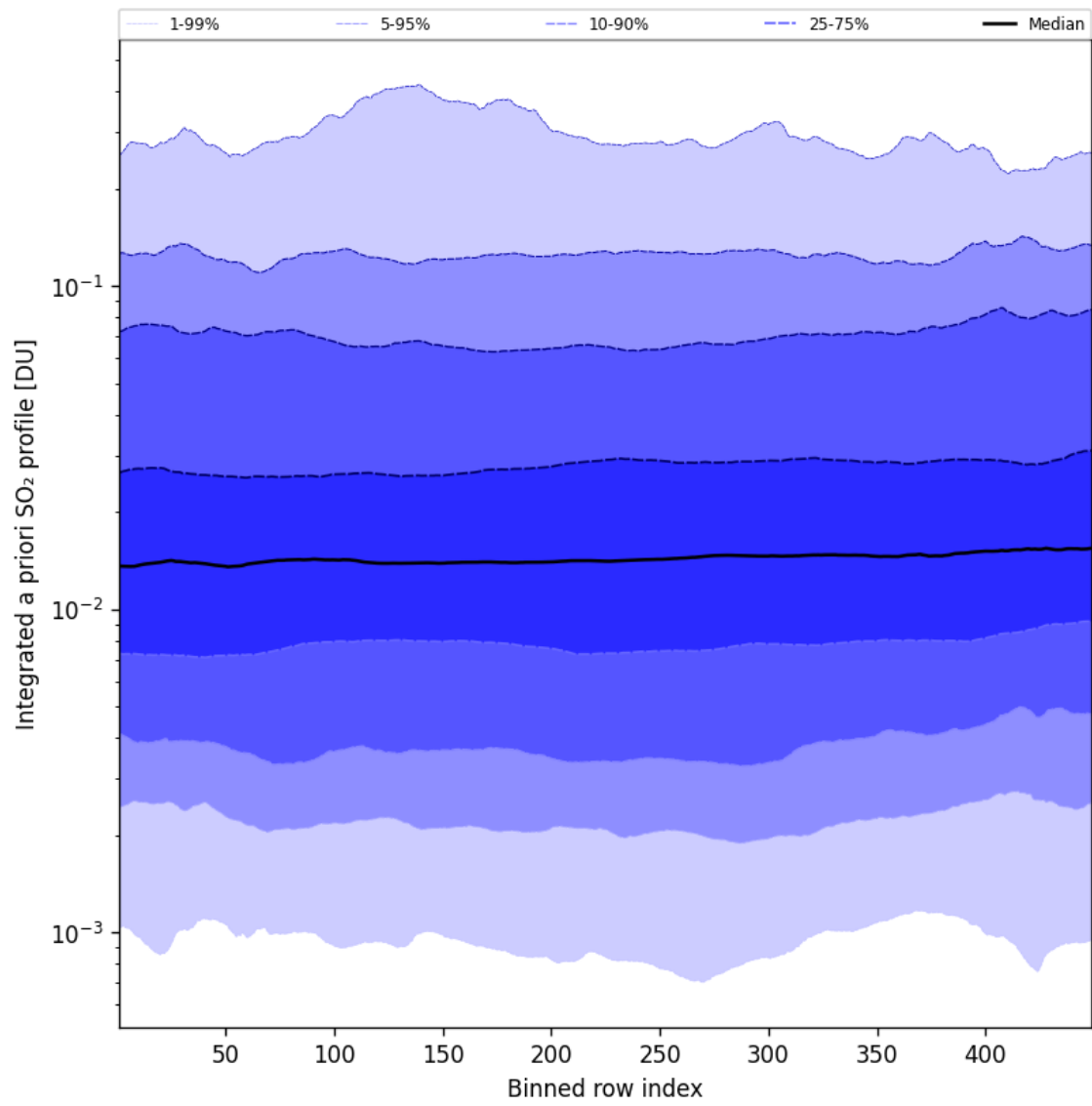
Figure 103: Along track statistics of “Integrated a priori SO 2 profile” for 2025-09-06 to 2025-09-07
