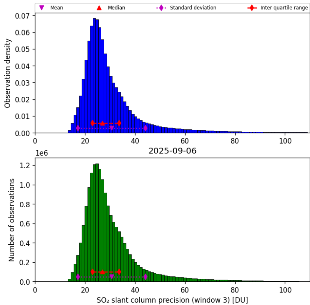
Figure 72: Histogram of “SO 2 slant column precision (window 3)” for 2025-09-06 to 2025-09-07
