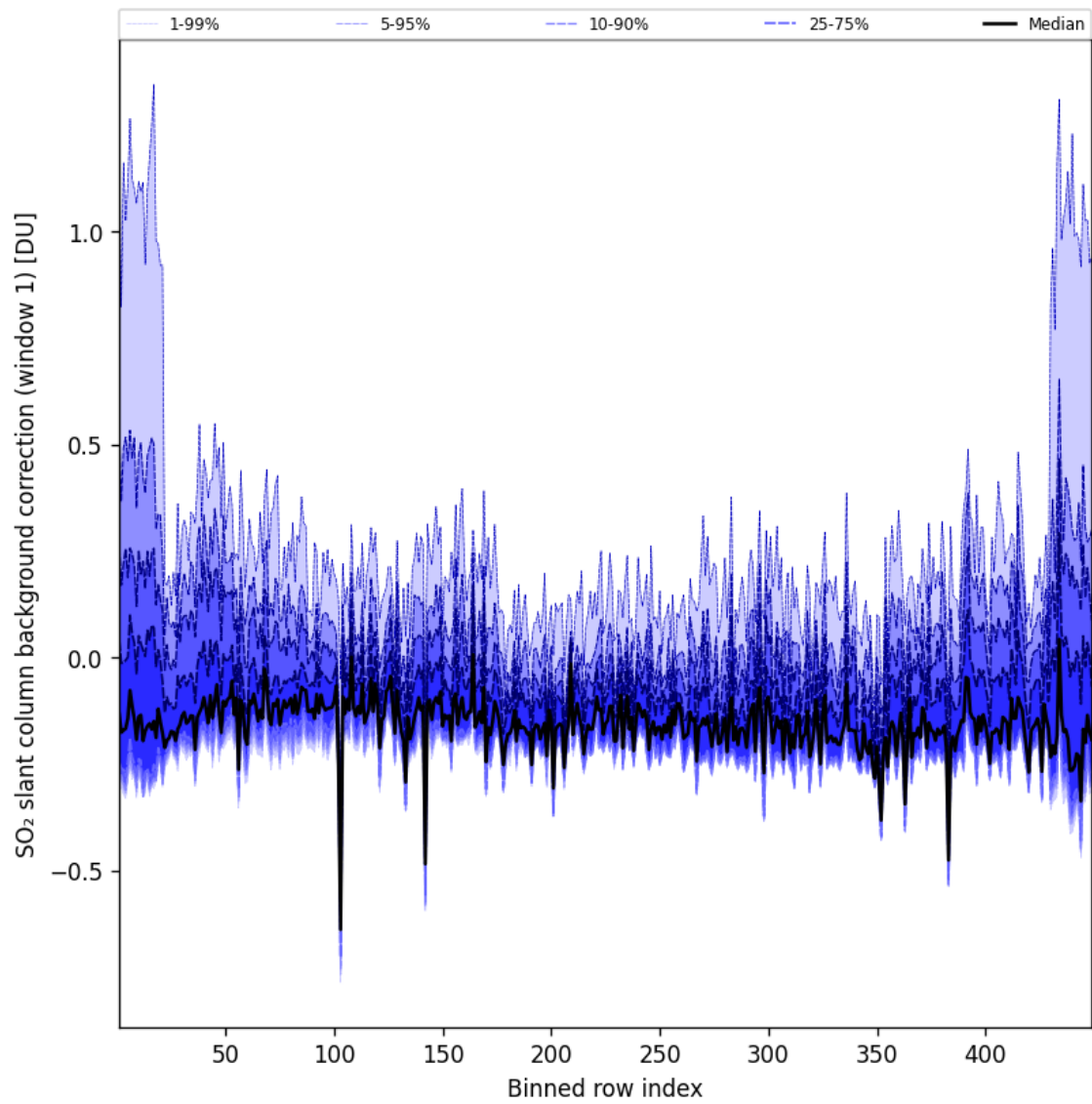
Figure 93: Along track statistics of “SO 2 slant column background correction (window 1)” for 2025-09-06 to 2025-09-07
