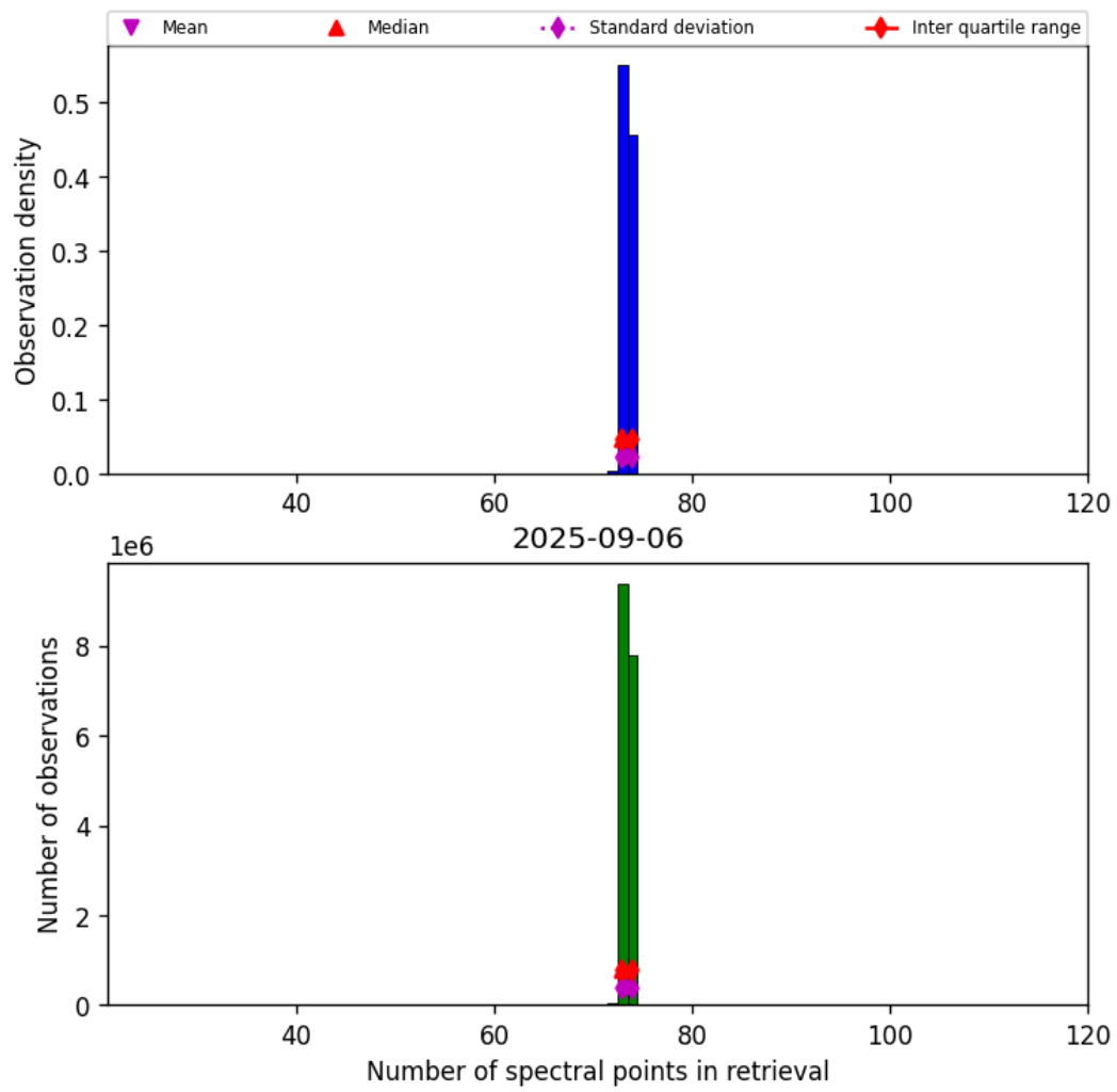
Figure 83: Histogram of “Number of spectral points in retrieval” for 2025-09-06 to 2025-09-07
