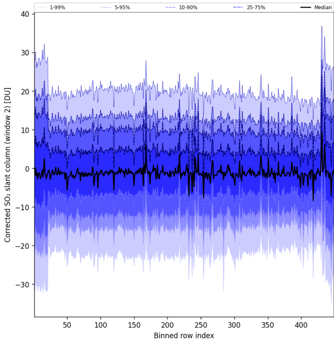
Figure 96: Along track statistics of “Corrected SO 2 slant column (window 2)” for 2025-09-06 to 2025-09-07
