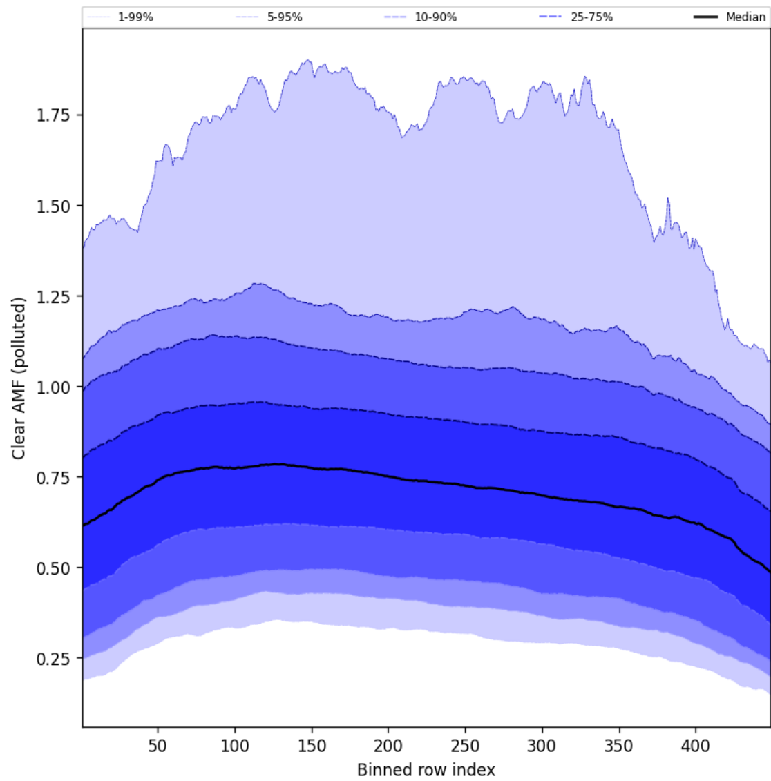
Figure 109: Along track statistics of “Clear AMF (polluted)” for 2025-09-06 to 2025-09-07
