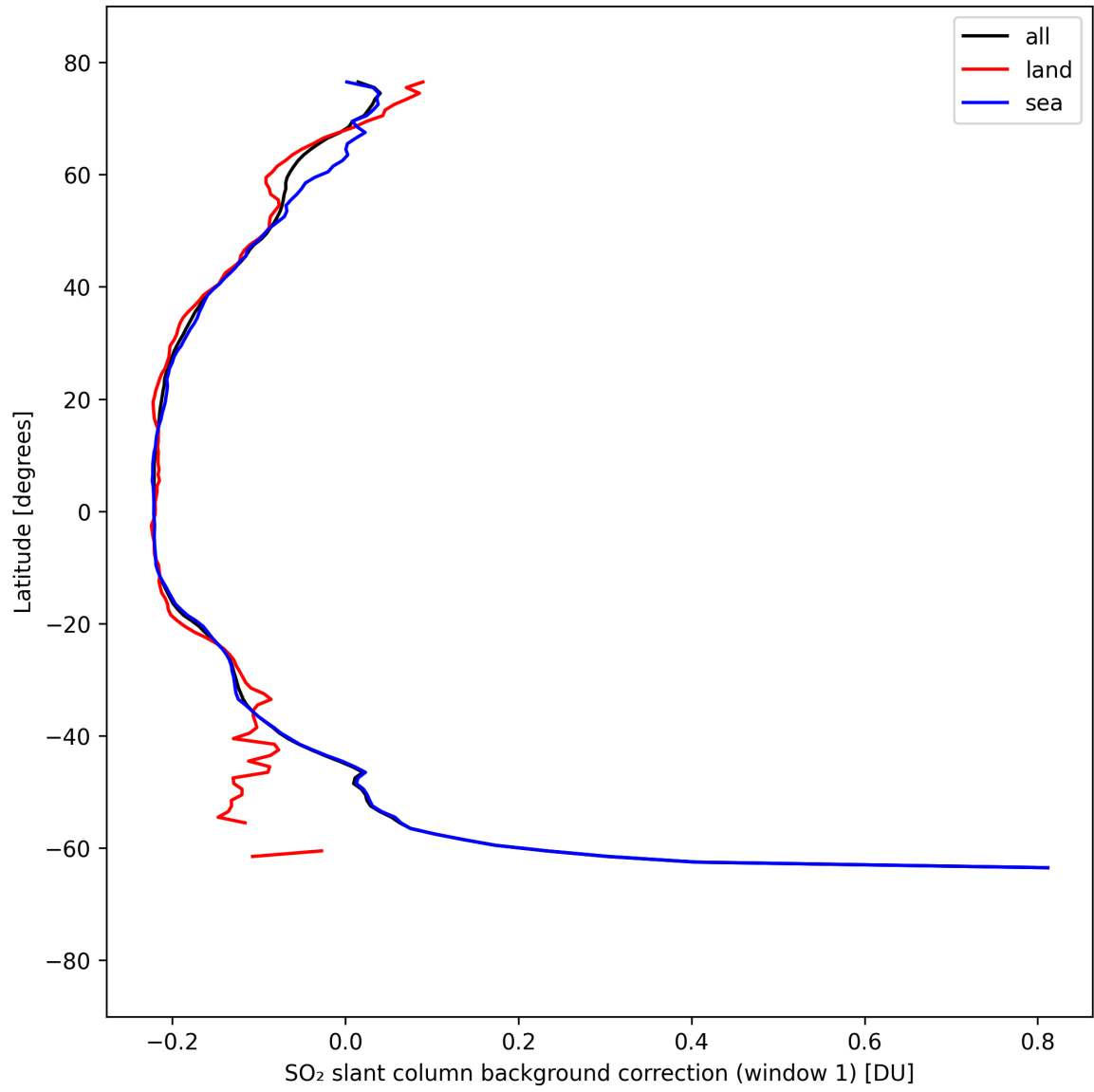
Figure 39: Zonal average of "SO 2 slant column background correction (window 1)" for 2025-09-06 to 2025-09-07.
