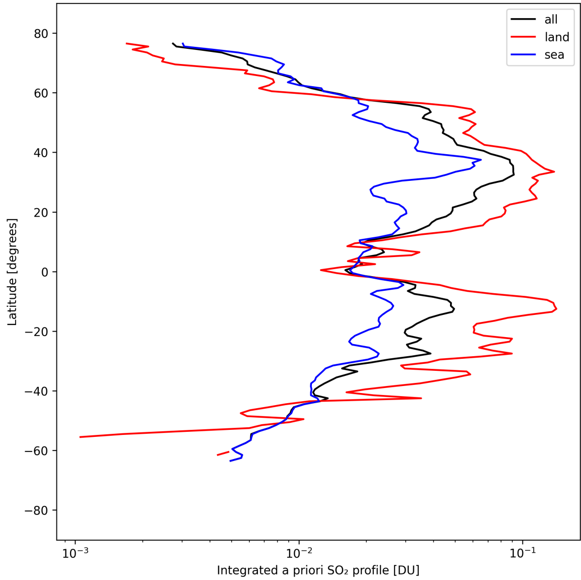
Figure 49: Zonal average of “Integrated a priori SO 2 profile” for 2025-09-06 to 2025-09-07.
