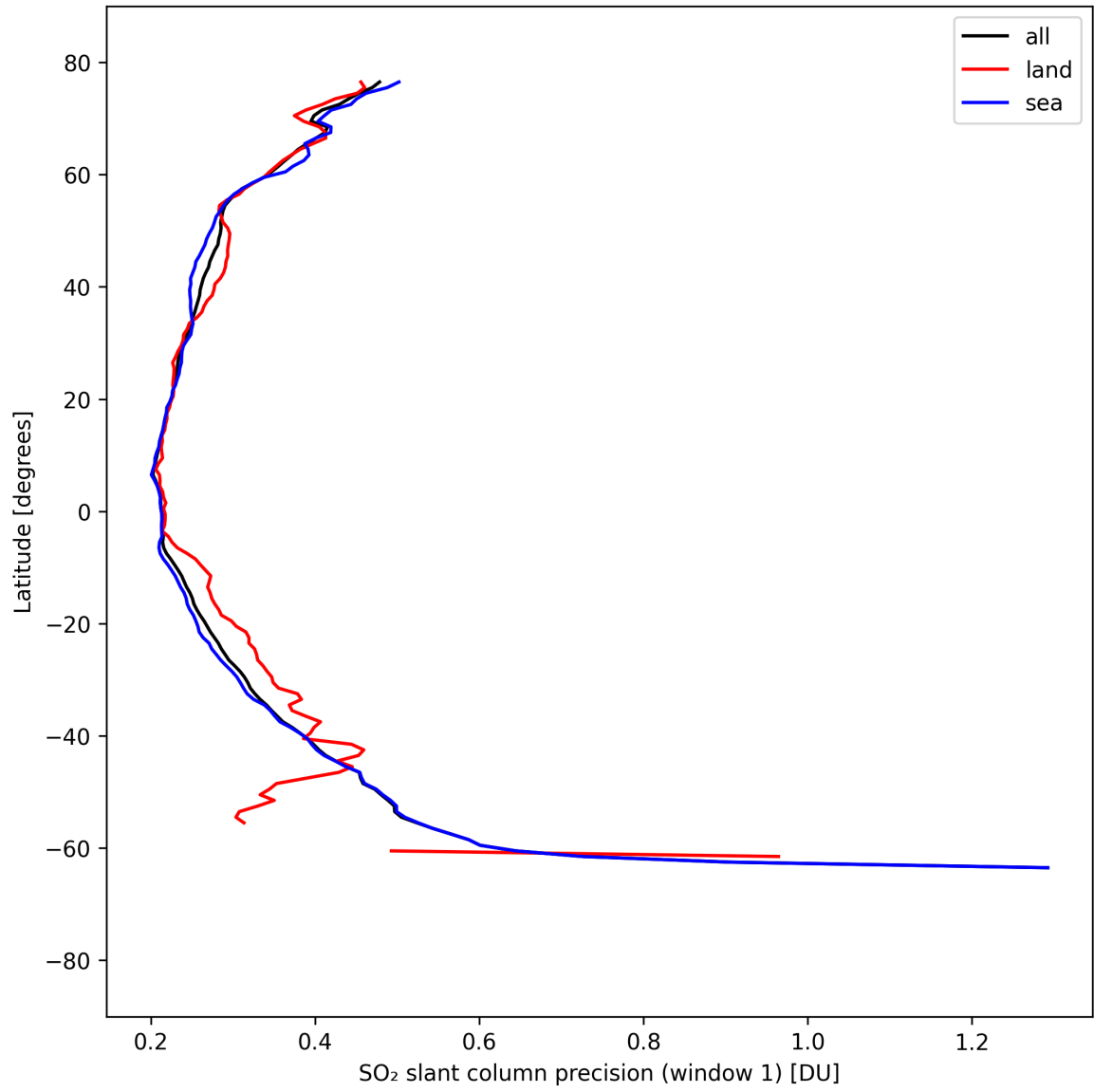
Figure 37: Zonal average of “SO 2 slant column precision (window 1)” for 2025-09-06 to 2025-09-07.
