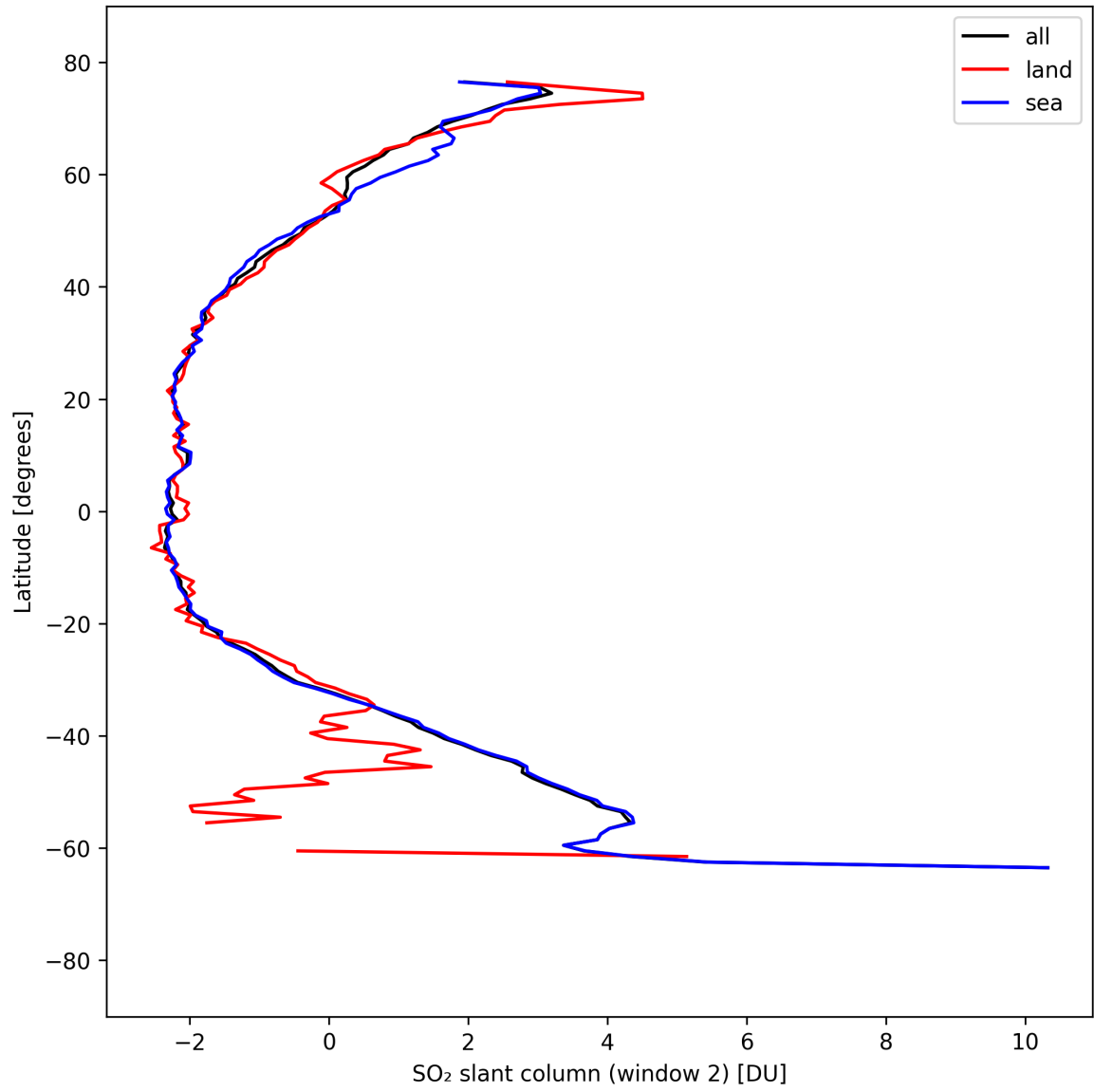
Figure 40: Zonal average of “SO 2 slant column (window 2)” for 2025-09-06 to 2025-09-07.
