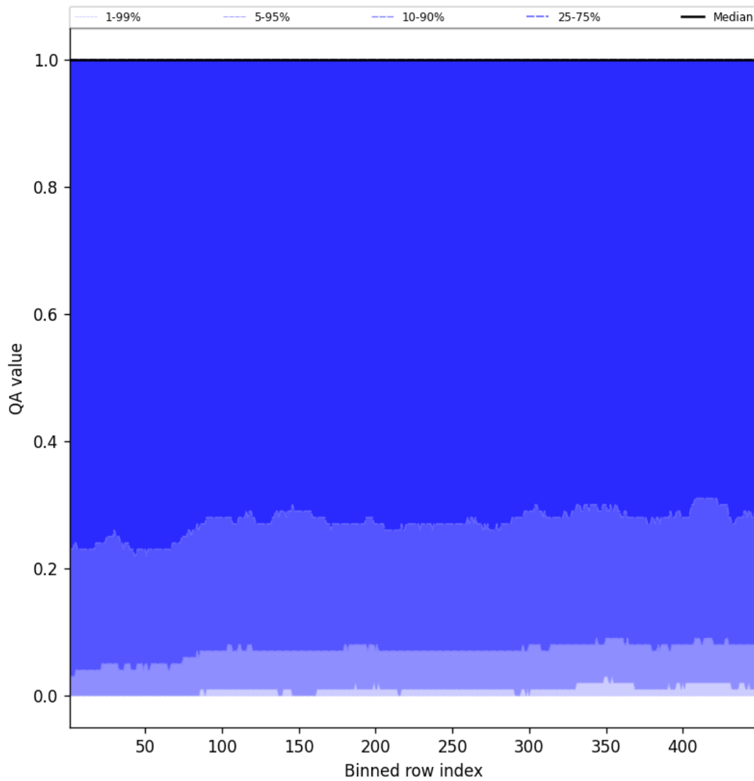
Figure 84: Along track statistics of “QA value” for 2025-09-06 to 2025-09-07
