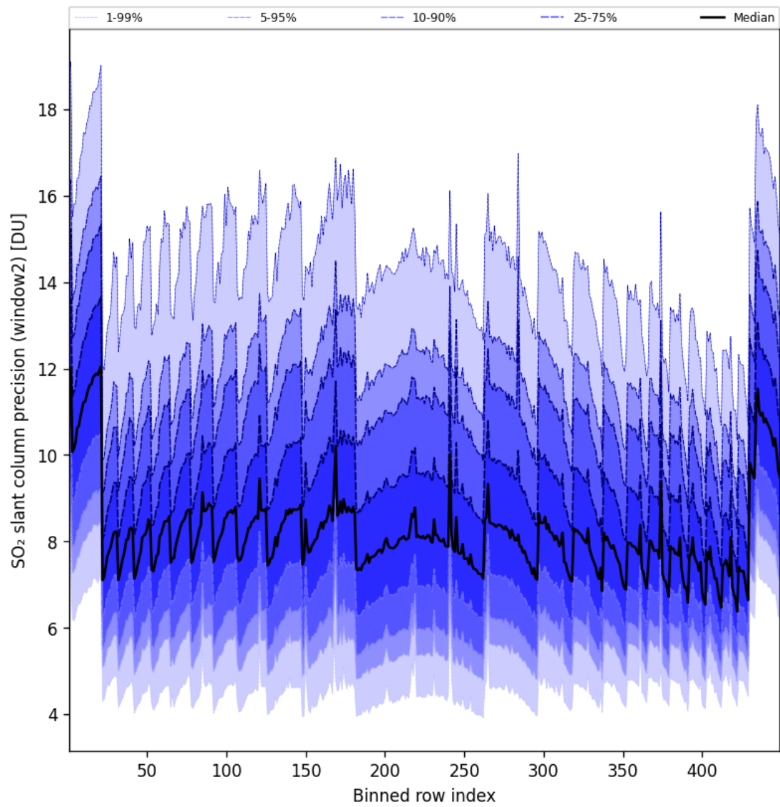
Figure 95: Along track statistics of “SO 2 slant column precision (window2)” for 2025-09-06 to 2025-09-07
