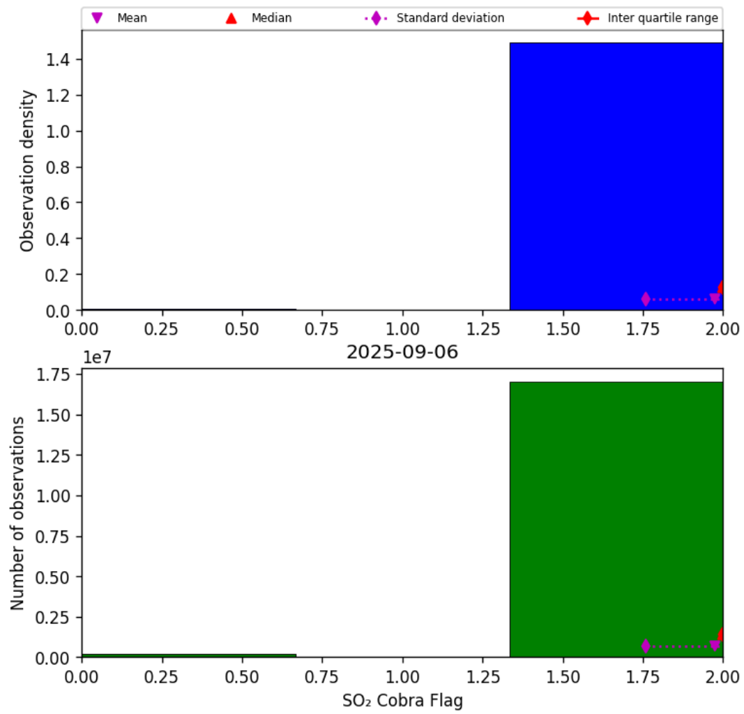
Figure 75: Histogram of "SO 2 Cobra Flag" for 2025-09-06 to 2025-09-07
