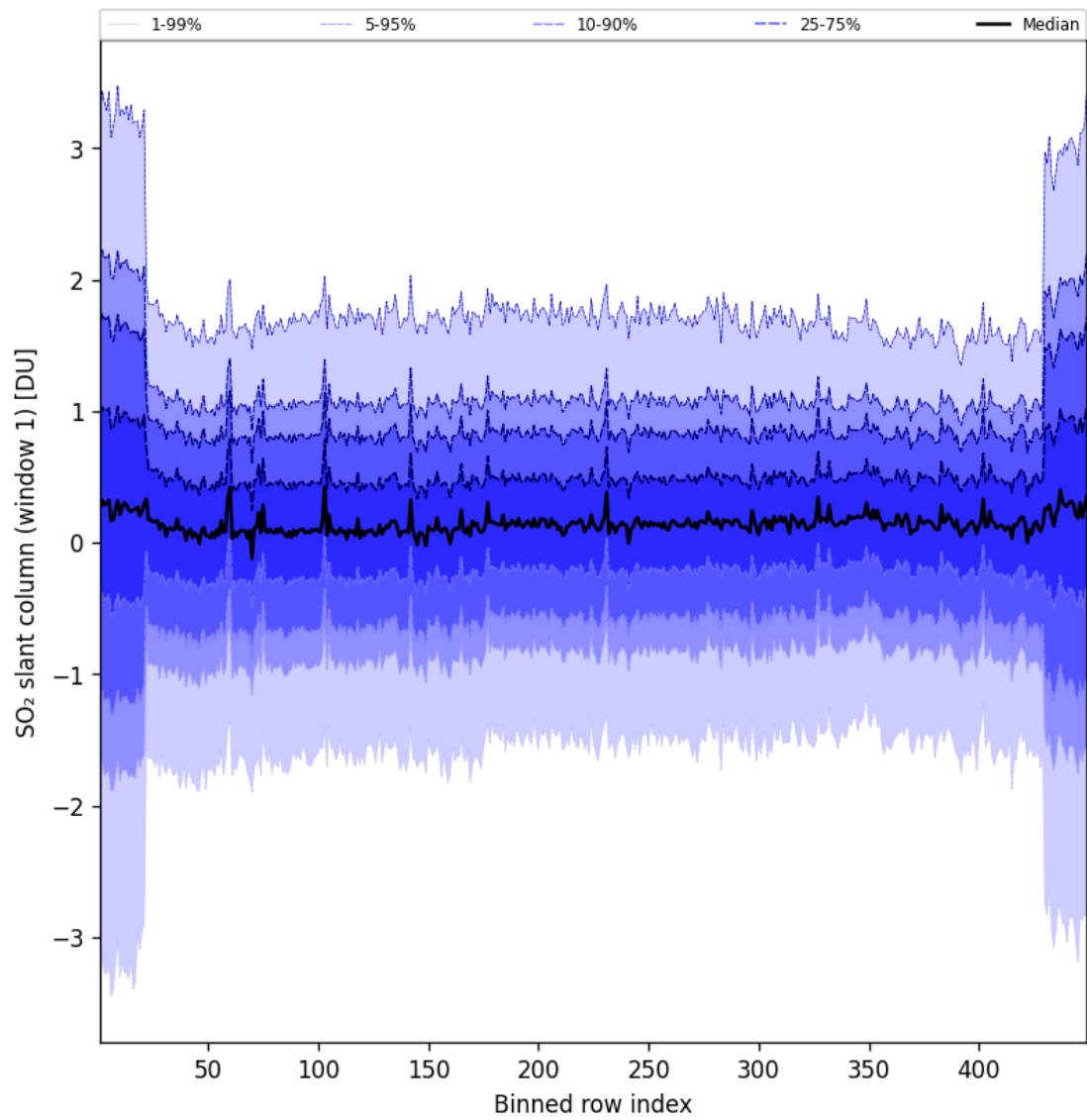
Figure 90: Along track statistics of “SO 2 slant column (window 1)” for 2025-09-06 to 2025-09-07
