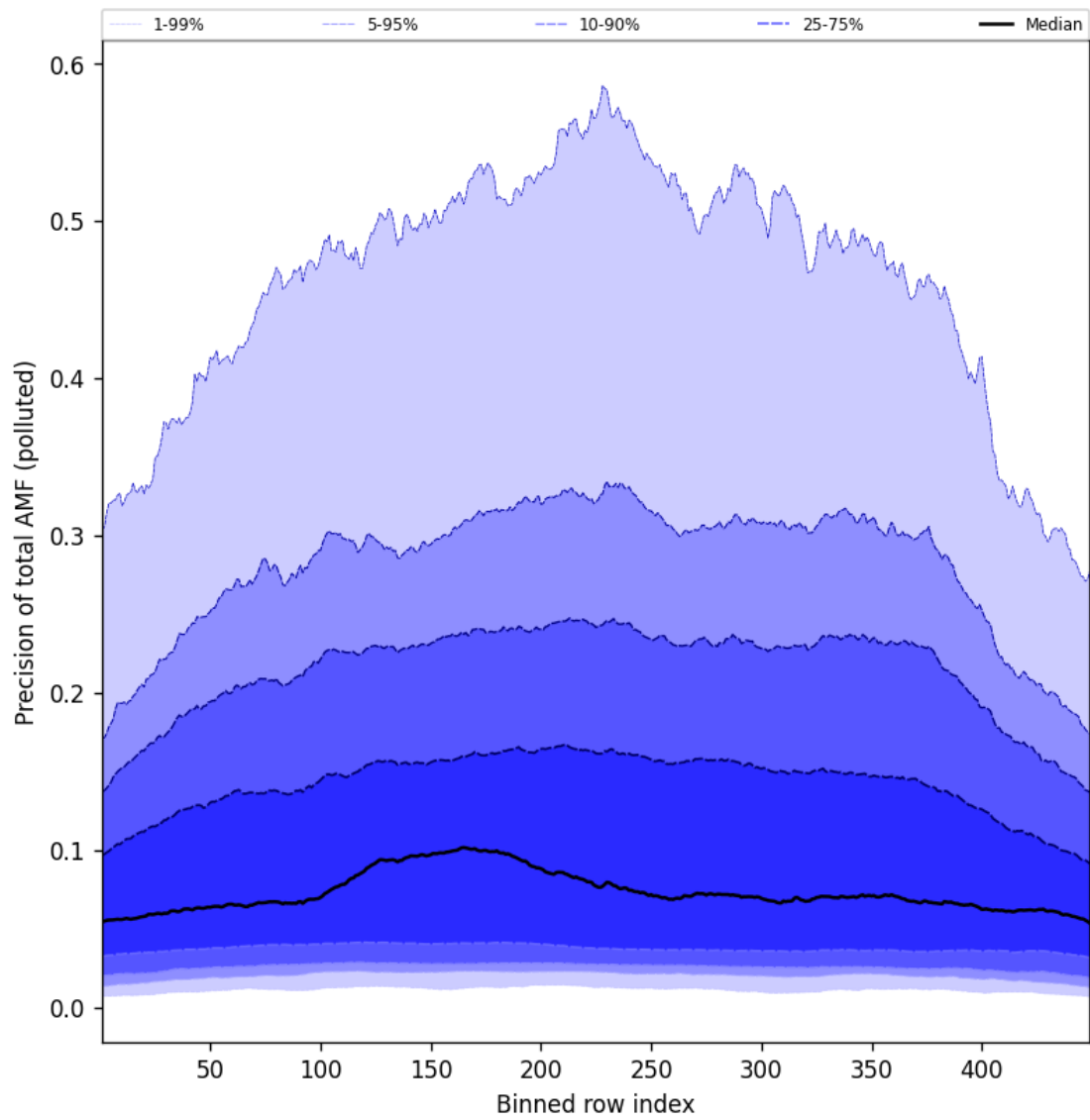
Figure 108: Along track statistics of “Precision of total AMF (polluted)” for 2025-09-06 to 2025-09-07
