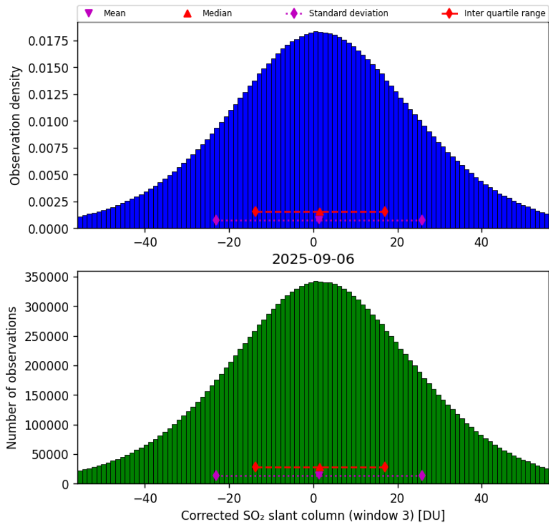
Figure 73: Histogram of “Corrected SO 2 slant column (window 3)” for 2025-09-06 to 2025-09-07
