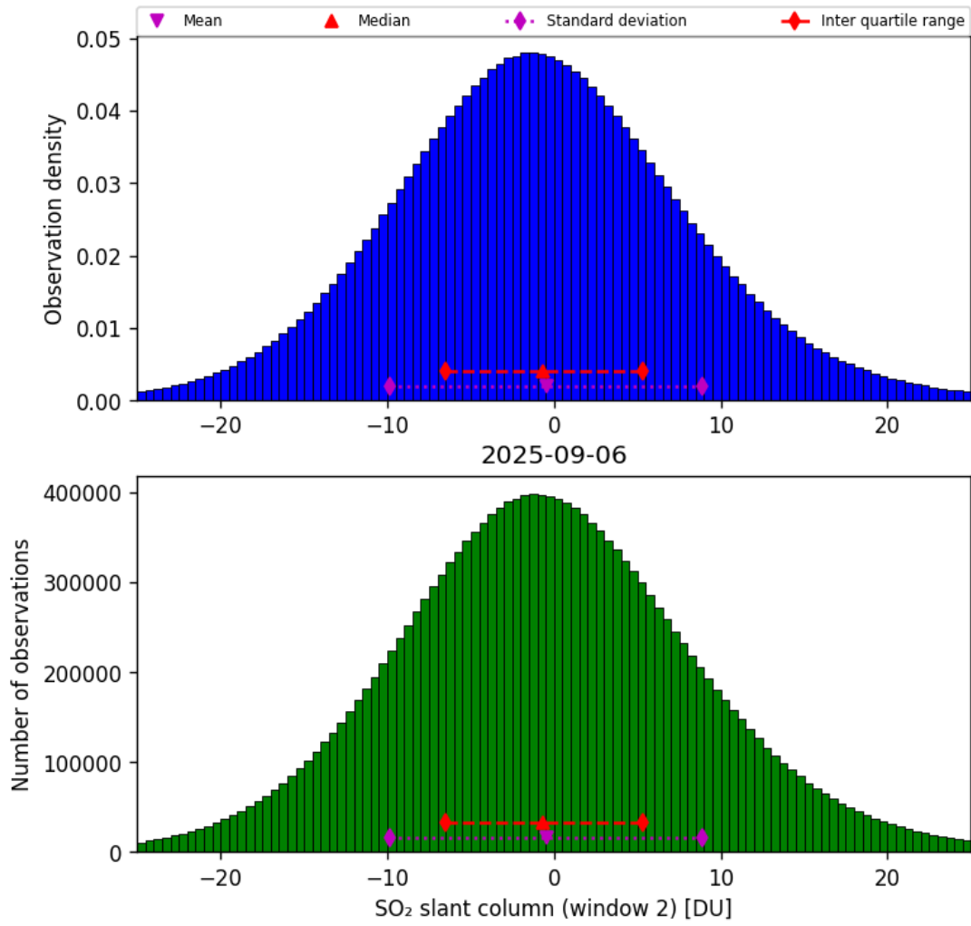
Figure 67: Histogram of “SO 2 slant column (window 2)” for 2025-09-06 to 2025-09-07
