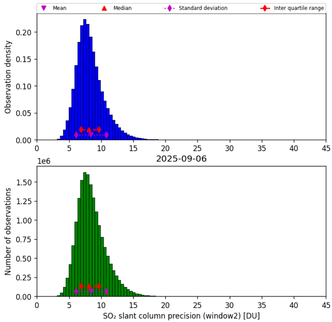
Figure 68: Histogram of “SO 2 slant column precision (window2)” for 2025-09-06 to 2025-09-07
