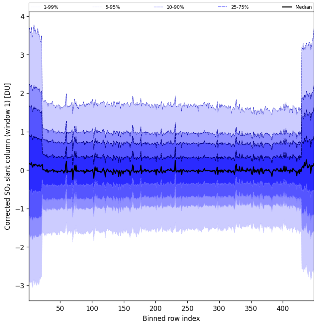
Figure 92: Along track statistics of “Corrected SO 2 slant column (window 1)” for 2025-09-06 to 2025-09-07
