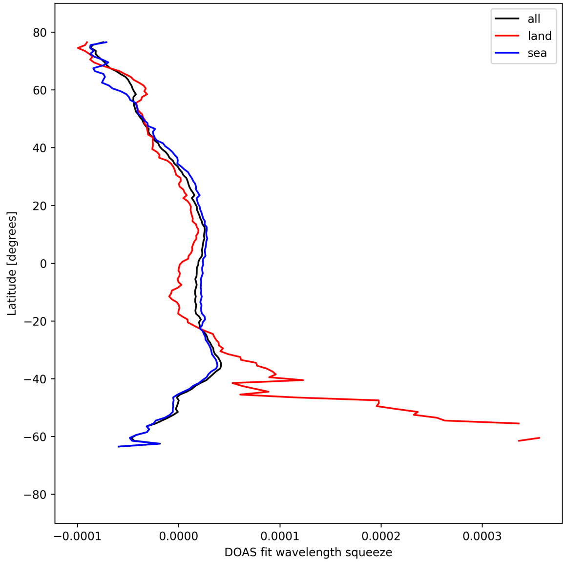
Figure 51: Zonal average of “DOAS fit wavelength squeeze” for 2025-09-06 to 2025-09-07.
