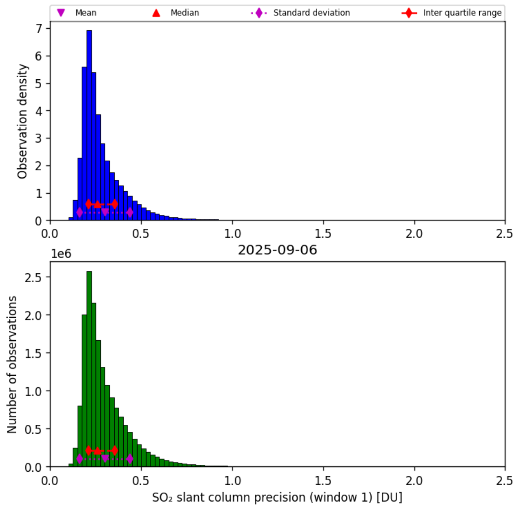
Figure 64: Histogram of “SO 2 slant column precision (window 1)” for 2025-09-06 to 2025-09-07
