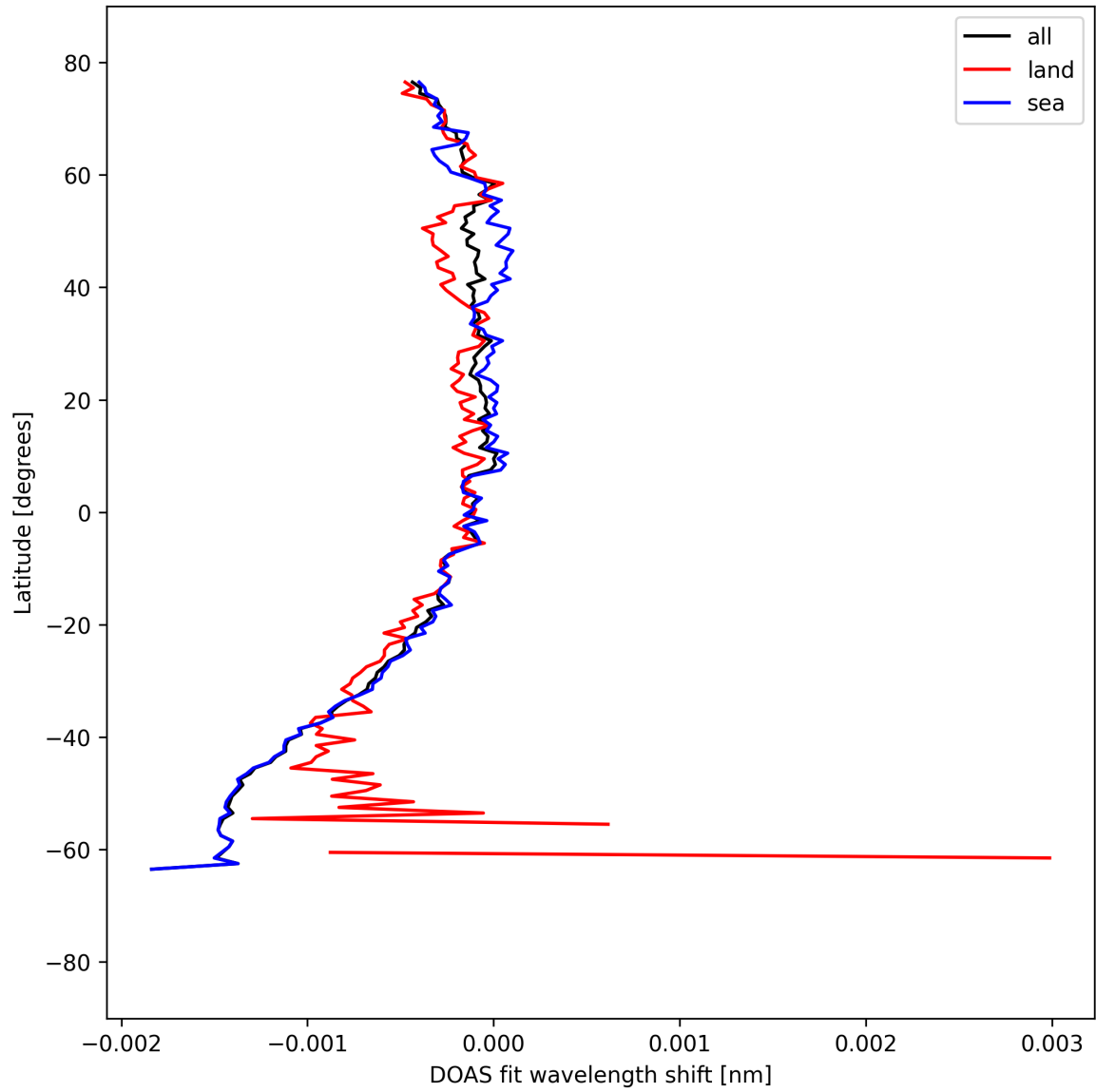
Figure 50: Zonal average of "DOAS fit wavelength shift" for 2025-09-06 to 2025-09-07.
