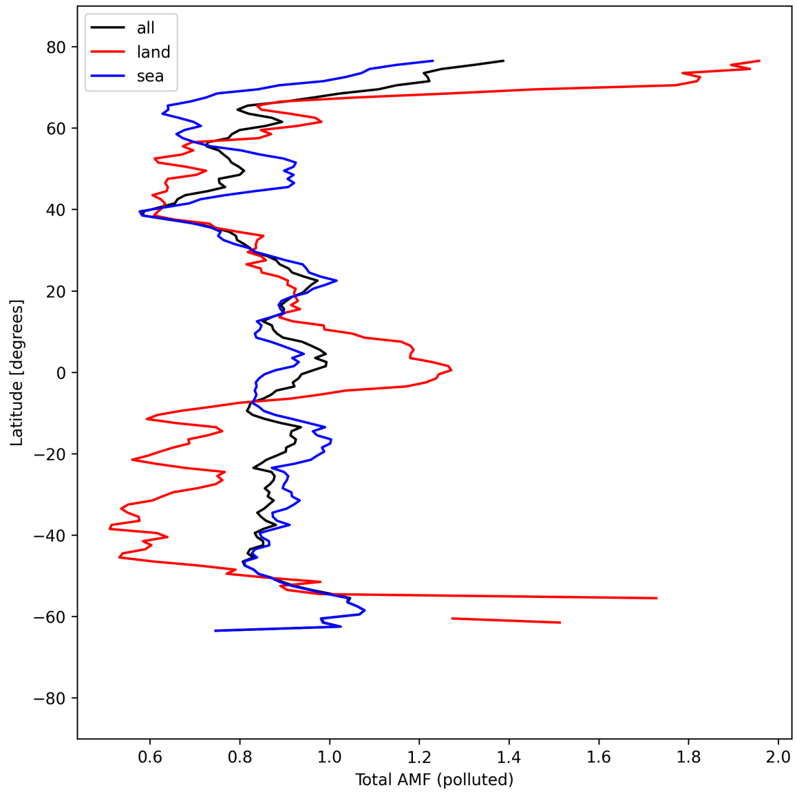
Figure 53: Zonal average of “Total AMF (polluted)” for 2025-09-06 to 2025-09-07.
