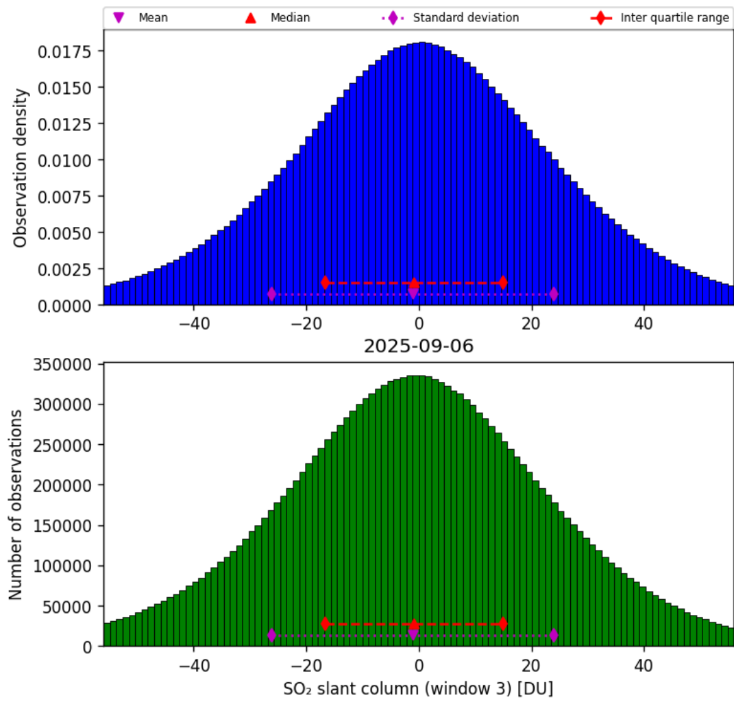
Figure 71: Histogram of “SO 2 slant column (window 3)” for 2025-09-06 to 2025-09-07
