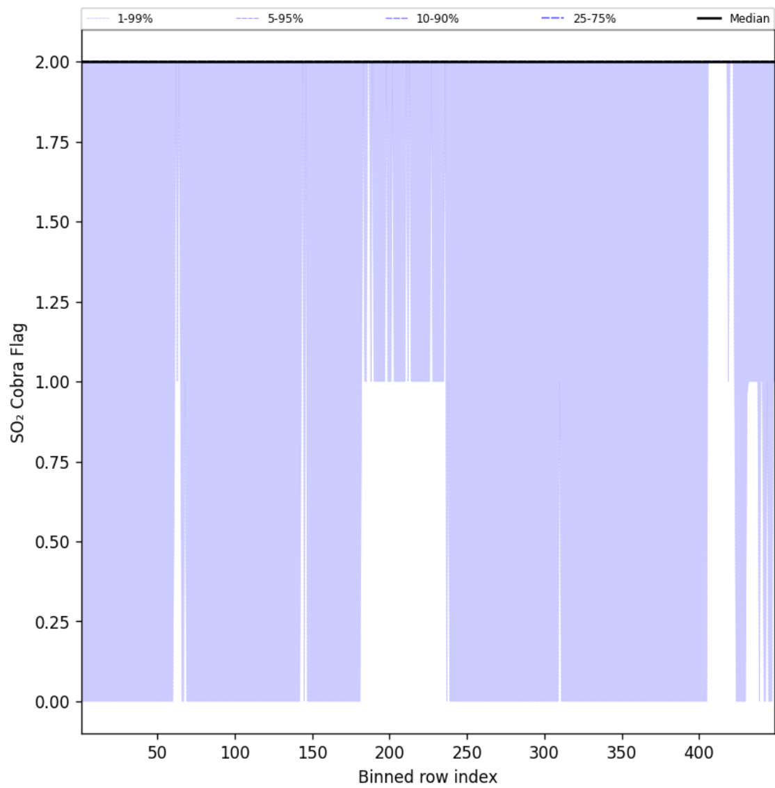
Figure 102: Along track statistics of “SO 2 Cobra Flag” for 2025-09-06 to 2025-09-07
