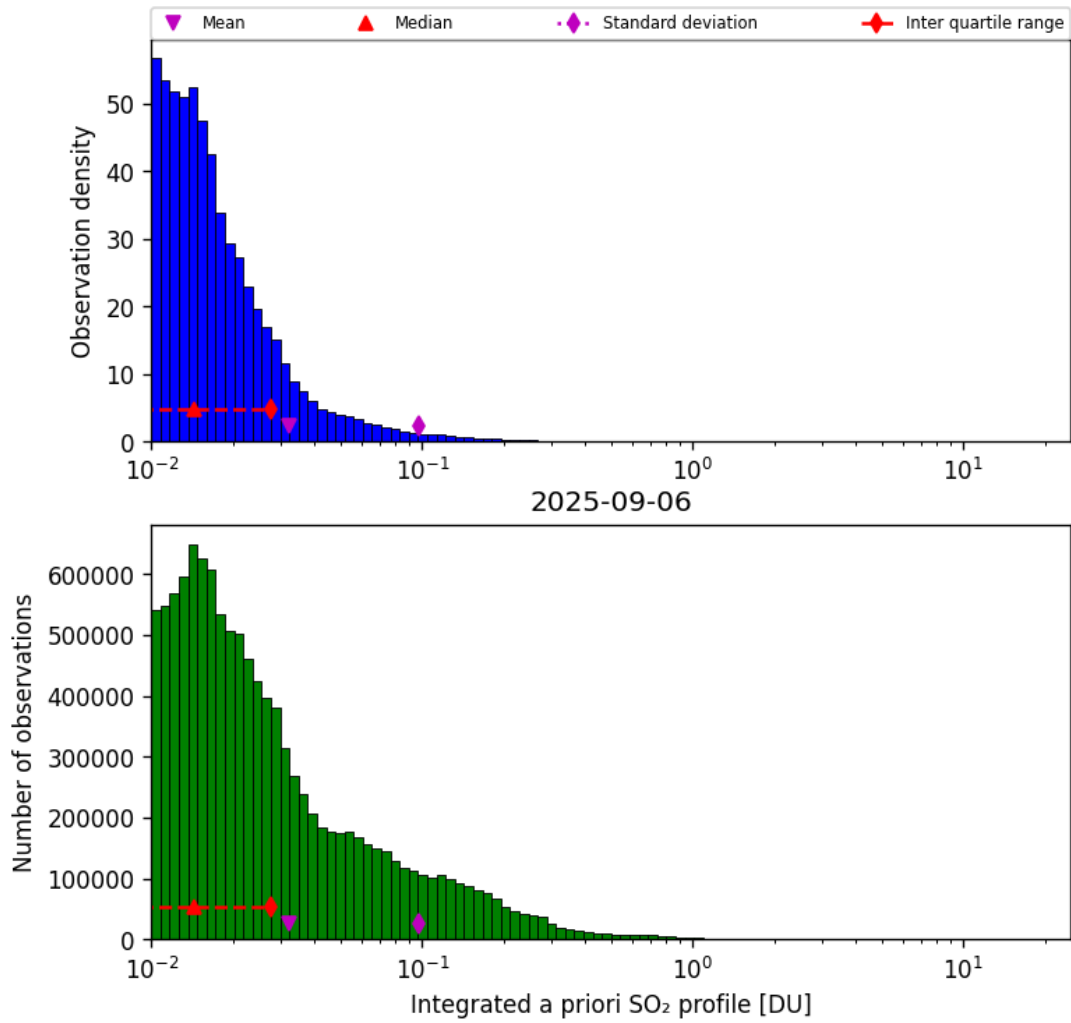
Figure 76: Histogram of “Integrated a priori SO 2 profile” for 2025-09-06 to 2025-09-07
