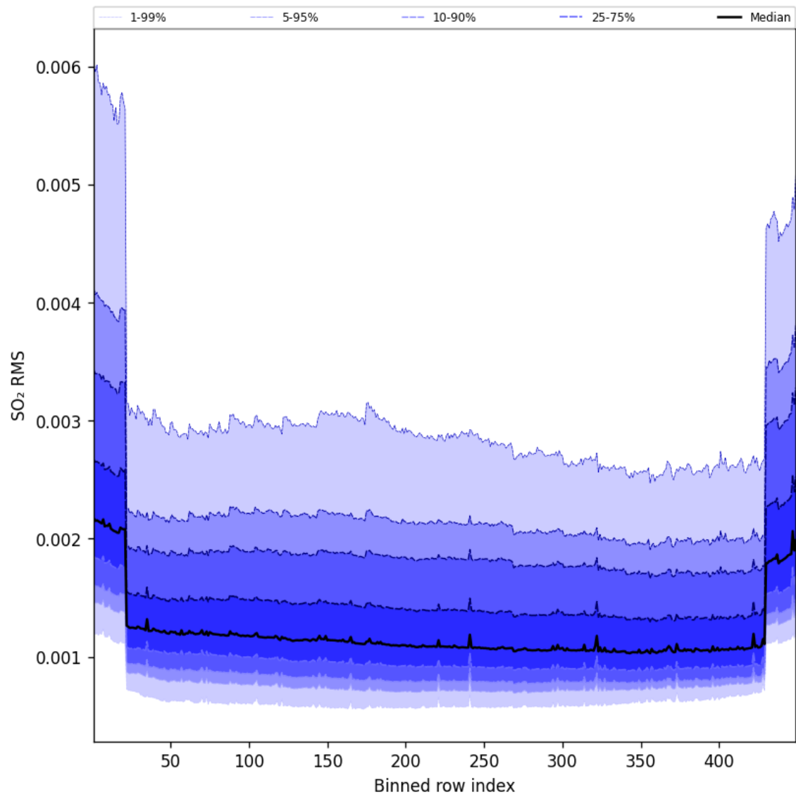
Figure 106: Along track statistics of “SO 2 RMS” for 2025-09-06 to 2025-09-07
