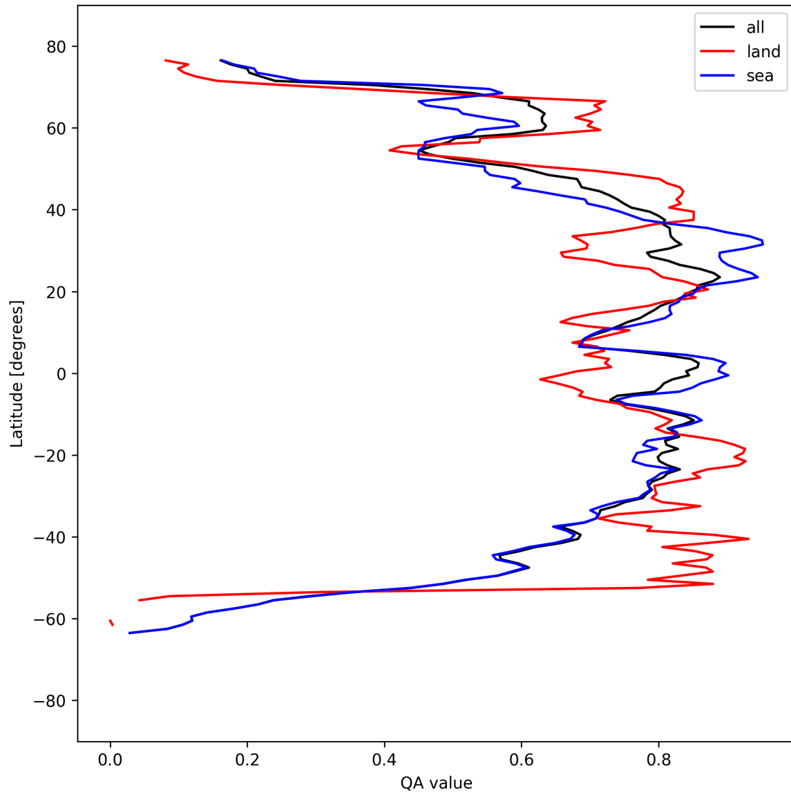
Figure 30: Zonal average of “QA value” for 2025-09-06 to 2025-09-07.
