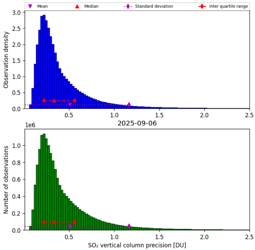
Figure 59: Histogram of “SO 2 vertical column precision” for 2025-09-06 to 2025-09-07
