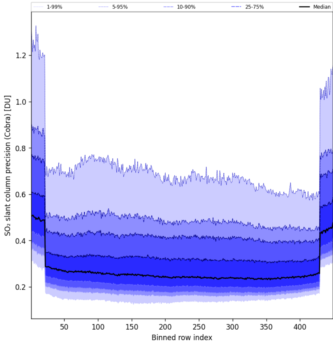
Figure 89: Along track statistics of “SO 2 slant column precision (Cobra)” for 2025-09-06 to 2025-09-07
