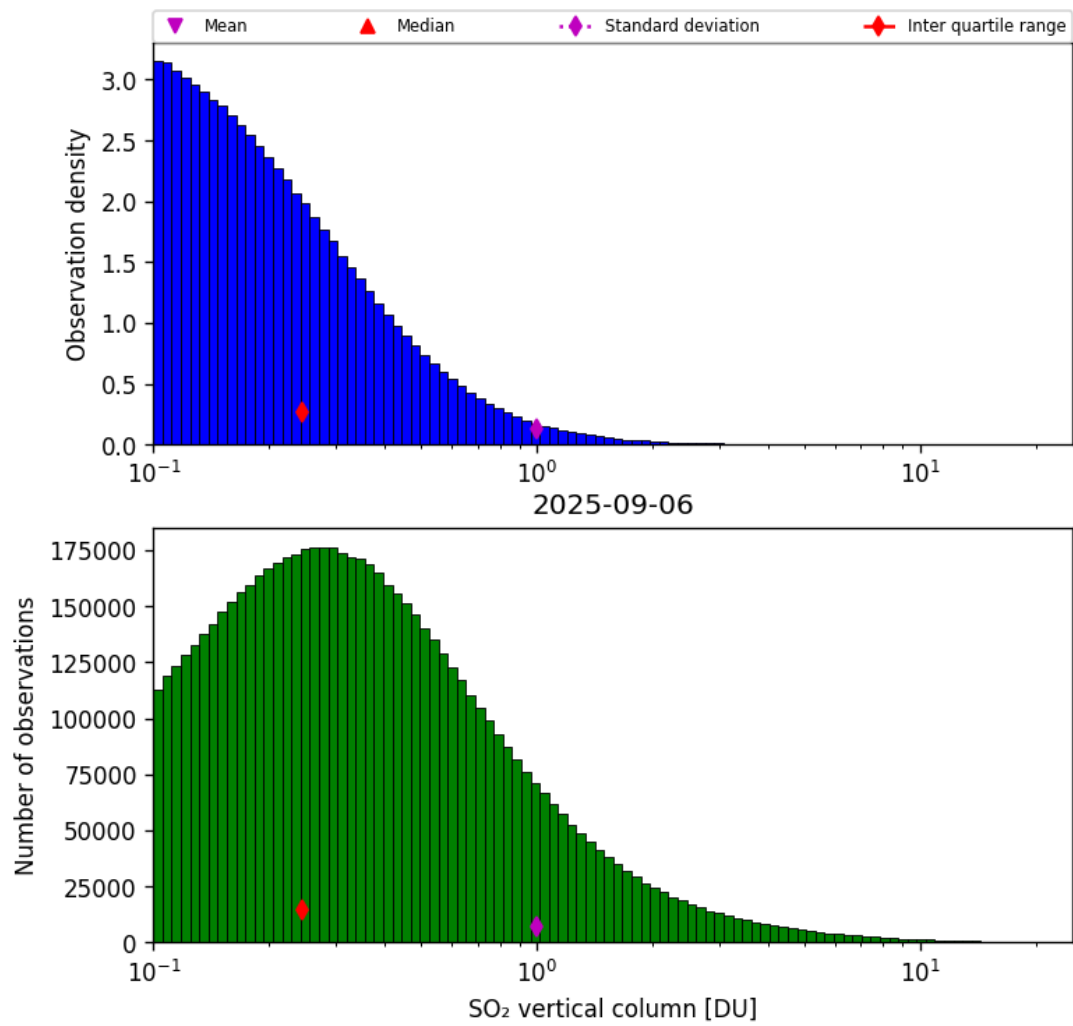
Figure 58: Histogram of “SO 2 vertical column” for 2025-09-06 to 2025-09-07
