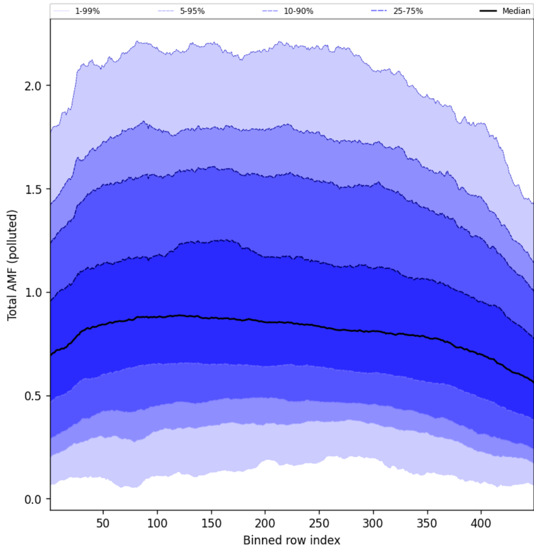
Figure 107: Along track statistics of “Total AMF (polluted)” for 2025-09-08 to 2025-09-08
