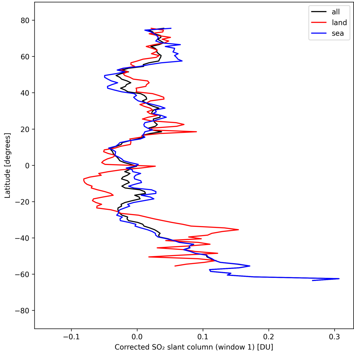
Figure 38: Zonal average of “Corrected SO 2 slant column (window 1)” for 2025-09-08 to 2025-09-08.
