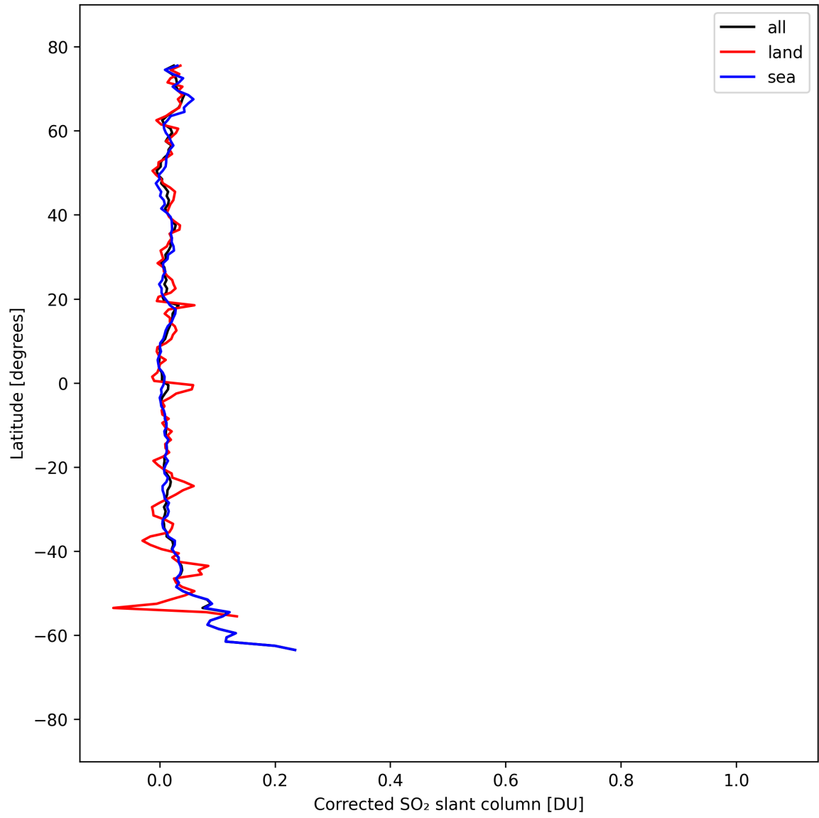
Figure 33: Zonal average of “Corrected SO 2 slant column” for 2025-09-08 to 2025-09-08.
