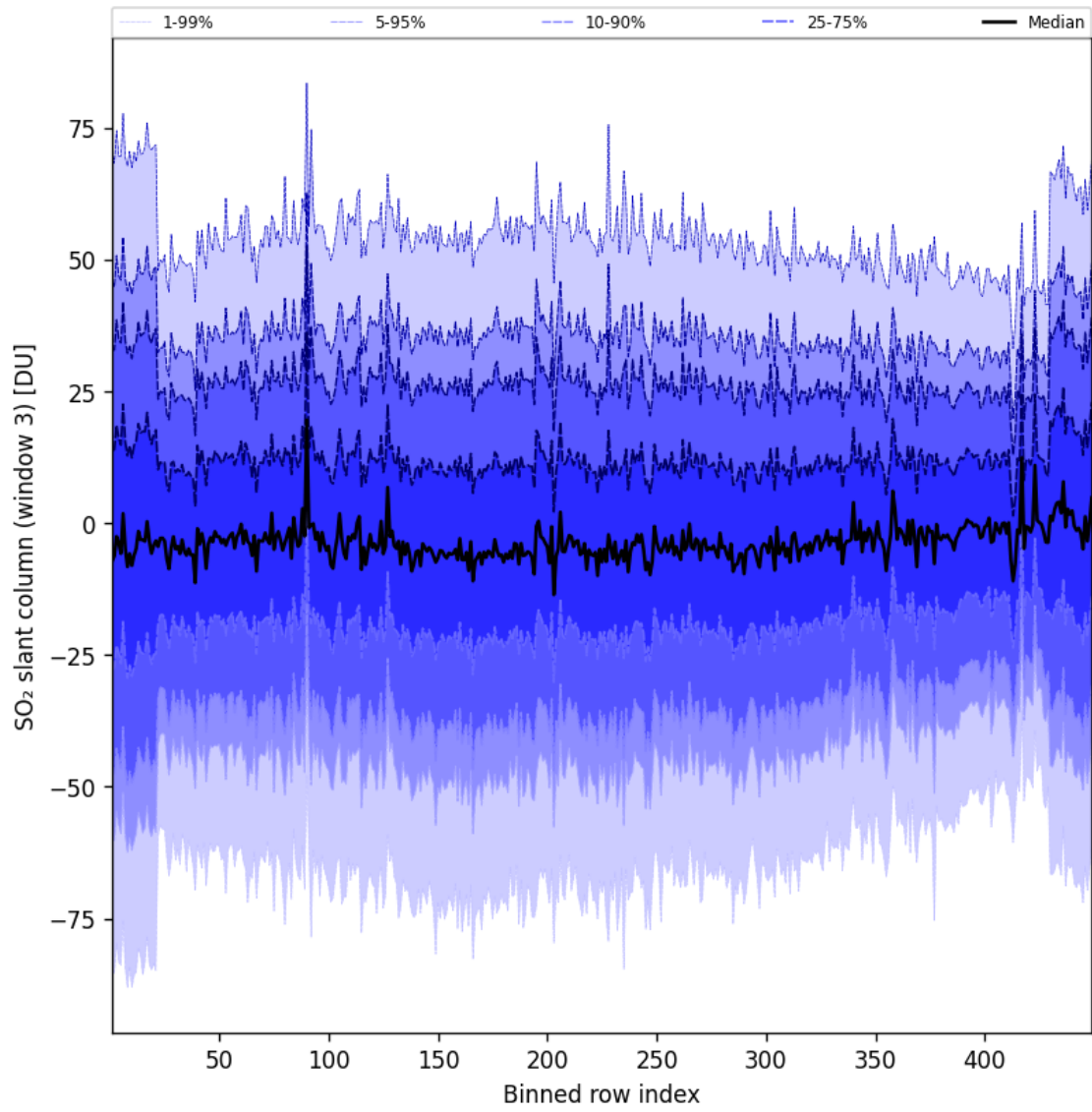
Figure 98: Along track statistics of “SO 2 slant column (window 3)” for 2025-09-08 to 2025-09-08
