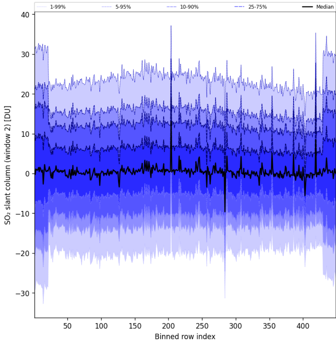
Figure 94: Along track statistics of “SO 2 slant column (window 2)” for 2025-09-08 to 2025-09-08
