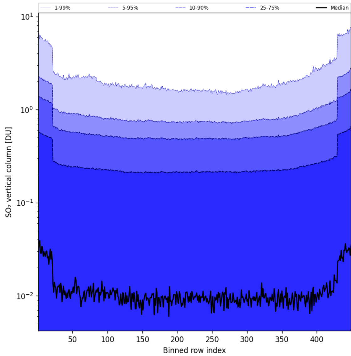
Figure 85: Along track statistics of “SO 2 vertical column” for 2025-09-08 to 2025-09-08
