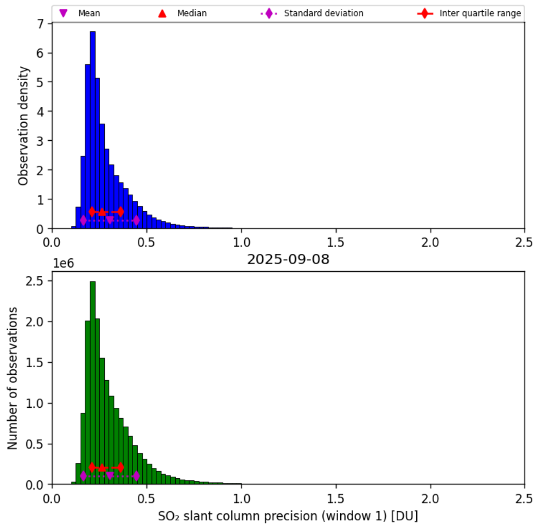
Figure 64: Histogram of “SO 2 slant column precision (window 1)” for 2025-09-08 to 2025-09-08
