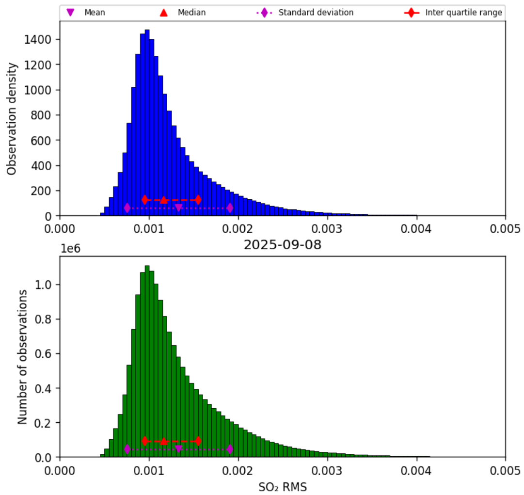
Figure 79: Histogram of “SO 2 RMS” for 2025-09-08 to 2025-09-08
