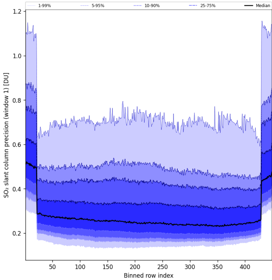
Figure 91: Along track statistics of “SO 2 slant column precision (window 1)” for 2025-09-08 to 2025-09-08
