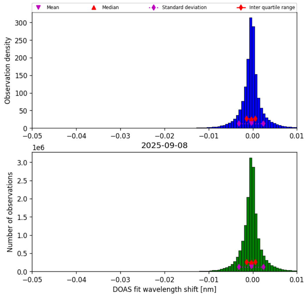
Figure 77: Histogram of “DOAS fit wavelength shift” for 2025-09-08 to 2025-09-08
