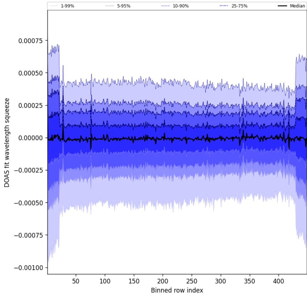
Figure 105: Along track statistics of “DOAS fit wavelength squeeze” for 2025-09-08 to 2025-09-08
