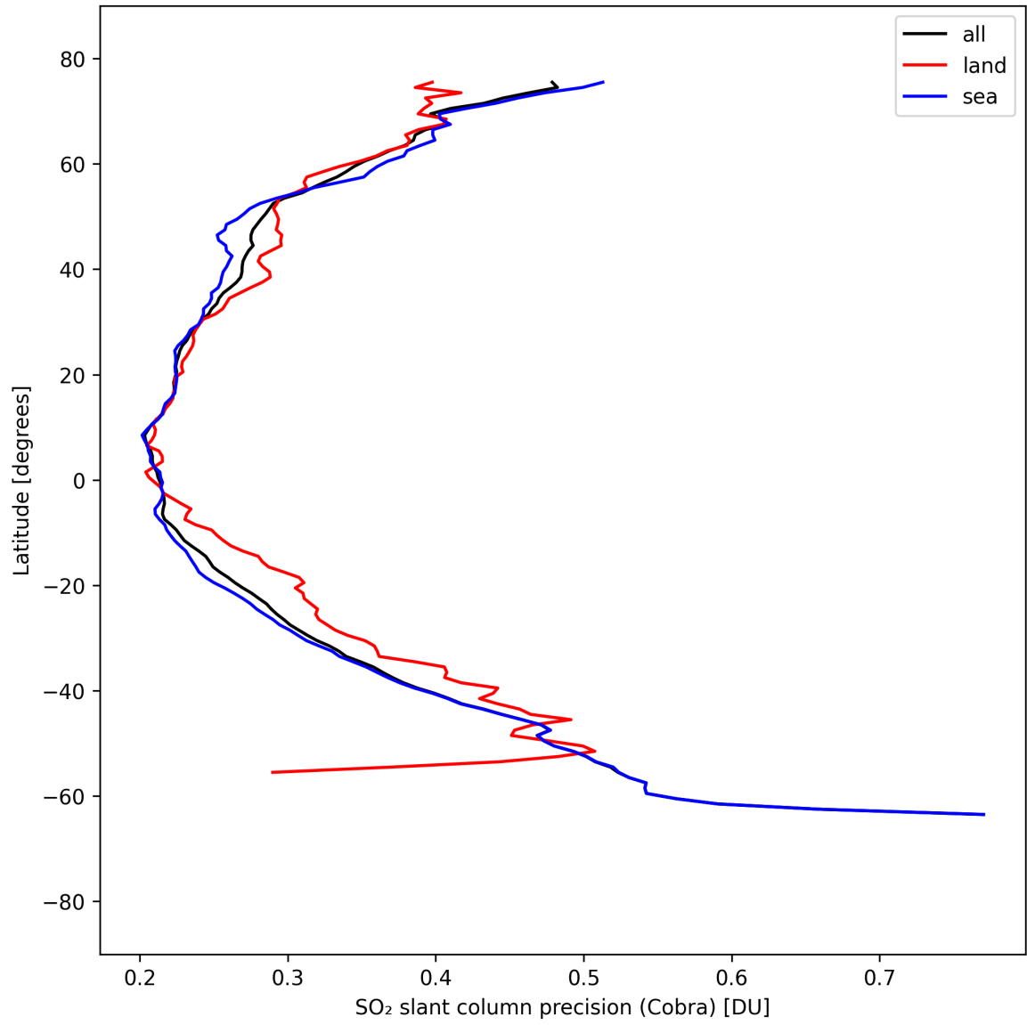
Figure 35: Zonal average of “SO 2 slant column precision (Cobra)” for 2025-09-08 to 2025-09-08.
