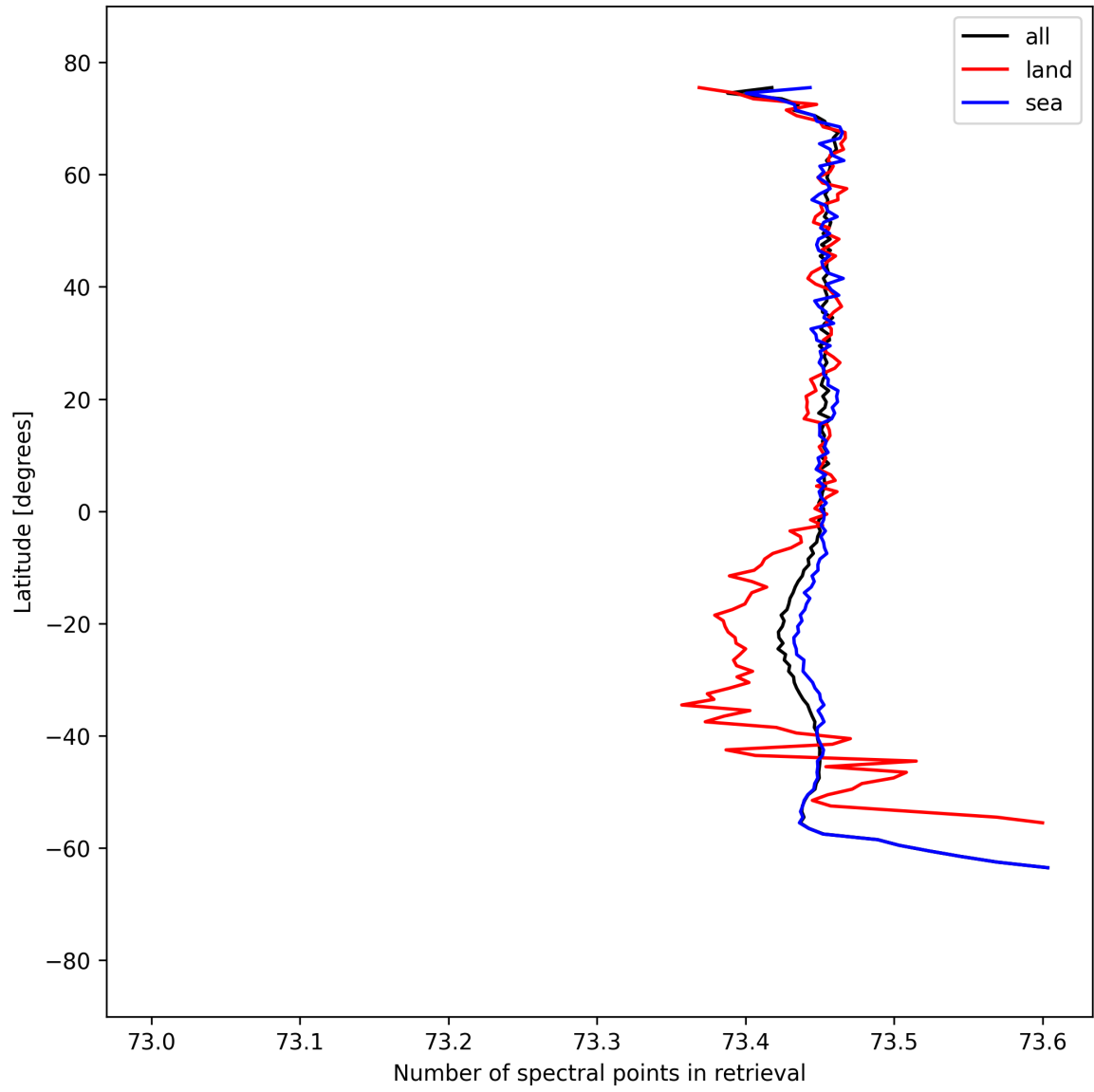
Figure 56: Zonal average of “Number of spectral points in retrieval” for 2025-09-08 to 2025-09-08.
