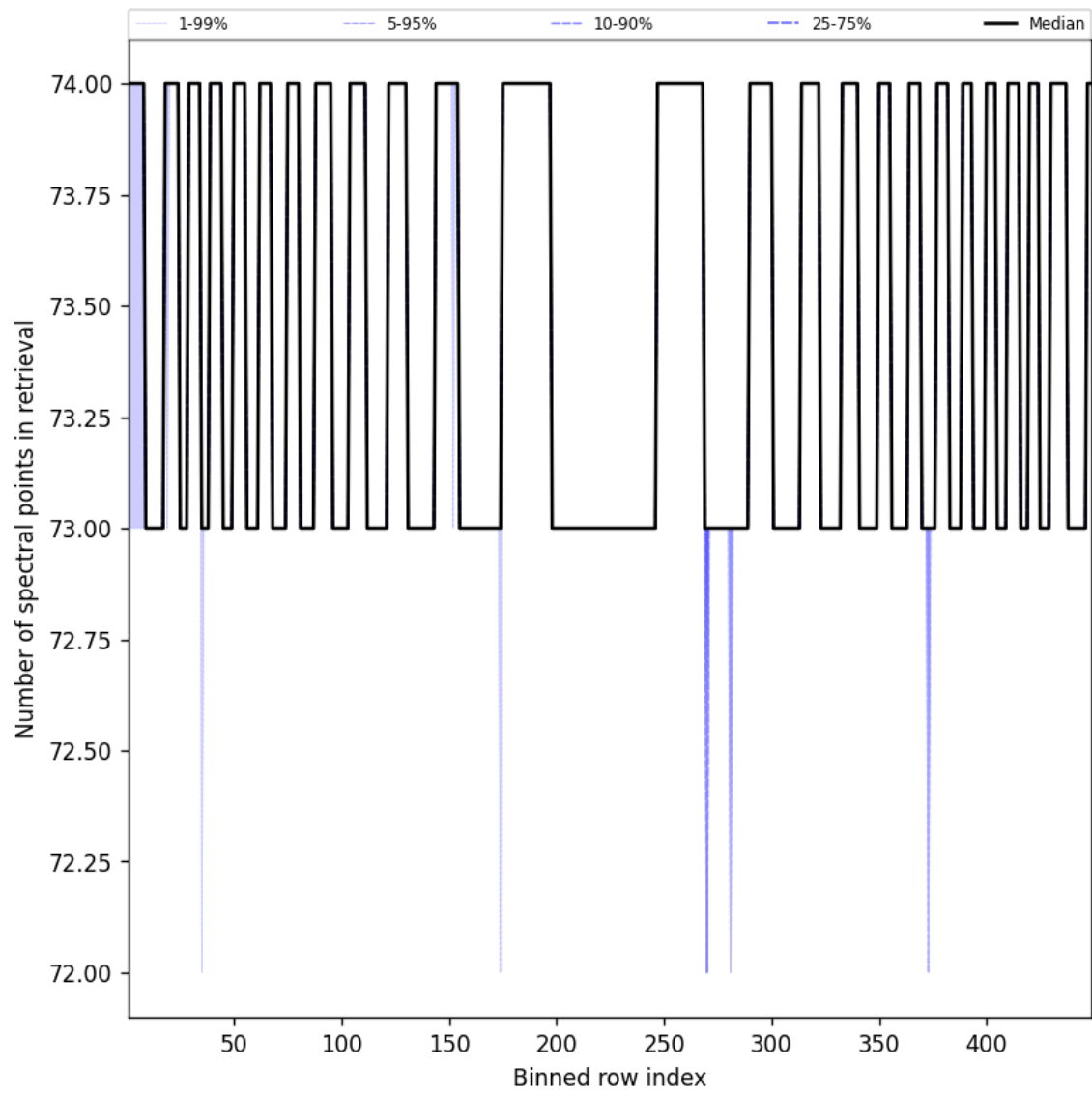
Figure 110: Along track statistics of “Number of spectral points in retrieval” for 2025-09-08 to 2025-09-08
