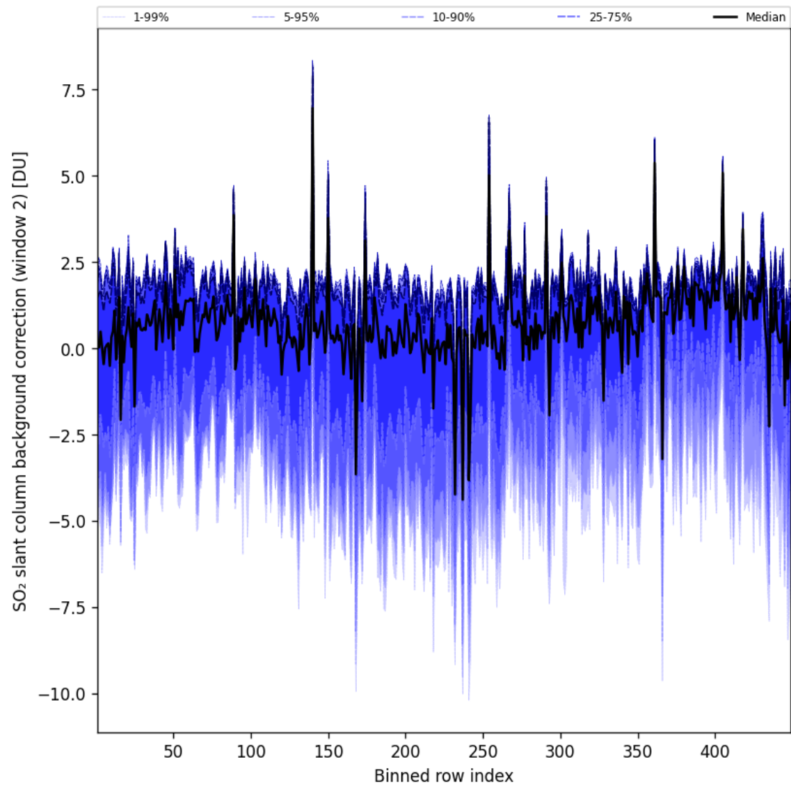
Figure 97: Along track statistics of “SO 2 slant column background correction (window 2)” for 2025-09-08 to 2025-09-08
