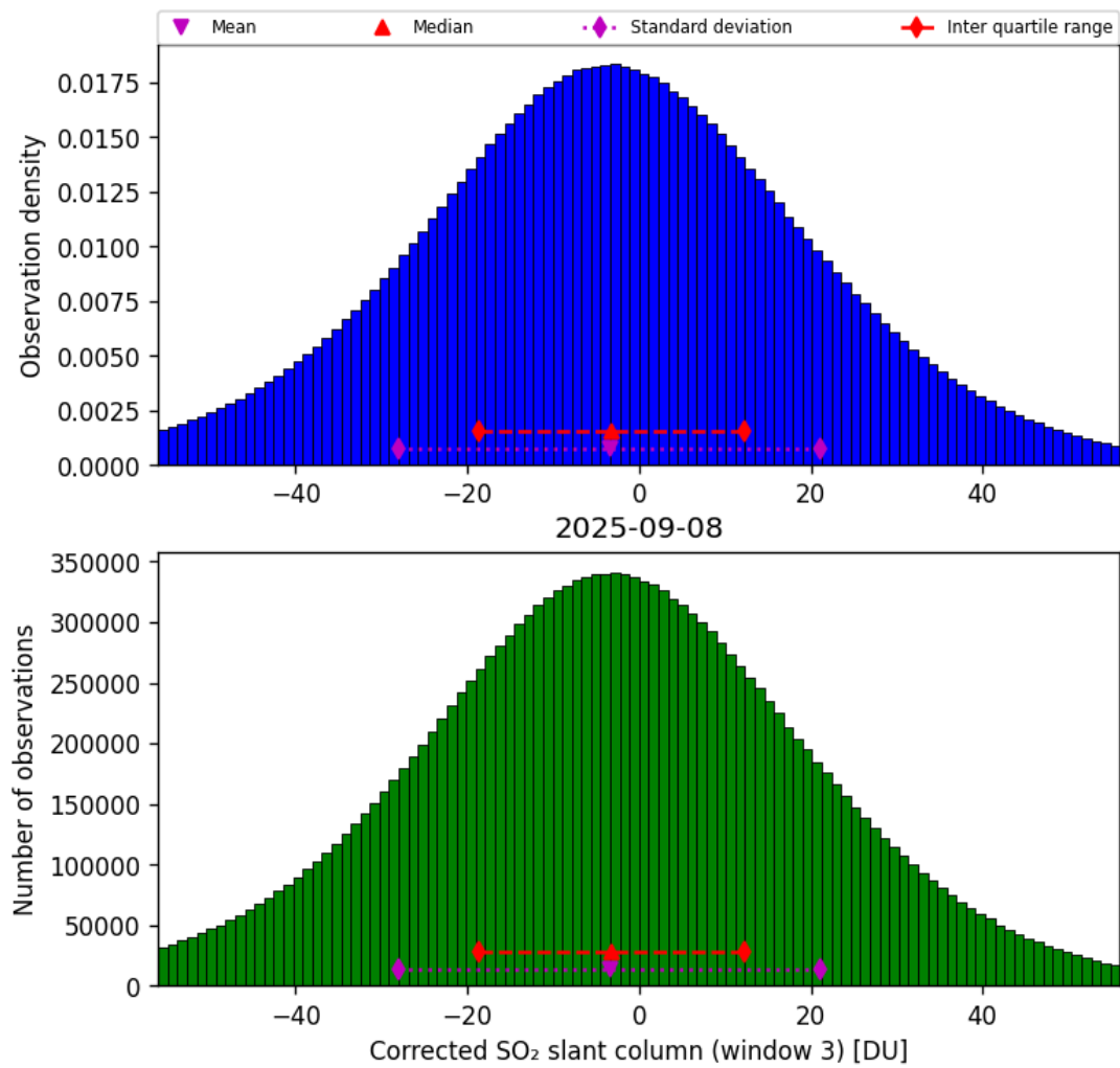
Figure 73: Histogram of “Corrected SO 2 slant column (window 3)” for 2025-09-08 to 2025-09-08
