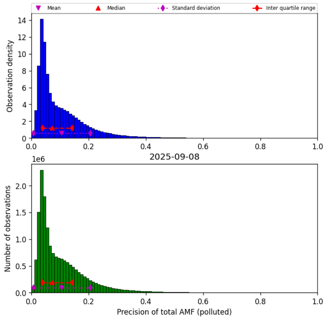
Figure 81: Histogram of “Precision of total AMF (polluted)” for 2025-09-08 to 2025-09-08
