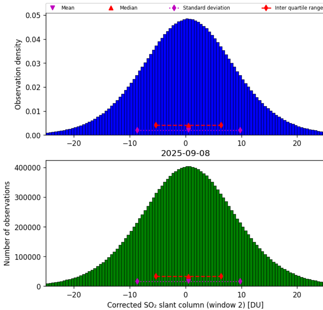
Figure 69: Histogram of “Corrected SO 2 slant column (window 2)” for 2025-09-08 to 2025-09-08
