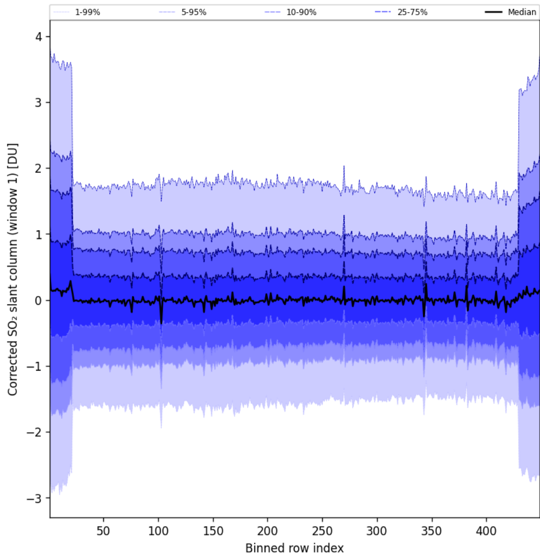
Figure 92: Along track statistics of “Corrected SO 2 slant column (window 1)” for 2025-09-08 to 2025-09-08
