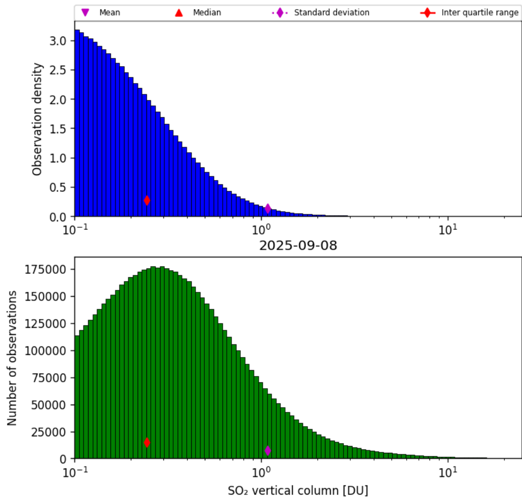
Figure 58: Histogram of “SO 2 vertical column” for 2025-09-08 to 2025-09-08
