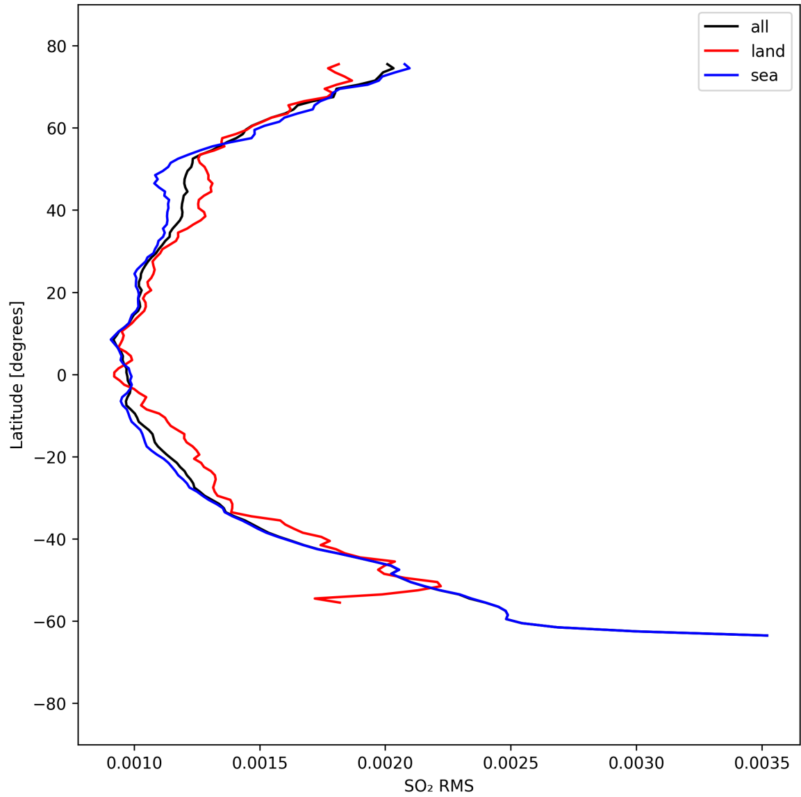
Figure 52: Zonal average of “SO 2 RMS” for 2025-09-08 to 2025-09-08.
