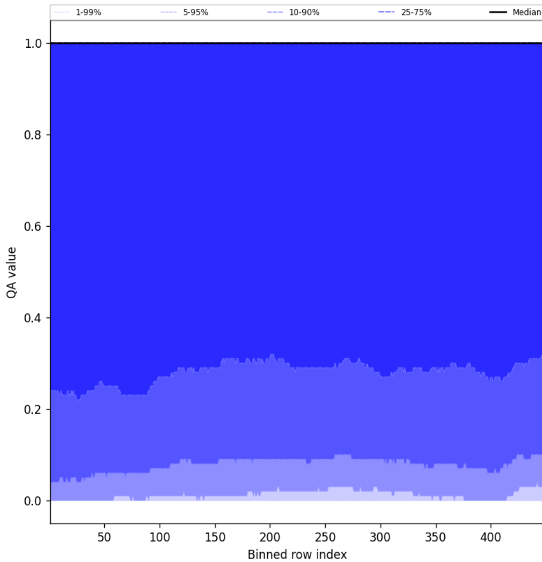
Figure 84: Along track statistics of “QA value” for 2025-09-08 to 2025-09-08
