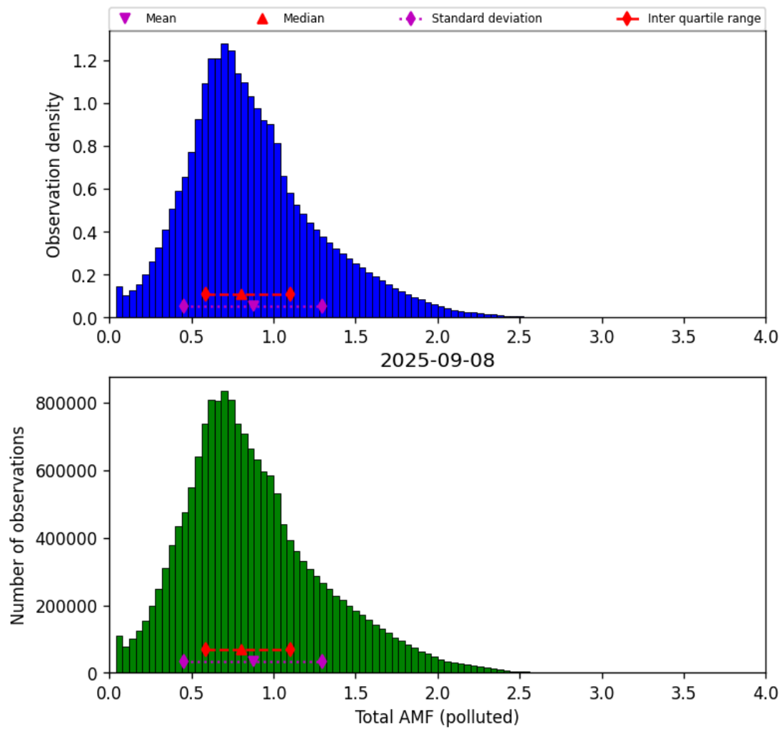
Figure 80: Histogram of “Total AMF (polluted)” for 2025-09-08 to 2025-09-08
