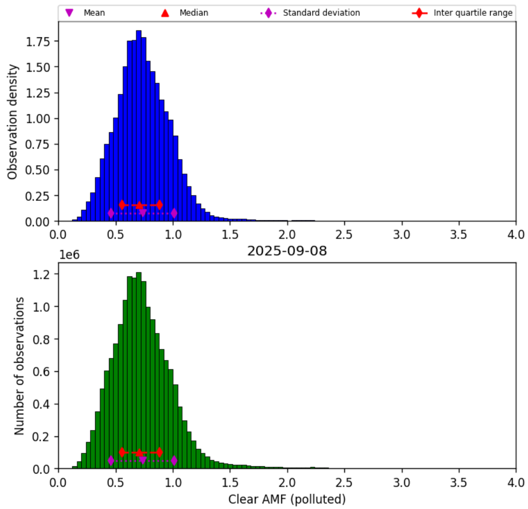
Figure 82: Histogram of “Clear AMF (polluted)” for 2025-09-08 to 2025-09-08
