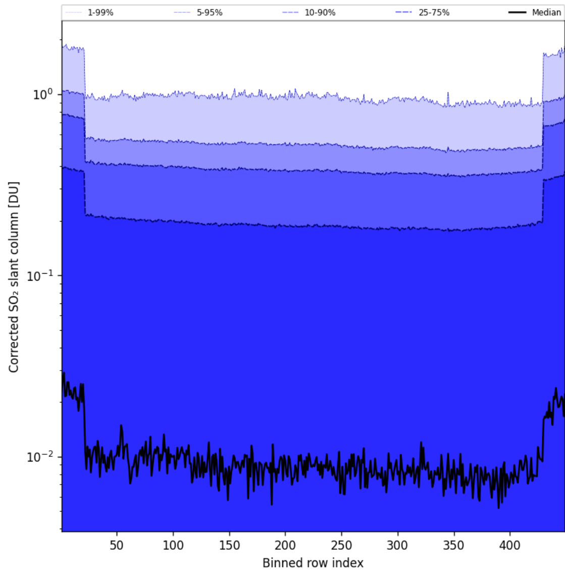
Figure 87: Along track statistics of “Corrected SO 2 slant column” for 2025-09-08 to 2025-09-08
