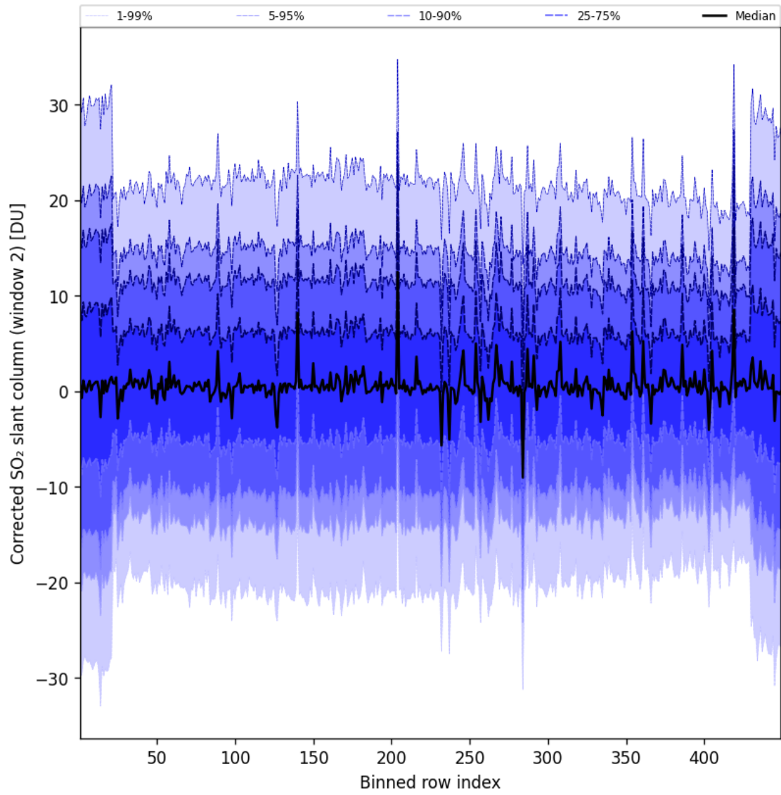
Figure 96: Along track statistics of “Corrected SO 2 slant column (window 2)” for 2025-09-08 to 2025-09-08
