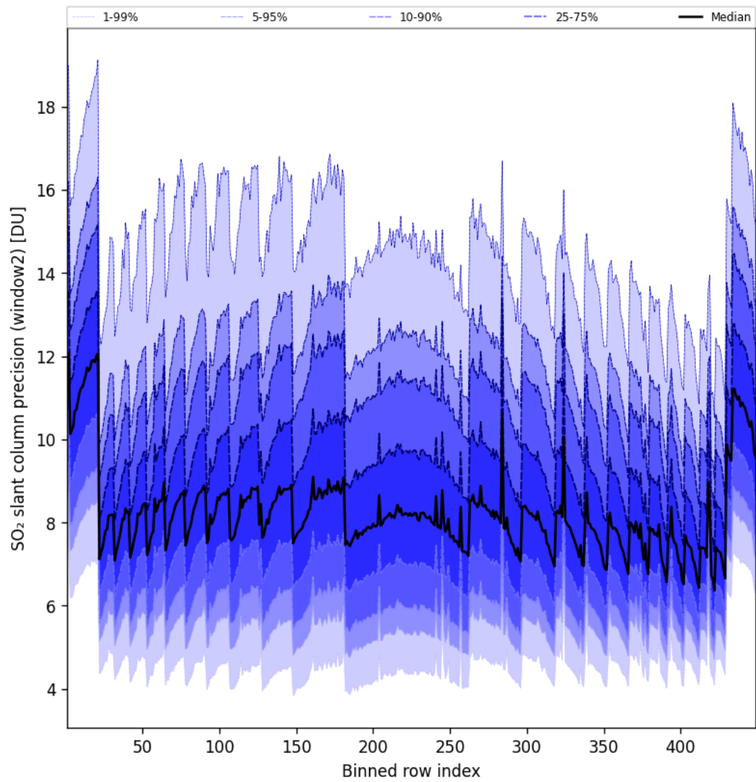
Figure 95: Along track statistics of “SO 2 slant column precision (window2)” for 2025-09-08 to 2025-09-08
