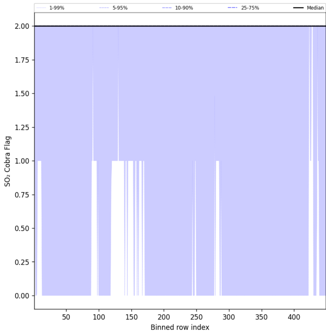
Figure 102: Along track statistics of "SO 2 Cobra Flag" for 2025-09-08 to 2025-09-08
