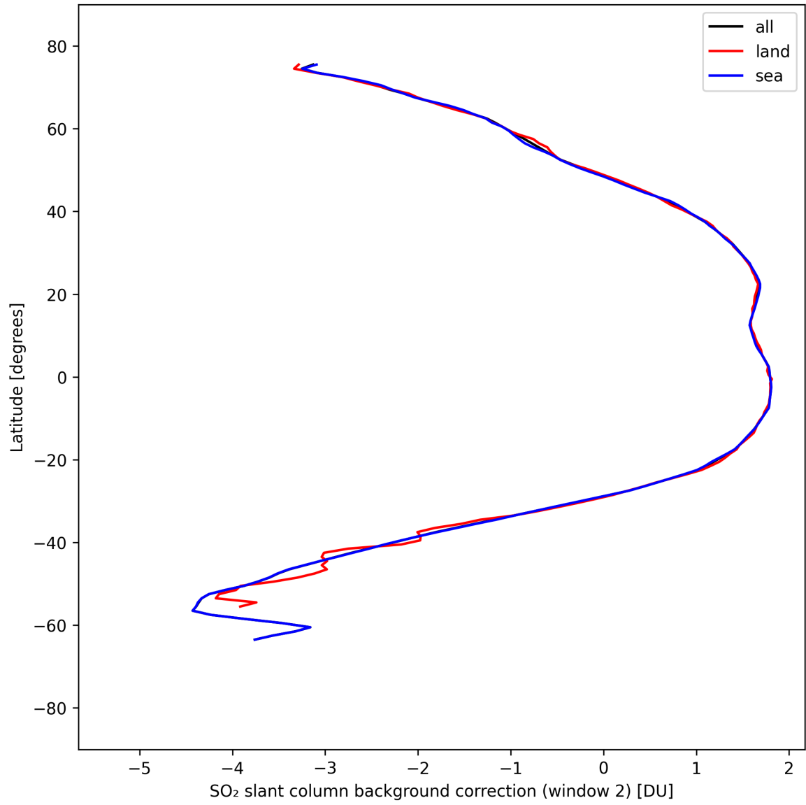
Figure 43: Zonal average of “SO 2 slant column background correction (window 2)” for 2025-09-08 to 2025-09-08.
