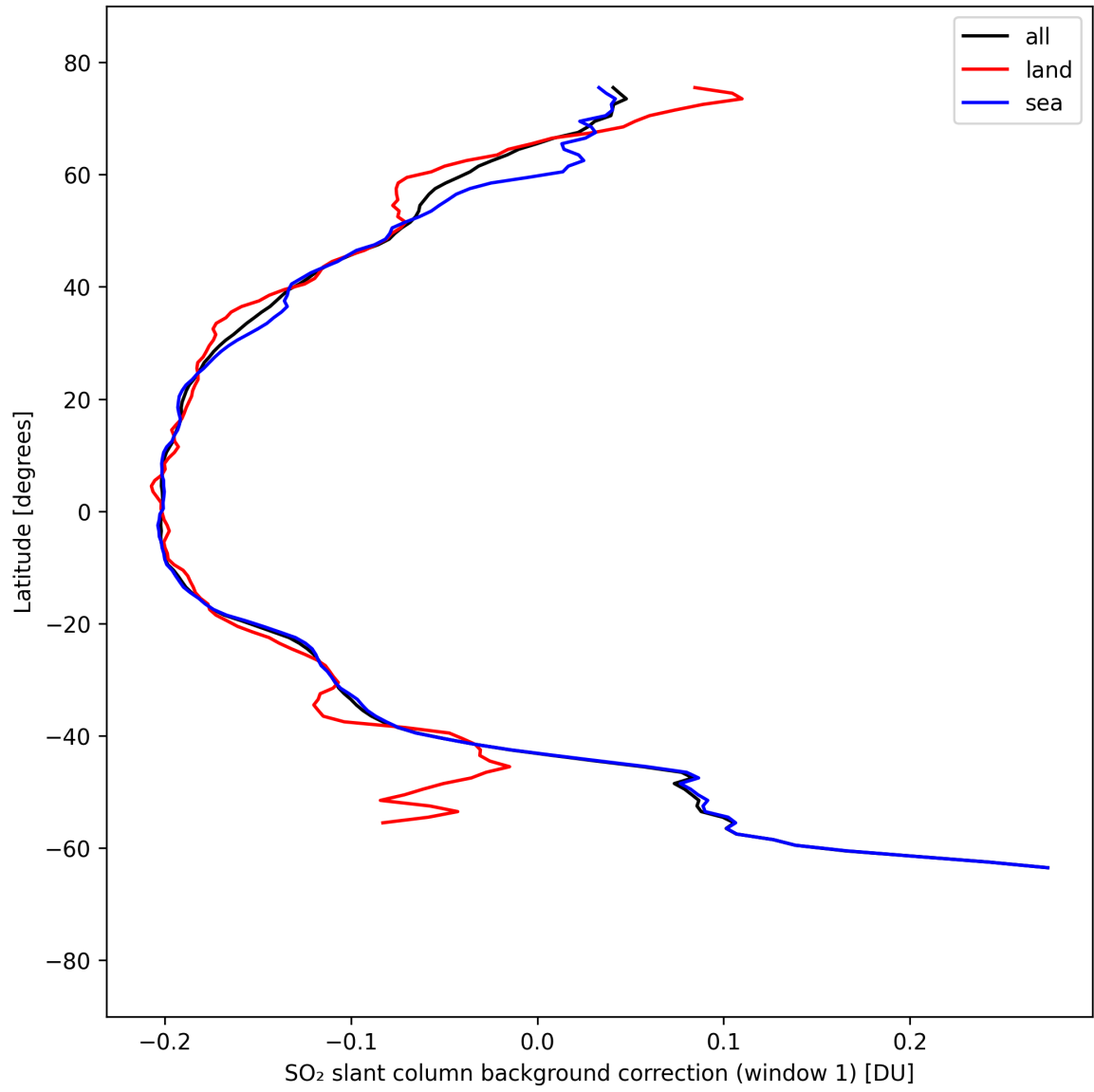
Figure 39: Zonal average of “SO 2 slant column background correction (window 1)” for 2025-09-08 to 2025-09-08.
