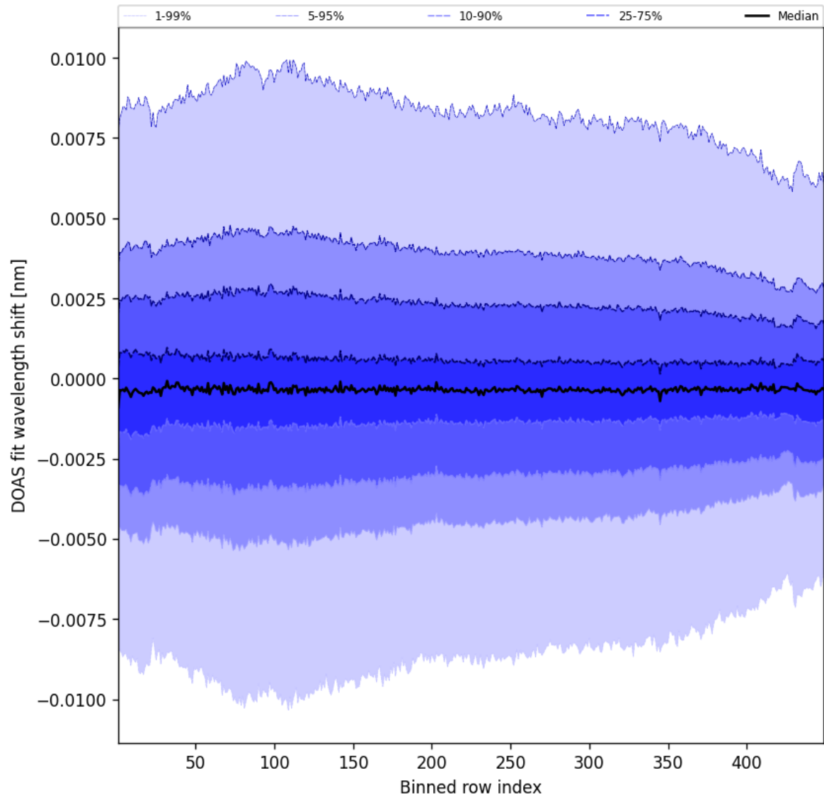
Figure 104: Along track statistics of “DOAS fit wavelength shift” for 2025-09-08 to 2025-09-08
