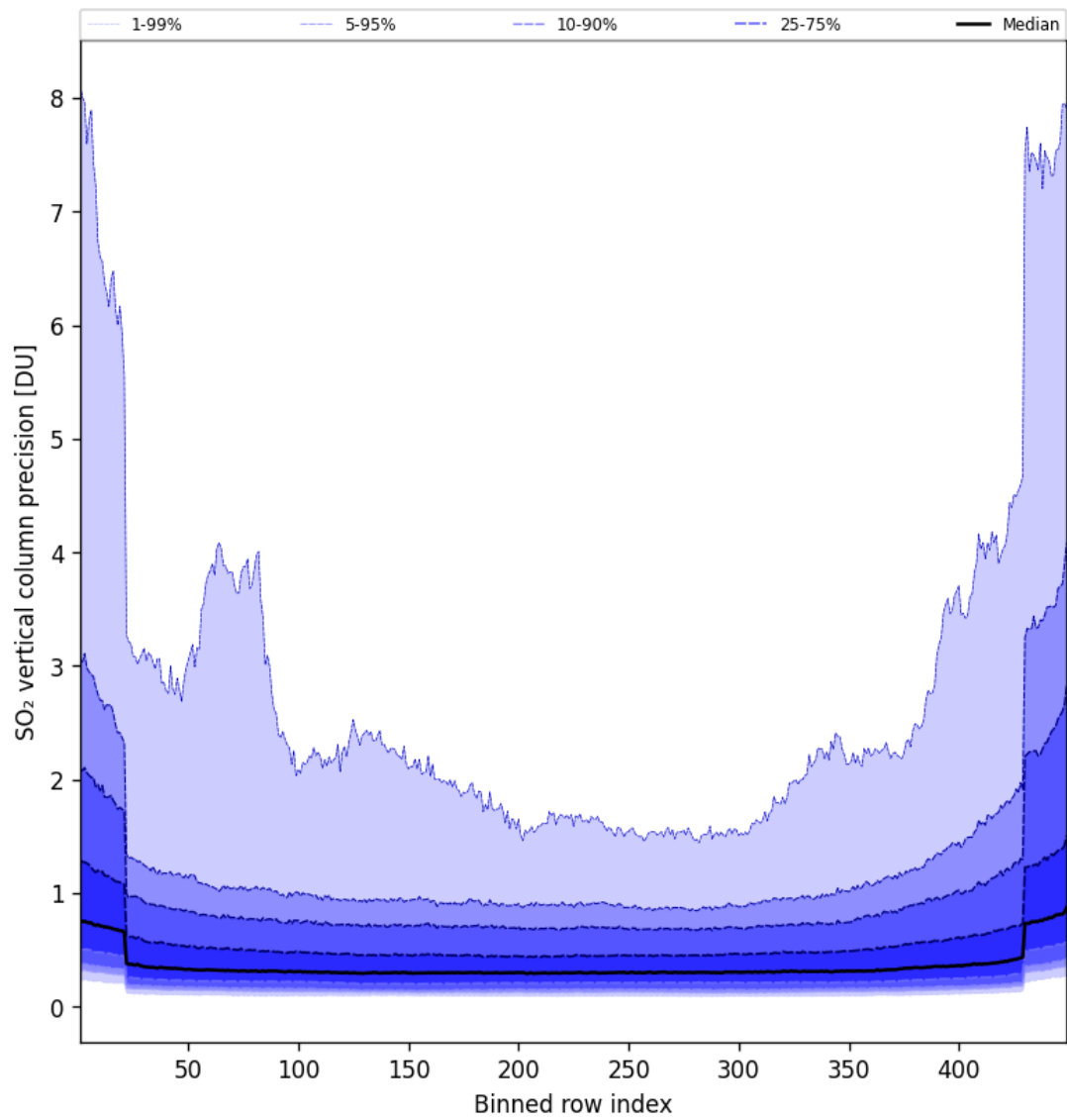
Figure 86: Along track statistics of “SO 2 vertical column precision” for 2025-09-08 to 2025-09-08
