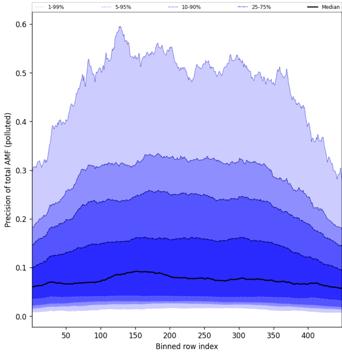
Figure 108: Along track statistics of “Precision of total AMF (polluted)” for 2025-09-08 to 2025-09-08
