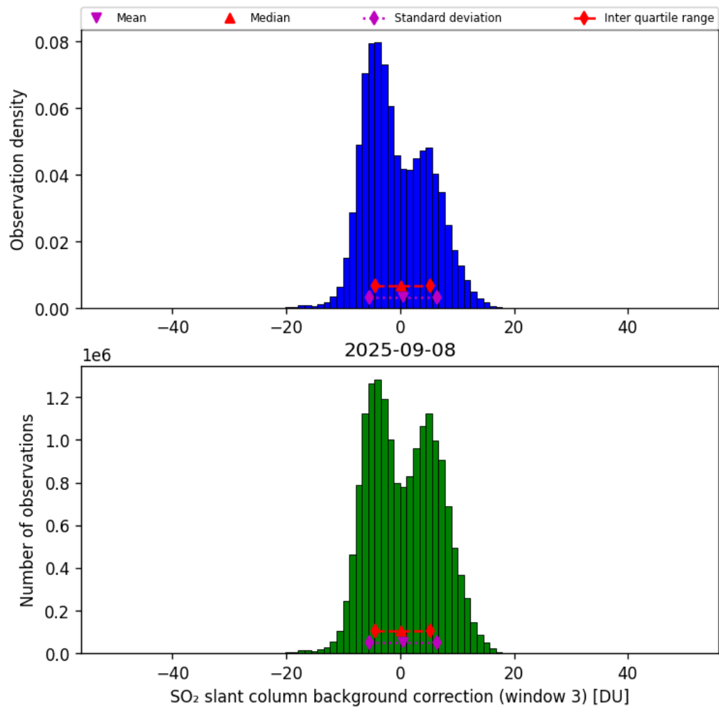
Figure 74: Histogram of “SO 2 slant column background correction (window 3)” for 2025-09-08 to 2025-09-08
