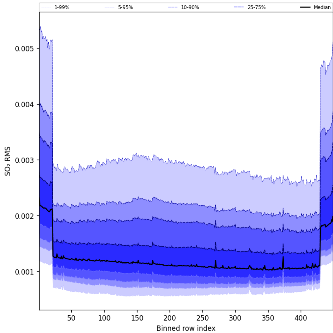
Figure 106: Along track statistics of “SO 2 RMS” for 2025-09-08 to 2025-09-08
