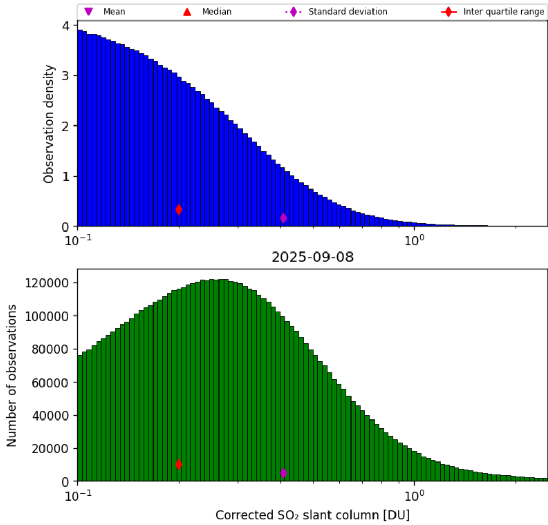
Figure 60: Histogram of “Corrected SO 2 slant column” for 2025-09-08 to 2025-09-08
