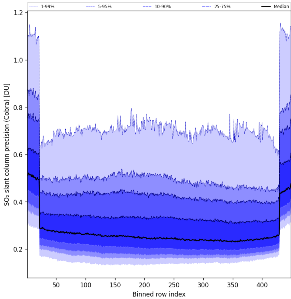
Figure 89: Along track statistics of “SO 2 slant column precision (Cobra)” for 2025-09-08 to 2025-09-08
