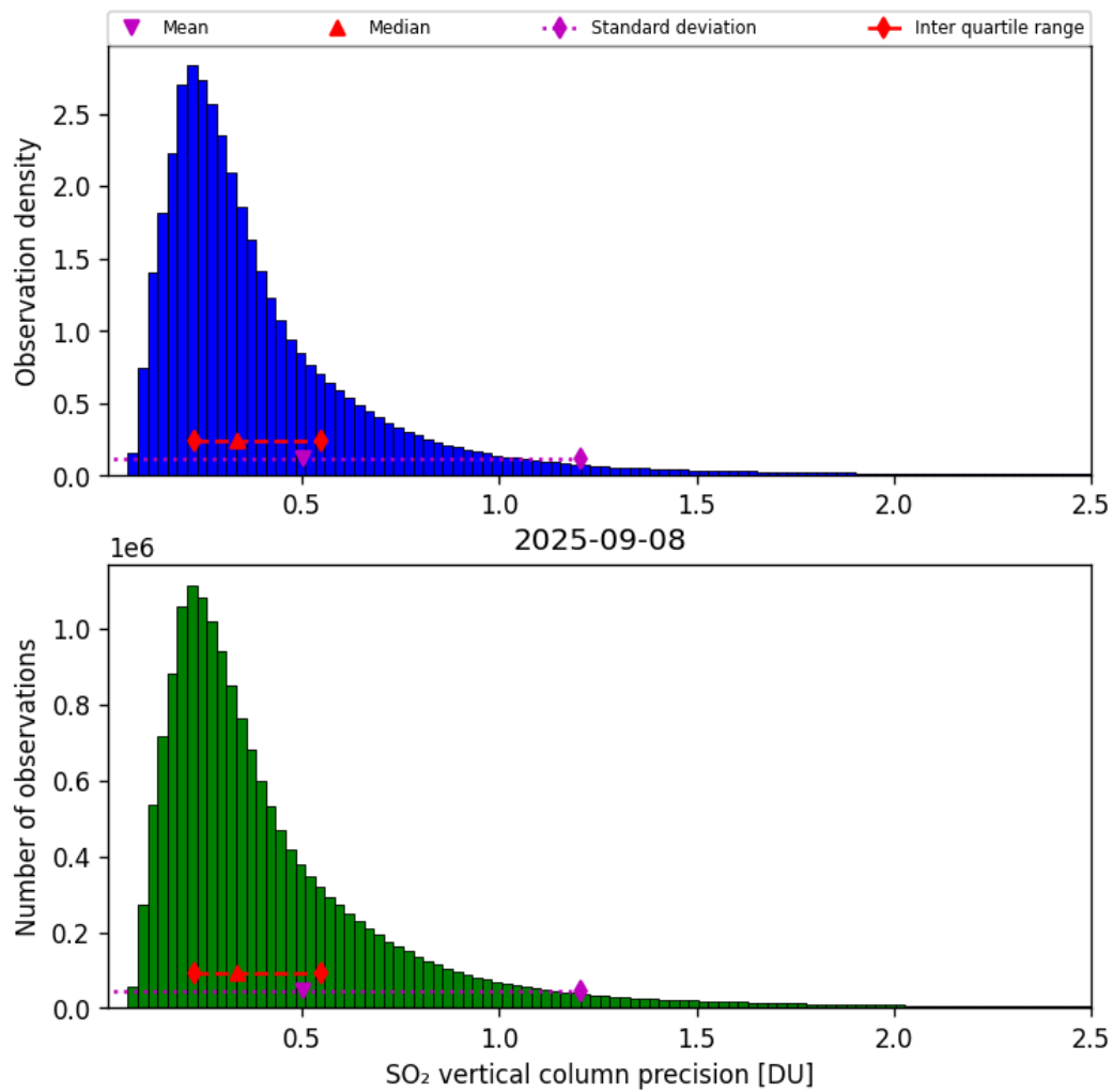
Figure 59: Histogram of “SO 2 vertical column precision” for 2025-09-08 to 2025-09-08
