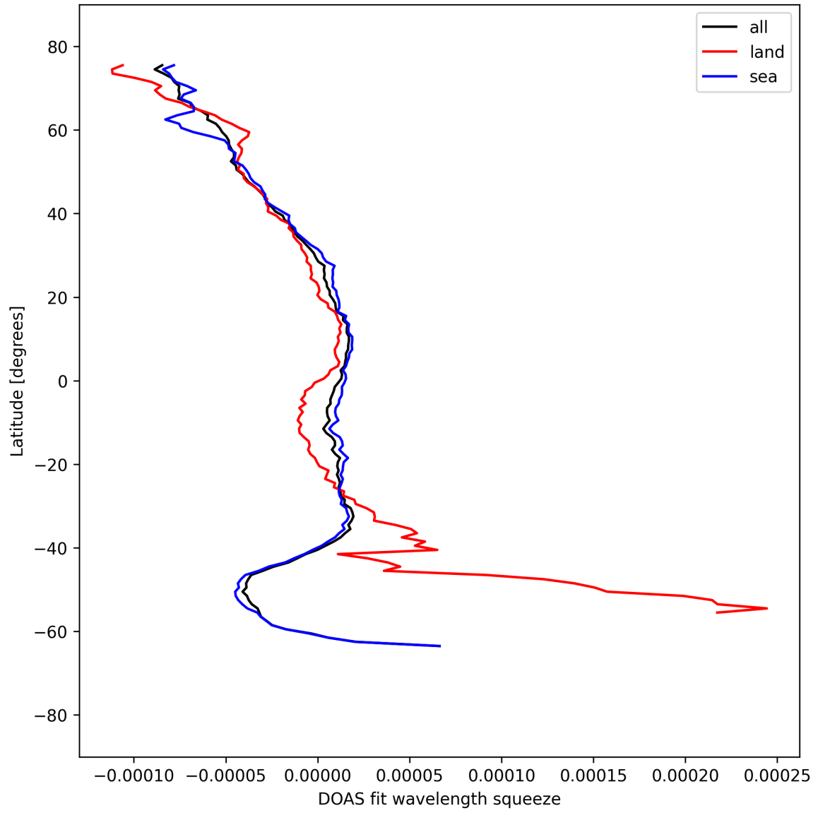
Figure 51: Zonal average of "DOAS fit wavelength squeeze" for 2025-09-08 to 2025-09-08.
