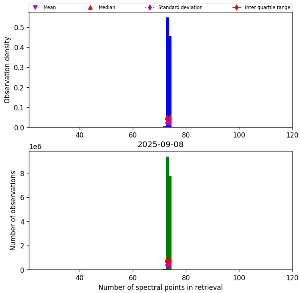
Figure 83: Histogram of “Number of spectral points in retrieval” for 2025-09-08 to 2025-09-08
