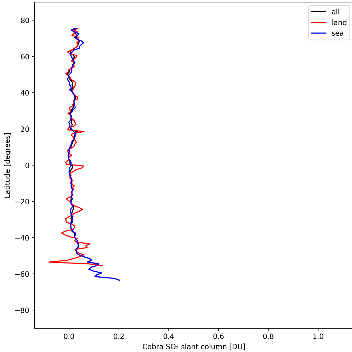
Figure 34: Zonal average of “Cobra SO 2 slant column” for 2025-09-08 to 2025-09-08.
