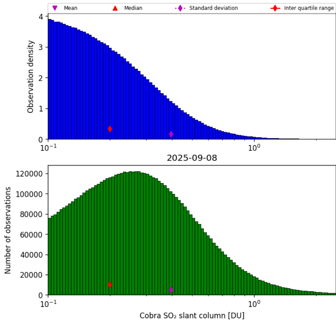
Figure 61: Histogram of “Cobra SO 2 slant column” for 2025-09-08 to 2025-09-08
