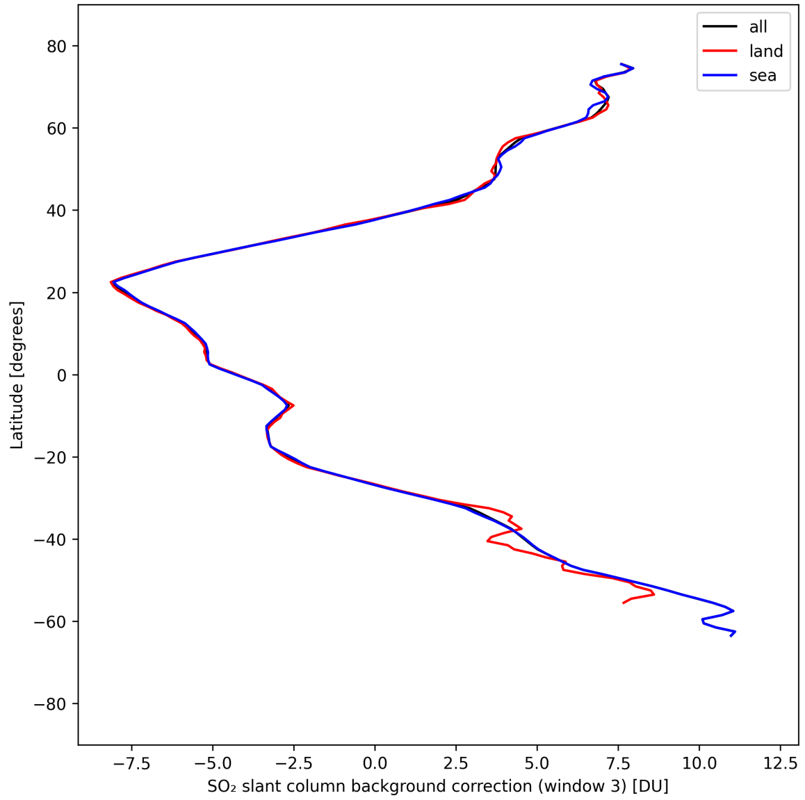
Figure 47: Zonal average of “SO 2 slant column background correction (window 3)” for 2025-09-08 to 2025-09-08.
