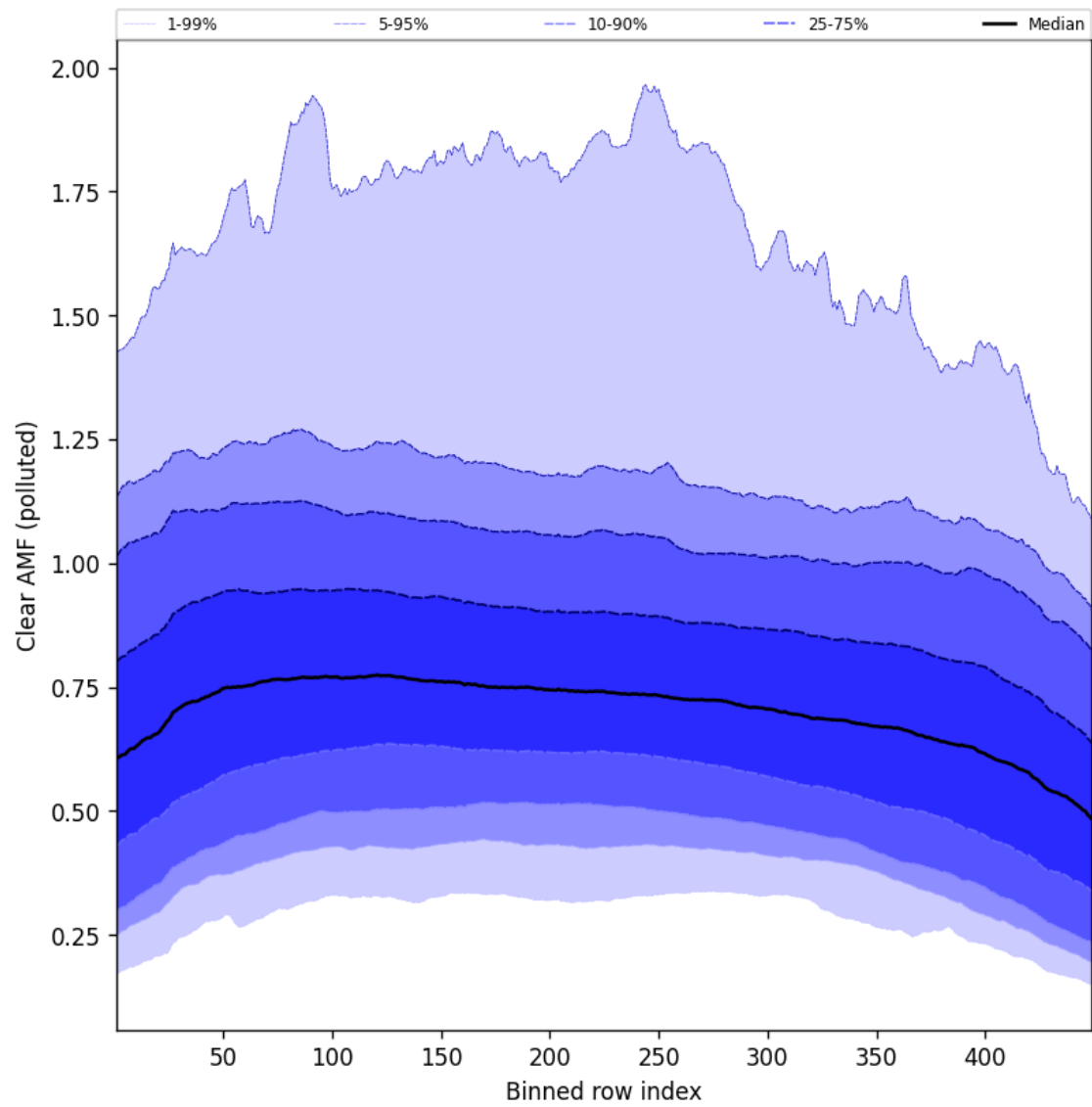
Figure 109: Along track statistics of “Clear AMF (polluted)” for 2025-09-08 to 2025-09-08
