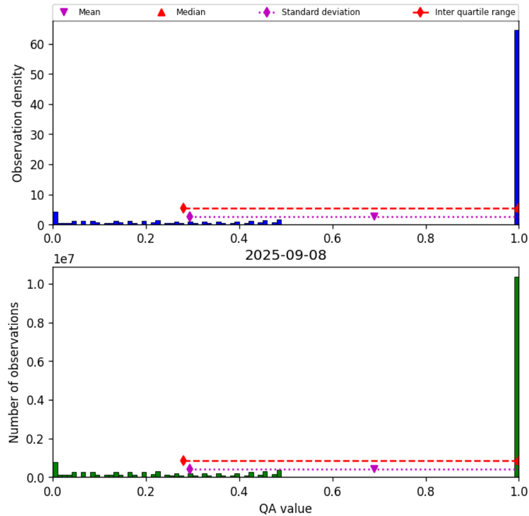
Figure 57: Histogram of “QA value” for 2025-09-08 to 2025-09-08
