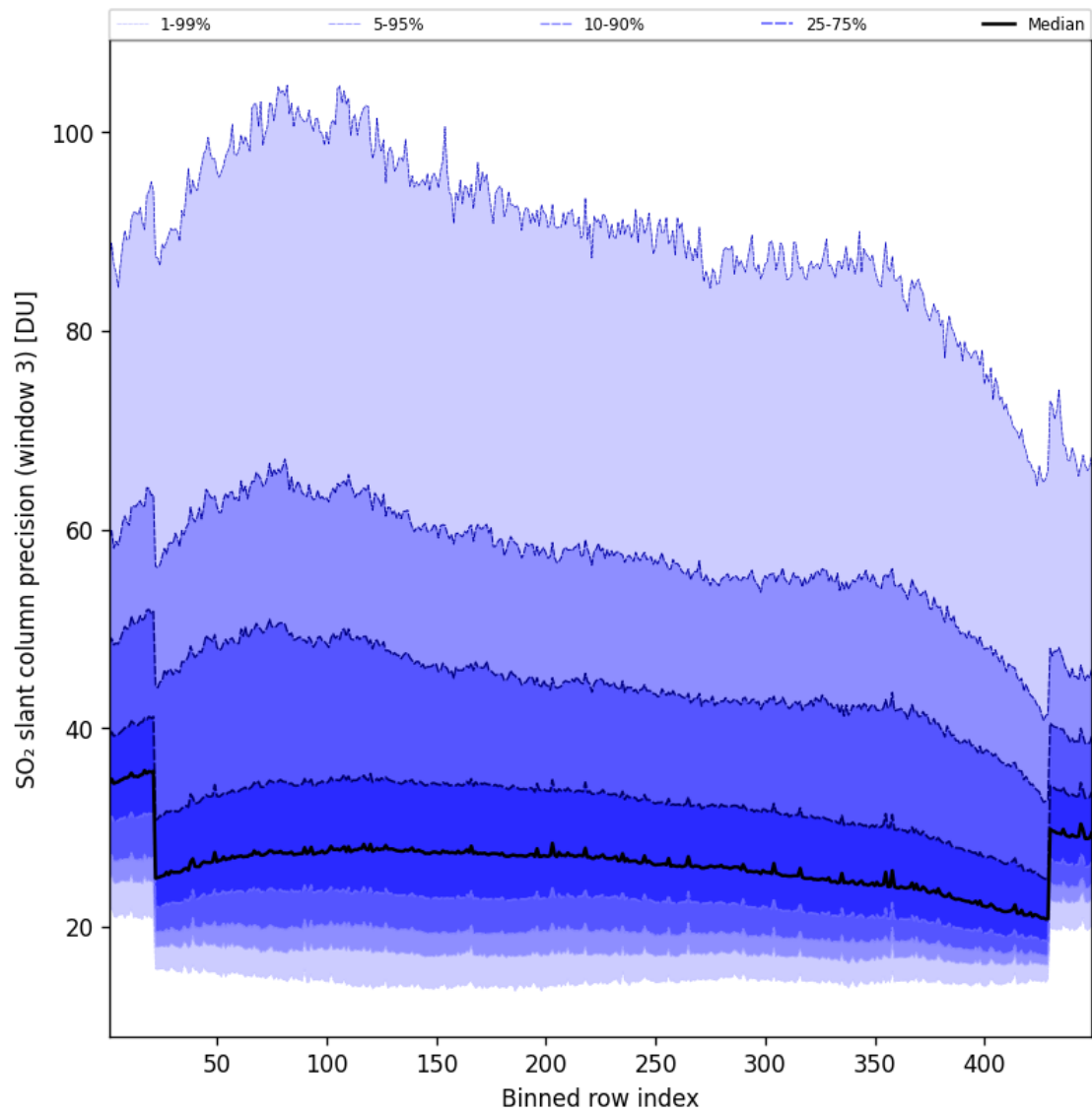
Figure 99: Along track statistics of “SO 2 slant column precision (window 3)” for 2025-09-08 to 2025-09-08
