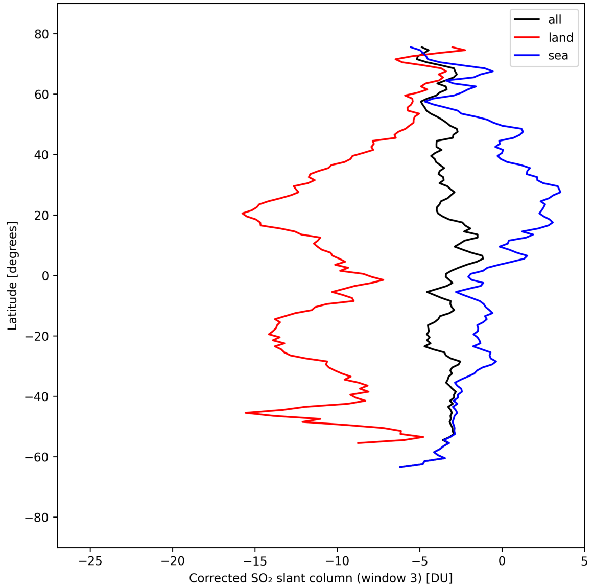
Figure 46: Zonal average of “Corrected SO 2 slant column (window 3)” for 2025-09-08 to 2025-09-08.
