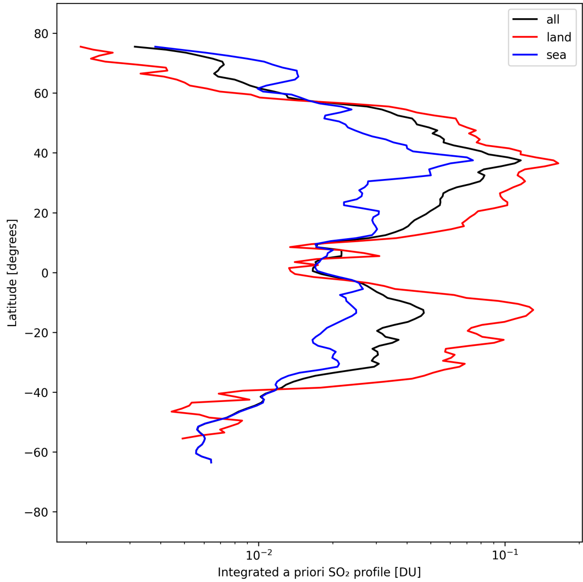
Figure 49: Zonal average of “Integrated a priori SO 2 profile” for 2025-09-08 to 2025-09-08.
