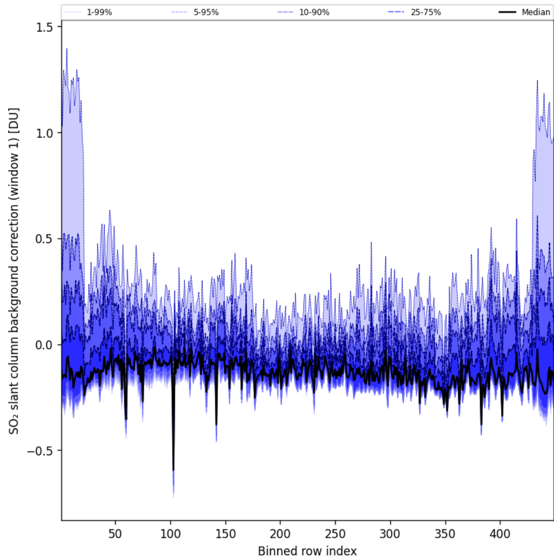
Figure 93: Along track statistics of “SO 2 slant column background correction (window 1)” for 2025-09-08 to 2025-09-08
