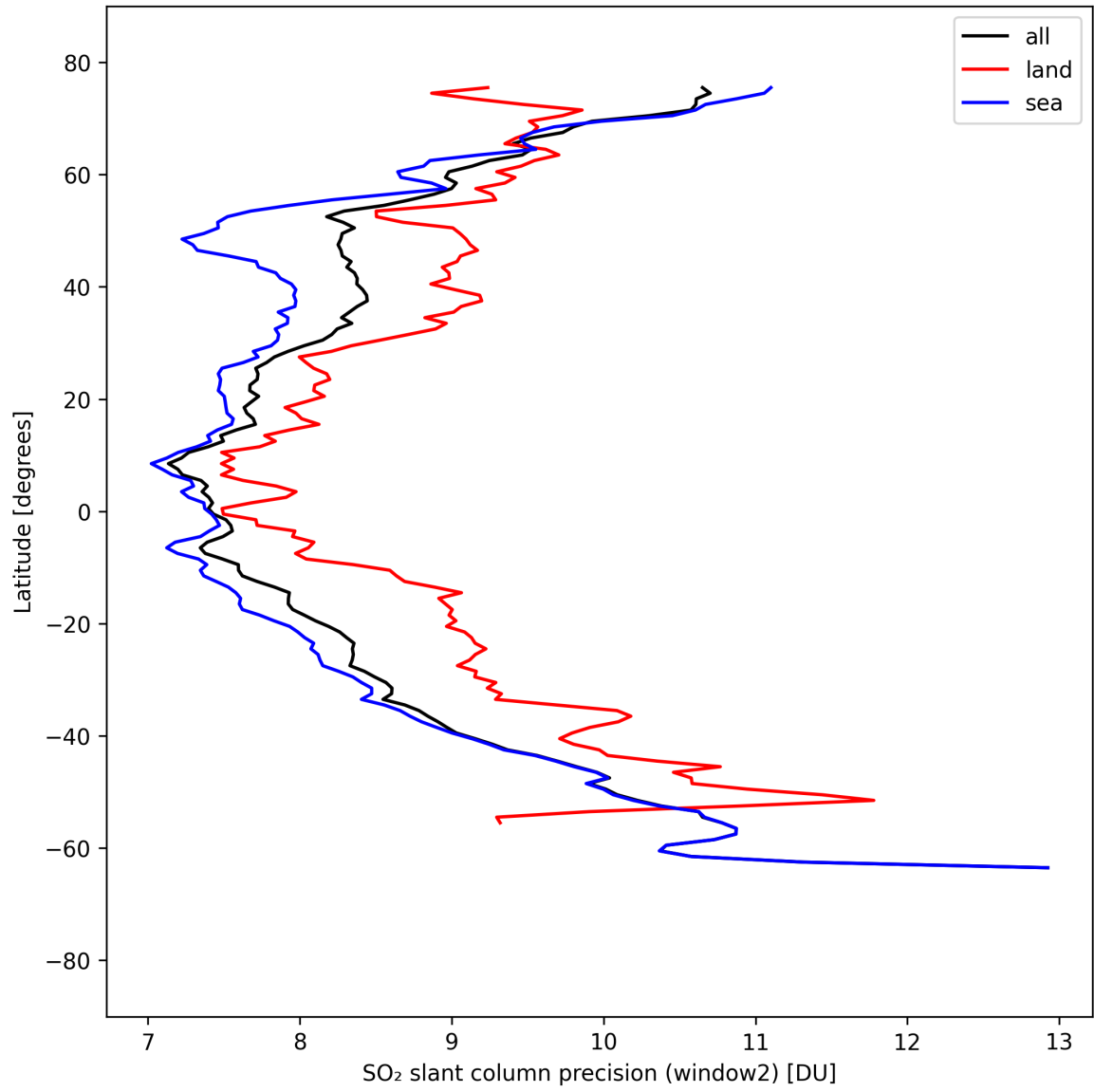
Figure 41: Zonal average of “SO 2 slant column precision (window2)” for 2025-09-08 to 2025-09-08.
