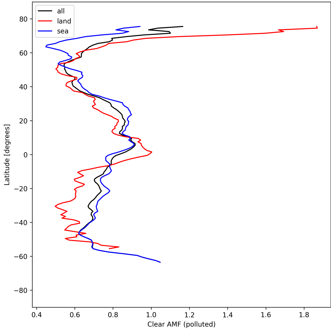
Figure 55: Zonal average of “Clear AMF (polluted)” for 2025-09-08 to 2025-09-08.
