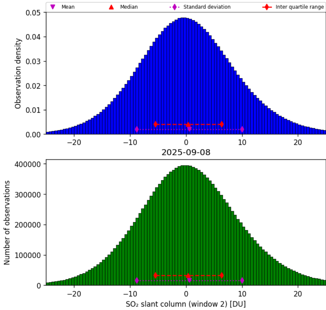
Figure 67: Histogram of “SO 2 slant column (window 2)” for 2025-09-08 to 2025-09-08
