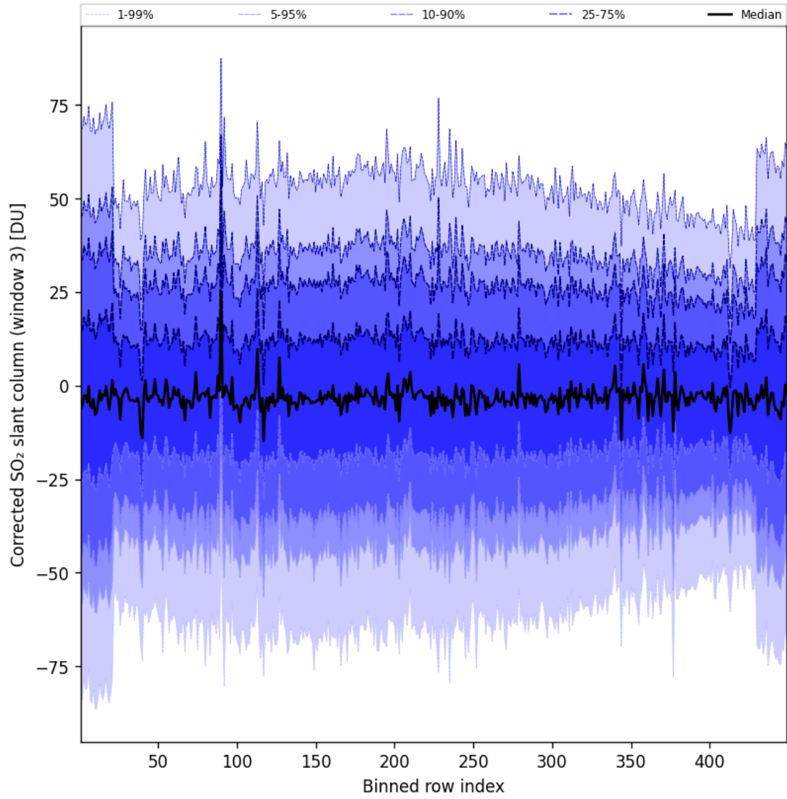
Figure 100: Along track statistics of “Corrected SO 2 slant column (window 3)” for 2025-09-08 to 2025-09-08
