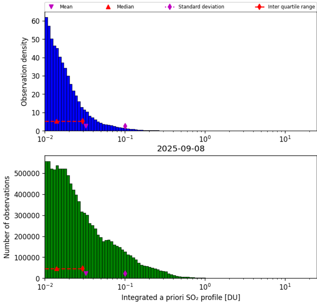
Figure 76: Histogram of “Integrated a priori SO 2 profile” for 2025-09-08 to 2025-09-08
