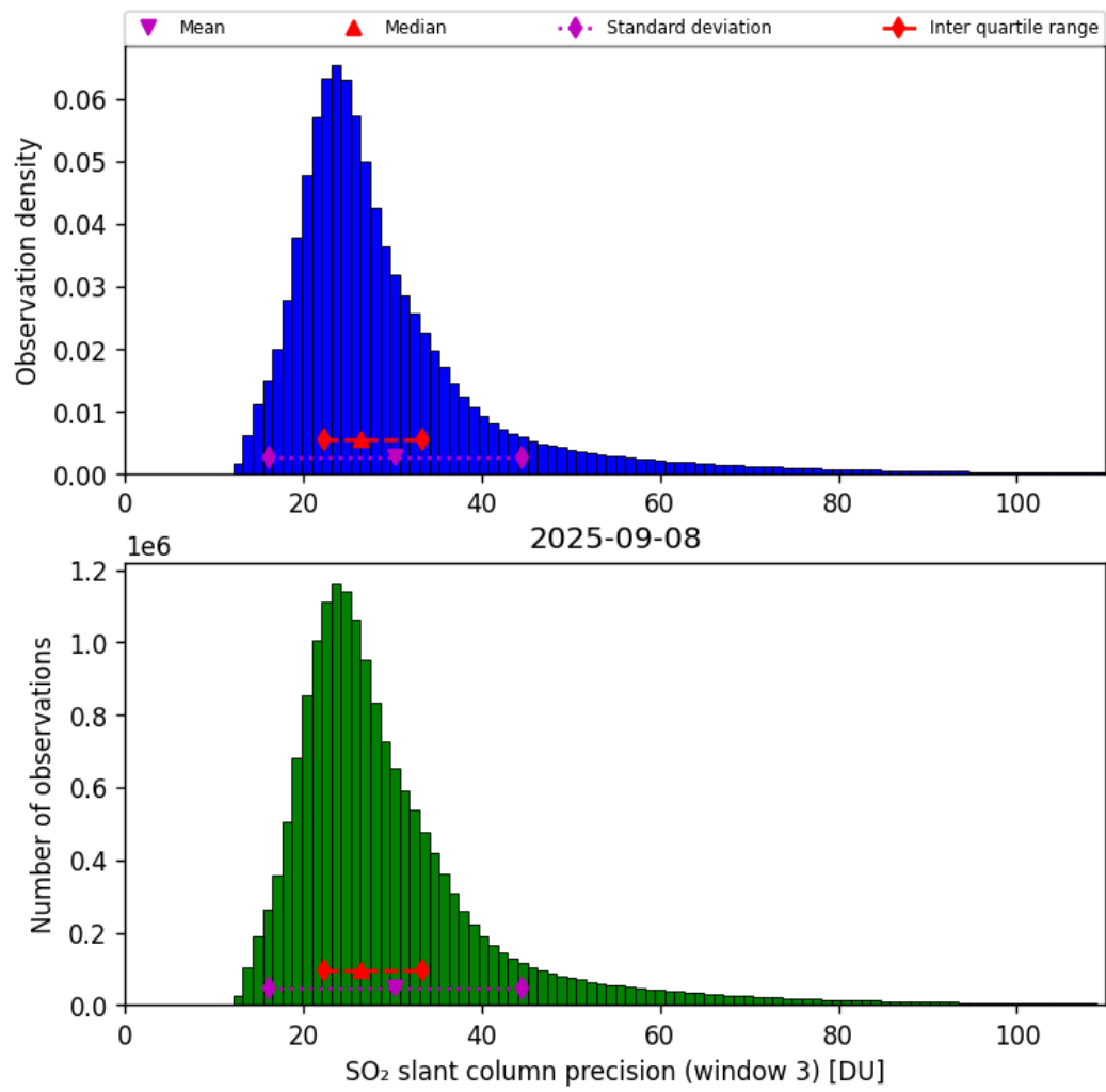
Figure 72: Histogram of “SO 2 slant column precision (window 3)” for 2025-09-08 to 2025-09-08
