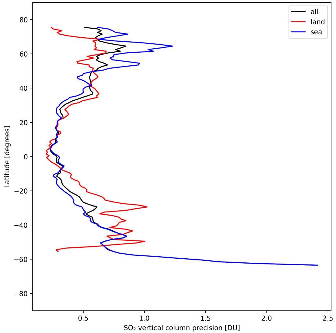
Figure 32: Zonal average of “SO 2 vertical column precision” for 2025-09-08 to 2025-09-08.
