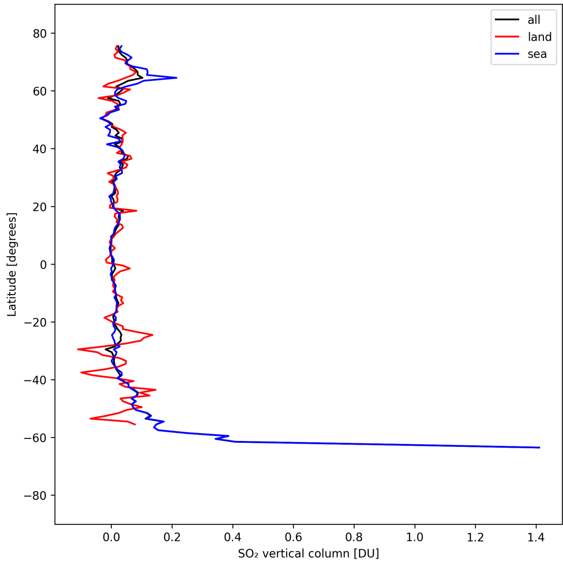
Figure 31: Zonal average of “SO 2 vertical column” for 2025-09-08 to 2025-09-08.
