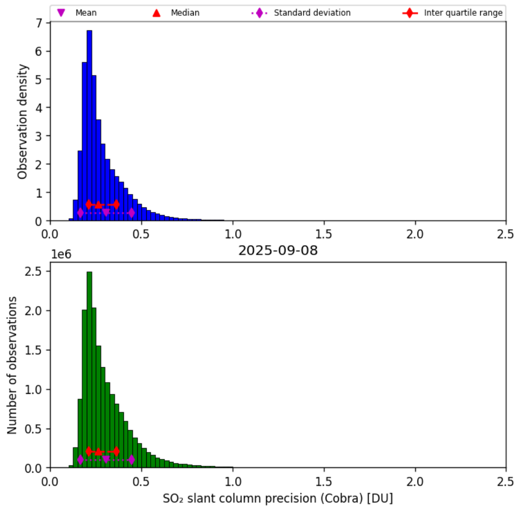
Figure 62: Histogram of “SO 2 slant column precision (Cobra)” for 2025-09-08 to 2025-09-08
