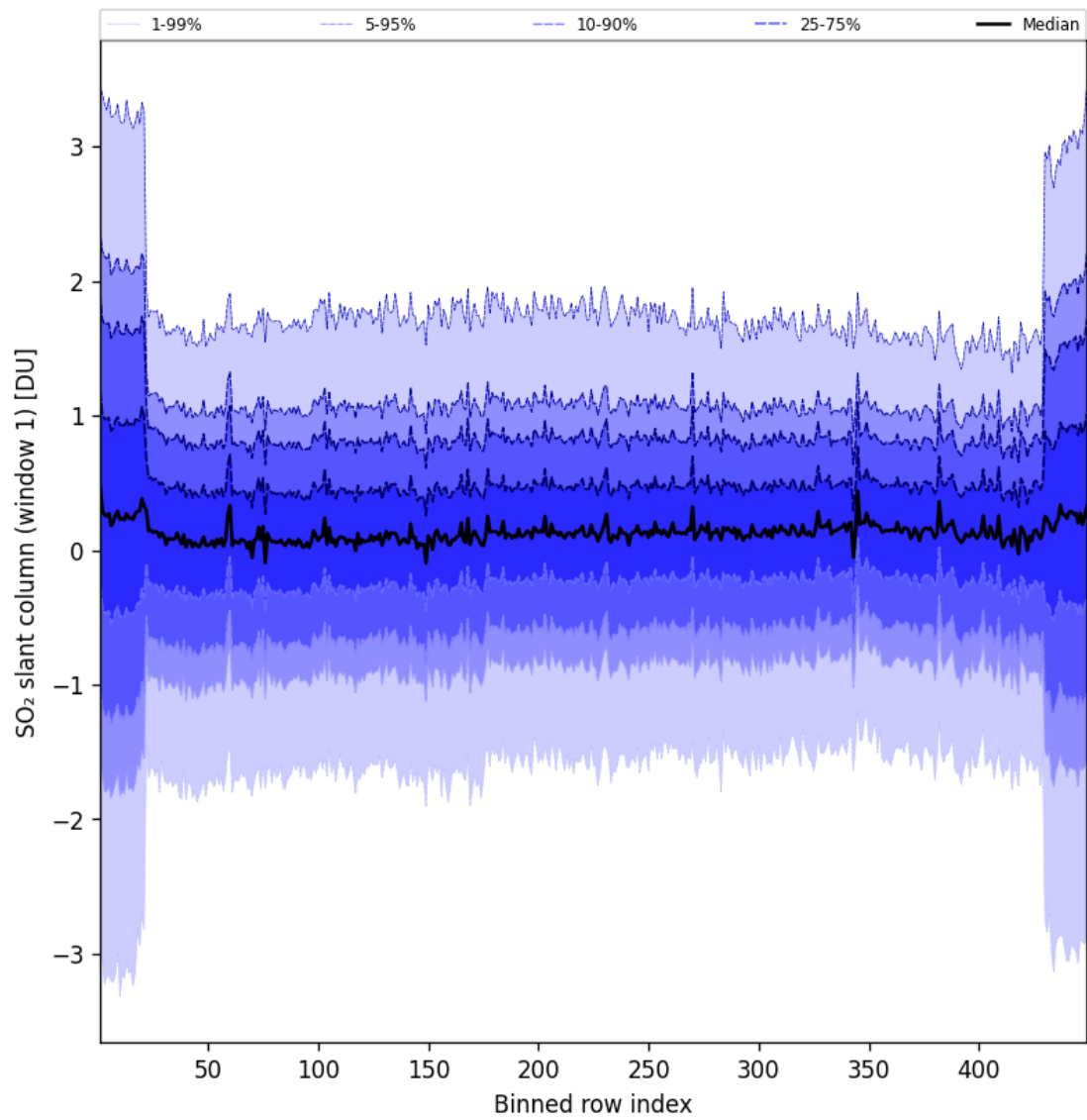
Figure 90: Along track statistics of “SO 2 slant column (window 1)” for 2025-09-08 to 2025-09-08
