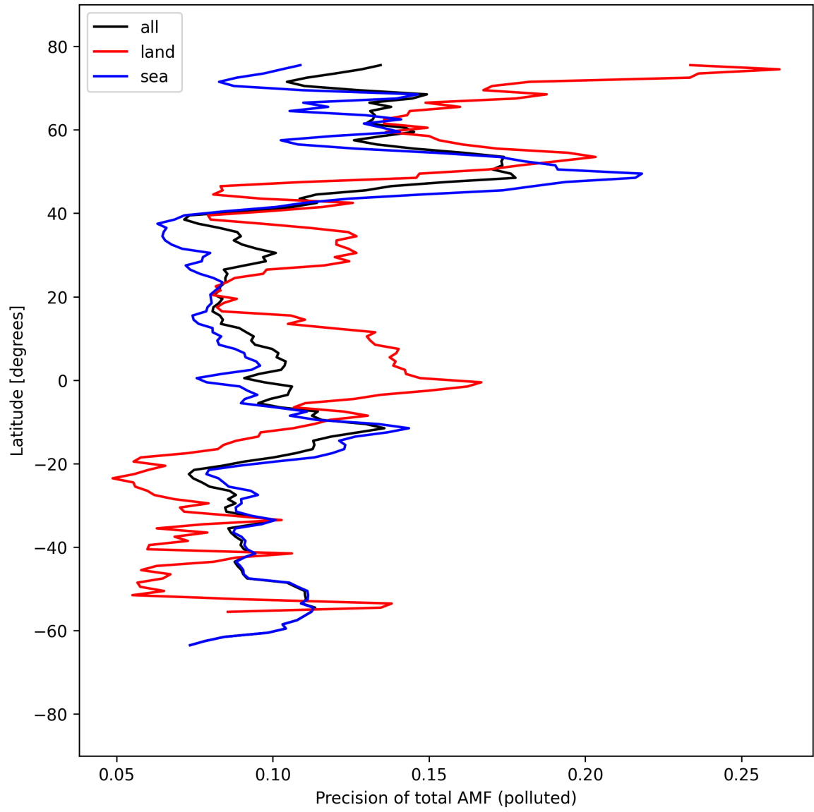
Figure 54: Zonal average of “Precision of total AMF (polluted)” for 2025-09-08 to 2025-09-08.
