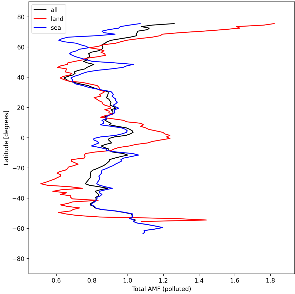
Figure 53: Zonal average of “Total AMF (polluted)” for 2025-09-08 to 2025-09-08.
