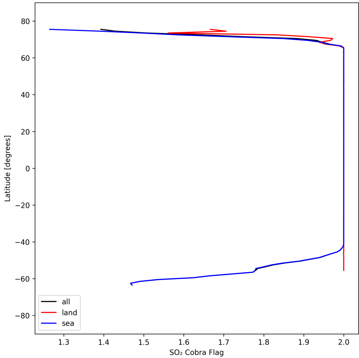
Figure 48: Zonal average of "SO 2 Cobra Flag" for 2025-09-08 to 2025-09-08.
