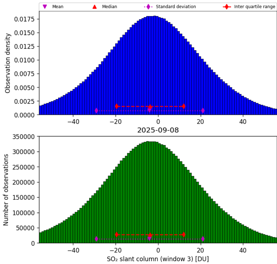
Figure 71: Histogram of “SO 2 slant column (window 3)” for 2025-09-08 to 2025-09-08
