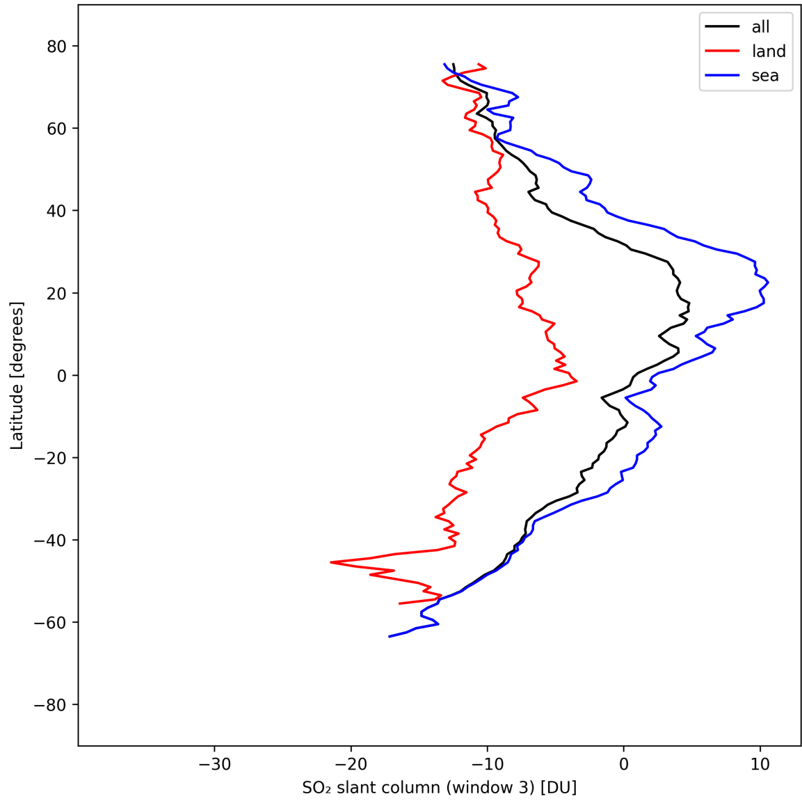
Figure 44: Zonal average of “SO 2 slant column (window 3)” for 2025-09-08 to 2025-09-08.
