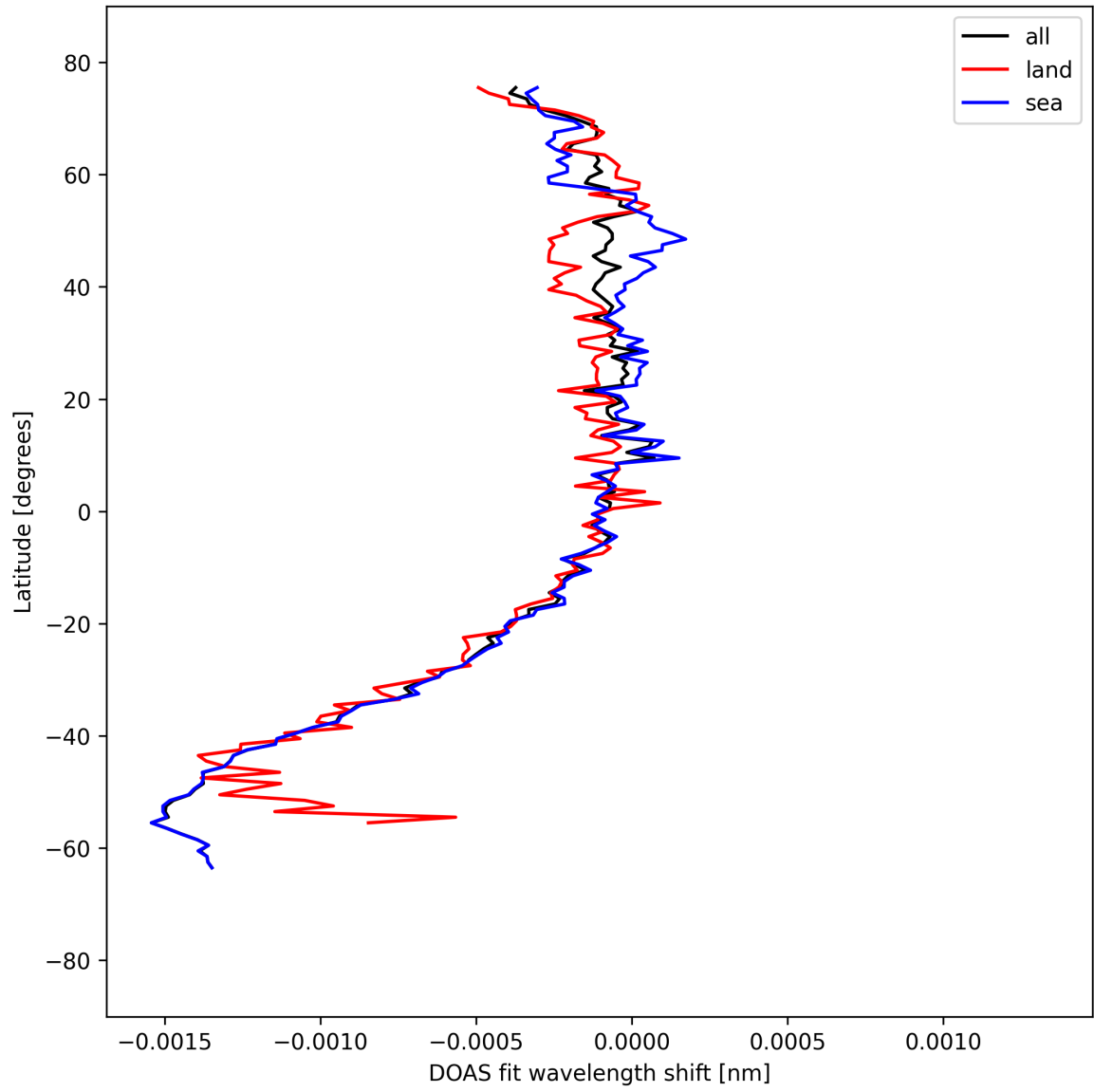
Figure 50: Zonal average of “DOAS fit wavelength shift” for 2025-09-08 to 2025-09-08.
