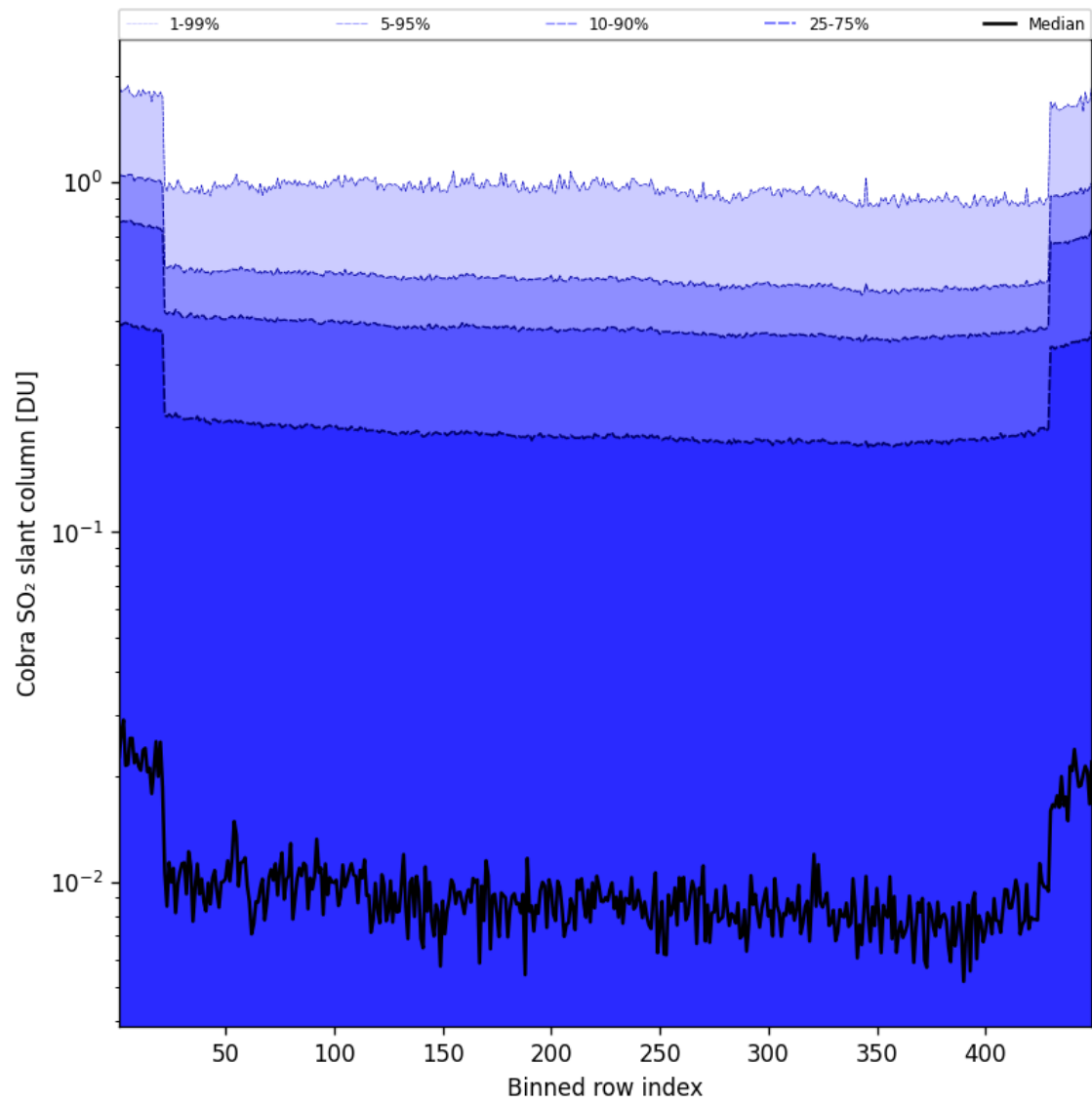
Figure 88: Along track statistics of “Cobra SO 2 slant column” for 2025-09-08 to 2025-09-08
