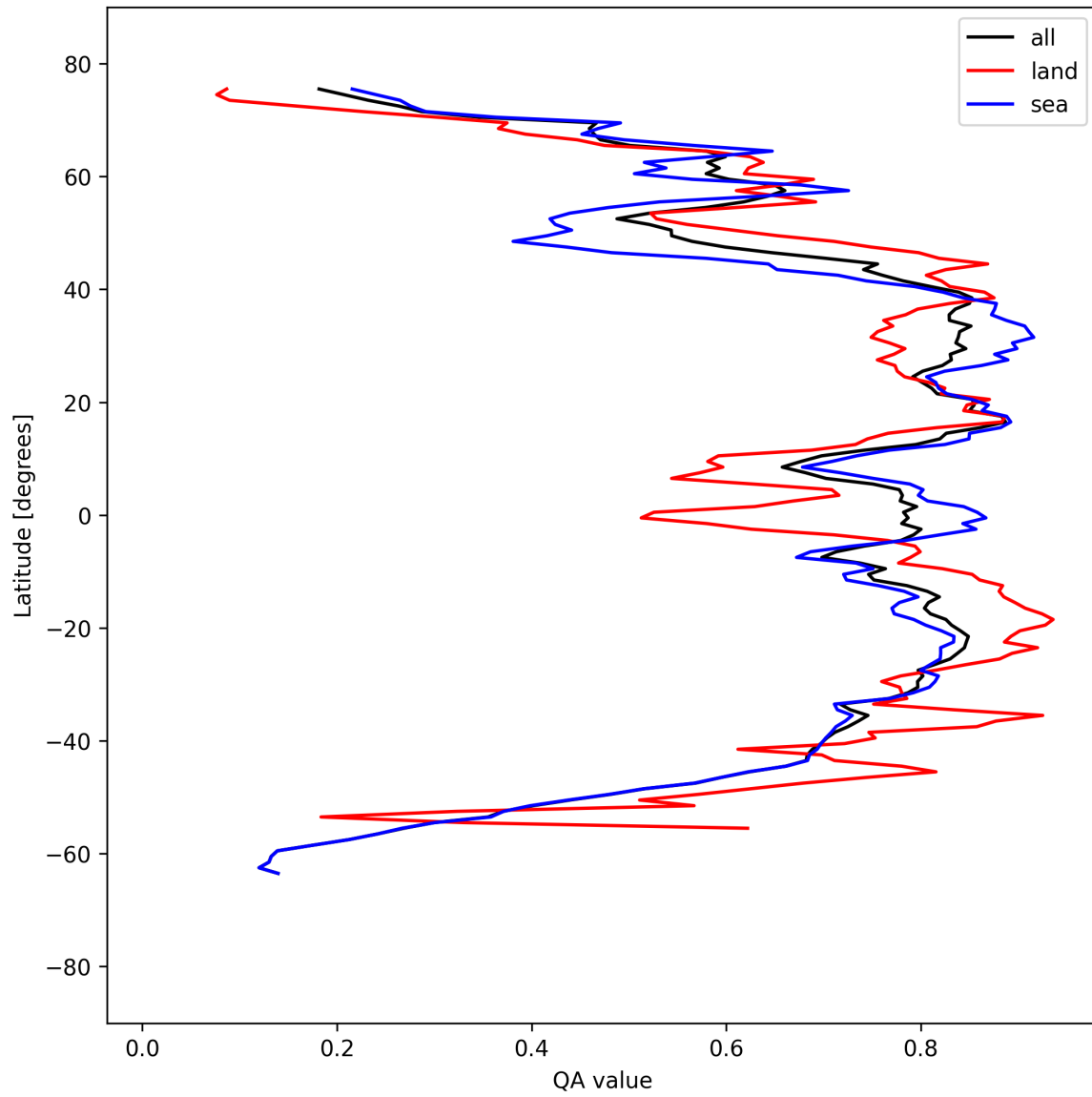
Figure 30: Zonal average of “QA value” for 2025-09-08 to 2025-09-08.
