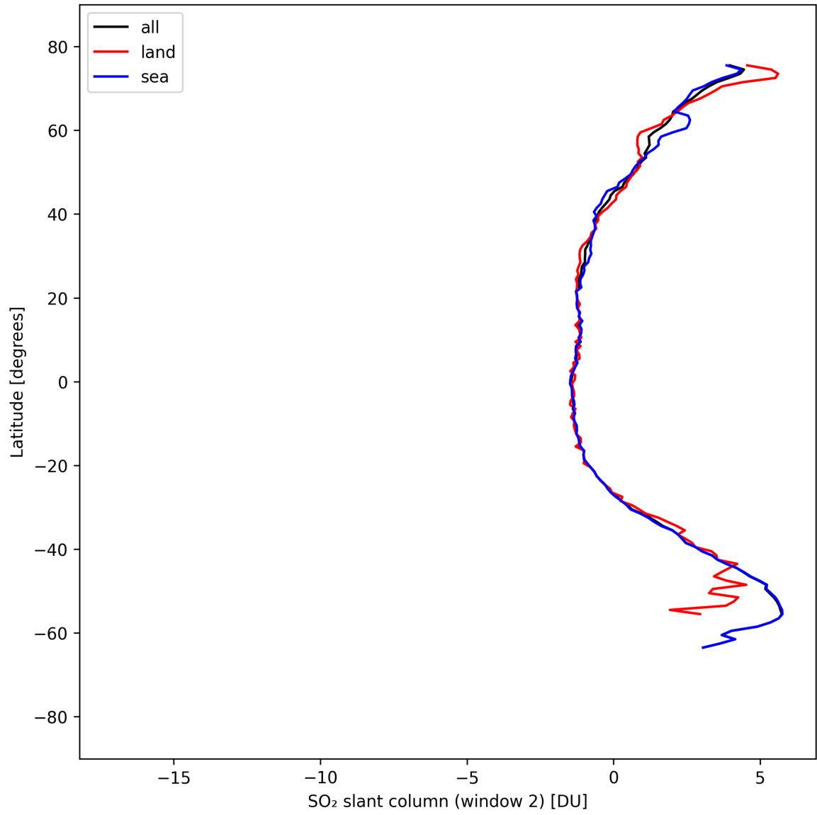
Figure 40: Zonal average of “SO 2 slant column (window 2)” for 2025-09-08 to 2025-09-08.
