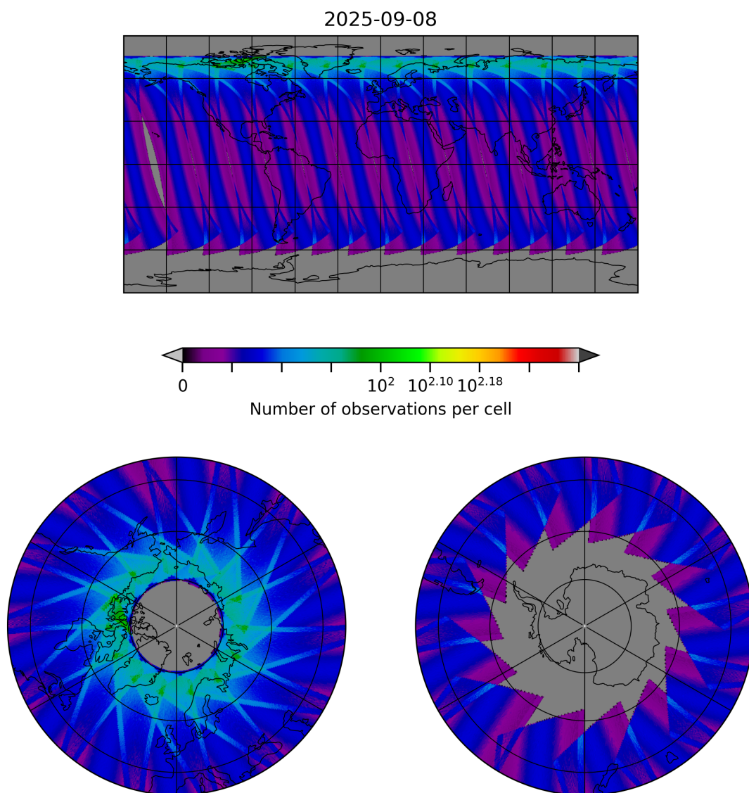
Figure 29: Map of the number of observations for 2025-09-08 to 2025-09-08
