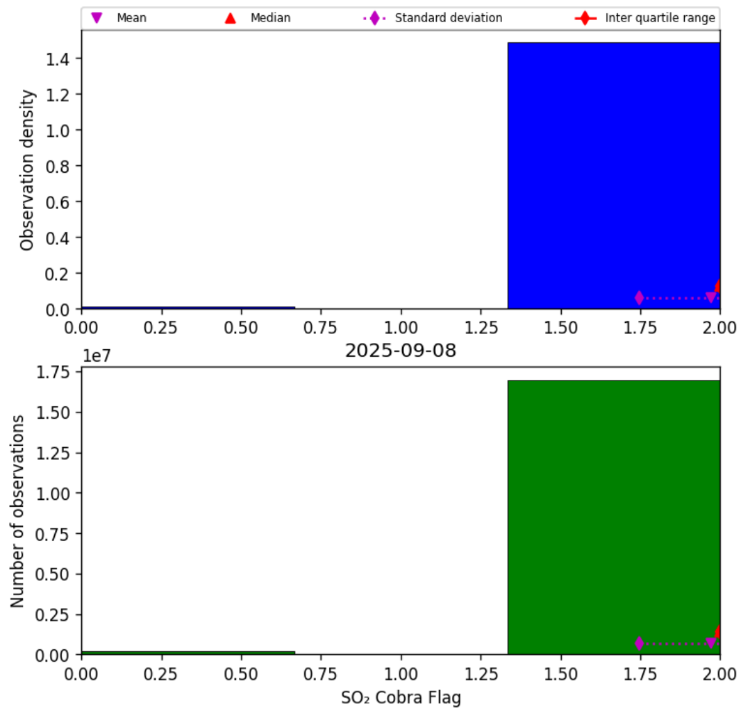
Figure 75: Histogram of “SO 2 Cobra Flag” for 2025-09-08 to 2025-09-08
