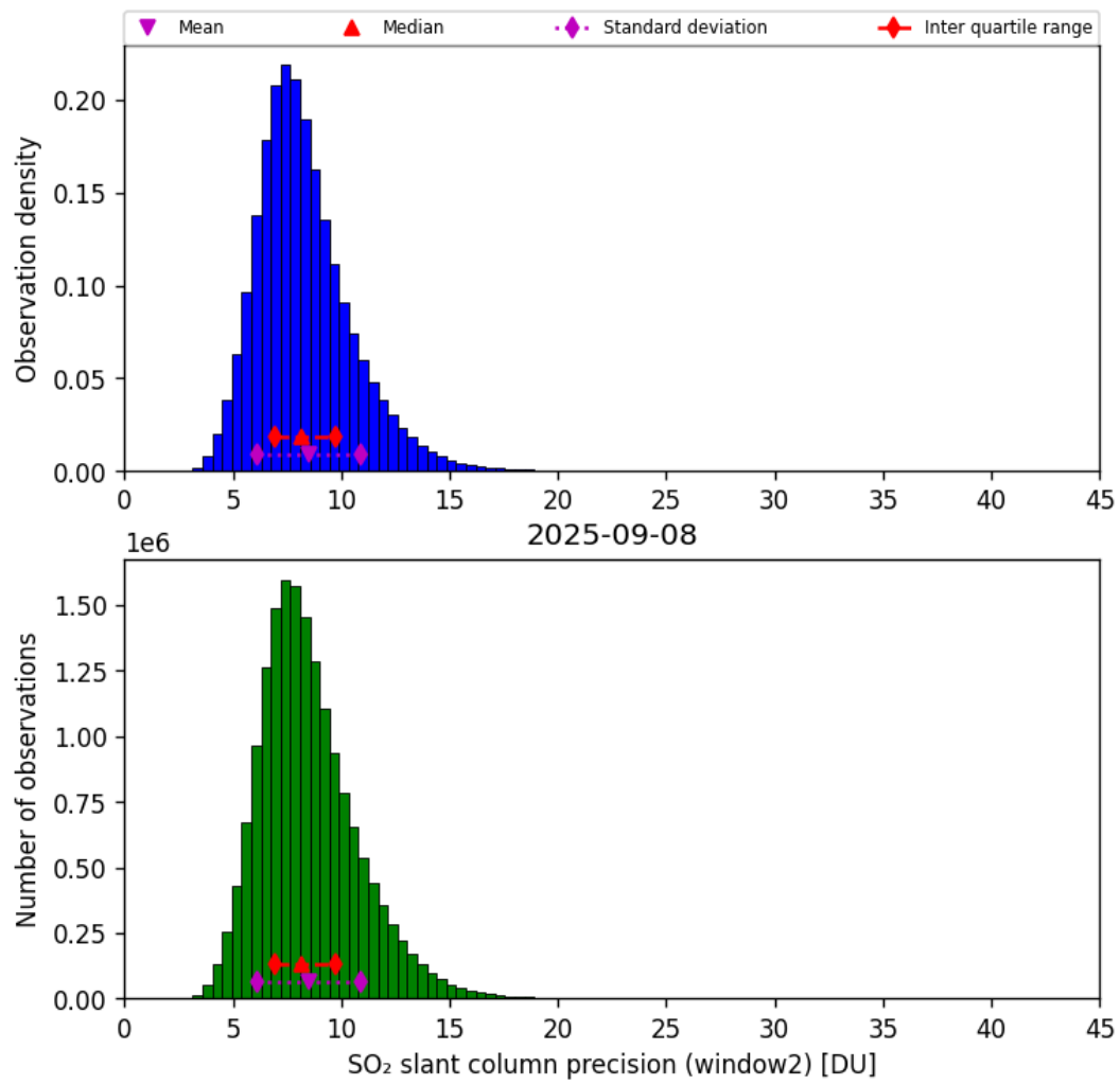
Figure 68: Histogram of “SO 2 slant column precision (window2)” for 2025-09-08 to 2025-09-08
