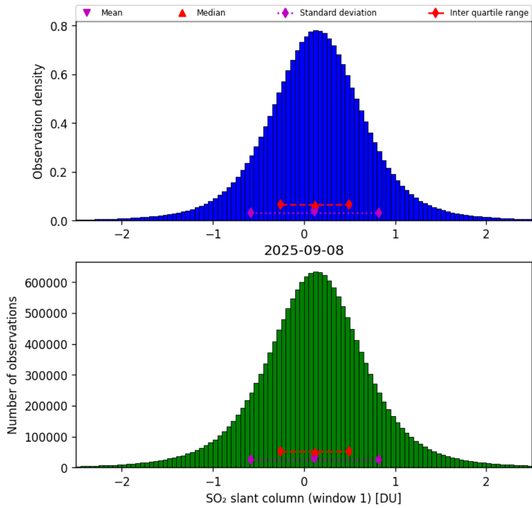
Figure 63: Histogram of “SO 2 slant column (window 1)” for 2025-09-08 to 2025-09-08
