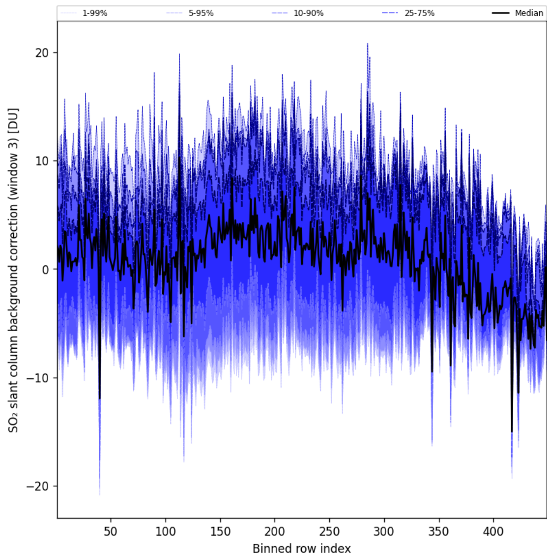
Figure 101: Along track statistics of “SO 2 slant column background correction (window 3)” for 2025-09-08 to 2025-09-08
