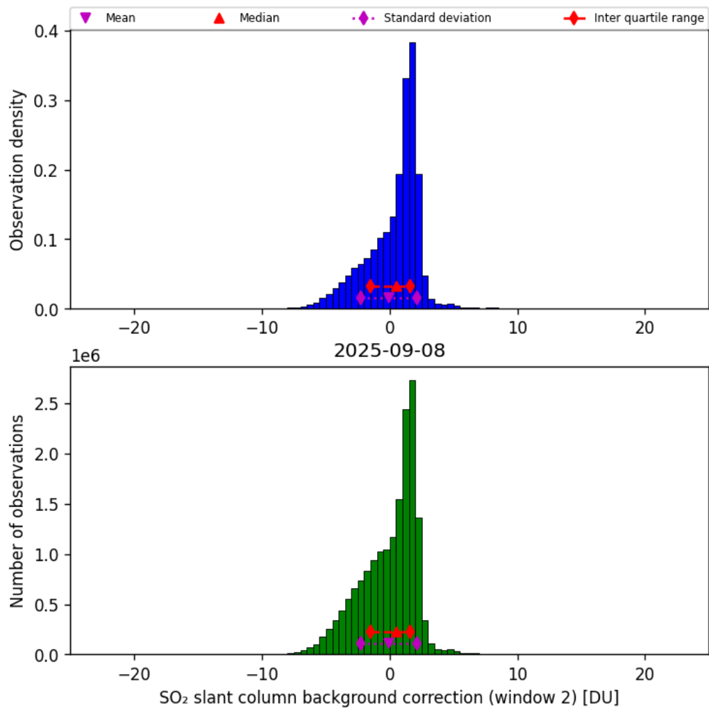
Figure 70: Histogram of “SO 2 slant column background correction (window 2)” for 2025-09-08 to 2025-09-08
