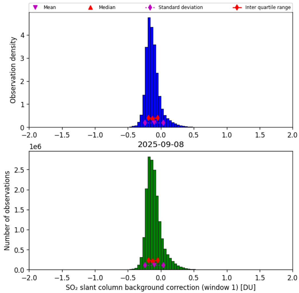
Figure 66: Histogram of “SO 2 slant column background correction (window 1)” for 2025-09-08 to 2025-09-08
