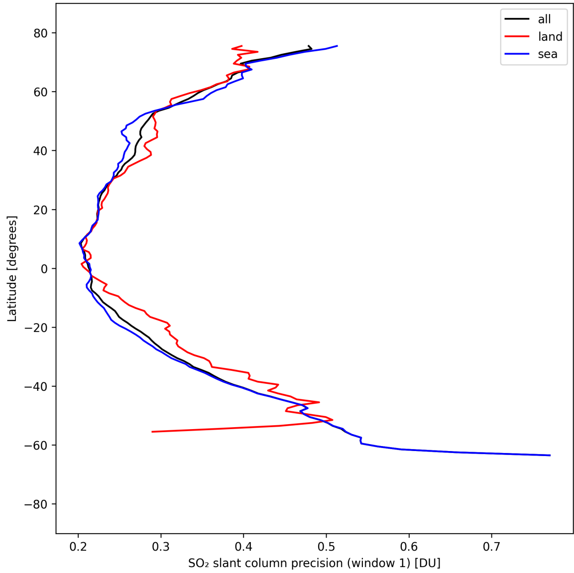
Figure 37: Zonal average of “SO 2 slant column precision (window 1)” for 2025-09-08 to 2025-09-08.
