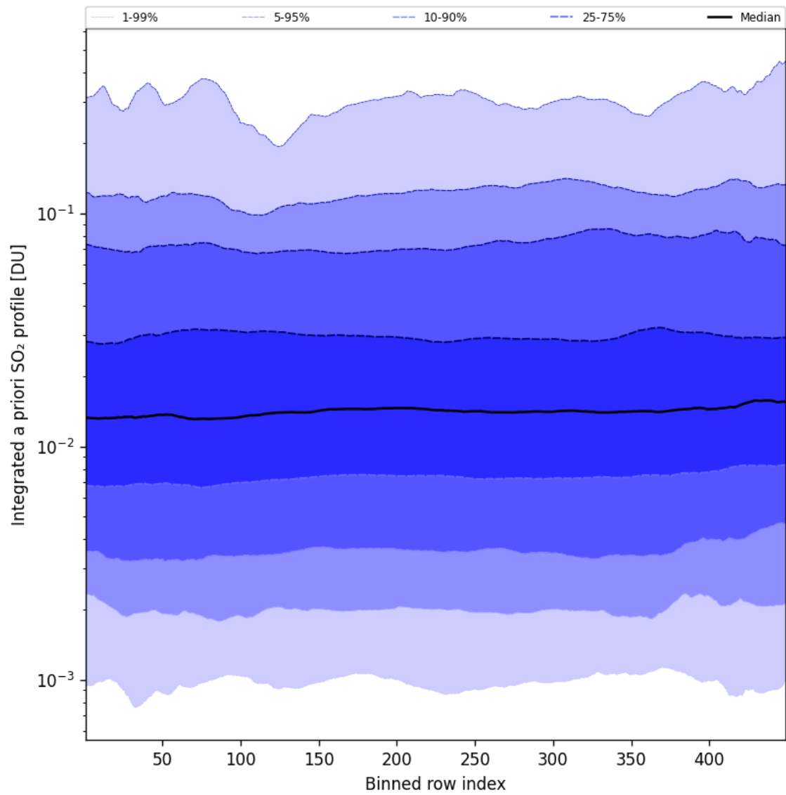
Figure 103: Along track statistics of “Integrated a priori SO 2 profile” for 2025-09-08 to 2025-09-08
