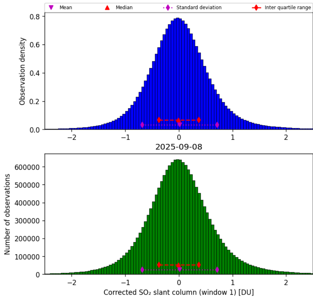
Figure 65: Histogram of “Corrected SO 2 slant column (window 1)” for 2025-09-08 to 2025-09-08
