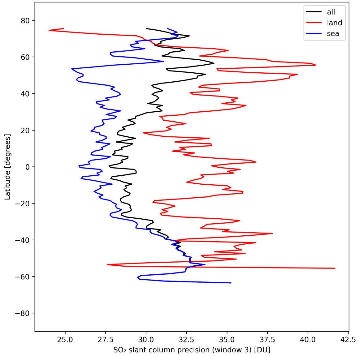
Figure 45: Zonal average of “SO 2 slant column precision (window 3)” for 2025-09-08 to 2025-09-08.
