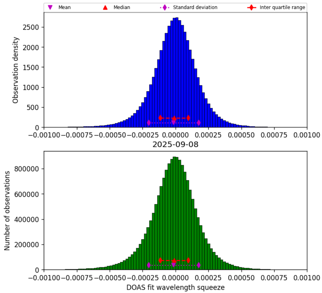
Figure 78: Histogram of “DOAS fit wavelength squeeze” for 2025-09-08 to 2025-09-08
