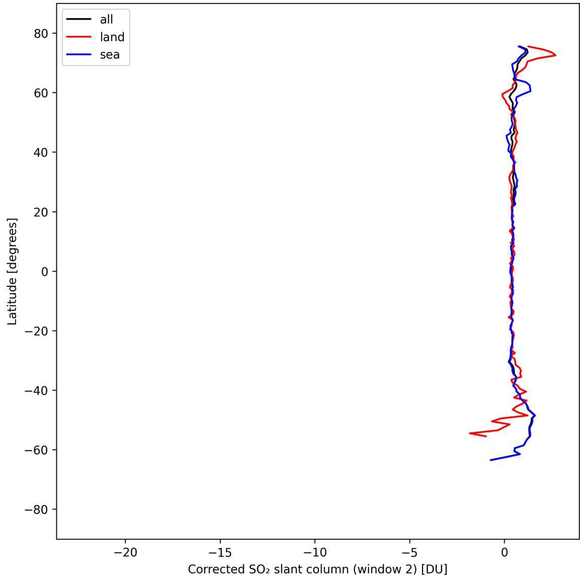
Figure 42: Zonal average of “Corrected SO 2 slant column (window 2)” for 2025-09-08 to 2025-09-08.
