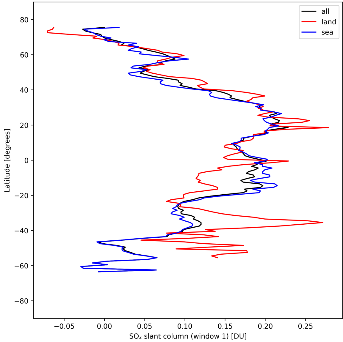
Figure 36: Zonal average of “SO 2 slant column (window 1)” for 2025-09-08 to 2025-09-08.
