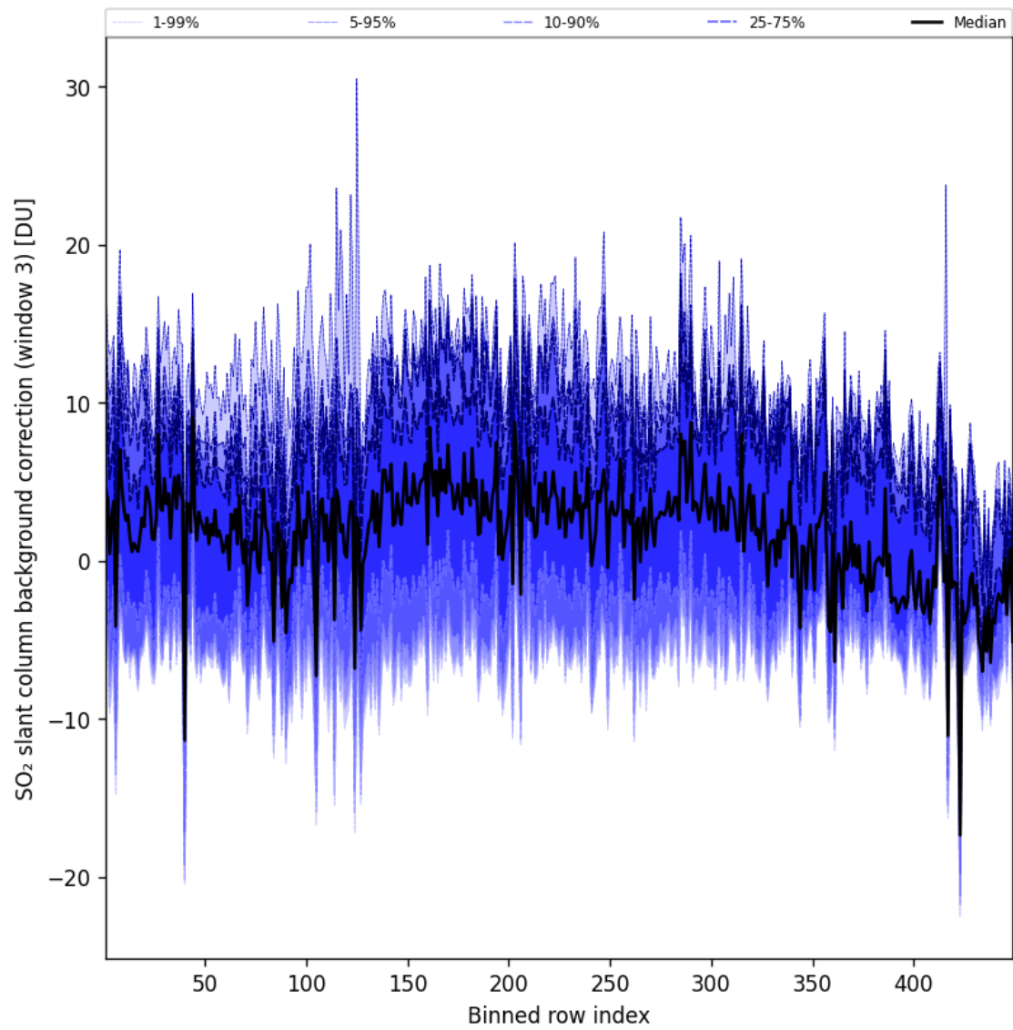
Figure 101: Along track statistics of “SO 2 slant column background correction (window 3)” for 2025-09-10 to 2025-09-11
