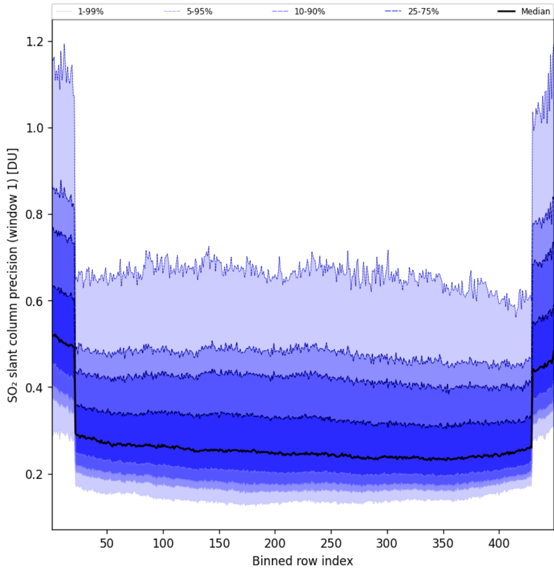
Figure 91: Along track statistics of “SO 2 slant column precision (window 1)” for 2025-09-10 to 2025-09-11
