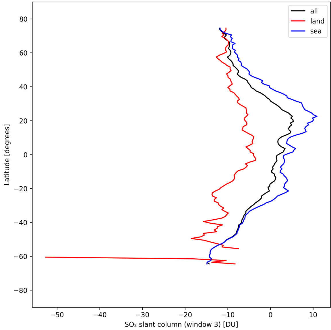
Figure 44: Zonal average of “SO 2 slant column (window 3)” for 2025-09-10 to 2025-09-11.
