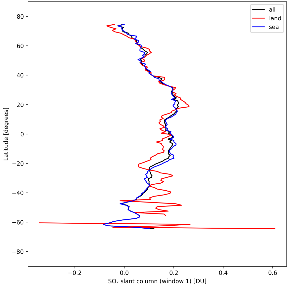
Figure 36: Zonal average of “SO 2 slant column (window 1)” for 2025-09-10 to 2025-09-11.
