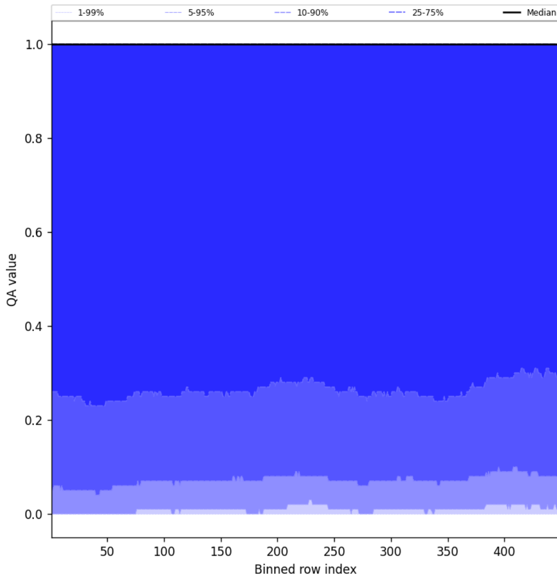
Figure 84: Along track statistics of “QA value” for 2025-09-10 to 2025-09-11
