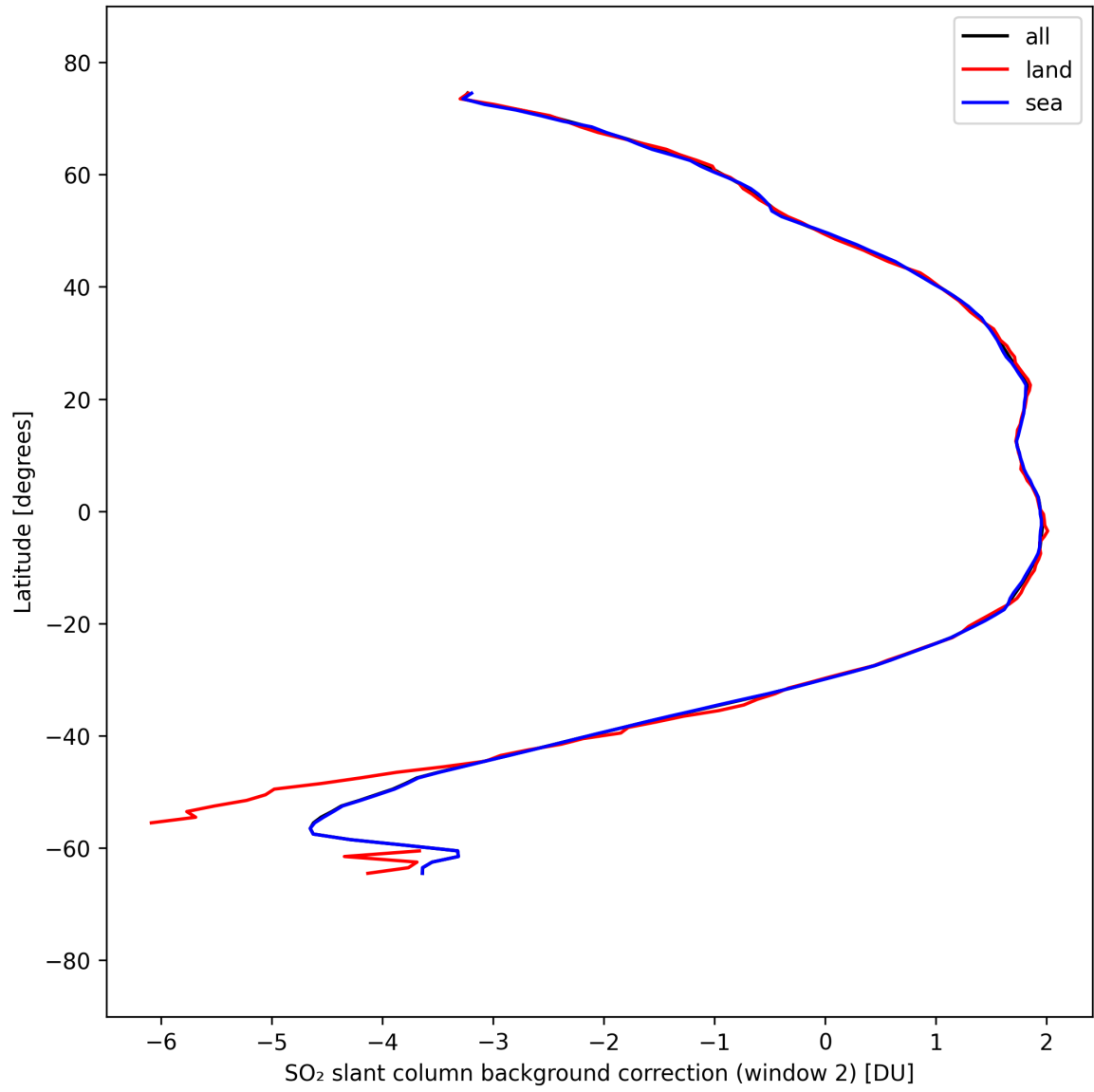
Figure 43: Zonal average of “SO 2 slant column background correction (window 2)” for 2025-09-10 to 2025-09-11.
