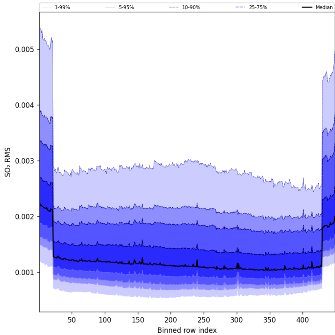
Figure 106: Along track statistics of “SO 2 RMS” for 2025-09-10 to 2025-09-11
