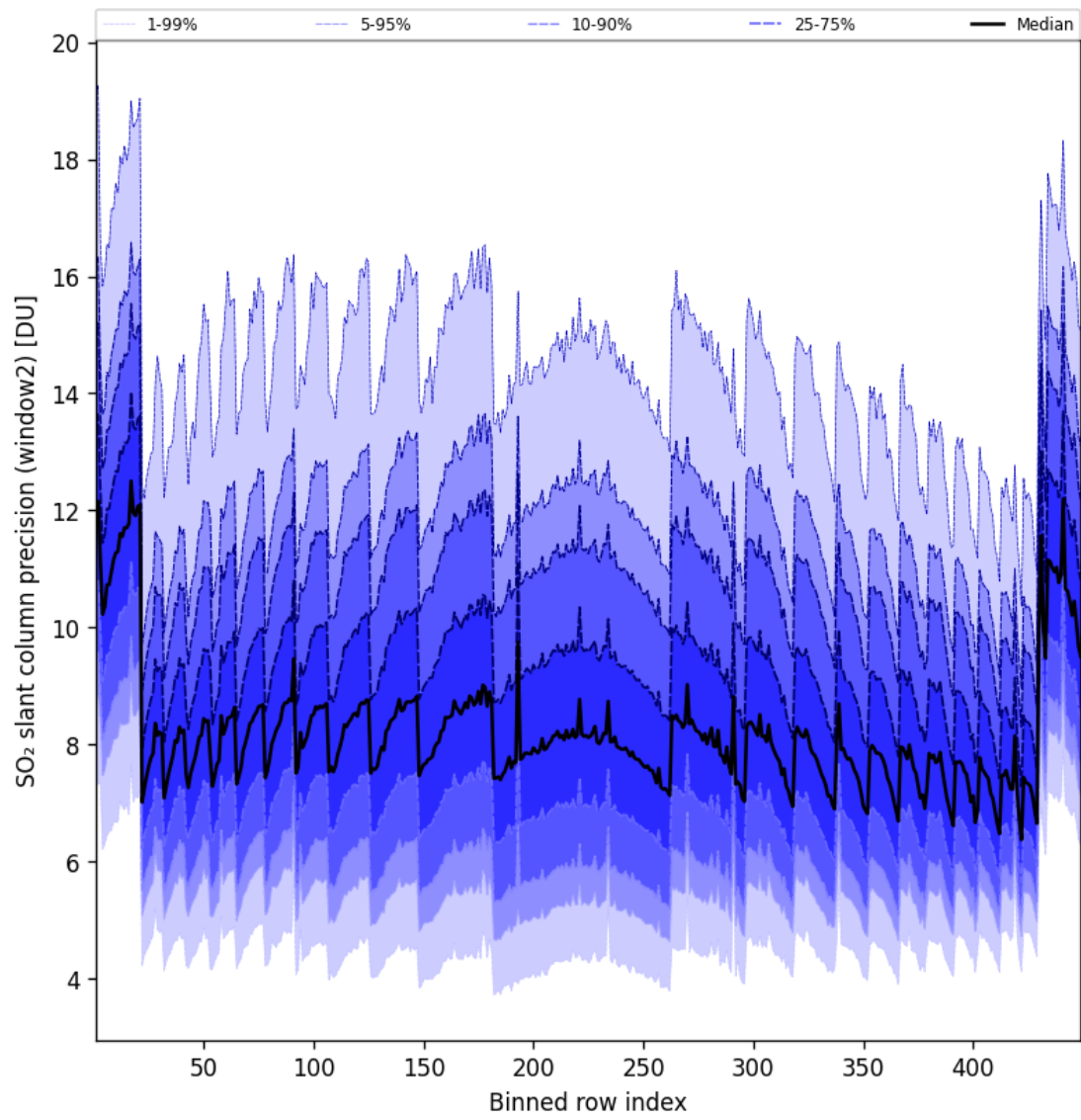
Figure 95: Along track statistics of “SO 2 slant column precision (window2)” for 2025-09-10 to 2025-09-11
