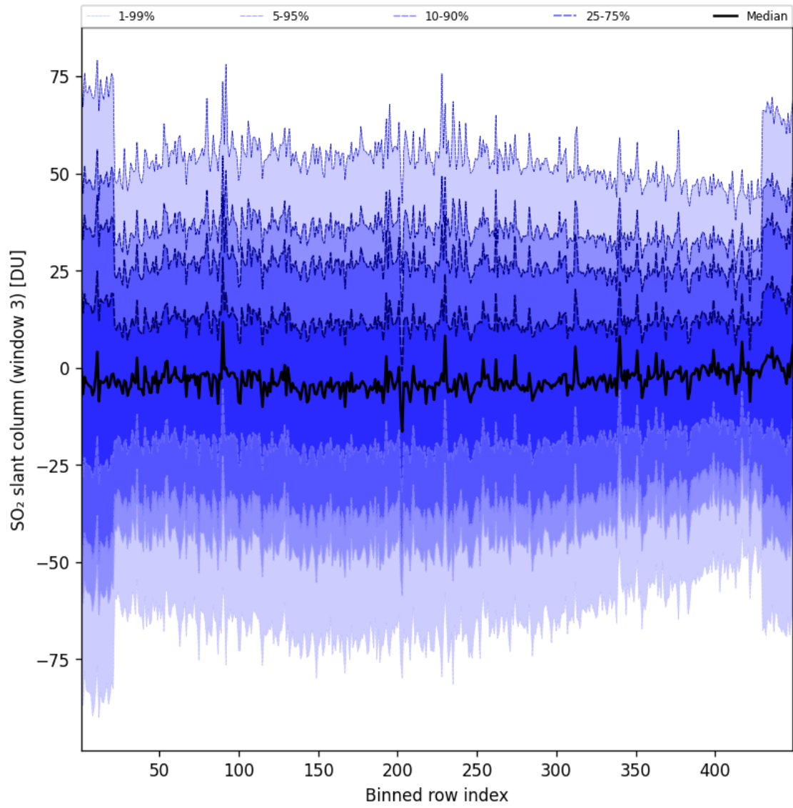
Figure 98: Along track statistics of “SO 2 slant column (window 3)” for 2025-09-10 to 2025-09-11
