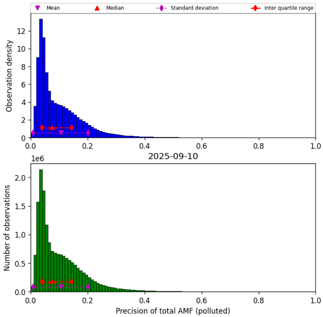
Figure 81: Histogram of “Precision of total AMF (polluted)” for 2025-09-10 to 2025-09-11
