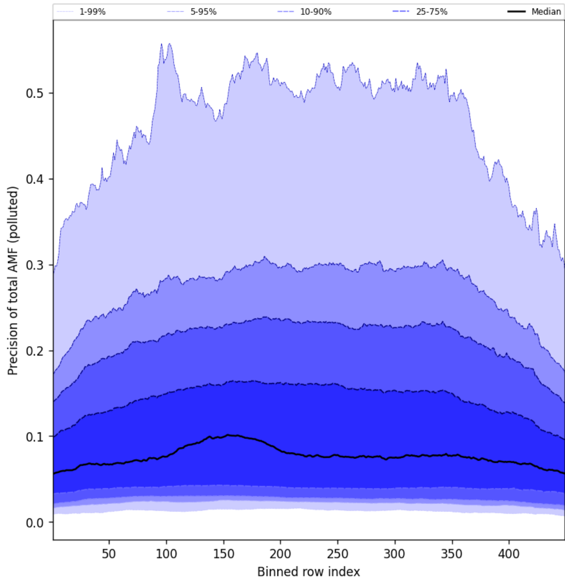
Figure 108: Along track statistics of “Precision of total AMF (polluted)” for 2025-09-10 to 2025-09-11
