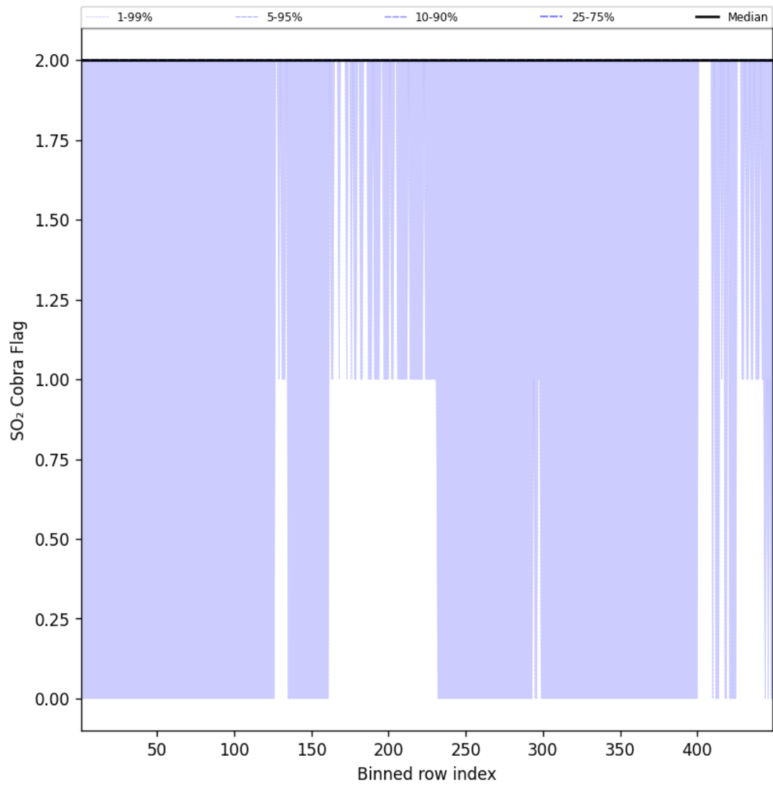
Figure 102: Along track statistics of “SO 2 Cobra Flag” for 2025-09-10 to 2025-09-11
