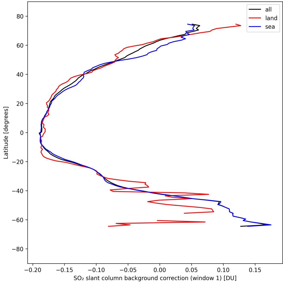
Figure 39: Zonal average of “SO 2 slant column background correction (window 1)” for 2025-09-10 to 2025-09-11.
