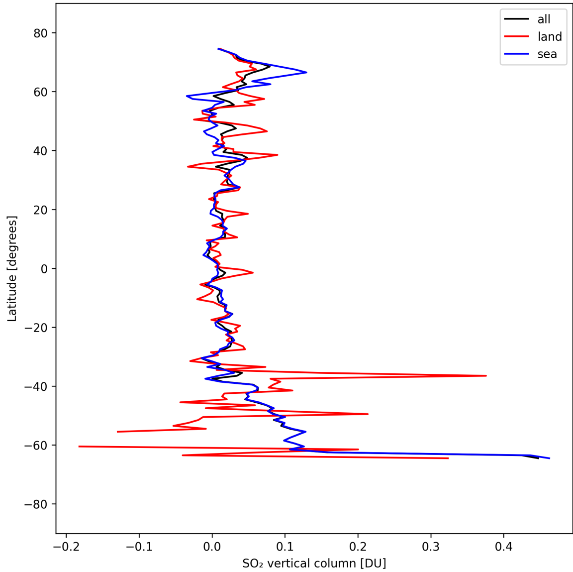
Figure 31: Zonal average of “SO 2 vertical column” for 2025-09-10 to 2025-09-11.
