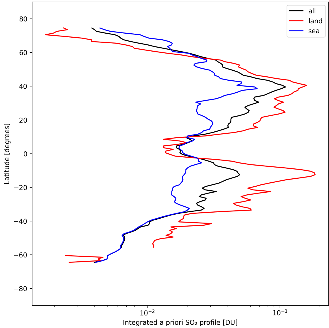
Figure 49: Zonal average of “Integrated a priori SO 2 profile” for 2025-09-10 to 2025-09-11.
