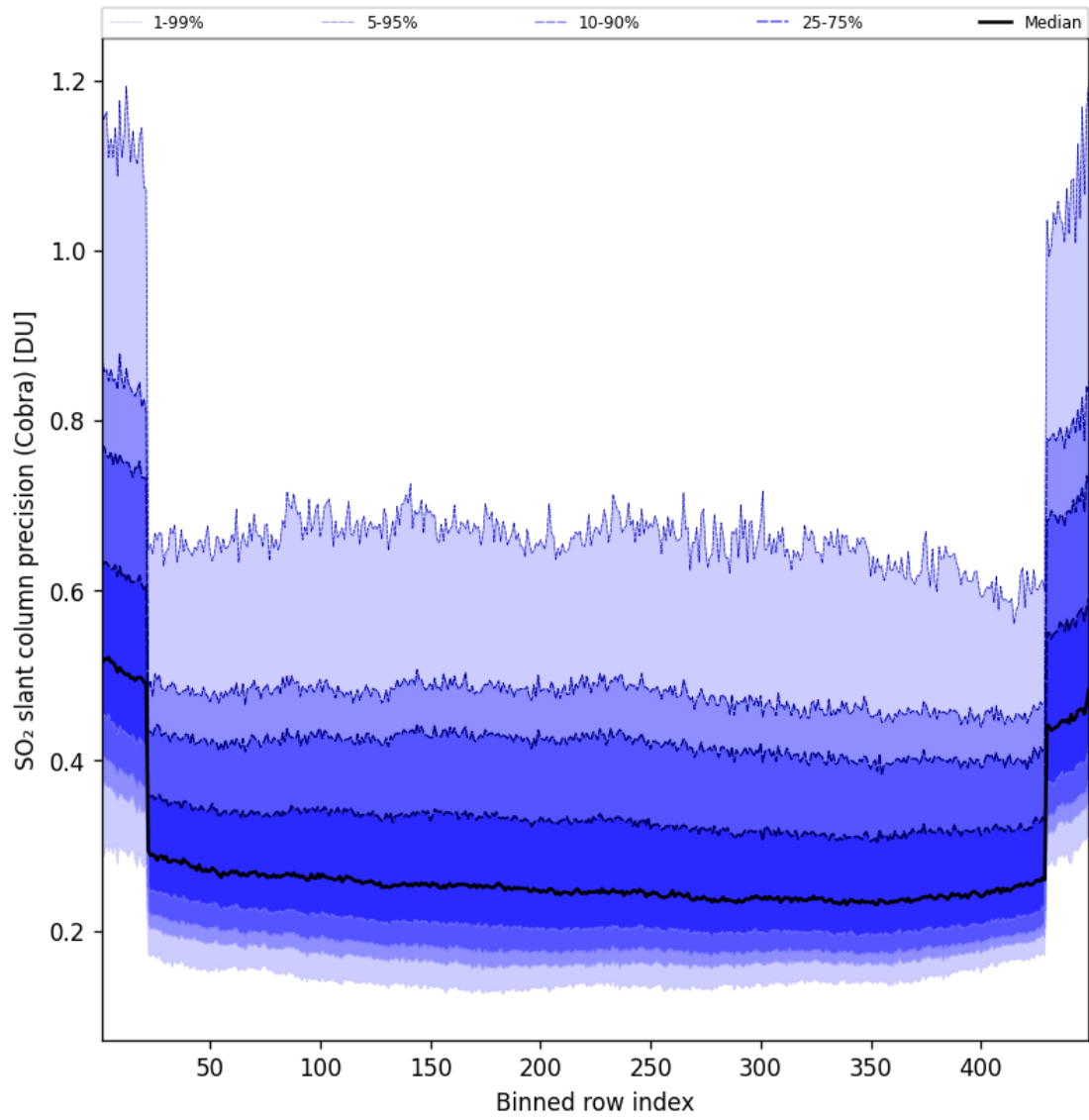
Figure 89: Along track statistics of “SO 2 slant column precision (Cobra)” for 2025-09-10 to 2025-09-11
