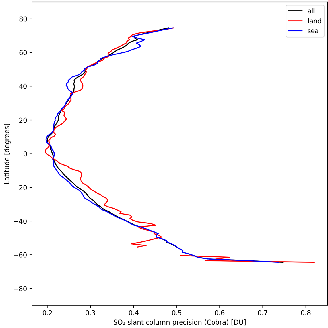
Figure 35: Zonal average of “SO 2 slant column precision (Cobra)” for 2025-09-10 to 2025-09-11.
