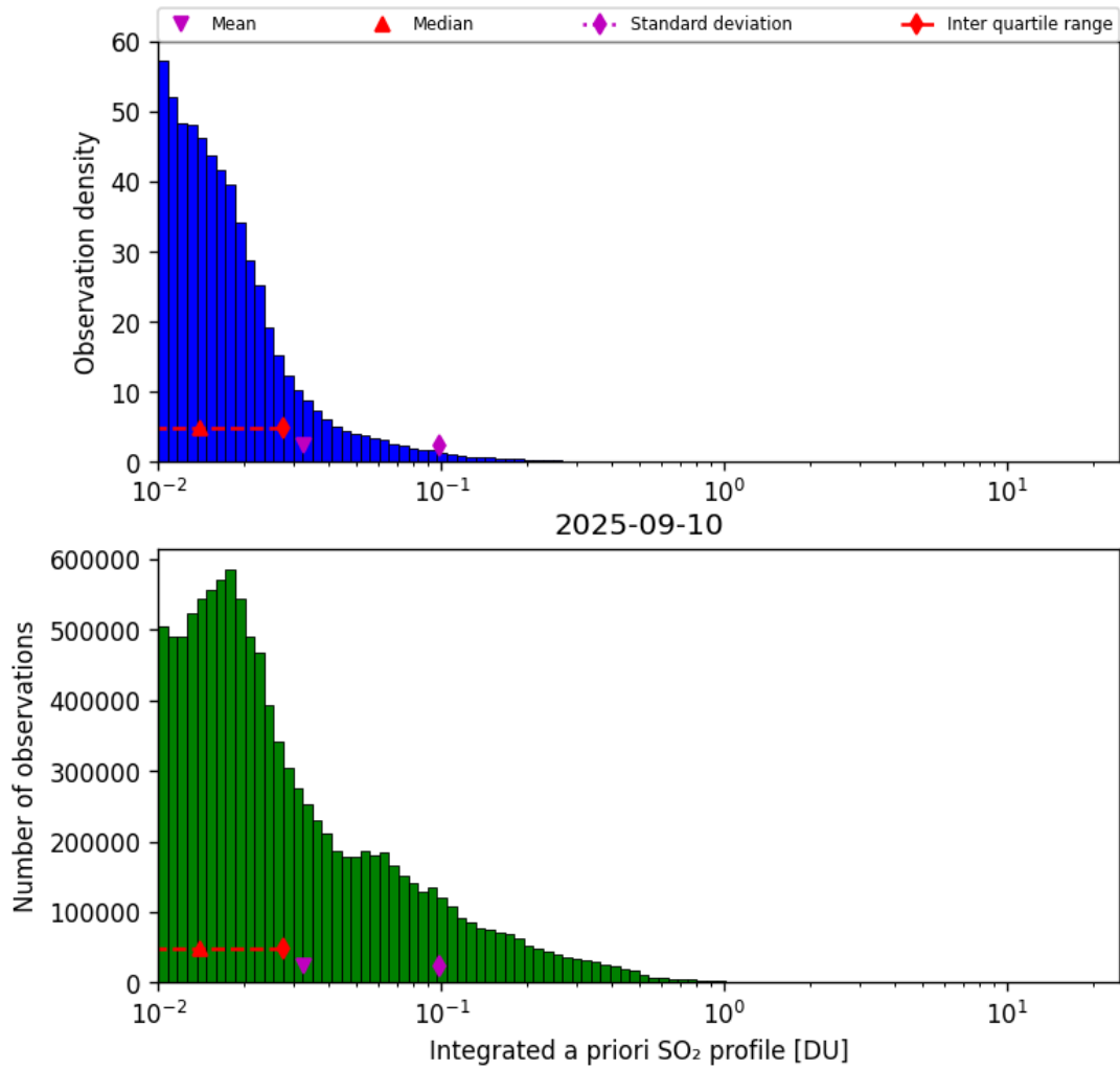
Figure 76: Histogram of “Integrated a priori SO 2 profile” for 2025-09-10 to 2025-09-11
