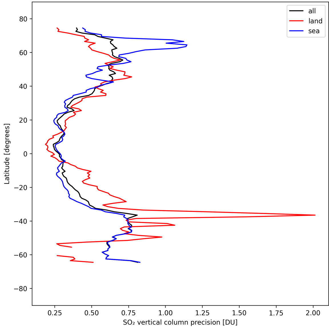
Figure 32: Zonal average of “SO 2 vertical column precision” for 2025-09-10 to 2025-09-11.
