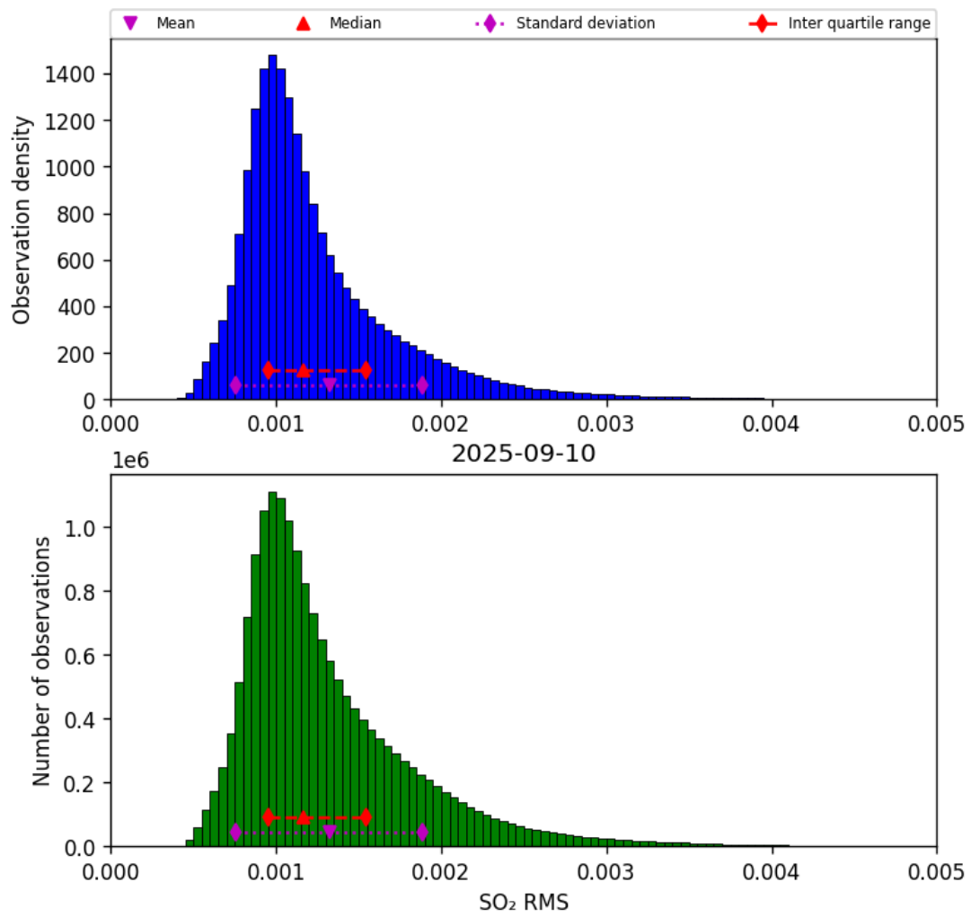
Figure 79: Histogram of “SO 2 RMS” for 2025-09-10 to 2025-09-11
