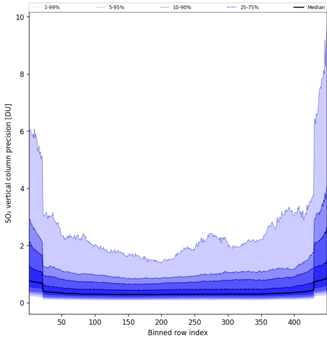
Figure 86: Along track statistics of “SO 2 vertical column precision” for 2025-09-10 to 2025-09-11
