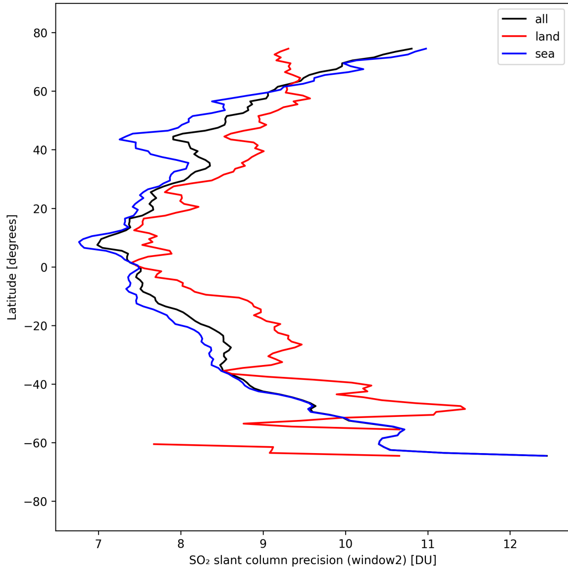
Figure 41: Zonal average of "SO 2 slant column precision (window2)" for 2025-09-10 to 2025-09-11.
