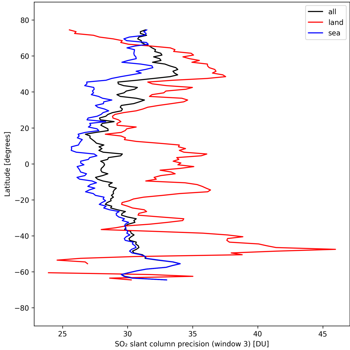
Figure 45: Zonal average of “SO 2 slant column precision (window 3)” for 2025-09-10 to 2025-09-11.
