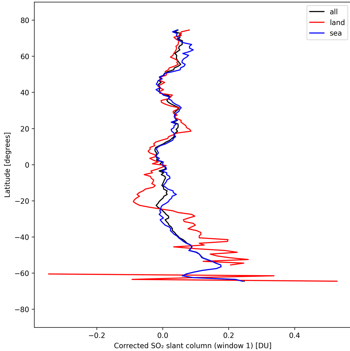
Figure 38: Zonal average of “Corrected SO 2 slant column (window 1)” for 2025-09-10 to 2025-09-11.
