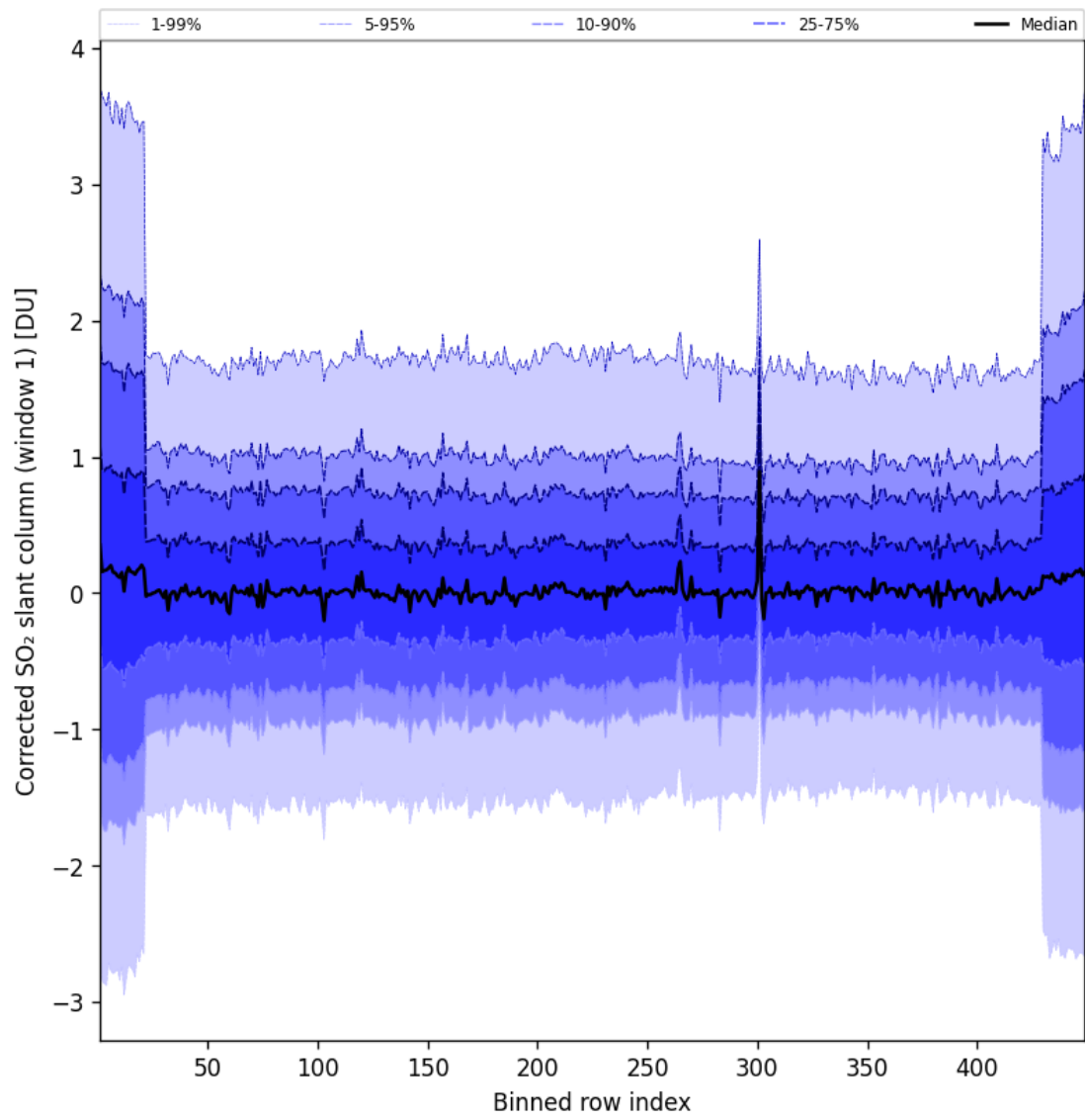
Figure 92: Along track statistics of “Corrected SO 2 slant column (window 1)” for 2025-09-10 to 2025-09-11
