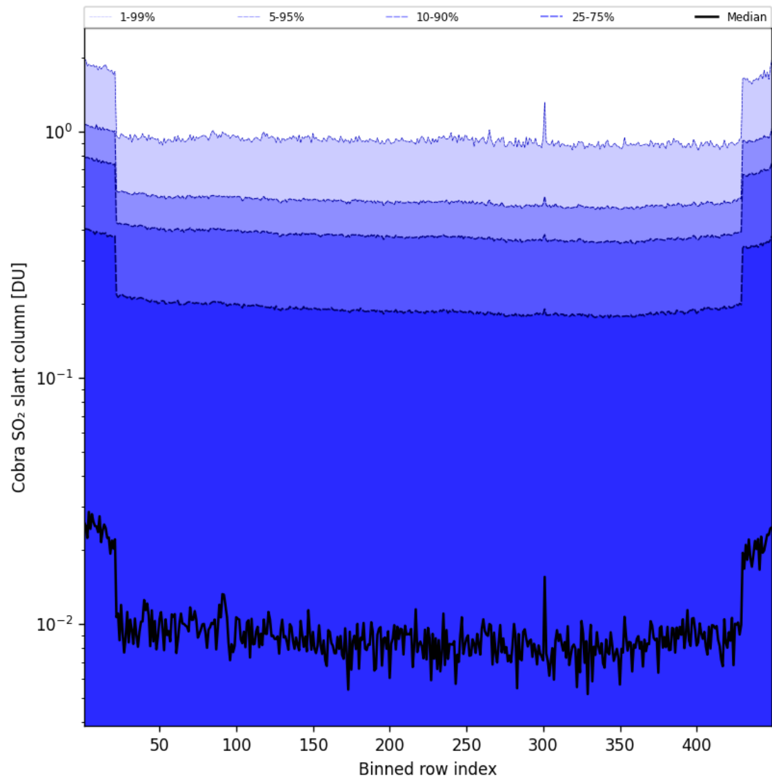
Figure 88: Along track statistics of “Cobra SO 2 slant column” for 2025-09-10 to 2025-09-11
