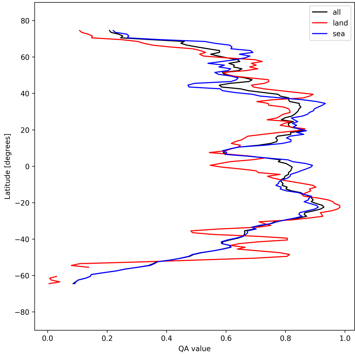
Figure 30: Zonal average of “QA value” for 2025-09-10 to 2025-09-11.
