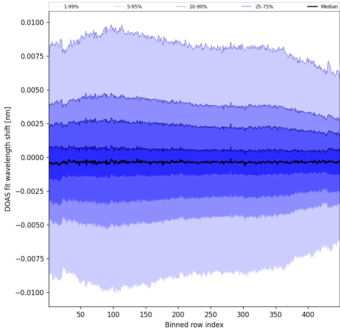
Figure 104: Along track statistics of “DOAS fit wavelength shift” for 2025-09-10 to 2025-09-11
