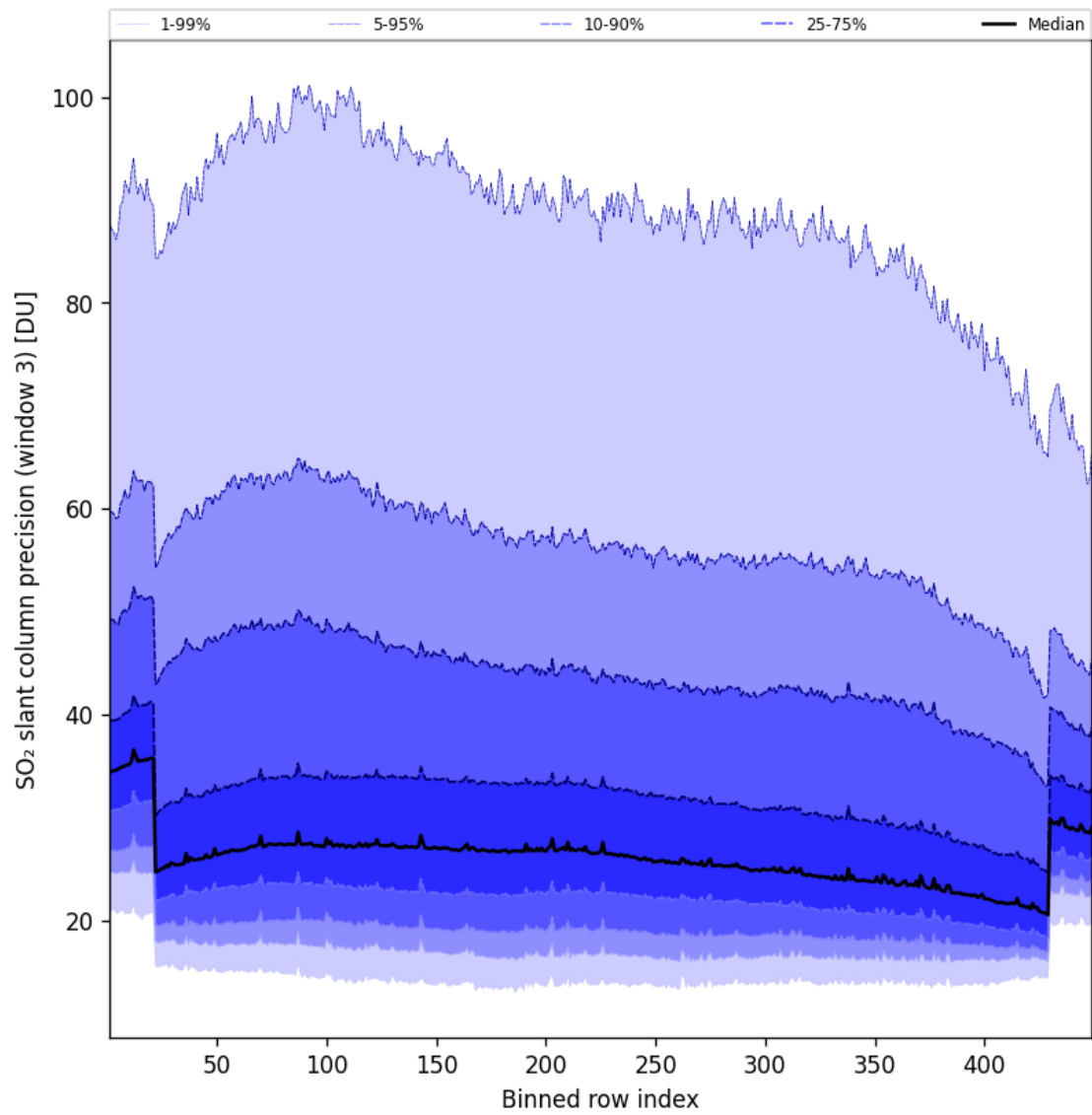
Figure 99: Along track statistics of “SO 2 slant column precision (window 3)” for 2025-09-10 to 2025-09-11
