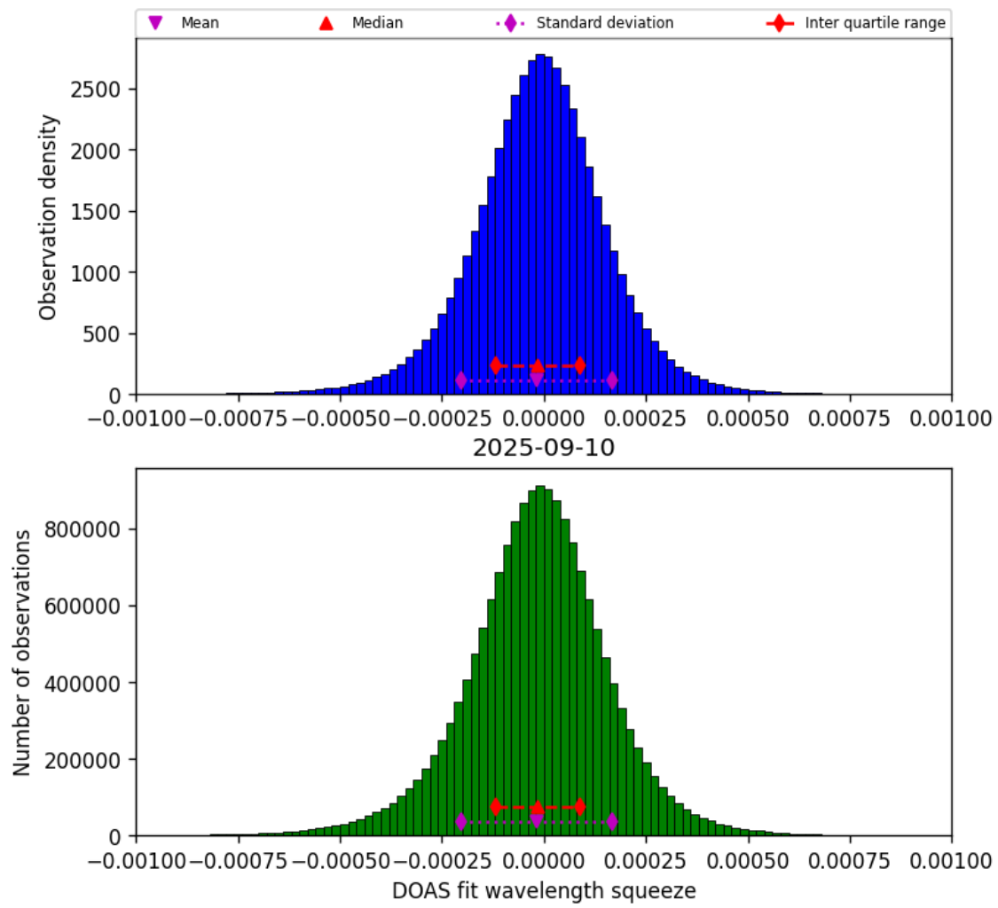
Figure 78: Histogram of “DOAS fit wavelength squeeze” for 2025-09-10 to 2025-09-11
