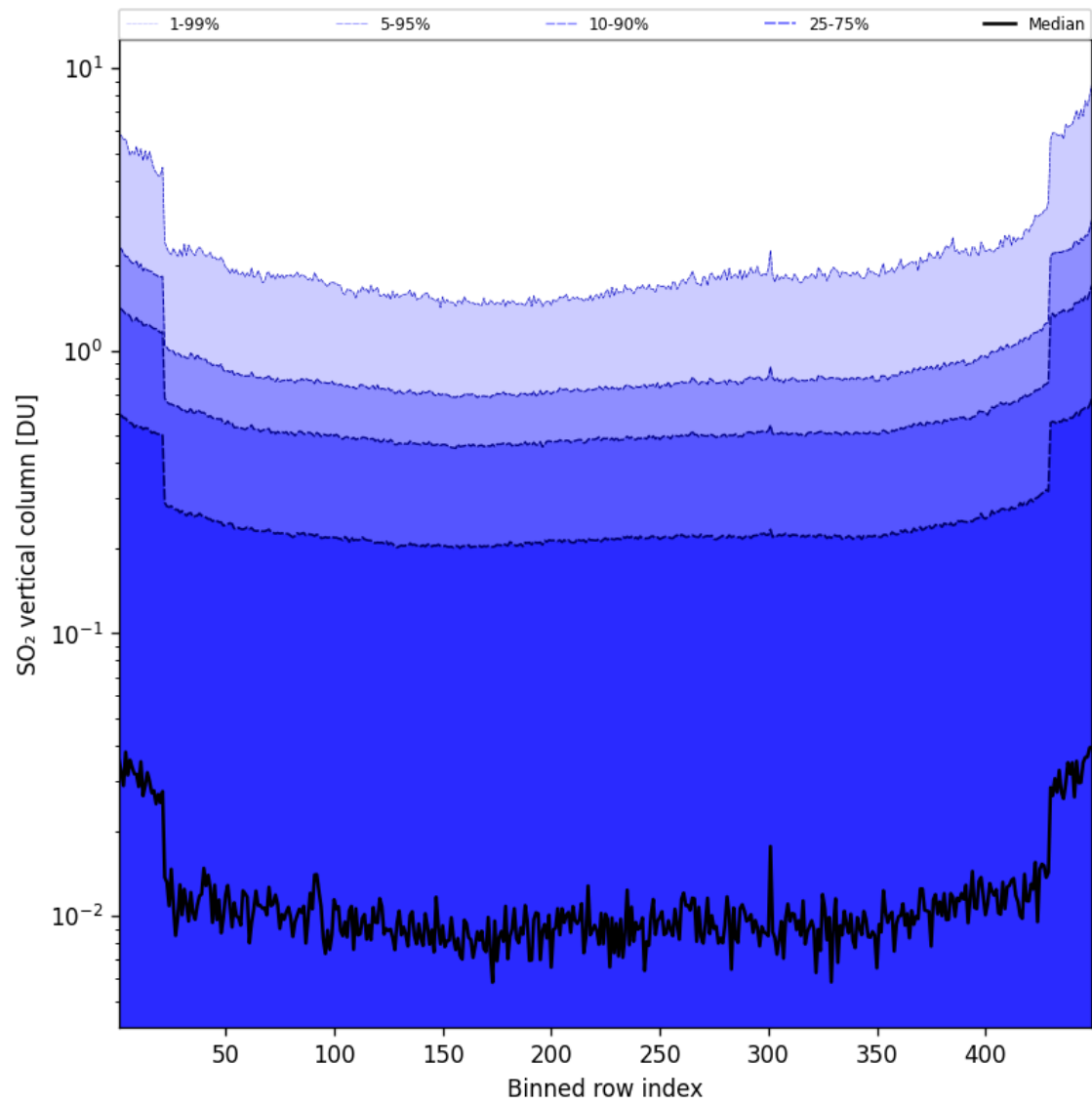
Figure 85: Along track statistics of “SO 2 vertical column” for 2025-09-10 to 2025-09-11
