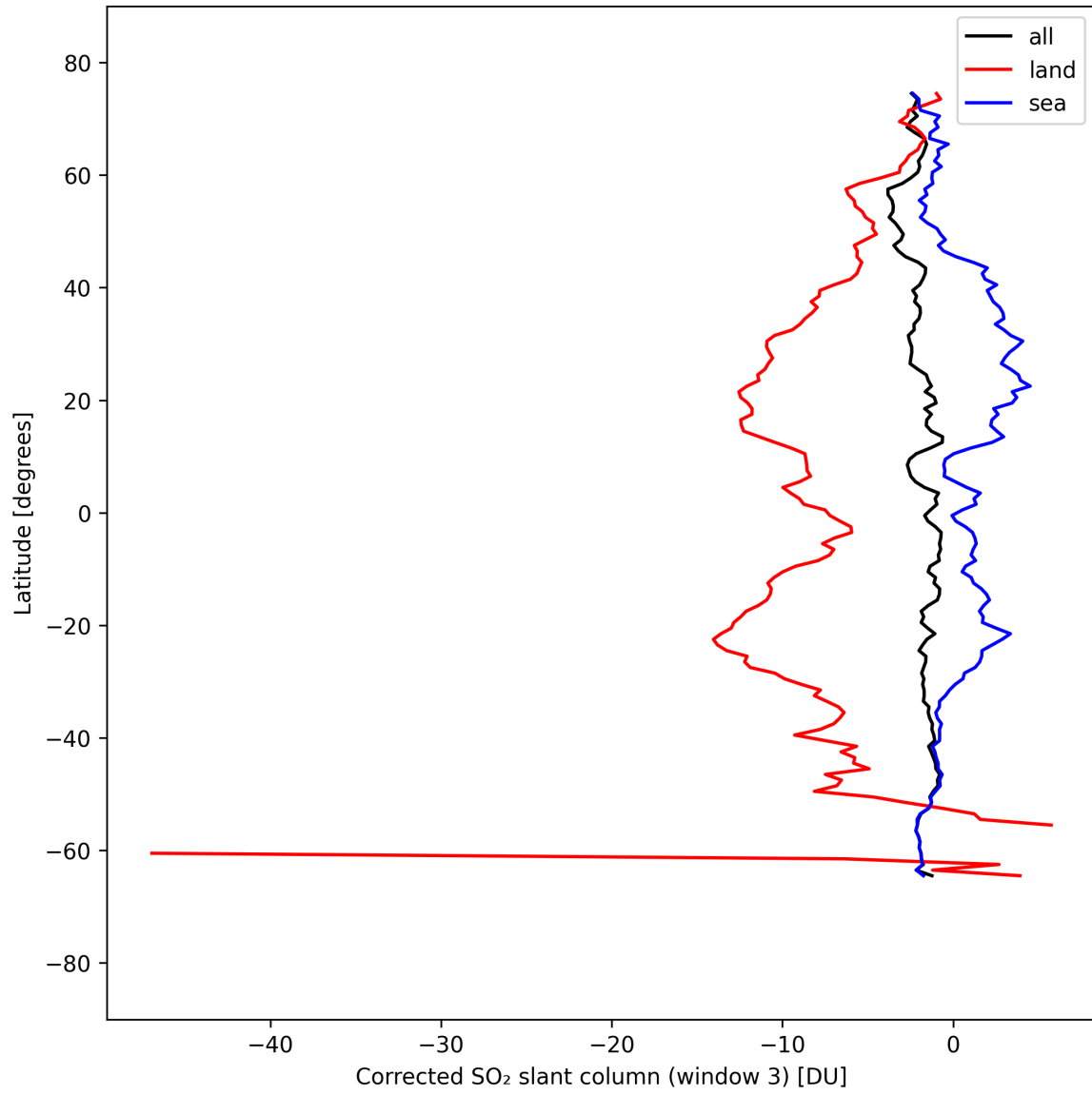
Figure 46: Zonal average of “Corrected SO 2 slant column (window 3)” for 2025-09-10 to 2025-09-11.
