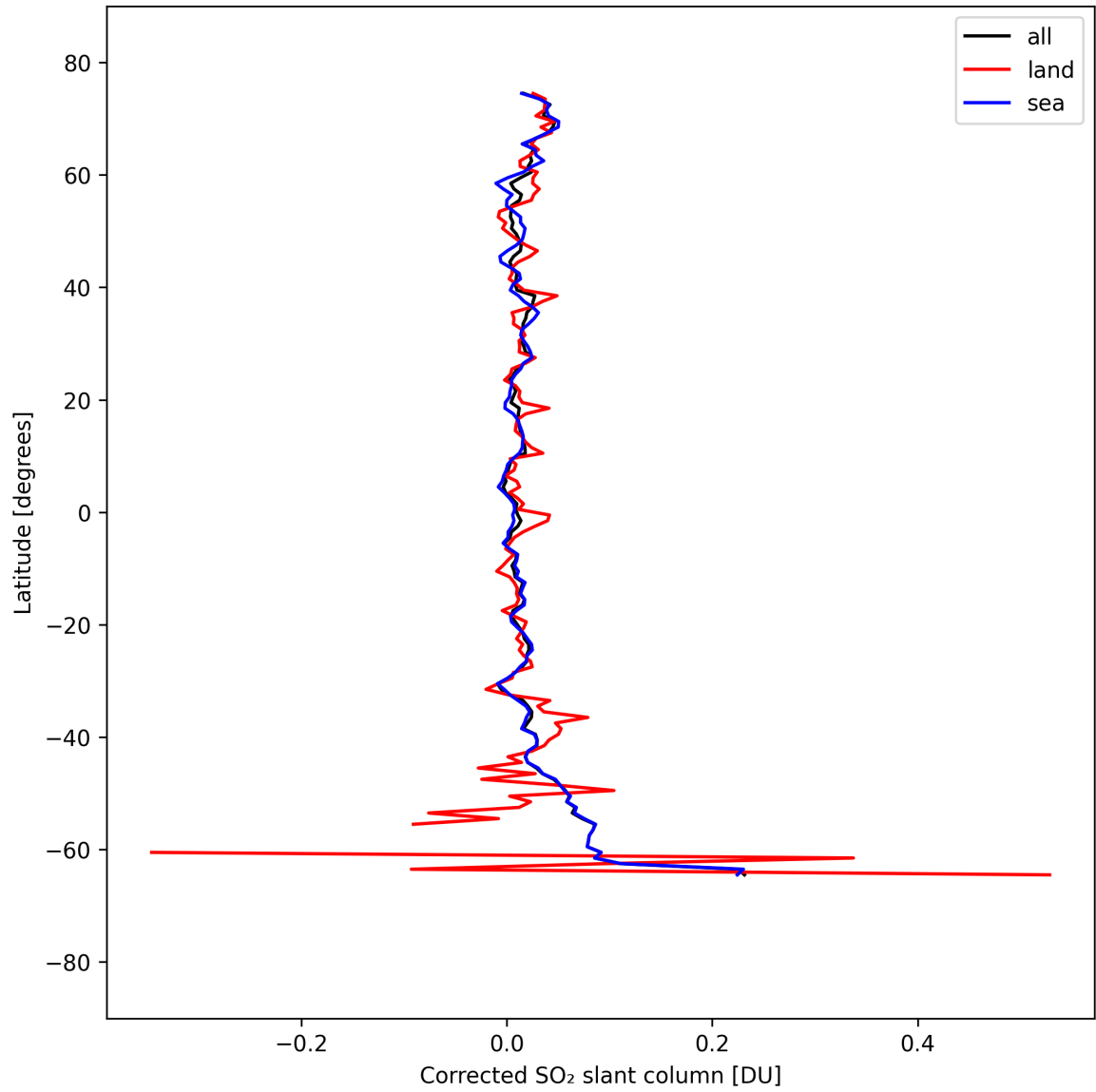
Figure 33: Zonal average of “Corrected SO 2 slant column” for 2025-09-10 to 2025-09-11.
