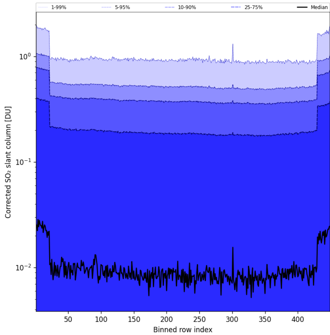
Figure 87: Along track statistics of “Corrected SO 2 slant column” for 2025-09-10 to 2025-09-11
