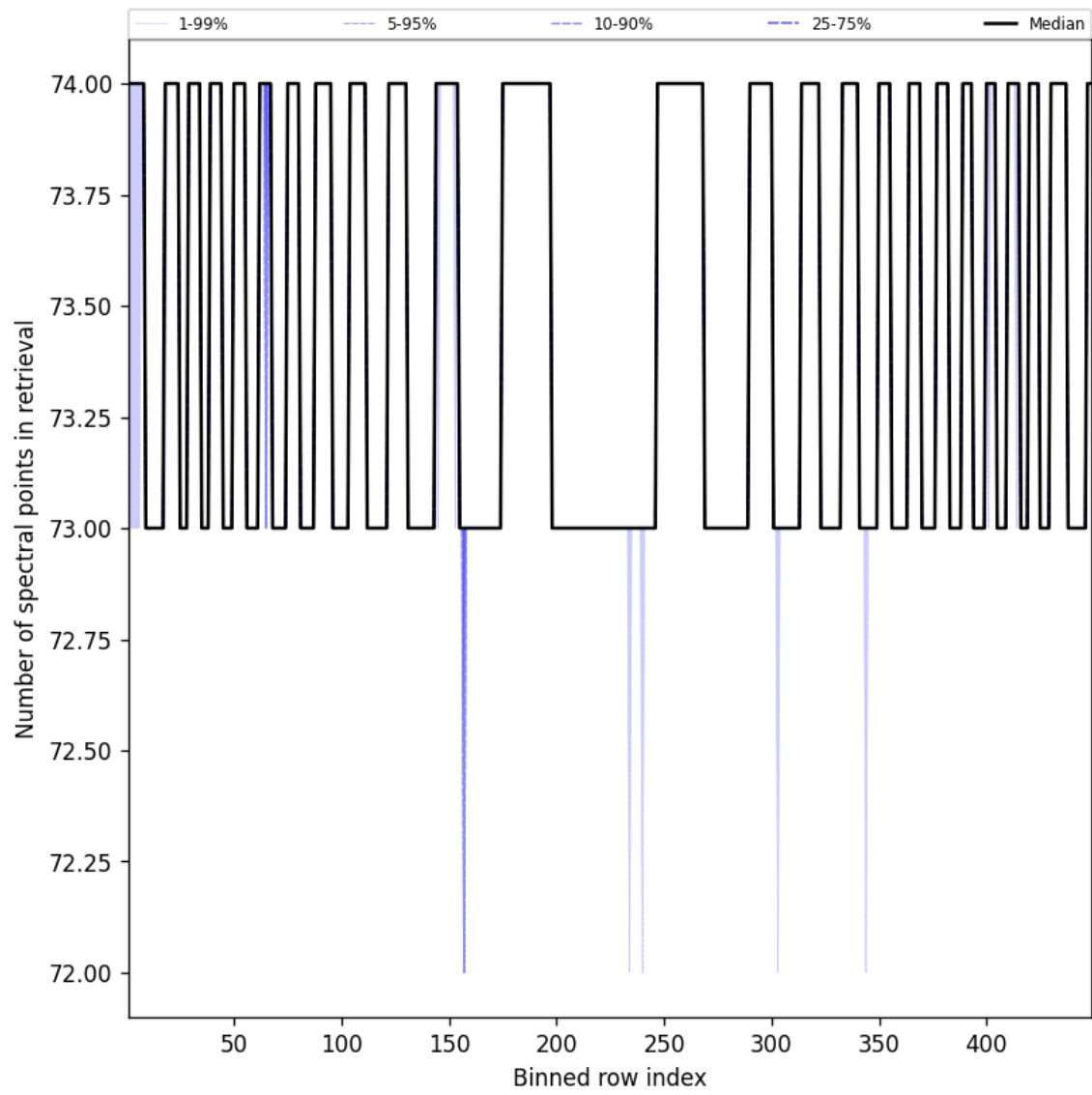
Figure 110: Along track statistics of “Number of spectral points in retrieval” for 2025-09-10 to 2025-09-11
