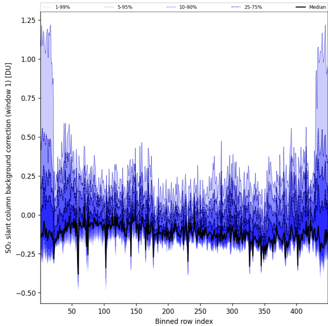
Figure 93: Along track statistics of “SO 2 slant column background correction (window 1)” for 2025-09-10 to 2025-09-11
