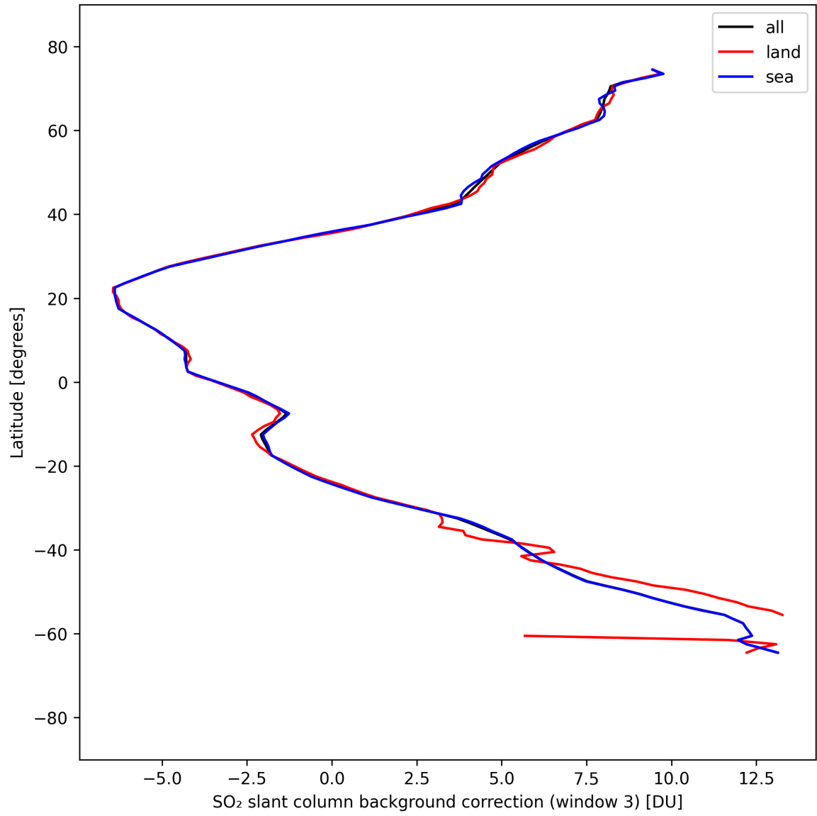
Figure 47: Zonal average of “SO 2 slant column background correction (window 3)” for 2025-09-10 to 2025-09-11.
