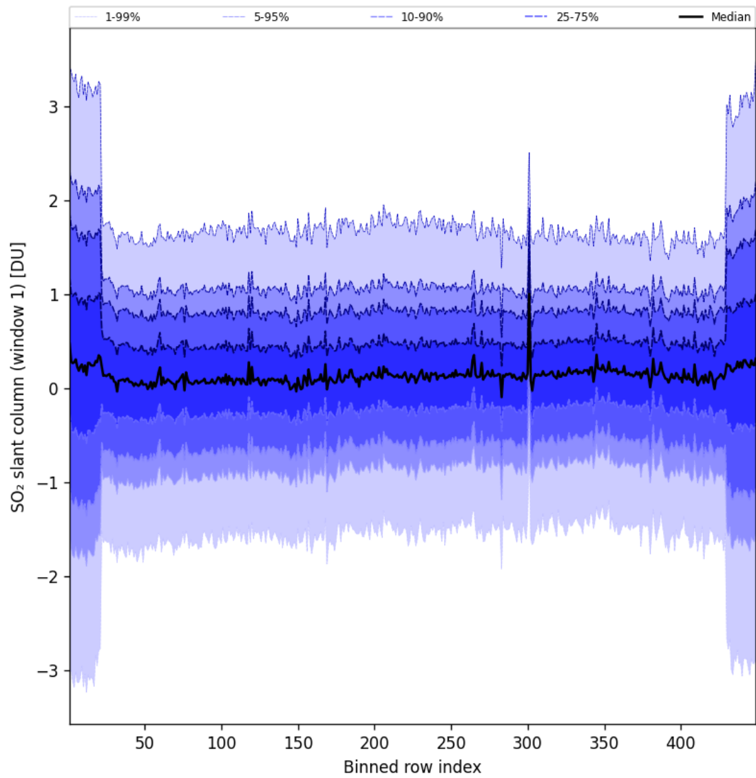
Figure 90: Along track statistics of “SO 2 slant column (window 1)” for 2025-09-10 to 2025-09-11
