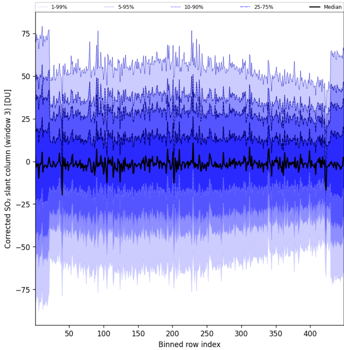
Figure 100: Along track statistics of “Corrected SO 2 slant column (window 3)” for 2025-09-10 to 2025-09-11
