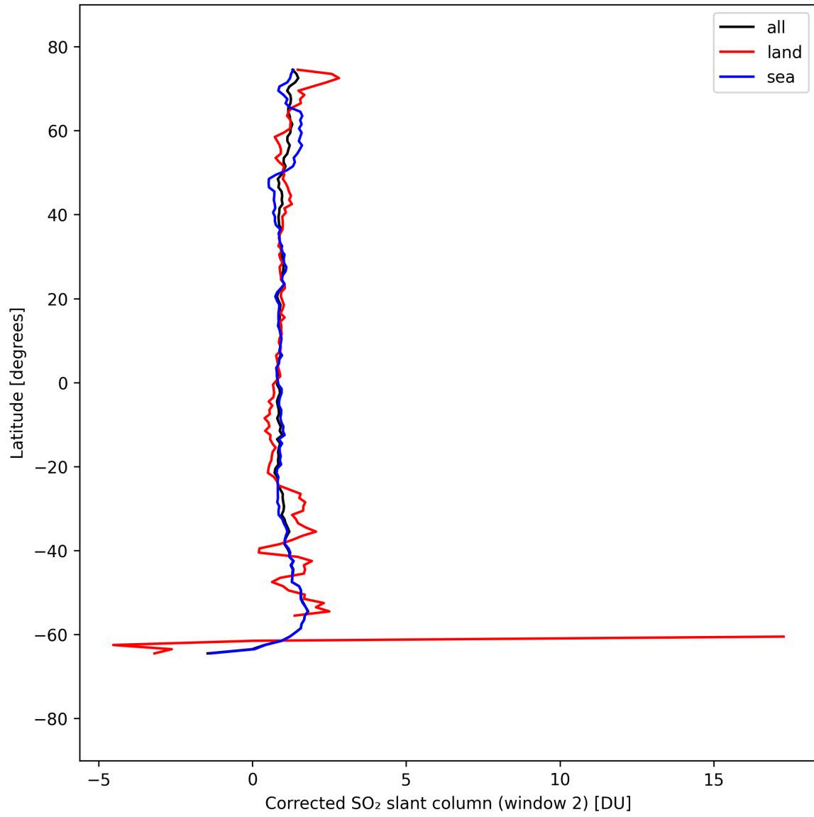
Figure 42: Zonal average of “Corrected SO 2 slant column (window 2)” for 2025-09-10 to 2025-09-11.
