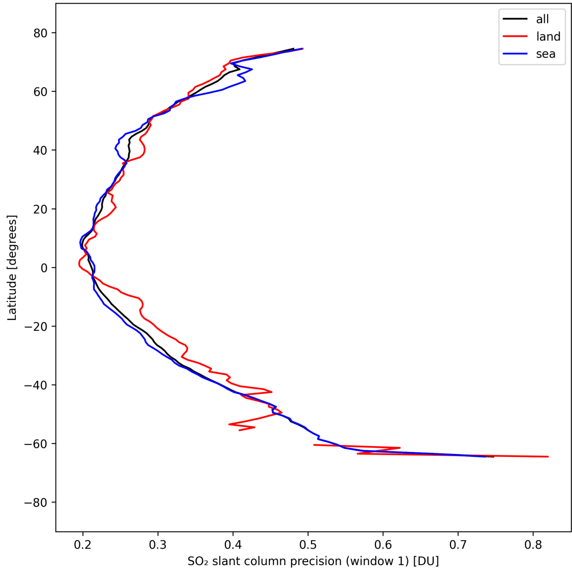
Figure 37: Zonal average of “SO 2 slant column precision (window 1)” for 2025-09-10 to 2025-09-11.
