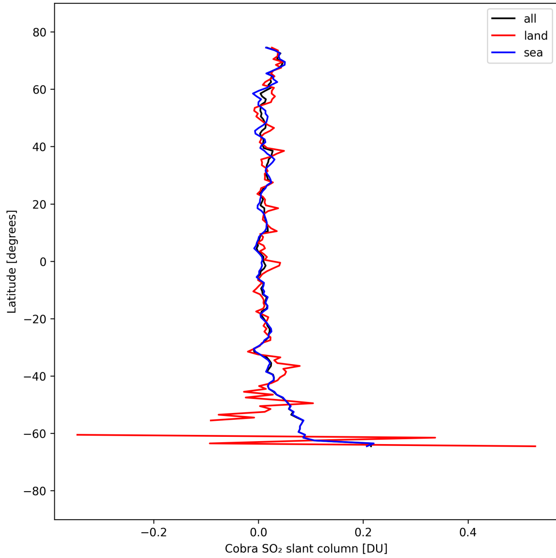
Figure 34: Zonal average of “Cobra SO 2 slant column” for 2025-09-10 to 2025-09-11.
