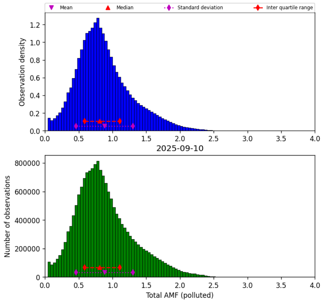
Figure 80: Histogram of “Total AMF (polluted)” for 2025-09-10 to 2025-09-11
