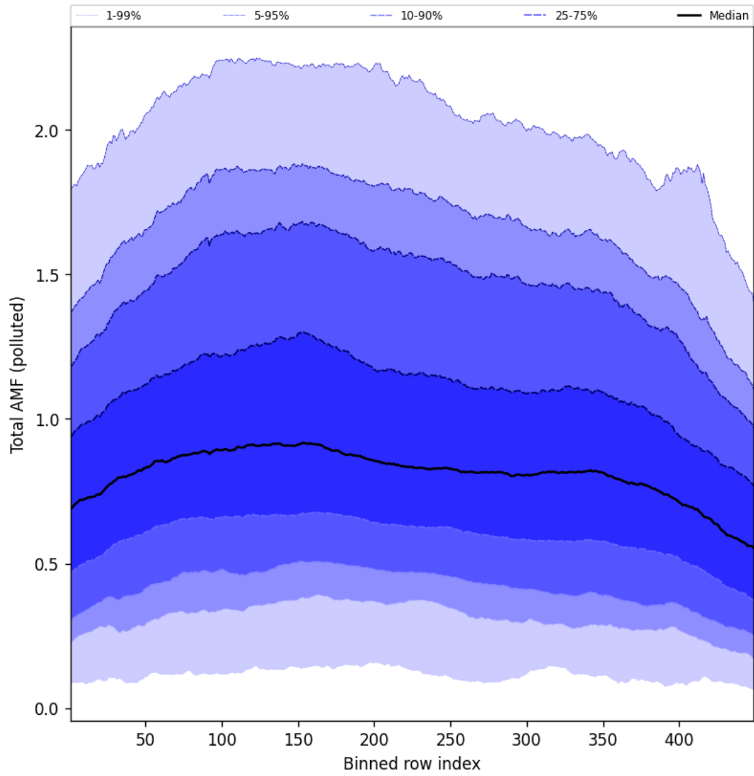
Figure 107: Along track statistics of “Total AMF (polluted)” for 2025-09-10 to 2025-09-11
