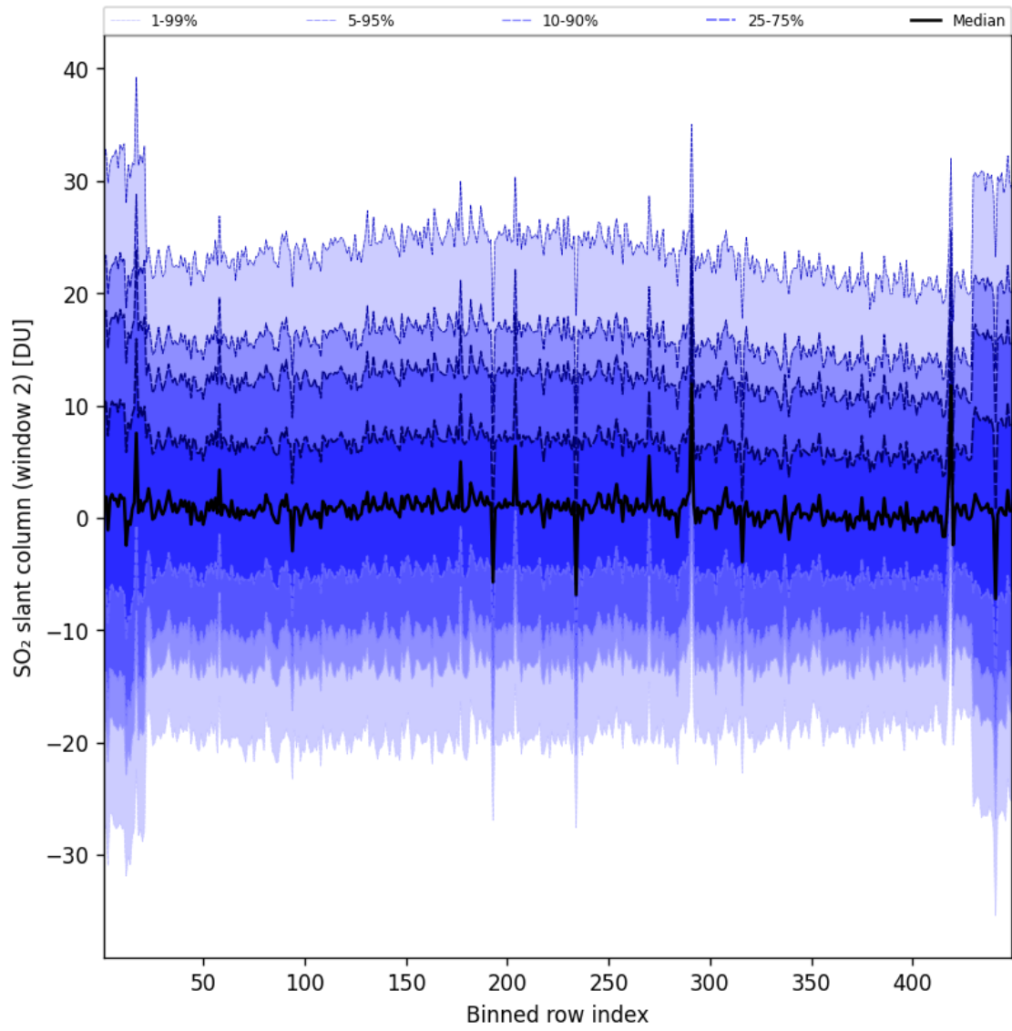
Figure 94: Along track statistics of “SO 2 slant column (window 2)” for 2025-09-10 to 2025-09-11
