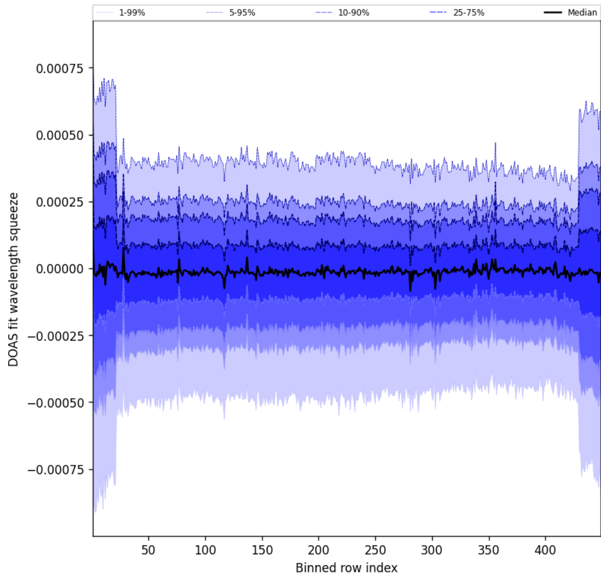
Figure 105: Along track statistics of “DOAS fit wavelength squeeze” for 2025-09-10 to 2025-09-11
