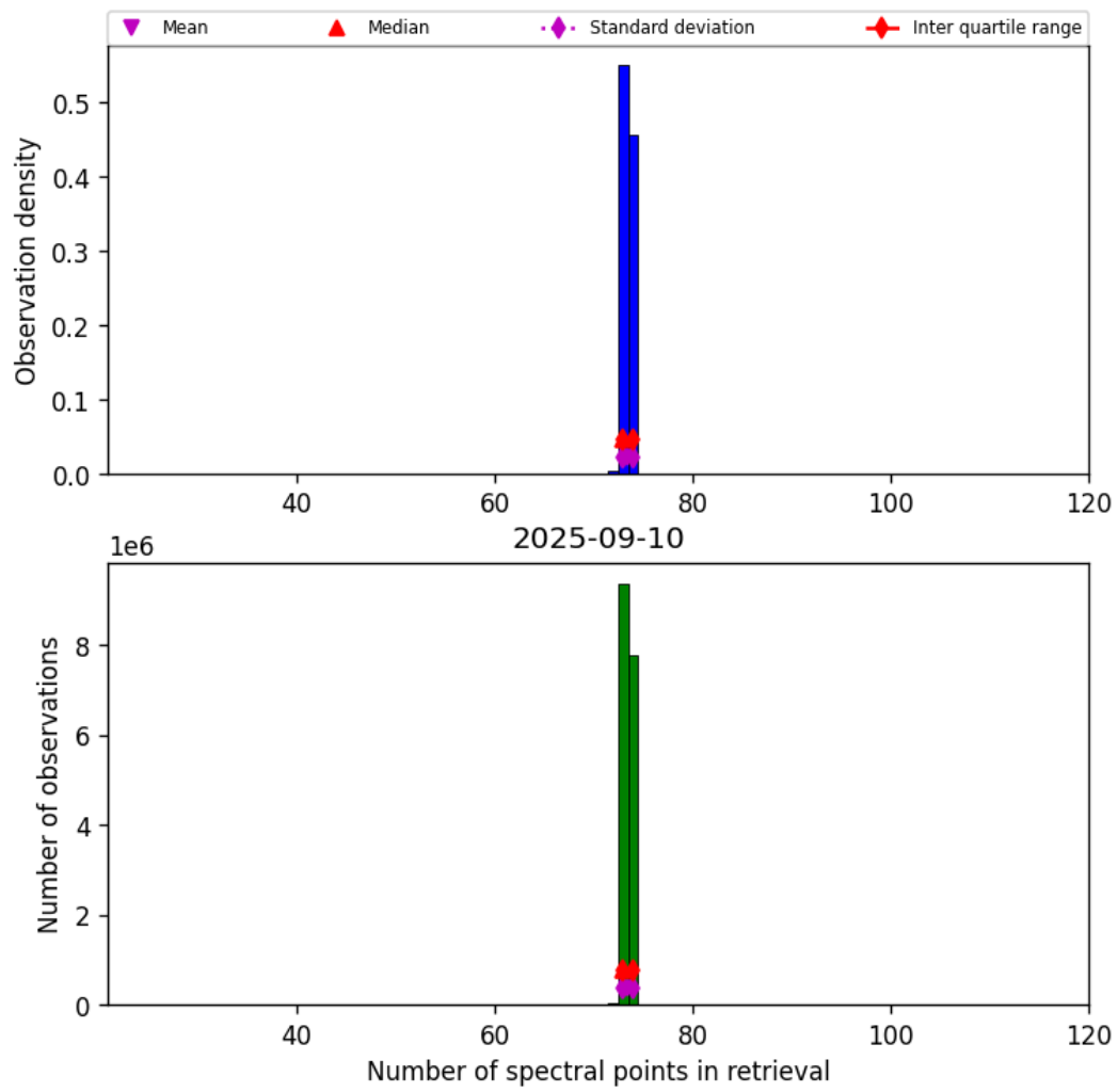
Figure 83: Histogram of “Number of spectral points in retrieval” for 2025-09-10 to 2025-09-11
