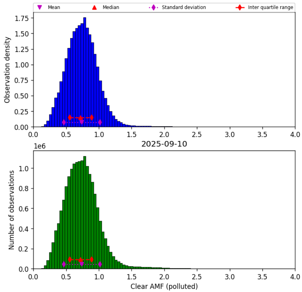
Figure 82: Histogram of “Clear AMF (polluted)” for 2025-09-10 to 2025-09-11
