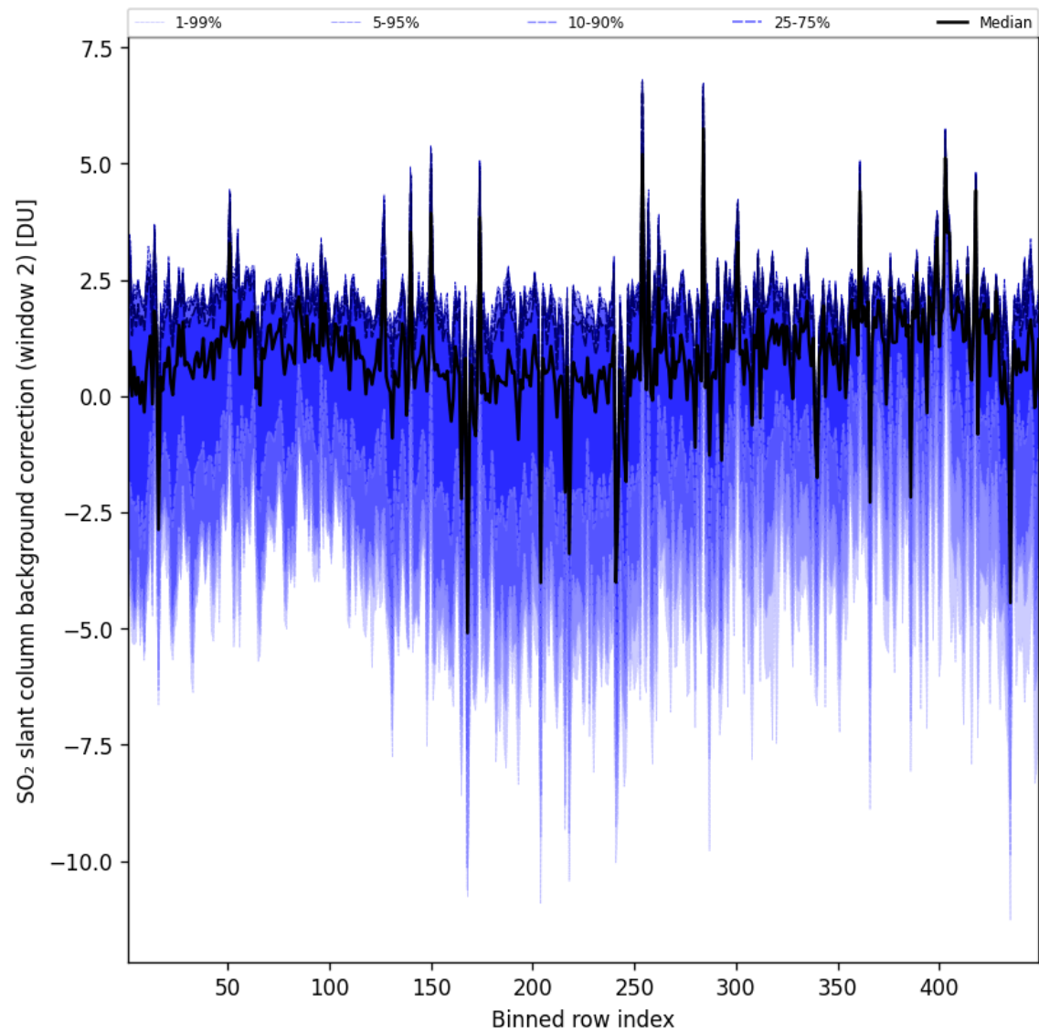
Figure 97: Along track statistics of “SO 2 slant column background correction (window 2)” for 2025-09-10 to 2025-09-11
