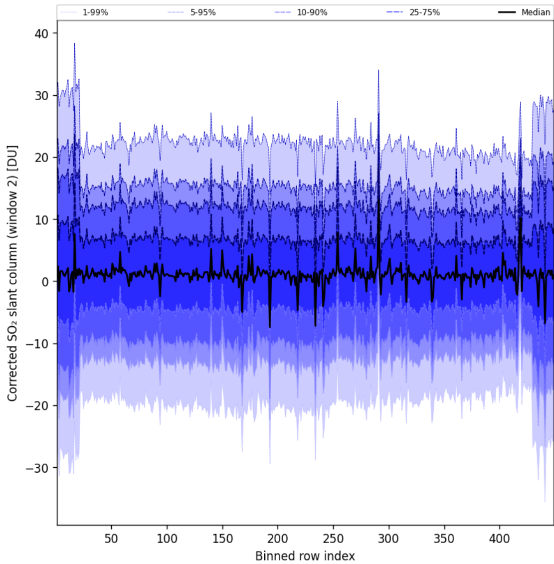
Figure 96: Along track statistics of “Corrected SO 2 slant column (window 2)” for 2025-09-10 to 2025-09-11
