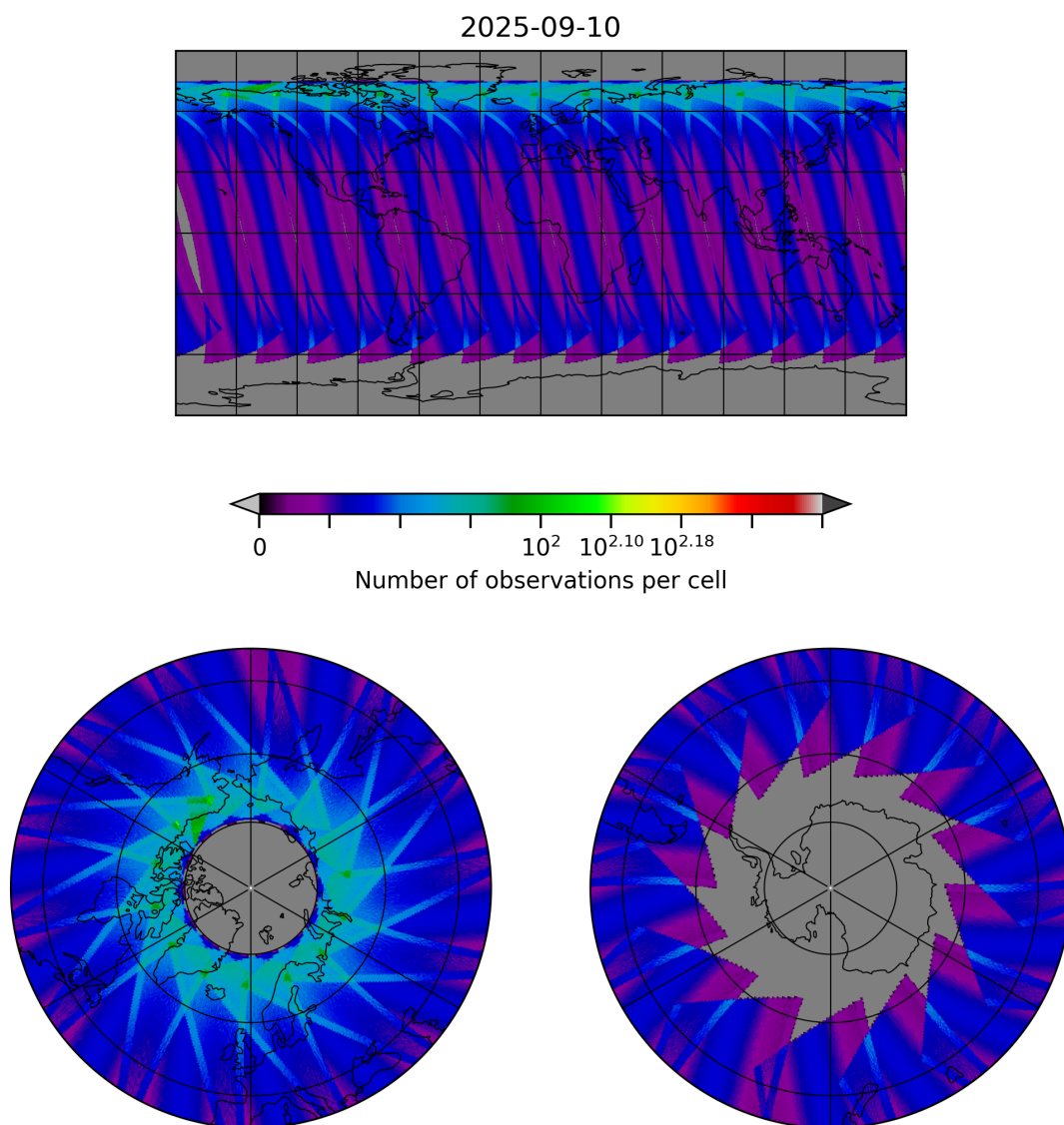
Figure 29: Map of the number of observations for 2025-09-10 to 2025-09-11
