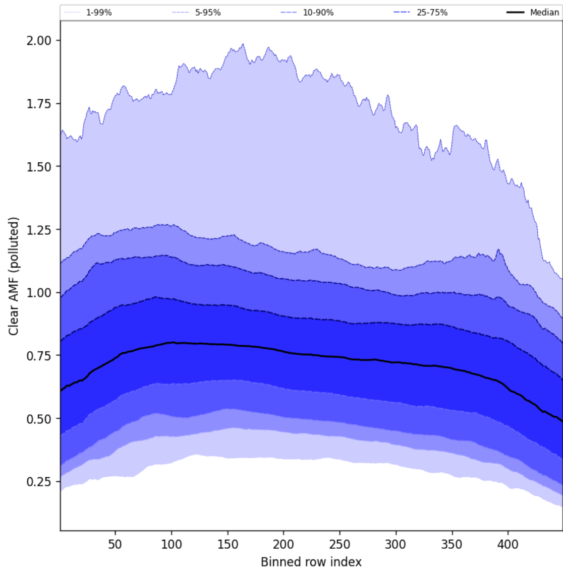
Figure 109: Along track statistics of “Clear AMF (polluted)” for 2025-09-10 to 2025-09-11
