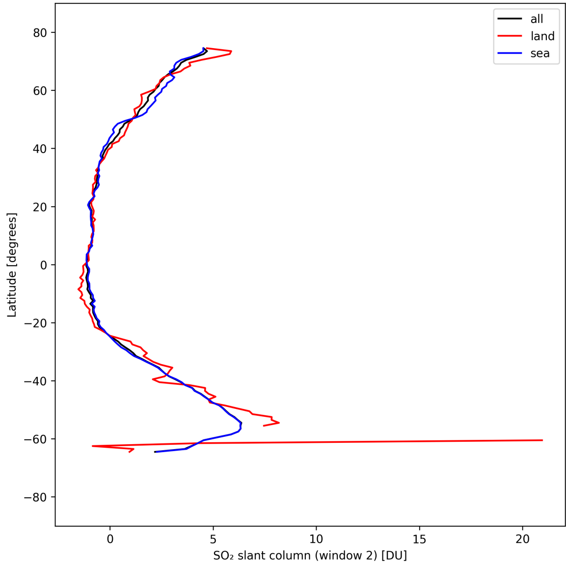
Figure 40: Zonal average of “SO 2 slant column (window 2)” for 2025-09-10 to 2025-09-11.
