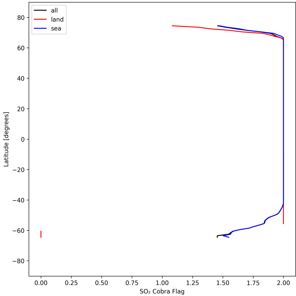
Figure 48: Zonal average of "SO 2 Cobra Flag" for 2025-09-10 to 2025-09-11.
