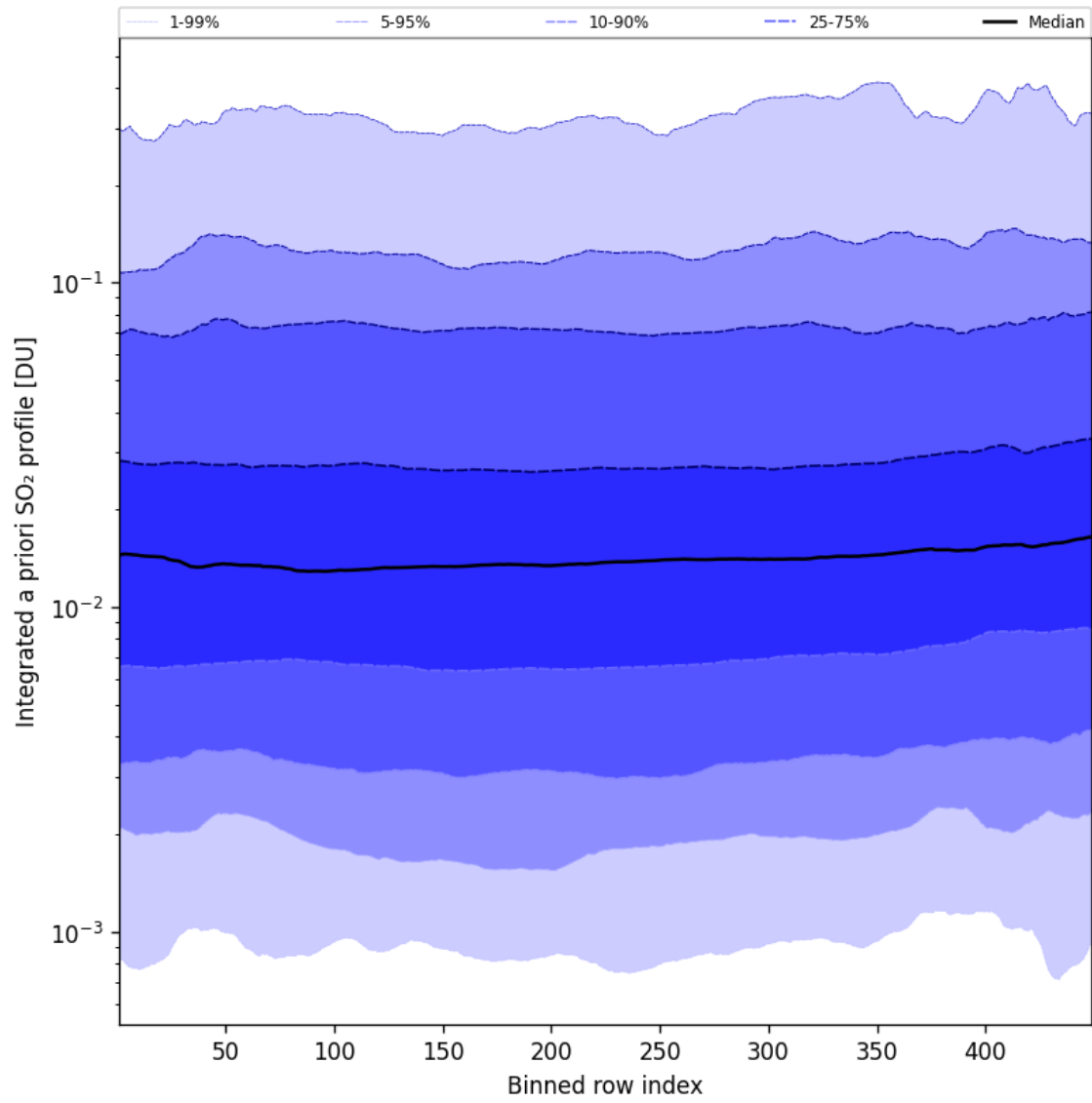
Figure 103: Along track statistics of “Integrated a priori SO 2 profile” for 2025-09-10 to 2025-09-11
