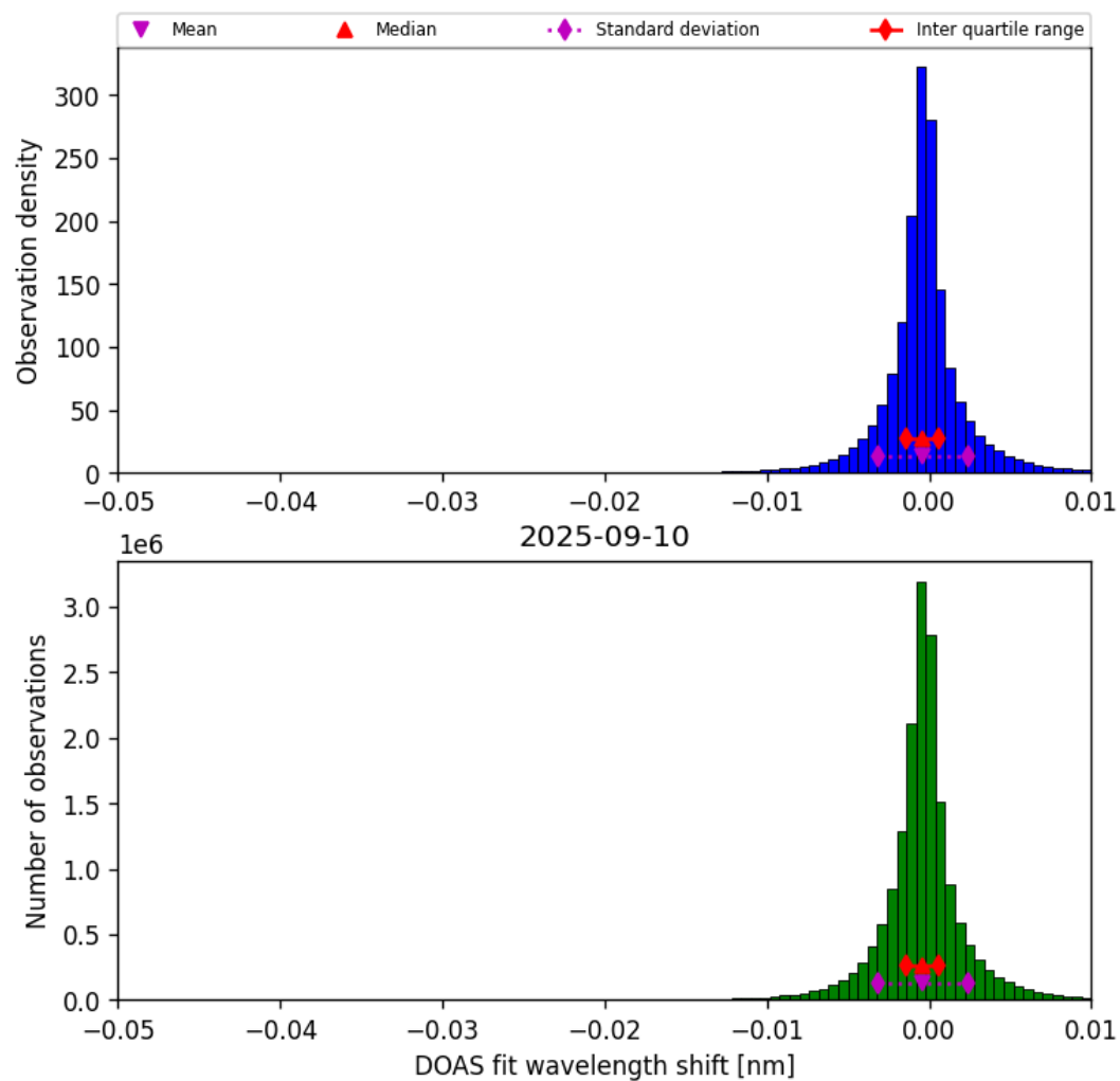
Figure 77: Histogram of “DOAS fit wavelength shift” for 2025-09-10 to 2025-09-11
