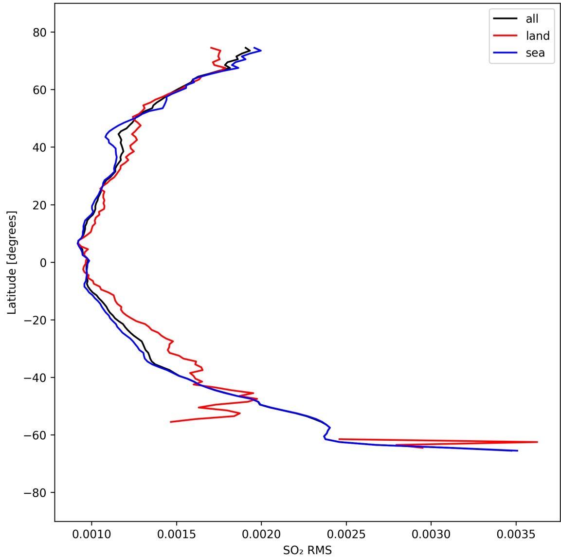
Figure 52: Zonal average of “SO 2 RMS” for 2025-09-11 to 2025-09-12.
