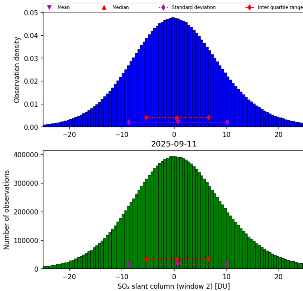
Figure 67: Histogram of “SO 2 slant column (window 2)” for 2025-09-11 to 2025-09-12
