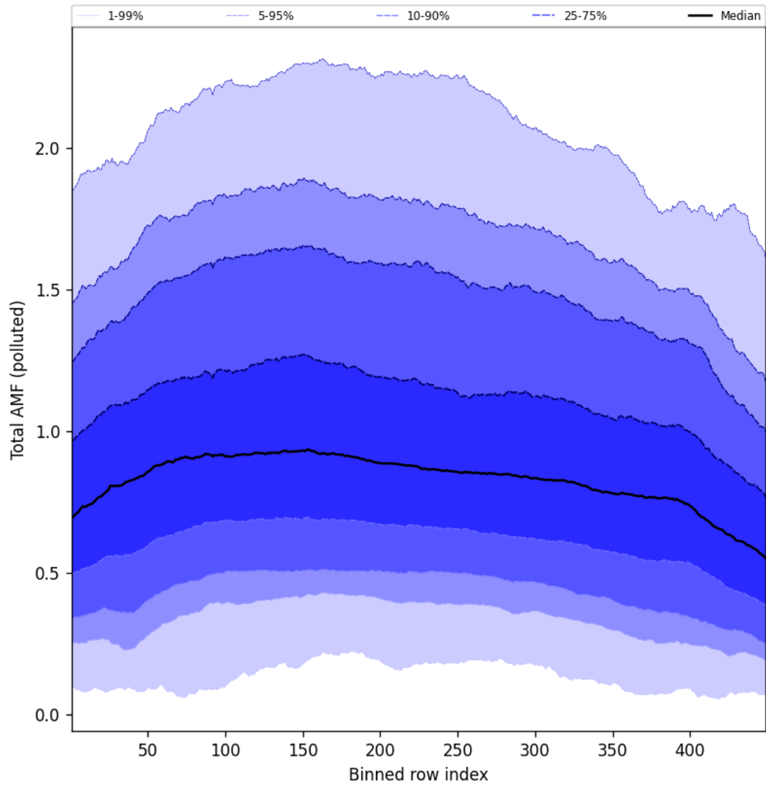
Figure 107: Along track statistics of “Total AMF (polluted)” for 2025-09-11 to 2025-09-12
