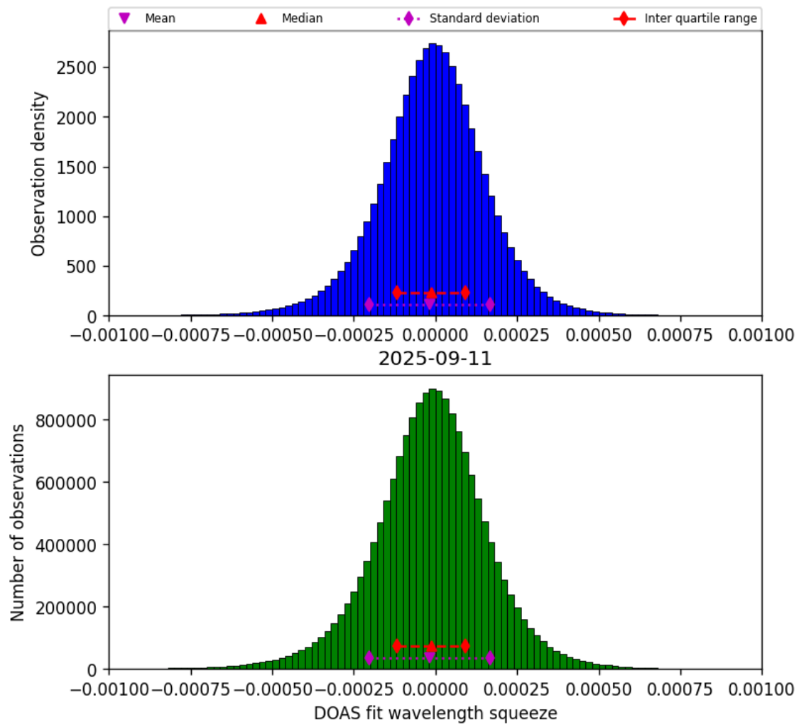
Figure 78: Histogram of “DOAS fit wavelength squeeze” for 2025-09-11 to 2025-09-12
