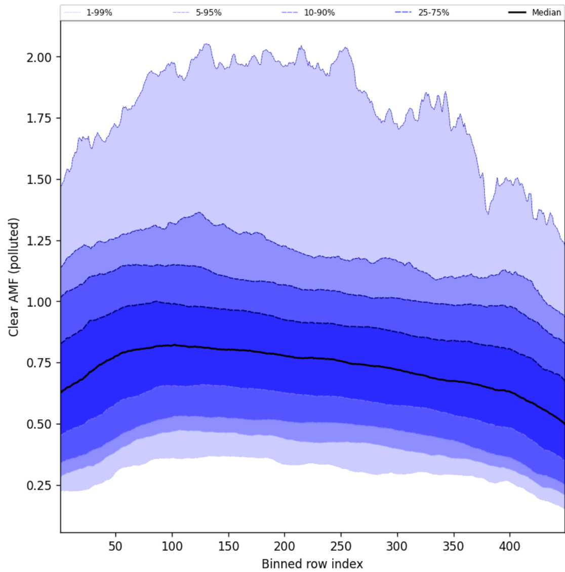
Figure 109: Along track statistics of “Clear AMF (polluted)” for 2025-09-11 to 2025-09-12
