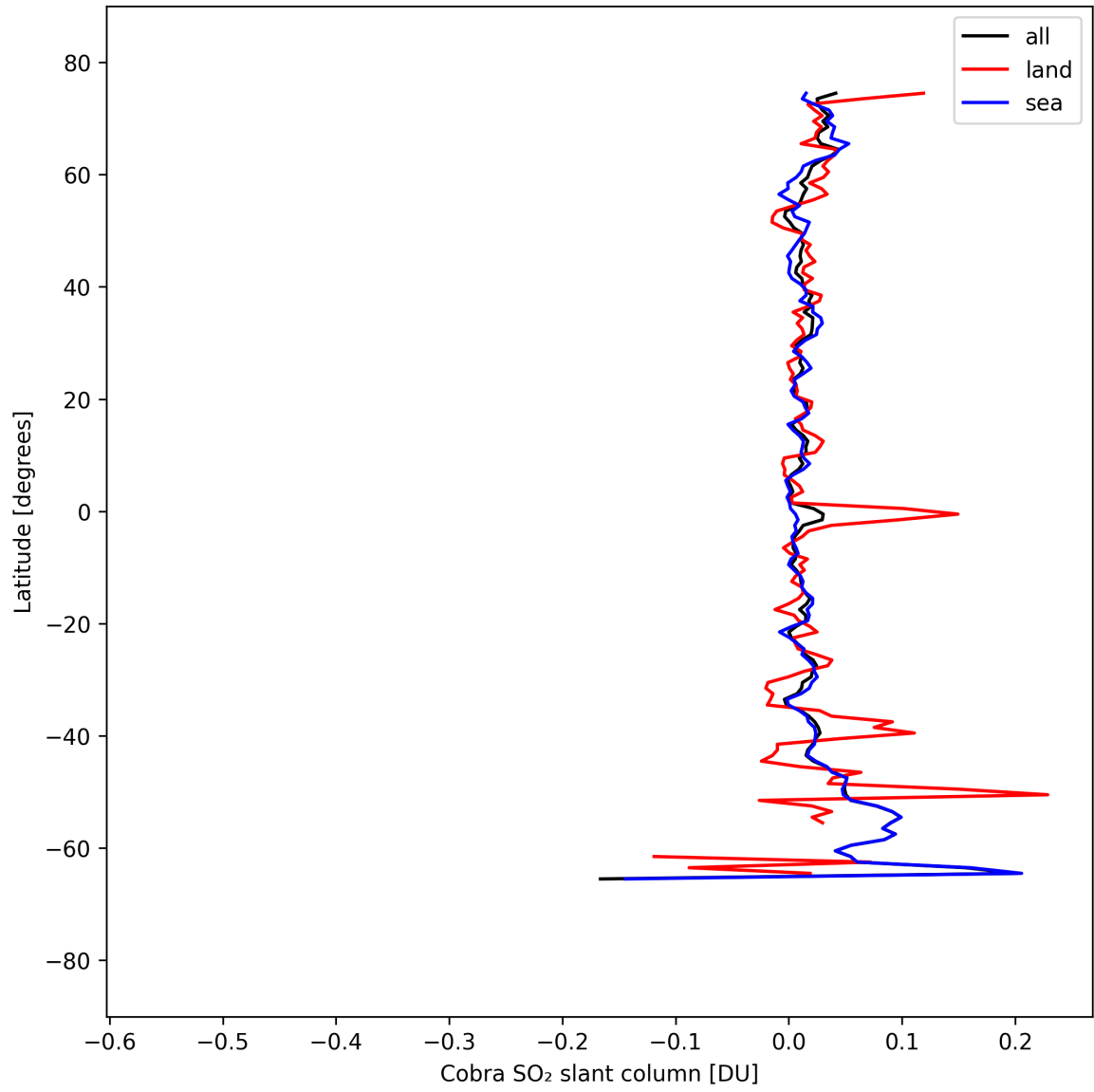
Figure 34: Zonal average of “Cobra SO 2 slant column” for 2025-09-11 to 2025-09-12.
