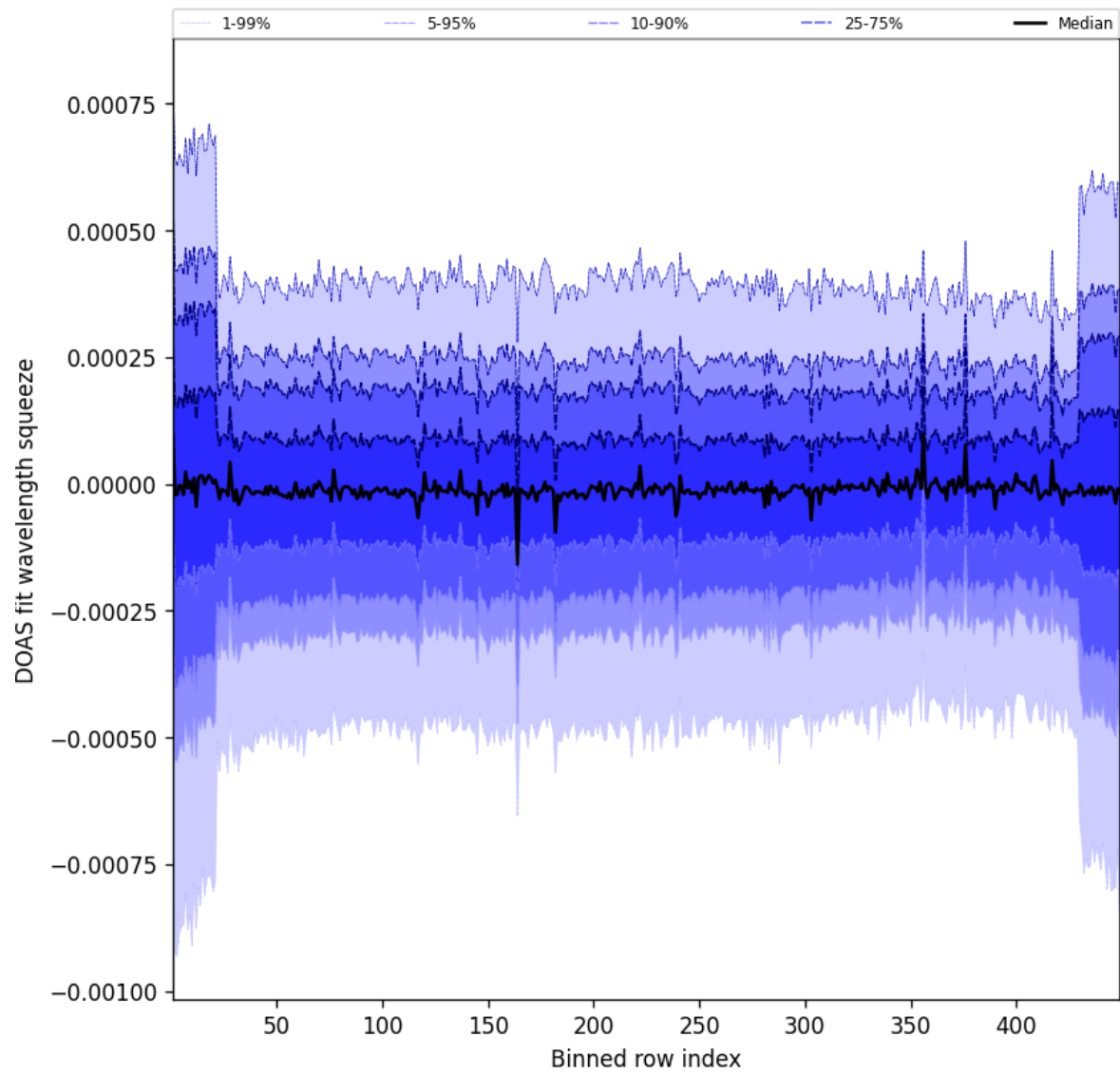
Figure 105: Along track statistics of “DOAS fit wavelength squeeze” for 2025-09-11 to 2025-09-12
