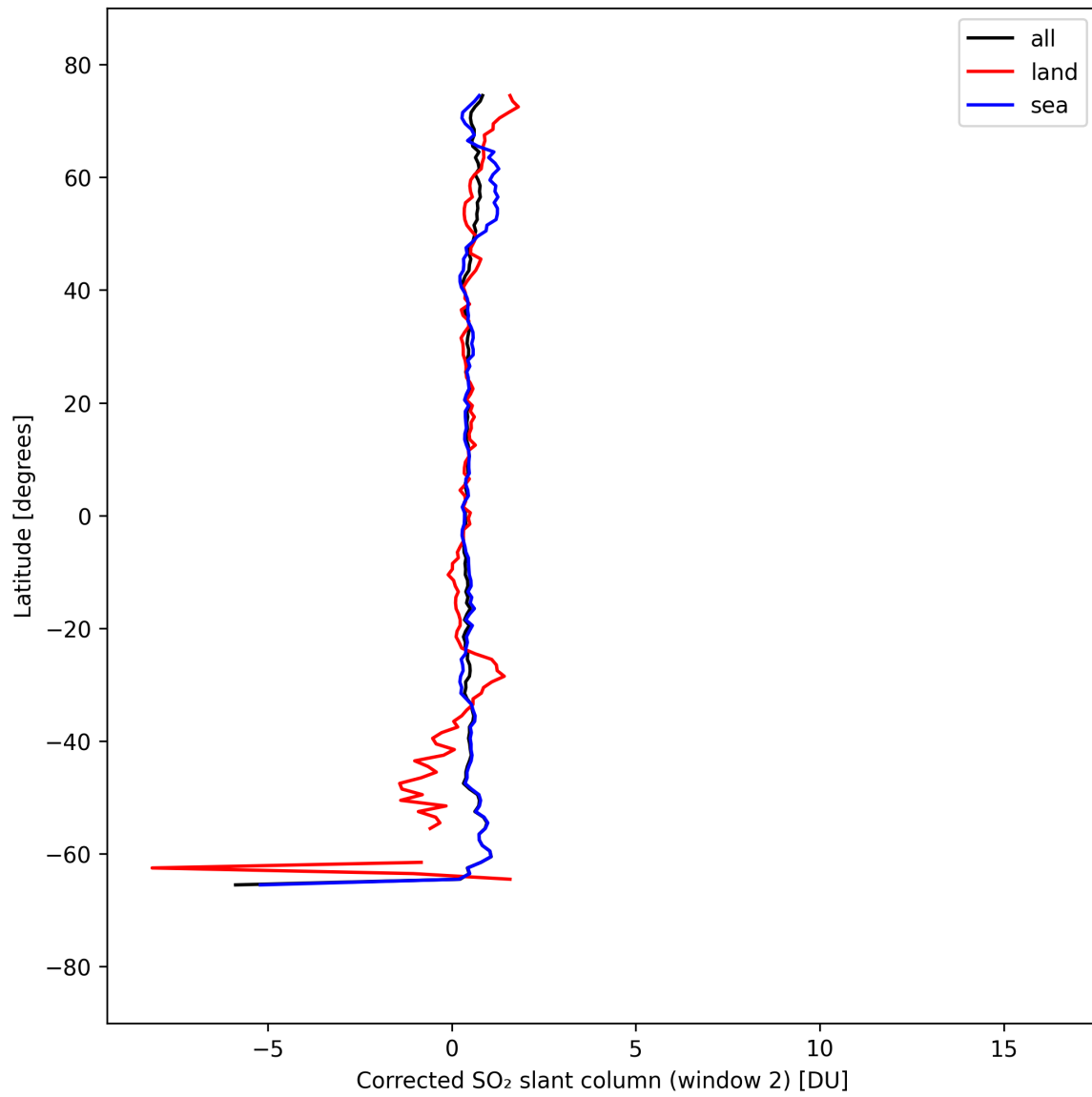
Figure 42: Zonal average of “Corrected SO 2 slant column (window 2)” for 2025-09-11 to 2025-09-12.
