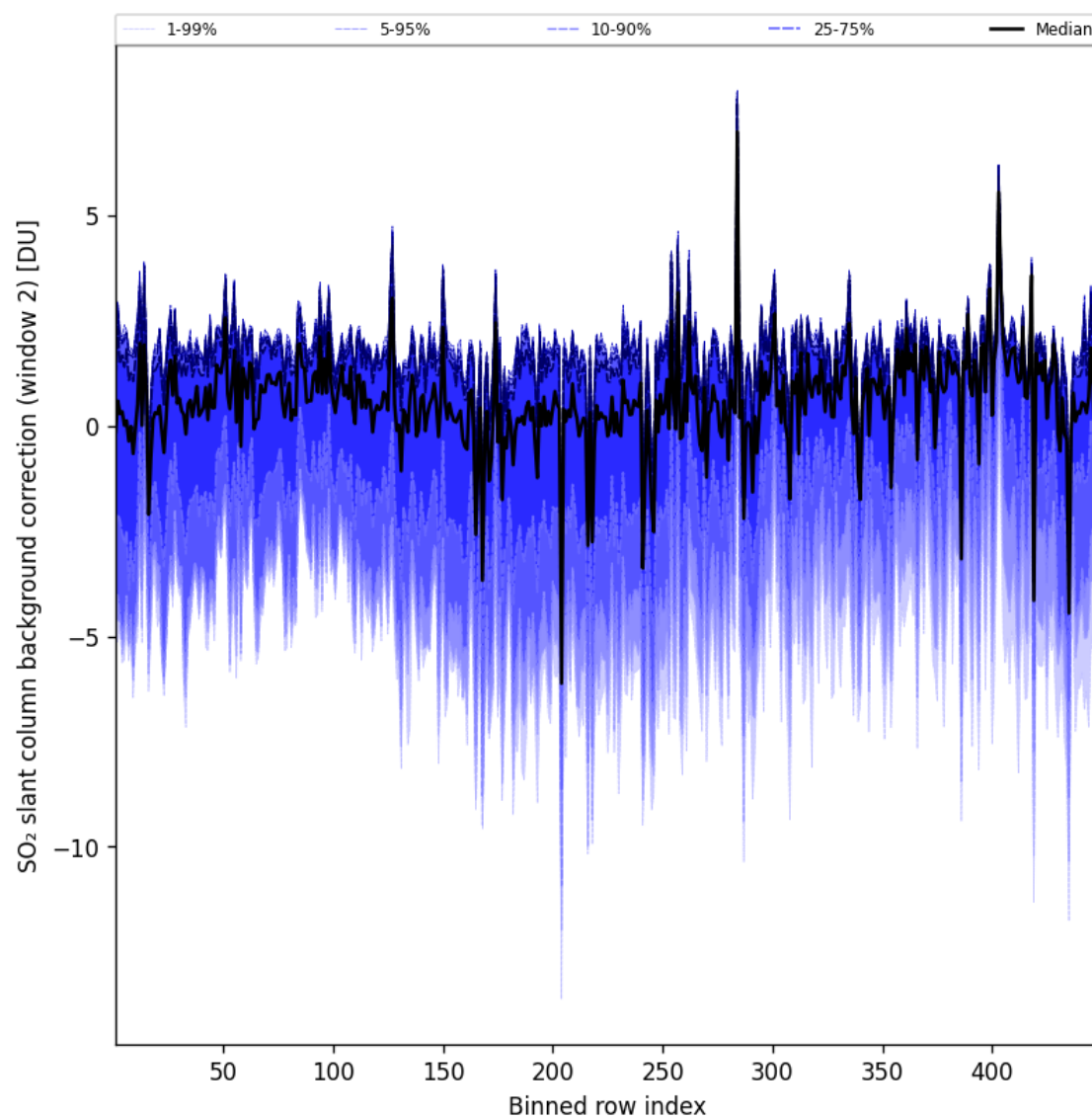
Figure 97: Along track statistics of “SO 2 slant column background correction (window 2)” for 2025-09-11 to 2025-09-12
