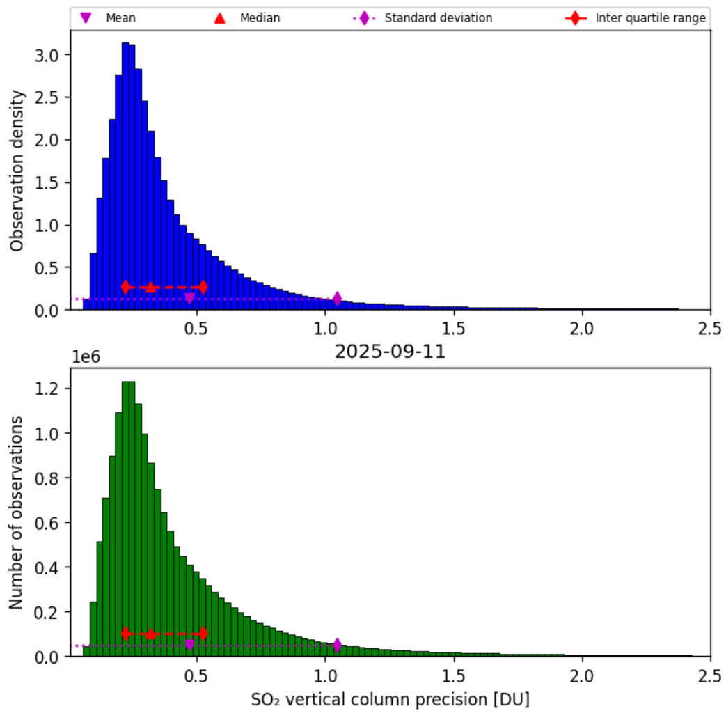
Figure 59: Histogram of “SO 2 vertical column precision” for 2025-09-11 to 2025-09-12
