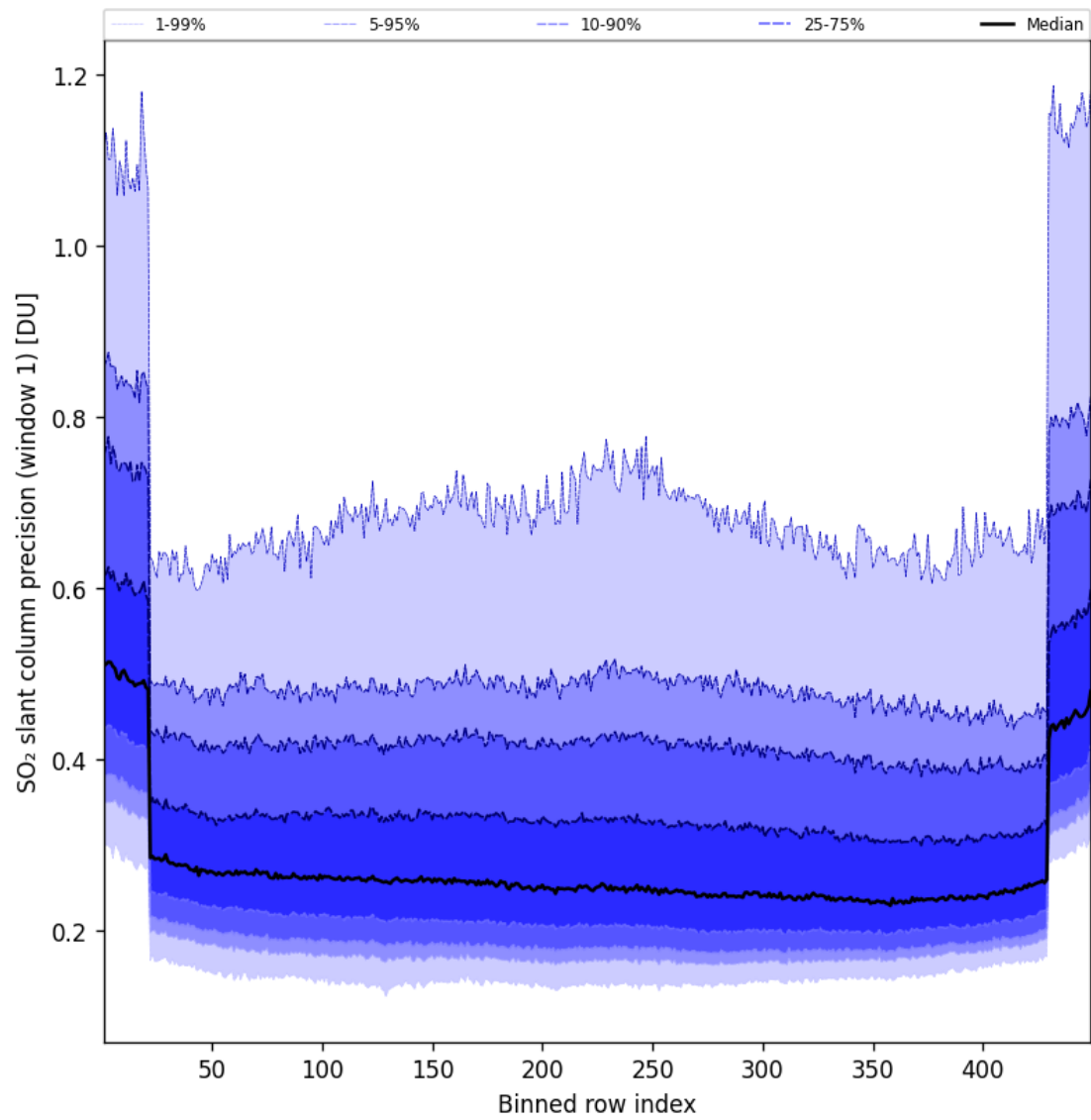
Figure 91: Along track statistics of “SO 2 slant column precision (window 1)” for 2025-09-11 to 2025-09-12
