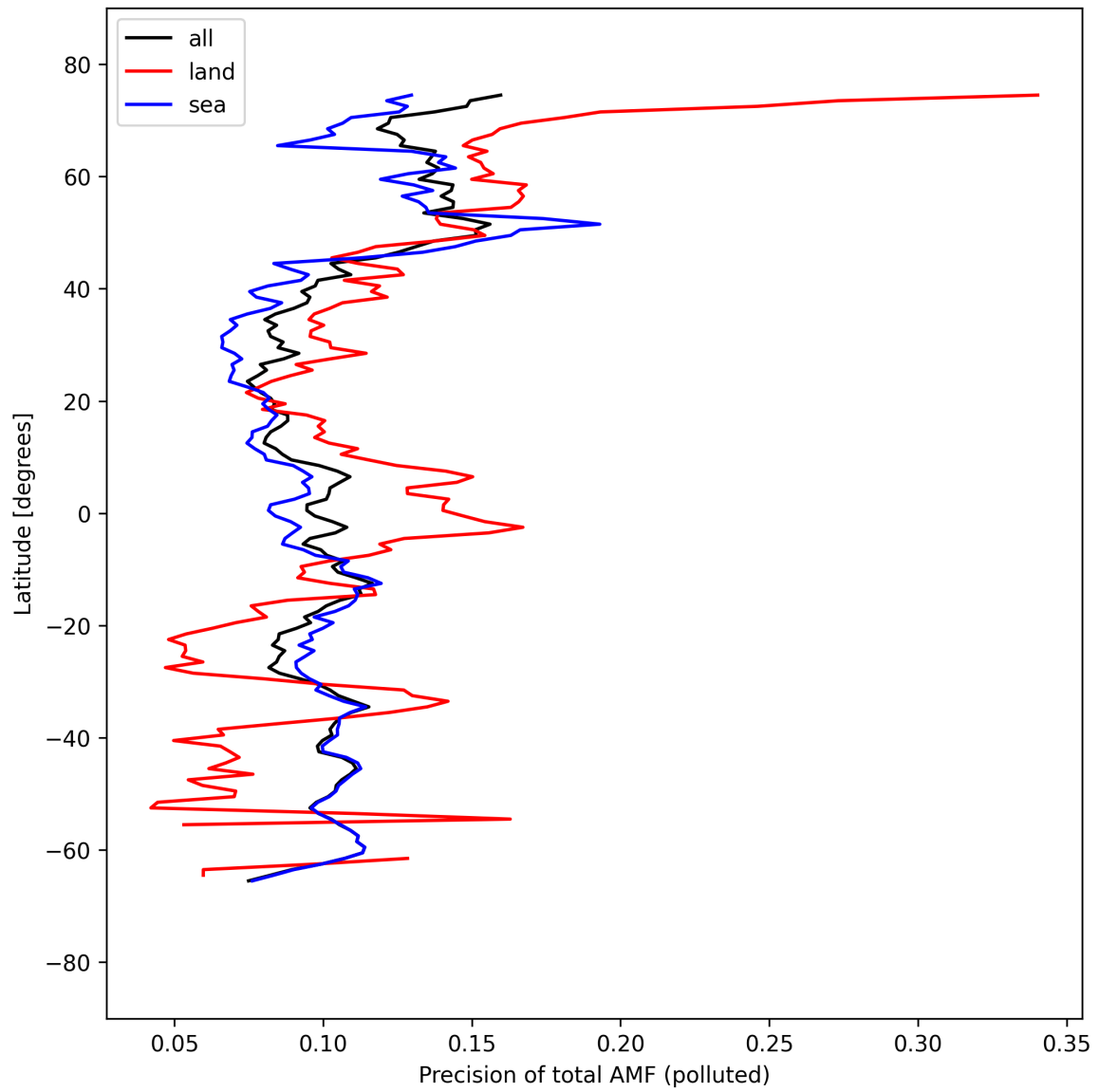
Figure 54: Zonal average of “Precision of total AMF (polluted)” for 2025-09-11 to 2025-09-12.
