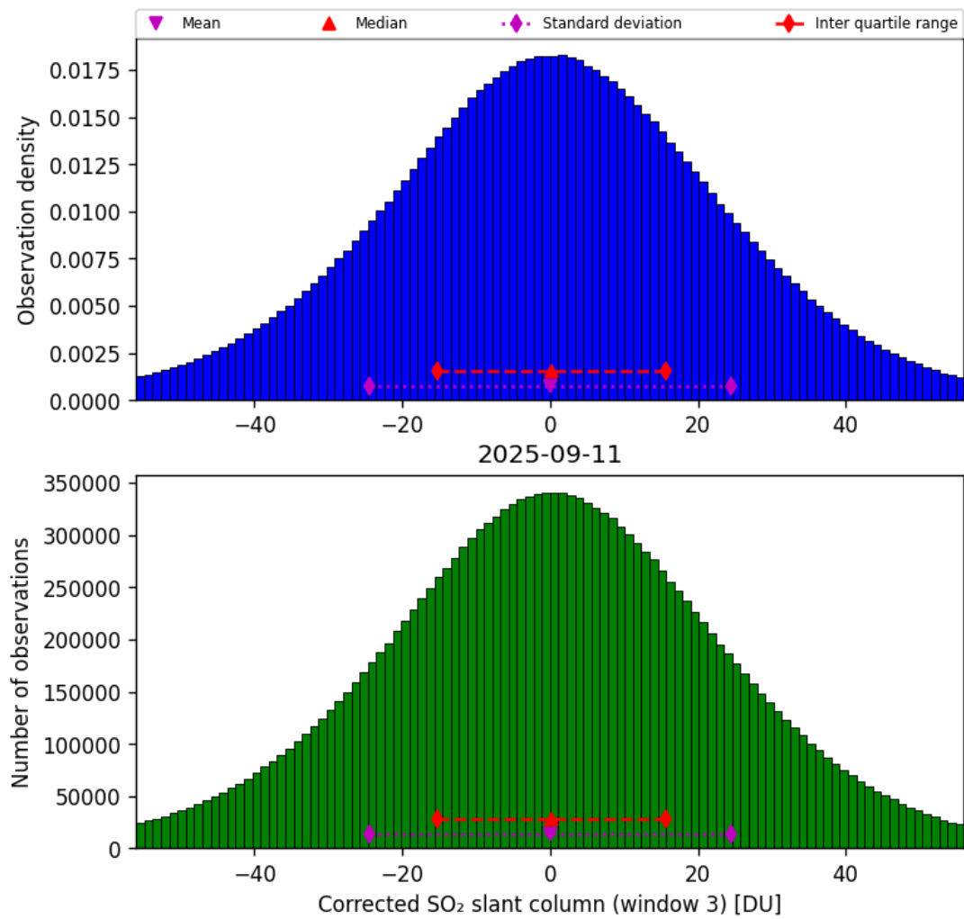
Figure 73: Histogram of “Corrected SO 2 slant column (window 3)” for 2025-09-11 to 2025-09-12
