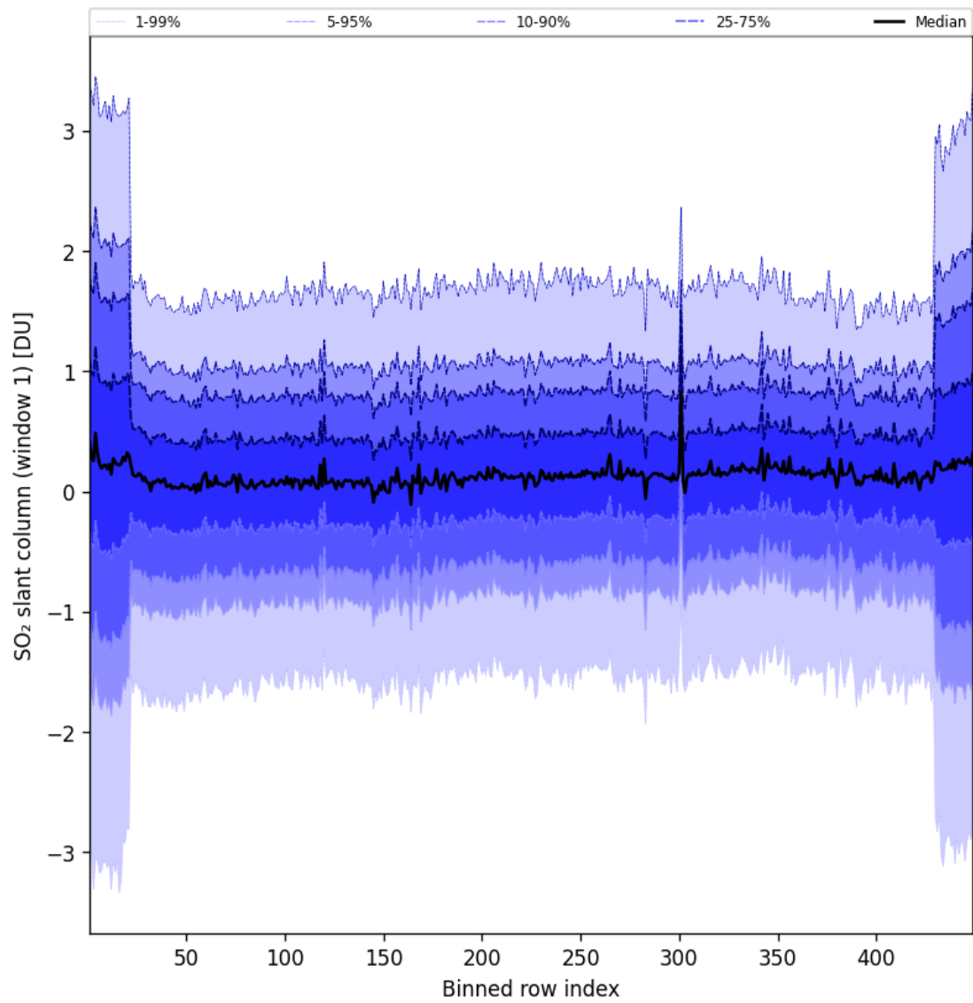
Figure 90: Along track statistics of “SO 2 slant column (window 1)” for 2025-09-11 to 2025-09-12
