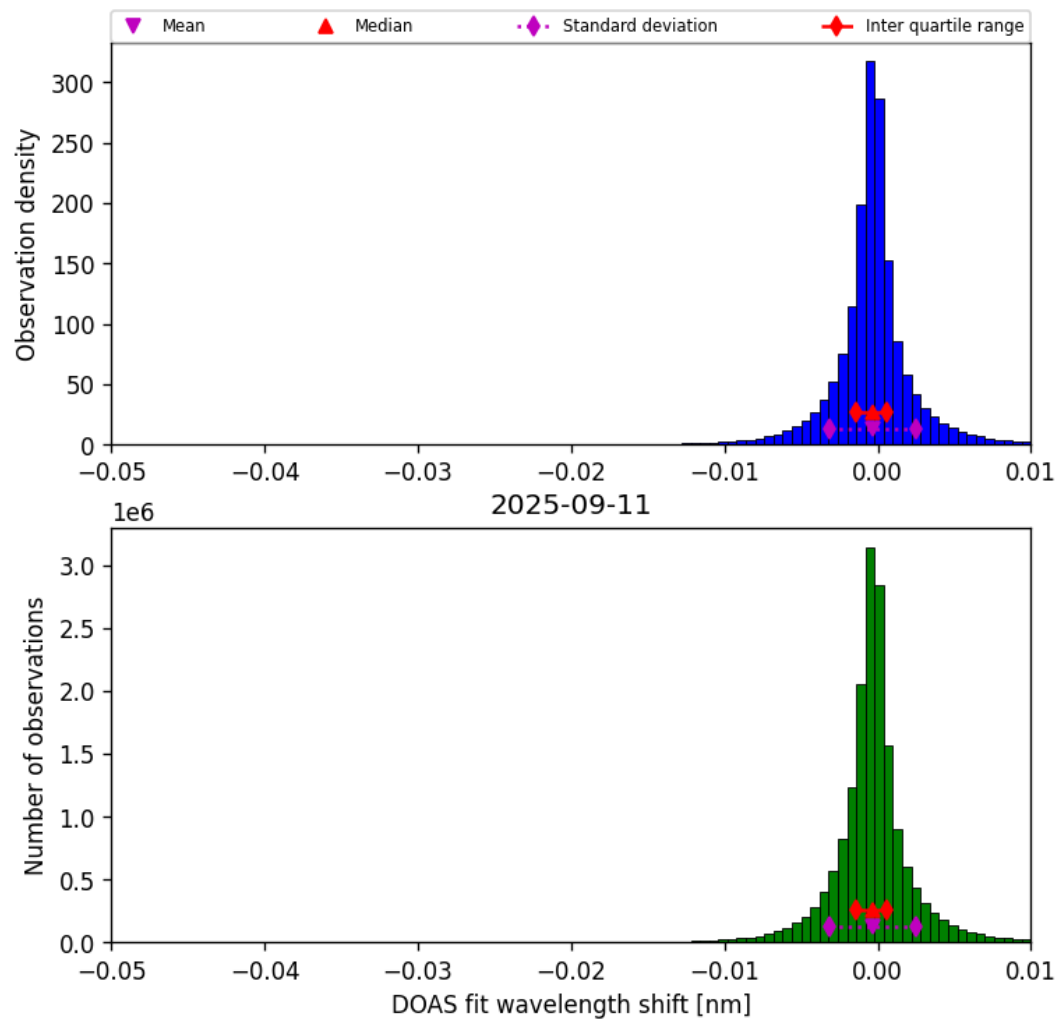
Figure 77: Histogram of “DOAS fit wavelength shift” for 2025-09-11 to 2025-09-12
