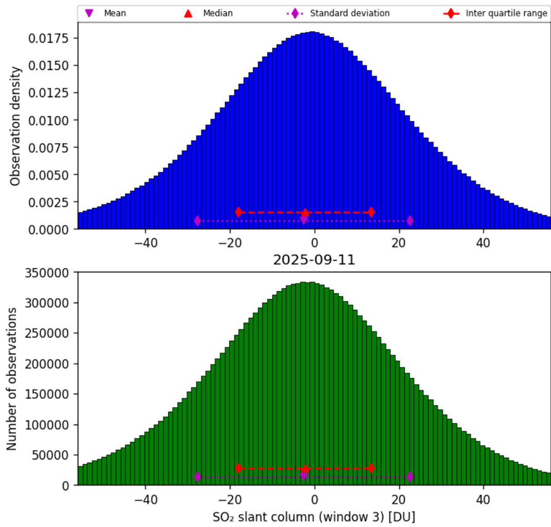
Figure 71: Histogram of “SO 2 slant column (window 3)” for 2025-09-11 to 2025-09-12
