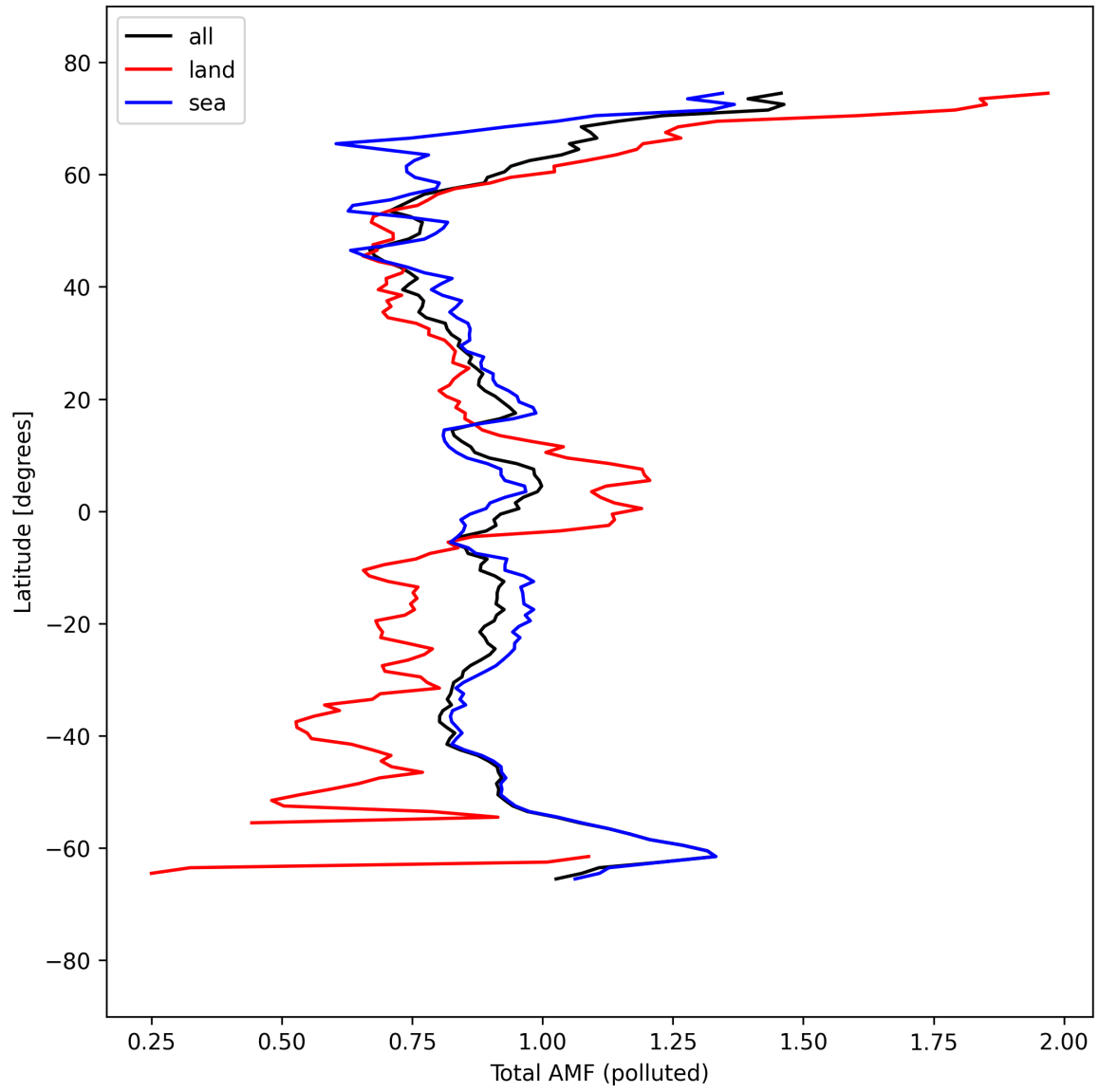
Figure 53: Zonal average of “Total AMF (polluted)” for 2025-09-11 to 2025-09-12.
