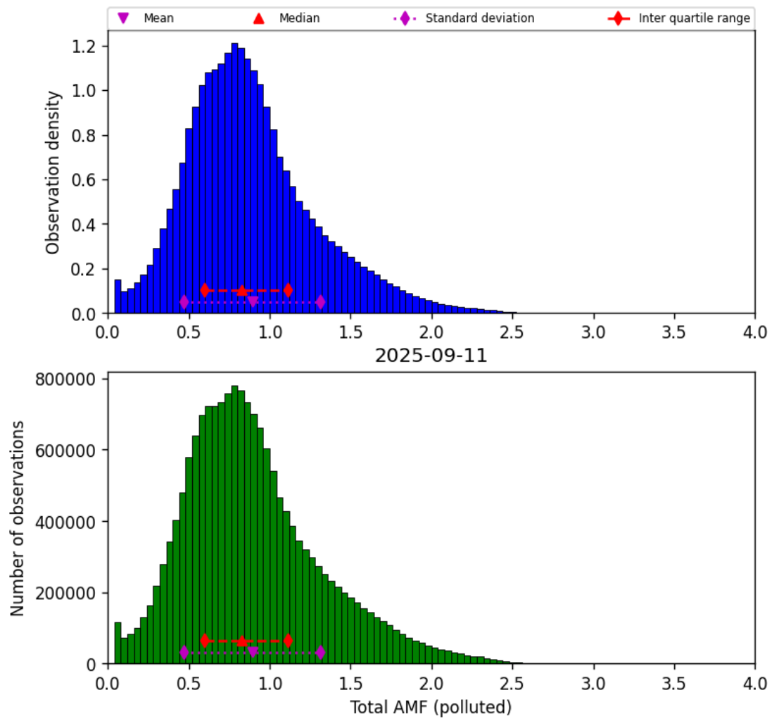
Figure 80: Histogram of “Total AMF (polluted)” for 2025-09-11 to 2025-09-12
