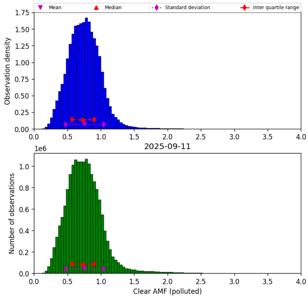
Figure 82: Histogram of “Clear AMF (polluted)” for 2025-09-11 to 2025-09-12
