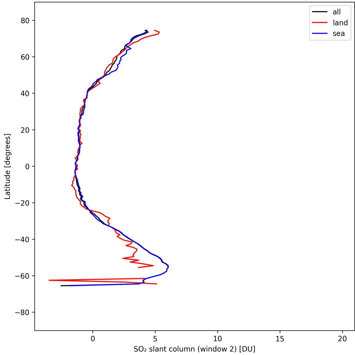
Figure 40: Zonal average of “SO 2 slant column (window 2)” for 2025-09-11 to 2025-09-12.
