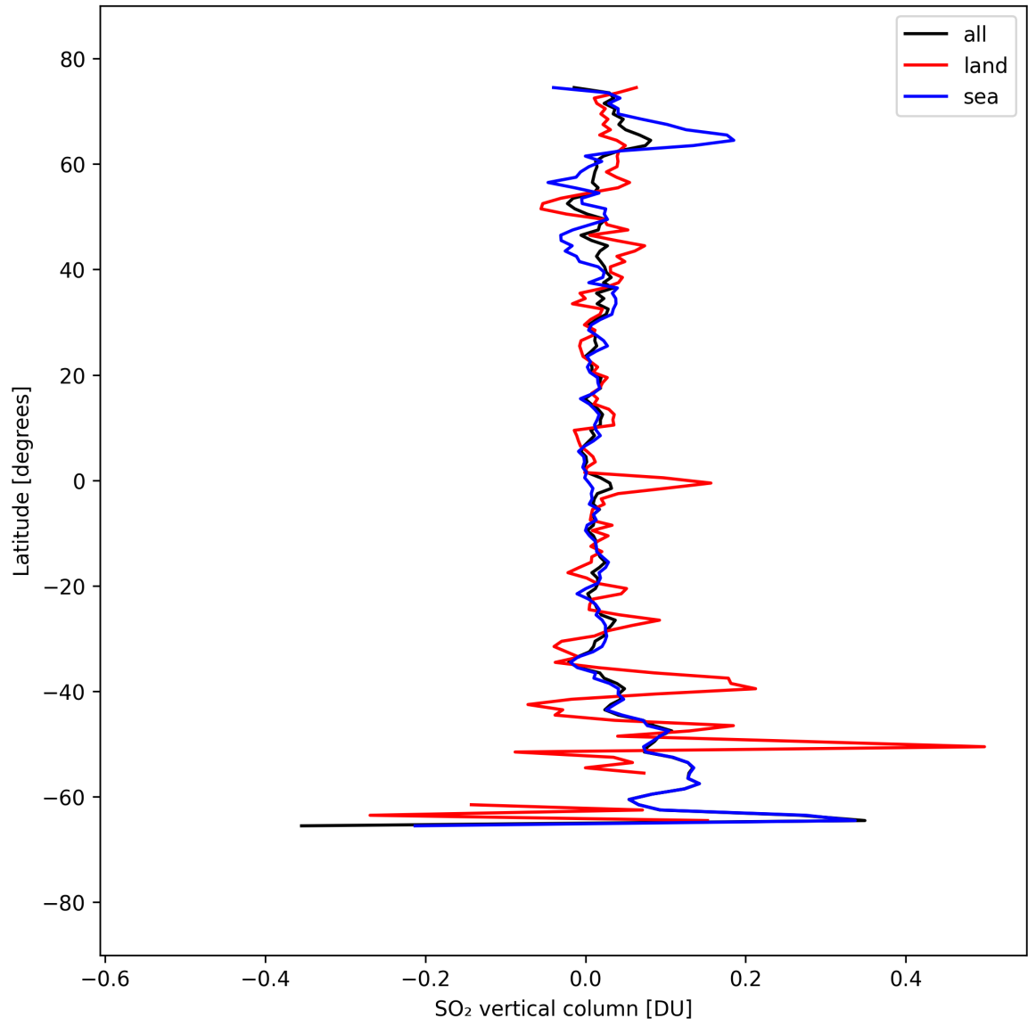
Figure 31: Zonal average of “SO 2 vertical column” for 2025-09-11 to 2025-09-12.
