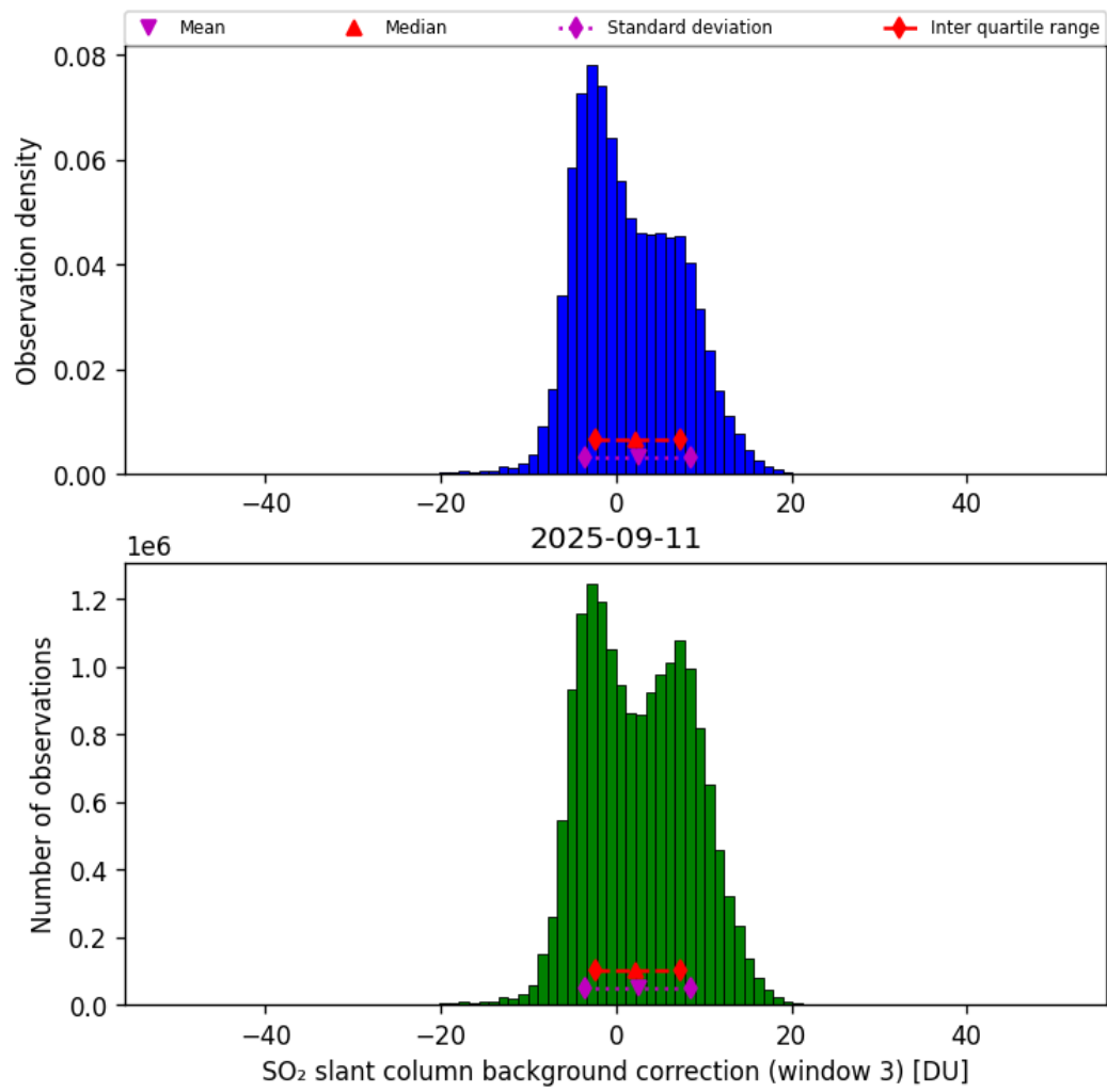
Figure 74: Histogram of “SO 2 slant column background correction (window 3)” for 2025-09-11 to 2025-09-12
