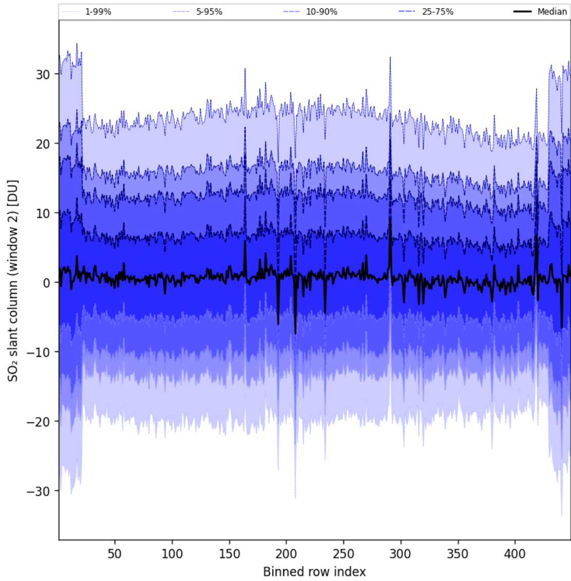
Figure 94: Along track statistics of “SO 2 slant column (window 2)” for 2025-09-11 to 2025-09-12
