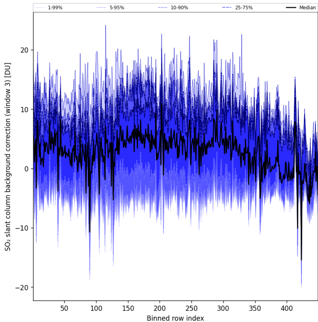
Figure 101: Along track statistics of “SO 2 slant column background correction (window 3)” for 2025-09-11 to 2025-09-12
