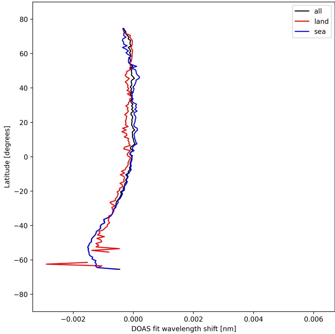
Figure 50: Zonal average of “DOAS fit wavelength shift” for 2025-09-11 to 2025-09-12.
