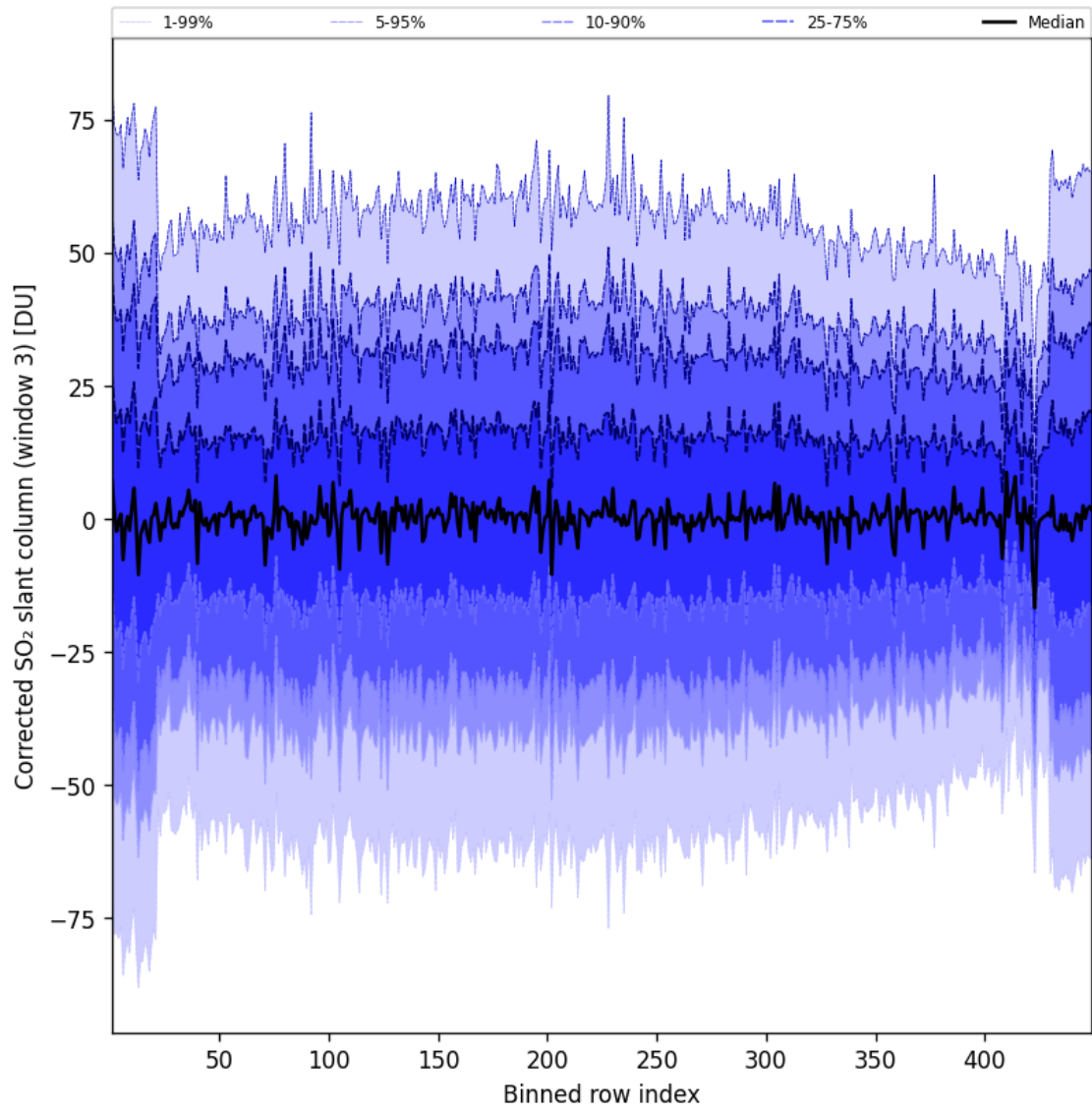
Figure 100: Along track statistics of “Corrected SO 2 slant column (window 3)” for 2025-09-11 to 2025-09-12
