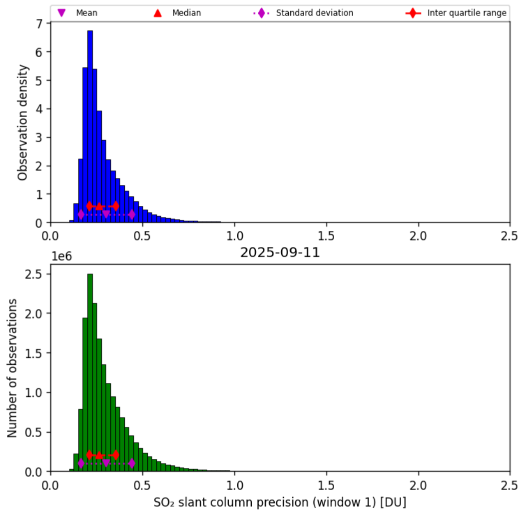
Figure 64: Histogram of “SO 2 slant column precision (window 1)” for 2025-09-11 to 2025-09-12
