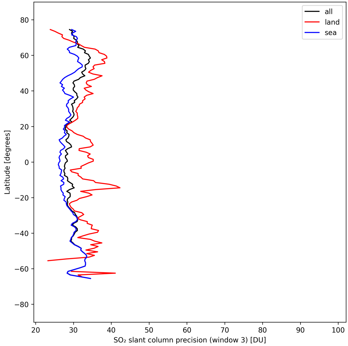
Figure 45: Zonal average of “SO 2 slant column precision (window 3)” for 2025-09-11 to 2025-09-12.
