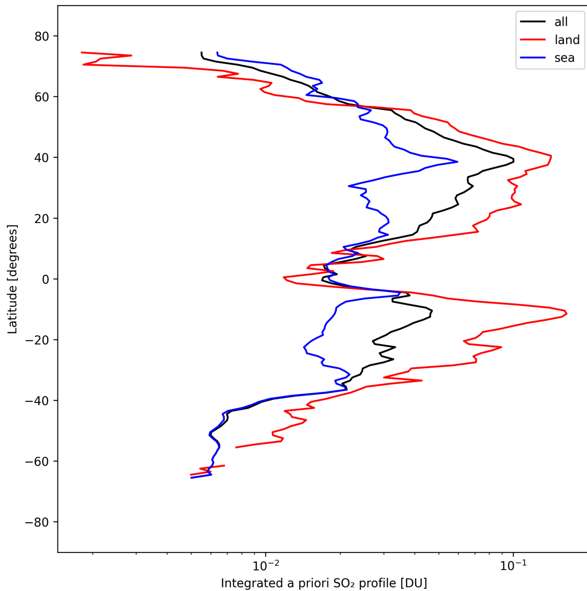
Figure 49: Zonal average of “Integrated a priori SO 2 profile” for 2025-09-11 to 2025-09-12.
