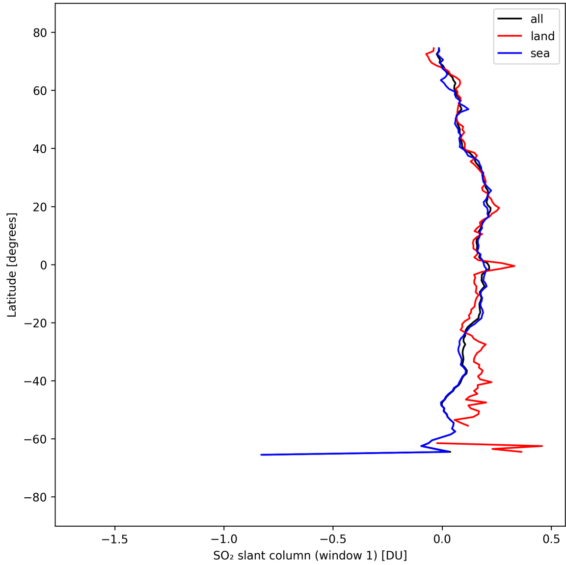
Figure 36: Zonal average of “SO 2 slant column (window 1)” for 2025-09-11 to 2025-09-12.
