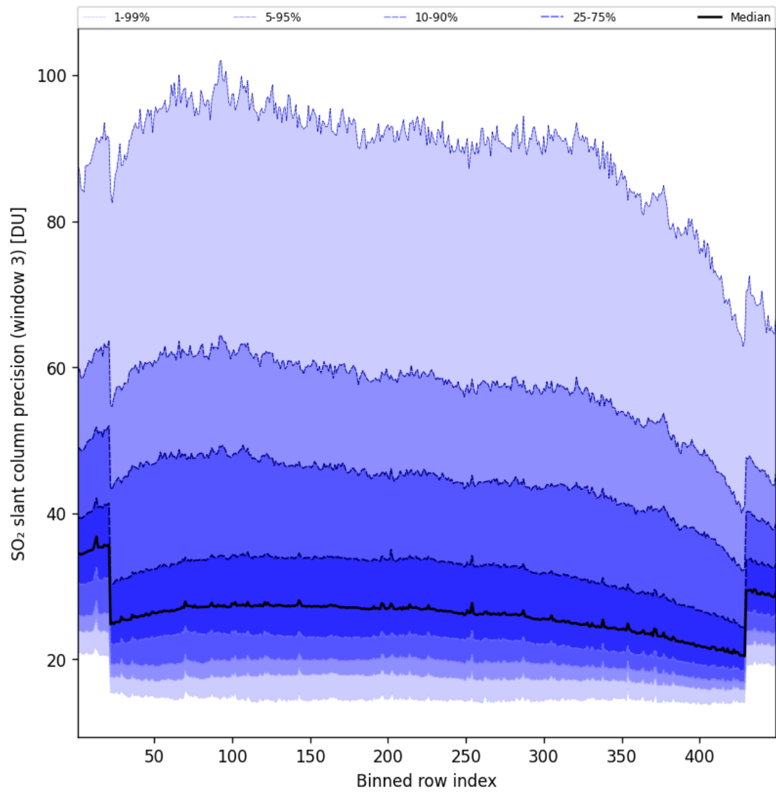
Figure 99: Along track statistics of “SO 2 slant column precision (window 3)” for 2025-09-11 to 2025-09-12
