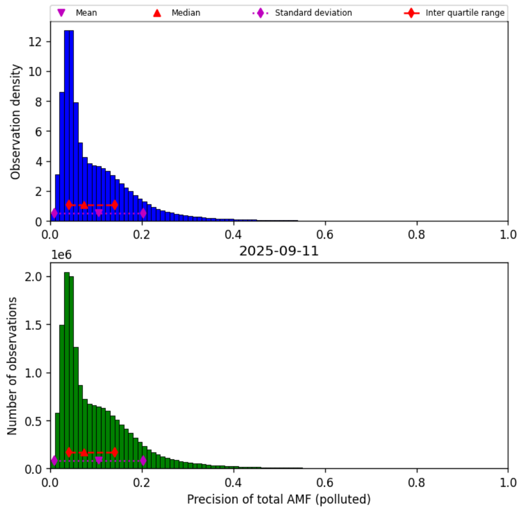
Figure 81: Histogram of “Precision of total AMF (polluted)” for 2025-09-11 to 2025-09-12
