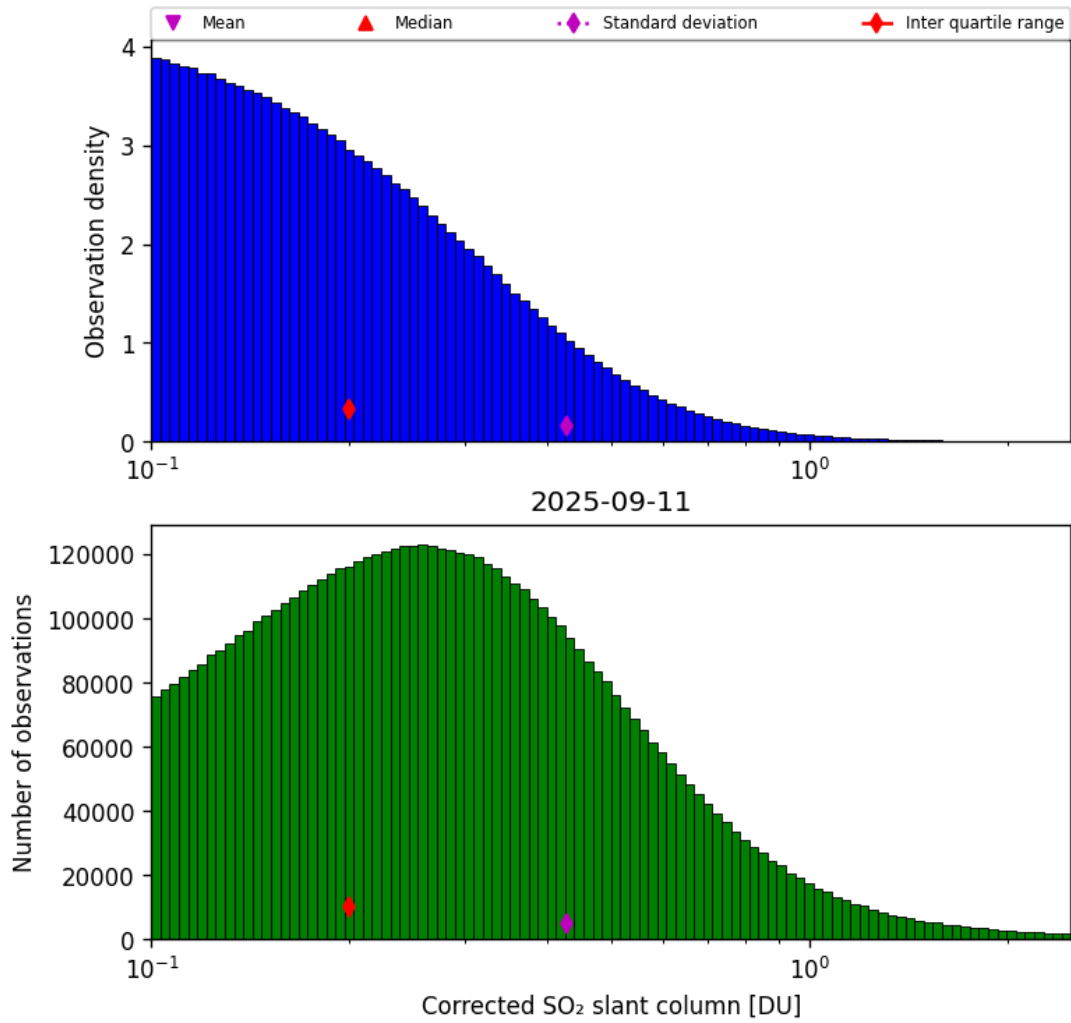
Figure 60: Histogram of “Corrected SO 2 slant column” for 2025-09-11 to 2025-09-12
