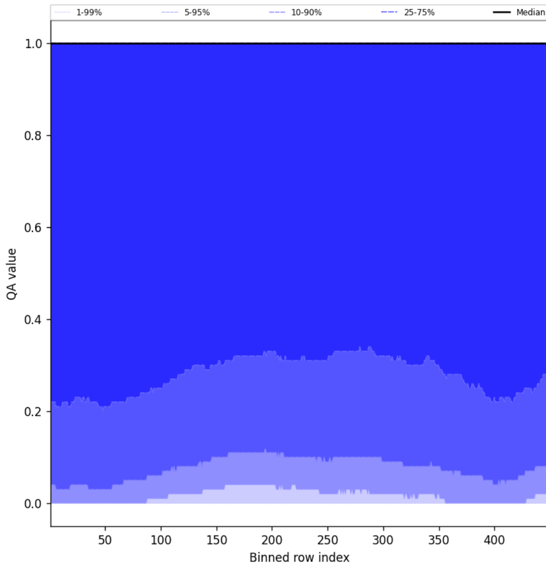
Figure 84: Along track statistics of “QA value” for 2025-09-11 to 2025-09-12
