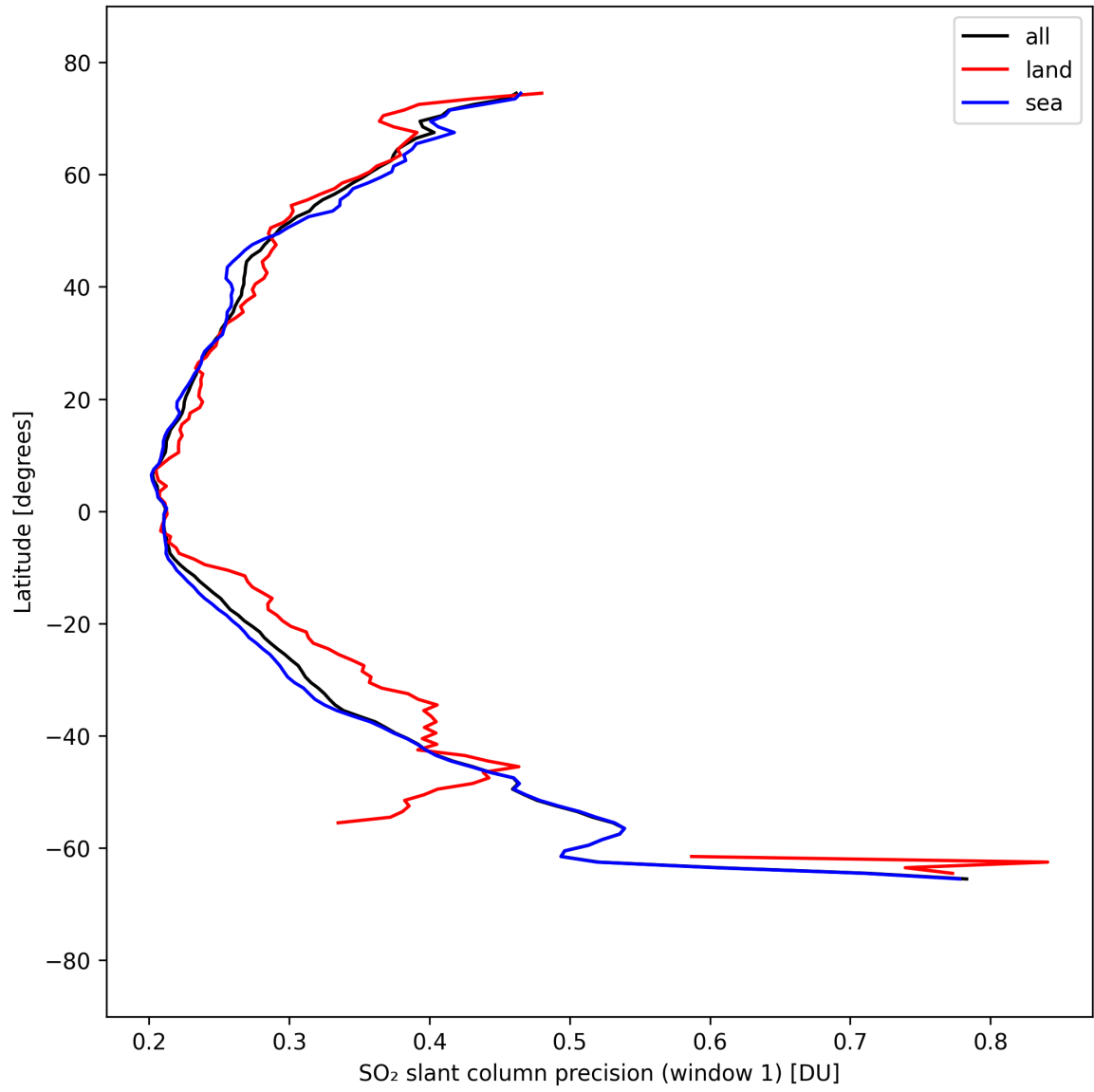
Figure 37: Zonal average of “SO 2 slant column precision (window 1)” for 2025-09-11 to 2025-09-12.
