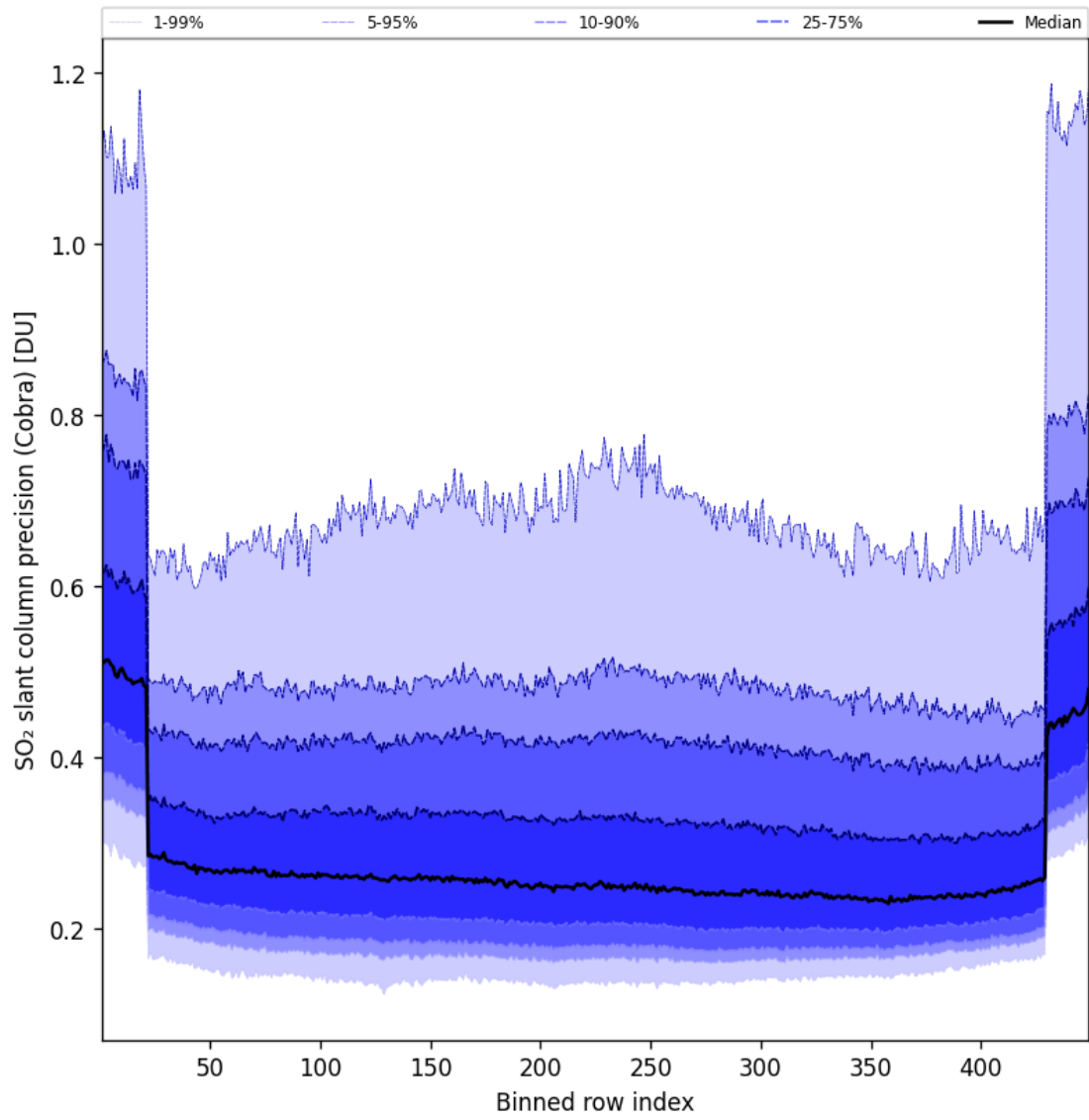
Figure 89: Along track statistics of “SO 2 slant column precision (Cobra)” for 2025-09-11 to 2025-09-12
