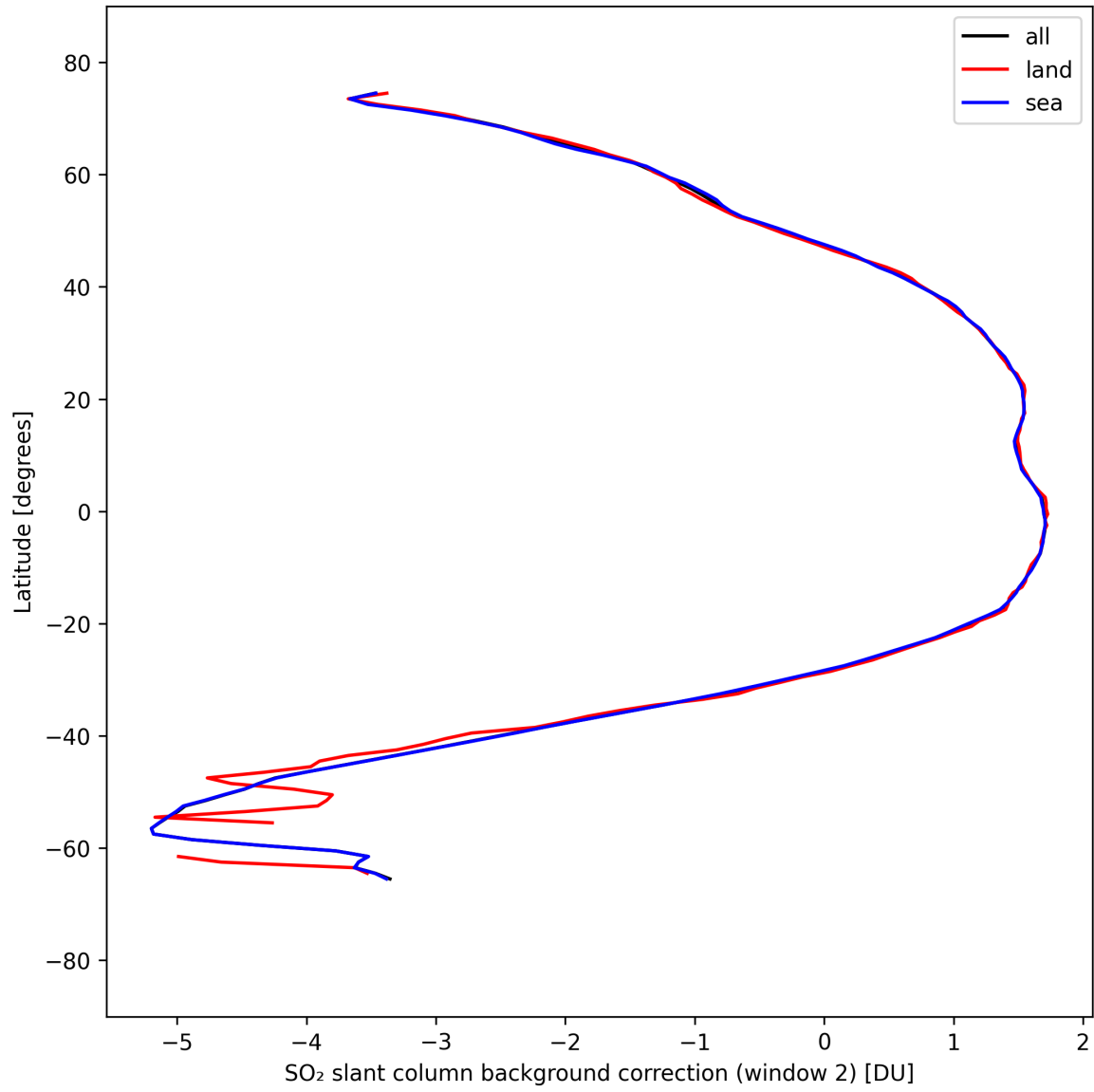
Figure 43: Zonal average of “SO 2 slant column background correction (window 2)” for 2025-09-11 to 2025-09-12.
