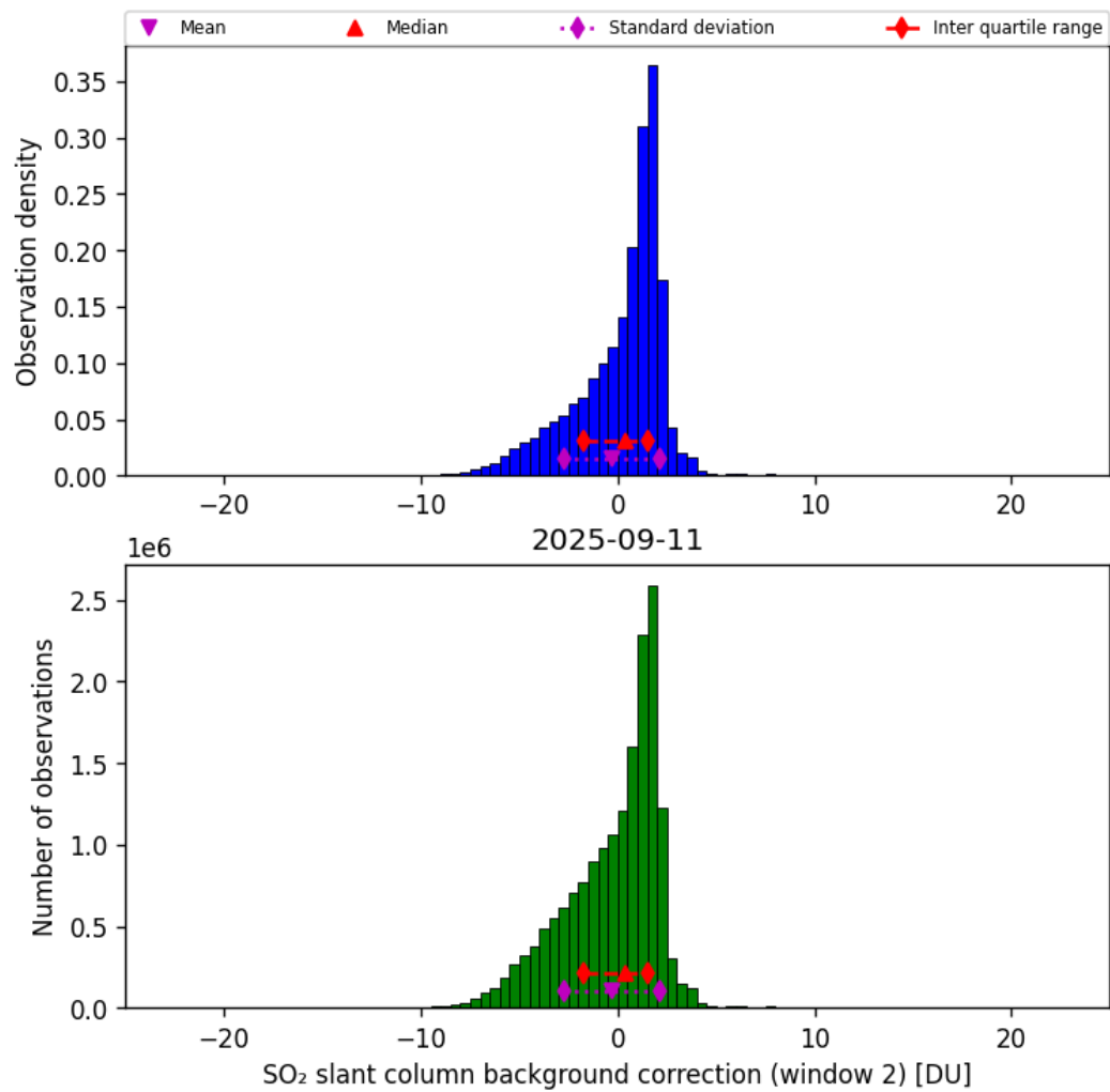
Figure 70: Histogram of “SO 2 slant column background correction (window 2)” for 2025-09-11 to 2025-09-12
