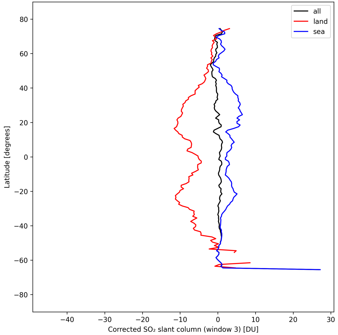
Figure 46: Zonal average of “Corrected SO 2 slant column (window 3)” for 2025-09-11 to 2025-09-12.
