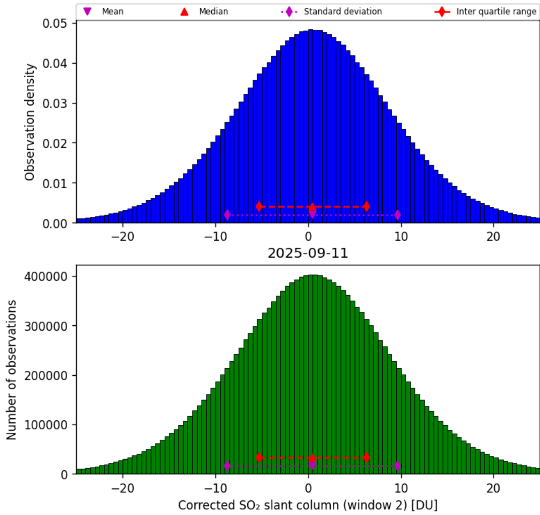
Figure 69: Histogram of “Corrected SO 2 slant column (window 2)” for 2025-09-11 to 2025-09-12
