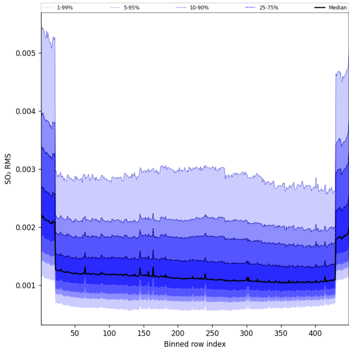
Figure 106: Along track statistics of “SO 2 RMS” for 2025-09-11 to 2025-09-12
