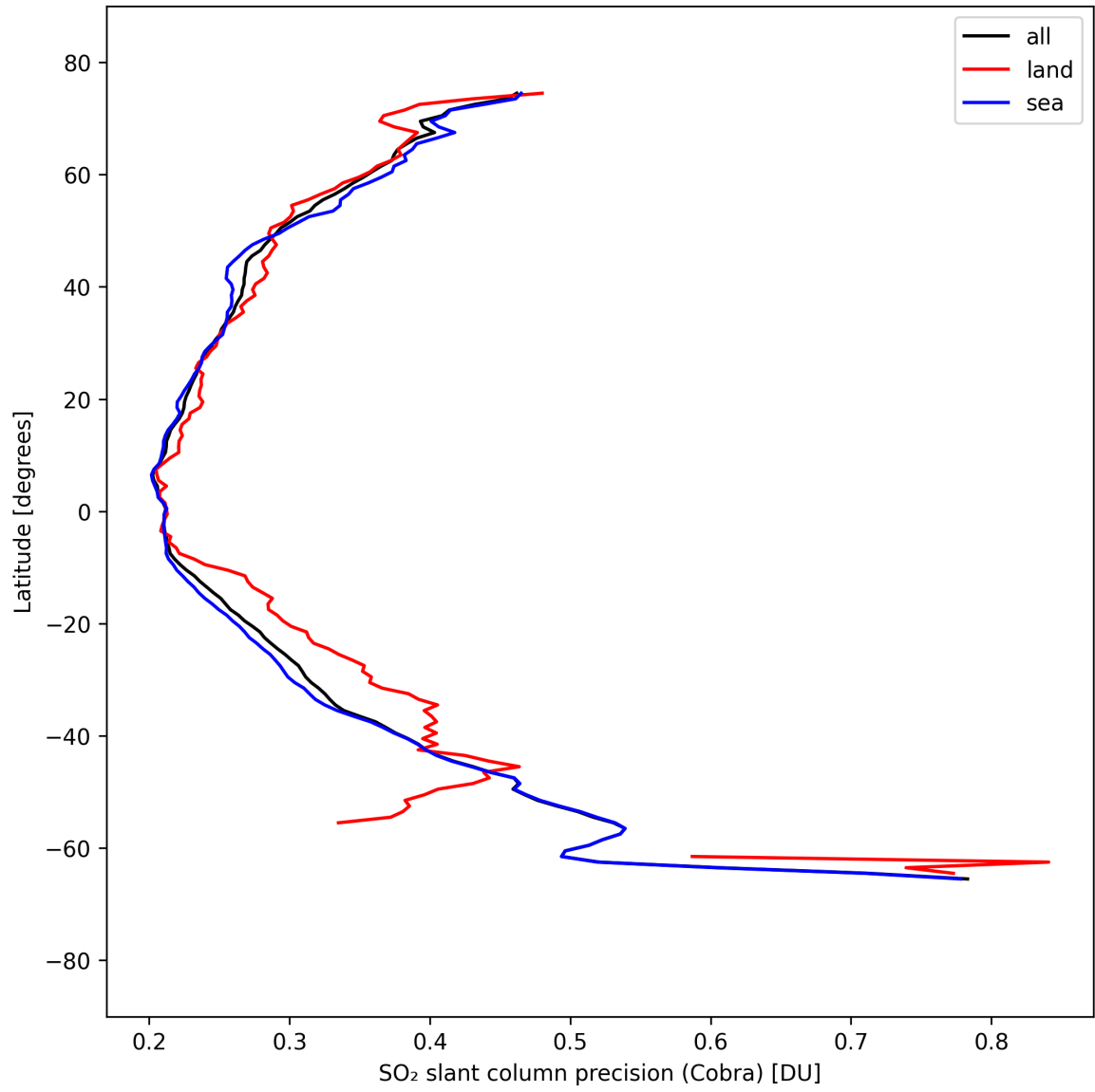
Figure 35: Zonal average of “SO 2 slant column precision (Cobra)” for 2025-09-11 to 2025-09-12.
