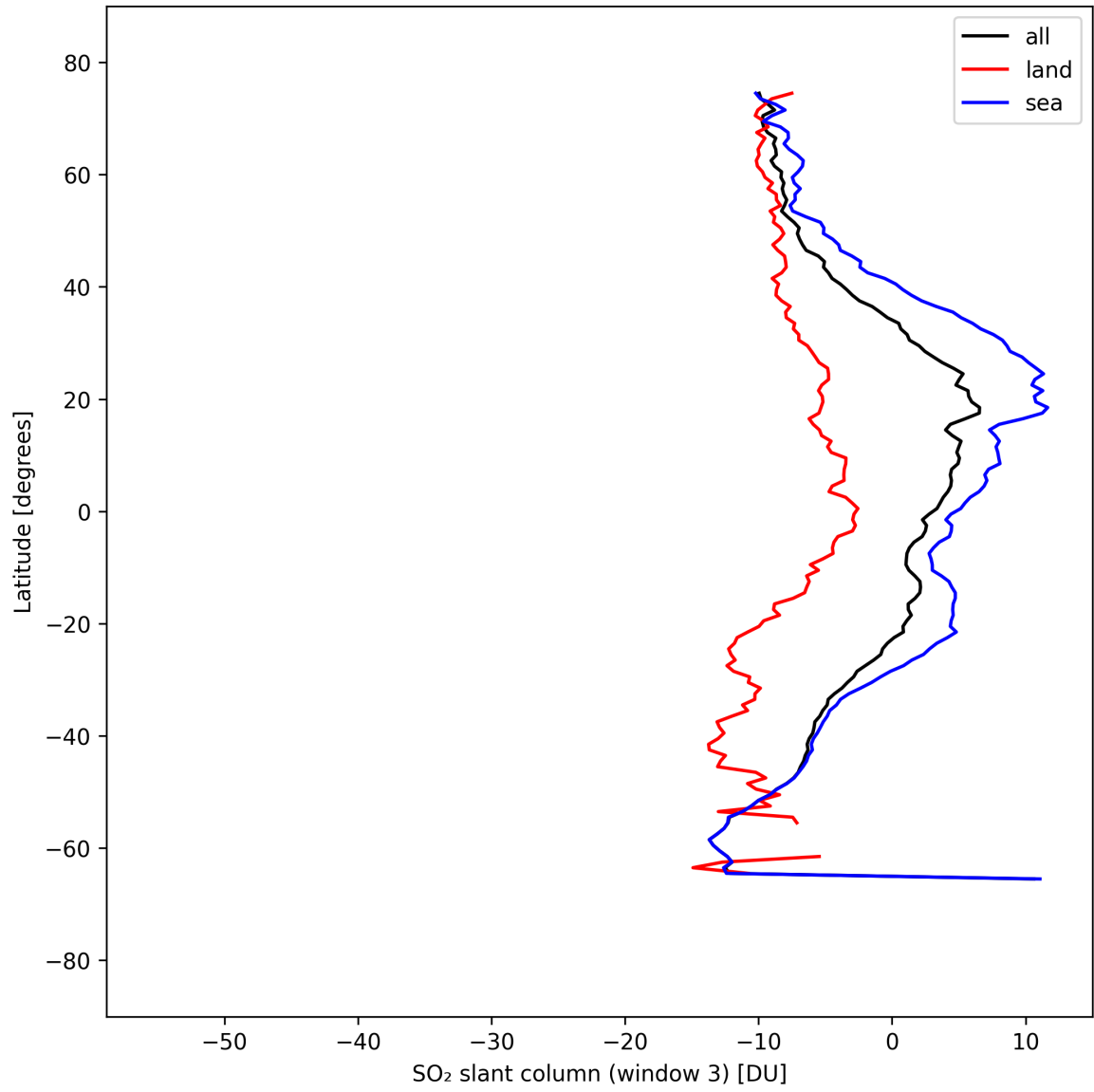
Figure 44: Zonal average of “SO 2 slant column (window 3)” for 2025-09-11 to 2025-09-12.
