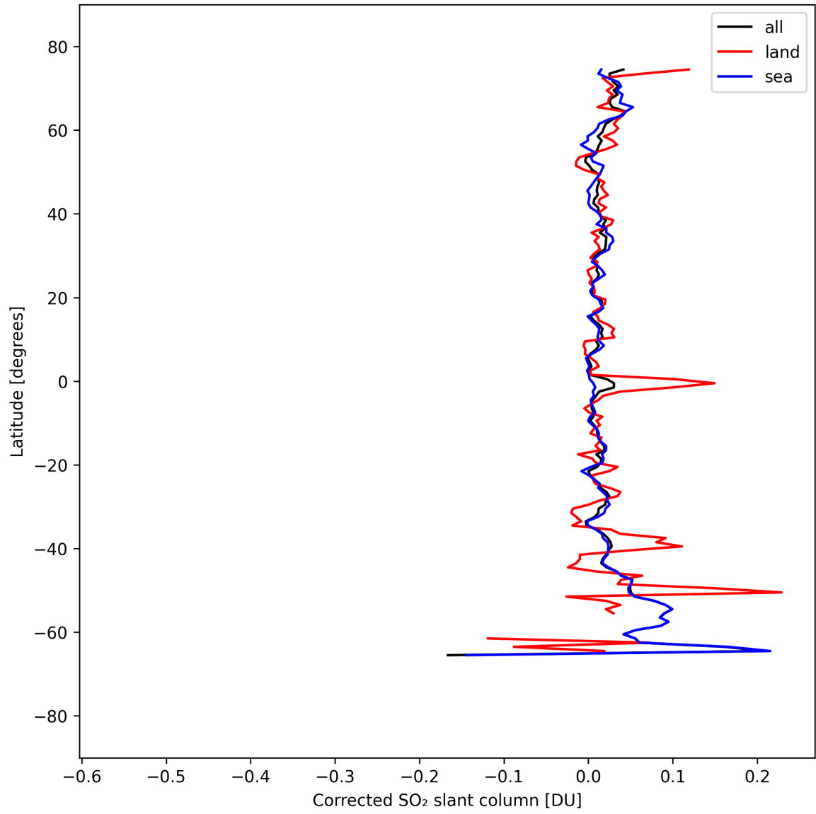
Figure 33: Zonal average of “Corrected SO 2 slant column” for 2025-09-11 to 2025-09-12.
