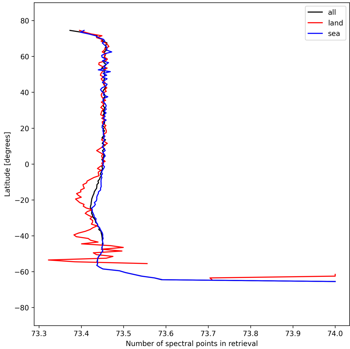
Figure 56: Zonal average of “Number of spectral points in retrieval” for 2025-09-11 to 2025-09-12.
