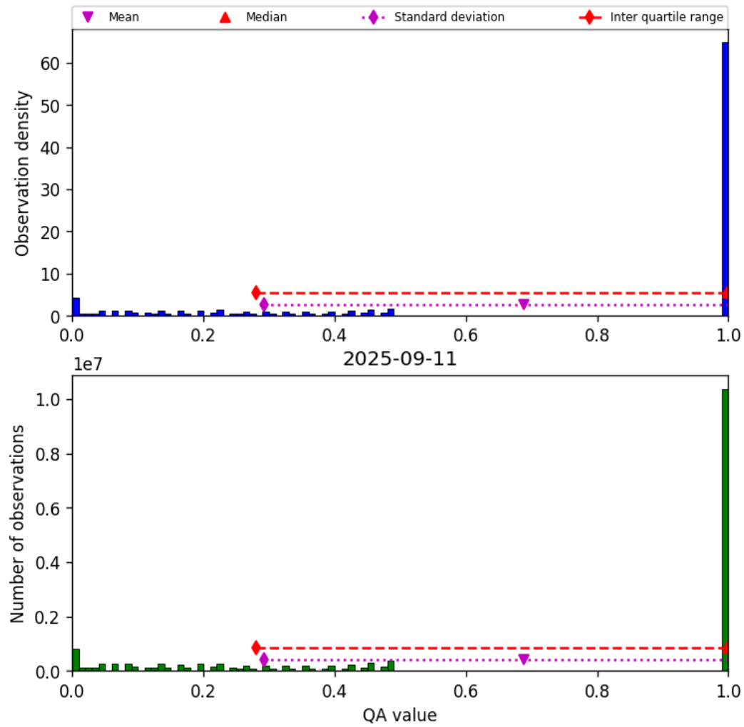
Figure 57: Histogram of “QA value” for 2025-09-11 to 2025-09-12
