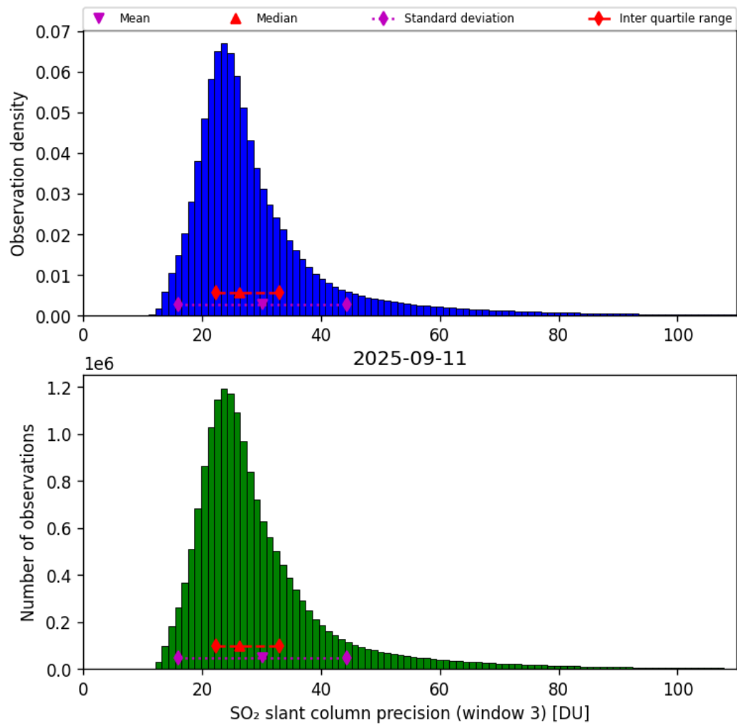
Figure 72: Histogram of “SO 2 slant column precision (window 3)” for 2025-09-11 to 2025-09-12
