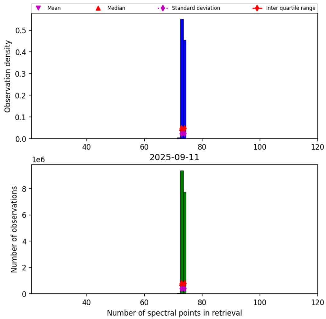
Figure 83: Histogram of “Number of spectral points in retrieval” for 2025-09-11 to 2025-09-12
