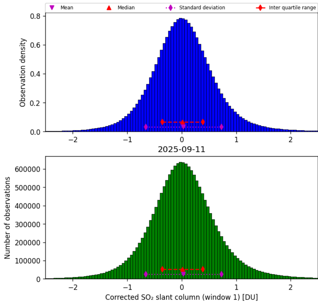
Figure 65: Histogram of “Corrected SO 2 slant column (window 1)” for 2025-09-11 to 2025-09-12
