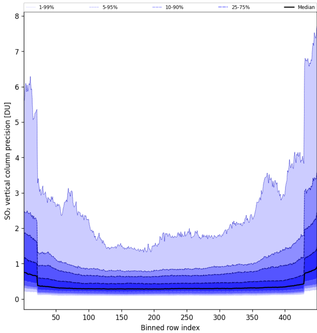
Figure 86: Along track statistics of “SO 2 vertical column precision” for 2025-09-11 to 2025-09-12
