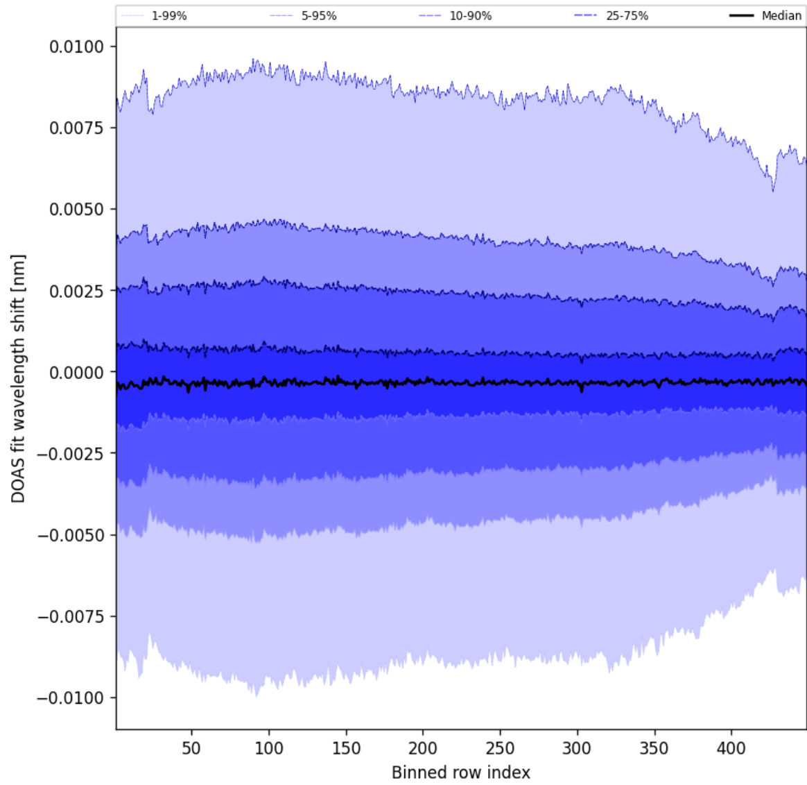
Figure 104: Along track statistics of “DOAS fit wavelength shift” for 2025-09-11 to 2025-09-12
