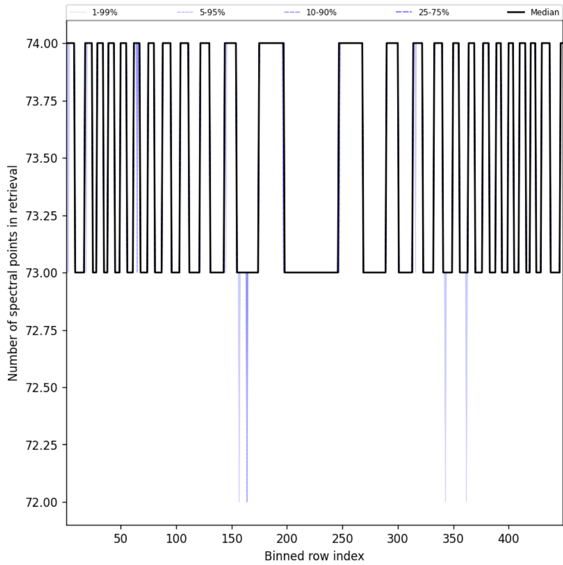
Figure 110: Along track statistics of “Number of spectral points in retrieval” for 2025-09-11 to 2025-09-12
