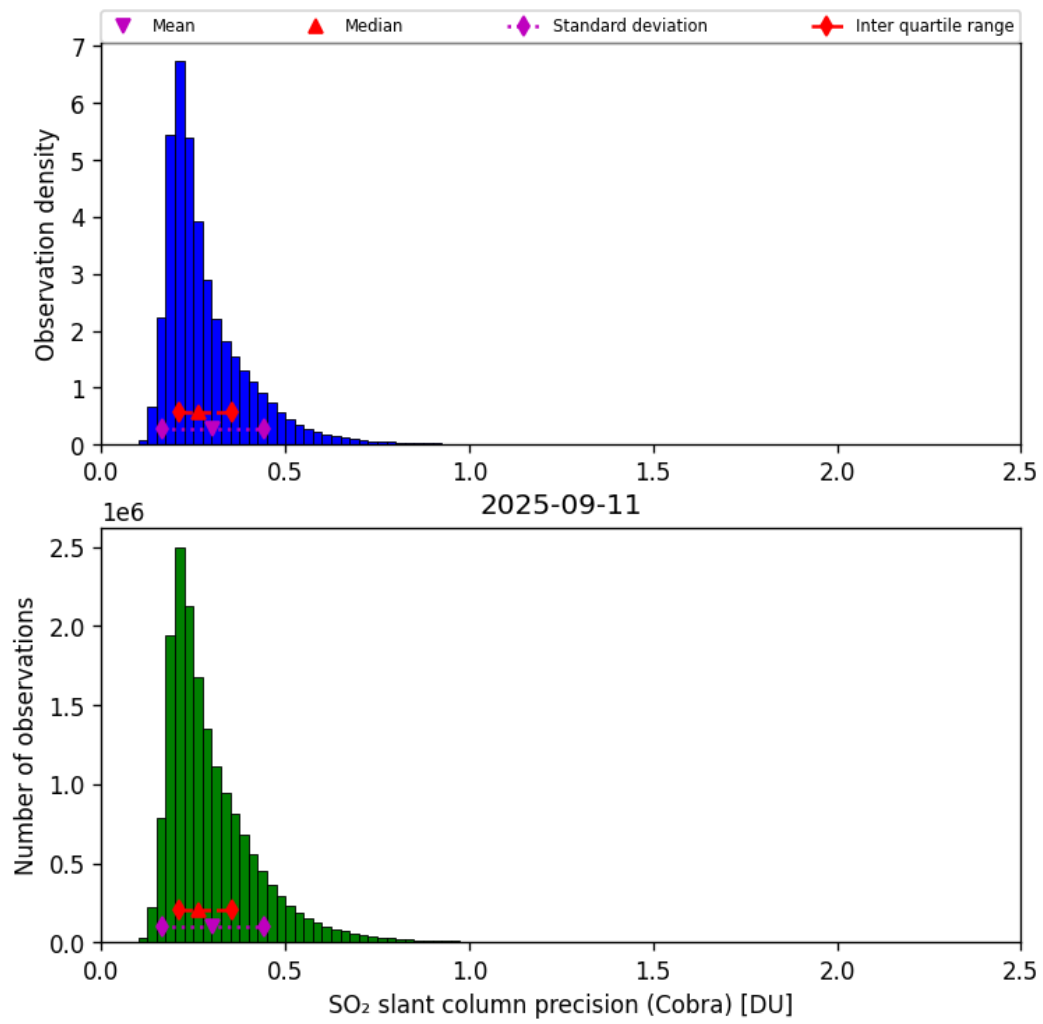
Figure 62: Histogram of “SO 2 slant column precision (Cobra)” for 2025-09-11 to 2025-09-12
