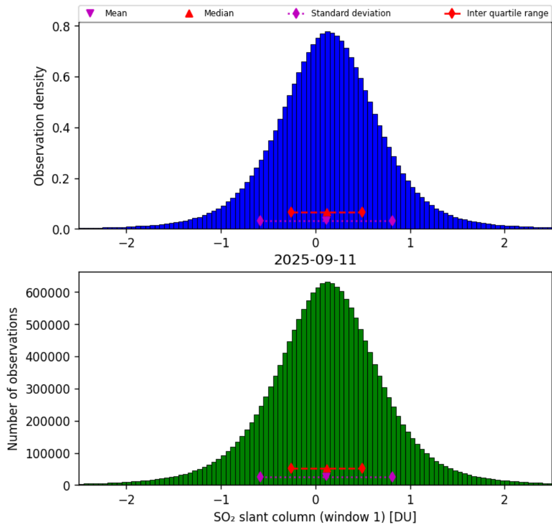
Figure 63: Histogram of “SO 2 slant column (window 1)” for 2025-09-11 to 2025-09-12
