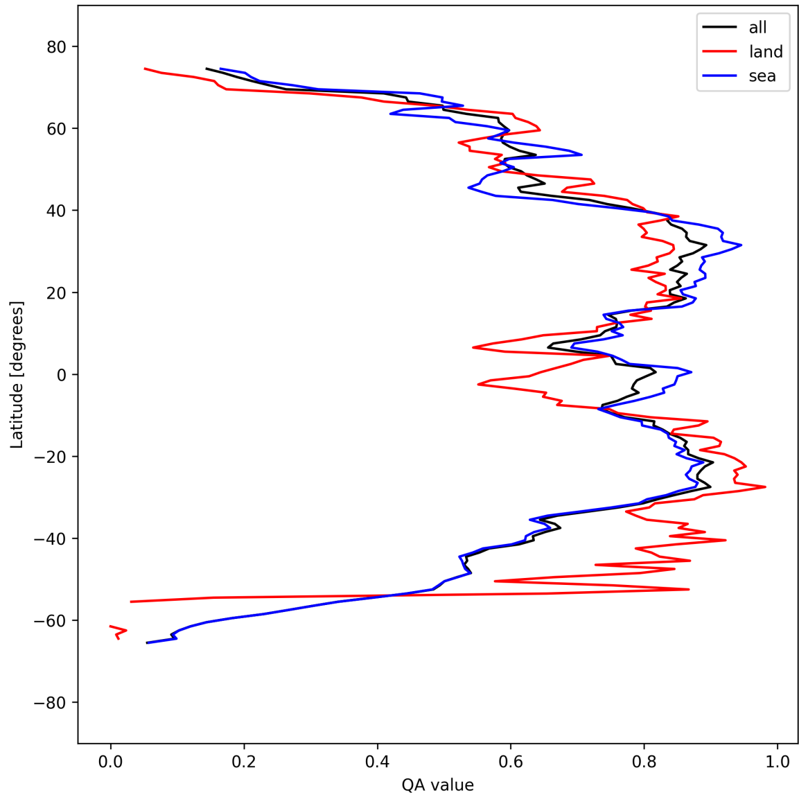
Figure 30: Zonal average of “QA value” for 2025-09-11 to 2025-09-12.
