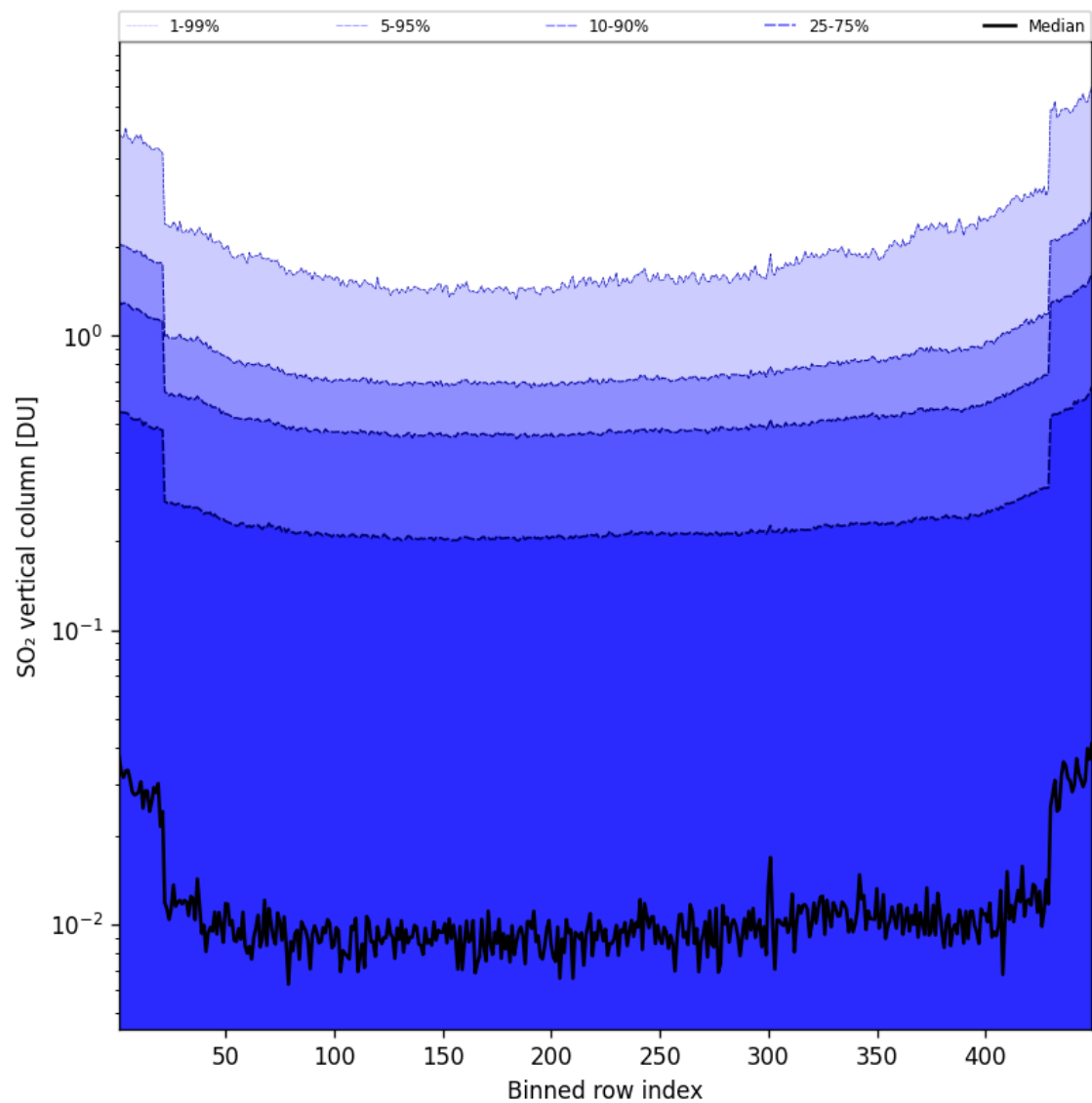
Figure 85: Along track statistics of “SO 2 vertical column” for 2025-09-11 to 2025-09-12
