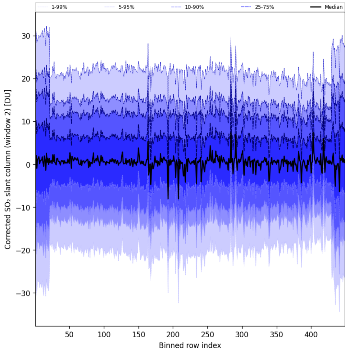
Figure 96: Along track statistics of “Corrected SO 2 slant column (window 2)” for 2025-09-11 to 2025-09-12
