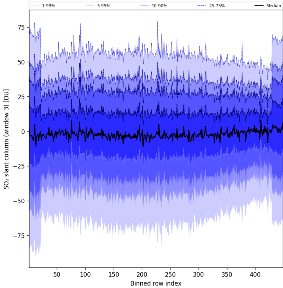
Figure 98: Along track statistics of “SO 2 slant column (window 3)” for 2025-09-11 to 2025-09-12
