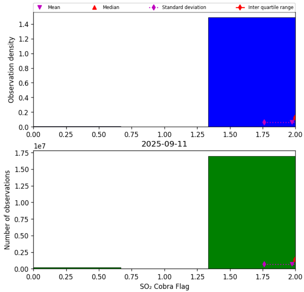
Figure 75: Histogram of “SO 2 Cobra Flag” for 2025-09-11 to 2025-09-12
