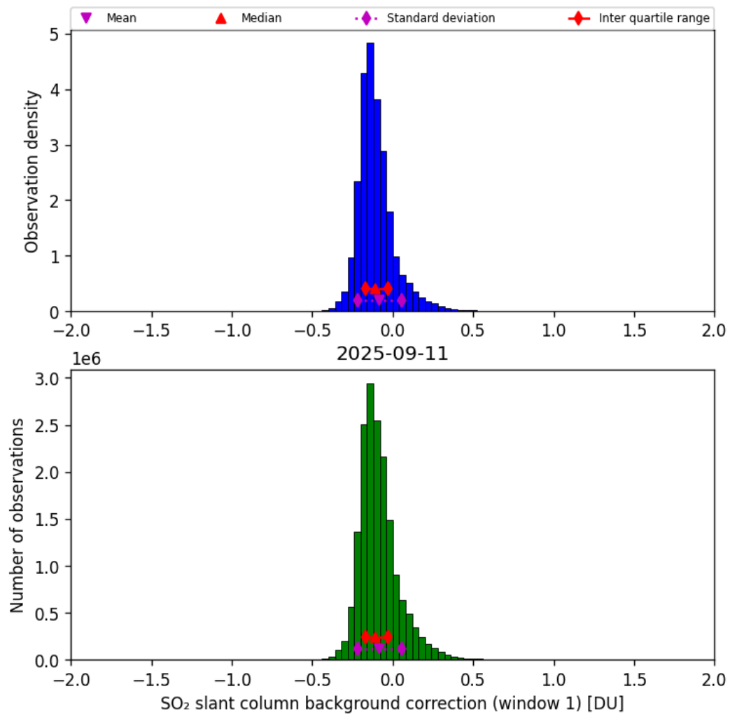
Figure 66: Histogram of “SO 2 slant column background correction (window 1)” for 2025-09-11 to 2025-09-12
