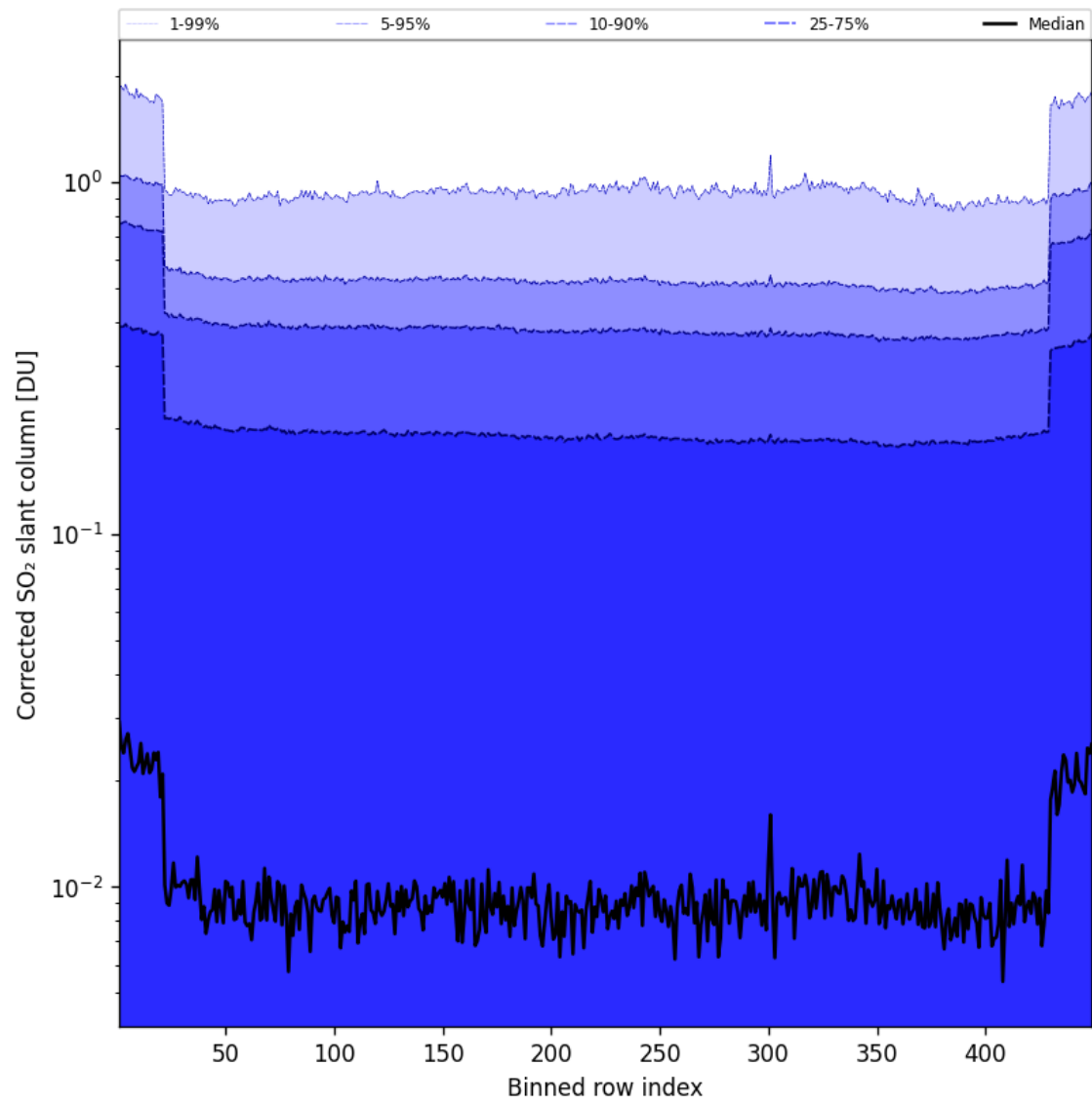
Figure 87: Along track statistics of “Corrected SO 2 slant column” for 2025-09-11 to 2025-09-12
