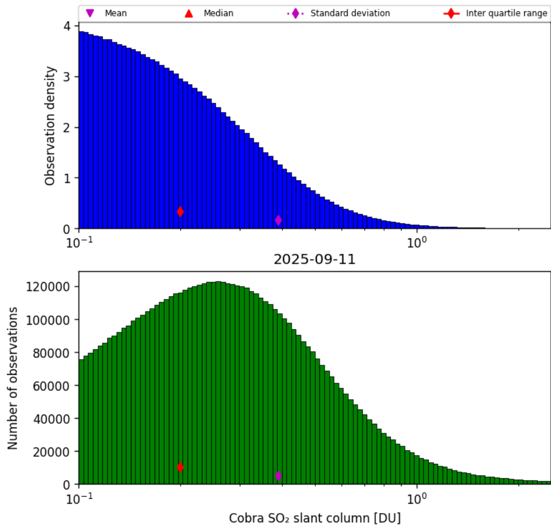
Figure 61: Histogram of “Cobra SO 2 slant column” for 2025-09-11 to 2025-09-12
