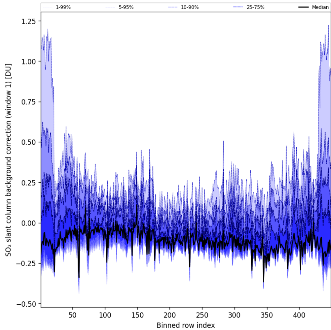
Figure 93: Along track statistics of “SO 2 slant column background correction (window 1)” for 2025-09-11 to 2025-09-12
