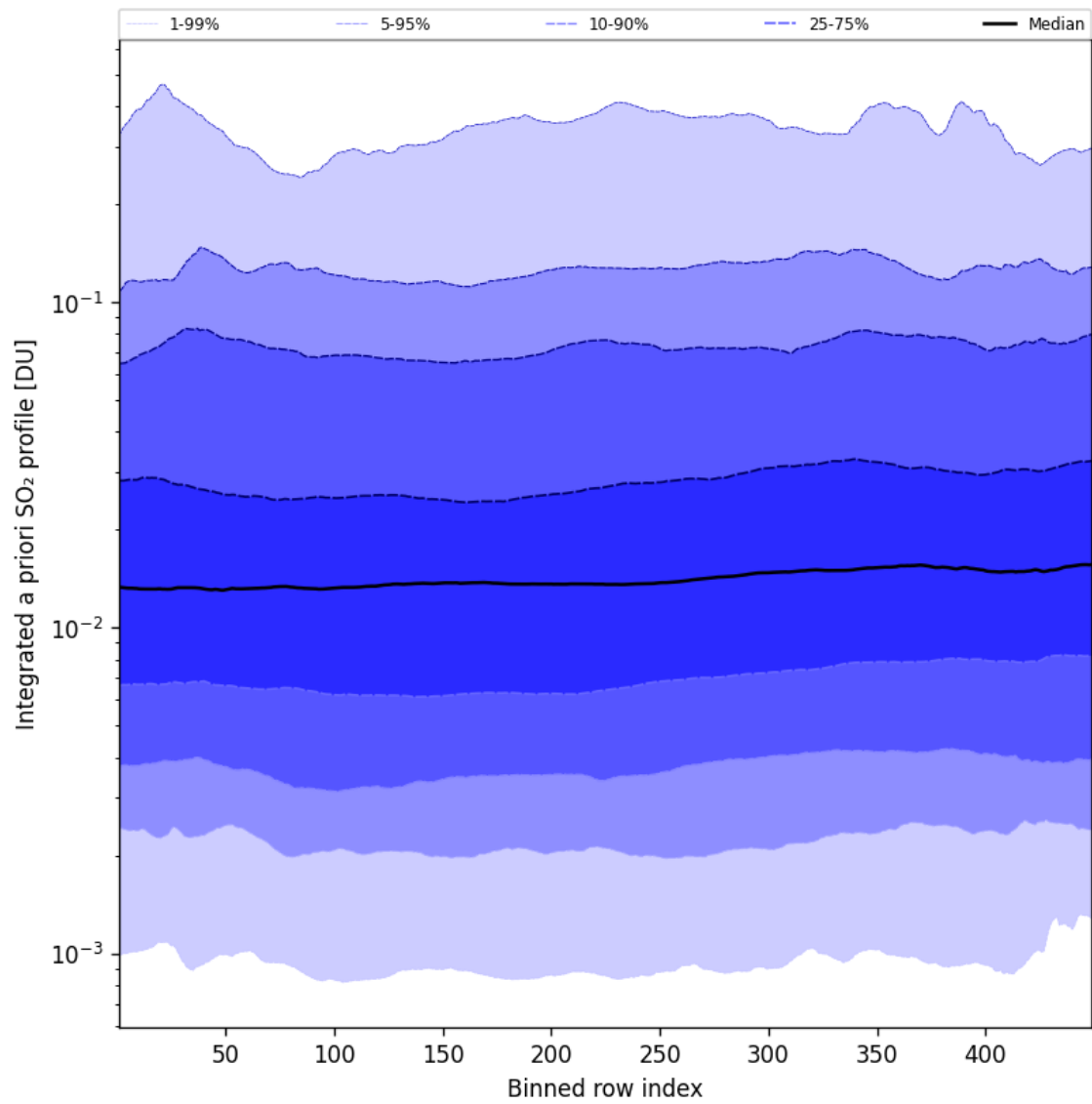
Figure 103: Along track statistics of “Integrated a priori SO 2 profile” for 2025-09-11 to 2025-09-12
