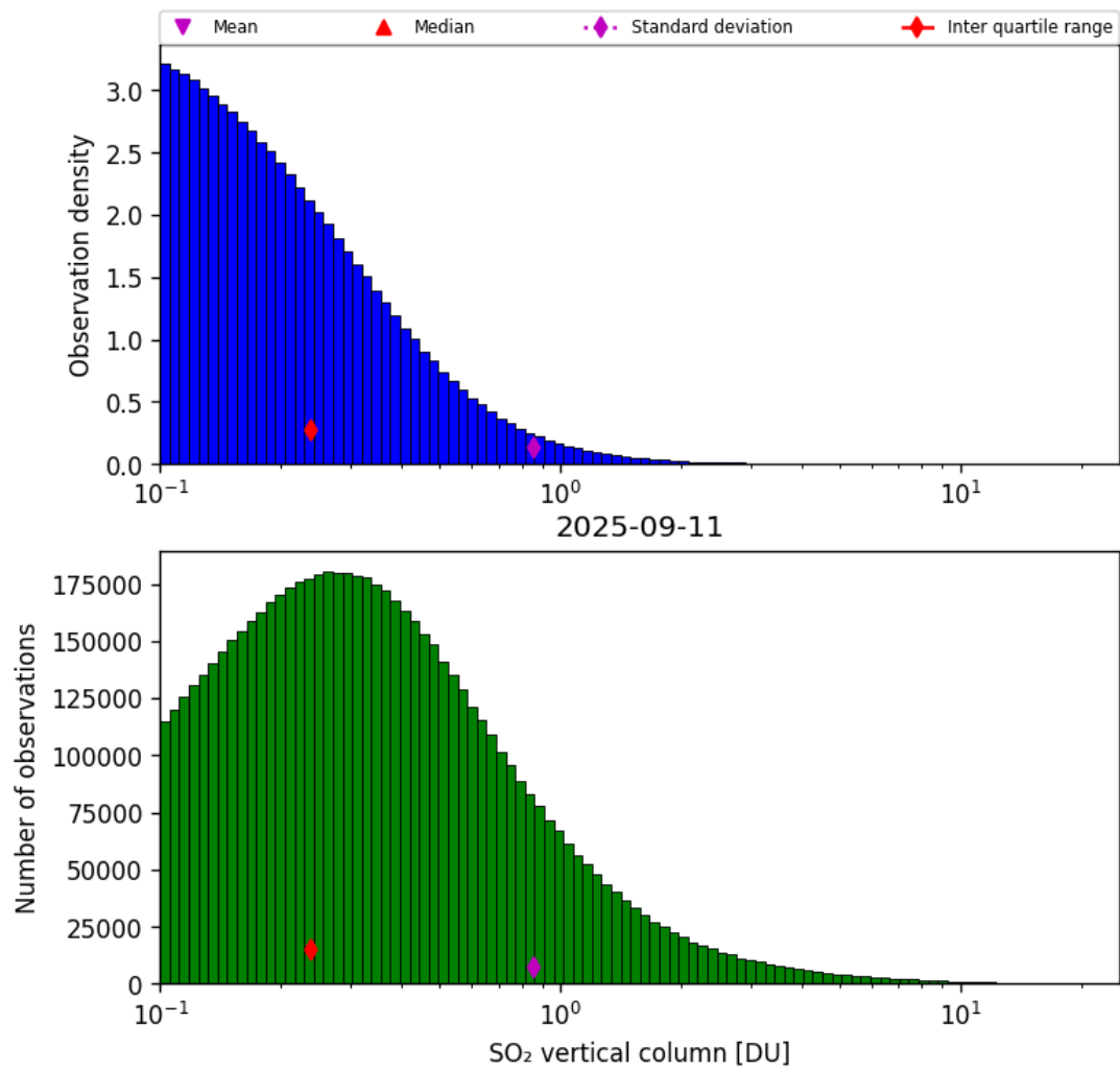
Figure 58: Histogram of “SO 2 vertical column” for 2025-09-11 to 2025-09-12
