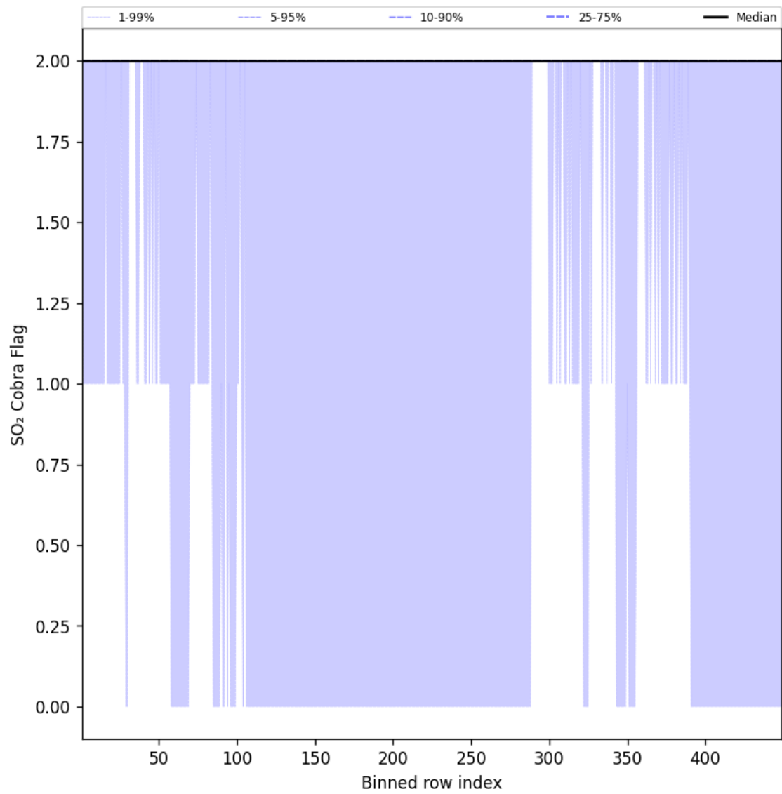
Figure 102: Along track statistics of "SO 2 Cobra Flag" for 2025-09-11 to 2025-09-12
