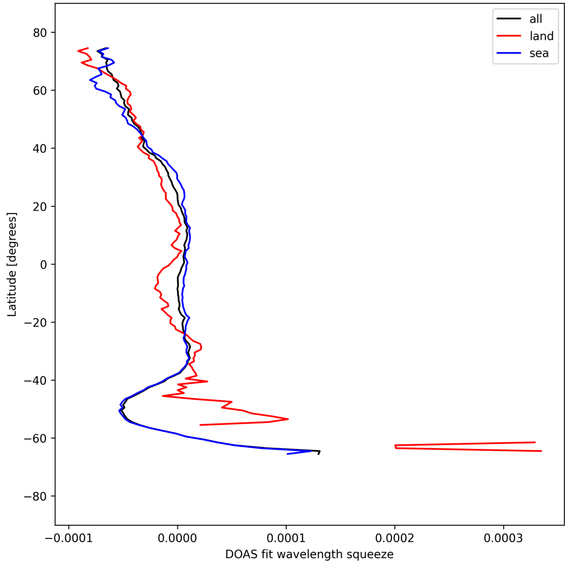
Figure 51: Zonal average of "DOAS fit wavelength squeeze" for 2025-09-11 to 2025-09-12.
