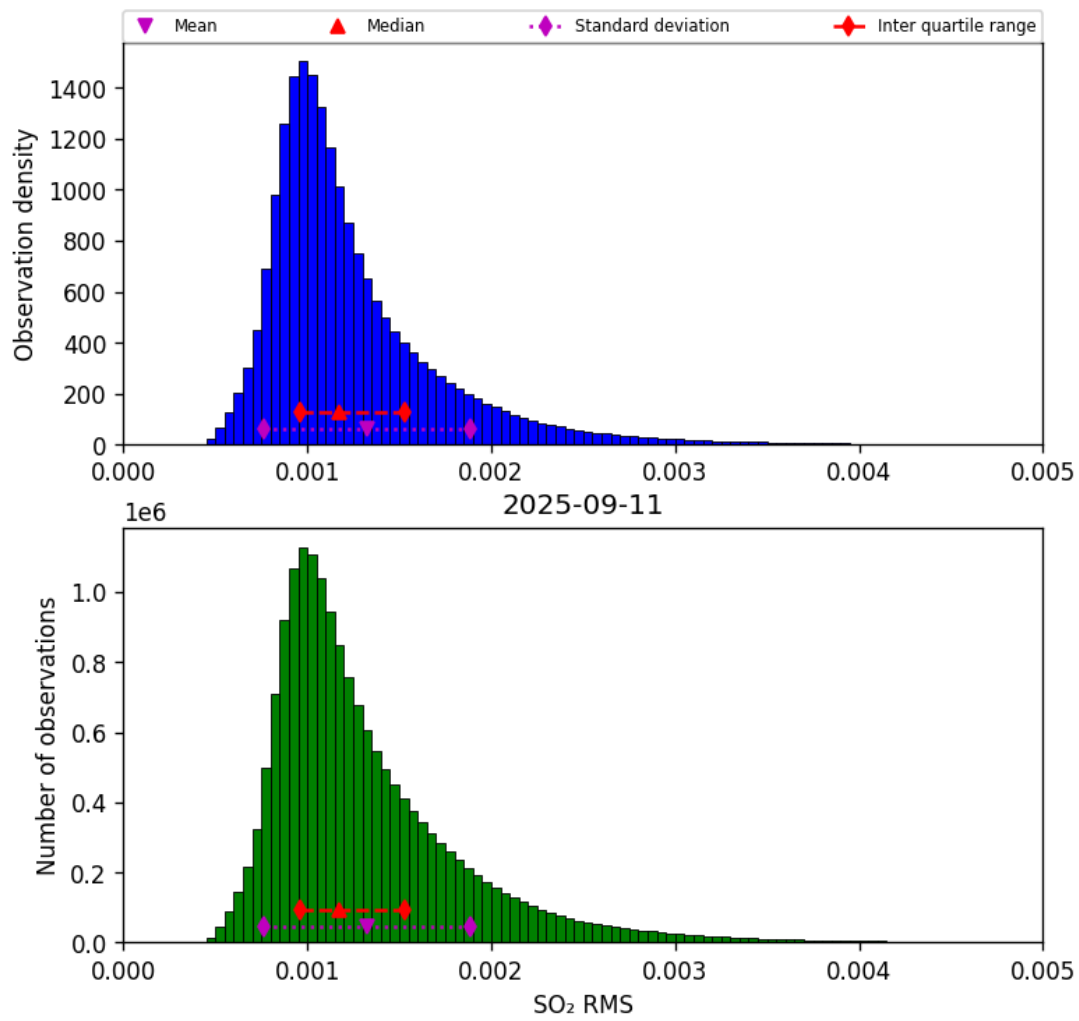
Figure 79: Histogram of “SO 2 RMS” for 2025-09-11 to 2025-09-12
