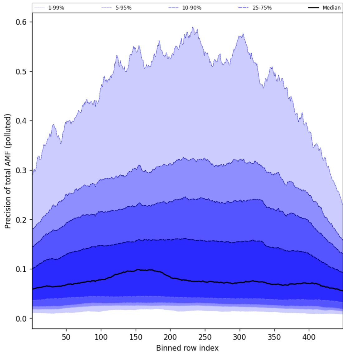
Figure 108: Along track statistics of “Precision of total AMF (polluted)” for 2025-09-11 to 2025-09-12
