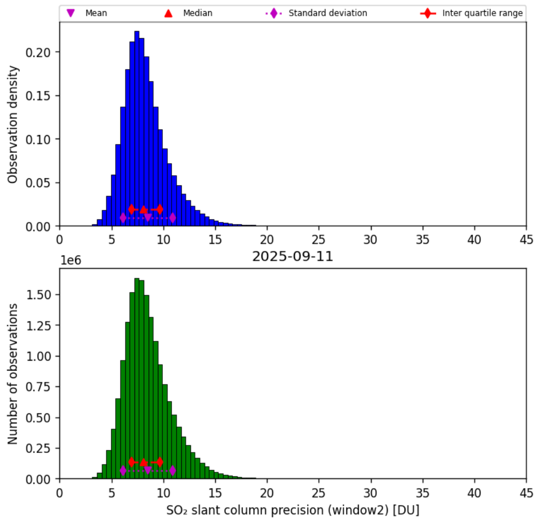
Figure 68: Histogram of “SO 2 slant column precision (window2)” for 2025-09-11 to 2025-09-12
