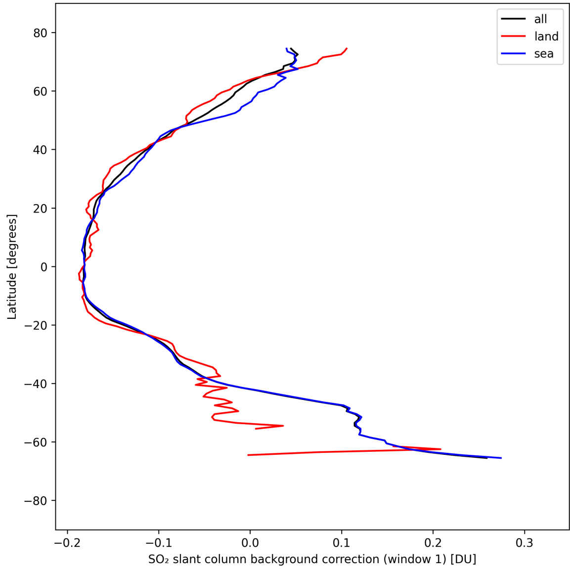
Figure 39: Zonal average of "SO 2 slant column background correction (window 1)" for 2025-09-11 to 2025-09-12.
