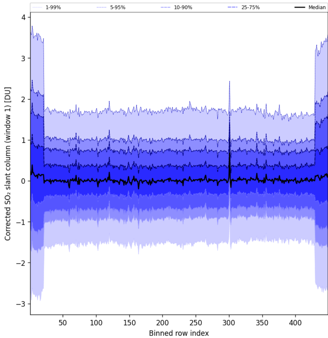
Figure 92: Along track statistics of “Corrected SO 2 slant column (window 1)” for 2025-09-11 to 2025-09-12
