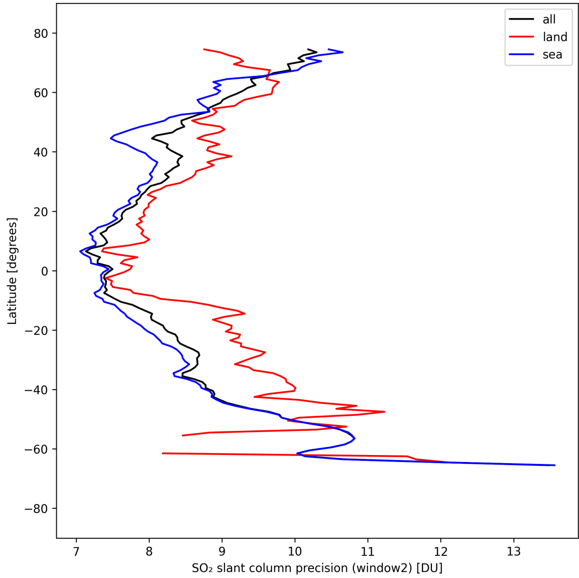
Figure 41: Zonal average of “SO 2 slant column precision (window2)” for 2025-09-11 to 2025-09-12.
