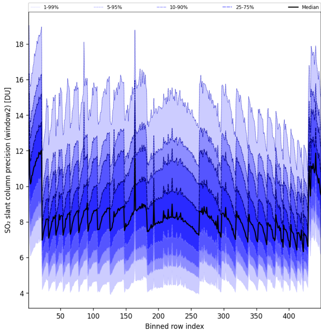
Figure 95: Along track statistics of “SO 2 slant column precision (window2)” for 2025-09-11 to 2025-09-12
