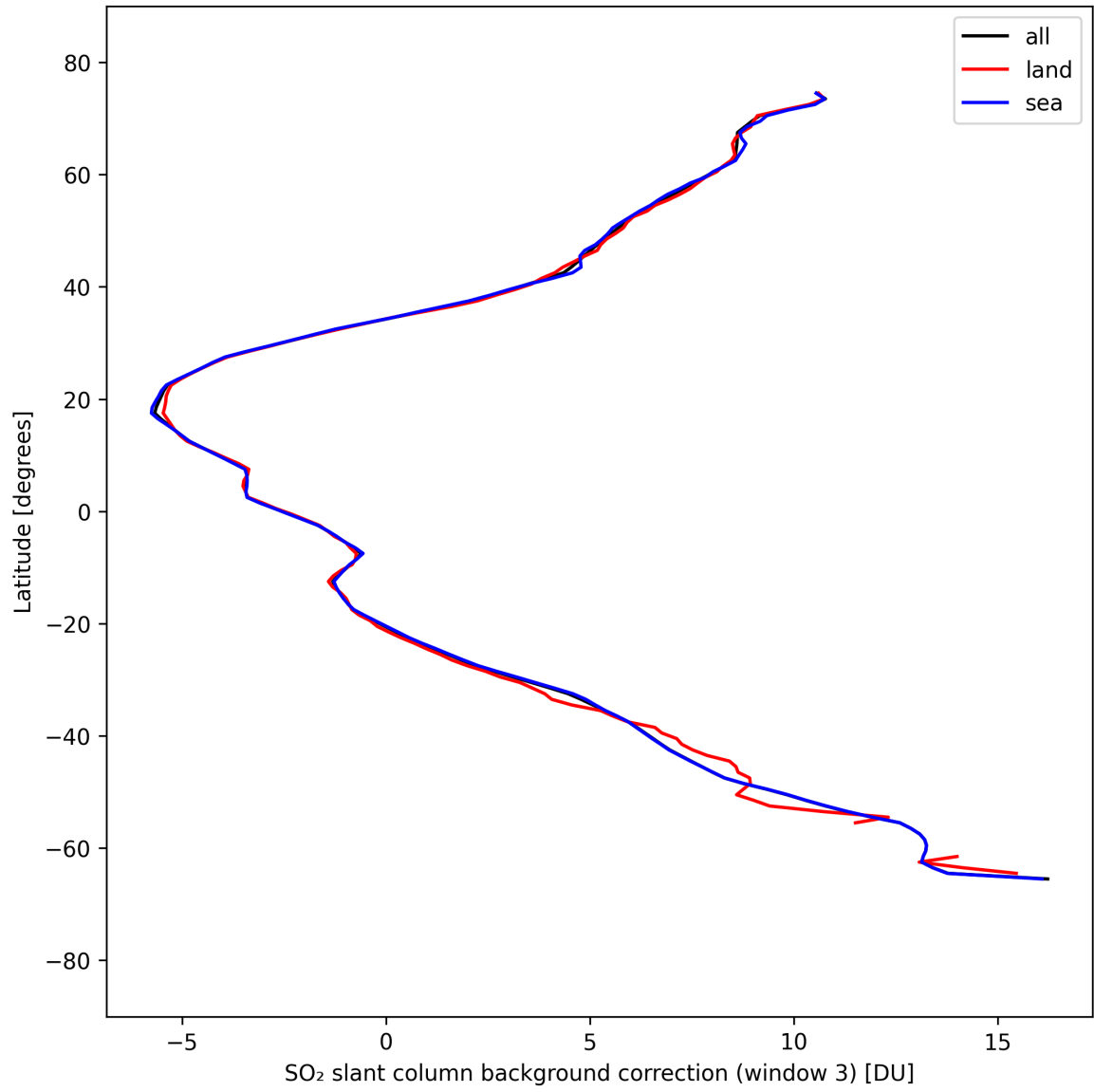
Figure 47: Zonal average of “SO 2 slant column background correction (window 3)” for 2025-09-11 to 2025-09-12.
