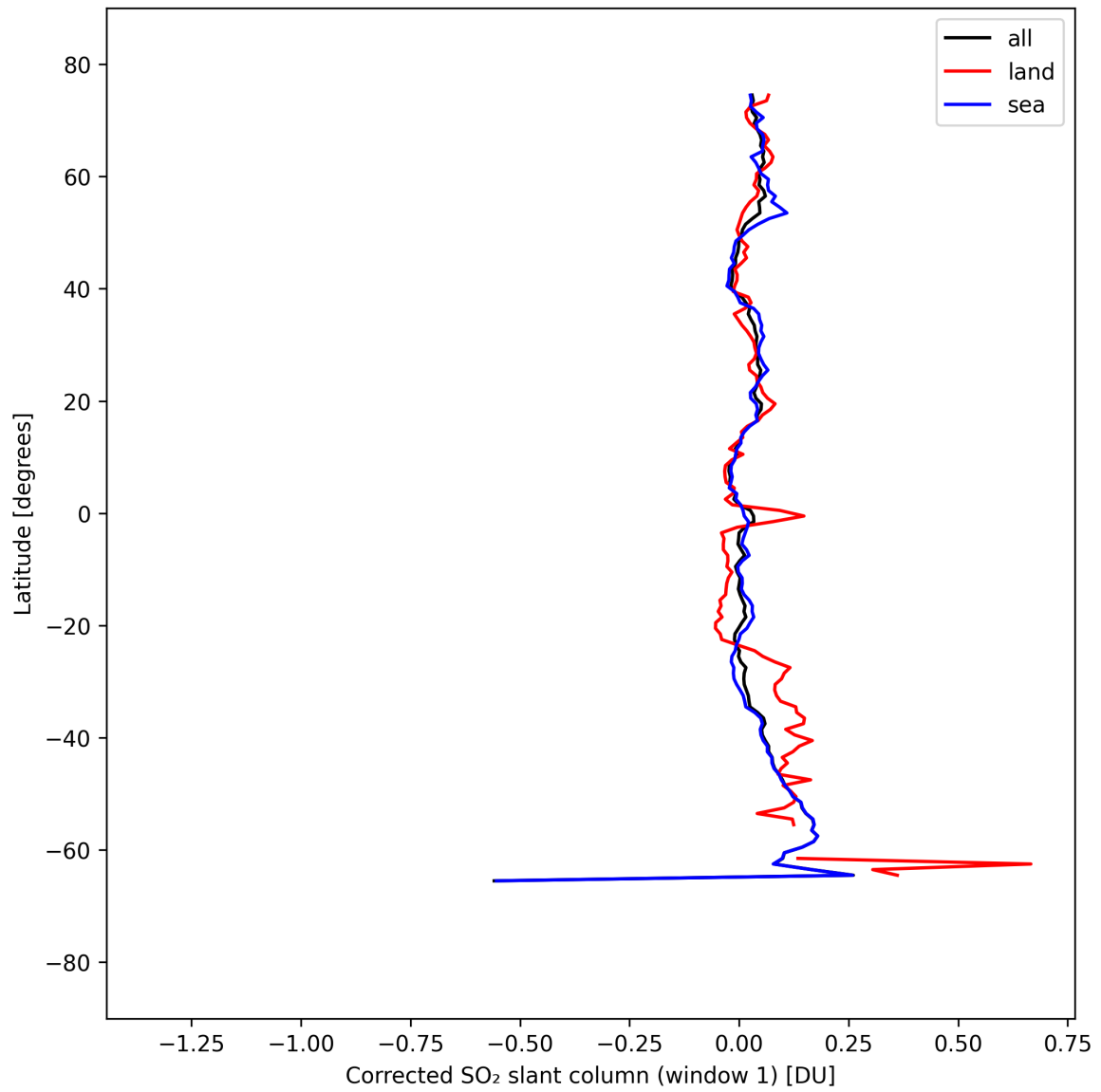
Figure 38: Zonal average of “Corrected SO 2 slant column (window 1)” for 2025-09-11 to 2025-09-12.
