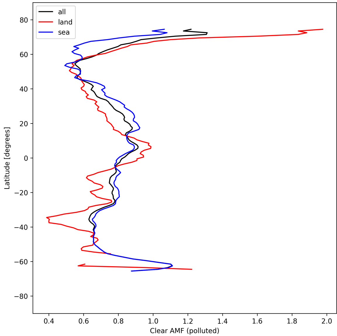
Figure 55: Zonal average of “Clear AMF (polluted)” for 2025-09-11 to 2025-09-12.
