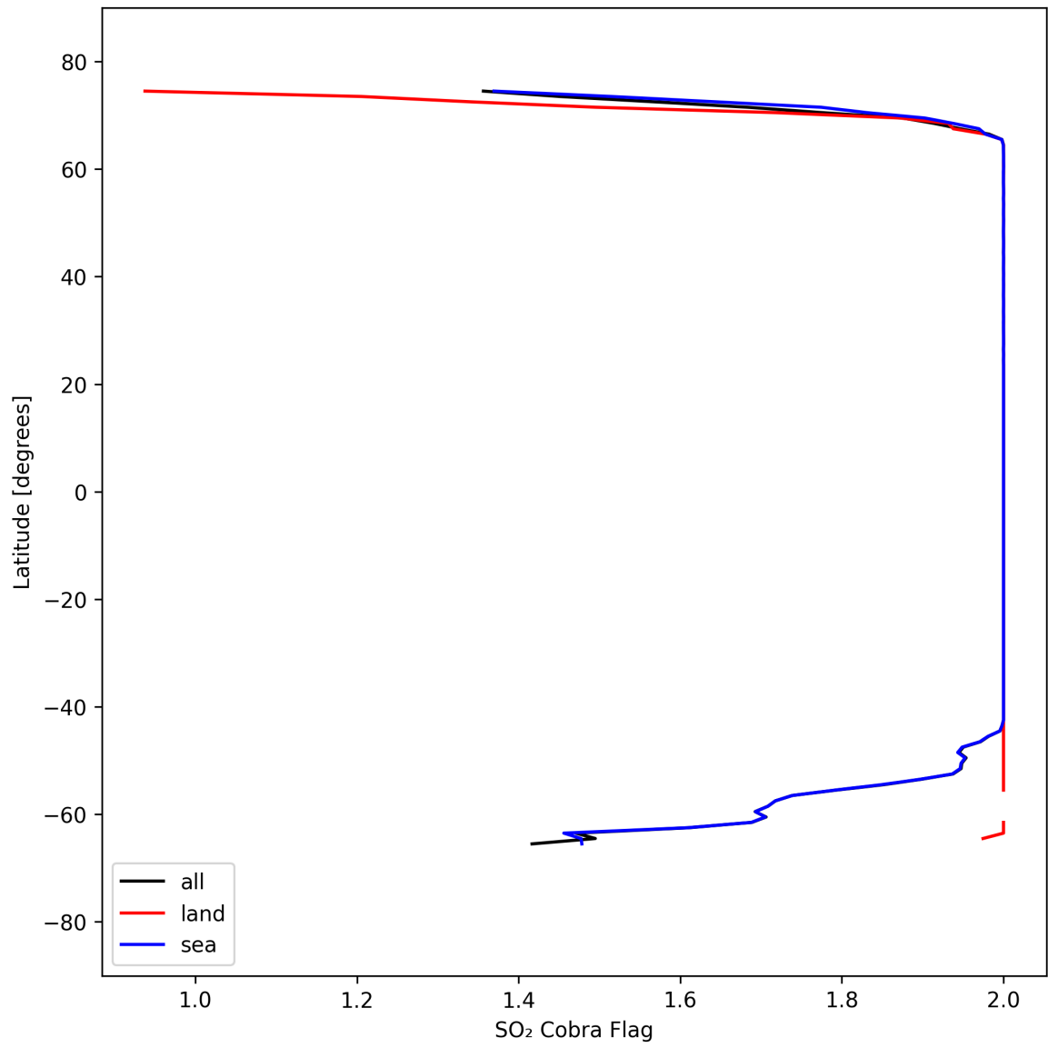
Figure 48: Zonal average of "SO 2 Cobra Flag" for 2025-09-11 to 2025-09-12.
