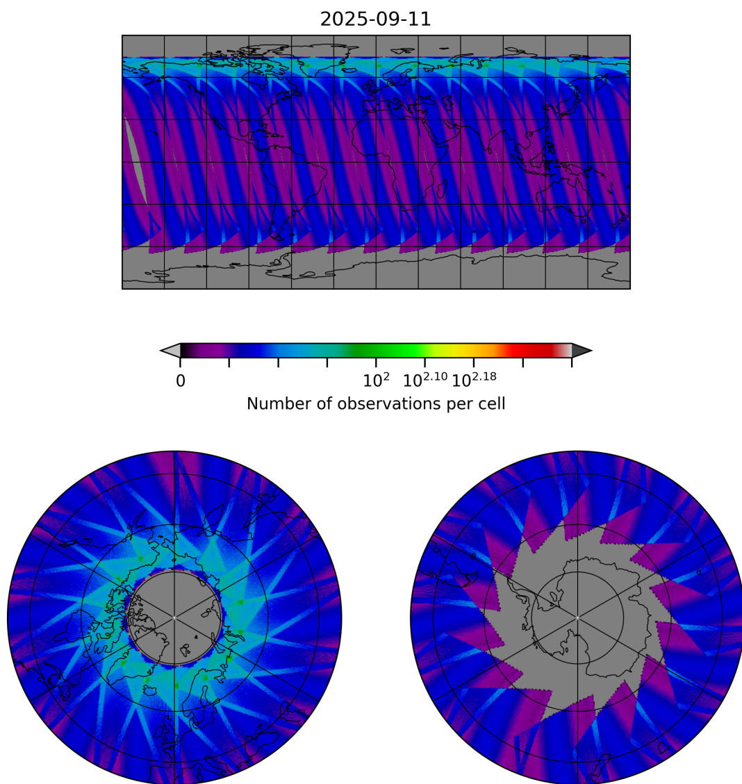
Figure 29: Map of the number of observations for 2025-09-11 to 2025-09-12
