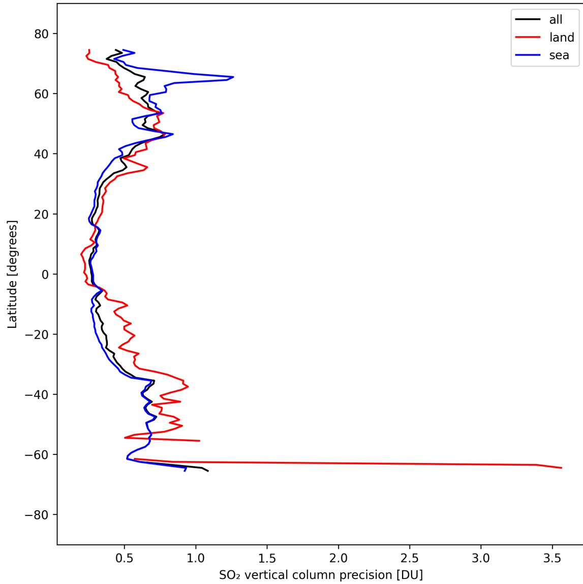
Figure 32: Zonal average of “SO 2 vertical column precision” for 2025-09-11 to 2025-09-12.
