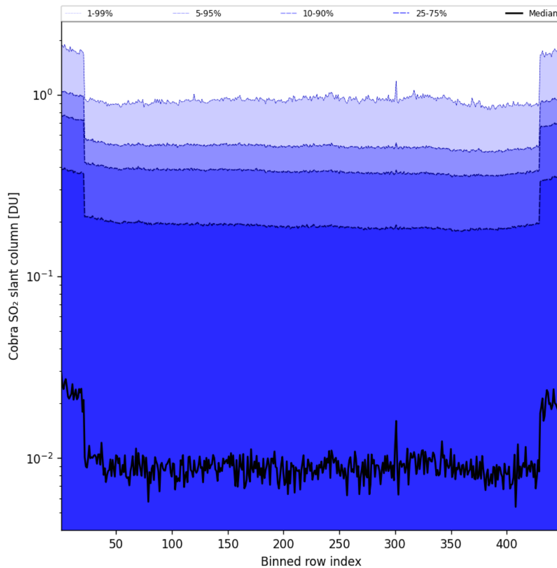
Figure 88: Along track statistics of “Cobra SO 2 slant column” for 2025-09-11 to 2025-09-12
