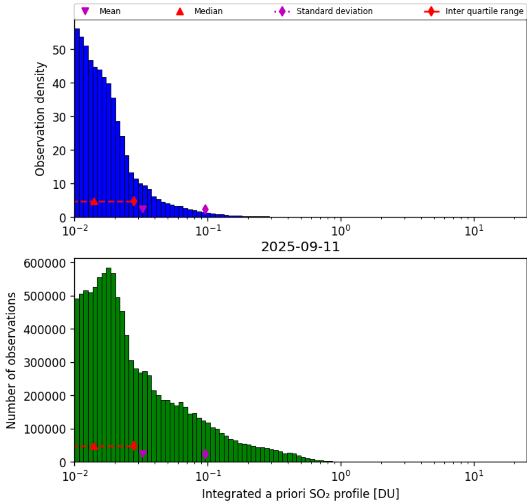
Figure 76: Histogram of “Integrated a priori SO 2 profile” for 2025-09-11 to 2025-09-12
