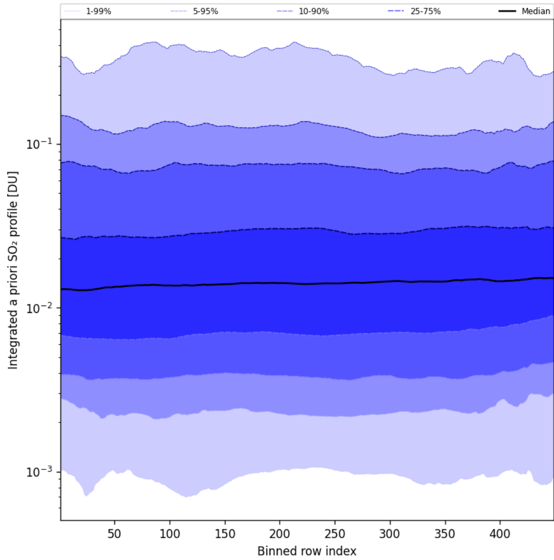
Figure 103: Along track statistics of “Integrated a priori SO 2 profile” for 2025-09-12 to 2025-09-13
