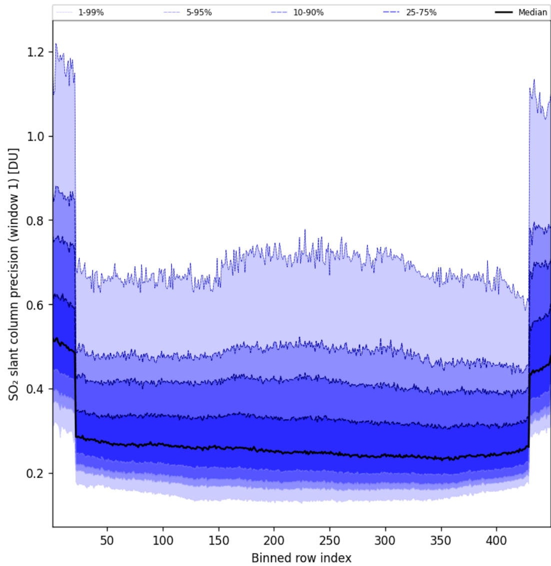
Figure 91: Along track statistics of “SO 2 slant column precision (window 1)” for 2025-09-12 to 2025-09-13
