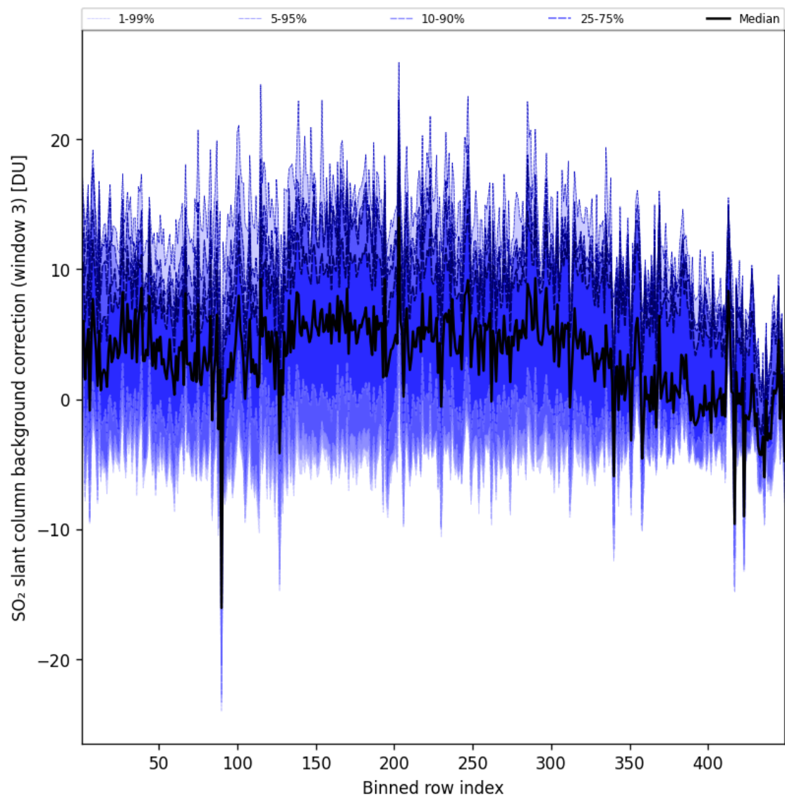
Figure 101: Along track statistics of “SO 2 slant column background correction (window 3)” for 2025-09-12 to 2025-09-13
