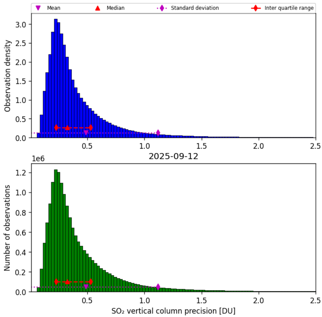
Figure 59: Histogram of “SO 2 vertical column precision” for 2025-09-12 to 2025-09-13
