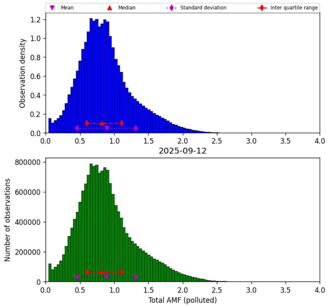
Figure 80: Histogram of “Total AMF (polluted)” for 2025-09-12 to 2025-09-13
