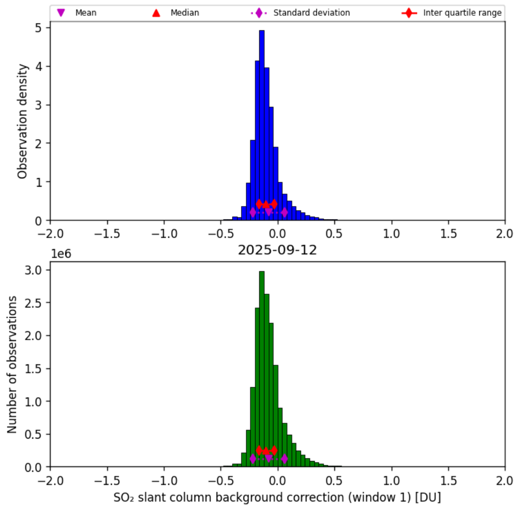
Figure 66: Histogram of “SO 2 slant column background correction (window 1)” for 2025-09-12 to 2025-09-13
