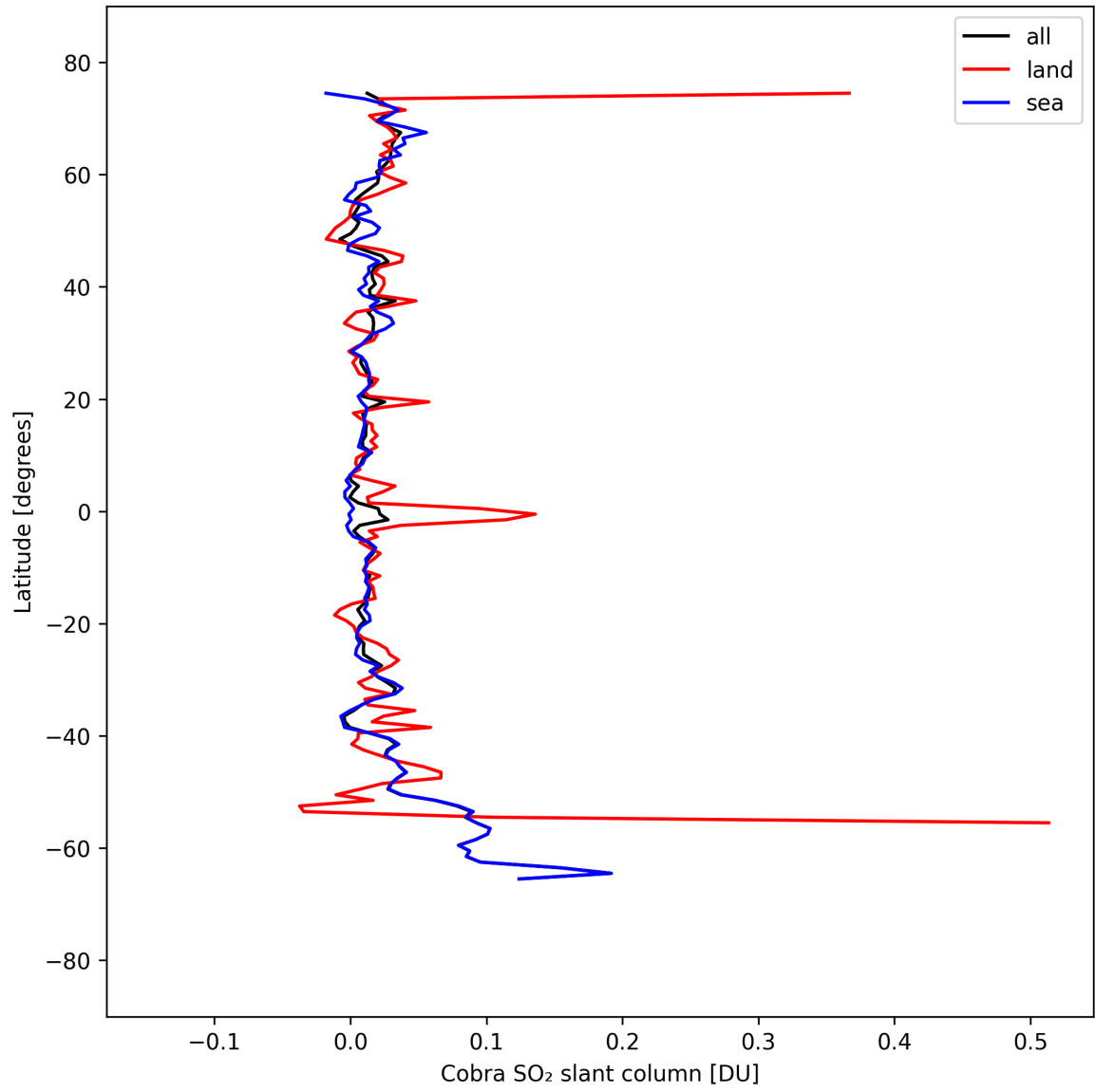
Figure 34: Zonal average of "Cobra SO 2 slant column" for 2025-09-12 to 2025-09-13.
