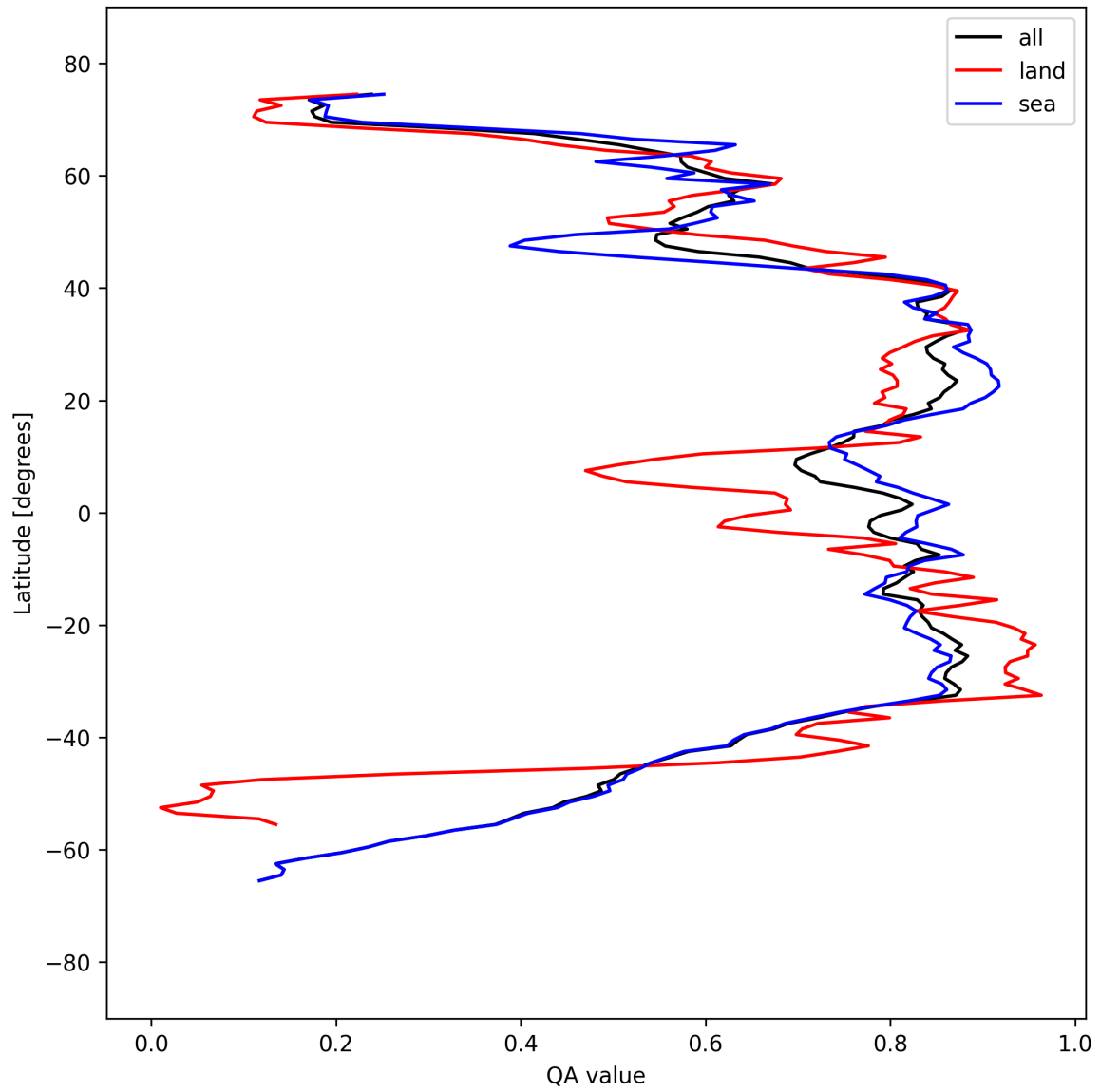
Figure 30: Zonal average of “QA value” for 2025-09-12 to 2025-09-13.
