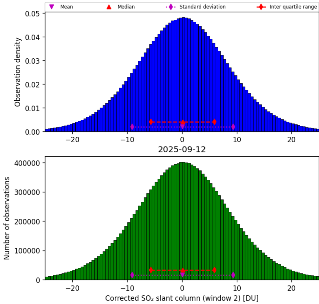
Figure 69: Histogram of “Corrected SO 2 slant column (window 2)” for 2025-09-12 to 2025-09-13
