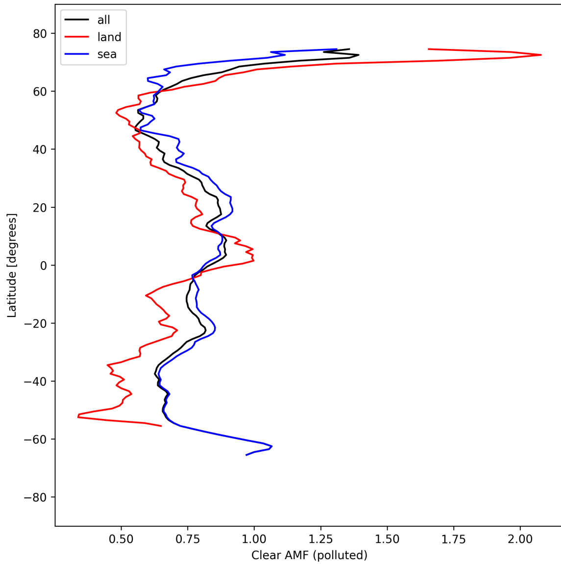
Figure 55: Zonal average of “Clear AMF (polluted)” for 2025-09-12 to 2025-09-13.
