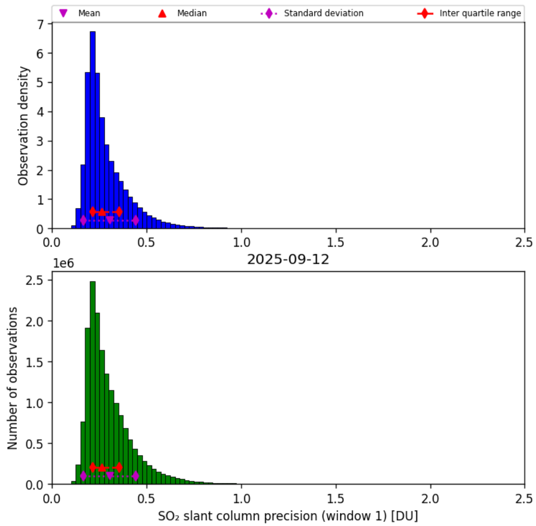
Figure 64: Histogram of “SO 2 slant column precision (window 1)” for 2025-09-12 to 2025-09-13
