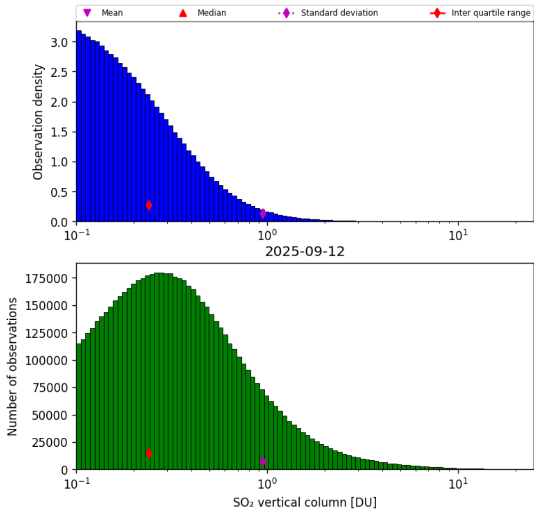
Figure 58: Histogram of “SO 2 vertical column” for 2025-09-12 to 2025-09-13
