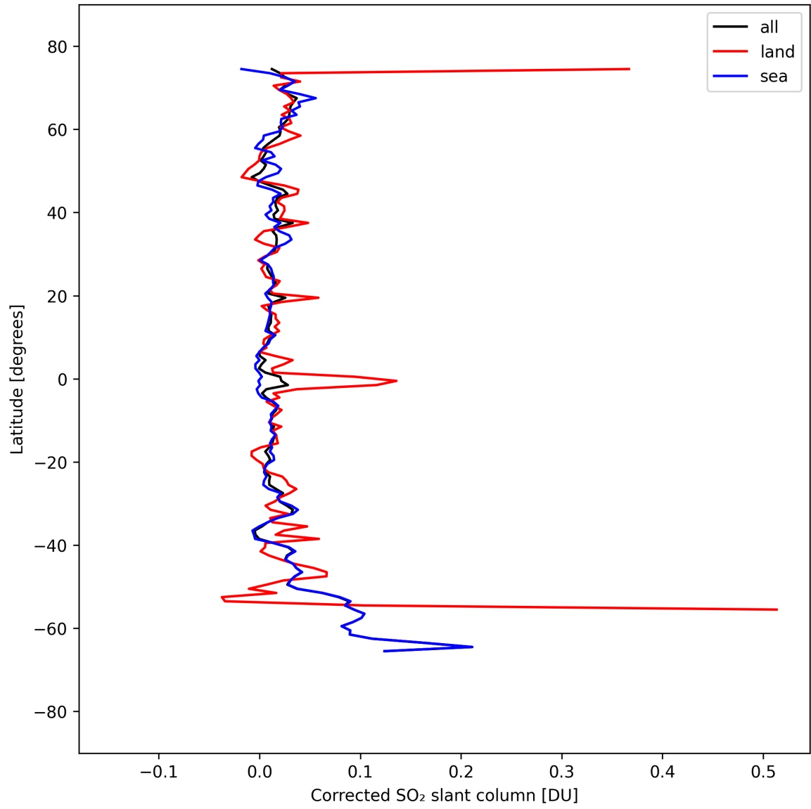
Figure 33: Zonal average of “Corrected SO 2 slant column” for 2025-09-12 to 2025-09-13.
