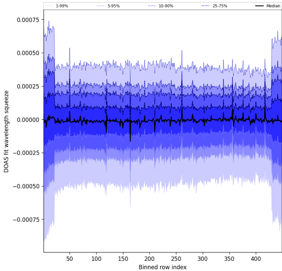
Figure 105: Along track statistics of “DOAS fit wavelength squeeze” for 2025-09-12 to 2025-09-13
