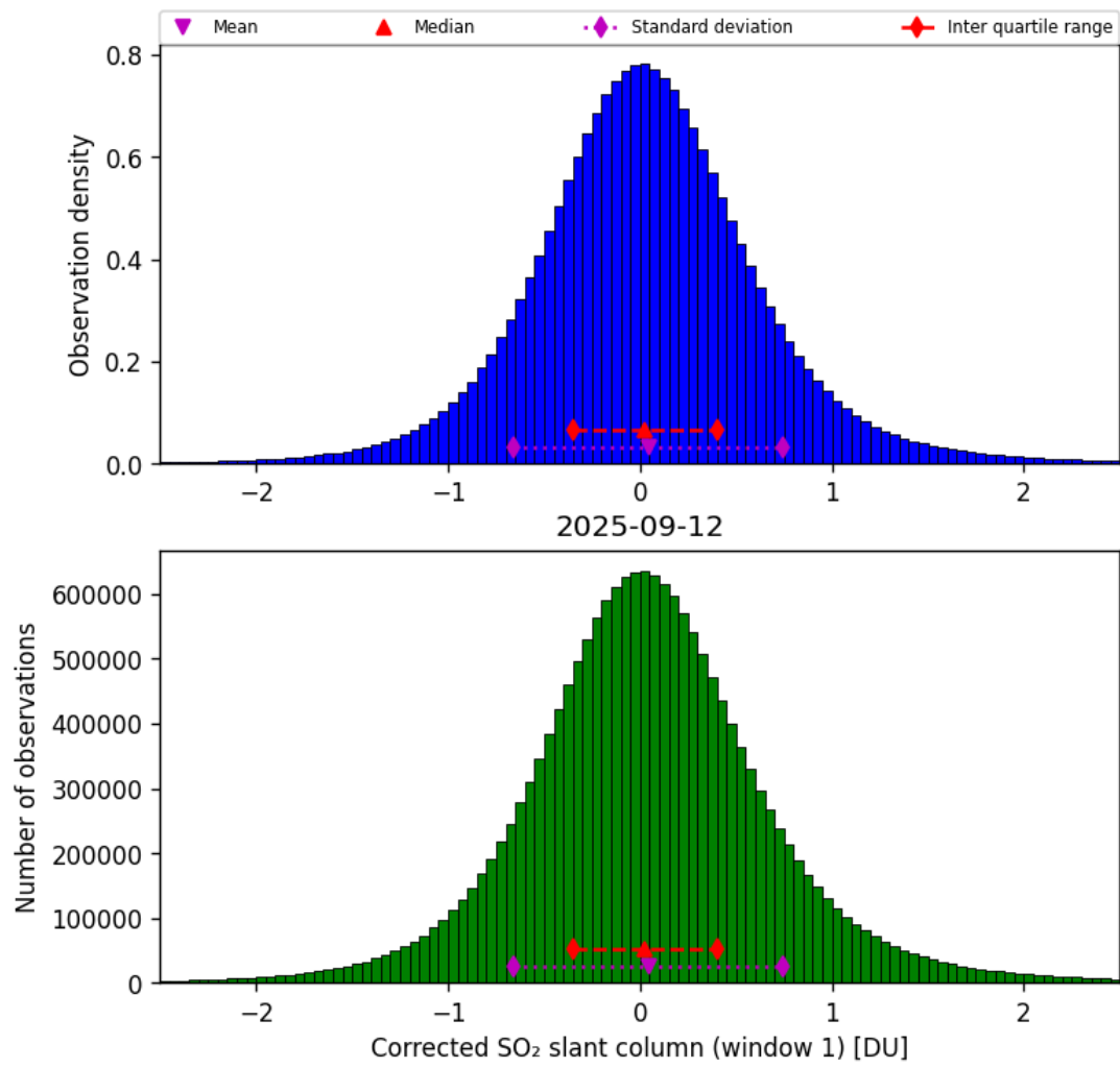
Figure 65: Histogram of “Corrected SO 2 slant column (window 1)” for 2025-09-12 to 2025-09-13
