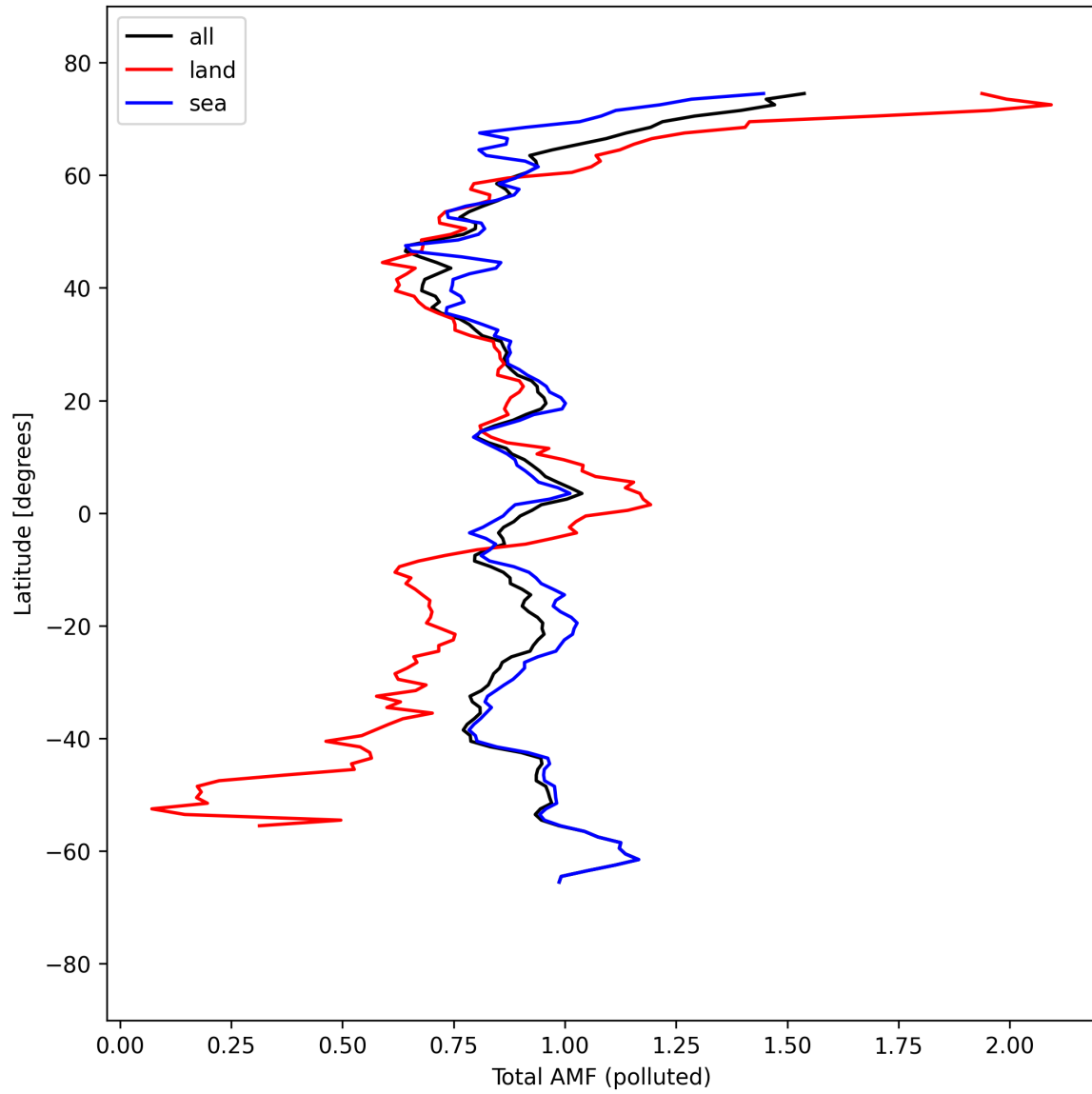
Figure 53: Zonal average of “Total AMF (polluted)” for 2025-09-12 to 2025-09-13.
