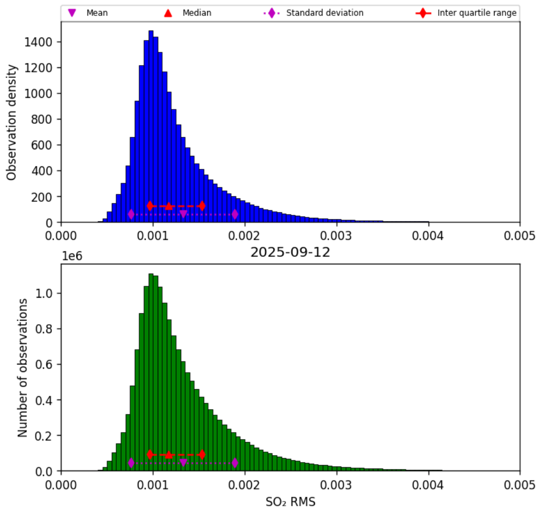
Figure 79: Histogram of “SO 2 RMS” for 2025-09-12 to 2025-09-13
