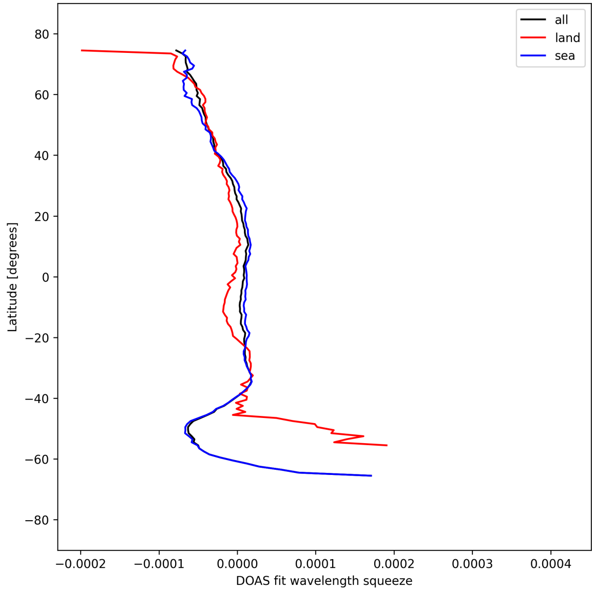
Figure 51: Zonal average of “DOAS fit wavelength squeeze” for 2025-09-12 to 2025-09-13.
