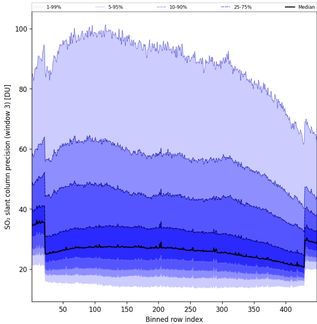
Figure 99: Along track statistics of “SO 2 slant column precision (window 3)” for 2025-09-12 to 2025-09-13
