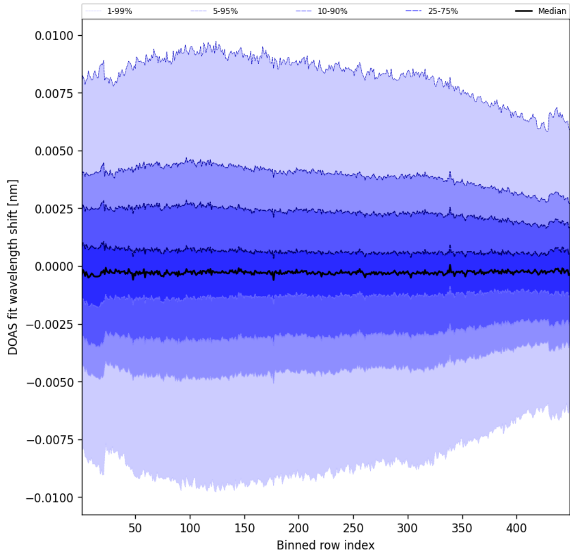
Figure 104: Along track statistics of “DOAS fit wavelength shift” for 2025-09-12 to 2025-09-13
