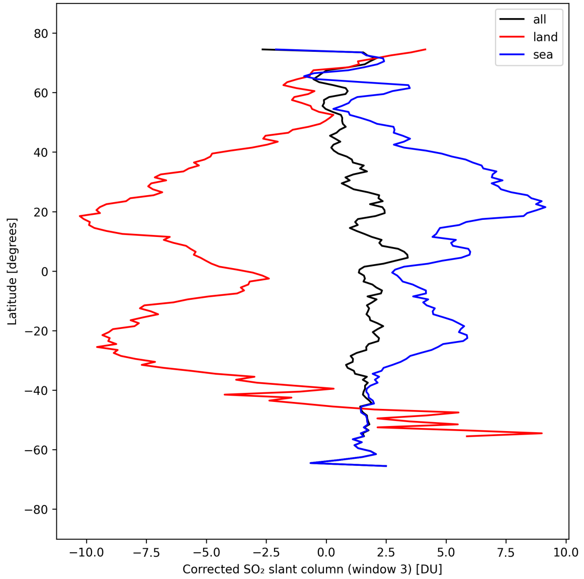
Figure 46: Zonal average of “Corrected SO 2 slant column (window 3)” for 2025-09-12 to 2025-09-13.
