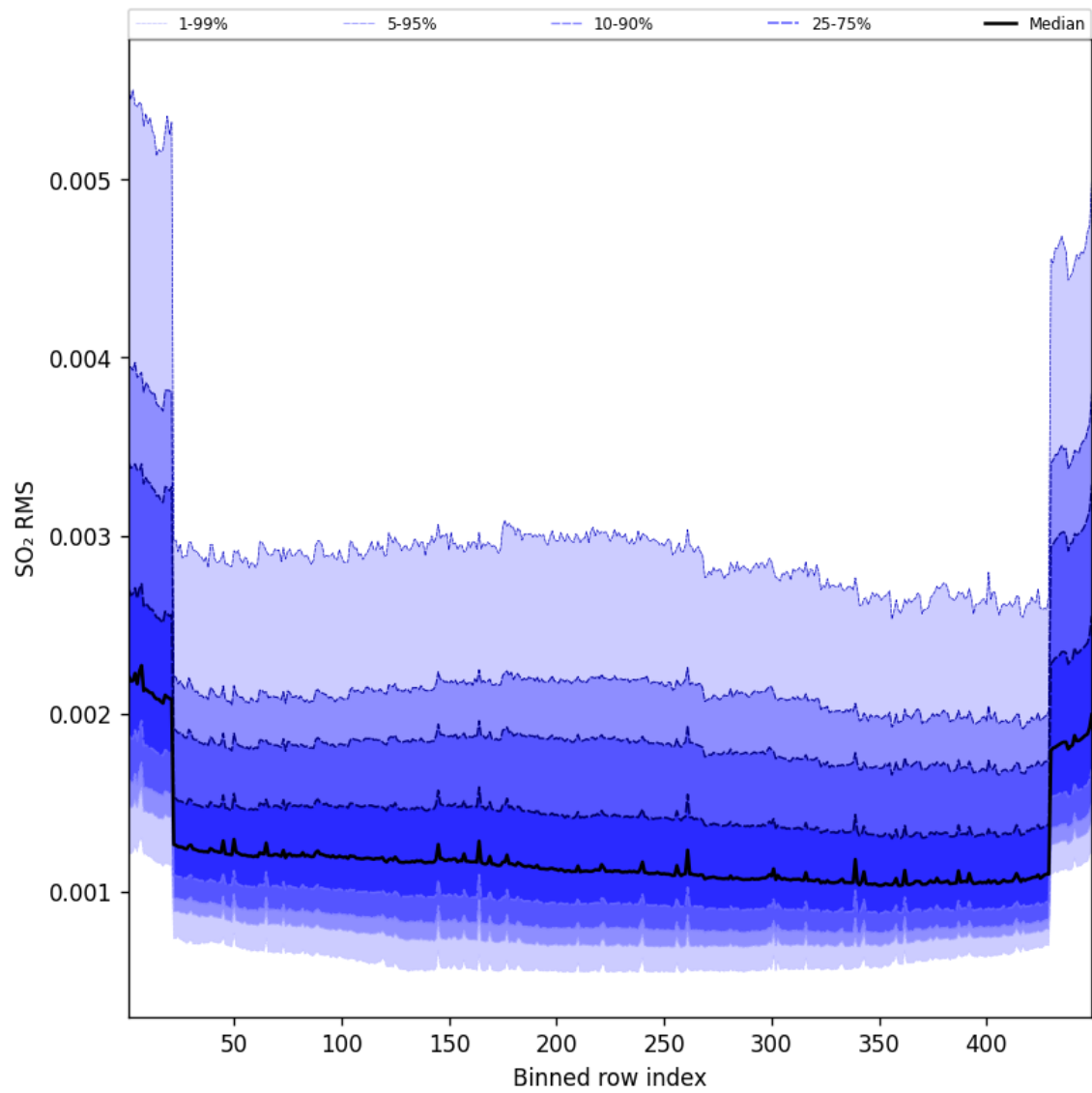
Figure 106: Along track statistics of “SO 2 RMS” for 2025-09-12 to 2025-09-13
