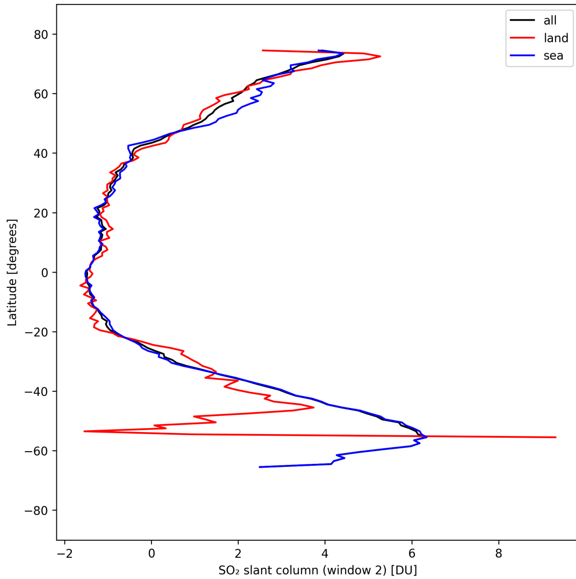
Figure 40: Zonal average of “SO 2 slant column (window 2)” for 2025-09-12 to 2025-09-13.
