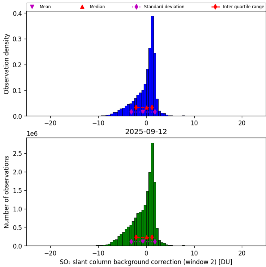
Figure 70: Histogram of “SO 2 slant column background correction (window 2)” for 2025-09-12 to 2025-09-13
