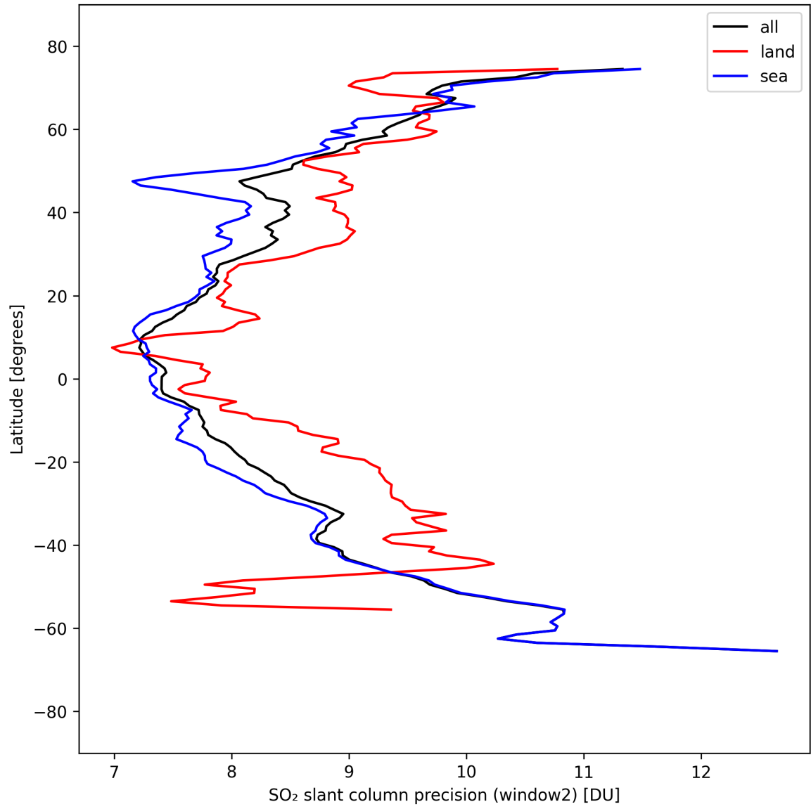
Figure 41: Zonal average of “SO 2 slant column precision (window2)” for 2025-09-12 to 2025-09-13.
