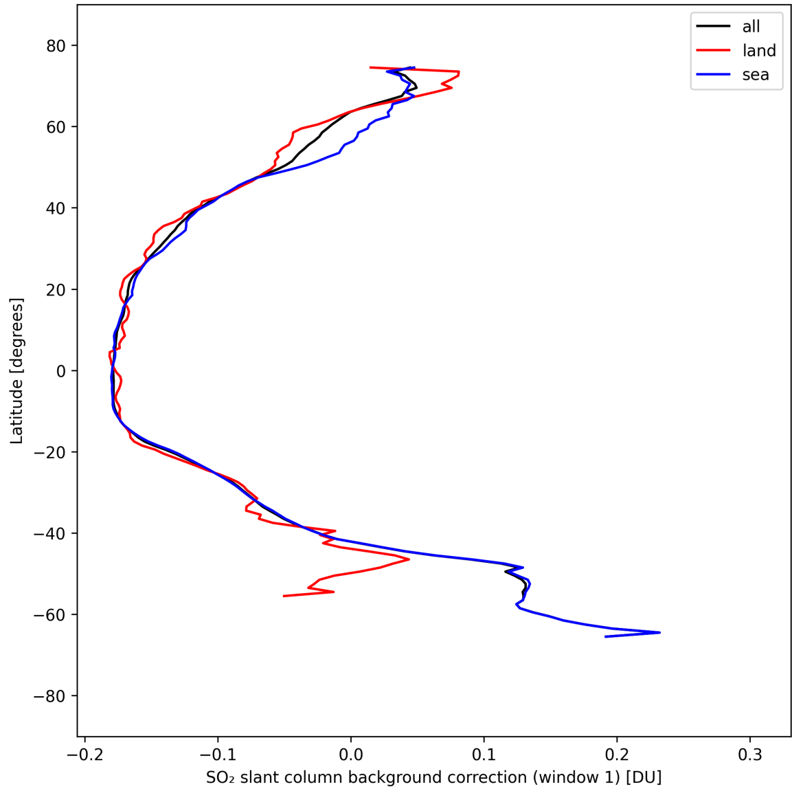
Figure 39: Zonal average of “SO 2 slant column background correction (window 1)” for 2025-09-12 to 2025-09-13.
