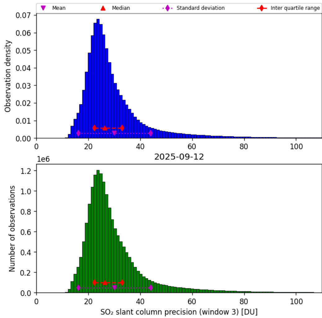
Figure 72: Histogram of “SO 2 slant column precision (window 3)” for 2025-09-12 to 2025-09-13
