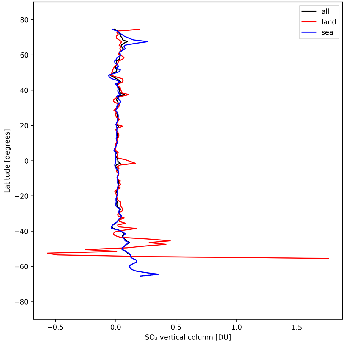
Figure 31: Zonal average of “SO 2 vertical column” for 2025-09-12 to 2025-09-13.
