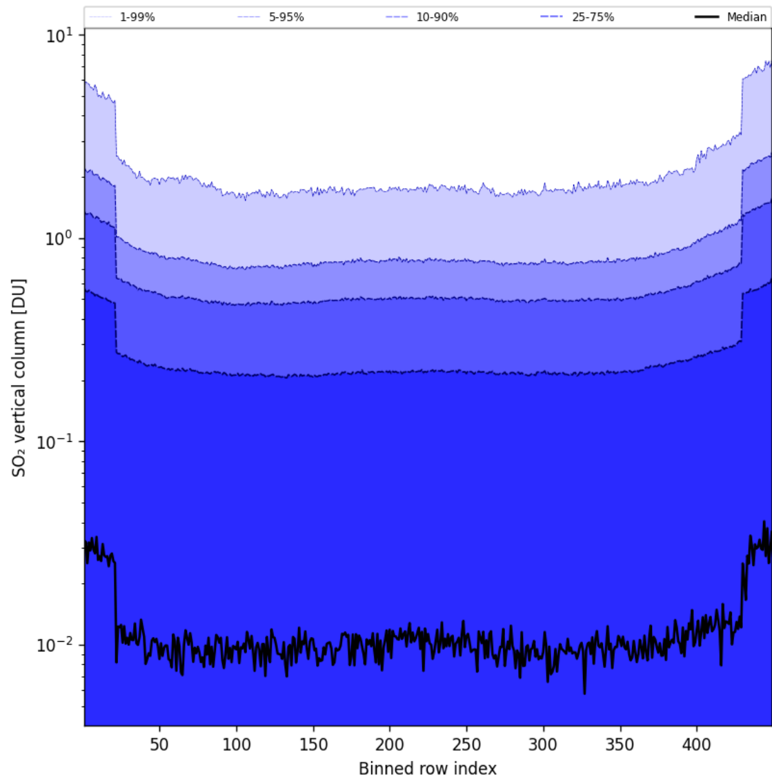
Figure 85: Along track statistics of “SO 2 vertical column” for 2025-09-12 to 2025-09-13
