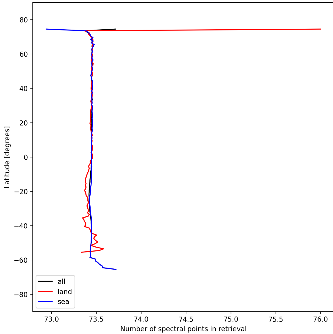
Figure 56: Zonal average of “Number of spectral points in retrieval” for 2025-09-12 to 2025-09-13.
