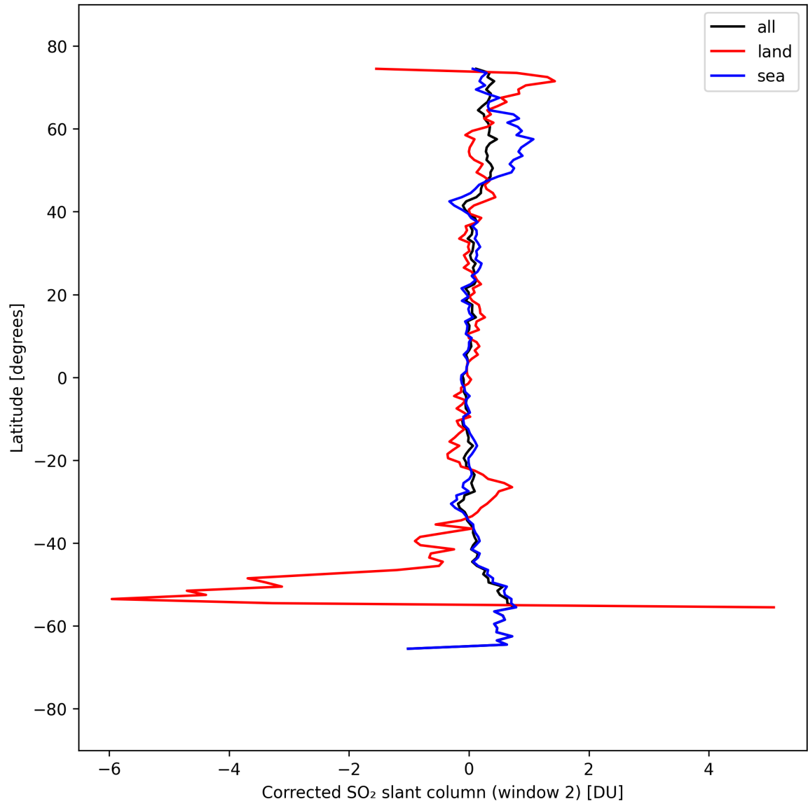
Figure 42: Zonal average of “Corrected SO 2 slant column (window 2)” for 2025-09-12 to 2025-09-13.
