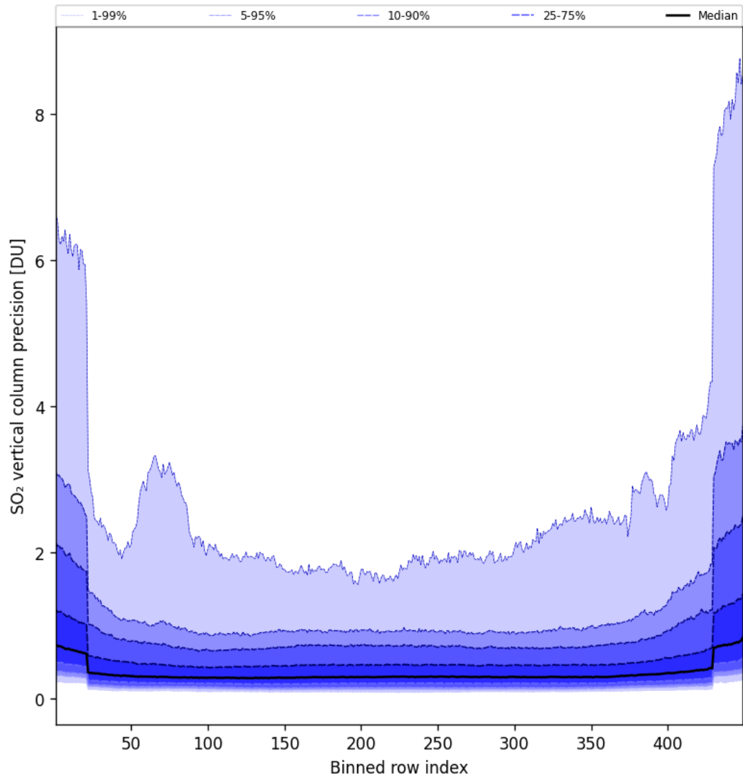
Figure 86: Along track statistics of “SO 2 vertical column precision” for 2025-09-12 to 2025-09-13
