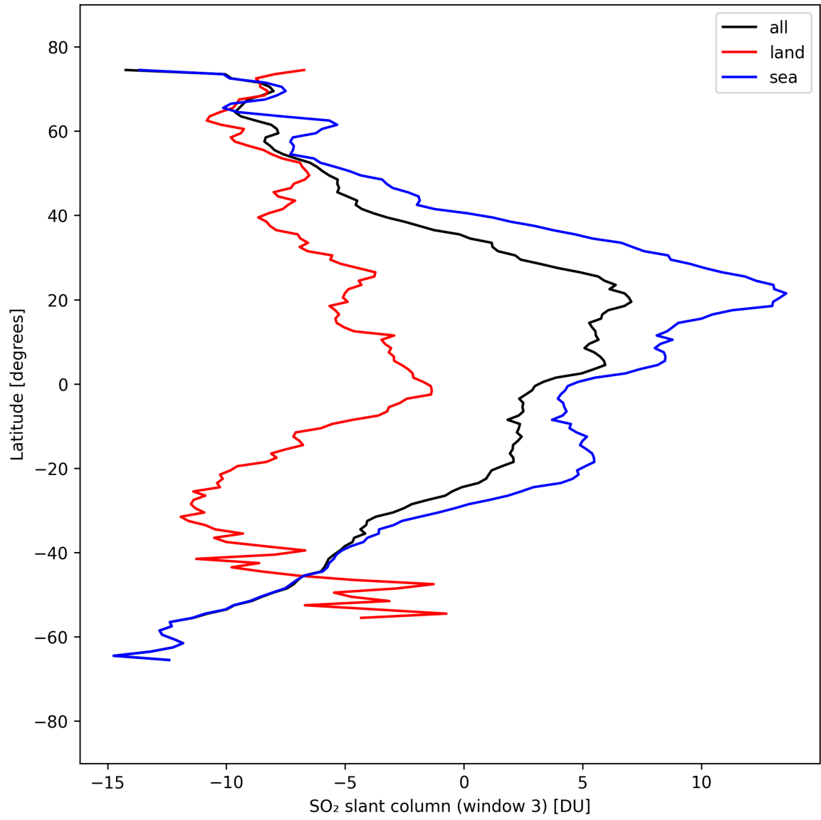
Figure 44: Zonal average of “SO 2 slant column (window 3)” for 2025-09-12 to 2025-09-13.
