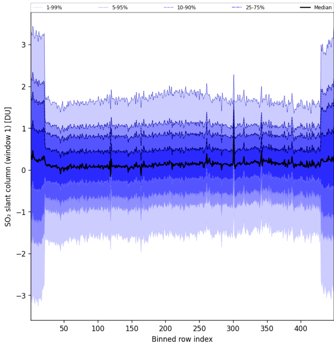
Figure 90: Along track statistics of “SO 2 slant column (window 1)” for 2025-09-12 to 2025-09-13
