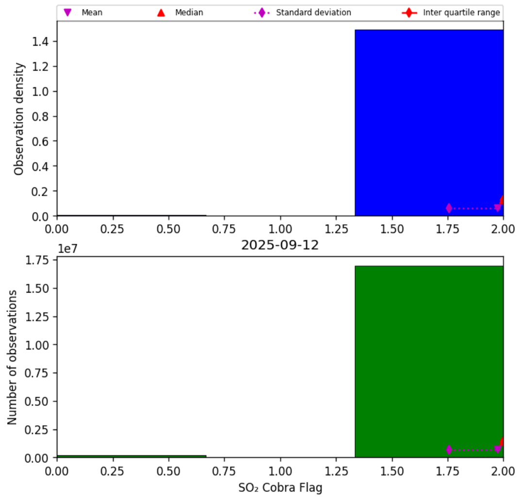
Figure 75: Histogram of "SO 2 Cobra Flag" for 2025-09-12 to 2025-09-13
