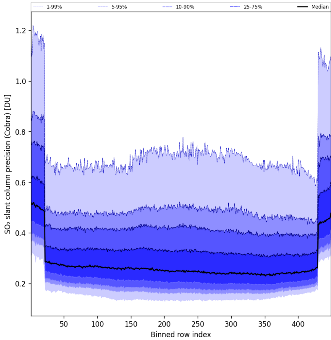
Figure 89: Along track statistics of “SO 2 slant column precision (Cobra)” for 2025-09-12 to 2025-09-13
