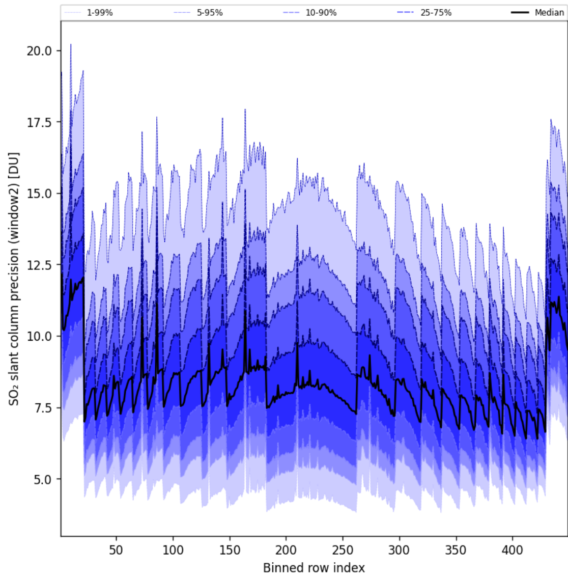
Figure 95: Along track statistics of “SO 2 slant column precision (window2)” for 2025-09-12 to 2025-09-13
