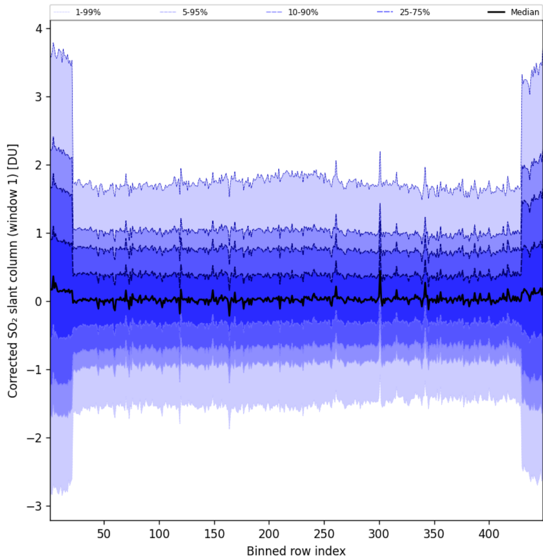
Figure 92: Along track statistics of “Corrected SO 2 slant column (window 1)” for 2025-09-12 to 2025-09-13
