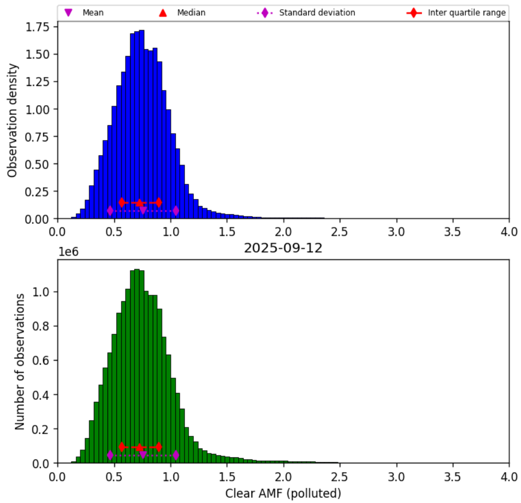
Figure 82: Histogram of “Clear AMF (polluted)” for 2025-09-12 to 2025-09-13
