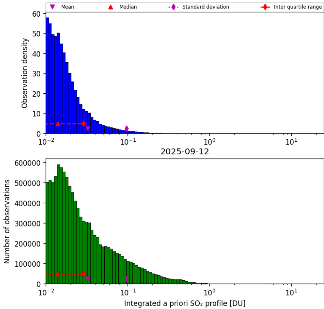
Figure 76: Histogram of “Integrated a priori SO 2 profile” for 2025-09-12 to 2025-09-13
