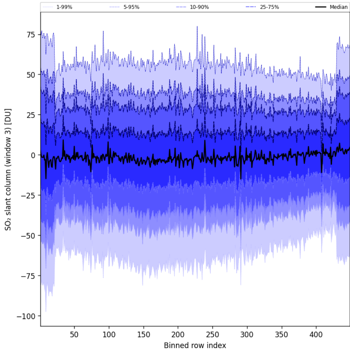
Figure 98: Along track statistics of “SO 2 slant column (window 3)” for 2025-09-12 to 2025-09-13
