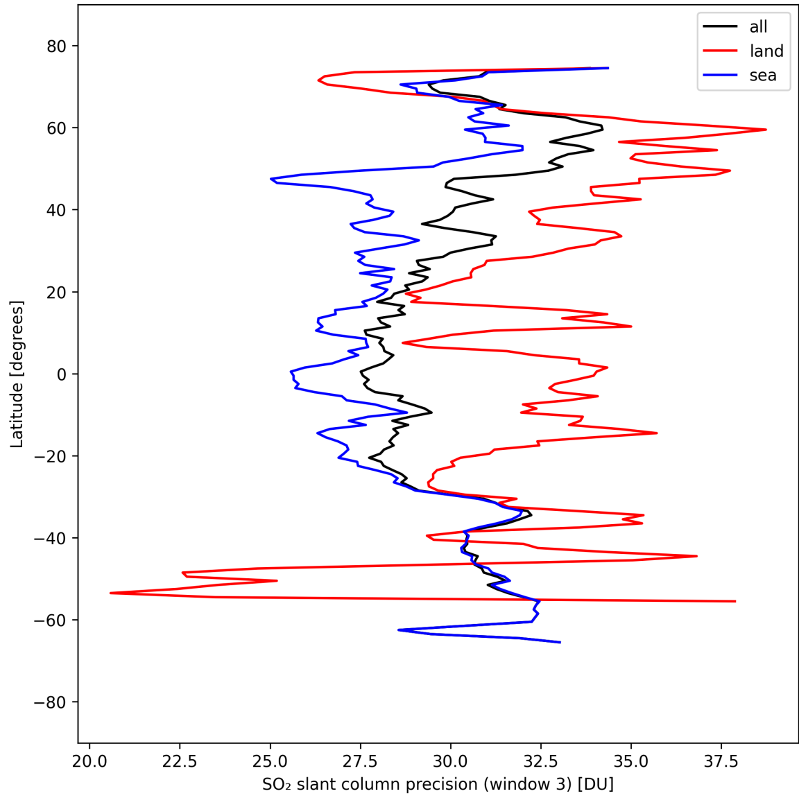
Figure 45: Zonal average of “SO 2 slant column precision (window 3)” for 2025-09-12 to 2025-09-13.
