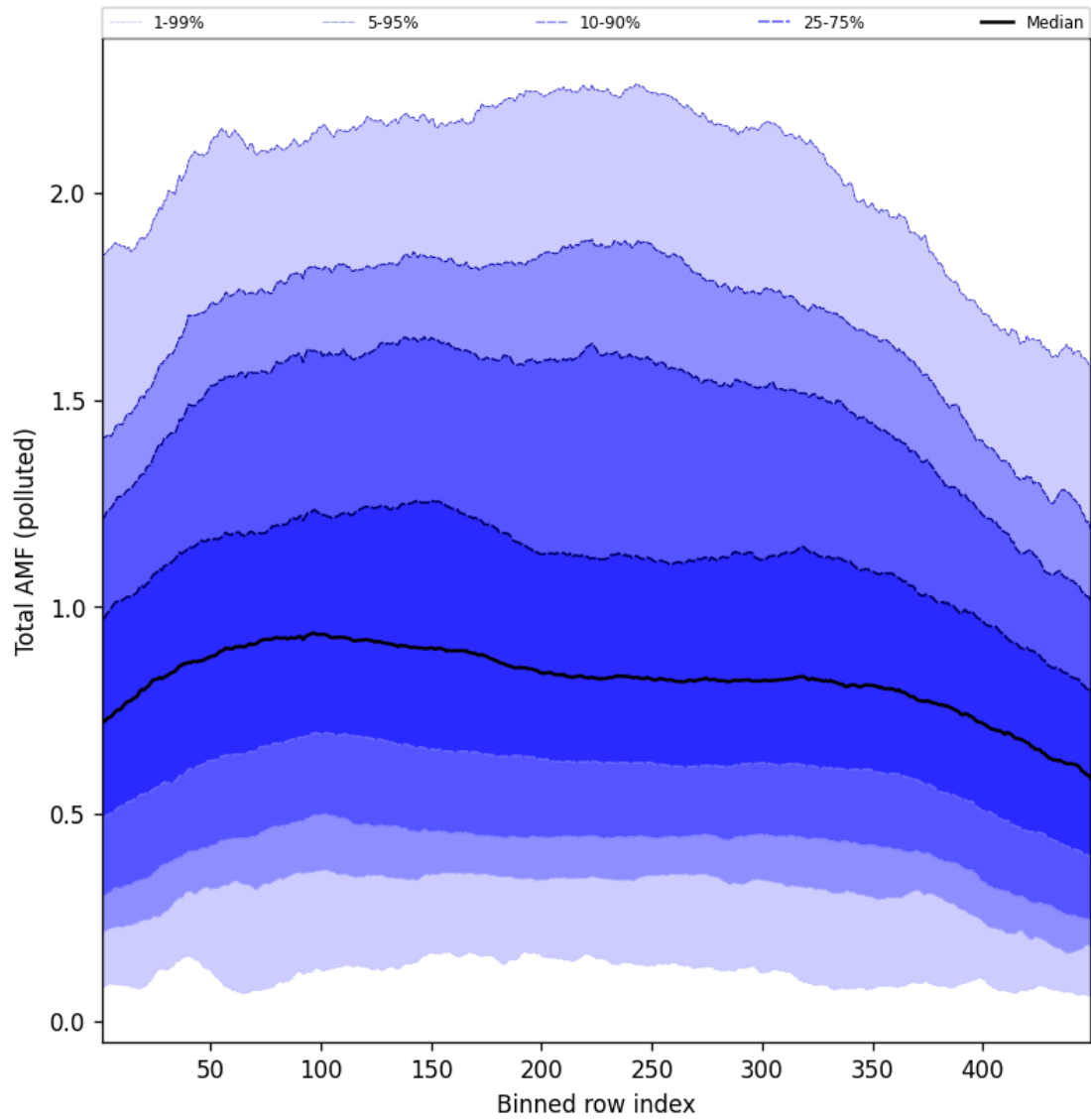
Figure 107: Along track statistics of “Total AMF (polluted)” for 2025-09-12 to 2025-09-13
