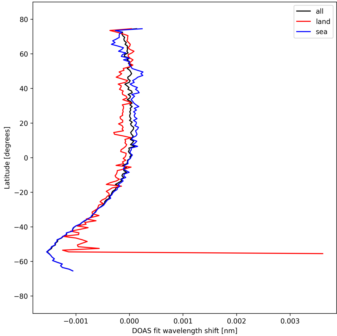
Figure 50: Zonal average of “DOAS fit wavelength shift” for 2025-09-12 to 2025-09-13.
