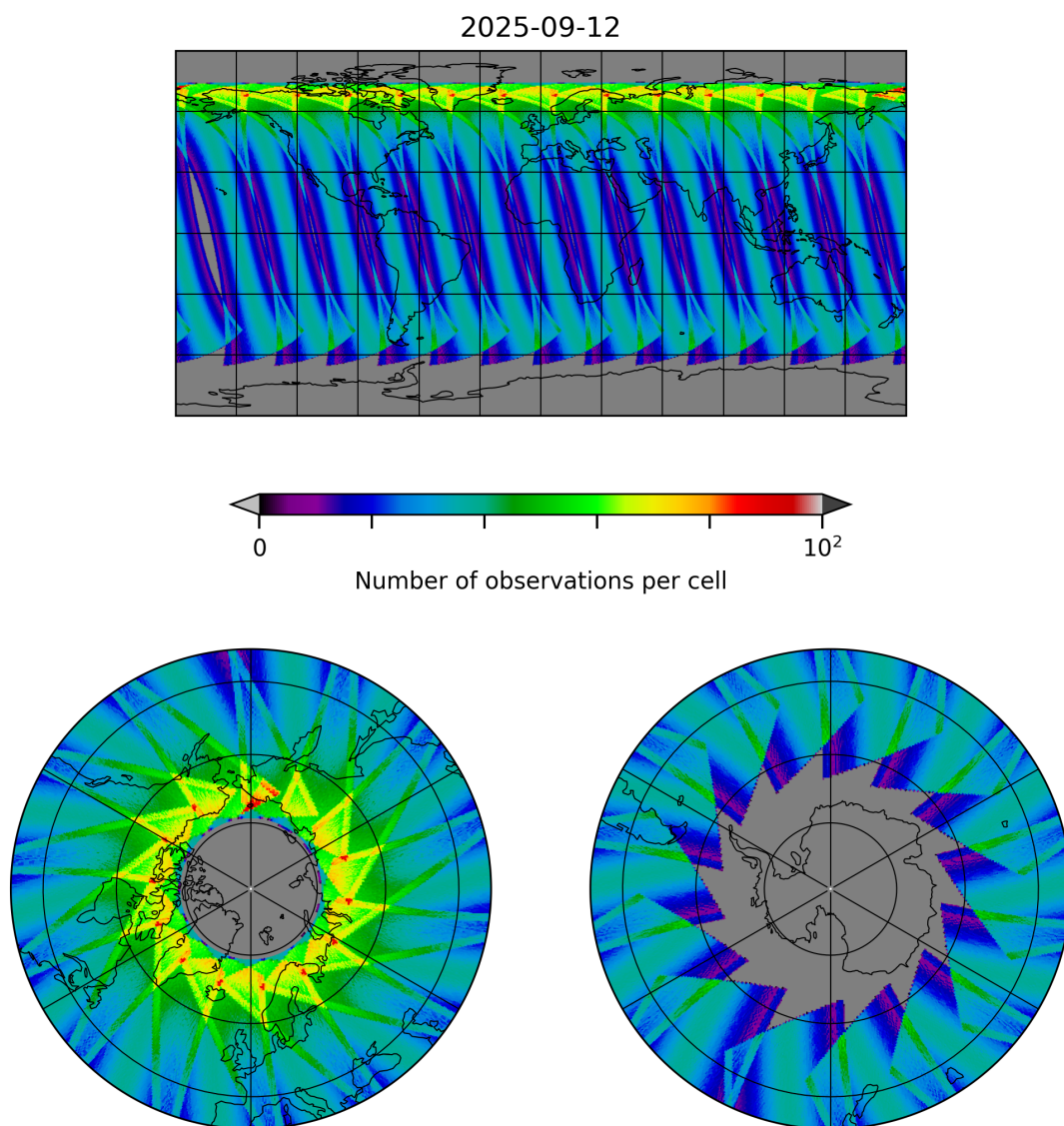
Figure 29: Map of the number of observations for 2025-09-12 to 2025-09-13
