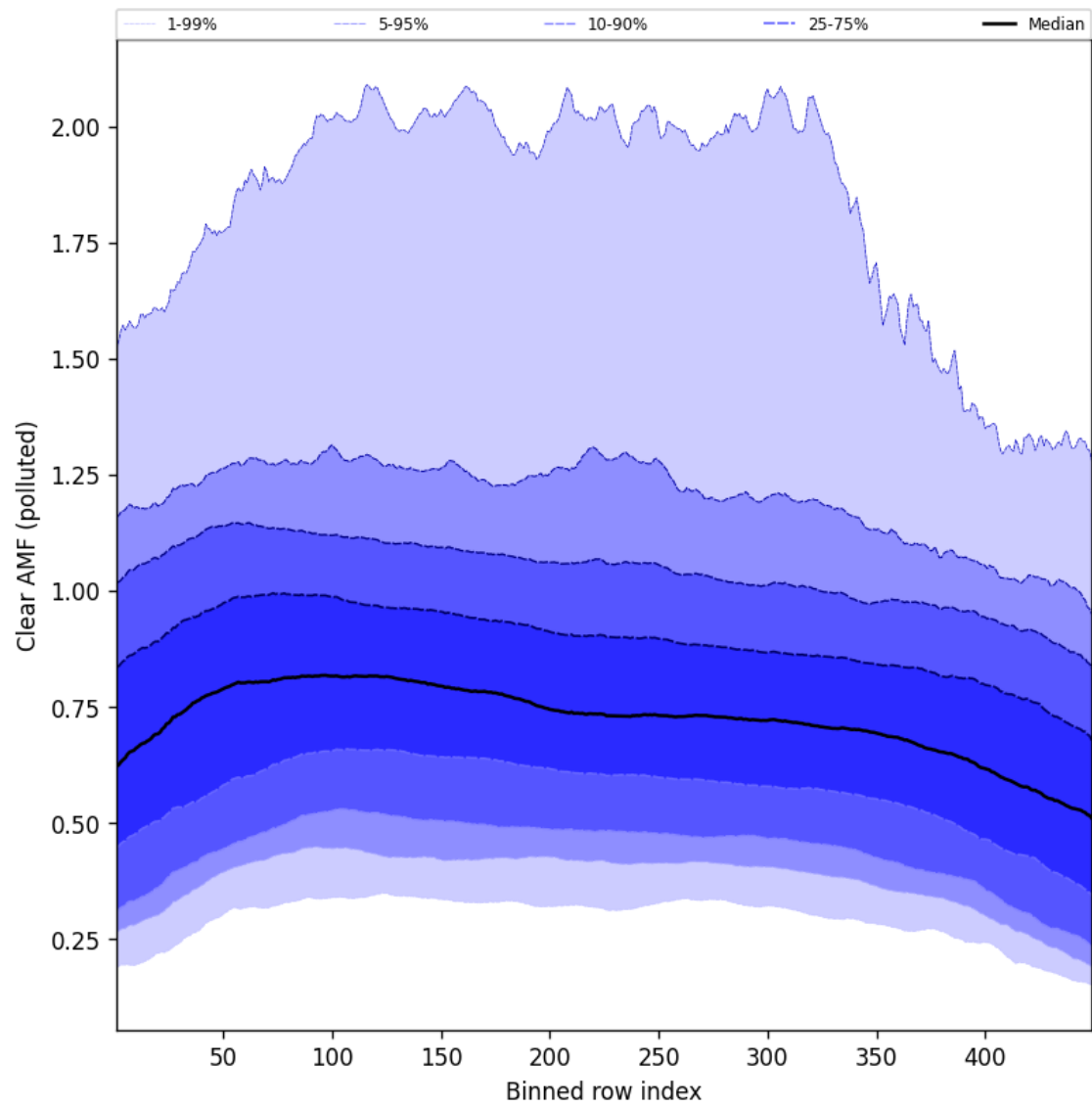
Figure 109: Along track statistics of “Clear AMF (polluted)” for 2025-09-12 to 2025-09-13
