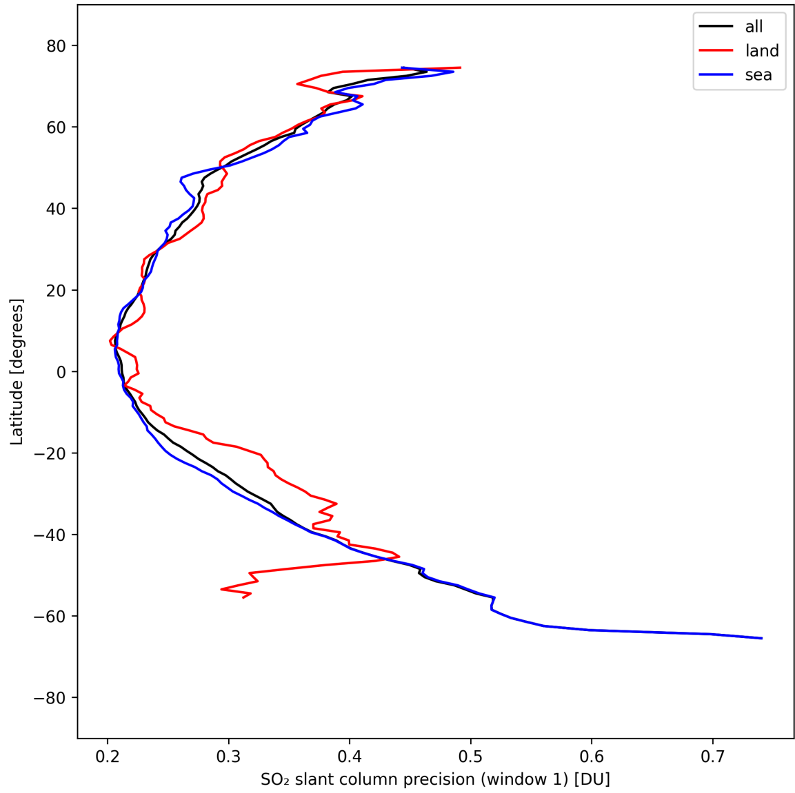
Figure 37: Zonal average of “SO 2 slant column precision (window 1)” for 2025-09-12 to 2025-09-13.
