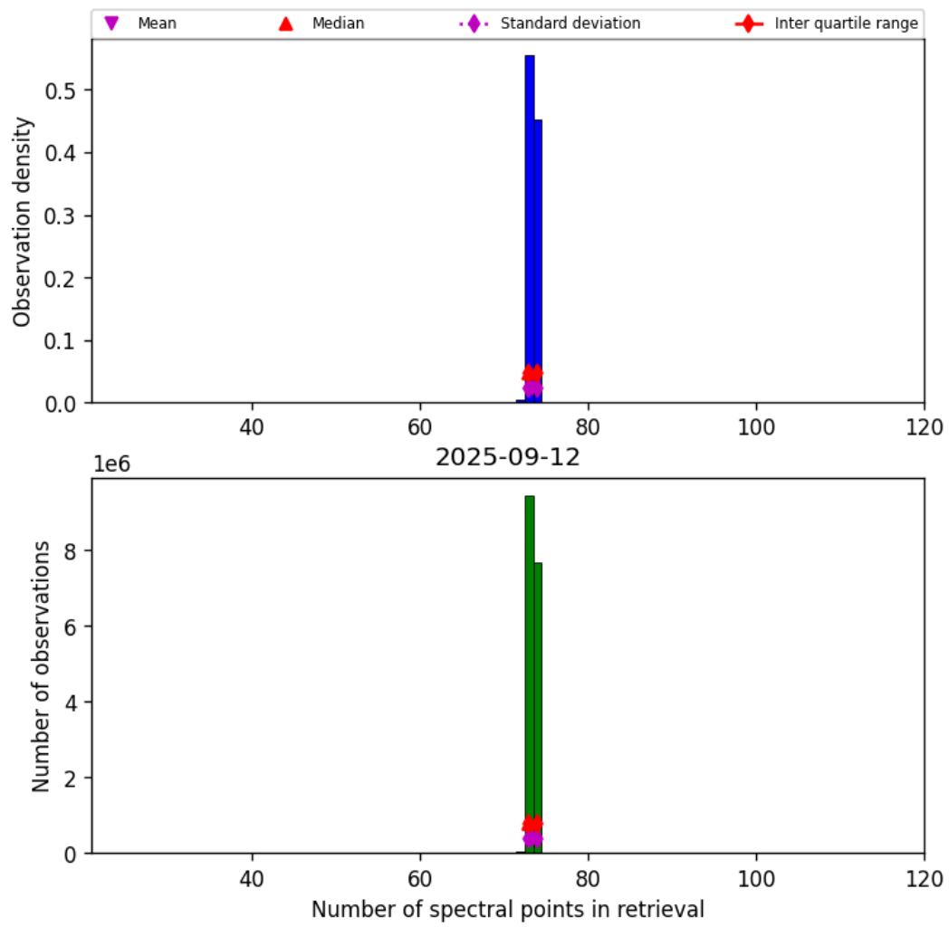
Figure 83: Histogram of "Number of spectral points in retrieval" for 2025-09-12 to 2025-09-13
