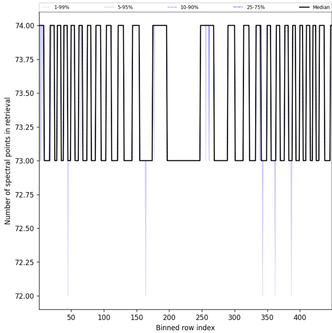
Figure 110: Along track statistics of “Number of spectral points in retrieval” for 2025-09-12 to 2025-09-13
