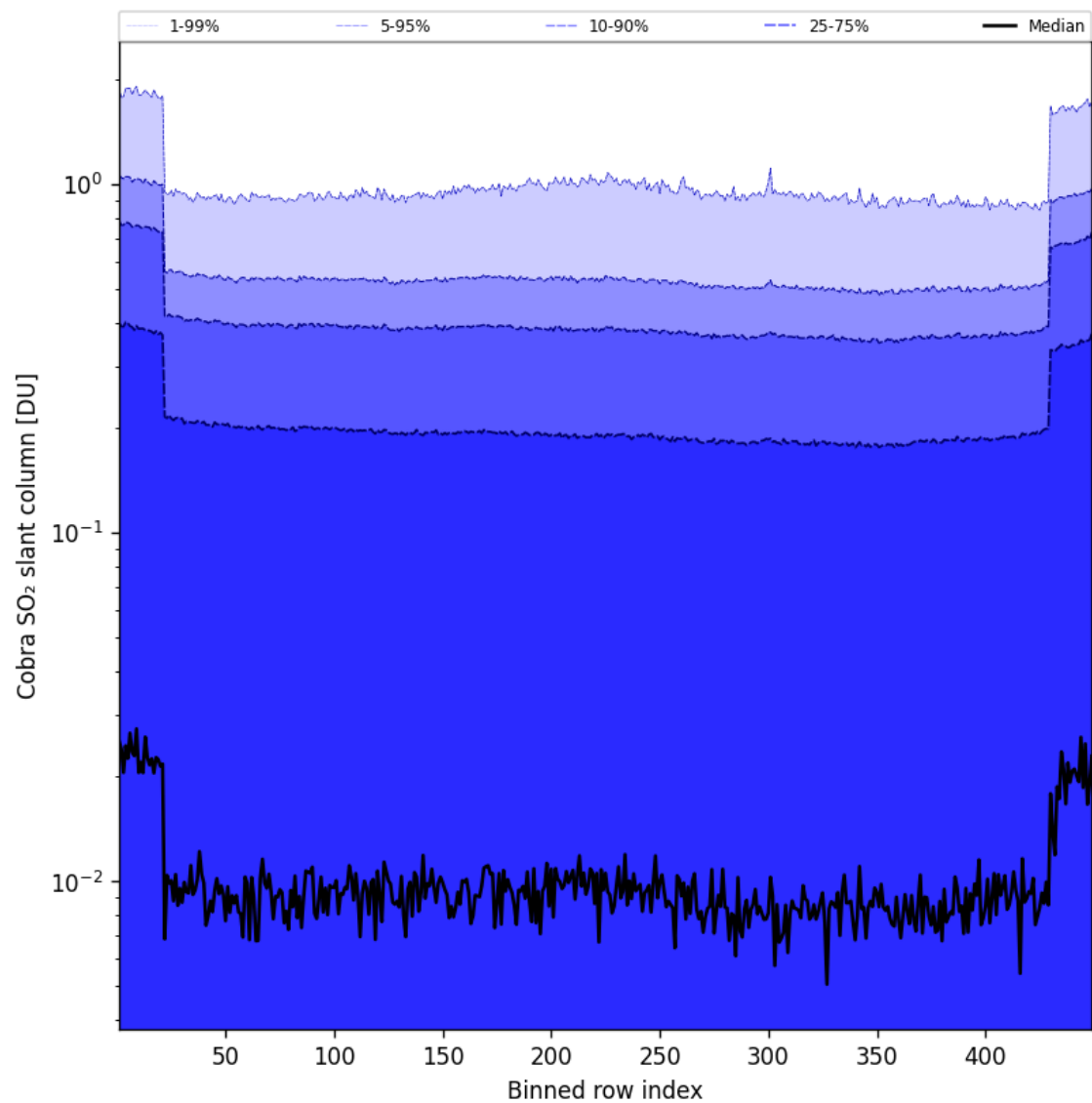
Figure 88: Along track statistics of “Cobra SO 2 slant column” for 2025-09-12 to 2025-09-13
