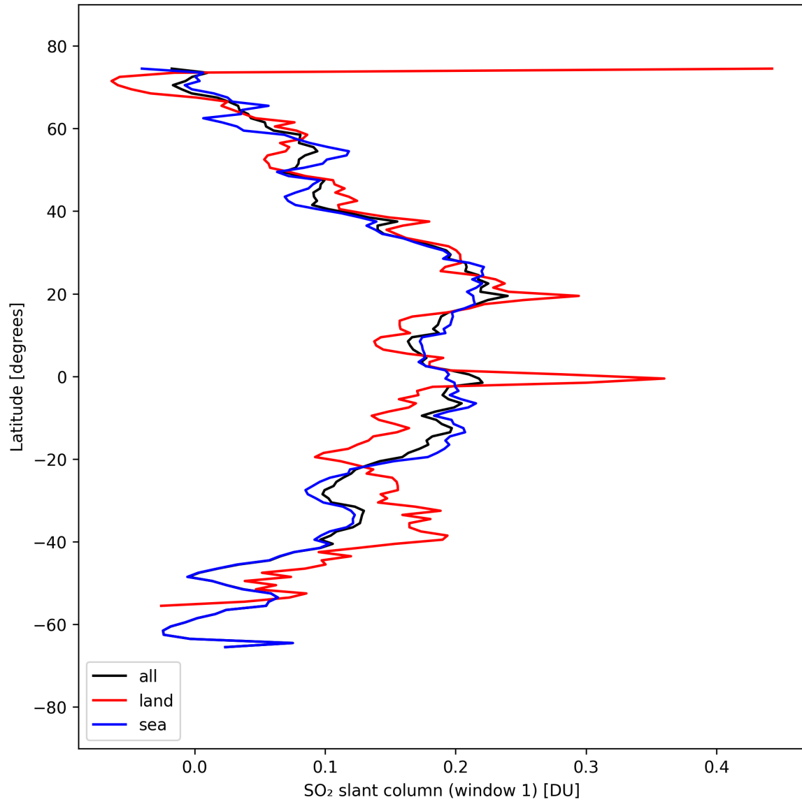
Figure 36: Zonal average of “SO 2 slant column (window 1)” for 2025-09-12 to 2025-09-13.
