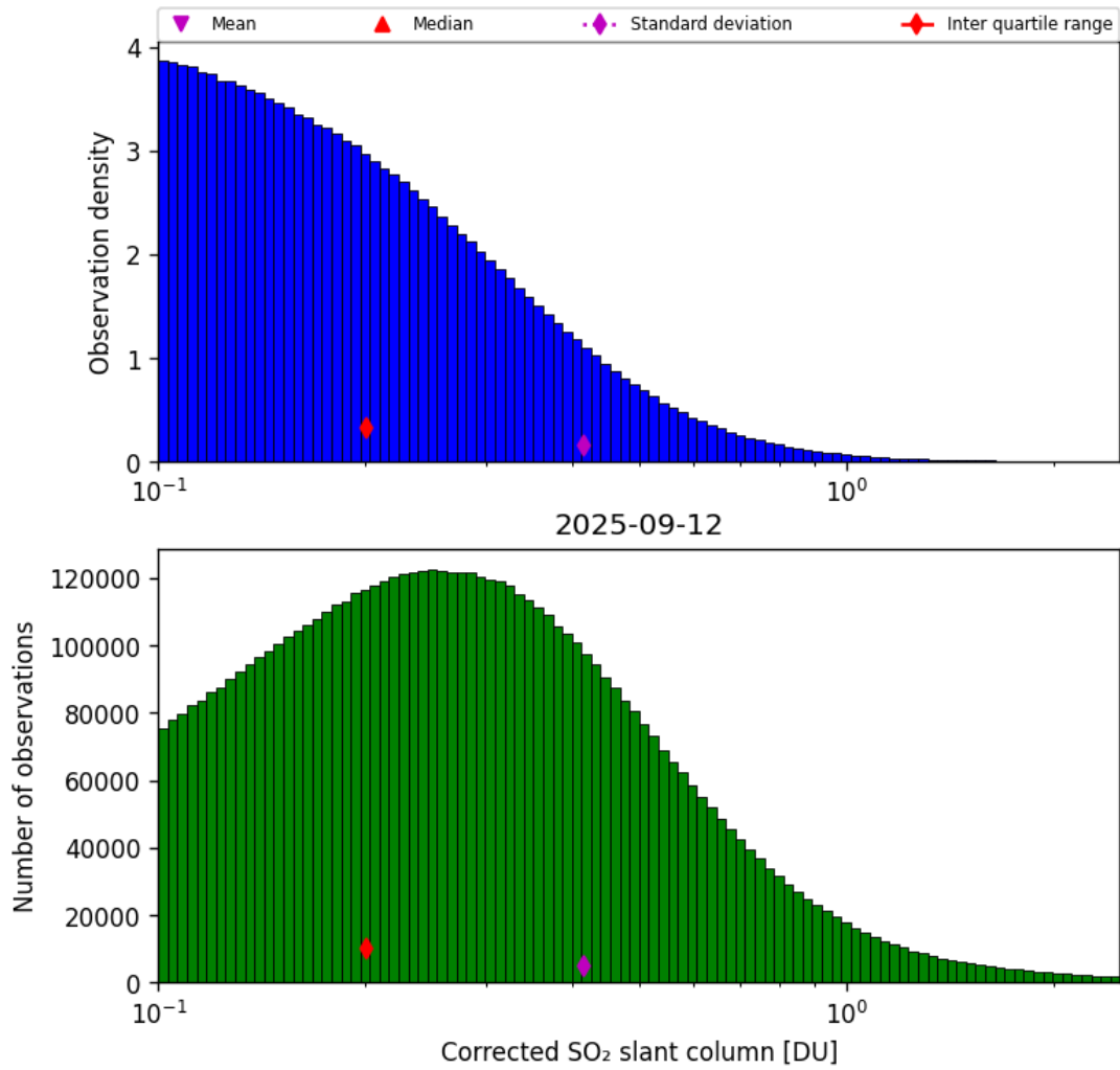
Figure 60: Histogram of “Corrected SO 2 slant column” for 2025-09-12 to 2025-09-13
