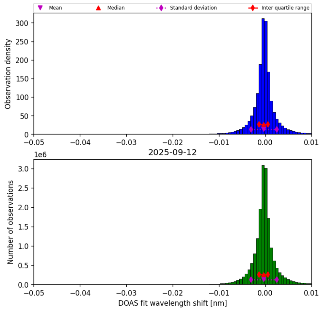
Figure 77: Histogram of “DOAS fit wavelength shift” for 2025-09-12 to 2025-09-13
