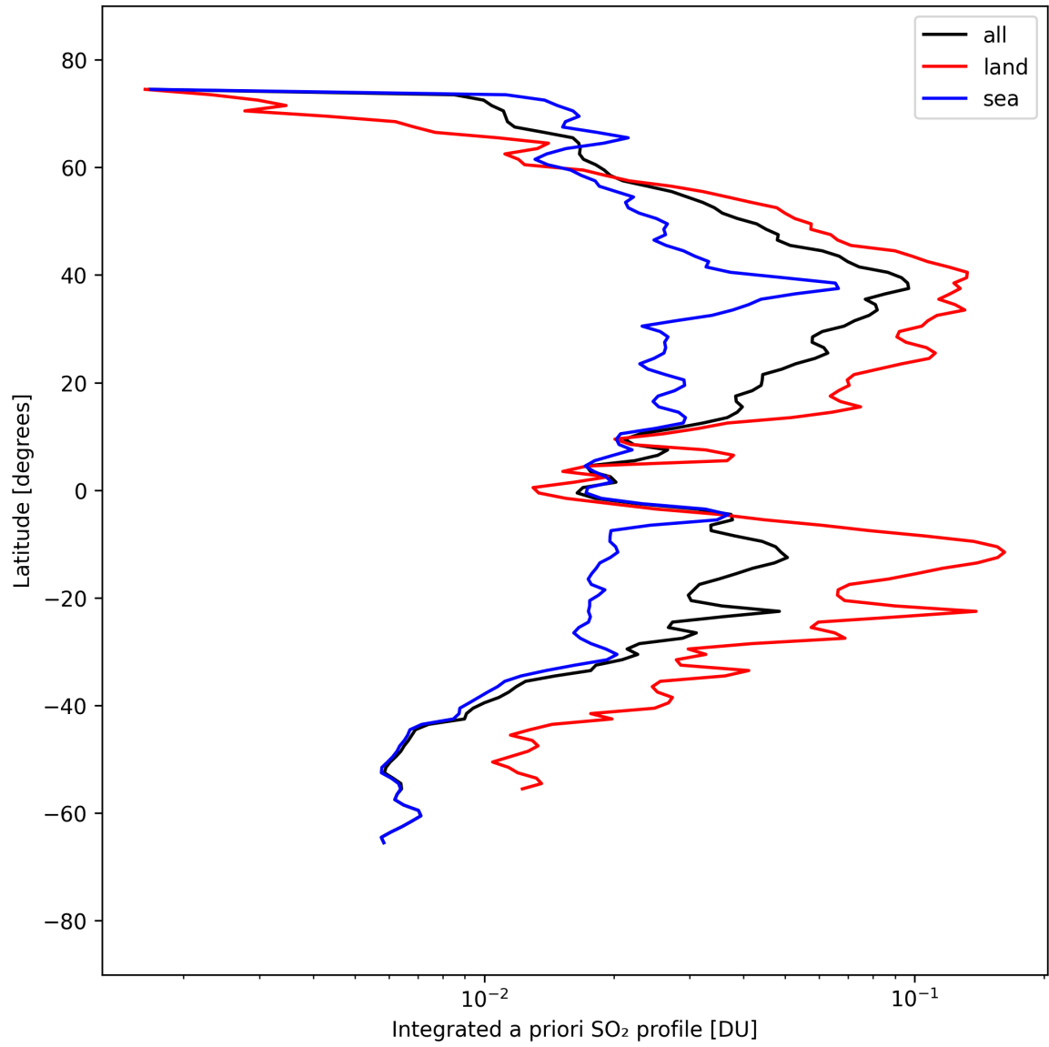
Figure 49: Zonal average of “Integrated a priori SO 2 profile” for 2025-09-12 to 2025-09-13.
