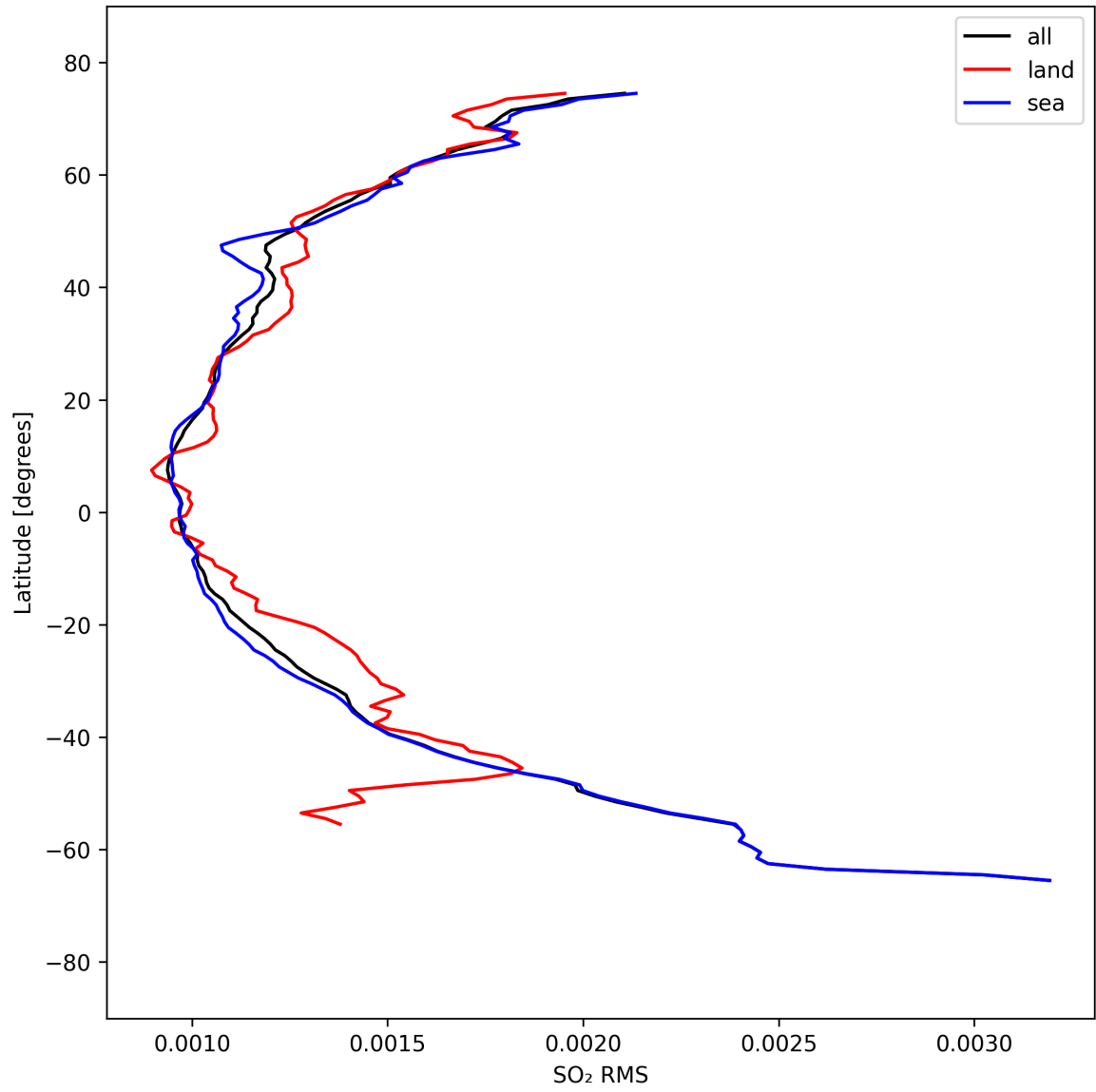
Figure 52: Zonal average of “SO 2 RMS” for 2025-09-12 to 2025-09-13.
