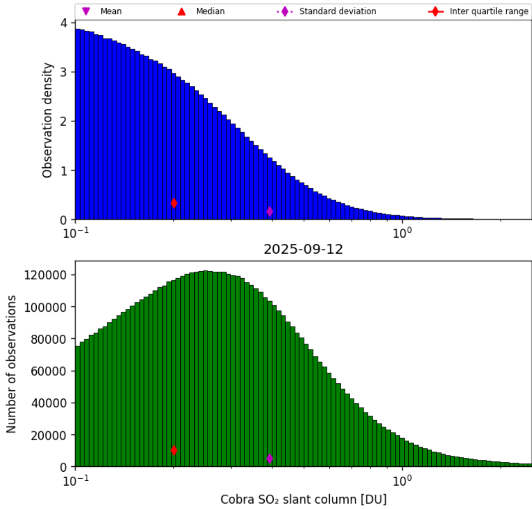
Figure 61: Histogram of “Cobra SO 2 slant column” for 2025-09-12 to 2025-09-13
