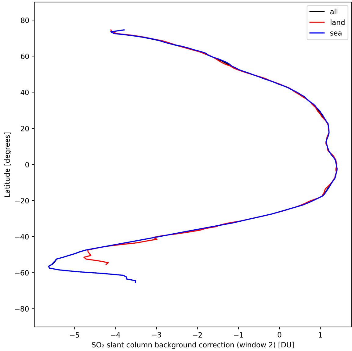
Figure 43: Zonal average of “SO 2 slant column background correction (window 2)” for 2025-09-12 to 2025-09-13.
