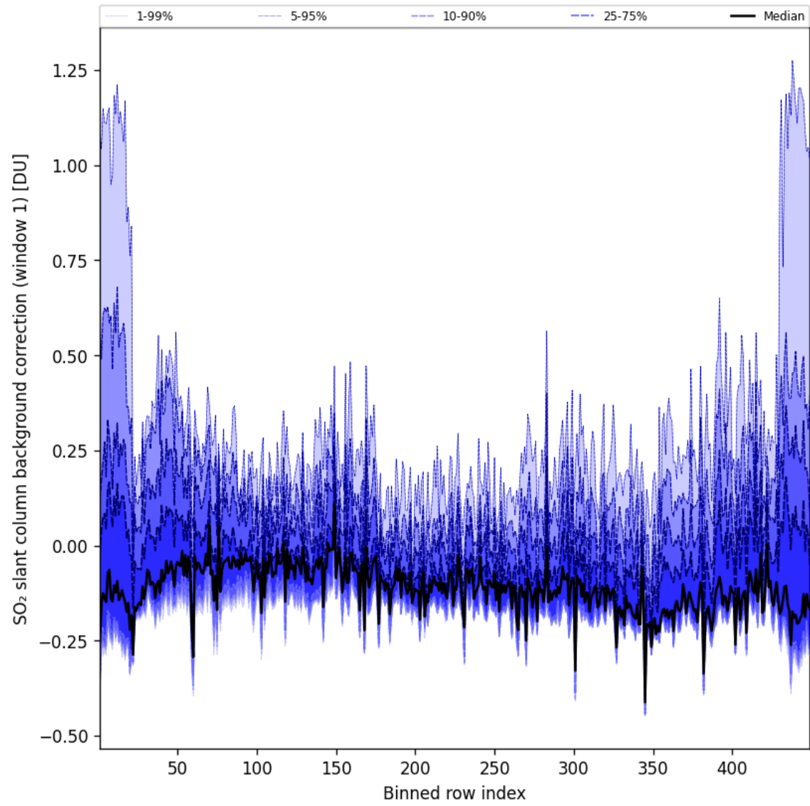
Figure 93: Along track statistics of “SO 2 slant column background correction (window 1)” for 2025-09-12 to 2025-09-13
