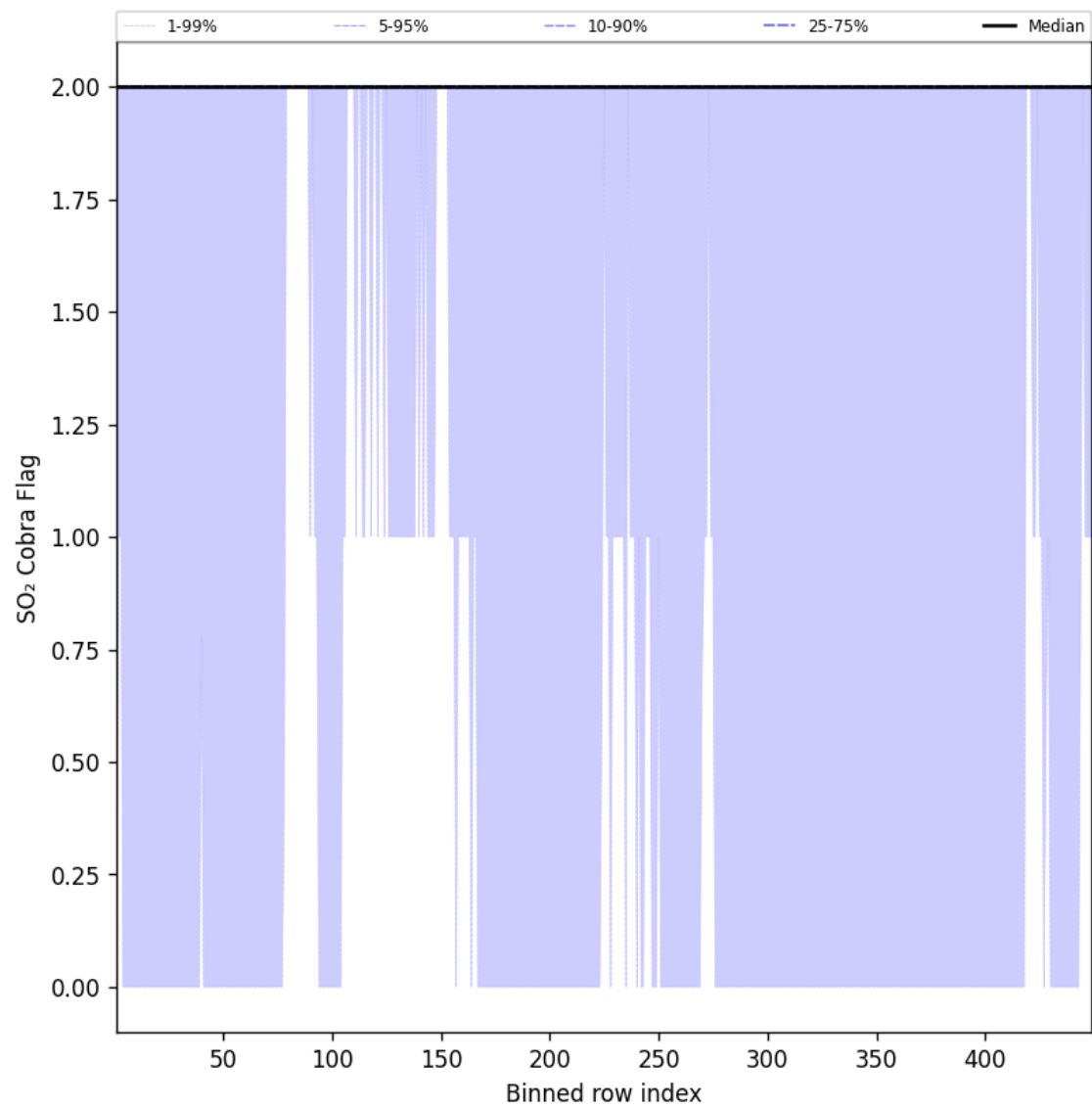
Figure 102: Along track statistics of “SO 2 Cobra Flag” for 2025-09-12 to 2025-09-13
