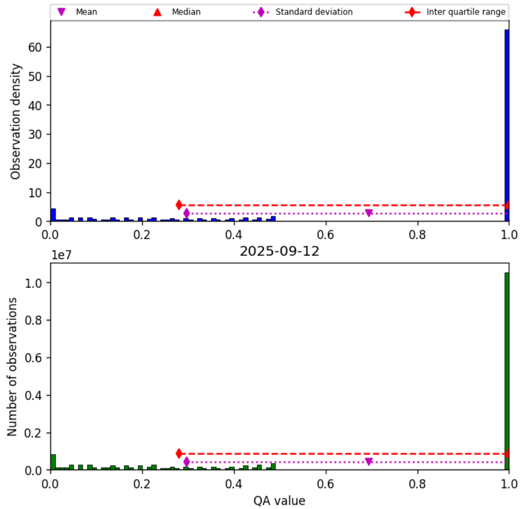
Figure 57: Histogram of “QA value” for 2025-09-12 to 2025-09-13
