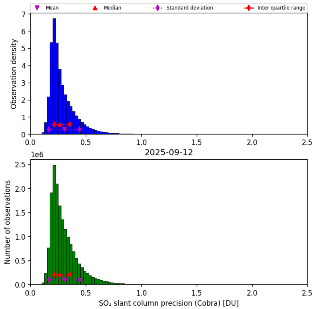
Figure 62: Histogram of “SO 2 slant column precision (Cobra)” for 2025-09-12 to 2025-09-13
