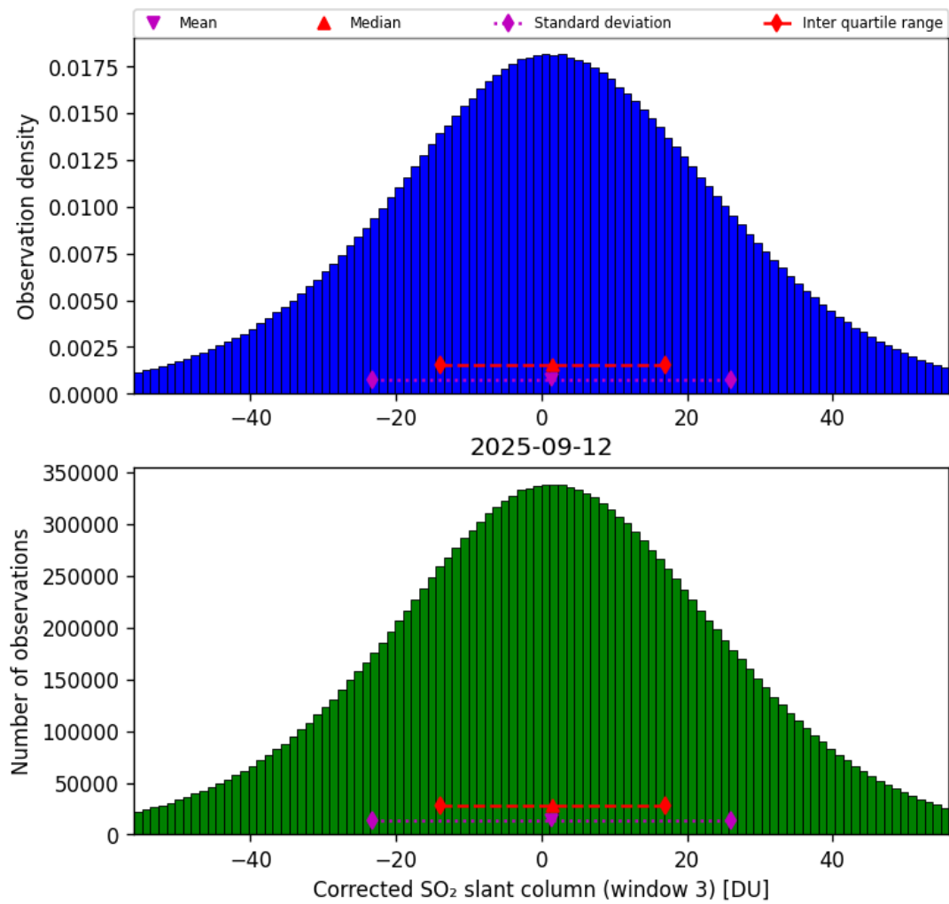
Figure 73: Histogram of “Corrected SO 2 slant column (window 3)” for 2025-09-12 to 2025-09-13
