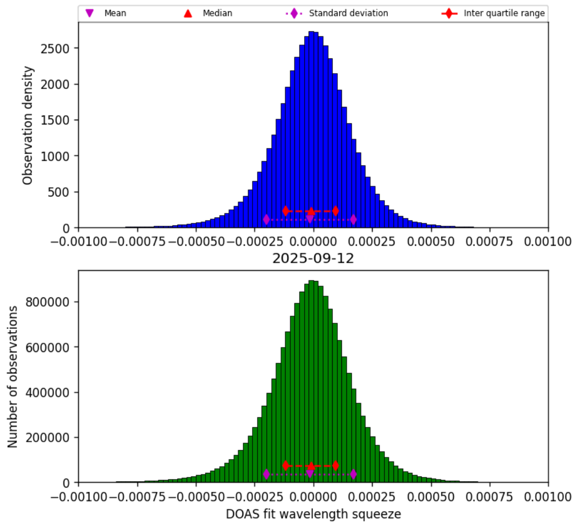
Figure 78: Histogram of “DOAS fit wavelength squeeze” for 2025-09-12 to 2025-09-13
