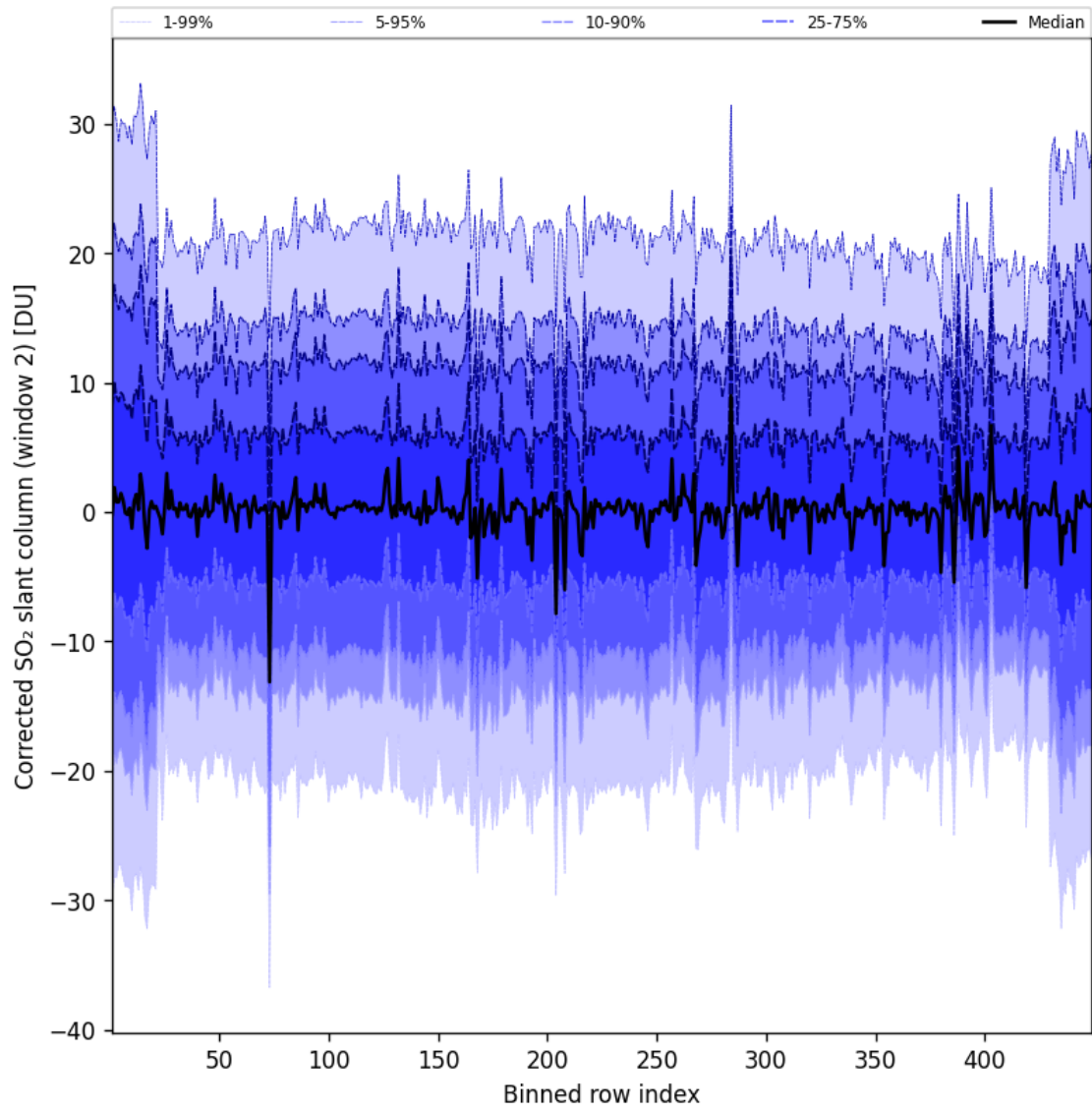
Figure 96: Along track statistics of "Corrected SO 2 slant column (window 2)" for 2025-09-12 to 2025-09-13
