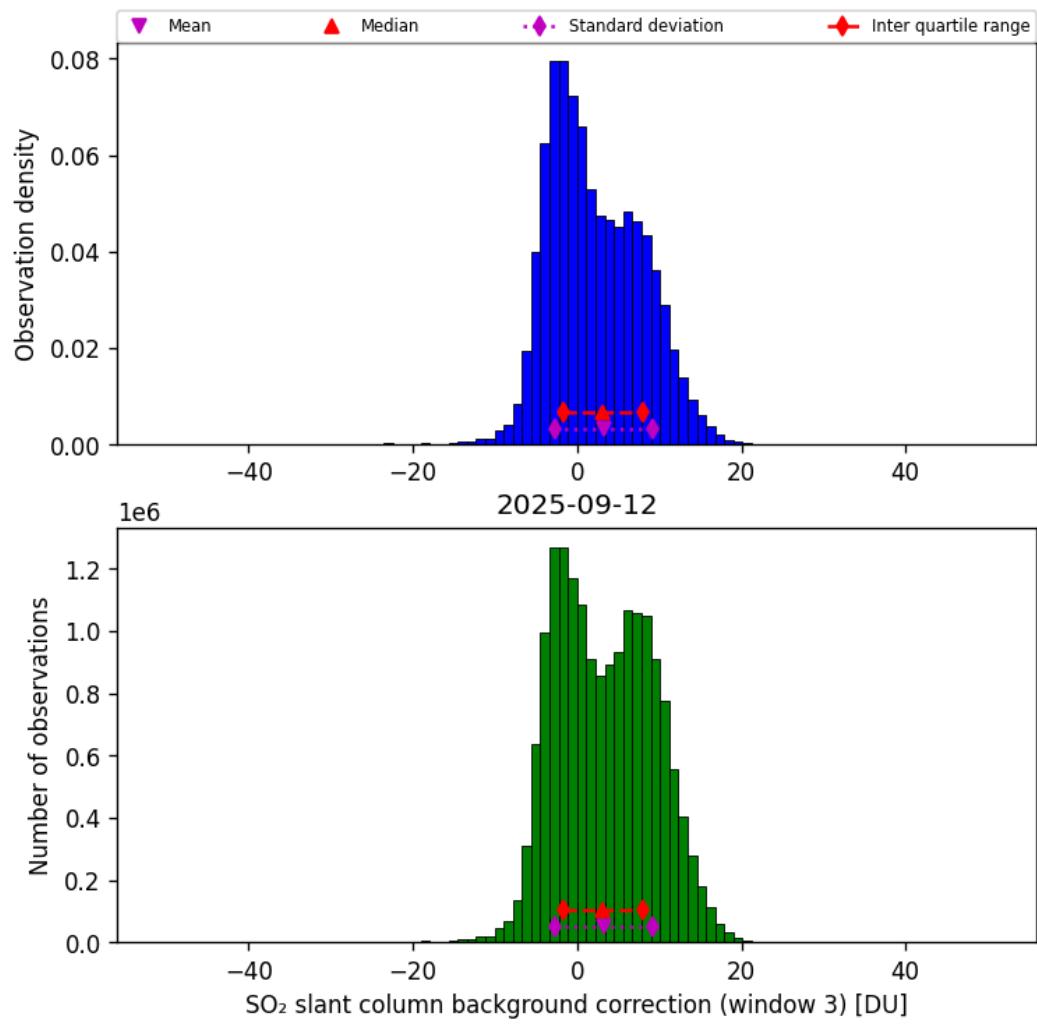
Figure 74: Histogram of “SO 2 slant column background correction (window 3)” for 2025-09-12 to 2025-09-13
