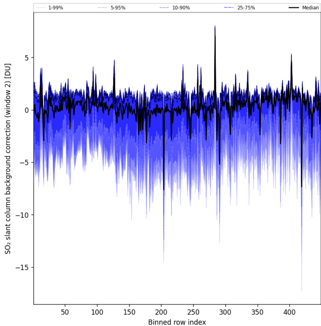
Figure 97: Along track statistics of “SO 2 slant column background correction (window 2)” for 2025-09-12 to 2025-09-13
