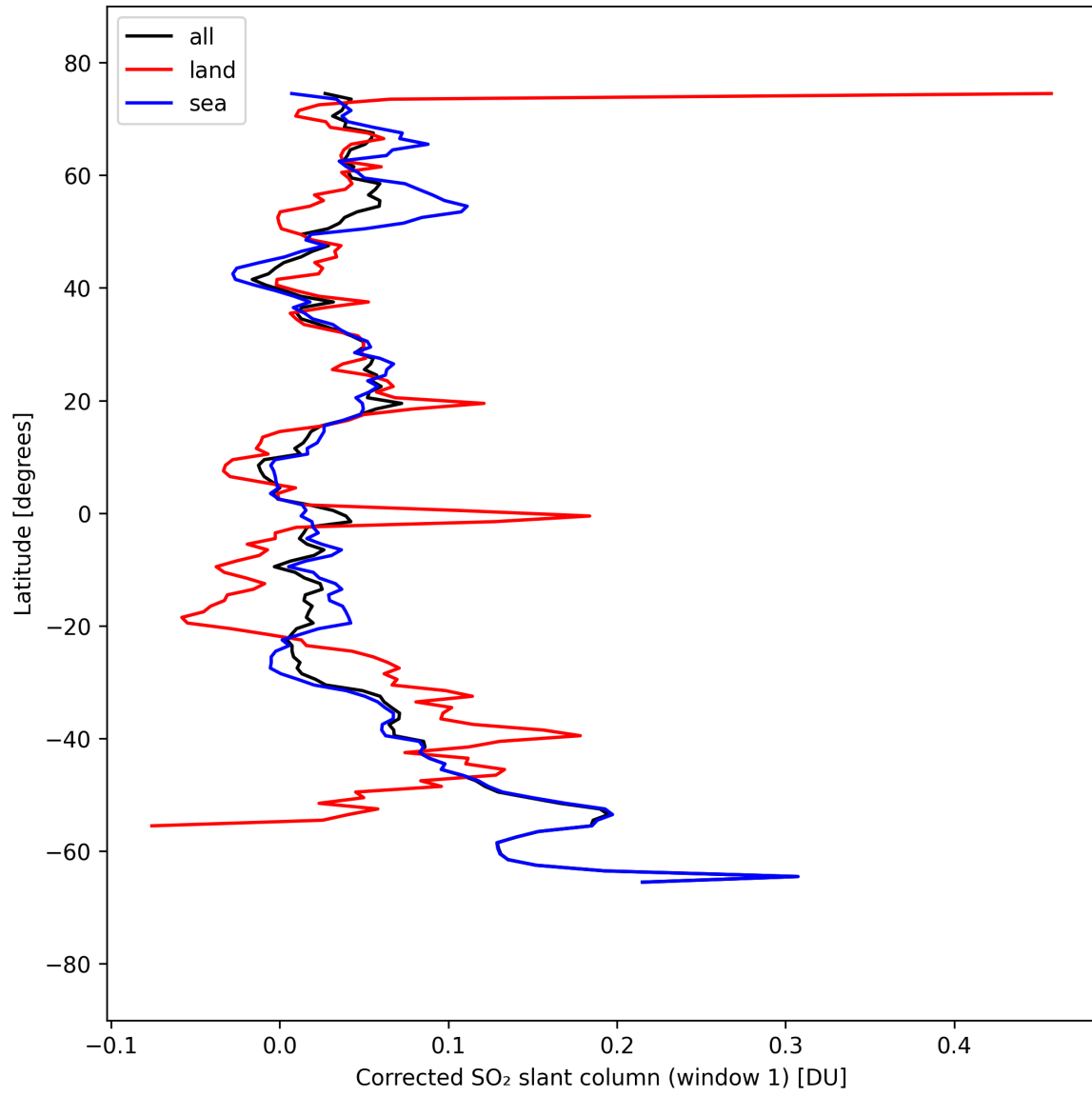
Figure 38: Zonal average of “Corrected SO 2 slant column (window 1)” for 2025-09-12 to 2025-09-13.
