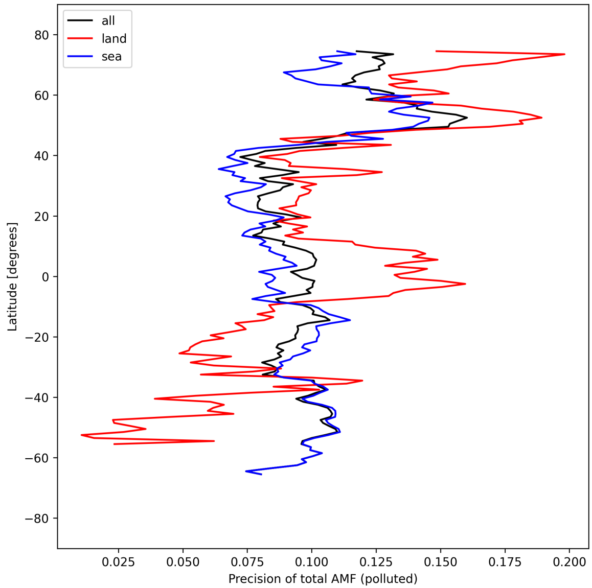
Figure 54: Zonal average of “Precision of total AMF (polluted)” for 2025-09-12 to 2025-09-13.
