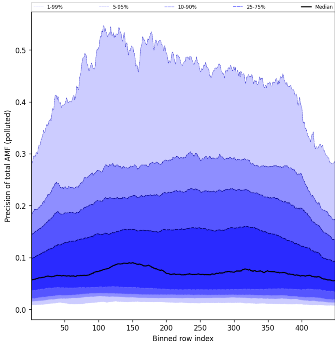
Figure 108: Along track statistics of “Precision of total AMF (polluted)” for 2025-09-12 to 2025-09-13
