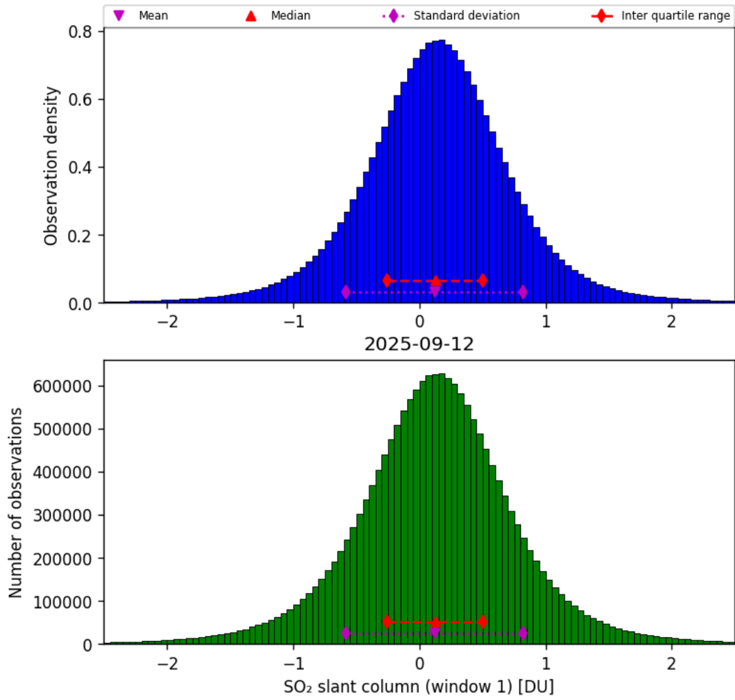
Figure 63: Histogram of “SO 2 slant column (window 1)” for 2025-09-12 to 2025-09-13
