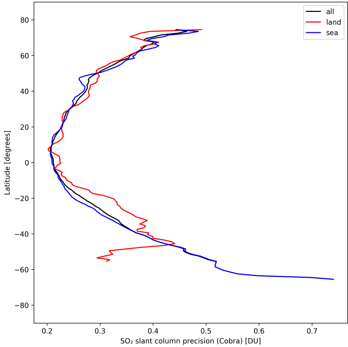
Figure 35: Zonal average of “SO 2 slant column precision (Cobra)” for 2025-09-12 to 2025-09-13.
