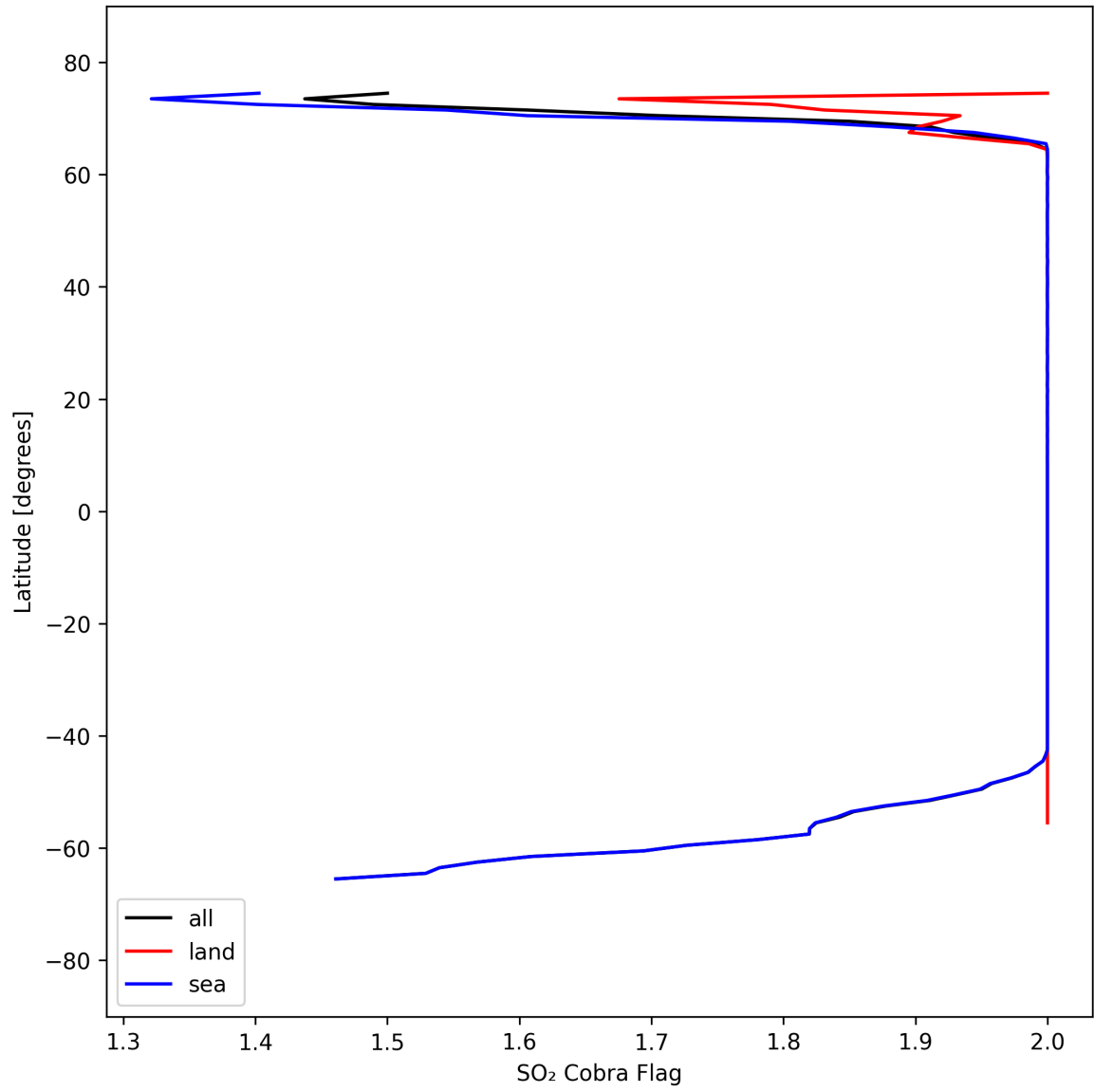
Figure 48: Zonal average of "SO 2 Cobra Flag" for 2025-09-12 to 2025-09-13.
