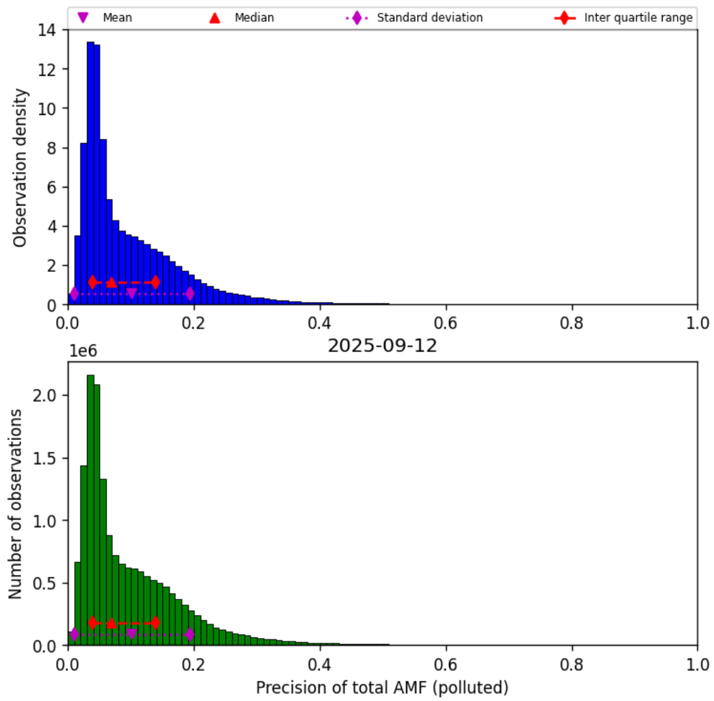
Figure 81: Histogram of “Precision of total AMF (polluted)” for 2025-09-12 to 2025-09-13
