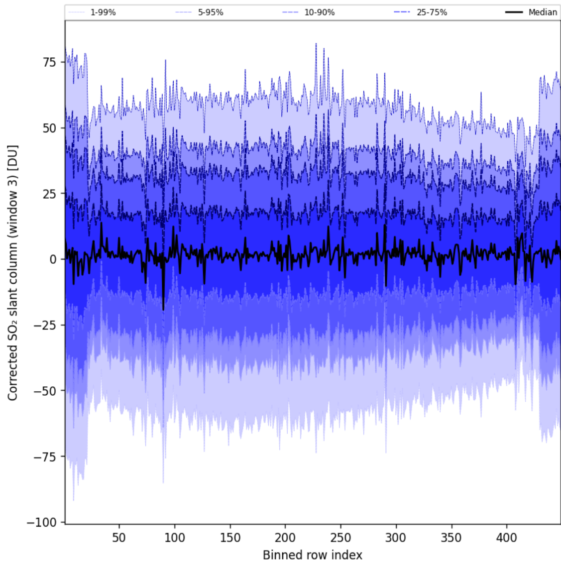
Figure 100: Along track statistics of “Corrected SO 2 slant column (window 3)” for 2025-09-12 to 2025-09-13
