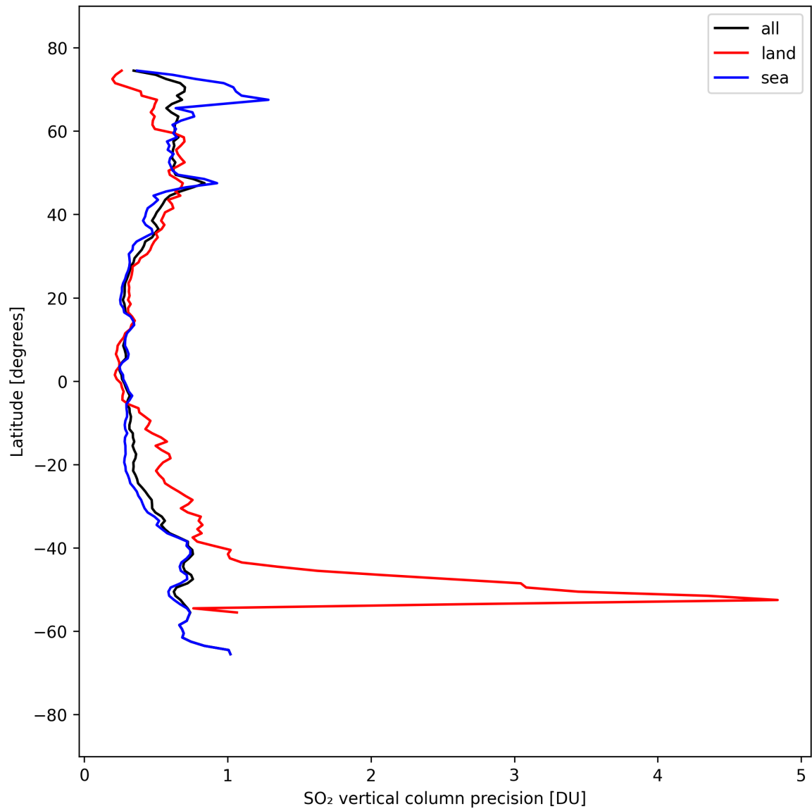
Figure 32: Zonal average of “SO 2 vertical column precision” for 2025-09-12 to 2025-09-13.
