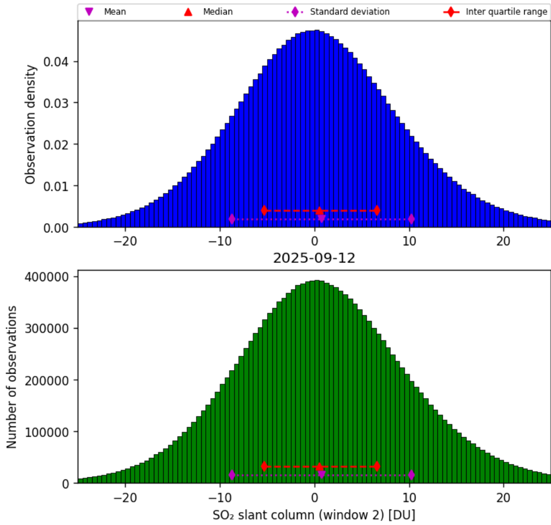
Figure 67: Histogram of “SO 2 slant column (window 2)” for 2025-09-12 to 2025-09-13
