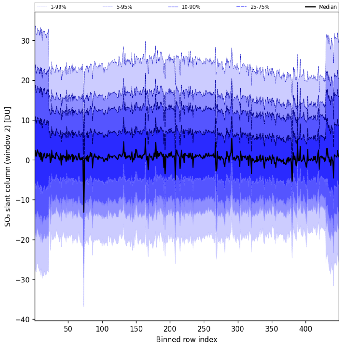
Figure 94: Along track statistics of “SO 2 slant column (window 2)” for 2025-09-12 to 2025-09-13
