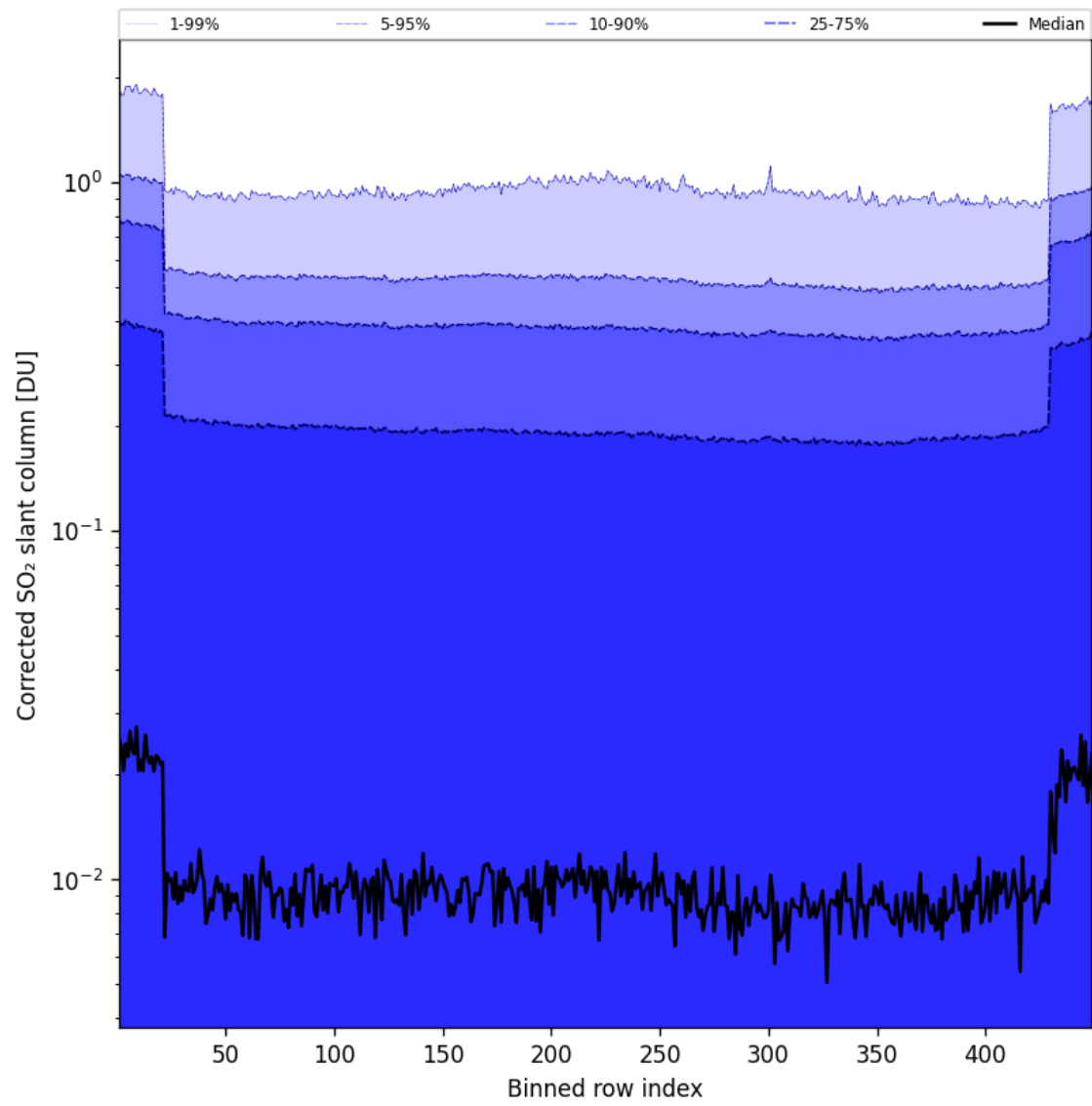
Figure 87: Along track statistics of “Corrected SO 2 slant column” for 2025-09-12 to 2025-09-13
