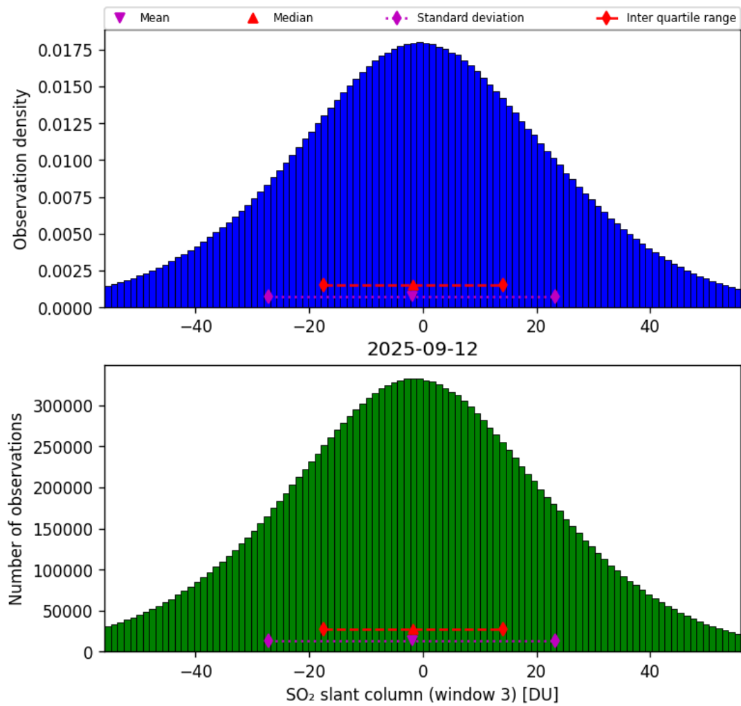
Figure 71: Histogram of “SO 2 slant column (window 3)” for 2025-09-12 to 2025-09-13
