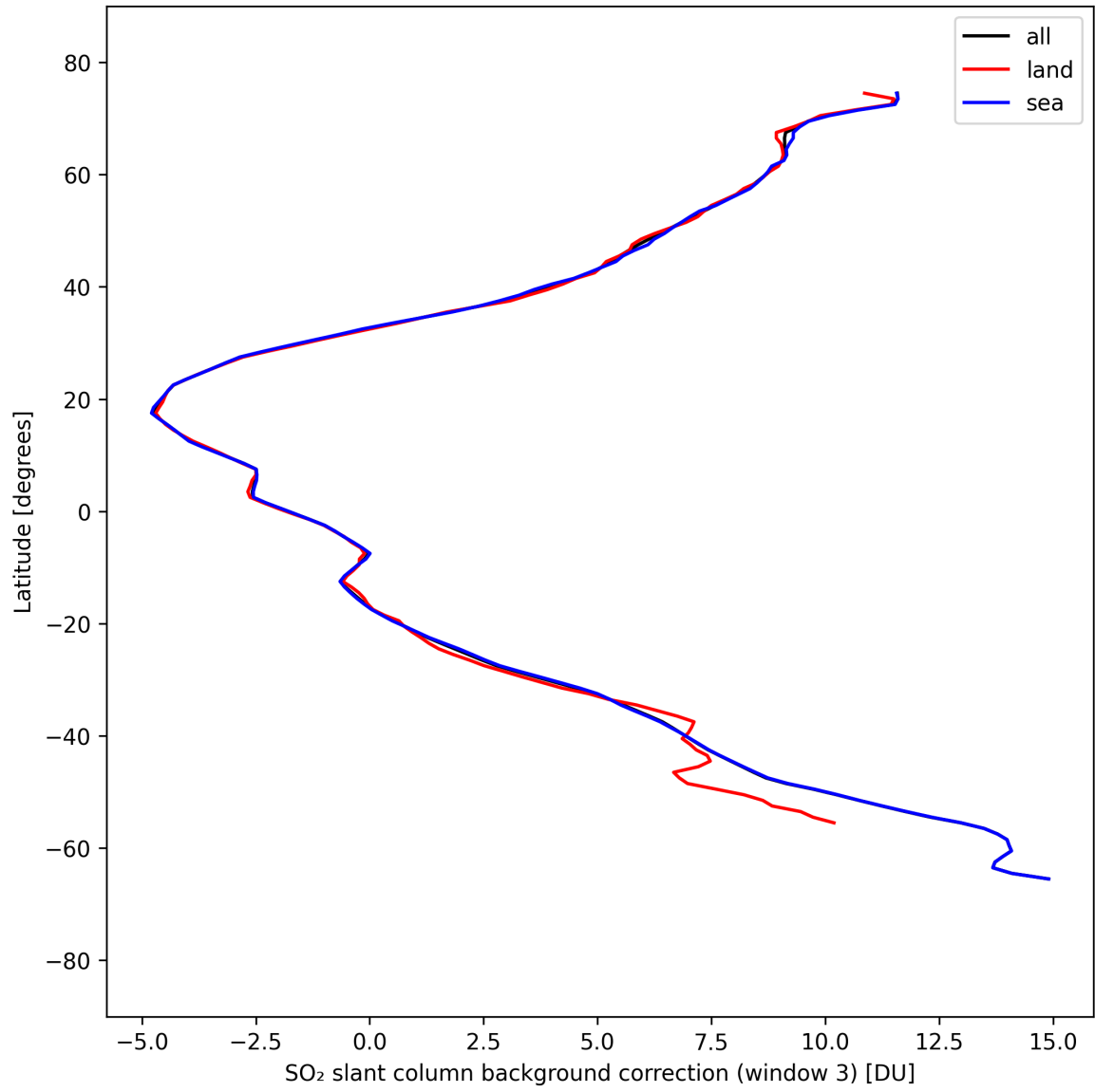
Figure 47: Zonal average of “SO 2 slant column background correction (window 3)” for 2025-09-12 to 2025-09-13.
