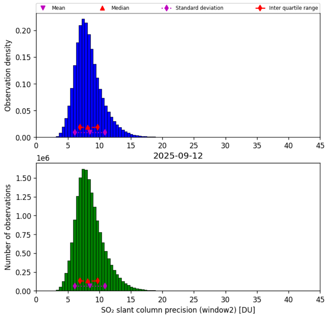
Figure 68: Histogram of “SO 2 slant column precision (window2)” for 2025-09-12 to 2025-09-13
