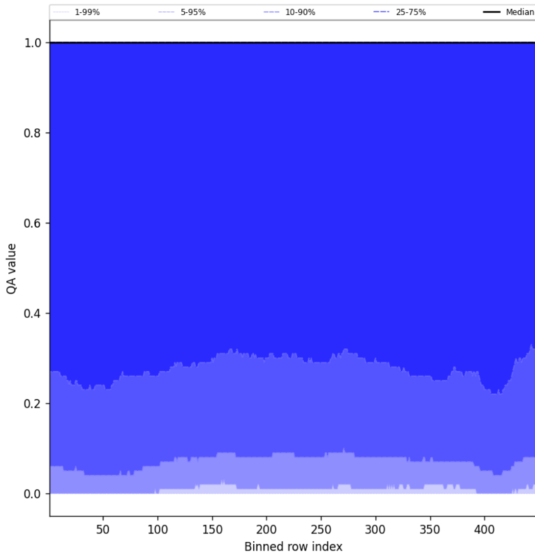
Figure 84: Along track statistics of “QA value” for 2025-09-12 to 2025-09-13
