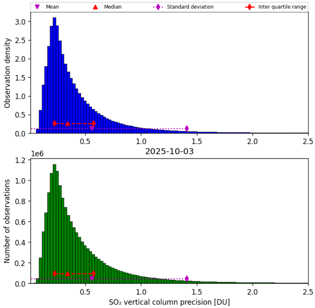
Figure 59: Histogram of “SO 2 vertical column precision” for 2025-10-03 to 2025-10-04
