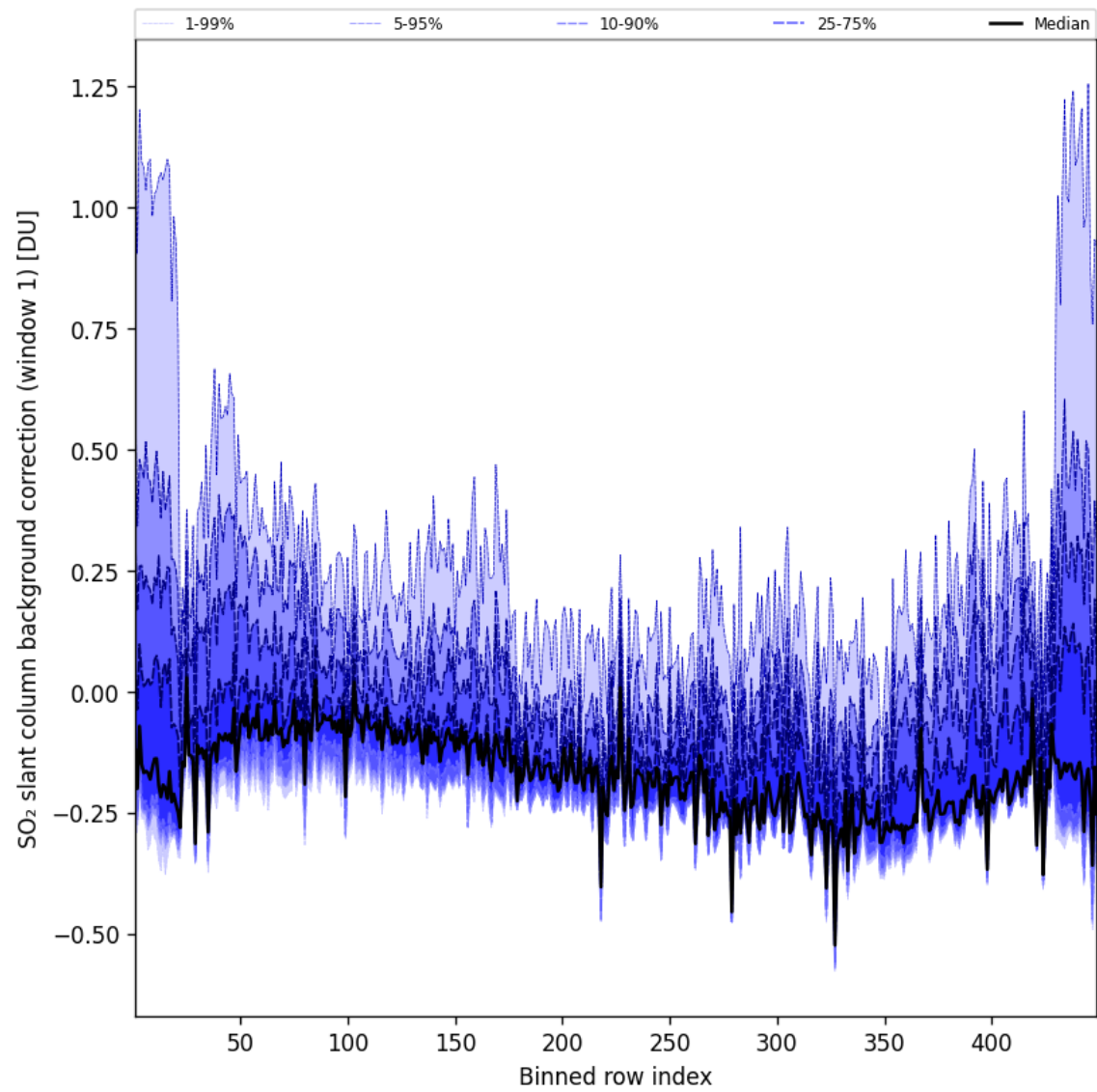
Figure 93: Along track statistics of “SO 2 slant column background correction (window 1)” for 2025-10-03 to 2025-10-04
