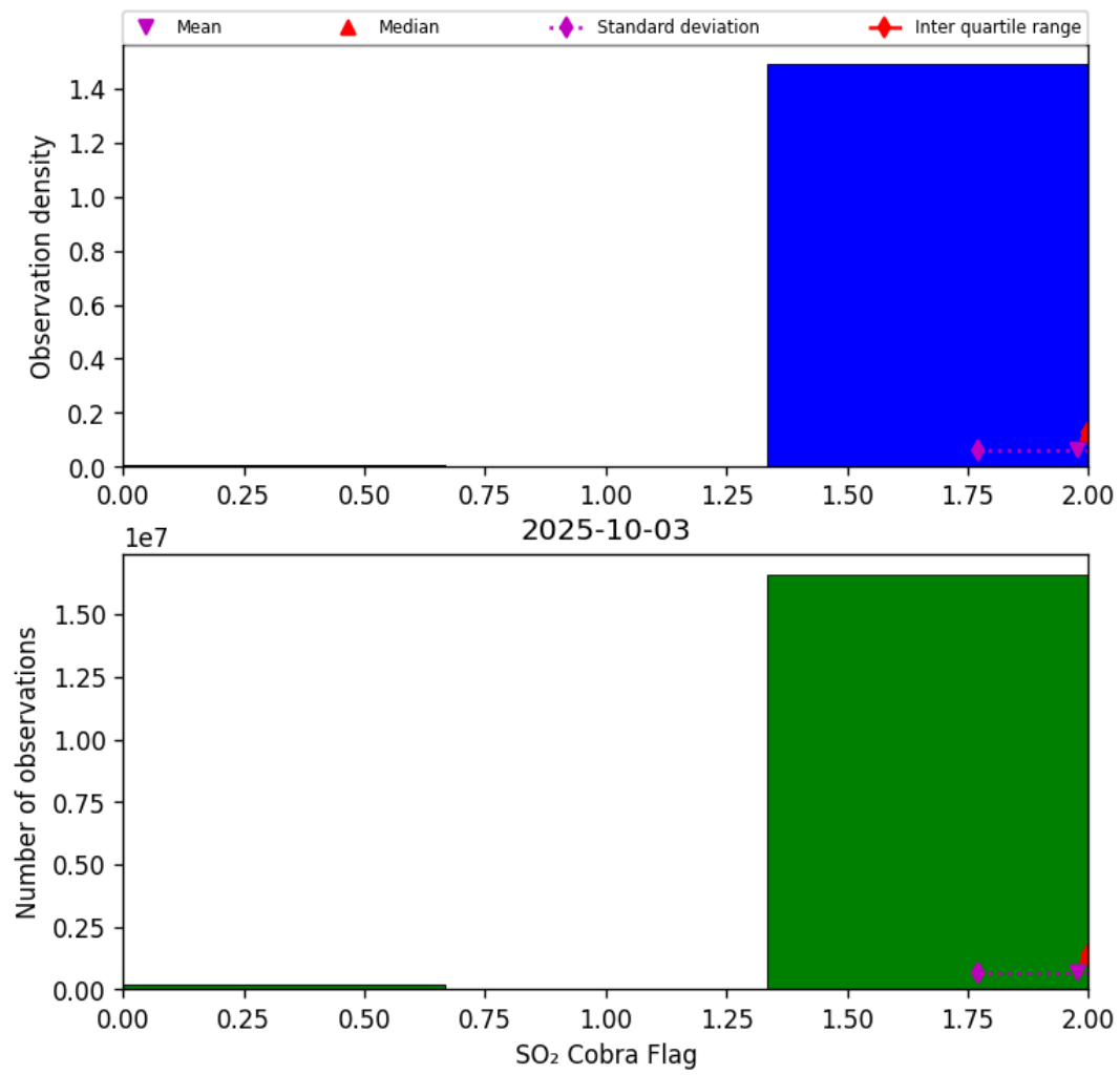
Figure 75: Histogram of “SO 2 Cobra Flag” for 2025-10-03 to 2025-10-04
