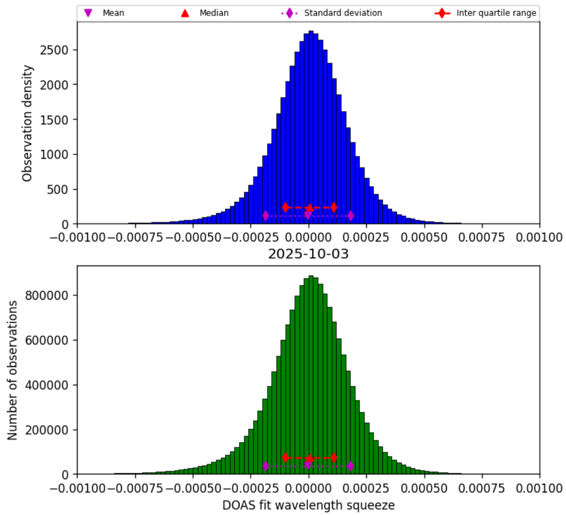
Figure 78: Histogram of “DOAS fit wavelength squeeze” for 2025-10-03 to 2025-10-04
