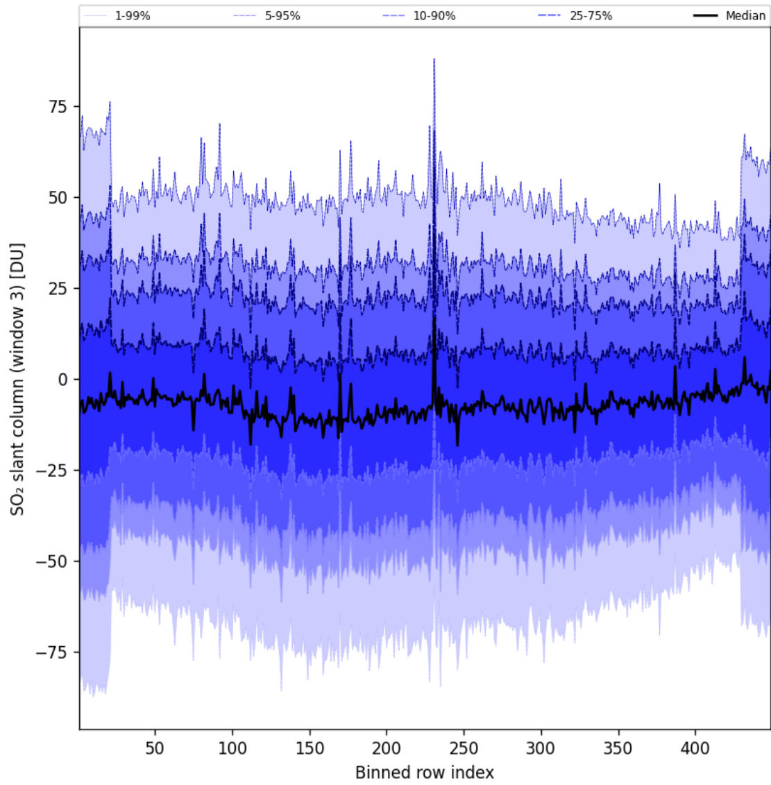
Figure 98: Along track statistics of “SO 2 slant column (window 3)” for 2025-10-03 to 2025-10-04
