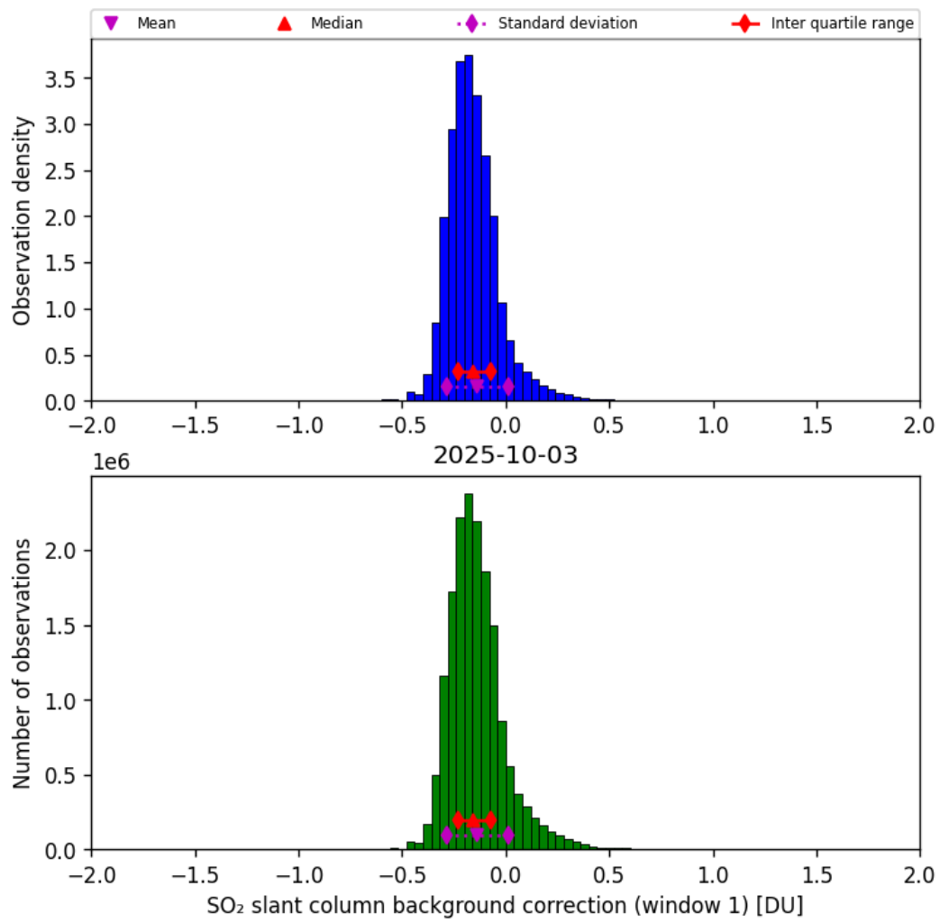
Figure 66: Histogram of “SO 2 slant column background correction (window 1)” for 2025-10-03 to 2025-10-04
