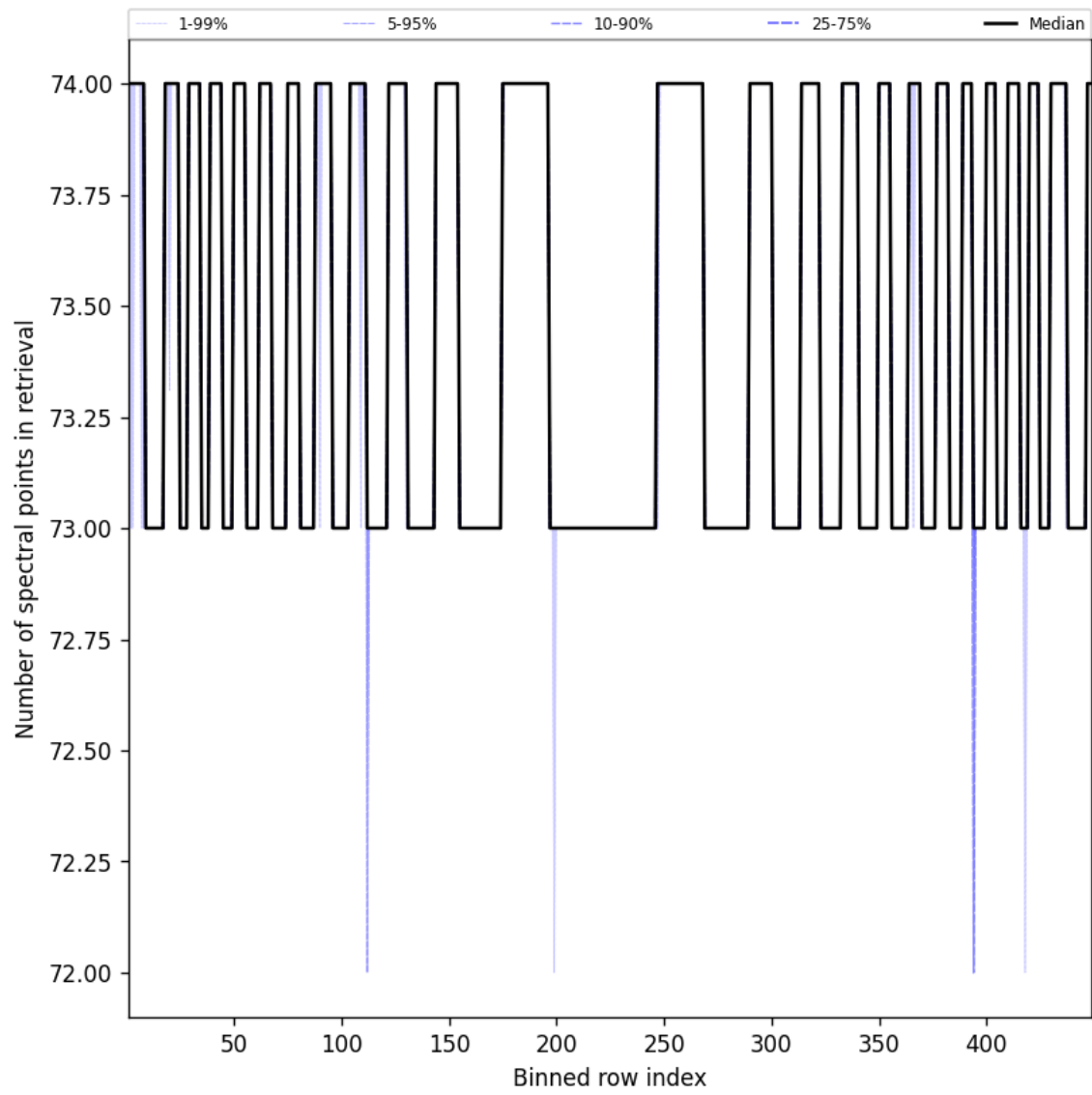
Figure 110: Along track statistics of “Number of spectral points in retrieval” for 2025-10-03 to 2025-10-04
