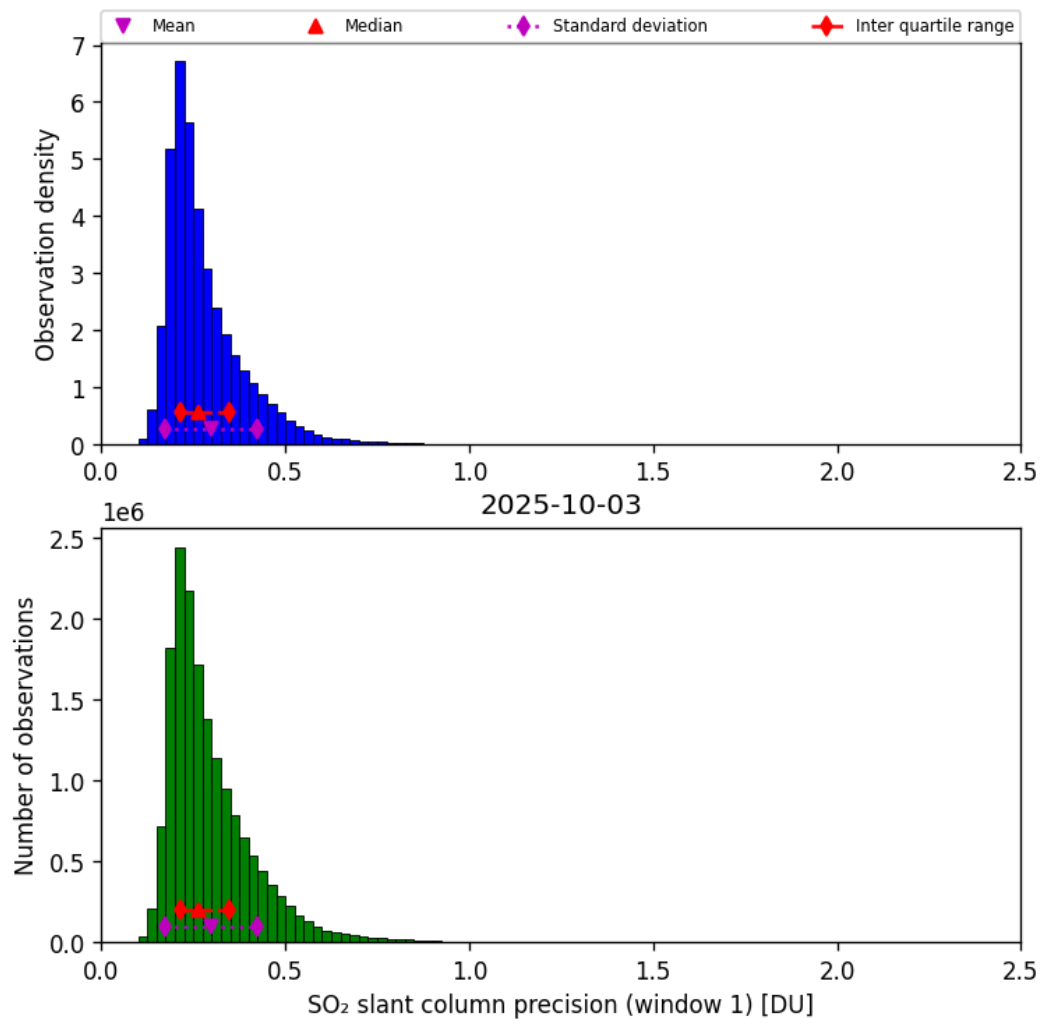
Figure 64: Histogram of “SO 2 slant column precision (window 1)” for 2025-10-03 to 2025-10-04
