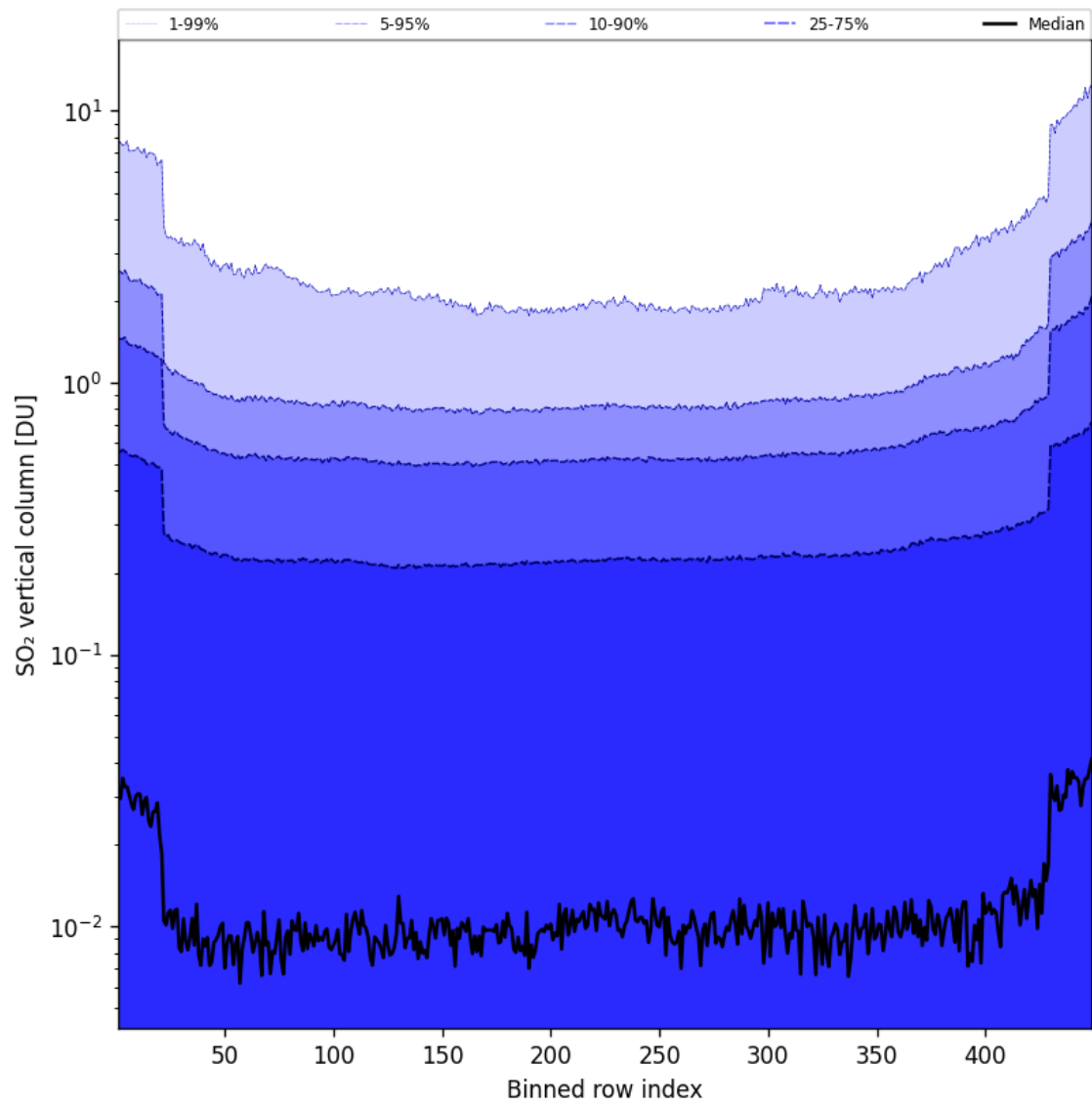
Figure 85: Along track statistics of “SO 2 vertical column” for 2025-10-03 to 2025-10-04
