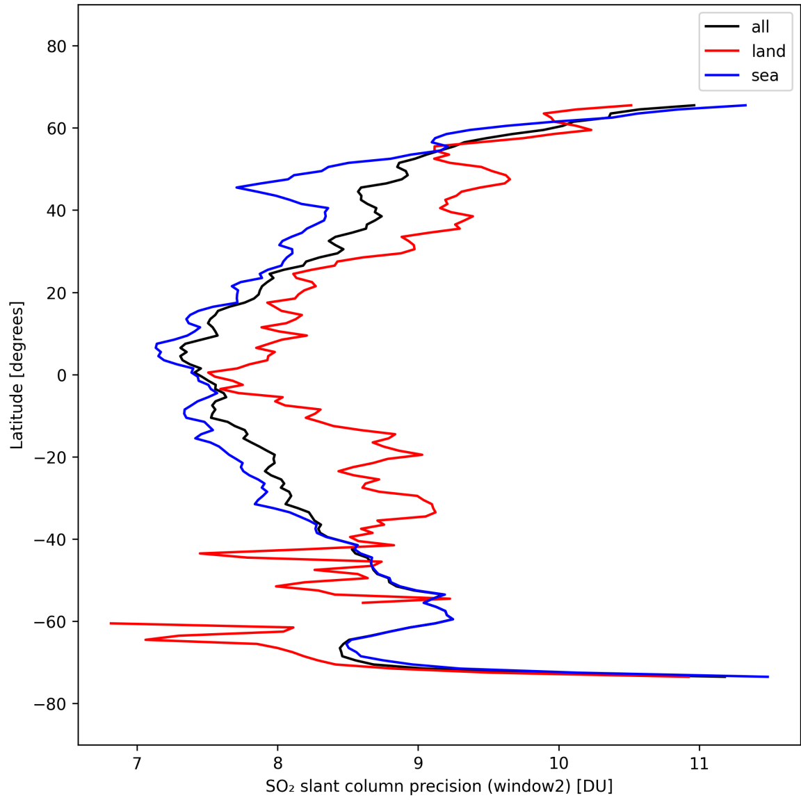
Figure 41: Zonal average of “SO 2 slant column precision (window2)” for 2025-10-03 to 2025-10-04.
