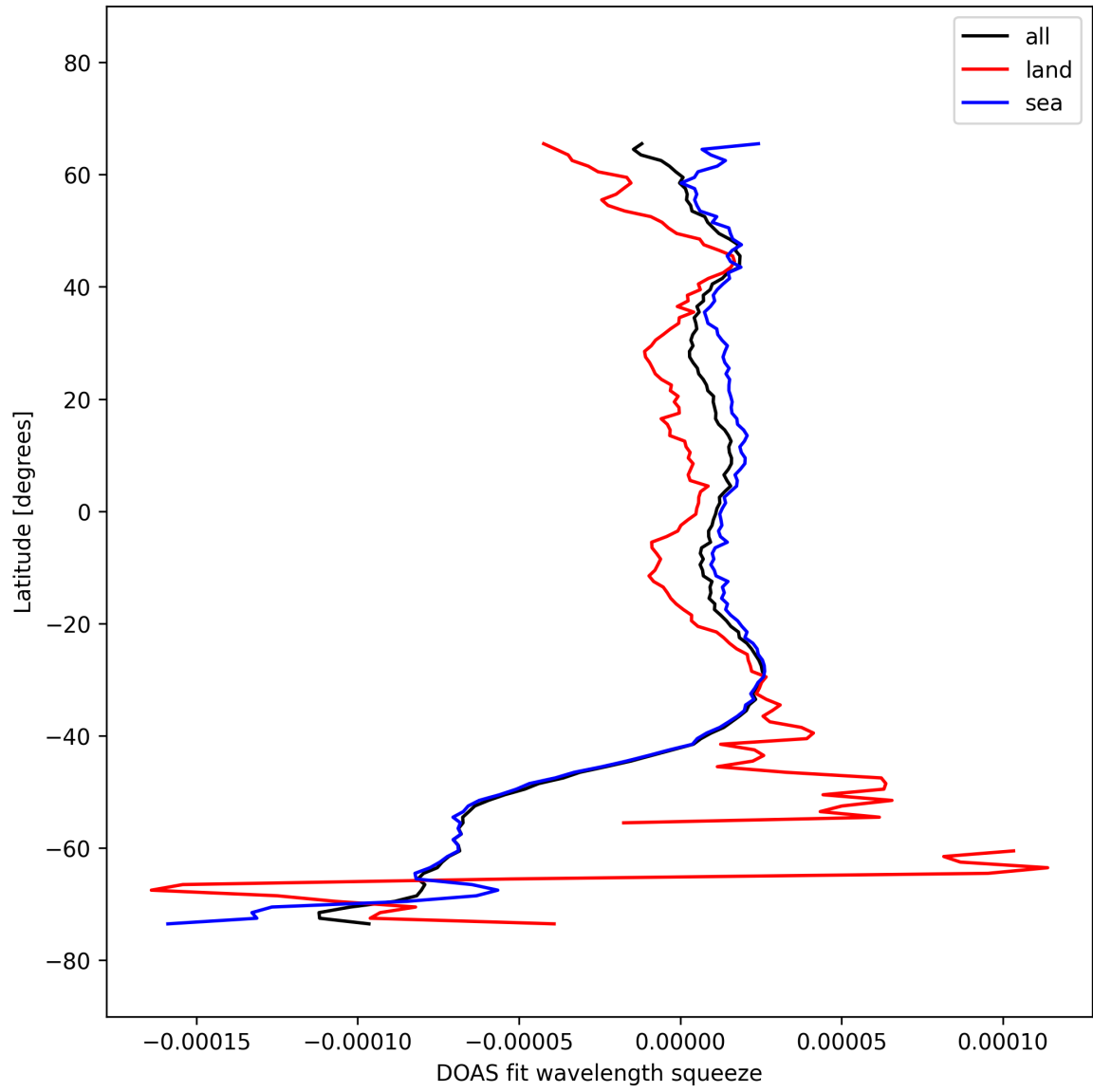
Figure 51: Zonal average of “DOAS fit wavelength squeeze” for 2025-10-03 to 2025-10-04.
