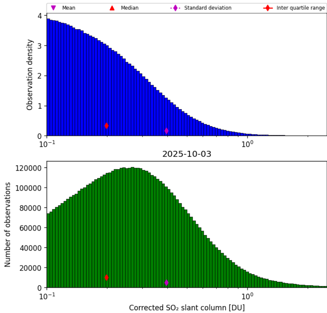
Figure 60: Histogram of “Corrected SO 2 slant column” for 2025-10-03 to 2025-10-04
