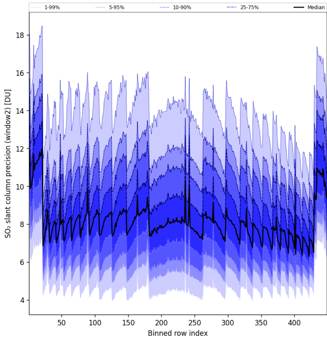
Figure 95: Along track statistics of “SO 2 slant column precision (window2)” for 2025-10-03 to 2025-10-04
