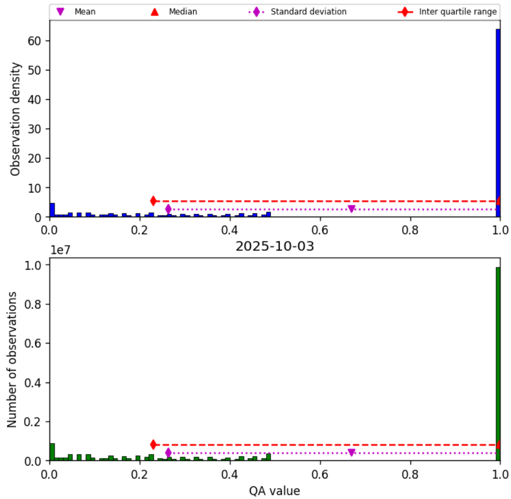
Figure 57: Histogram of “QA value” for 2025-10-03 to 2025-10-04
