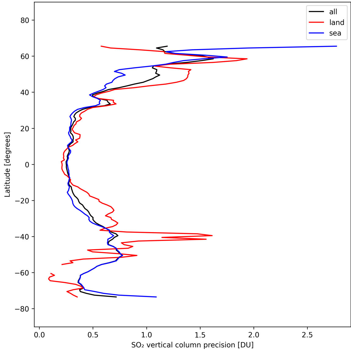
Figure 32: Zonal average of “SO 2 vertical column precision” for 2025-10-03 to 2025-10-04.
