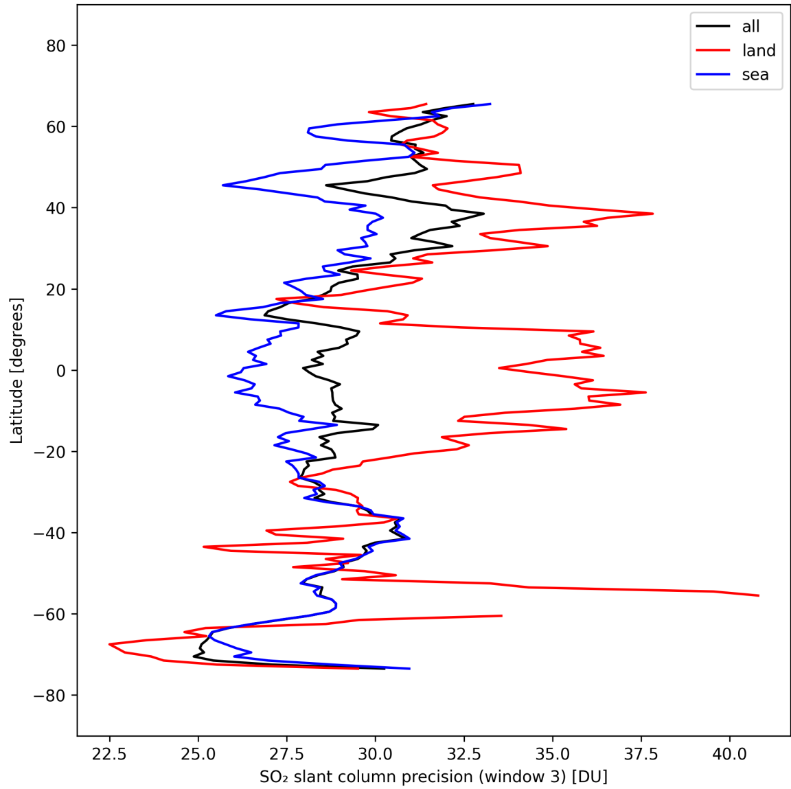
Figure 45: Zonal average of “SO 2 slant column precision (window 3)” for 2025-10-03 to 2025-10-04.
