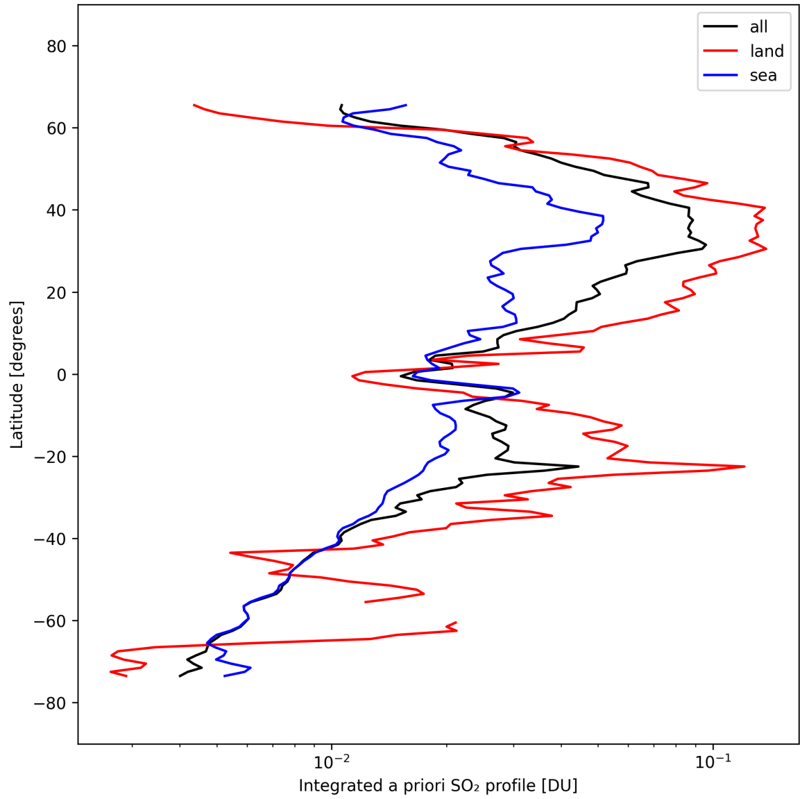
Figure 49: Zonal average of “Integrated a priori SO 2 profile” for 2025-10-03 to 2025-10-04.
