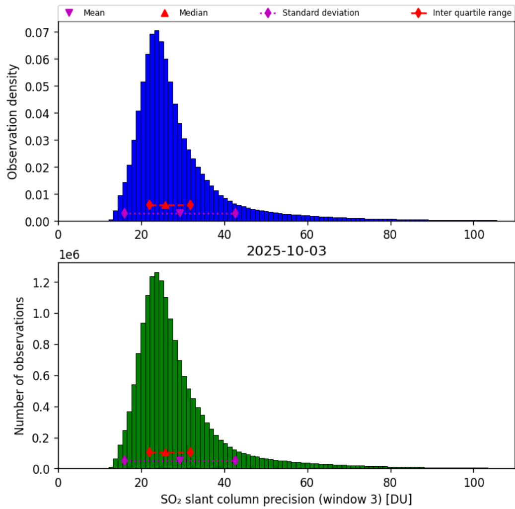
Figure 72: Histogram of “SO 2 slant column precision (window 3)” for 2025-10-03 to 2025-10-04
