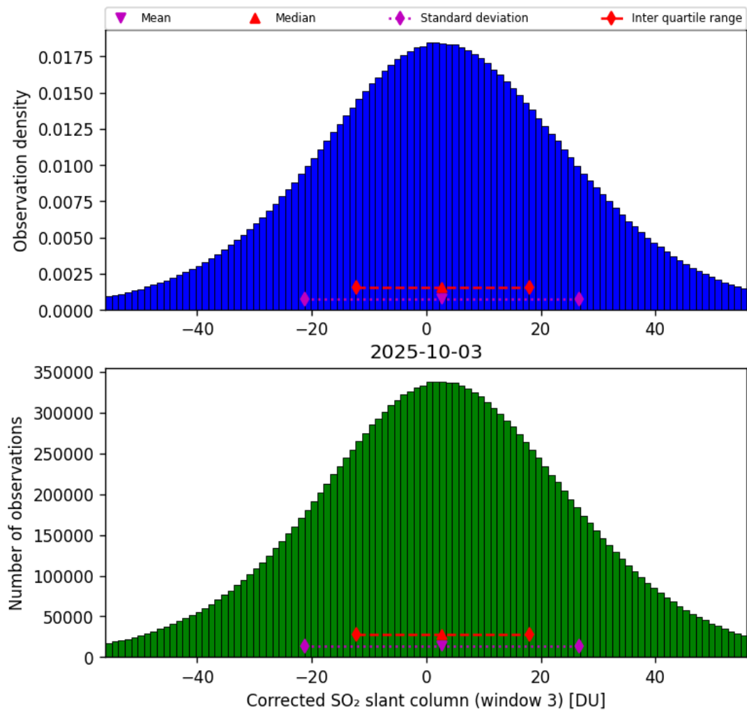
Figure 73: Histogram of “Corrected SO 2 slant column (window 3)” for 2025-10-03 to 2025-10-04
