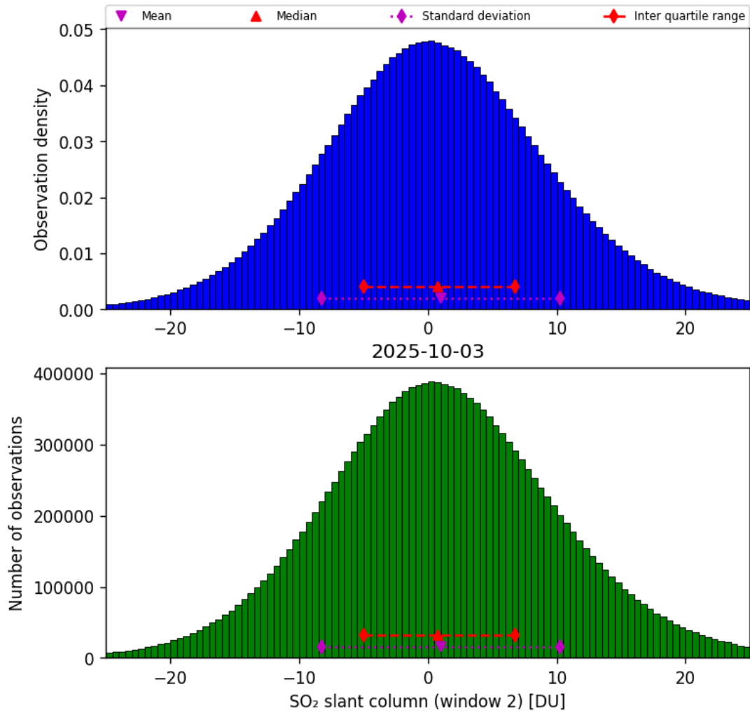
Figure 67: Histogram of “SO 2 slant column (window 2)” for 2025-10-03 to 2025-10-04
