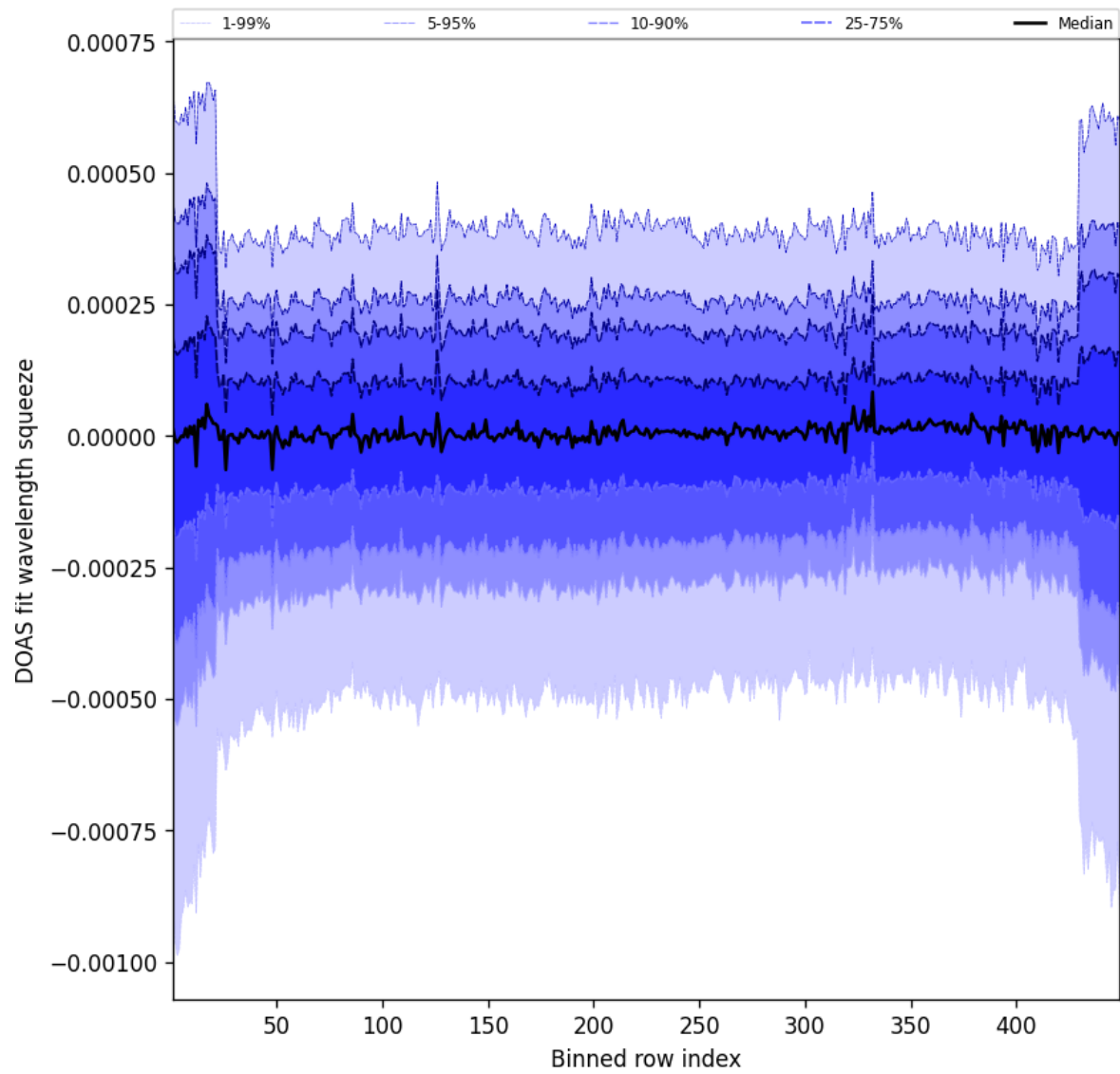
Figure 105: Along track statistics of “DOAS fit wavelength squeeze” for 2025-10-03 to 2025-10-04
