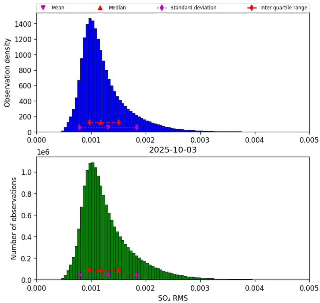
Figure 79: Histogram of “SO 2 RMS” for 2025-10-03 to 2025-10-04
