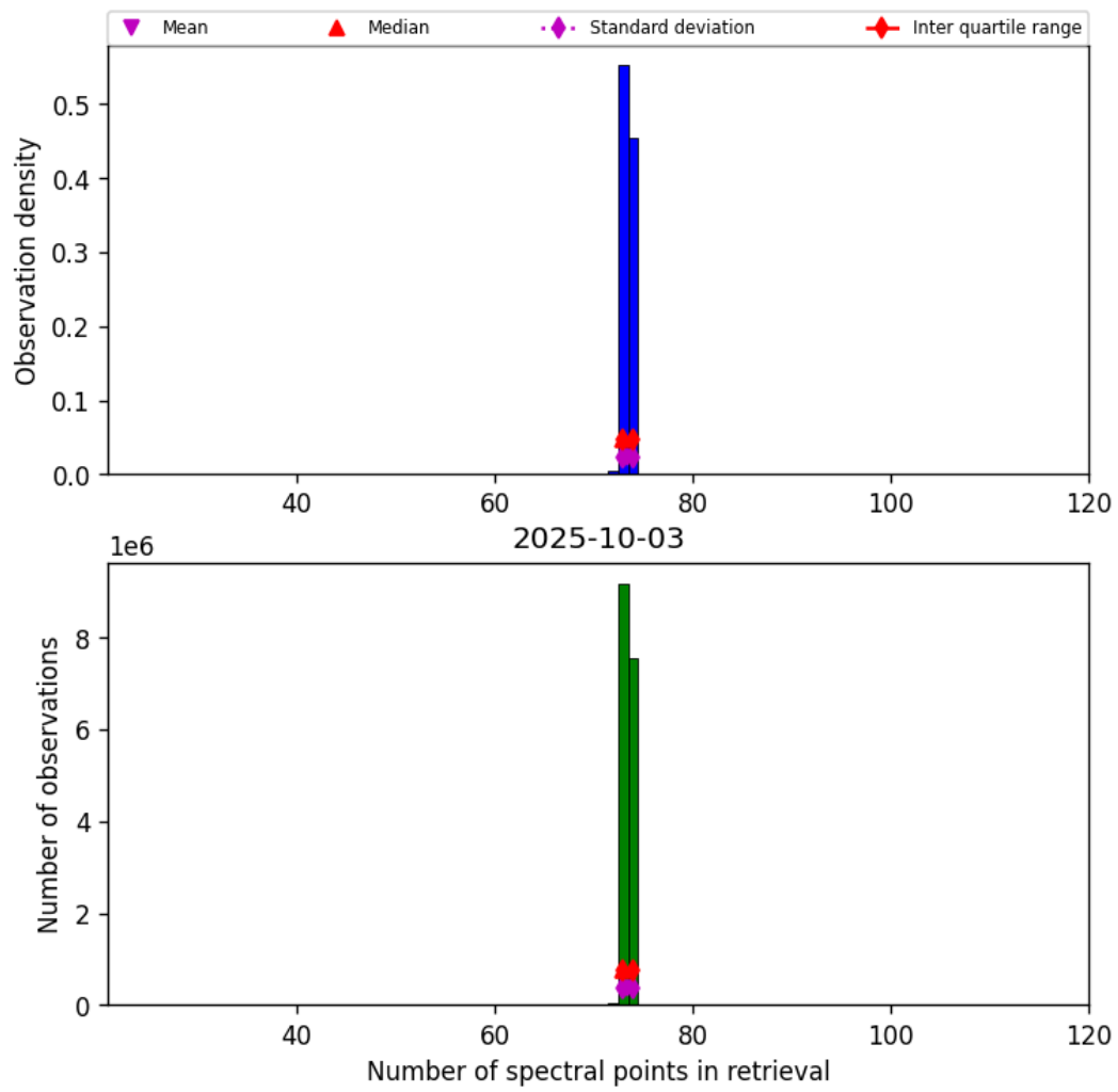
Figure 83: Histogram of “Number of spectral points in retrieval” for 2025-10-03 to 2025-10-04
