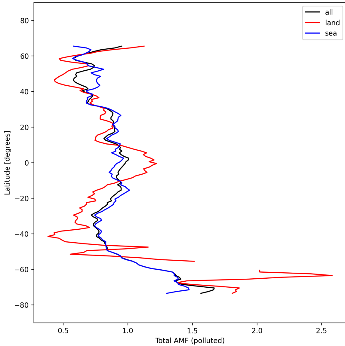
Figure 53: Zonal average of “Total AMF (polluted)” for 2025-10-03 to 2025-10-04.
