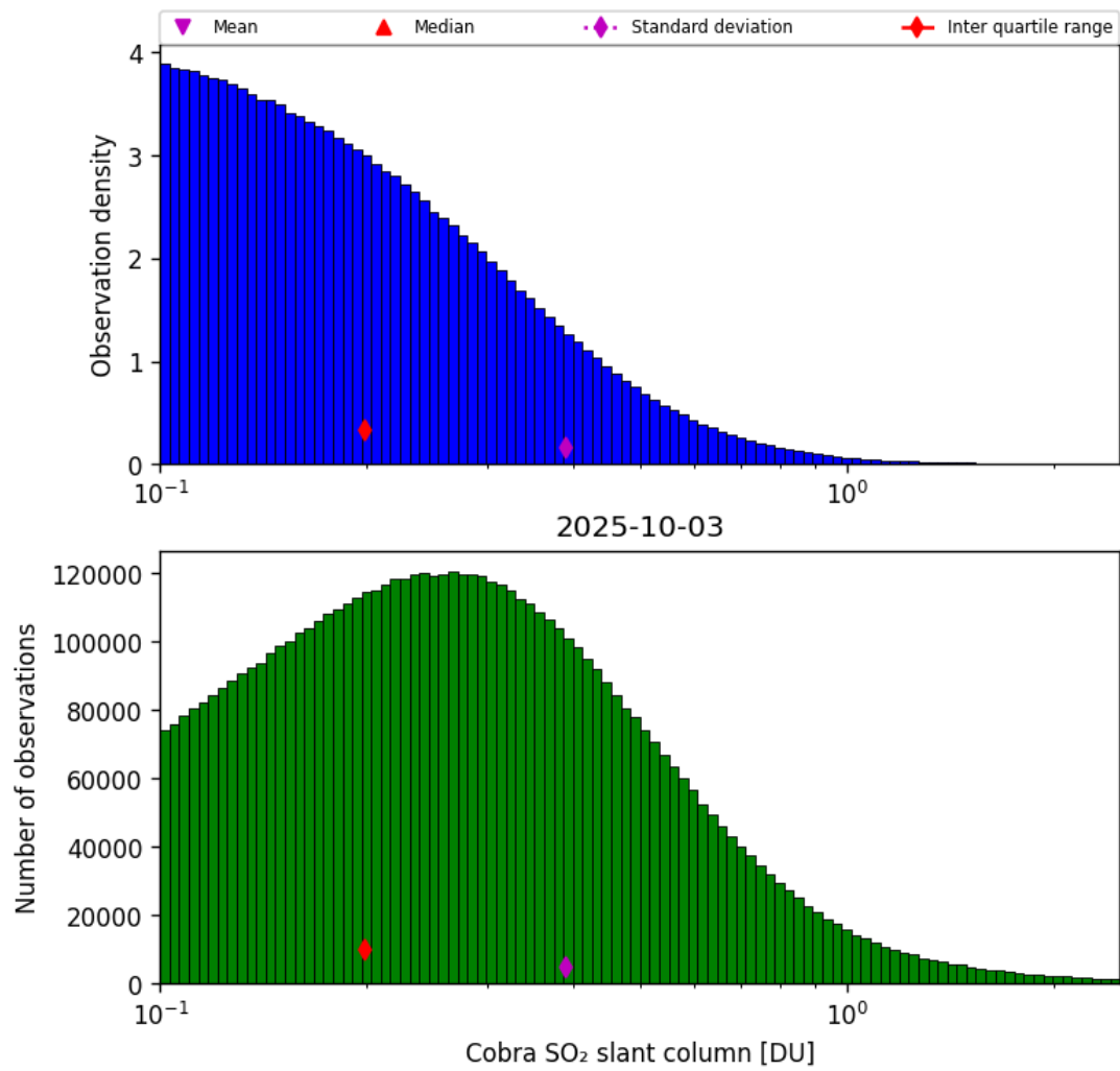
Figure 61: Histogram of “Cobra SO 2 slant column” for 2025-10-03 to 2025-10-04
