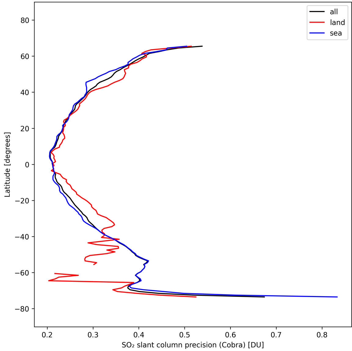
Figure 35: Zonal average of “SO 2 slant column precision (Cobra)” for 2025-10-03 to 2025-10-04.
