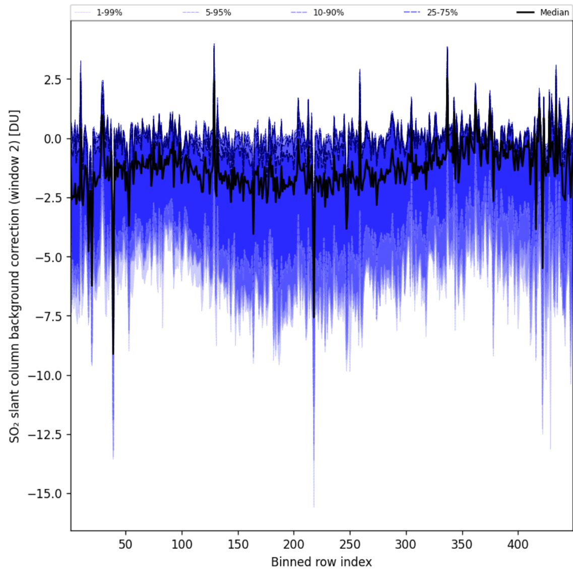
Figure 97: Along track statistics of “SO 2 slant column background correction (window 2)” for 2025-10-03 to 2025-10-04
