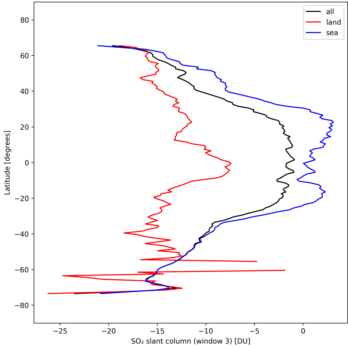
Figure 44: Zonal average of “SO 2 slant column (window 3)” for 2025-10-03 to 2025-10-04.
