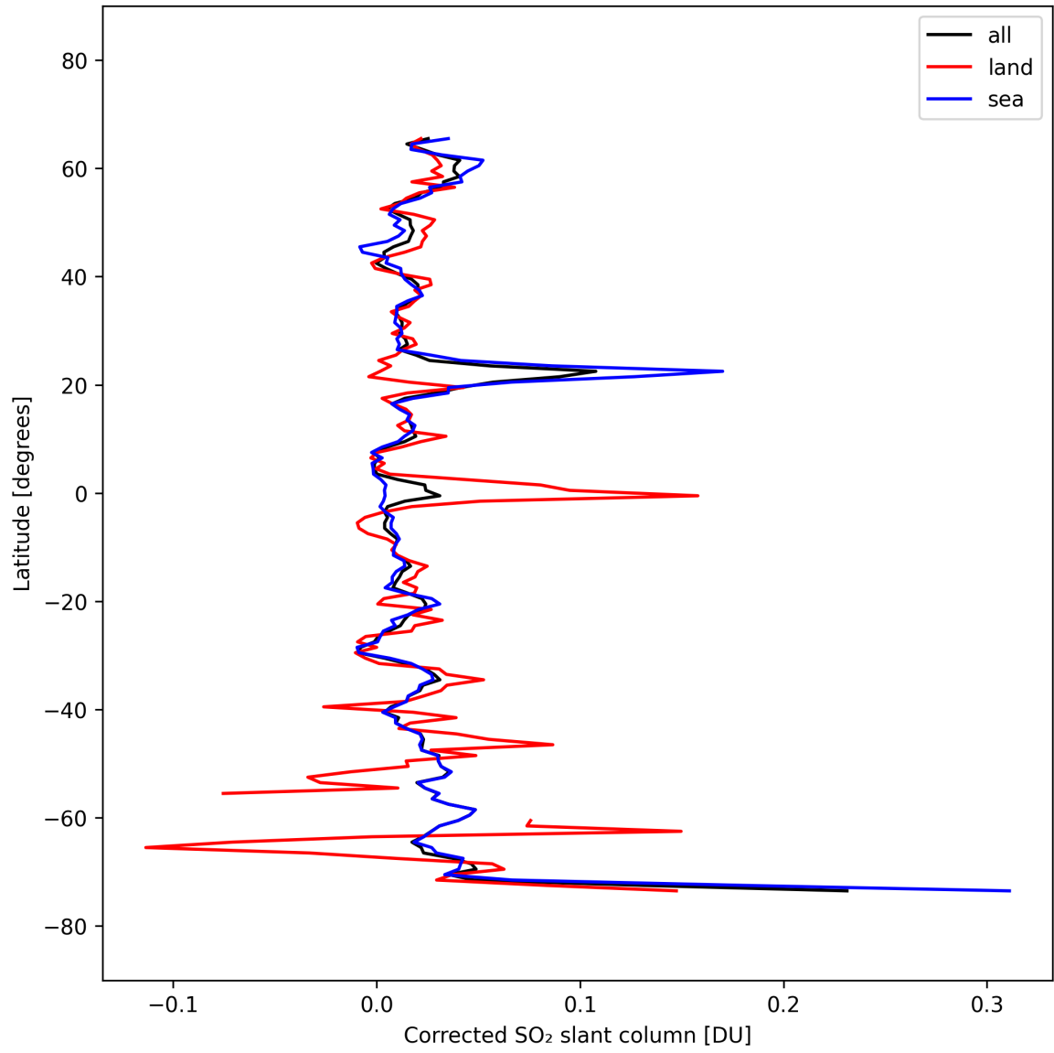
Figure 33: Zonal average of “Corrected SO 2 slant column” for 2025-10-03 to 2025-10-04.
