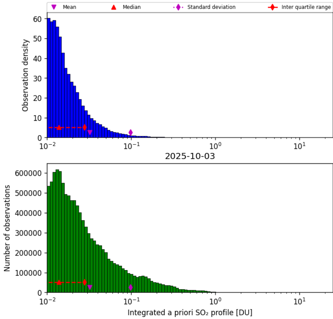
Figure 76: Histogram of “Integrated a priori SO 2 profile” for 2025-10-03 to 2025-10-04
