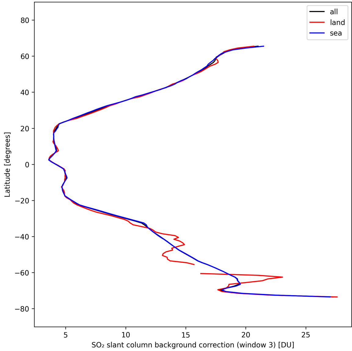
Figure 47: Zonal average of “SO 2 slant column background correction (window 3)” for 2025-10-03 to 2025-10-04.
