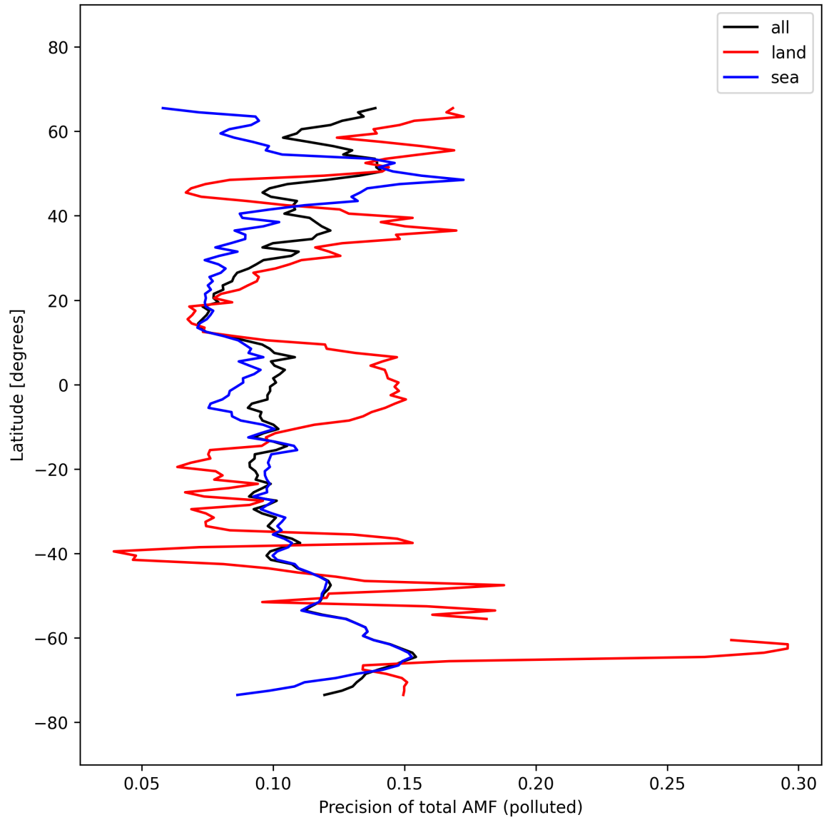
Figure 54: Zonal average of “Precision of total AMF (polluted)” for 2025-10-03 to 2025-10-04.
