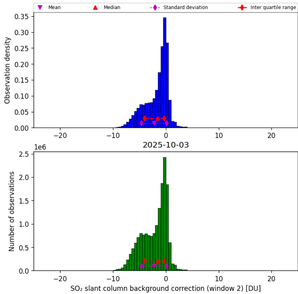
Figure 70: Histogram of “SO 2 slant column background correction (window 2)” for 2025-10-03 to 2025-10-04
