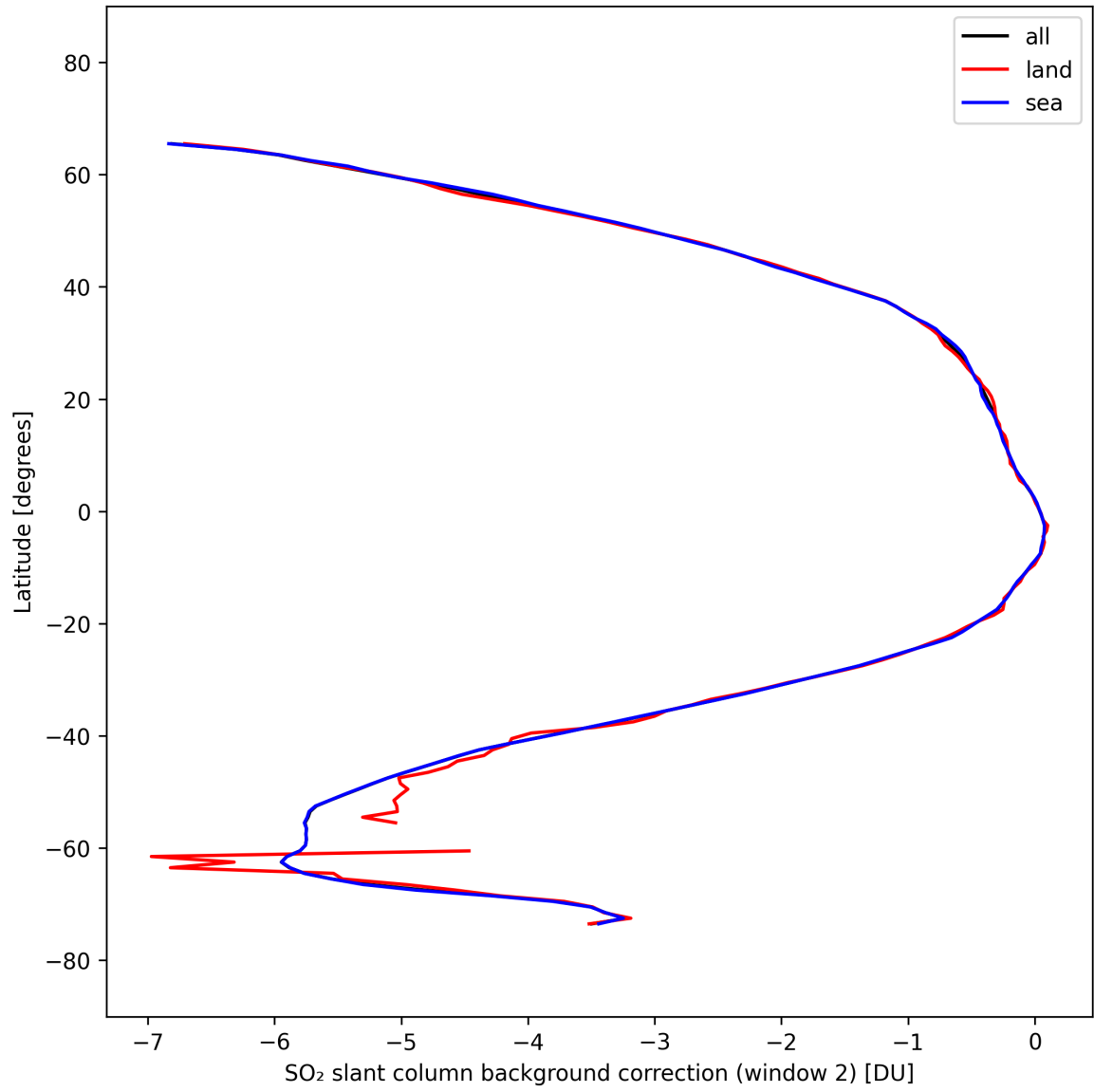
Figure 43: Zonal average of “SO 2 slant column background correction (window 2)” for 2025-10-03 to 2025-10-04.
