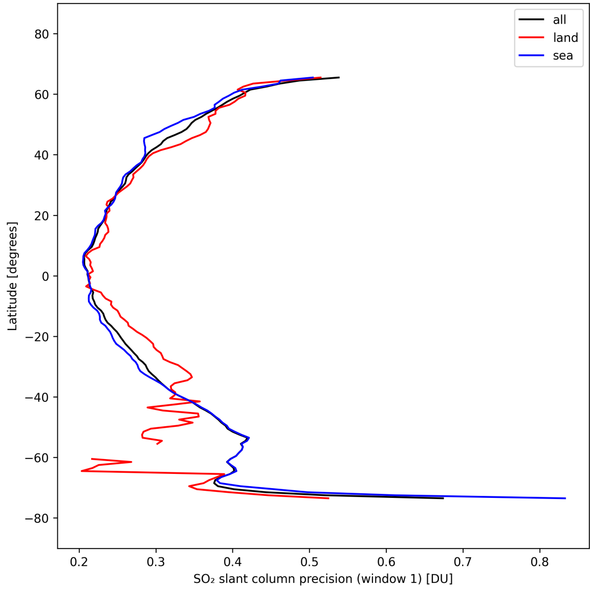
Figure 37: Zonal average of “SO 2 slant column precision (window 1)” for 2025-10-03 to 2025-10-04.
