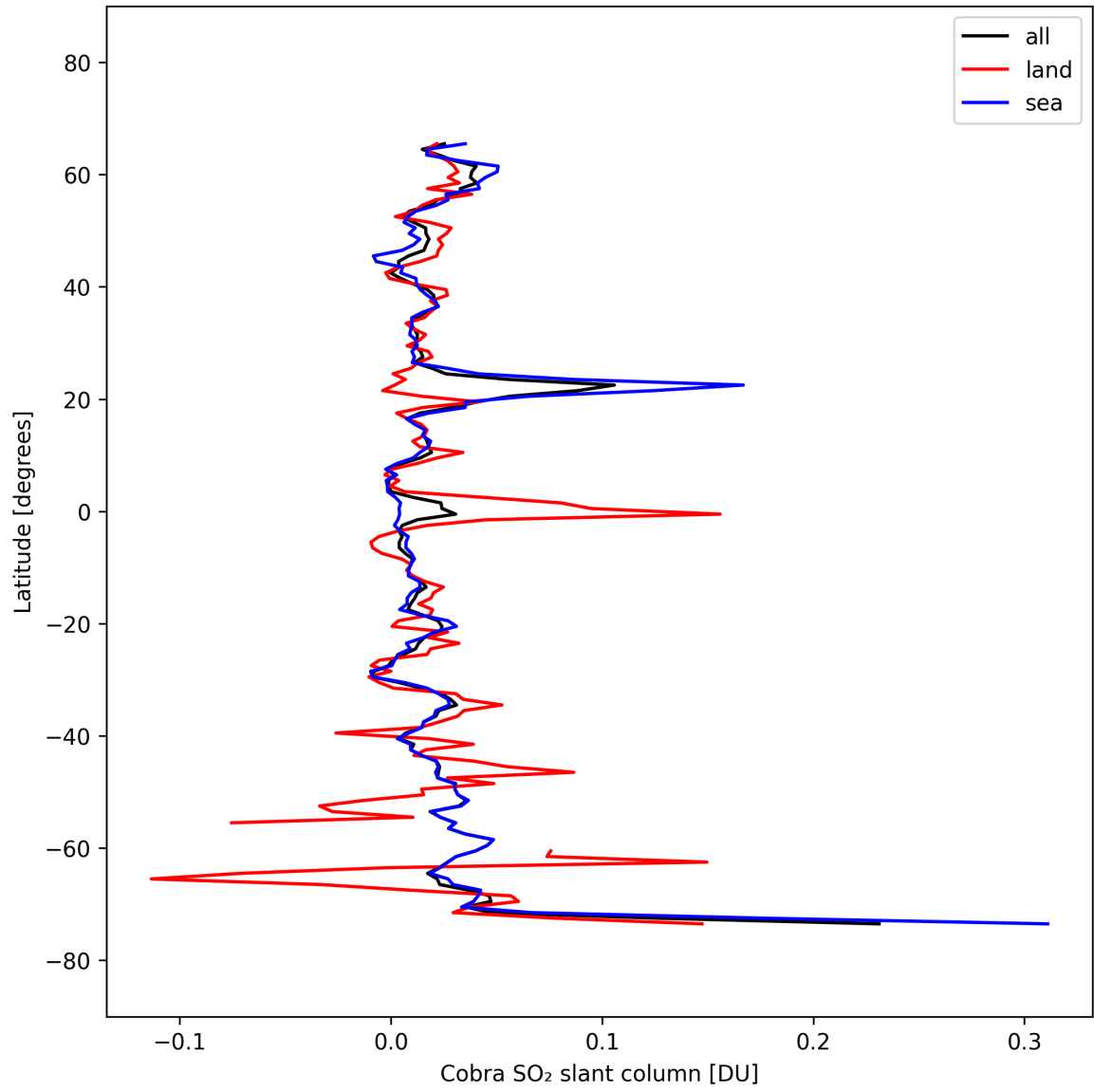
Figure 34: Zonal average of “Cobra SO 2 slant column” for 2025-10-03 to 2025-10-04.
