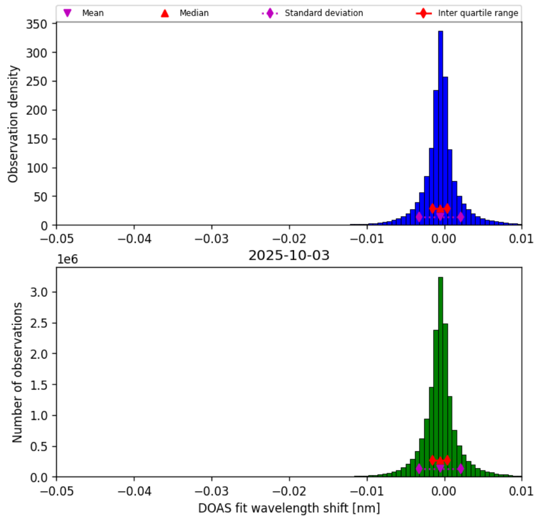
Figure 77: Histogram of “DOAS fit wavelength shift” for 2025-10-03 to 2025-10-04
