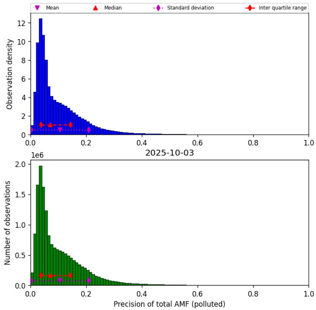
Figure 81: Histogram of “Precision of total AMF (polluted)” for 2025-10-03 to 2025-10-04
