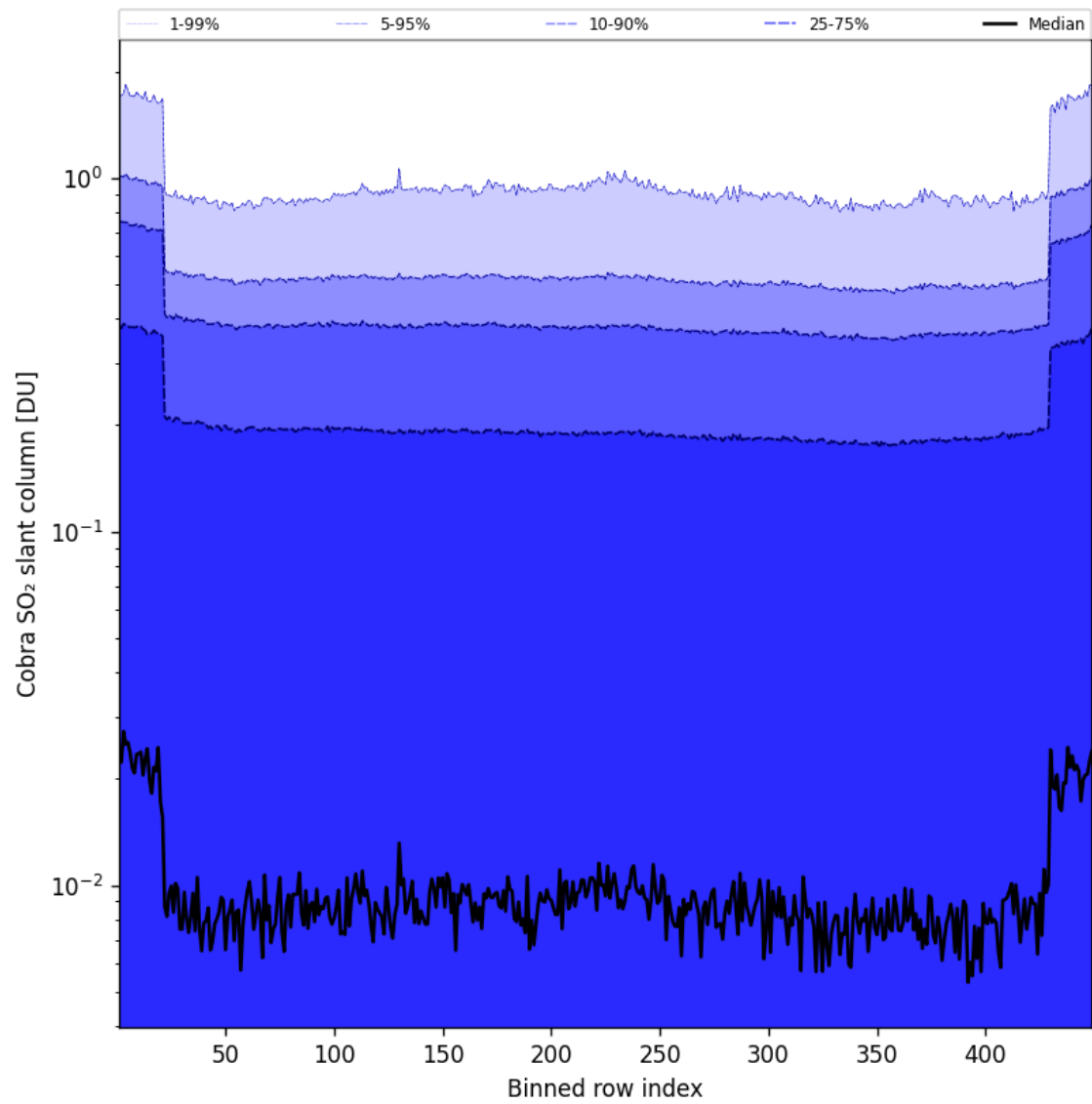
Figure 88: Along track statistics of “Cobra SO 2 slant column” for 2025-10-03 to 2025-10-04
