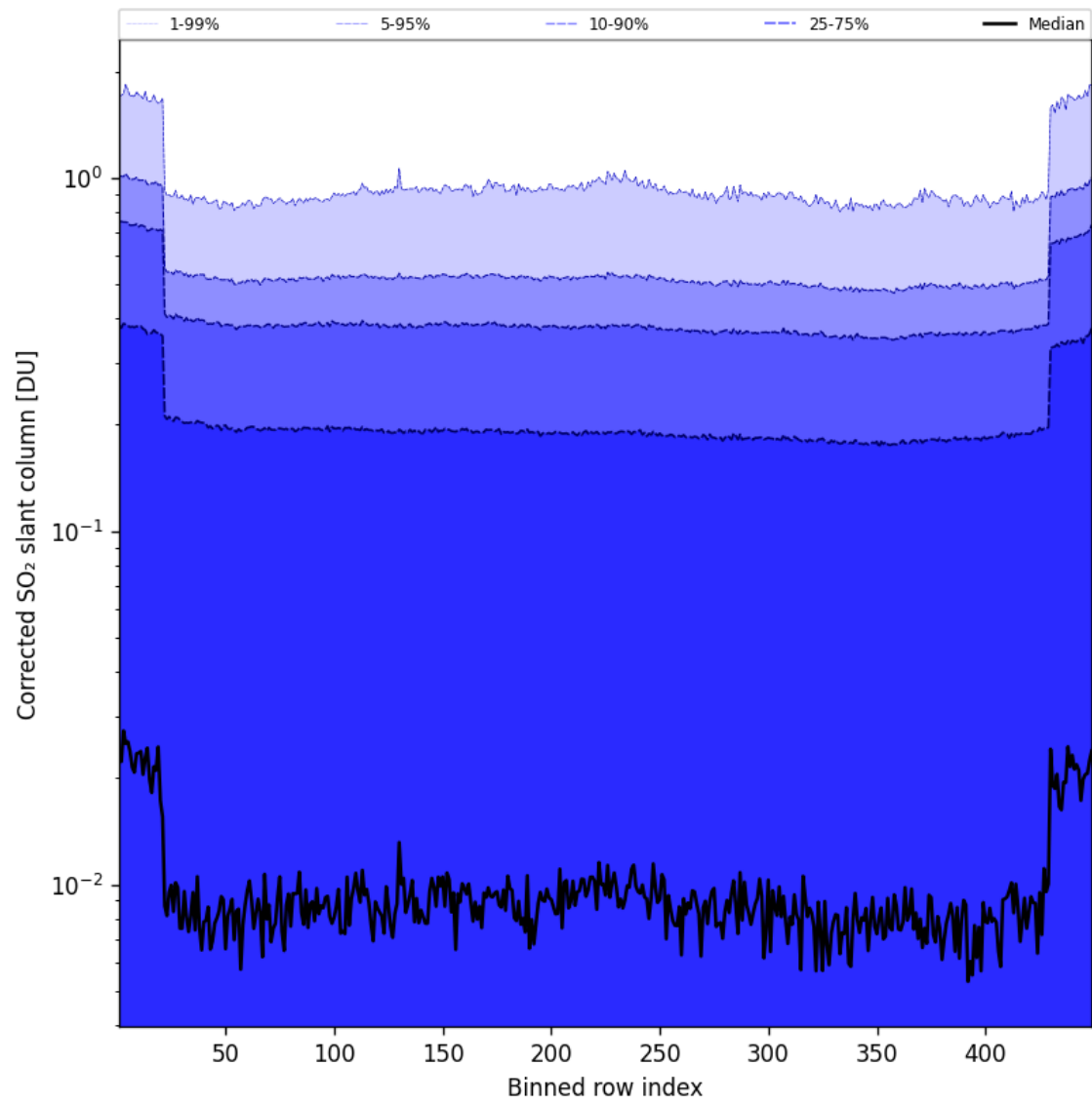
Figure 87: Along track statistics of "Corrected SO 2 slant column" for 2025-10-03 to 2025-10-04
