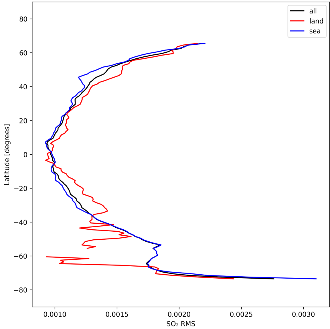
Figure 52: Zonal average of “SO 2 RMS” for 2025-10-03 to 2025-10-04.
