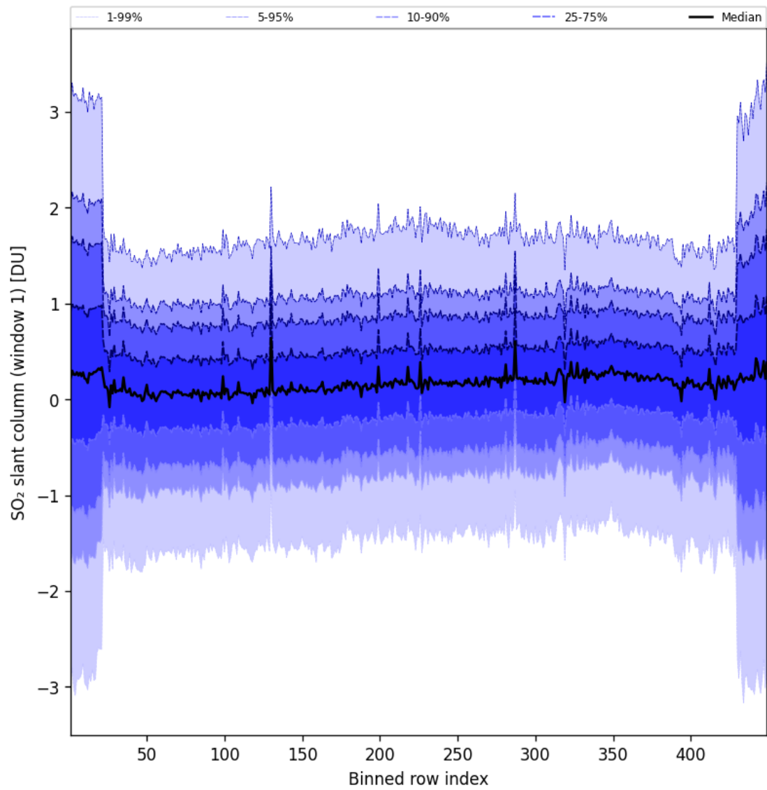
Figure 90: Along track statistics of “SO 2 slant column (window 1)” for 2025-10-03 to 2025-10-04
