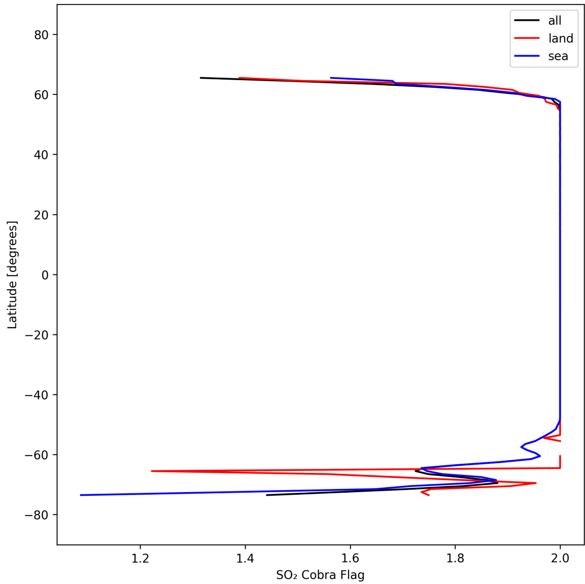
Figure 48: Zonal average of “SO 2 Cobra Flag” for 2025-10-03 to 2025-10-04.
