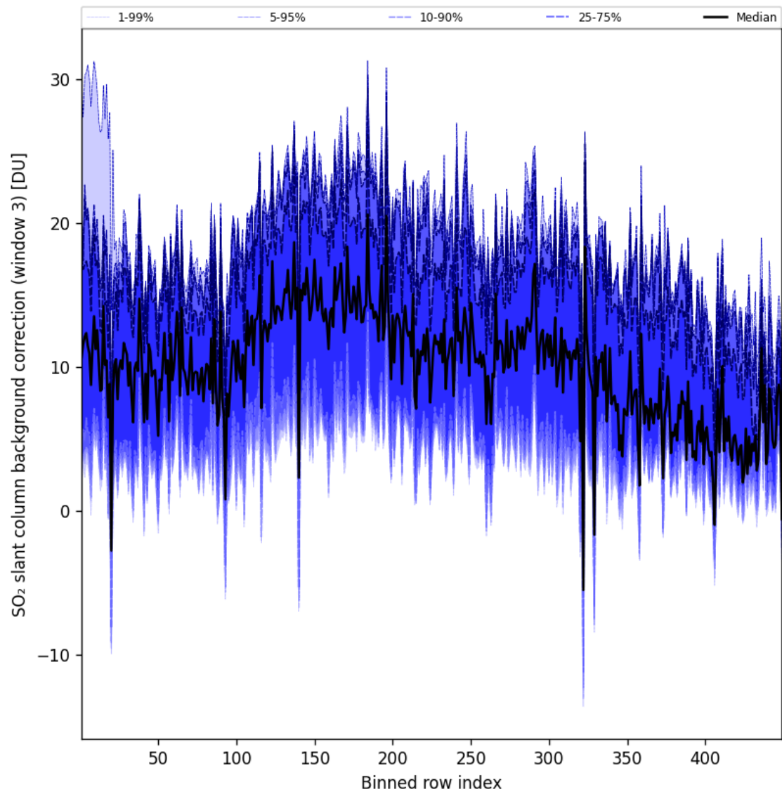
Figure 101: Along track statistics of “SO 2 slant column background correction (window 3)” for 2025-10-03 to 2025-10-04
