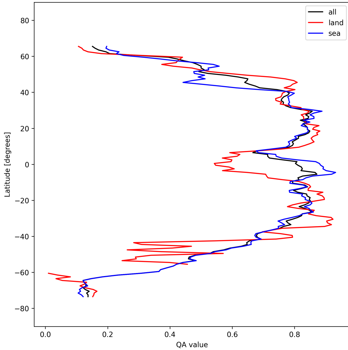
Figure 30: Zonal average of “QA value” for 2025-10-03 to 2025-10-04.
