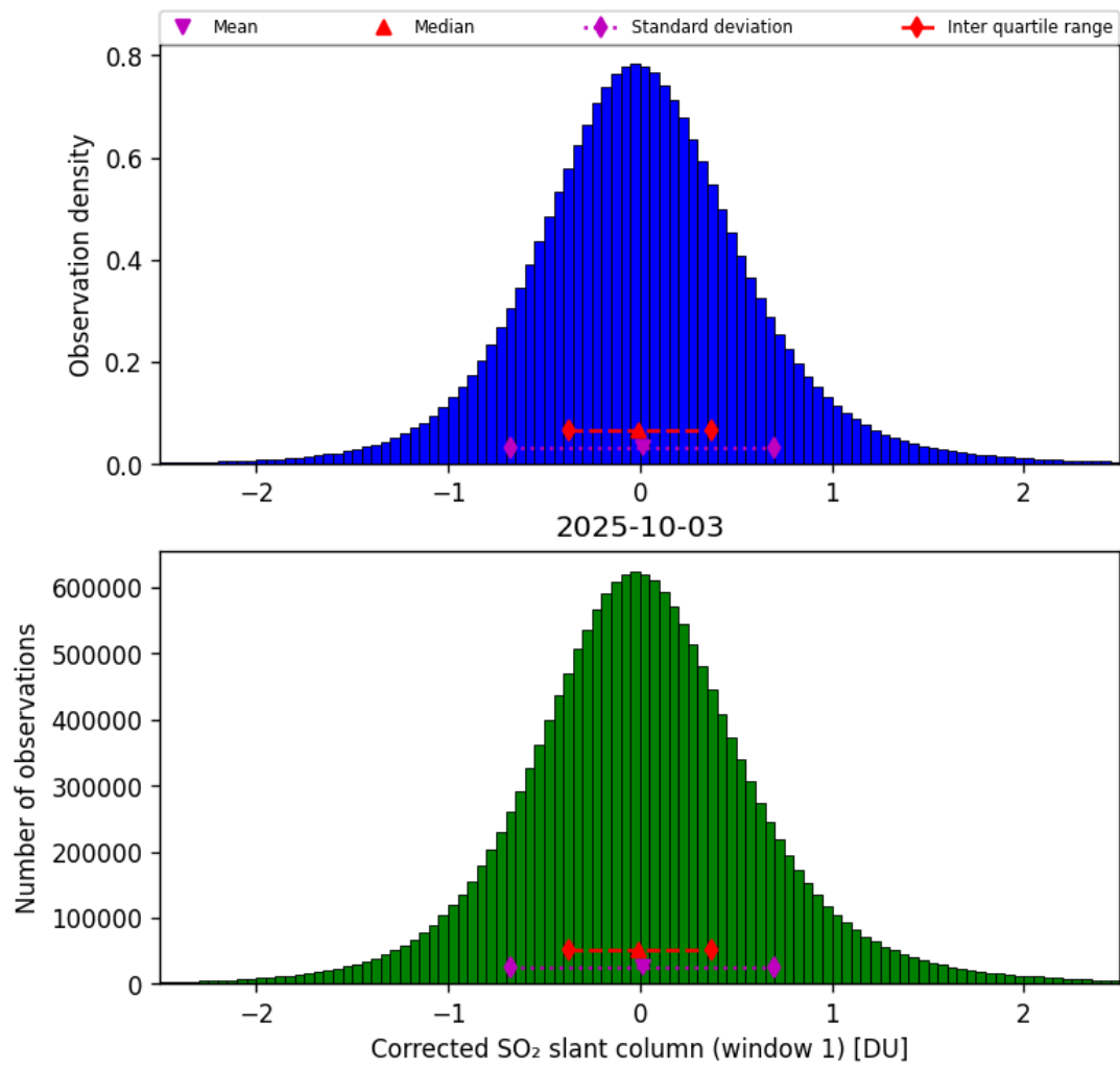
Figure 65: Histogram of “Corrected SO 2 slant column (window 1)” for 2025-10-03 to 2025-10-04
