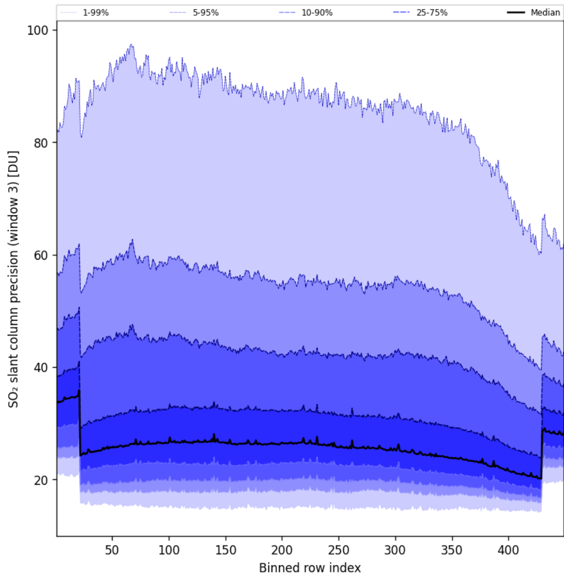
Figure 99: Along track statistics of “SO 2 slant column precision (window 3)” for 2025-10-03 to 2025-10-04
