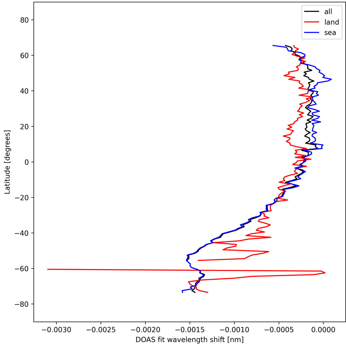
Figure 50: Zonal average of "DOAS fit wavelength shift" for 2025-10-03 to 2025-10-04.
