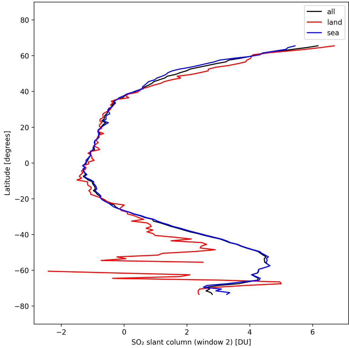
Figure 40: Zonal average of “SO 2 slant column (window 2)” for 2025-10-03 to 2025-10-04.
