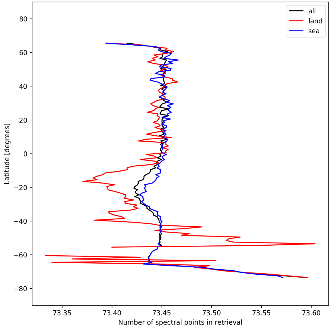
Figure 56: Zonal average of “Number of spectral points in retrieval” for 2025-10-03 to 2025-10-04.
