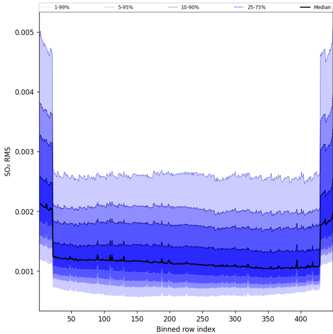
Figure 106: Along track statistics of “SO 2 RMS” for 2025-10-03 to 2025-10-04
