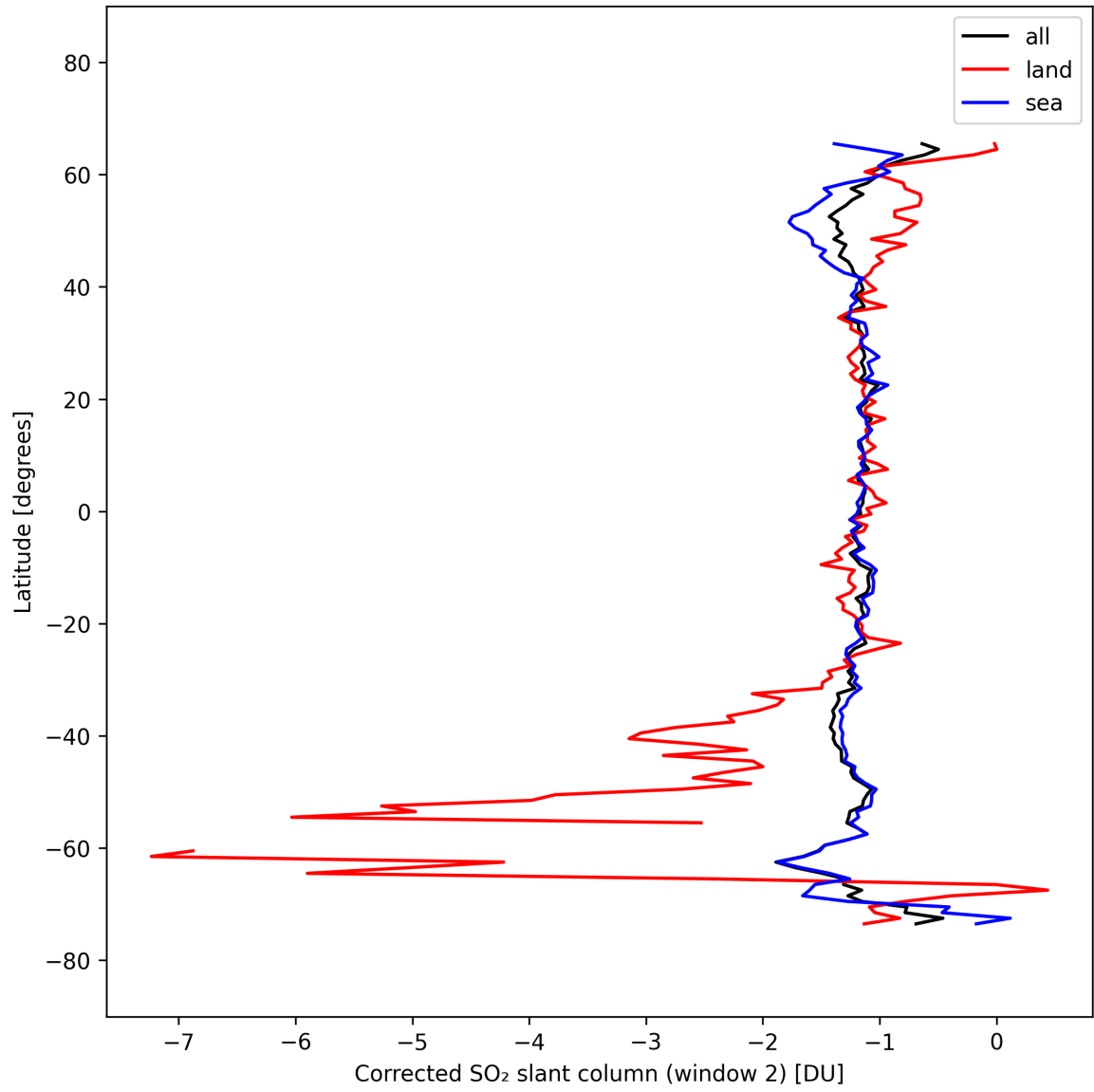
Figure 42: Zonal average of “Corrected SO 2 slant column (window 2)” for 2025-10-03 to 2025-10-04.
