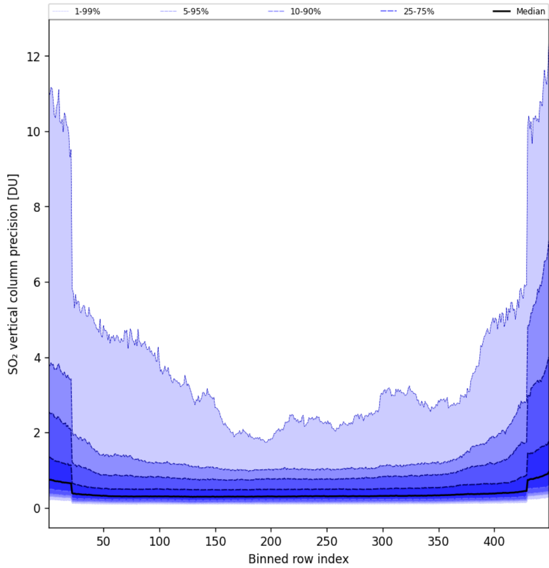
Figure 86: Along track statistics of “SO 2 vertical column precision” for 2025-10-03 to 2025-10-04
