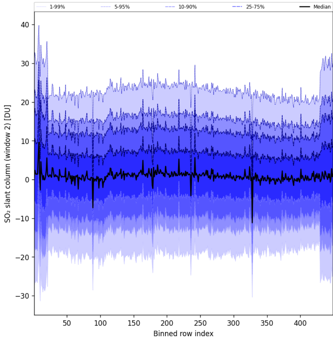
Figure 94: Along track statistics of “SO 2 slant column (window 2)” for 2025-10-03 to 2025-10-04
