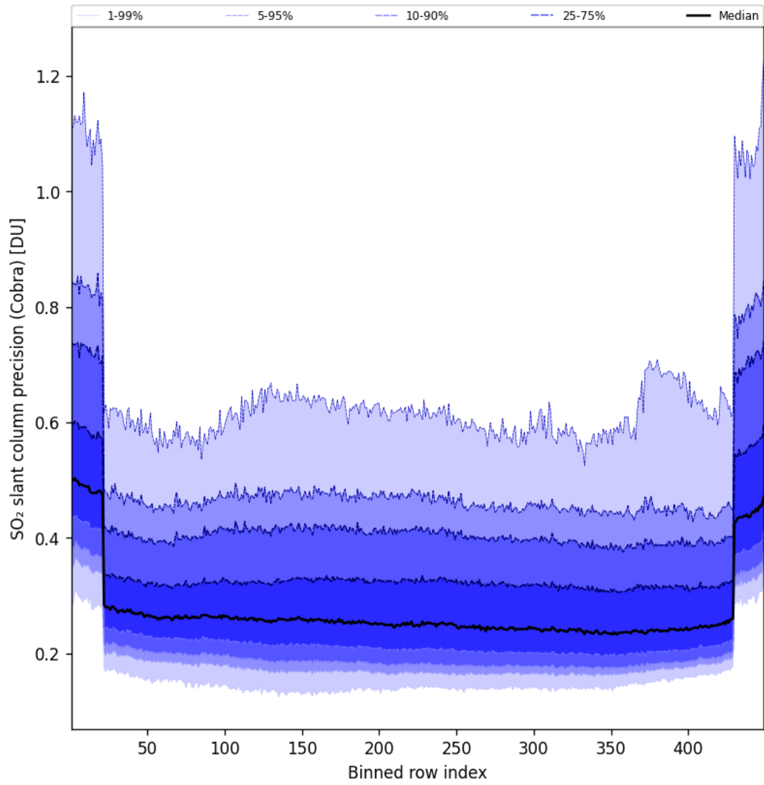
Figure 89: Along track statistics of “SO 2 slant column precision (Cobra)” for 2025-10-03 to 2025-10-04
