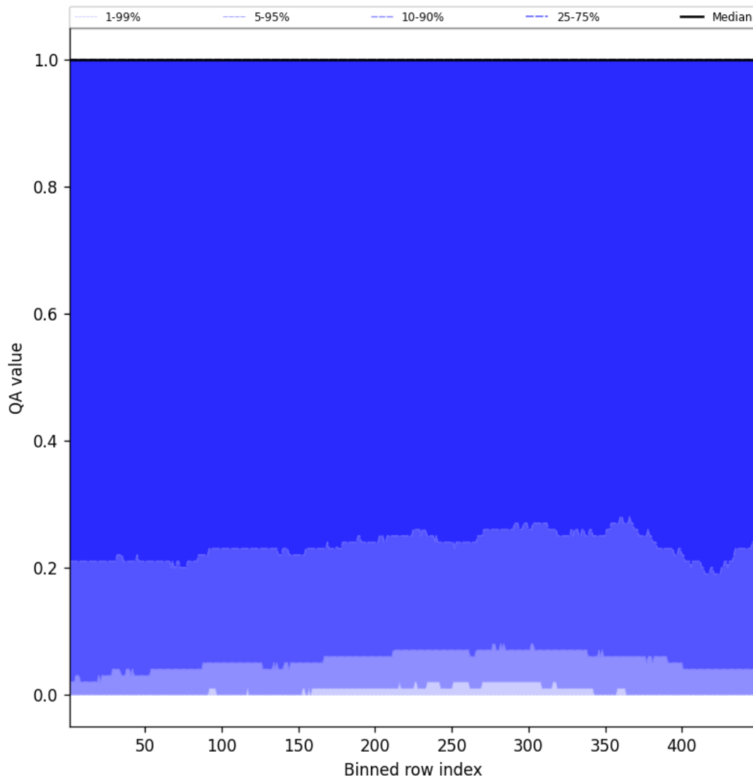
Figure 84: Along track statistics of “QA value” for 2025-10-03 to 2025-10-04
