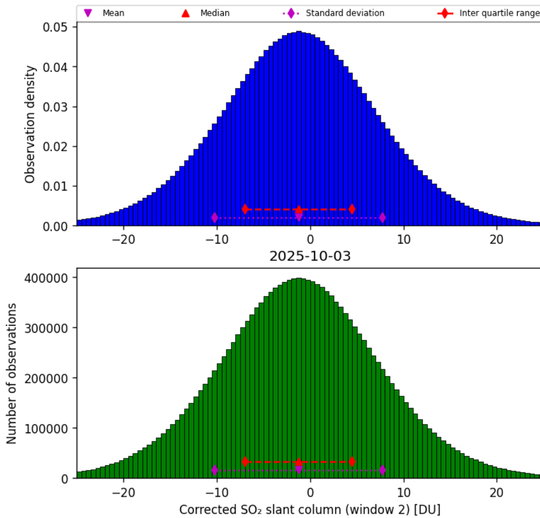
Figure 69: Histogram of “Corrected SO 2 slant column (window 2)” for 2025-10-03 to 2025-10-04
