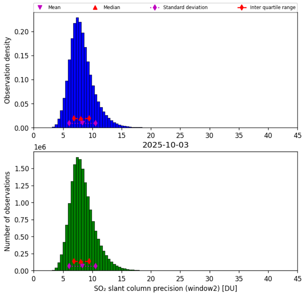
Figure 68: Histogram of “SO 2 slant column precision (window2)” for 2025-10-03 to 2025-10-04
