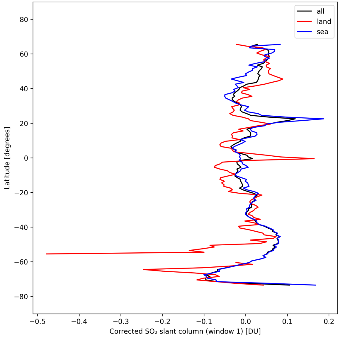
Figure 38: Zonal average of “Corrected SO 2 slant column (window 1)” for 2025-10-03 to 2025-10-04.
