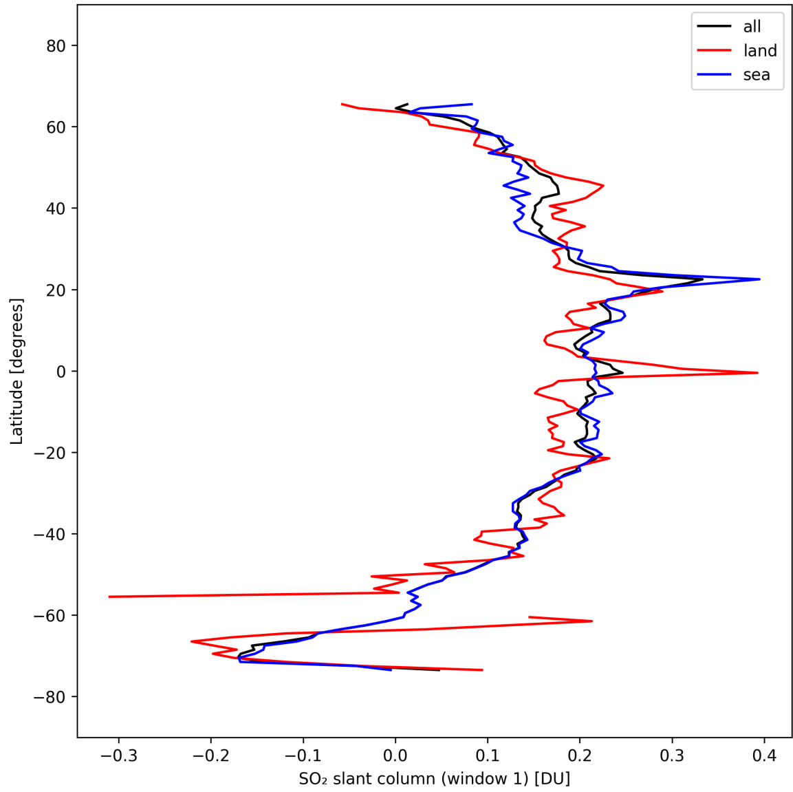
Figure 36: Zonal average of “SO 2 slant column (window 1)” for 2025-10-03 to 2025-10-04.
