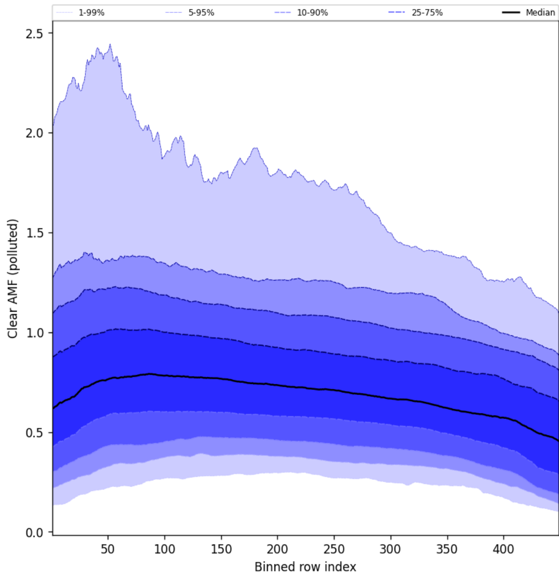
Figure 109: Along track statistics of “Clear AMF (polluted)” for 2025-10-03 to 2025-10-04
