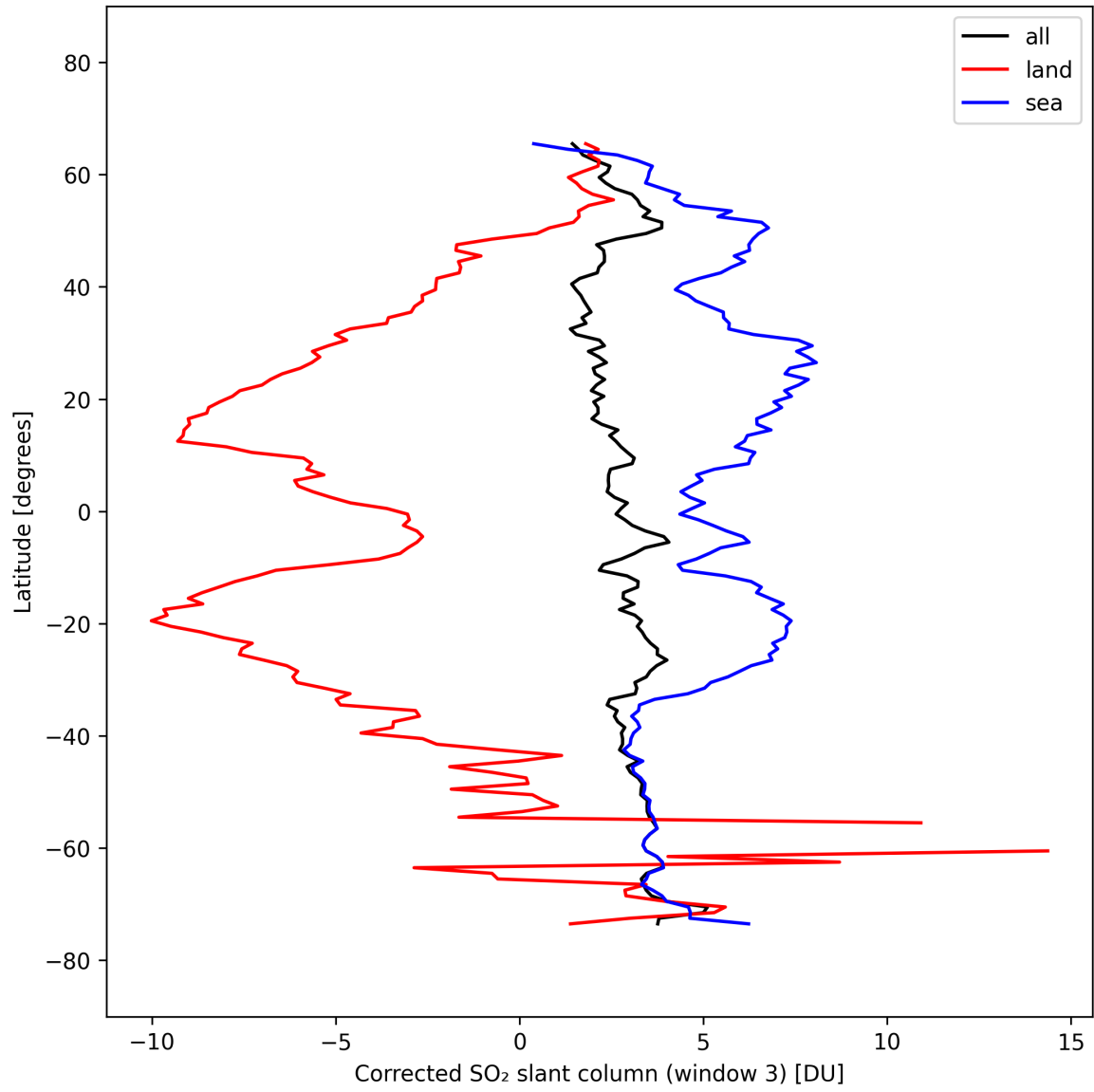
Figure 46: Zonal average of “Corrected SO 2 slant column (window 3)” for 2025-10-03 to 2025-10-04.
