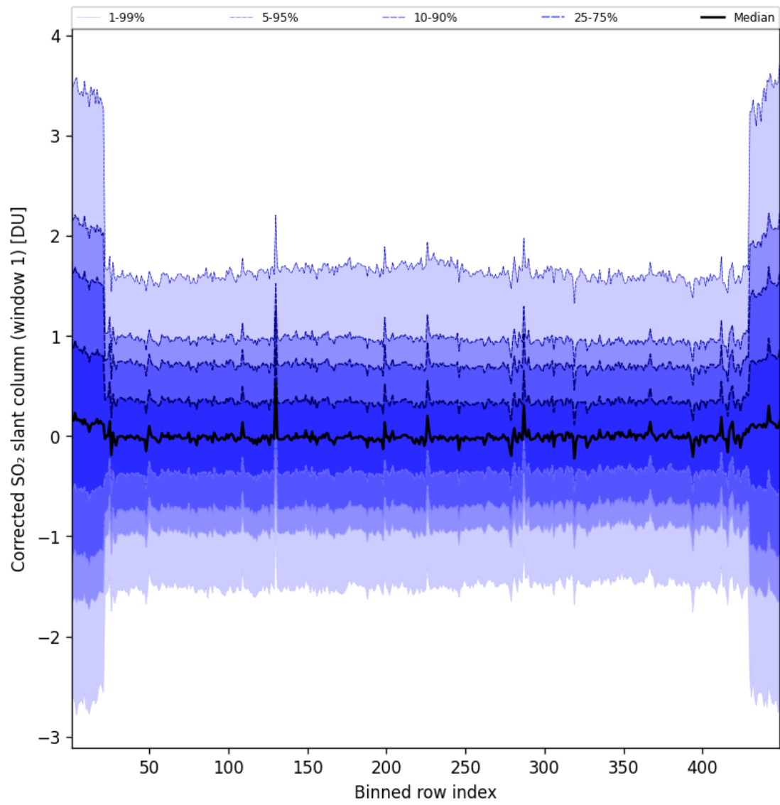
Figure 92: Along track statistics of “Corrected SO 2 slant column (window 1)” for 2025-10-03 to 2025-10-04
