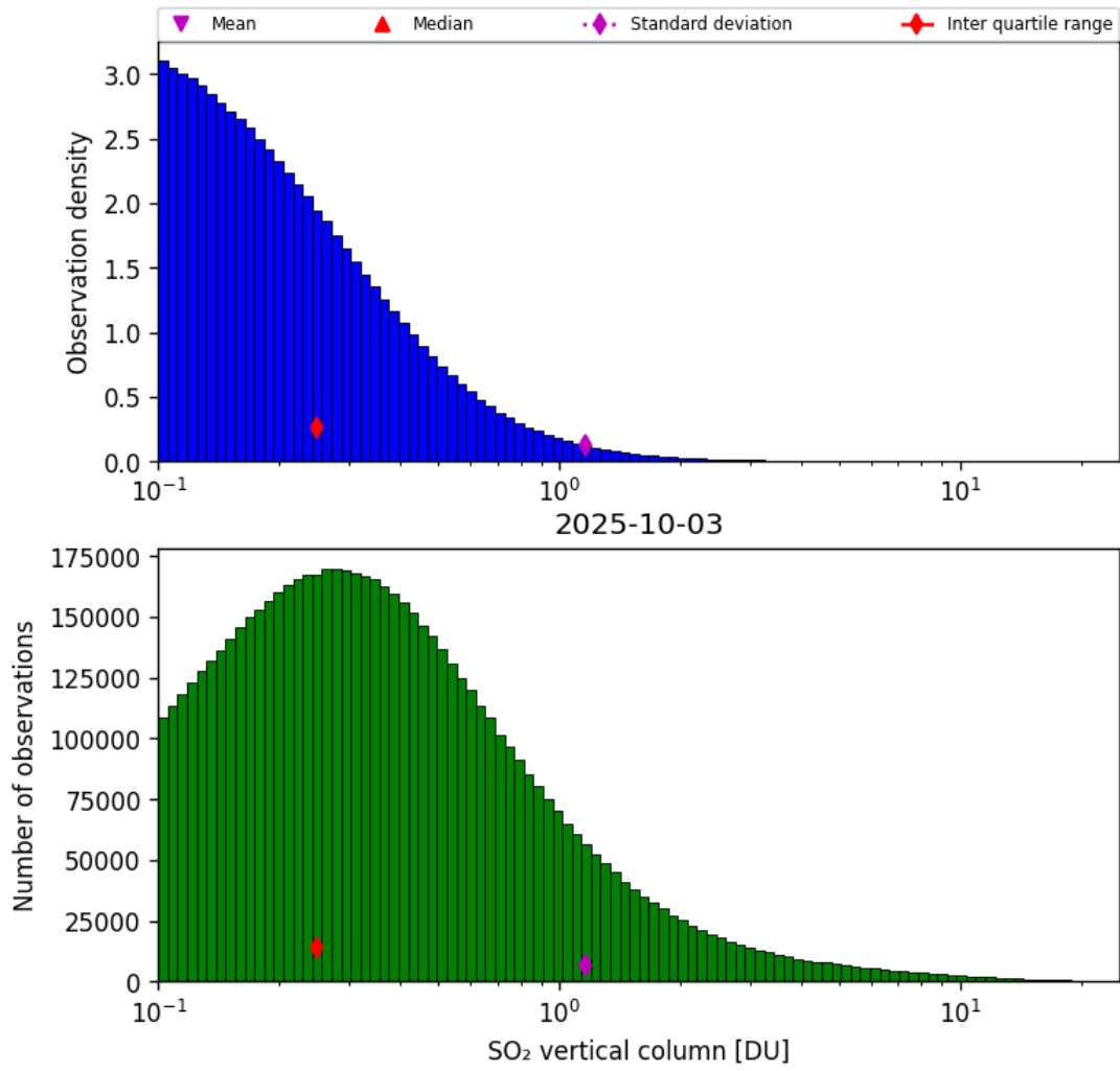
Figure 58: Histogram of “SO 2 vertical column” for 2025-10-03 to 2025-10-04
