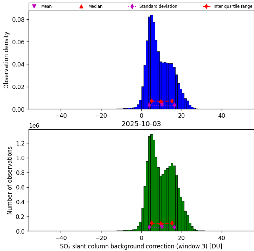
Figure 74: Histogram of “SO 2 slant column background correction (window 3)” for 2025-10-03 to 2025-10-04
