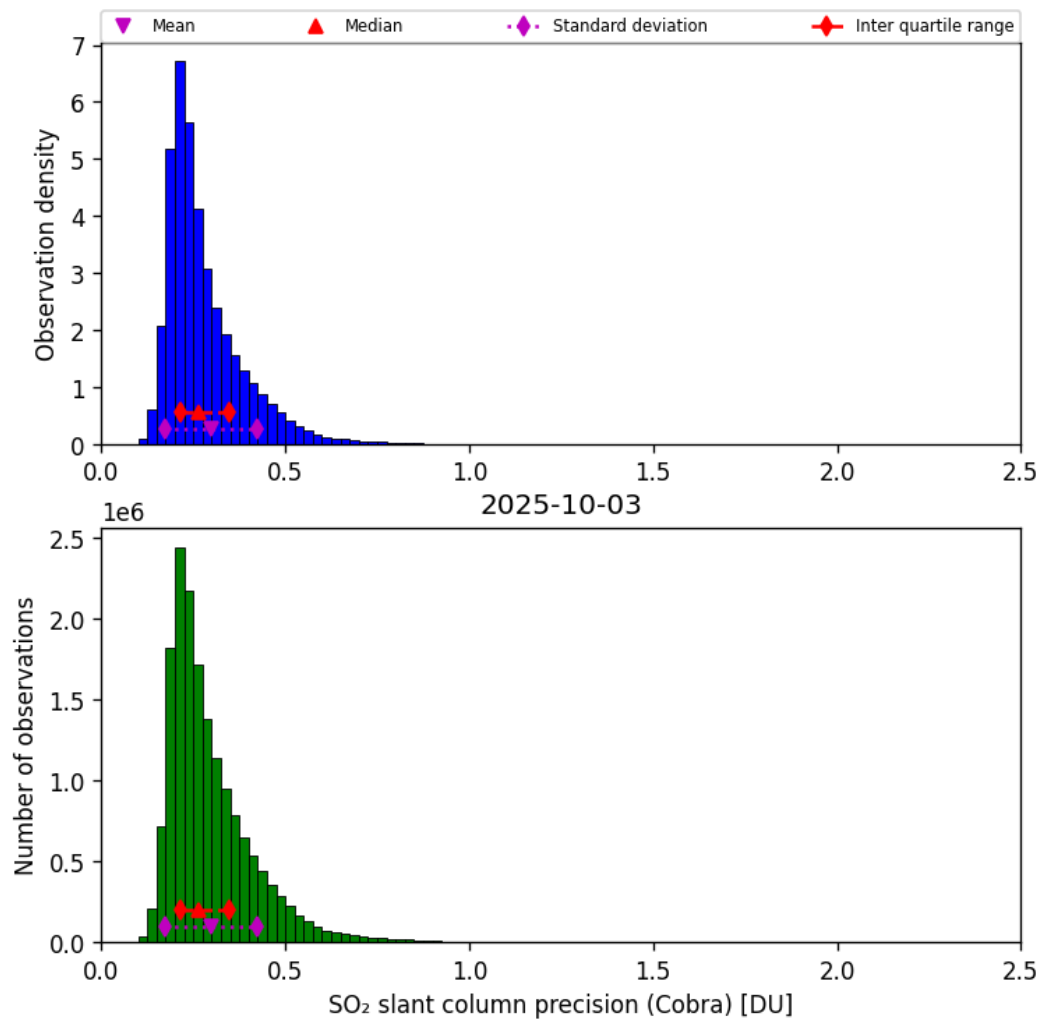
Figure 62: Histogram of “SO 2 slant column precision (Cobra)” for 2025-10-03 to 2025-10-04
