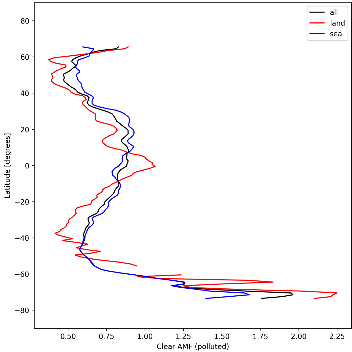
Figure 55: Zonal average of “Clear AMF (polluted)” for 2025-10-03 to 2025-10-04.
