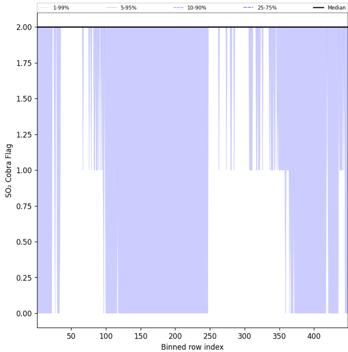
Figure 102: Along track statistics of "SO 2 Cobra Flag" for 2025-10-03 to 2025-10-04
