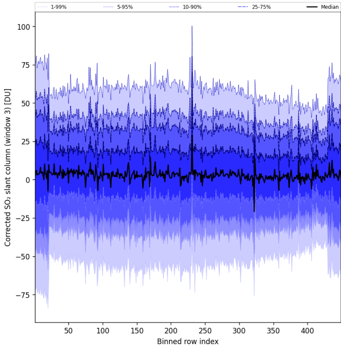
Figure 100: Along track statistics of “Corrected SO 2 slant column (window 3)” for 2025-10-03 to 2025-10-04
