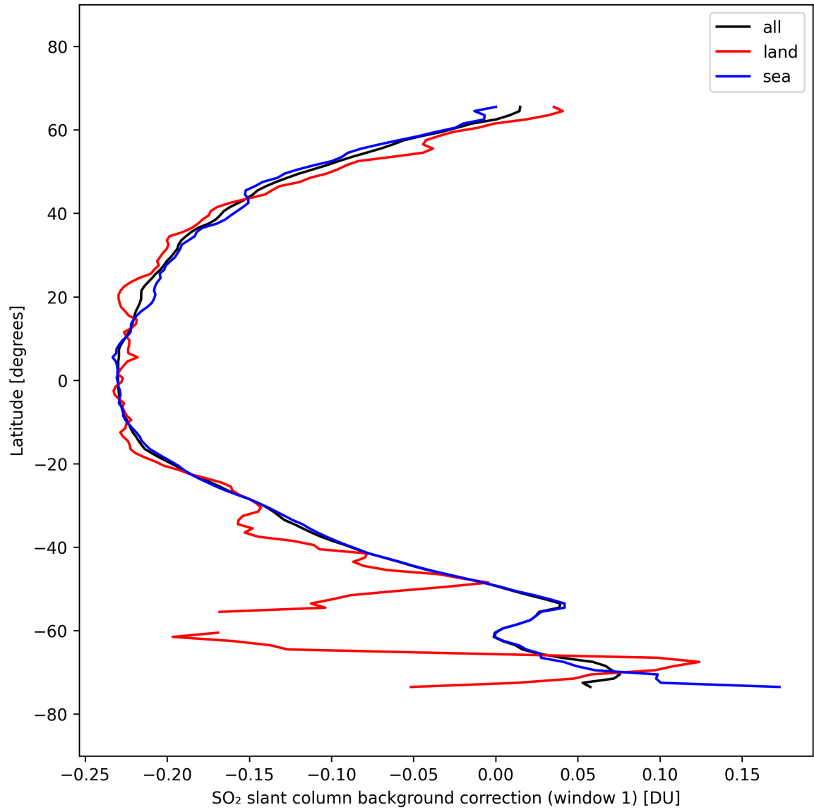
Figure 39: Zonal average of “SO 2 slant column background correction (window 1)” for 2025-10-03 to 2025-10-04.
