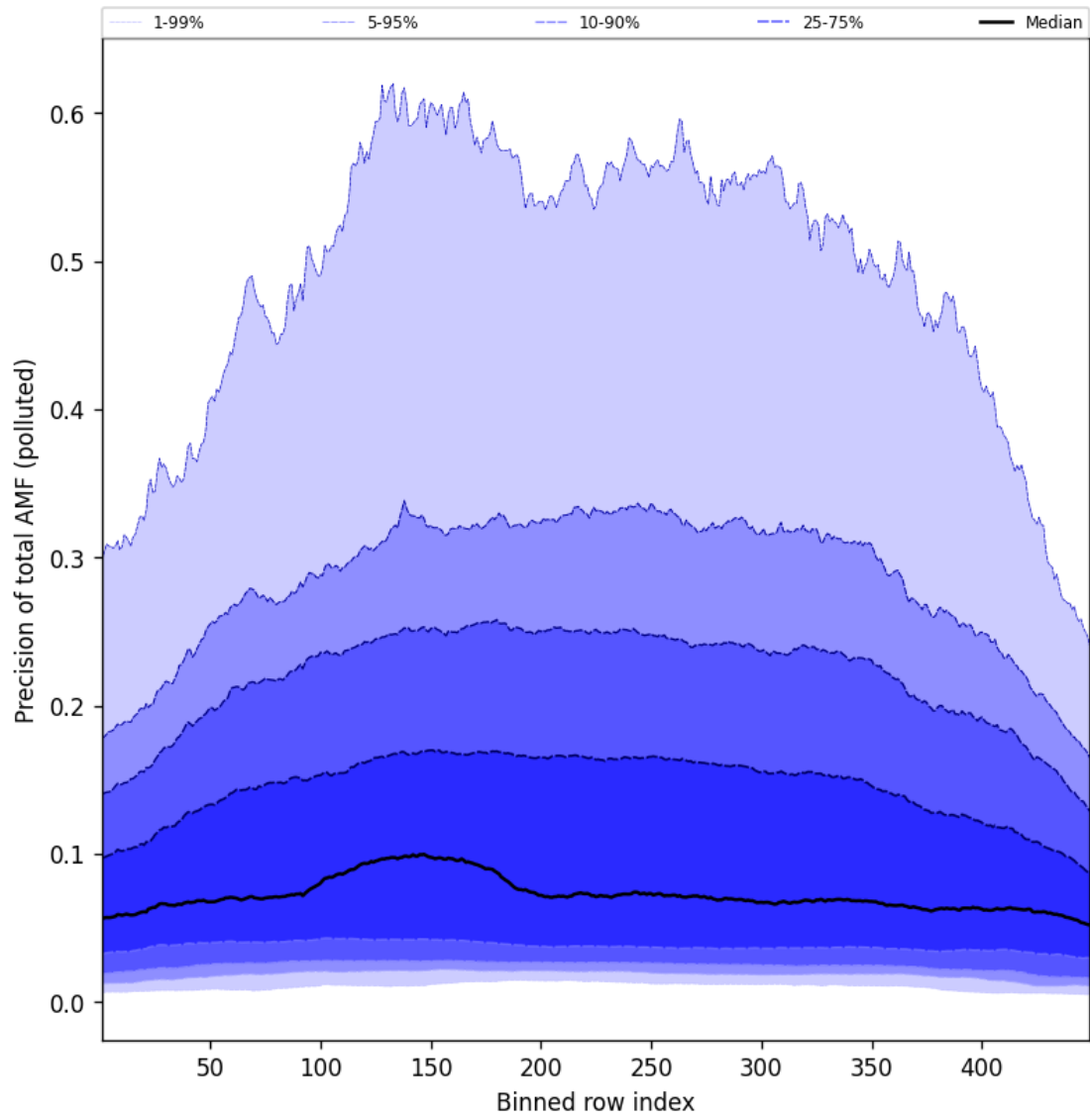
Figure 108: Along track statistics of “Precision of total AMF (polluted)” for 2025-10-03 to 2025-10-04
