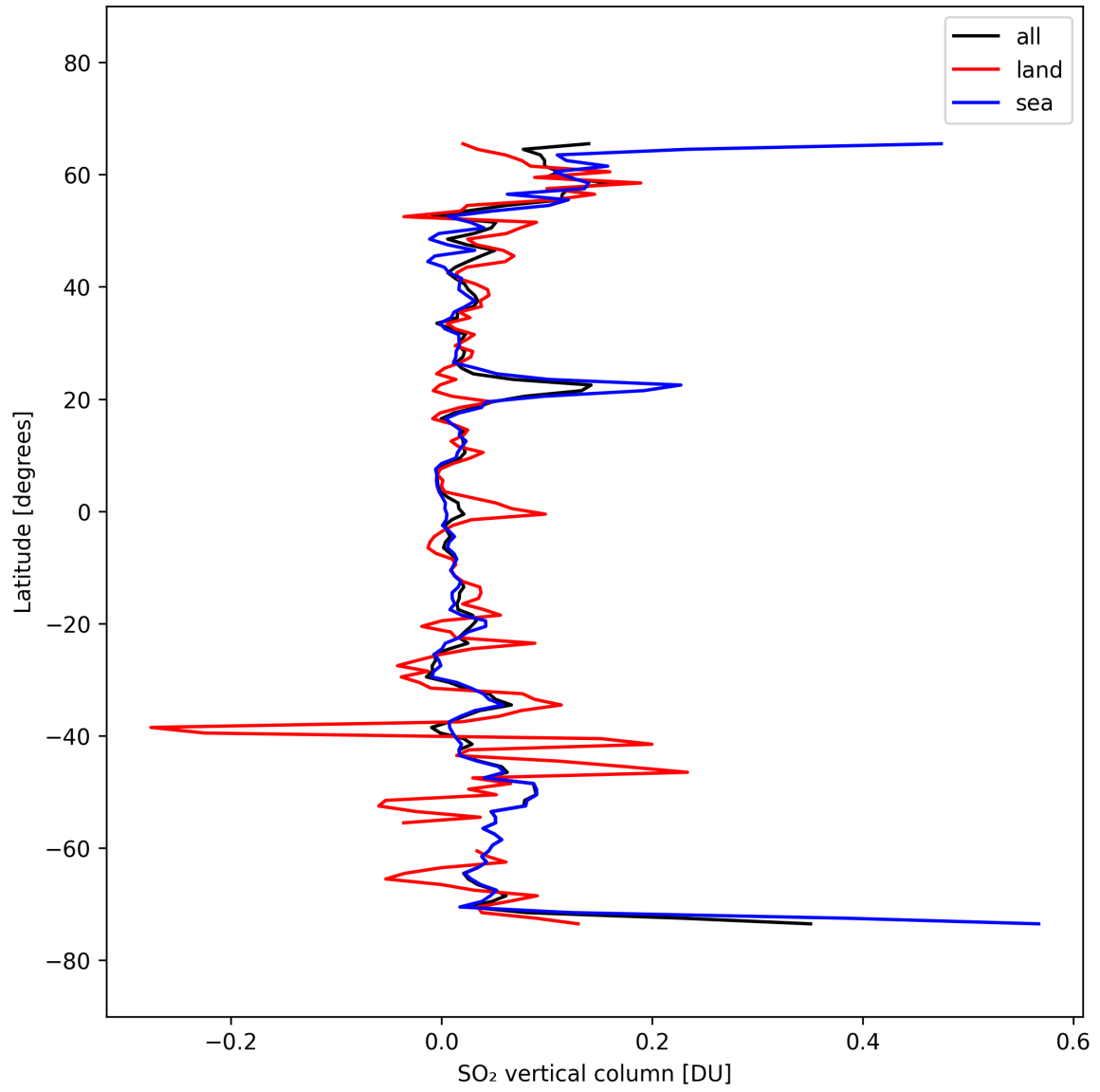
Figure 31: Zonal average of “SO 2 vertical column” for 2025-10-03 to 2025-10-04.
