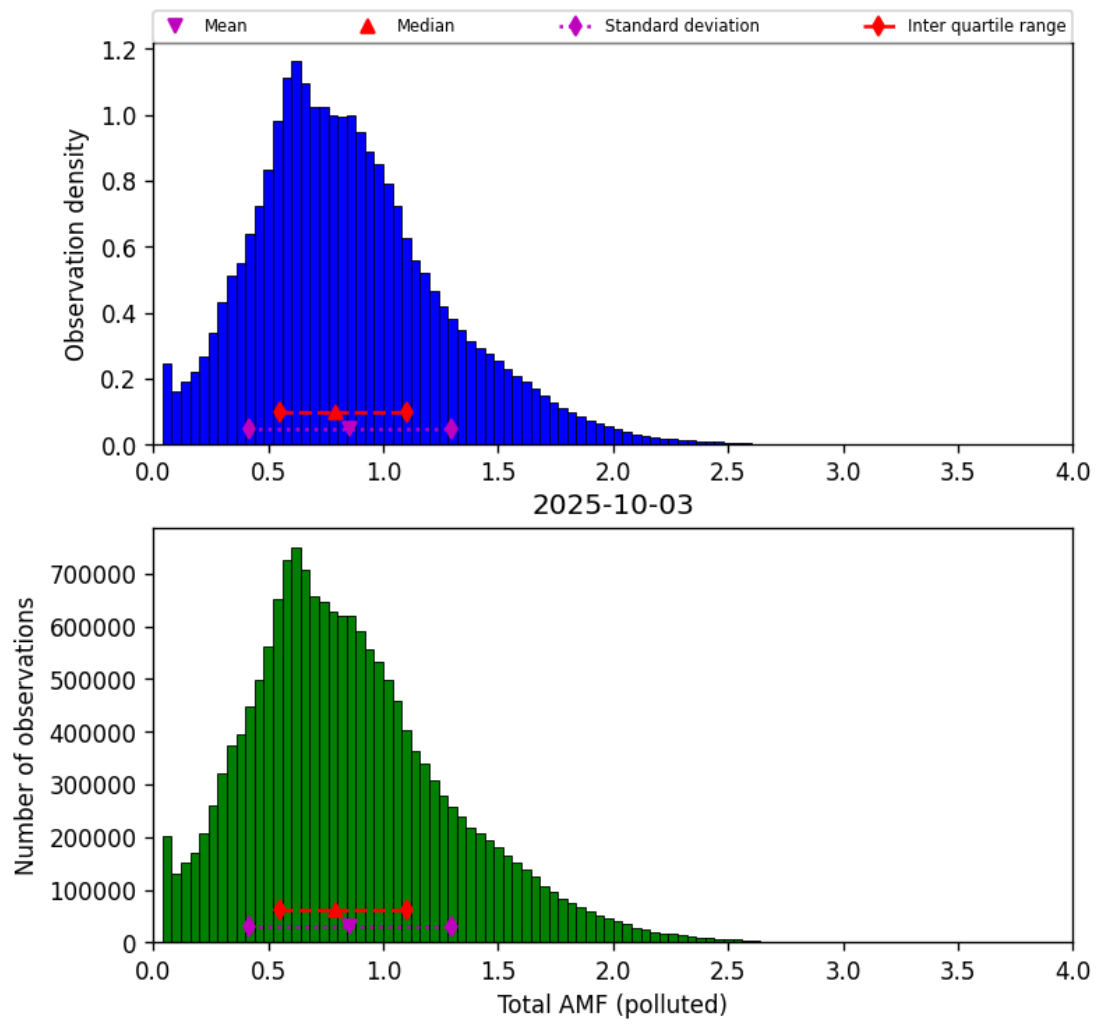
Figure 80: Histogram of “Total AMF (polluted)” for 2025-10-03 to 2025-10-04
