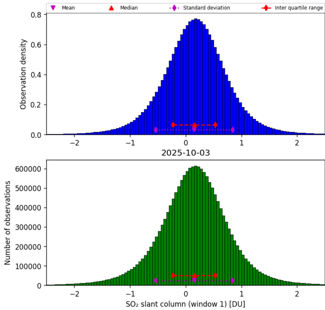
Figure 63: Histogram of “SO 2 slant column (window 1)” for 2025-10-03 to 2025-10-04
