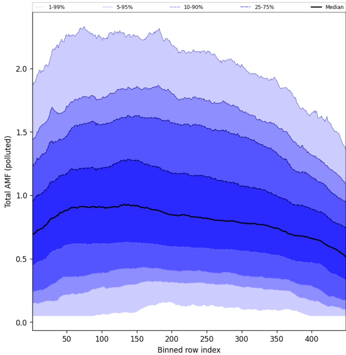
Figure 107: Along track statistics of “Total AMF (polluted)” for 2025-10-03 to 2025-10-04
