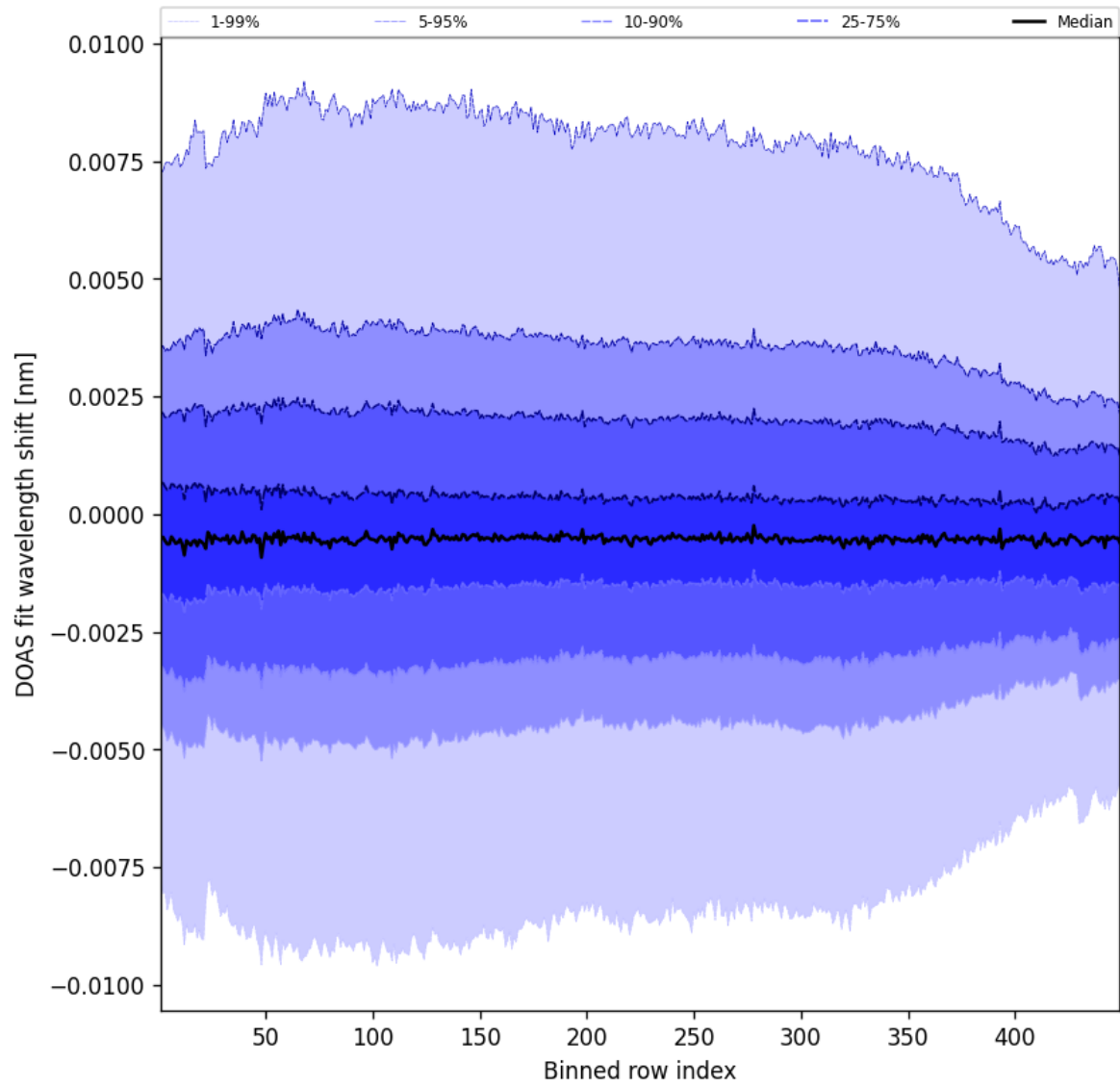
Figure 104: Along track statistics of “DOAS fit wavelength shift” for 2025-10-03 to 2025-10-04
