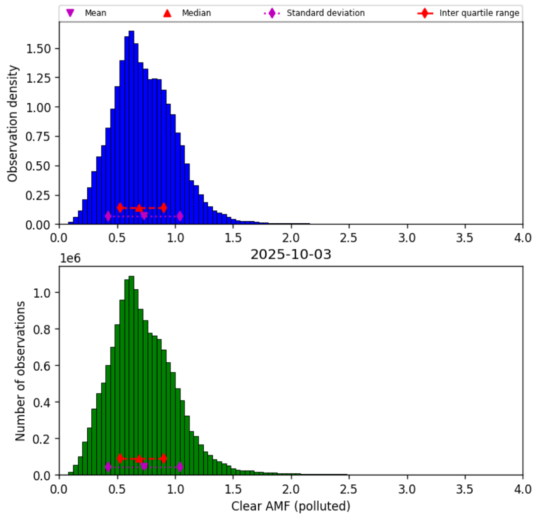
Figure 82: Histogram of “Clear AMF (polluted)” for 2025-10-03 to 2025-10-04
