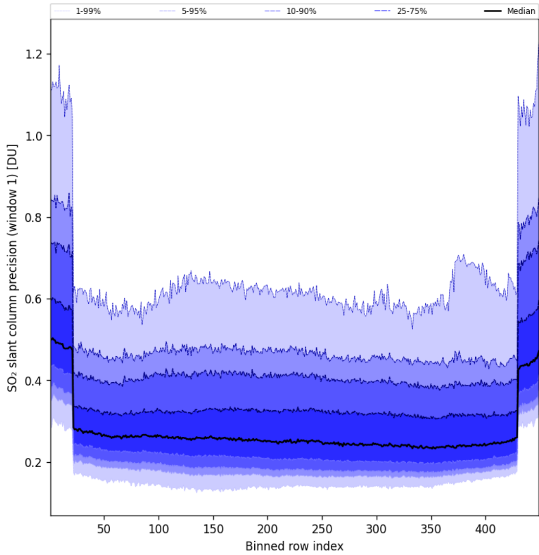
Figure 91: Along track statistics of “SO 2 slant column precision (window 1)” for 2025-10-03 to 2025-10-04
