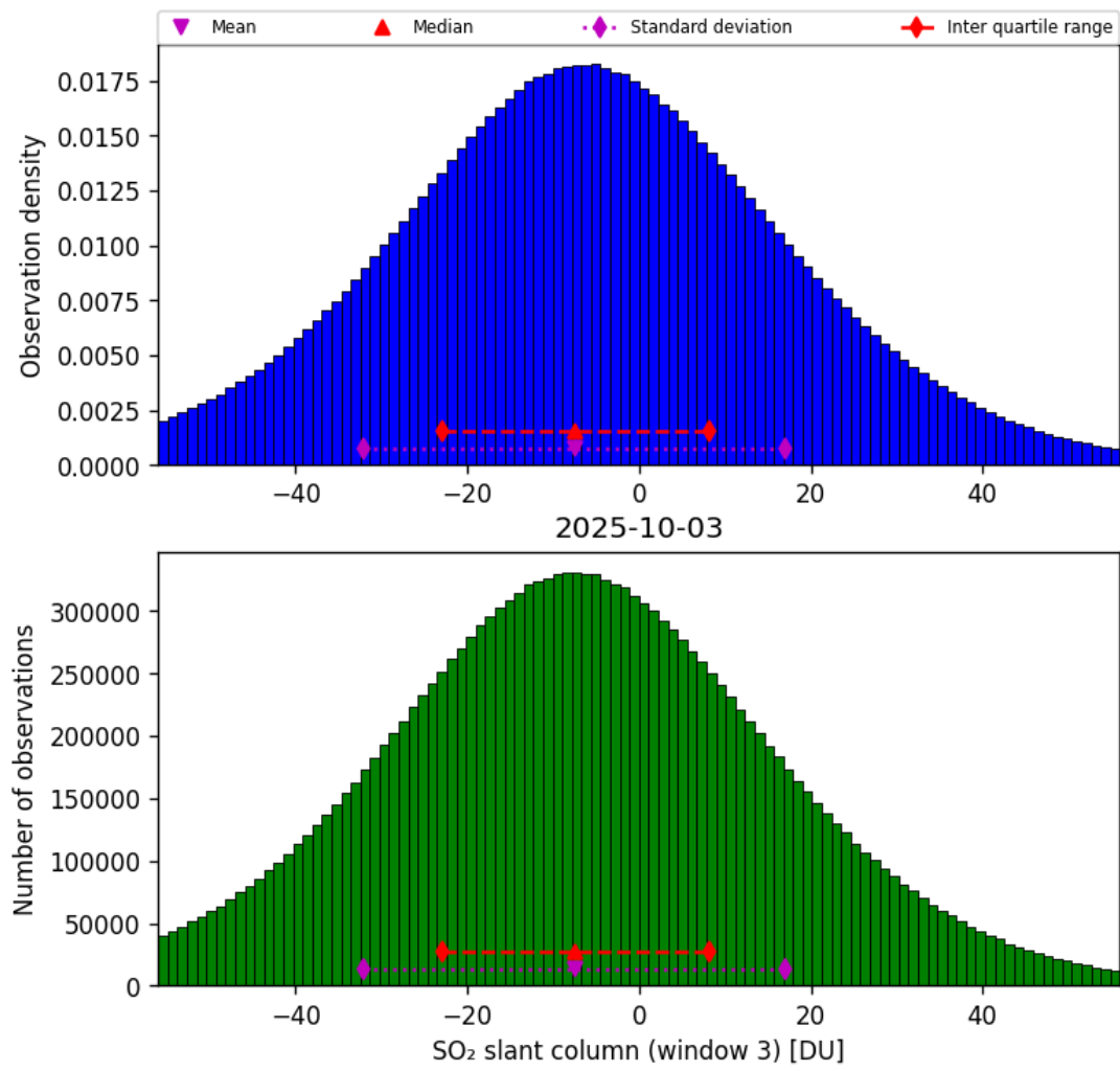
Figure 71: Histogram of “SO 2 slant column (window 3)” for 2025-10-03 to 2025-10-04
