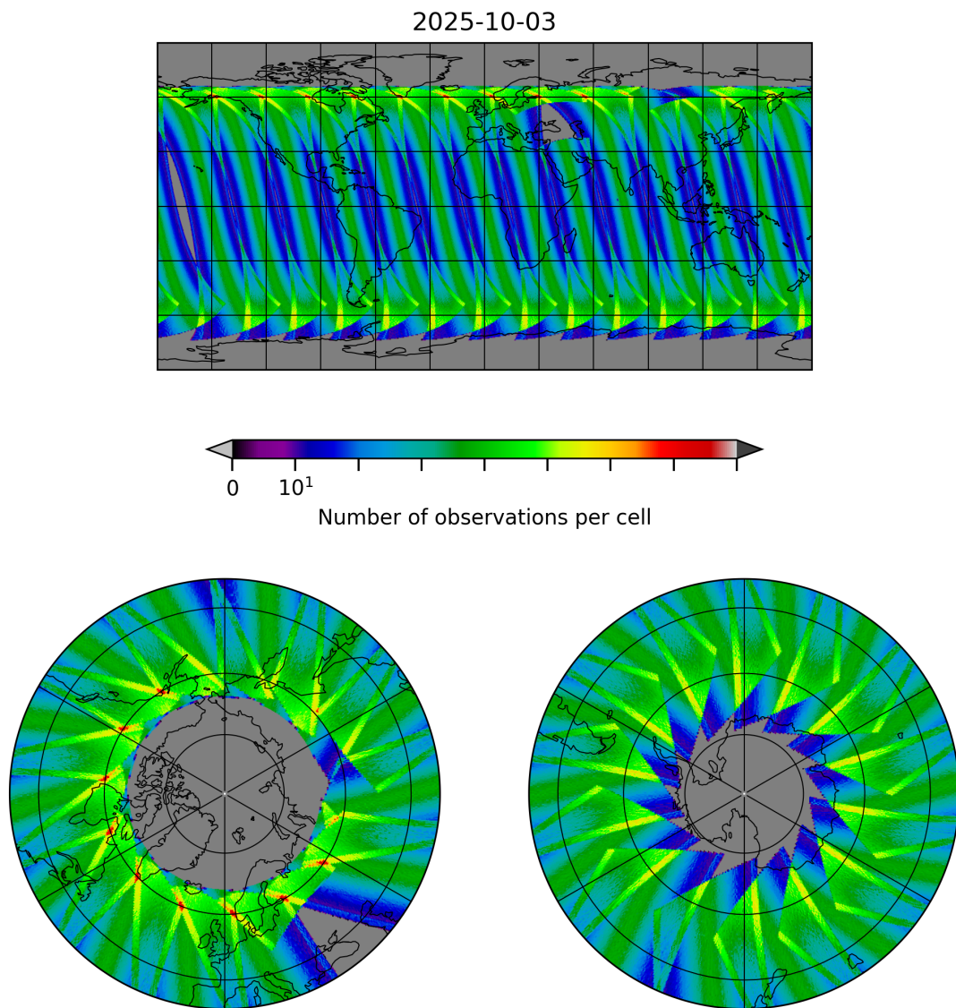
Figure 29: Map of the number of observations for 2025-10-03 to 2025-10-04
