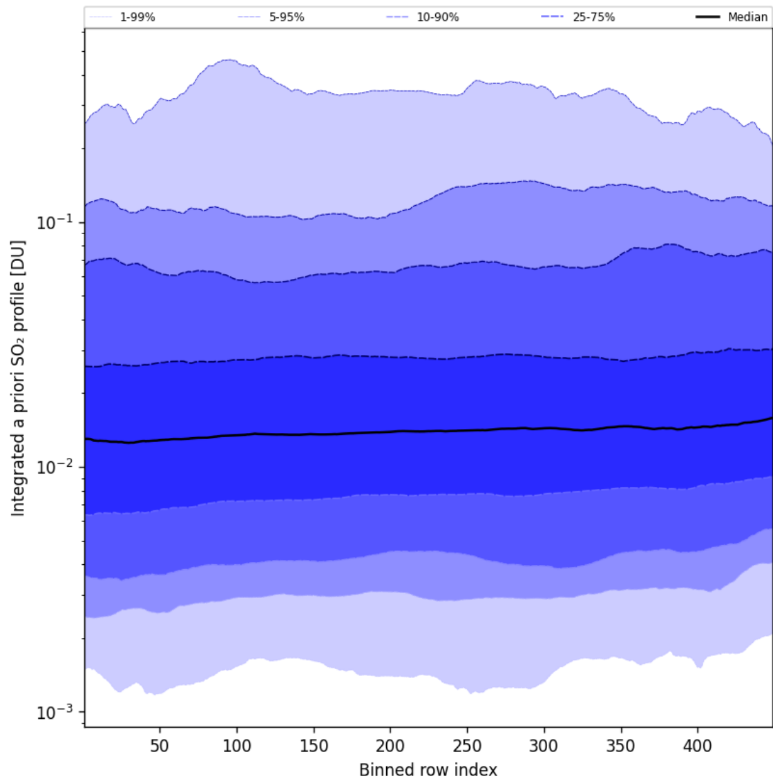
Figure 103: Along track statistics of “Integrated a priori SO 2 profile” for 2025-10-03 to 2025-10-04
