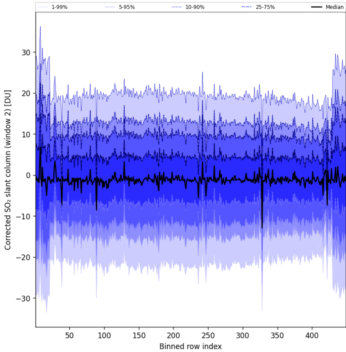
Figure 96: Along track statistics of “Corrected SO 2 slant column (window 2)” for 2025-10-03 to 2025-10-04
