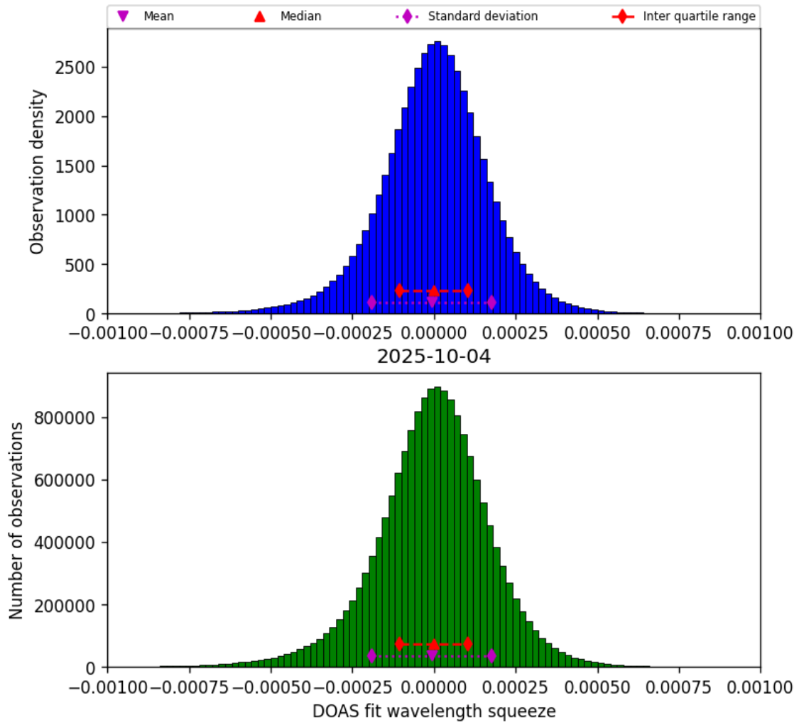
Figure 78: Histogram of “DOAS fit wavelength squeeze” for 2025-10-04 to 2025-10-04
