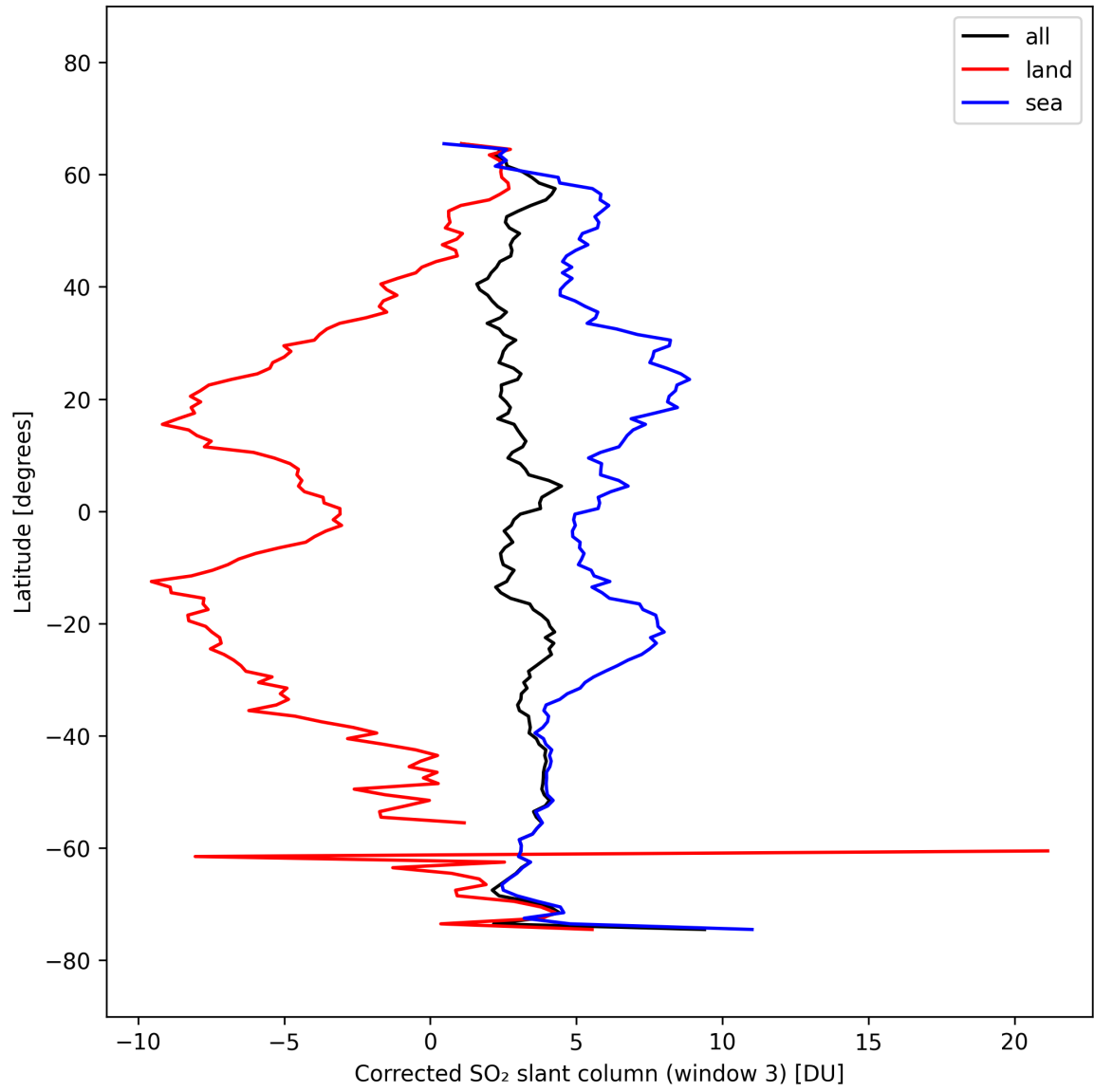
Figure 46: Zonal average of “Corrected SO 2 slant column (window 3)” for 2025-10-04 to 2025-10-04.
