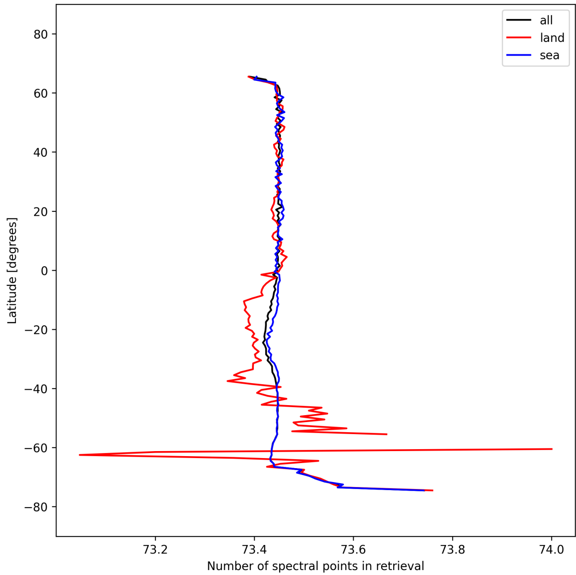
Figure 56: Zonal average of “Number of spectral points in retrieval” for 2025-10-04 to 2025-10-04.
