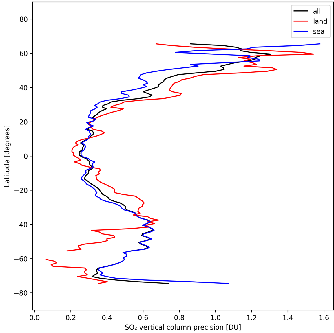
Figure 32: Zonal average of “SO 2 vertical column precision” for 2025-10-04 to 2025-10-04.
