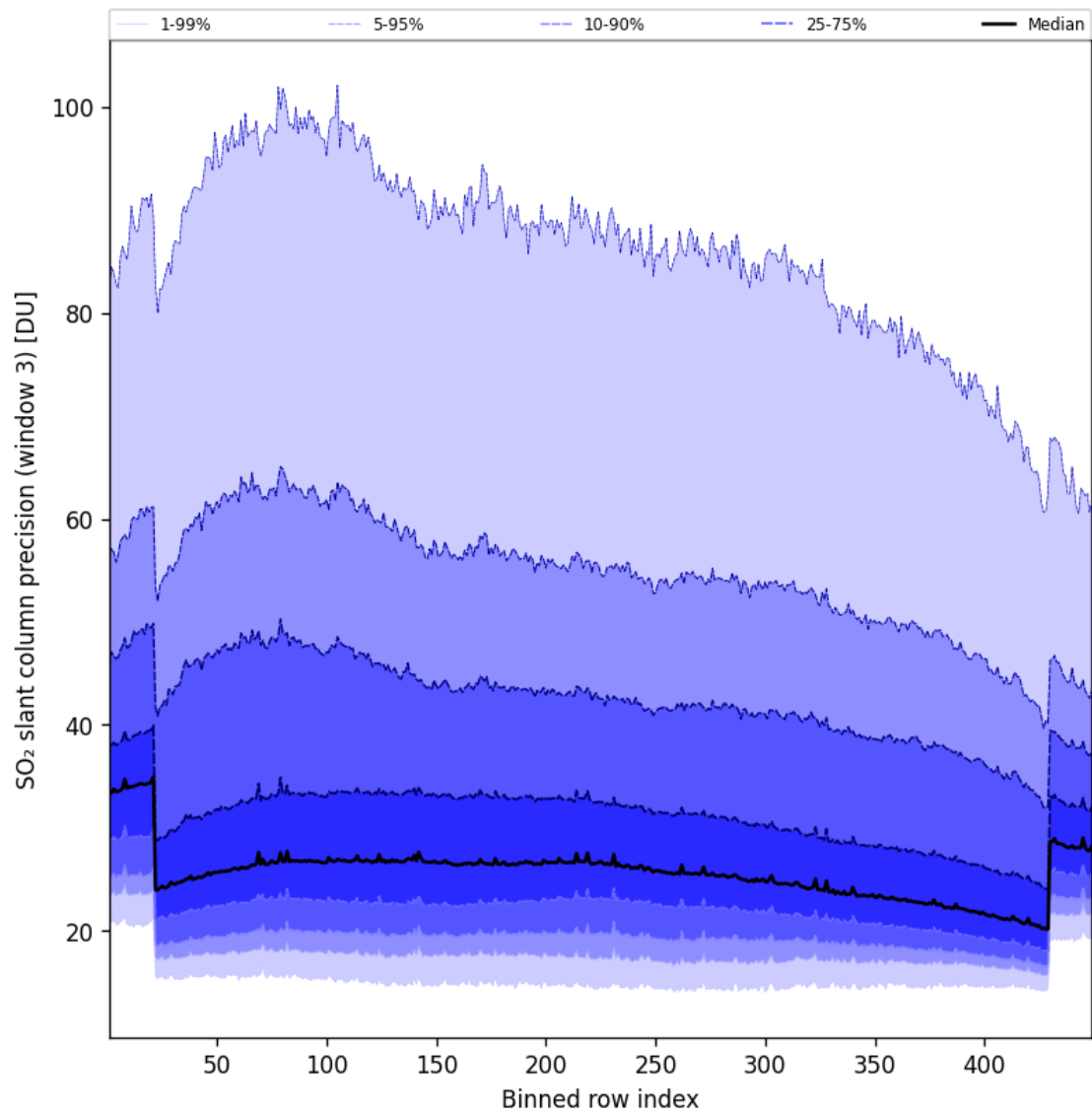
Figure 99: Along track statistics of “SO 2 slant column precision (window 3)” for 2025-10-04 to 2025-10-04
