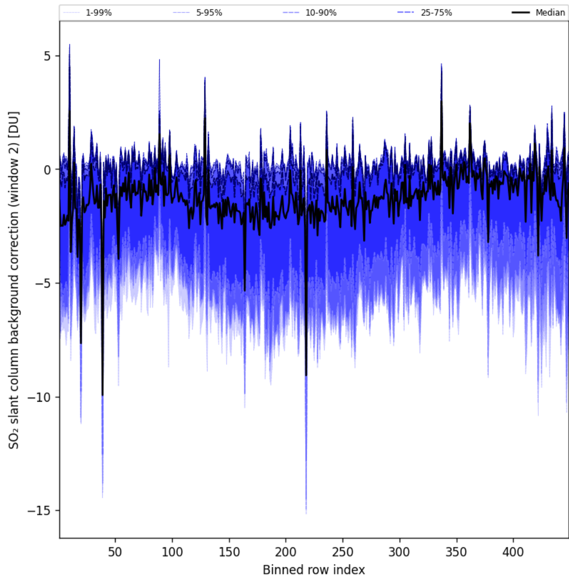
Figure 97: Along track statistics of “SO 2 slant column background correction (window 2)” for 2025-10-04 to 2025-10-04
