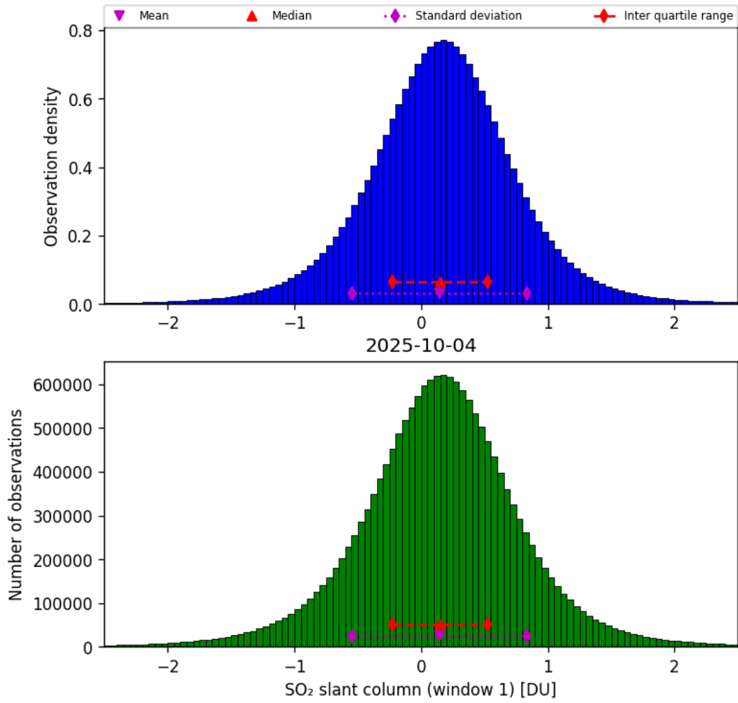
Figure 63: Histogram of “SO 2 slant column (window 1)” for 2025-10-04 to 2025-10-04
