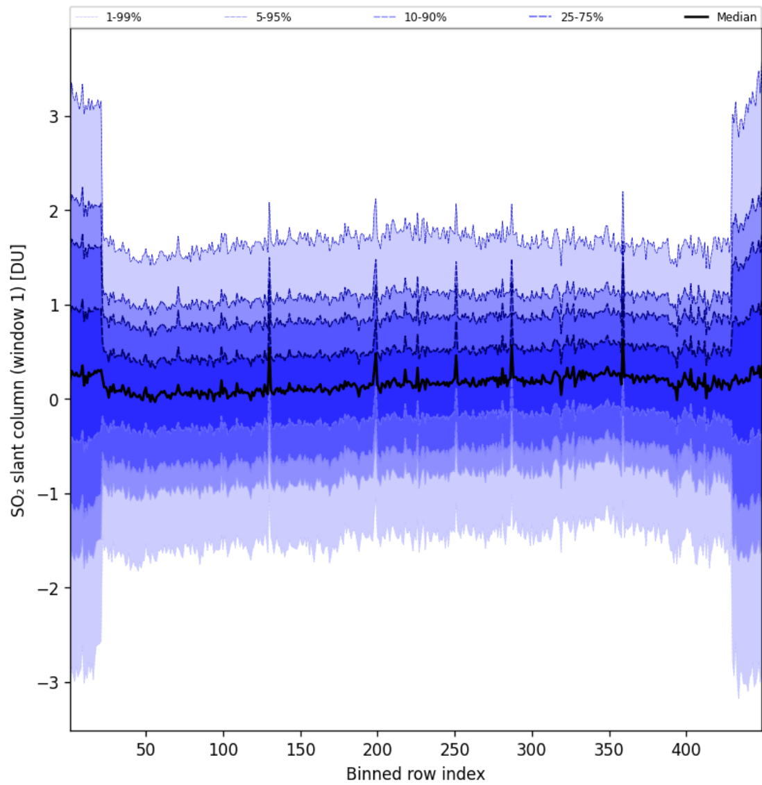
Figure 90: Along track statistics of “SO 2 slant column (window 1)” for 2025-10-04 to 2025-10-04
