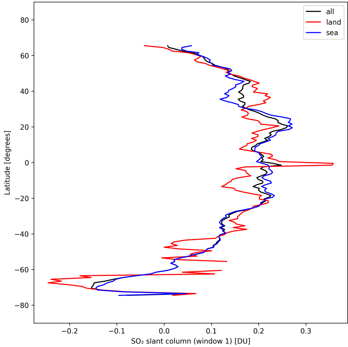
Figure 36: Zonal average of “SO 2 slant column (window 1)” for 2025-10-04 to 2025-10-04.
