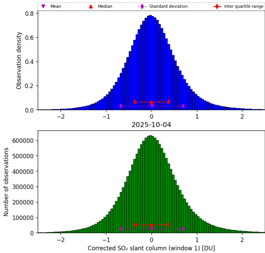
Figure 65: Histogram of “Corrected SO 2 slant column (window 1)” for 2025-10-04 to 2025-10-04
