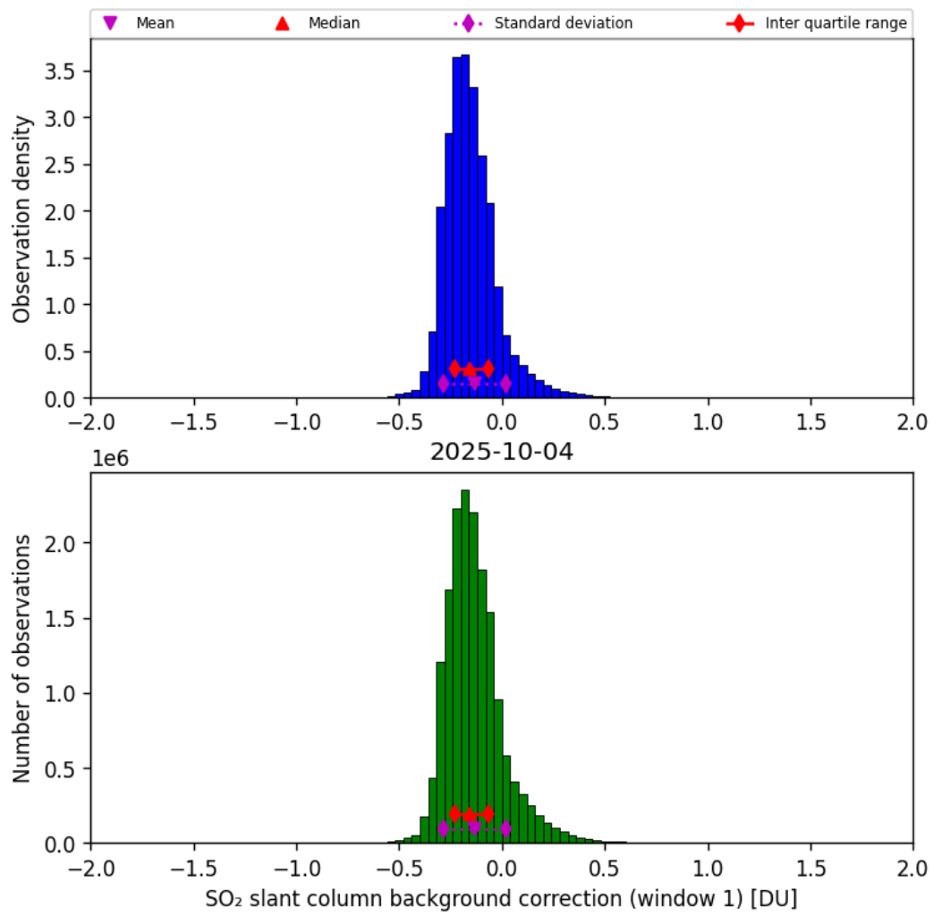
Figure 66: Histogram of “SO 2 slant column background correction (window 1)” for 2025-10-04 to 2025-10-04
