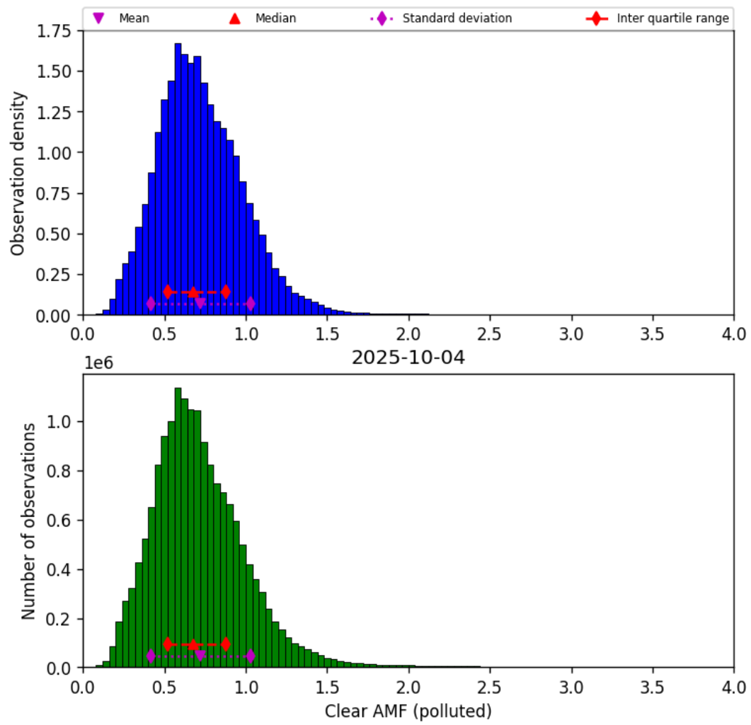
Figure 82: Histogram of “Clear AMF (polluted)” for 2025-10-04 to 2025-10-04
