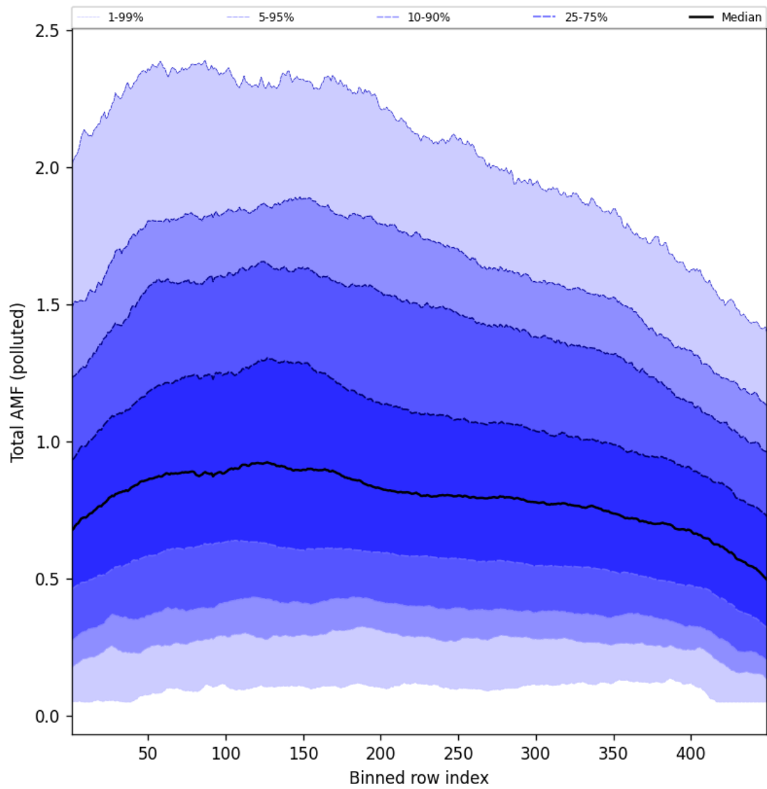
Figure 107: Along track statistics of “Total AMF (polluted)” for 2025-10-04 to 2025-10-04
