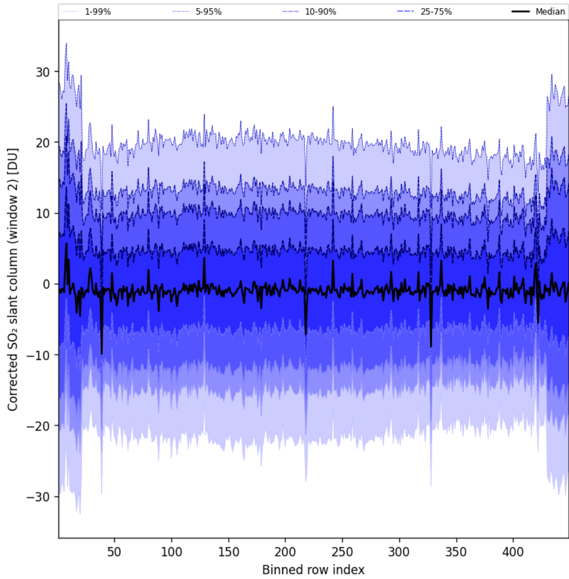
Figure 96: Along track statistics of “Corrected SO 2 slant column (window 2)” for 2025-10-04 to 2025-10-04
