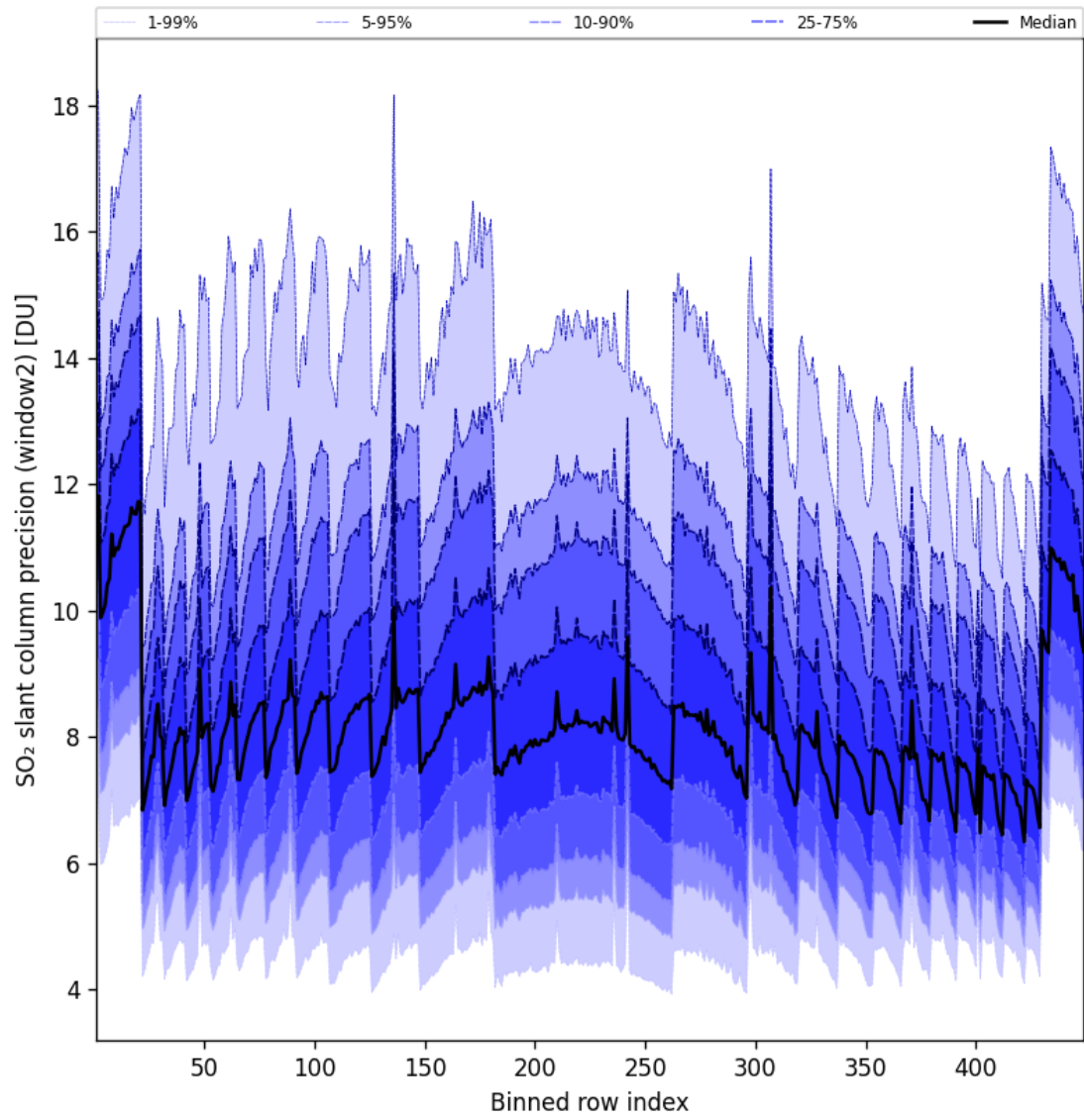
Figure 95: Along track statistics of “SO 2 slant column precision (window2)” for 2025-10-04 to 2025-10-04
