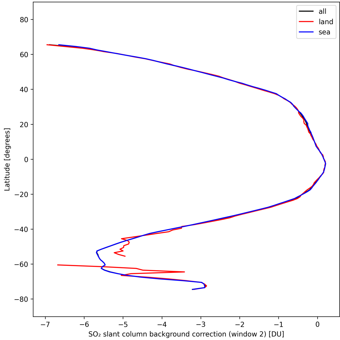
Figure 43: Zonal average of “SO 2 slant column background correction (window 2)” for 2025-10-04 to 2025-10-04.
