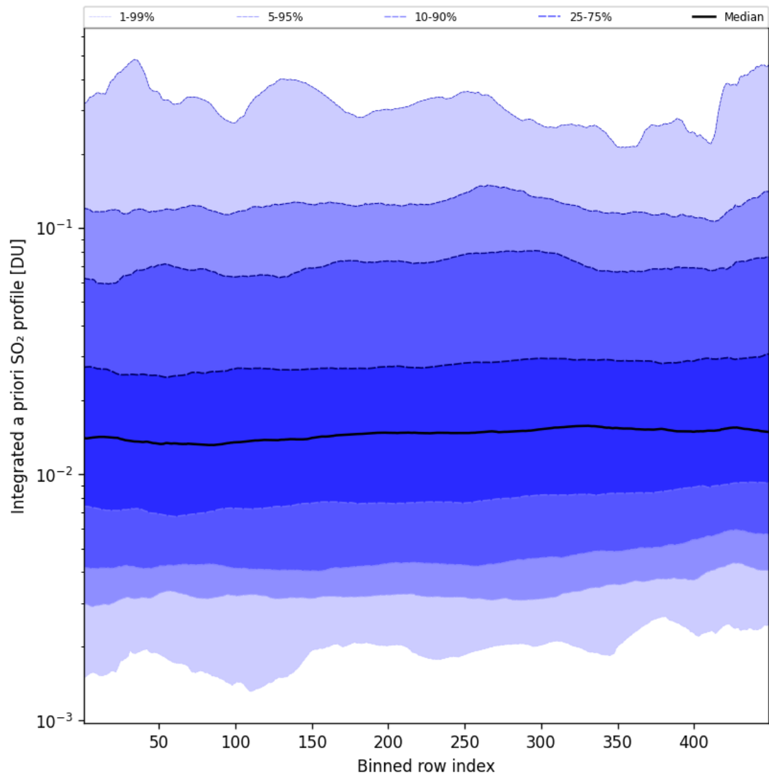
Figure 103: Along track statistics of “Integrated a priori SO 2 profile” for 2025-10-04 to 2025-10-04
