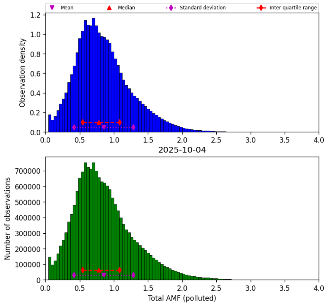
Figure 80: Histogram of “Total AMF (polluted)” for 2025-10-04 to 2025-10-04
