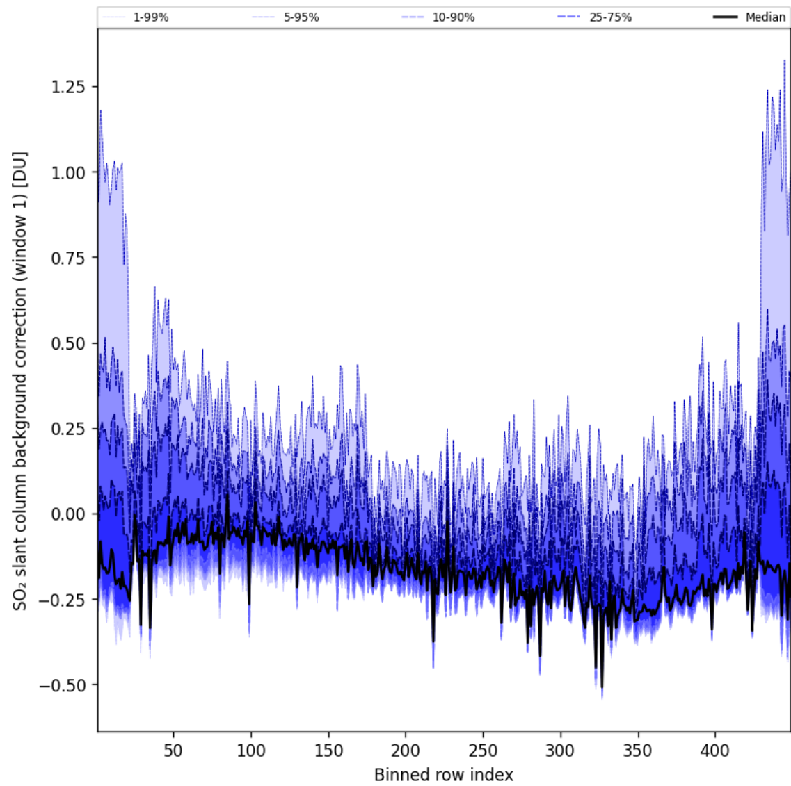
Figure 93: Along track statistics of “SO 2 slant column background correction (window 1)” for 2025-10-04 to 2025-10-04
