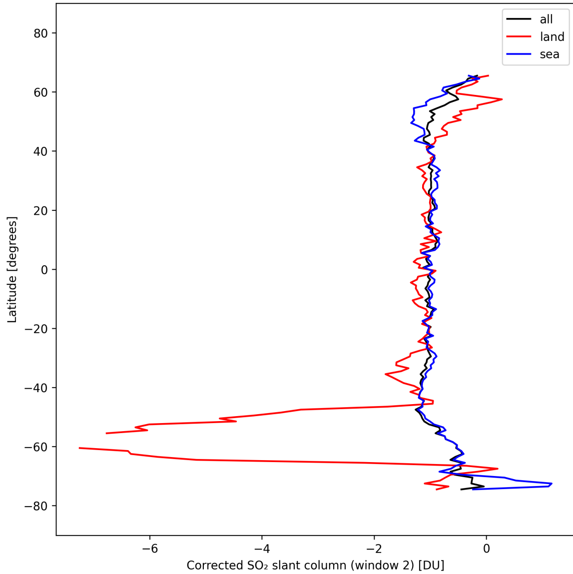
Figure 42: Zonal average of “Corrected SO 2 slant column (window 2)” for 2025-10-04 to 2025-10-04.
