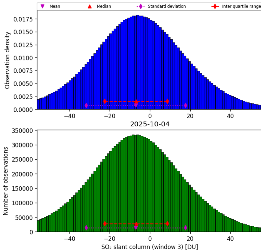
Figure 71: Histogram of “SO 2 slant column (window 3)” for 2025-10-04 to 2025-10-04
