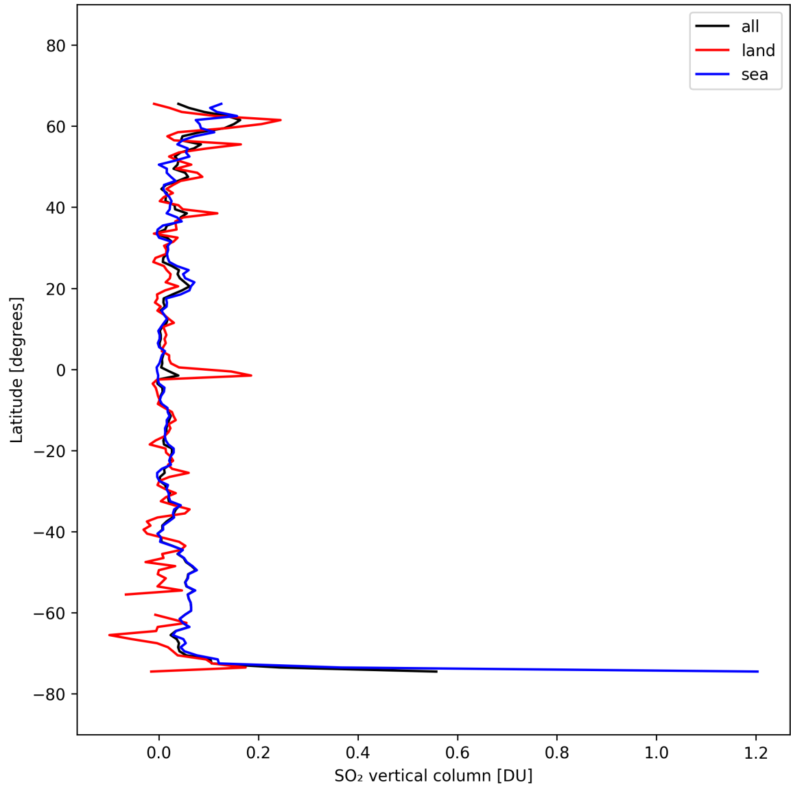
Figure 31: Zonal average of “SO 2 vertical column” for 2025-10-04 to 2025-10-04.
