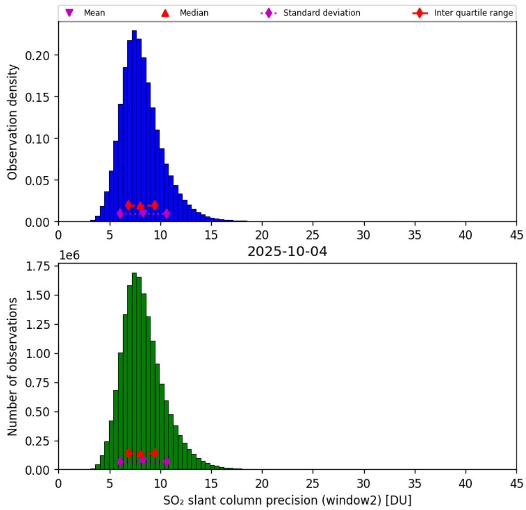
Figure 68: Histogram of “SO 2 slant column precision (window2)” for 2025-10-04 to 2025-10-04
