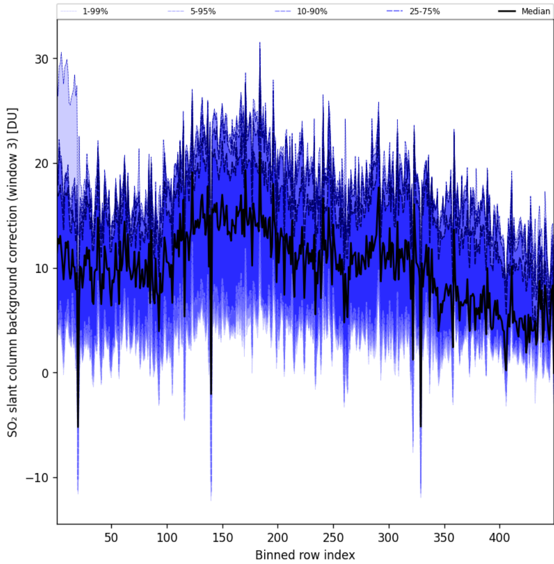
Figure 101: Along track statistics of “SO 2 slant column background correction (window 3)” for 2025-10-04 to 2025-10-04
