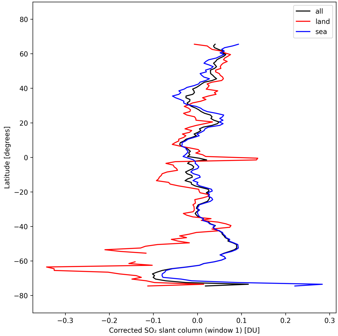
Figure 38: Zonal average of “Corrected SO 2 slant column (window 1)” for 2025-10-04 to 2025-10-04.
