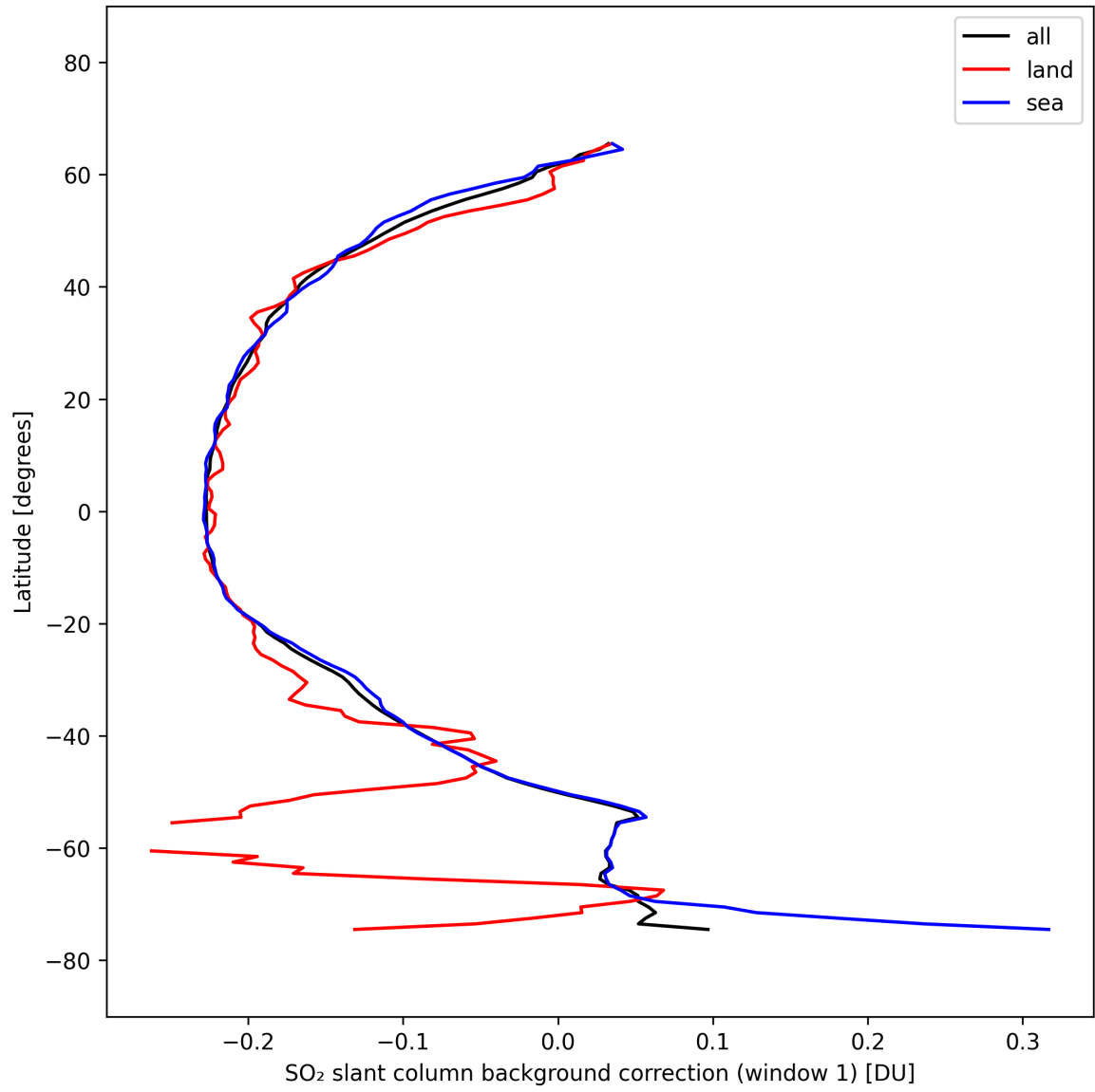
Figure 39: Zonal average of “SO 2 slant column background correction (window 1)” for 2025-10-04 to 2025-10-04.
