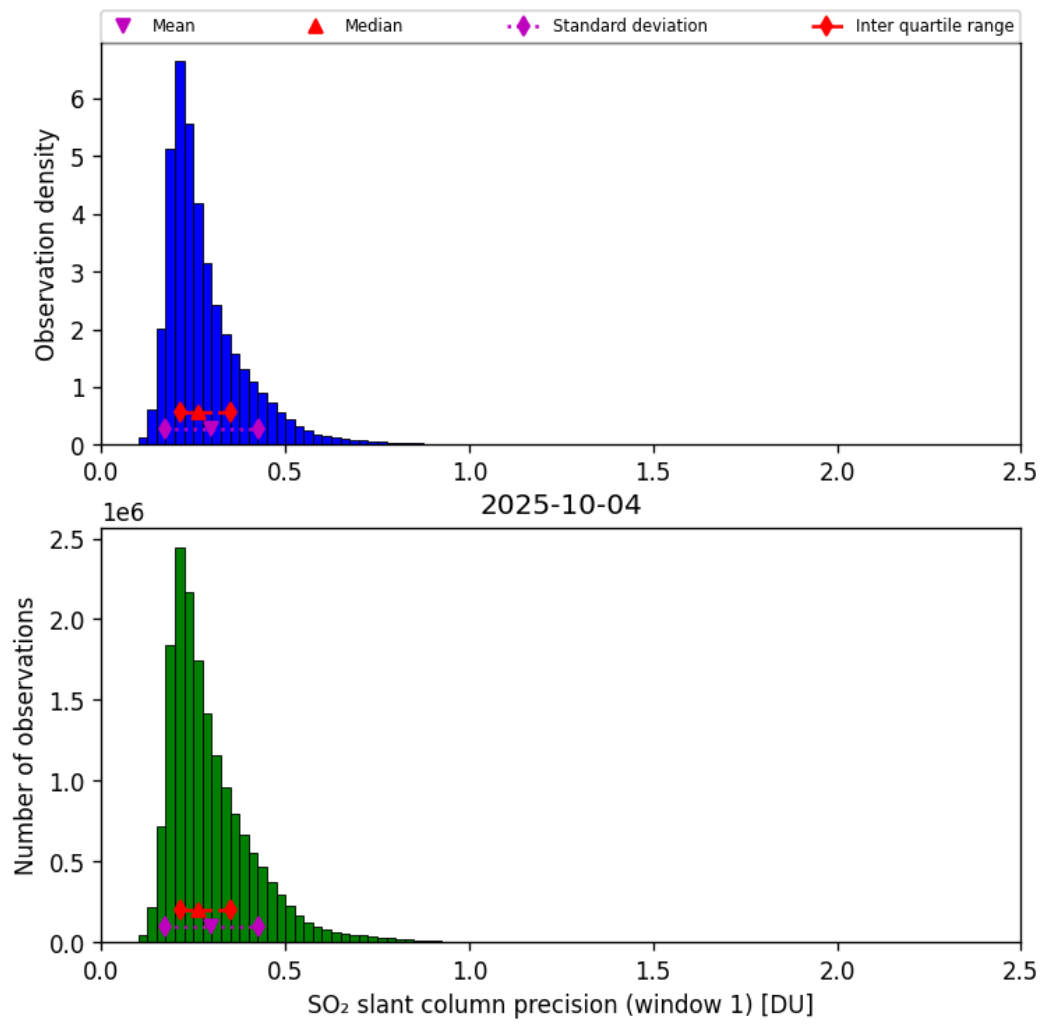
Figure 64: Histogram of “SO 2 slant column precision (window 1)” for 2025-10-04 to 2025-10-04
