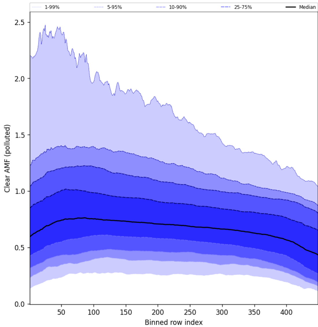
Figure 109: Along track statistics of “Clear AMF (polluted)” for 2025-10-04 to 2025-10-04
