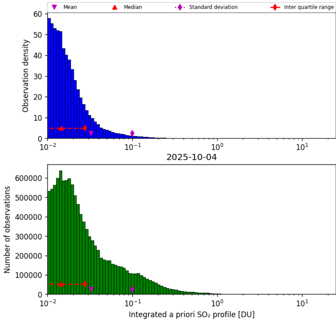
Figure 76: Histogram of “Integrated a priori SO 2 profile” for 2025-10-04 to 2025-10-04
