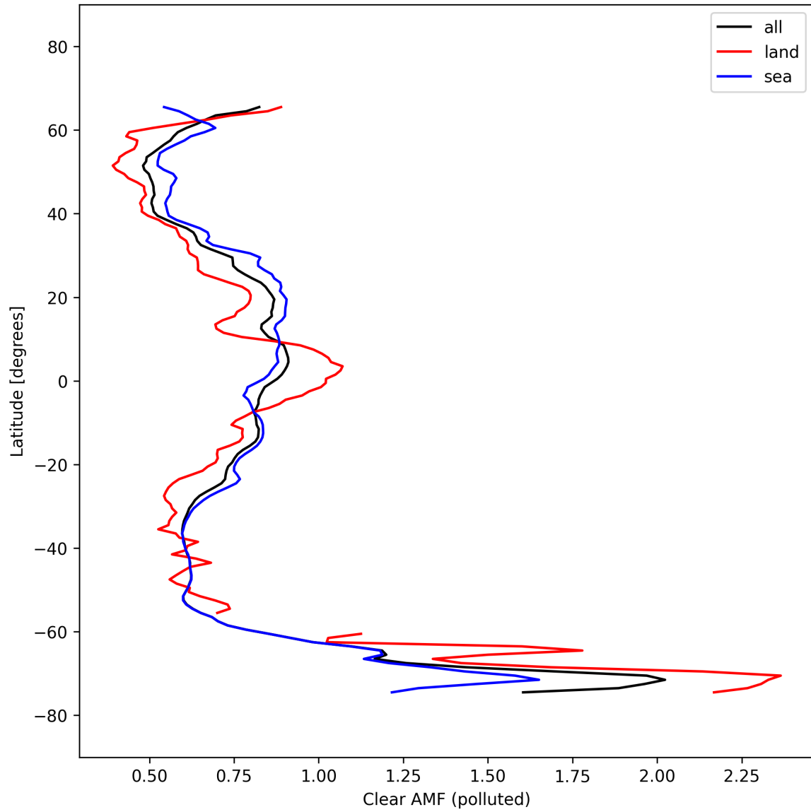
Figure 55: Zonal average of “Clear AMF (polluted)” for 2025-10-04 to 2025-10-04.
