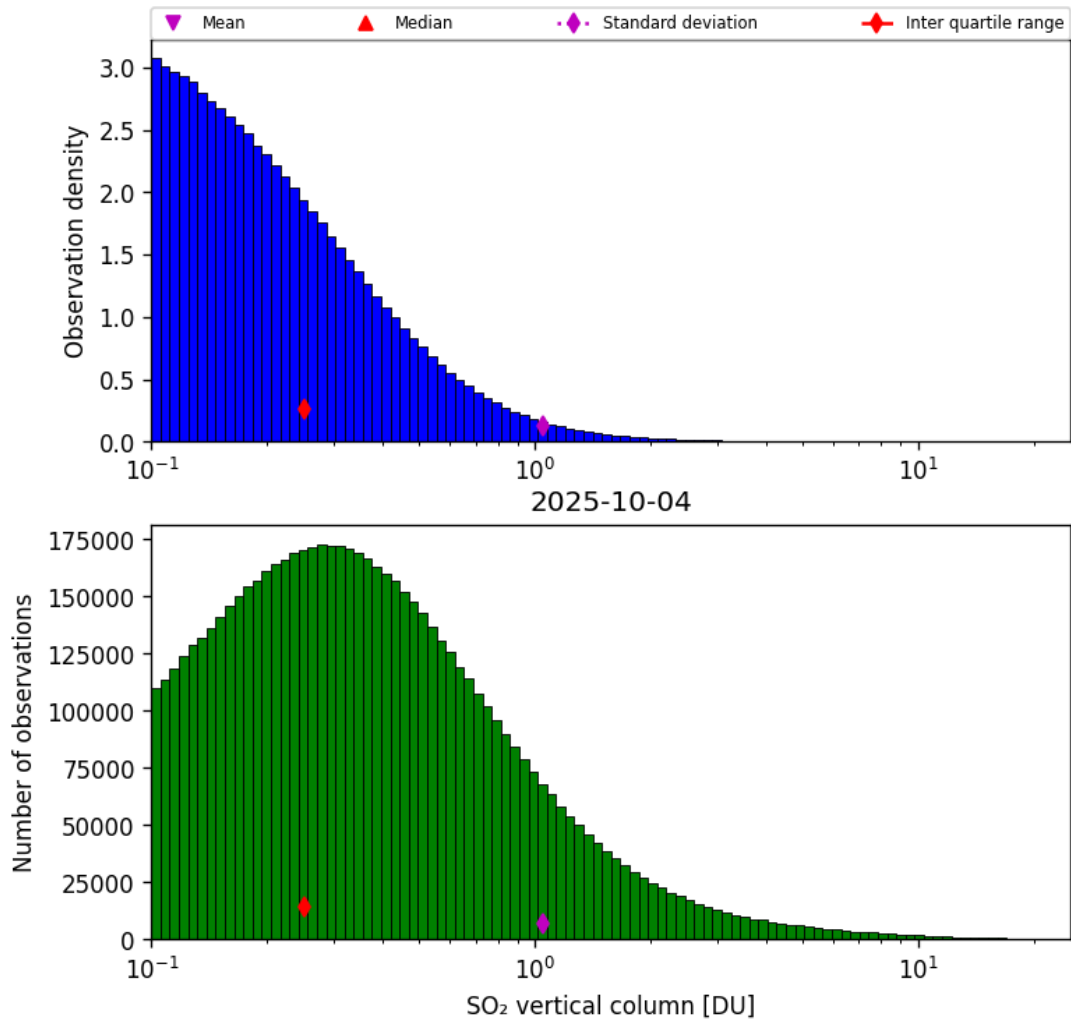
Figure 58: Histogram of “SO 2 vertical column” for 2025-10-04 to 2025-10-04
