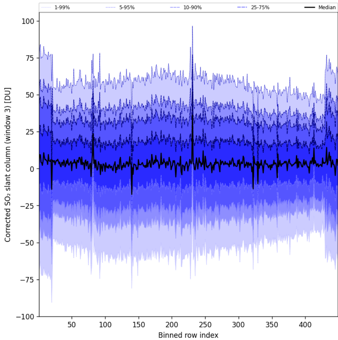
Figure 100: Along track statistics of “Corrected SO 2 slant column (window 3)” for 2025-10-04 to 2025-10-04
