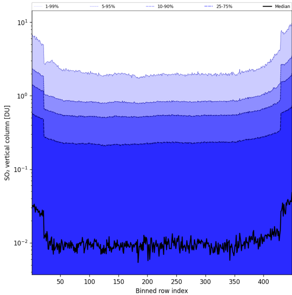
Figure 85: Along track statistics of “SO 2 vertical column” for 2025-10-04 to 2025-10-04
