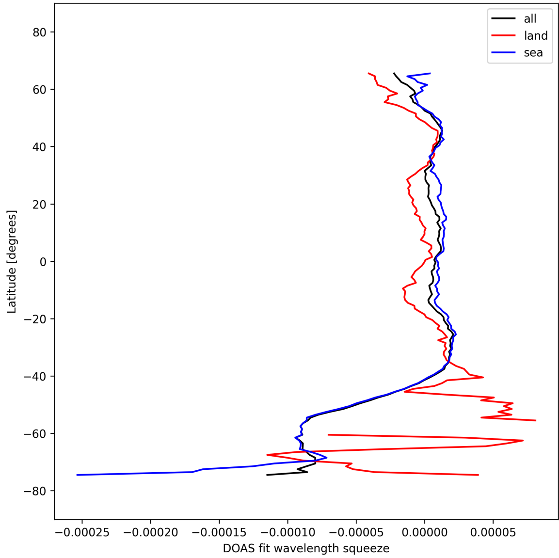
Figure 51: Zonal average of “DOAS fit wavelength squeeze” for 2025-10-04 to 2025-10-04.
