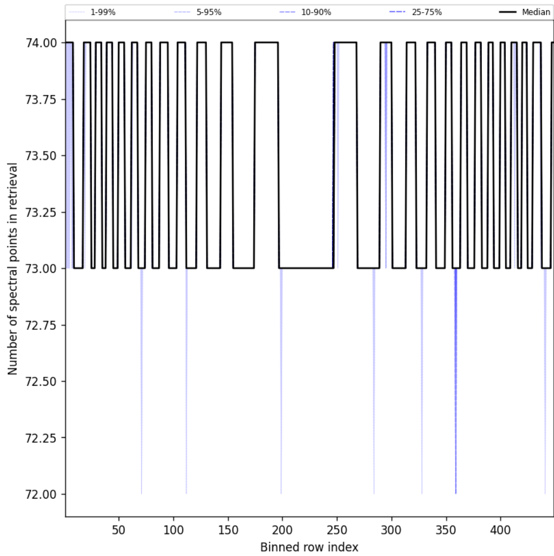
Figure 110: Along track statistics of “Number of spectral points in retrieval” for 2025-10-04 to 2025-10-04
