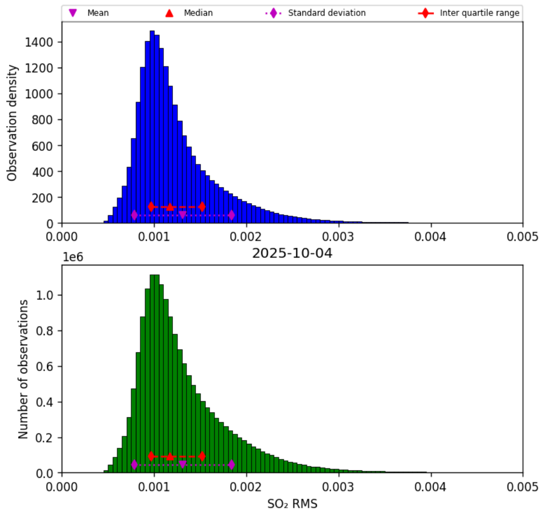
Figure 79: Histogram of “SO 2 RMS” for 2025-10-04 to 2025-10-04
