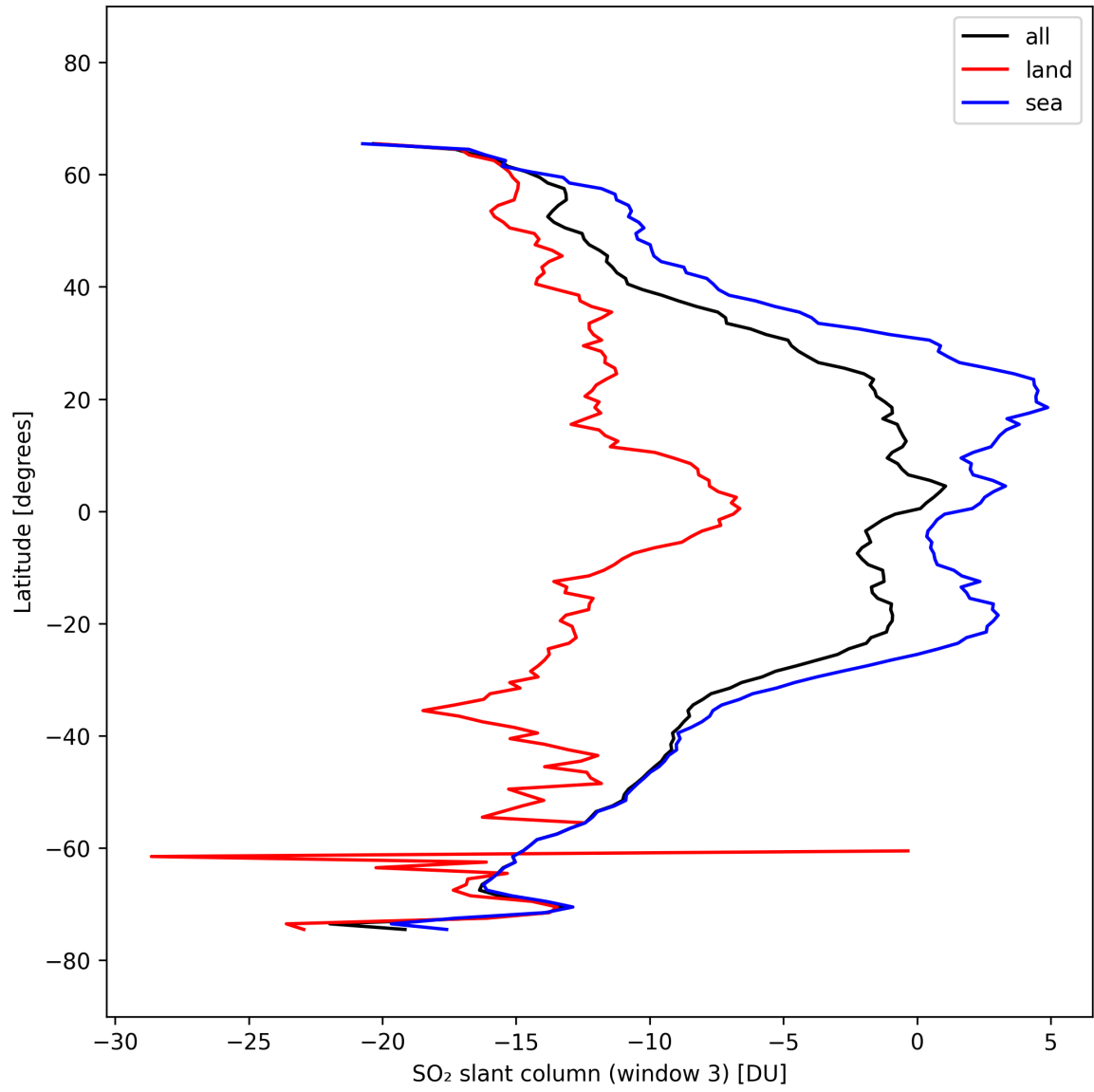
Figure 44: Zonal average of “SO 2 slant column (window 3)” for 2025-10-04 to 2025-10-04.
