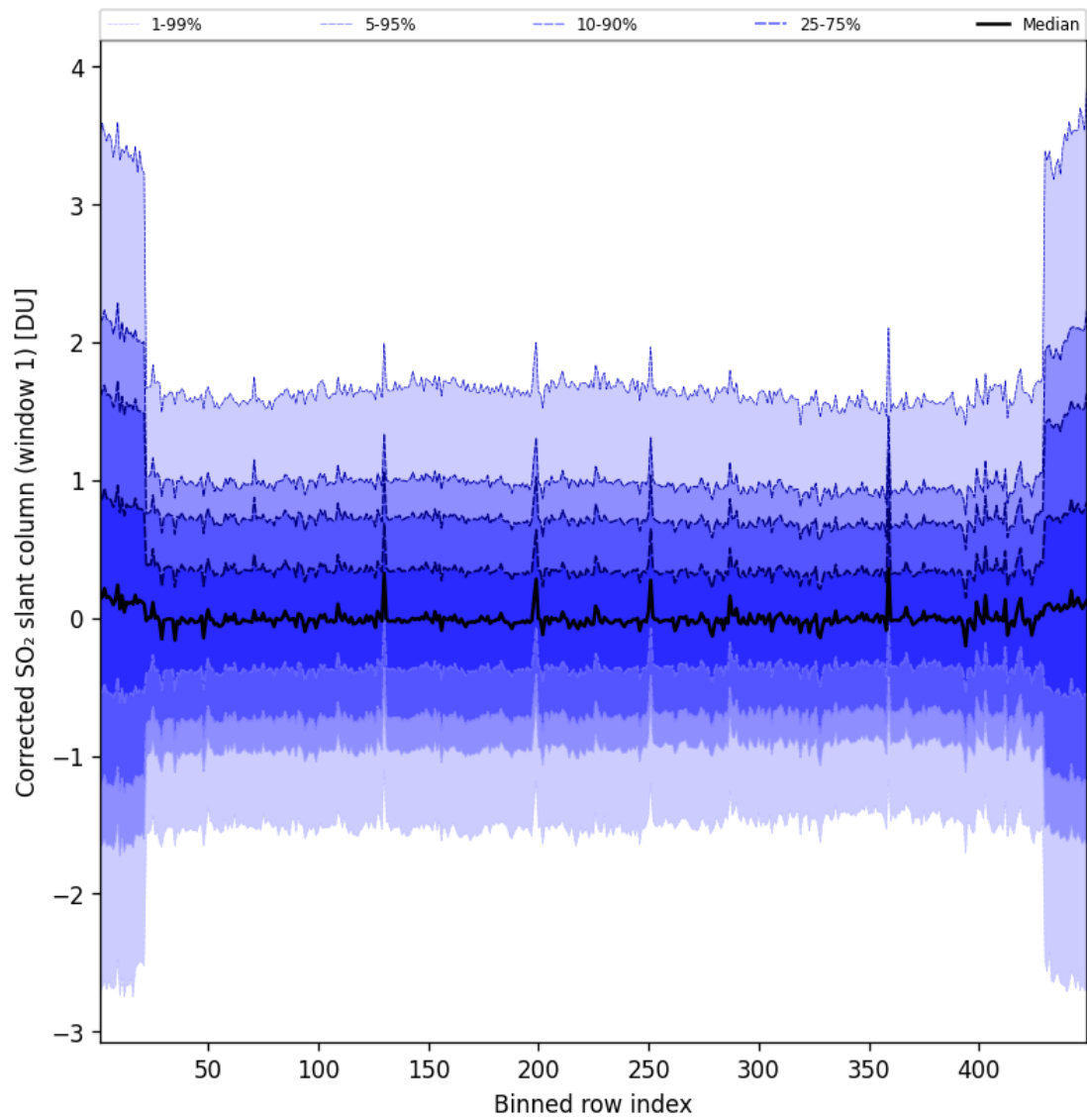
Figure 92: Along track statistics of “Corrected SO 2 slant column (window 1)” for 2025-10-04 to 2025-10-04
