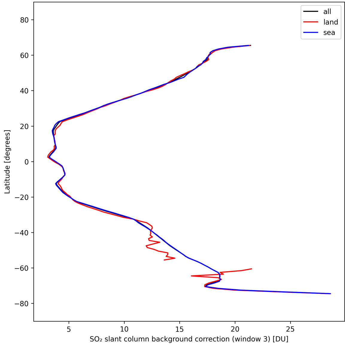
Figure 47: Zonal average of “SO 2 slant column background correction (window 3)” for 2025-10-04 to 2025-10-04.
