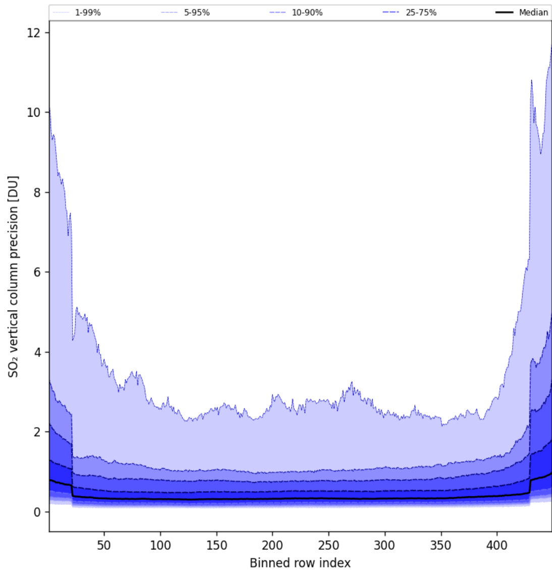
Figure 86: Along track statistics of “SO 2 vertical column precision” for 2025-10-04 to 2025-10-04
