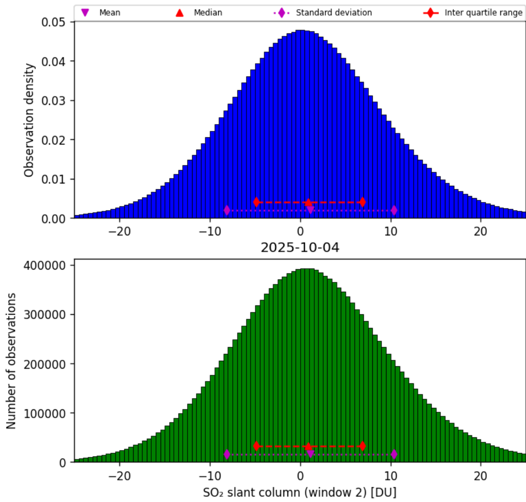
Figure 67: Histogram of “SO 2 slant column (window 2)” for 2025-10-04 to 2025-10-04
