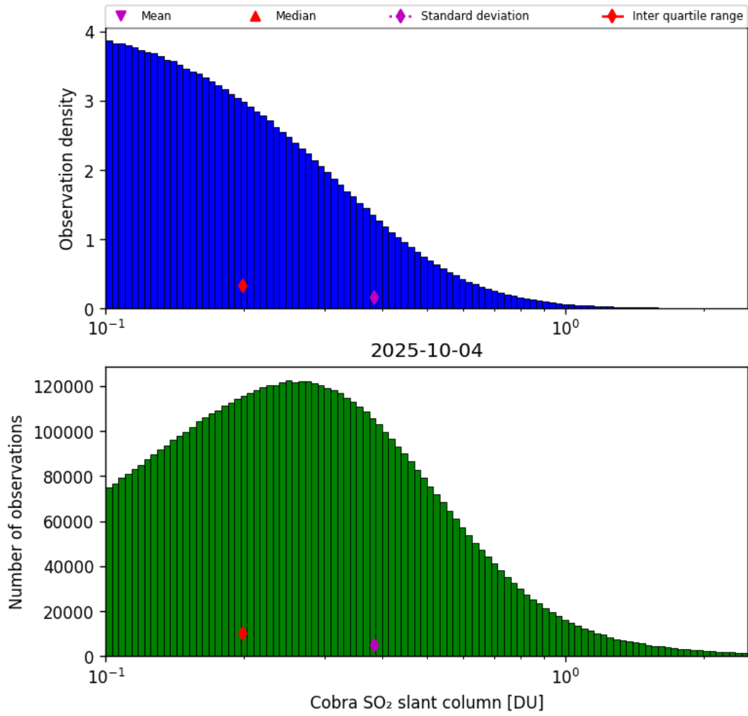
Figure 61: Histogram of “Cobra SO 2 slant column” for 2025-10-04 to 2025-10-04
