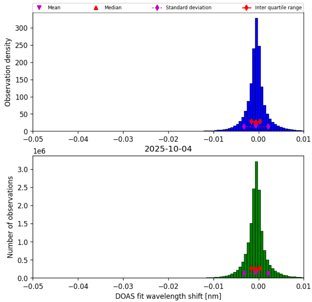
Figure 77: Histogram of “DOAS fit wavelength shift” for 2025-10-04 to 2025-10-04
