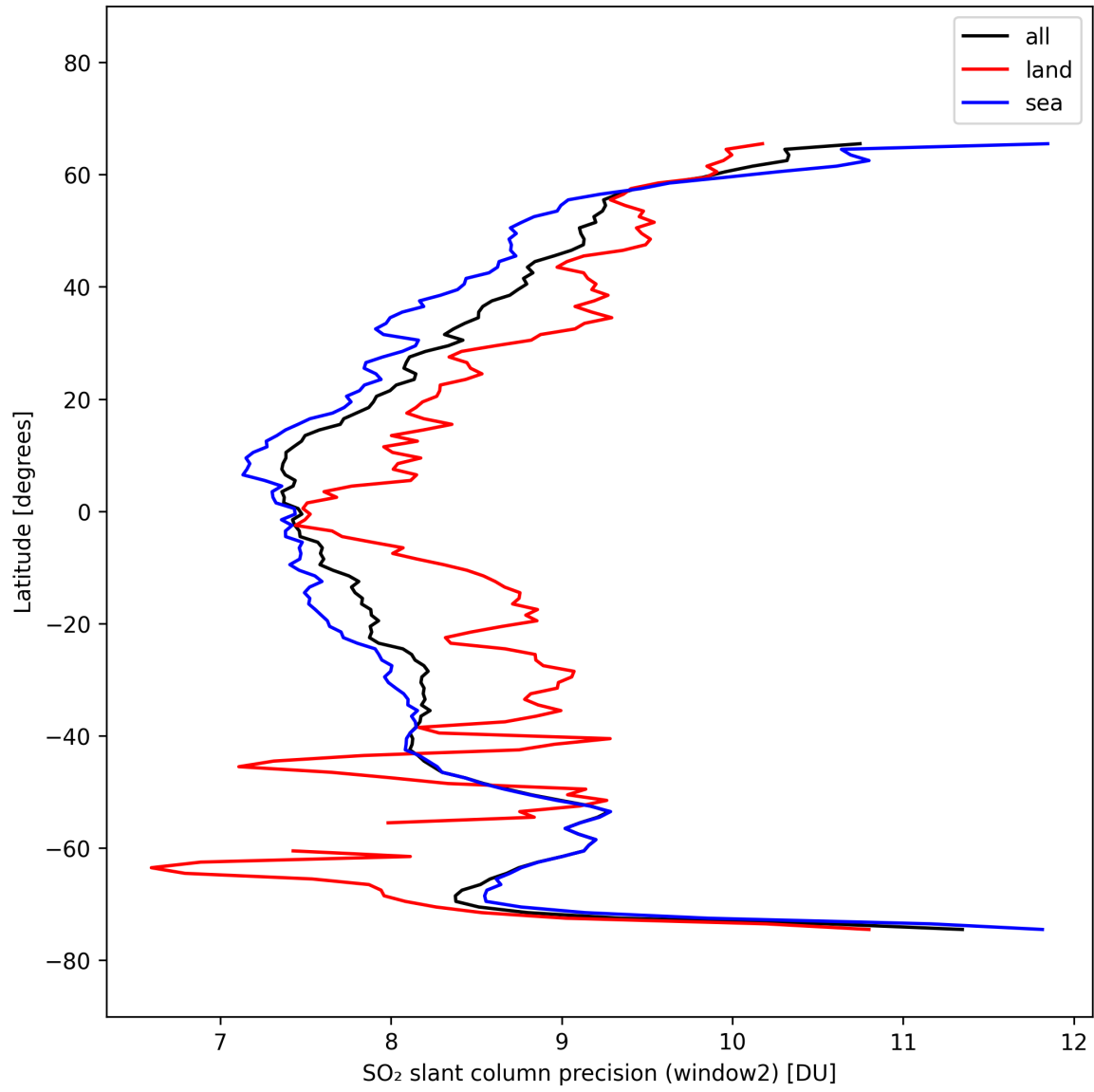
Figure 41: Zonal average of “SO 2 slant column precision (window2)” for 2025-10-04 to 2025-10-04.
