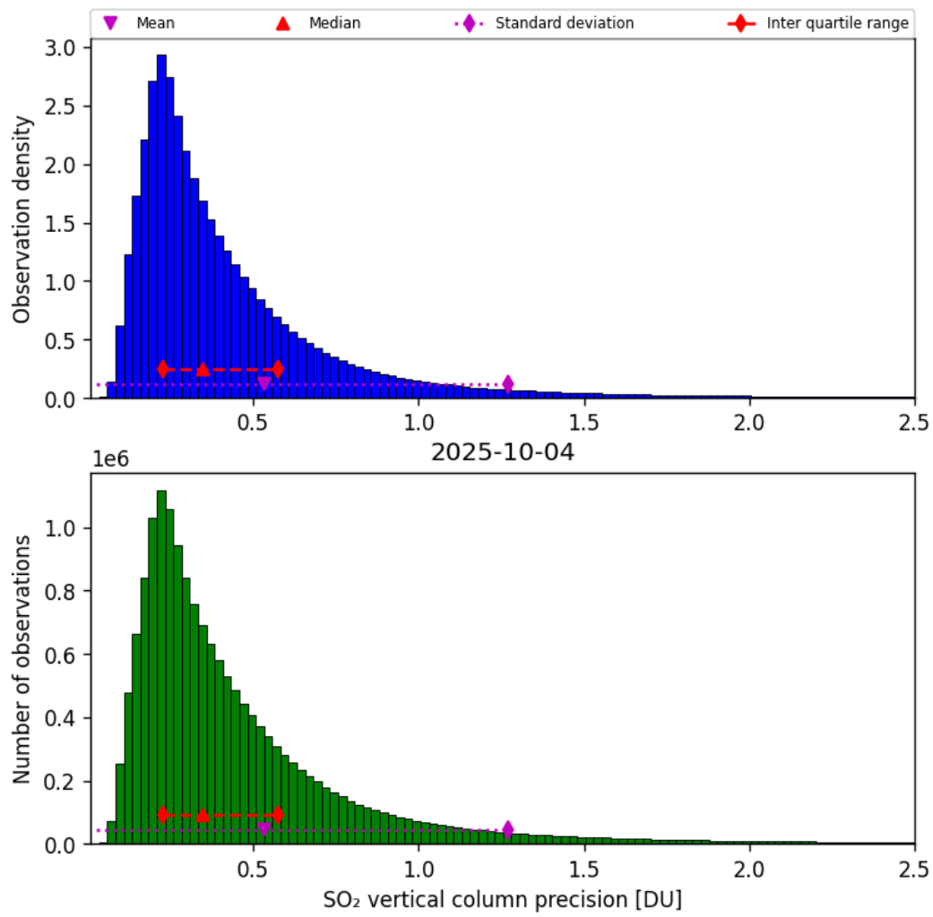
Figure 59: Histogram of “SO 2 vertical column precision” for 2025-10-04 to 2025-10-04
