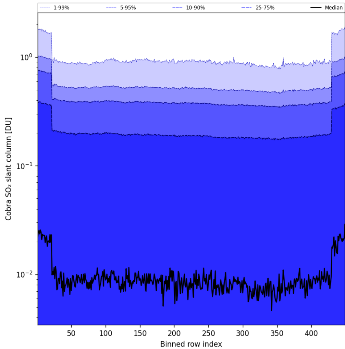
Figure 88: Along track statistics of “Cobra SO 2 slant column” for 2025-10-04 to 2025-10-04
