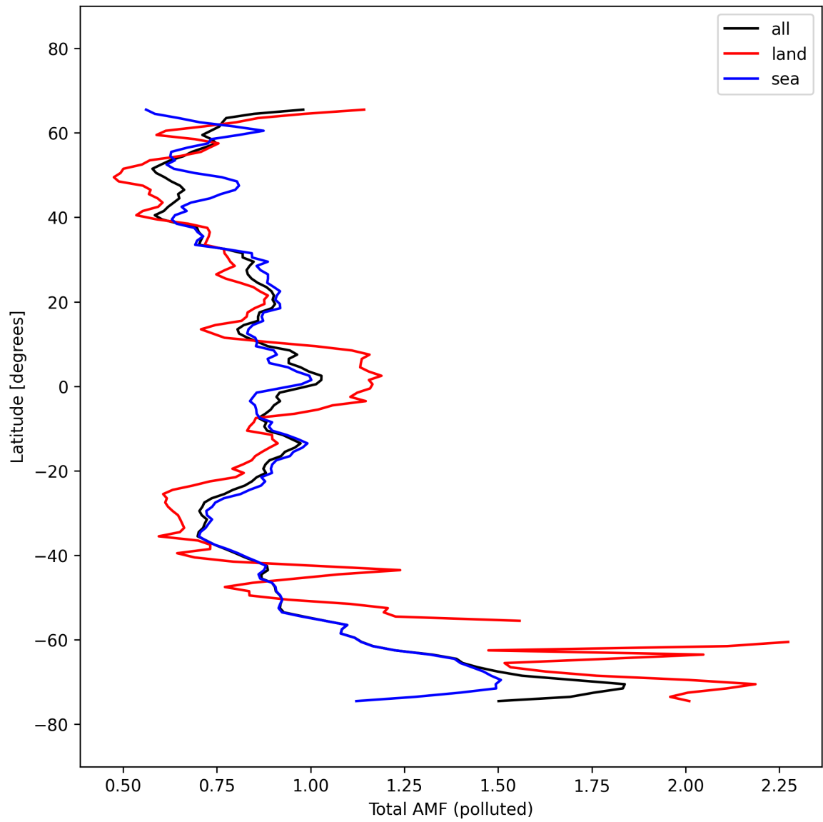
Figure 53: Zonal average of “Total AMF (polluted)” for 2025-10-04 to 2025-10-04.
