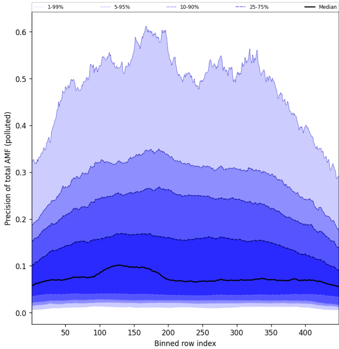
Figure 108: Along track statistics of “Precision of total AMF (polluted)” for 2025-10-04 to 2025-10-04
