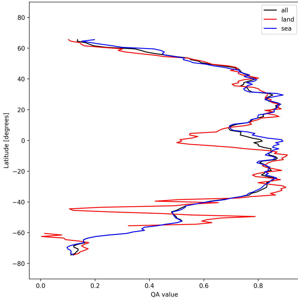
Figure 30: Zonal average of “QA value” for 2025-10-04 to 2025-10-04.
