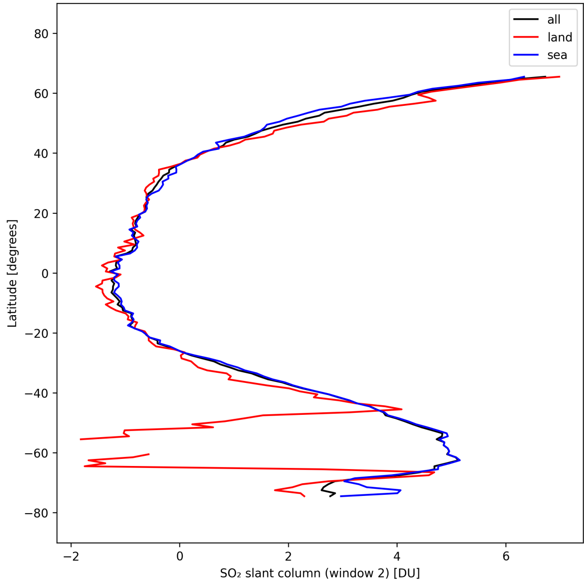
Figure 40: Zonal average of “SO 2 slant column (window 2)” for 2025-10-04 to 2025-10-04.
