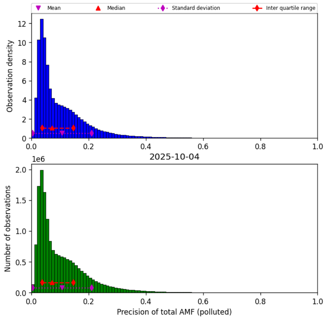
Figure 81: Histogram of “Precision of total AMF (polluted)” for 2025-10-04 to 2025-10-04
