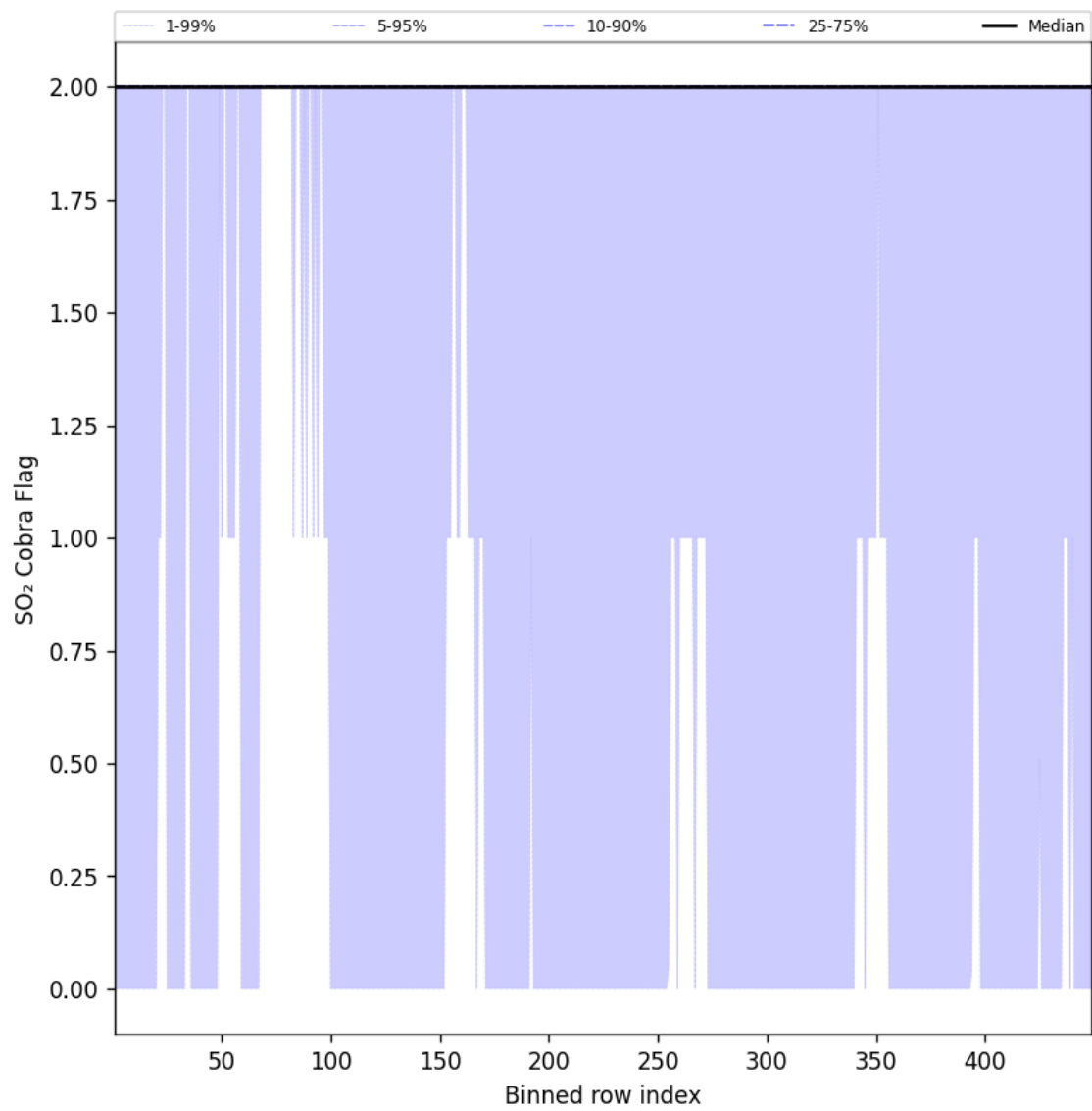
Figure 102: Along track statistics of “SO 2 Cobra Flag” for 2025-10-04 to 2025-10-04
