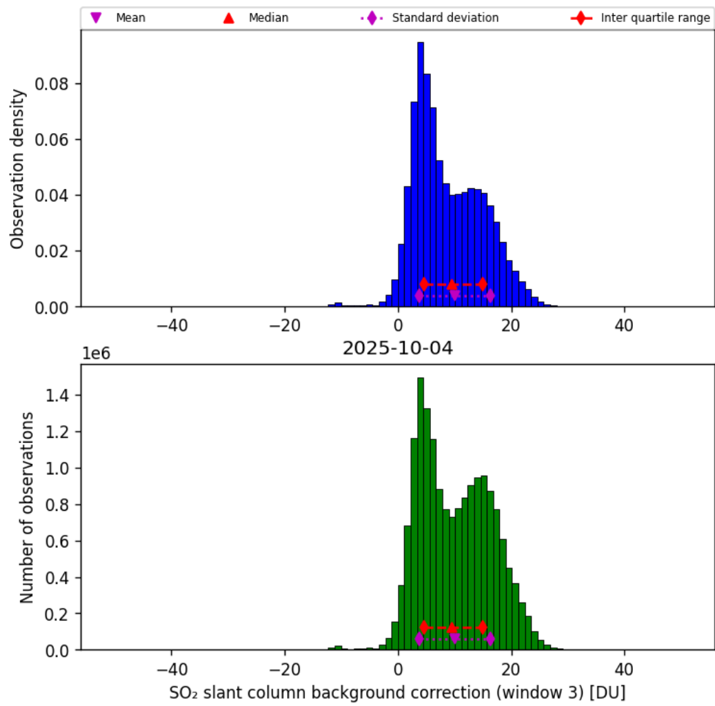
Figure 74: Histogram of “SO 2 slant column background correction (window 3)” for 2025-10-04 to 2025-10-04
