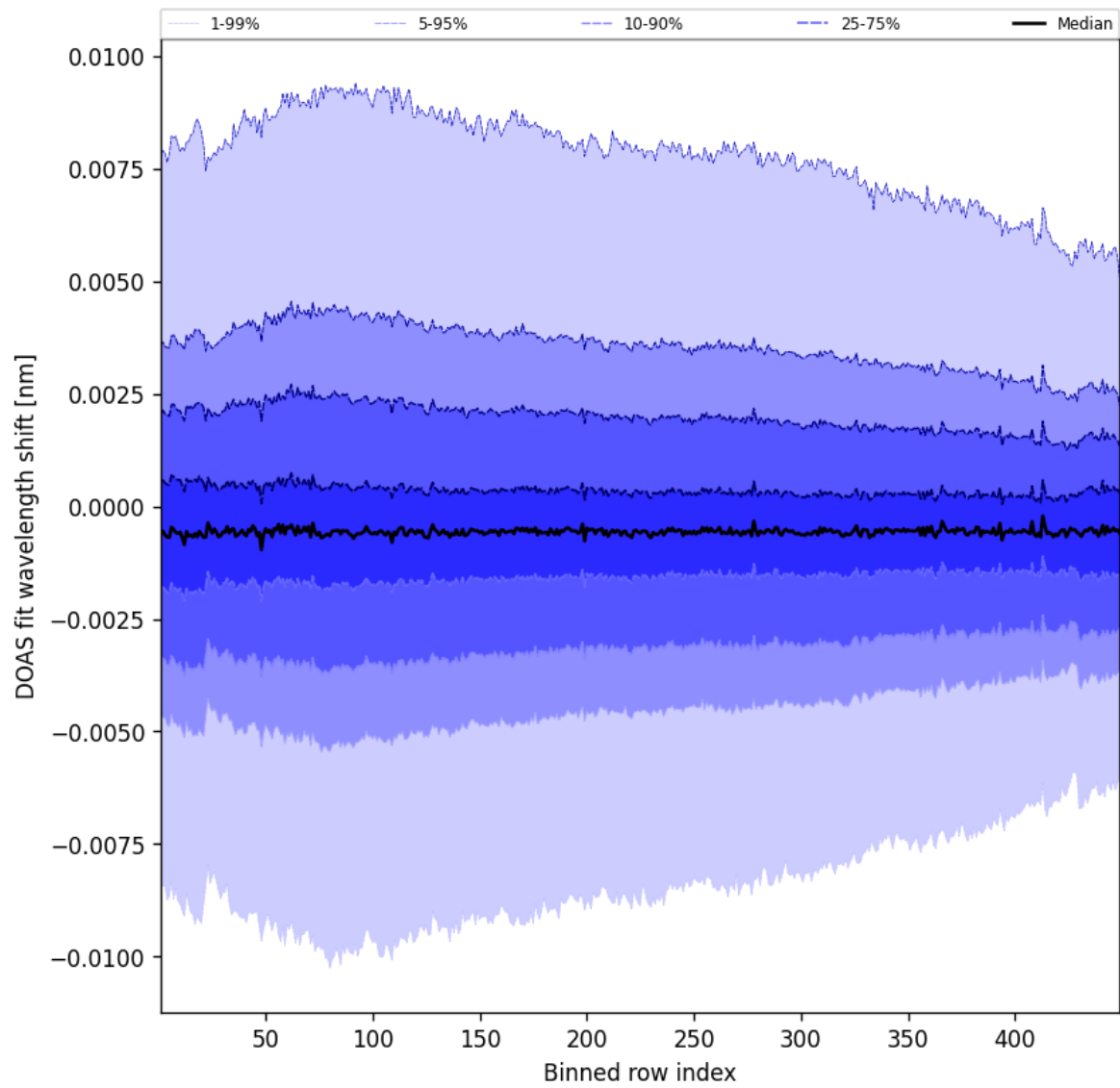
Figure 104: Along track statistics of “DOAS fit wavelength shift” for 2025-10-04 to 2025-10-04
