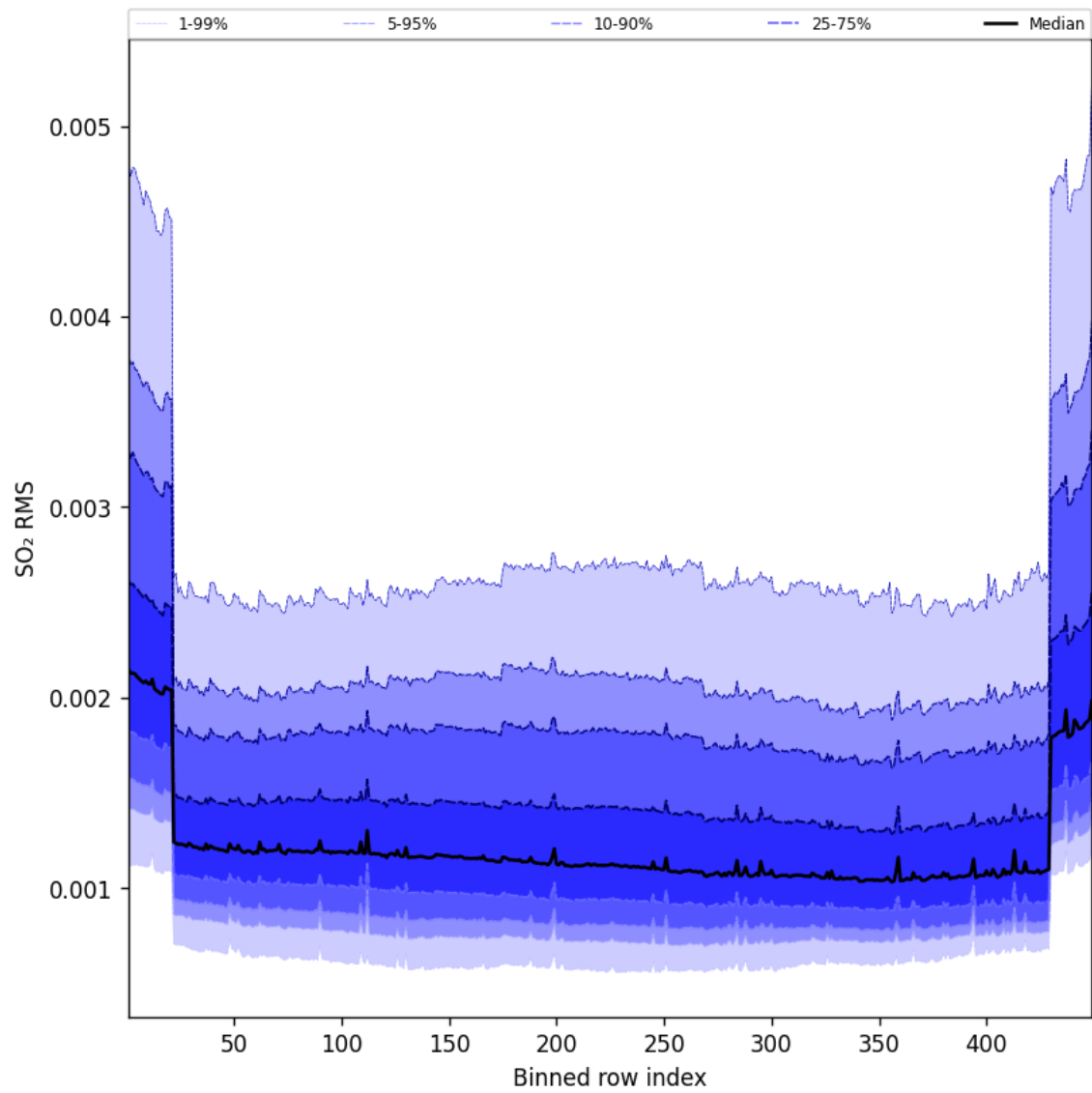
Figure 106: Along track statistics of “SO 2 RMS” for 2025-10-04 to 2025-10-04
