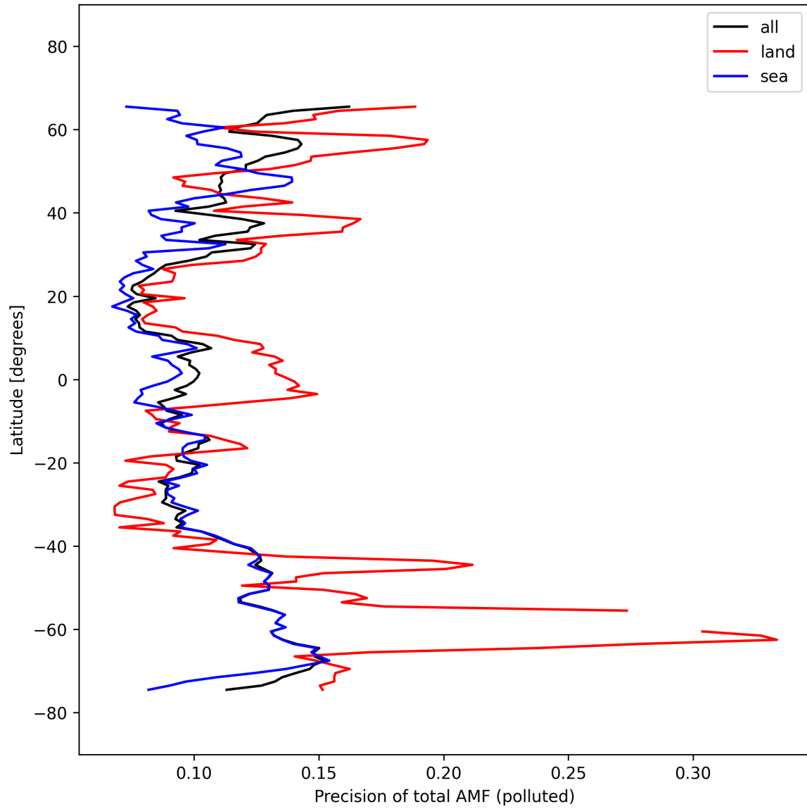
Figure 54: Zonal average of “Precision of total AMF (polluted)” for 2025-10-04 to 2025-10-04.
