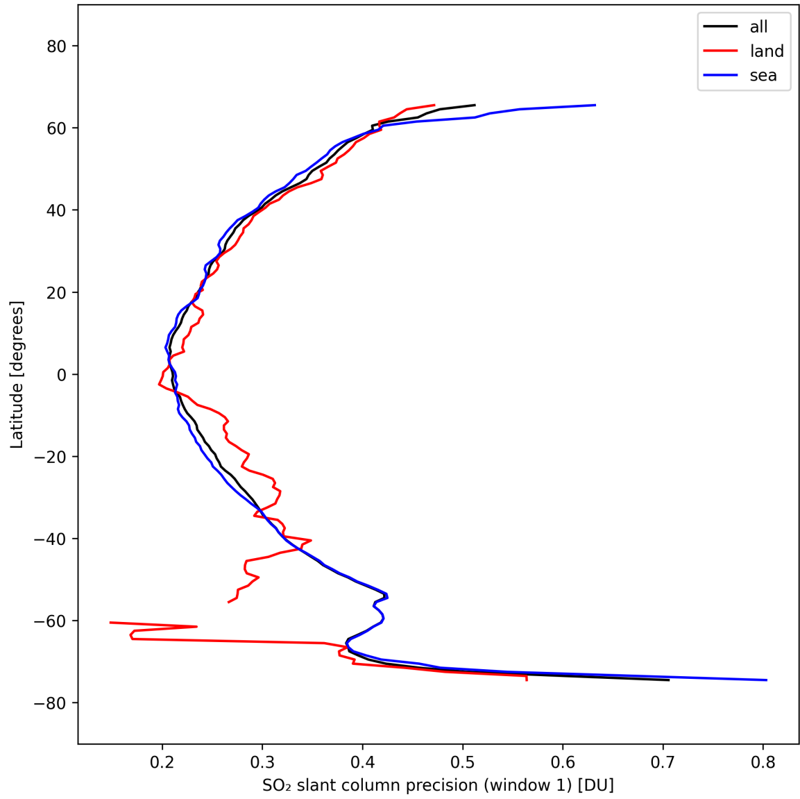
Figure 37: Zonal average of “SO 2 slant column precision (window 1)” for 2025-10-04 to 2025-10-04.
