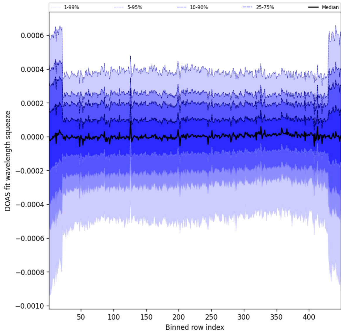
Figure 105: Along track statistics of “DOAS fit wavelength squeeze” for 2025-10-04 to 2025-10-04
