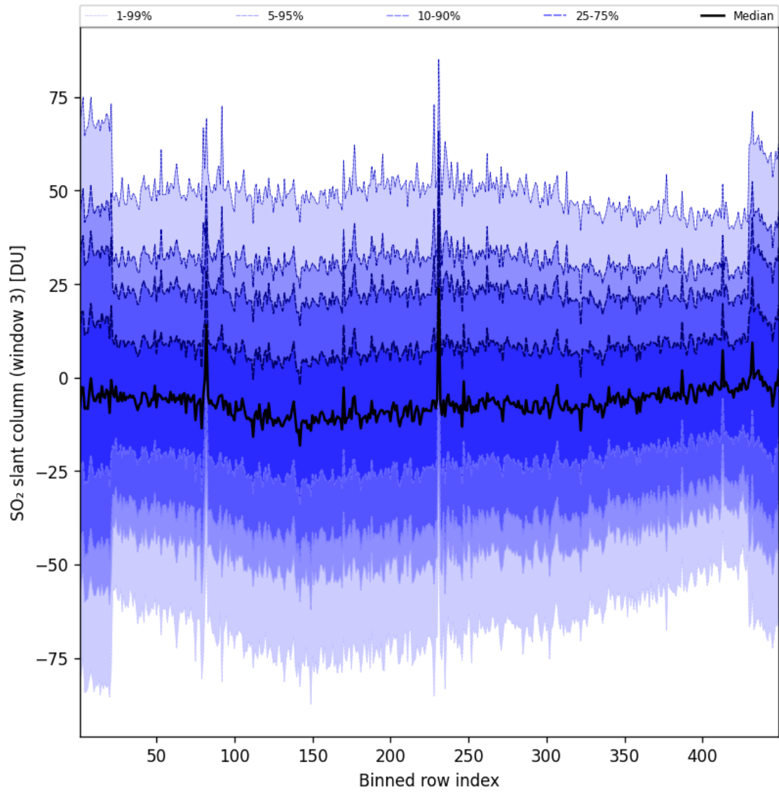
Figure 98: Along track statistics of “SO 2 slant column (window 3)” for 2025-10-04 to 2025-10-04
