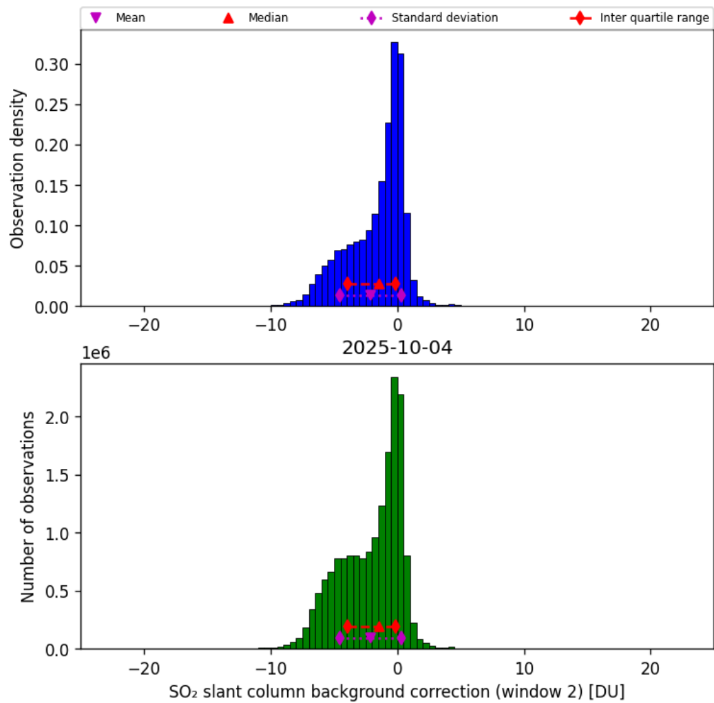
Figure 70: Histogram of “SO 2 slant column background correction (window 2)” for 2025-10-04 to 2025-10-04
