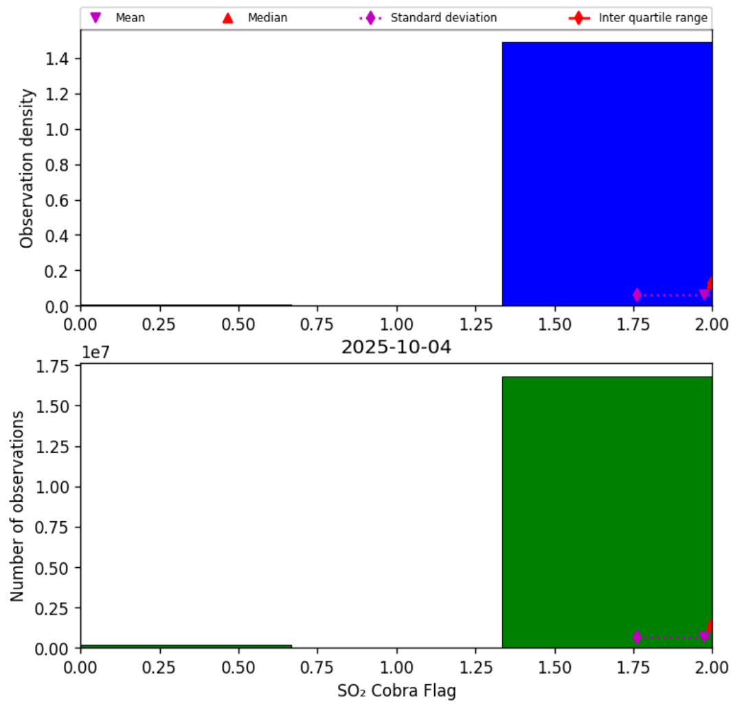
Figure 75: Histogram of “SO 2 Cobra Flag” for 2025-10-04 to 2025-10-04
