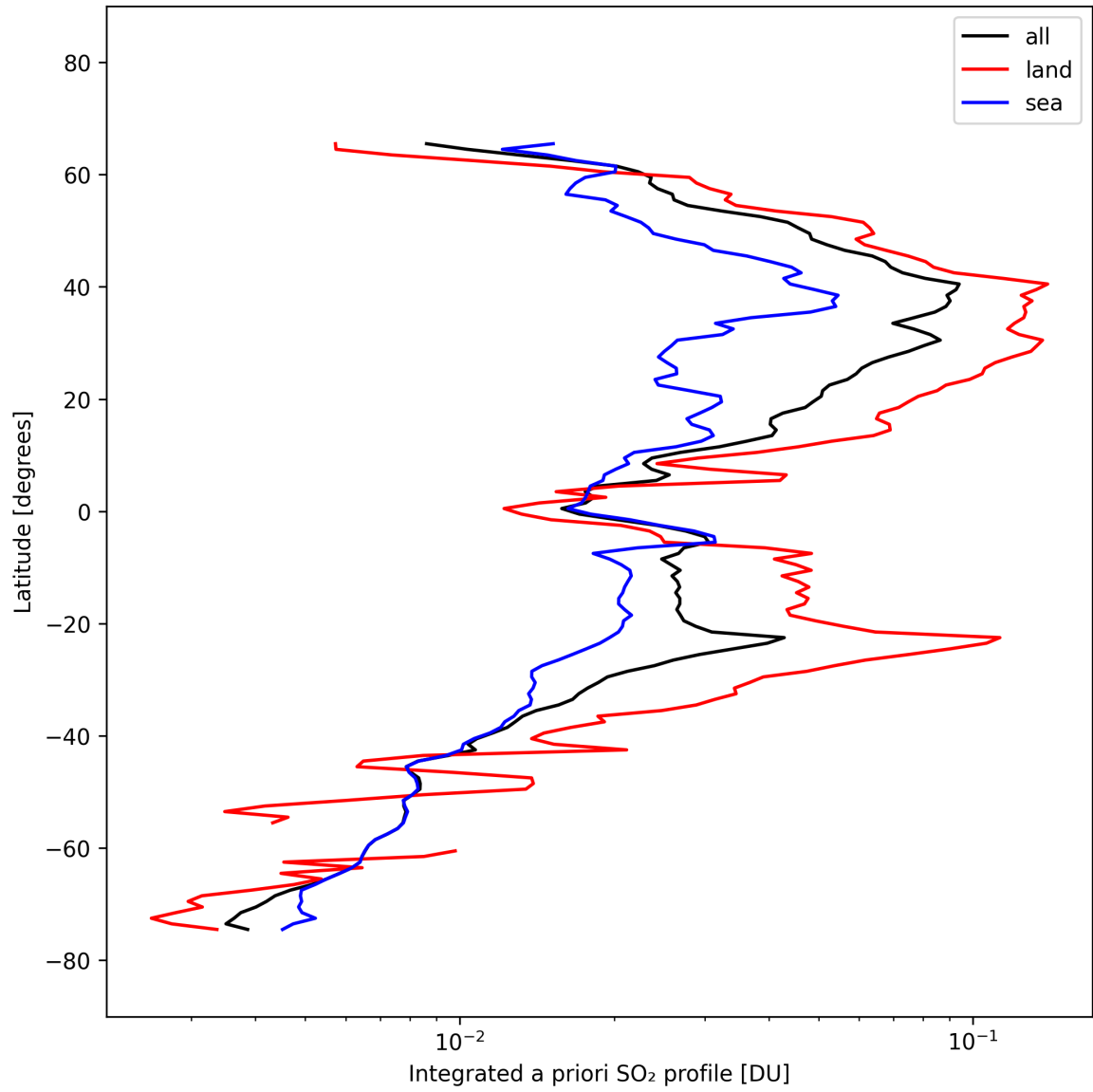
Figure 49: Zonal average of “Integrated a priori SO 2 profile” for 2025-10-04 to 2025-10-04.
