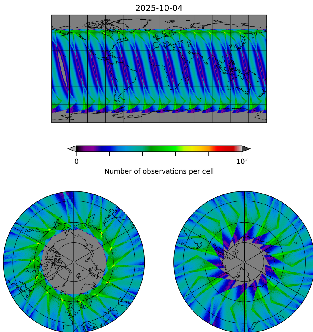
Figure 29: Map of the number of observations for 2025-10-04 to 2025-10-04
