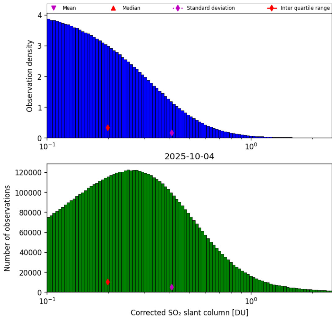
Figure 60: Histogram of “Corrected SO 2 slant column” for 2025-10-04 to 2025-10-04
