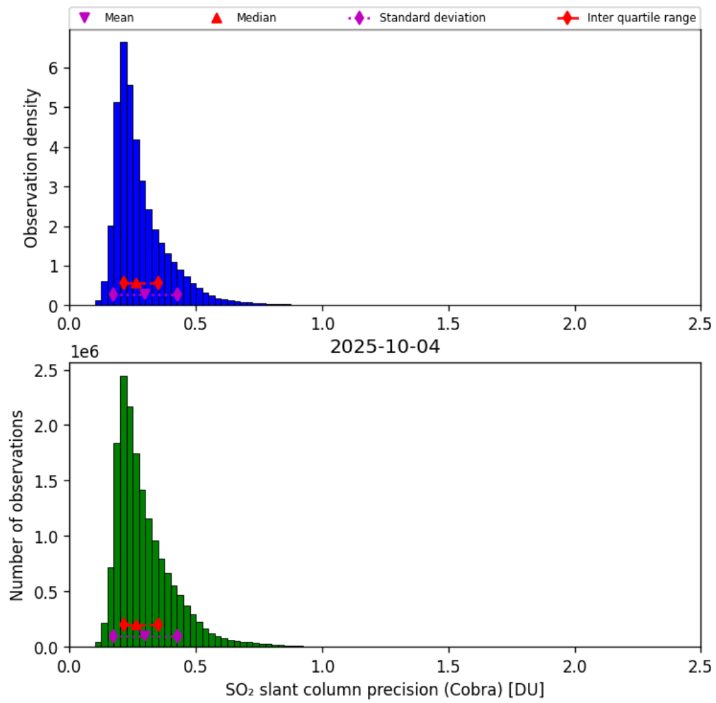
Figure 62: Histogram of “SO 2 slant column precision (Cobra)” for 2025-10-04 to 2025-10-04
