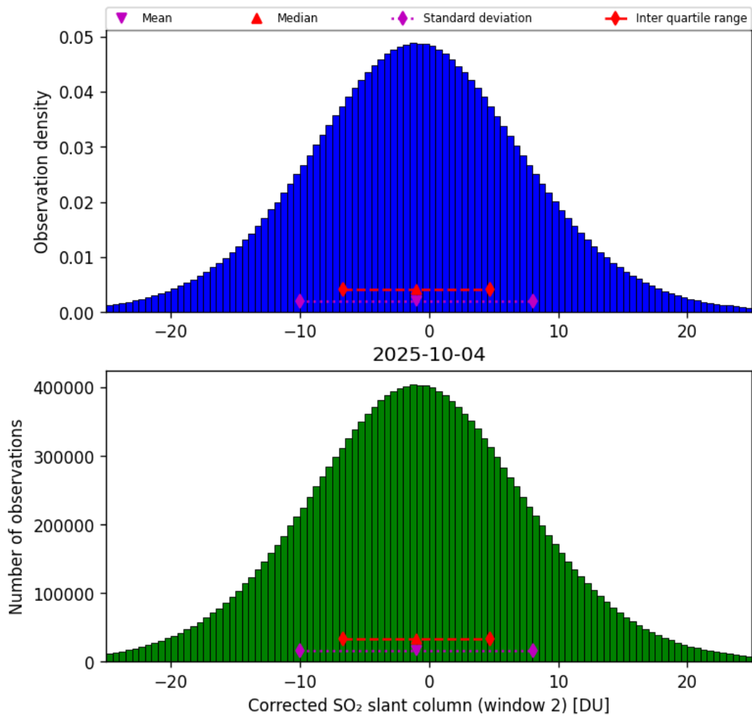
Figure 69: Histogram of “Corrected SO 2 slant column (window 2)” for 2025-10-04 to 2025-10-04
