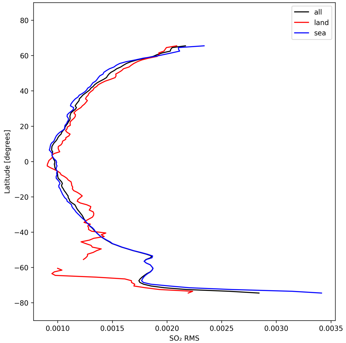
Figure 52: Zonal average of “SO 2 RMS” for 2025-10-04 to 2025-10-04.
