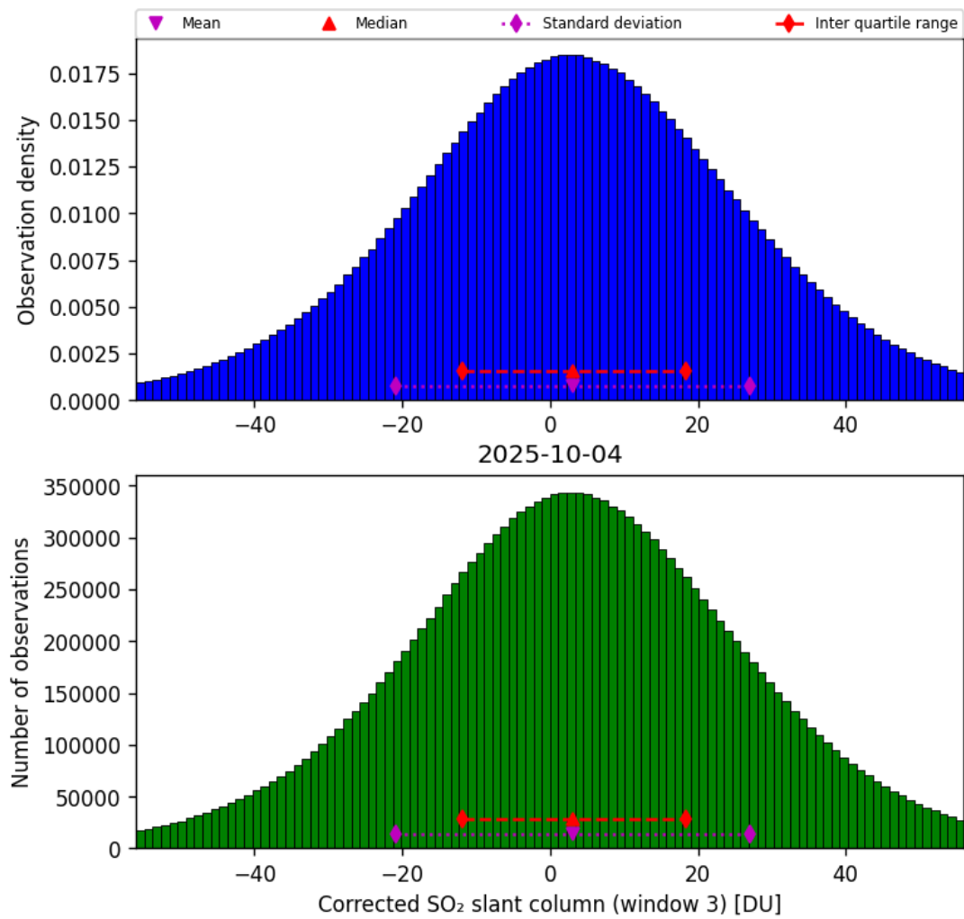
Figure 73: Histogram of “Corrected SO 2 slant column (window 3)” for 2025-10-04 to 2025-10-04
