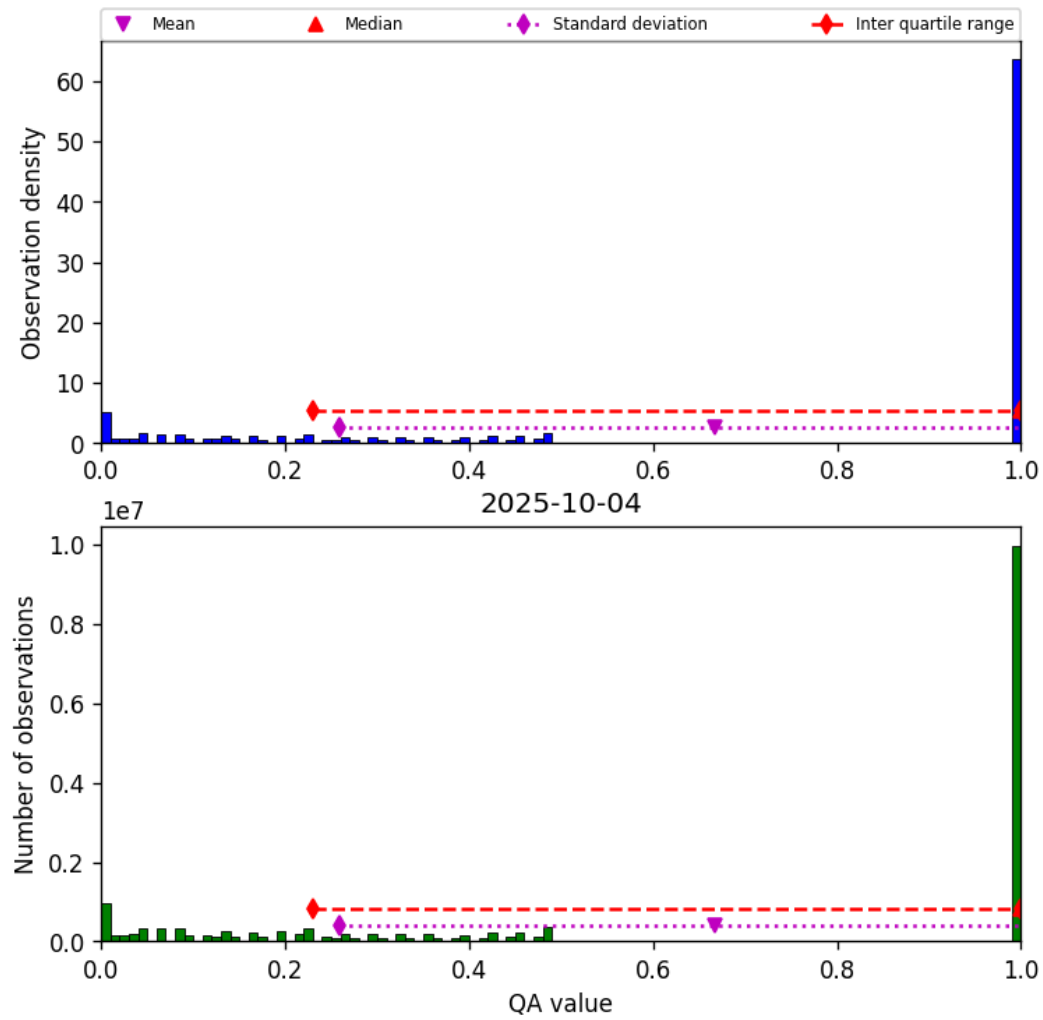
Figure 57: Histogram of “QA value” for 2025-10-04 to 2025-10-04
