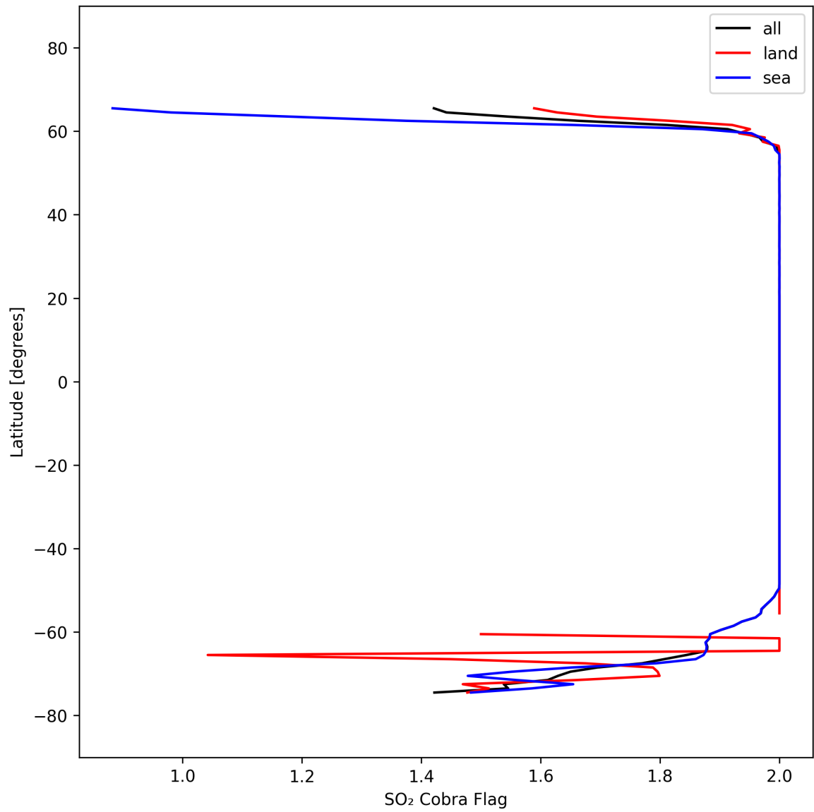
Figure 48: Zonal average of “SO 2 Cobra Flag” for 2025-10-04 to 2025-10-04.
