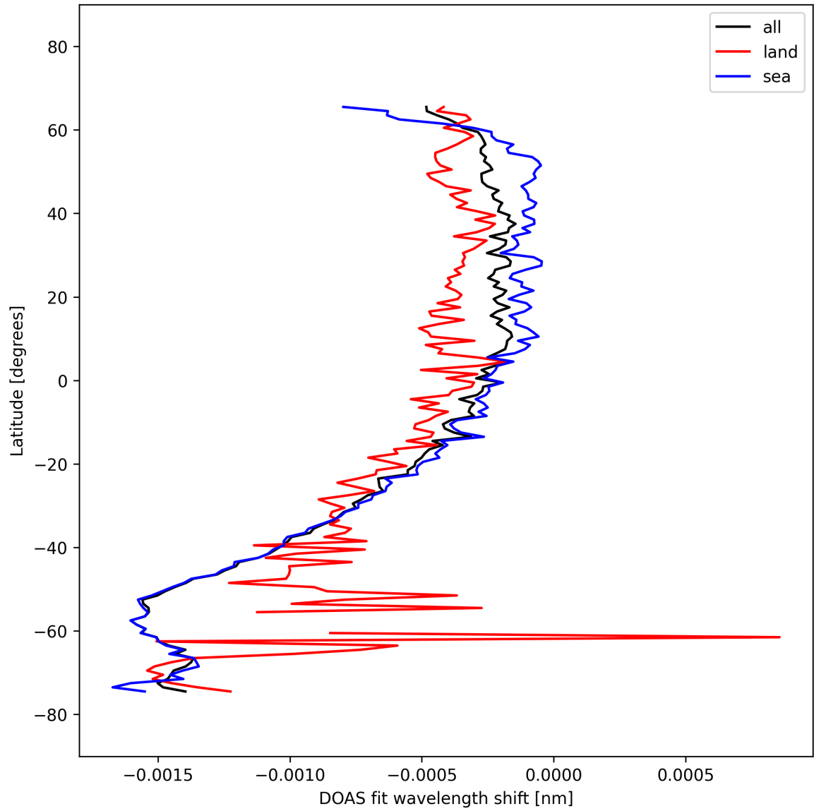
Figure 50: Zonal average of “DOAS fit wavelength shift” for 2025-10-04 to 2025-10-04.
