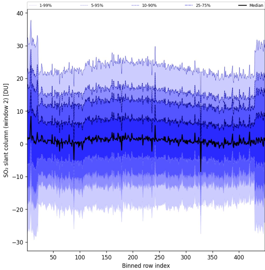
Figure 94: Along track statistics of “SO 2 slant column (window 2)” for 2025-10-04 to 2025-10-04
