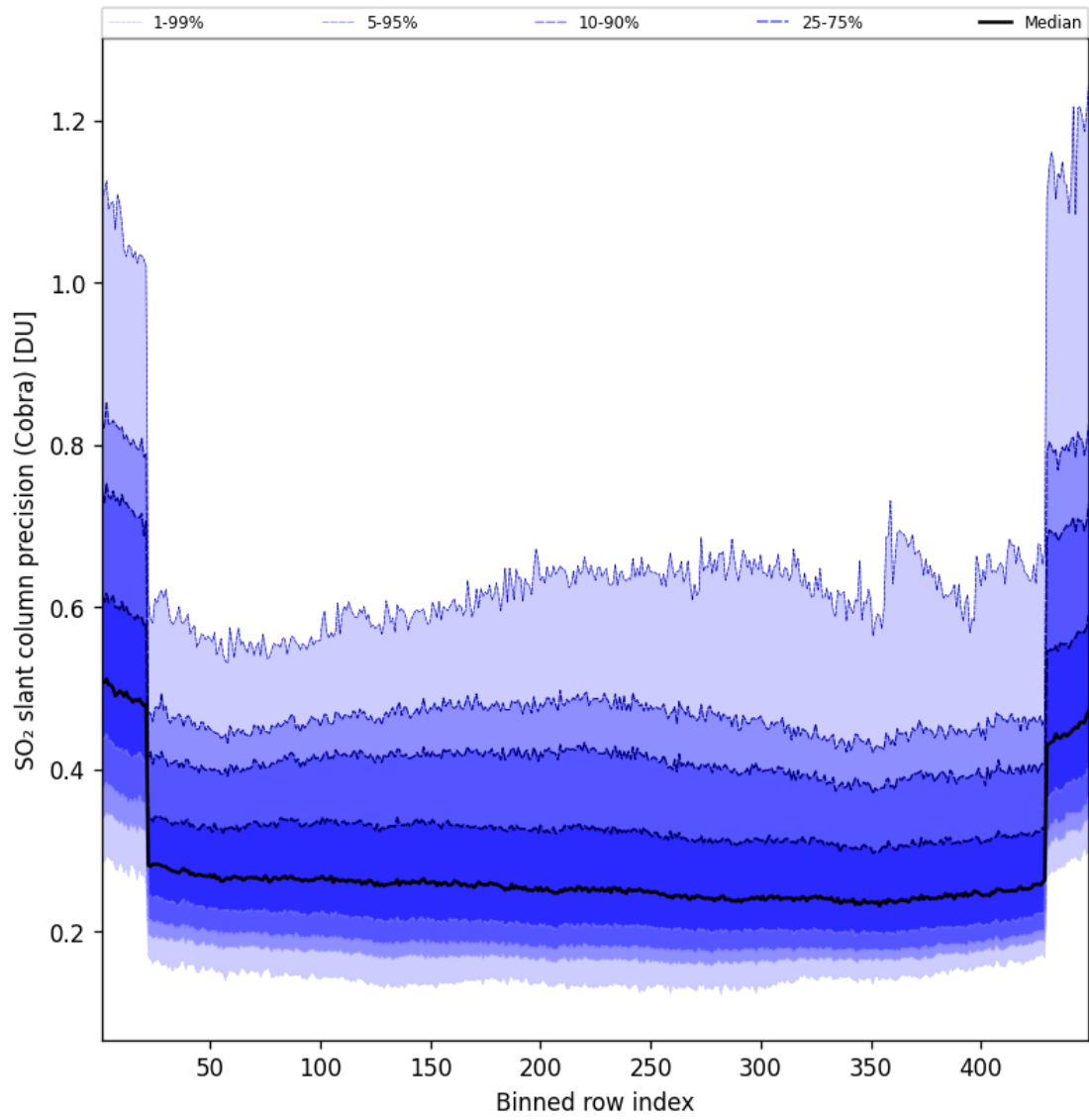
Figure 89: Along track statistics of “SO 2 slant column precision (Cobra)” for 2025-10-04 to 2025-10-04
