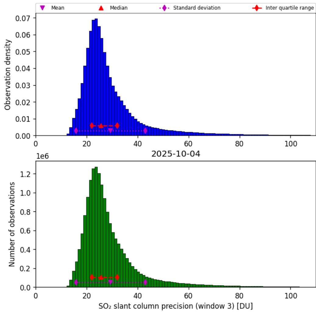
Figure 72: Histogram of “SO 2 slant column precision (window 3)” for 2025-10-04 to 2025-10-04
