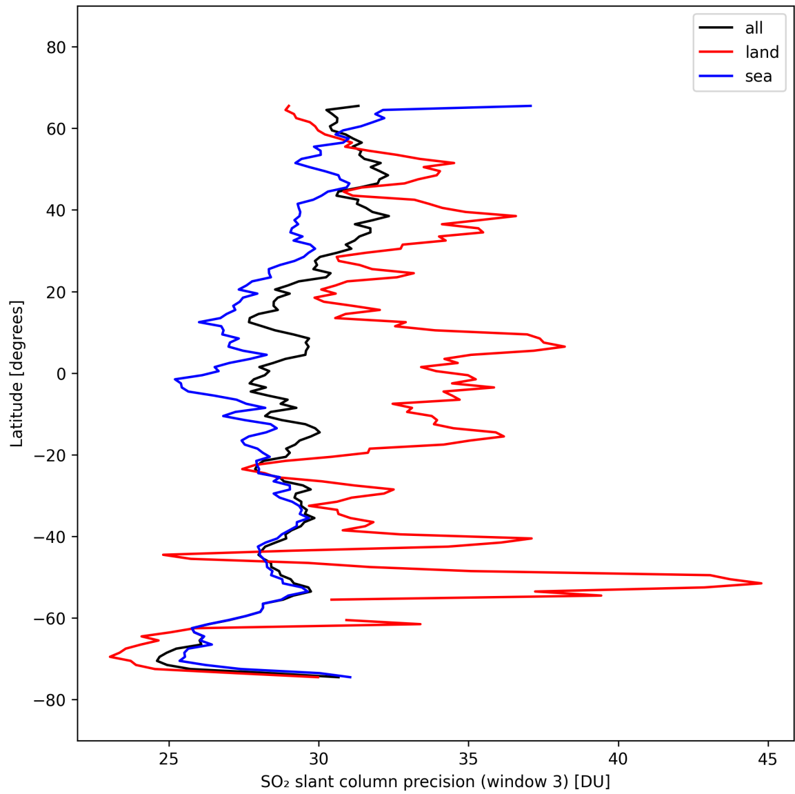
Figure 45: Zonal average of “SO 2 slant column precision (window 3)” for 2025-10-04 to 2025-10-04.
