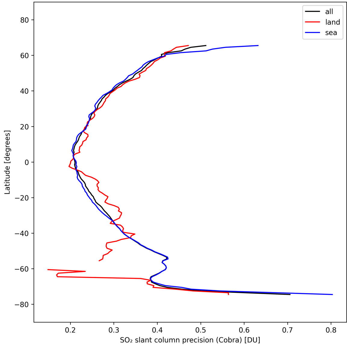
Figure 35: Zonal average of “SO 2 slant column precision (Cobra)” for 2025-10-04 to 2025-10-04.
