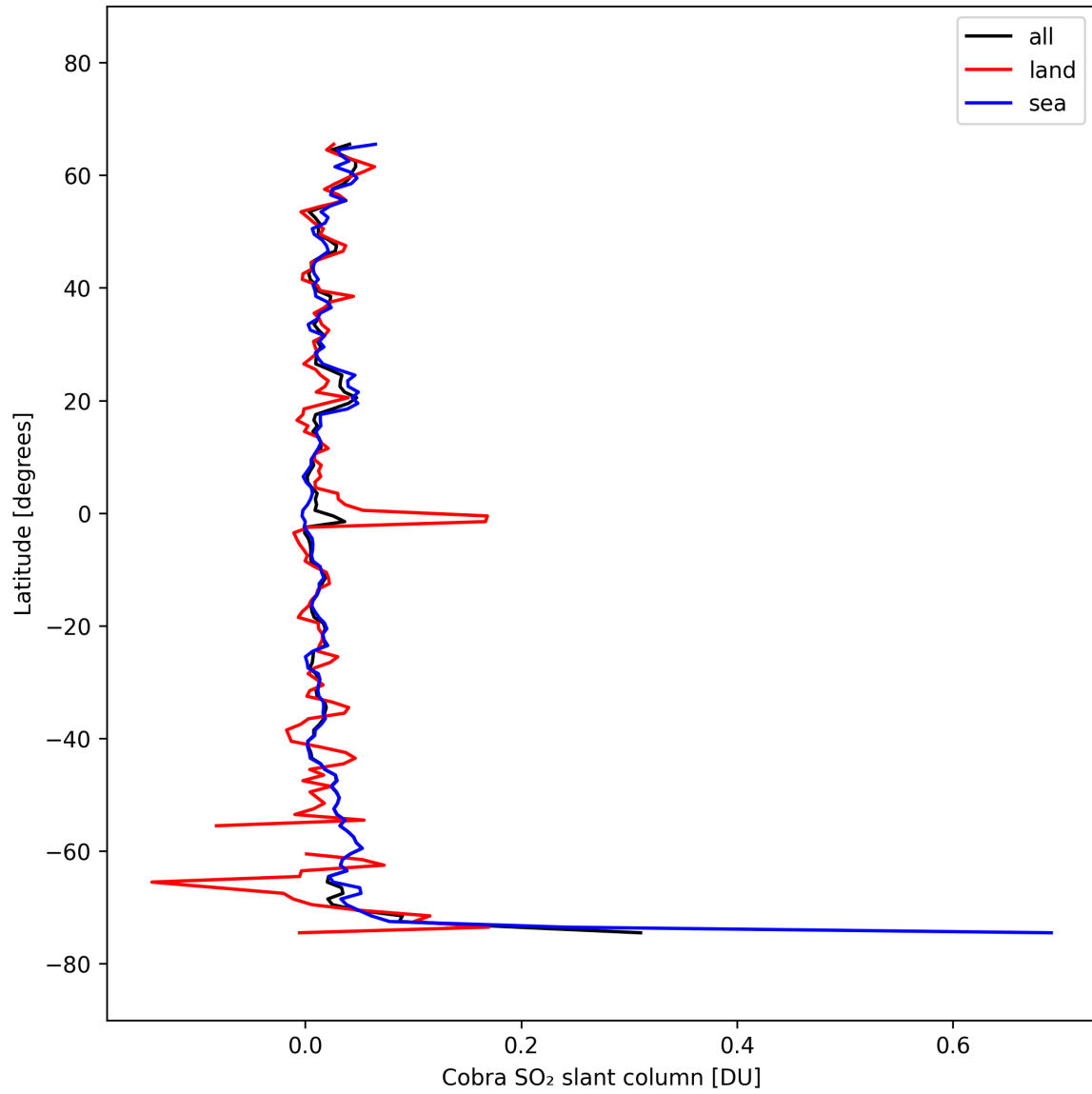
Figure 34: Zonal average of “Cobra SO 2 slant column” for 2025-10-04 to 2025-10-04.
