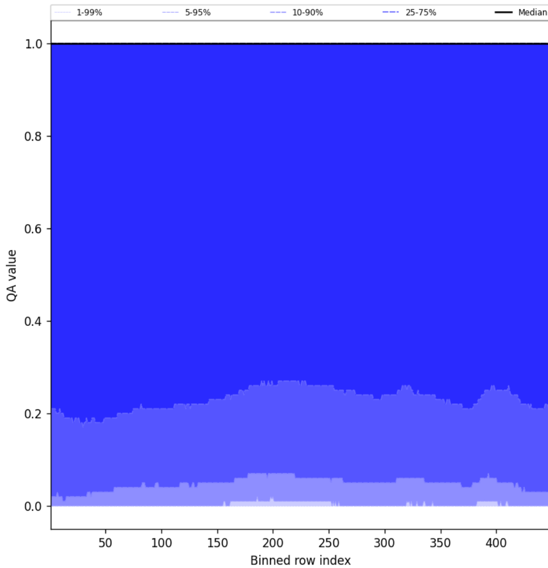
Figure 84: Along track statistics of “QA value” for 2025-10-04 to 2025-10-04
