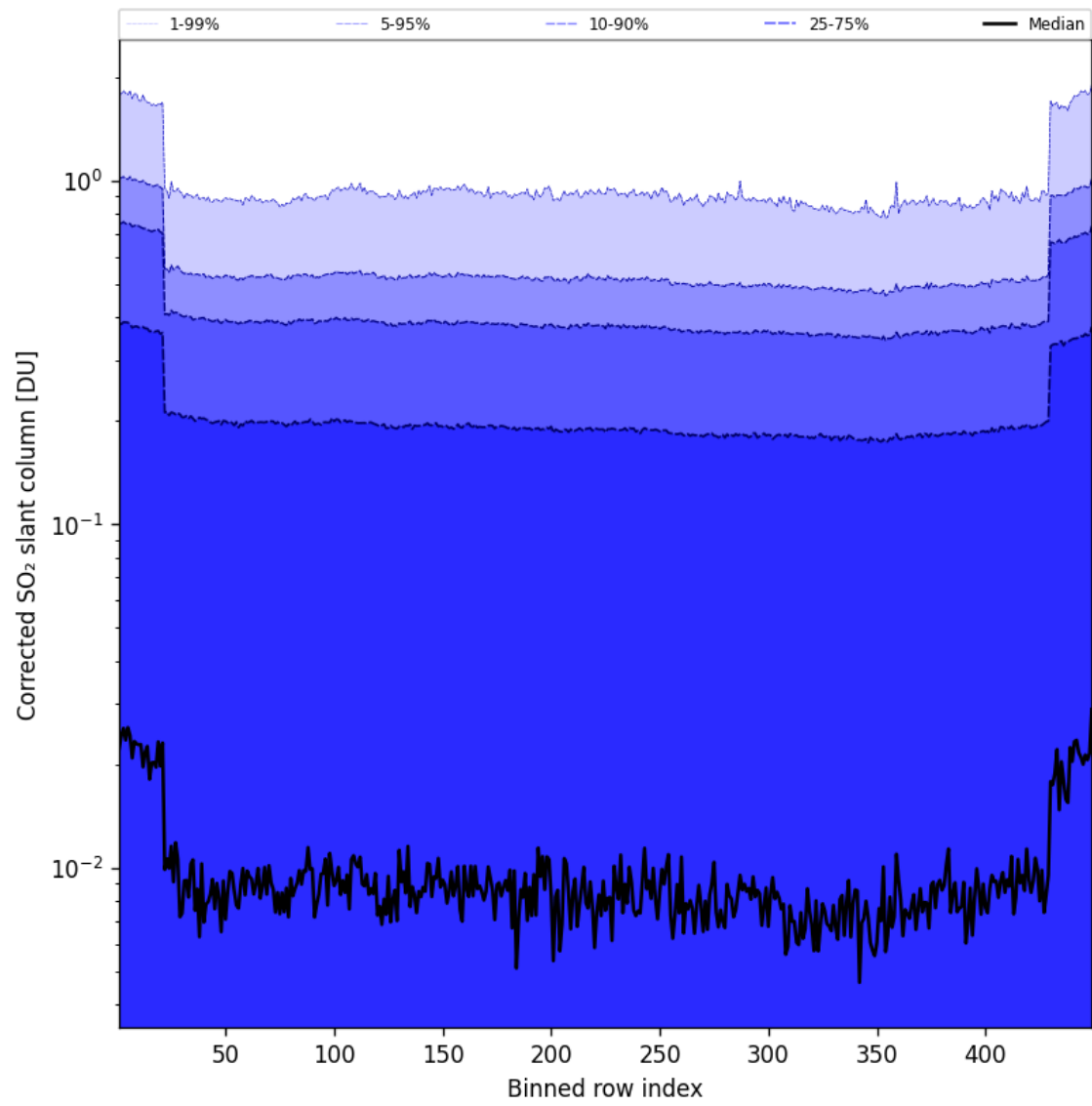
Figure 87: Along track statistics of “Corrected SO 2 slant column” for 2025-10-04 to 2025-10-04
