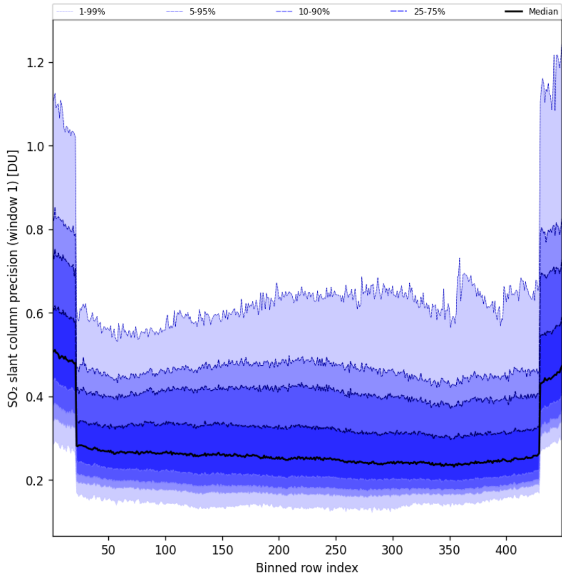
Figure 91: Along track statistics of “SO 2 slant column precision (window 1)” for 2025-10-04 to 2025-10-04
