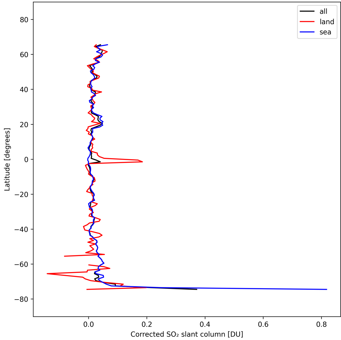
Figure 33: Zonal average of “Corrected SO 2 slant column” for 2025-10-04 to 2025-10-04.
