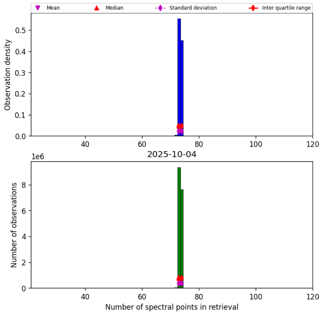
Figure 83: Histogram of “Number of spectral points in retrieval” for 2025-10-04 to 2025-10-04
