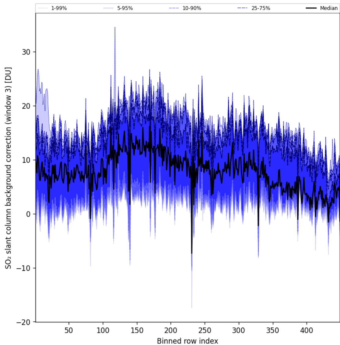
Figure 101: Along track statistics of “SO 2 slant column background correction (window 3)” for 2025-10-06 to 2025-10-07
