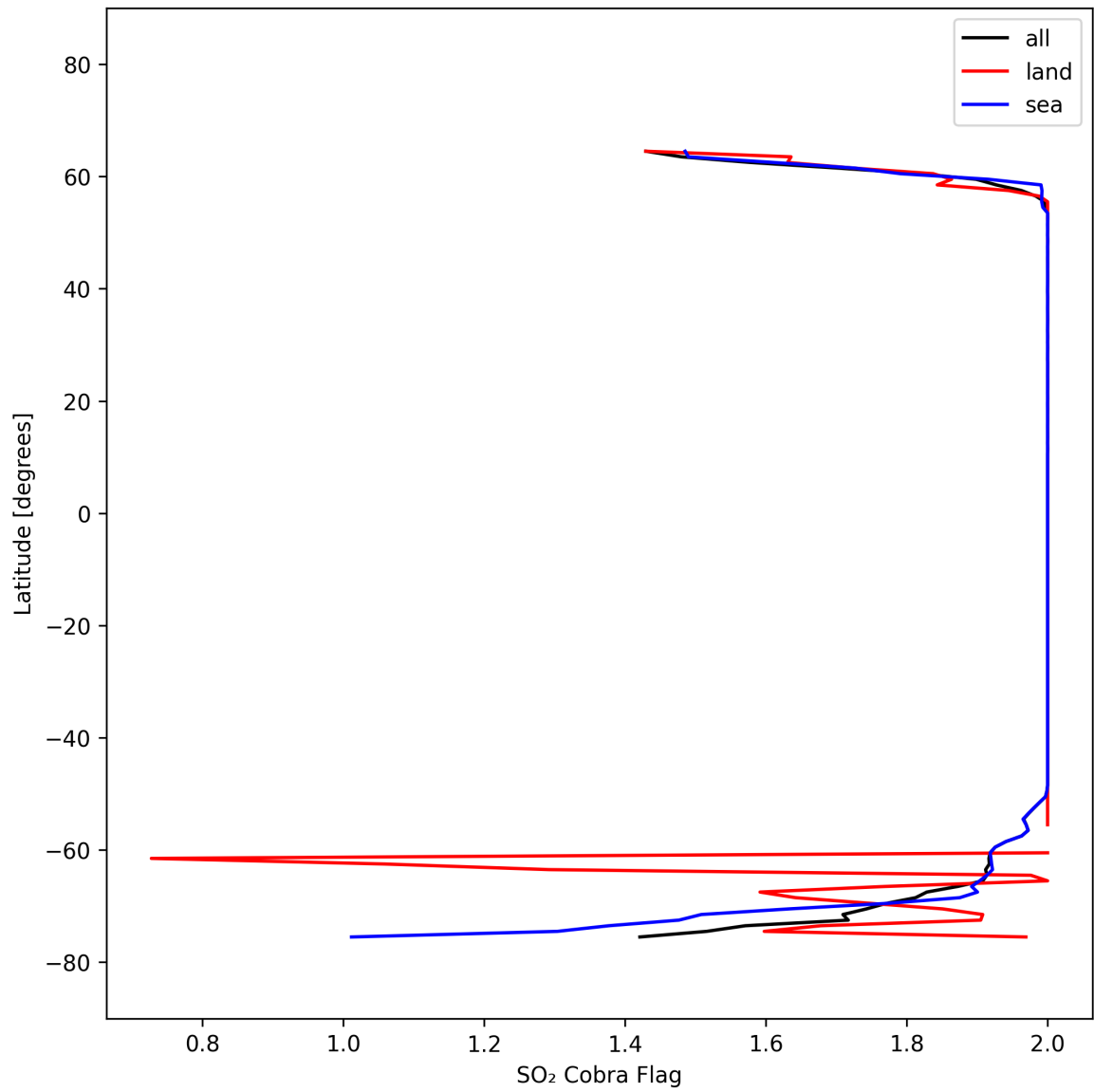
Figure 48: Zonal average of "SO 2 Cobra Flag" for 2025-10-06 to 2025-10-07.
