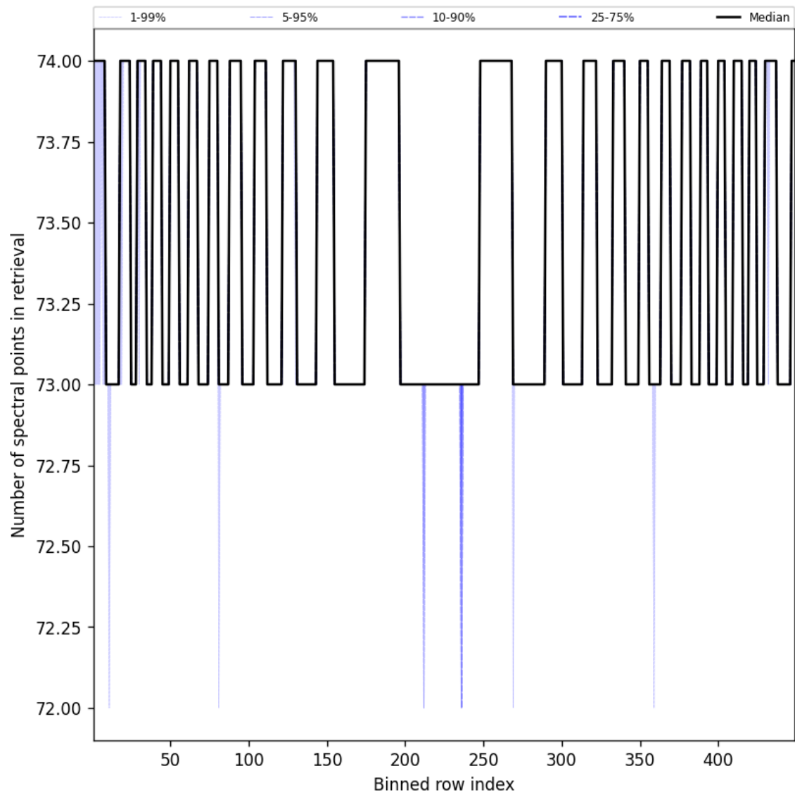
Figure 110: Along track statistics of “Number of spectral points in retrieval” for 2025-10-06 to 2025-10-07
