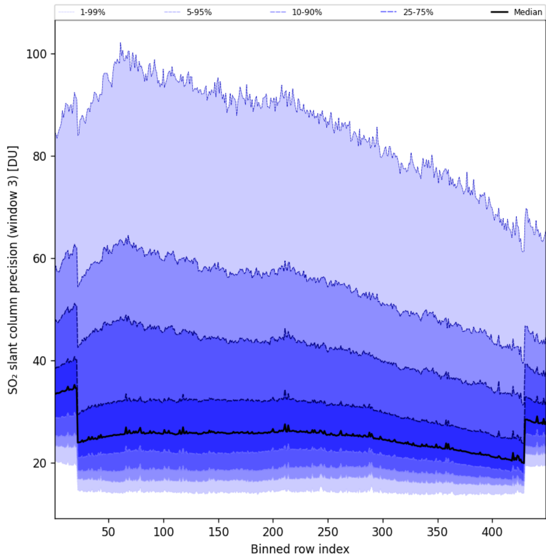
Figure 99: Along track statistics of “SO 2 slant column precision (window 3)” for 2025-10-06 to 2025-10-07
