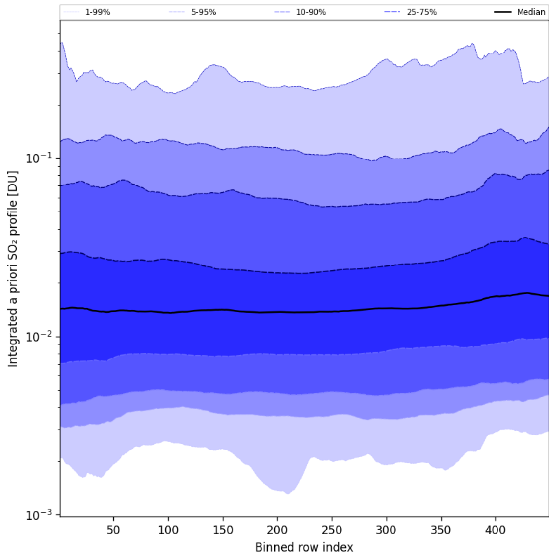
Figure 103: Along track statistics of “Integrated a priori SO 2 profile” for 2025-10-06 to 2025-10-07
