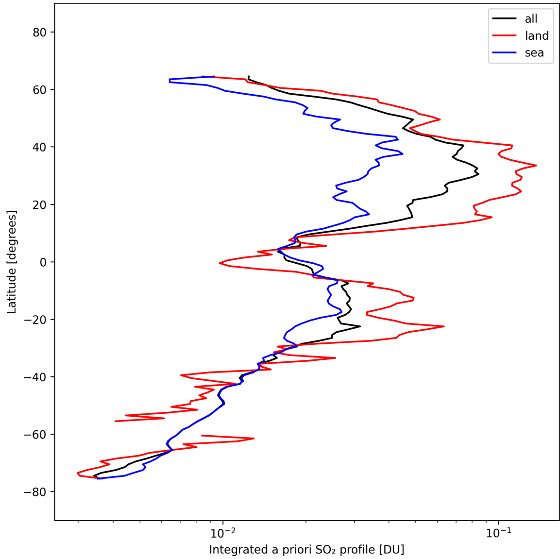
Figure 49: Zonal average of “Integrated a priori SO 2 profile” for 2025-10-06 to 2025-10-07.
