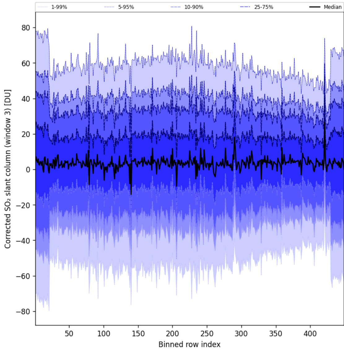
Figure 100: Along track statistics of “Corrected SO 2 slant column (window 3)” for 2025-10-06 to 2025-10-07
