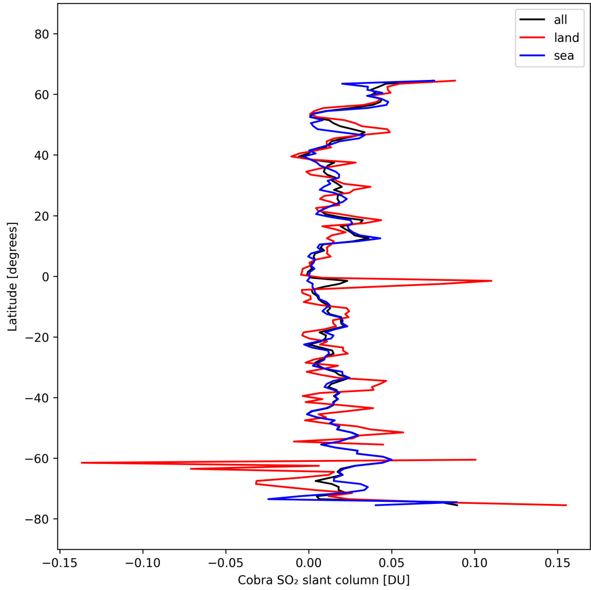
Figure 34: Zonal average of “Cobra SO 2 slant column” for 2025-10-06 to 2025-10-07.
