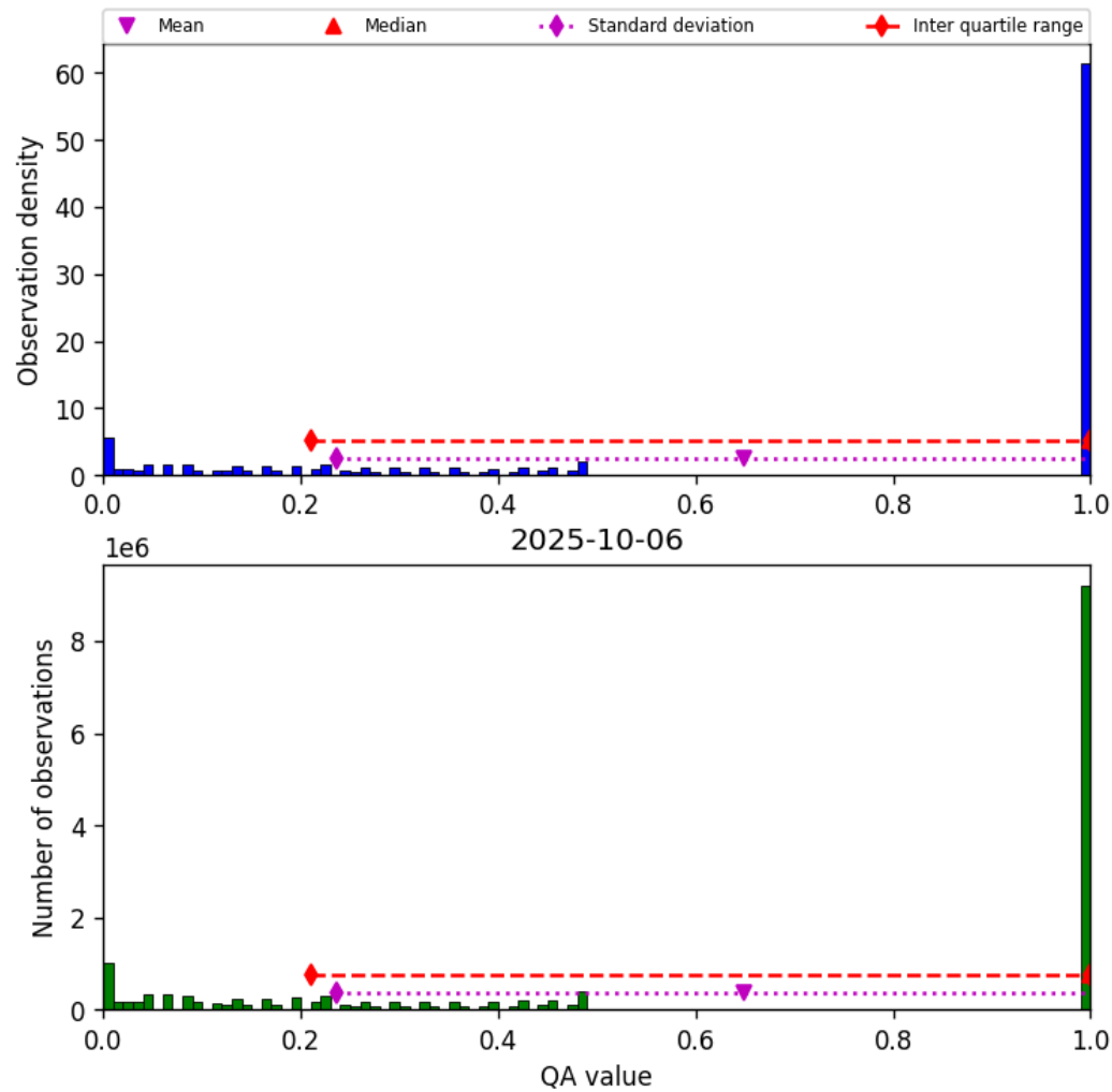
Figure 57: Histogram of “QA value” for 2025-10-06 to 2025-10-07
