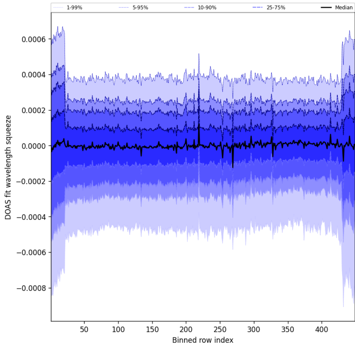
Figure 105: Along track statistics of “DOAS fit wavelength squeeze” for 2025-10-06 to 2025-10-07
