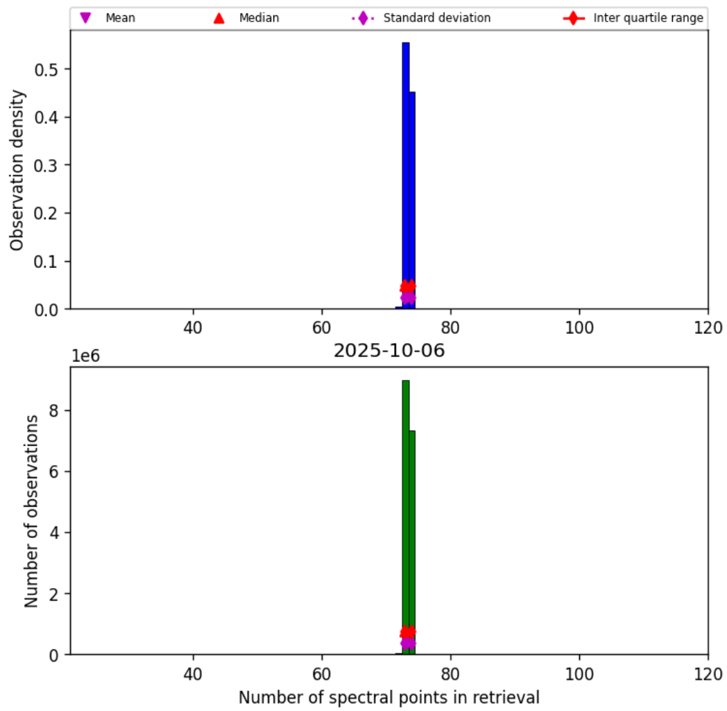
Figure 83: Histogram of “Number of spectral points in retrieval” for 2025-10-06 to 2025-10-07
