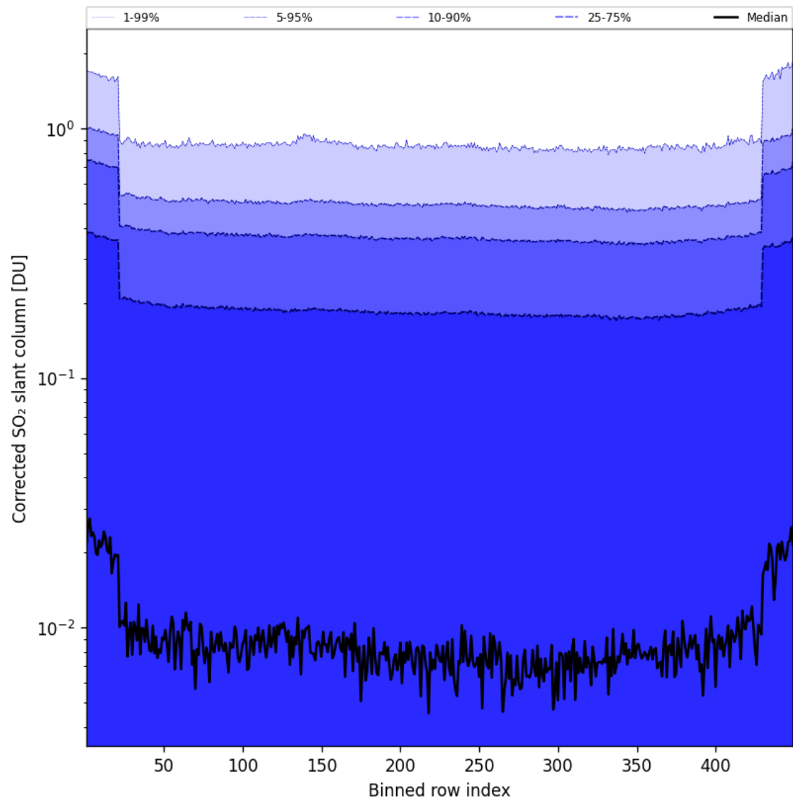
Figure 87: Along track statistics of “Corrected SO 2 slant column” for 2025-10-06 to 2025-10-07
