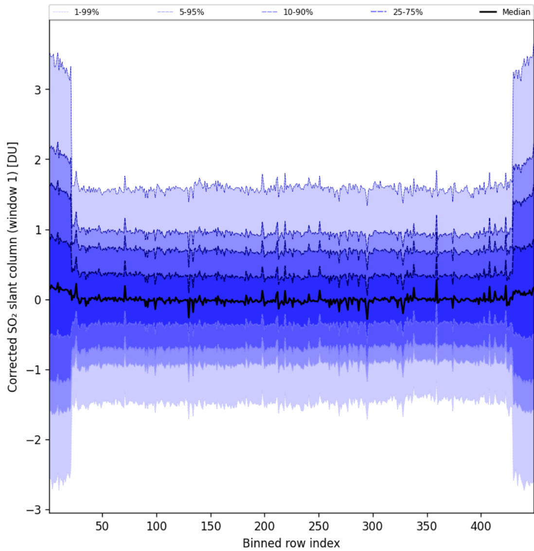
Figure 92: Along track statistics of “Corrected SO 2 slant column (window 1)” for 2025-10-06 to 2025-10-07
