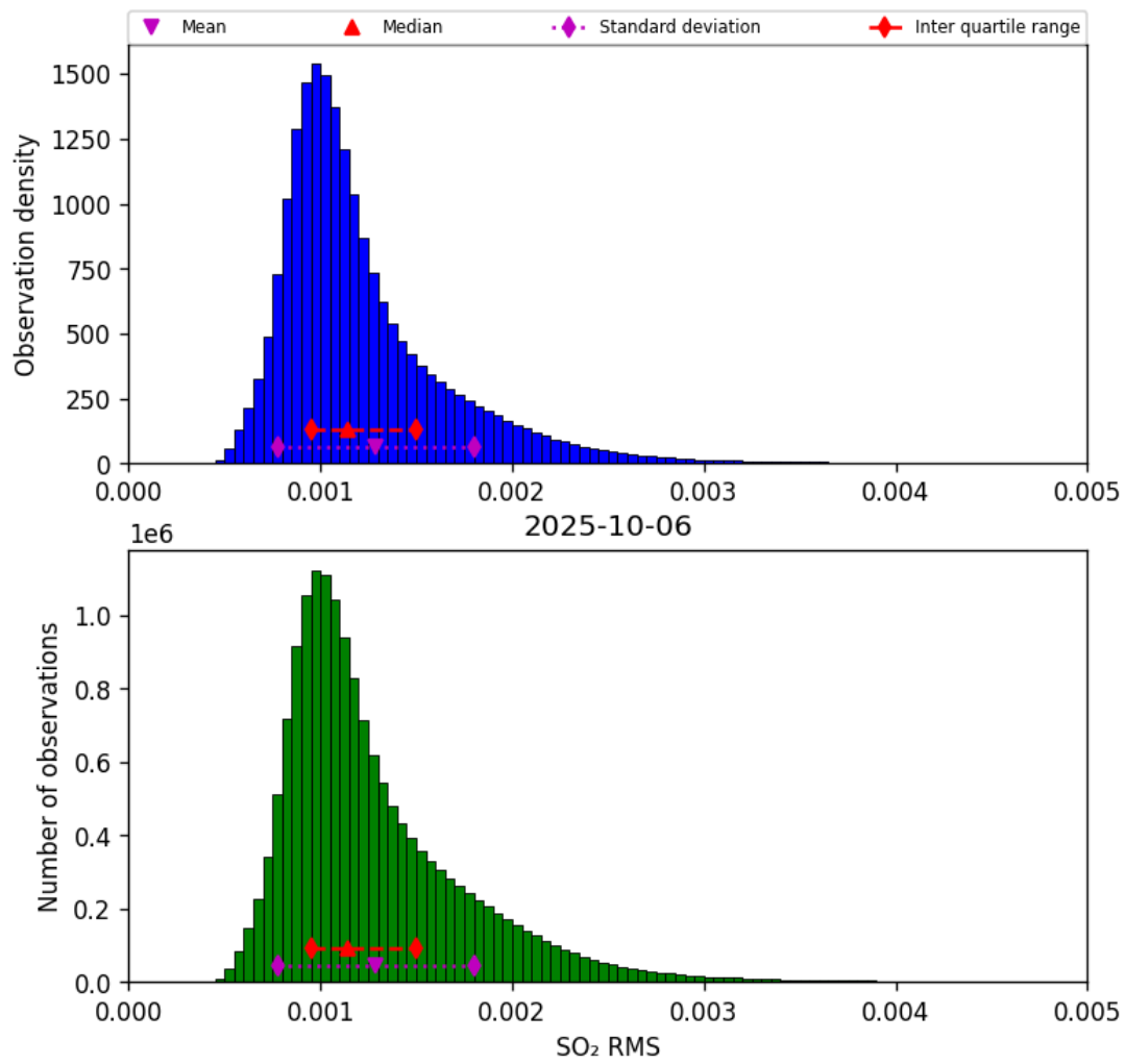
Figure 79: Histogram of “SO 2 RMS” for 2025-10-06 to 2025-10-07
