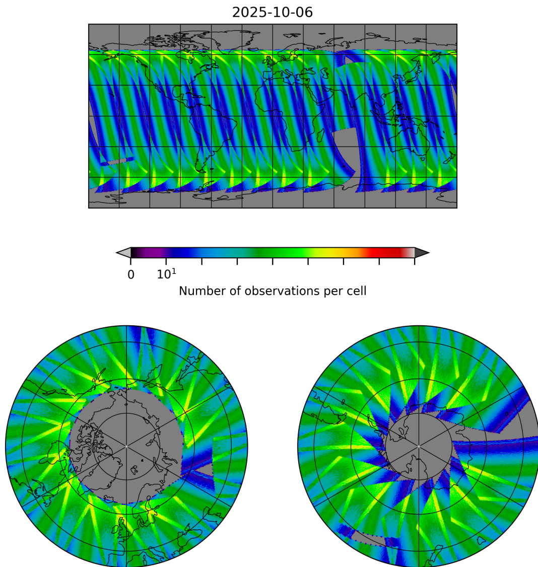
Figure 29: Map of the number of observations for 2025-10-06 to 2025-10-07
