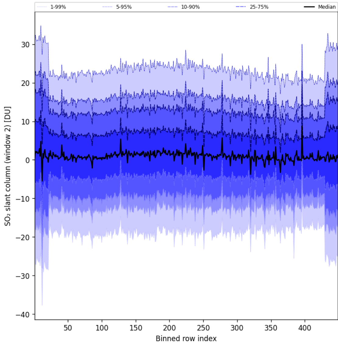
Figure 94: Along track statistics of “SO 2 slant column (window 2)” for 2025-10-06 to 2025-10-07
