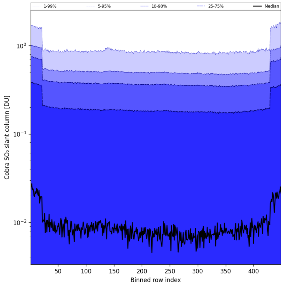
Figure 88: Along track statistics of "Cobra SO 2 slant column" for 2025-10-06 to 2025-10-07
