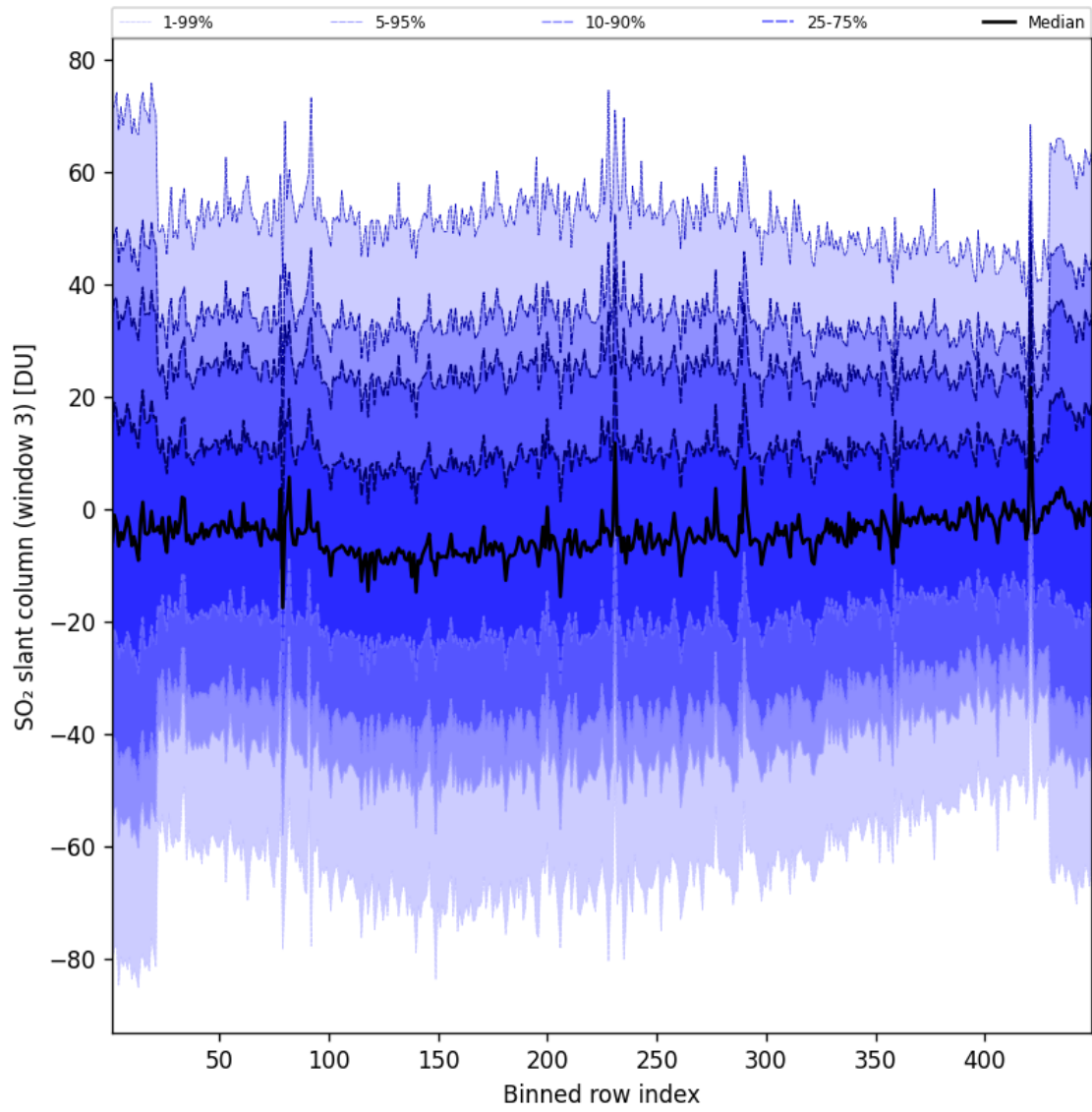
Figure 98: Along track statistics of “SO 2 slant column (window 3)” for 2025-10-06 to 2025-10-07
