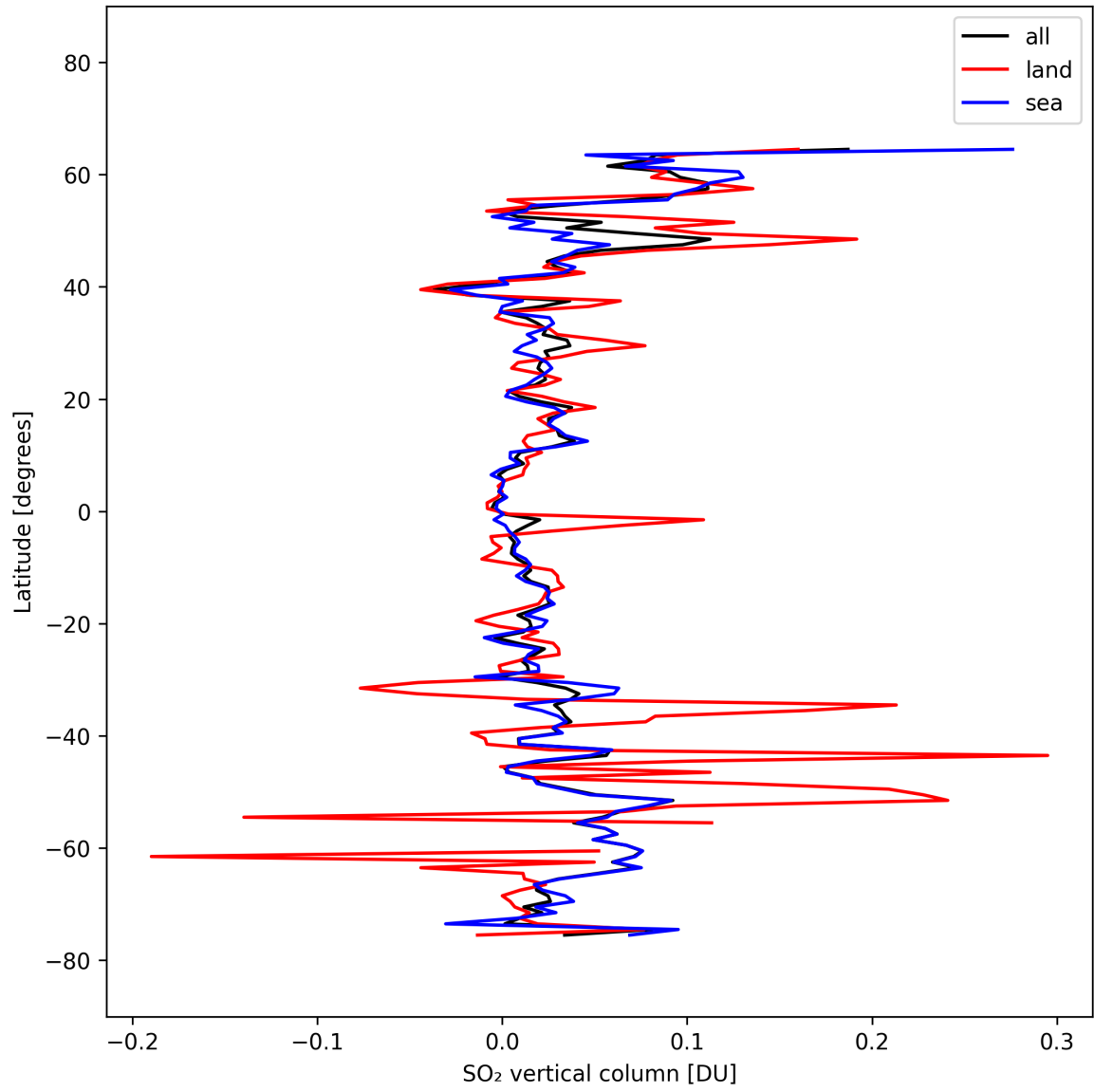
Figure 31: Zonal average of “SO 2 vertical column” for 2025-10-06 to 2025-10-07.
