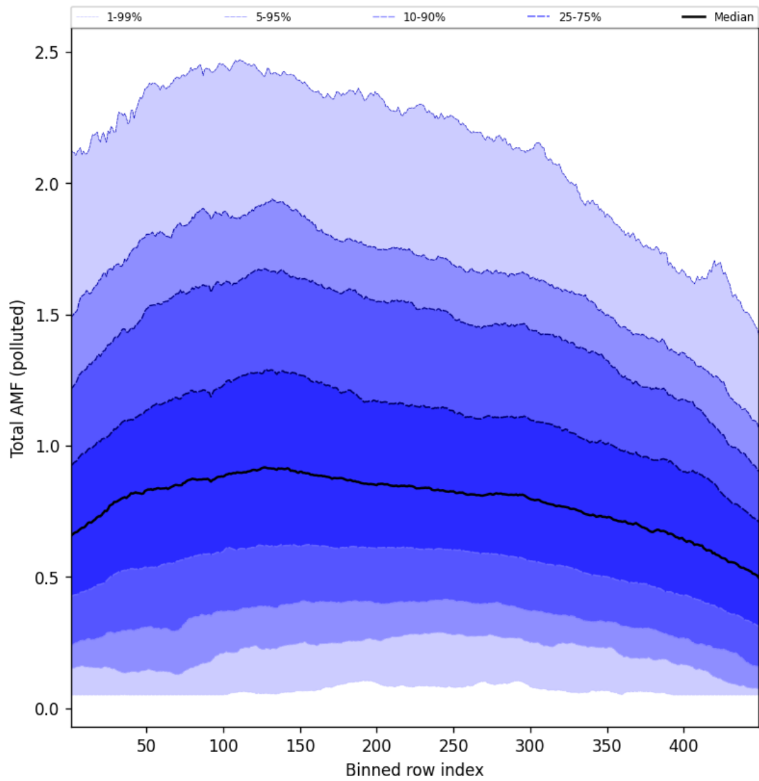
Figure 107: Along track statistics of “Total AMF (polluted)” for 2025-10-06 to 2025-10-07
