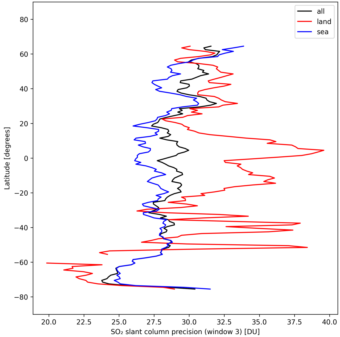
Figure 45: Zonal average of “SO 2 slant column precision (window 3)” for 2025-10-06 to 2025-10-07.
