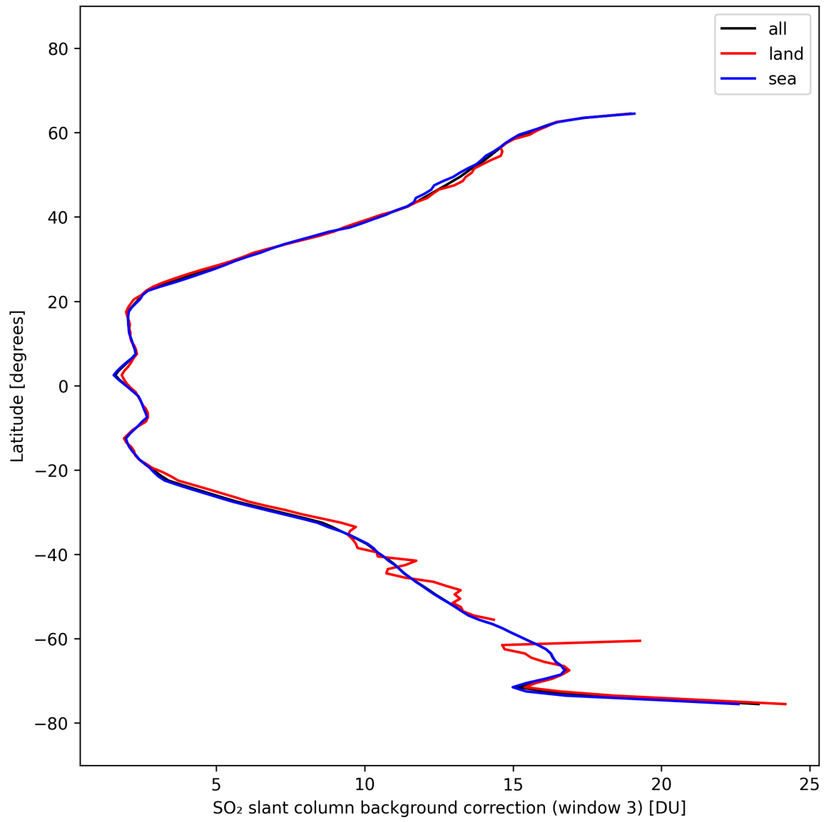
Figure 47: Zonal average of “SO 2 slant column background correction (window 3)” for 2025-10-06 to 2025-10-07.
