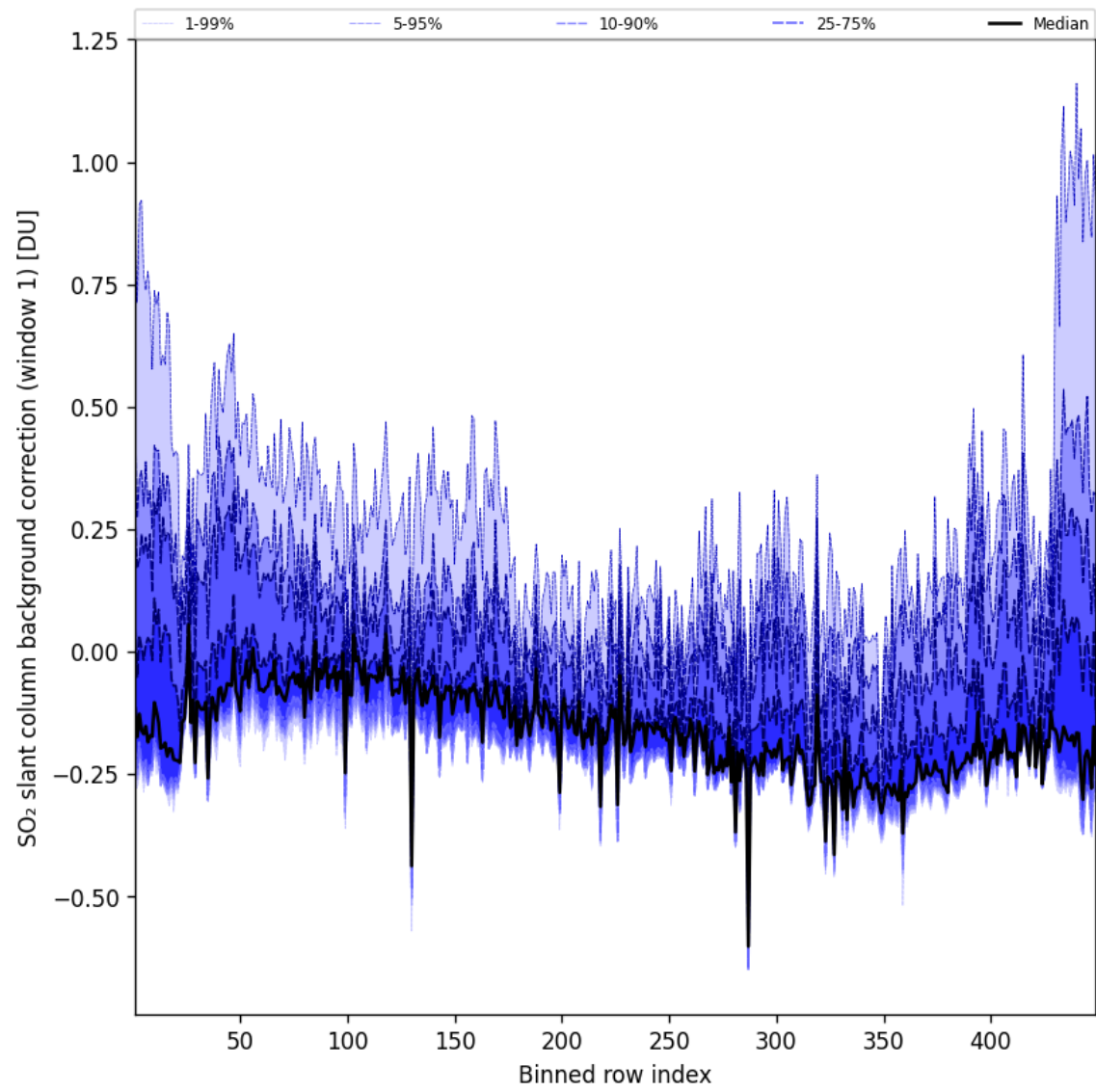
Figure 93: Along track statistics of “SO 2 slant column background correction (window 1)” for 2025-10-06 to 2025-10-07
