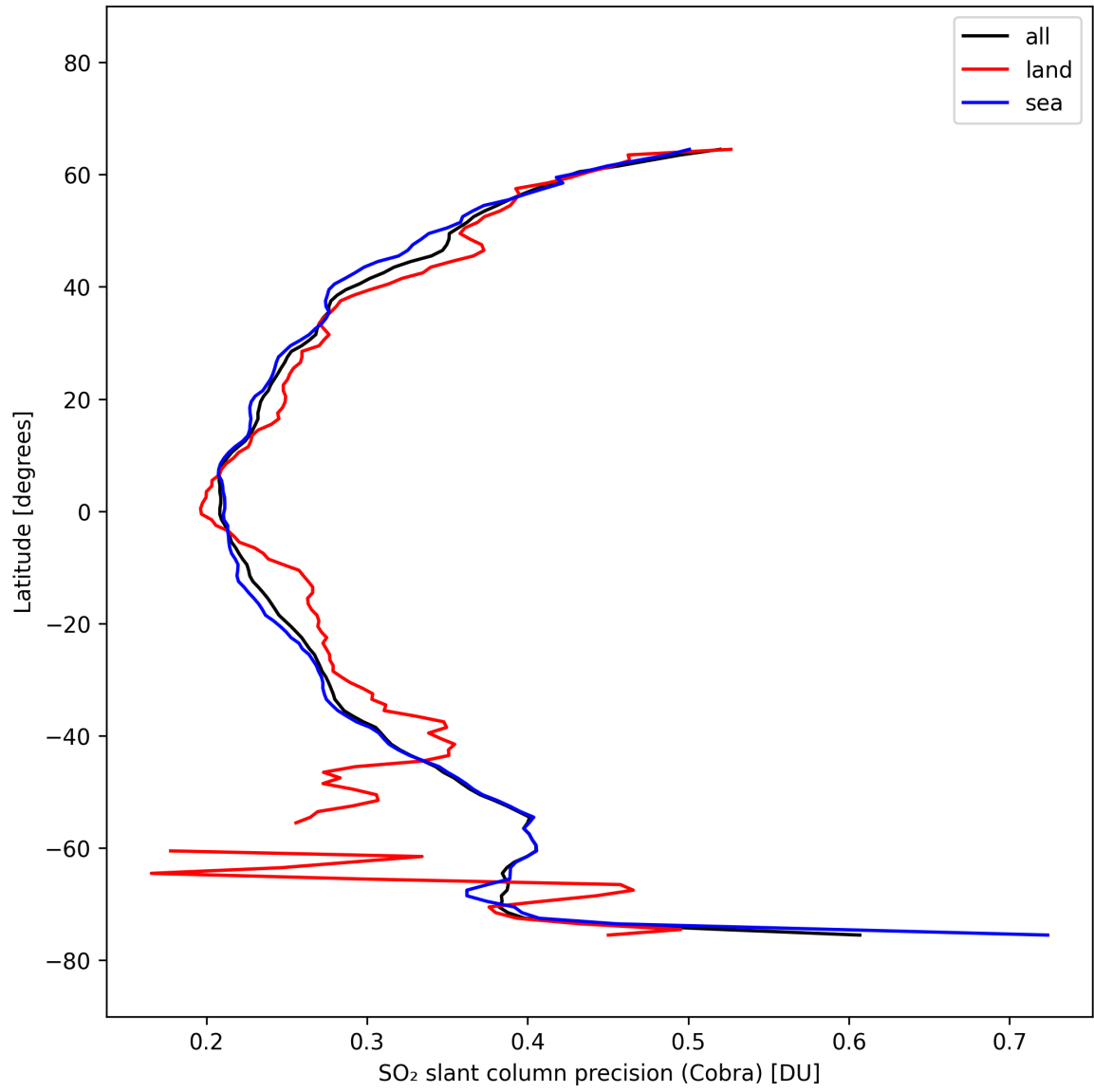
Figure 35: Zonal average of “SO 2 slant column precision (Cobra)” for 2025-10-06 to 2025-10-07.
