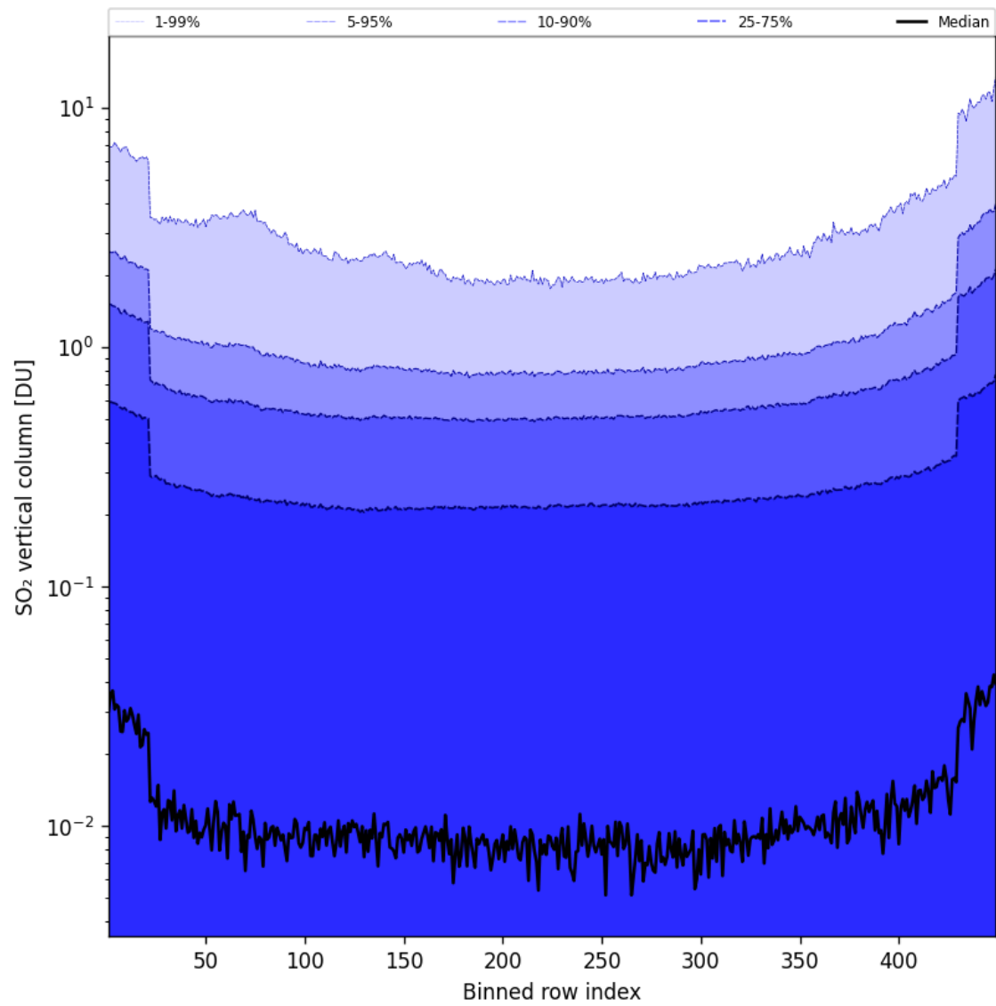
Figure 85: Along track statistics of “SO 2 vertical column” for 2025-10-06 to 2025-10-07
