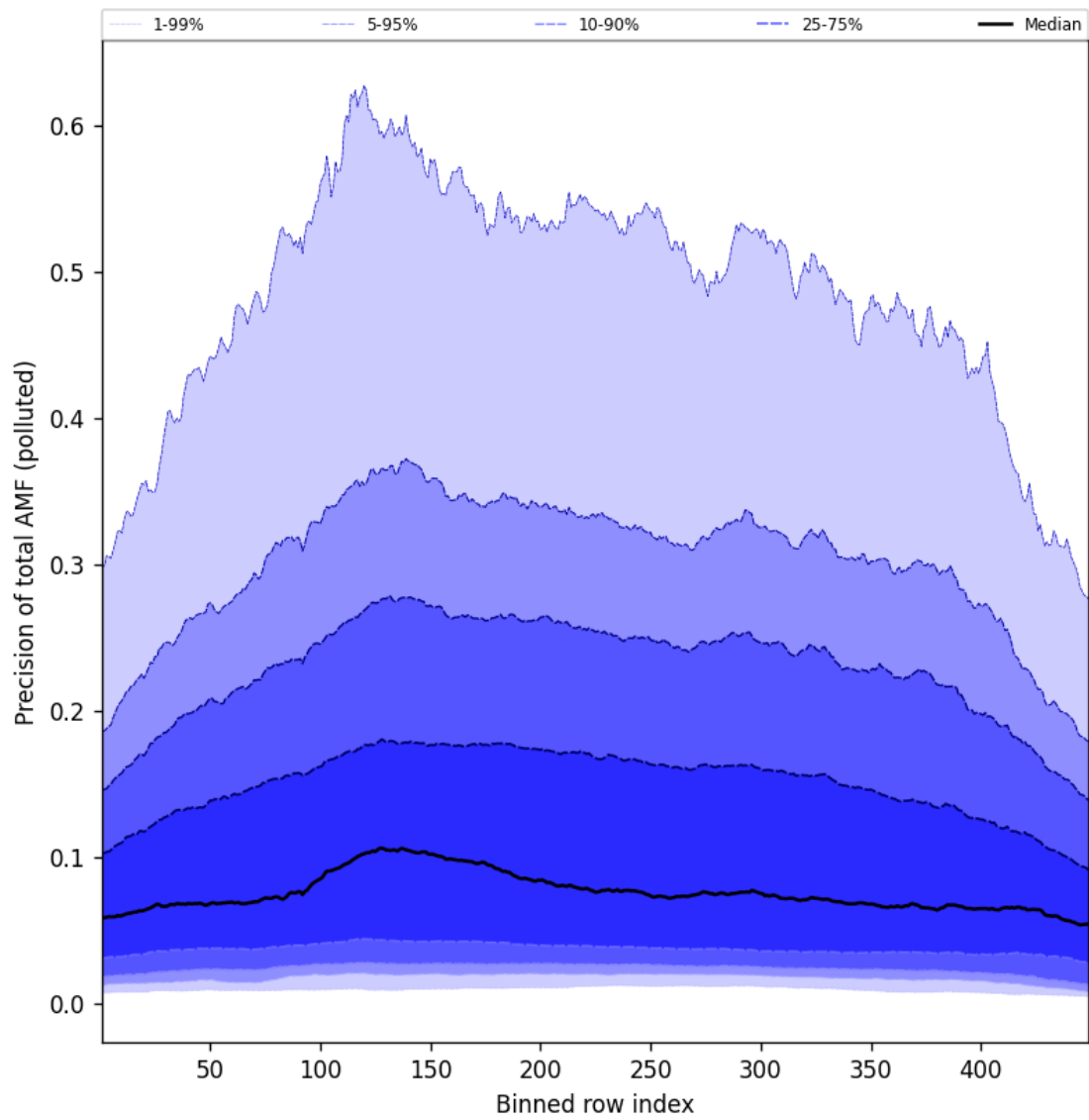
Figure 108: Along track statistics of “Precision of total AMF (polluted)” for 2025-10-06 to 2025-10-07
