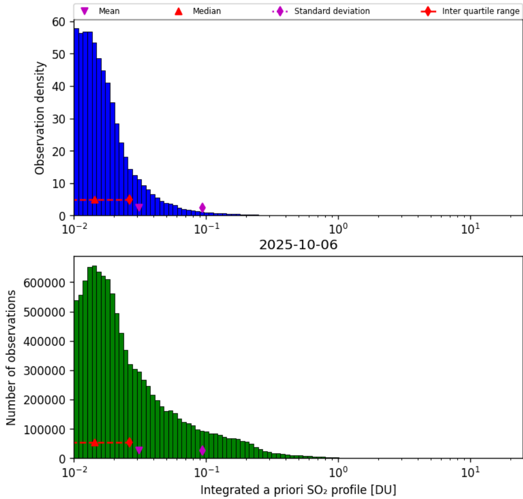
Figure 76: Histogram of “Integrated a priori SO 2 profile” for 2025-10-06 to 2025-10-07
