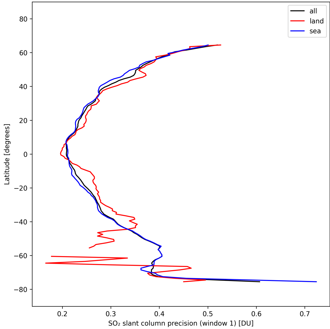
Figure 37: Zonal average of “SO 2 slant column precision (window 1)” for 2025-10-06 to 2025-10-07.
