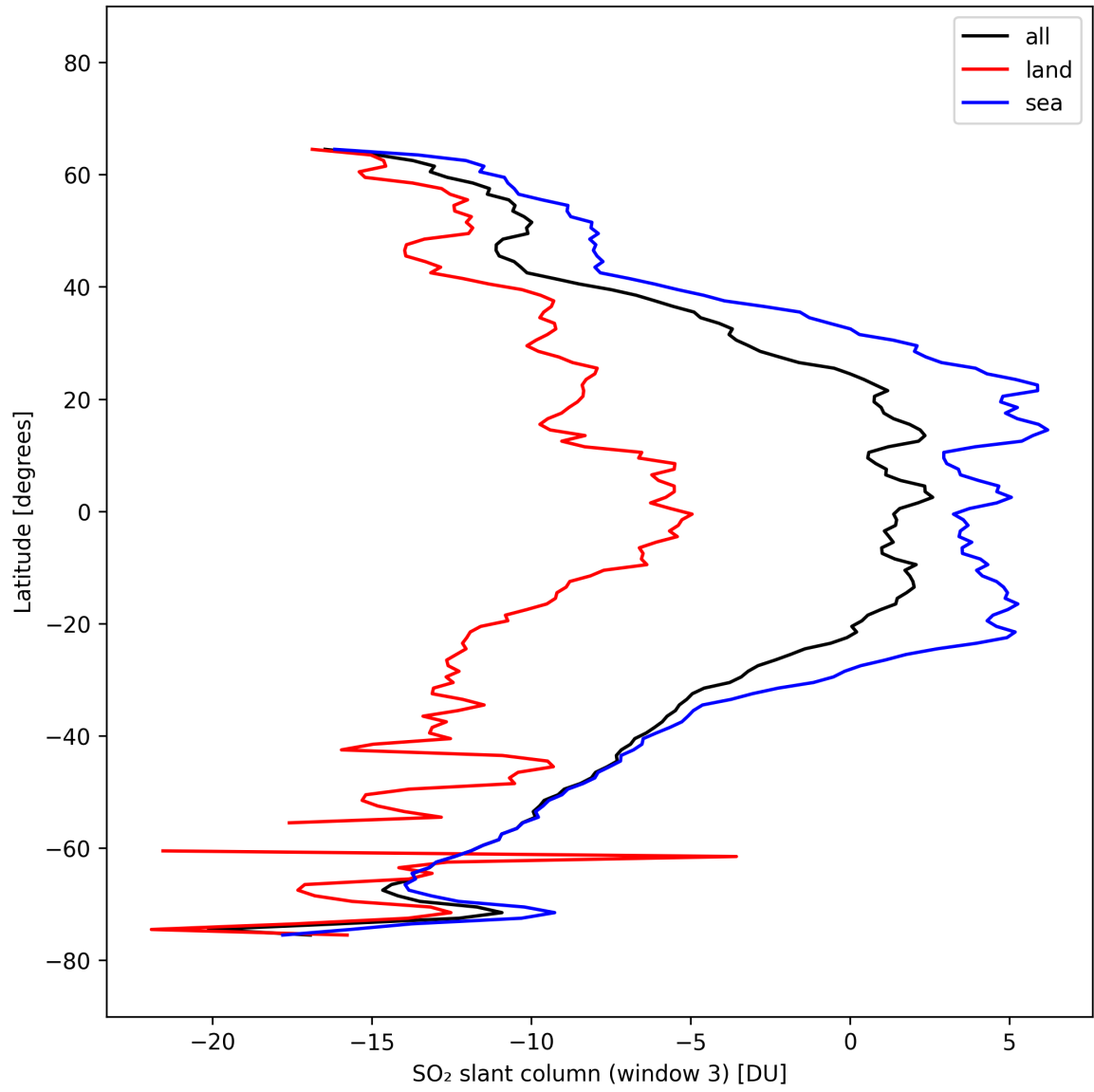
Figure 44: Zonal average of “SO 2 slant column (window 3)” for 2025-10-06 to 2025-10-07.
