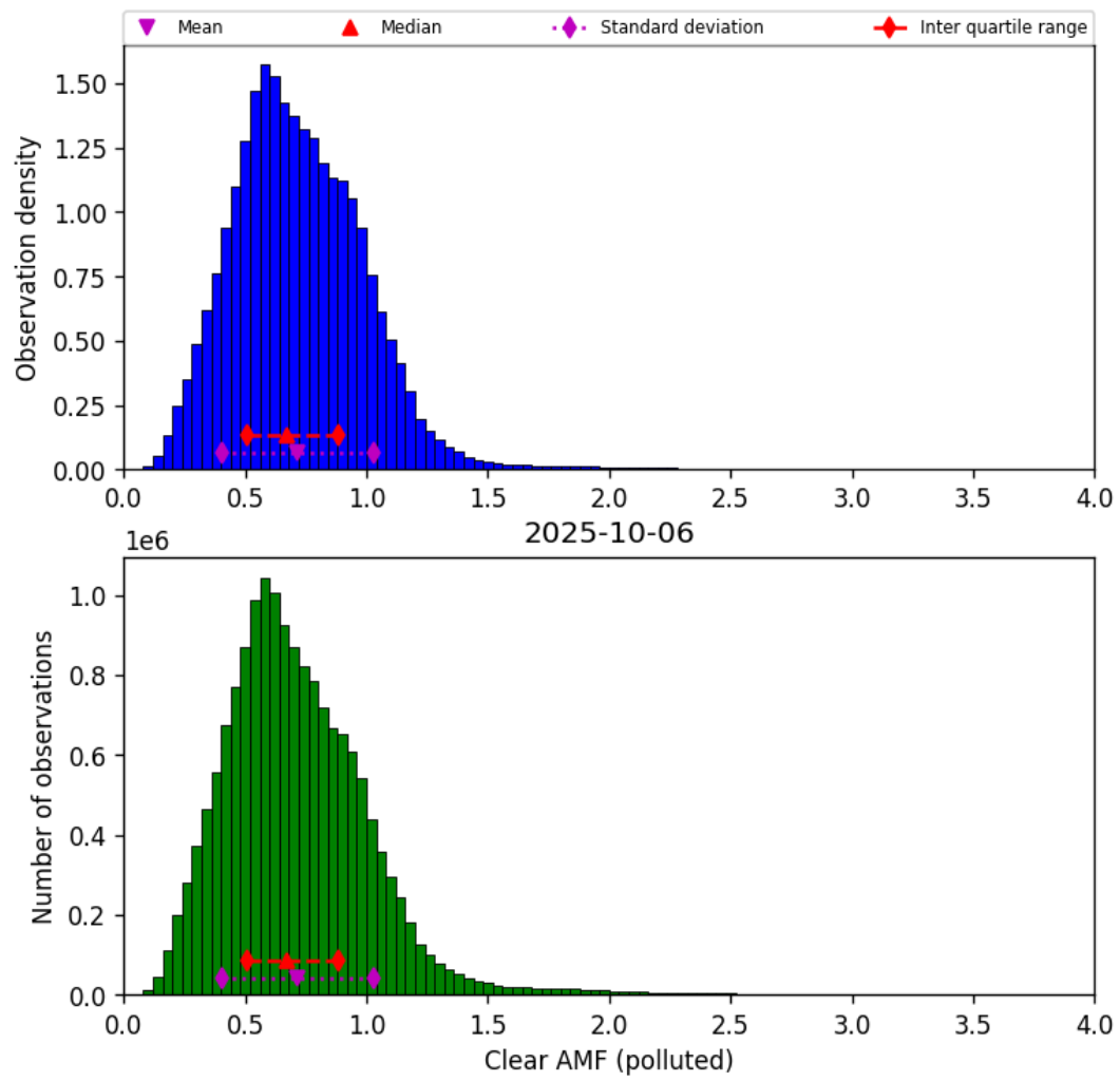
Figure 82: Histogram of “Clear AMF (polluted)” for 2025-10-06 to 2025-10-07
