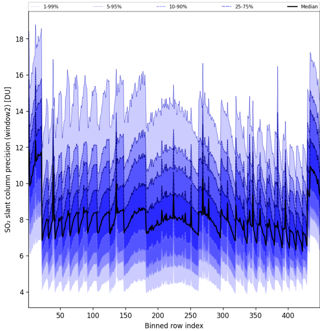
Figure 95: Along track statistics of “SO 2 slant column precision (window2)” for 2025-10-06 to 2025-10-07
