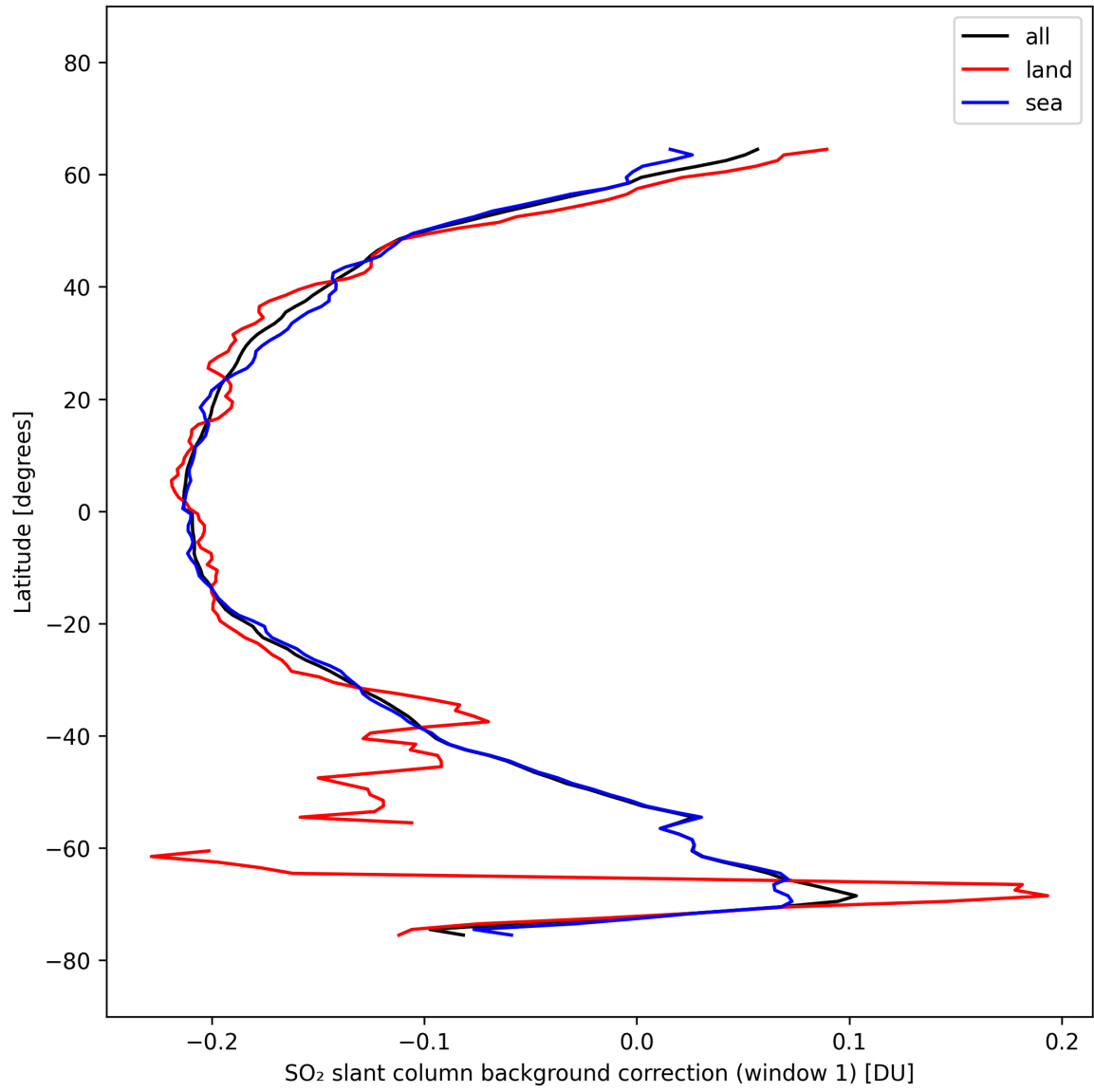
Figure 39: Zonal average of “SO 2 slant column background correction (window 1)” for 2025-10-06 to 2025-10-07.
