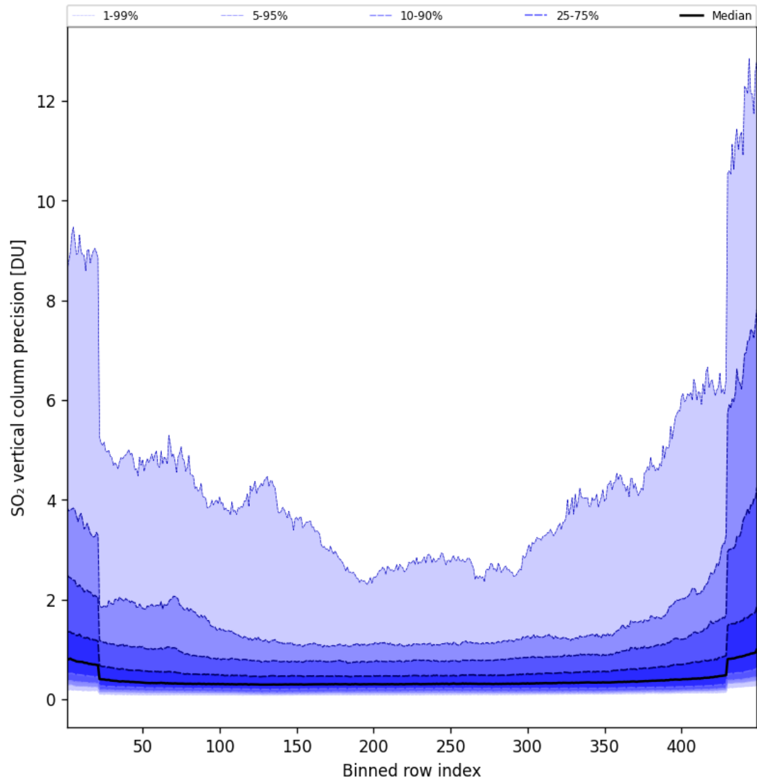
Figure 86: Along track statistics of “SO 2 vertical column precision” for 2025-10-06 to 2025-10-07
