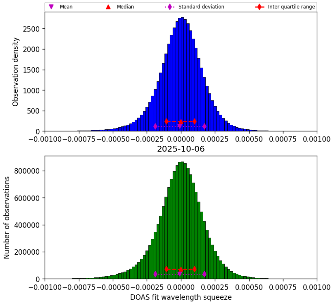
Figure 78: Histogram of “DOAS fit wavelength squeeze” for 2025-10-06 to 2025-10-07
