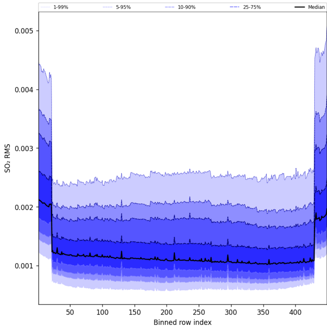
Figure 106: Along track statistics of “SO 2 RMS” for 2025-10-06 to 2025-10-07
