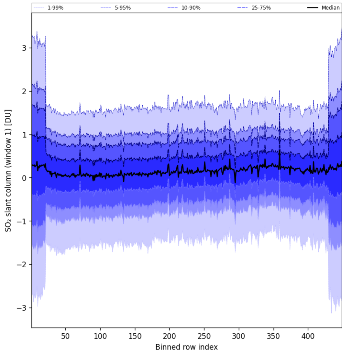
Figure 90: Along track statistics of “SO 2 slant column (window 1)” for 2025-10-06 to 2025-10-07
