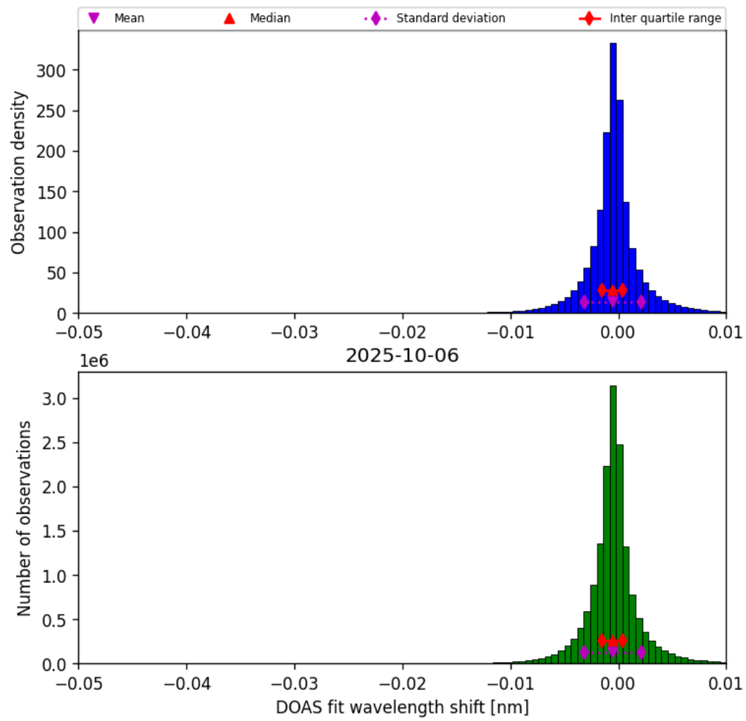
Figure 77: Histogram of “DOAS fit wavelength shift” for 2025-10-06 to 2025-10-07
