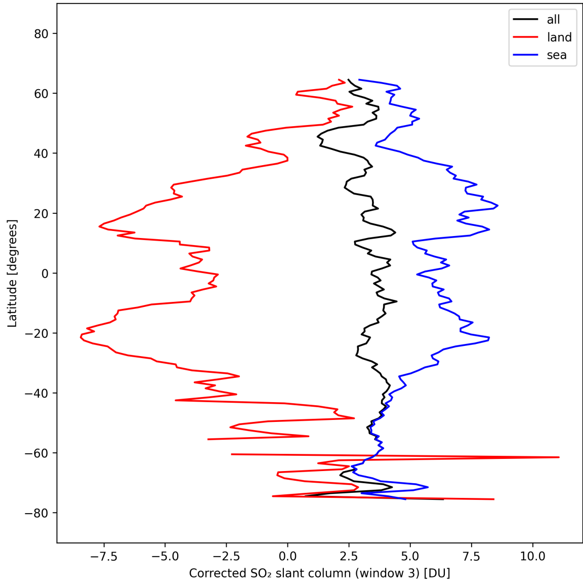
Figure 46: Zonal average of “Corrected SO 2 slant column (window 3)” for 2025-10-06 to 2025-10-07.
