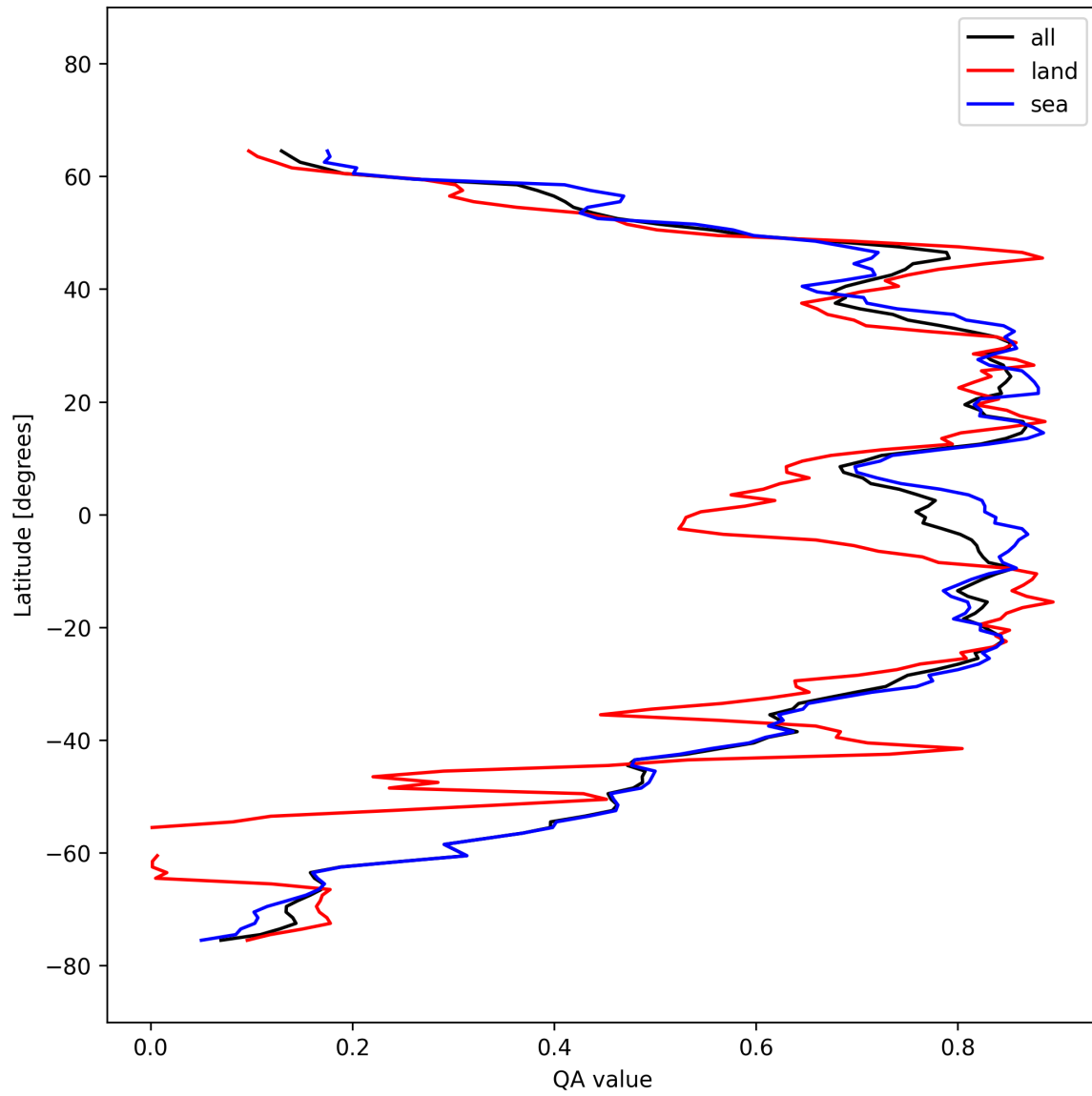
Figure 30: Zonal average of “QA value” for 2025-10-06 to 2025-10-07.
