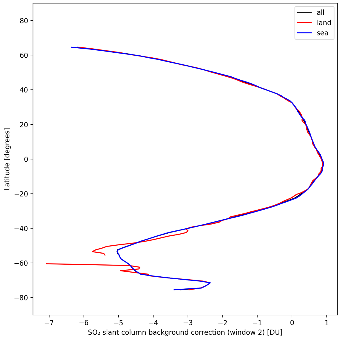
Figure 43: Zonal average of “SO 2 slant column background correction (window 2)” for 2025-10-06 to 2025-10-07.
