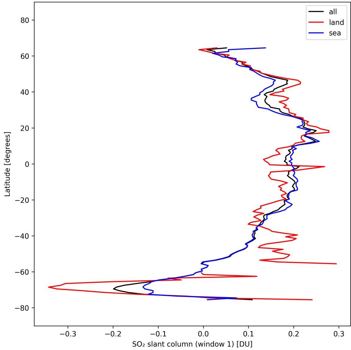
Figure 36: Zonal average of “SO 2 slant column (window 1)” for 2025-10-06 to 2025-10-07.
