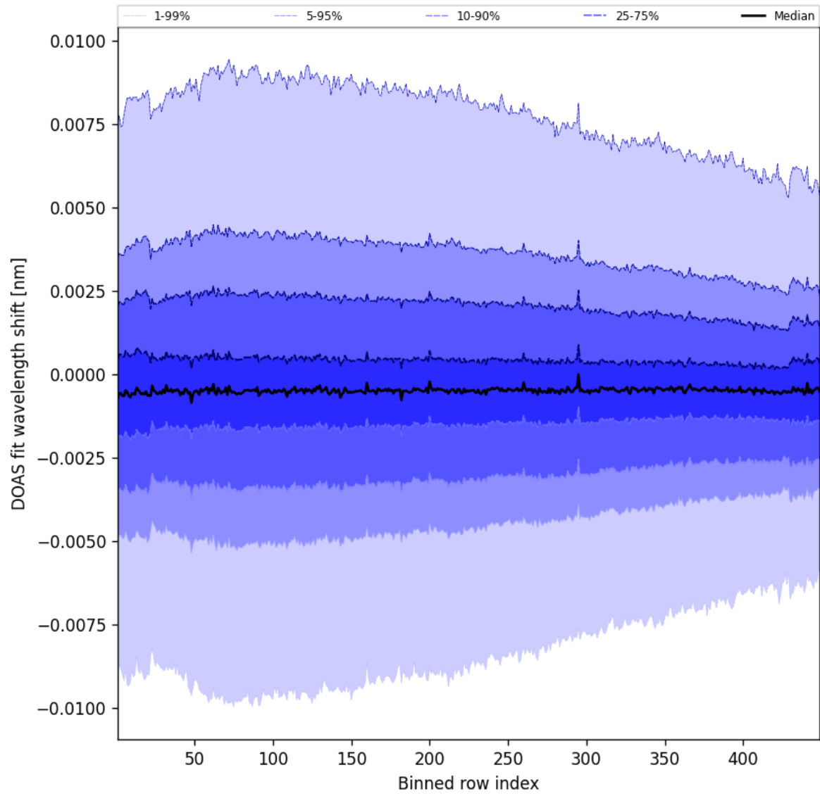
Figure 104: Along track statistics of “DOAS fit wavelength shift” for 2025-10-06 to 2025-10-07
