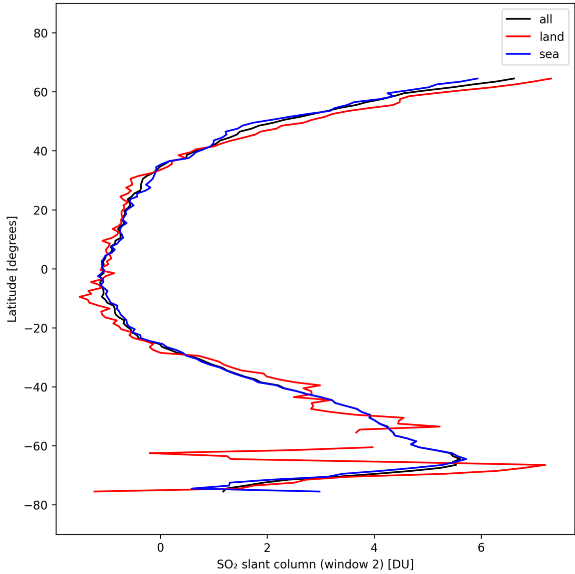
Figure 40: Zonal average of “SO 2 slant column (window 2)” for 2025-10-06 to 2025-10-07.
