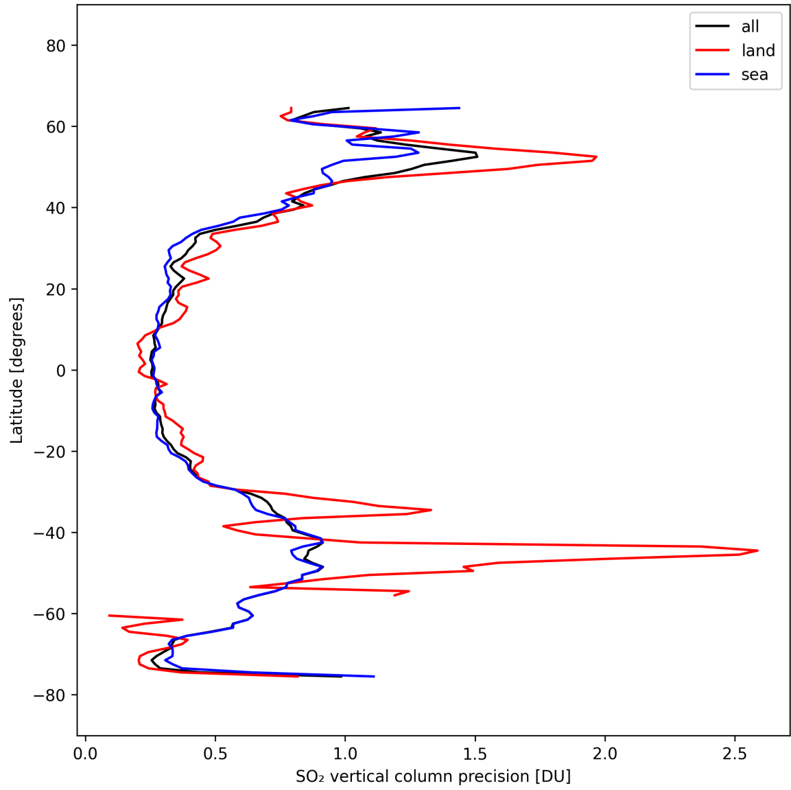
Figure 32: Zonal average of “SO 2 vertical column precision” for 2025-10-06 to 2025-10-07.
