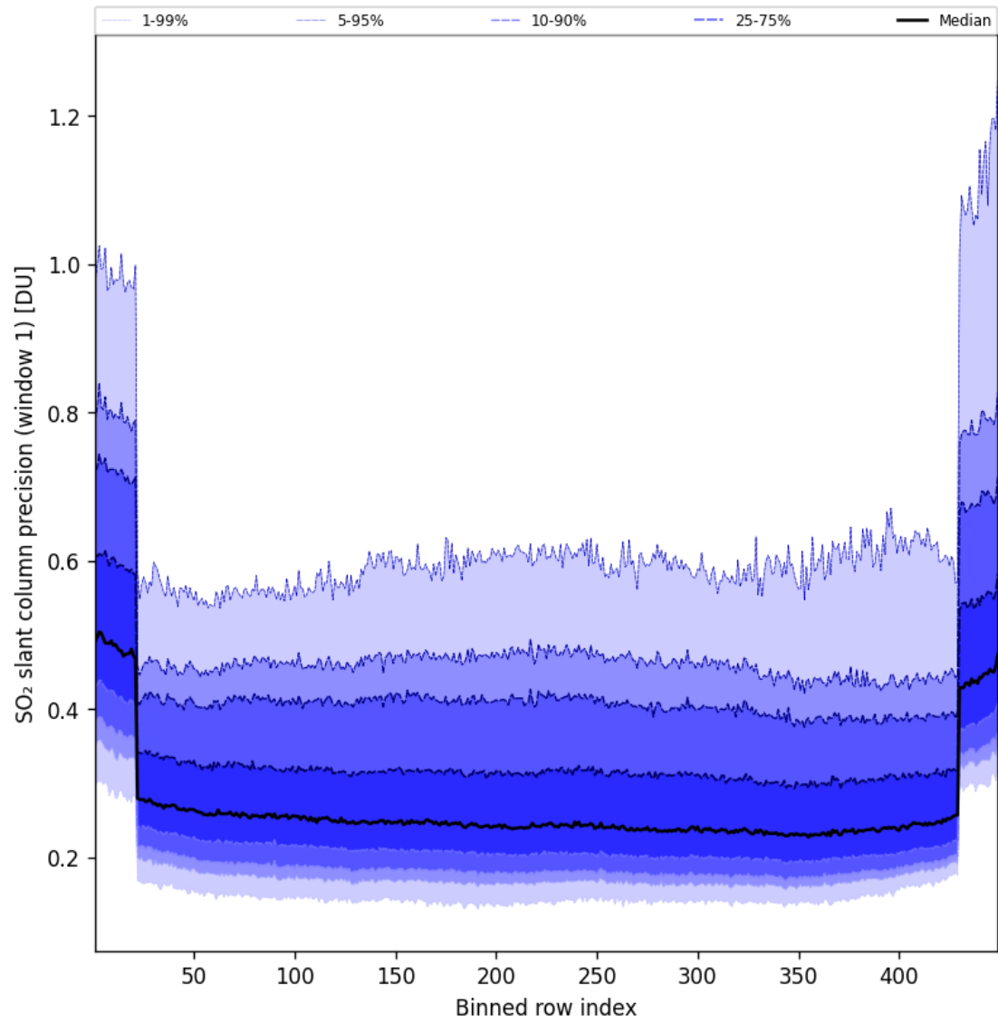
Figure 91: Along track statistics of “SO 2 slant column precision (window 1)” for 2025-10-06 to 2025-10-07
