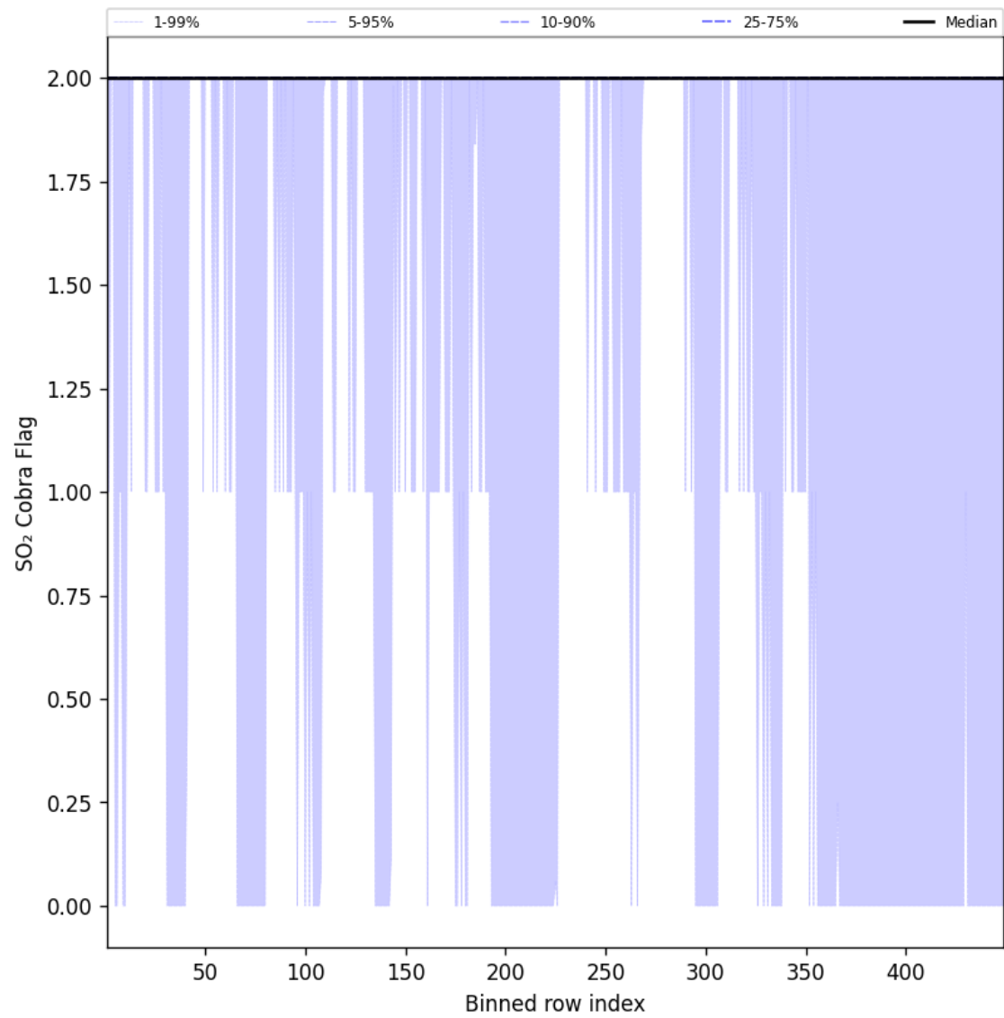
Figure 102: Along track statistics of "SO 2 Cobra Flag" for 2025-10-06 to 2025-10-07
