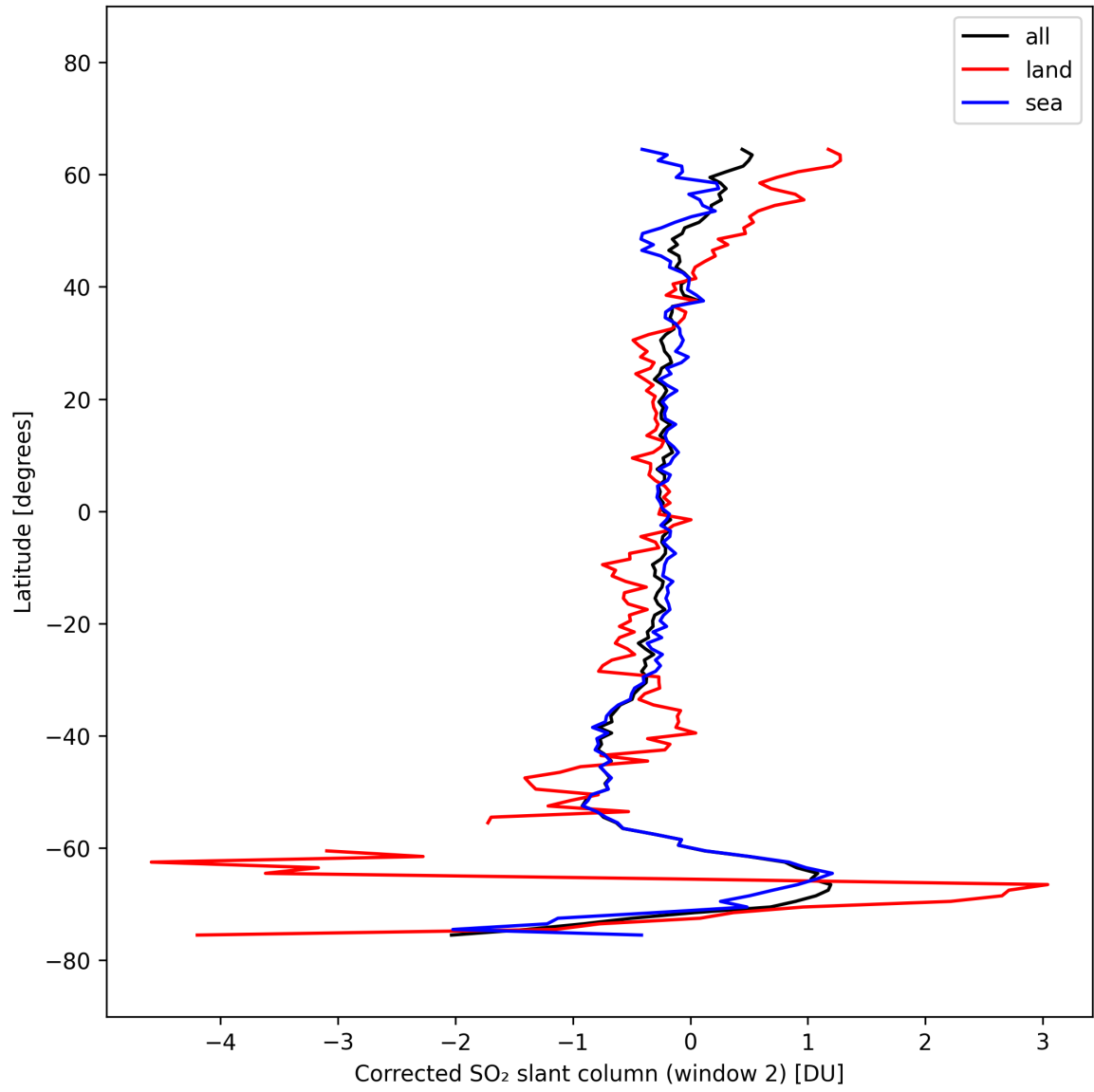
Figure 42: Zonal average of “Corrected SO 2 slant column (window 2)” for 2025-10-06 to 2025-10-07.
