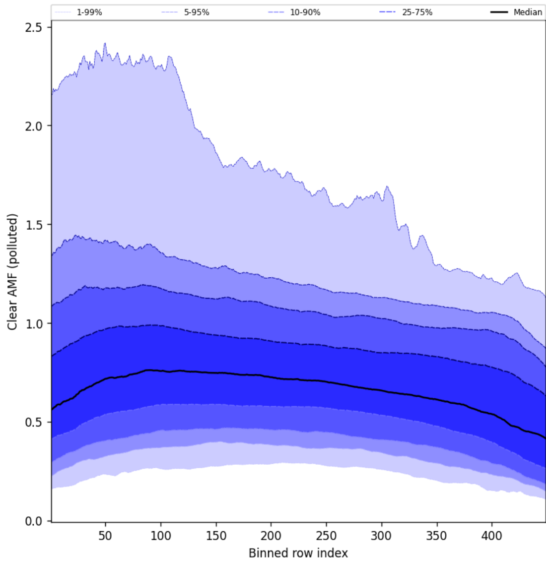
Figure 109: Along track statistics of “Clear AMF (polluted)” for 2025-10-06 to 2025-10-07
