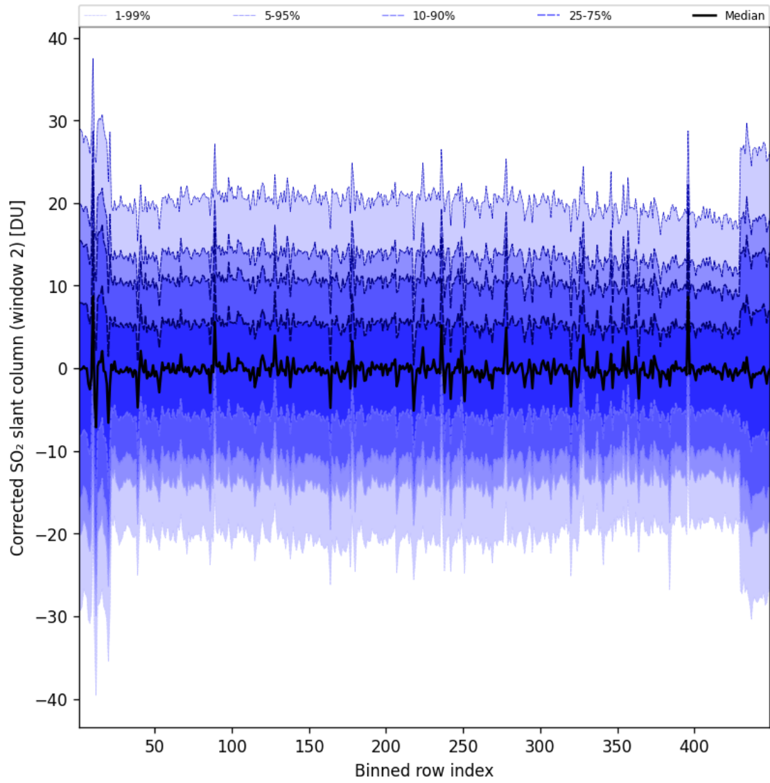
Figure 96: Along track statistics of “Corrected SO 2 slant column (window 2)” for 2025-10-06 to 2025-10-07
