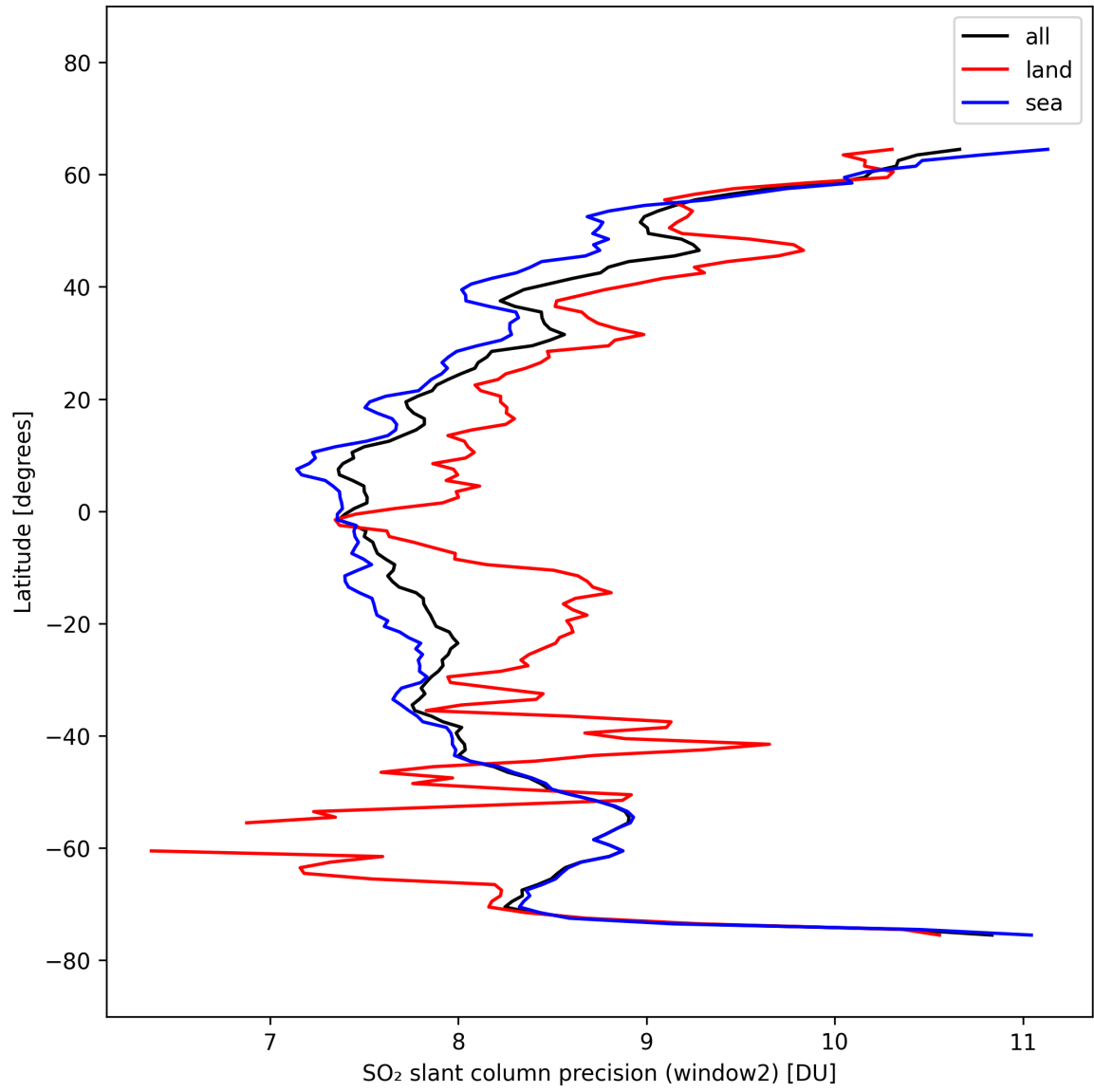
Figure 41: Zonal average of “SO 2 slant column precision (window2)” for 2025-10-06 to 2025-10-07.
