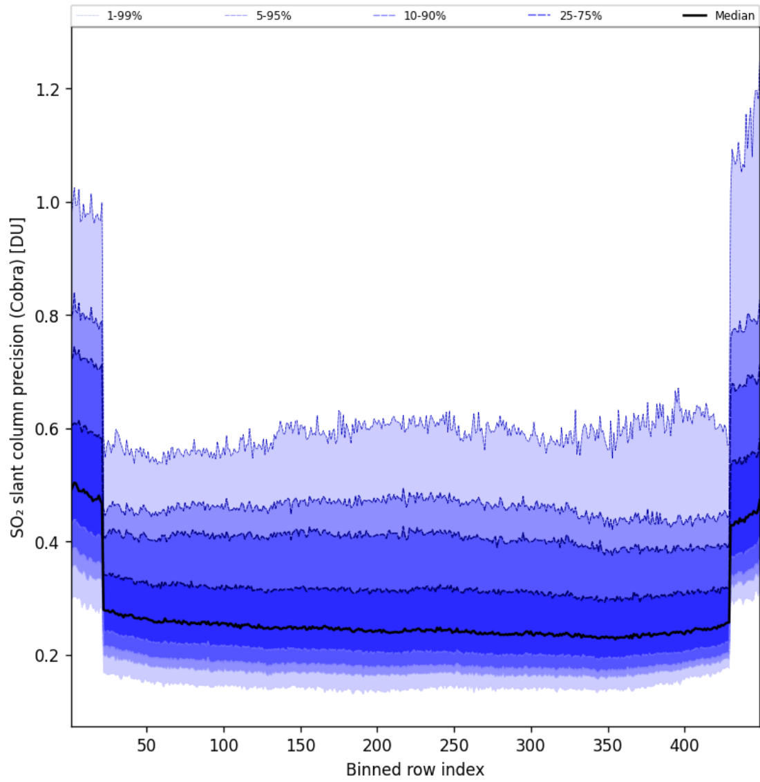
Figure 89: Along track statistics of “SO 2 slant column precision (Cobra)” for 2025-10-06 to 2025-10-07
