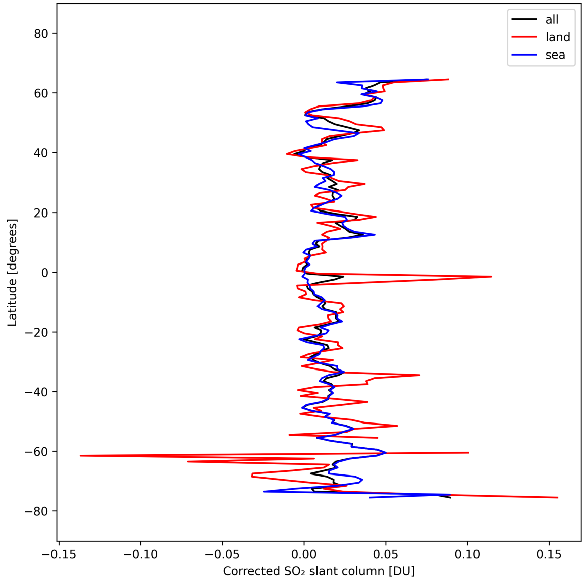
Figure 33: Zonal average of “Corrected SO 2 slant column” for 2025-10-06 to 2025-10-07.
