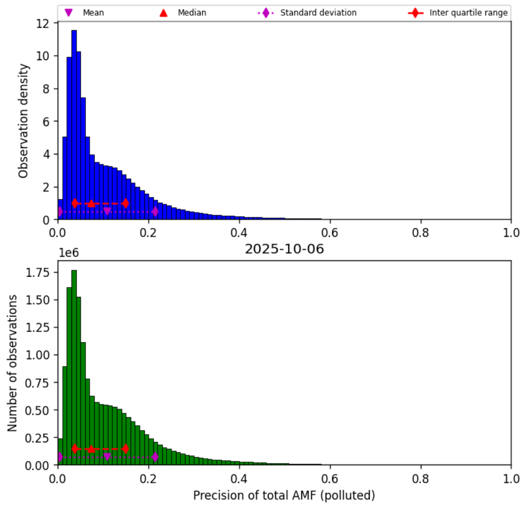
Figure 81: Histogram of “Precision of total AMF (polluted)” for 2025-10-06 to 2025-10-07
