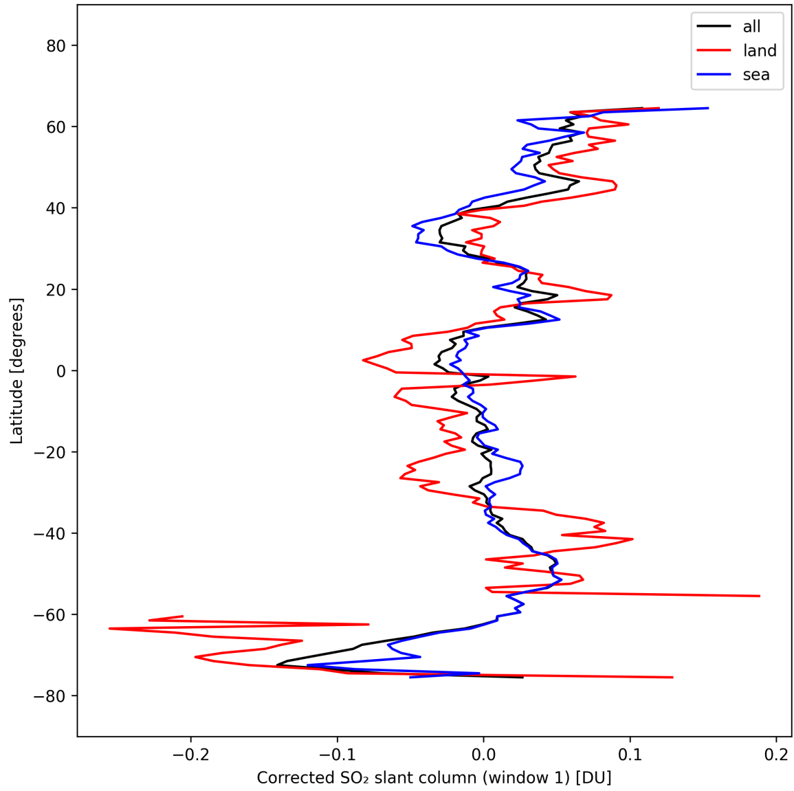
Figure 38: Zonal average of “Corrected SO 2 slant column (window 1)” for 2025-10-06 to 2025-10-07.
