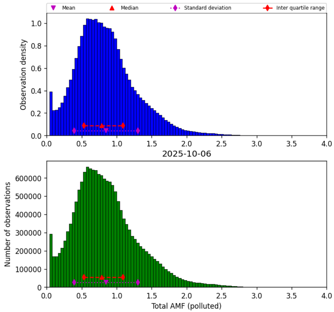
Figure 80: Histogram of “Total AMF (polluted)” for 2025-10-06 to 2025-10-07
