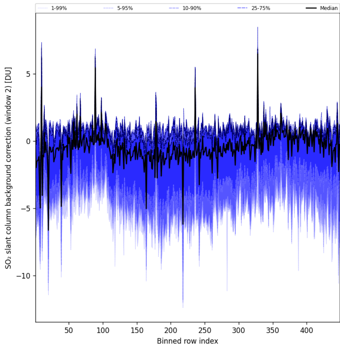
Figure 97: Along track statistics of “SO 2 slant column background correction (window 2)” for 2025-10-06 to 2025-10-07
