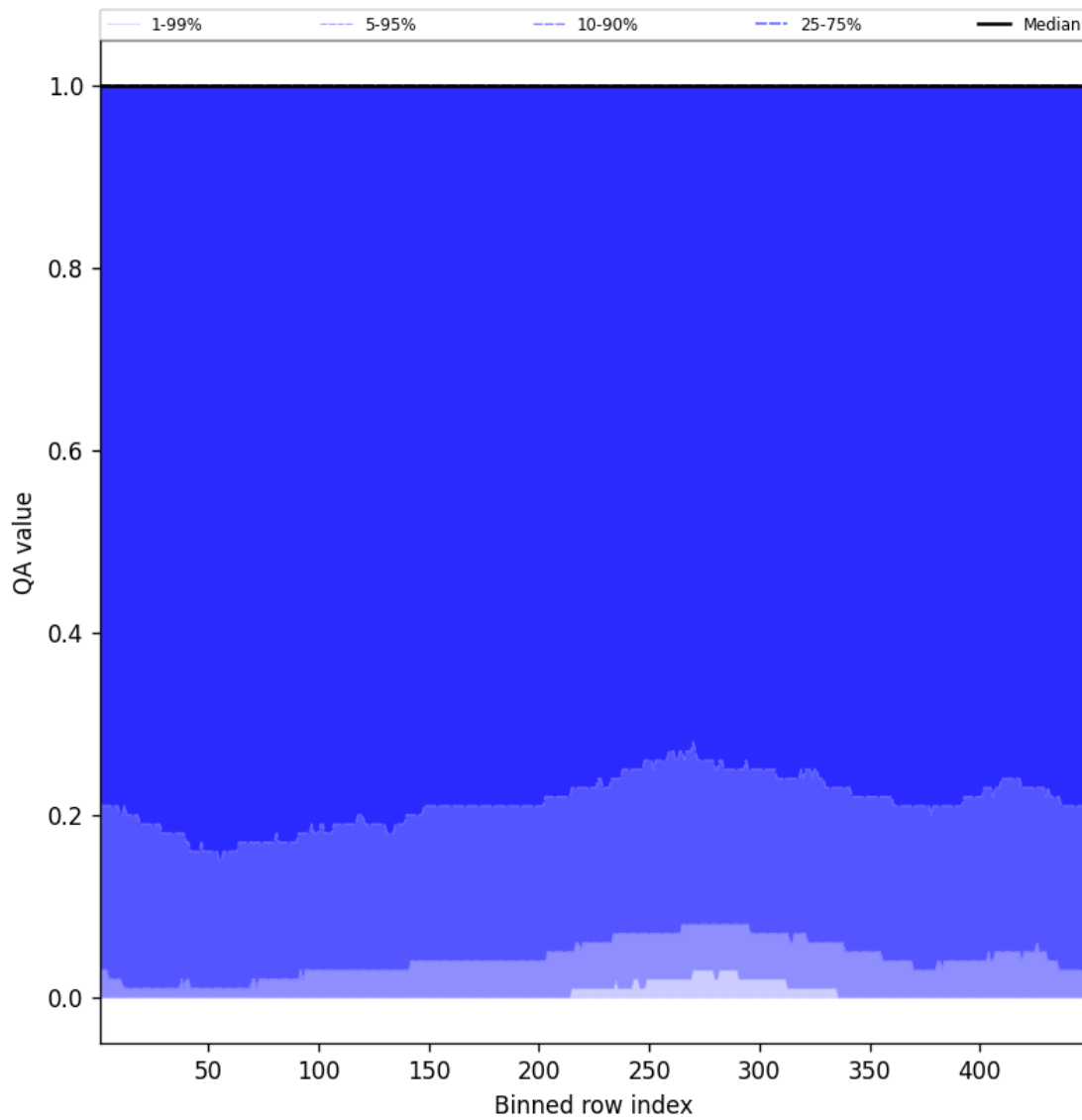
Figure 84: Along track statistics of “QA value” for 2025-10-06 to 2025-10-07
