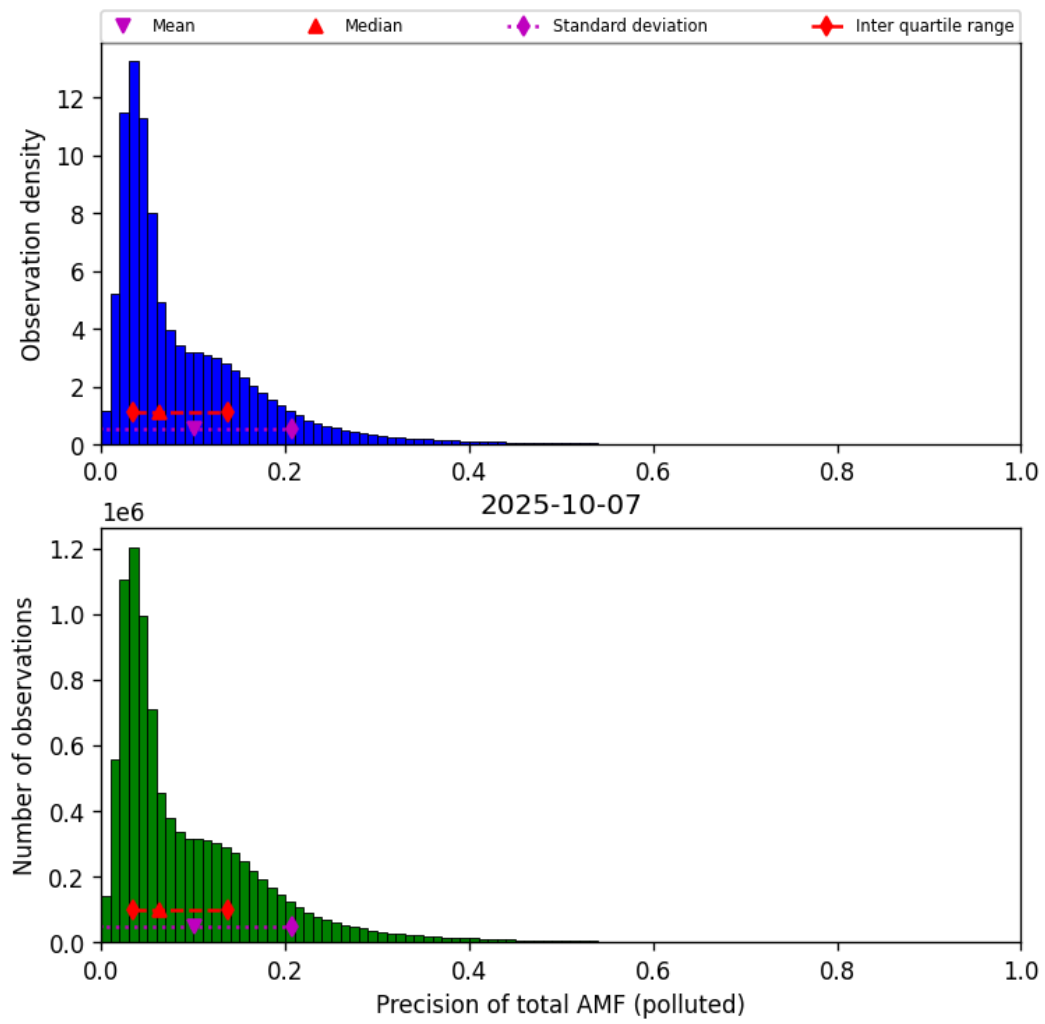
Figure 81: Histogram of “Precision of total AMF (polluted)” for 2025-10-07 to 2025-10-07
