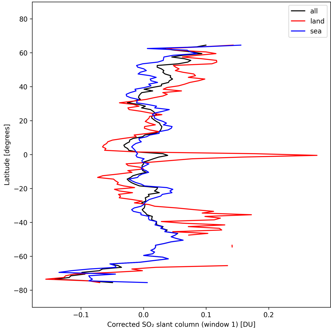
Figure 38: Zonal average of “Corrected SO 2 slant column (window 1)” for 2025-10-07 to 2025-10-07.
