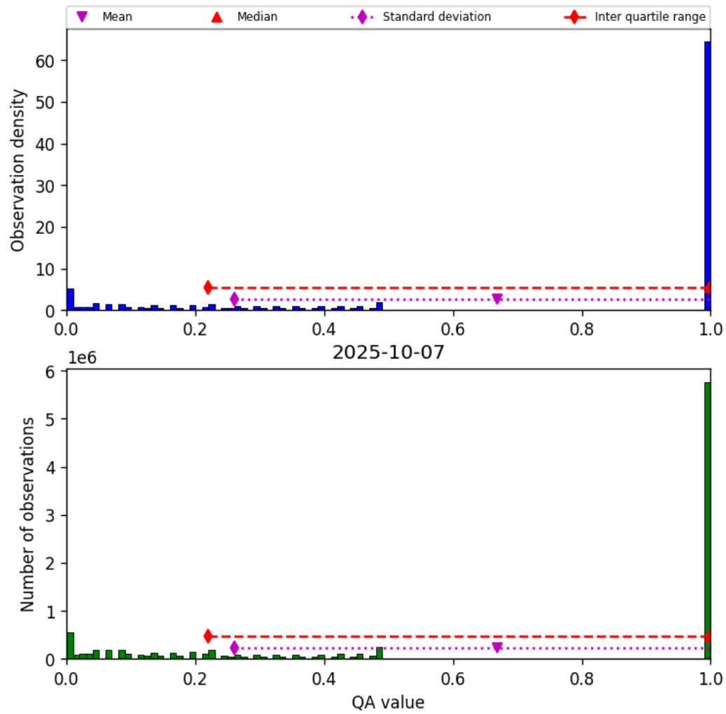
Figure 57: Histogram of “QA value” for 2025-10-07 to 2025-10-07
