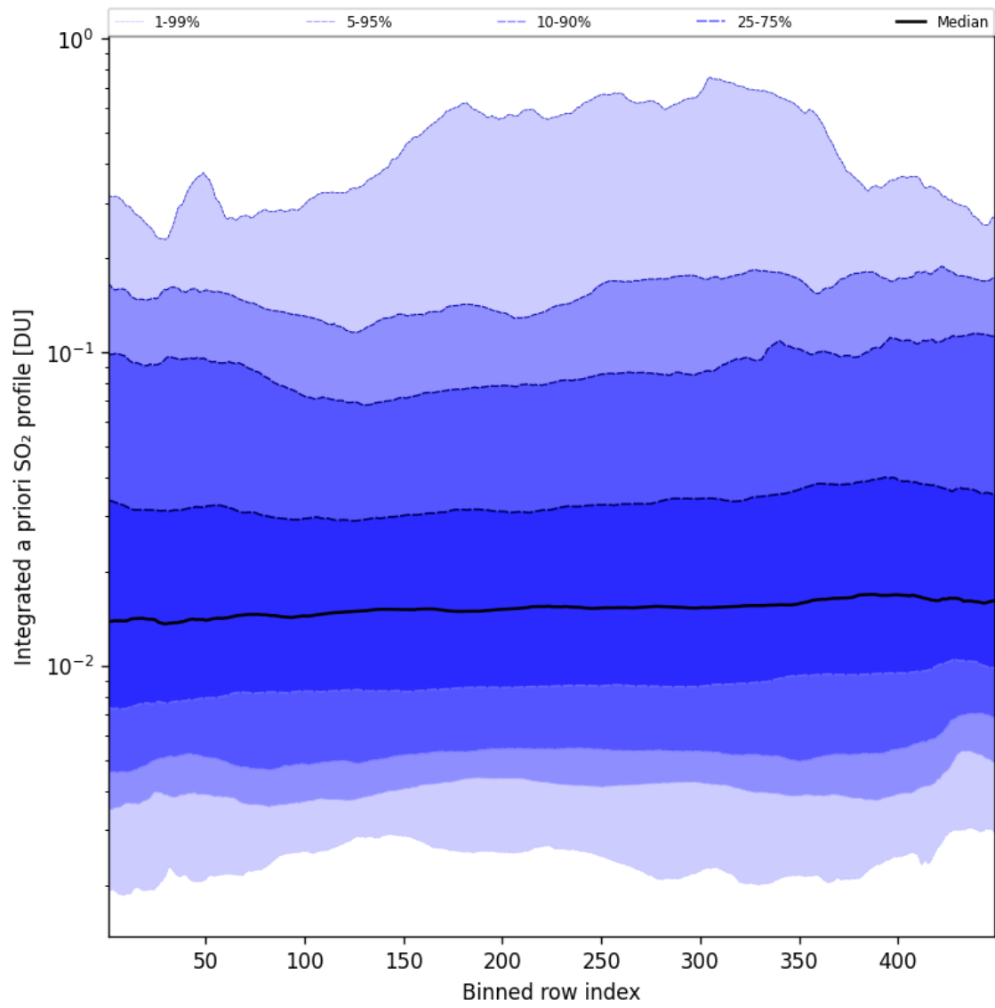
Figure 103: Along track statistics of “Integrated a priori SO 2 profile” for 2025-10-07 to 2025-10-07
