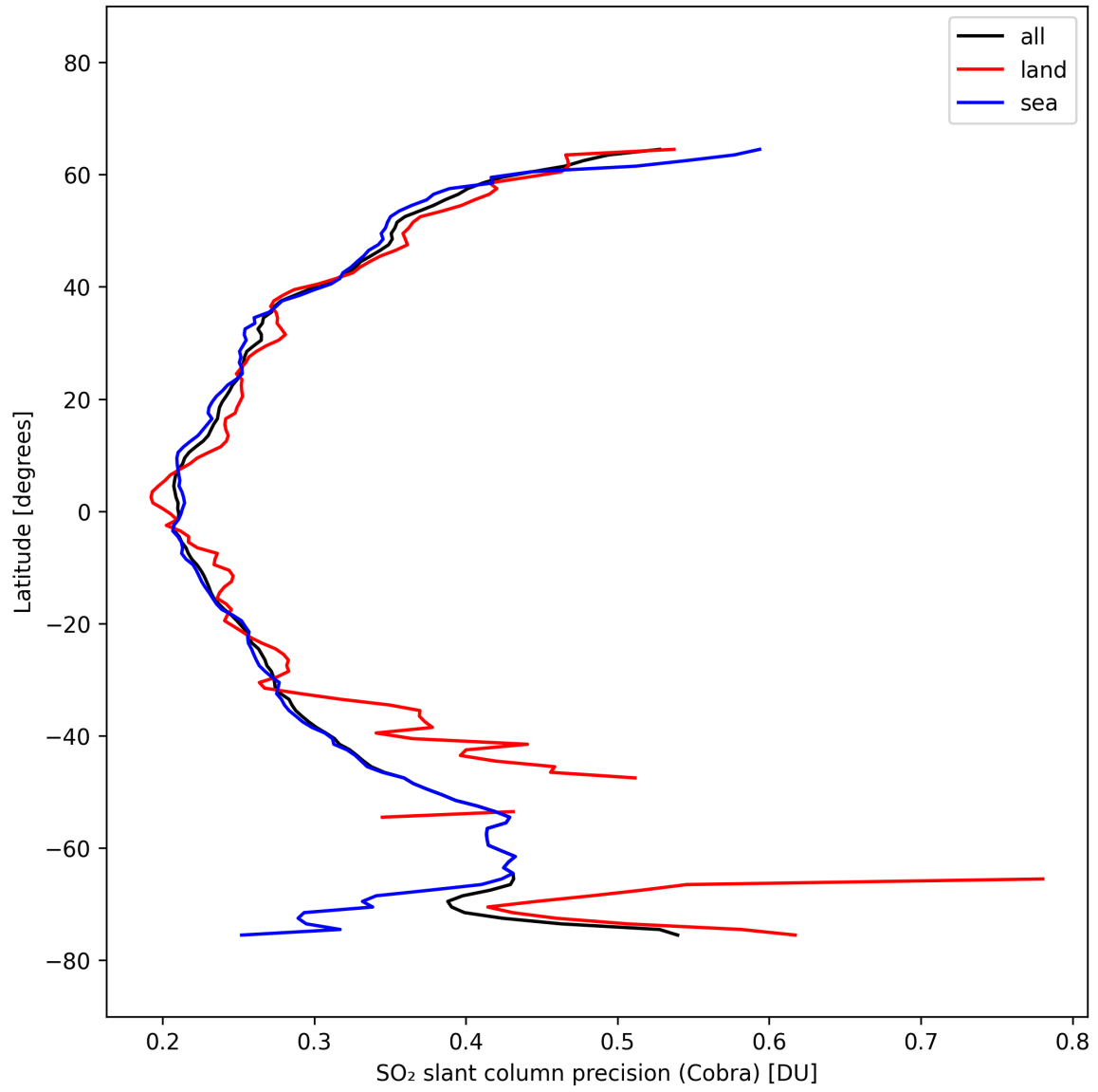
Figure 35: Zonal average of “SO 2 slant column precision (Cobra)” for 2025-10-07 to 2025-10-07.
