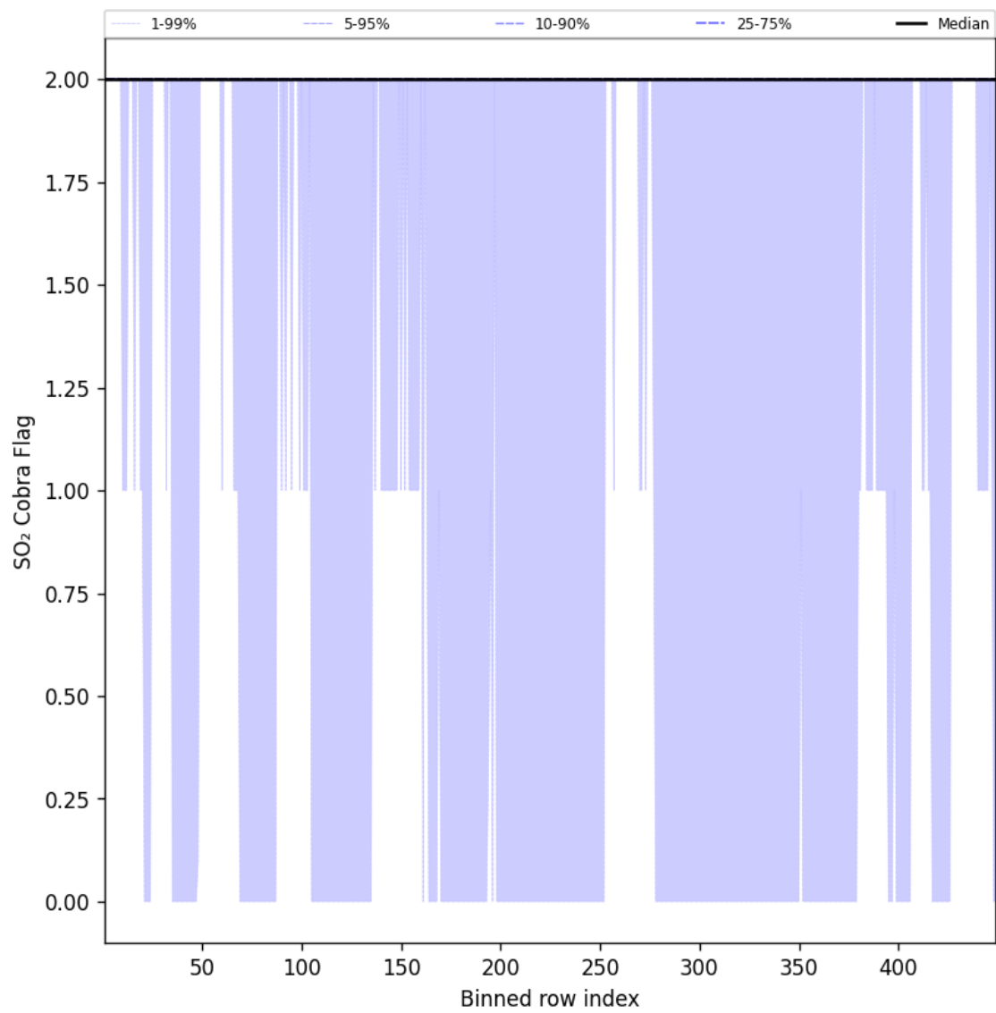
Figure 102: Along track statistics of “SO 2 Cobra Flag” for 2025-10-07 to 2025-10-07
