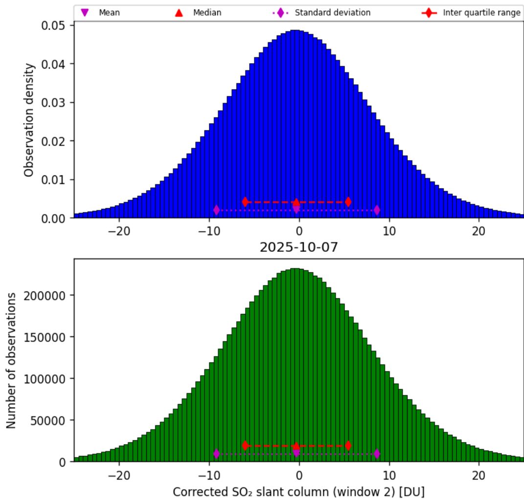
Figure 69: Histogram of “Corrected SO 2 slant column (window 2)” for 2025-10-07 to 2025-10-07
