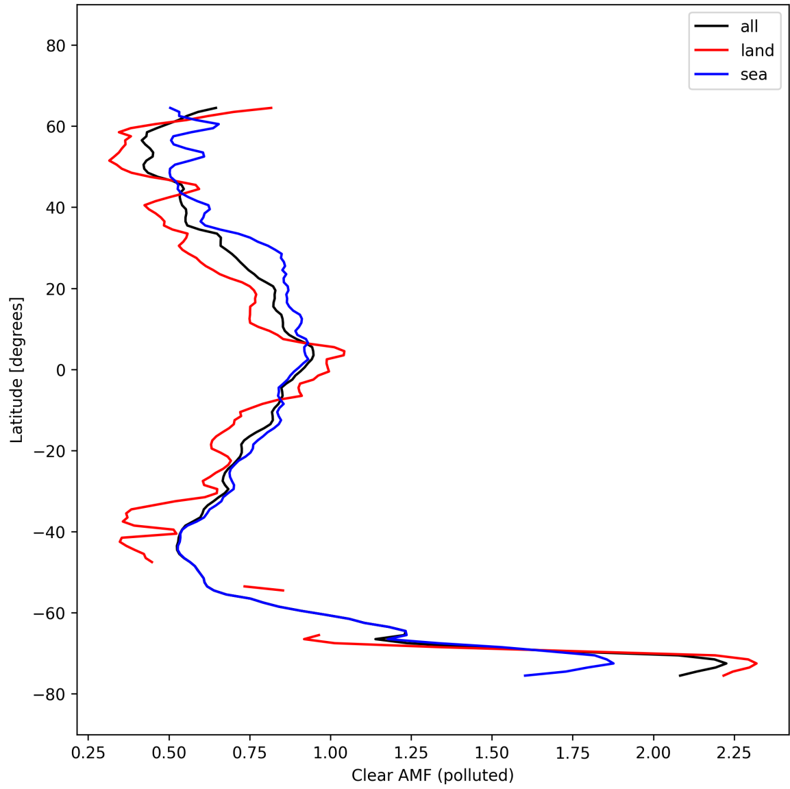
Figure 55: Zonal average of “Clear AMF (polluted)” for 2025-10-07 to 2025-10-07.
