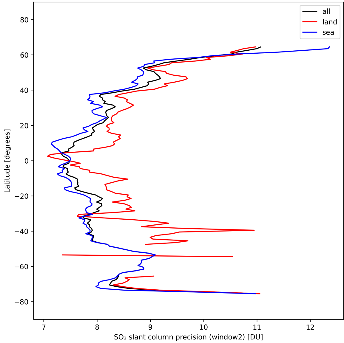
Figure 41: Zonal average of “SO 2 slant column precision (window2)” for 2025-10-07 to 2025-10-07.
