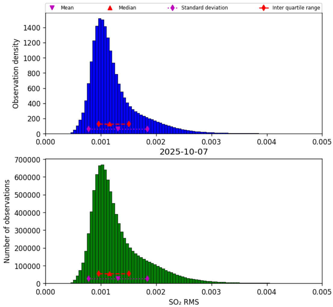
Figure 79: Histogram of “SO 2 RMS” for 2025-10-07 to 2025-10-07
