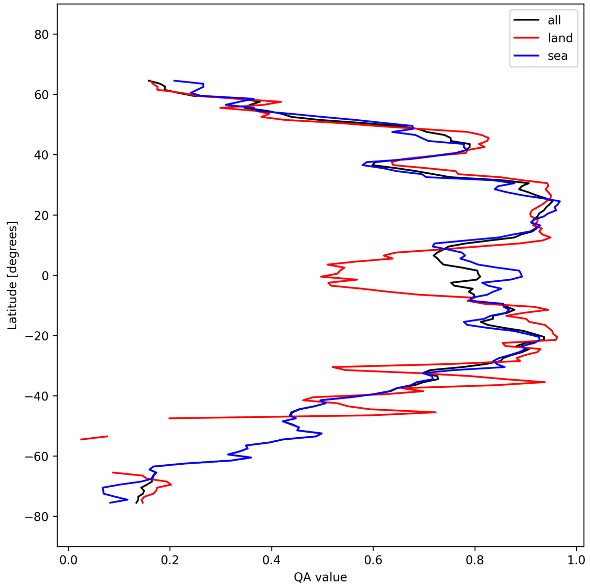
Figure 30: Zonal average of “QA value” for 2025-10-07 to 2025-10-07.
