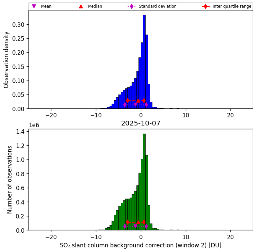
Figure 70: Histogram of “SO 2 slant column background correction (window 2)” for 2025-10-07 to 2025-10-07
