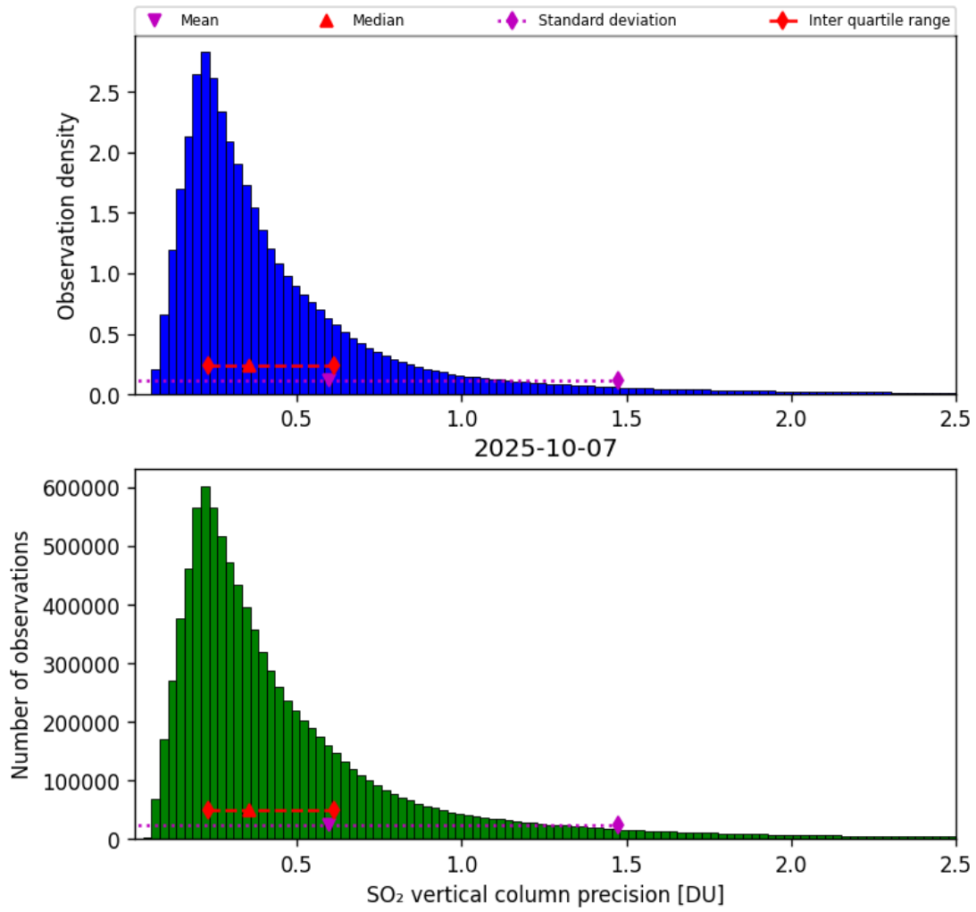
Figure 59: Histogram of “SO 2 vertical column precision” for 2025-10-07 to 2025-10-07
