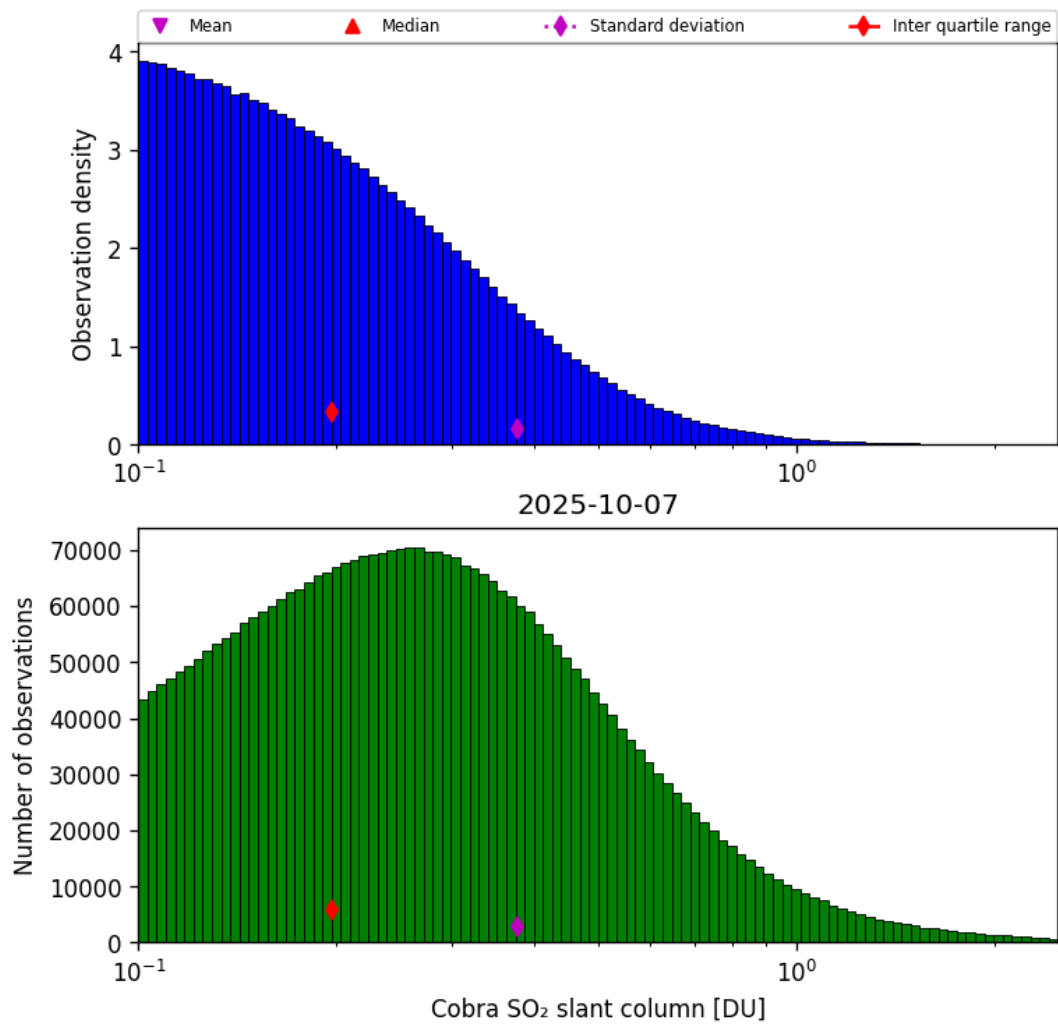
Figure 61: Histogram of “Cobra SO 2 slant column” for 2025-10-07 to 2025-10-07
