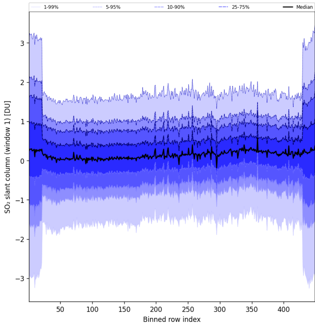
Figure 90: Along track statistics of “SO 2 slant column (window 1)” for 2025-10-07 to 2025-10-07
