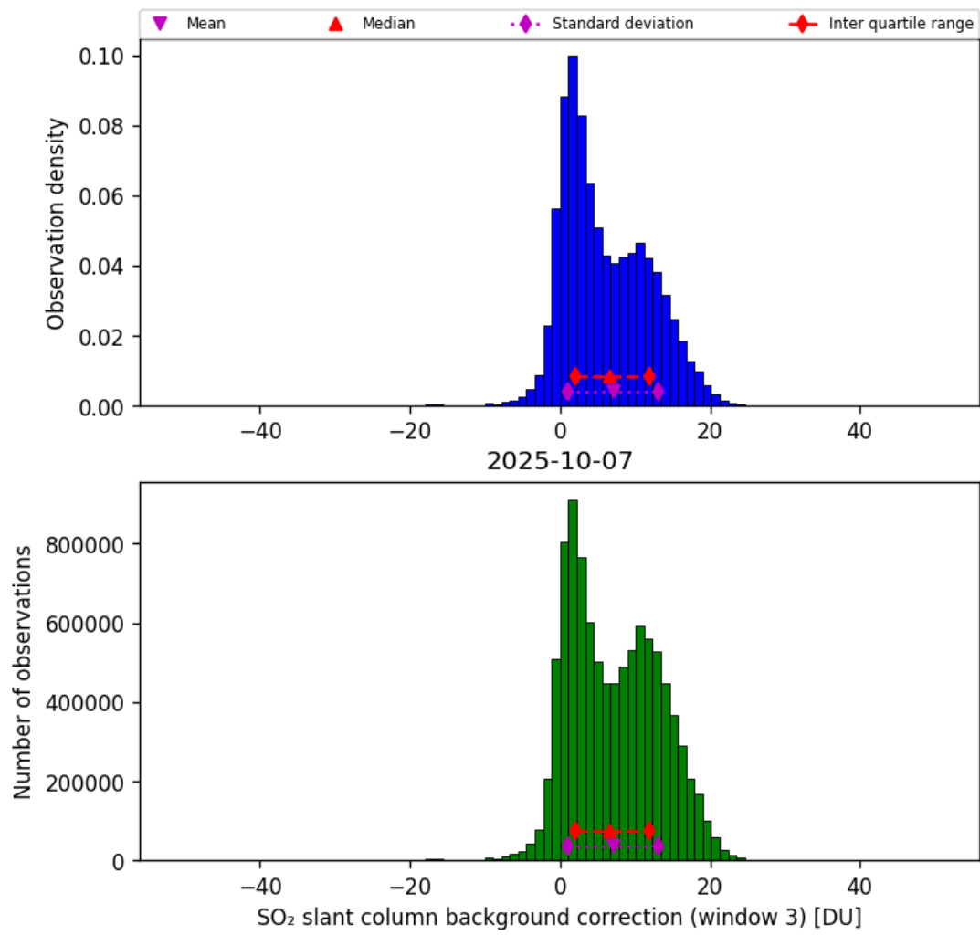
Figure 74: Histogram of “SO 2 slant column background correction (window 3)” for 2025-10-07 to 2025-10-07
