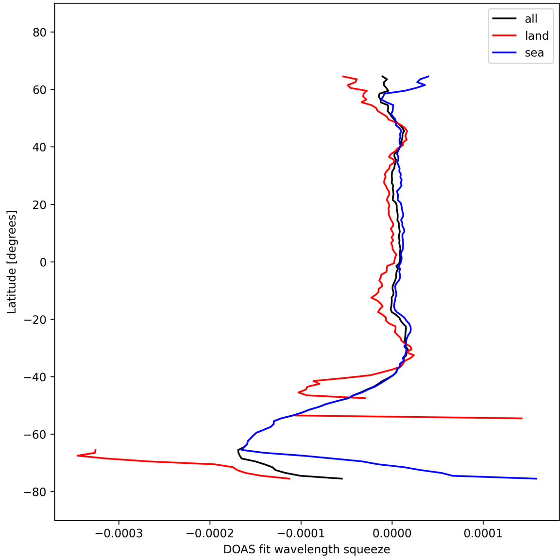
Figure 51: Zonal average of “DOAS fit wavelength squeeze” for 2025-10-07 to 2025-10-07.
