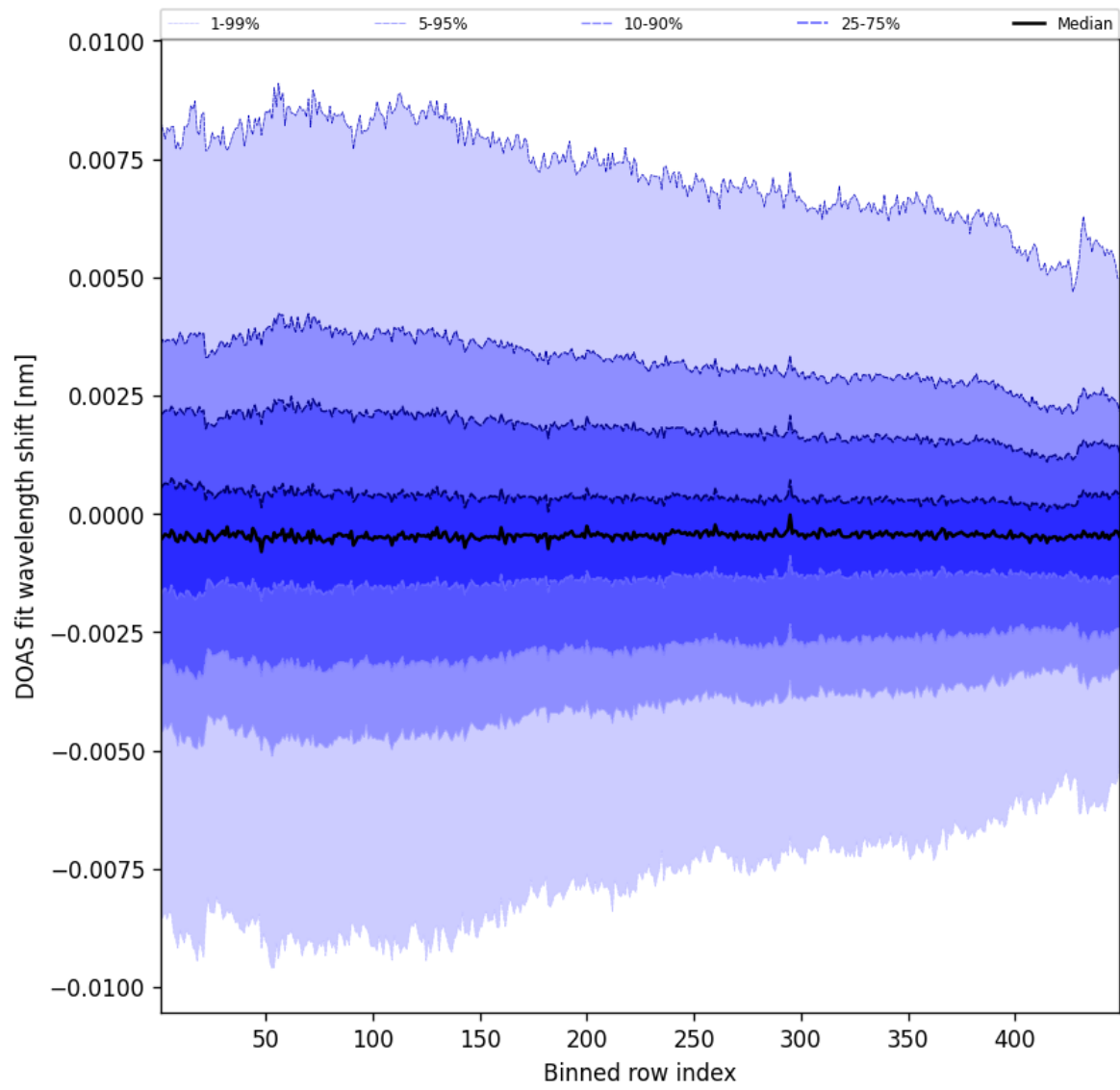
Figure 104: Along track statistics of “DOAS fit wavelength shift” for 2025-10-07 to 2025-10-07
