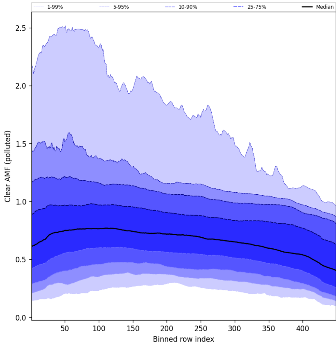
Figure 109: Along track statistics of “Clear AMF (polluted)” for 2025-10-07 to 2025-10-07
