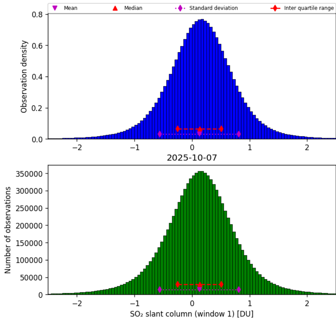
Figure 63: Histogram of “SO 2 slant column (window 1)” for 2025-10-07 to 2025-10-07
