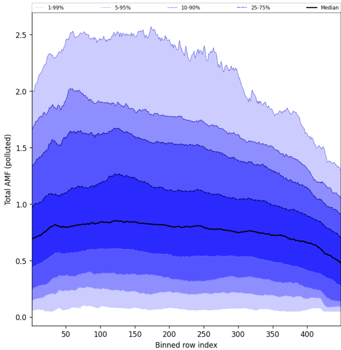
Figure 107: Along track statistics of “Total AMF (polluted)” for 2025-10-07 to 2025-10-07
