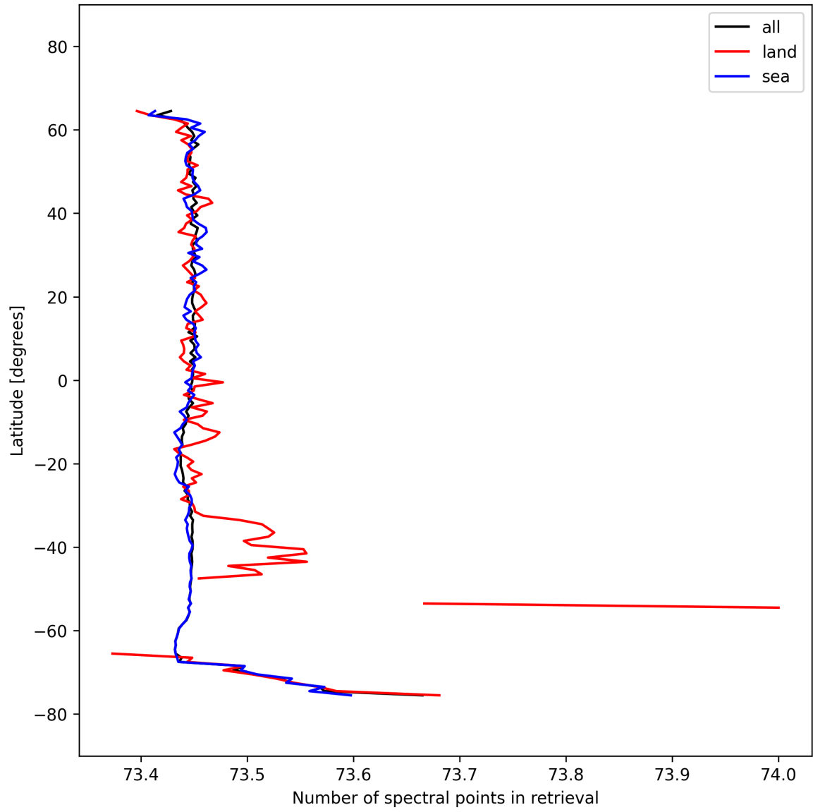
Figure 56: Zonal average of “Number of spectral points in retrieval” for 2025-10-07 to 2025-10-07.
