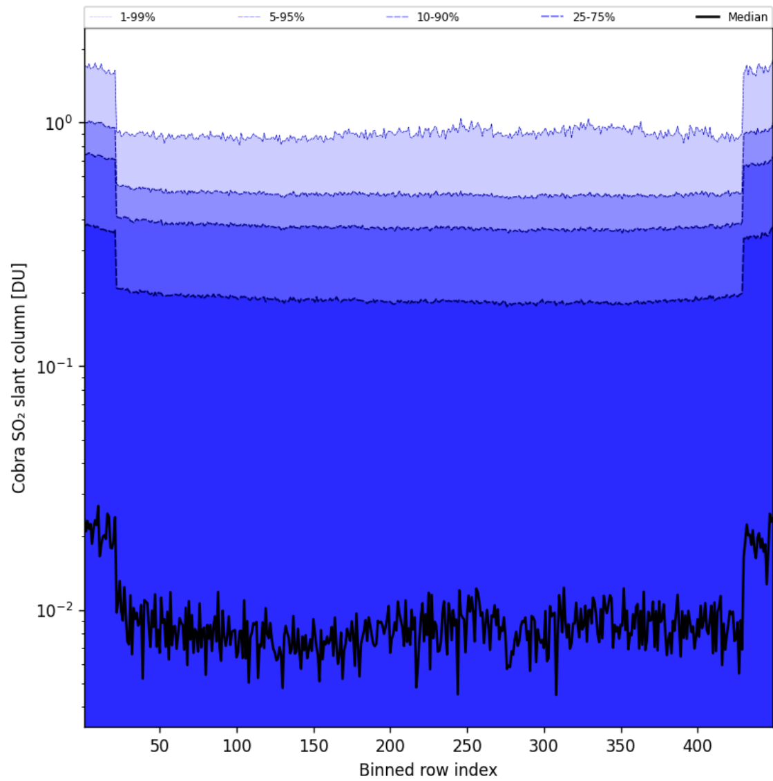
Figure 88: Along track statistics of “Cobra SO 2 slant column” for 2025-10-07 to 2025-10-07
