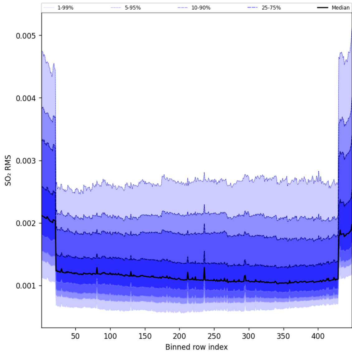
Figure 106: Along track statistics of “SO 2 RMS” for 2025-10-07 to 2025-10-07
