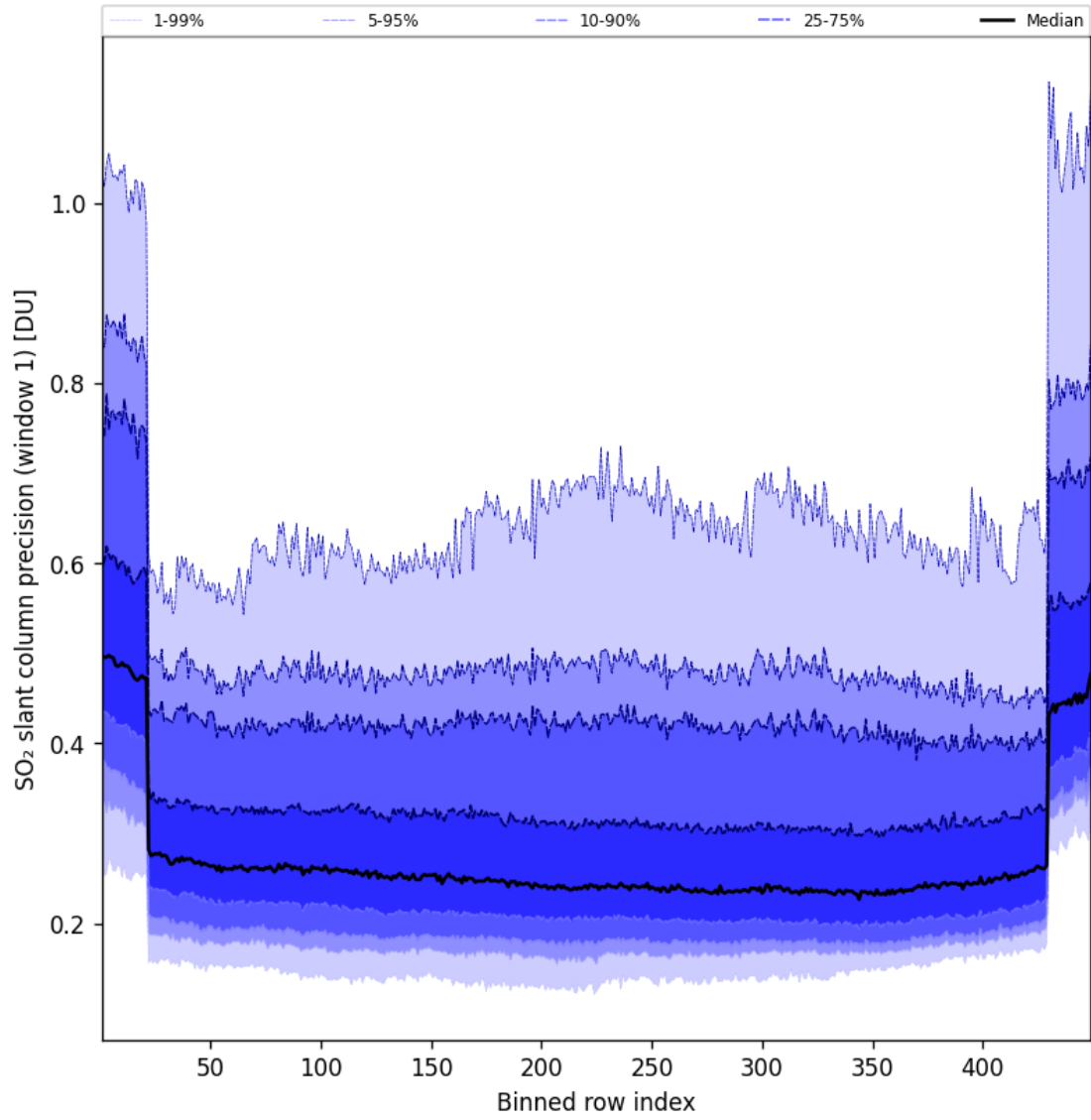
Figure 91: Along track statistics of “SO 2 slant column precision (window 1)” for 2025-10-07 to 2025-10-07
