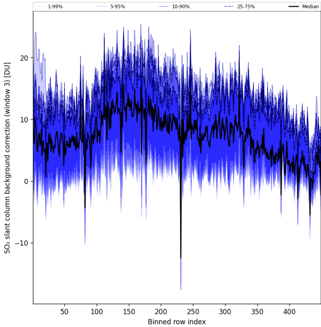
Figure 101: Along track statistics of “SO 2 slant column background correction (window 3)” for 2025-10-07 to 2025-10-07
