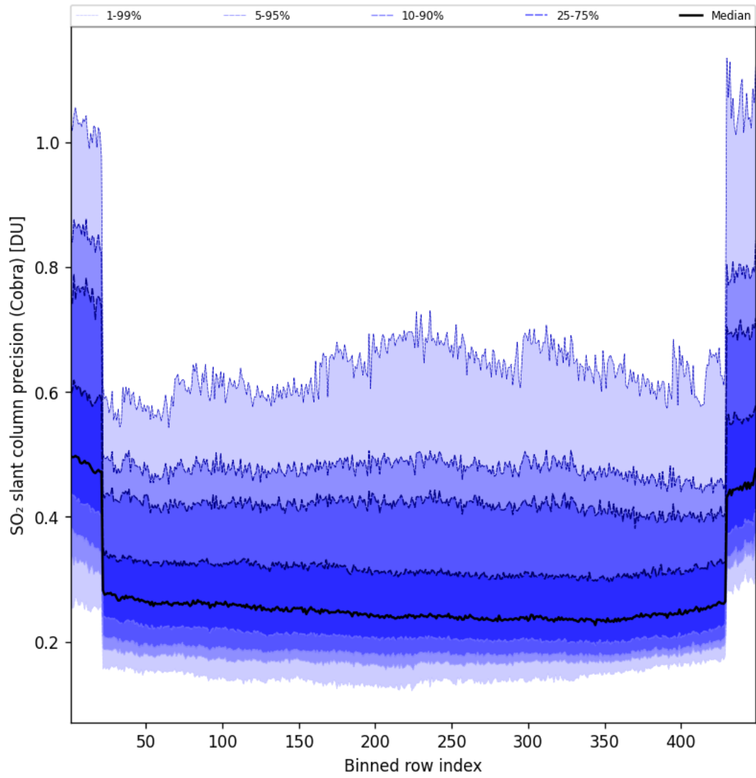
Figure 89: Along track statistics of “SO 2 slant column precision (Cobra)” for 2025-10-07 to 2025-10-07
