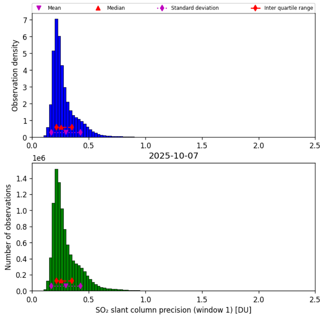
Figure 64: Histogram of “SO 2 slant column precision (window 1)” for 2025-10-07 to 2025-10-07
