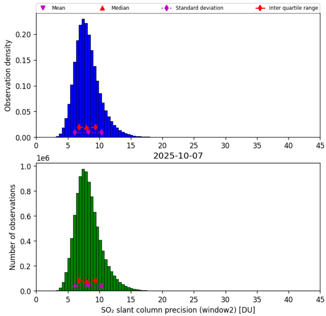
Figure 68: Histogram of “SO 2 slant column precision (window2)” for 2025-10-07 to 2025-10-07
