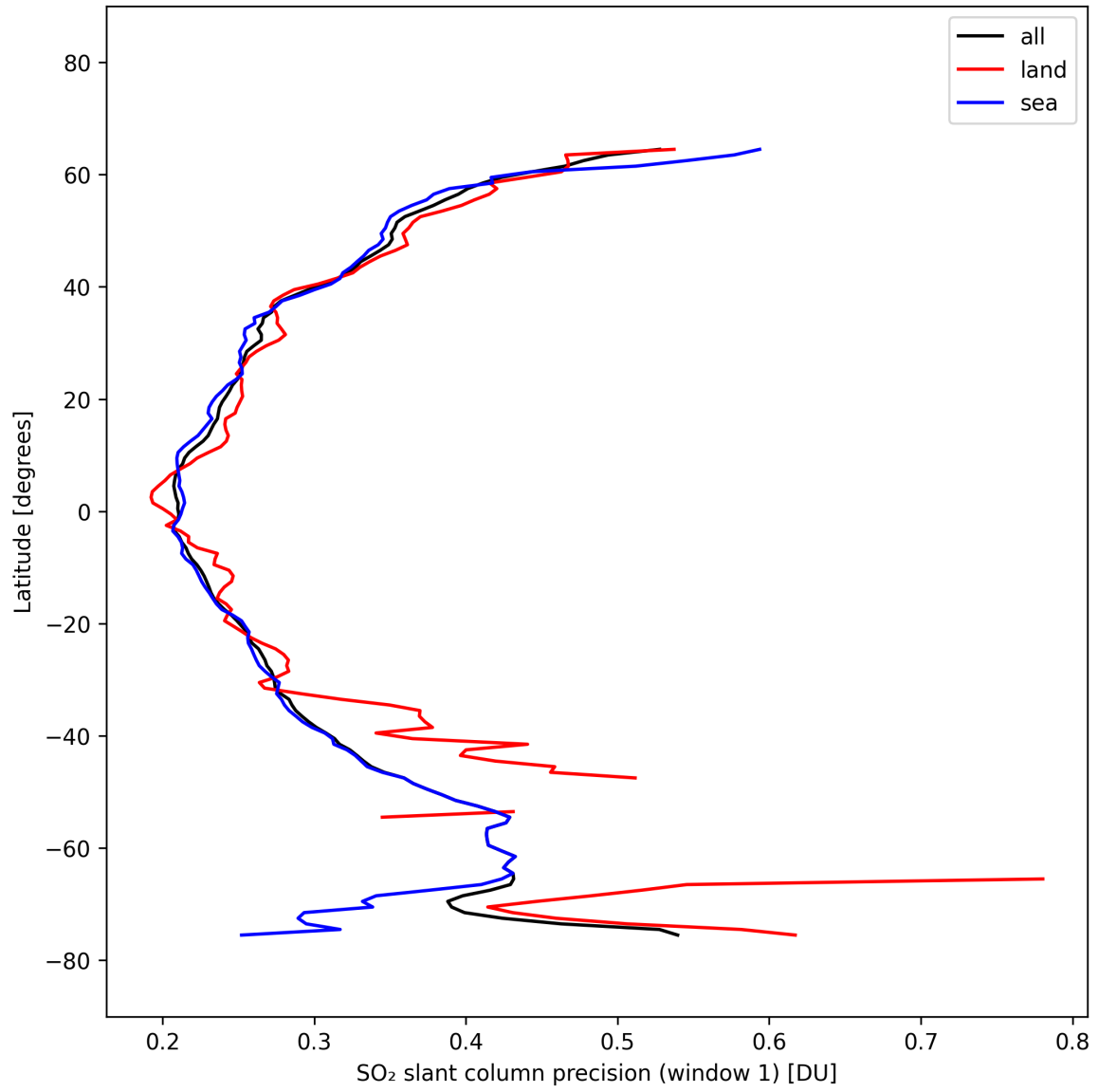
Figure 37: Zonal average of “SO 2 slant column precision (window 1)” for 2025-10-07 to 2025-10-07.
