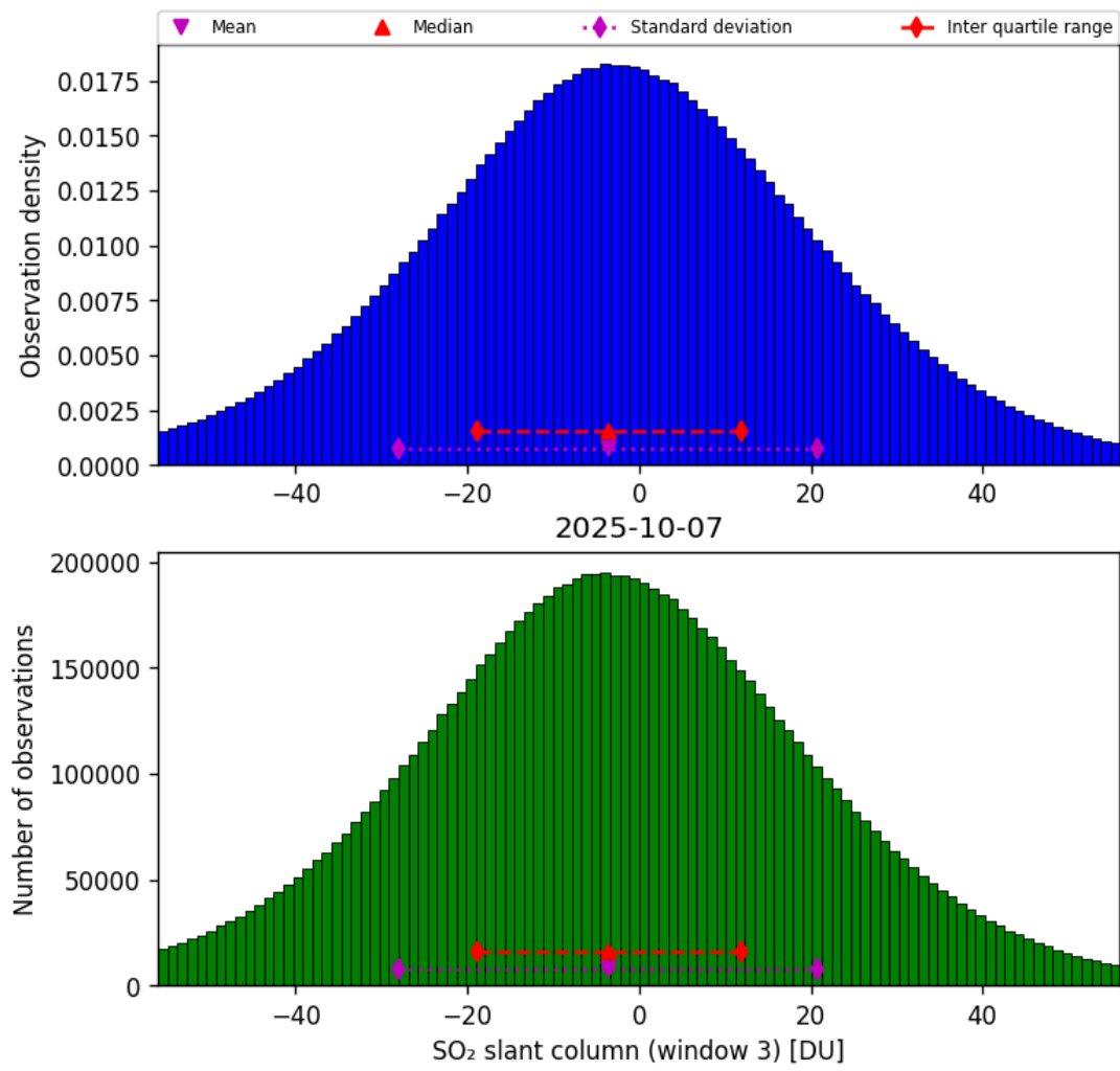
Figure 71: Histogram of “SO 2 slant column (window 3)” for 2025-10-07 to 2025-10-07
