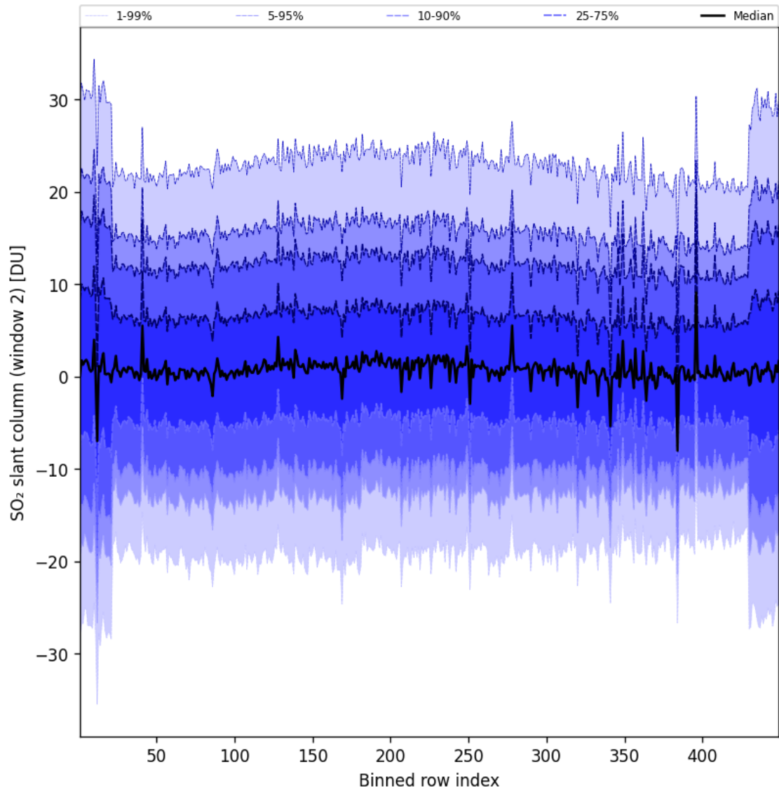
Figure 94: Along track statistics of “SO 2 slant column (window 2)” for 2025-10-07 to 2025-10-07
