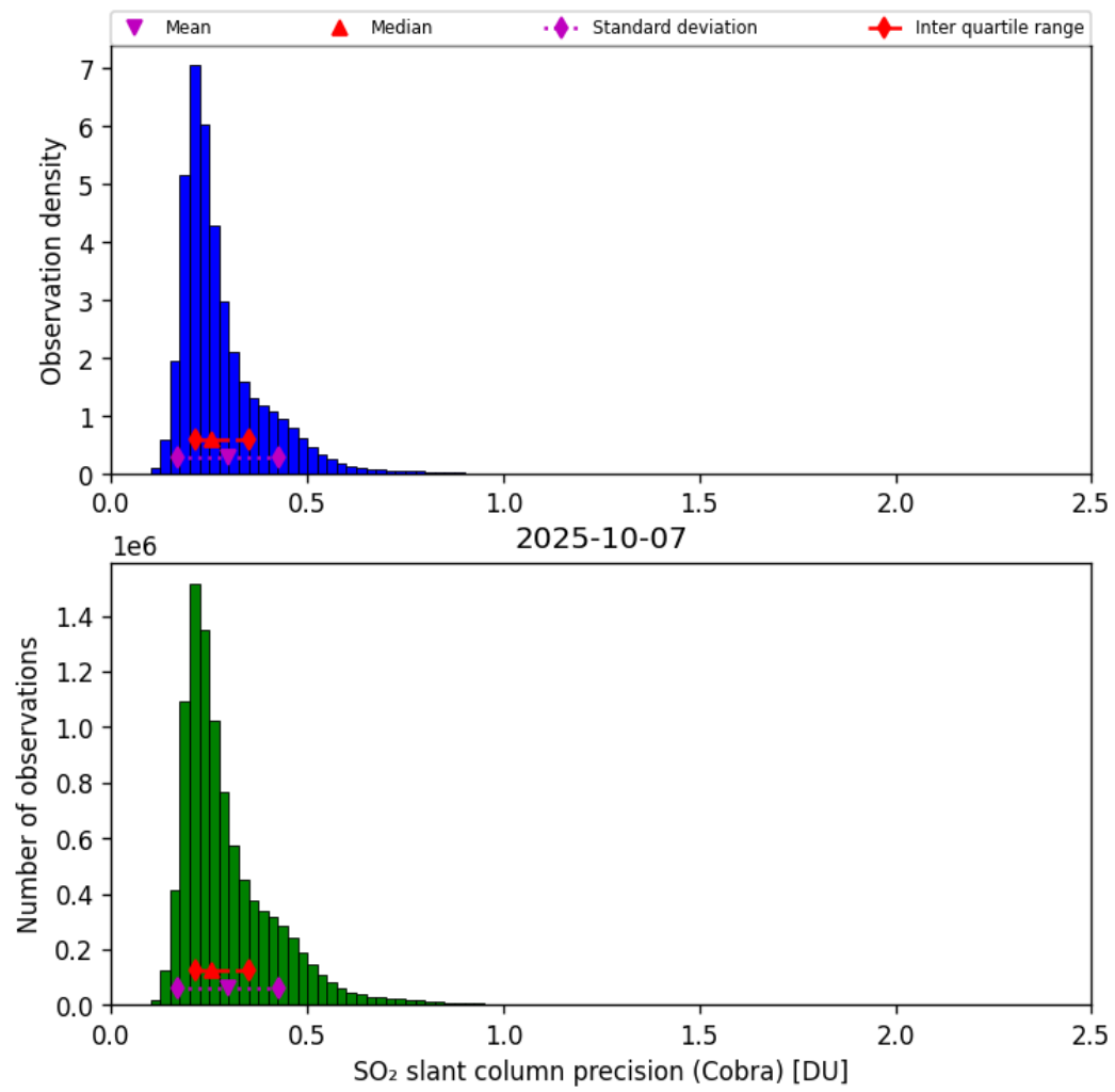
Figure 62: Histogram of “SO 2 slant column precision (Cobra)” for 2025-10-07 to 2025-10-07
