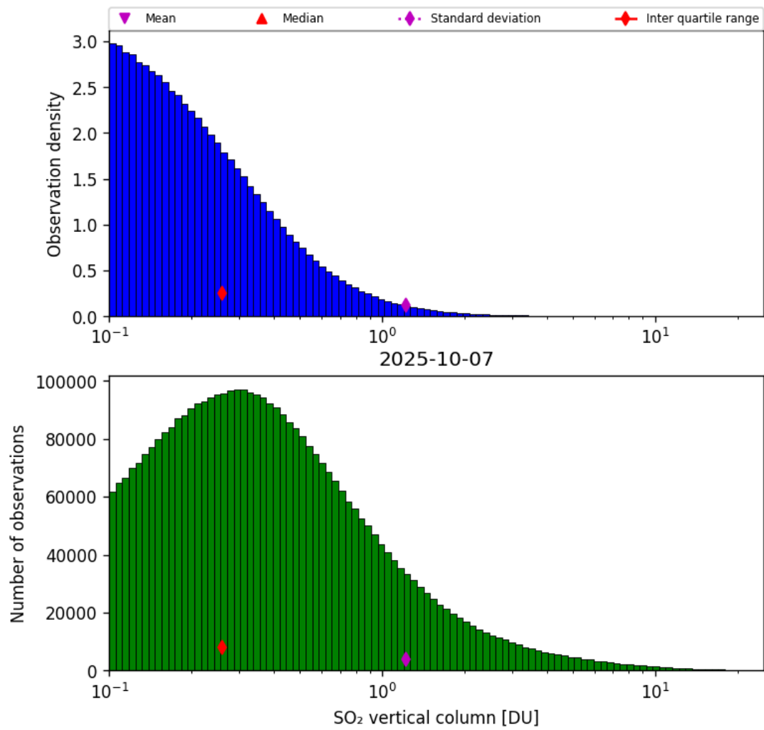
Figure 58: Histogram of “SO 2 vertical column” for 2025-10-07 to 2025-10-07
