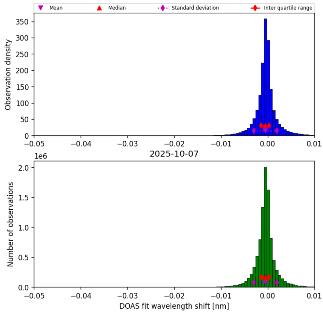
Figure 77: Histogram of “DOAS fit wavelength shift” for 2025-10-07 to 2025-10-07
