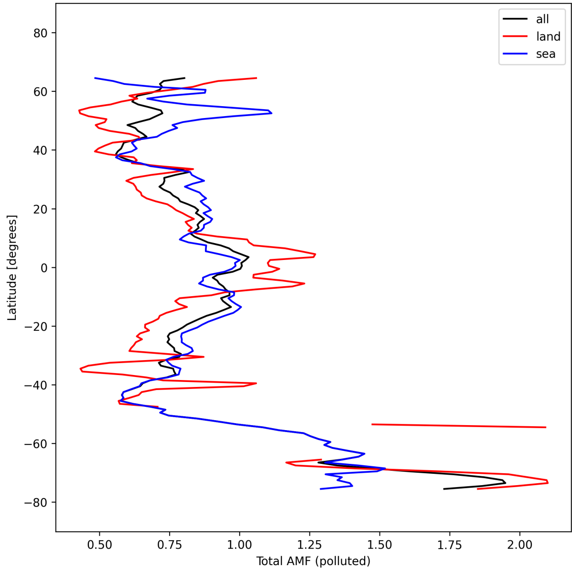
Figure 53: Zonal average of “Total AMF (polluted)” for 2025-10-07 to 2025-10-07.
