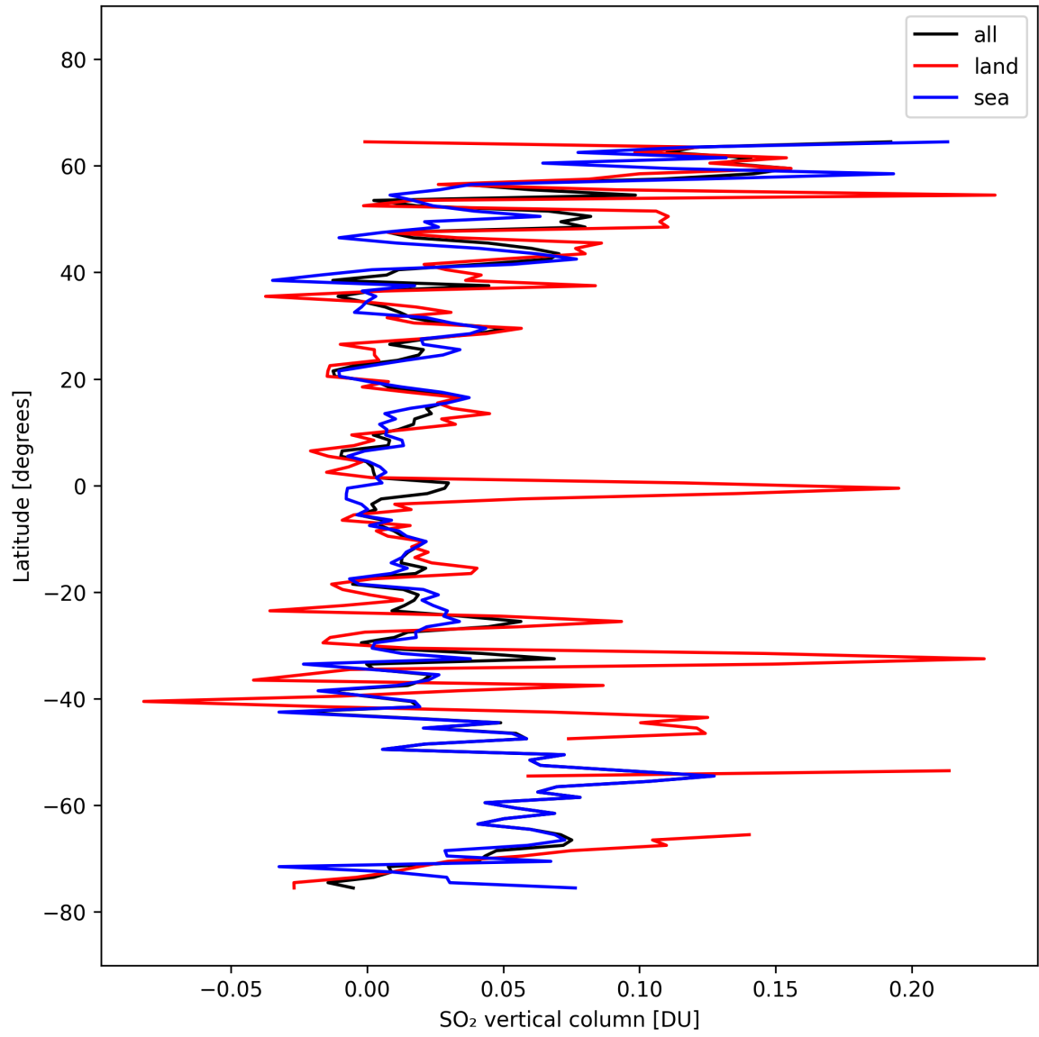
Figure 31: Zonal average of “SO 2 vertical column” for 2025-10-07 to 2025-10-07.
