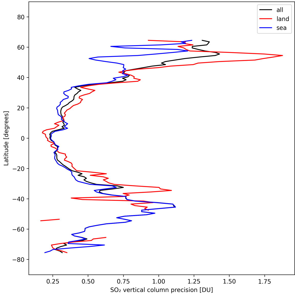
Figure 32: Zonal average of “SO 2 vertical column precision” for 2025-10-07 to 2025-10-07.
