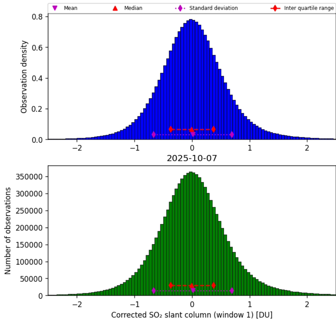
Figure 65: Histogram of “Corrected SO 2 slant column (window 1)” for 2025-10-07 to 2025-10-07
