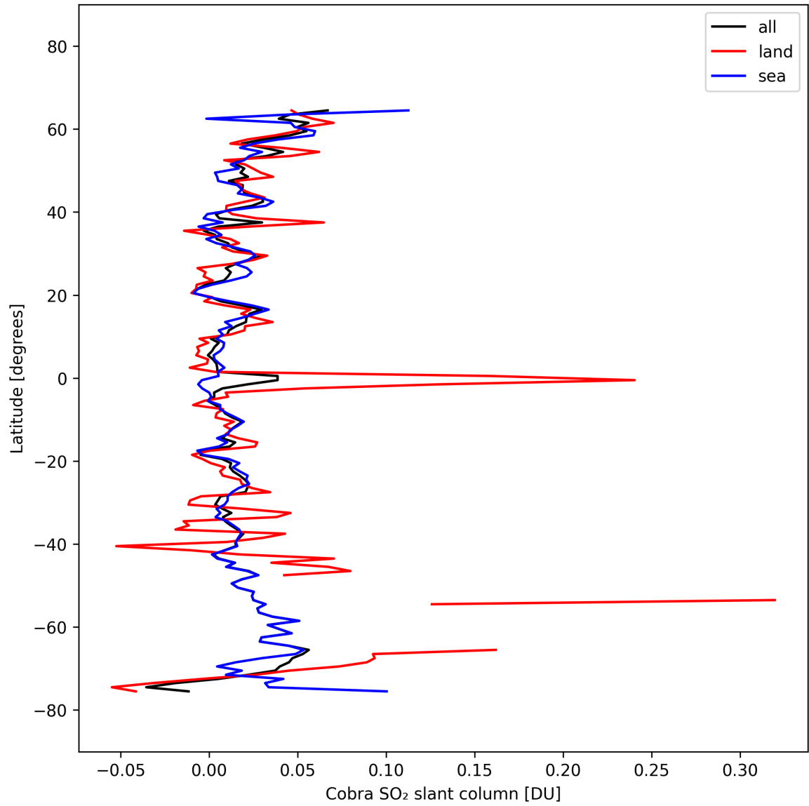
Figure 34: Zonal average of “Cobra SO 2 slant column” for 2025-10-07 to 2025-10-07.
