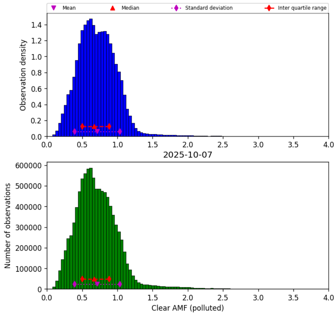
Figure 82: Histogram of “Clear AMF (polluted)” for 2025-10-07 to 2025-10-07
