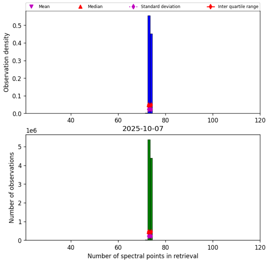
Figure 83: Histogram of “Number of spectral points in retrieval” for 2025-10-07 to 2025-10-07
