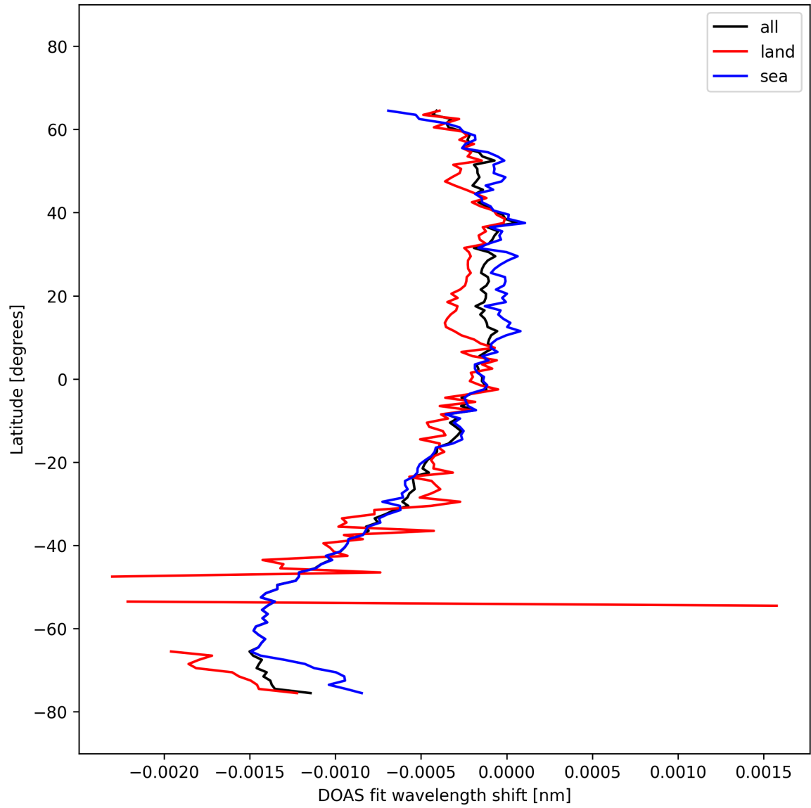
Figure 50: Zonal average of "DOAS fit wavelength shift" for 2025-10-07 to 2025-10-07.
