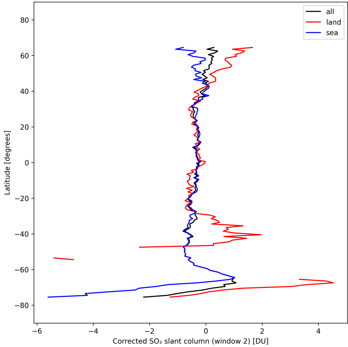
Figure 42: Zonal average of “Corrected SO 2 slant column (window 2)” for 2025-10-07 to 2025-10-07.
