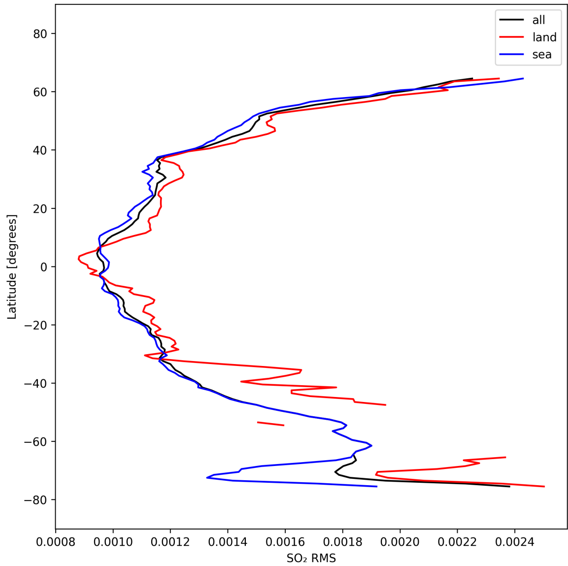
Figure 52: Zonal average of “SO 2 RMS” for 2025-10-07 to 2025-10-07.
