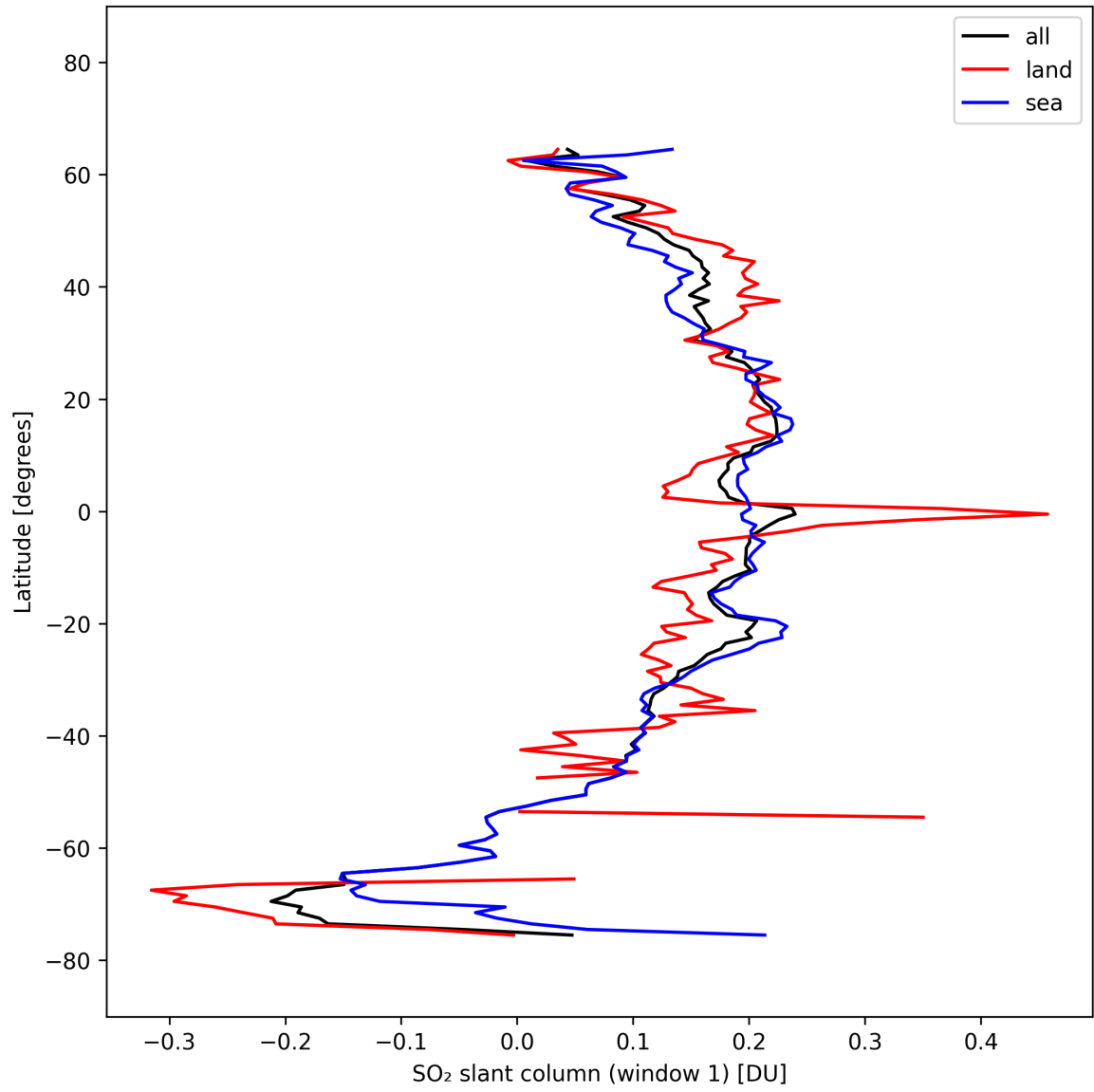
Figure 36: Zonal average of “SO 2 slant column (window 1)” for 2025-10-07 to 2025-10-07.
