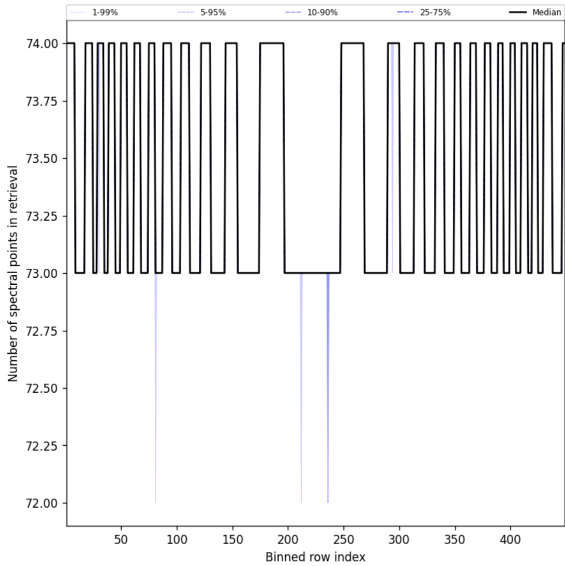
Figure 110: Along track statistics of “Number of spectral points in retrieval” for 2025-10-07 to 2025-10-07
