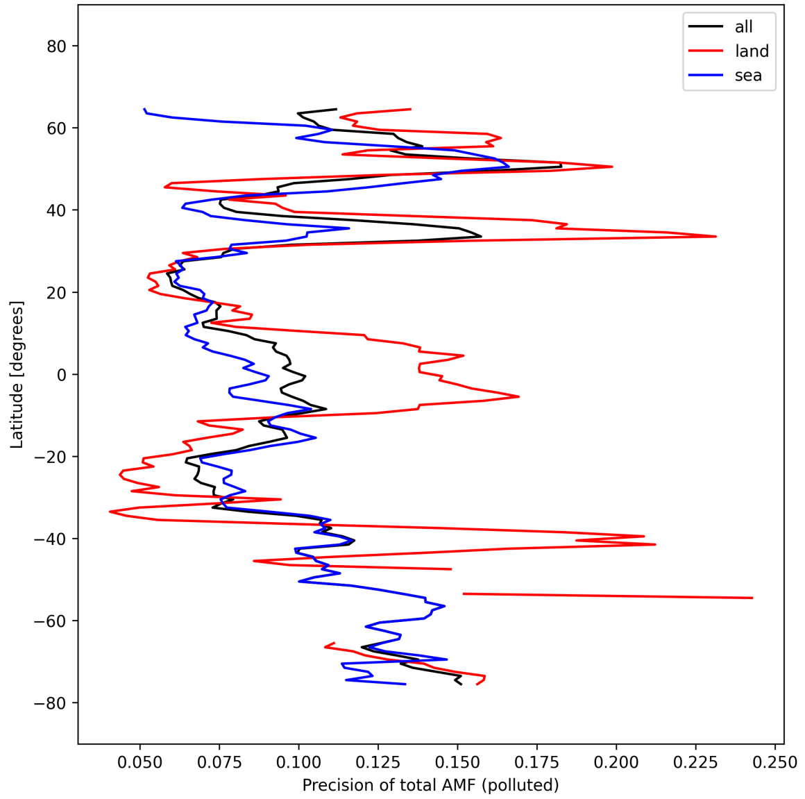
Figure 54: Zonal average of “Precision of total AMF (polluted)” for 2025-10-07 to 2025-10-07.
