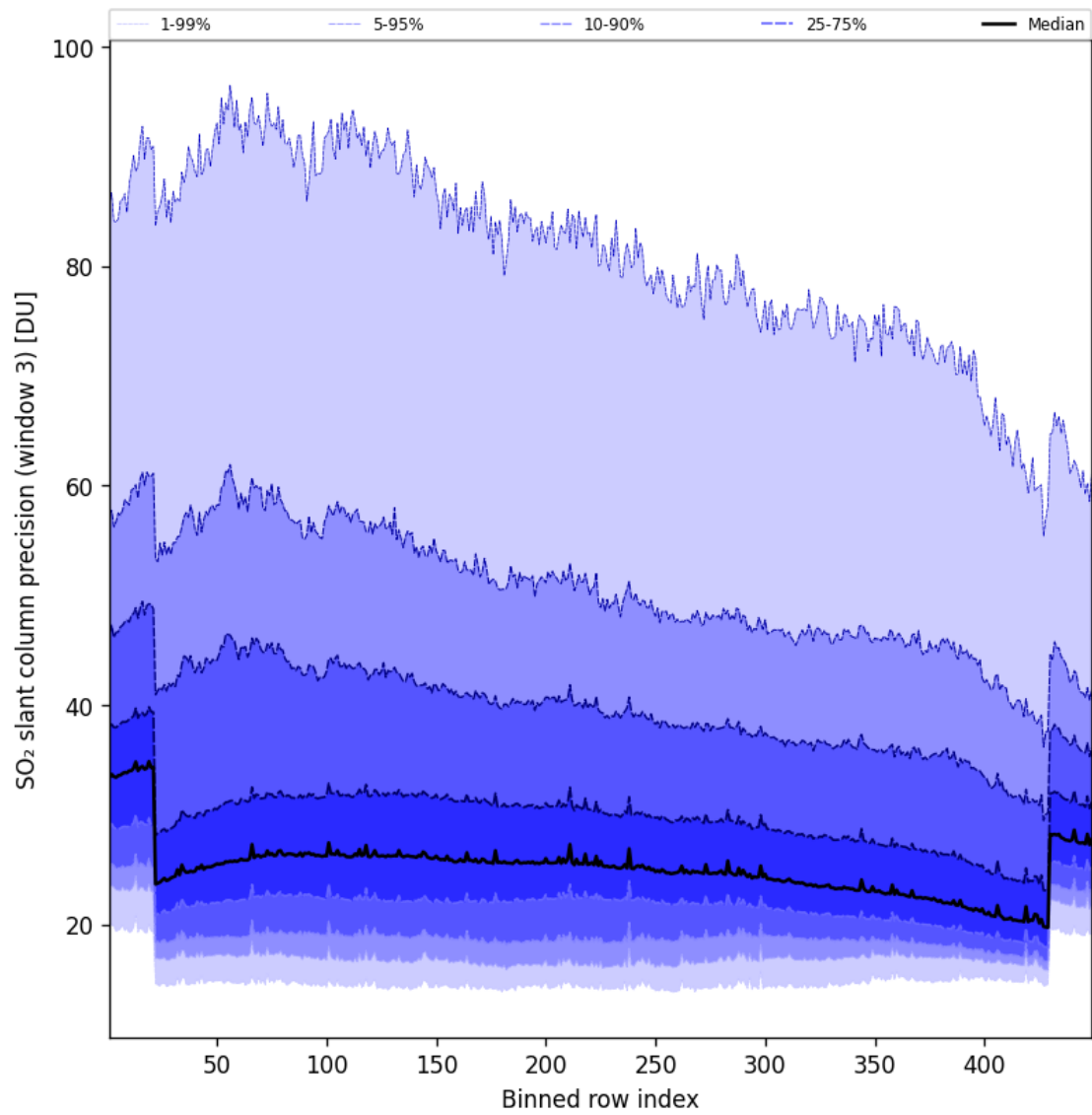
Figure 99: Along track statistics of “SO 2 slant column precision (window 3)” for 2025-10-07 to 2025-10-07
