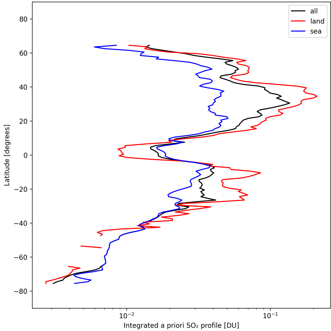
Figure 49: Zonal average of “Integrated a priori SO 2 profile” for 2025-10-07 to 2025-10-07.
