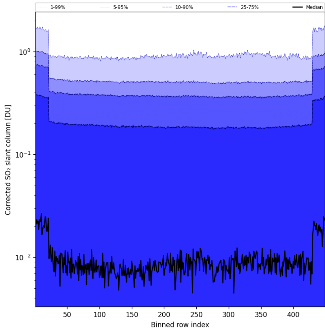
Figure 87: Along track statistics of "Corrected SO 2 slant column" for 2025-10-07 to 2025-10-07
