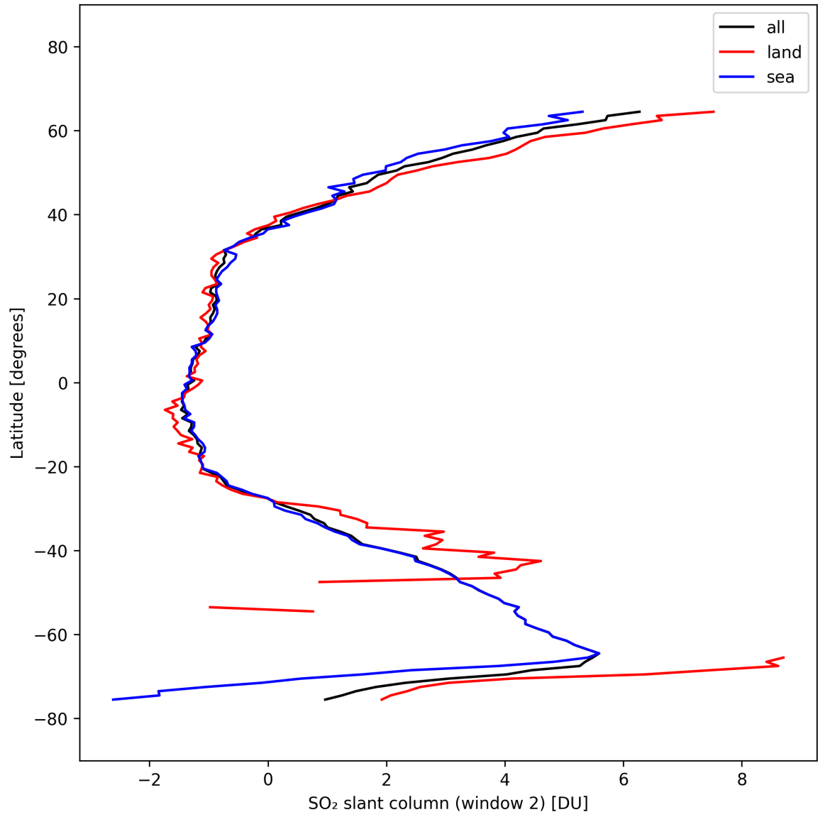
Figure 40: Zonal average of “SO 2 slant column (window 2)” for 2025-10-07 to 2025-10-07.
