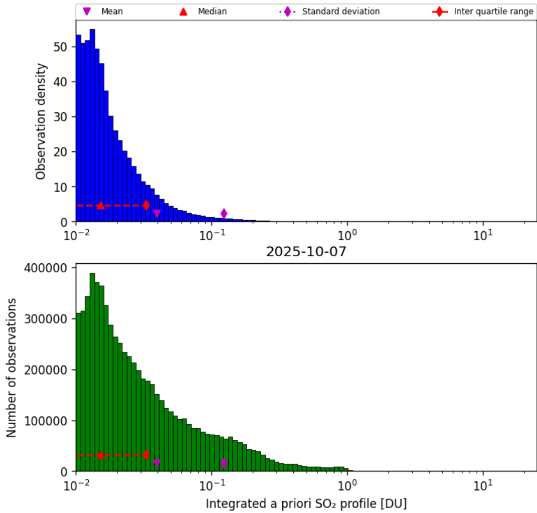
Figure 76: Histogram of “Integrated a priori SO 2 profile” for 2025-10-07 to 2025-10-07
