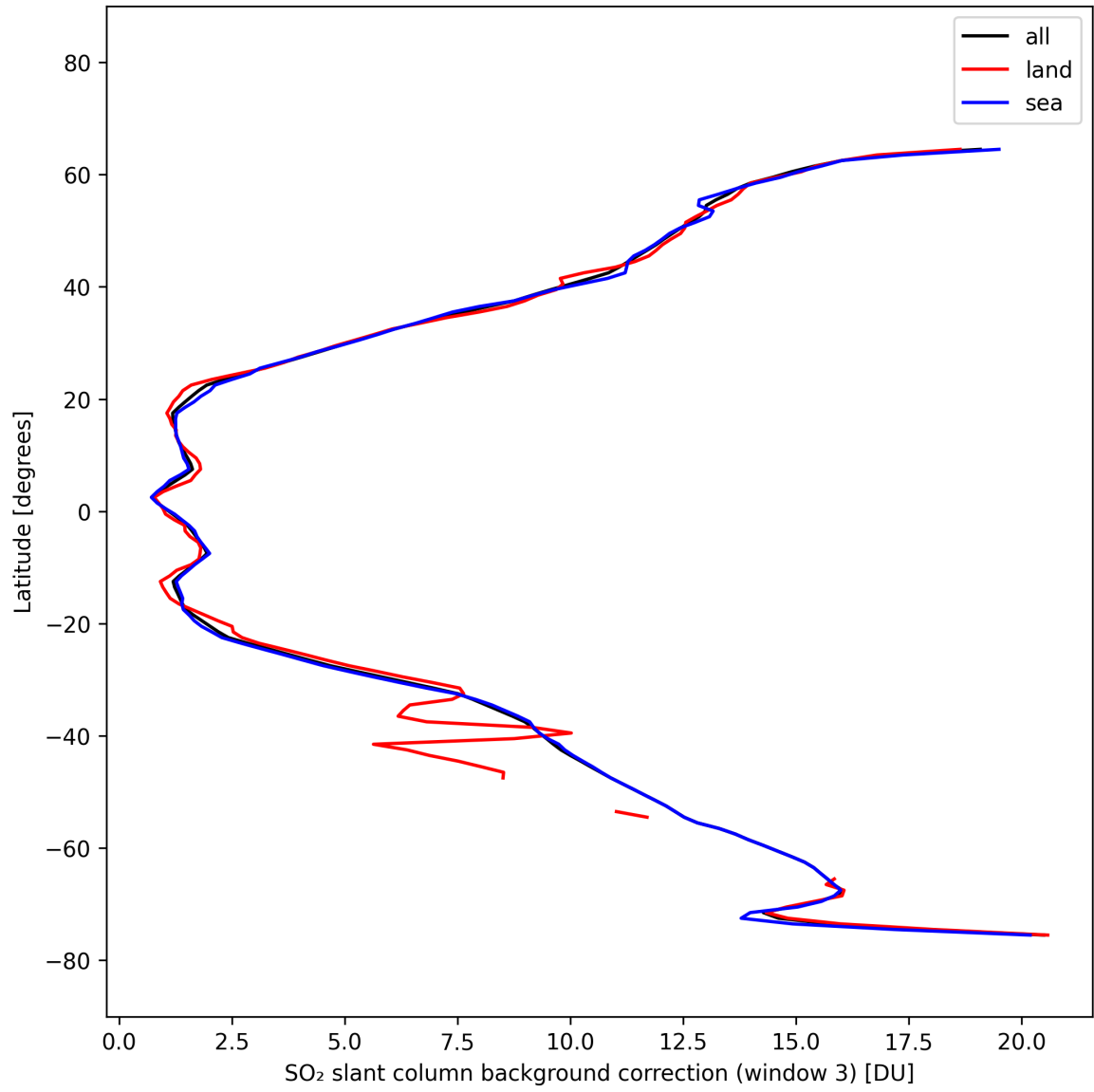
Figure 47: Zonal average of “SO 2 slant column background correction (window 3)” for 2025-10-07 to 2025-10-07.
