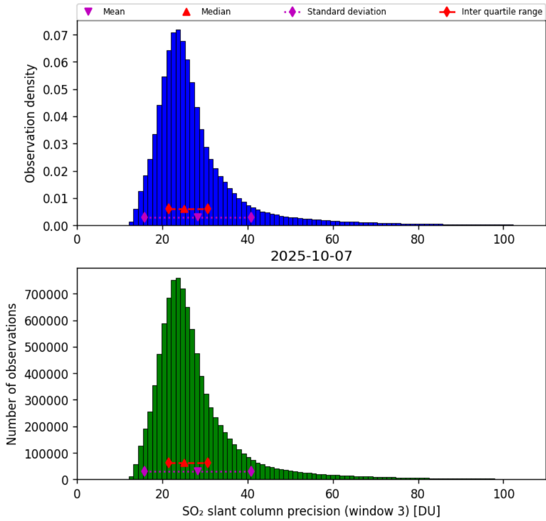
Figure 72: Histogram of “SO 2 slant column precision (window 3)” for 2025-10-07 to 2025-10-07
