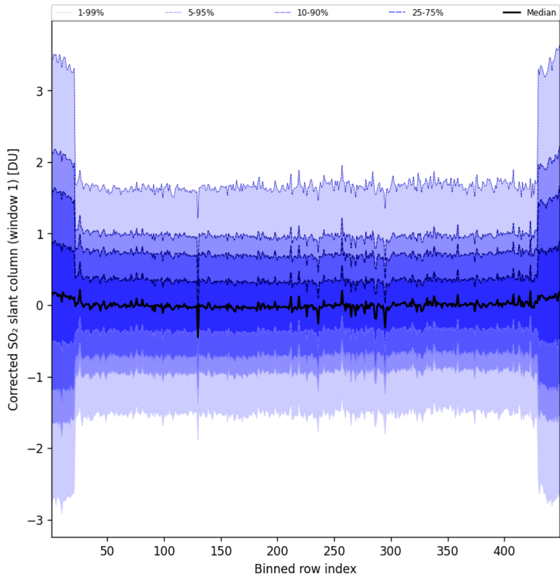
Figure 92: Along track statistics of “Corrected SO 2 slant column (window 1)” for 2025-10-07 to 2025-10-07
