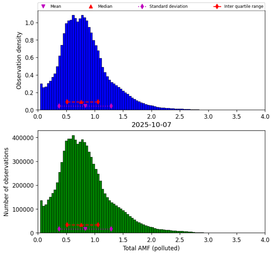
Figure 80: Histogram of “Total AMF (polluted)” for 2025-10-07 to 2025-10-07
