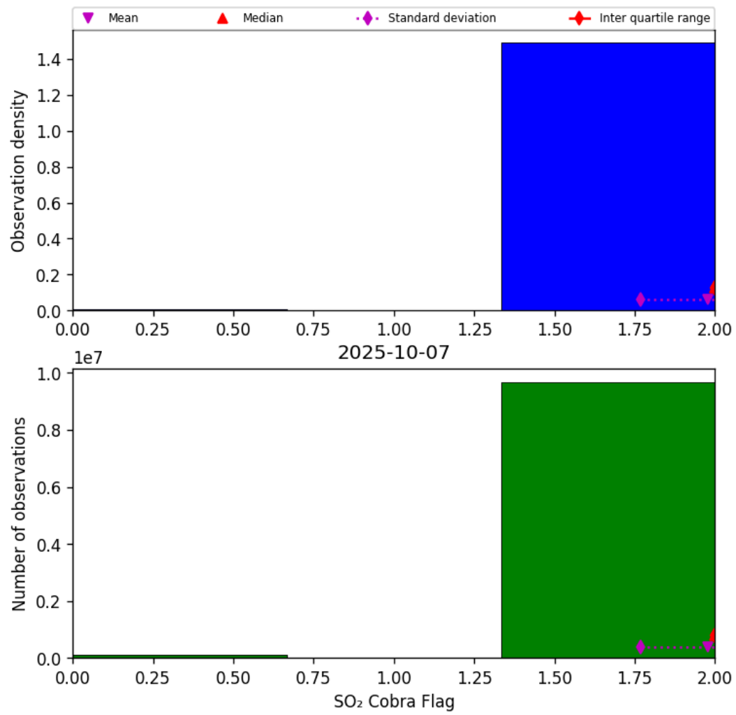
Figure 75: Histogram of “SO 2 Cobra Flag” for 2025-10-07 to 2025-10-07
