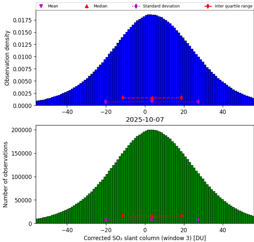
Figure 73: Histogram of “Corrected SO 2 slant column (window 3)” for 2025-10-07 to 2025-10-07
