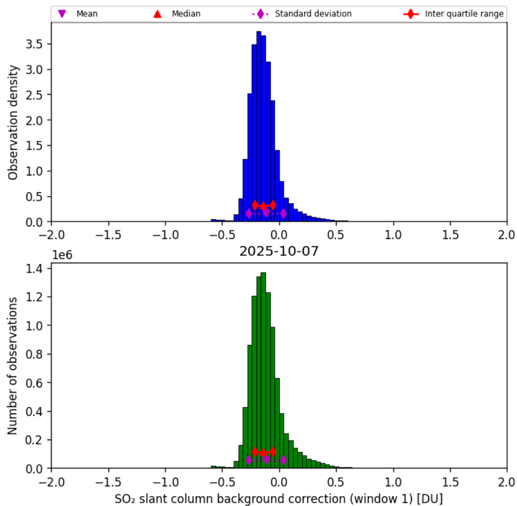
Figure 66: Histogram of “SO 2 slant column background correction (window 1)” for 2025-10-07 to 2025-10-07
