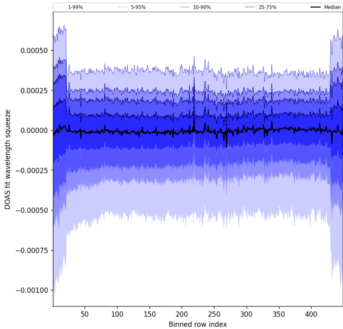
Figure 105: Along track statistics of “DOAS fit wavelength squeeze” for 2025-10-07 to 2025-10-07
