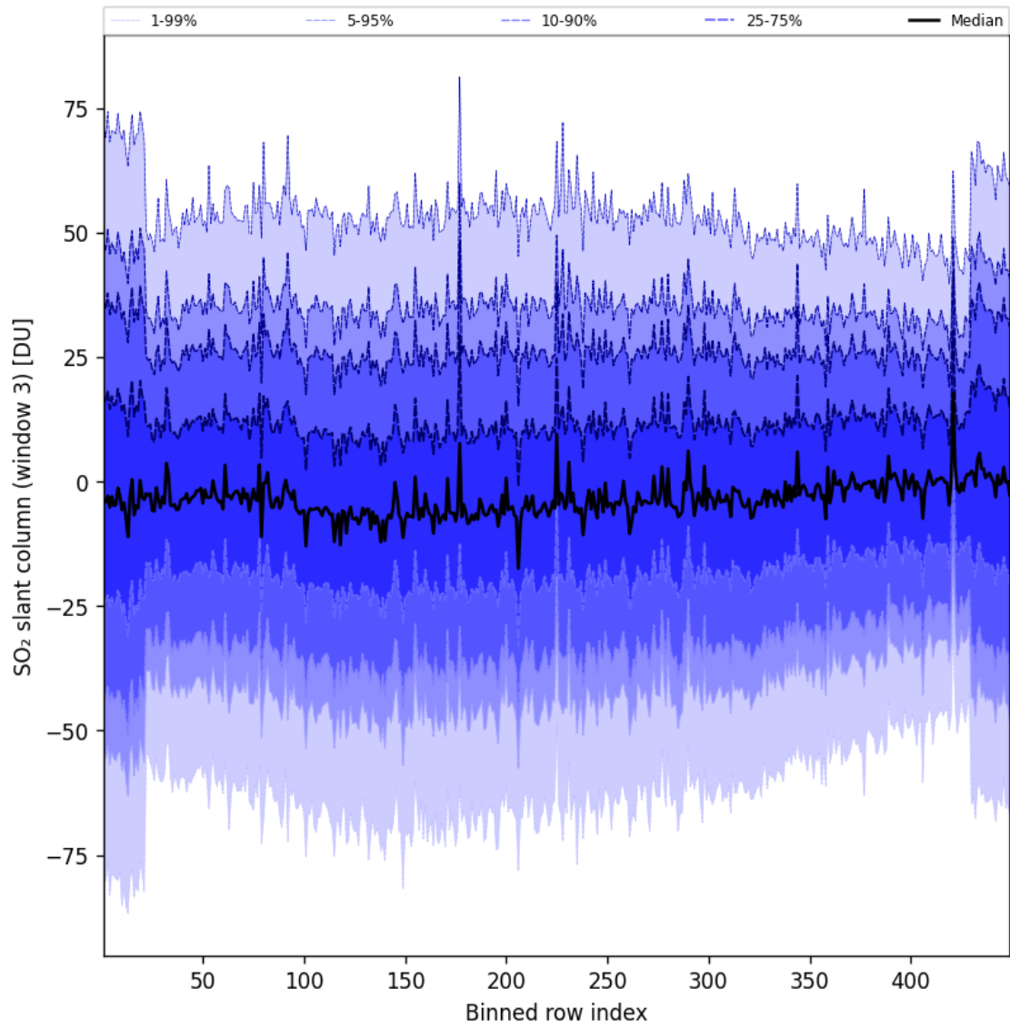
Figure 98: Along track statistics of “SO 2 slant column (window 3)” for 2025-10-07 to 2025-10-07
