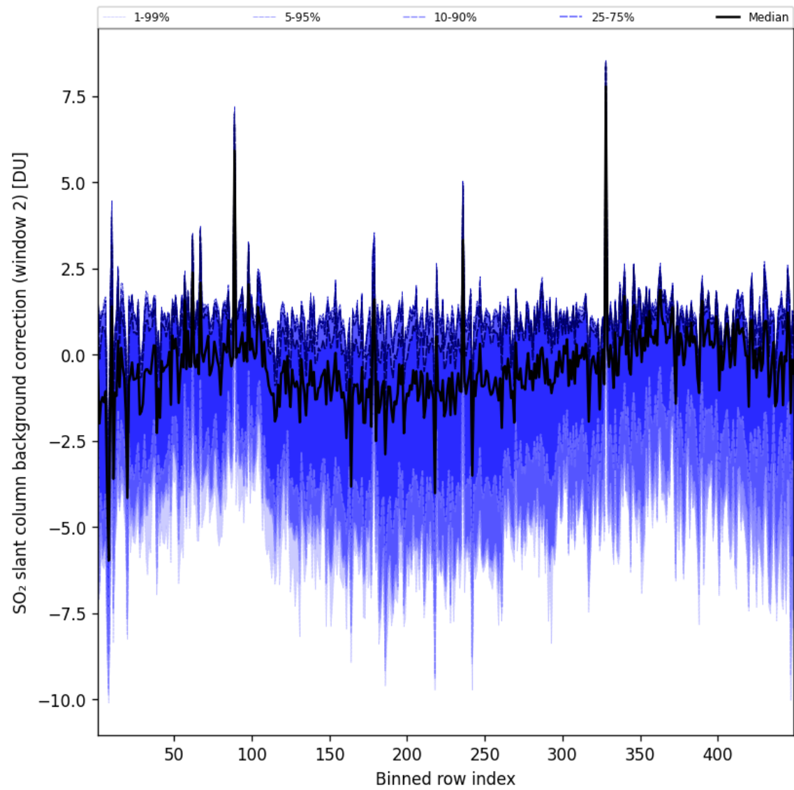
Figure 97: Along track statistics of “SO 2 slant column background correction (window 2)” for 2025-10-07 to 2025-10-07
