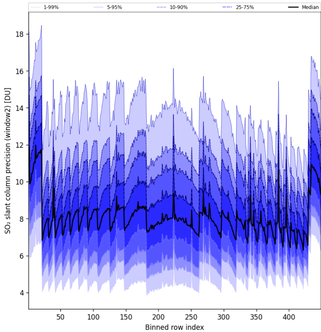
Figure 95: Along track statistics of “SO 2 slant column precision (window2)” for 2025-10-07 to 2025-10-07
