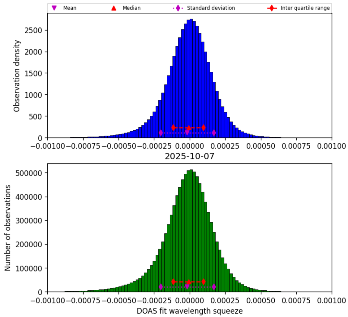
Figure 78: Histogram of “DOAS fit wavelength squeeze” for 2025-10-07 to 2025-10-07
