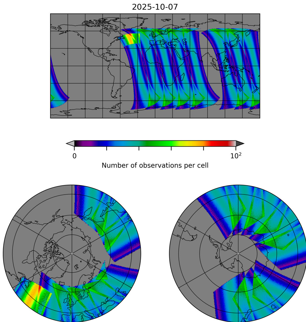
Figure 29: Map of the number of observations for 2025-10-07 to 2025-10-07
