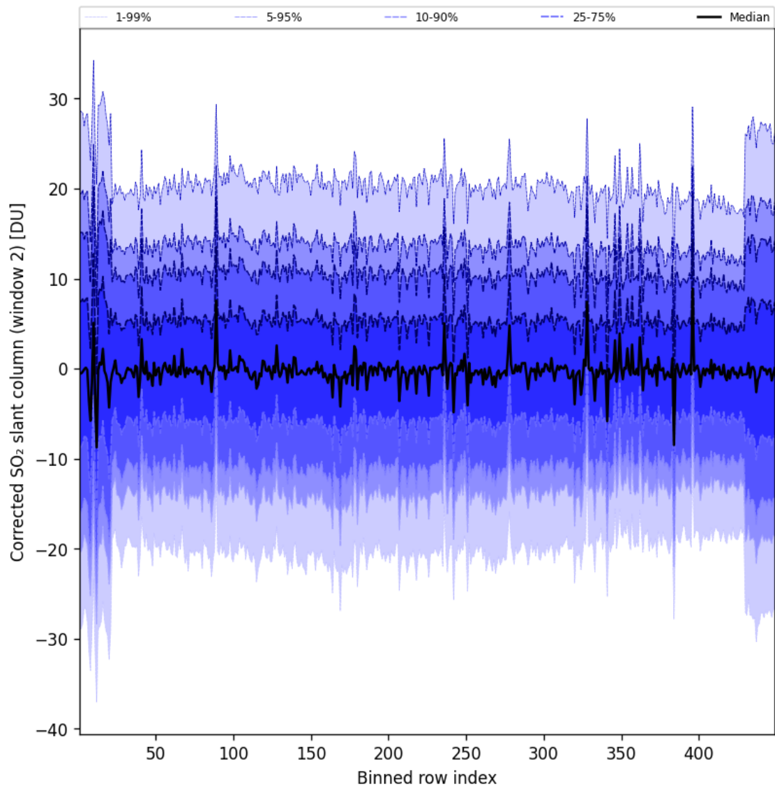
Figure 96: Along track statistics of “Corrected SO 2 slant column (window 2)” for 2025-10-07 to 2025-10-07
