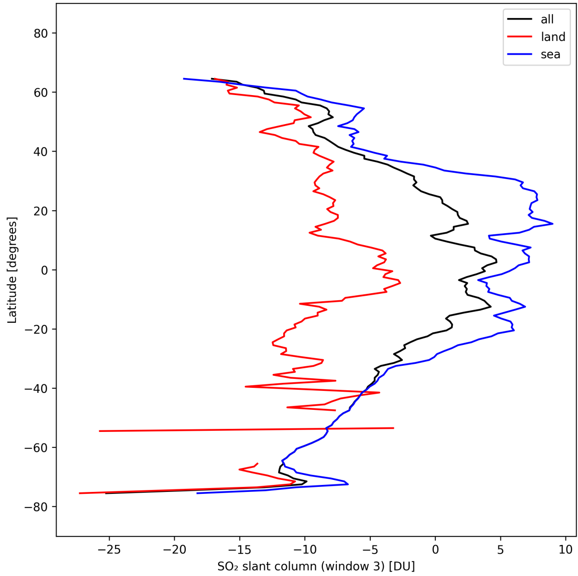
Figure 44: Zonal average of “SO 2 slant column (window 3)” for 2025-10-07 to 2025-10-07.
