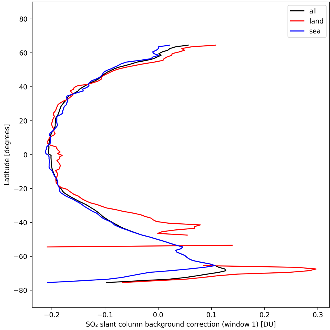
Figure 39: Zonal average of “SO 2 slant column background correction (window 1)” for 2025-10-07 to 2025-10-07.
