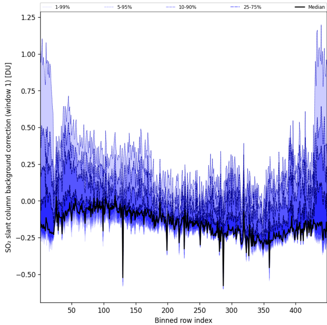
Figure 93: Along track statistics of “SO 2 slant column background correction (window 1)” for 2025-10-07 to 2025-10-07
