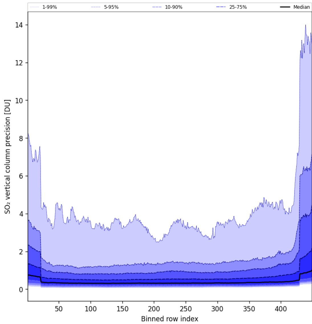
Figure 86: Along track statistics of “SO 2 vertical column precision” for 2025-10-07 to 2025-10-07
