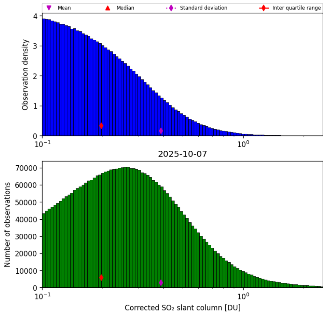
Figure 60: Histogram of “Corrected SO 2 slant column” for 2025-10-07 to 2025-10-07
