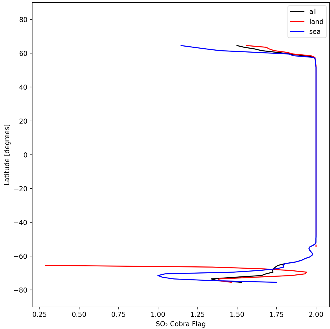
Figure 48: Zonal average of “SO 2 Cobra Flag” for 2025-10-07 to 2025-10-07.
