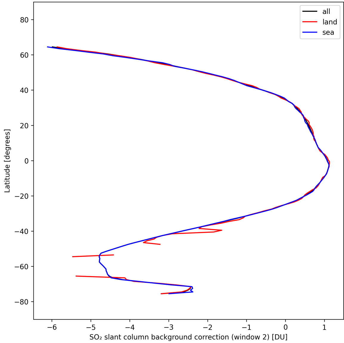
Figure 43: Zonal average of “SO 2 slant column background correction (window 2)” for 2025-10-07 to 2025-10-07.
