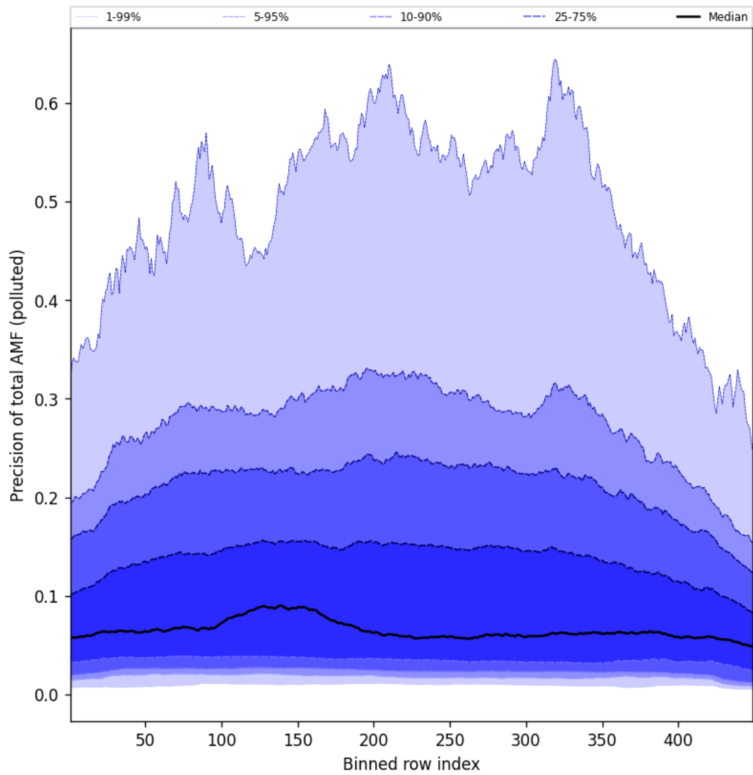
Figure 108: Along track statistics of “Precision of total AMF (polluted)” for 2025-10-07 to 2025-10-07
