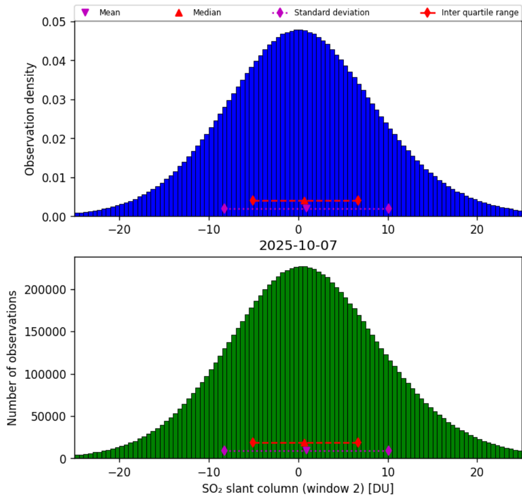
Figure 67: Histogram of “SO 2 slant column (window 2)” for 2025-10-07 to 2025-10-07
