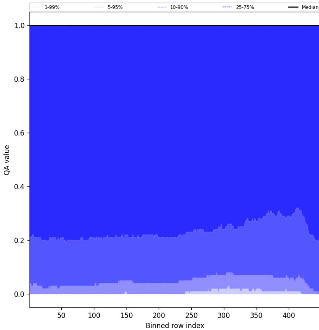
Figure 84: Along track statistics of “QA value” for 2025-10-07 to 2025-10-07
