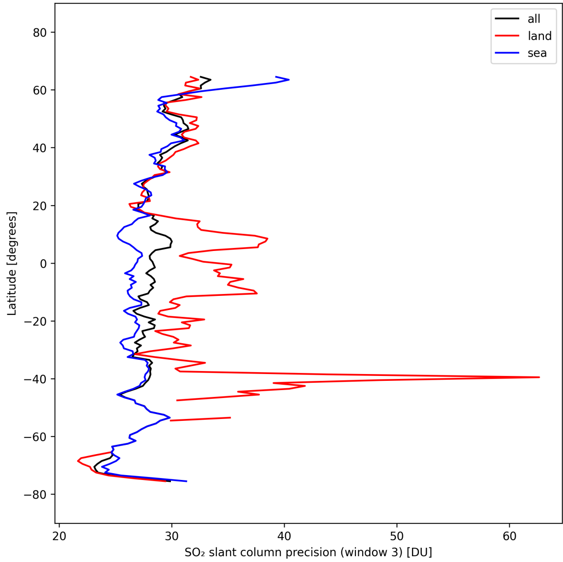
Figure 45: Zonal average of “SO 2 slant column precision (window 3)” for 2025-10-07 to 2025-10-07.
