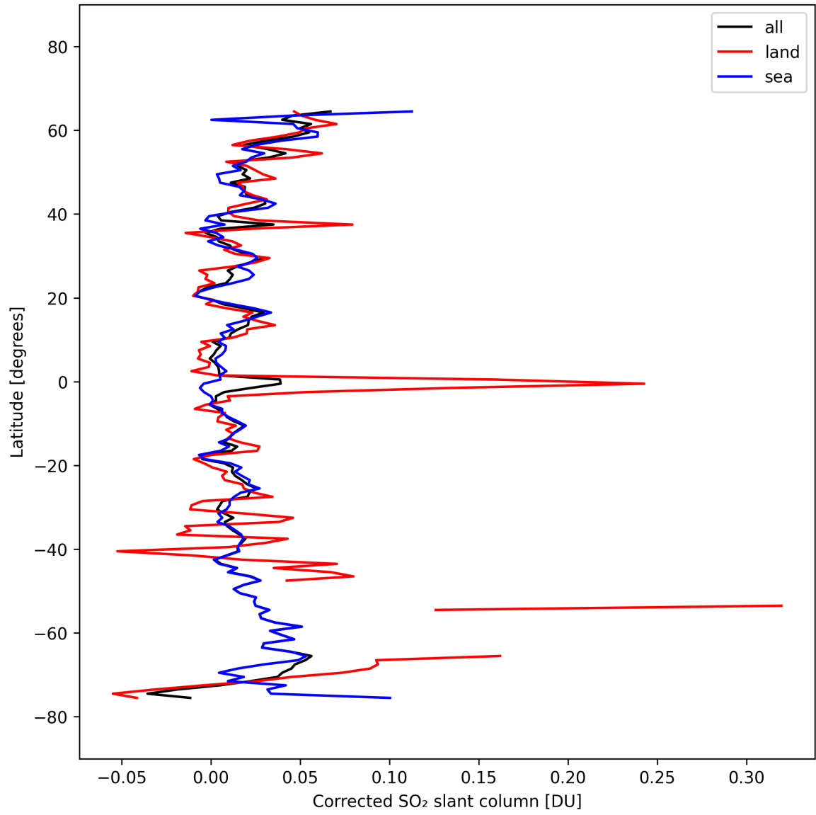
Figure 33: Zonal average of “Corrected SO 2 slant column” for 2025-10-07 to 2025-10-07.
