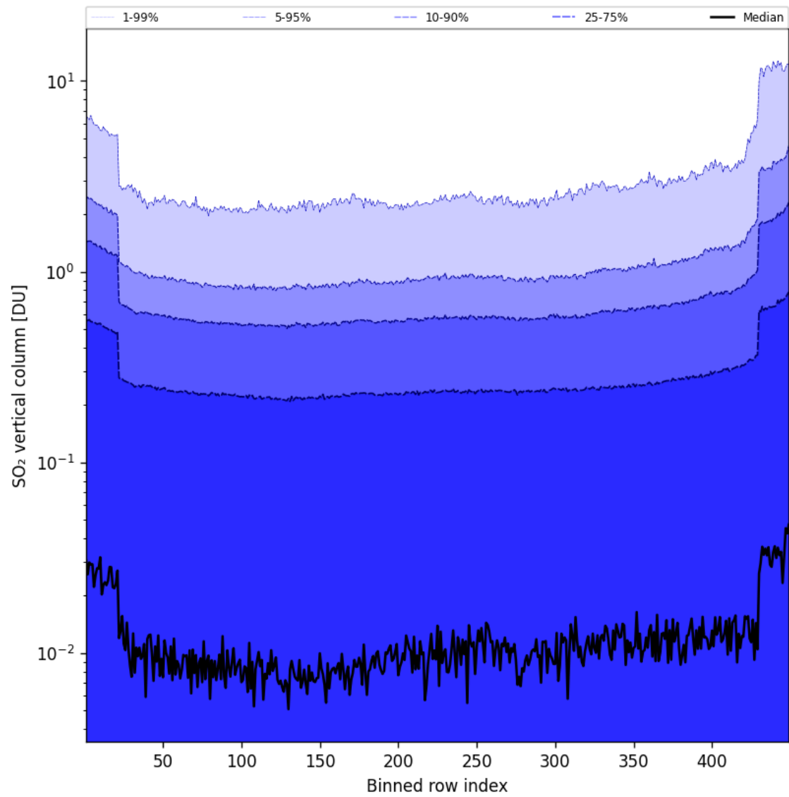
Figure 85: Along track statistics of “SO 2 vertical column” for 2025-10-07 to 2025-10-07
