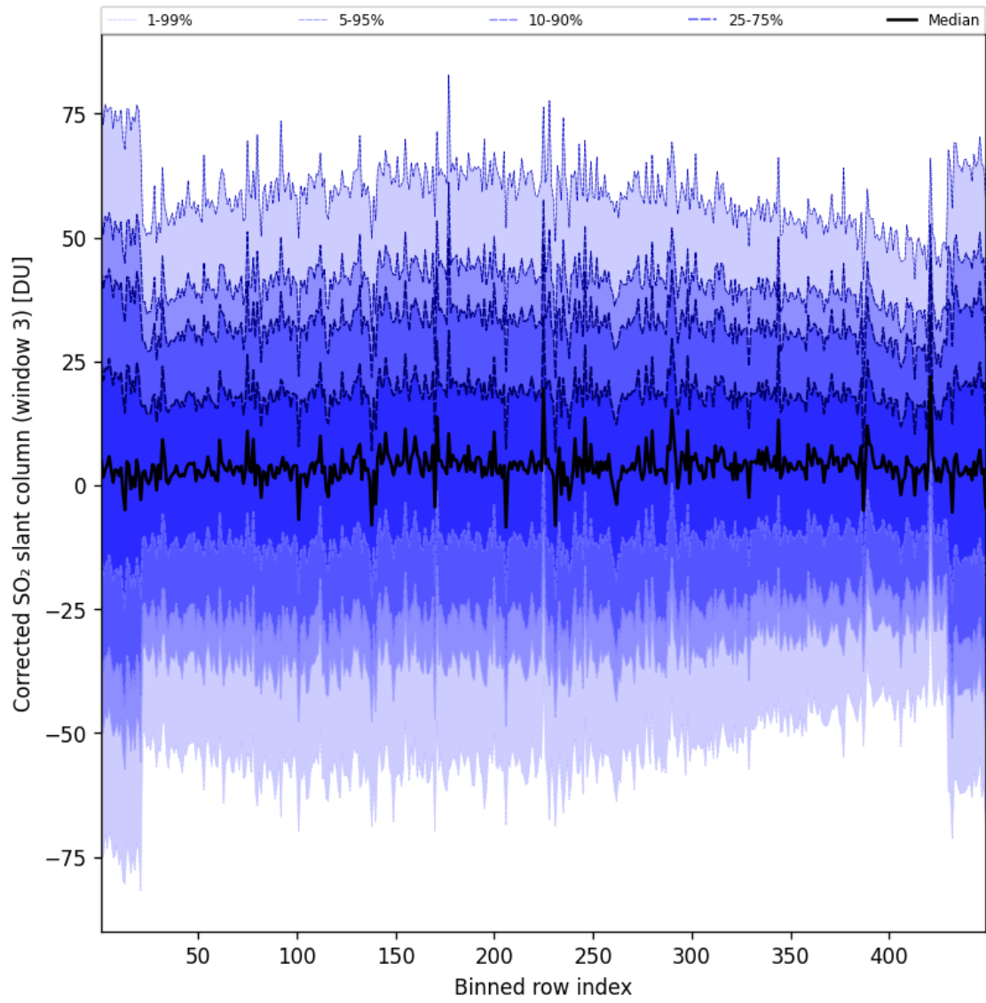
Figure 100: Along track statistics of “Corrected SO 2 slant column (window 3)” for 2025-10-07 to 2025-10-07
