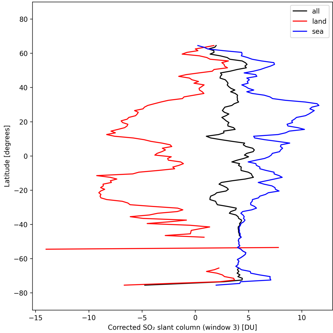
Figure 46: Zonal average of “Corrected SO 2 slant column (window 3)” for 2025-10-07 to 2025-10-07.
