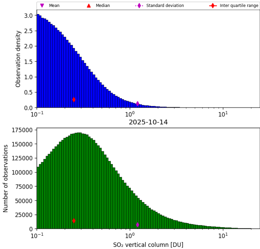
Figure 58: Histogram of “SO 2 vertical column” for 2025-10-14 to 2025-10-15
