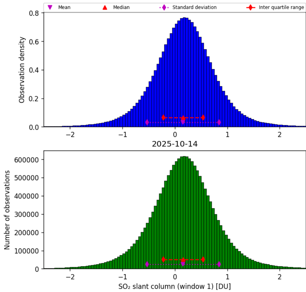
Figure 63: Histogram of “SO 2 slant column (window 1)” for 2025-10-14 to 2025-10-15
