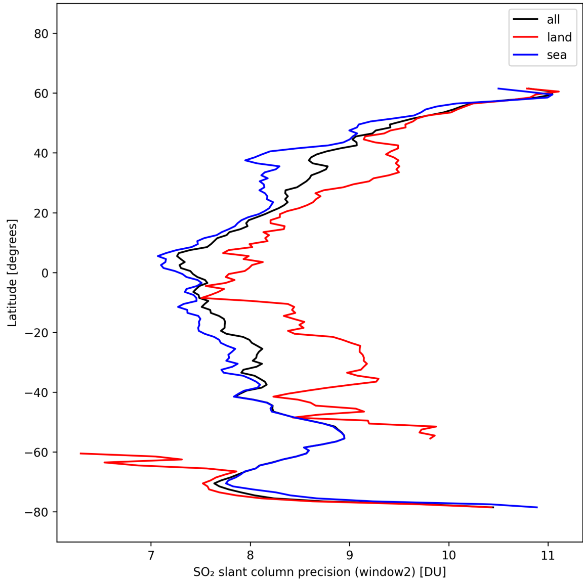
Figure 41: Zonal average of “SO 2 slant column precision (window2)” for 2025-10-14 to 2025-10-15.
