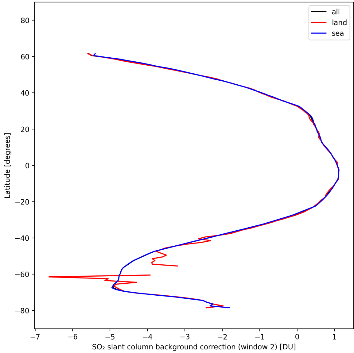
Figure 43: Zonal average of “SO 2 slant column background correction (window 2)” for 2025-10-14 to 2025-10-15.
