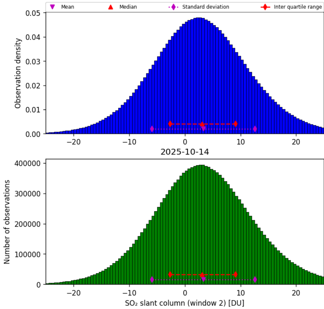
Figure 67: Histogram of “SO 2 slant column (window 2)” for 2025-10-14 to 2025-10-15
