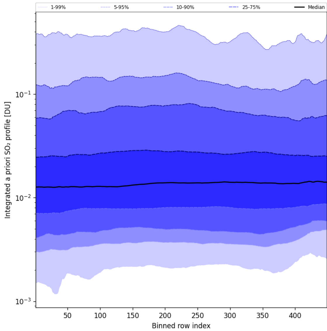
Figure 103: Along track statistics of “Integrated a priori SO 2 profile” for 2025-10-14 to 2025-10-15
