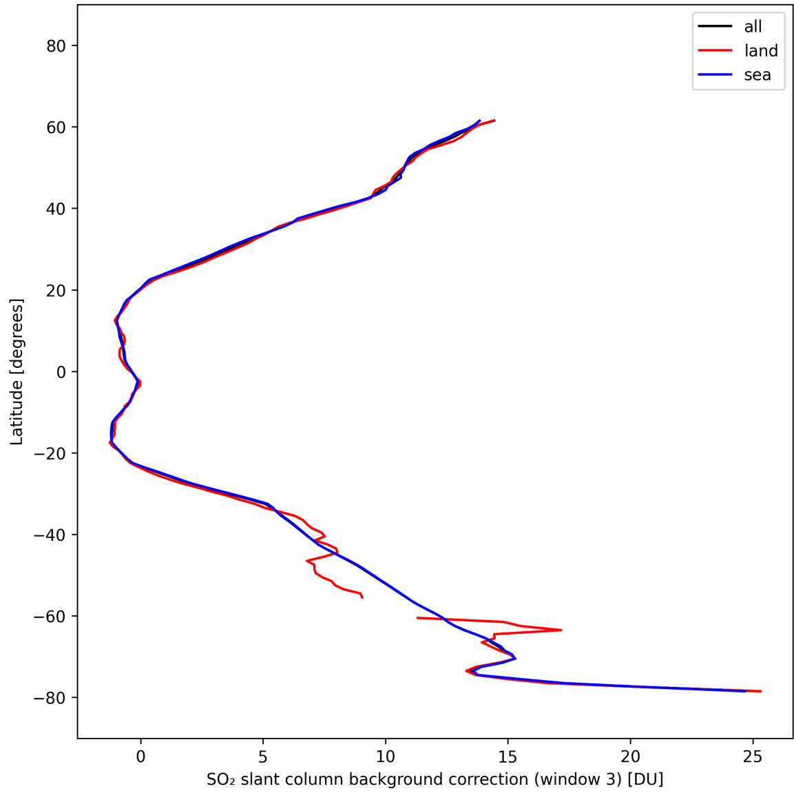
Figure 47: Zonal average of “SO 2 slant column background correction (window 3)” for 2025-10-14 to 2025-10-15.
