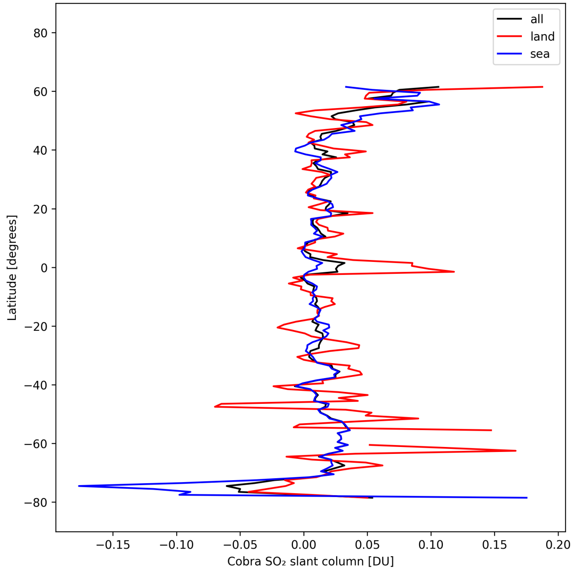
Figure 34: Zonal average of “Cobra SO 2 slant column” for 2025-10-14 to 2025-10-15.
