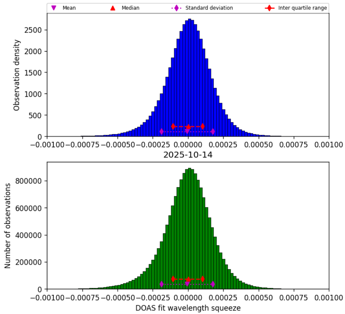
Figure 78: Histogram of “DOAS fit wavelength squeeze” for 2025-10-14 to 2025-10-15
