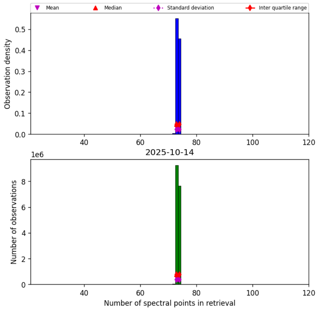
Figure 83: Histogram of “Number of spectral points in retrieval” for 2025-10-14 to 2025-10-15
