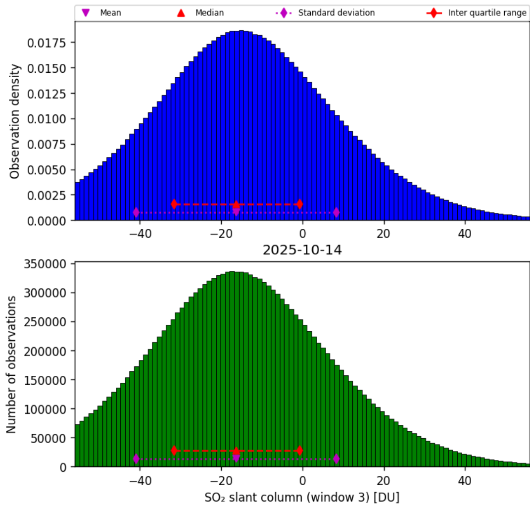
Figure 71: Histogram of “SO 2 slant column (window 3)” for 2025-10-14 to 2025-10-15
