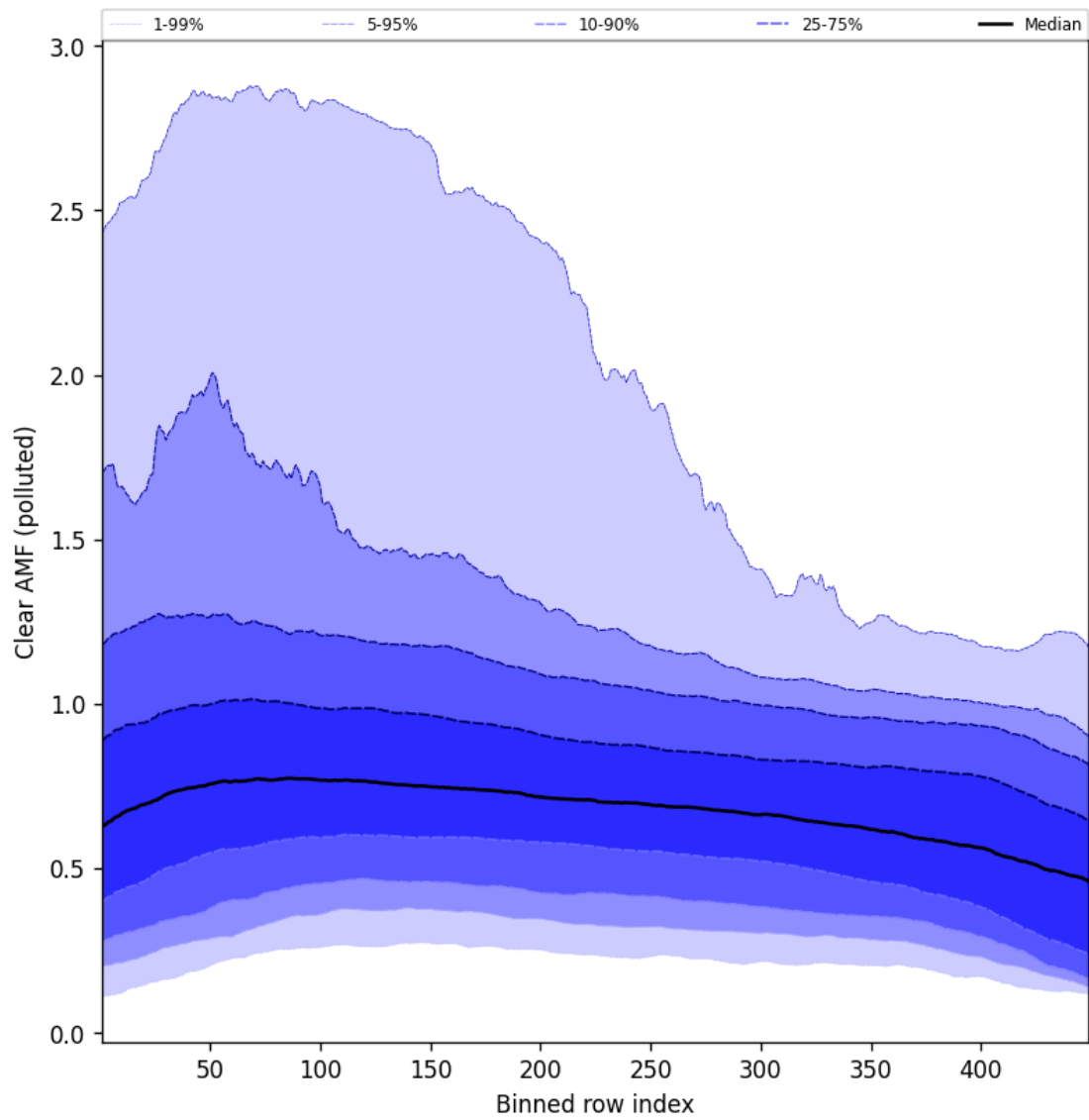
Figure 109: Along track statistics of “Clear AMF (polluted)” for 2025-10-14 to 2025-10-15
