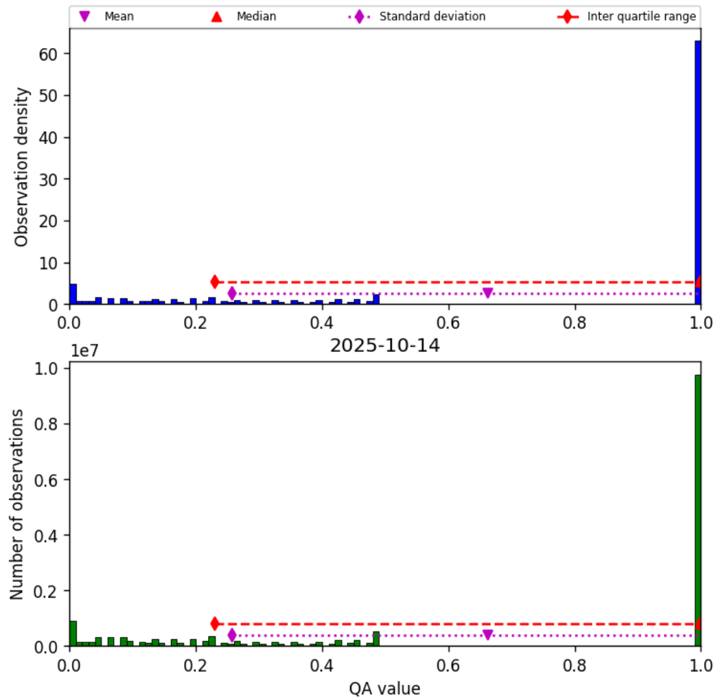
Figure 57: Histogram of “QA value” for 2025-10-14 to 2025-10-15
