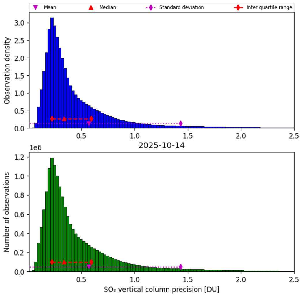
Figure 59: Histogram of “SO 2 vertical column precision” for 2025-10-14 to 2025-10-15
