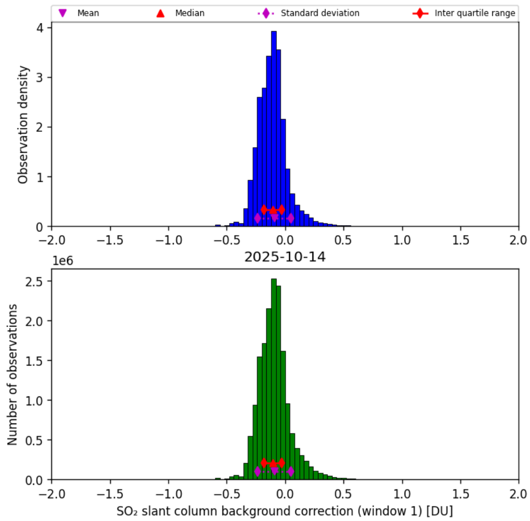
Figure 66: Histogram of “SO 2 slant column background correction (window 1)” for 2025-10-14 to 2025-10-15
