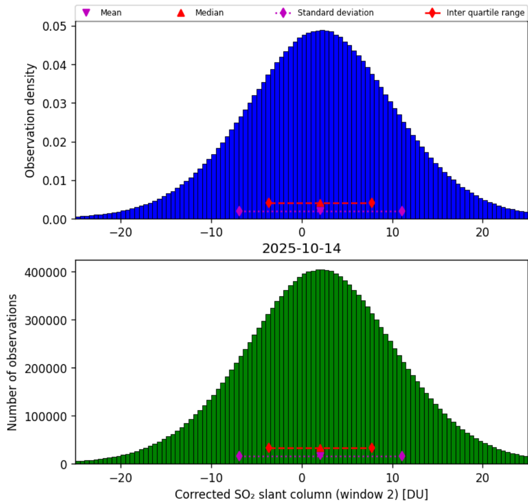
Figure 69: Histogram of “Corrected SO 2 slant column (window 2)” for 2025-10-14 to 2025-10-15
