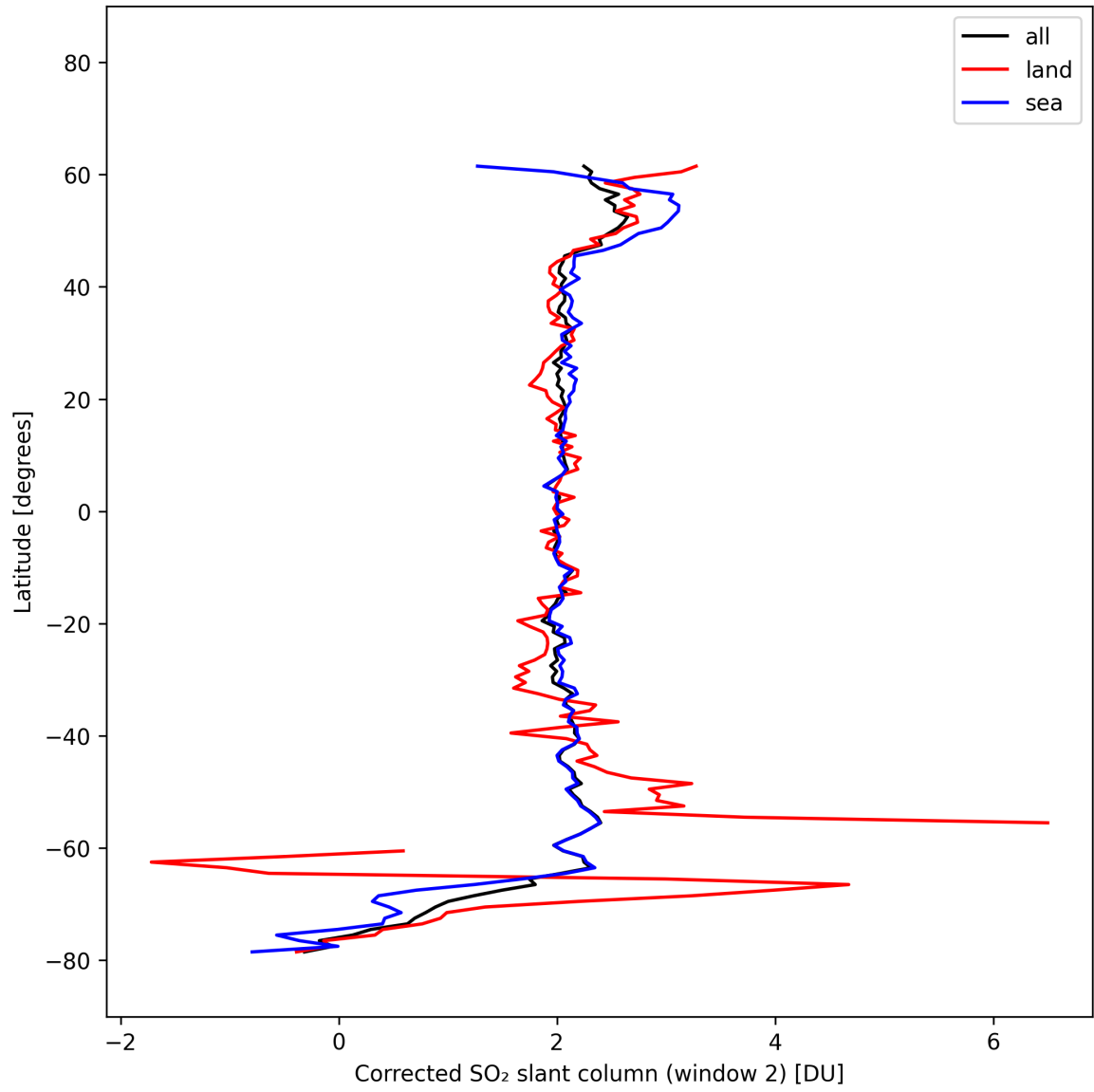
Figure 42: Zonal average of “Corrected SO 2 slant column (window 2)” for 2025-10-14 to 2025-10-15.
