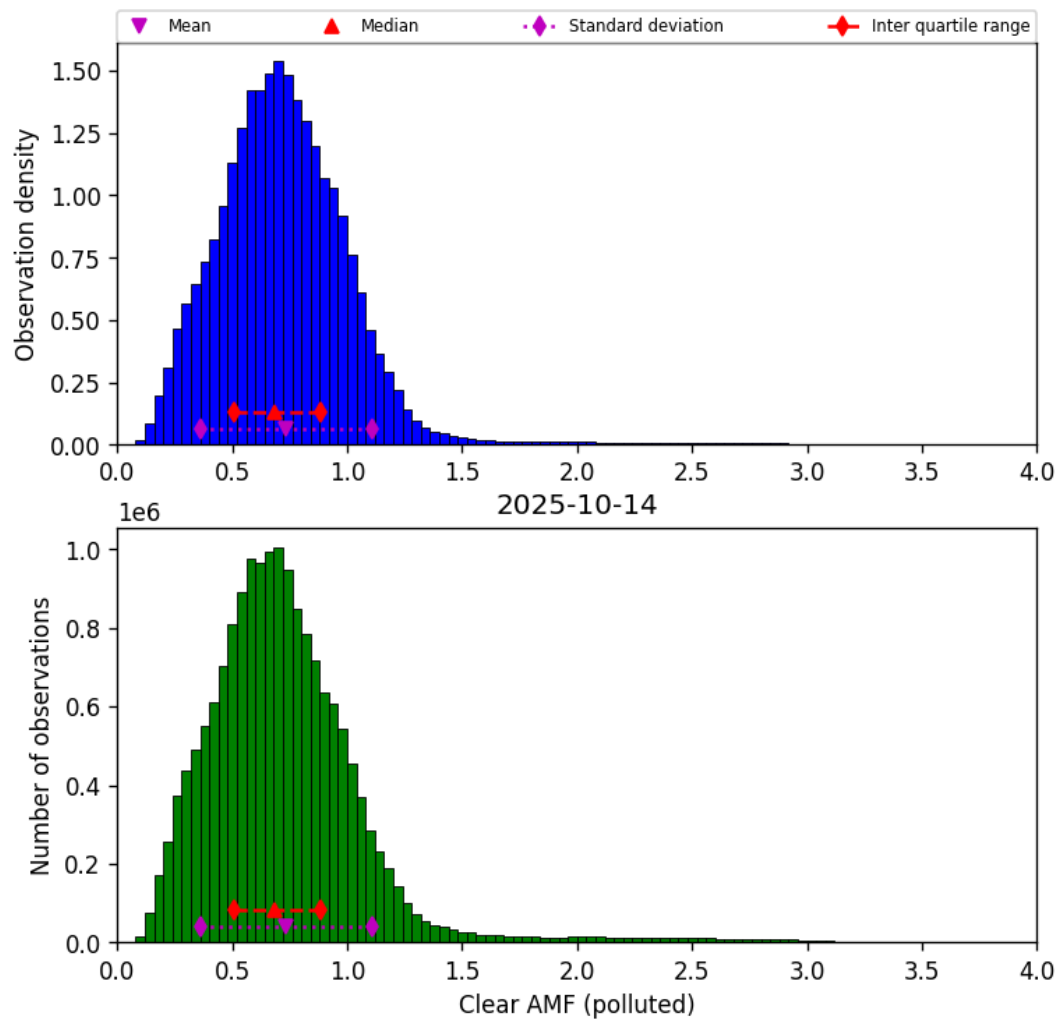
Figure 82: Histogram of “Clear AMF (polluted)” for 2025-10-14 to 2025-10-15
