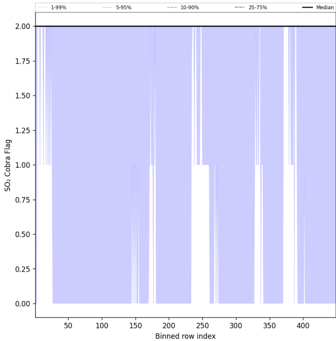
Figure 102: Along track statistics of “SO 2 Cobra Flag” for 2025-10-14 to 2025-10-15
