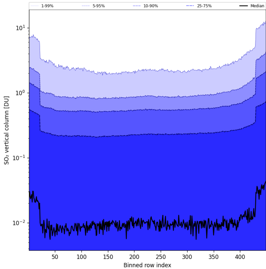
Figure 85: Along track statistics of “SO 2 vertical column” for 2025-10-14 to 2025-10-15
