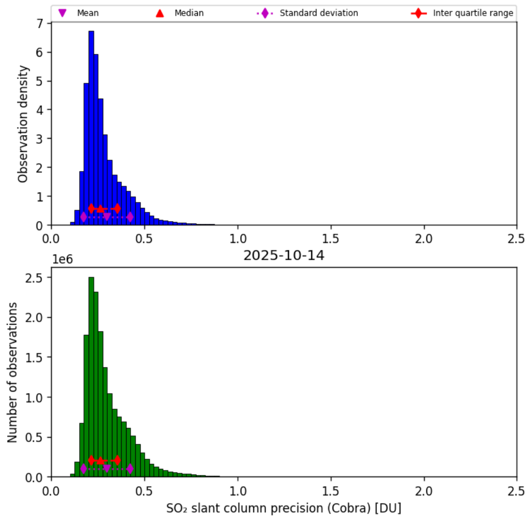
Figure 62: Histogram of “SO 2 slant column precision (Cobra)” for 2025-10-14 to 2025-10-15
