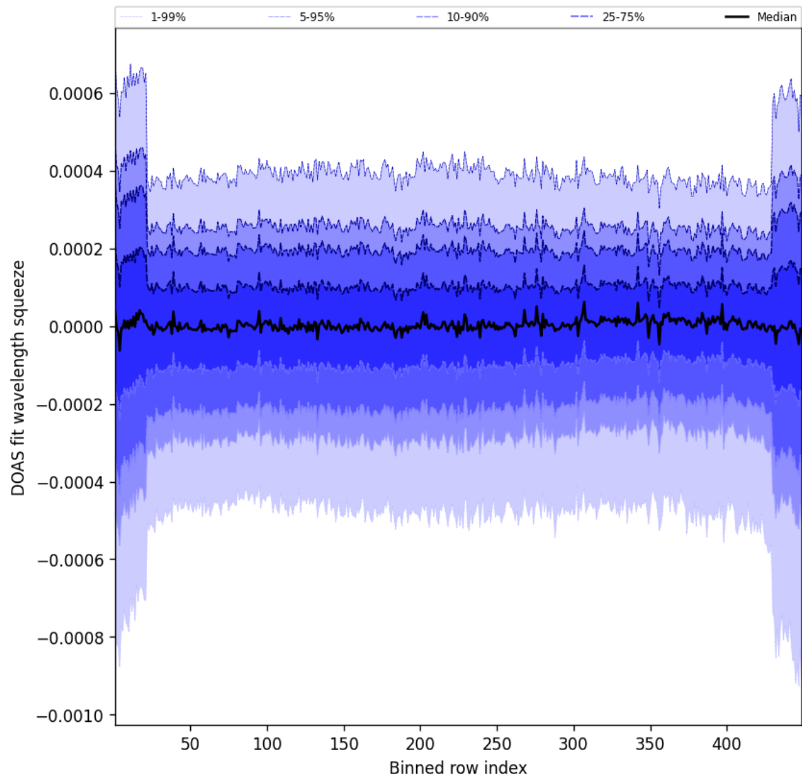
Figure 105: Along track statistics of “DOAS fit wavelength squeeze” for 2025-10-14 to 2025-10-15
