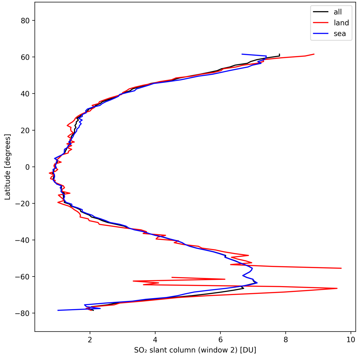
Figure 40: Zonal average of “SO 2 slant column (window 2)” for 2025-10-14 to 2025-10-15.
