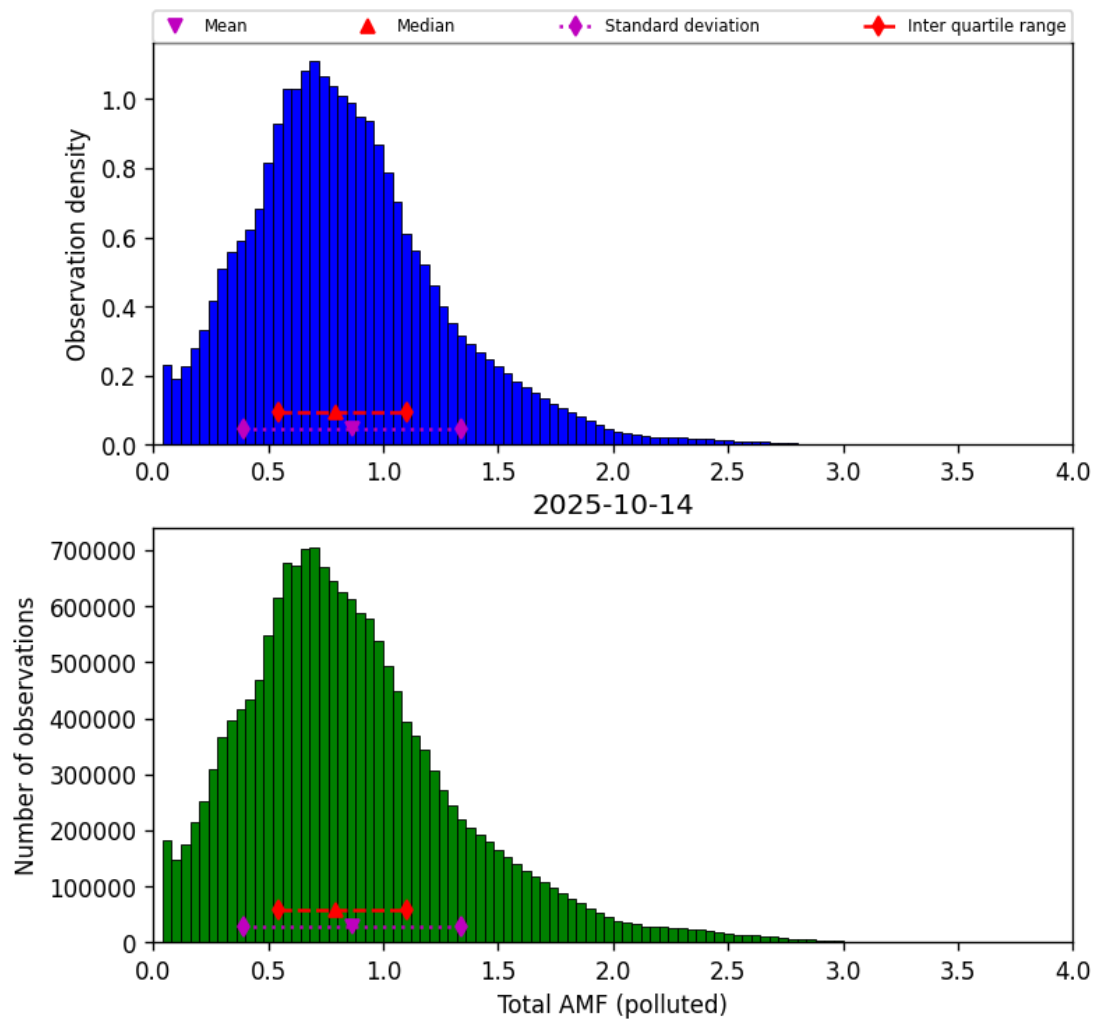
Figure 80: Histogram of “Total AMF (polluted)” for 2025-10-14 to 2025-10-15
