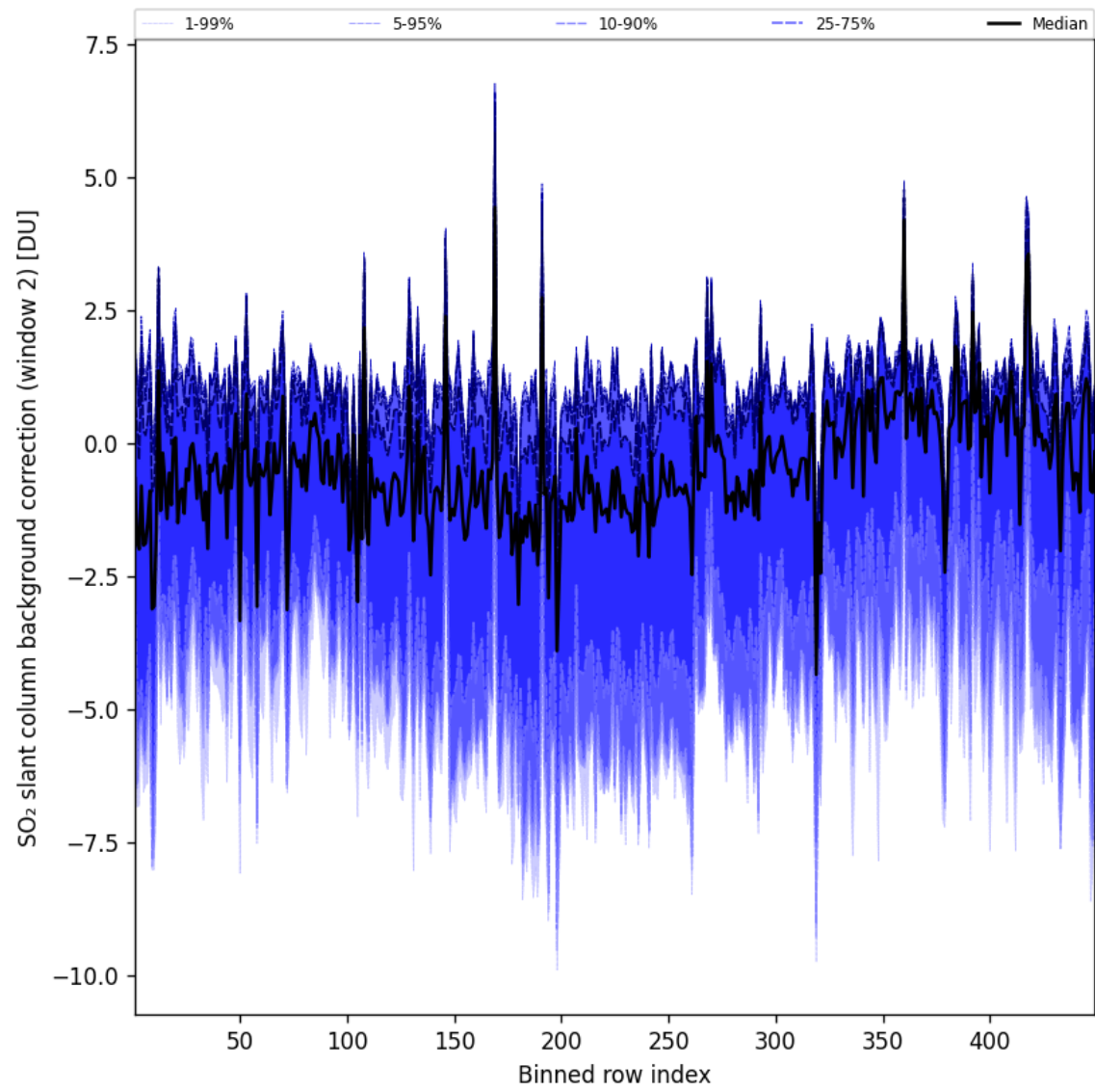
Figure 97: Along track statistics of “SO 2 slant column background correction (window 2)” for 2025-10-14 to 2025-10-15
