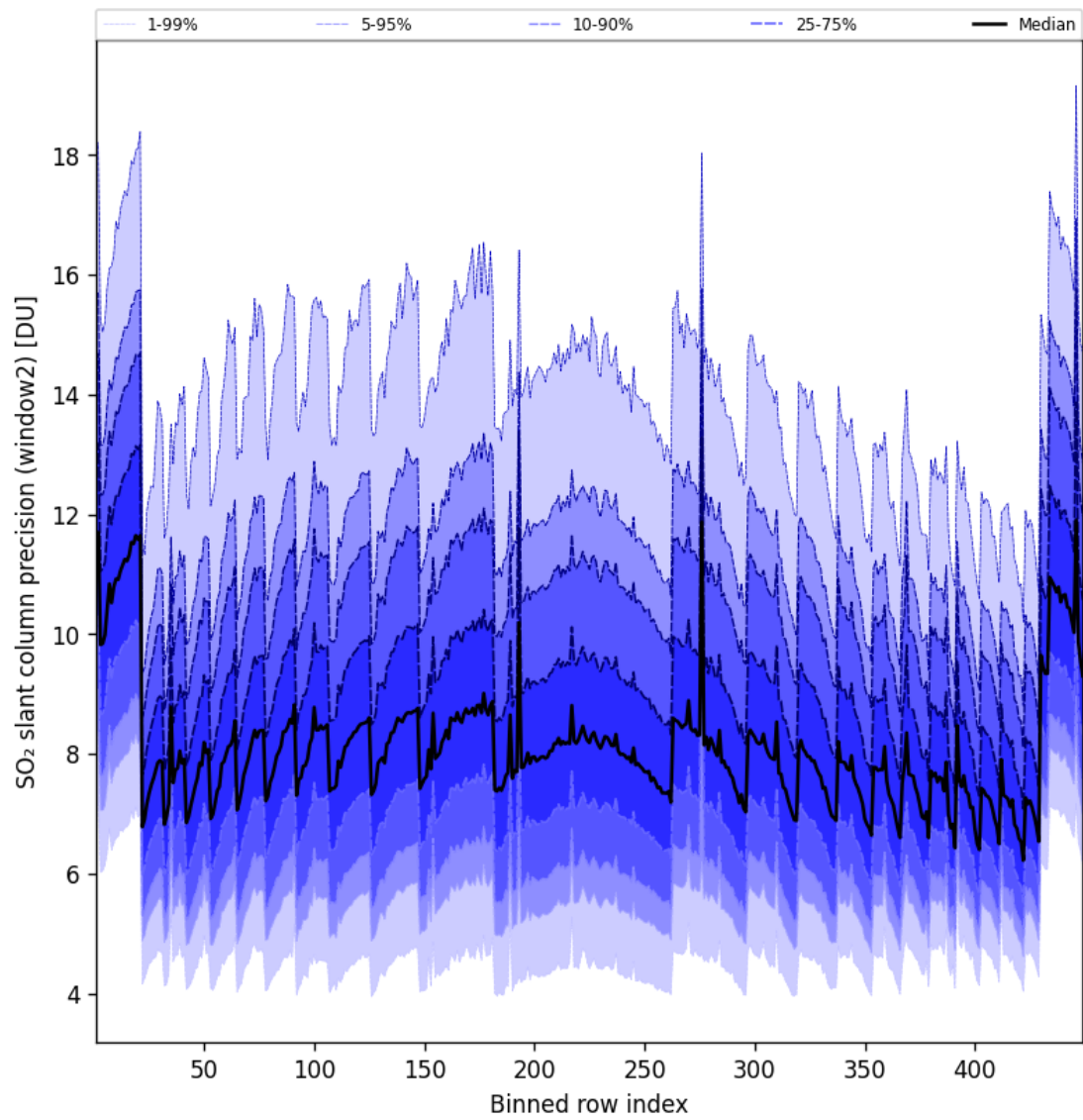
Figure 95: Along track statistics of “SO 2 slant column precision (window2)” for 2025-10-14 to 2025-10-15
