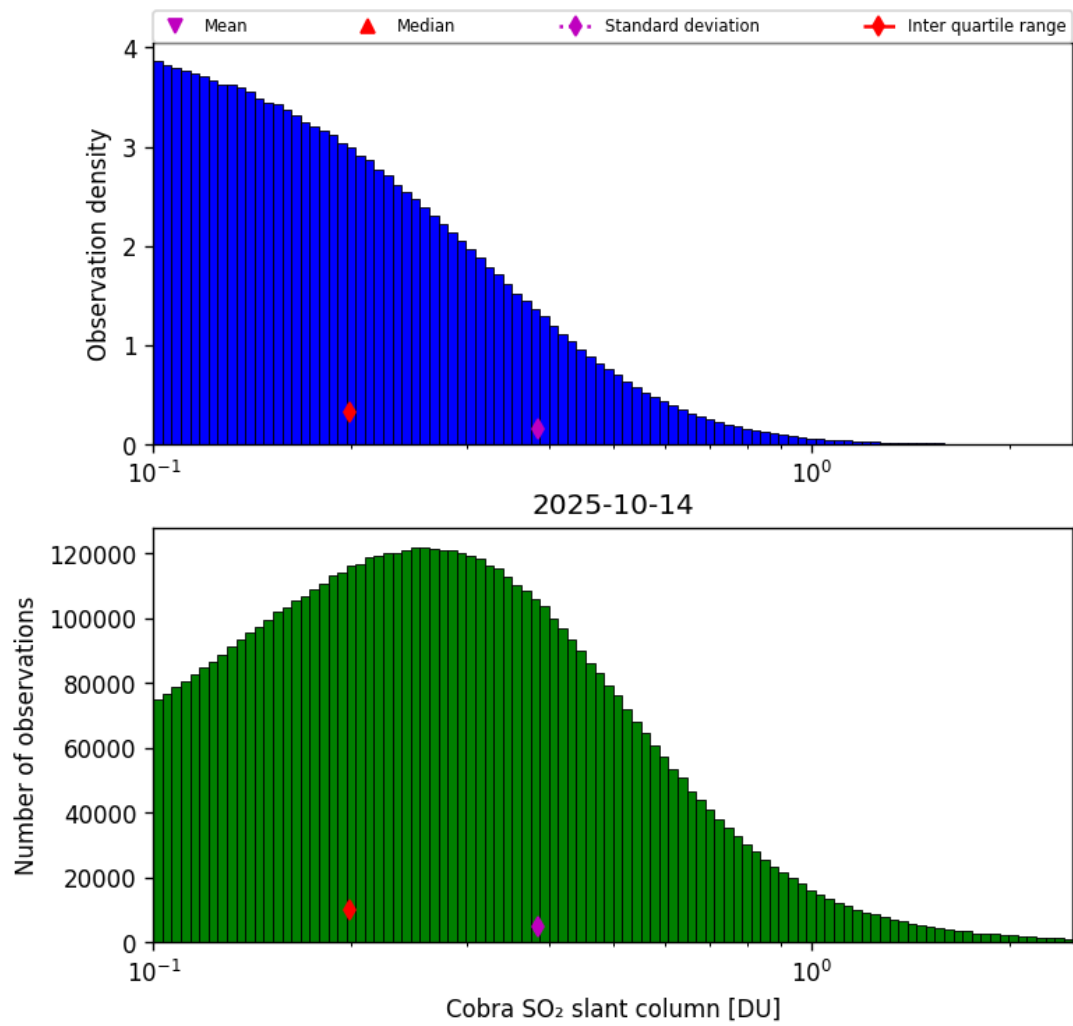
Figure 61: Histogram of “Cobra SO 2 slant column” for 2025-10-14 to 2025-10-15
