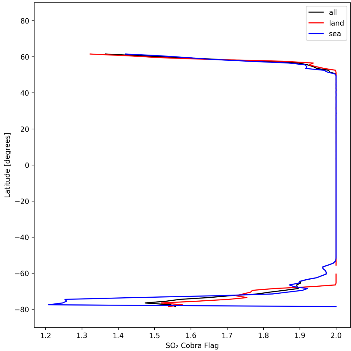
Figure 48: Zonal average of "SO 2 Cobra Flag" for 2025-10-14 to 2025-10-15.
