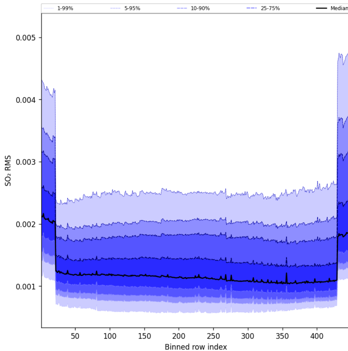
Figure 106: Along track statistics of “SO 2 RMS” for 2025-10-14 to 2025-10-15
