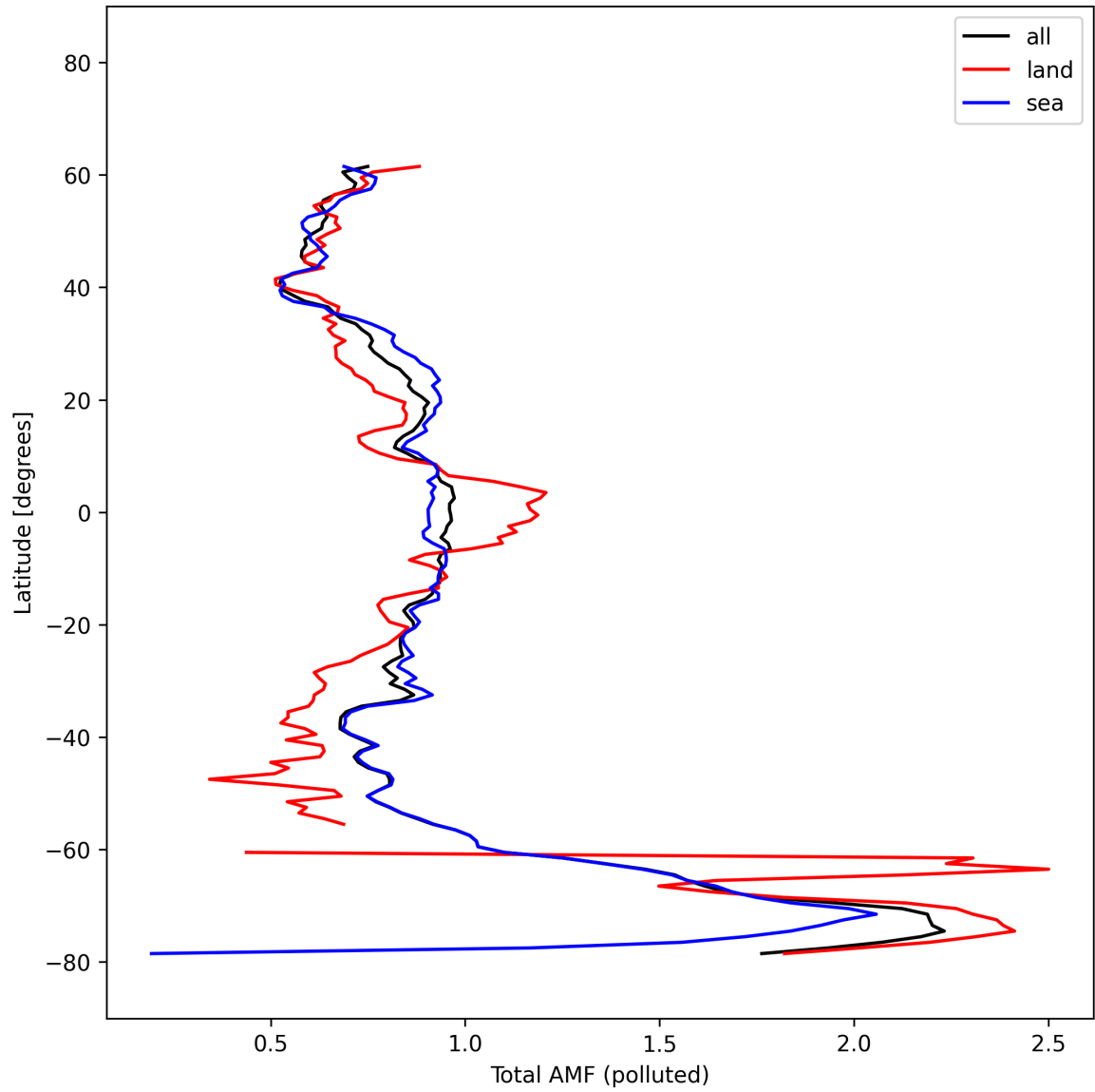
Figure 53: Zonal average of “Total AMF (polluted)” for 2025-10-14 to 2025-10-15.
