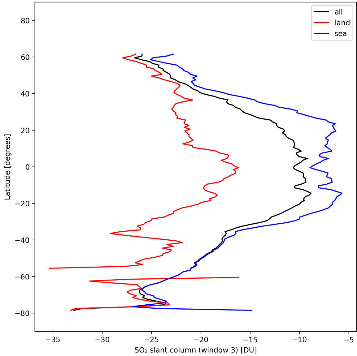
Figure 44: Zonal average of “SO 2 slant column (window 3)” for 2025-10-14 to 2025-10-15.
