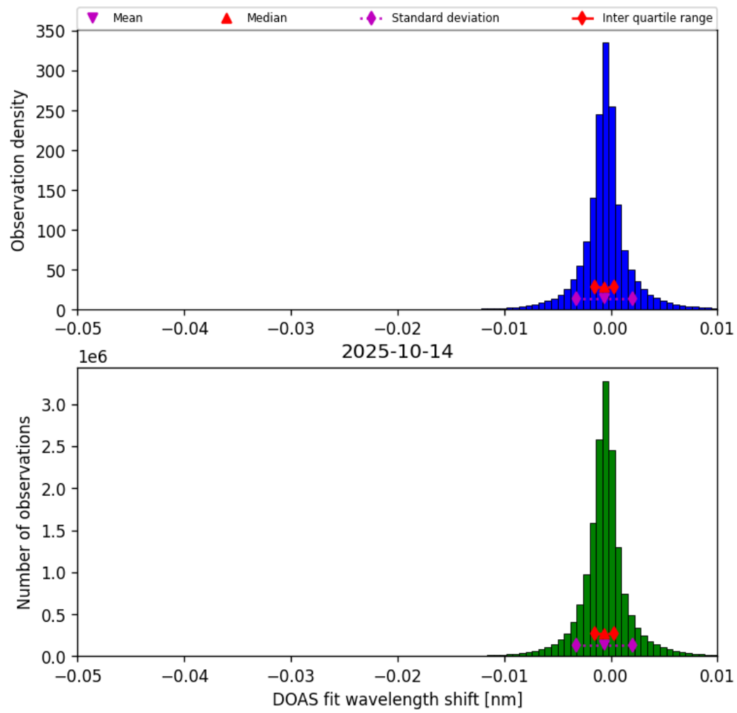
Figure 77: Histogram of “DOAS fit wavelength shift” for 2025-10-14 to 2025-10-15
