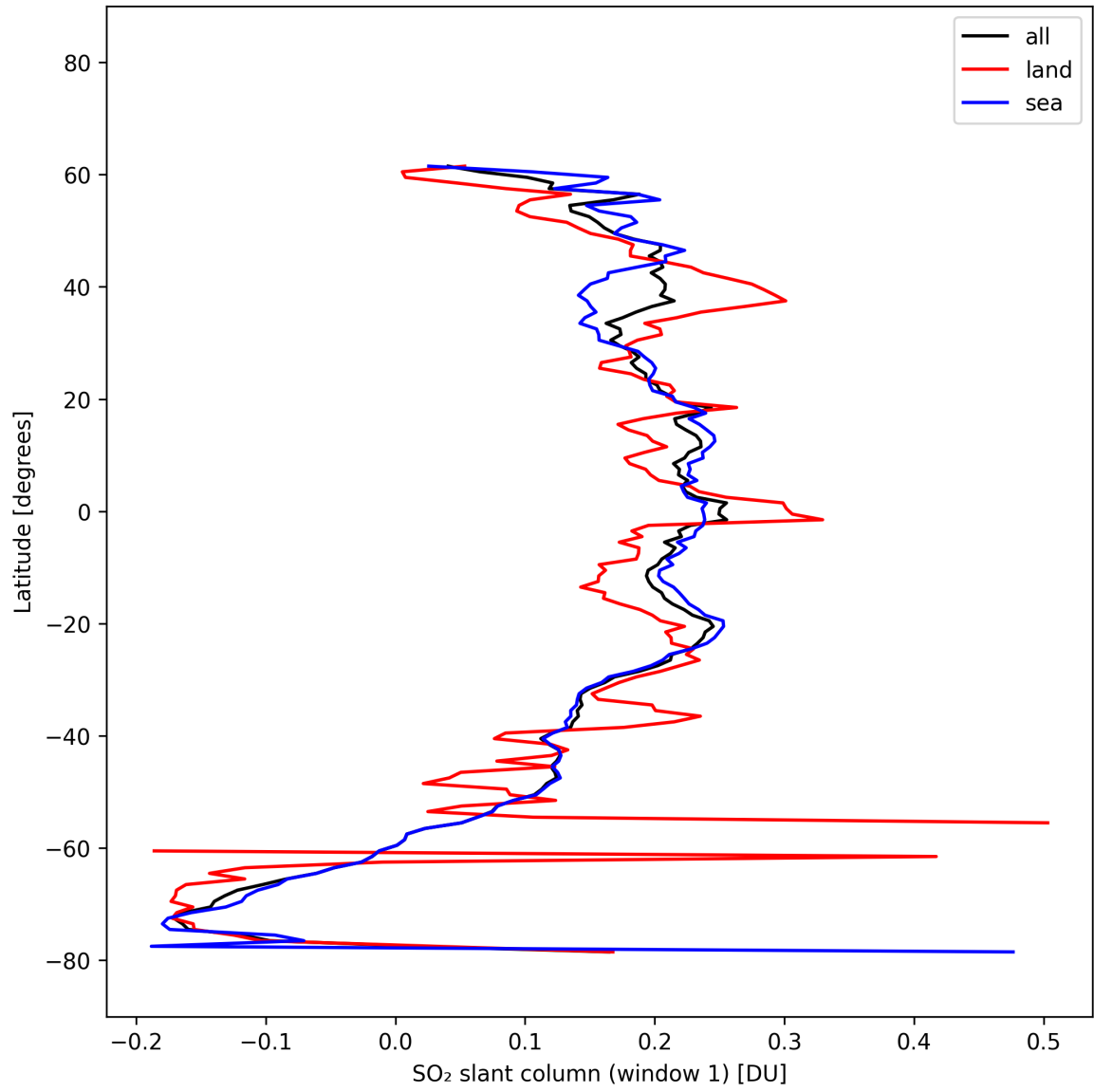
Figure 36: Zonal average of “SO 2 slant column (window 1)” for 2025-10-14 to 2025-10-15.
