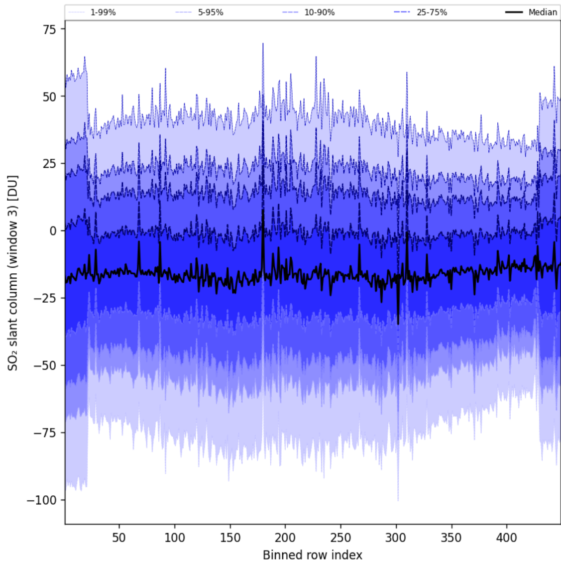
Figure 98: Along track statistics of “SO 2 slant column (window 3)” for 2025-10-14 to 2025-10-15
