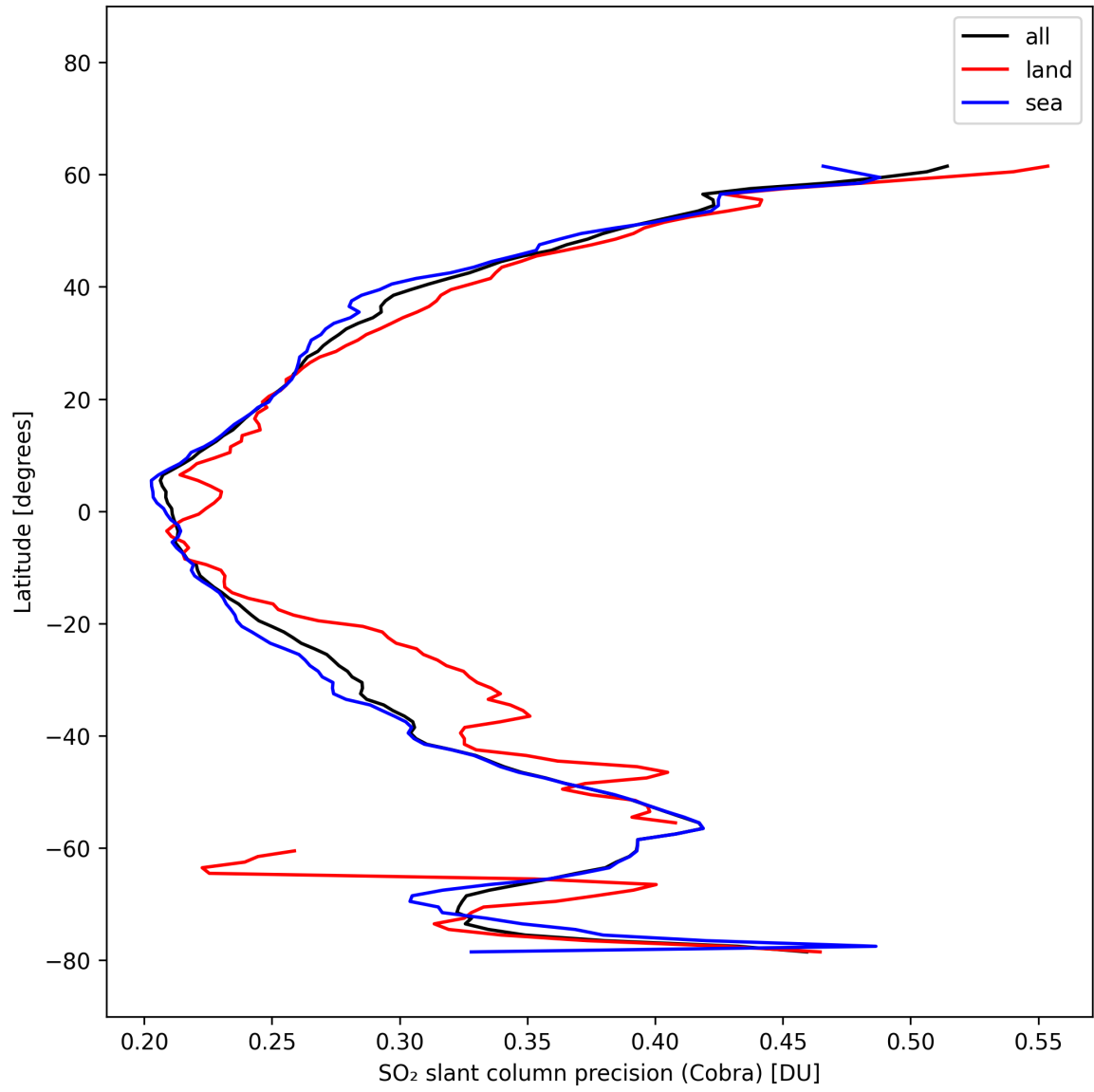
Figure 35: Zonal average of "SO 2 slant column precision (Cobra)" for 2025-10-14 to 2025-10-15.
