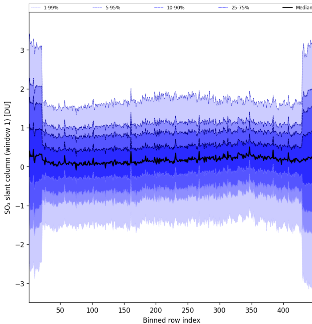
Figure 90: Along track statistics of “SO 2 slant column (window 1)” for 2025-10-14 to 2025-10-15
