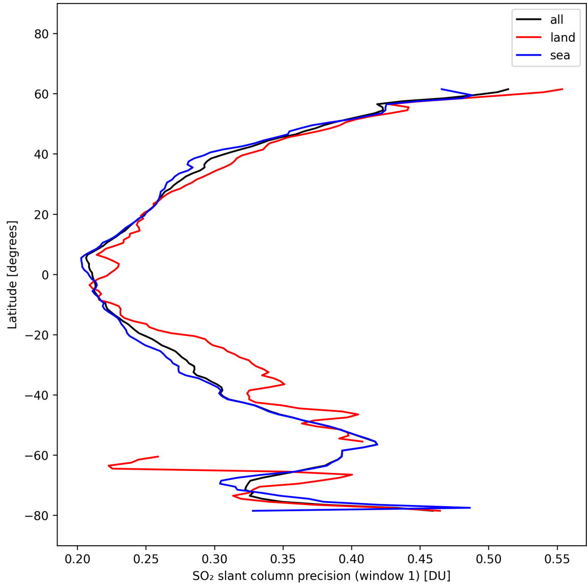
Figure 37: Zonal average of “SO 2 slant column precision (window 1)” for 2025-10-14 to 2025-10-15.
