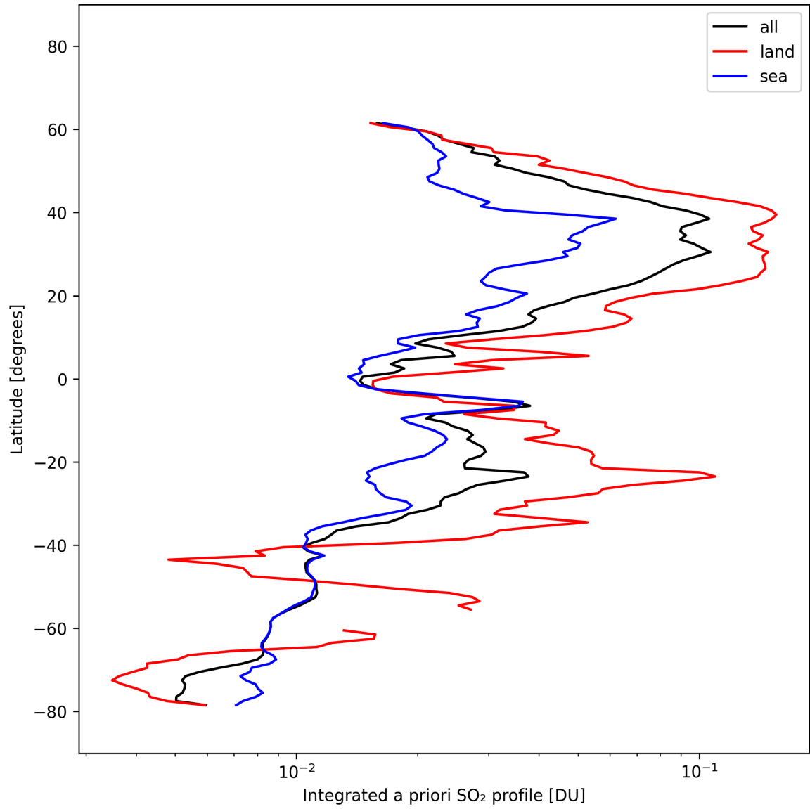
Figure 49: Zonal average of “Integrated a priori SO 2 profile” for 2025-10-14 to 2025-10-15.
