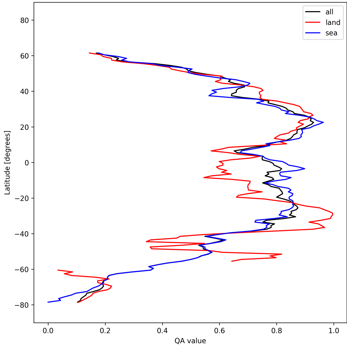
Figure 30: Zonal average of “QA value” for 2025-10-14 to 2025-10-15.
