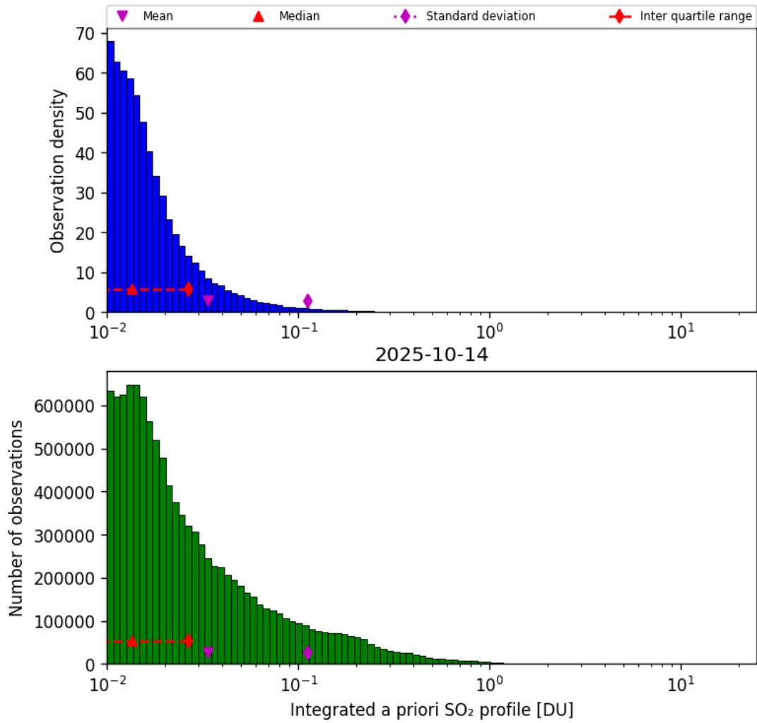
Figure 76: Histogram of “Integrated a priori SO 2 profile” for 2025-10-14 to 2025-10-15
