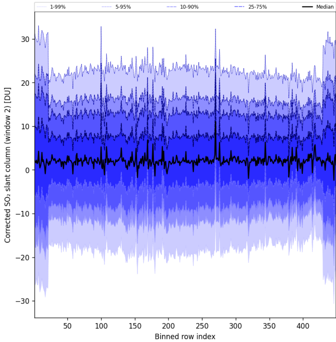
Figure 96: Along track statistics of “Corrected SO 2 slant column (window 2)” for 2025-10-14 to 2025-10-15
