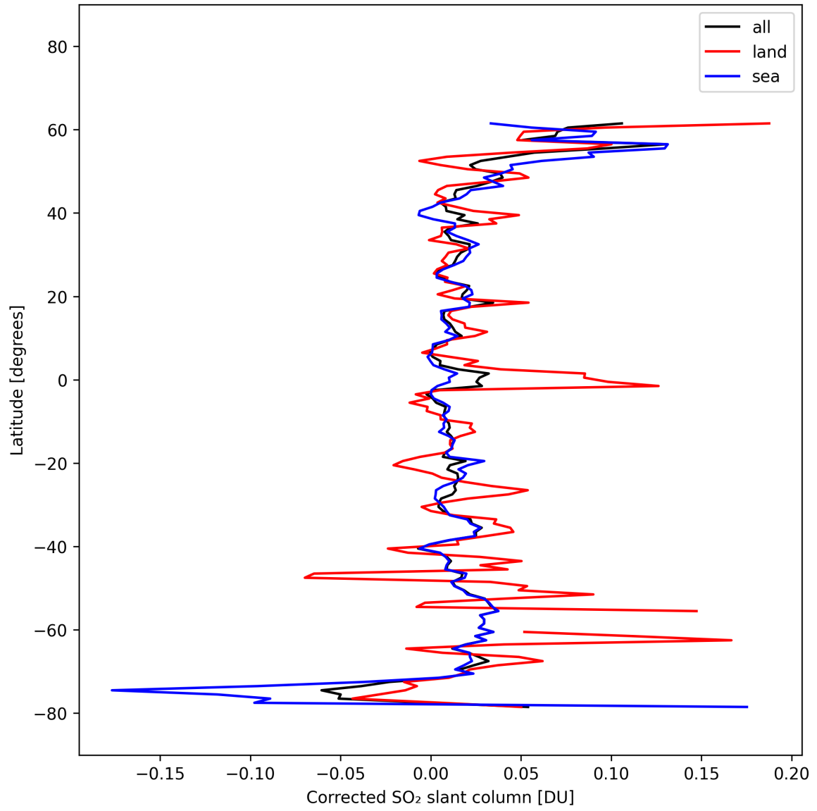
Figure 33: Zonal average of “Corrected SO 2 slant column” for 2025-10-14 to 2025-10-15.
