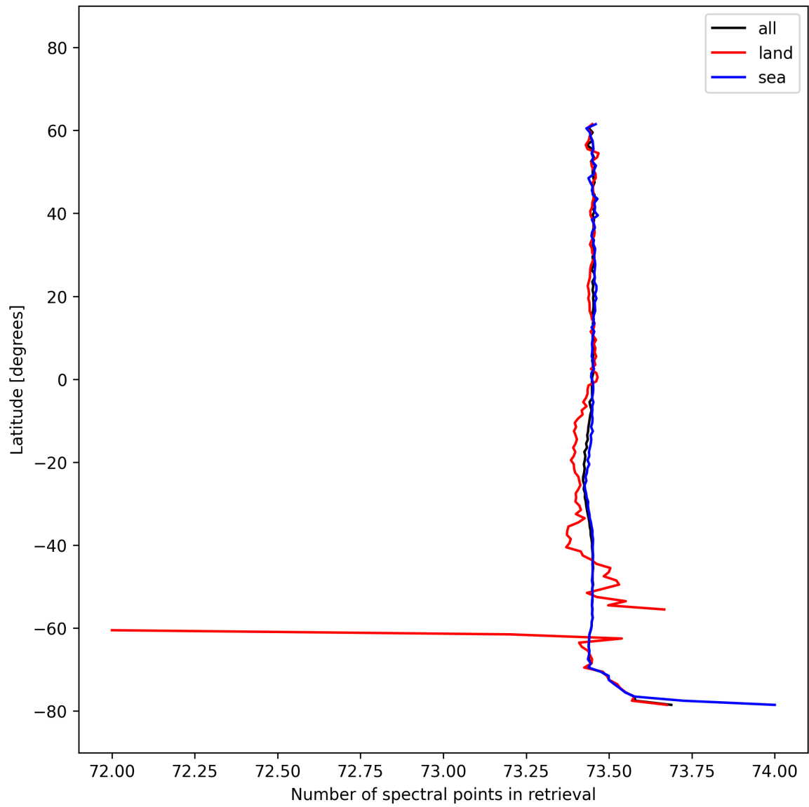
Figure 56: Zonal average of “Number of spectral points in retrieval” for 2025-10-14 to 2025-10-15.
