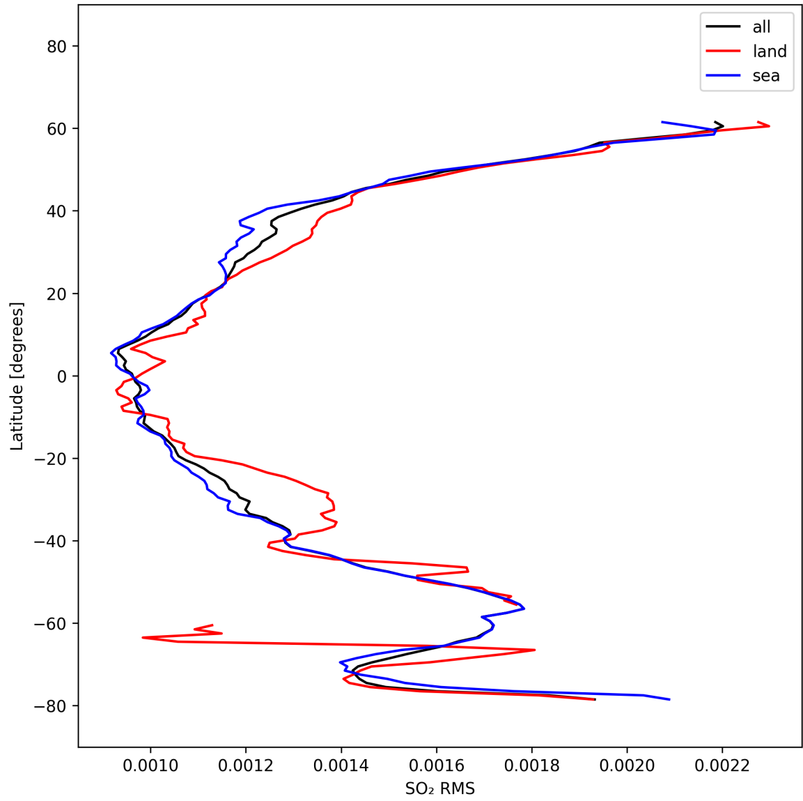
Figure 52: Zonal average of “SO 2 RMS” for 2025-10-14 to 2025-10-15.
