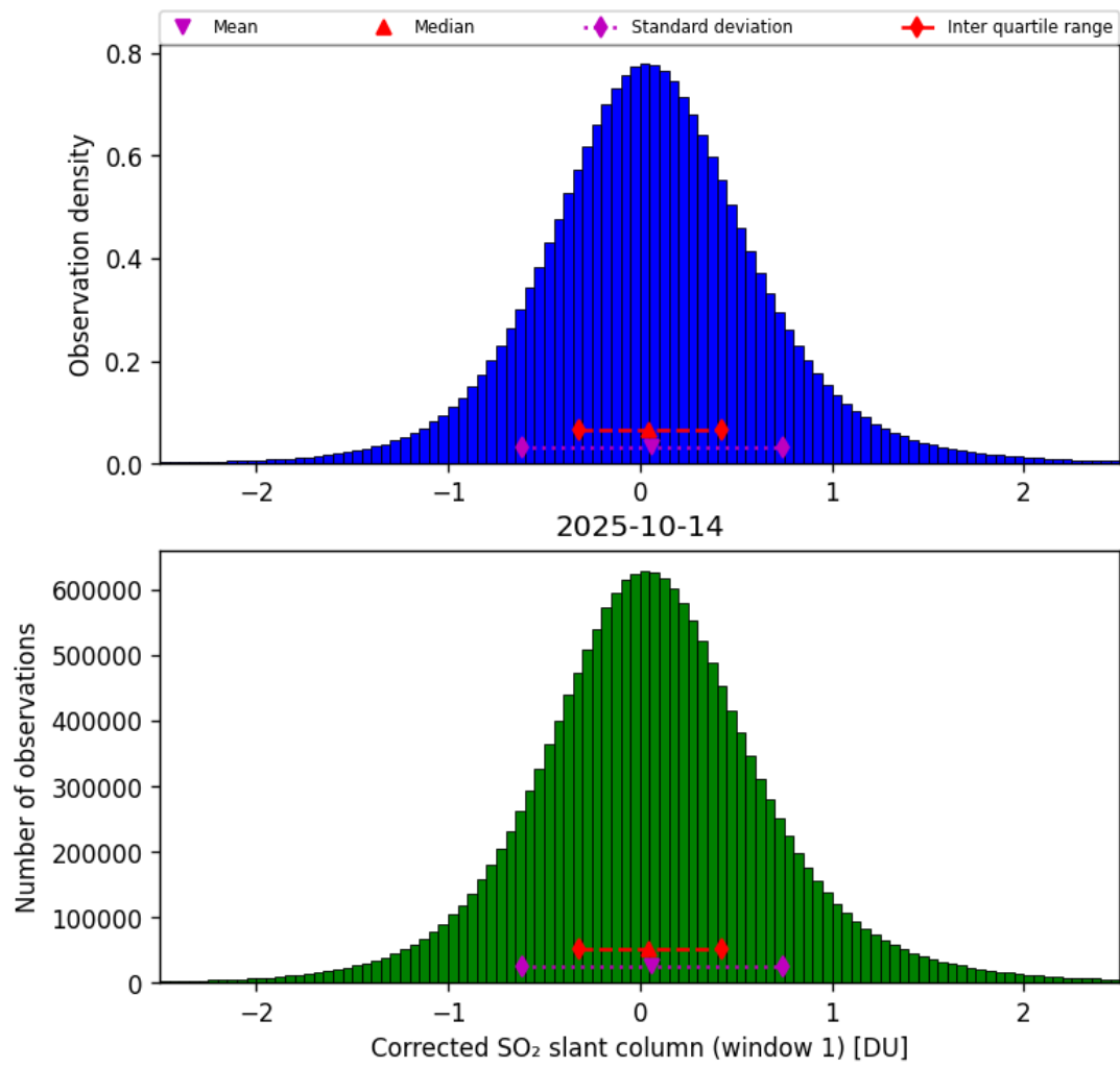
Figure 65: Histogram of “Corrected SO 2 slant column (window 1)” for 2025-10-14 to 2025-10-15
