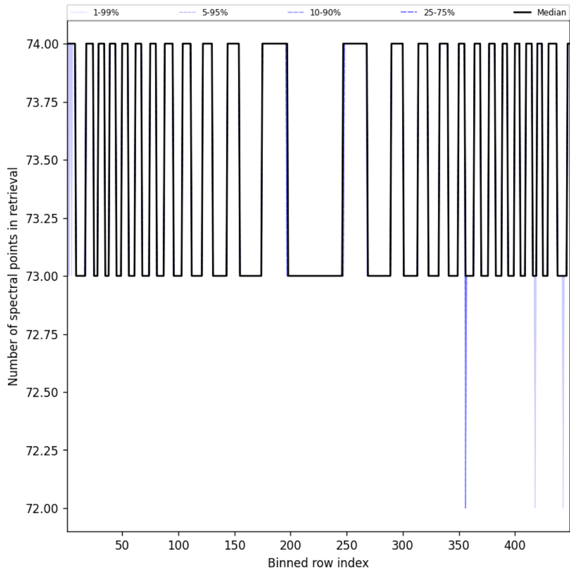
Figure 110: Along track statistics of “Number of spectral points in retrieval” for 2025-10-14 to 2025-10-15
