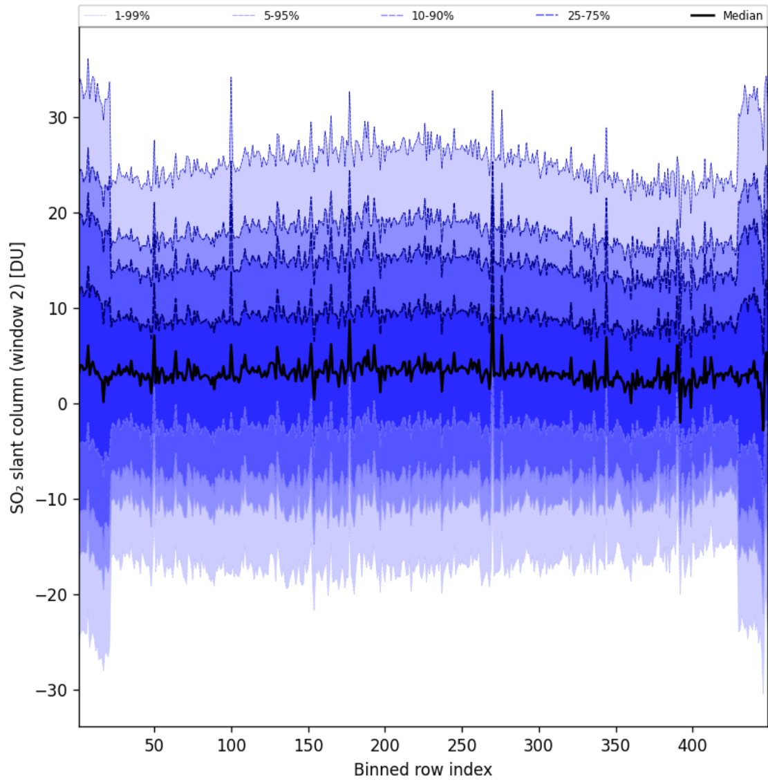
Figure 94: Along track statistics of “SO 2 slant column (window 2)” for 2025-10-14 to 2025-10-15
