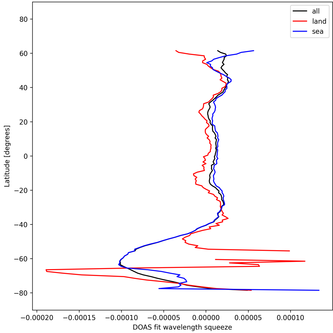
Figure 51: Zonal average of “DOAS fit wavelength squeeze” for 2025-10-14 to 2025-10-15.
