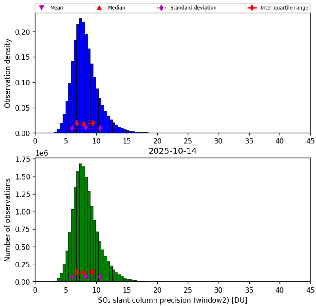
Figure 68: Histogram of “SO 2 slant column precision (window2)” for 2025-10-14 to 2025-10-15
