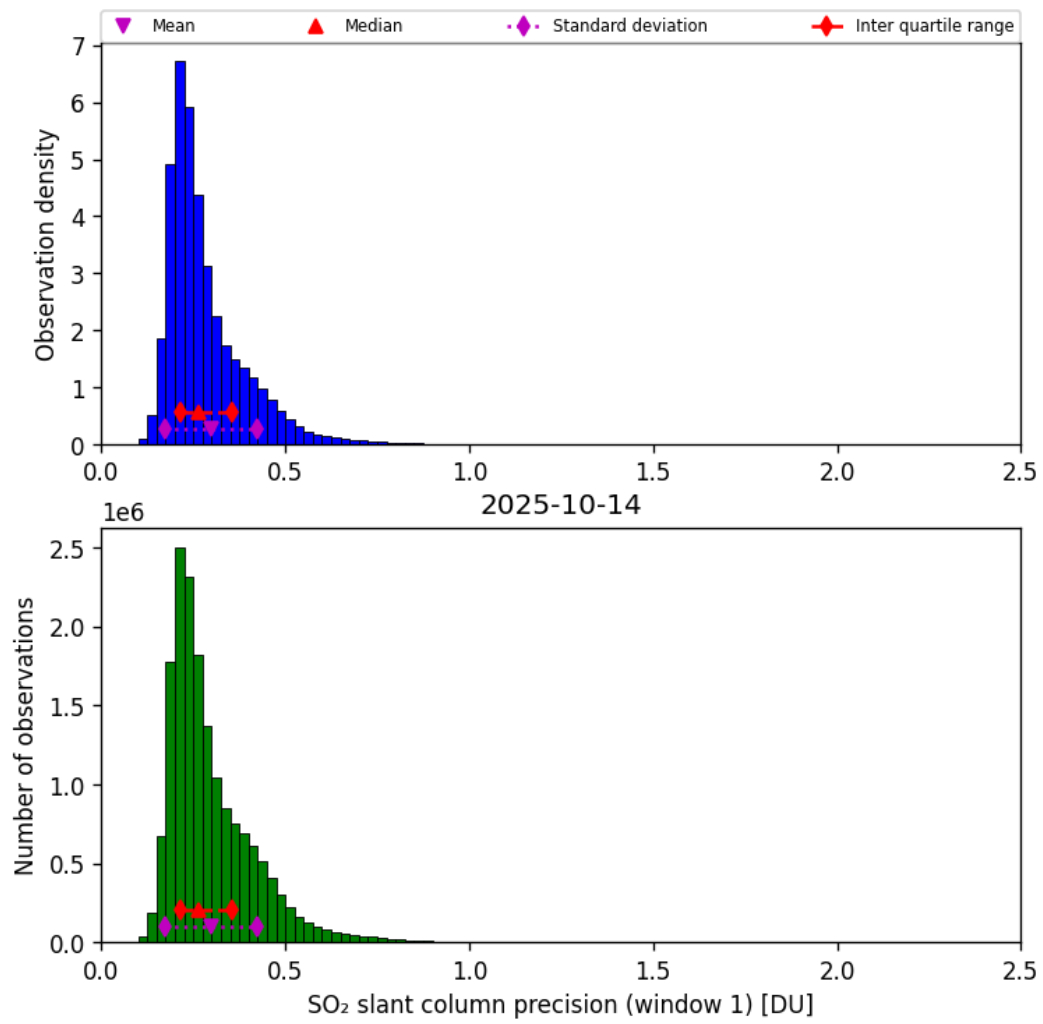
Figure 64: Histogram of “SO 2 slant column precision (window 1)” for 2025-10-14 to 2025-10-15
