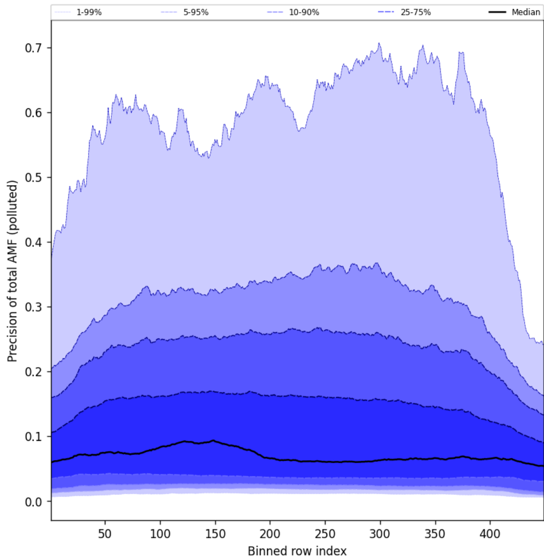
Figure 108: Along track statistics of “Precision of total AMF (polluted)” for 2025-10-14 to 2025-10-15
