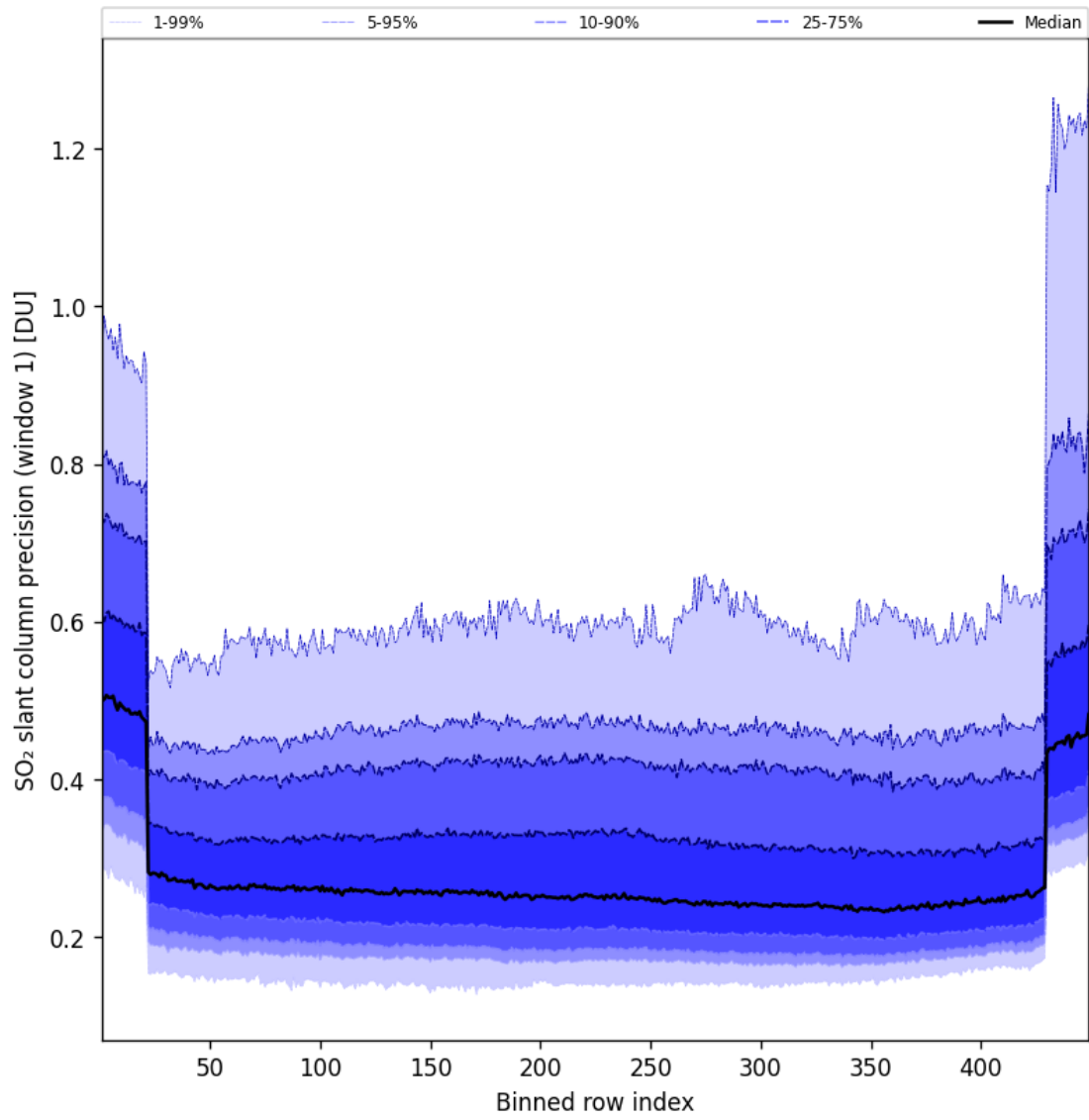
Figure 91: Along track statistics of “SO 2 slant column precision (window 1)” for 2025-10-14 to 2025-10-15
