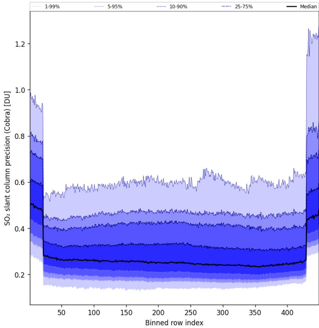
Figure 89: Along track statistics of “SO 2 slant column precision (Cobra)” for 2025-10-14 to 2025-10-15
