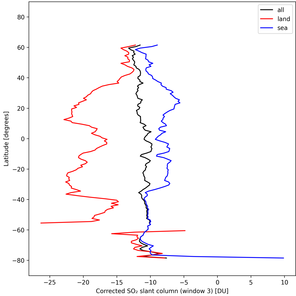
Figure 46: Zonal average of “Corrected SO 2 slant column (window 3)” for 2025-10-14 to 2025-10-15.
