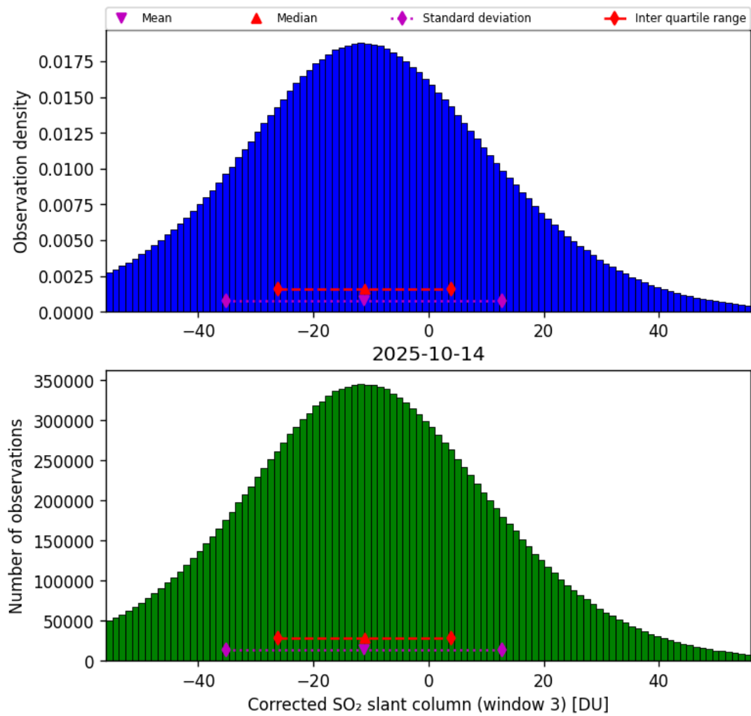
Figure 73: Histogram of “Corrected SO 2 slant column (window 3)” for 2025-10-14 to 2025-10-15
