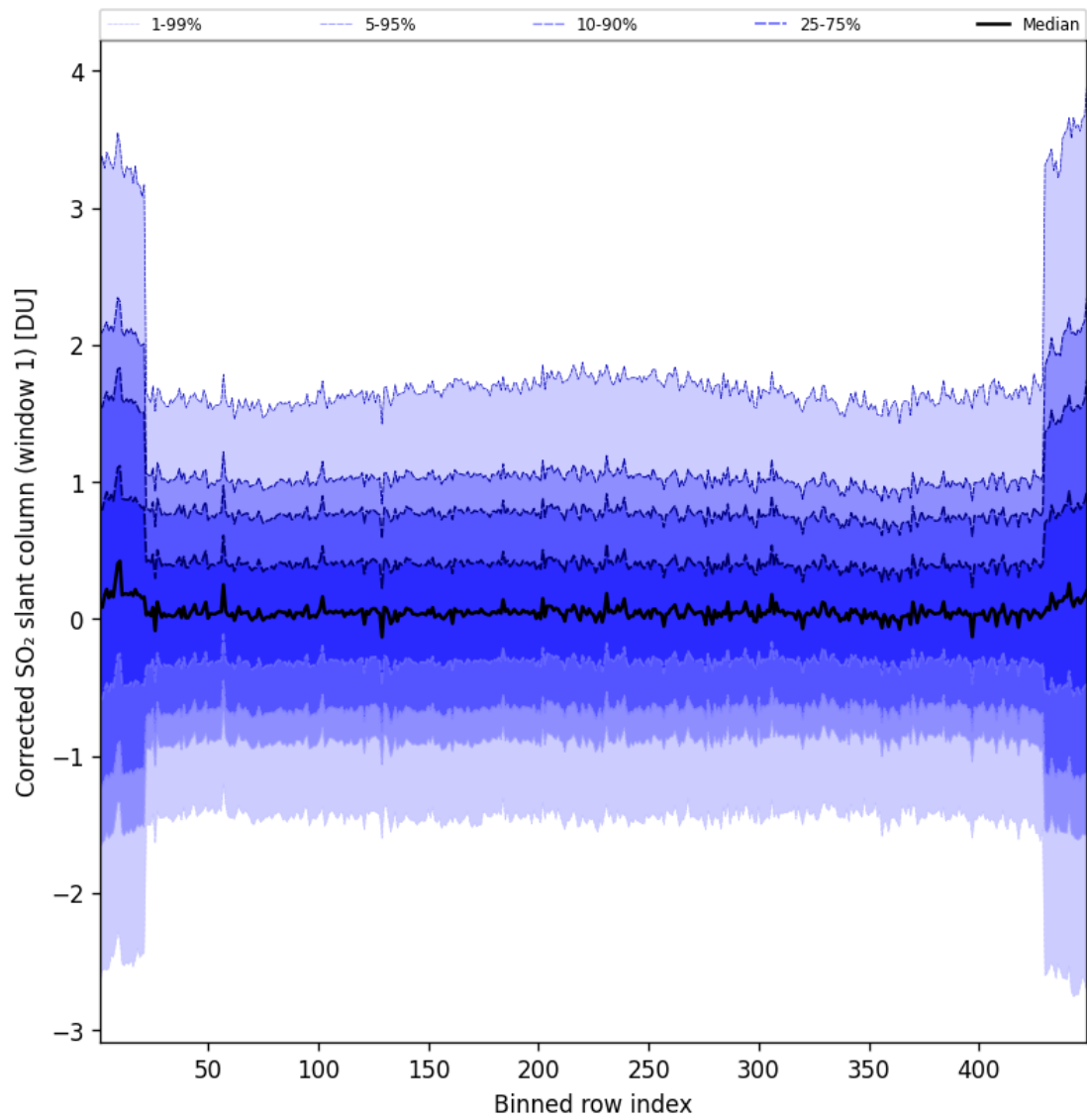
Figure 92: Along track statistics of “Corrected SO 2 slant column (window 1)” for 2025-10-14 to 2025-10-15
