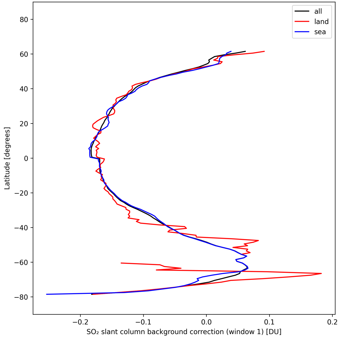
Figure 39: Zonal average of “SO 2 slant column background correction (window 1)” for 2025-10-14 to 2025-10-15.
