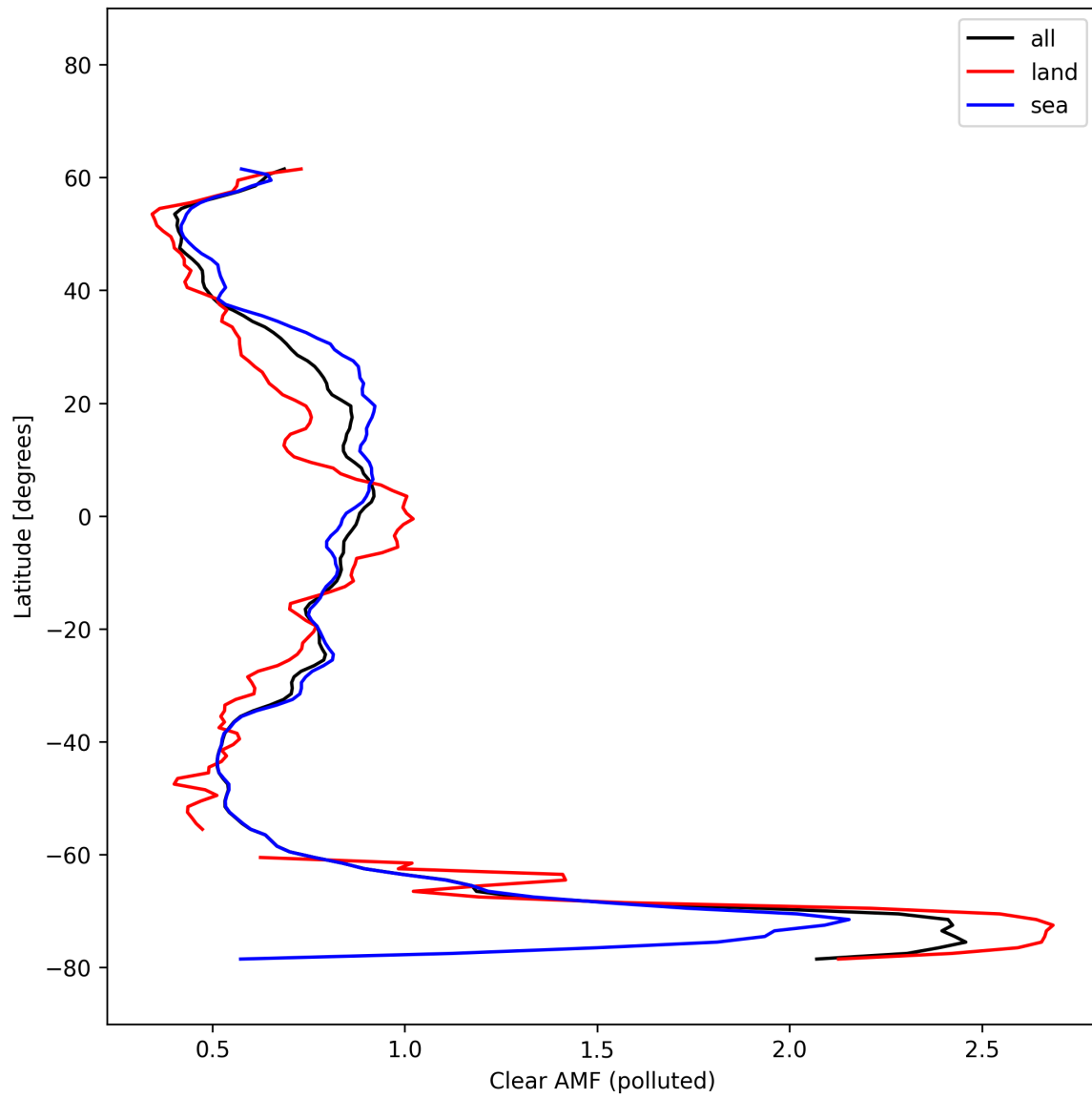
Figure 55: Zonal average of “Clear AMF (polluted)” for 2025-10-14 to 2025-10-15.
