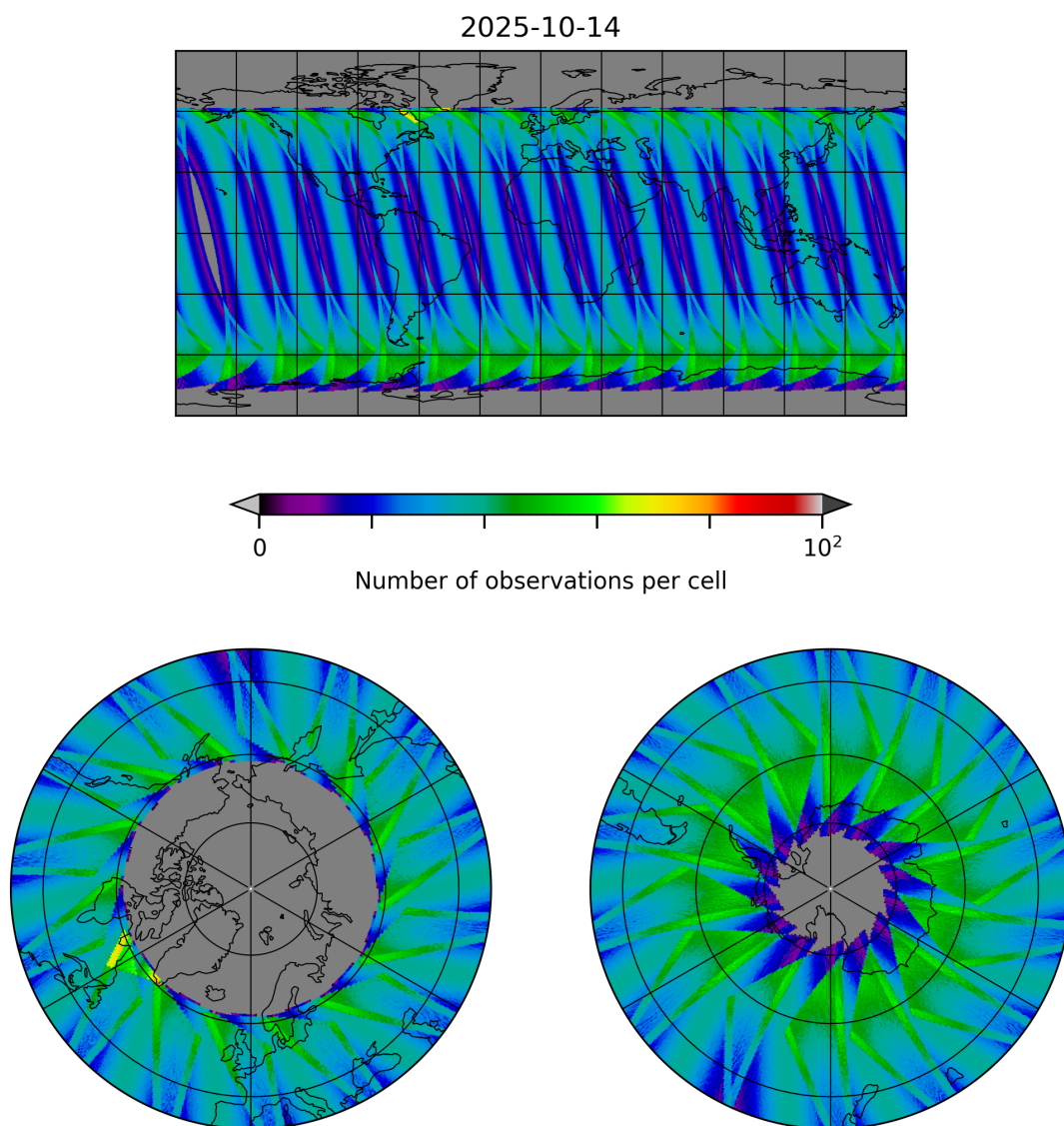
Figure 29: Map of the number of observations for 2025-10-14 to 2025-10-15
