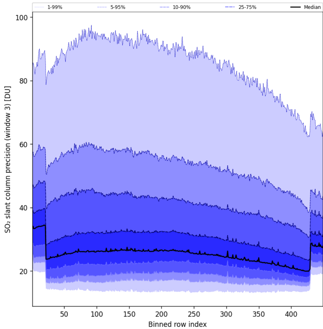
Figure 99: Along track statistics of “SO 2 slant column precision (window 3)” for 2025-10-14 to 2025-10-15
