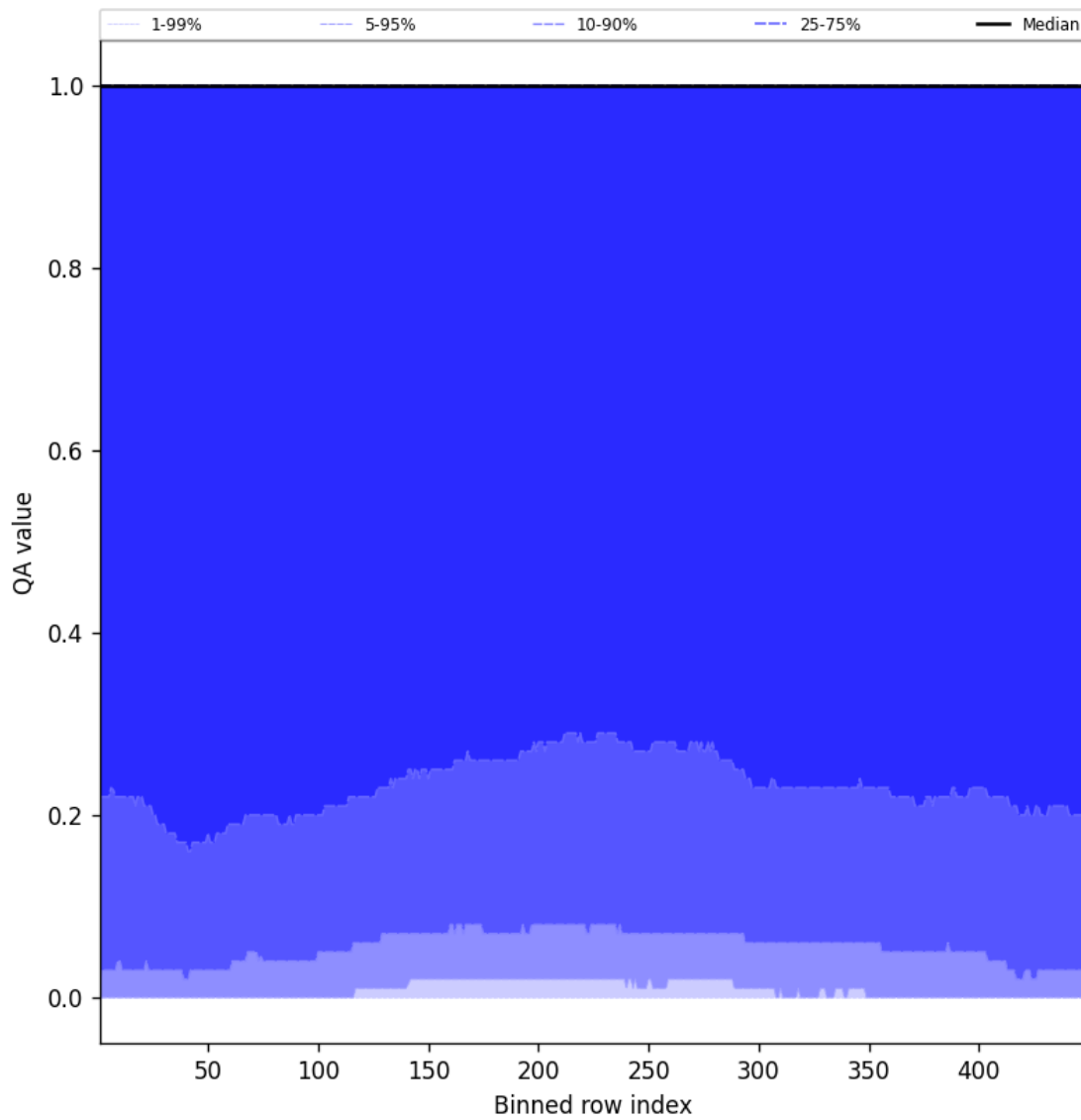
Figure 84: Along track statistics of “QA value” for 2025-10-14 to 2025-10-15
