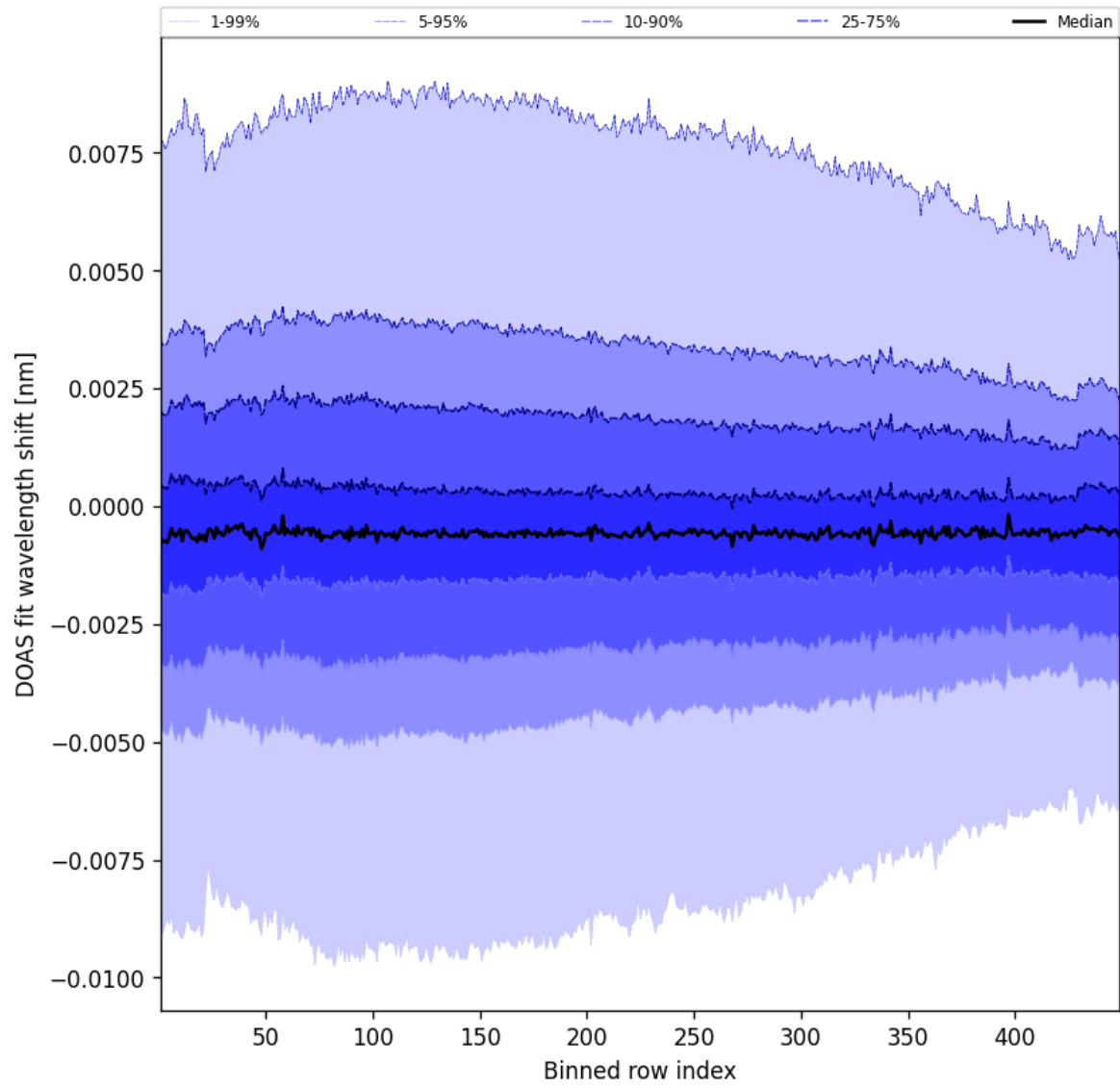
Figure 104: Along track statistics of “DOAS fit wavelength shift” for 2025-10-14 to 2025-10-15
