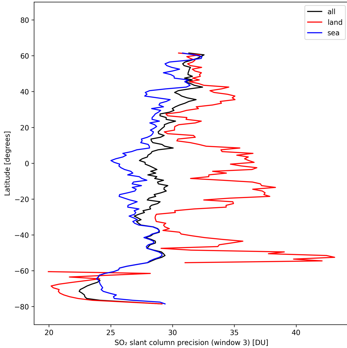
Figure 45: Zonal average of “SO 2 slant column precision (window 3)” for 2025-10-14 to 2025-10-15.
