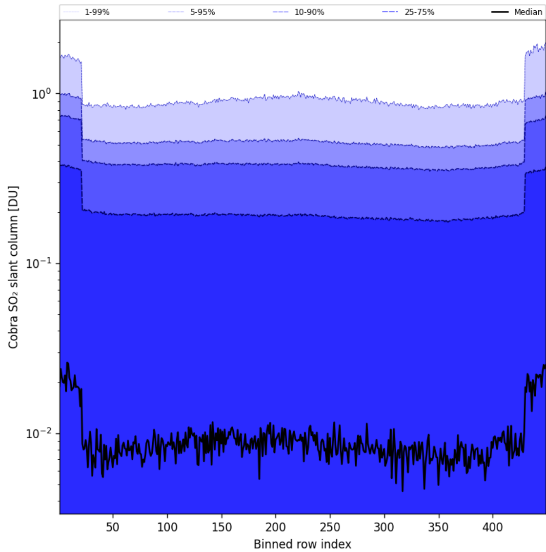
Figure 88: Along track statistics of “Cobra SO 2 slant column” for 2025-10-14 to 2025-10-15
