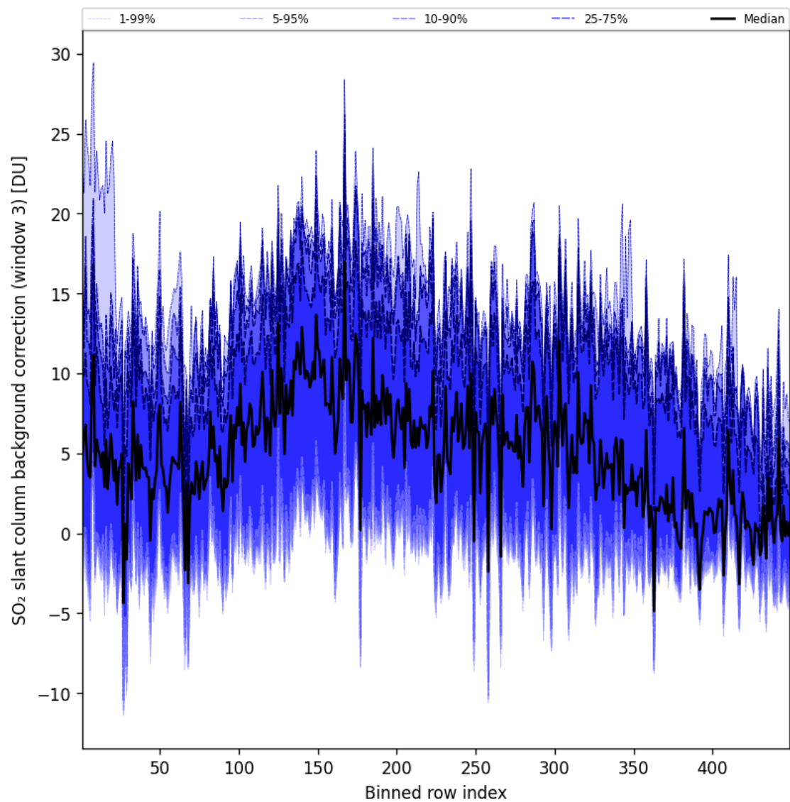
Figure 101: Along track statistics of “SO 2 slant column background correction (window 3)” for 2025-10-14 to 2025-10-15
