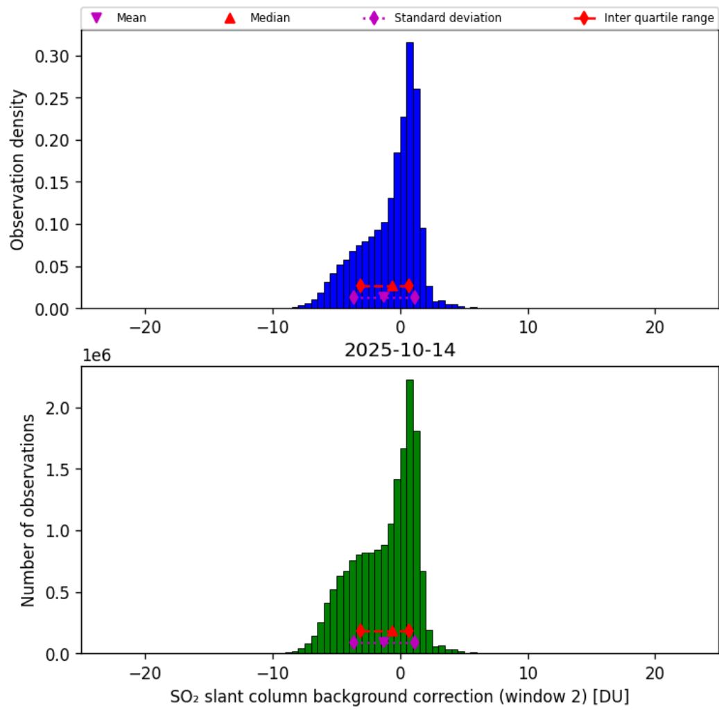
Figure 70: Histogram of “SO 2 slant column background correction (window 2)” for 2025-10-14 to 2025-10-15
