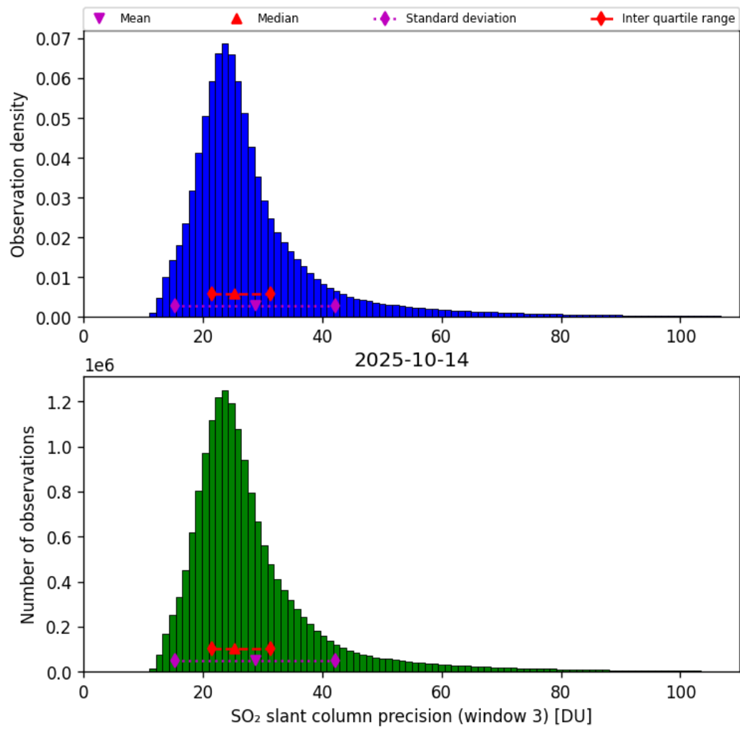
Figure 72: Histogram of “SO 2 slant column precision (window 3)” for 2025-10-14 to 2025-10-15
