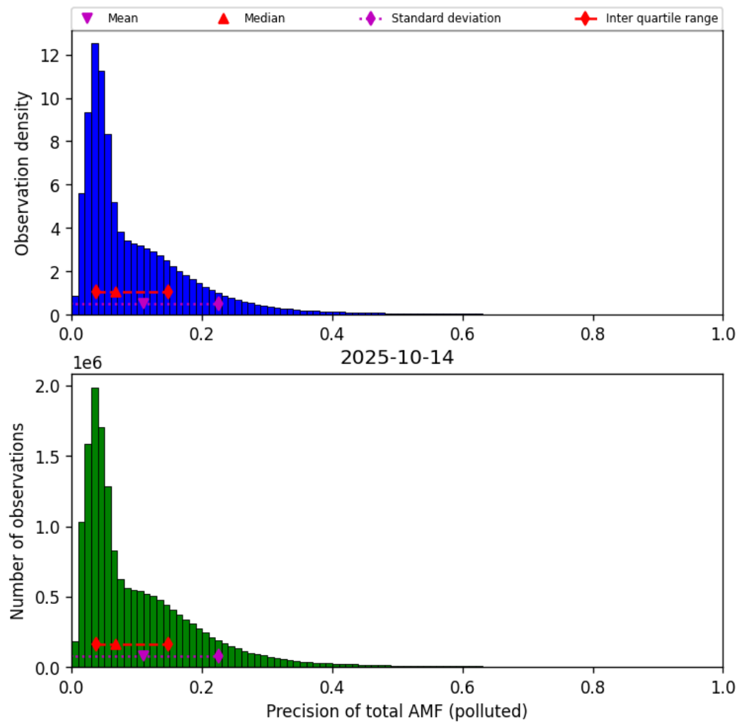
Figure 81: Histogram of “Precision of total AMF (polluted)” for 2025-10-14 to 2025-10-15
