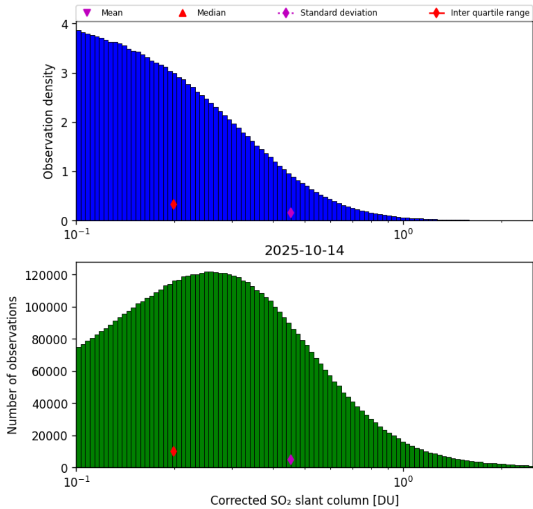
Figure 60: Histogram of "Corrected SO 2 slant column" for 2025-10-14 to 2025-10-15
