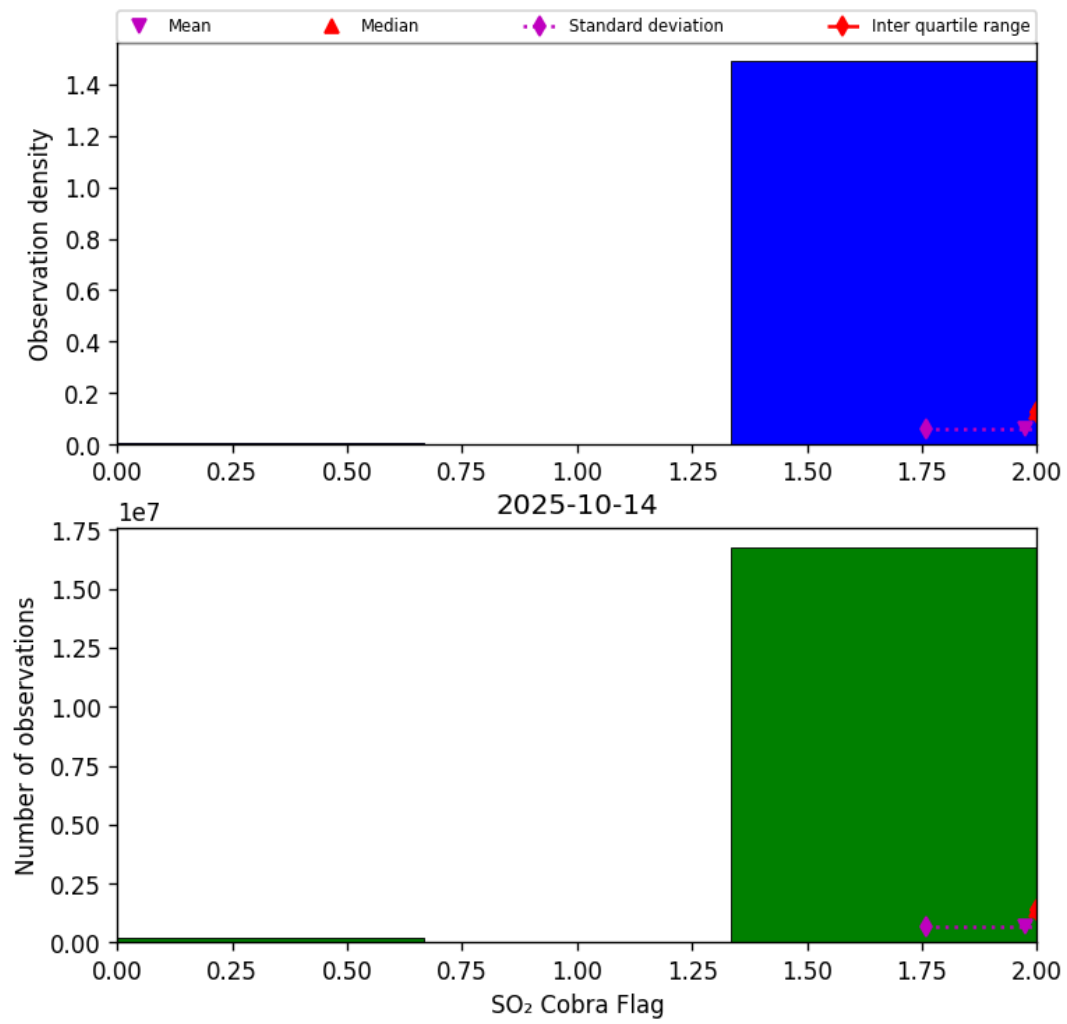
Figure 75: Histogram of “SO 2 Cobra Flag” for 2025-10-14 to 2025-10-15
