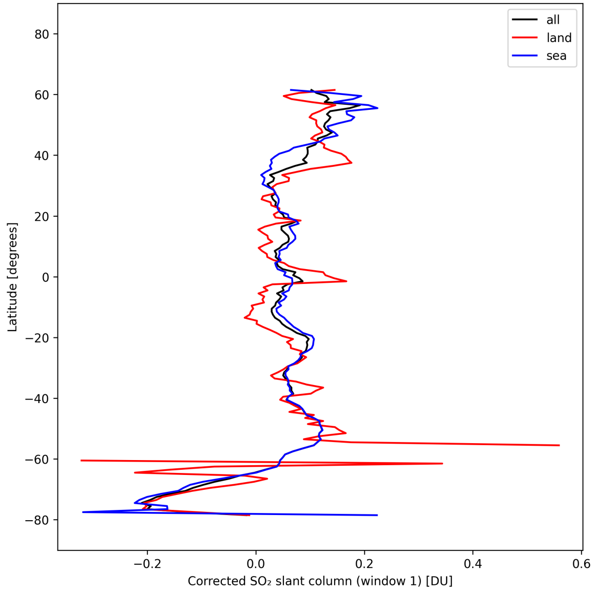
Figure 38: Zonal average of “Corrected SO 2 slant column (window 1)” for 2025-10-14 to 2025-10-15.
