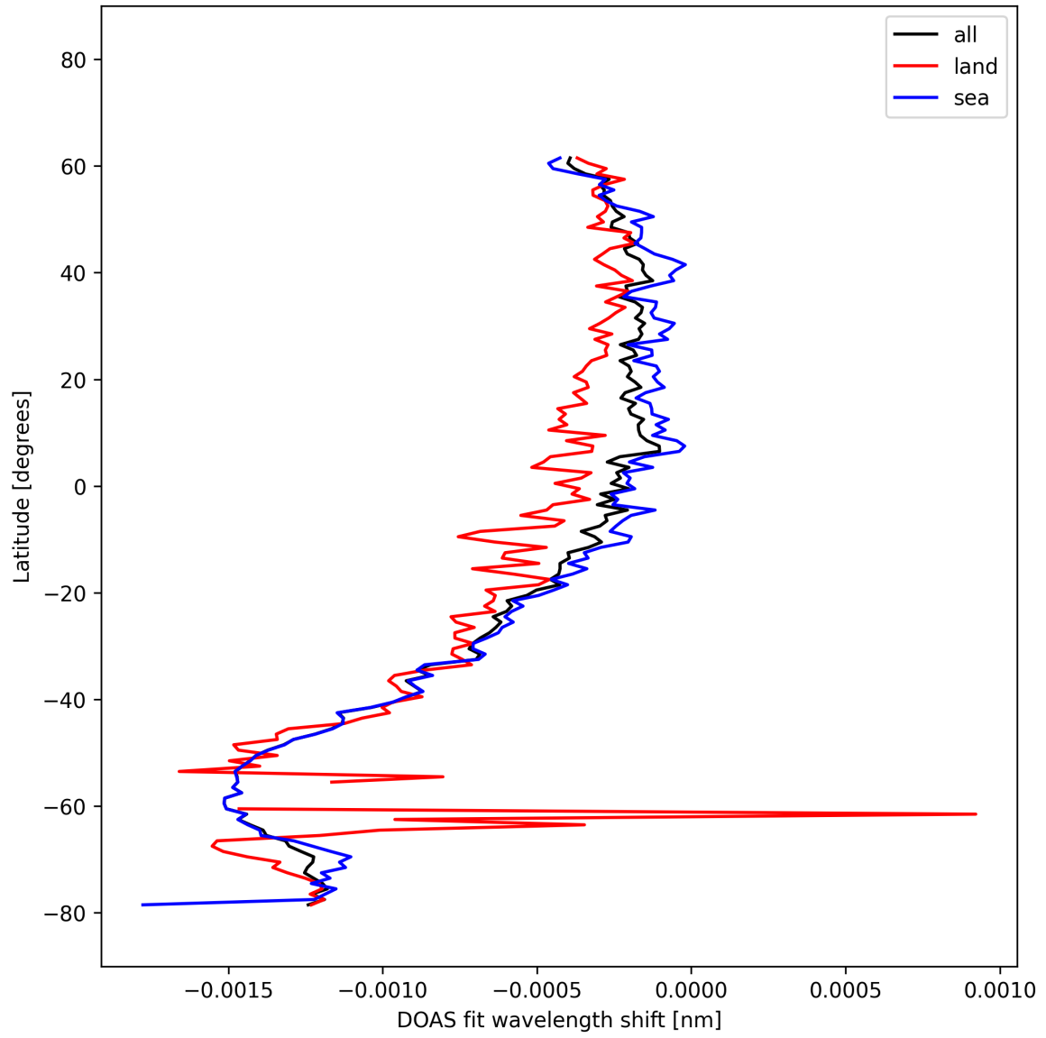
Figure 50: Zonal average of "DOAS fit wavelength shift" for 2025-10-14 to 2025-10-15.
