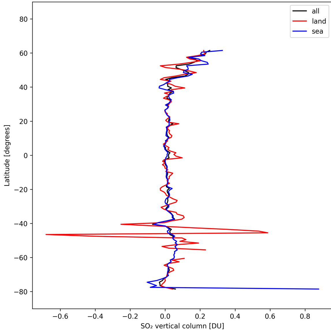
Figure 31: Zonal average of “SO 2 vertical column” for 2025-10-14 to 2025-10-15.
