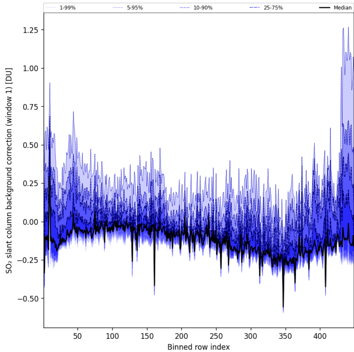
Figure 93: Along track statistics of “SO 2 slant column background correction (window 1)” for 2025-10-14 to 2025-10-15
