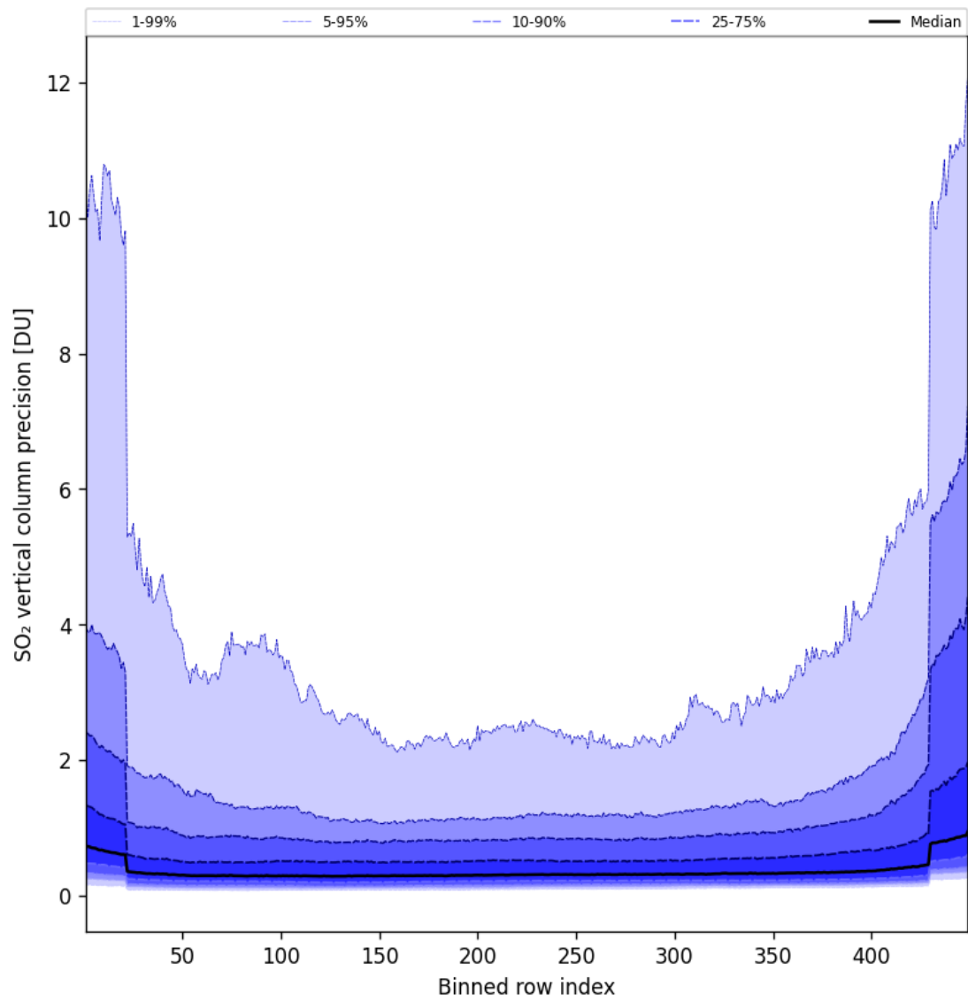
Figure 86: Along track statistics of “SO 2 vertical column precision” for 2025-10-14 to 2025-10-15
