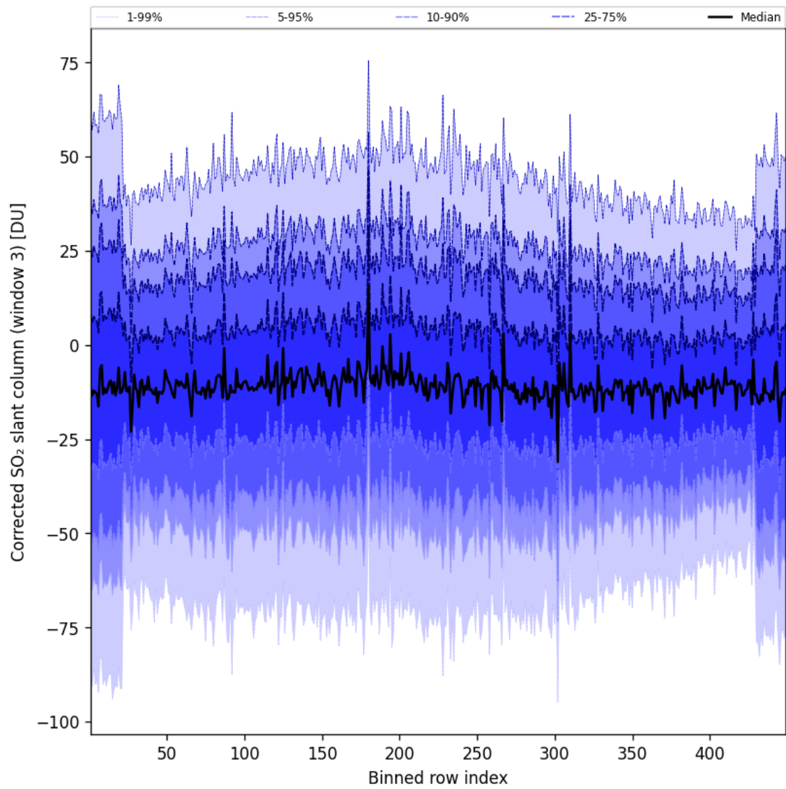
Figure 100: Along track statistics of “Corrected SO 2 slant column (window 3)” for 2025-10-14 to 2025-10-15
