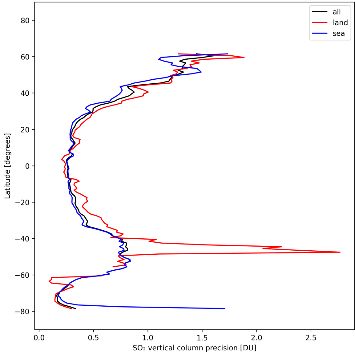
Figure 32: Zonal average of “SO 2 vertical column precision” for 2025-10-14 to 2025-10-15.
