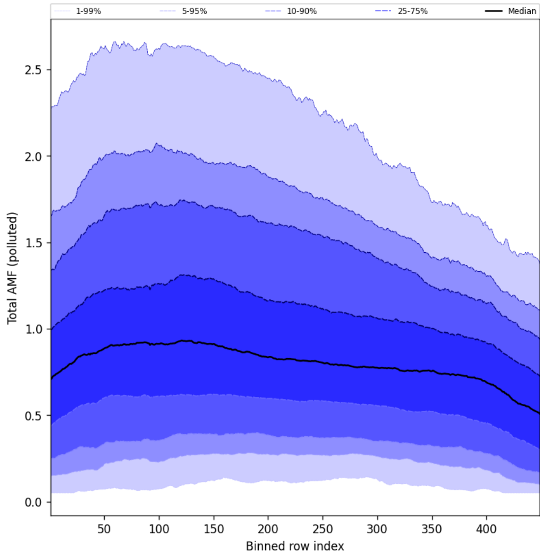
Figure 107: Along track statistics of “Total AMF (polluted)” for 2025-10-14 to 2025-10-15
