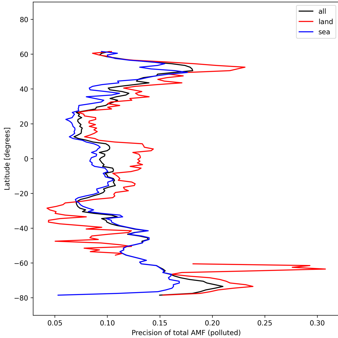
Figure 54: Zonal average of “Precision of total AMF (polluted)” for 2025-10-14 to 2025-10-15.
