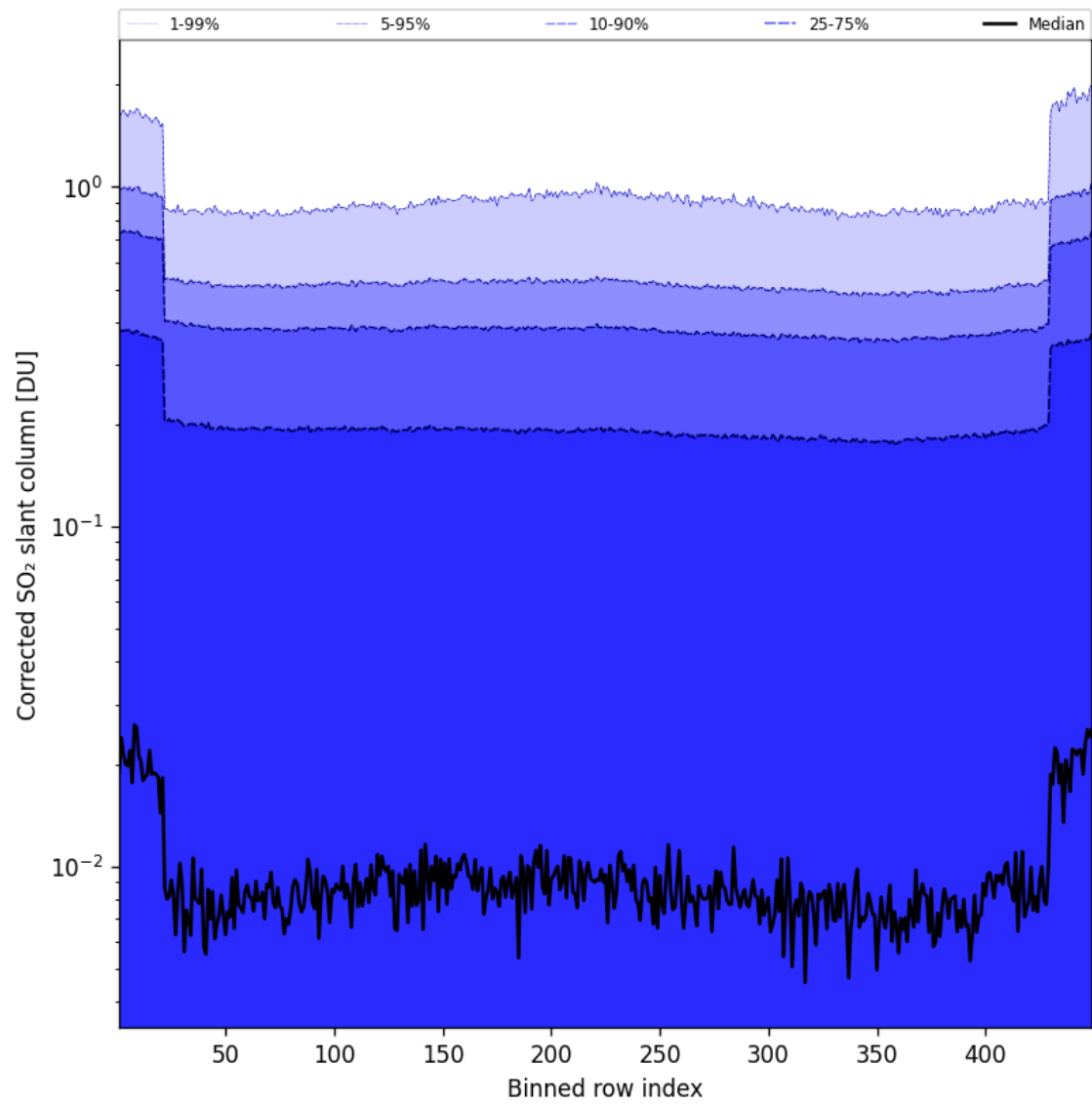
Figure 87: Along track statistics of "Corrected SO 2 slant column" for 2025-10-14 to 2025-10-15
