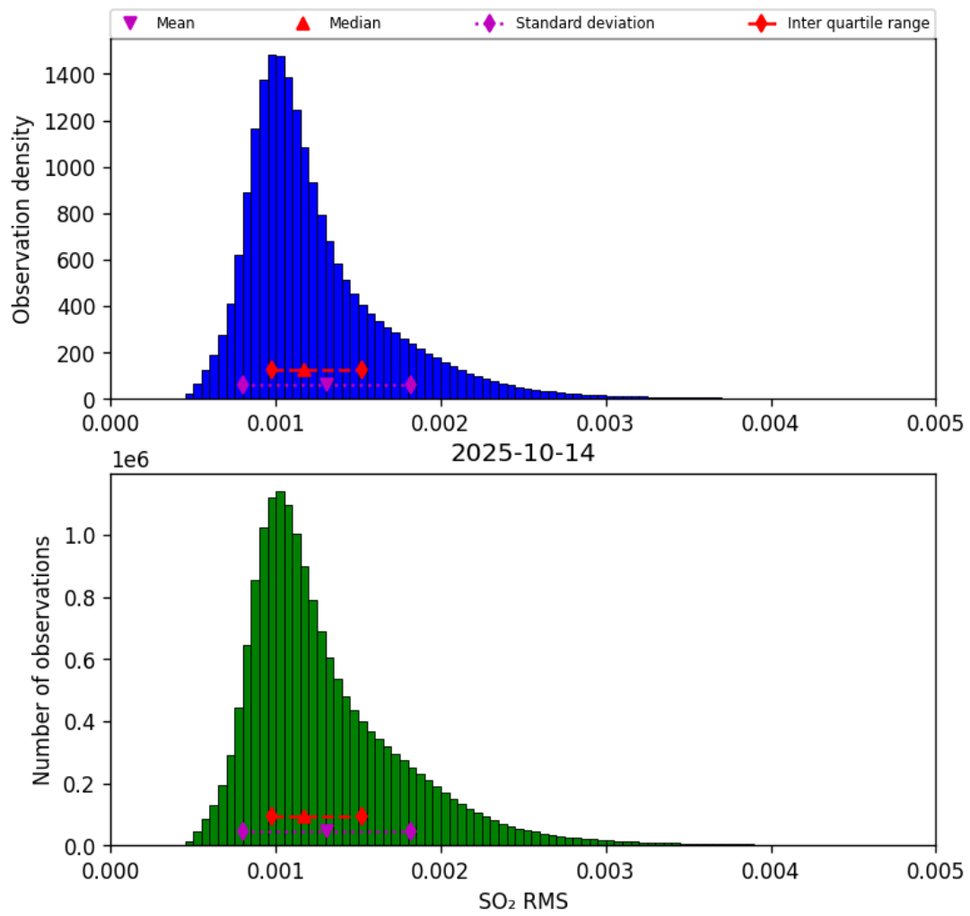
Figure 79: Histogram of “SO 2 RMS” for 2025-10-14 to 2025-10-15
