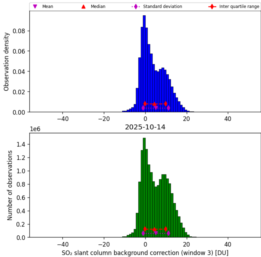
Figure 74: Histogram of “SO 2 slant column background correction (window 3)” for 2025-10-14 to 2025-10-15
