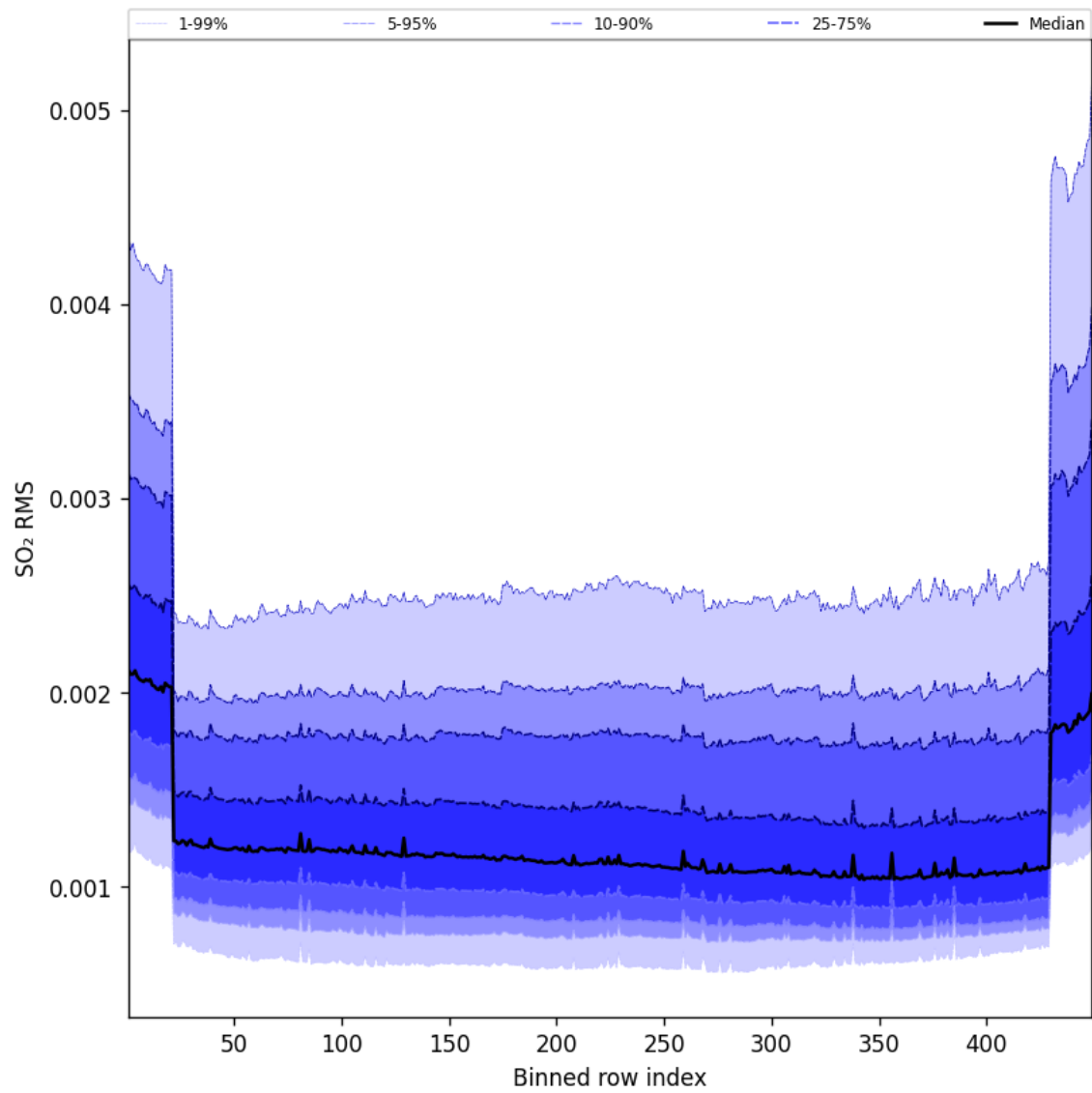
Figure 106: Along track statistics of “SO 2 RMS” for 2025-10-15 to 2025-10-15
