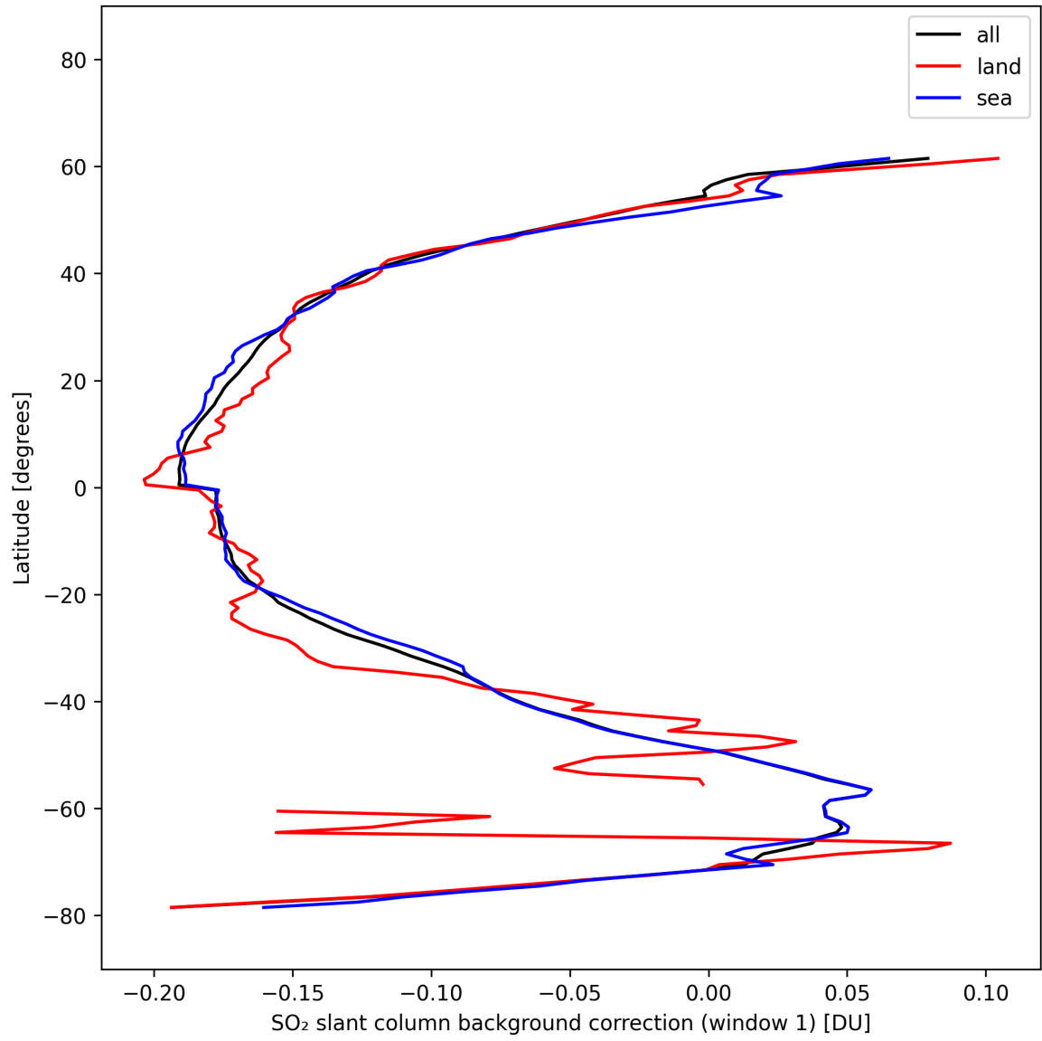
Figure 39: Zonal average of “SO 2 slant column background correction (window 1)” for 2025-10-15 to 2025-10-15.
