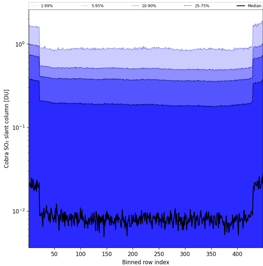
Figure 88: Along track statistics of “Cobra SO 2 slant column” for 2025-10-15 to 2025-10-15
