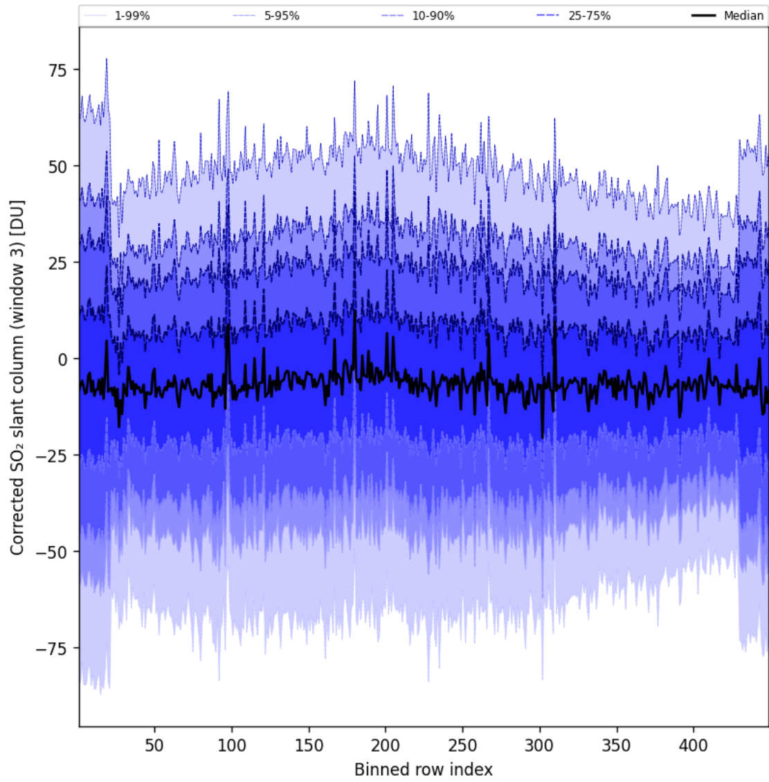
Figure 100: Along track statistics of “Corrected SO 2 slant column (window 3)” for 2025-10-15 to 2025-10-15
