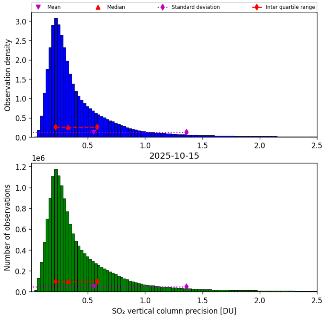
Figure 59: Histogram of “SO 2 vertical column precision” for 2025-10-15 to 2025-10-15
