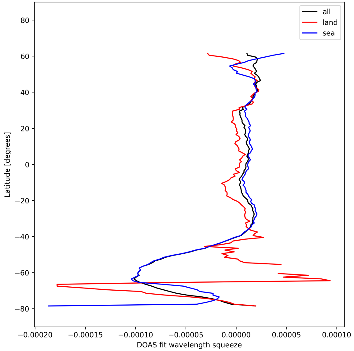
Figure 51: Zonal average of “DOAS fit wavelength squeeze” for 2025-10-15 to 2025-10-15.
