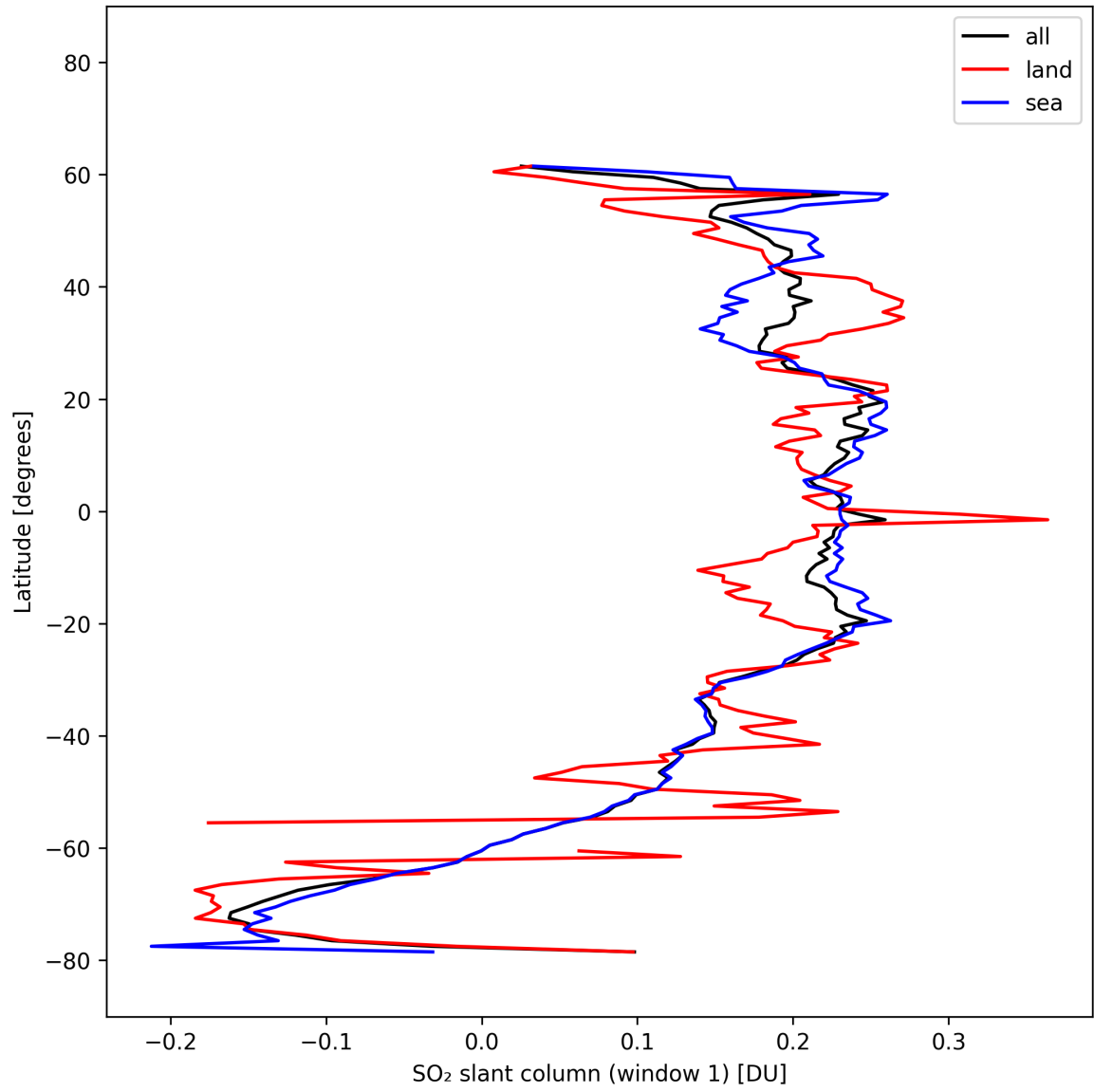
Figure 36: Zonal average of “SO 2 slant column (window 1)” for 2025-10-15 to 2025-10-15.
