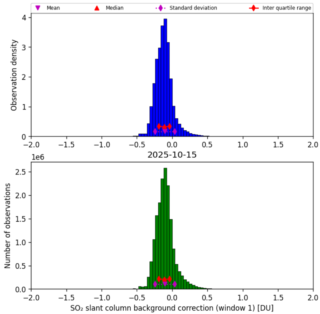
Figure 66: Histogram of “SO 2 slant column background correction (window 1)” for 2025-10-15 to 2025-10-15
