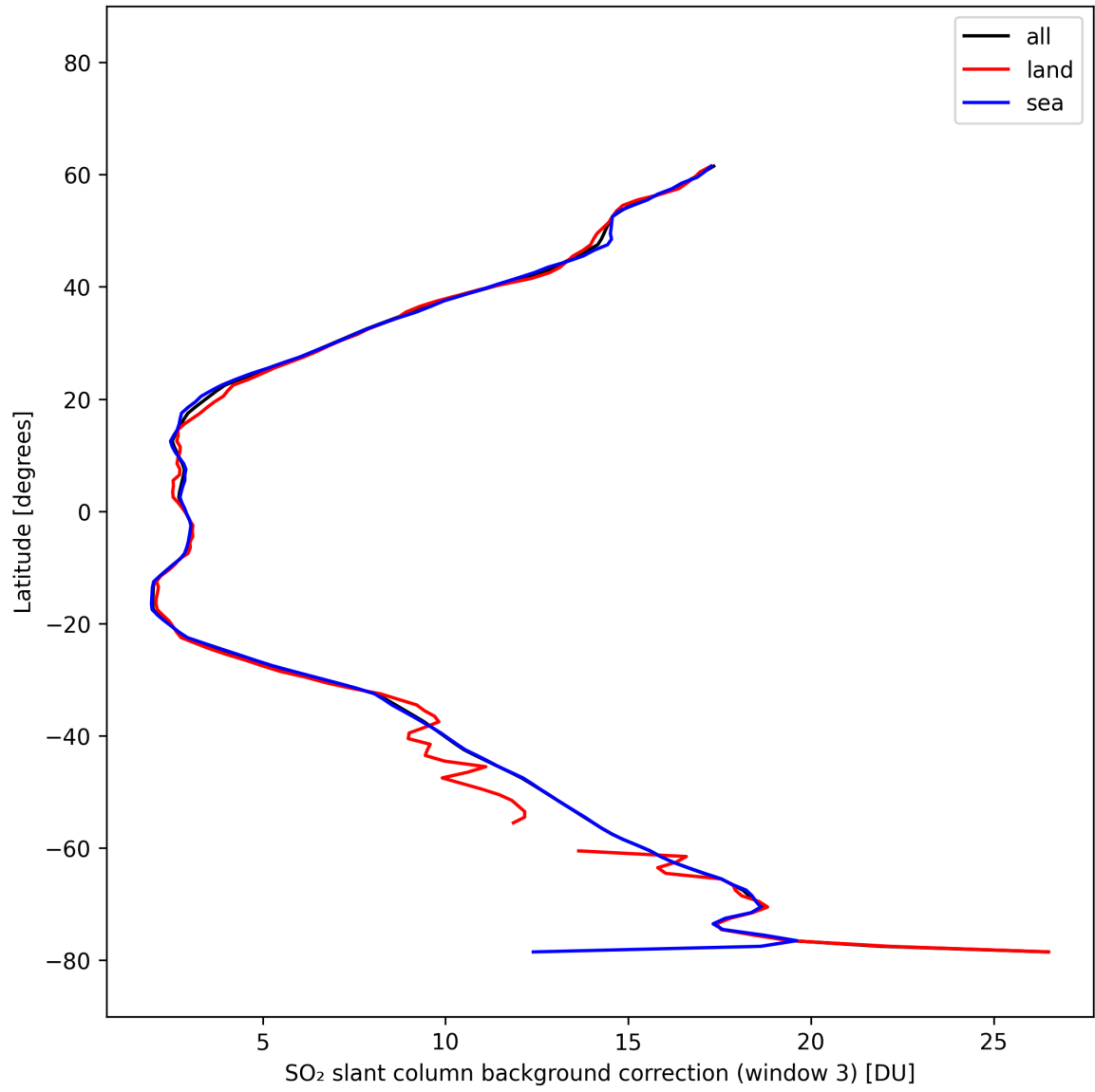
Figure 47: Zonal average of “SO 2 slant column background correction (window 3)” for 2025-10-15 to 2025-10-15.
