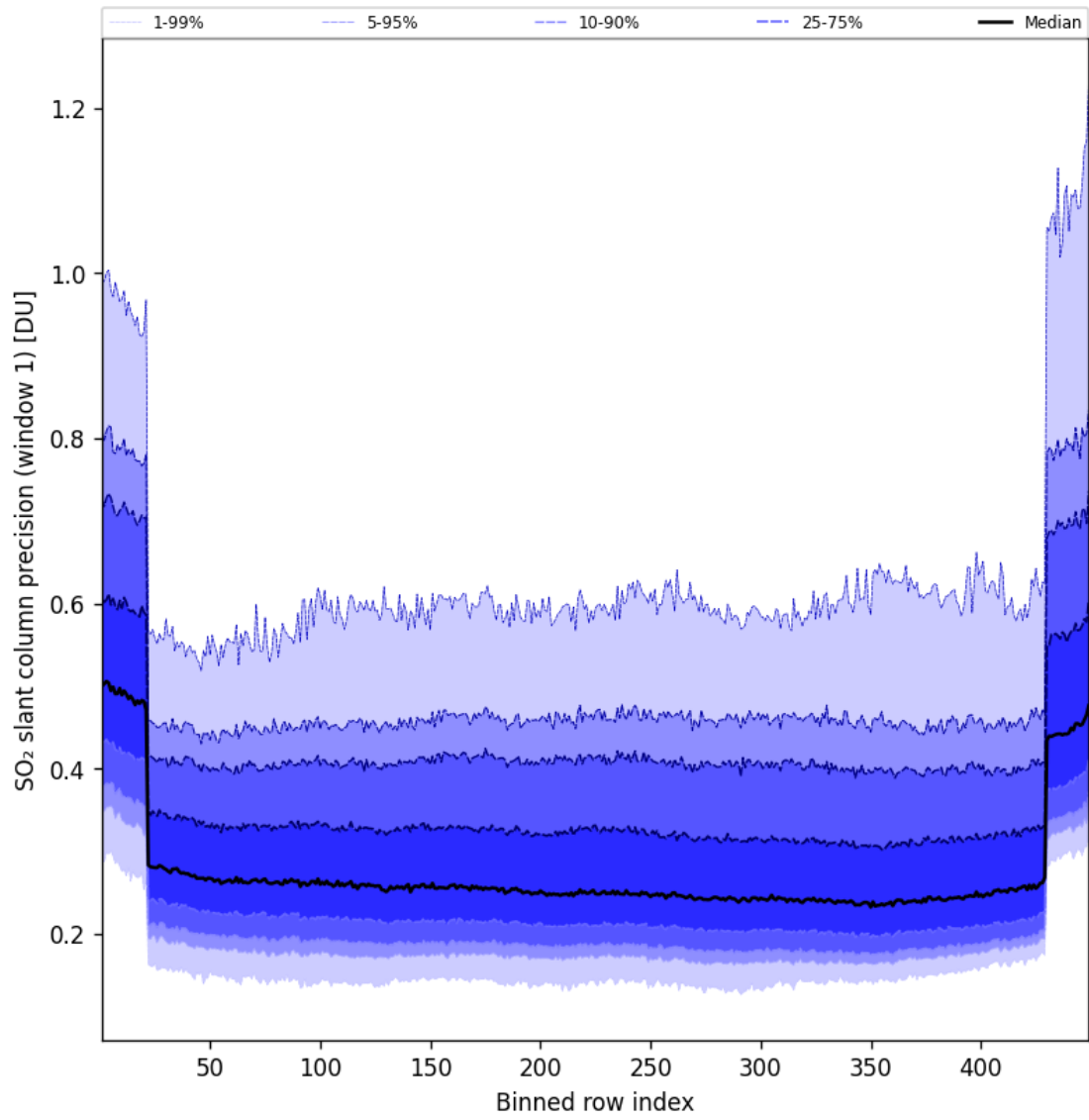
Figure 91: Along track statistics of “SO 2 slant column precision (window 1)” for 2025-10-15 to 2025-10-15
