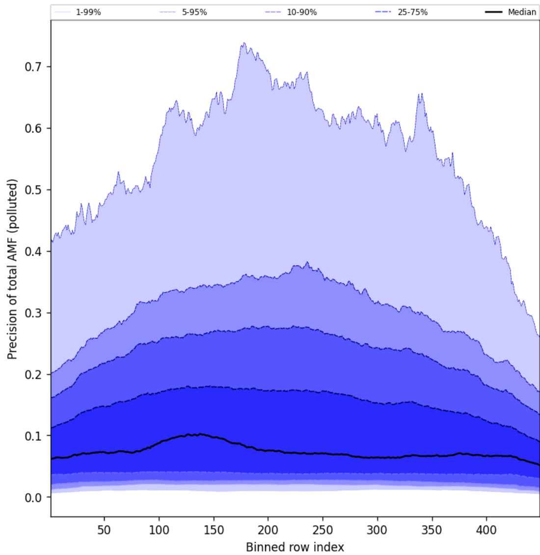
Figure 108: Along track statistics of “Precision of total AMF (polluted)” for 2025-10-15 to 2025-10-15
