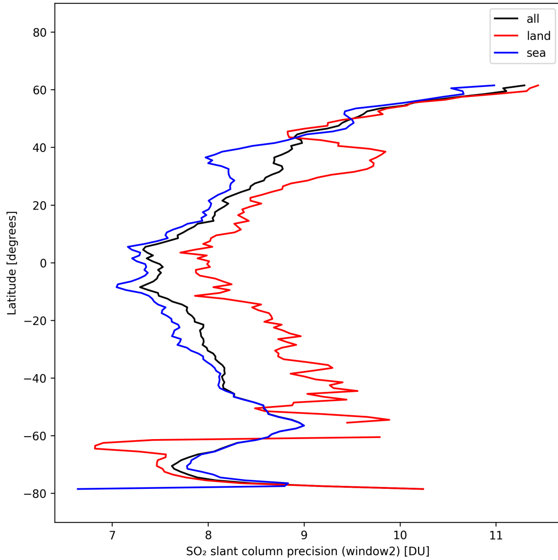
Figure 41: Zonal average of “SO 2 slant column precision (window2)” for 2025-10-15 to 2025-10-15.
