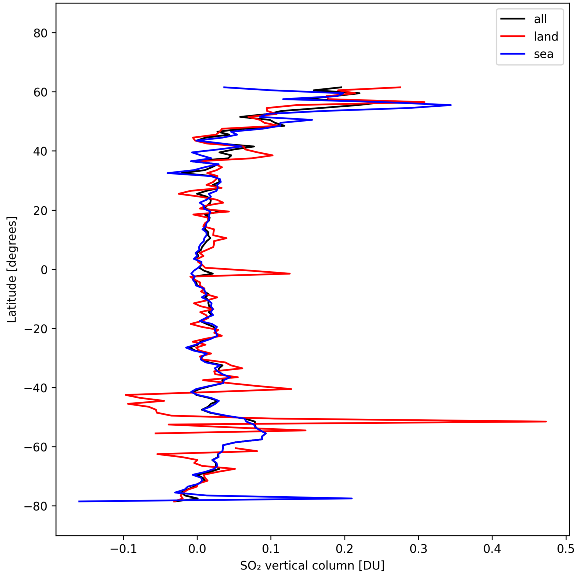
Figure 31: Zonal average of “SO 2 vertical column” for 2025-10-15 to 2025-10-15.
