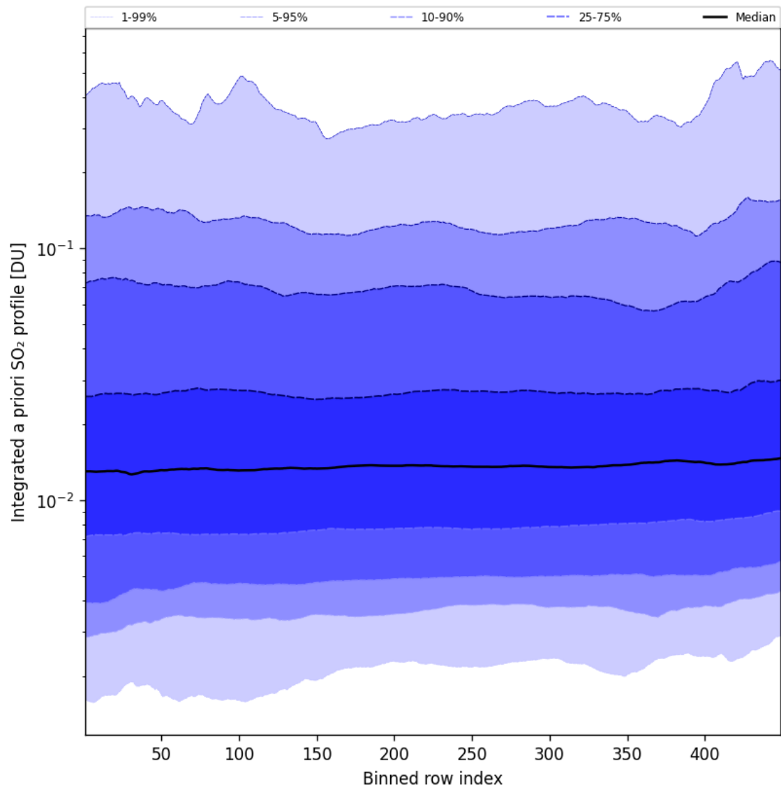
Figure 103: Along track statistics of “Integrated a priori SO 2 profile” for 2025-10-15 to 2025-10-15
