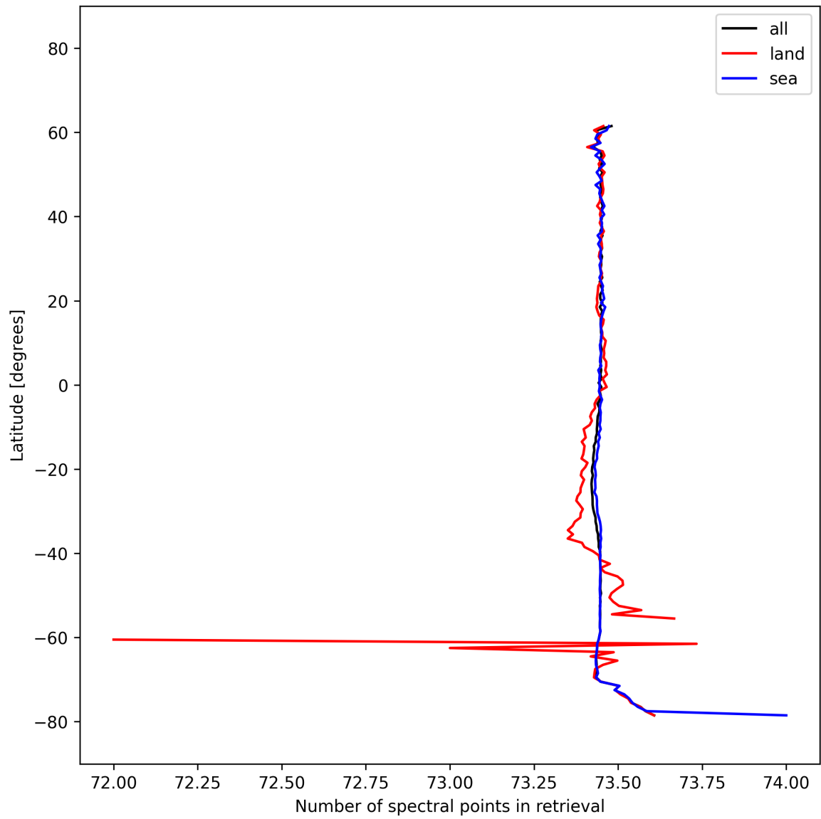
Figure 56: Zonal average of “Number of spectral points in retrieval” for 2025-10-15 to 2025-10-15.
