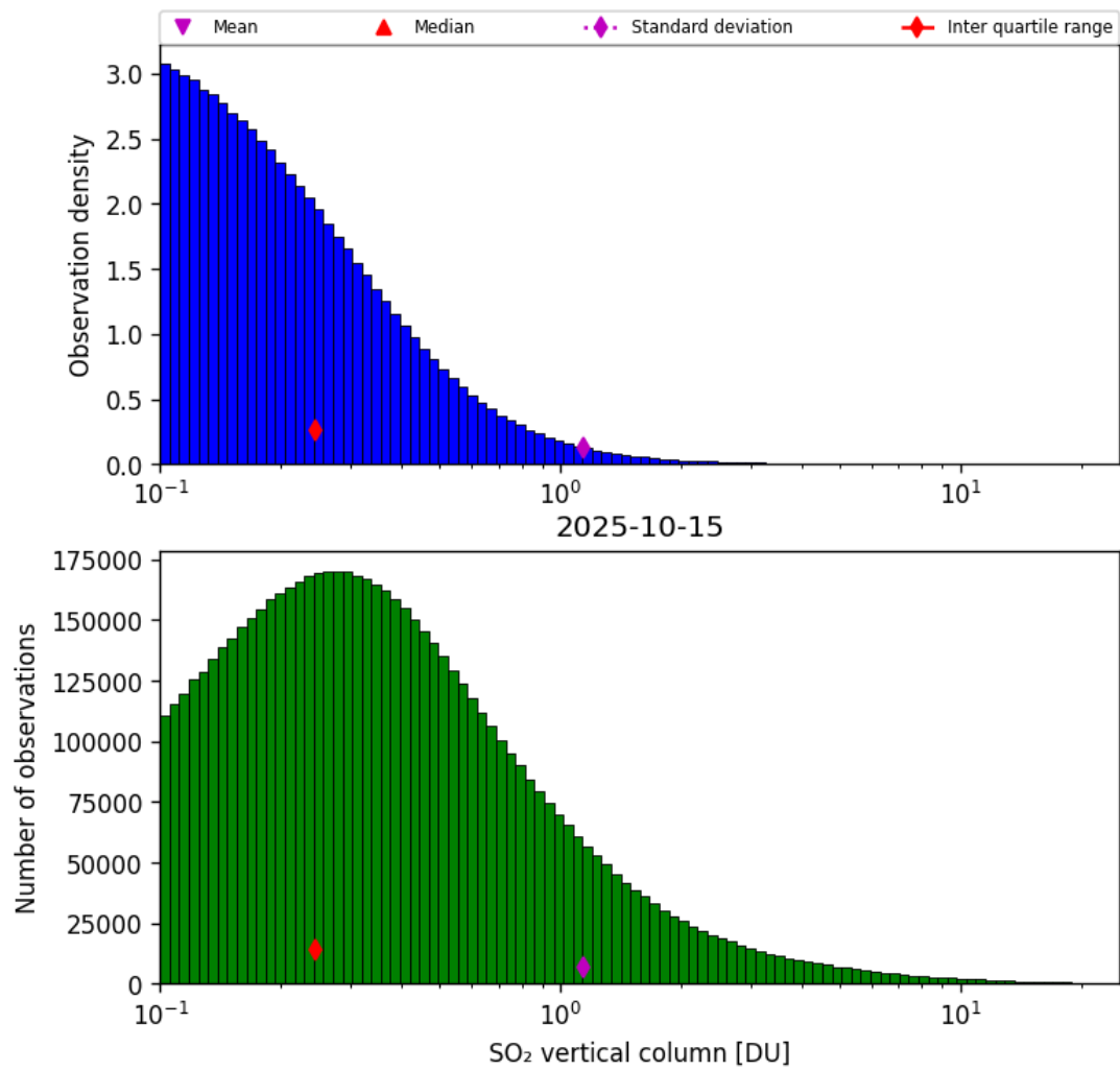
Figure 58: Histogram of “SO 2 vertical column” for 2025-10-15 to 2025-10-15
