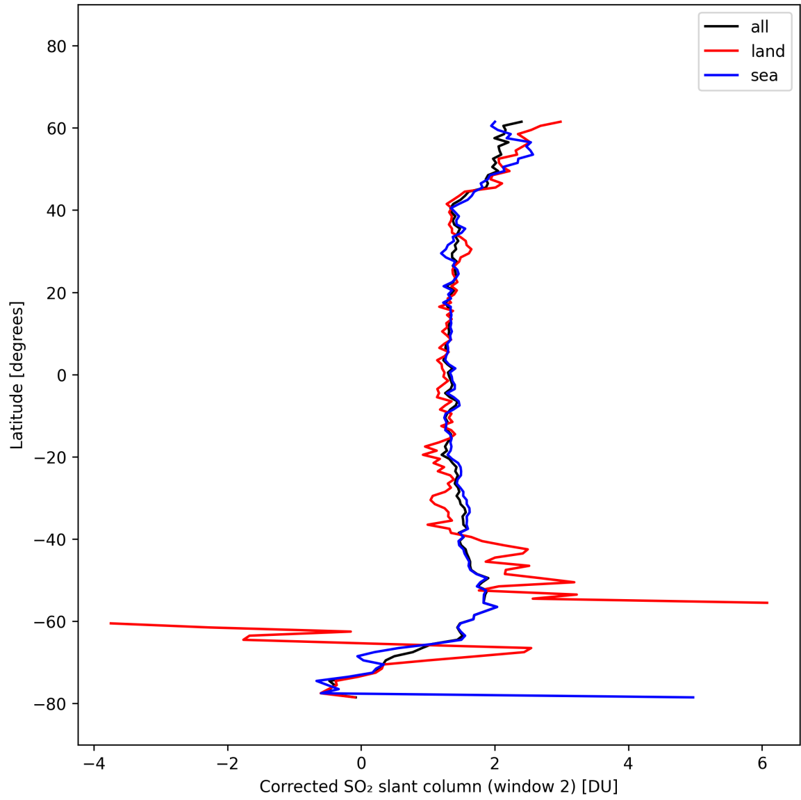
Figure 42: Zonal average of “Corrected SO 2 slant column (window 2)” for 2025-10-15 to 2025-10-15.
