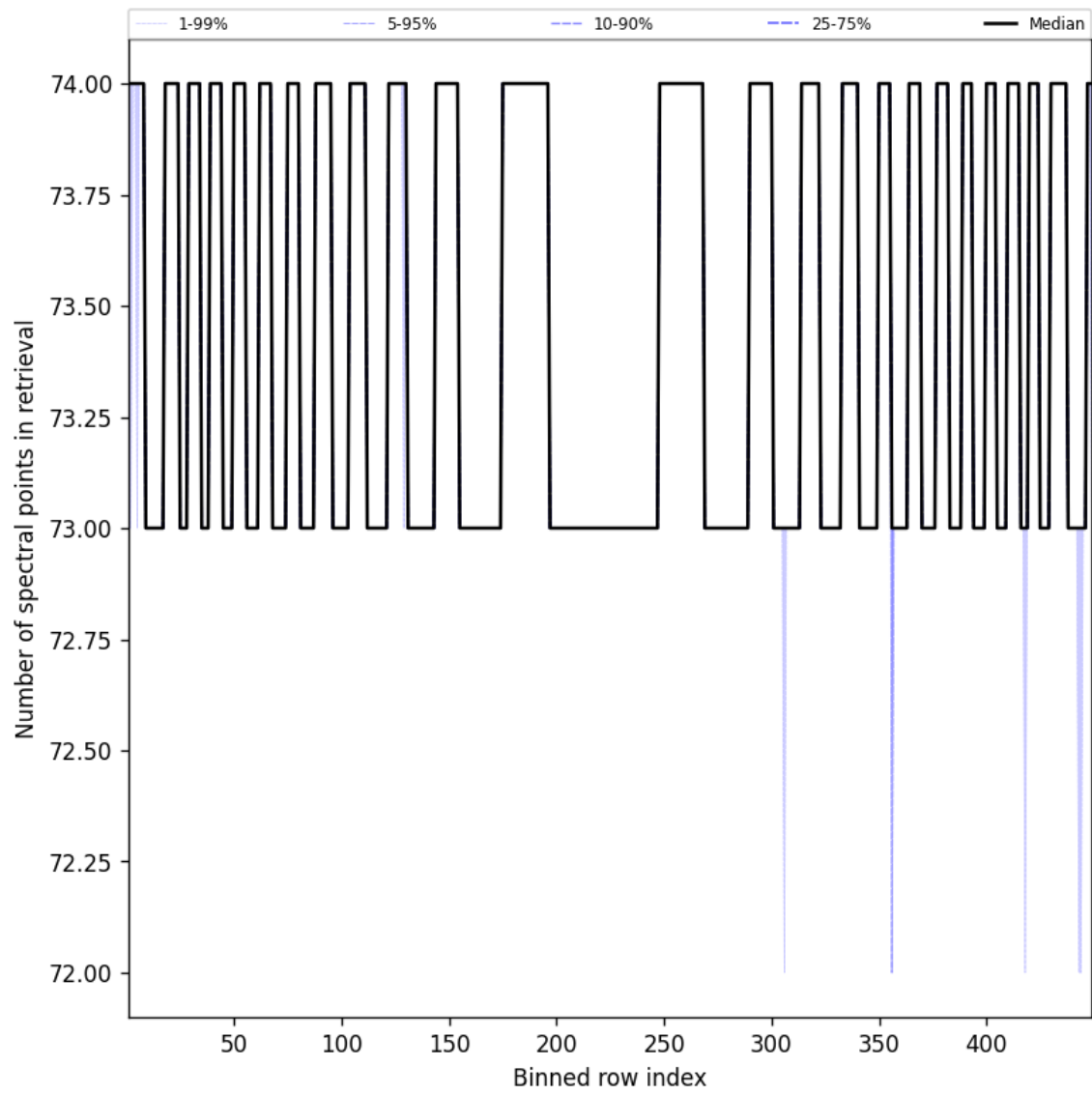
Figure 110: Along track statistics of “Number of spectral points in retrieval” for 2025-10-15 to 2025-10-15
