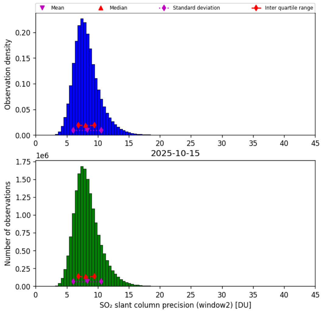
Figure 68: Histogram of “SO 2 slant column precision (window2)” for 2025-10-15 to 2025-10-15
