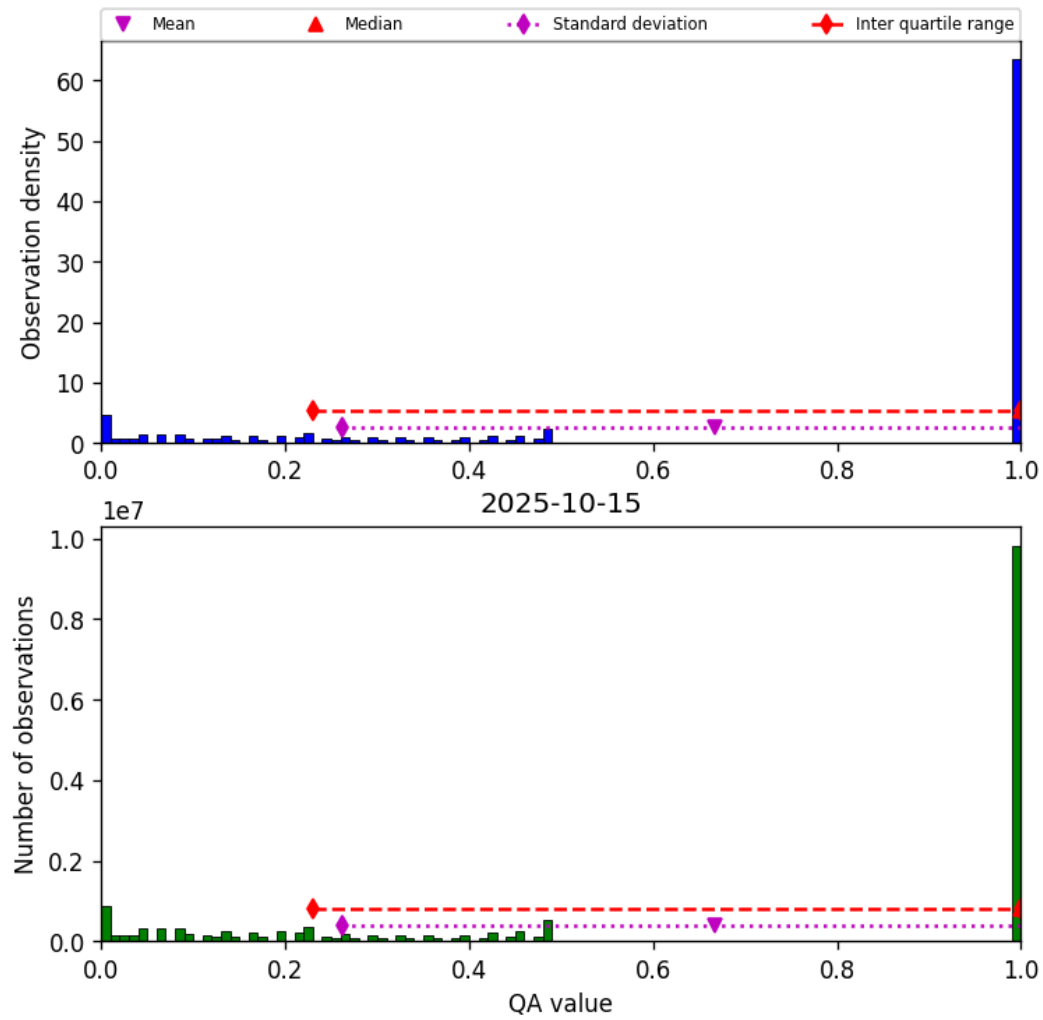
Figure 57: Histogram of “QA value” for 2025-10-15 to 2025-10-15
