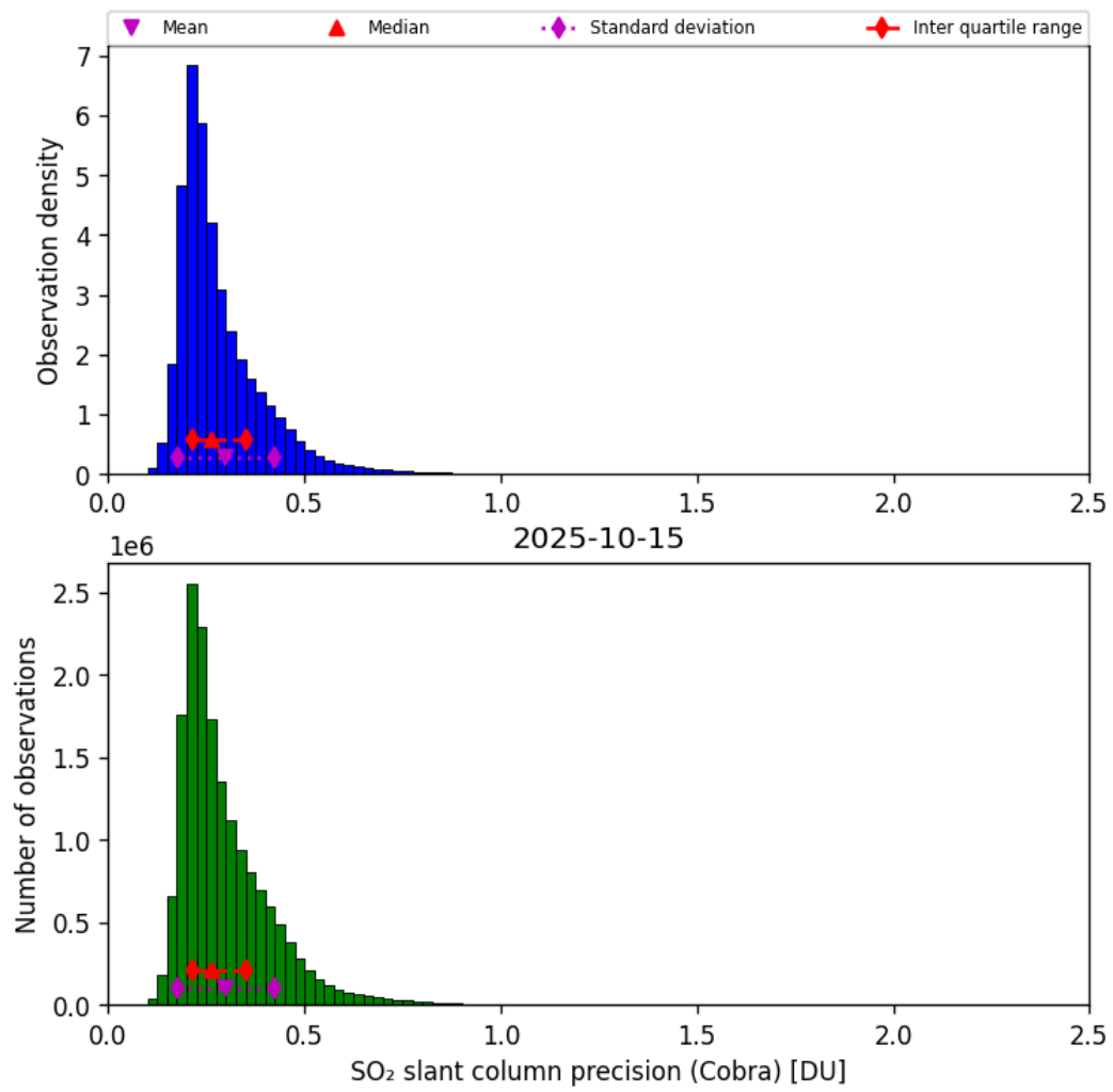
Figure 62: Histogram of “SO 2 slant column precision (Cobra)” for 2025-10-15 to 2025-10-15
