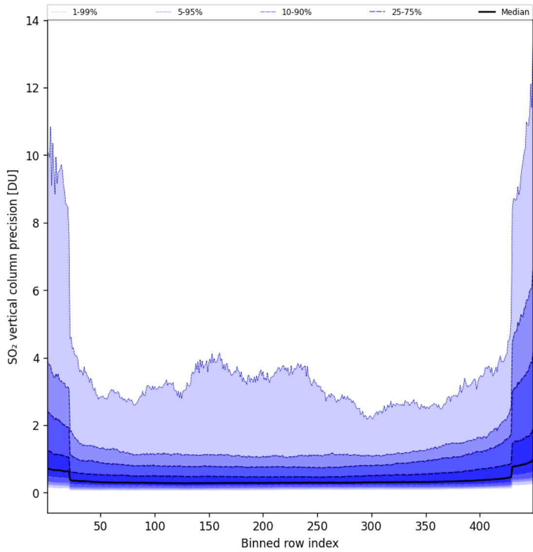
Figure 86: Along track statistics of “SO 2 vertical column precision” for 2025-10-15 to 2025-10-15
