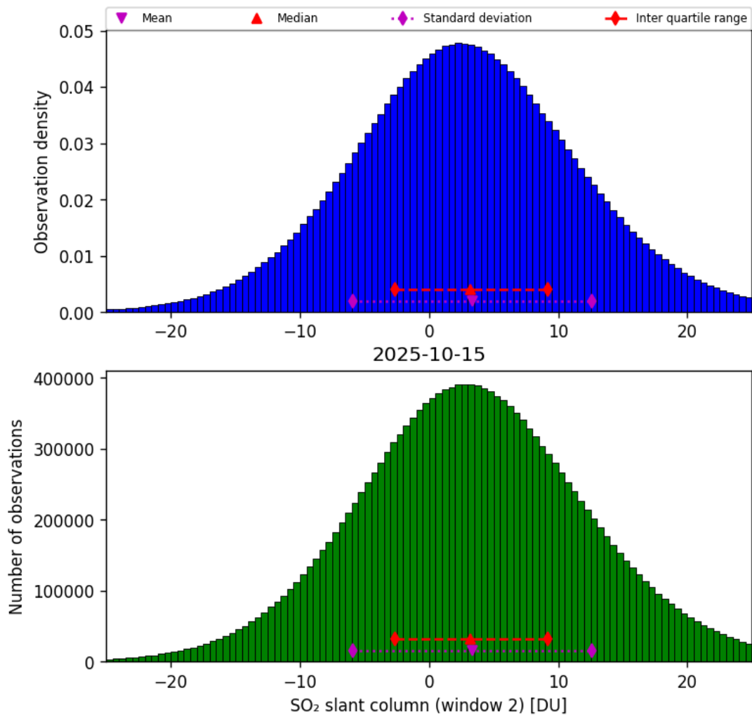
Figure 67: Histogram of “SO 2 slant column (window 2)” for 2025-10-15 to 2025-10-15
