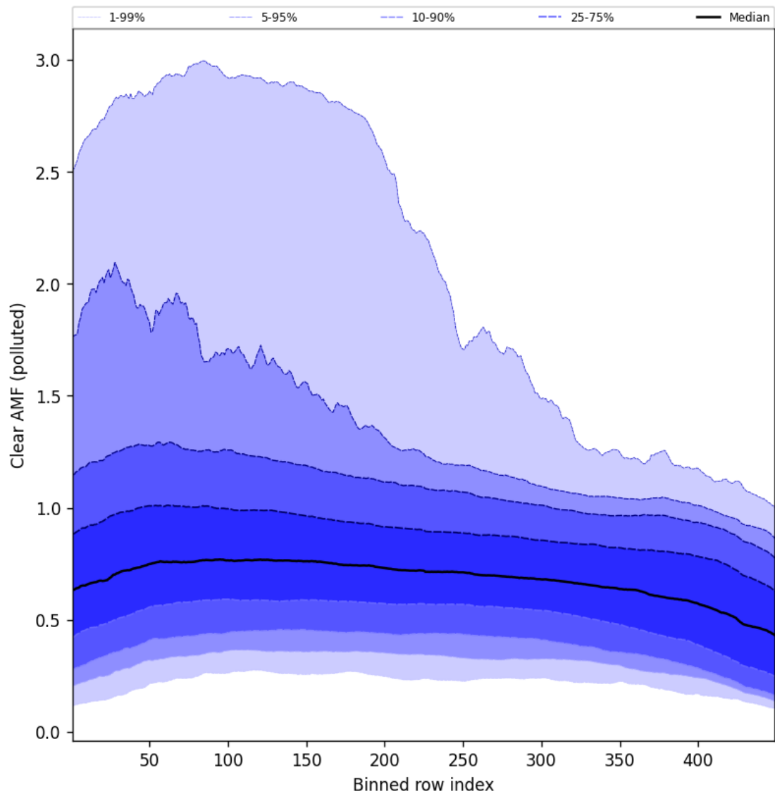
Figure 109: Along track statistics of “Clear AMF (polluted)” for 2025-10-15 to 2025-10-15
