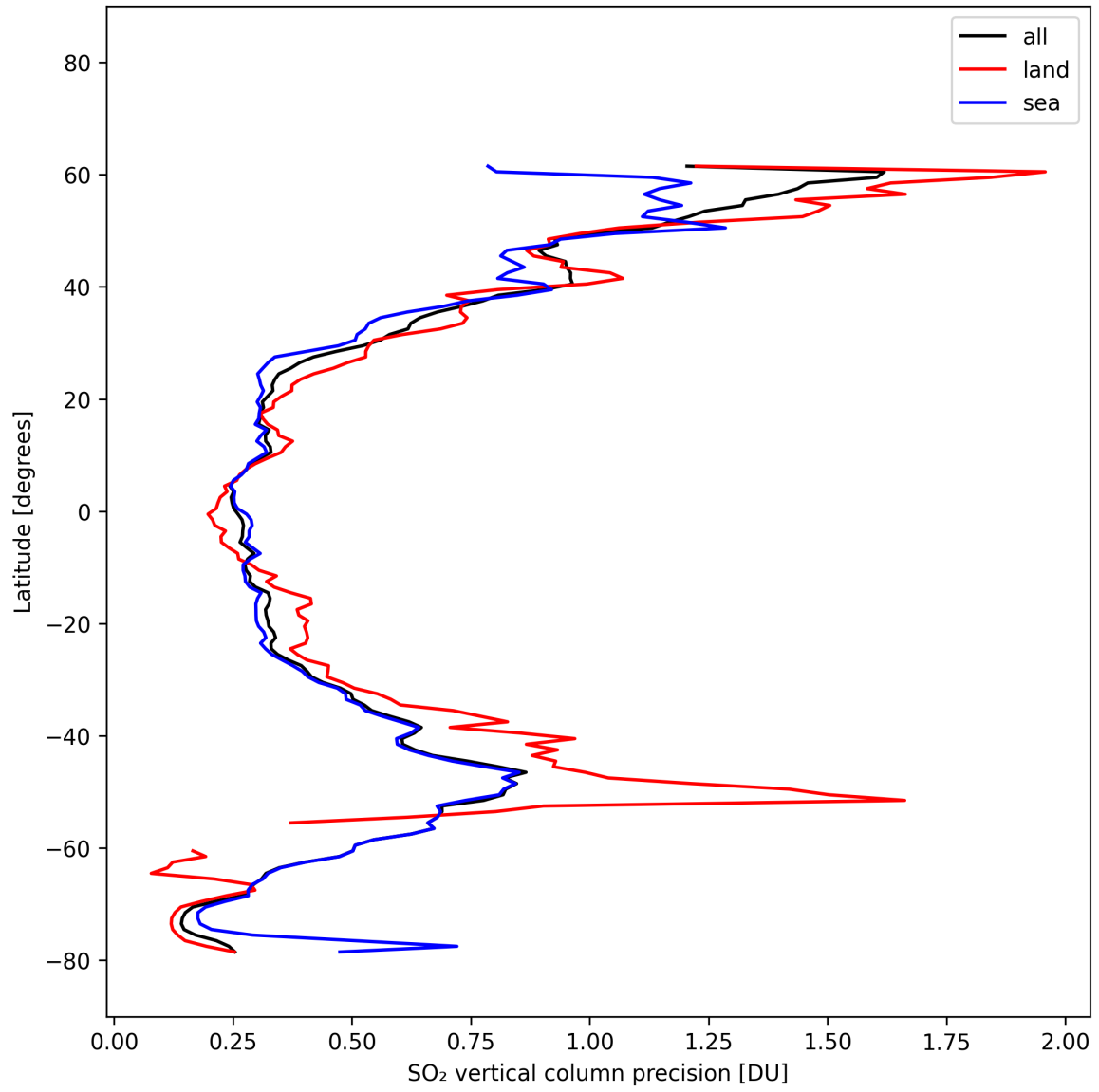
Figure 32: Zonal average of “SO 2 vertical column precision” for 2025-10-15 to 2025-10-15.
