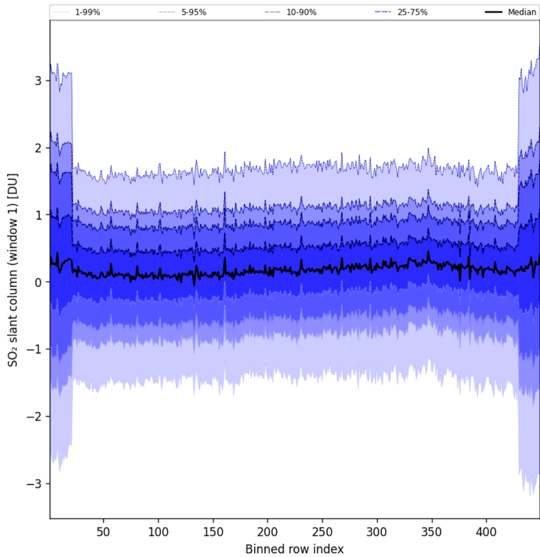
Figure 90: Along track statistics of “SO 2 slant column (window 1)” for 2025-10-15 to 2025-10-15
