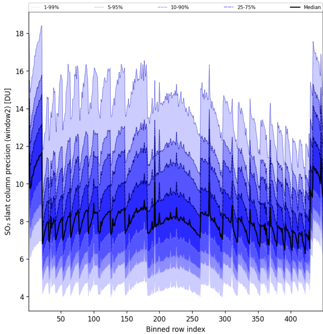
Figure 95: Along track statistics of “SO 2 slant column precision (window2)” for 2025-10-15 to 2025-10-15
