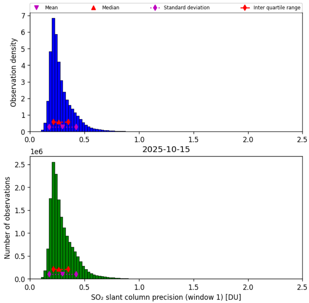
Figure 64: Histogram of “SO 2 slant column precision (window 1)” for 2025-10-15 to 2025-10-15
