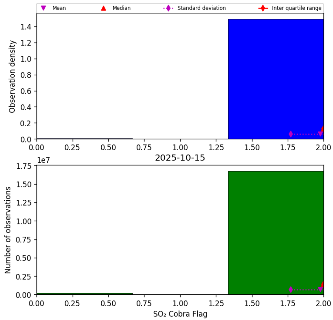
Figure 75: Histogram of “SO 2 Cobra Flag” for 2025-10-15 to 2025-10-15
