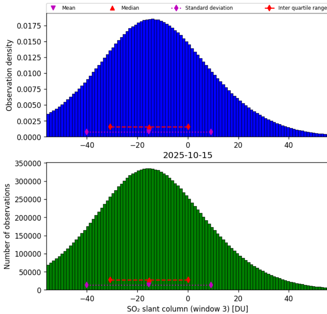
Figure 71: Histogram of “SO 2 slant column (window 3)” for 2025-10-15 to 2025-10-15
