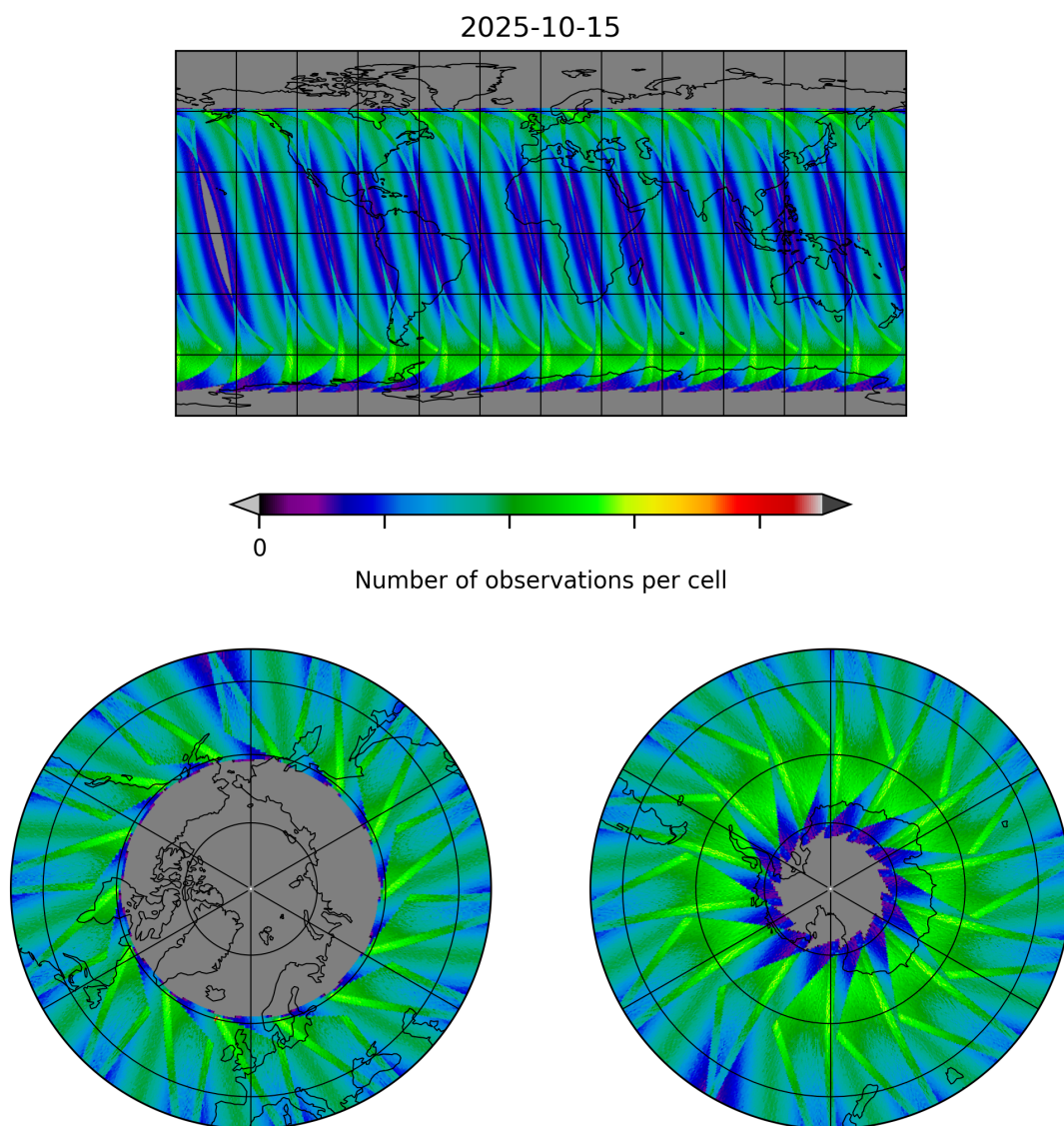
Figure 29: Map of the number of observations for 2025-10-15 to 2025-10-15
