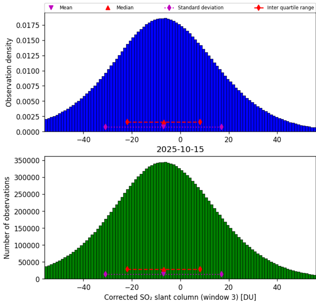
Figure 73: Histogram of “Corrected SO 2 slant column (window 3)” for 2025-10-15 to 2025-10-15
