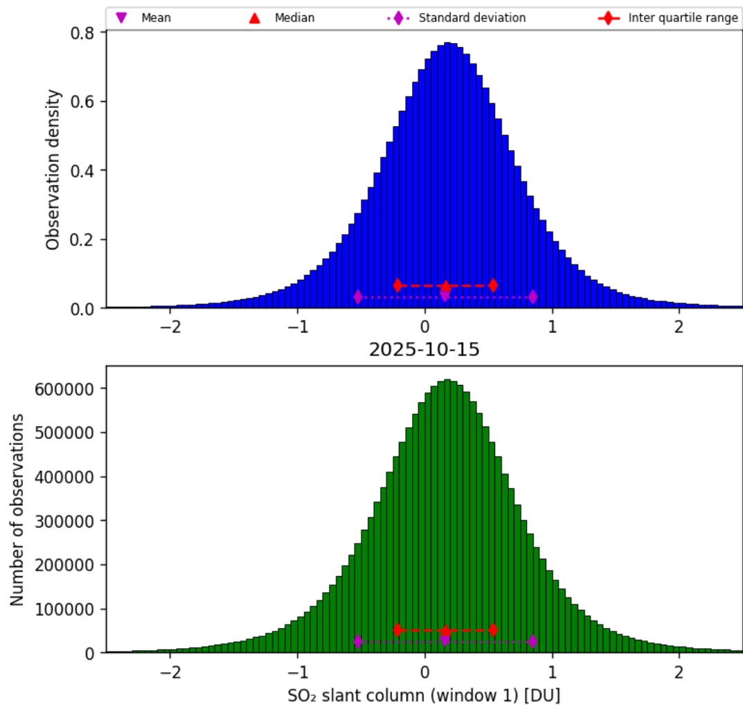
Figure 63: Histogram of “SO 2 slant column (window 1)” for 2025-10-15 to 2025-10-15
