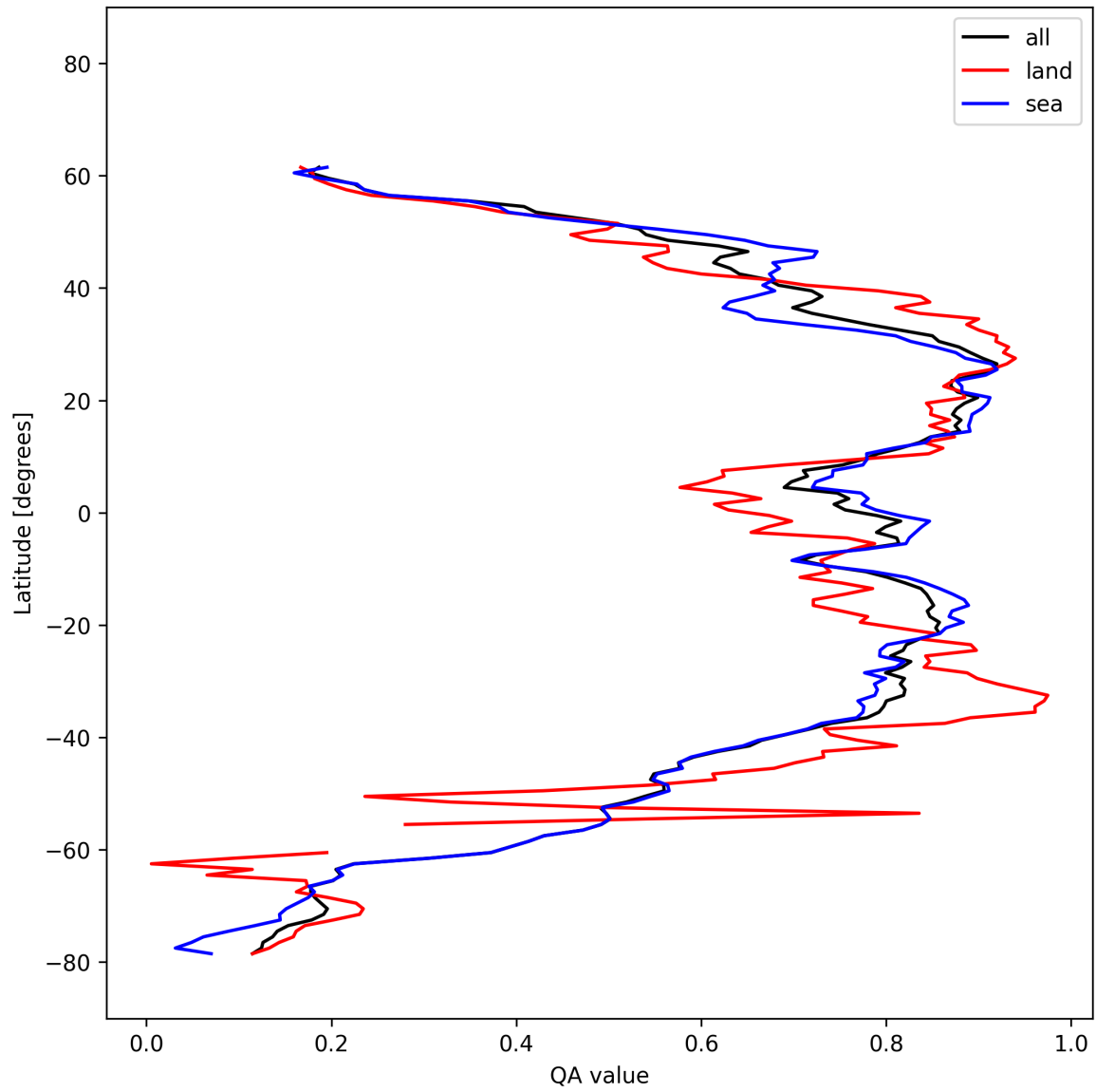
Figure 30: Zonal average of “QA value” for 2025-10-15 to 2025-10-15.
