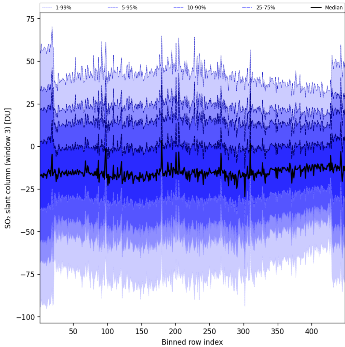
Figure 98: Along track statistics of “SO 2 slant column (window 3)” for 2025-10-15 to 2025-10-15
