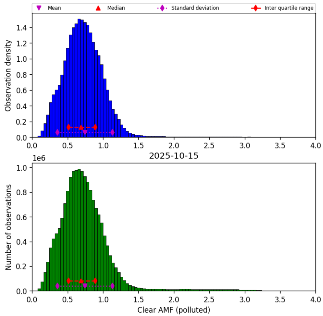
Figure 82: Histogram of "Clear AMF (polluted)" for 2025-10-15 to 2025-10-15
