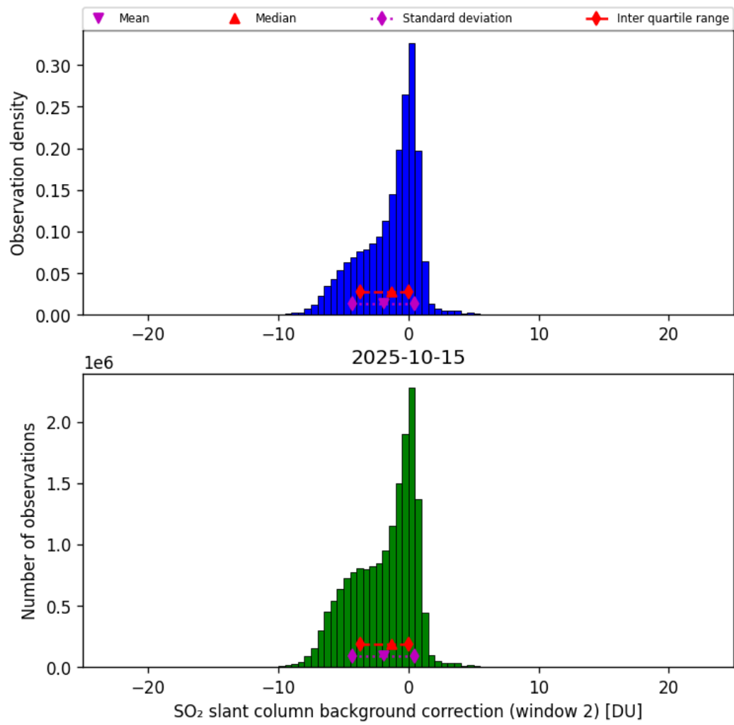
Figure 70: Histogram of “SO 2 slant column background correction (window 2)” for 2025-10-15 to 2025-10-15
