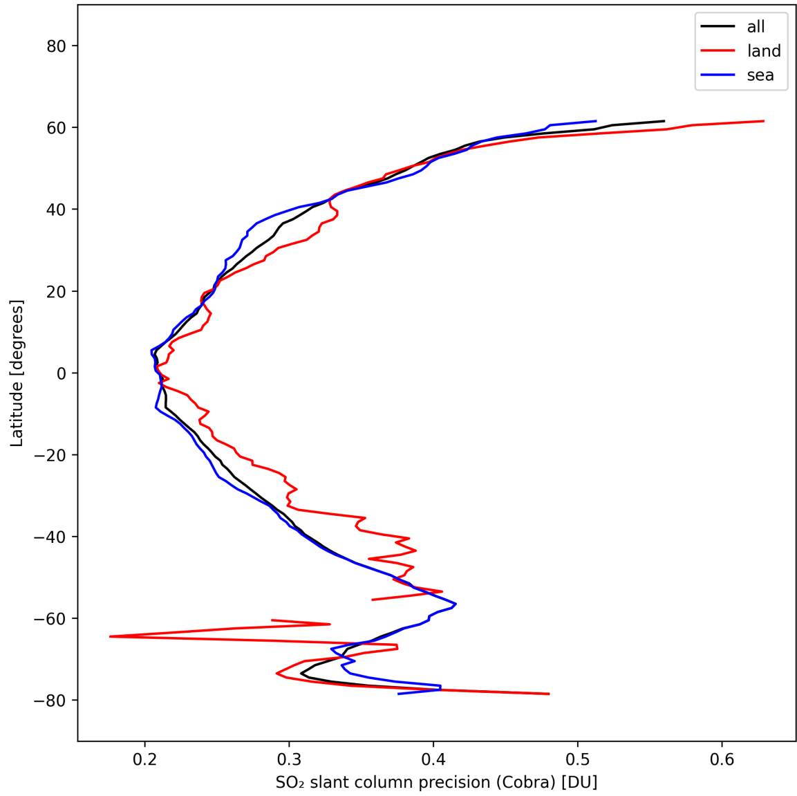
Figure 35: Zonal average of “SO 2 slant column precision (Cobra)” for 2025-10-15 to 2025-10-15.
