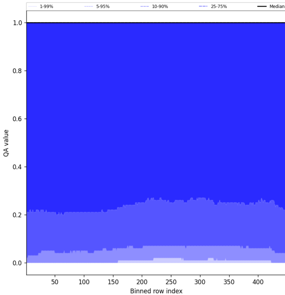
Figure 84: Along track statistics of “QA value” for 2025-10-15 to 2025-10-15
