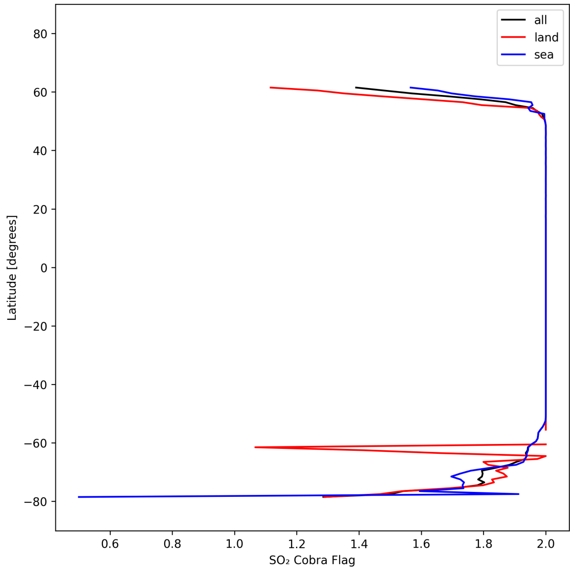
Figure 48: Zonal average of "SO 2 Cobra Flag" for 2025-10-15 to 2025-10-15.
