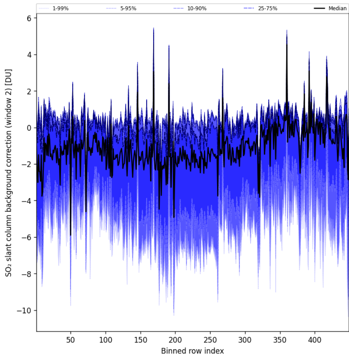
Figure 97: Along track statistics of “SO 2 slant column background correction (window 2)” for 2025-10-15 to 2025-10-15
