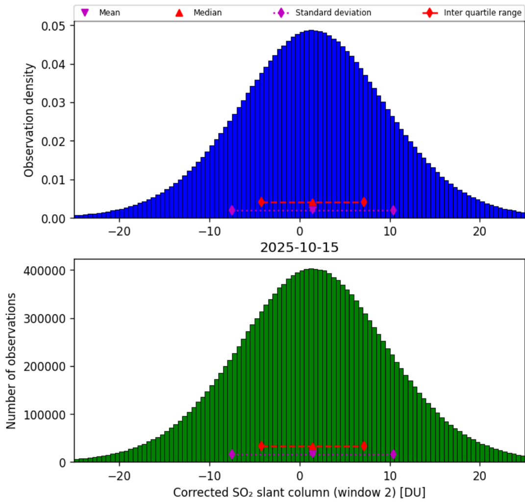
Figure 69: Histogram of “Corrected SO 2 slant column (window 2)” for 2025-10-15 to 2025-10-15
