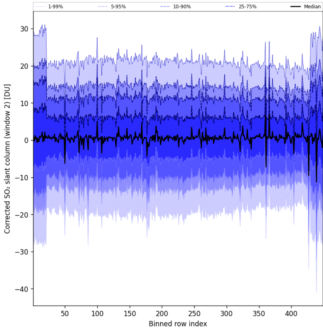
Figure 96: Along track statistics of “Corrected SO 2 slant column (window 2)” for 2025-10-16 to 2025-10-17
