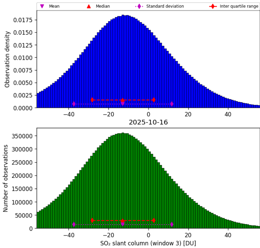
Figure 71: Histogram of “SO 2 slant column (window 3)” for 2025-10-16 to 2025-10-17
