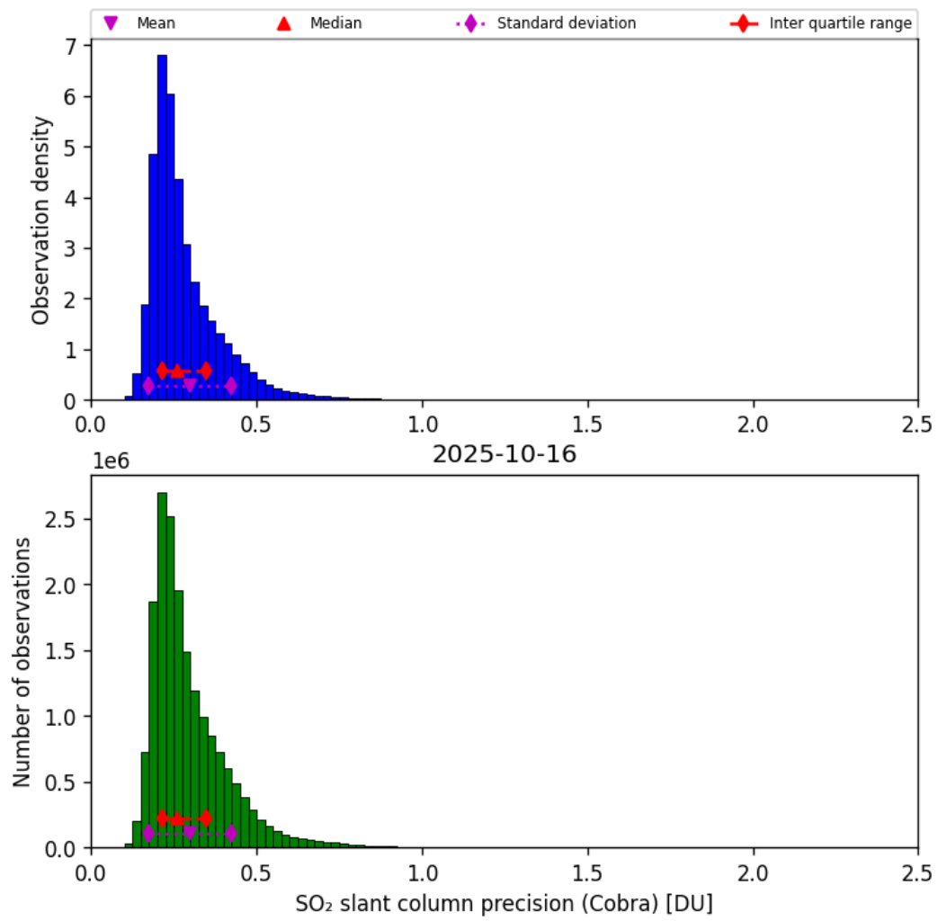
Figure 62: Histogram of “SO 2 slant column precision (Cobra)” for 2025-10-16 to 2025-10-17
