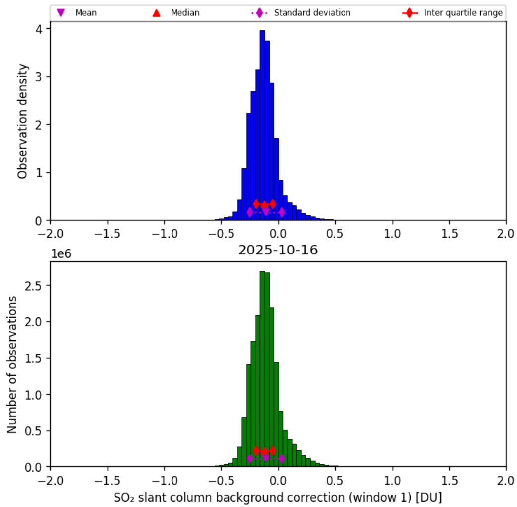
Figure 66: Histogram of “SO 2 slant column background correction (window 1)” for 2025-10-16 to 2025-10-17
