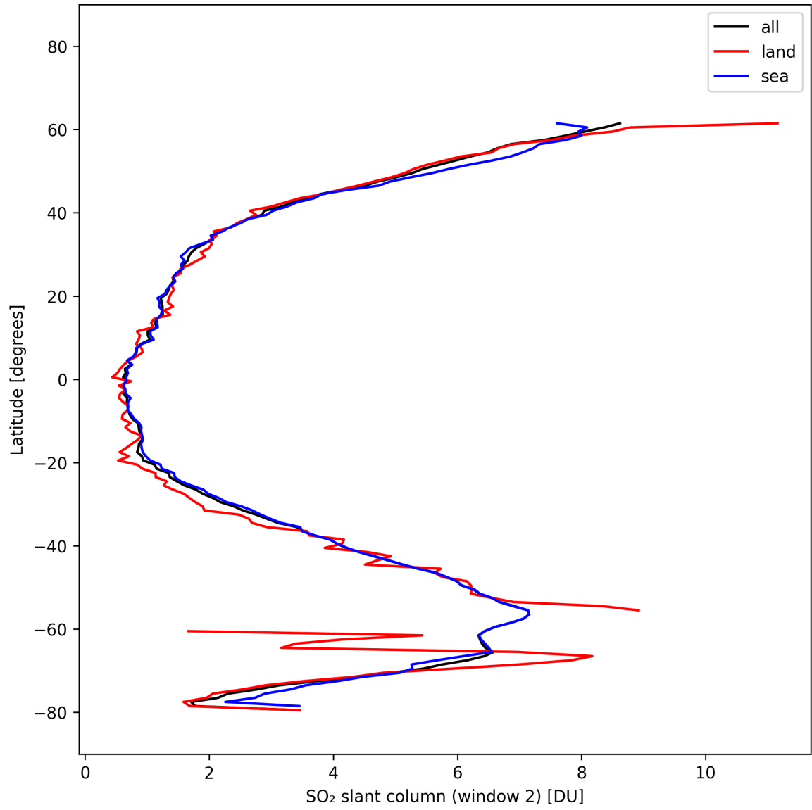
Figure 40: Zonal average of “SO 2 slant column (window 2)” for 2025-10-16 to 2025-10-17.
