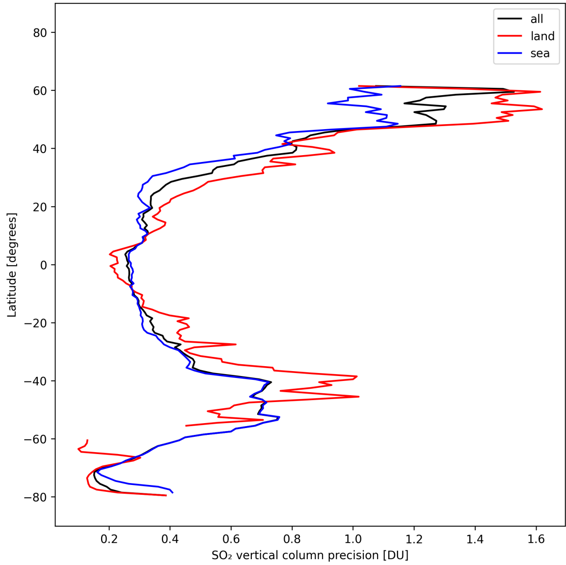
Figure 32: Zonal average of “SO 2 vertical column precision” for 2025-10-16 to 2025-10-17.
