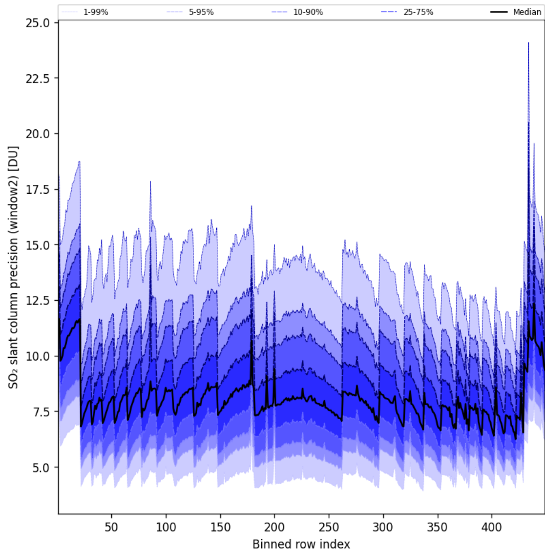
Figure 95: Along track statistics of “SO 2 slant column precision (window2)” for 2025-10-16 to 2025-10-17
