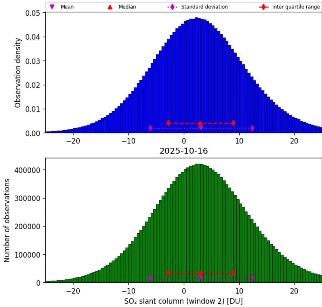
Figure 67: Histogram of “SO 2 slant column (window 2)” for 2025-10-16 to 2025-10-17
