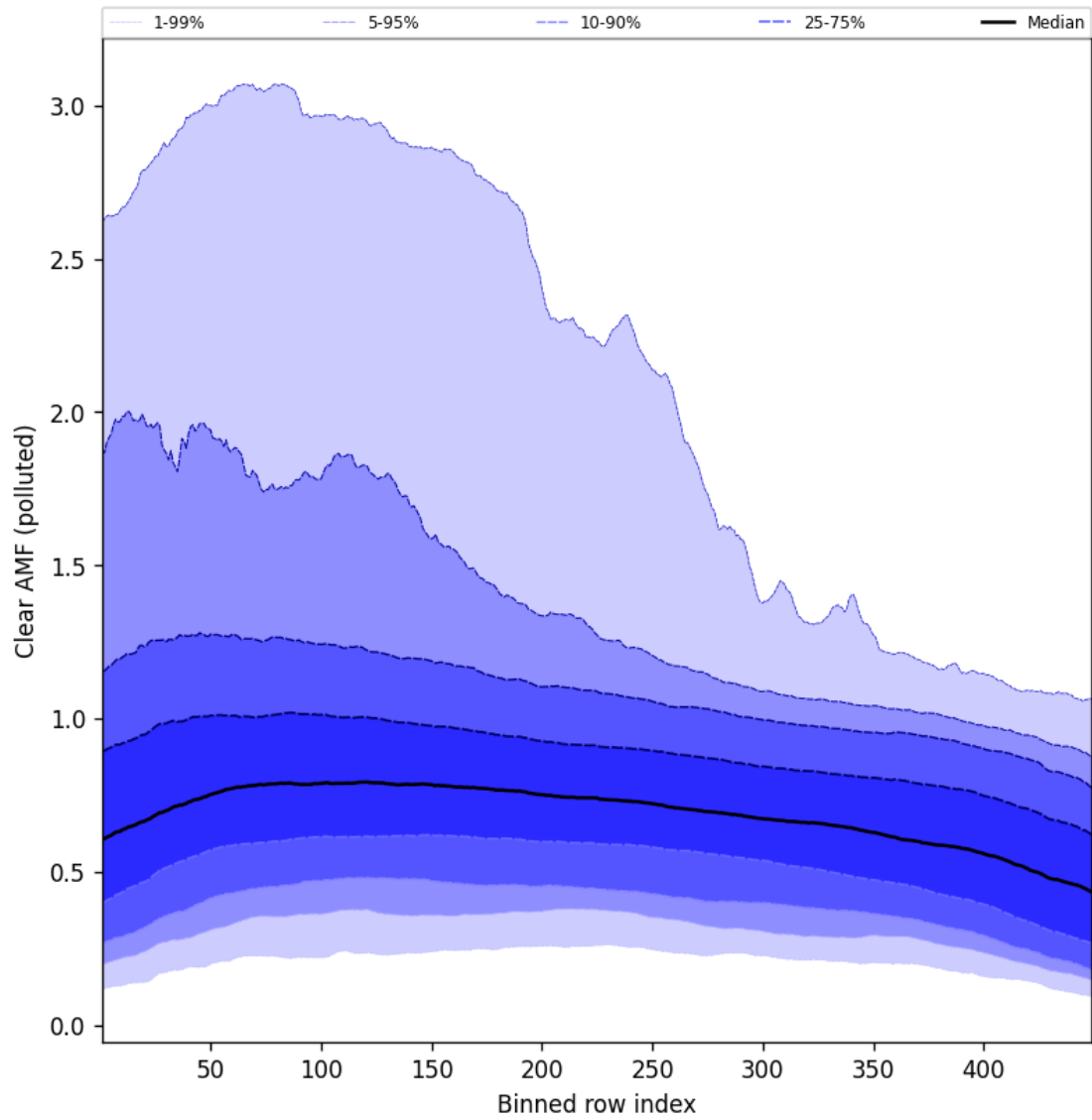
Figure 109: Along track statistics of “Clear AMF (polluted)” for 2025-10-16 to 2025-10-17
