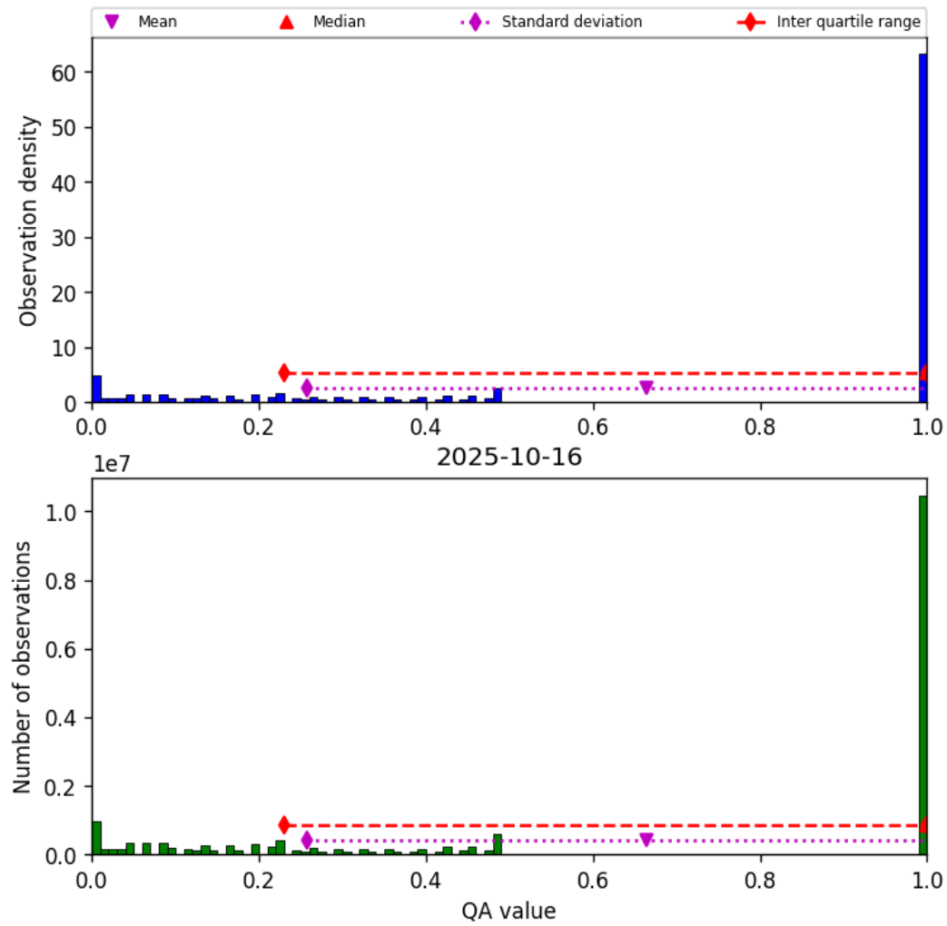
Figure 57: Histogram of “QA value” for 2025-10-16 to 2025-10-17
