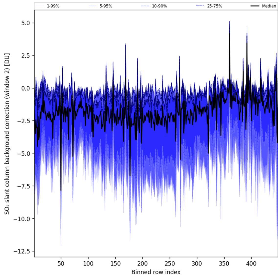
Figure 97: Along track statistics of “SO 2 slant column background correction (window 2)” for 2025-10-16 to 2025-10-17
