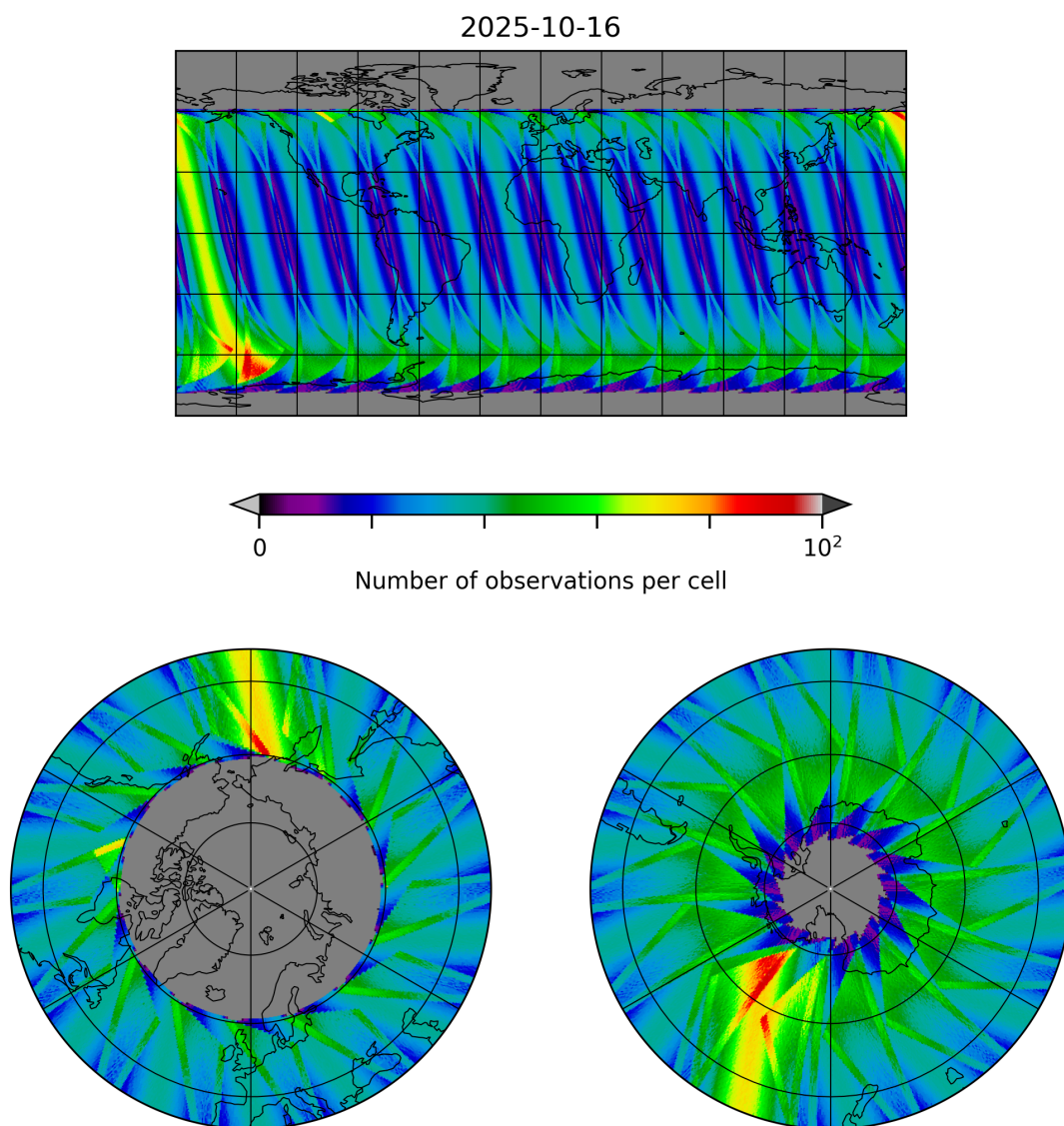
Figure 29: Map of the number of observations for 2025-10-16 to 2025-10-17
