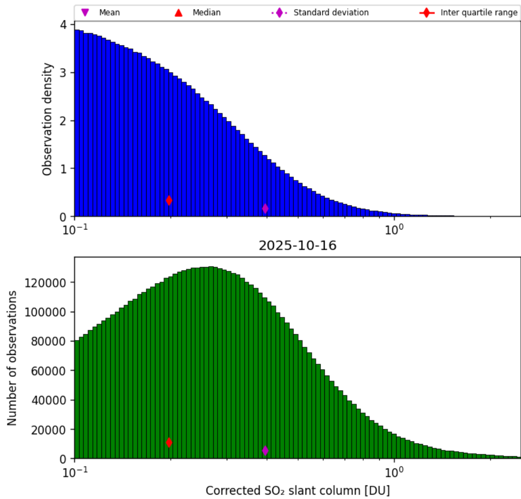
Figure 60: Histogram of “Corrected SO 2 slant column” for 2025-10-16 to 2025-10-17
