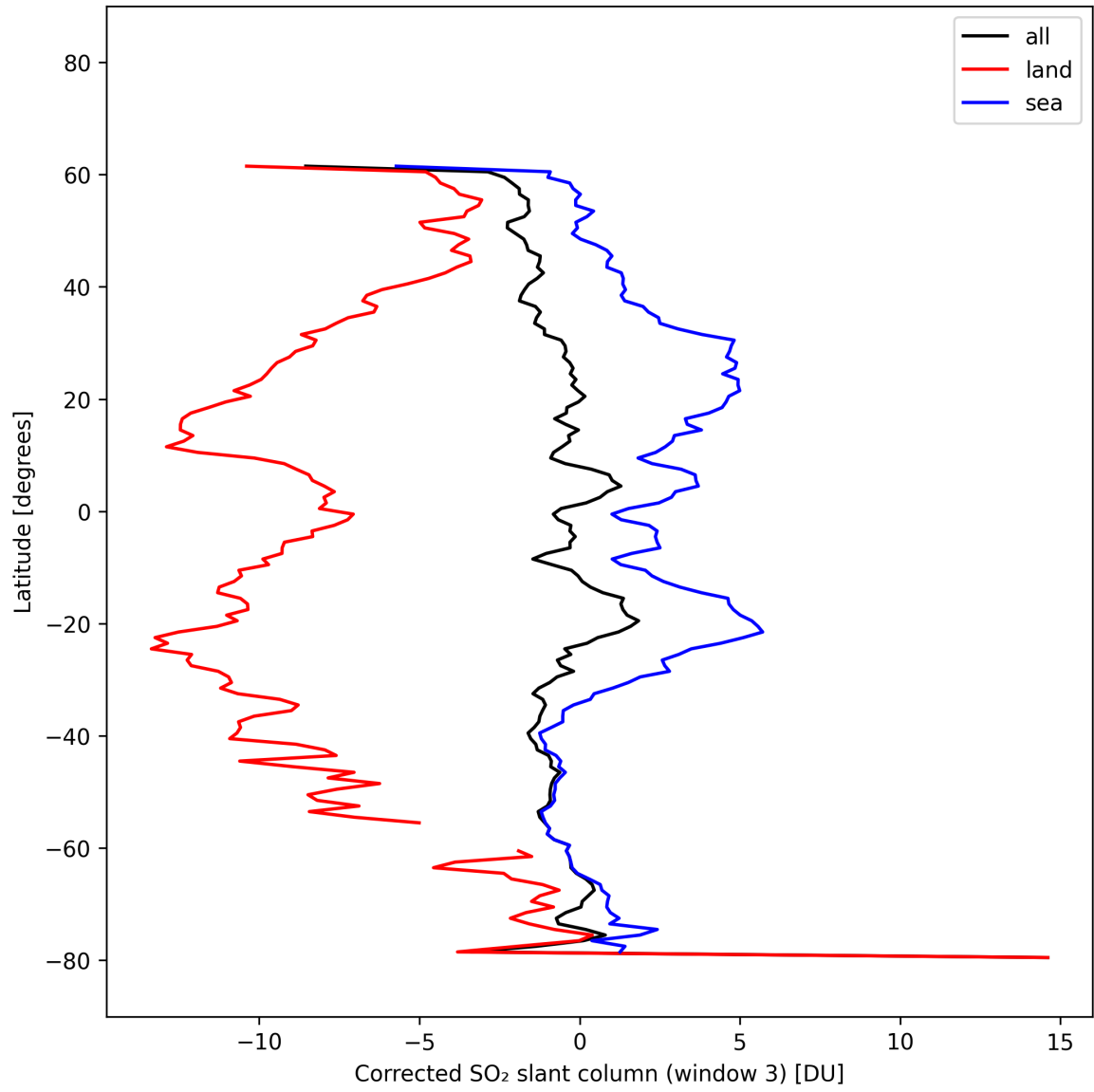
Figure 46: Zonal average of “Corrected SO 2 slant column (window 3)” for 2025-10-16 to 2025-10-17.
