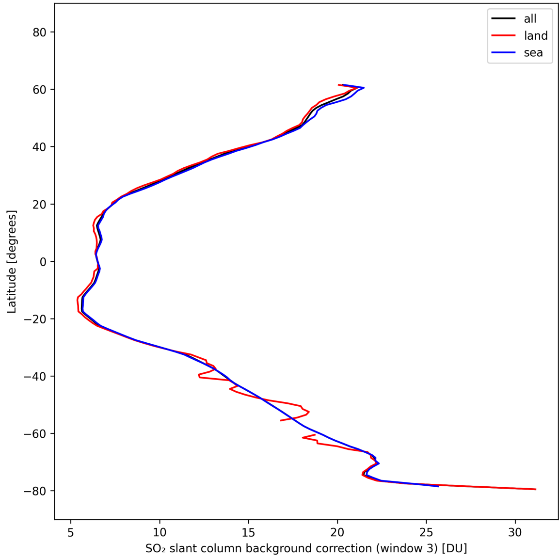
Figure 47: Zonal average of “SO 2 slant column background correction (window 3)” for 2025-10-16 to 2025-10-17.
