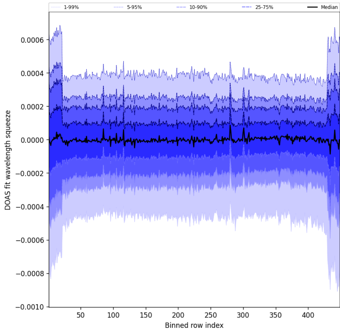
Figure 105: Along track statistics of “DOAS fit wavelength squeeze” for 2025-10-16 to 2025-10-17
