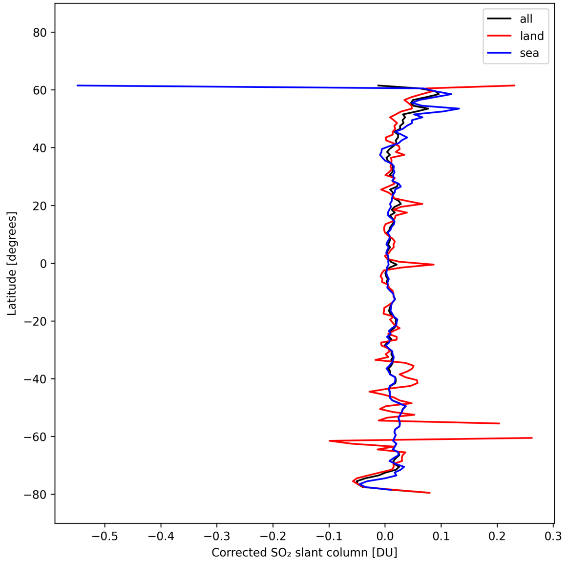
Figure 33: Zonal average of “Corrected SO 2 slant column” for 2025-10-16 to 2025-10-17.
