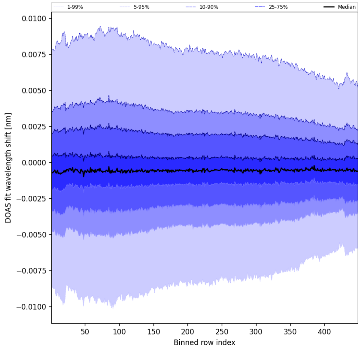
Figure 104: Along track statistics of “DOAS fit wavelength shift” for 2025-10-16 to 2025-10-17
