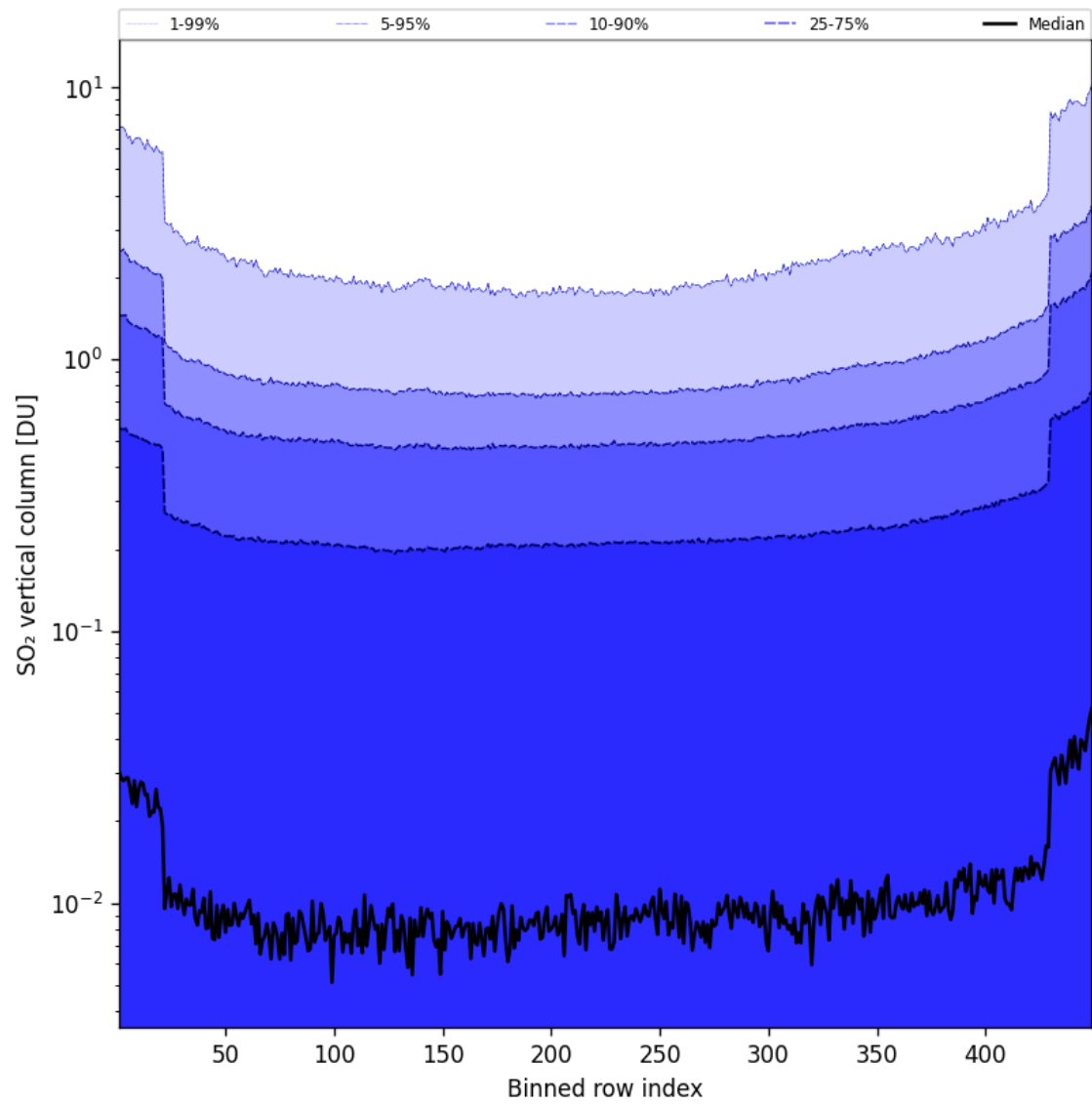
Figure 85: Along track statistics of “SO 2 vertical column” for 2025-10-16 to 2025-10-17
