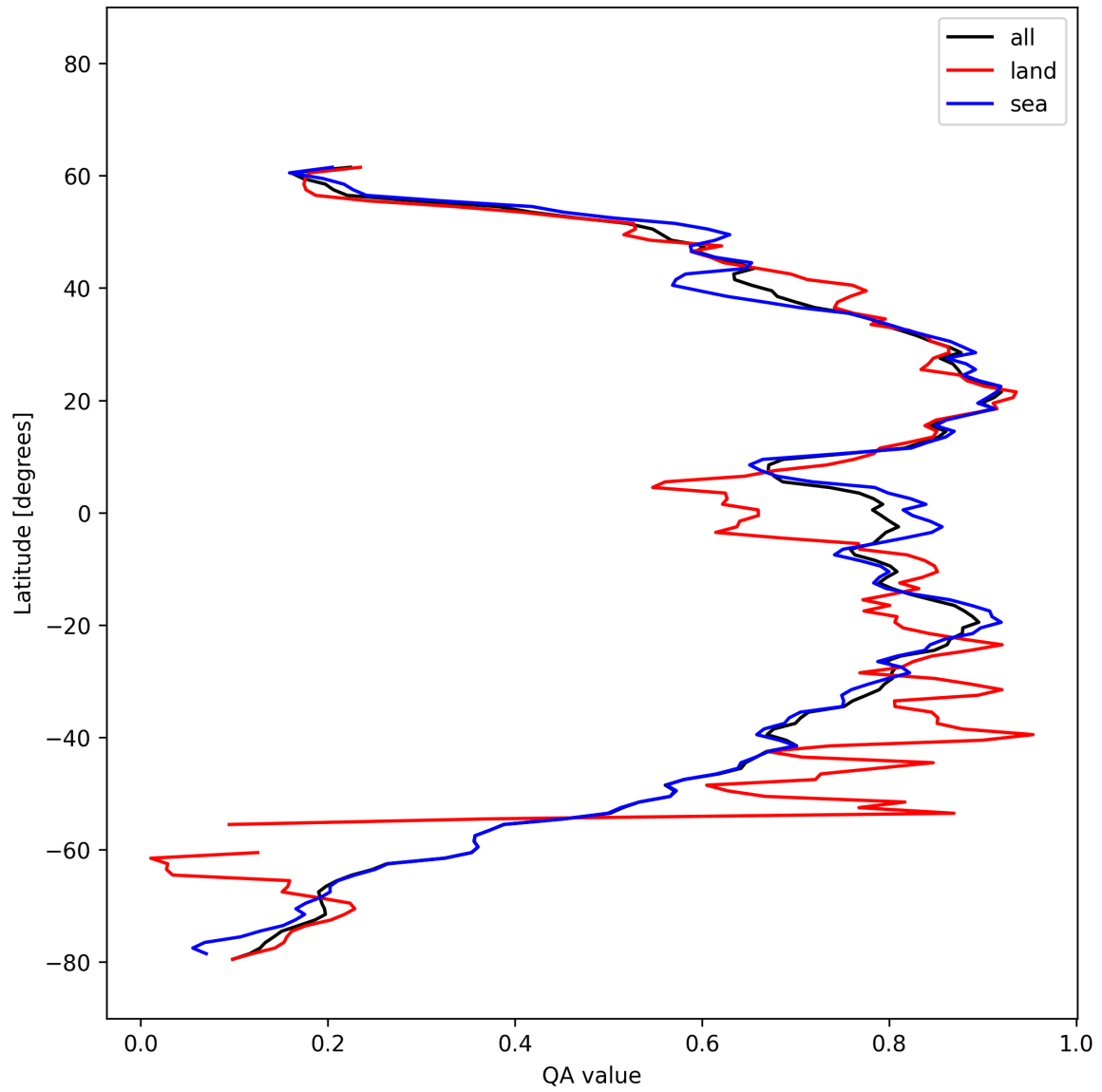
Figure 30: Zonal average of “QA value” for 2025-10-16 to 2025-10-17.
