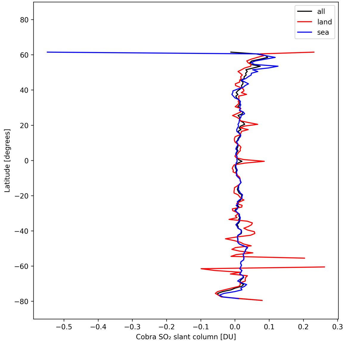
Figure 34: Zonal average of “Cobra SO 2 slant column” for 2025-10-16 to 2025-10-17.
