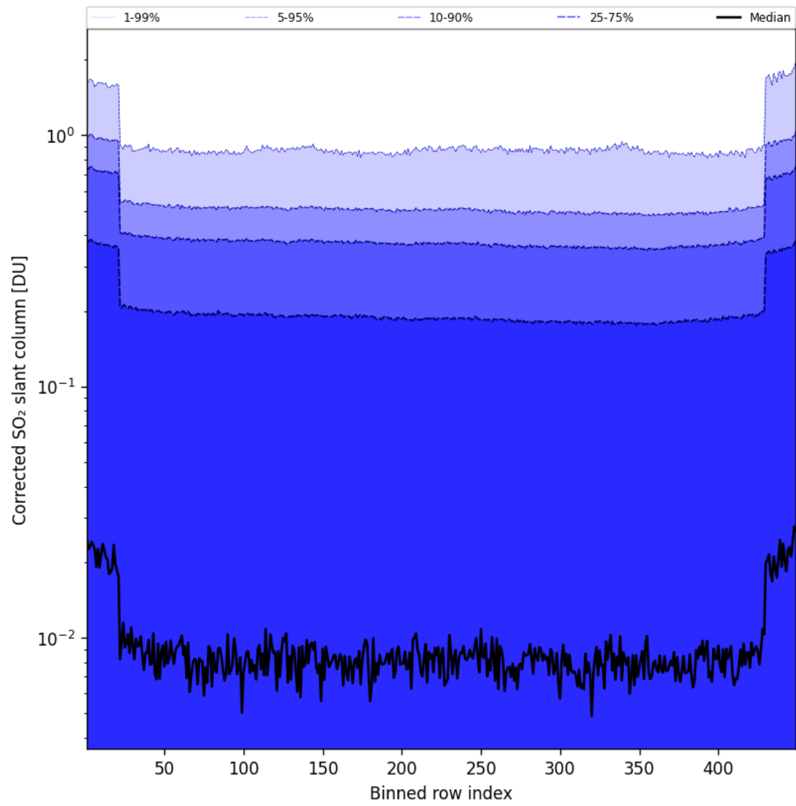
Figure 87: Along track statistics of “Corrected SO 2 slant column” for 2025-10-16 to 2025-10-17
