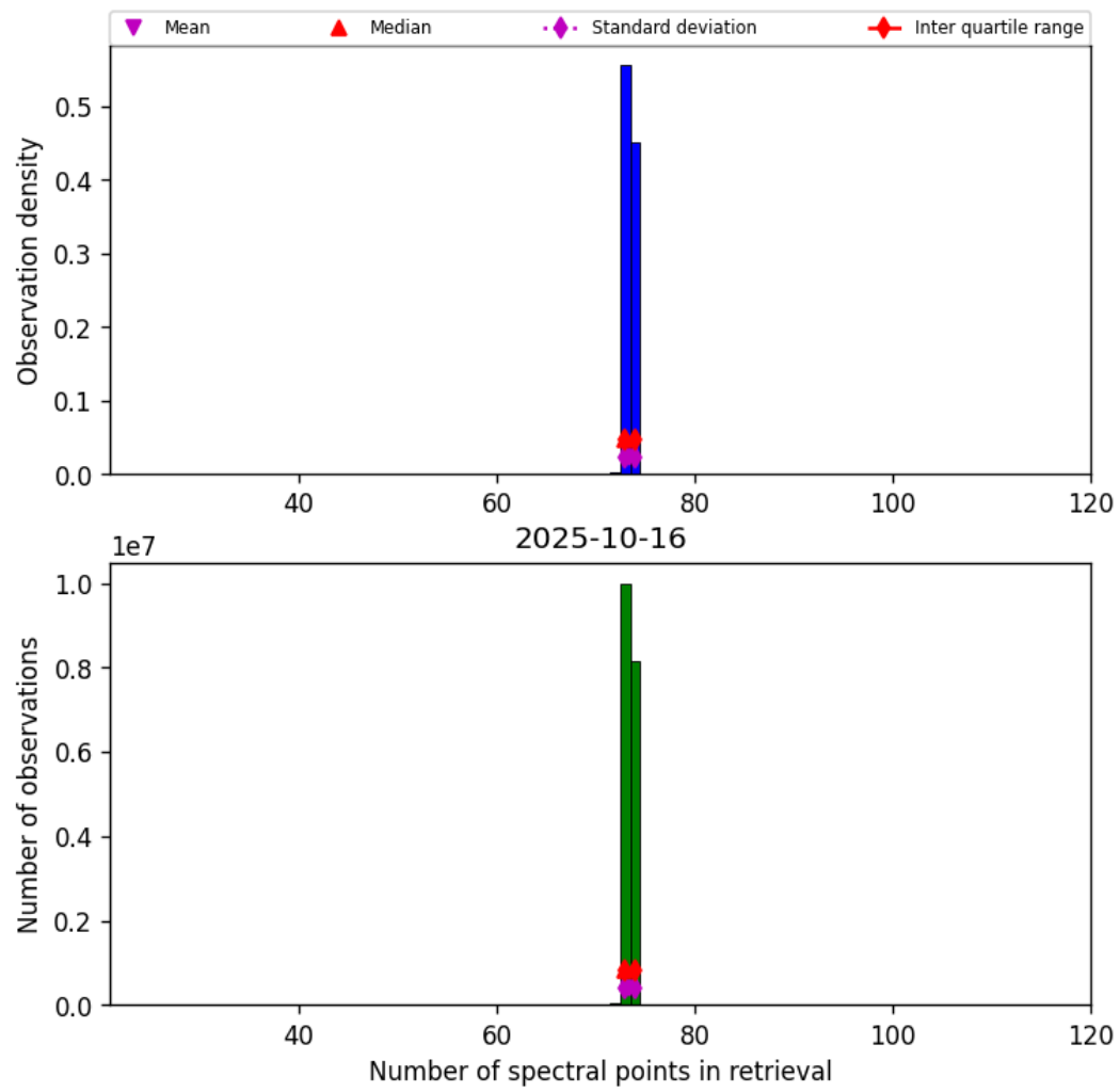
Figure 83: Histogram of “Number of spectral points in retrieval” for 2025-10-16 to 2025-10-17
