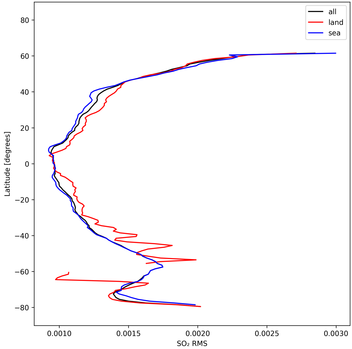
Figure 52: Zonal average of “SO 2 RMS” for 2025-10-16 to 2025-10-17.
