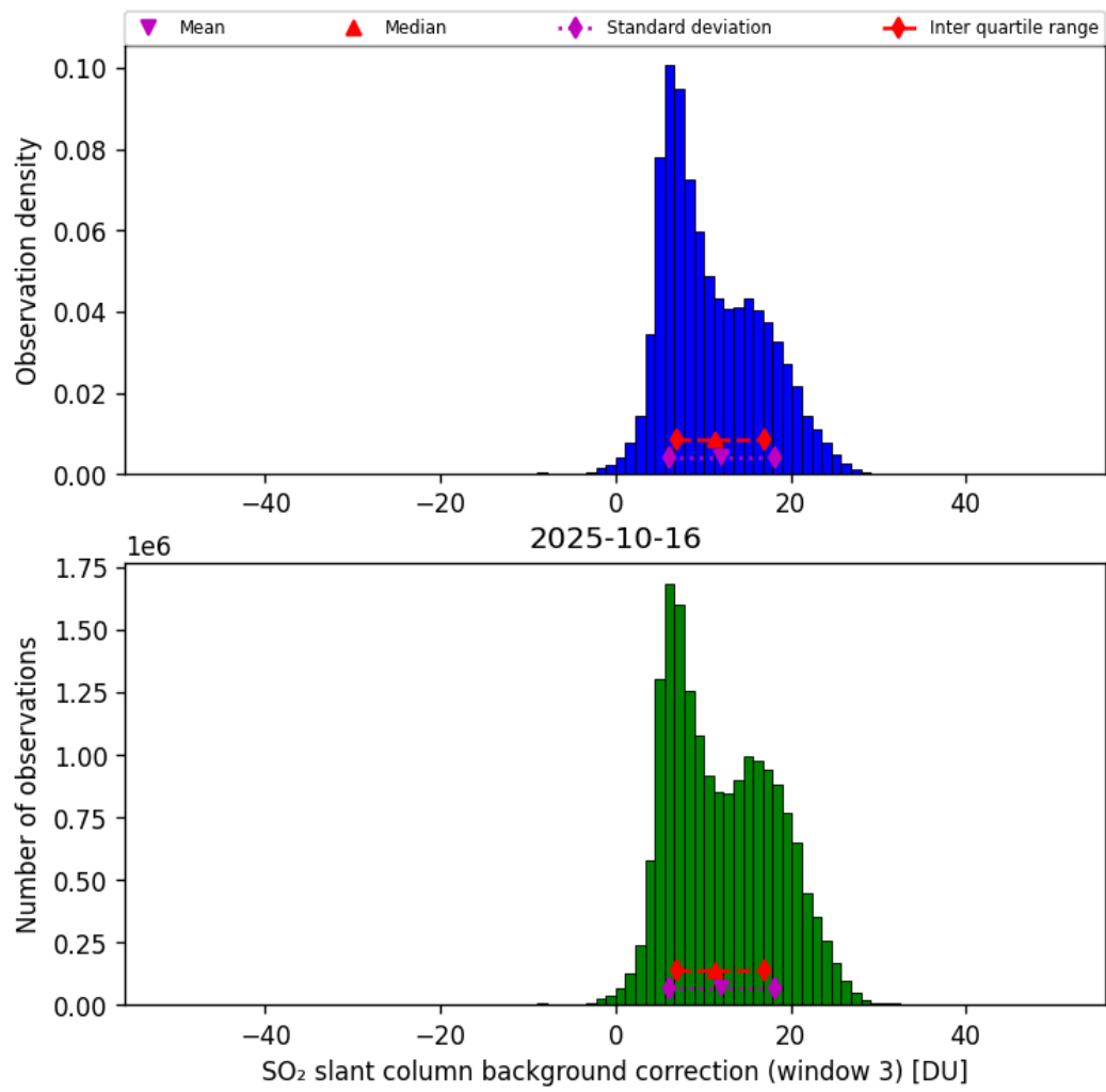
Figure 74: Histogram of “SO 2 slant column background correction (window 3)” for 2025-10-16 to 2025-10-17
