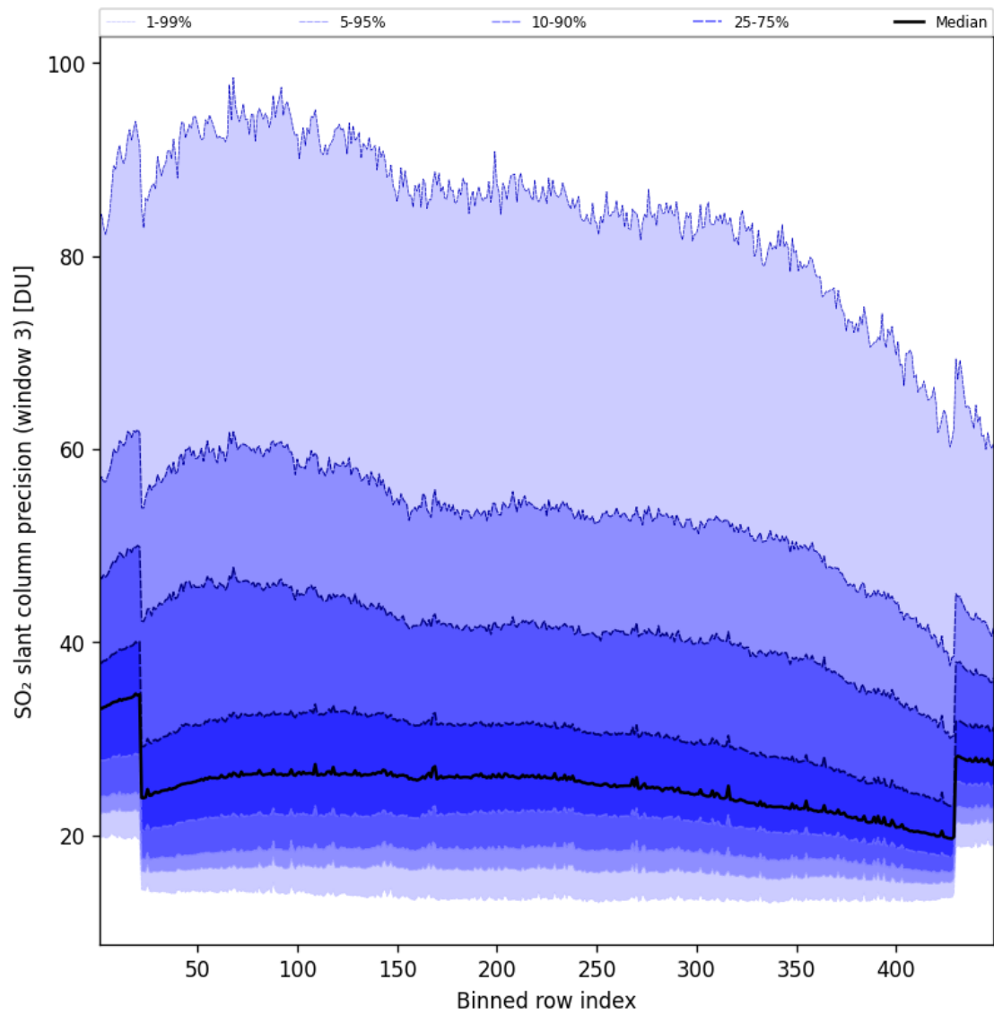
Figure 99: Along track statistics of “SO 2 slant column precision (window 3)” for 2025-10-16 to 2025-10-17
