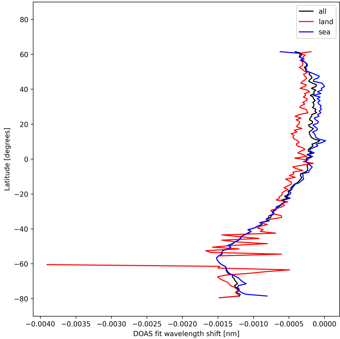
Figure 50: Zonal average of "DOAS fit wavelength shift" for 2025-10-16 to 2025-10-17.
