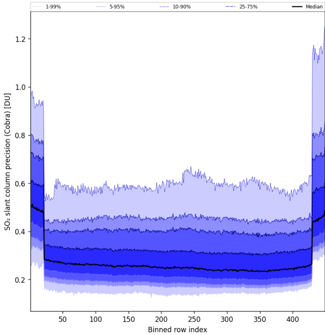
Figure 89: Along track statistics of “SO 2 slant column precision (Cobra)” for 2025-10-16 to 2025-10-17
