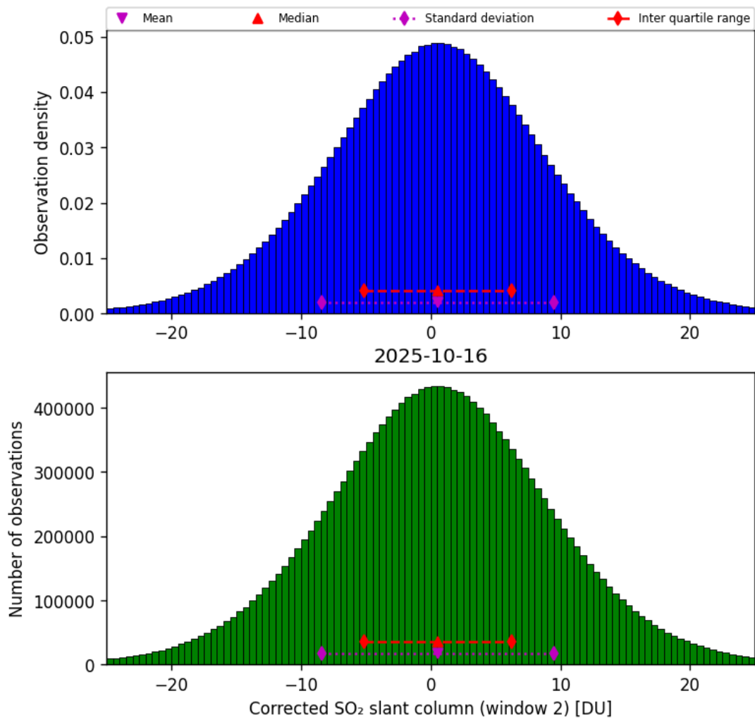
Figure 69: Histogram of “Corrected SO 2 slant column (window 2)” for 2025-10-16 to 2025-10-17
