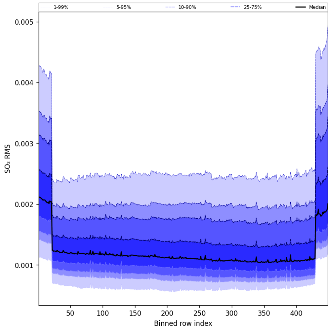
Figure 106: Along track statistics of “SO 2 RMS” for 2025-10-16 to 2025-10-17
