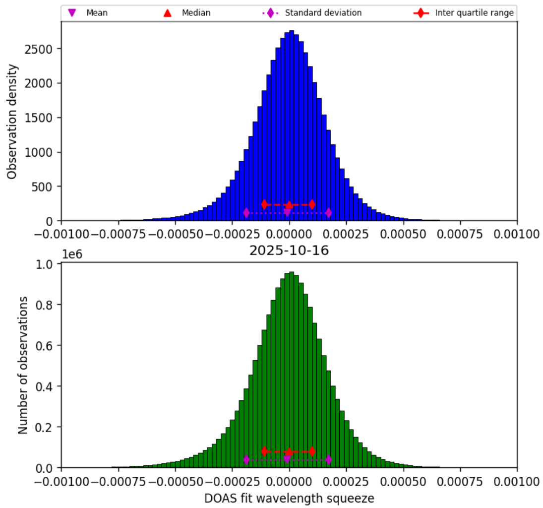
Figure 78: Histogram of “DOAS fit wavelength squeeze” for 2025-10-16 to 2025-10-17
