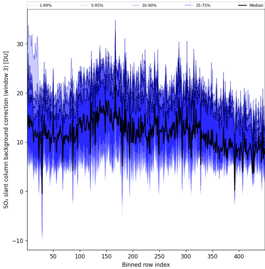
Figure 101: Along track statistics of “SO 2 slant column background correction (window 3)” for 2025-10-16 to 2025-10-17
