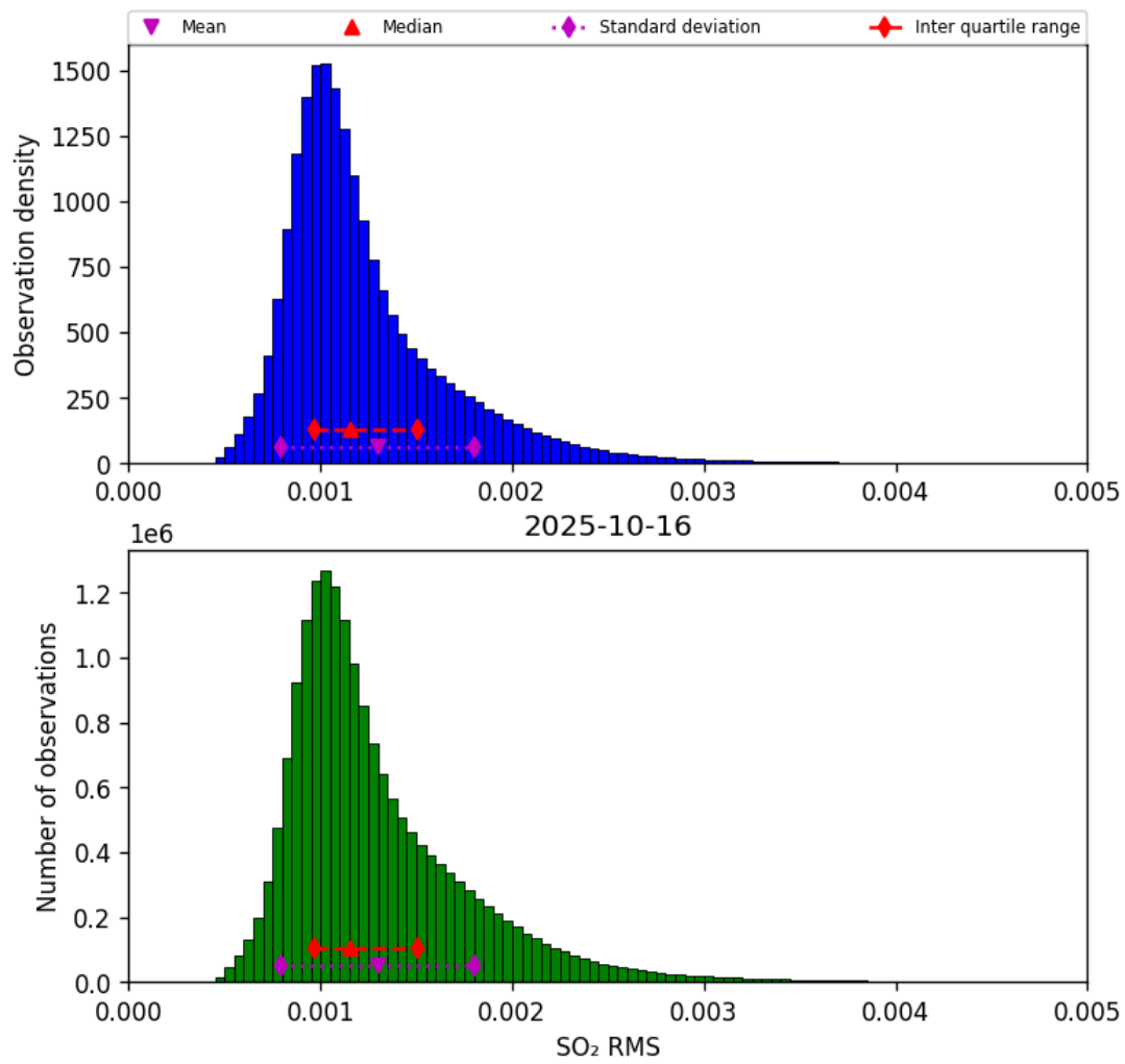
Figure 79: Histogram of “SO 2 RMS” for 2025-10-16 to 2025-10-17
