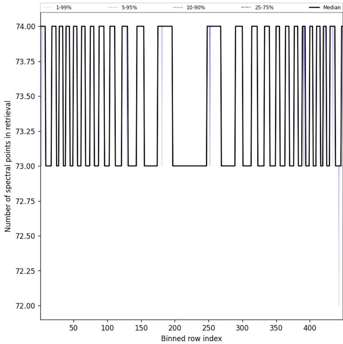
Figure 110: Along track statistics of “Number of spectral points in retrieval” for 2025-10-16 to 2025-10-17
