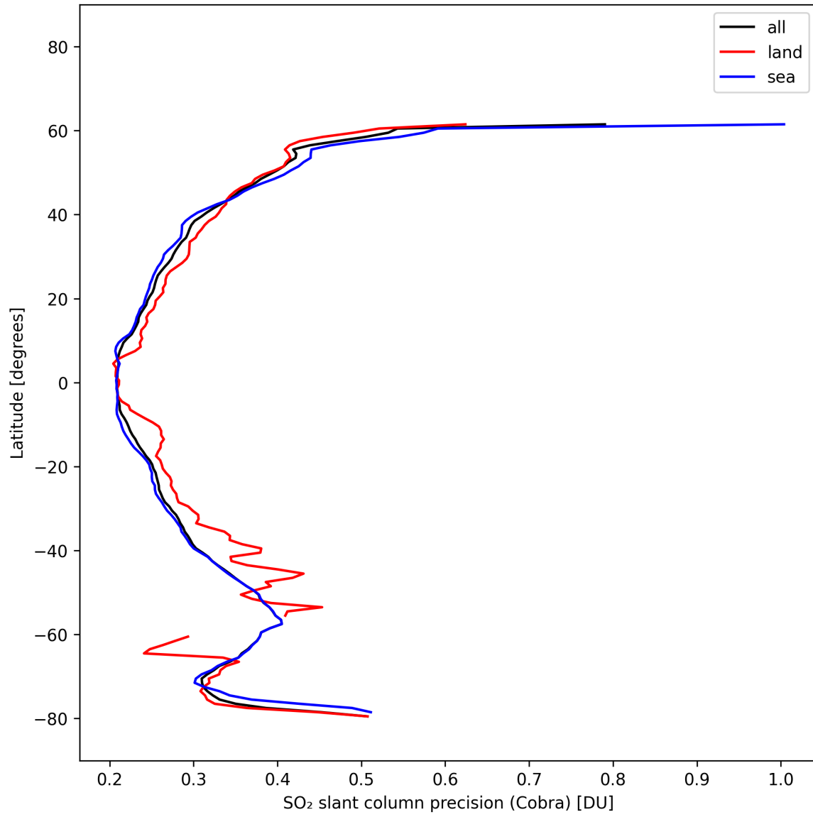
Figure 35: Zonal average of “SO 2 slant column precision (Cobra)” for 2025-10-16 to 2025-10-17.
