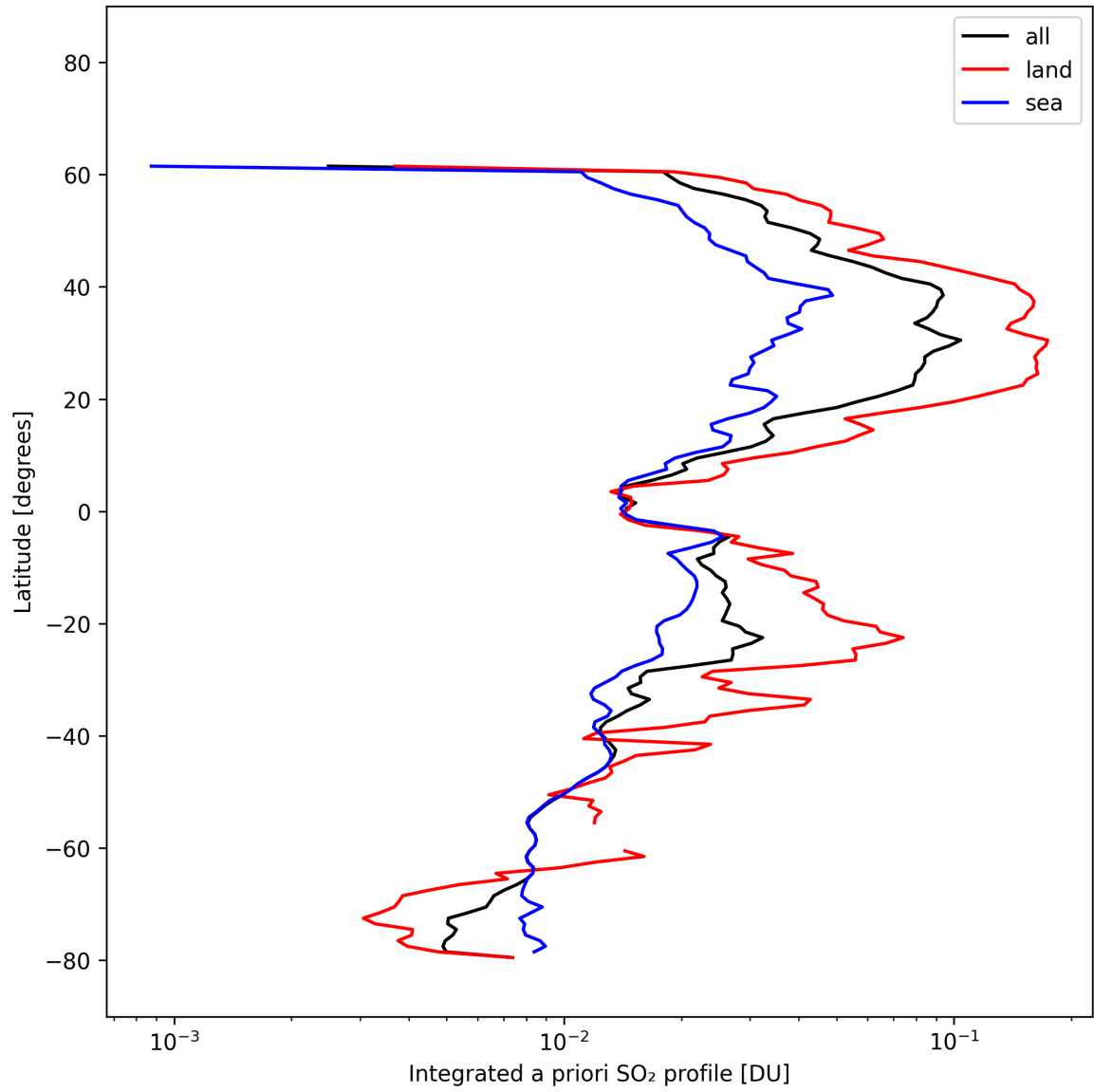
Figure 49: Zonal average of “Integrated a priori SO 2 profile” for 2025-10-16 to 2025-10-17.
