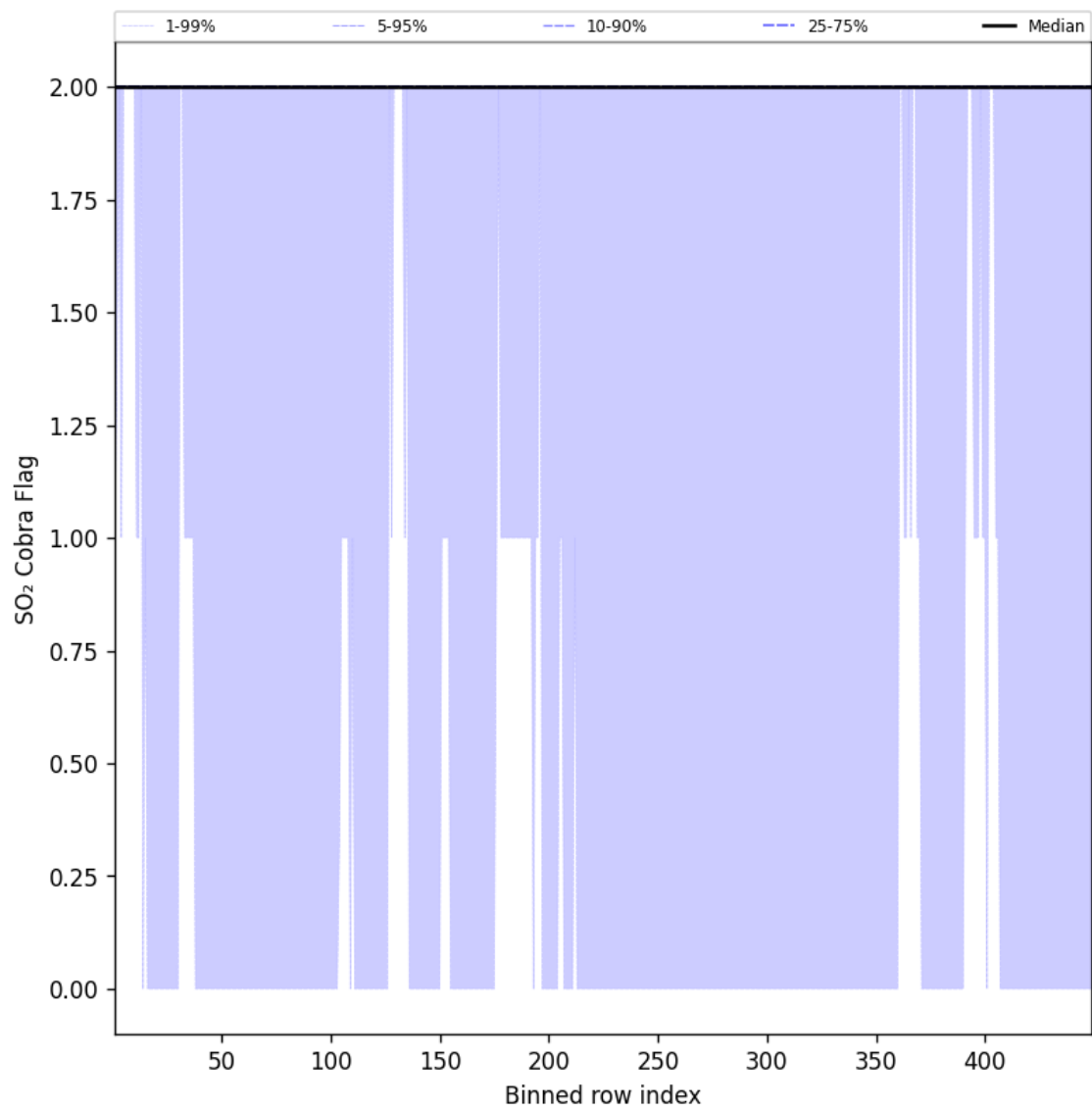
Figure 102: Along track statistics of “SO 2 Cobra Flag” for 2025-10-16 to 2025-10-17
