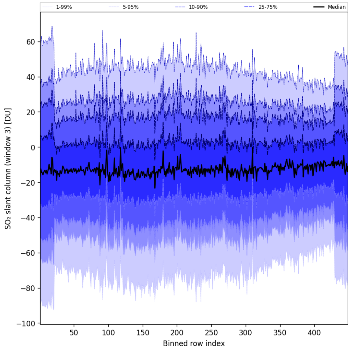
Figure 98: Along track statistics of “SO 2 slant column (window 3)” for 2025-10-16 to 2025-10-17
