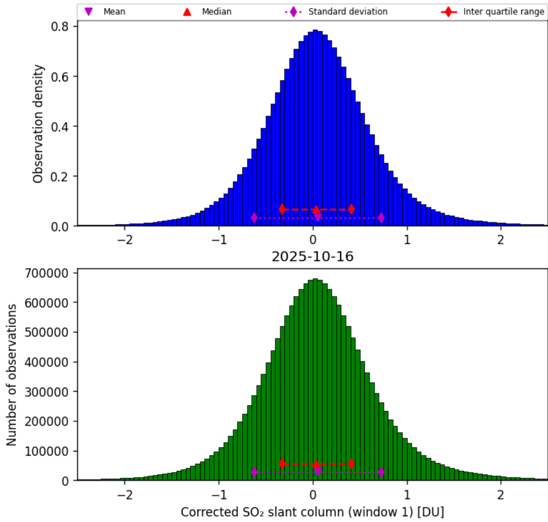
Figure 65: Histogram of “Corrected SO 2 slant column (window 1)” for 2025-10-16 to 2025-10-17
