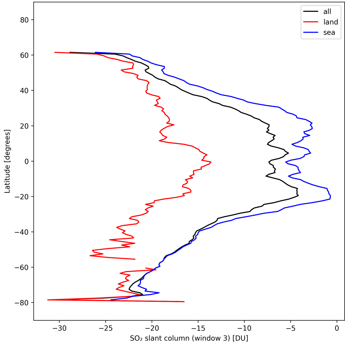
Figure 44: Zonal average of “SO 2 slant column (window 3)” for 2025-10-16 to 2025-10-17.
