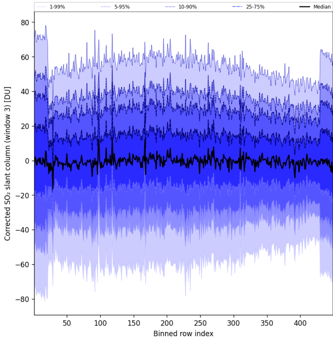
Figure 100: Along track statistics of “Corrected SO 2 slant column (window 3)” for 2025-10-16 to 2025-10-17
