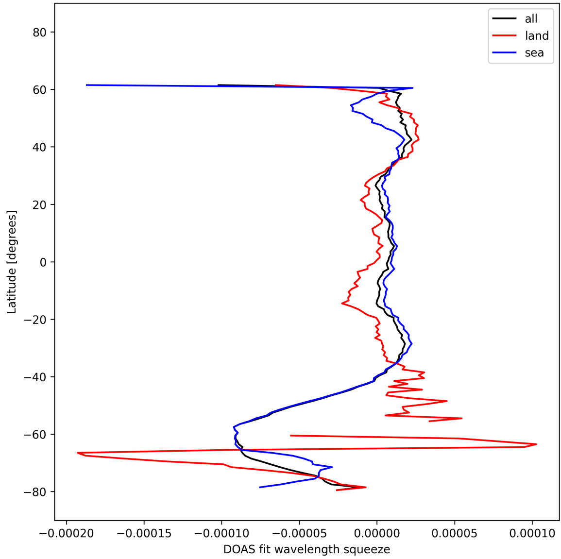
Figure 51: Zonal average of “DOAS fit wavelength squeeze” for 2025-10-16 to 2025-10-17.
