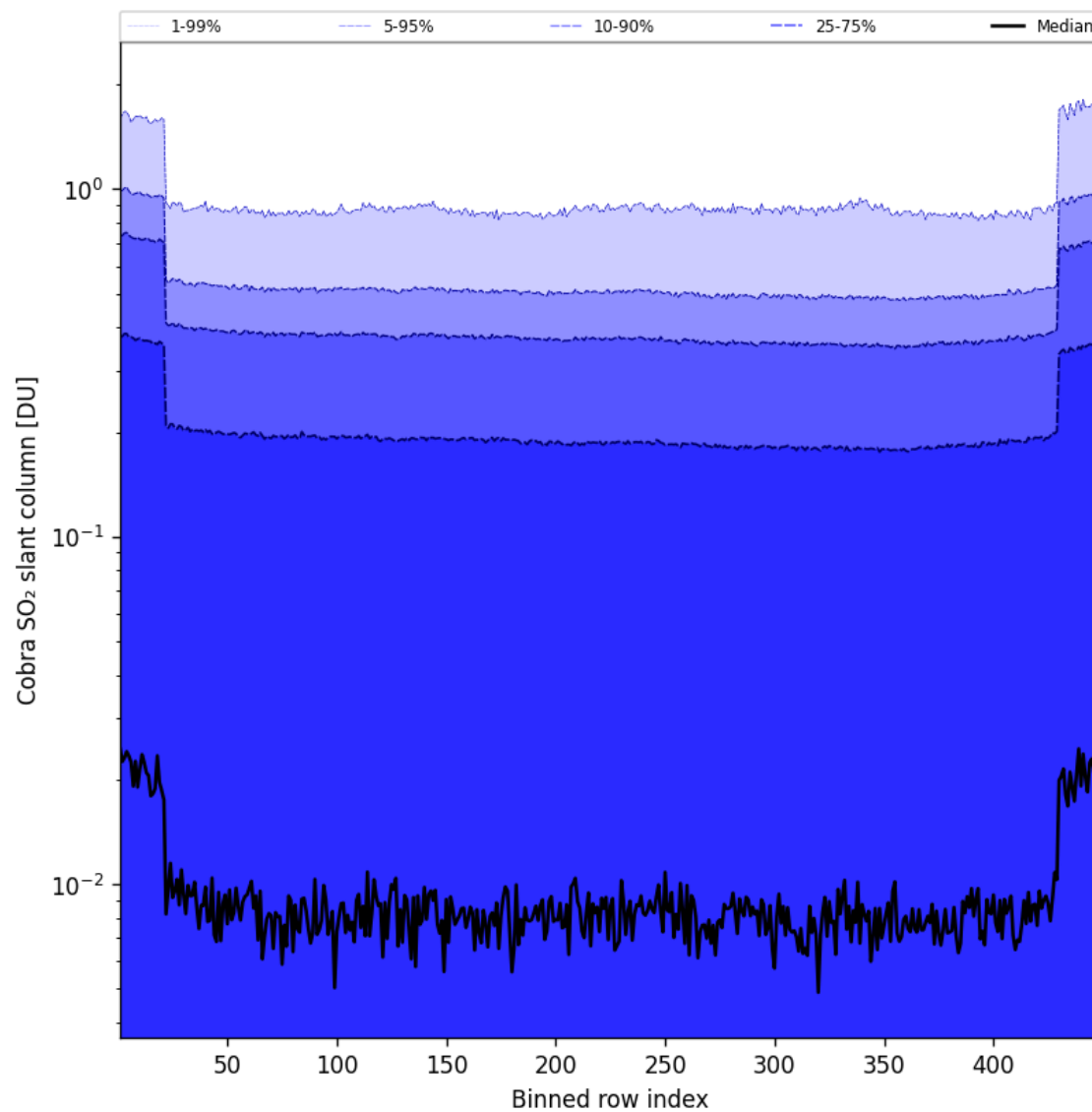
Figure 88: Along track statistics of "Cobra SO 2 slant column" for 2025-10-16 to 2025-10-17
