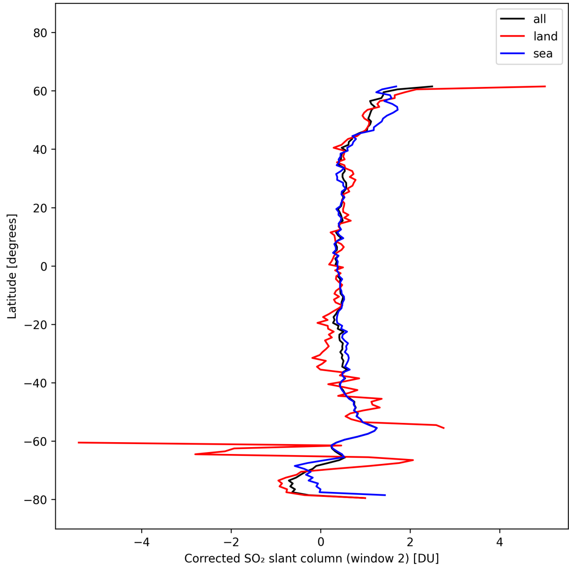
Figure 42: Zonal average of “Corrected SO 2 slant column (window 2)” for 2025-10-16 to 2025-10-17.
