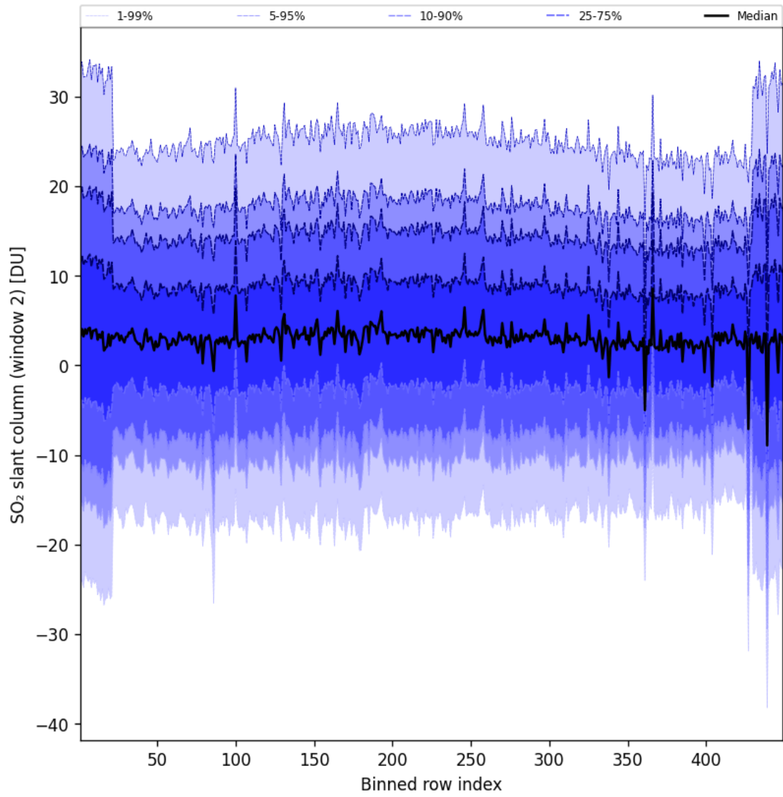
Figure 94: Along track statistics of “SO 2 slant column (window 2)” for 2025-10-16 to 2025-10-17
