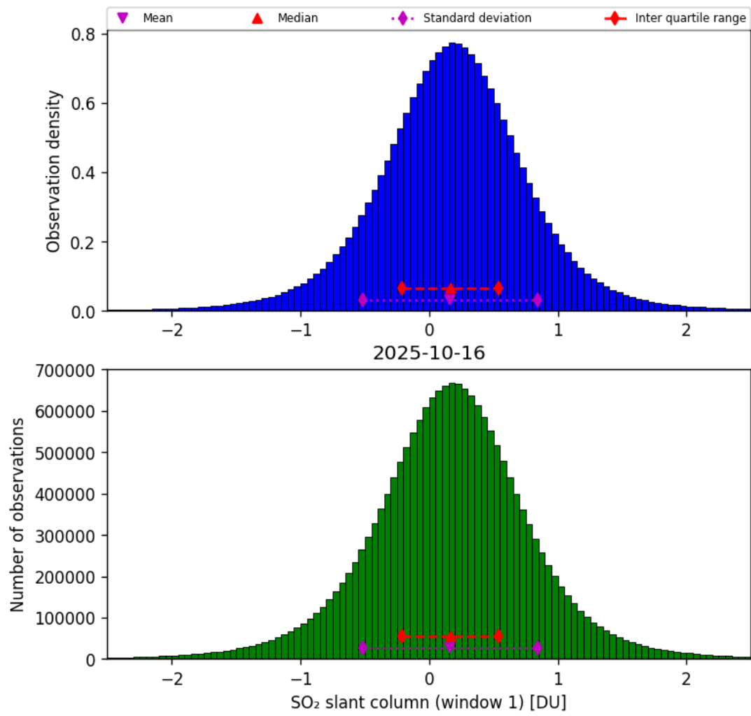
Figure 63: Histogram of “SO 2 slant column (window 1)” for 2025-10-16 to 2025-10-17
