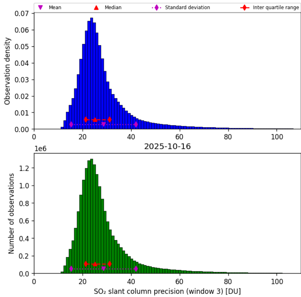
Figure 72: Histogram of “SO 2 slant column precision (window 3)” for 2025-10-16 to 2025-10-17
