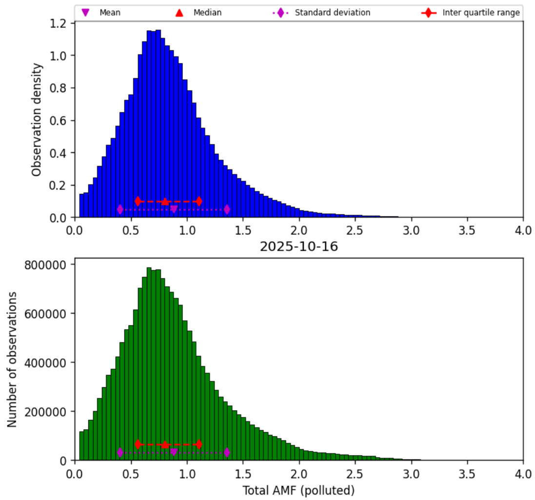
Figure 80: Histogram of “Total AMF (polluted)” for 2025-10-16 to 2025-10-17
