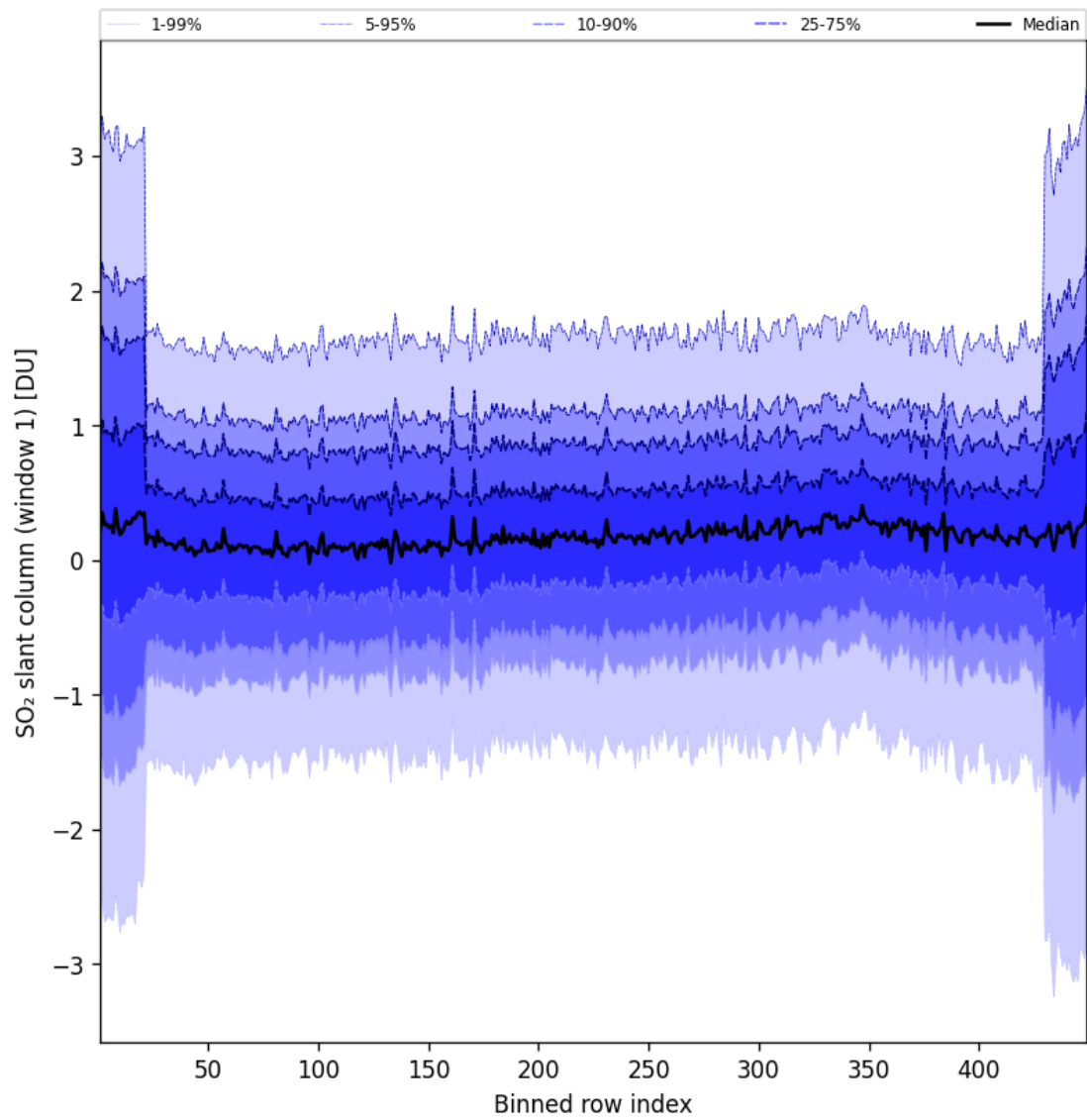
Figure 90: Along track statistics of “SO 2 slant column (window 1)” for 2025-10-16 to 2025-10-17
