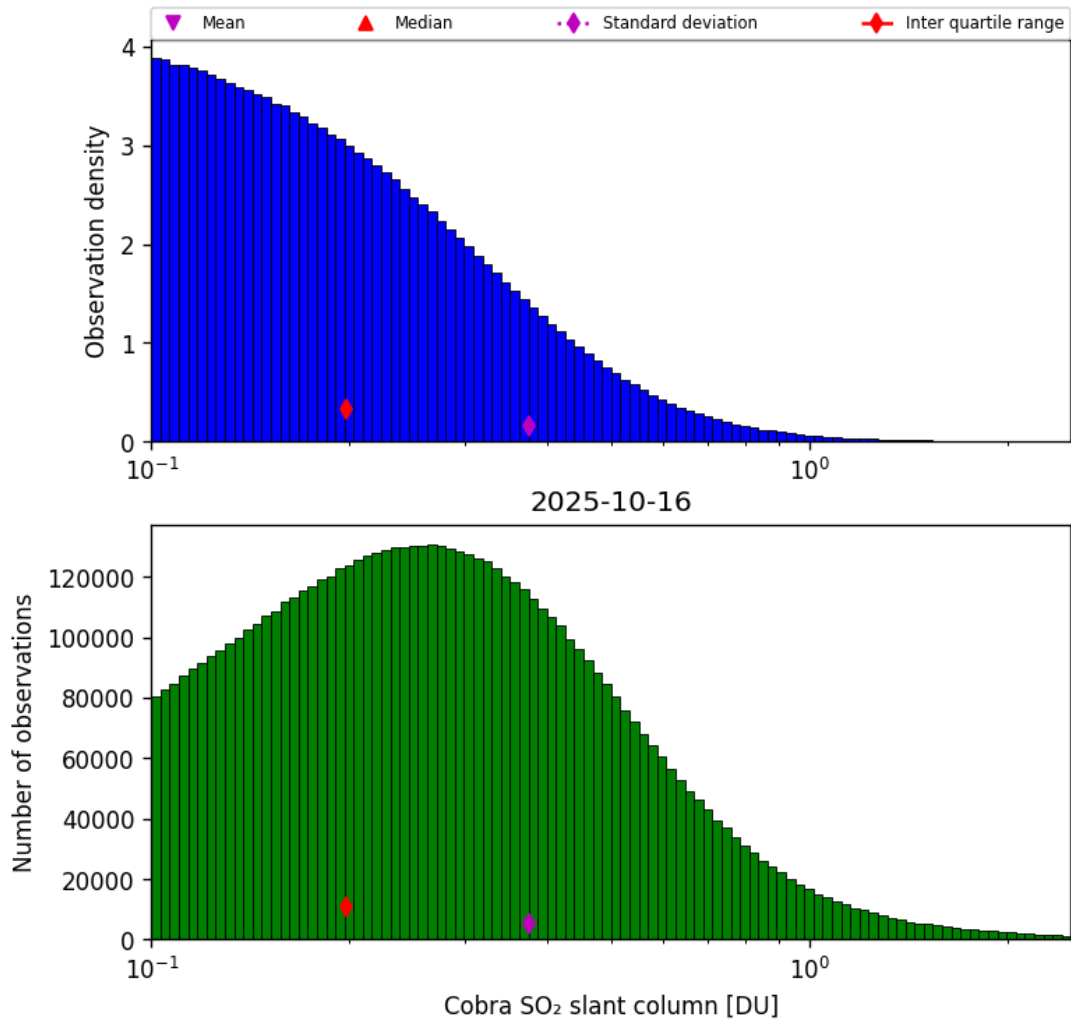
Figure 61: Histogram of “Cobra SO 2 slant column” for 2025-10-16 to 2025-10-17
