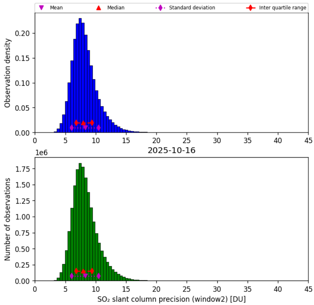
Figure 68: Histogram of “SO 2 slant column precision (window2)” for 2025-10-16 to 2025-10-17
