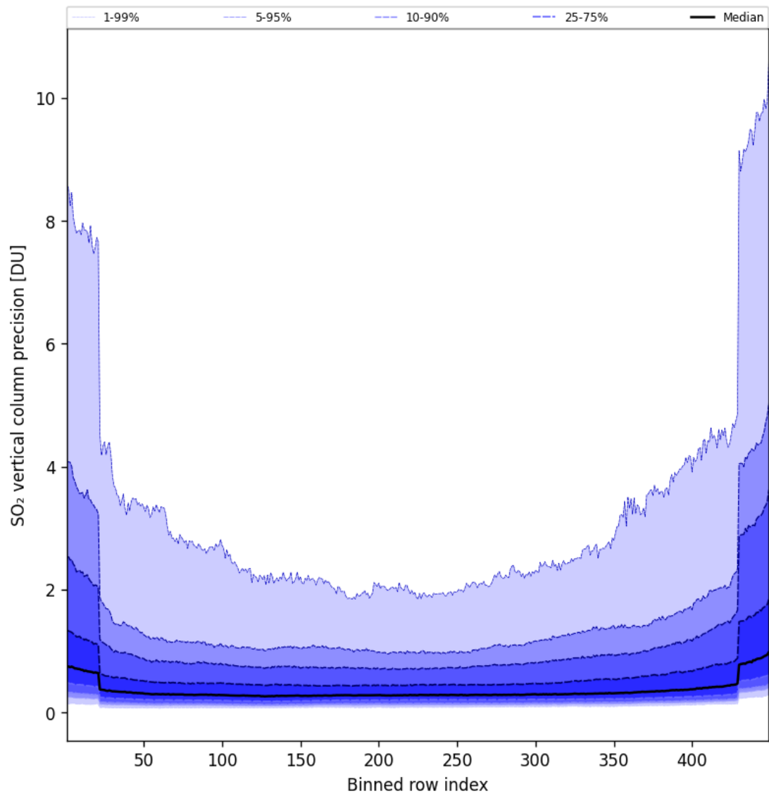
Figure 86: Along track statistics of “SO 2 vertical column precision” for 2025-10-16 to 2025-10-17
