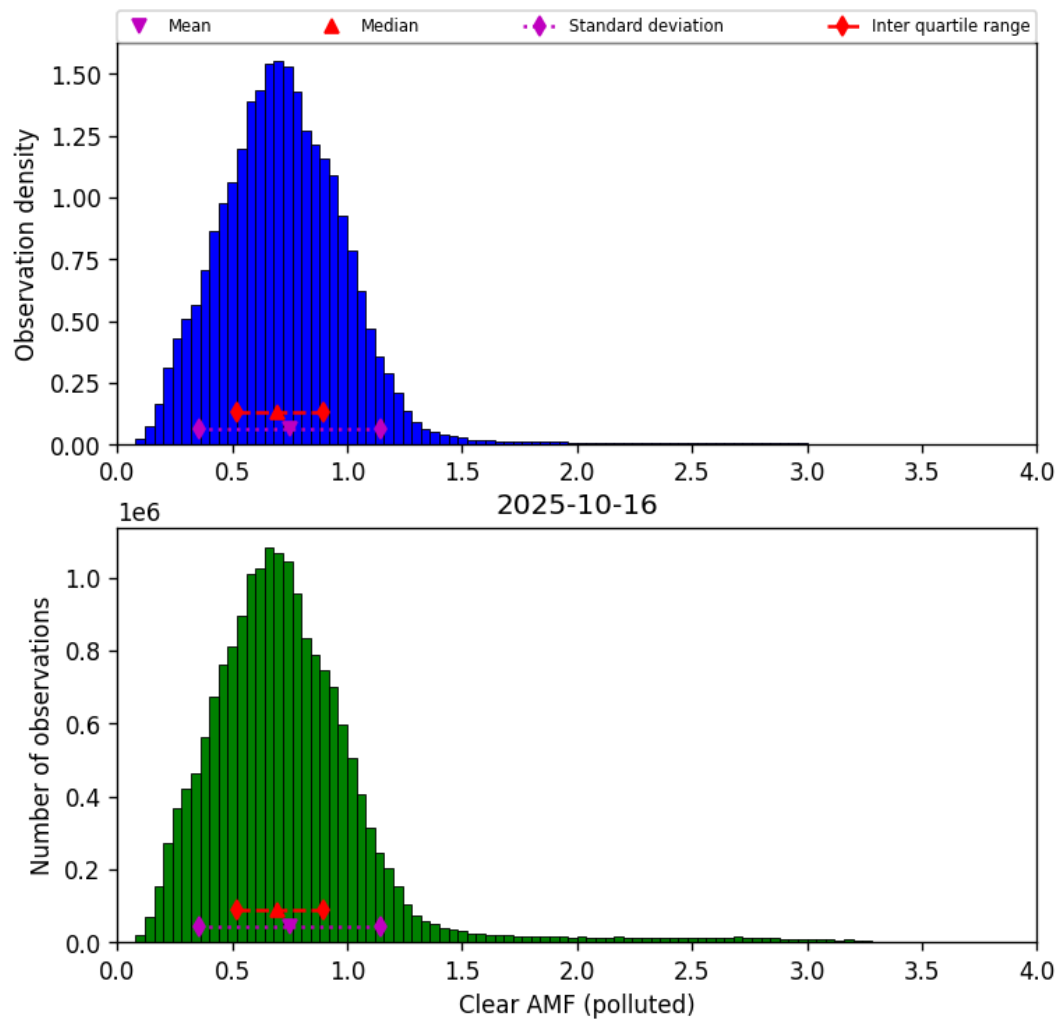
Figure 82: Histogram of “Clear AMF (polluted)” for 2025-10-16 to 2025-10-17
