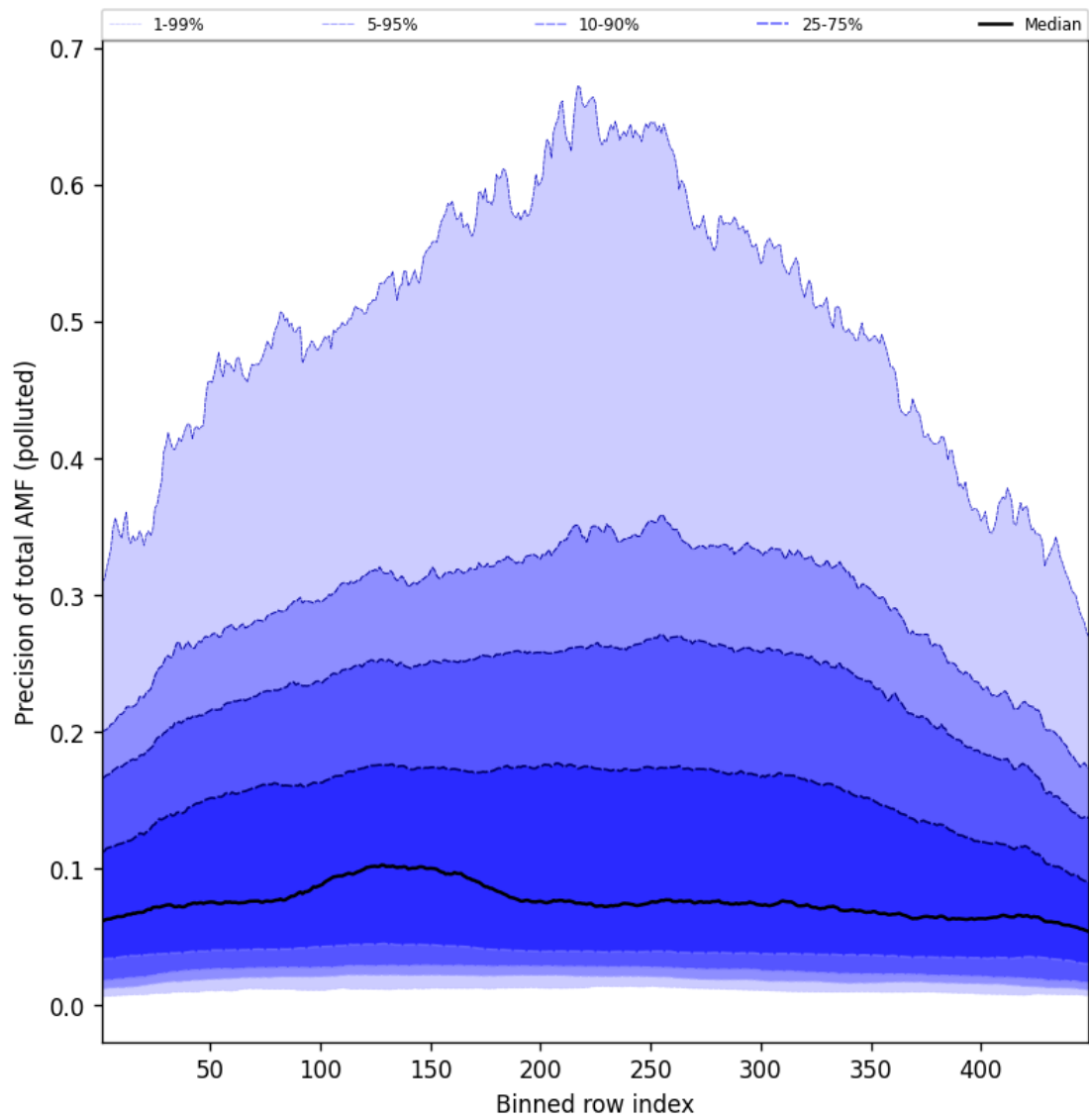
Figure 108: Along track statistics of “Precision of total AMF (polluted)” for 2025-10-16 to 2025-10-17
