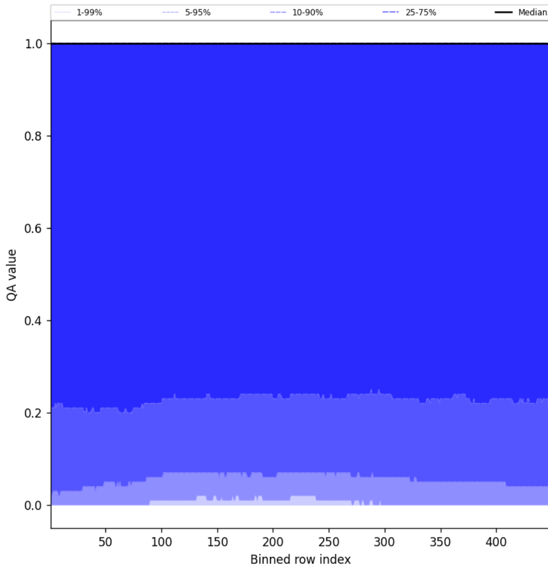
Figure 84: Along track statistics of “QA value” for 2025-10-16 to 2025-10-17
