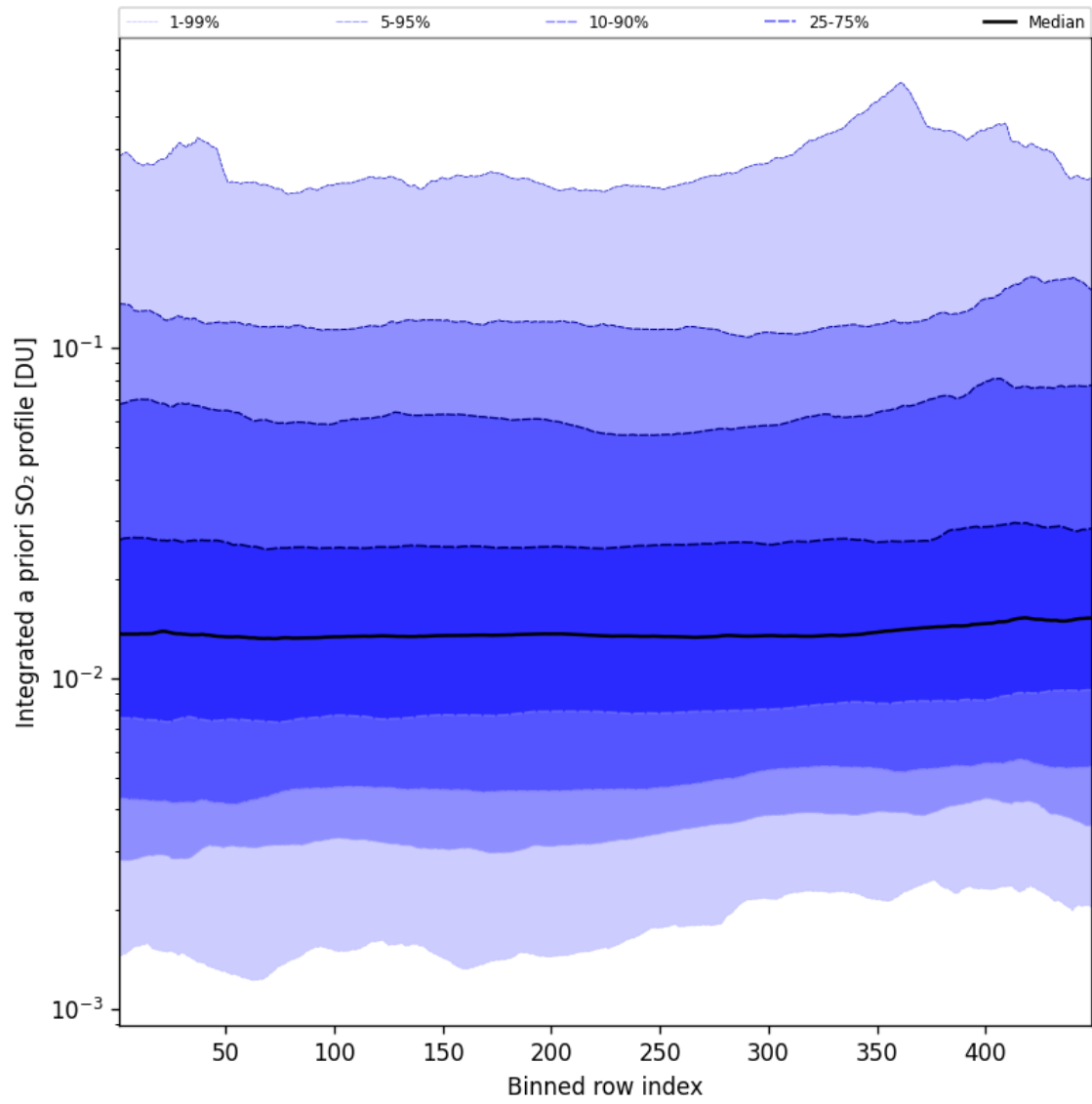
Figure 103: Along track statistics of “Integrated a priori SO 2 profile” for 2025-10-16 to 2025-10-17
