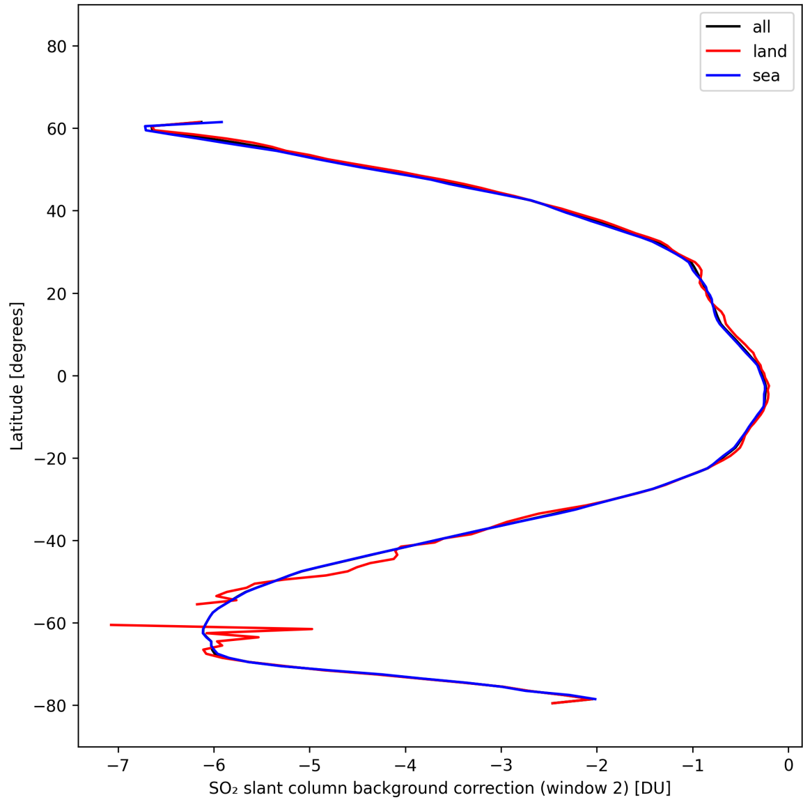
Figure 43: Zonal average of “SO 2 slant column background correction (window 2)” for 2025-10-16 to 2025-10-17.
