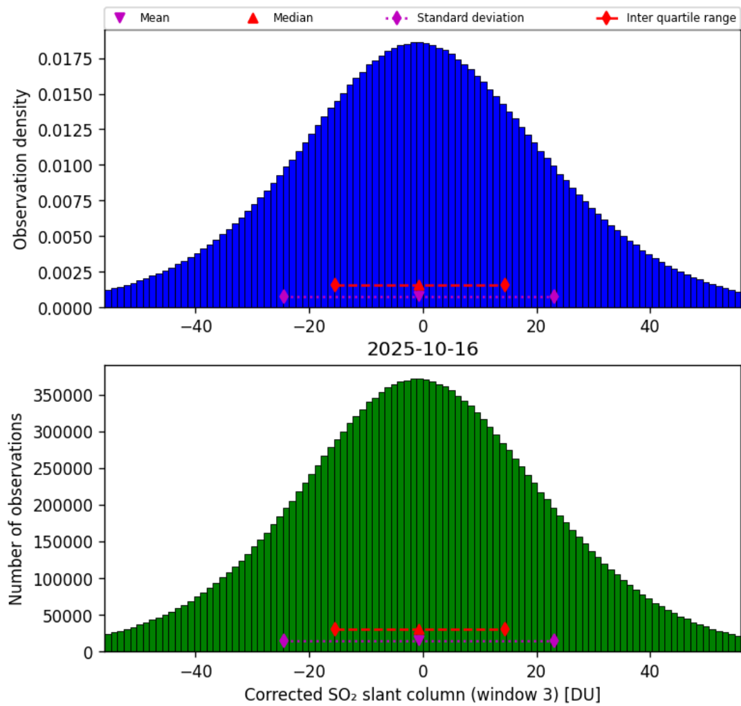
Figure 73: Histogram of “Corrected SO 2 slant column (window 3)” for 2025-10-16 to 2025-10-17
