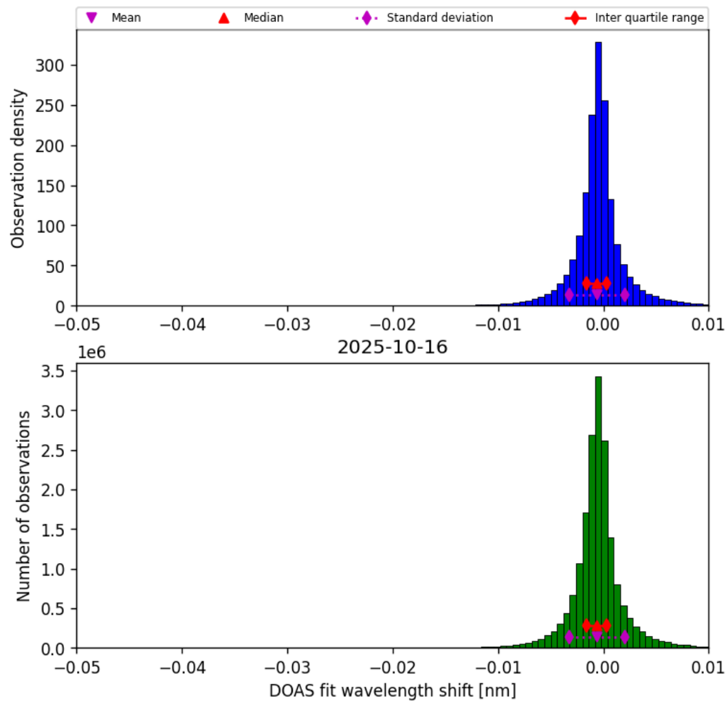
Figure 77: Histogram of “DOAS fit wavelength shift” for 2025-10-16 to 2025-10-17
