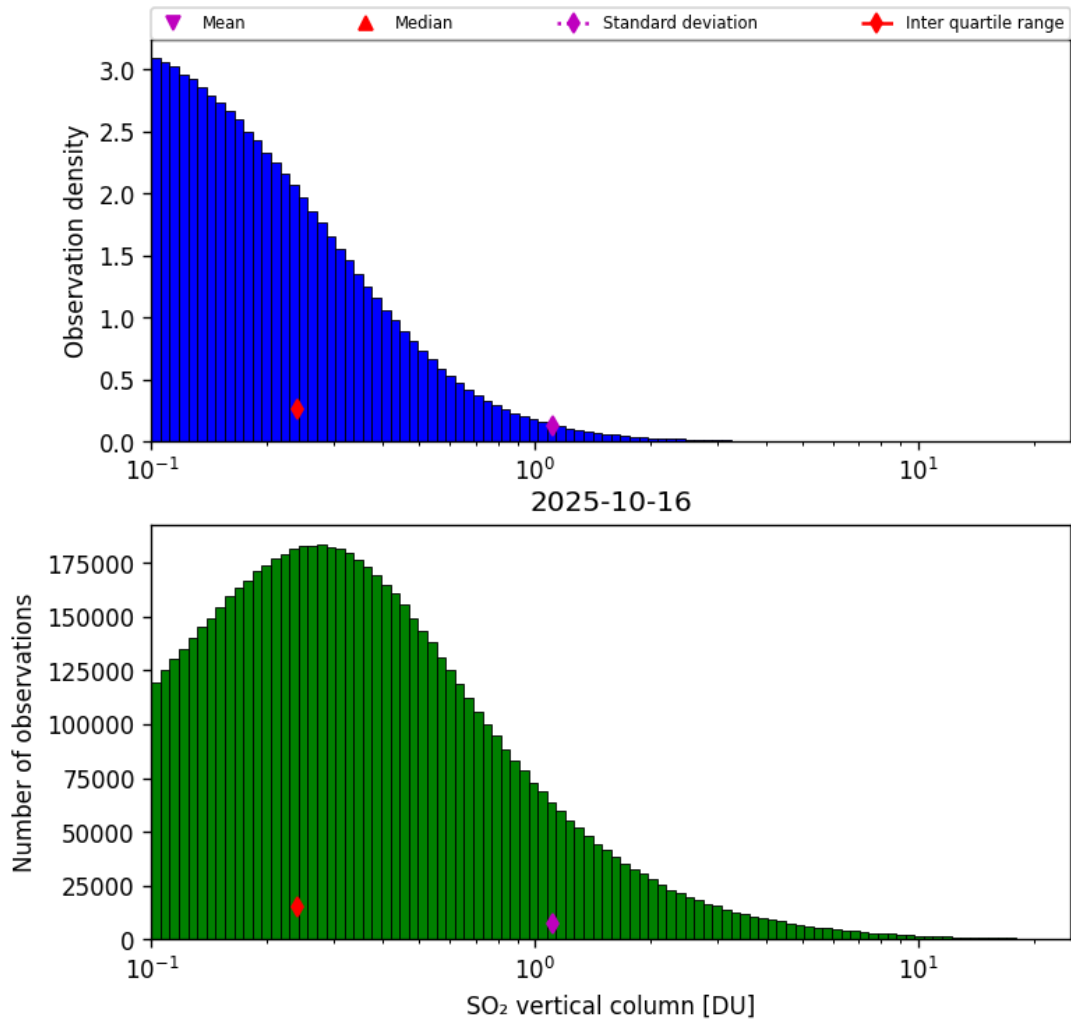
Figure 58: Histogram of “SO 2 vertical column” for 2025-10-16 to 2025-10-17
