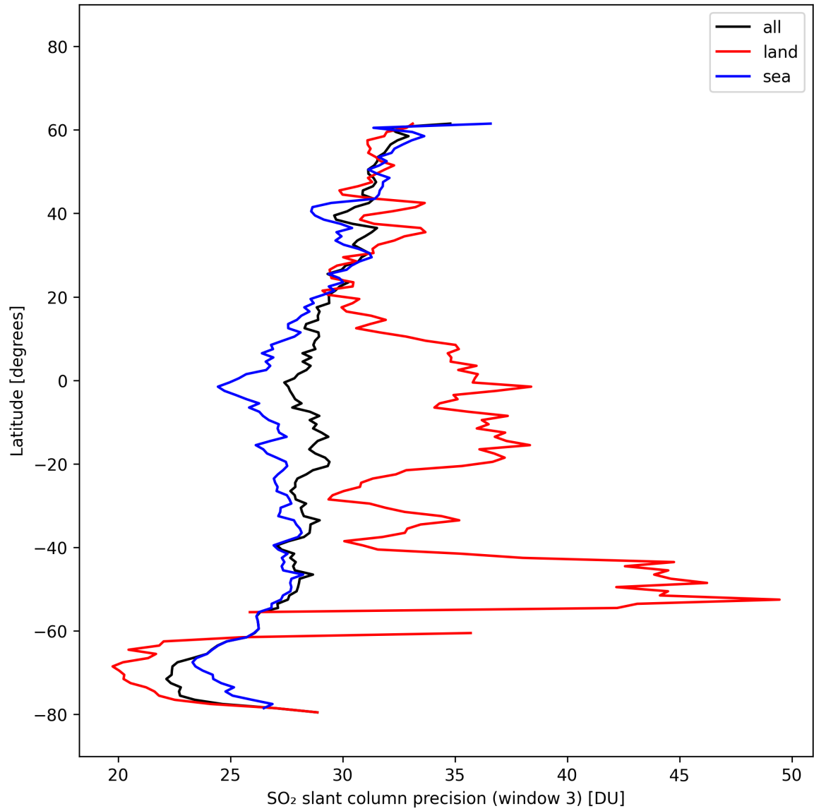
Figure 45: Zonal average of “SO 2 slant column precision (window 3)” for 2025-10-16 to 2025-10-17.
