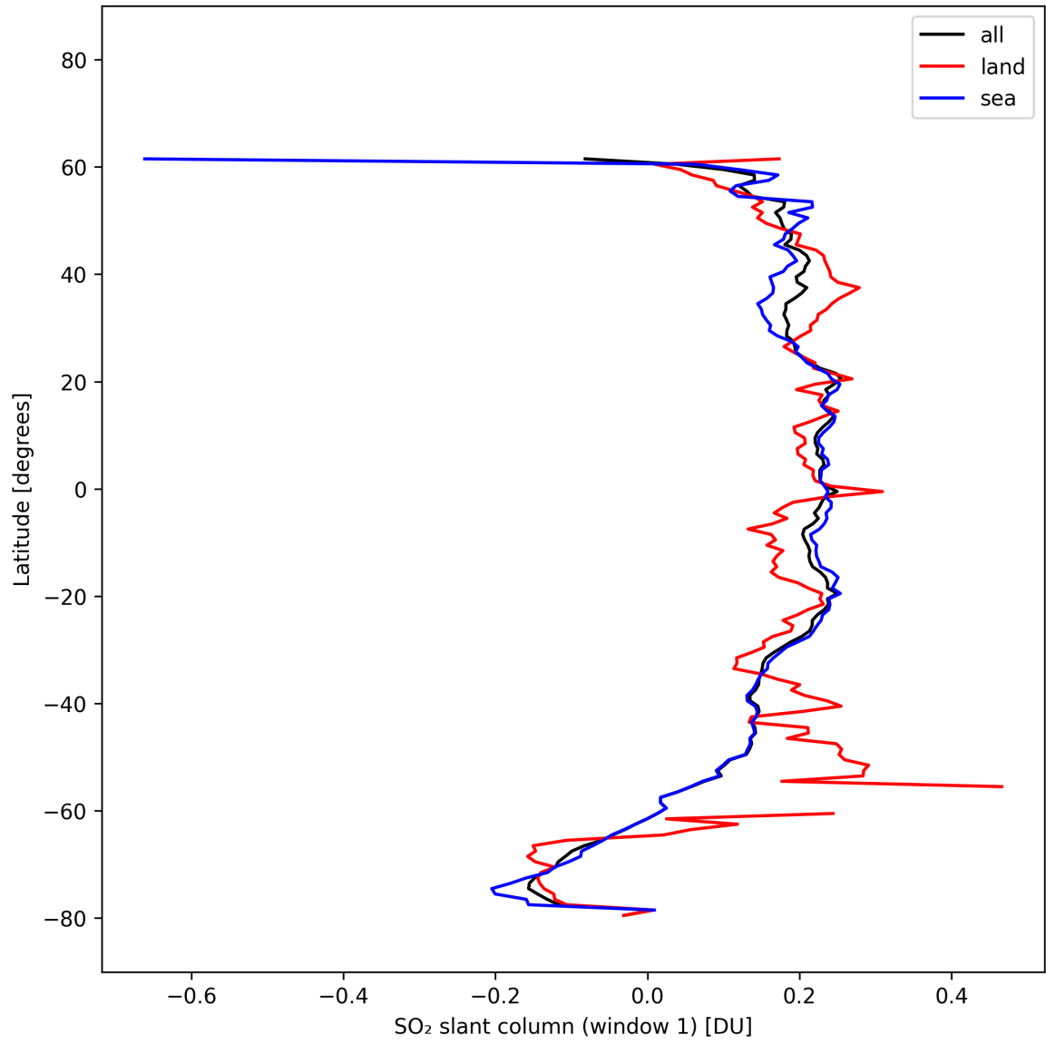
Figure 36: Zonal average of “SO 2 slant column (window 1)” for 2025-10-16 to 2025-10-17.
