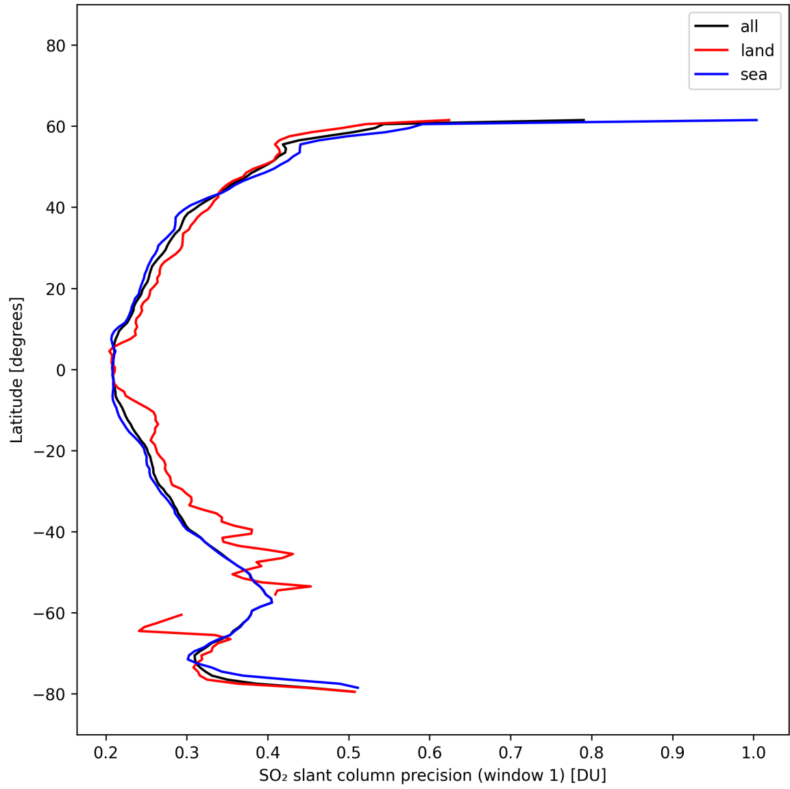
Figure 37: Zonal average of “SO 2 slant column precision (window 1)” for 2025-10-16 to 2025-10-17.
