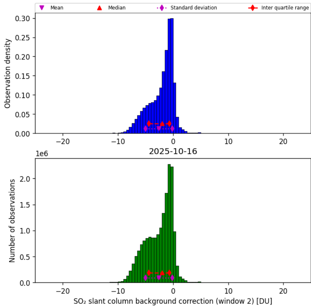
Figure 70: Histogram of “SO 2 slant column background correction (window 2)” for 2025-10-16 to 2025-10-17
