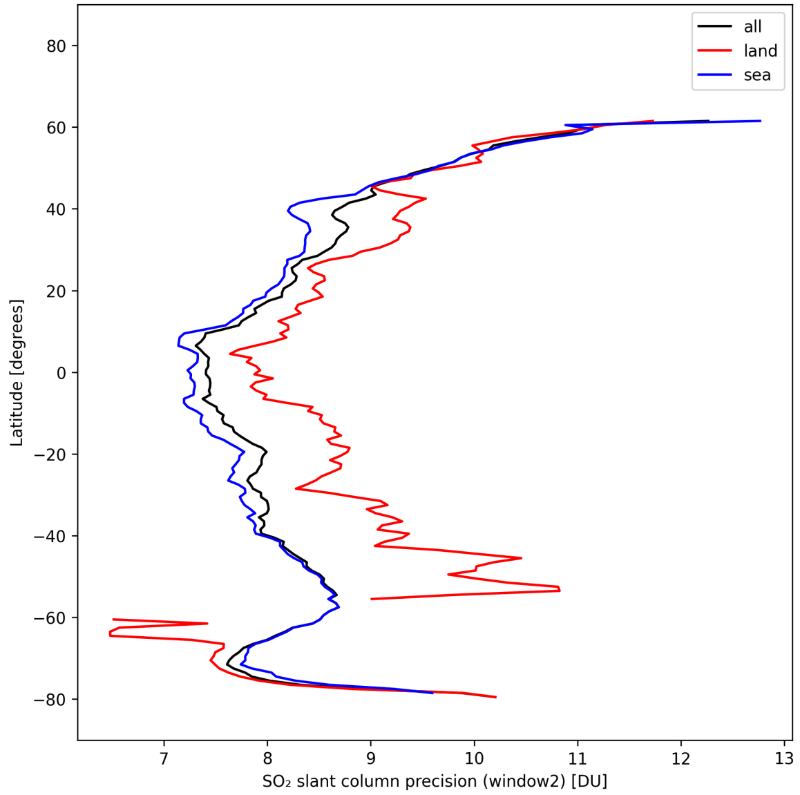
Figure 41: Zonal average of “SO 2 slant column precision (window2)” for 2025-10-16 to 2025-10-17.
