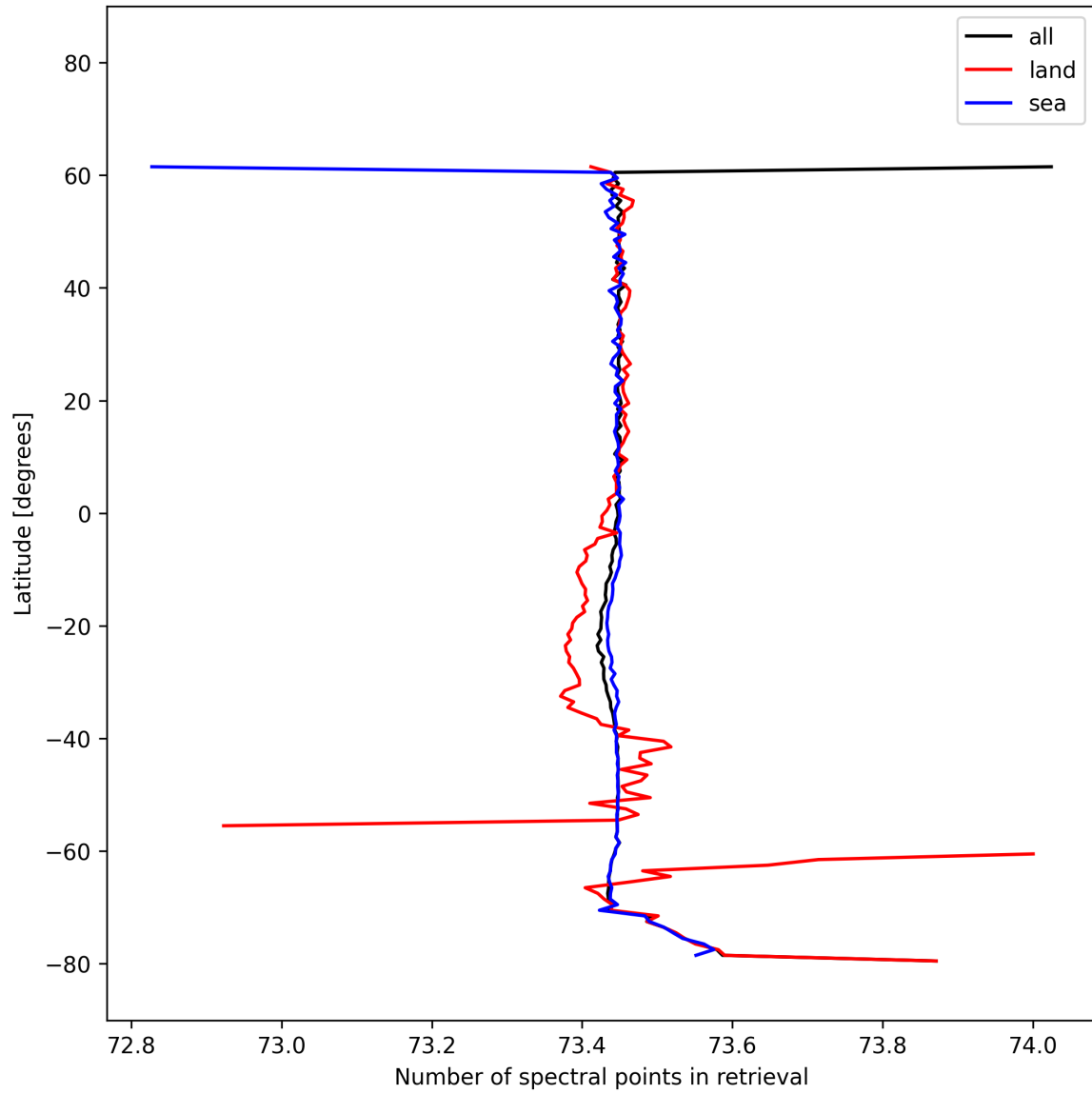
Figure 56: Zonal average of “Number of spectral points in retrieval” for 2025-10-16 to 2025-10-17.
