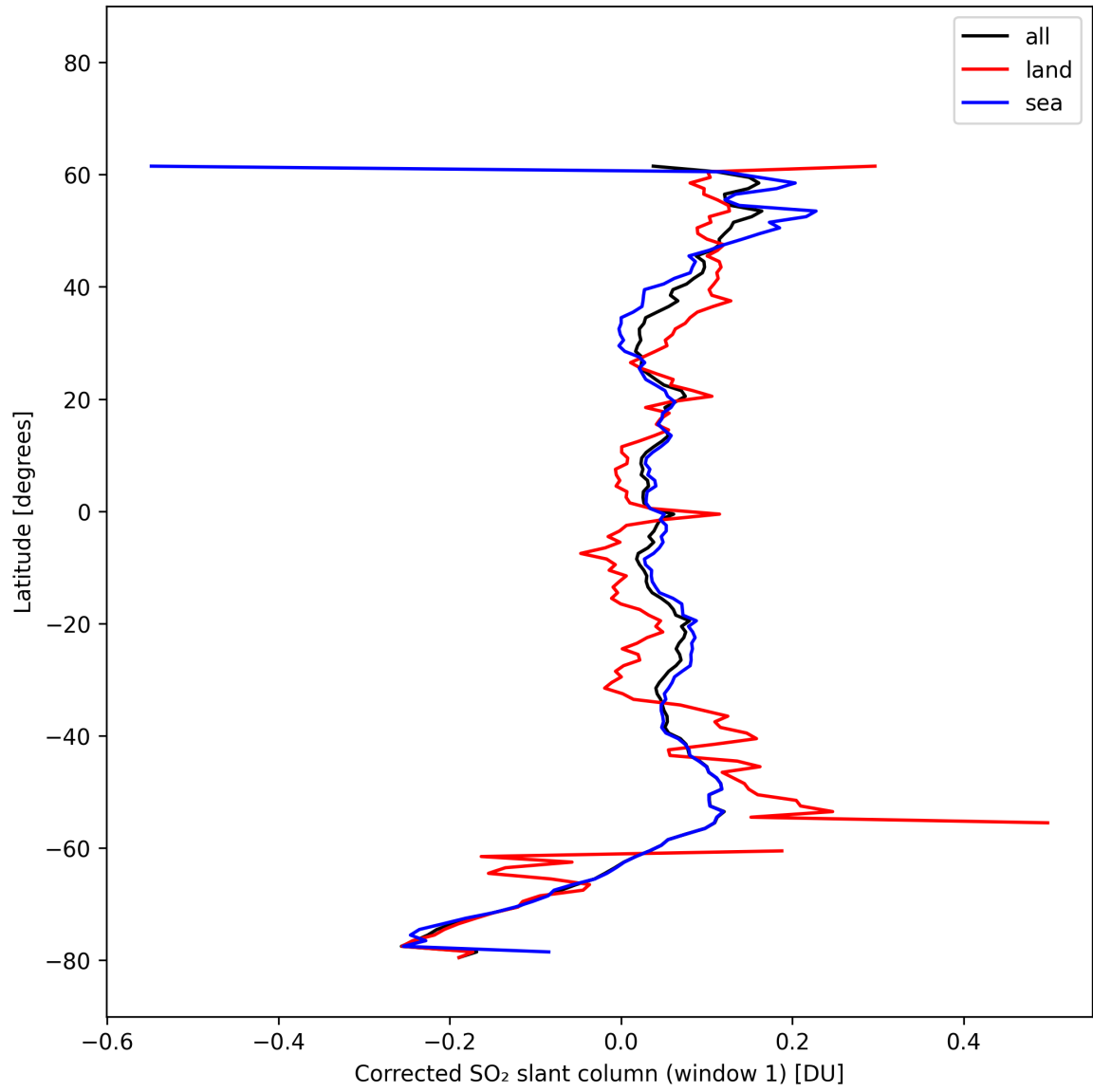
Figure 38: Zonal average of “Corrected SO 2 slant column (window 1)” for 2025-10-16 to 2025-10-17.
