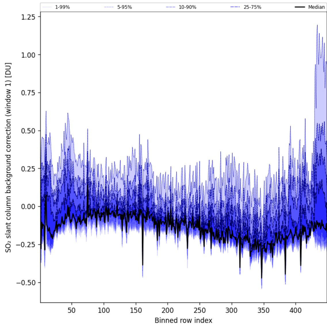
Figure 93: Along track statistics of "SO 2 slant column background correction (window 1)" for 2025-10-16 to 2025-10-17
