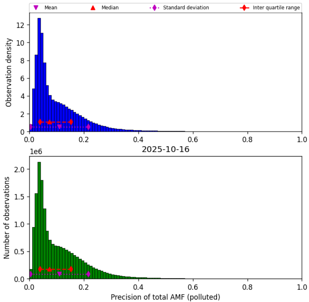
Figure 81: Histogram of “Precision of total AMF (polluted)” for 2025-10-16 to 2025-10-17
