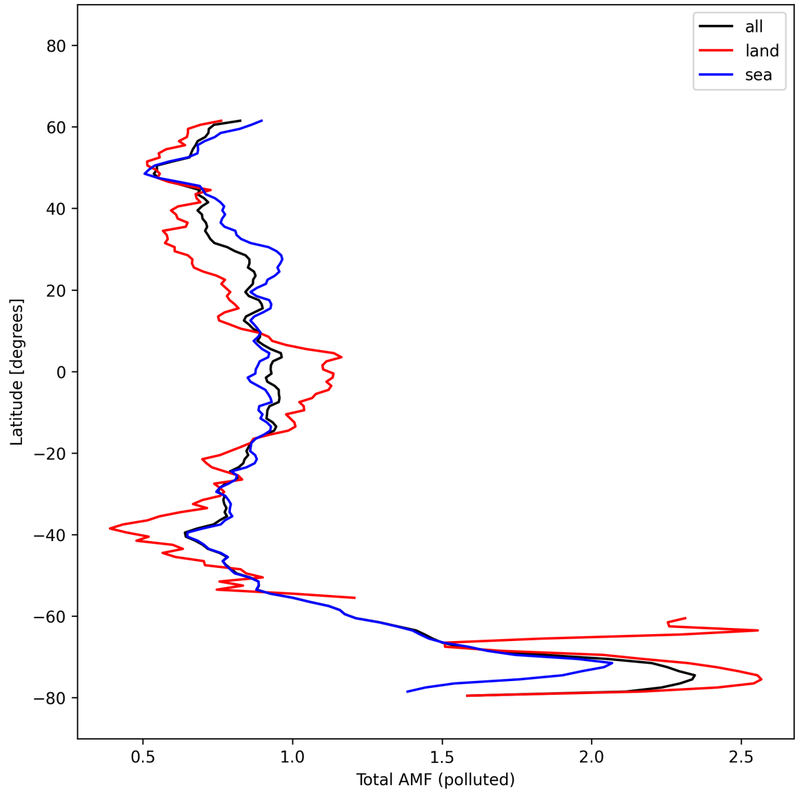
Figure 53: Zonal average of “Total AMF (polluted)” for 2025-10-16 to 2025-10-17.
