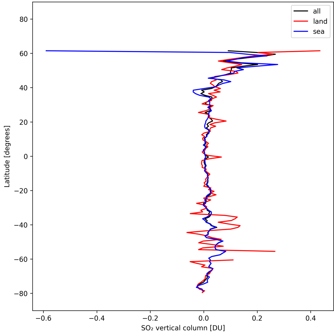
Figure 31: Zonal average of “SO 2 vertical column” for 2025-10-16 to 2025-10-17.
