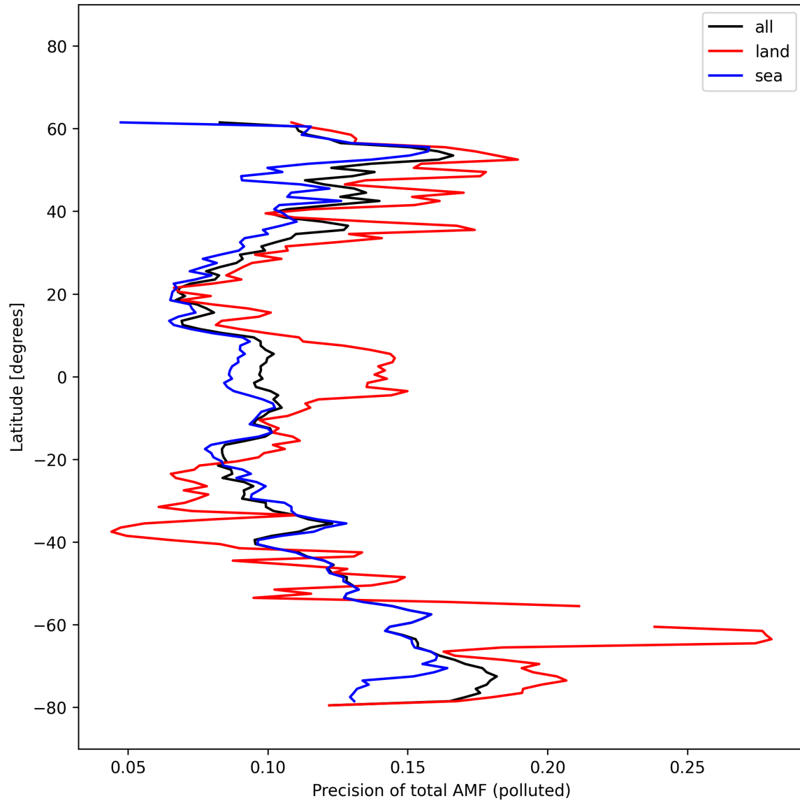
Figure 54: Zonal average of “Precision of total AMF (polluted)” for 2025-10-16 to 2025-10-17.
