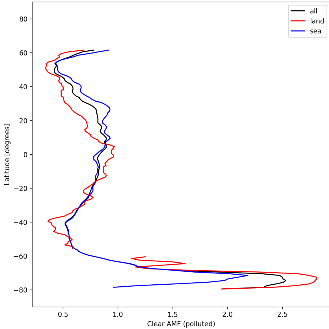
Figure 55: Zonal average of “Clear AMF (polluted)” for 2025-10-16 to 2025-10-17.
