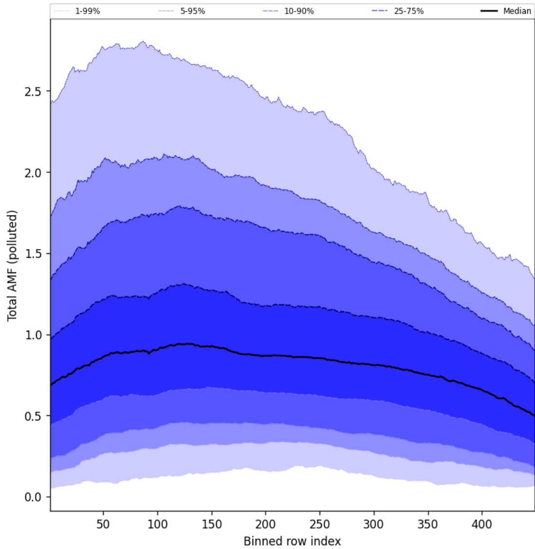
Figure 107: Along track statistics of “Total AMF (polluted)” for 2025-10-16 to 2025-10-17
