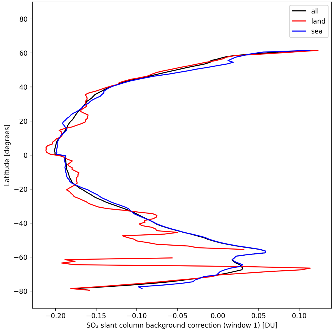
Figure 39: Zonal average of “SO 2 slant column background correction (window 1)” for 2025-10-16 to 2025-10-17.
