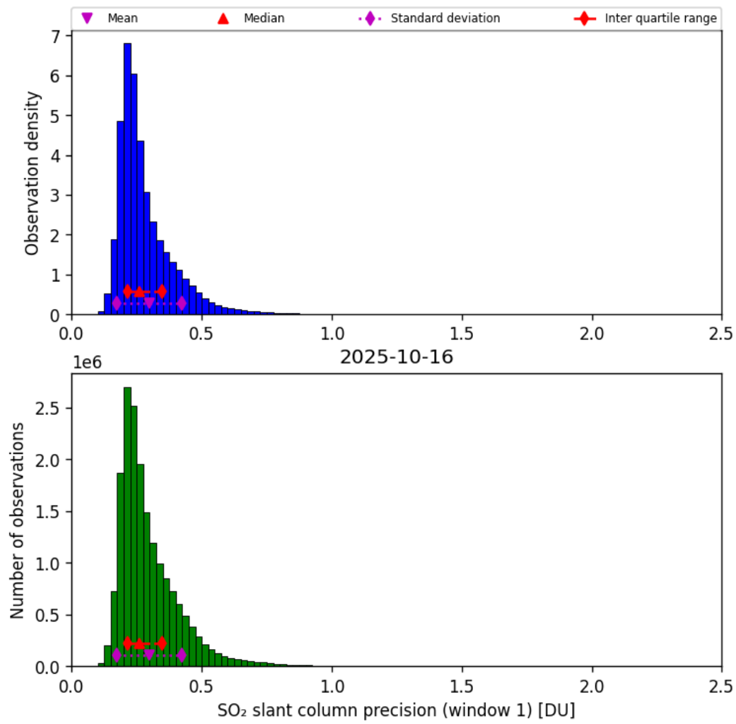
Figure 64: Histogram of “SO 2 slant column precision (window 1)” for 2025-10-16 to 2025-10-17
