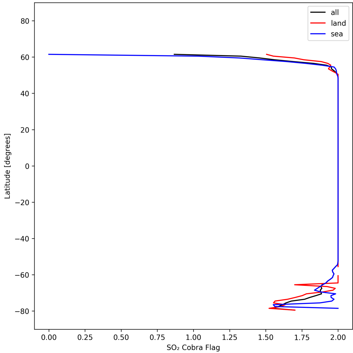
Figure 48: Zonal average of “SO 2 Cobra Flag” for 2025-10-16 to 2025-10-17.
