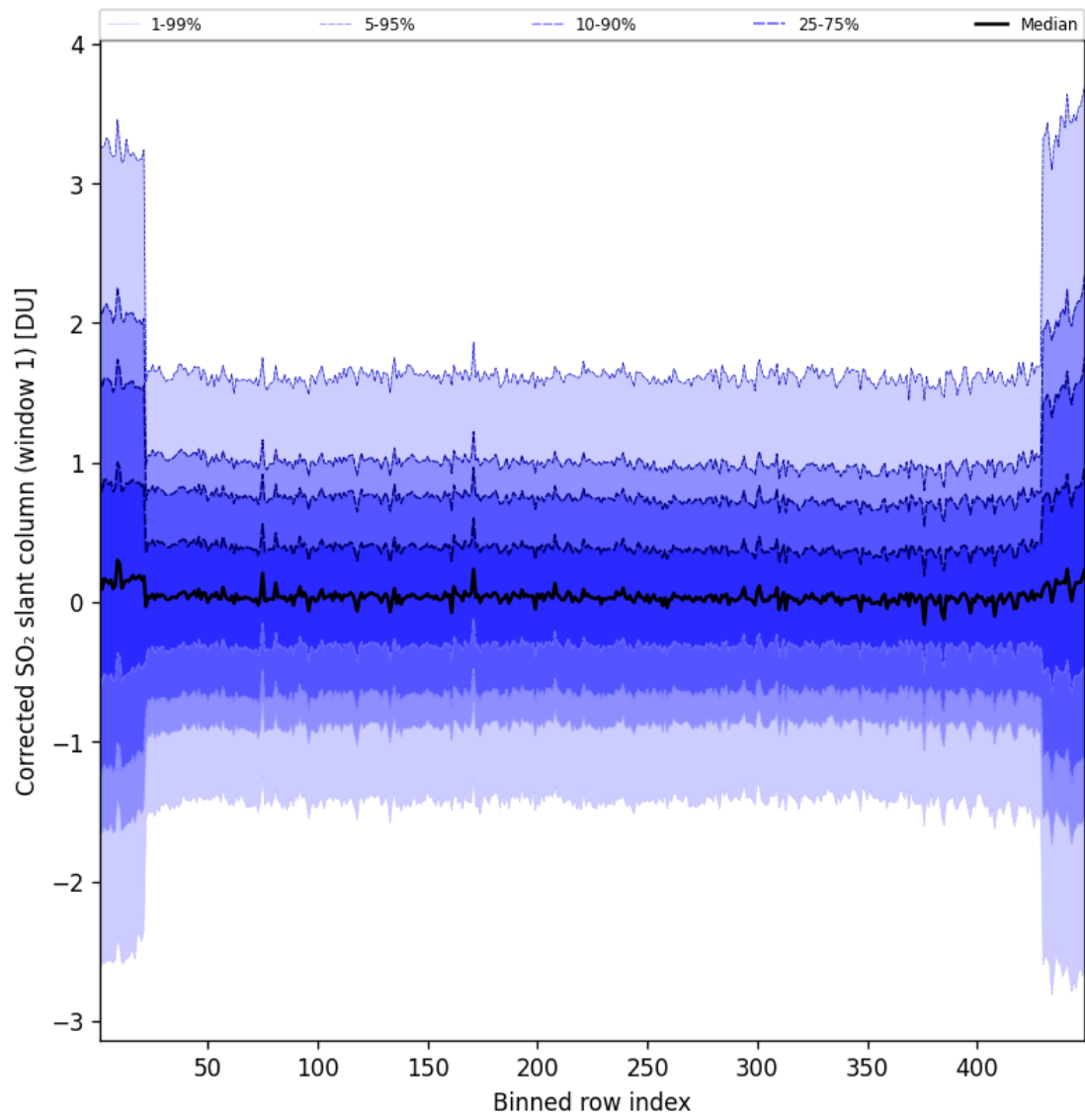
Figure 92: Along track statistics of “Corrected SO 2 slant column (window 1)” for 2025-10-16 to 2025-10-17
