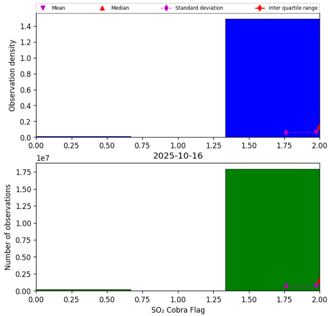
Figure 75: Histogram of “SO 2 Cobra Flag” for 2025-10-16 to 2025-10-17
