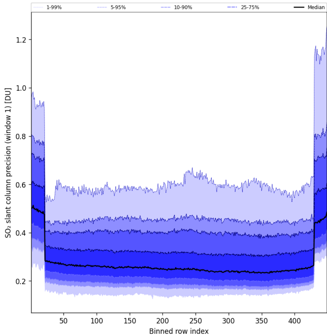
Figure 91: Along track statistics of “SO 2 slant column precision (window 1)” for 2025-10-16 to 2025-10-17
