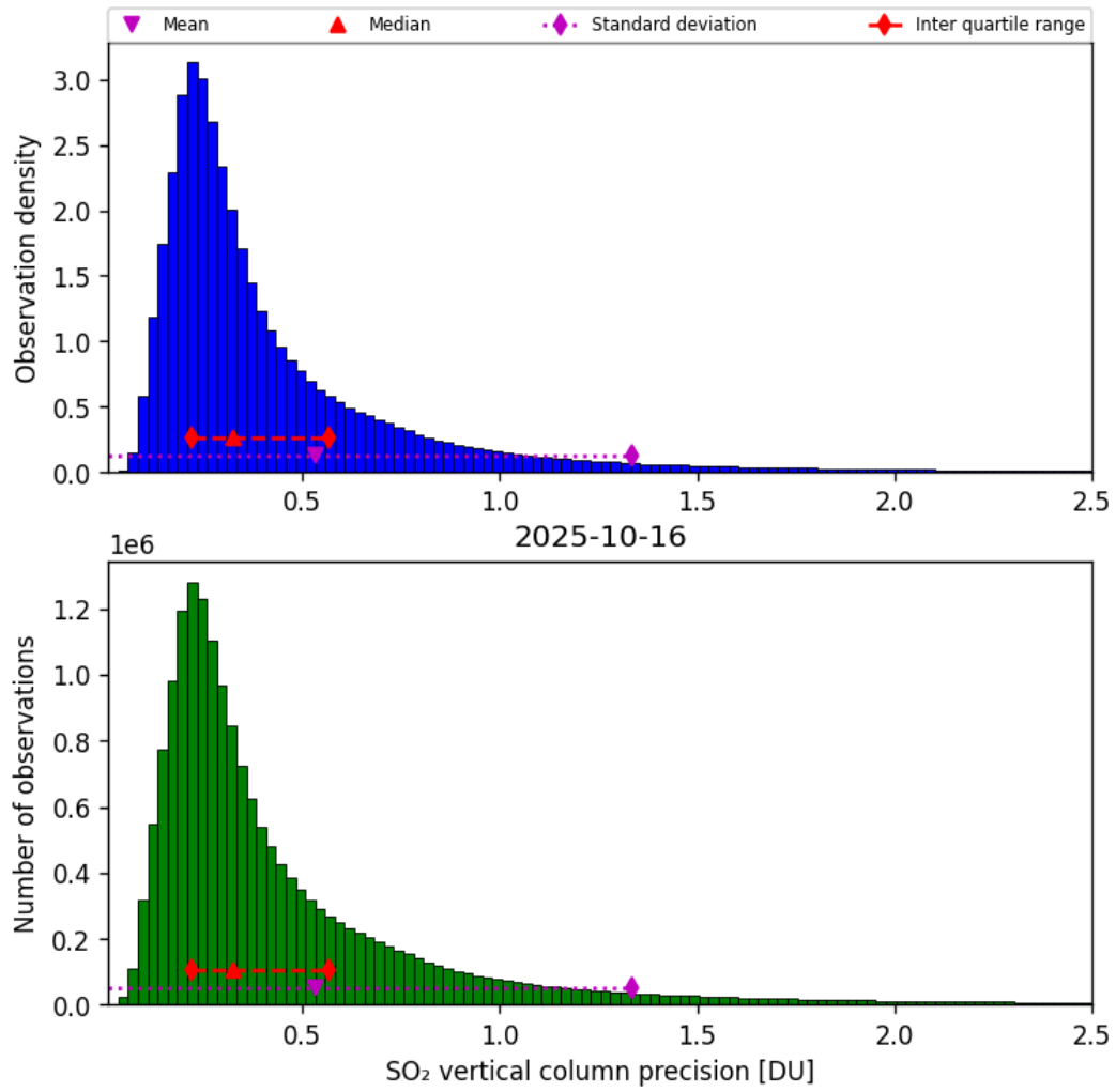
Figure 59: Histogram of “SO 2 vertical column precision” for 2025-10-16 to 2025-10-17
