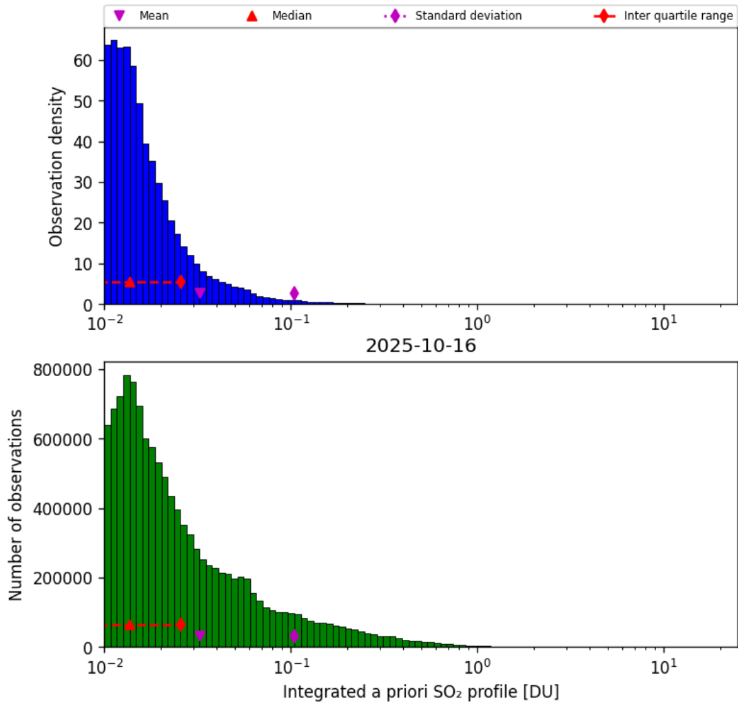
Figure 76: Histogram of “Integrated a priori SO 2 profile” for 2025-10-16 to 2025-10-17
