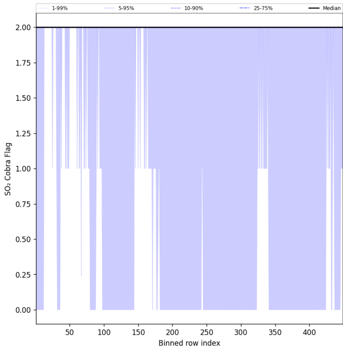
Figure 102: Along track statistics of “SO 2 Cobra Flag” for 2025-10-17 to 2025-10-18
