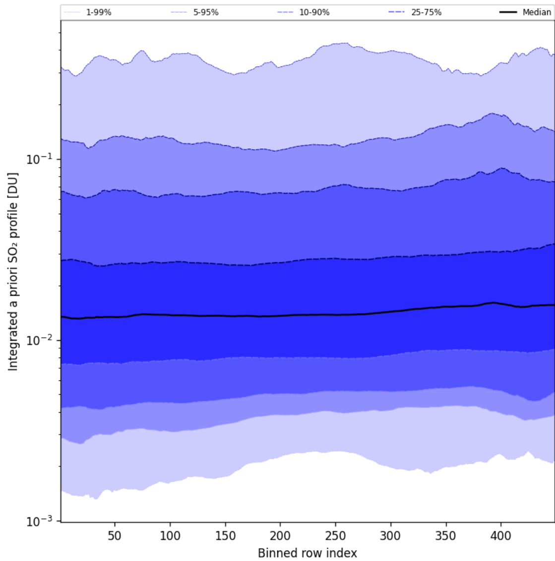
Figure 103: Along track statistics of “Integrated a priori SO 2 profile” for 2025-10-17 to 2025-10-18
