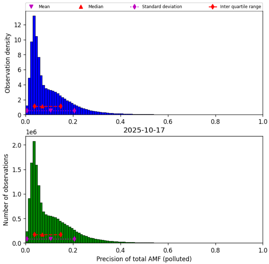
Figure 81: Histogram of “Precision of total AMF (polluted)” for 2025-10-17 to 2025-10-18
