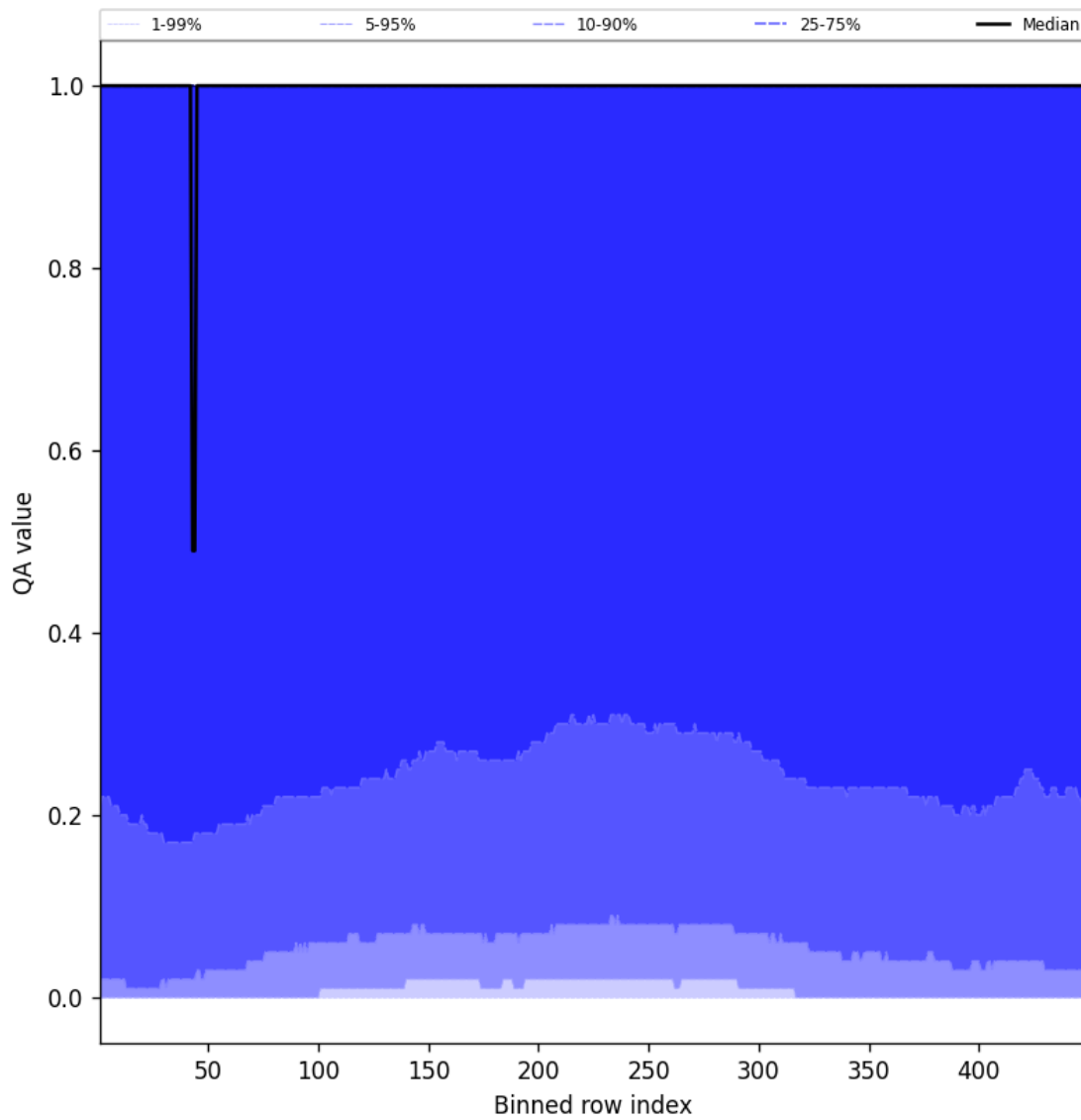
Figure 84: Along track statistics of “QA value” for 2025-10-17 to 2025-10-18
