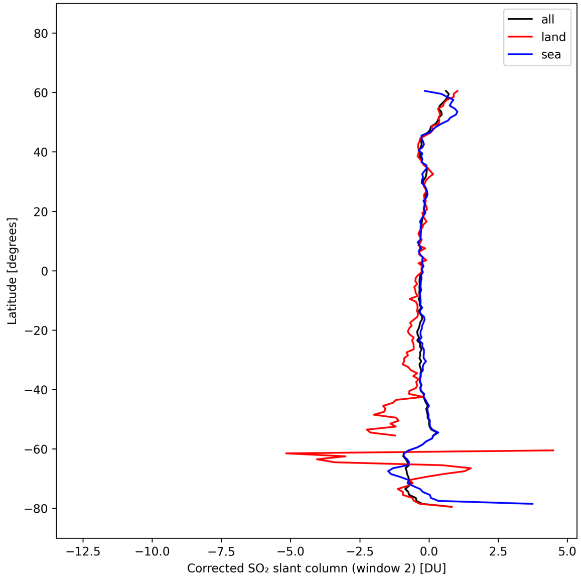
Figure 42: Zonal average of “Corrected SO 2 slant column (window 2)” for 2025-10-17 to 2025-10-18.
