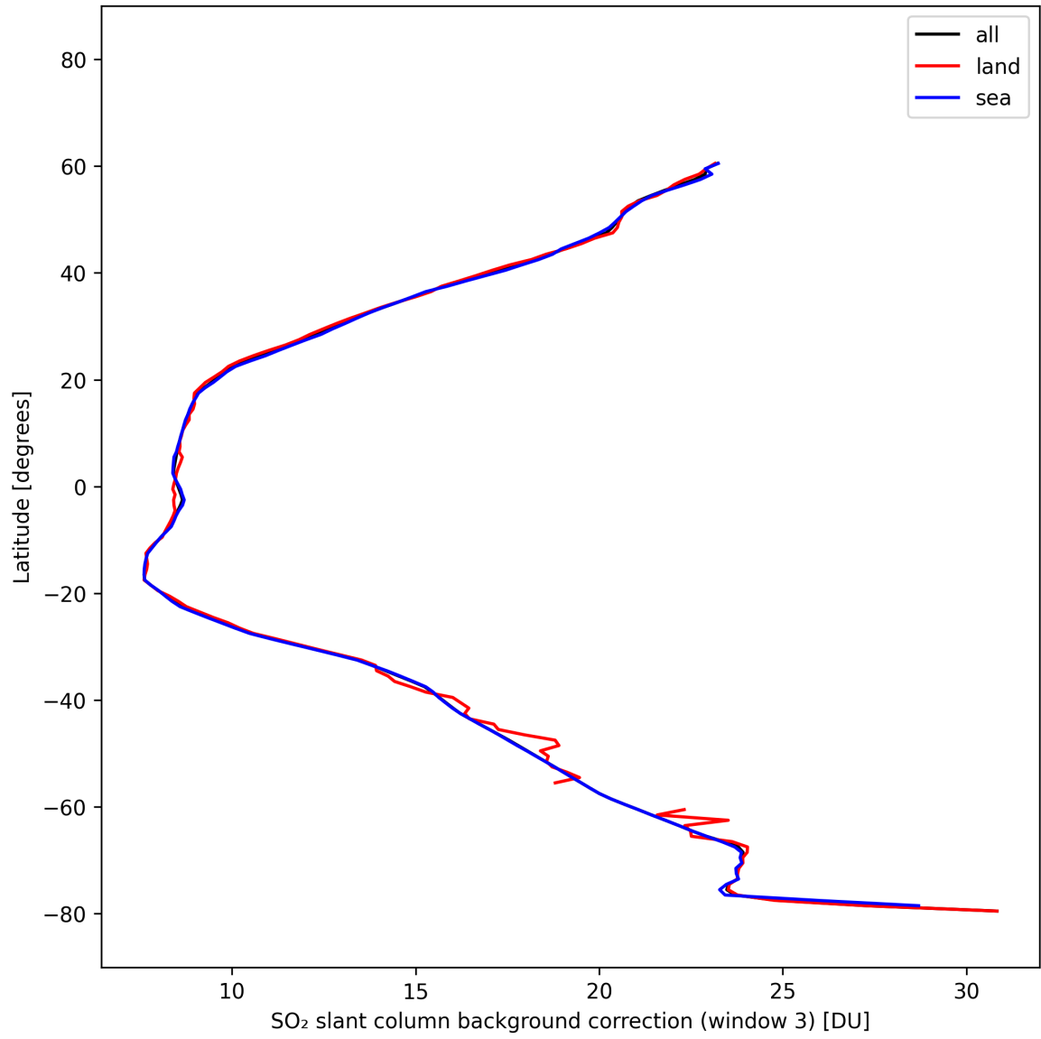
Figure 47: Zonal average of “SO 2 slant column background correction (window 3)” for 2025-10-17 to 2025-10-18.
