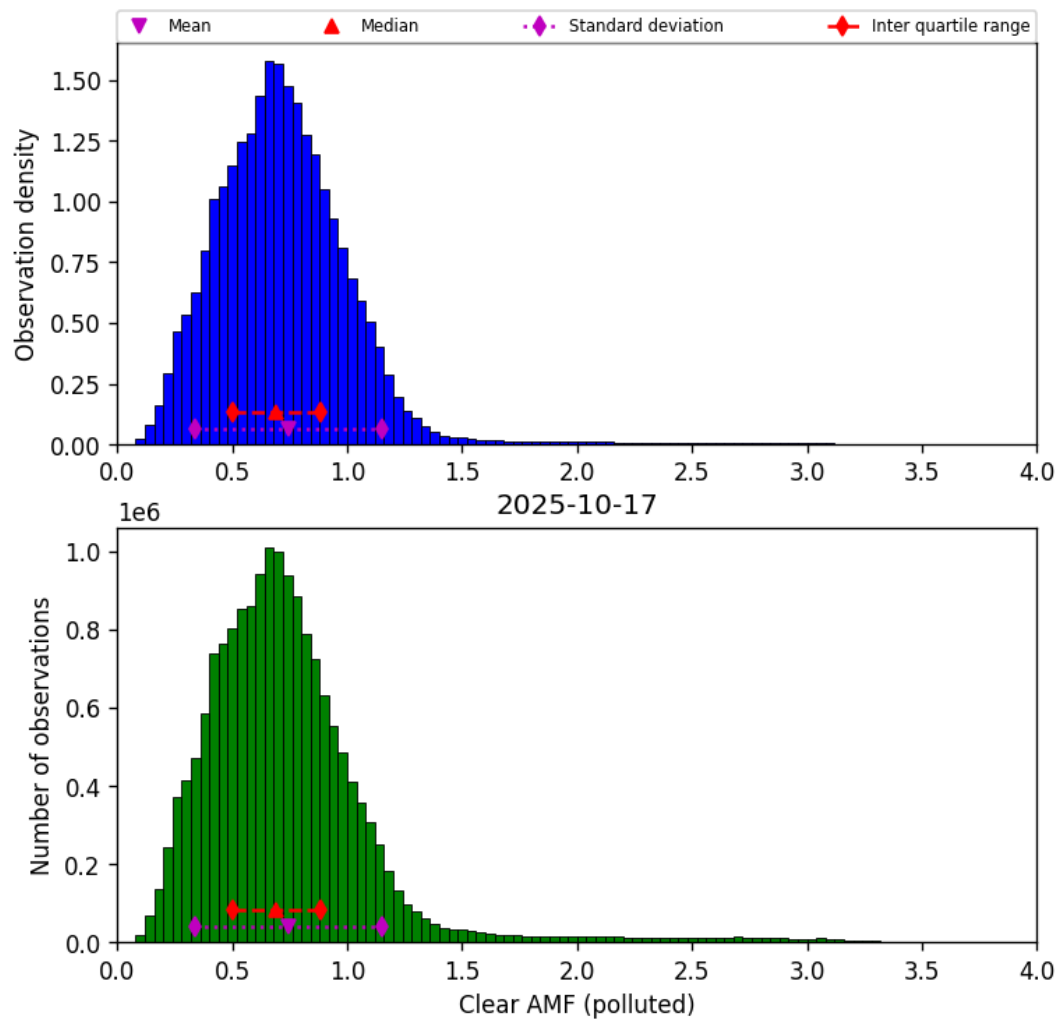
Figure 82: Histogram of “Clear AMF (polluted)” for 2025-10-17 to 2025-10-18
