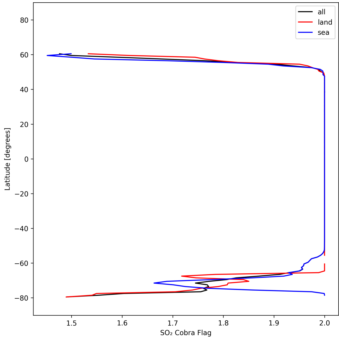
Figure 48: Zonal average of “SO 2 Cobra Flag” for 2025-10-17 to 2025-10-18.
