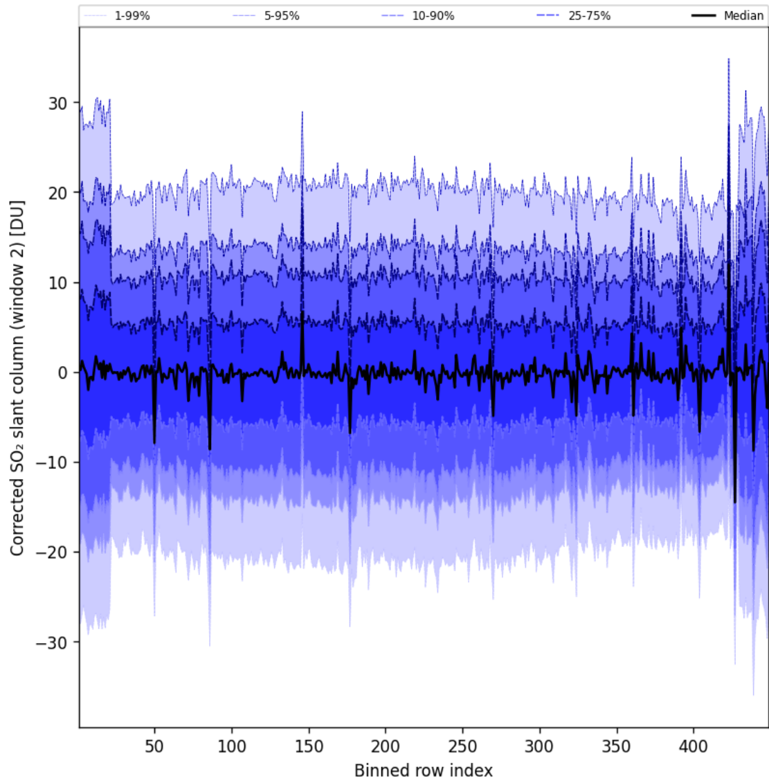
Figure 96: Along track statistics of “Corrected SO 2 slant column (window 2)” for 2025-10-17 to 2025-10-18
