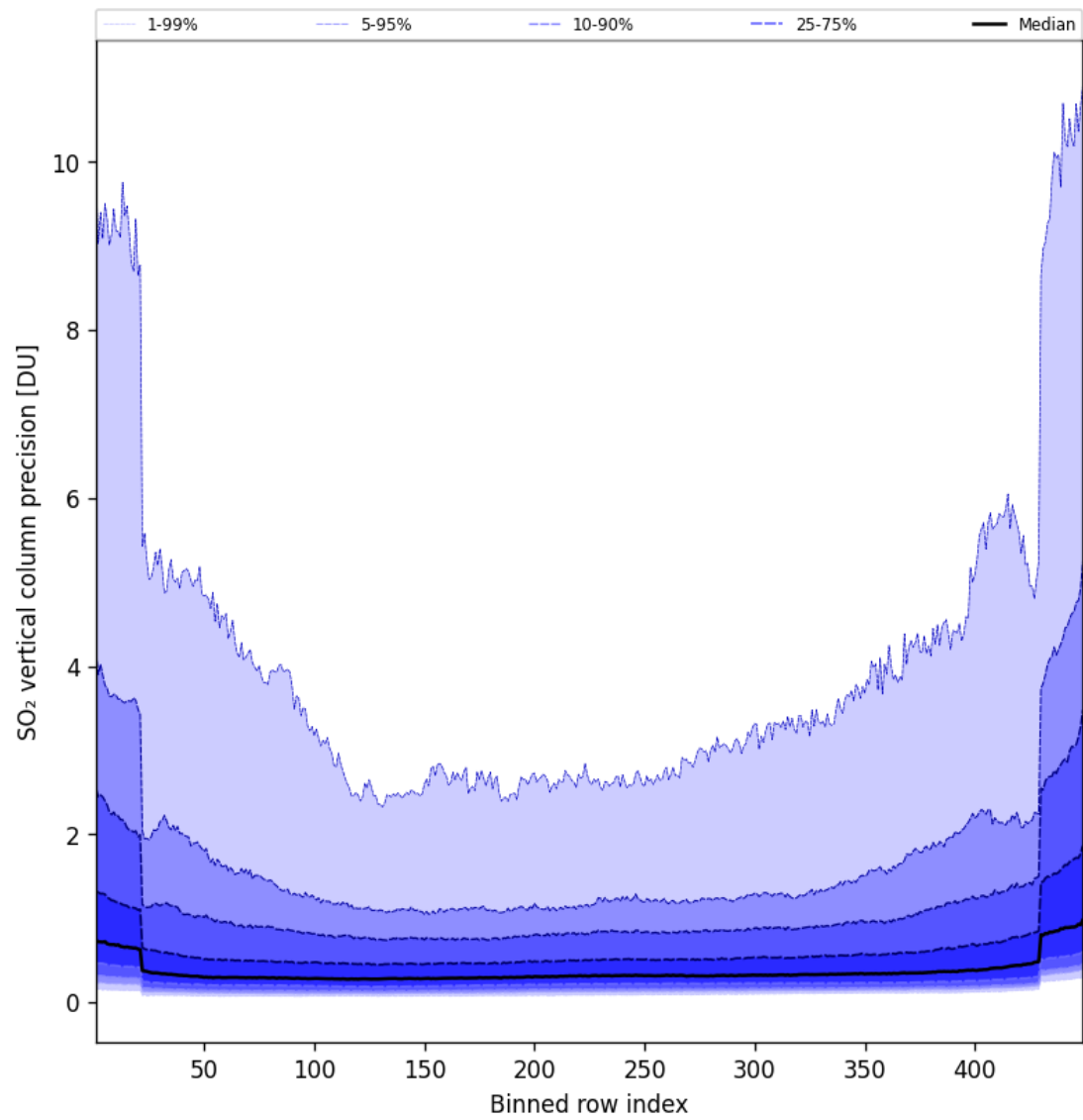
Figure 86: Along track statistics of “SO 2 vertical column precision” for 2025-10-17 to 2025-10-18
