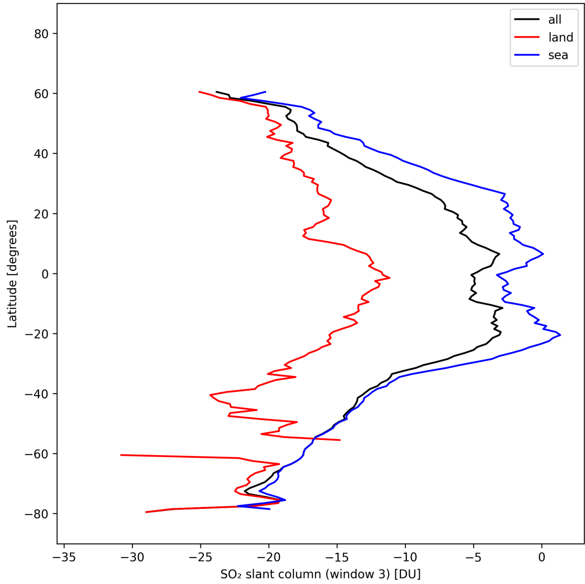
Figure 44: Zonal average of “SO 2 slant column (window 3)” for 2025-10-17 to 2025-10-18.
