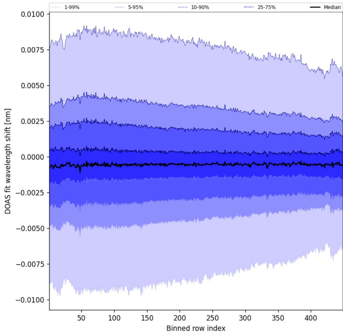
Figure 104: Along track statistics of “DOAS fit wavelength shift” for 2025-10-17 to 2025-10-18
