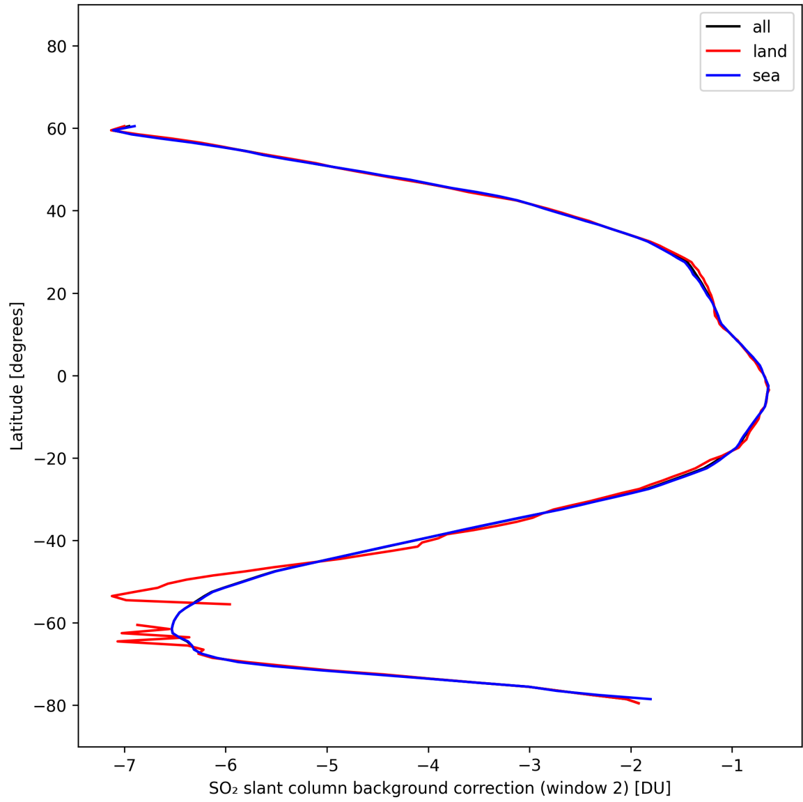
Figure 43: Zonal average of “SO 2 slant column background correction (window 2)” for 2025-10-17 to 2025-10-18.
