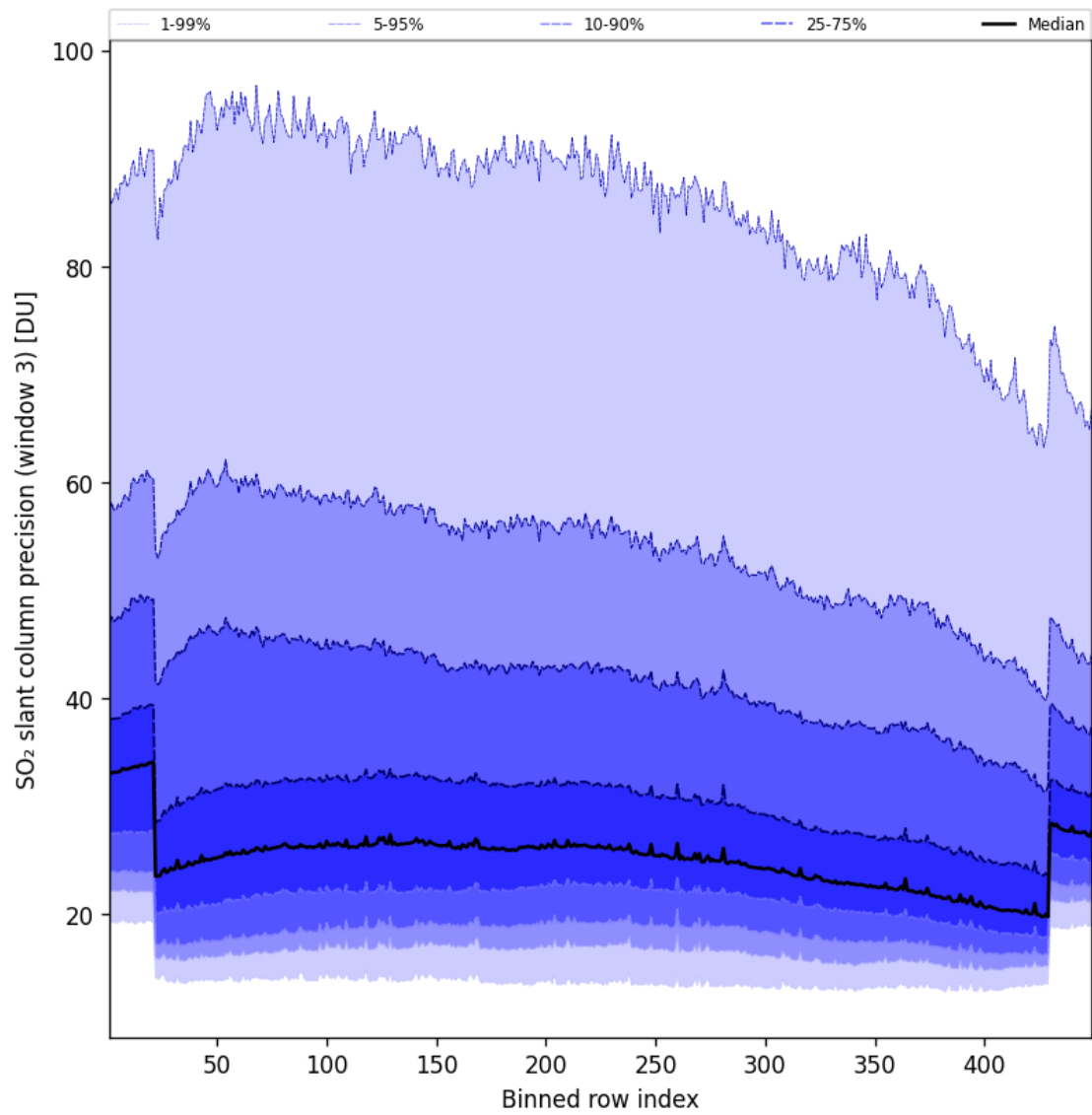
Figure 99: Along track statistics of “SO 2 slant column precision (window 3)” for 2025-10-17 to 2025-10-18
