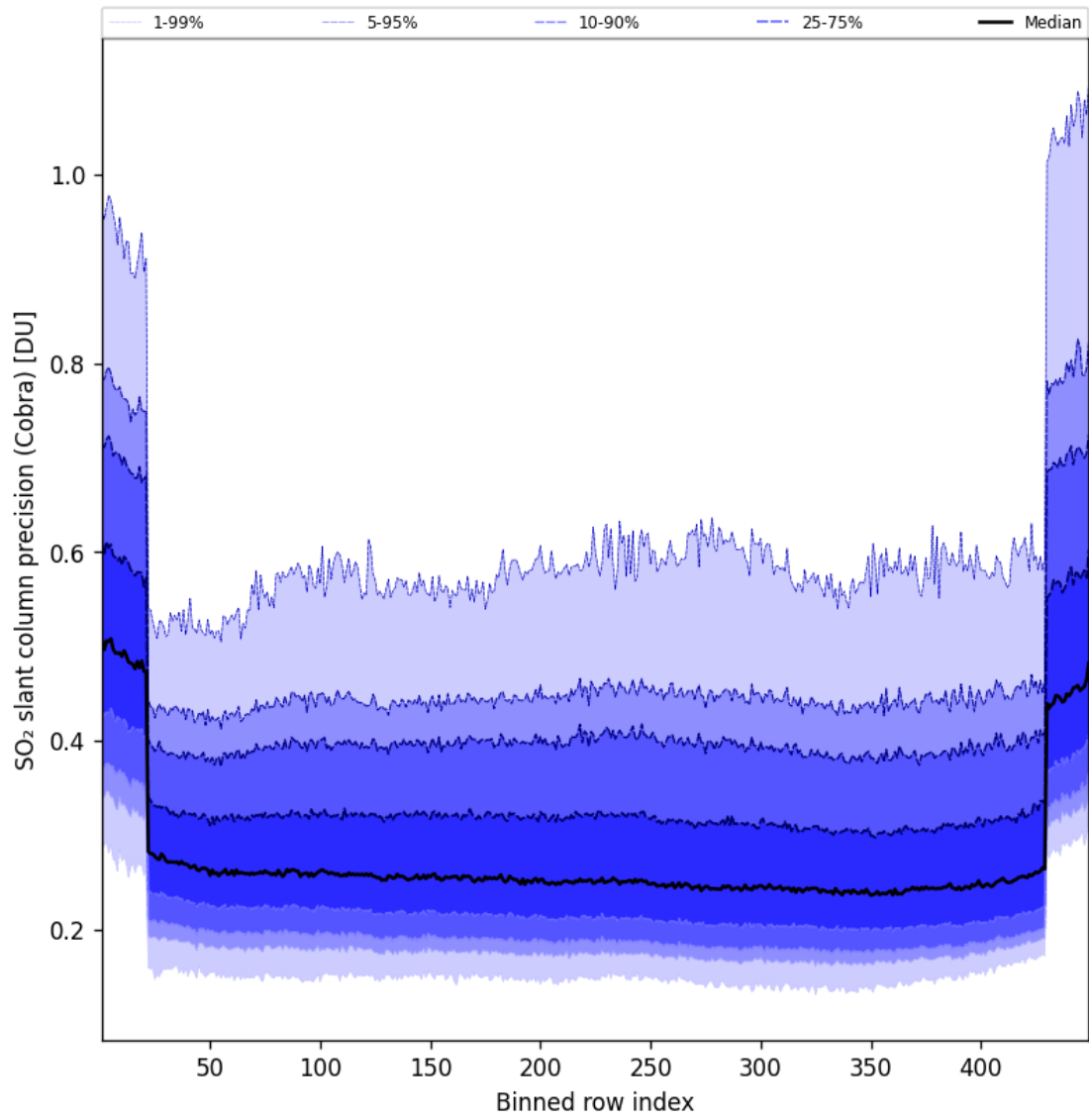
Figure 89: Along track statistics of “SO 2 slant column precision (Cobra)” for 2025-10-17 to 2025-10-18
