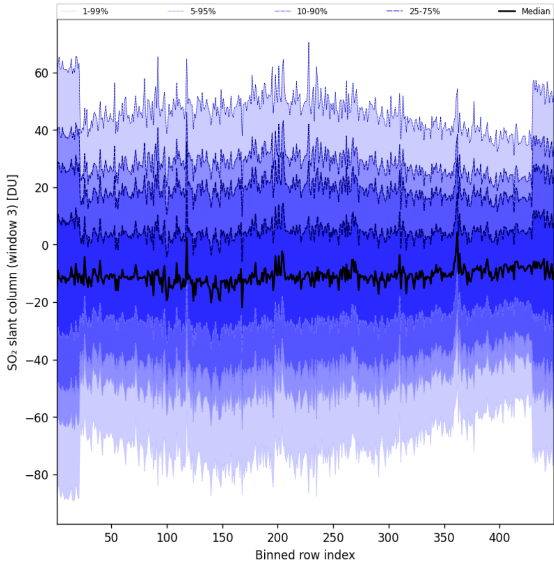
Figure 98: Along track statistics of “SO 2 slant column (window 3)” for 2025-10-17 to 2025-10-18
