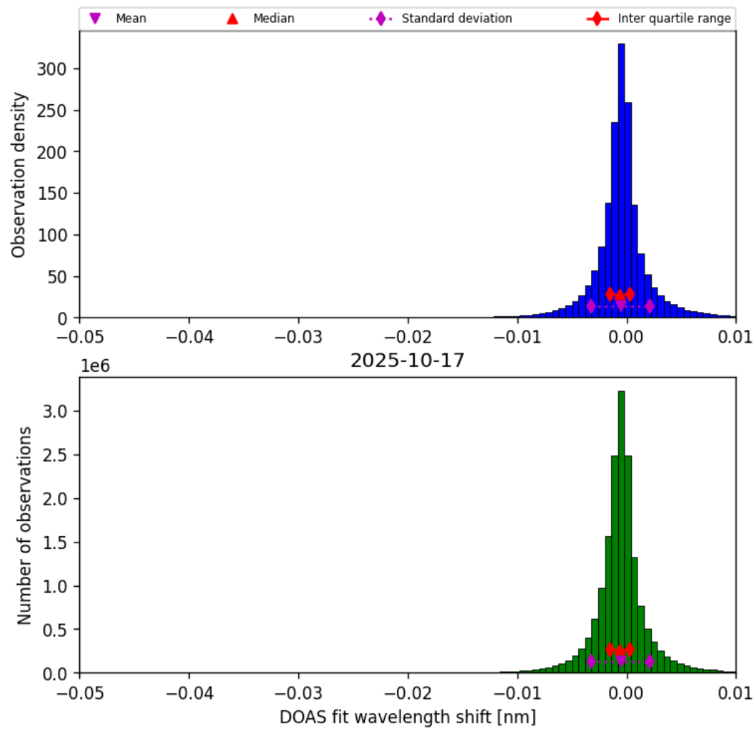
Figure 77: Histogram of “DOAS fit wavelength shift” for 2025-10-17 to 2025-10-18
