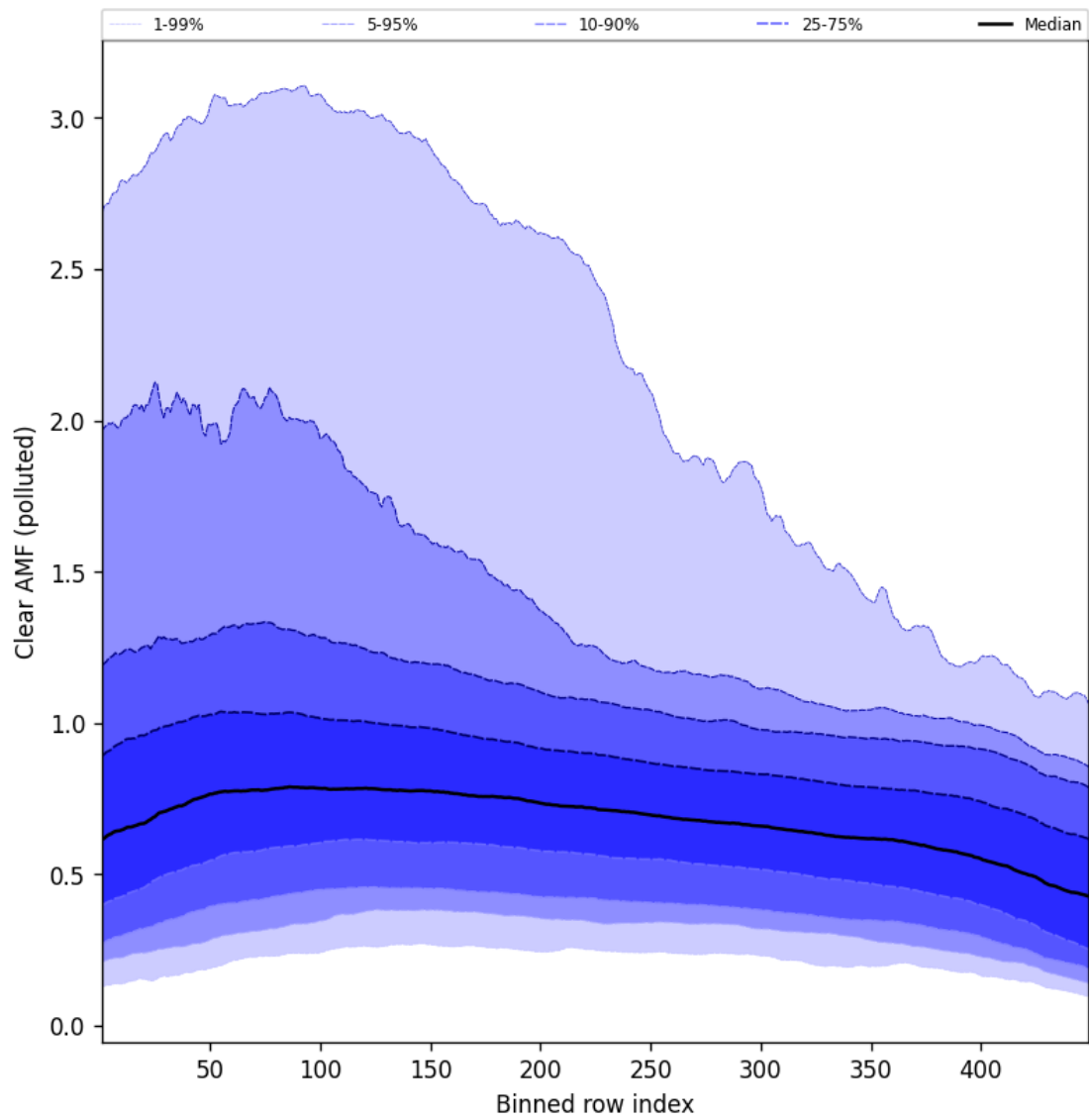
Figure 109: Along track statistics of “Clear AMF (polluted)” for 2025-10-17 to 2025-10-18
