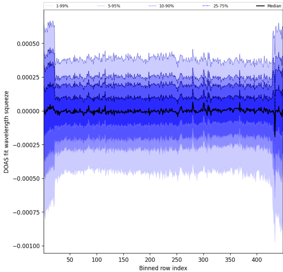
Figure 105: Along track statistics of “DOAS fit wavelength squeeze” for 2025-10-17 to 2025-10-18
