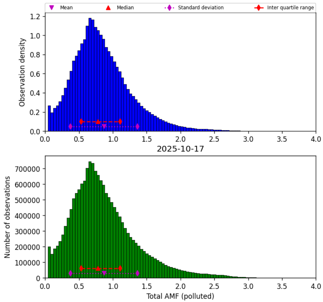
Figure 80: Histogram of “Total AMF (polluted)” for 2025-10-17 to 2025-10-18
