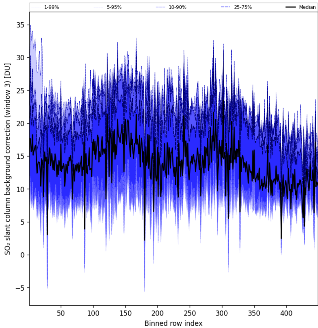
Figure 101: Along track statistics of “SO 2 slant column background correction (window 3)” for 2025-10-17 to 2025-10-18
