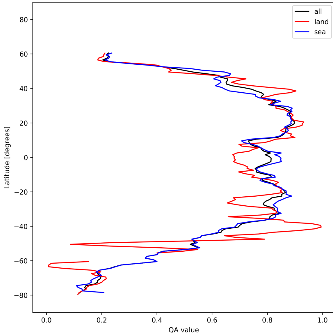
Figure 30: Zonal average of “QA value” for 2025-10-17 to 2025-10-18.
