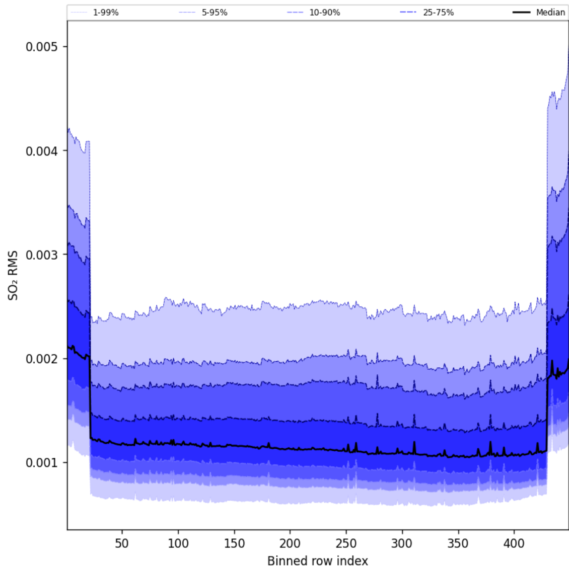
Figure 106: Along track statistics of “SO 2 RMS” for 2025-10-17 to 2025-10-18
