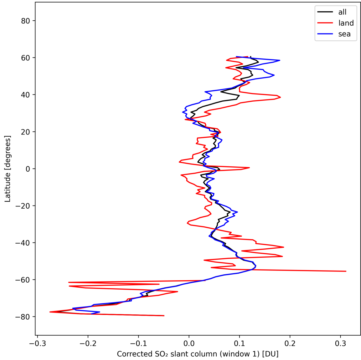
Figure 38: Zonal average of “Corrected SO 2 slant column (window 1)” for 2025-10-17 to 2025-10-18.
