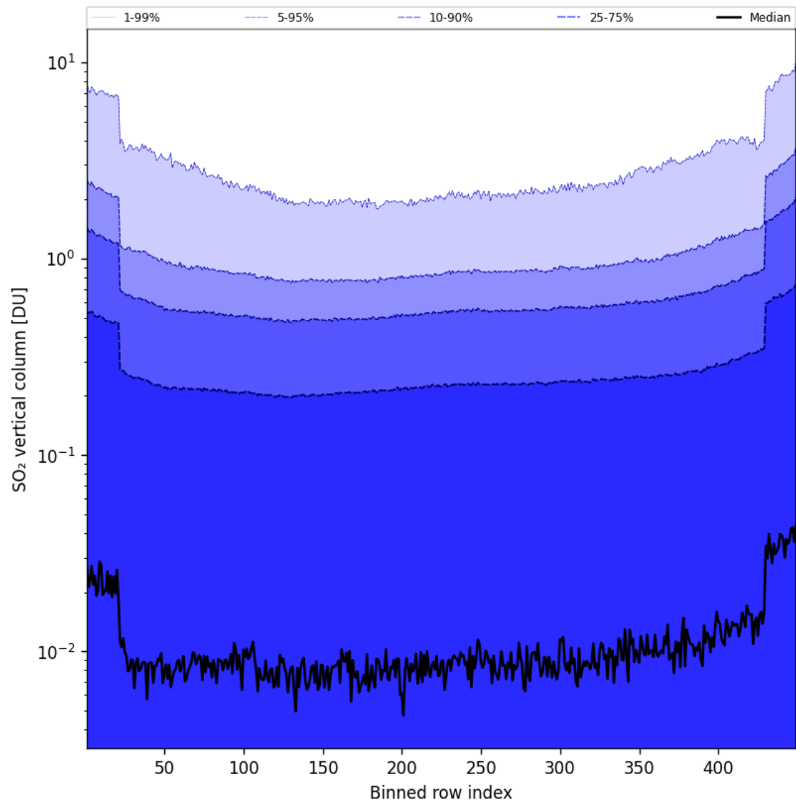
Figure 85: Along track statistics of “SO 2 vertical column” for 2025-10-17 to 2025-10-18
