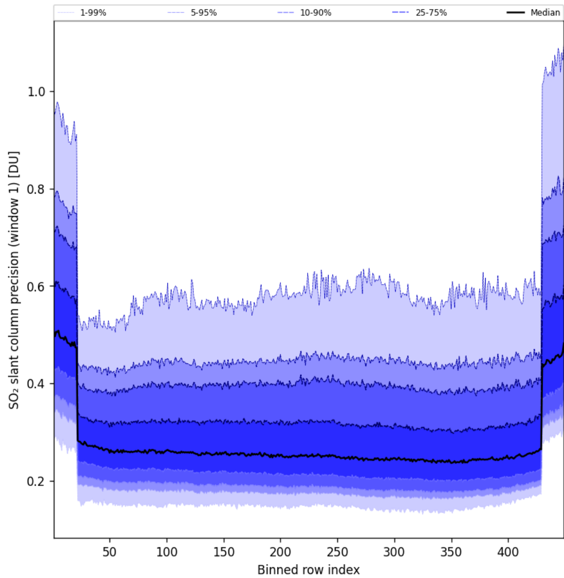
Figure 91: Along track statistics of “SO 2 slant column precision (window 1)” for 2025-10-17 to 2025-10-18
