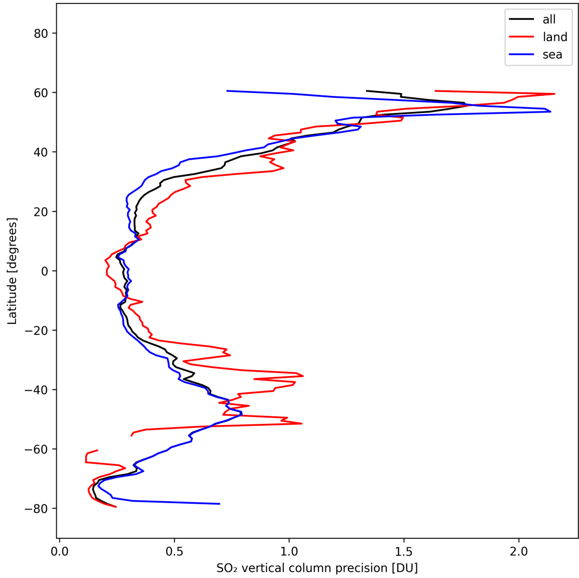
Figure 32: Zonal average of “SO 2 vertical column precision” for 2025-10-17 to 2025-10-18.
