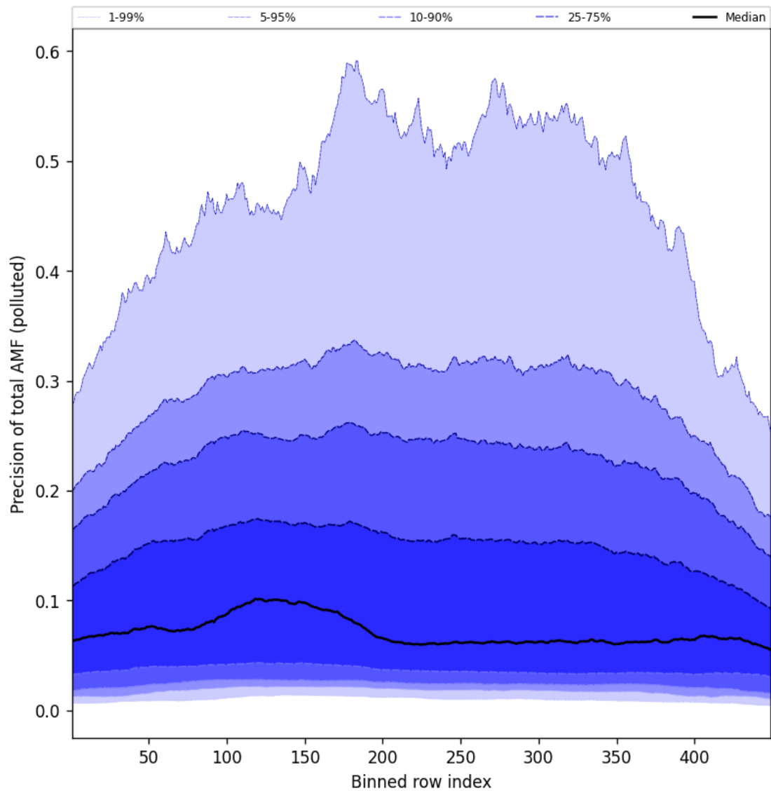
Figure 108: Along track statistics of “Precision of total AMF (polluted)” for 2025-10-17 to 2025-10-18
