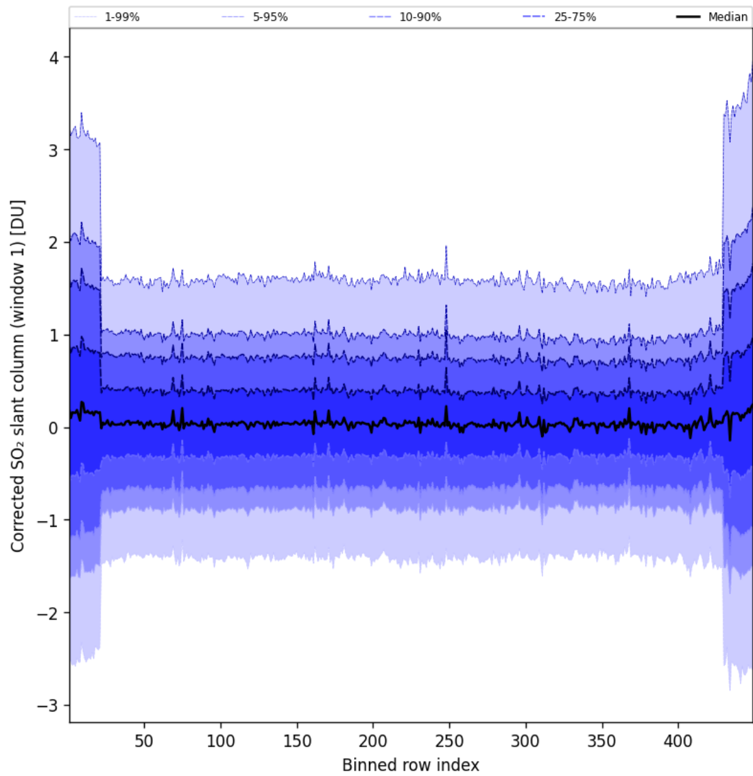
Figure 92: Along track statistics of “Corrected SO 2 slant column (window 1)” for 2025-10-17 to 2025-10-18
