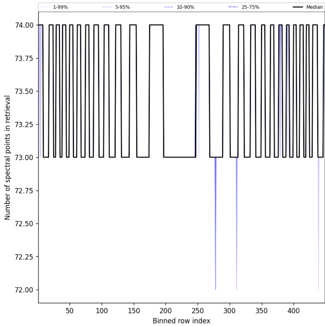
Figure 110: Along track statistics of “Number of spectral points in retrieval” for 2025-10-17 to 2025-10-18
