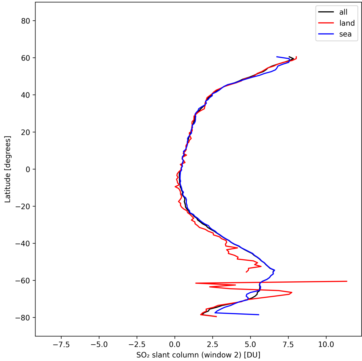
Figure 40: Zonal average of “SO 2 slant column (window 2)” for 2025-10-17 to 2025-10-18.
