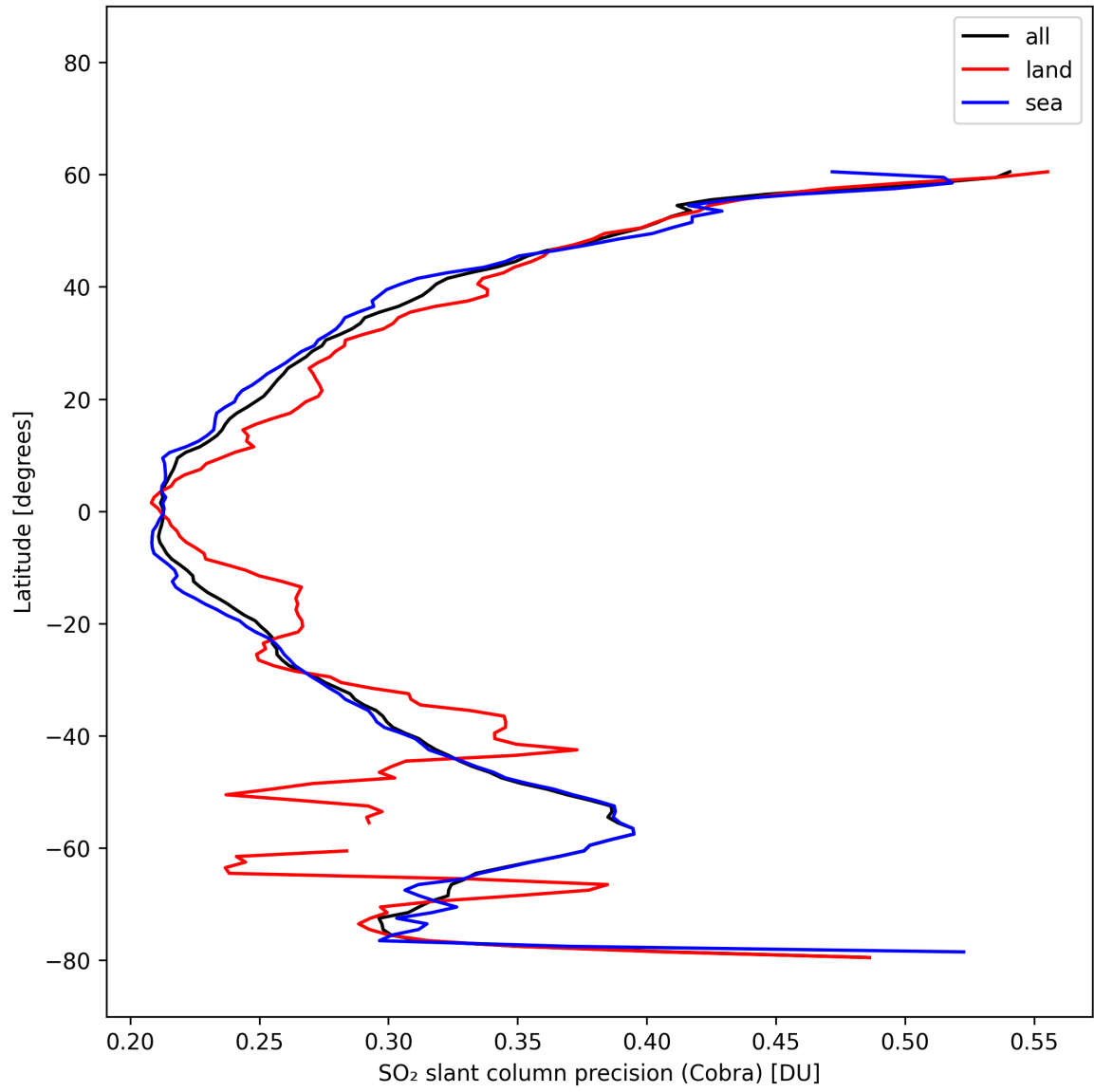
Figure 35: Zonal average of “SO 2 slant column precision (Cobra)” for 2025-10-17 to 2025-10-18.
