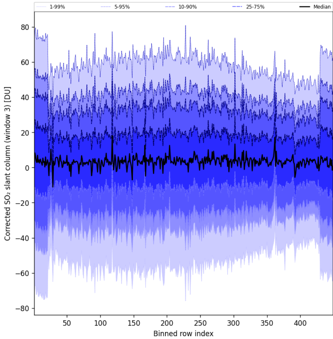
Figure 100: Along track statistics of “Corrected SO 2 slant column (window 3)” for 2025-10-17 to 2025-10-18
