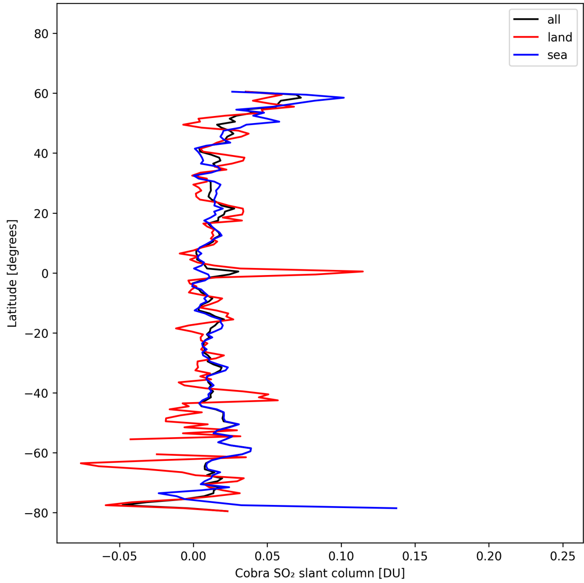
Figure 34: Zonal average of “Cobra SO 2 slant column” for 2025-10-17 to 2025-10-18.
