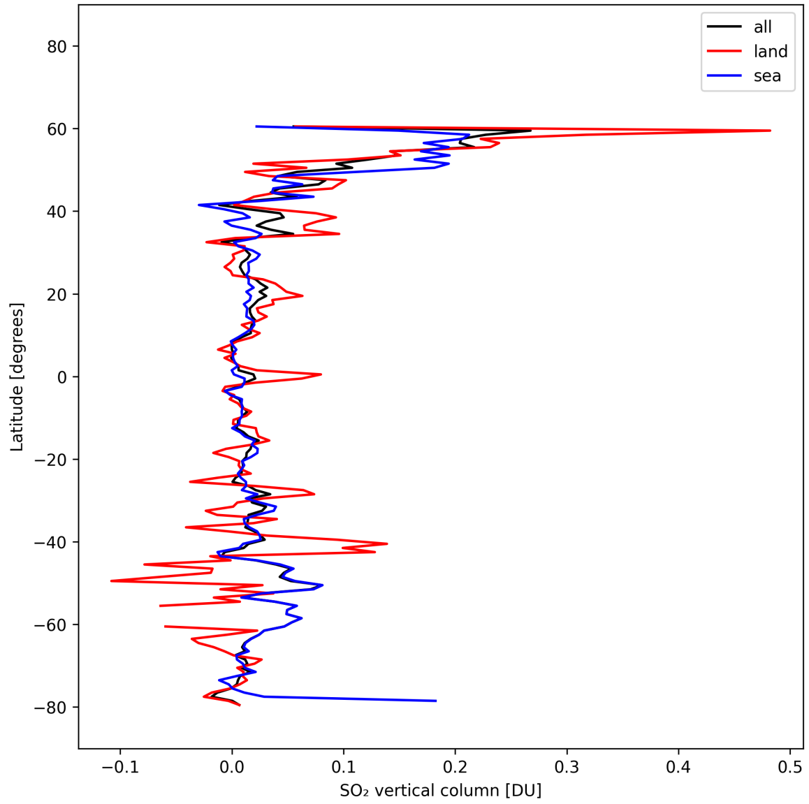
Figure 31: Zonal average of “SO 2 vertical column” for 2025-10-17 to 2025-10-18.
