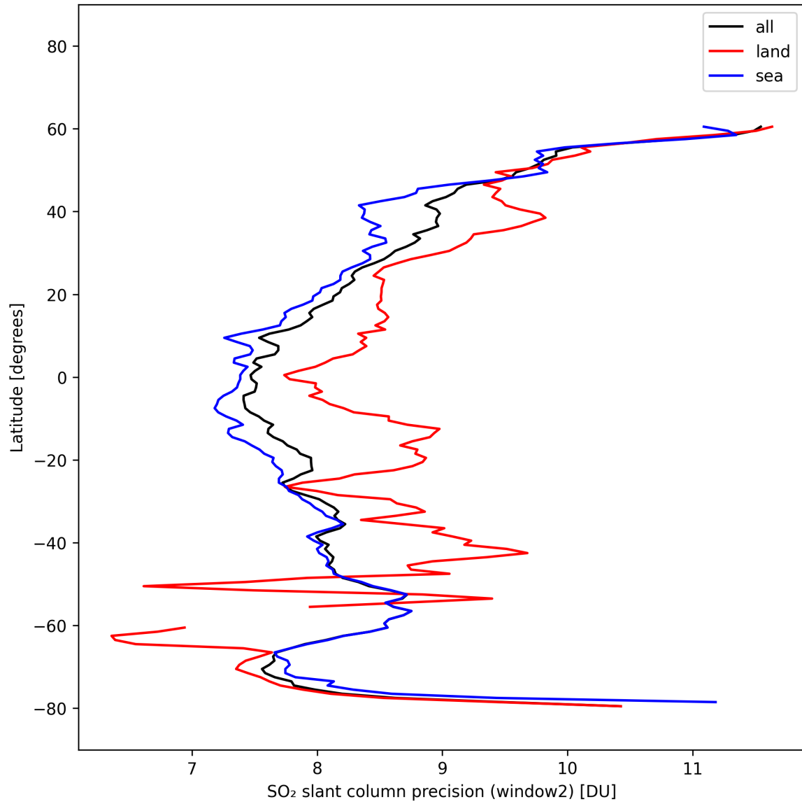
Figure 41: Zonal average of “SO 2 slant column precision (window2)” for 2025-10-17 to 2025-10-18.
