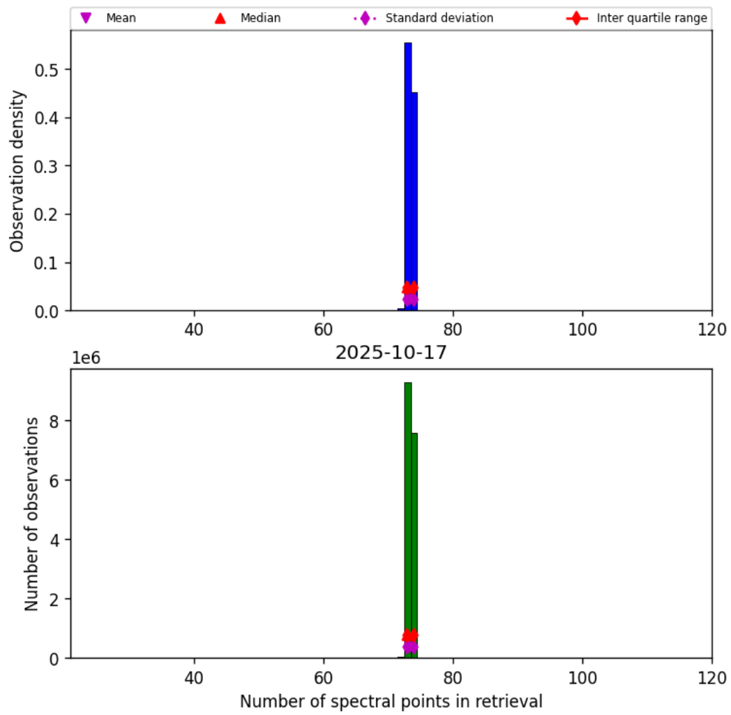
Figure 83: Histogram of “Number of spectral points in retrieval” for 2025-10-17 to 2025-10-18
