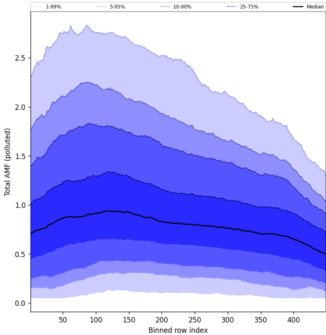
Figure 107: Along track statistics of “Total AMF (polluted)” for 2025-10-17 to 2025-10-18
