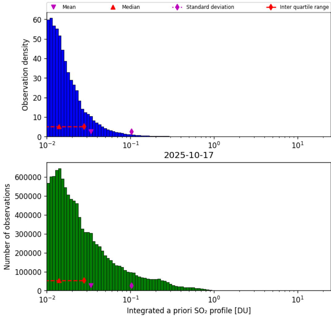
Figure 76: Histogram of “Integrated a priori SO 2 profile” for 2025-10-17 to 2025-10-18
