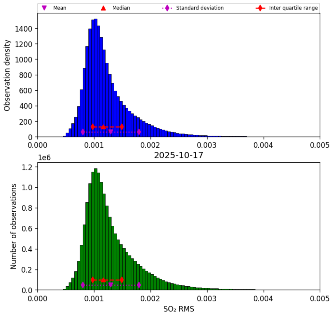
Figure 79: Histogram of "SO 2 RMS" for 2025-10-17 to 2025-10-18
