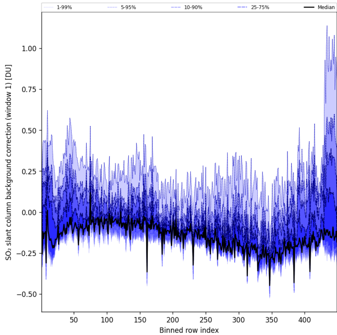
Figure 93: Along track statistics of “SO 2 slant column background correction (window 1)” for 2025-10-17 to 2025-10-18
