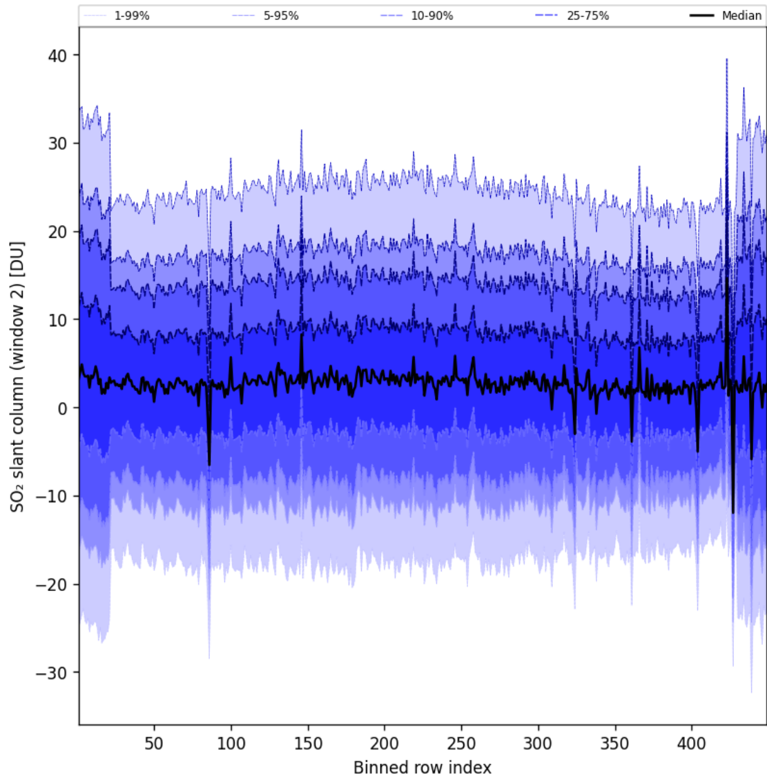
Figure 94: Along track statistics of “SO 2 slant column (window 2)” for 2025-10-17 to 2025-10-18
