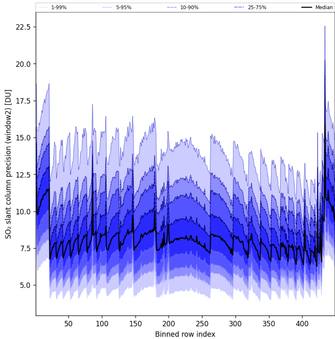
Figure 95: Along track statistics of “SO 2 slant column precision (window2)” for 2025-10-17 to 2025-10-18
