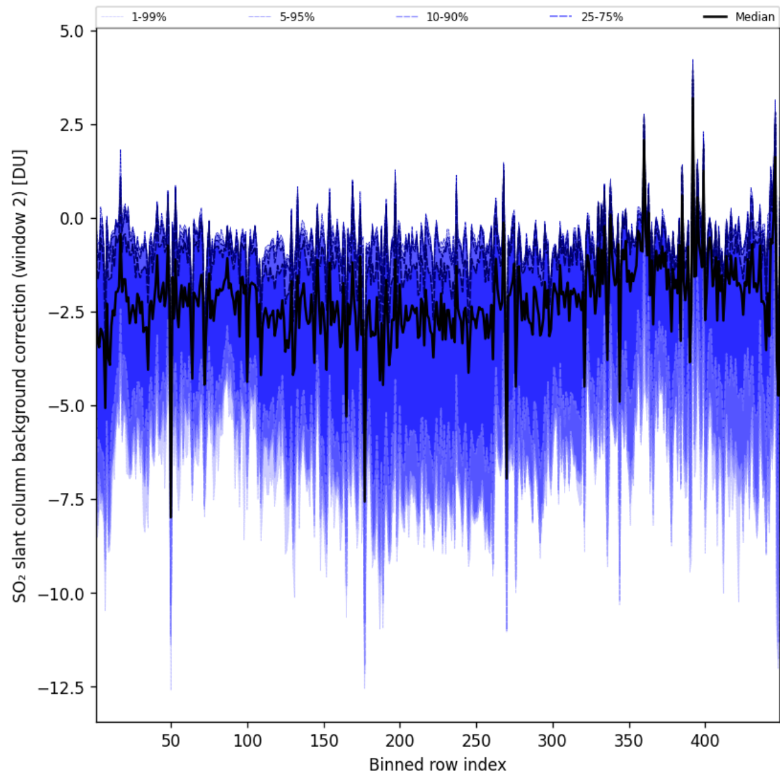
Figure 97: Along track statistics of “SO 2 slant column background correction (window 2)” for 2025-10-17 to 2025-10-18
