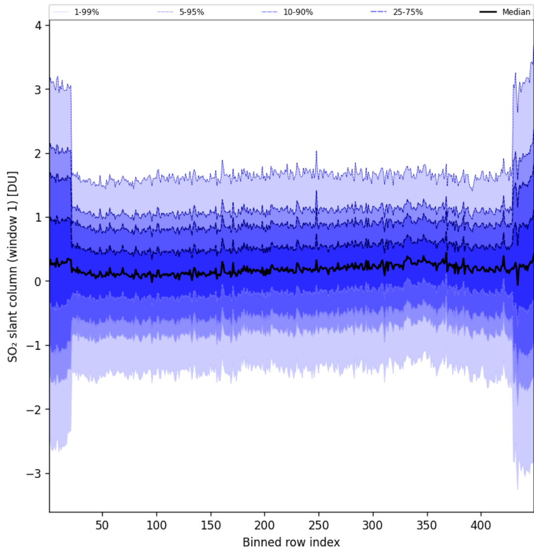
Figure 90: Along track statistics of “SO 2 slant column (window 1)” for 2025-10-17 to 2025-10-18
