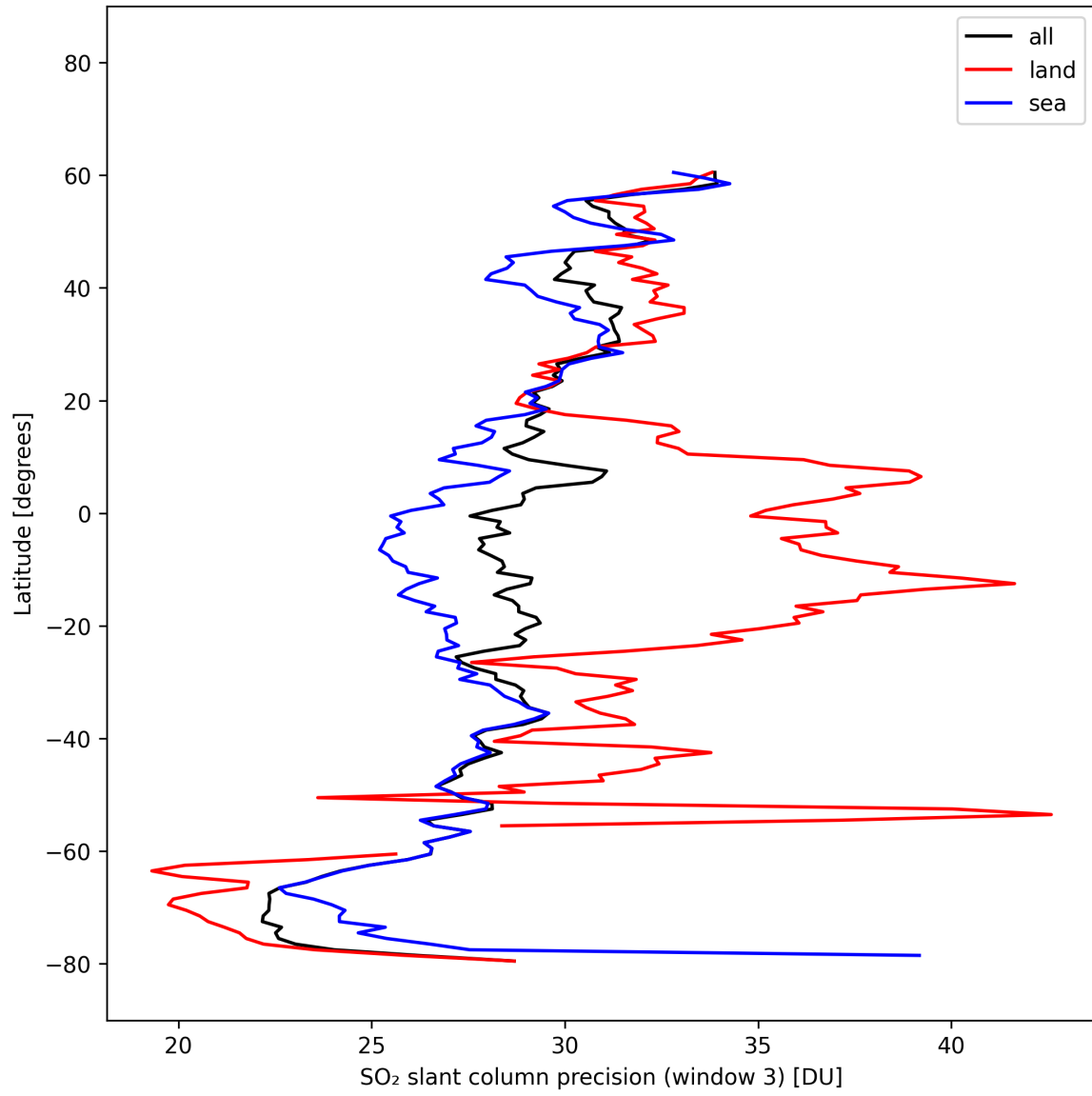
Figure 45: Zonal average of “SO 2 slant column precision (window 3)” for 2025-10-17 to 2025-10-18.
