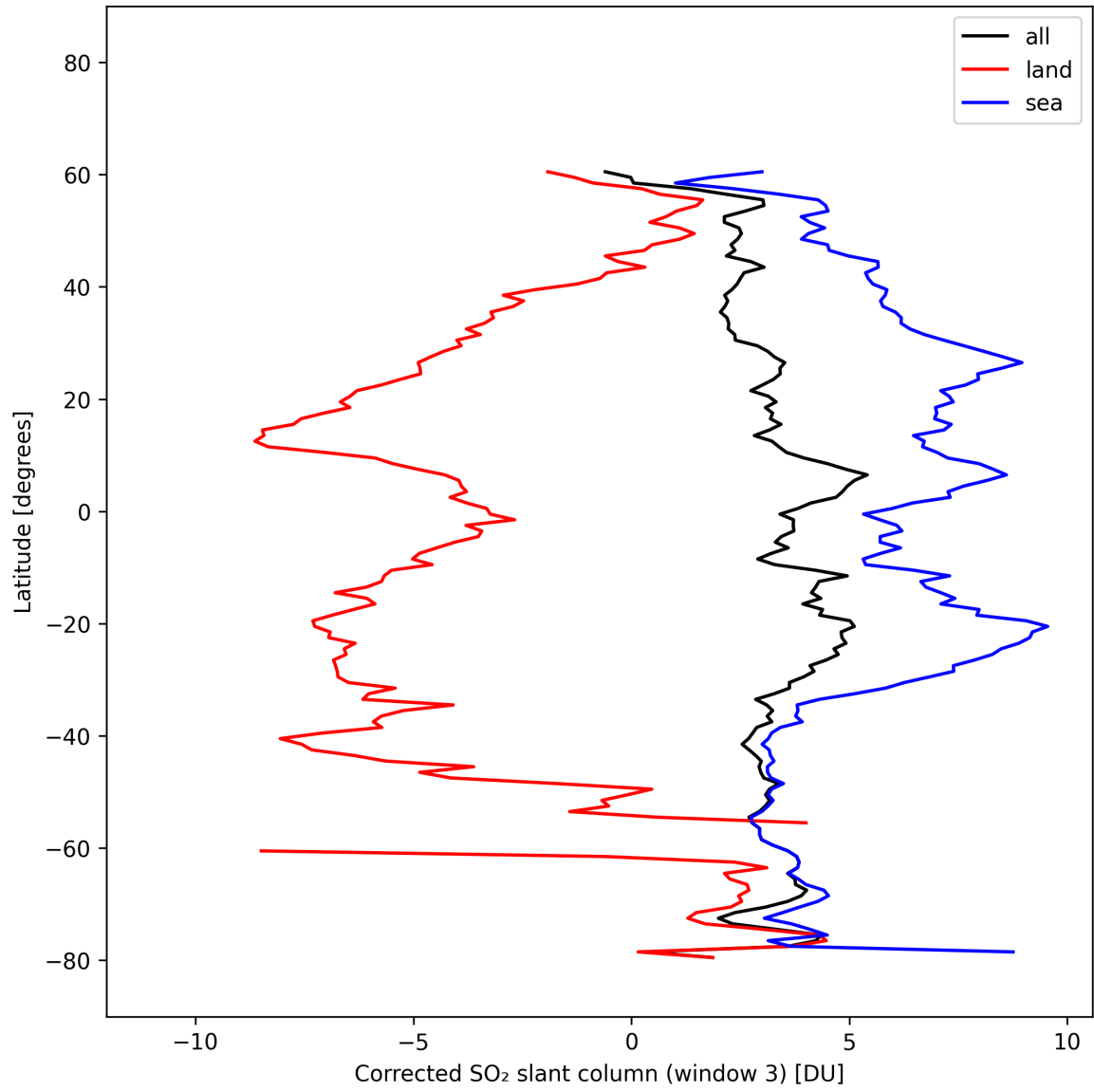
Figure 46: Zonal average of “Corrected SO 2 slant column (window 3)” for 2025-10-17 to 2025-10-18.
