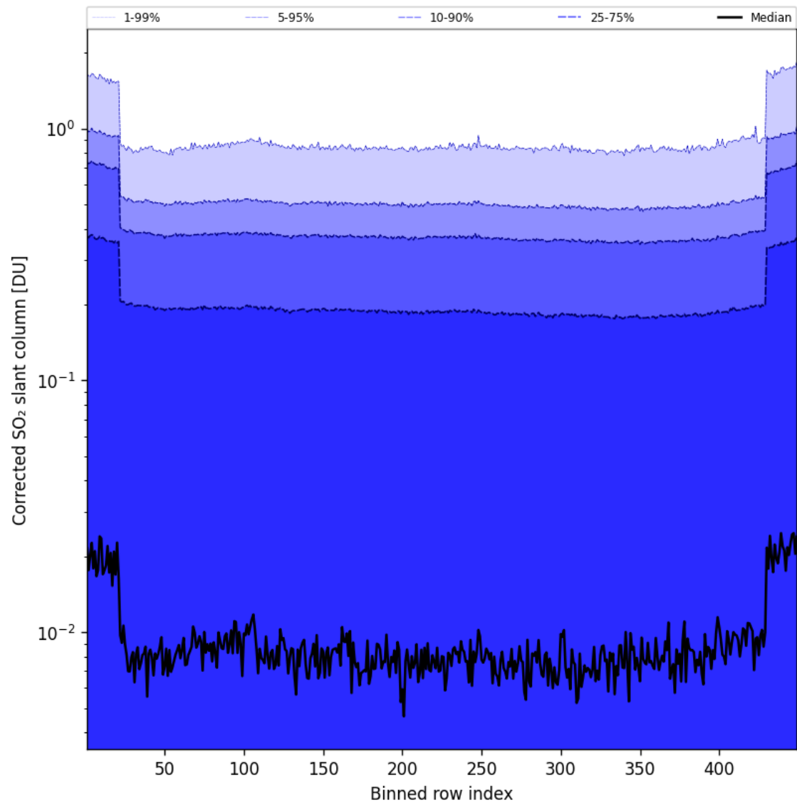
Figure 87: Along track statistics of "Corrected SO 2 slant column" for 2025-10-17 to 2025-10-18
