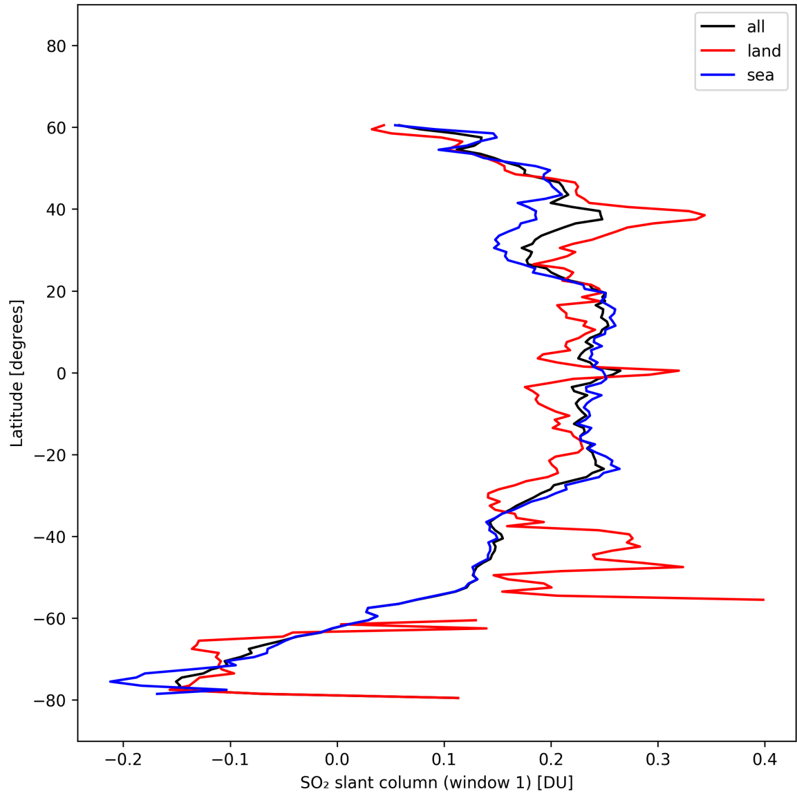
Figure 36: Zonal average of “SO 2 slant column (window 1)” for 2025-10-17 to 2025-10-18.
