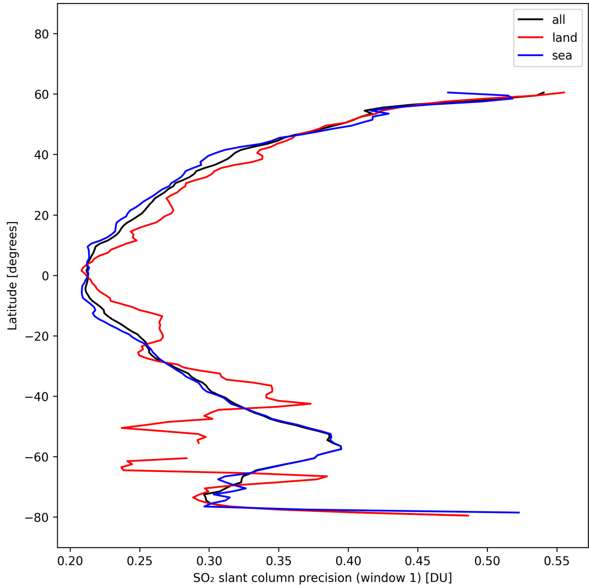
Figure 37: Zonal average of “SO 2 slant column precision (window 1)” for 2025-10-17 to 2025-10-18.
