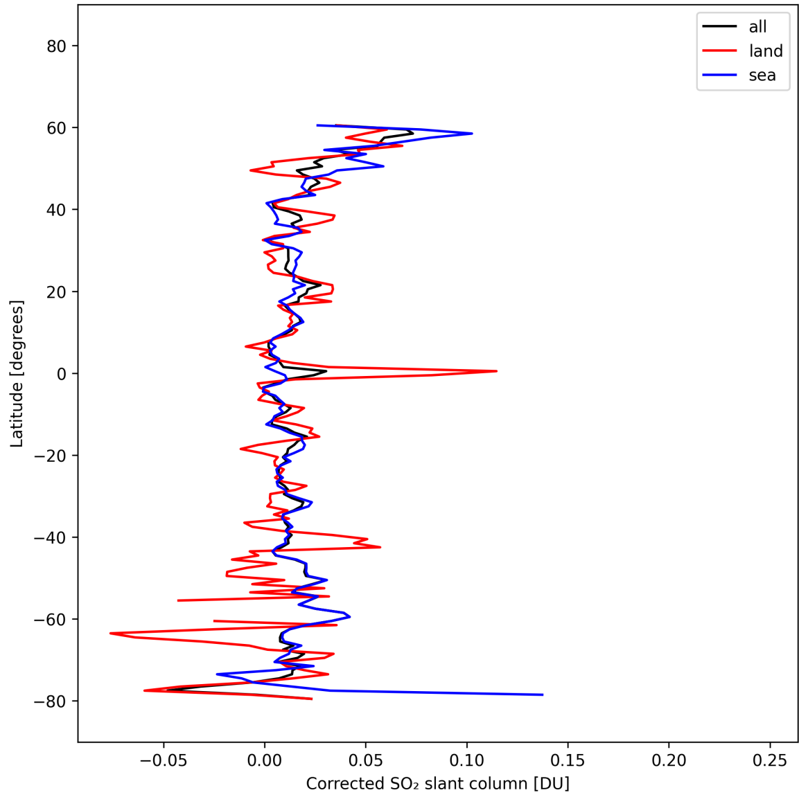
Figure 33: Zonal average of “Corrected SO 2 slant column” for 2025-10-17 to 2025-10-18.
