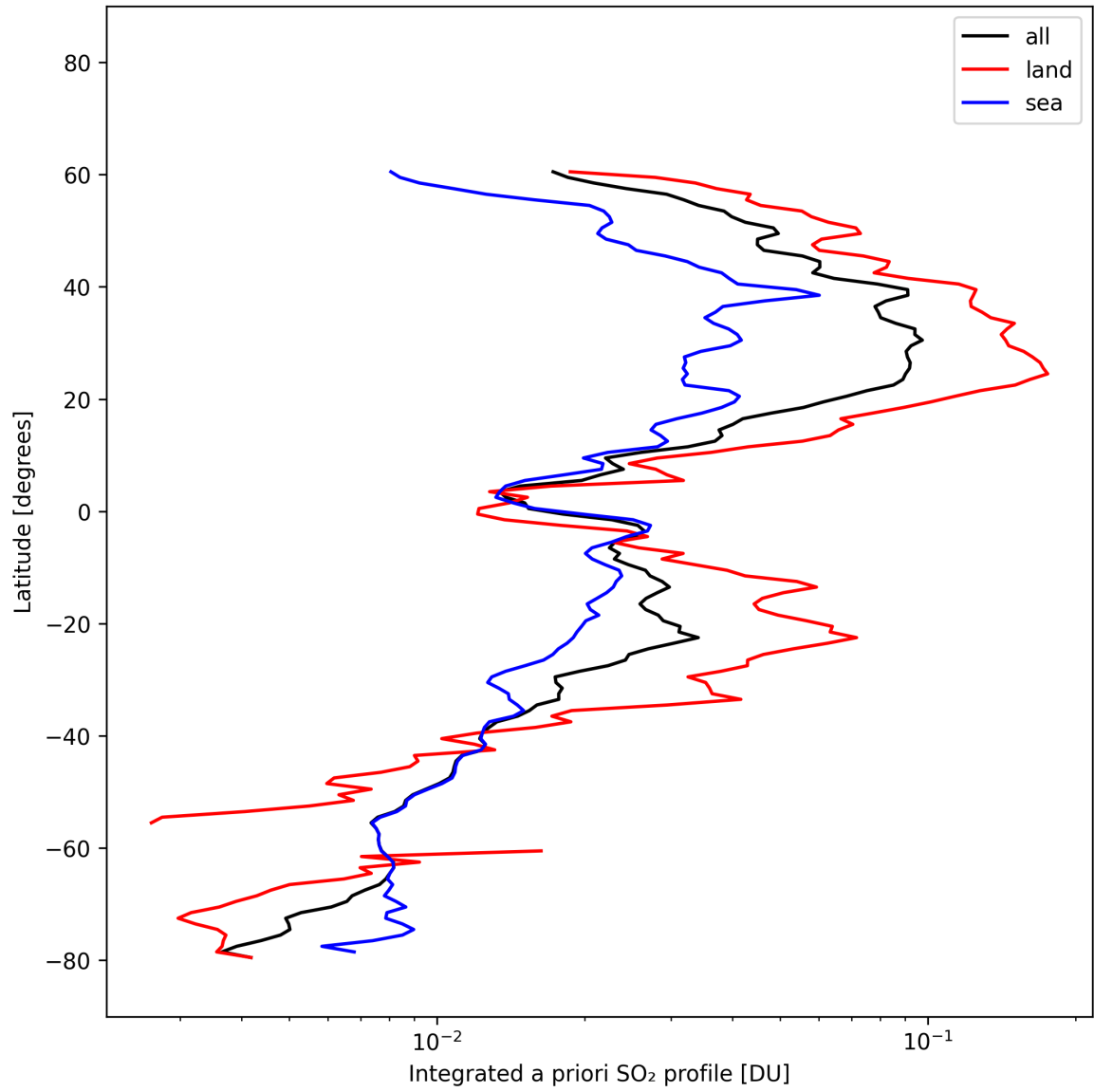
Figure 49: Zonal average of “Integrated a priori SO 2 profile” for 2025-10-17 to 2025-10-18.
