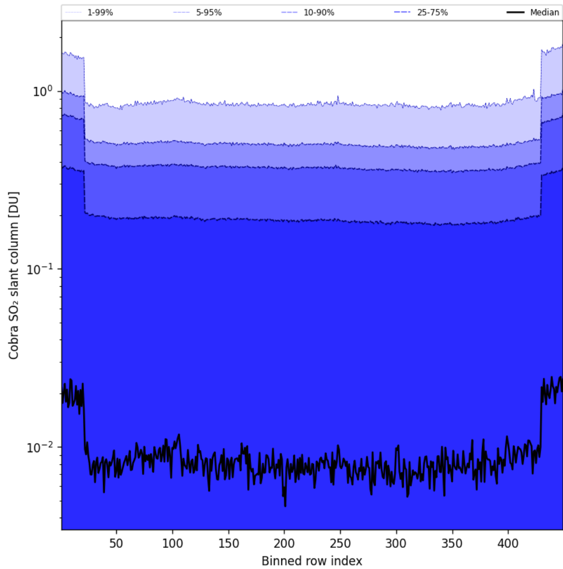
Figure 88: Along track statistics of “Cobra SO 2 slant column” for 2025-10-17 to 2025-10-18
