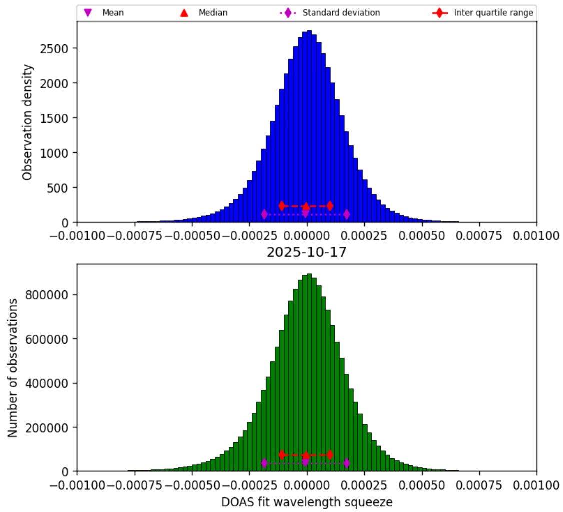
Figure 78: Histogram of “DOAS fit wavelength squeeze” for 2025-10-17 to 2025-10-18
