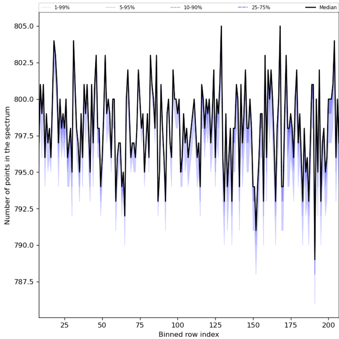
Figure 37: Along track statistics of “Number of points in the spectrum” for 2023-06-30 to 2023-07-02
