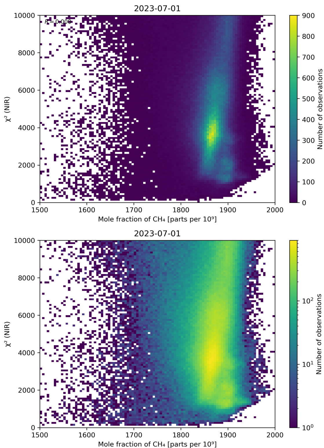
Figure 70: Scatter density plot of “Mole fraction of CH 4 ” against “ \chi^2 (NIR)” for 2023-06-30 to 2023-07-02.
