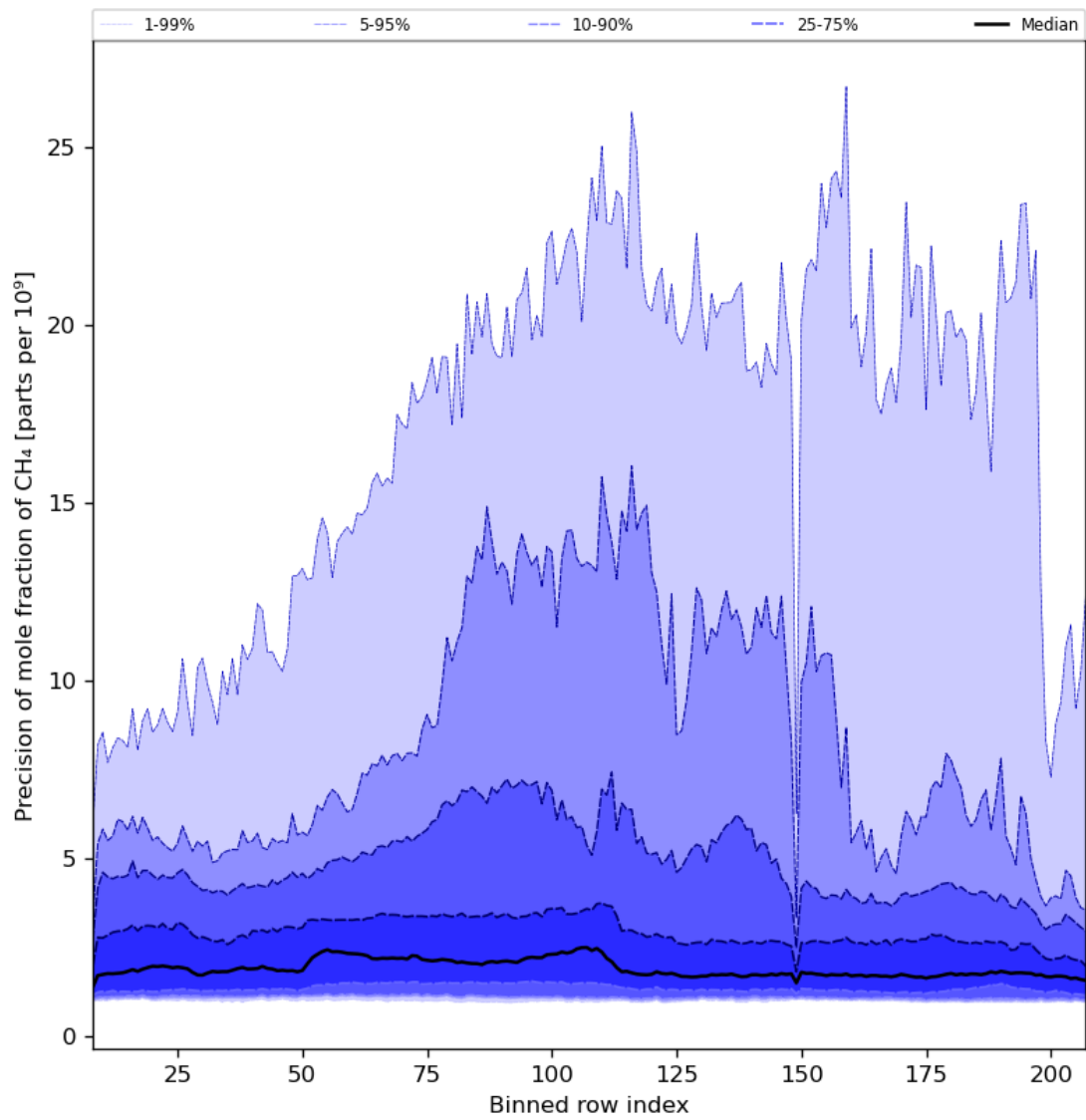
Figure 35: Along track statistics of “Precision of mole fraction of CH 4 ” for 2023-06-30 to 2023-07-02
