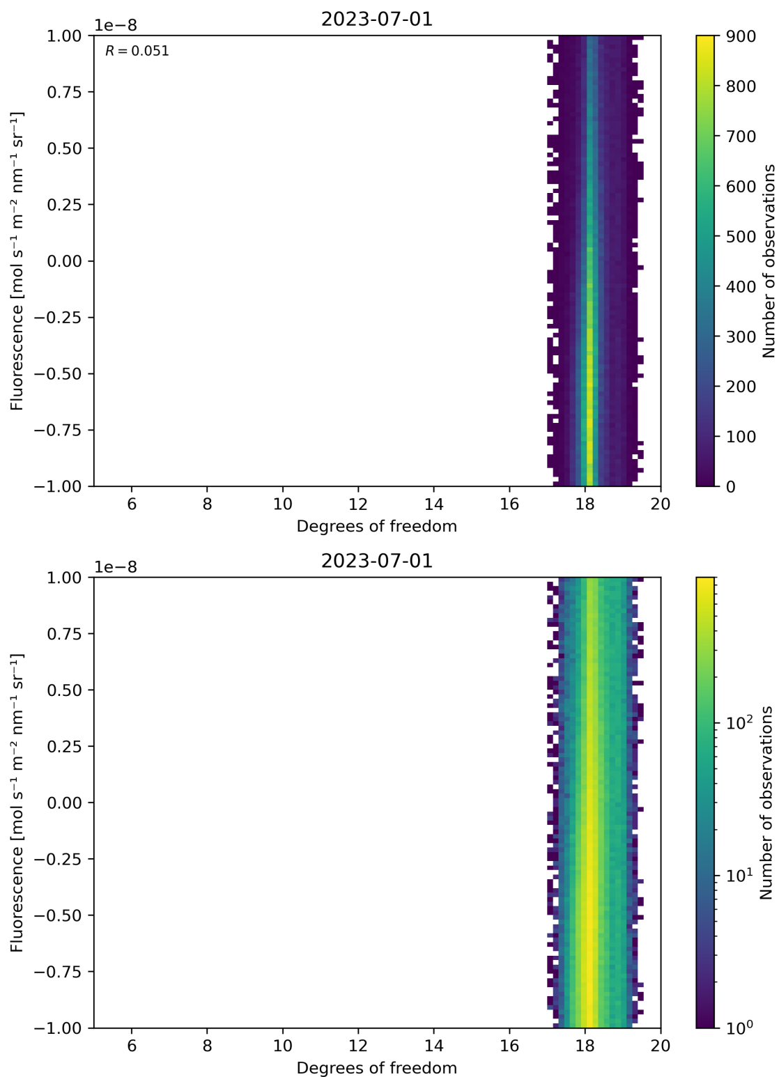
Figure 51: Scatter density plot of “Degrees of freedom” against “Fluorescence” for 2023-06-30 to 2023-07-02.
