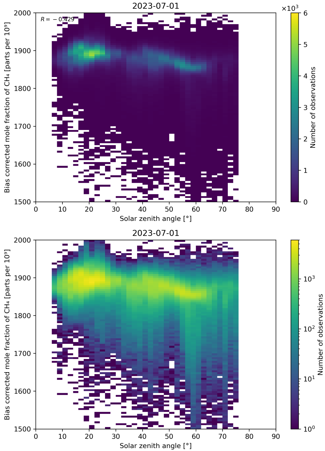
Figure 100: Scatter density plot of “Solar zenith angle” against “Bias corrected mole fraction of CH 4 ” for 2023-06-30 to 2023-07-02.
