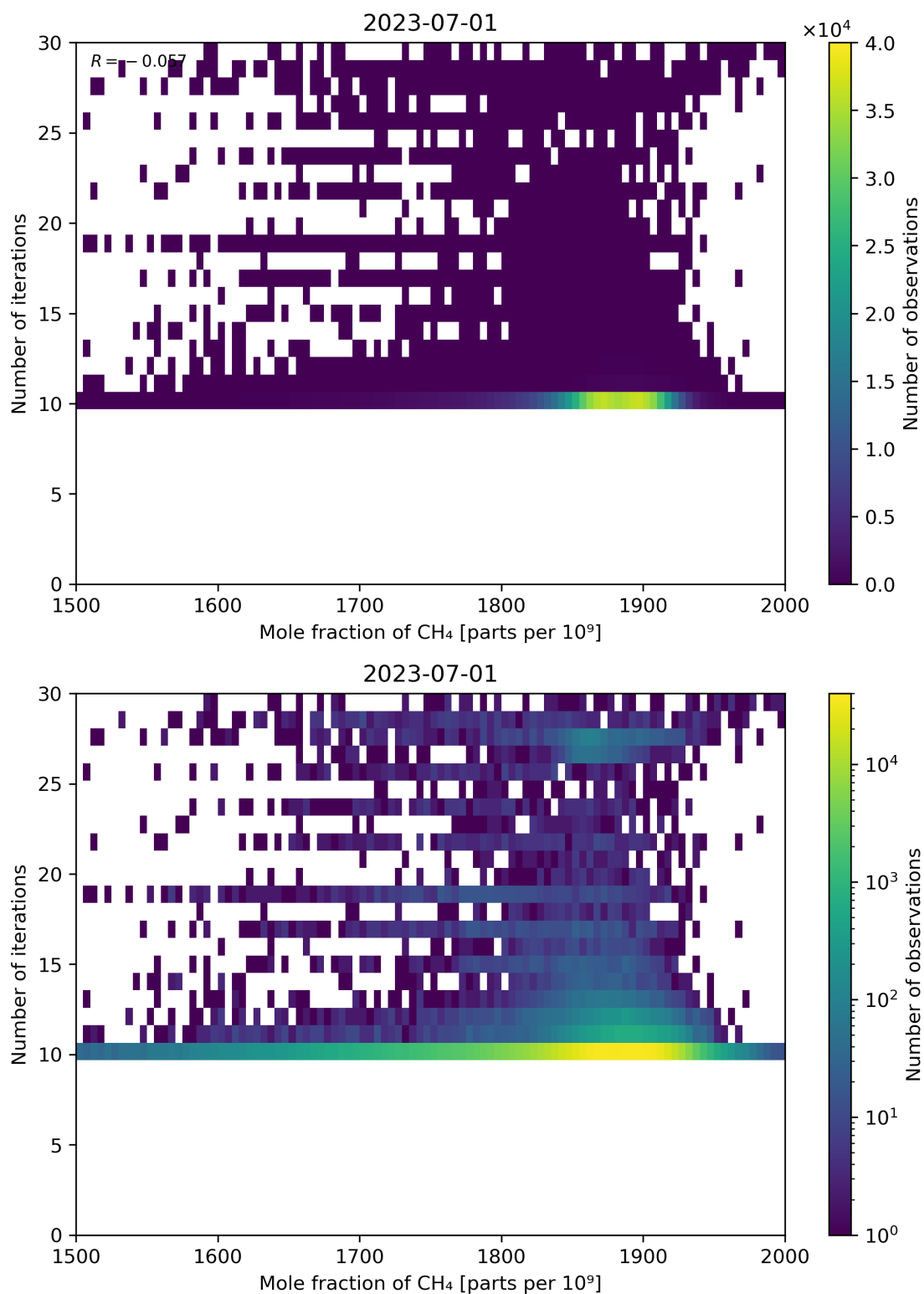
Figure 76: Scatter density plot of “Mole fraction of CH 4 ” against “Number of iterations” for 2023-06-30 to 2023-07-02.
