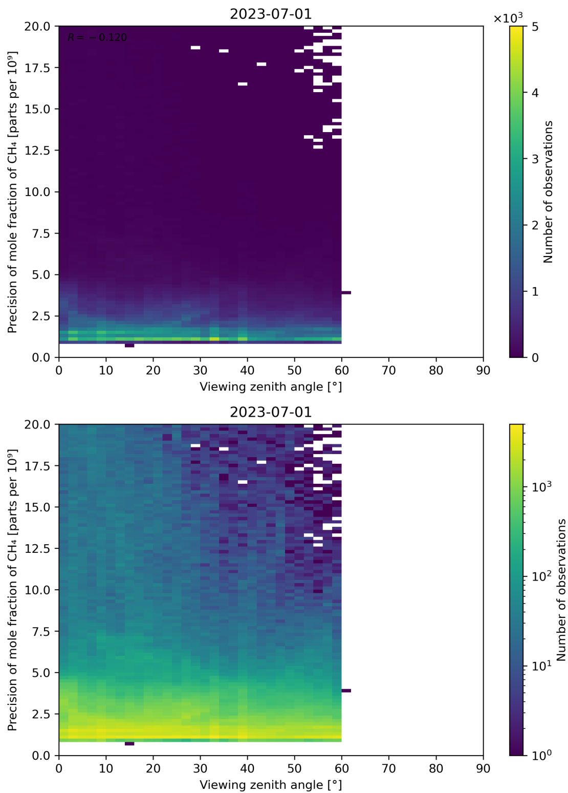
Figure 112: Scatter density plot of “Viewing zenith angle” against “Precision of mole fraction of CH 4 ” for 2023-06-30 to 2023-07-02.
