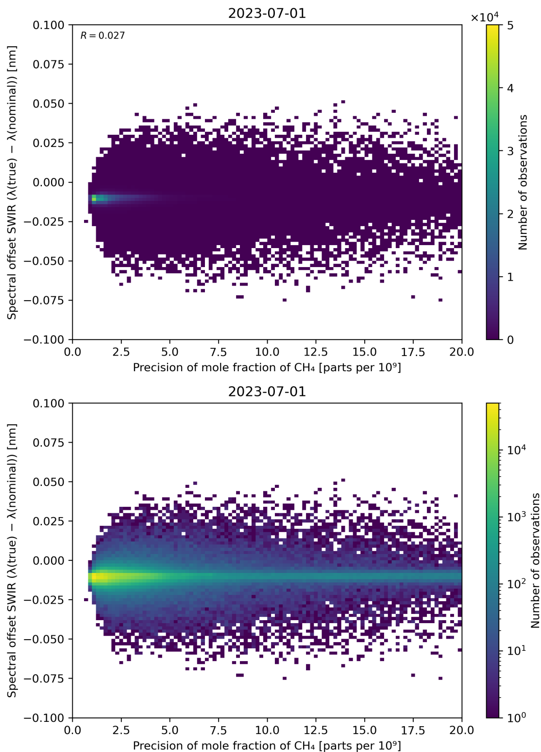
Figure 85: Scatter density plot of “Precision of mole fraction of CH 4 ” against “Spectral offset SWIR ( \lambda(\text{true}) - \lambda(\text{nominal}) )” for 2023-06-30 to 2023-07-02.
