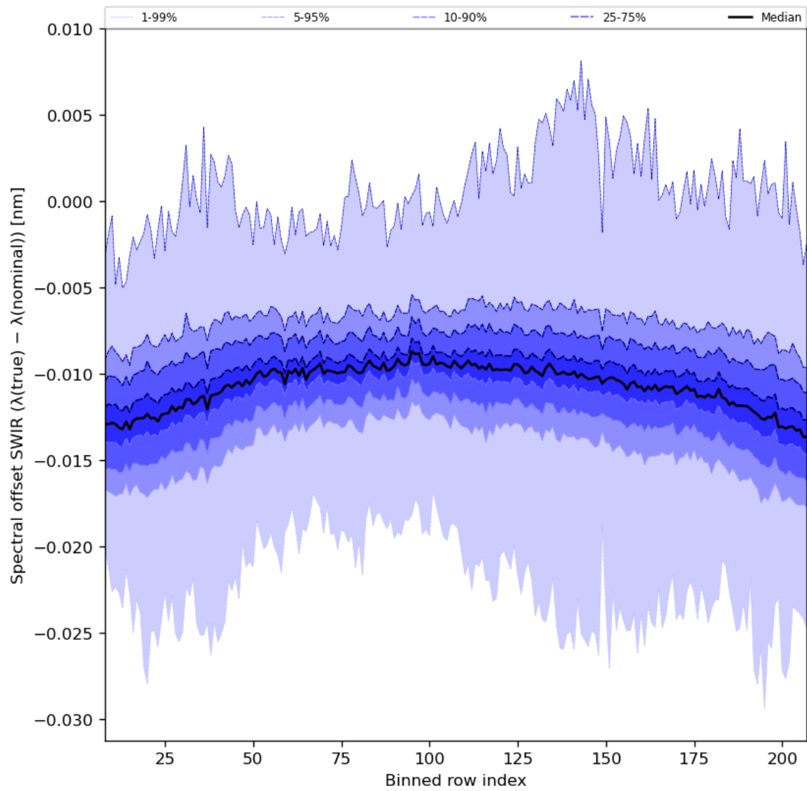
Figure 38: Along track statistics of “Spectral offset SWIR ( \lambda(\text{true}) - \lambda(\text{nominal}) )” for 2023-06-30 to 2023-07-02
