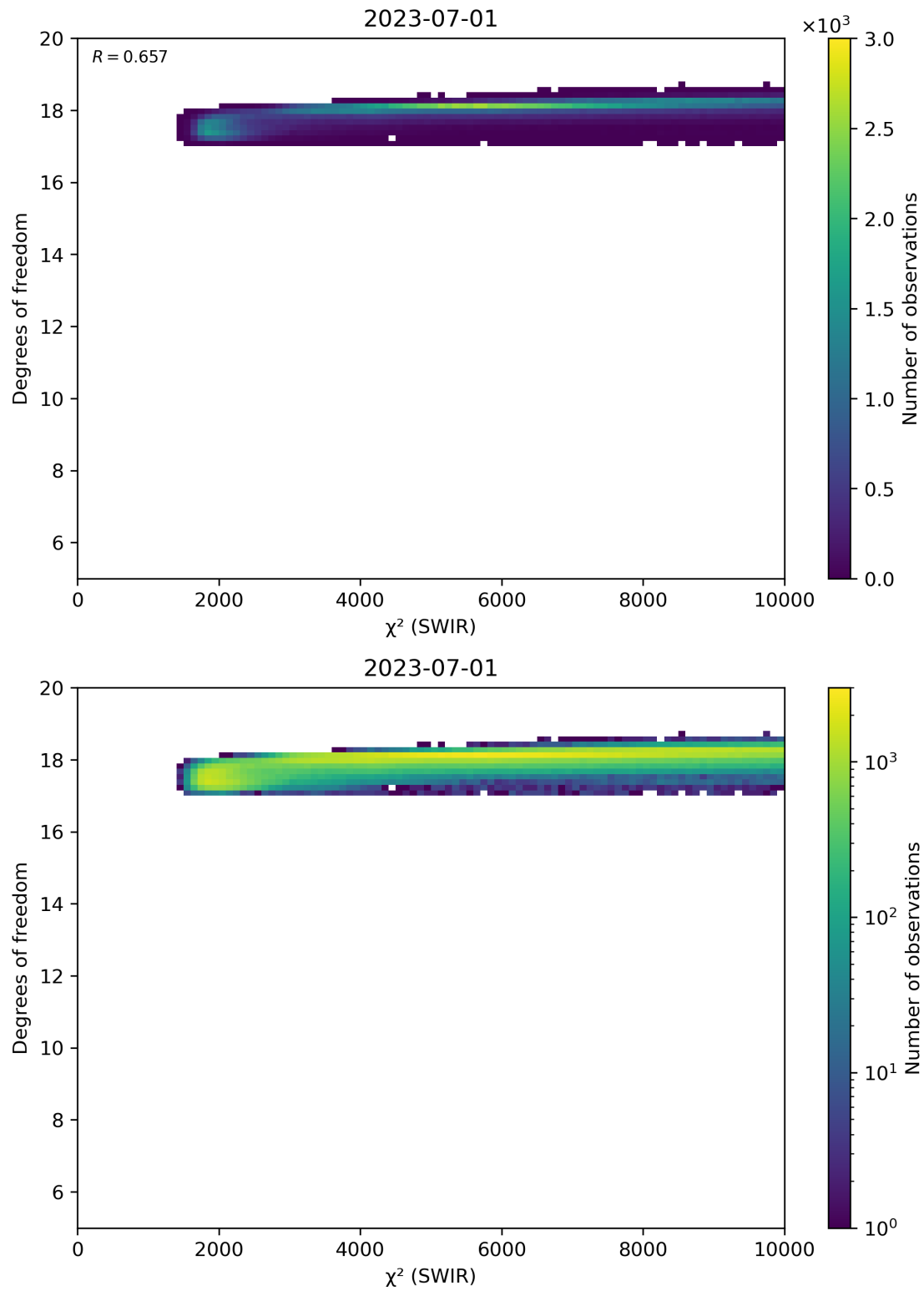
Figure 48: Scatter density plot of “ \chi^2 (SWIR)” against “Degrees of freedom” for 2023-06-30 to 2023-07-02.
