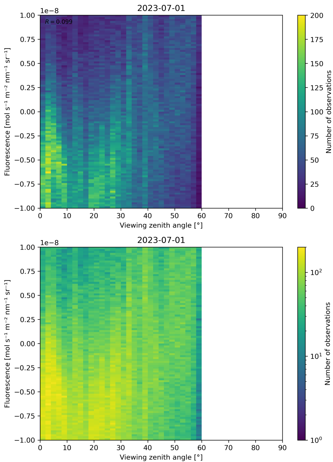
Figure 108: Scatter density plot of “Viewing zenith angle” against “Fluorescence” for 2023-06-30 to 2023-07-02.
