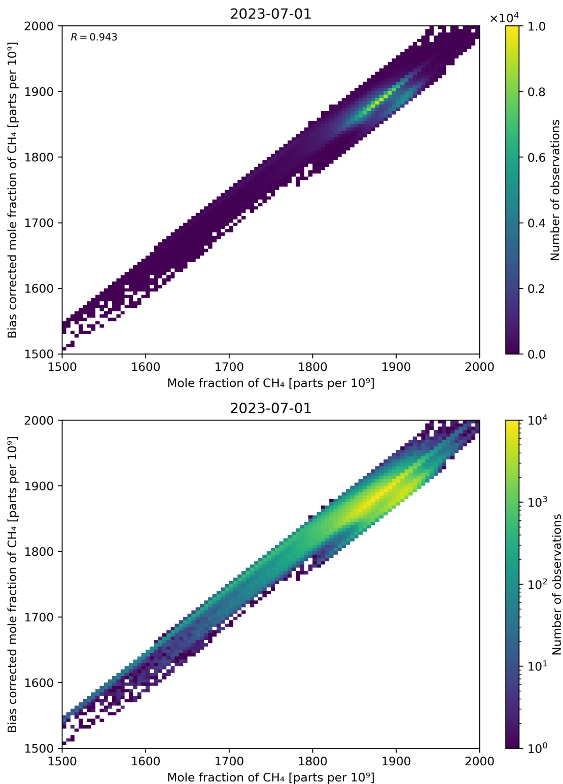
Figure 74: Scatter density plot of “Mole fraction of CH 4 ” against “Bias corrected mole fraction of CH 4 ” for 2023-06-30 to 2023-07-02.
