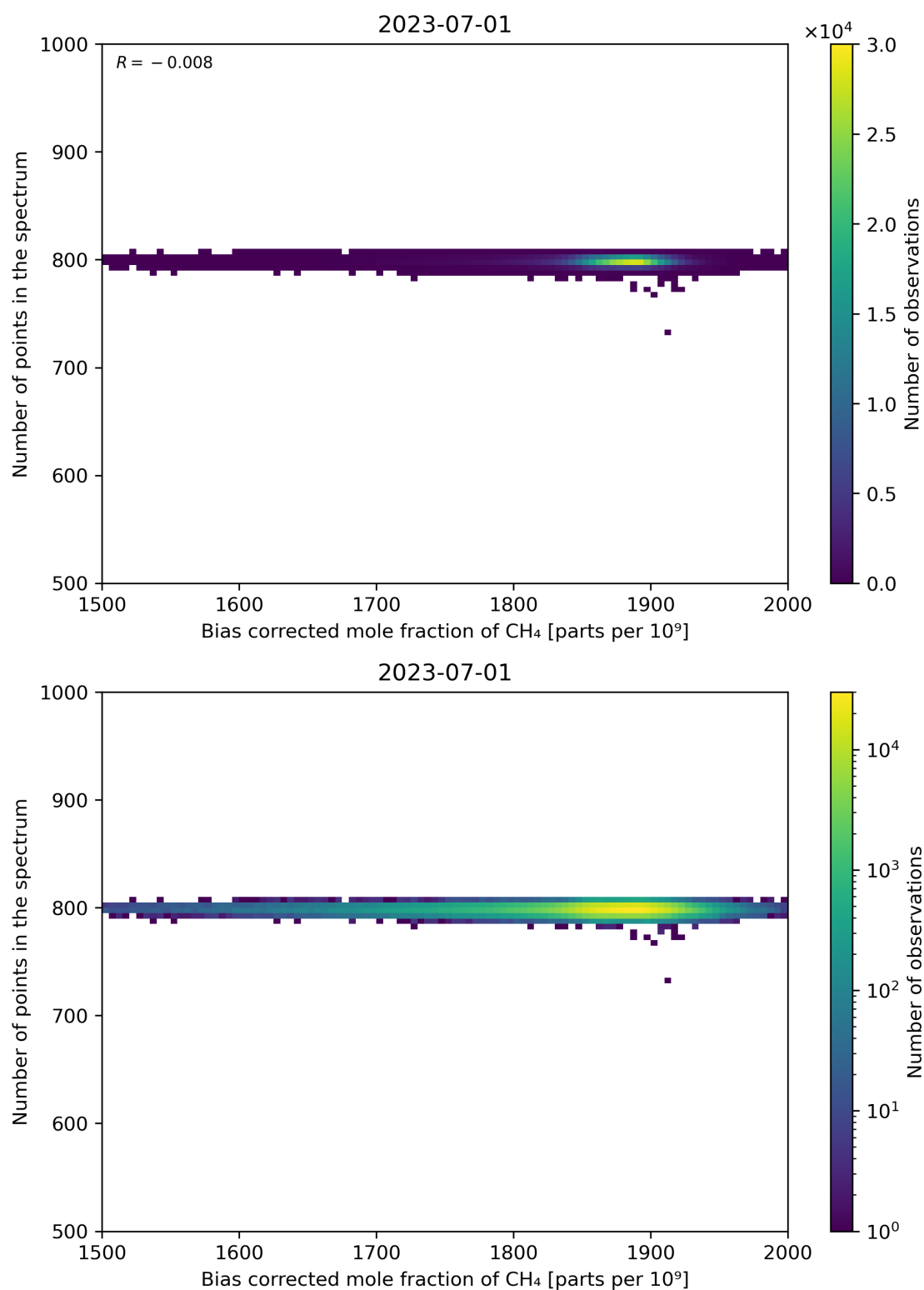
Figure 68: Scatter density plot of “Bias corrected mole fraction of CH 4 ” against “Number of points in the spectrum” for 2023-06-30 to 2023-07-02.
