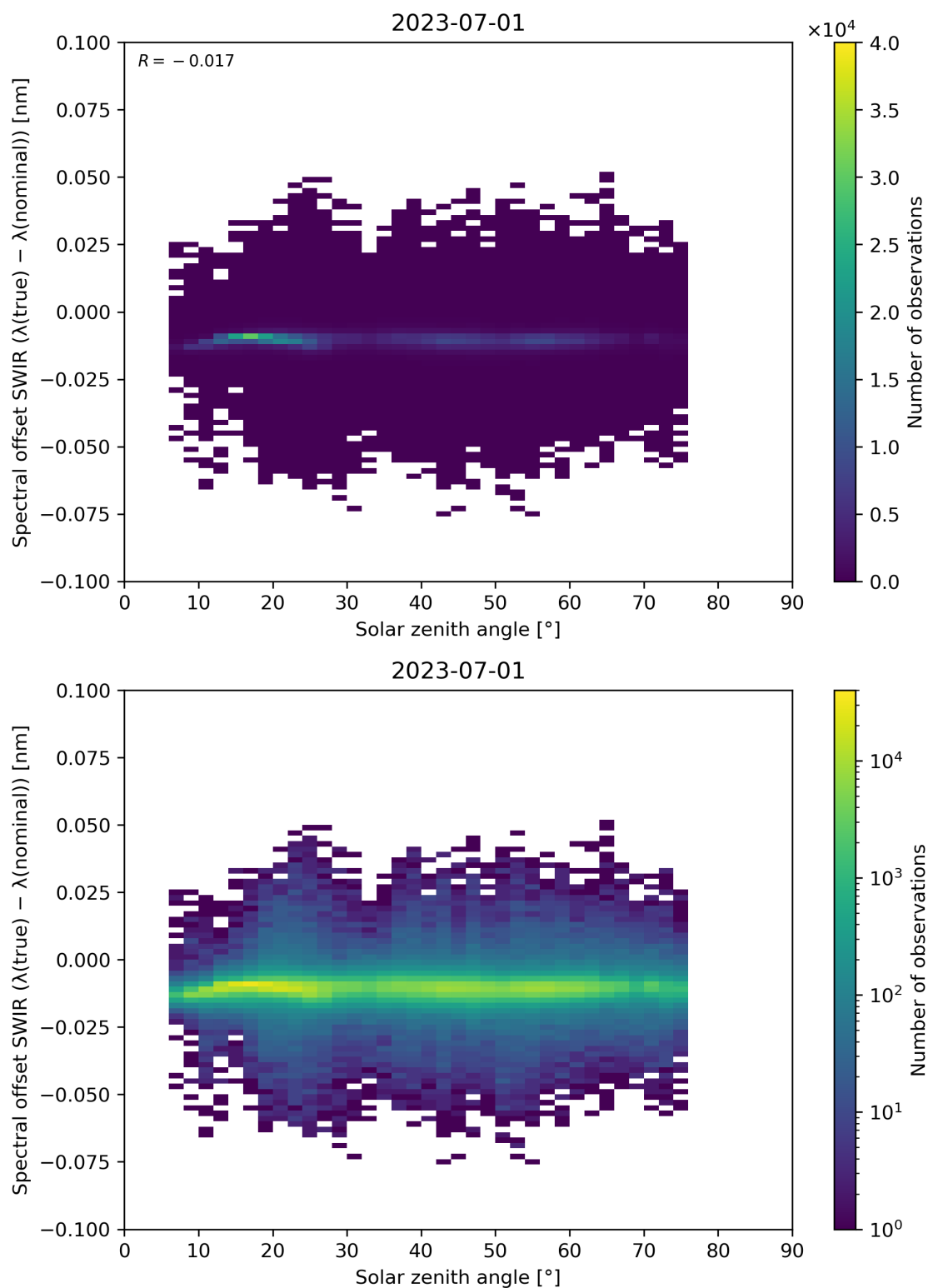
Figure 104: Scatter density plot of “Solar zenith angle” against “Spectral offset SWIR ( \lambda(\text{true}) - \lambda(\text{nominal}) )” for 2023-06-30 to 2023-07-02.
