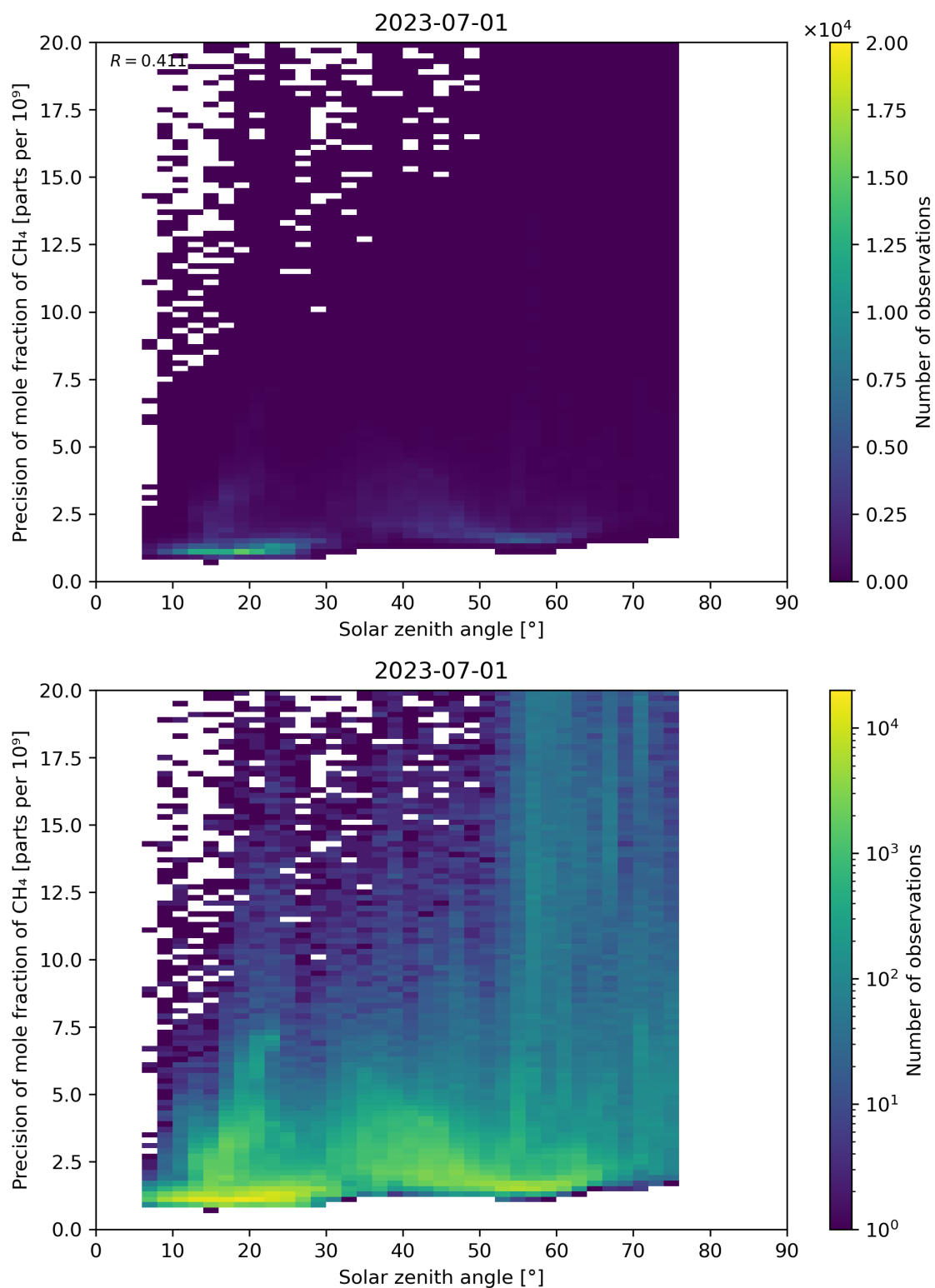
Figure 101: Scatter density plot of “Solar zenith angle” against “Precision of mole fraction of CH 4 ” for 2023-06-30 to 2023-07-02.
