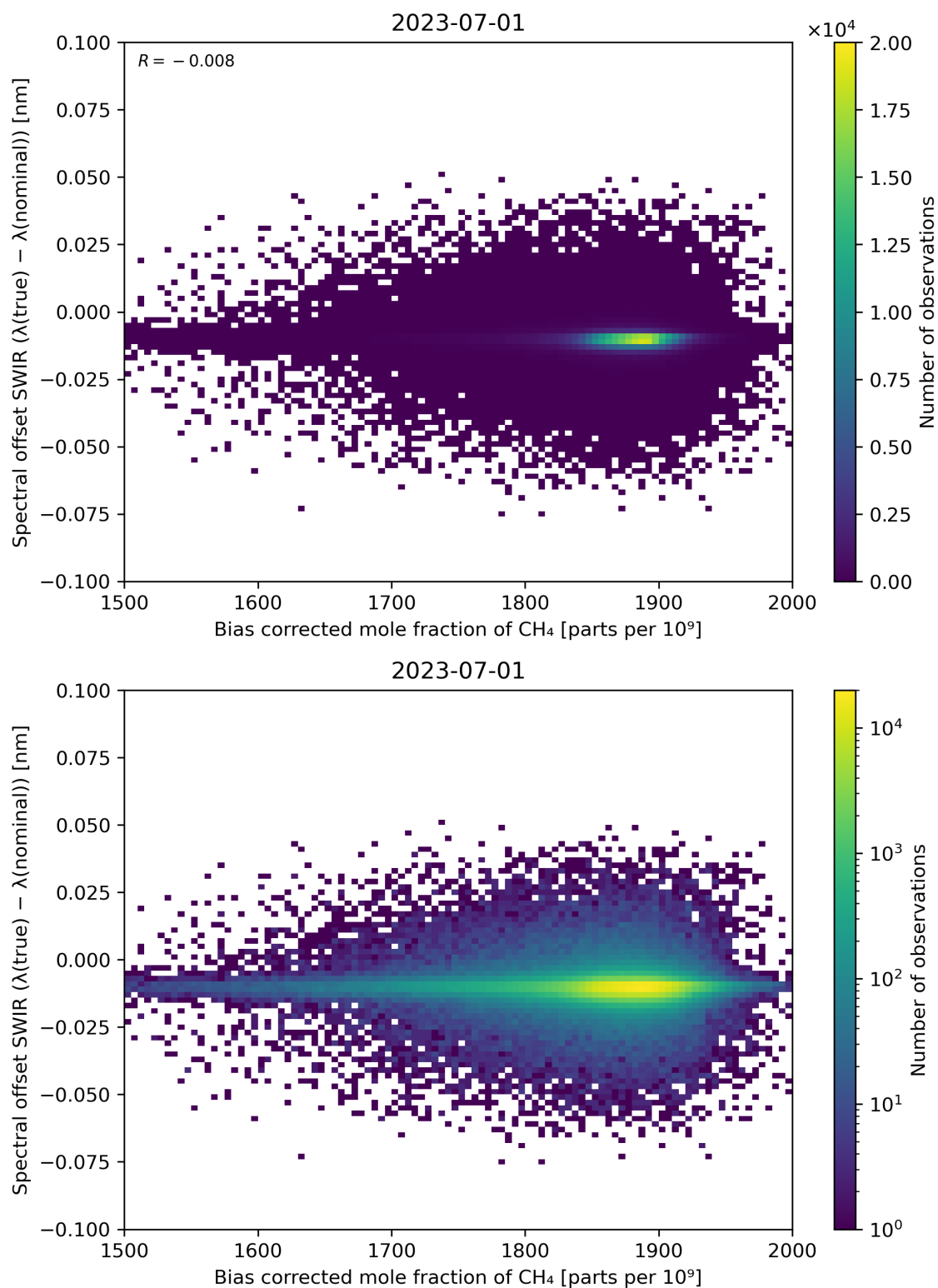
Figure 69: Scatter density plot of “Bias corrected mole fraction of \text{CH}_4 ” against “Spectral offset SWIR ( \lambda(\text{true}) - \lambda(\text{nominal}) )” for 2023-06-30 to 2023-07-02.
