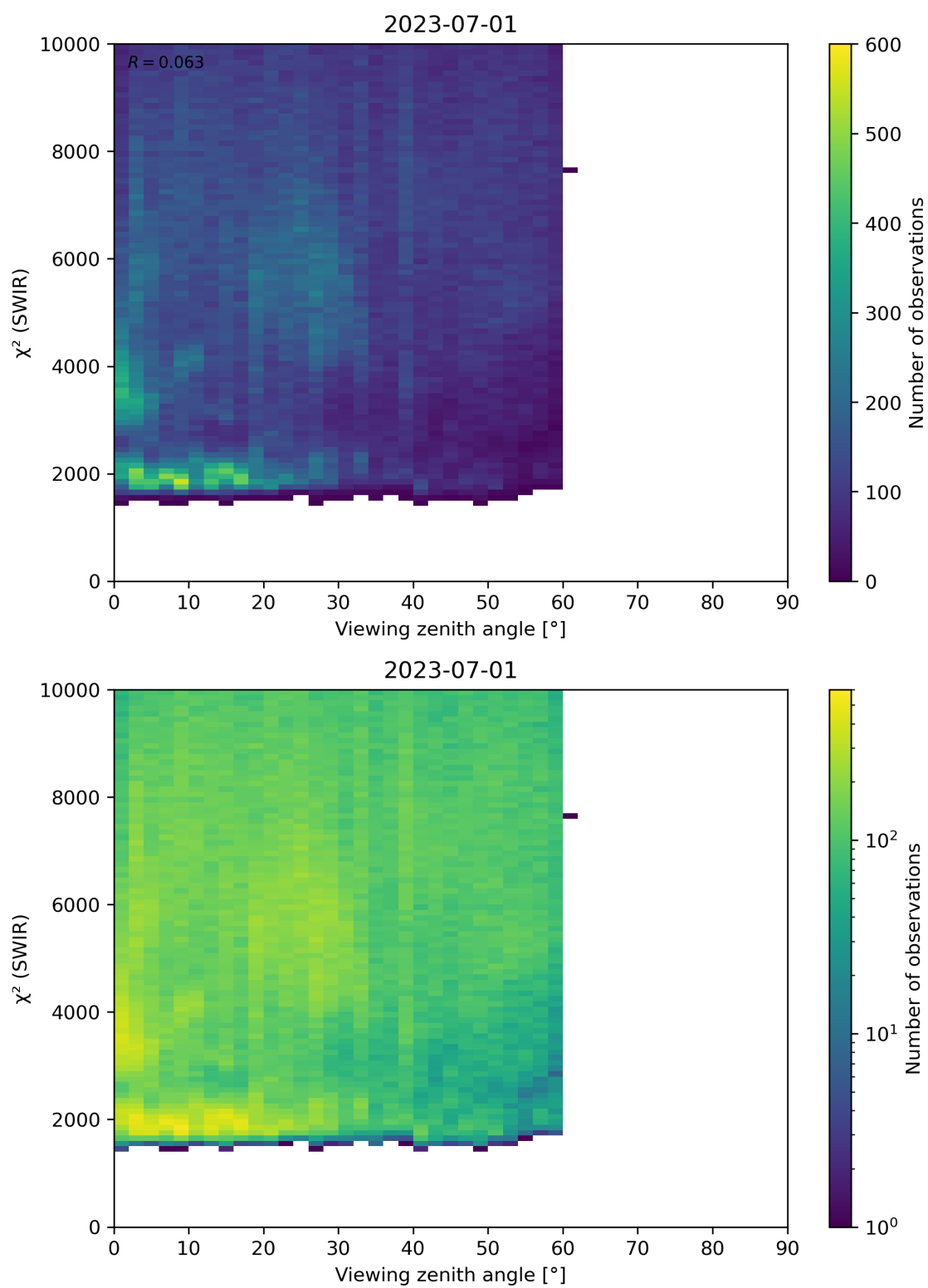
Figure 106: Scatter density plot of “Viewing zenith angle” against “ \chi^2 (SWIR)” for 2023-06-30 to 2023-07-02.
