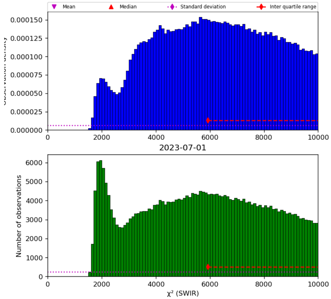
Figure 28: Histogram of “ \chi^2 (SWIR)” for 2023-06-30 to 2023-07-02
