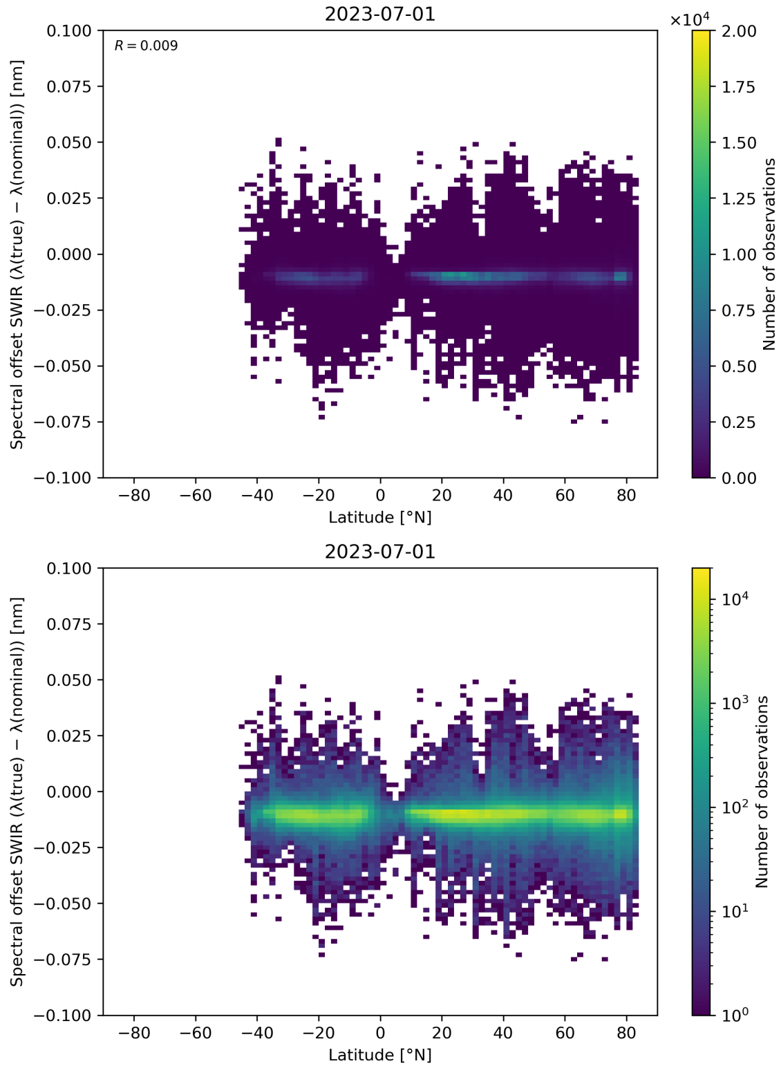
Figure 62: Scatter density plot of “Latitude” against “Spectral offset SWIR ( \lambda(\text{true}) - \lambda(\text{nominal}) )” for 2023-06-30 to 2023-07-02.
