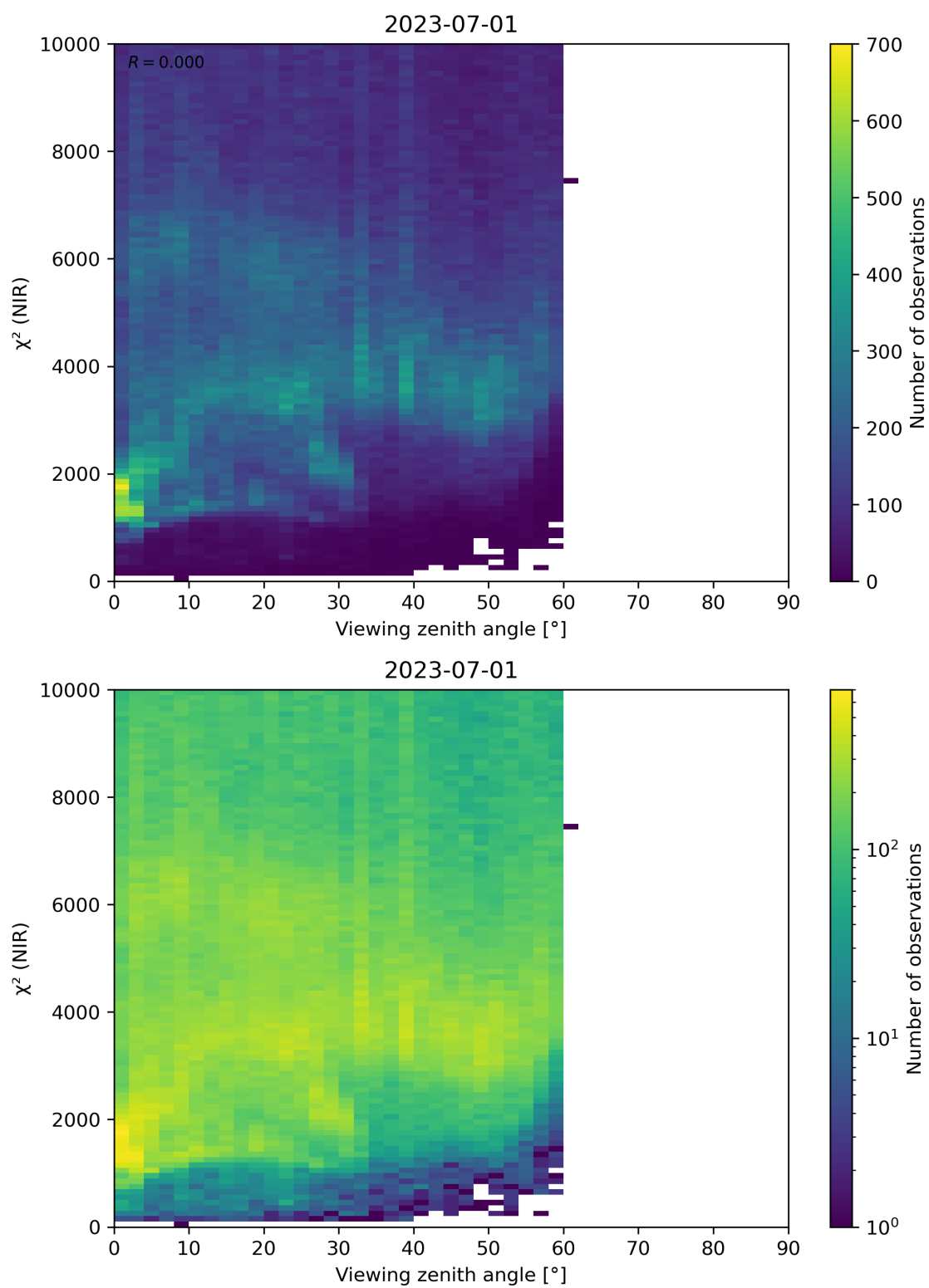
Figure 105: Scatter density plot of “Viewing zenith angle” against “ \chi^2 (NIR)” for 2023-06-30 to 2023-07-02.
