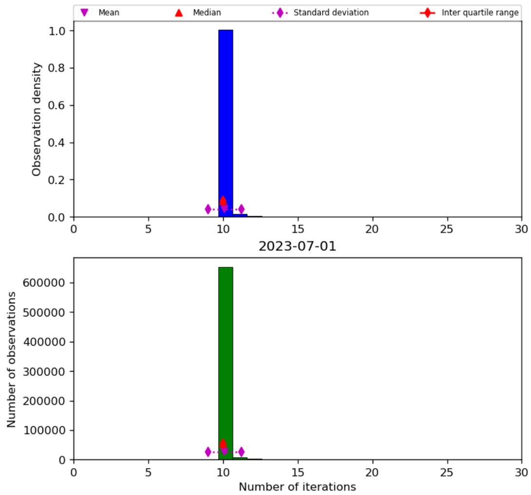
Figure 31: Histogram of “Number of iterations” for 2023-06-30 to 2023-07-02
