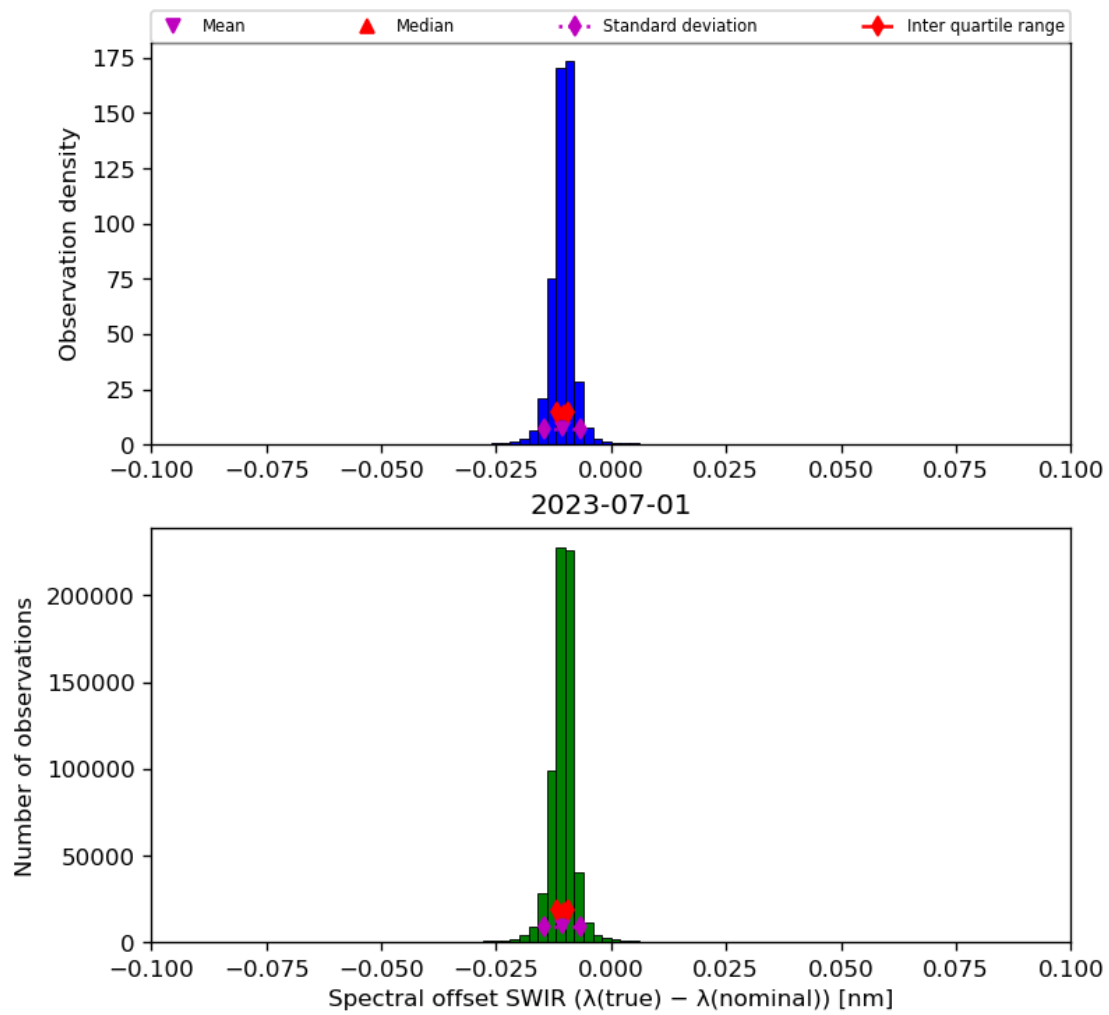
Figure 27: Histogram of “Spectral offset SWIR ( \lambda(\text{true}) - \lambda(\text{nominal}) )” for 2023-06-30 to 2023-07-02
