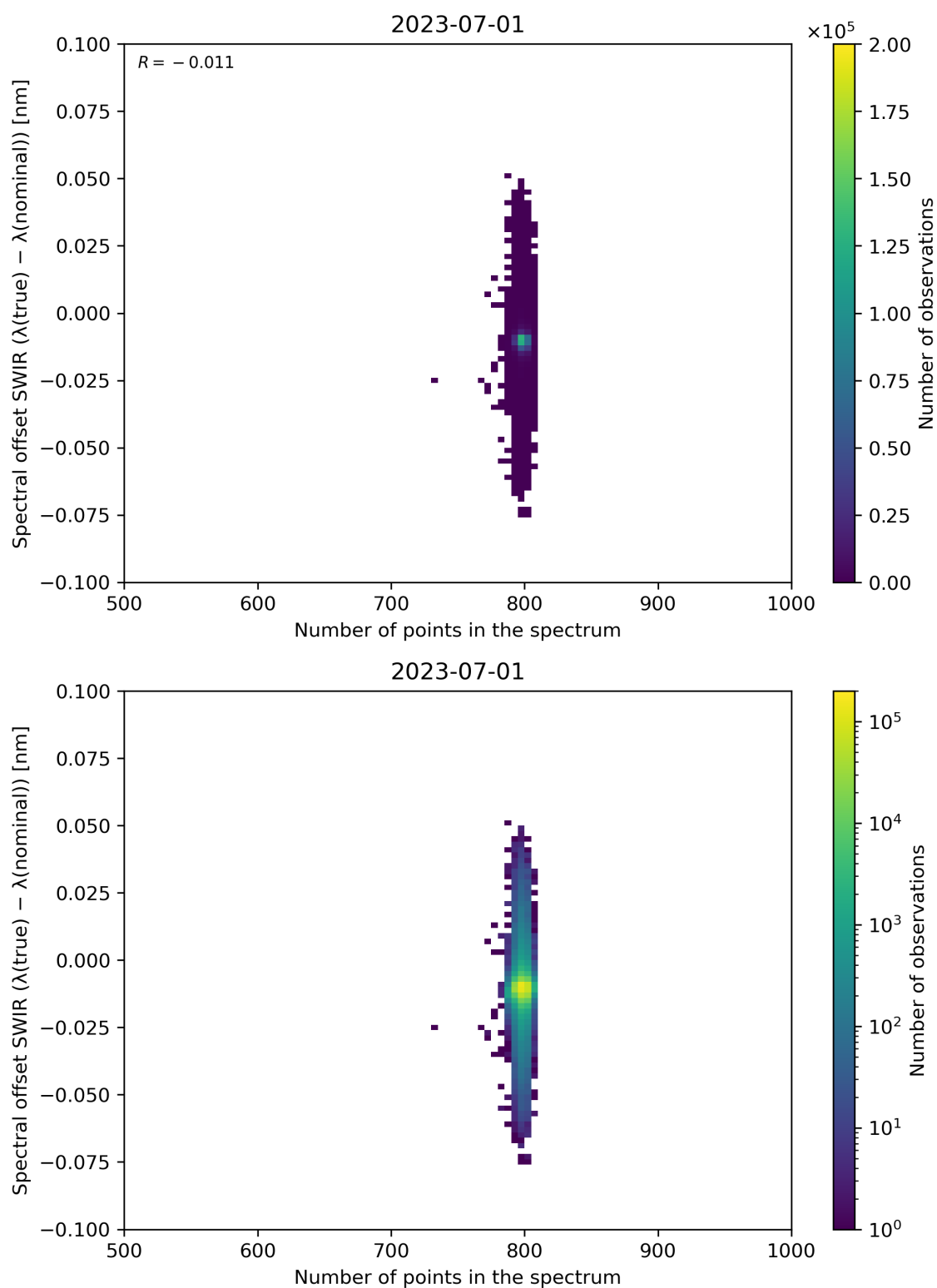
Figure 93: Scatter density plot of “Number of points in the spectrum” against “Spectral offset SWIR ( \lambda(\text{true}) - \lambda(\text{nominal}) )” for 2023-06-30 to 2023-07-02.
