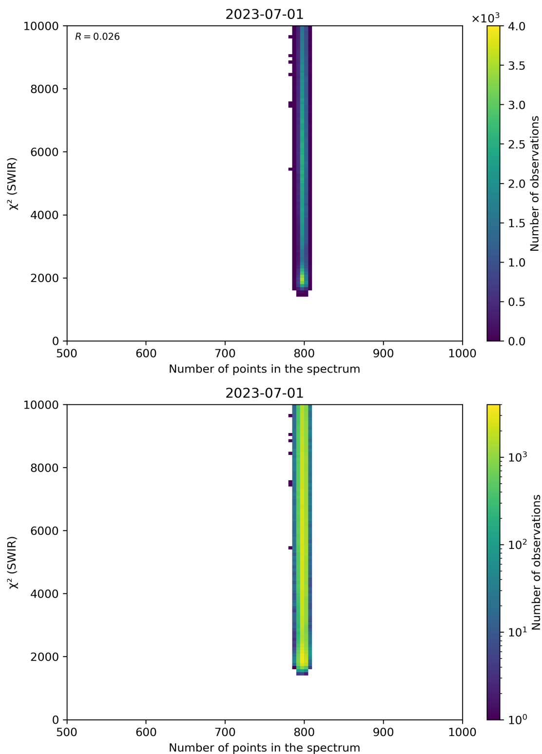
Figure 89: Scatter density plot of “Number of points in the spectrum” against “ \chi^2 (SWIR)” for 2023-06-30 to 2023-07-02.
