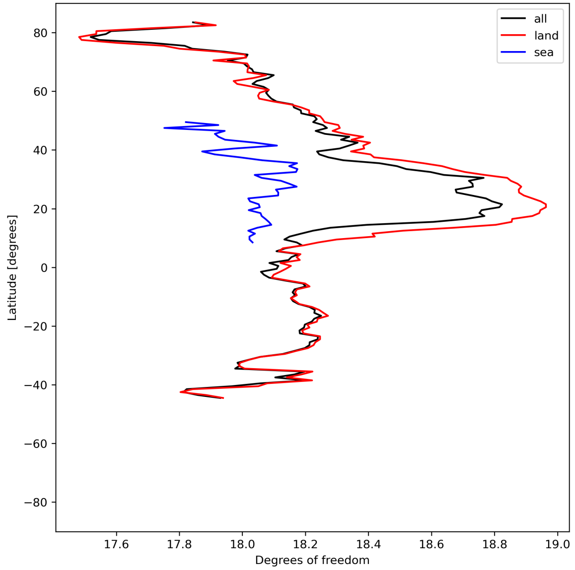
Figure 19: Zonal average of “Degrees of freedom” for 2023-06-30 to 2023-07-02.
