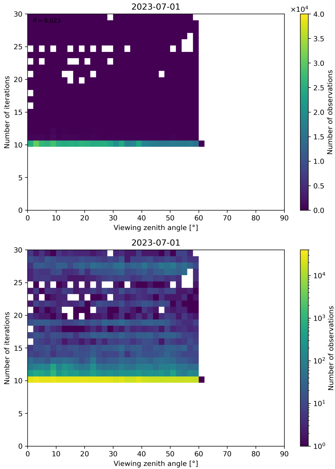
Figure 113: Scatter density plot of “Viewing zenith angle” against “Number of iterations” for 2023-06-30 to 2023-07-02.
