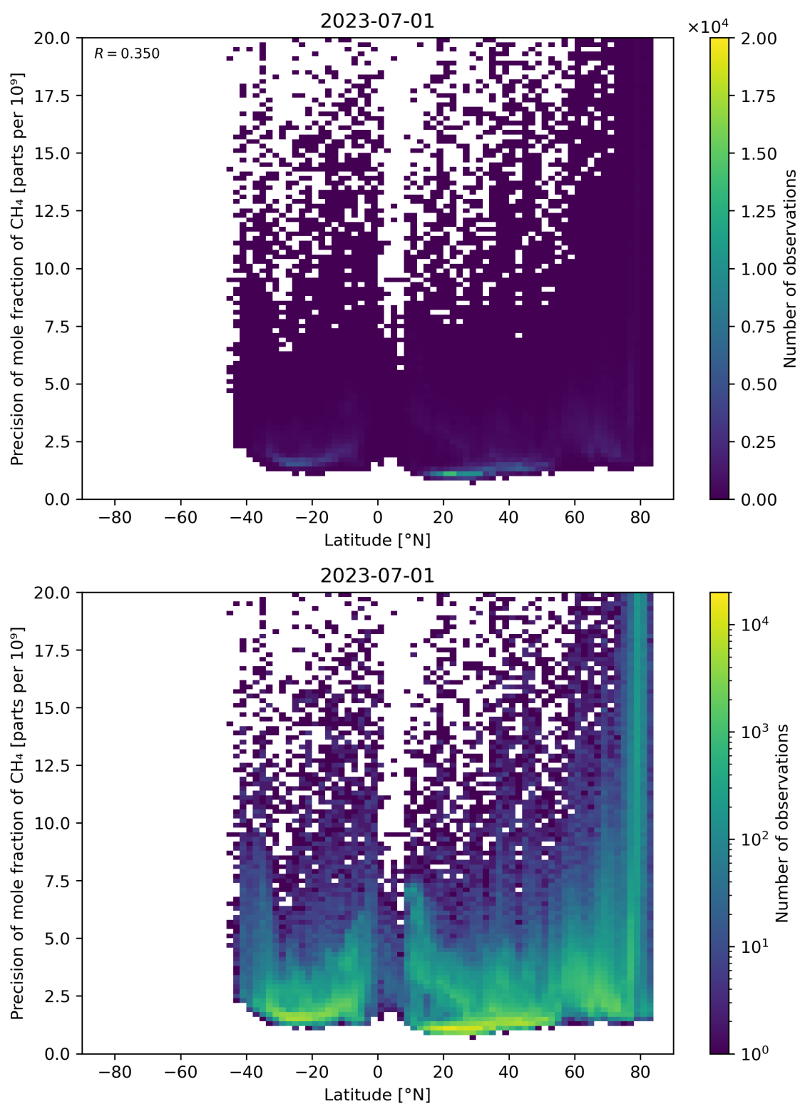
Figure 59: Scatter density plot of “Latitude” against “Precision of mole fraction of \text{CH}_4 ” for 2023-06-30 to 2023-07-02.
