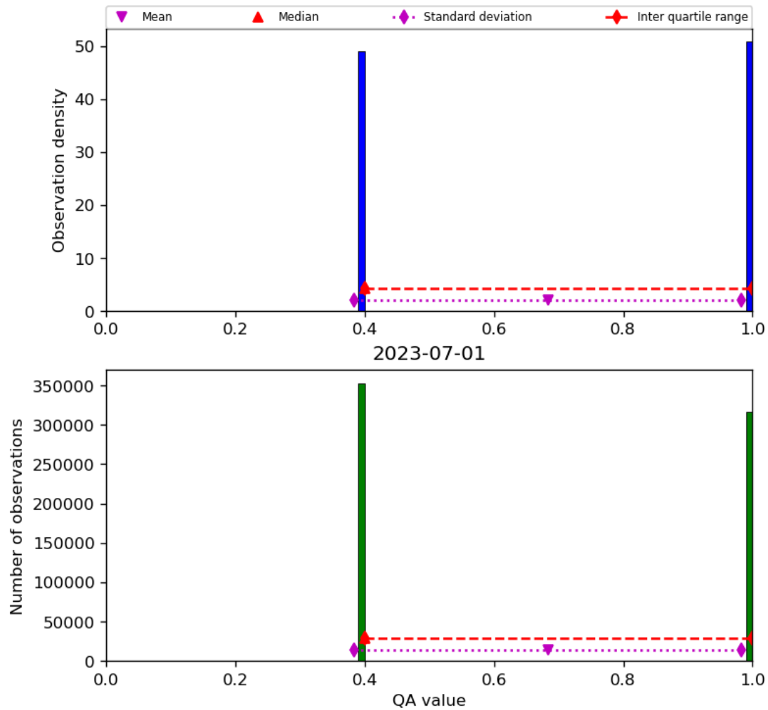
Figure 22: Histogram of “QA value” for 2023-06-30 to 2023-07-02
