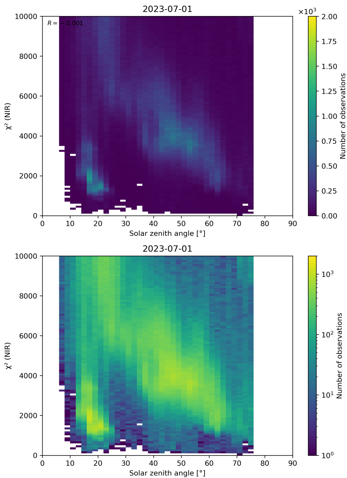
Figure 94: Scatter density plot of “Solar zenith angle” against “ \chi^2 (NIR)” for 2023-06-30 to 2023-07-02.
