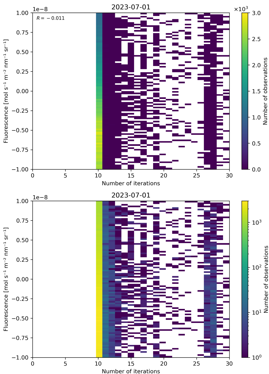
Figure 87: Scatter density plot of “Number of iterations” against “Fluorescence” for 2023-06-30 to 2023-07-02.
