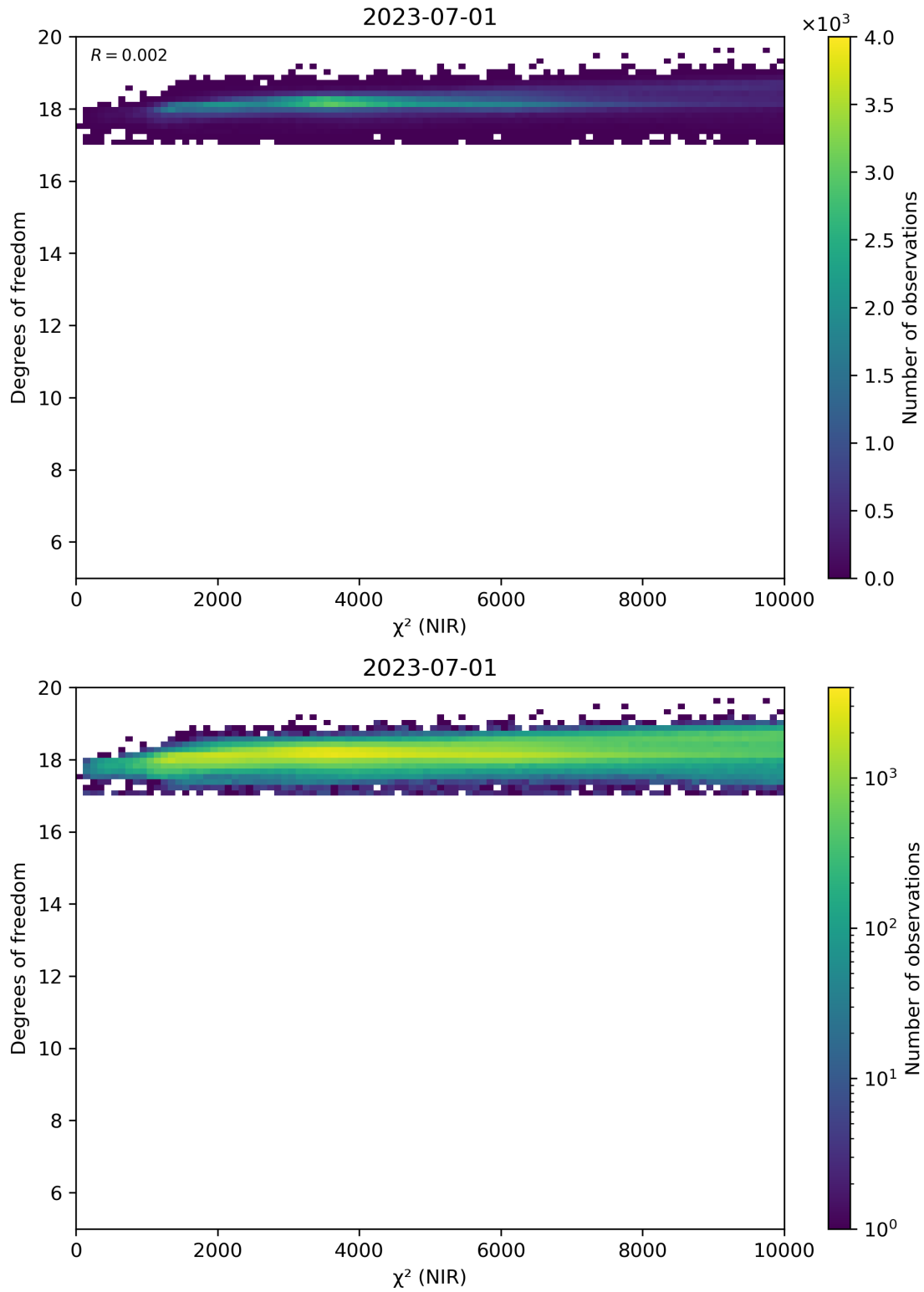
Figure 44: Scatter density plot of “ \chi^2 (NIR)” against “Degrees of freedom” for 2023-06-30 to 2023-07-02.
