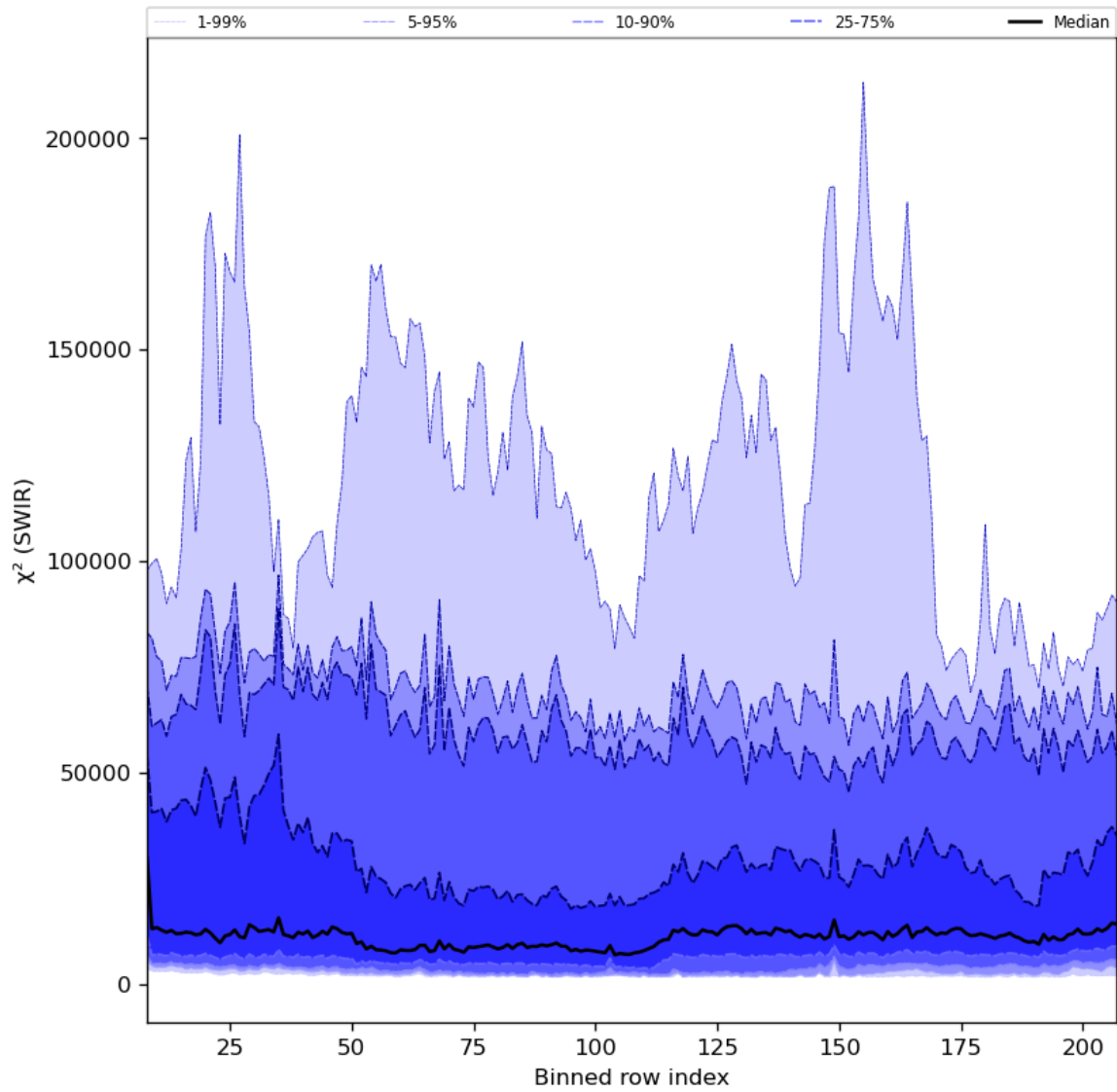
Figure 39: Along track statistics of “ \chi^2 (SWIR)” for 2023-06-30 to 2023-07-02
