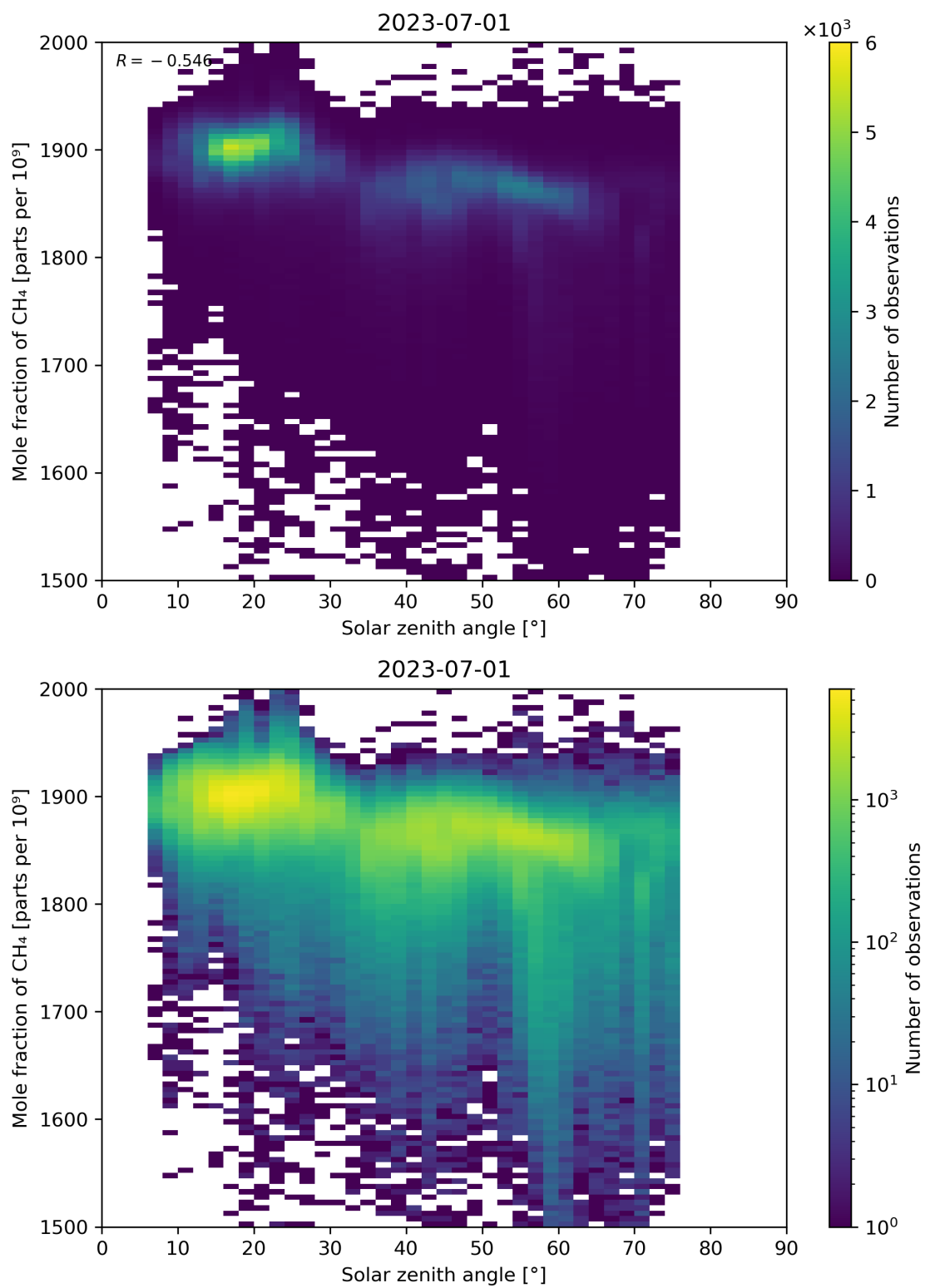
Figure 99: Scatter density plot of “Solar zenith angle” against “Mole fraction of CH 4 ” for 2023-06-30 to 2023-07-02.
