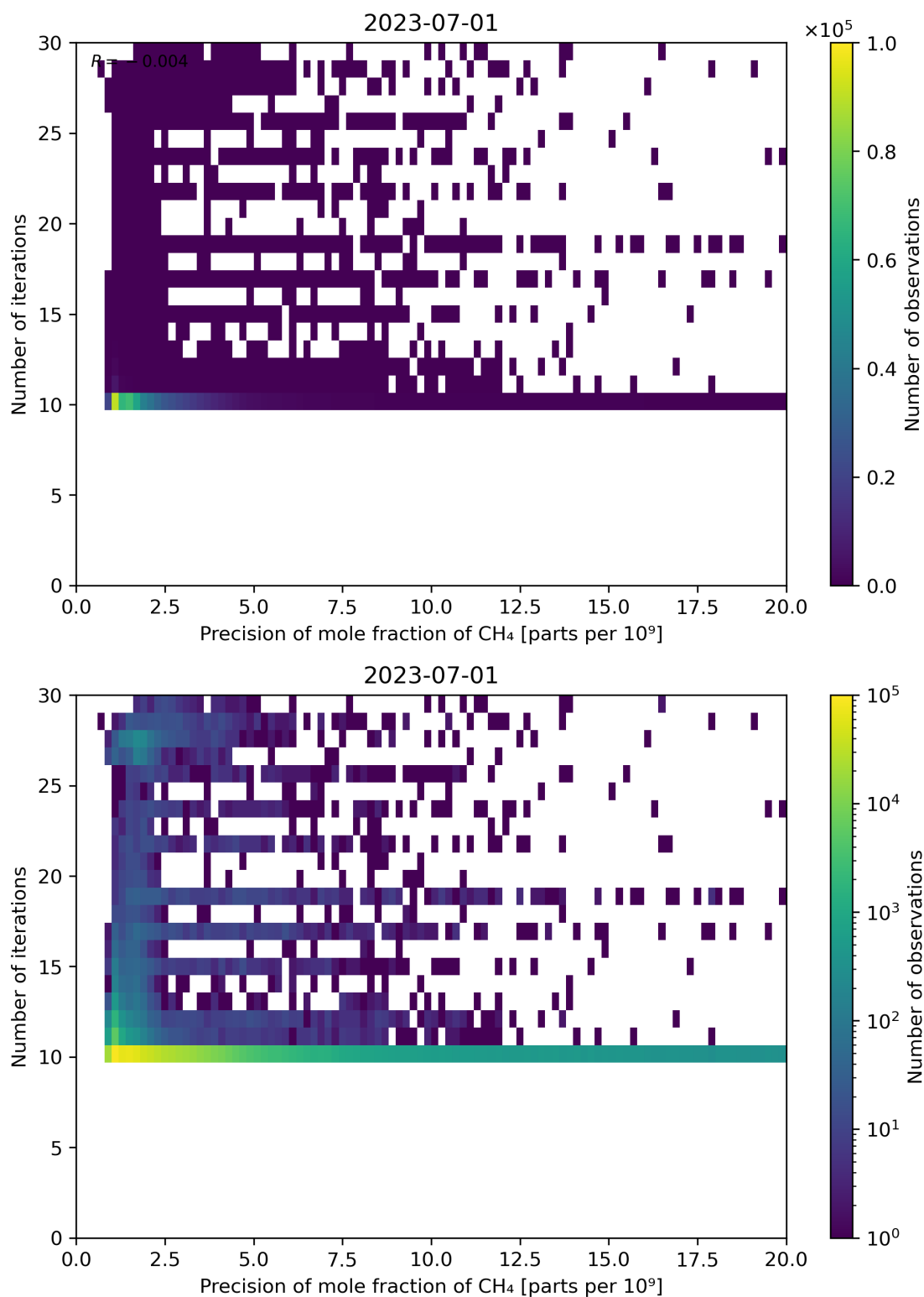
Figure 83: Scatter density plot of “Precision of mole fraction of CH 4 ” against “Number of iterations” for 2023-06-30 to 2023-07-02.
