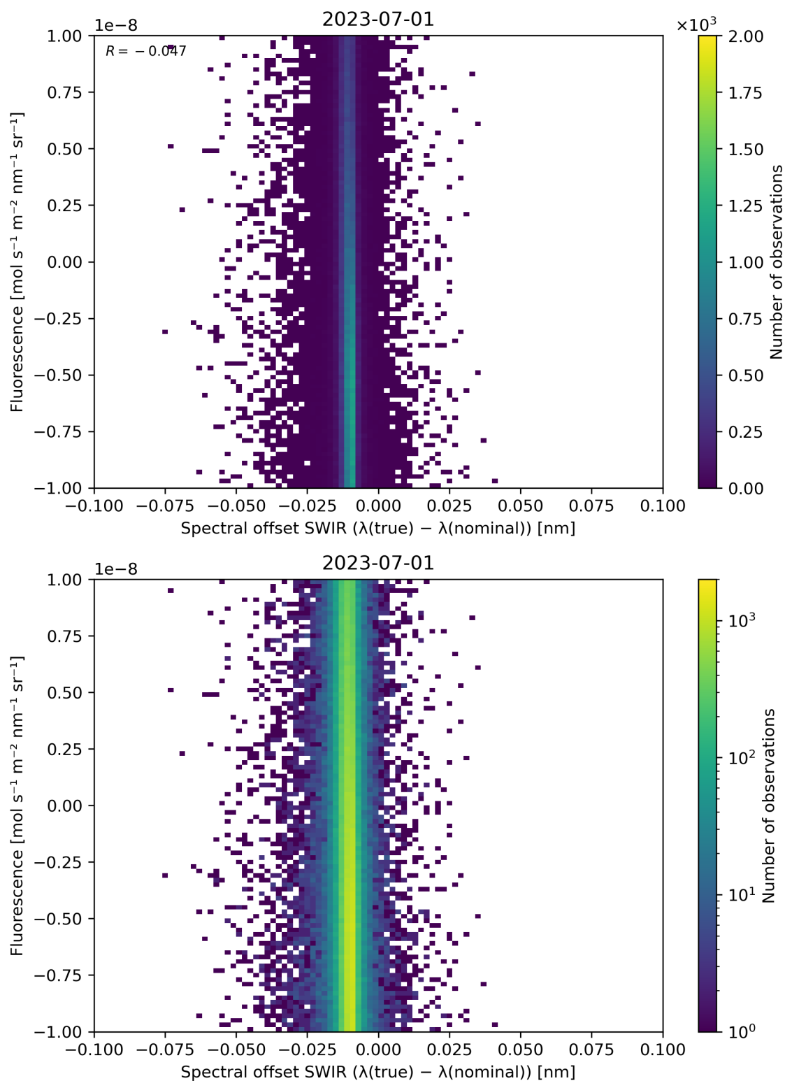
Figure 120: Scatter density plot of “Spectral offset SWIR ( \lambda(\text{true}) - \lambda(\text{nominal}) )” against “Fluorescence” for 2023-06-30 to 2023-07-02.
