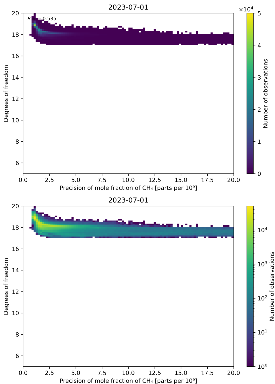
Figure 80: Scatter density plot of “Precision of mole fraction of CH 4 ” against “Degrees of freedom” for 2023-06-30 to 2023-07-02.
