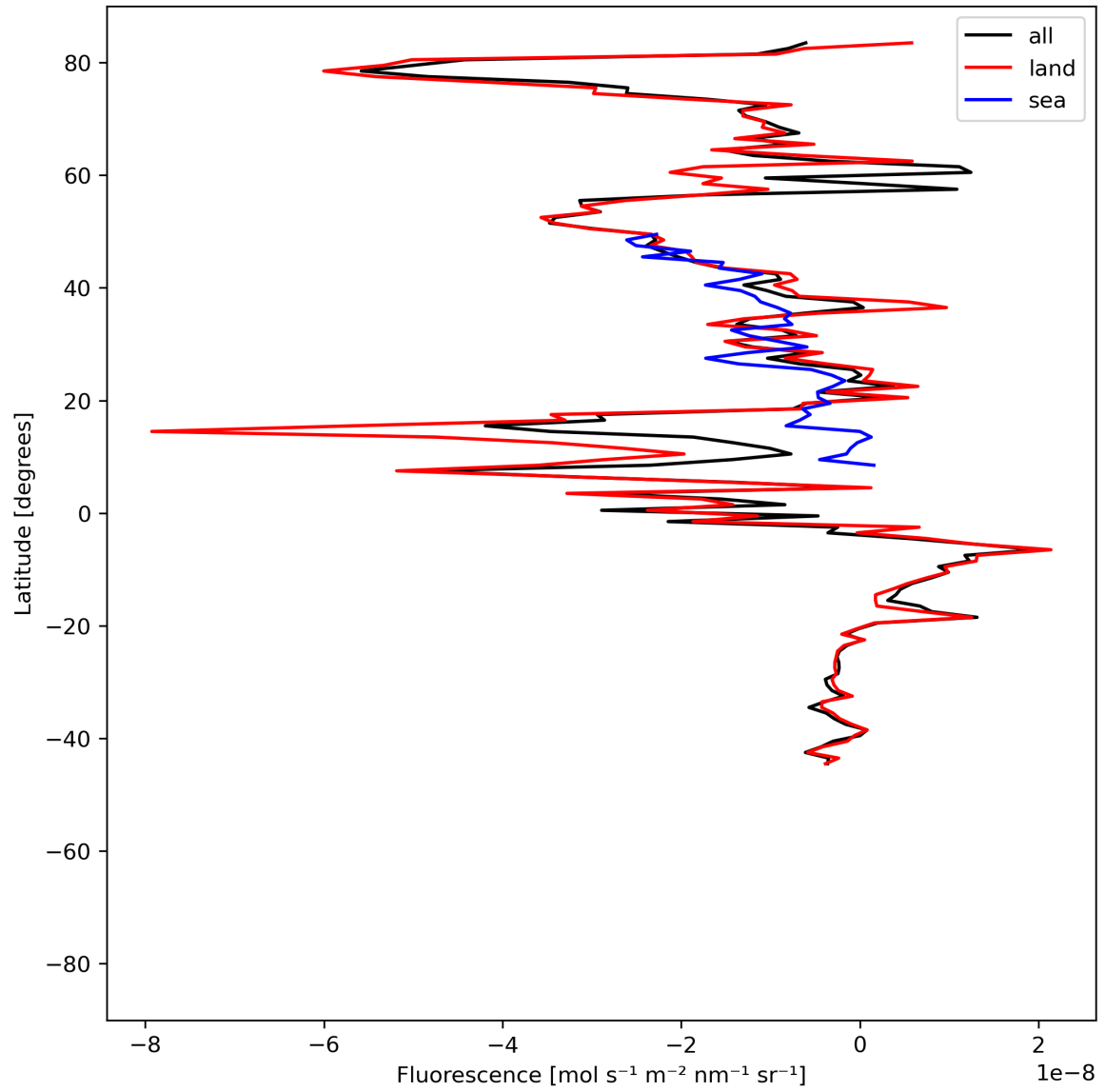
Figure 21: Zonal average of “Fluorescence” for 2023-06-30 to 2023-07-02.
