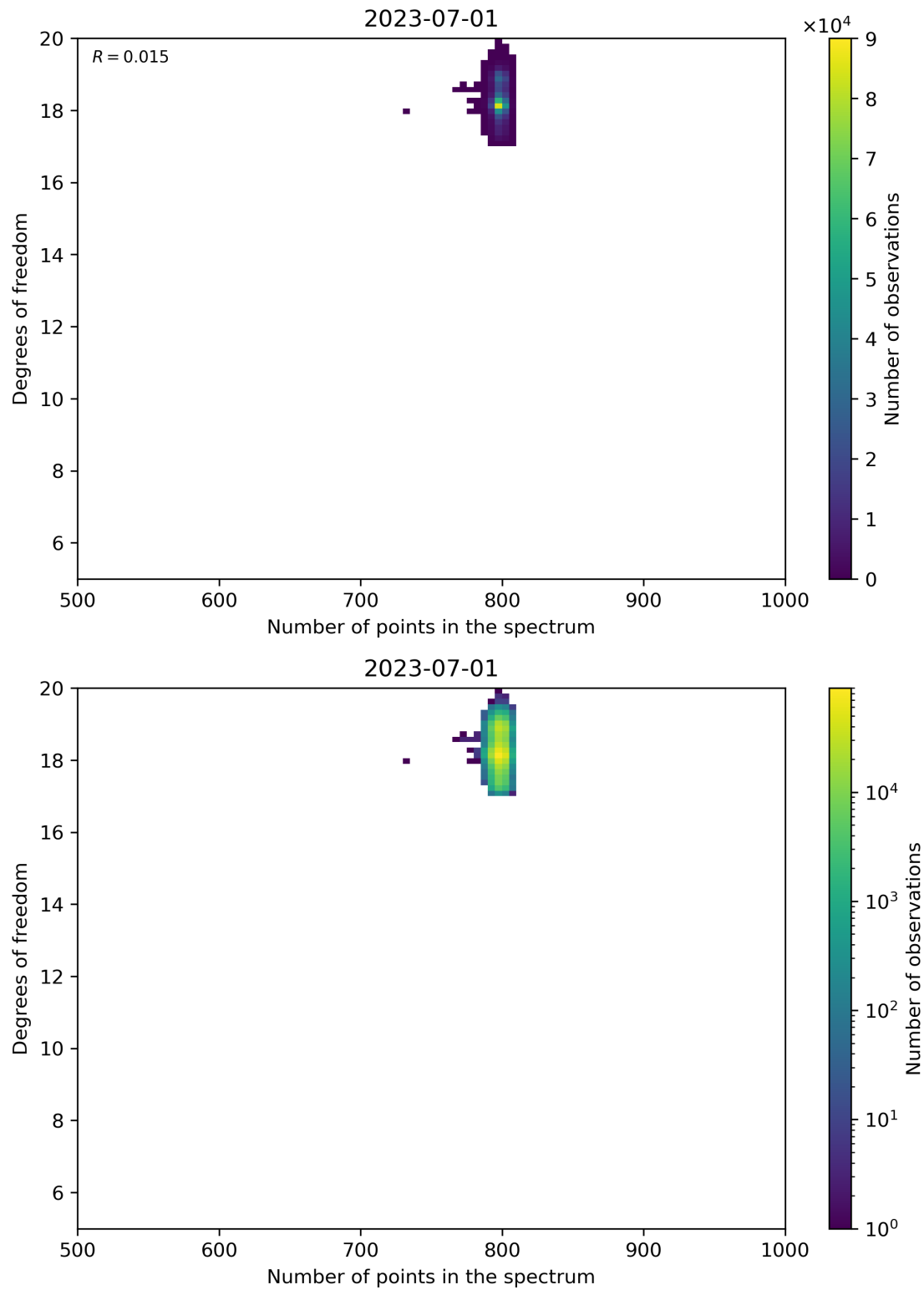
Figure 90: Scatter density plot of “Number of points in the spectrum” against “Degrees of freedom” for 2023-06-30 to 2023-07-02.
