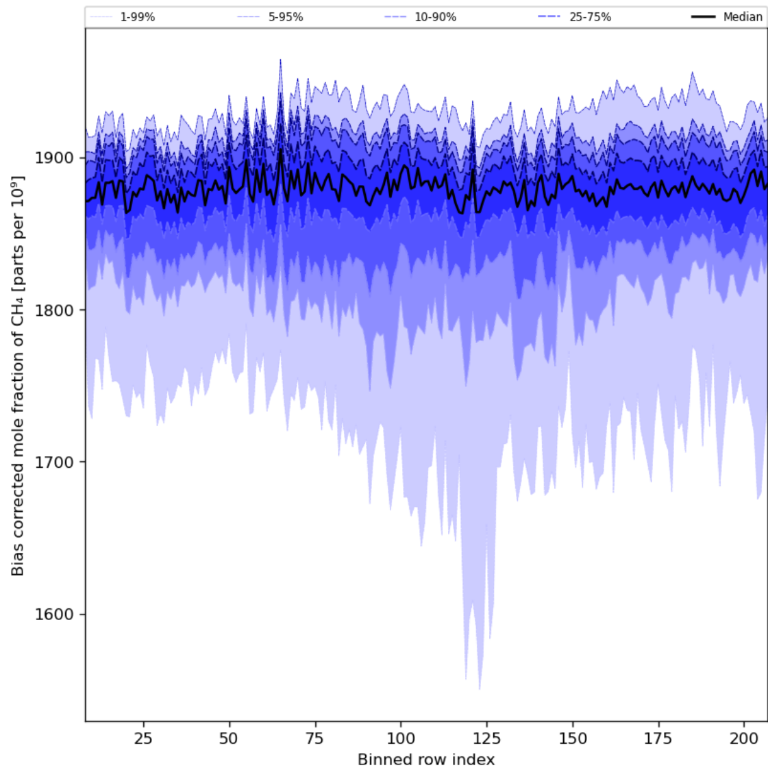
Figure 36: Along track statistics of “Bias corrected mole fraction of CH 4 ” for 2023-06-30 to 2023-07-02
