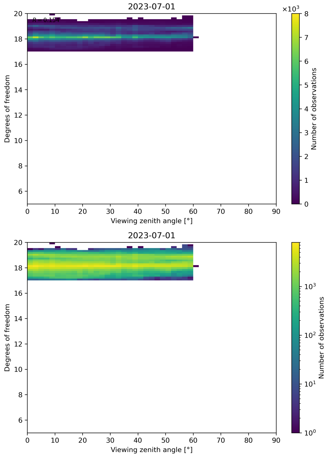
Figure 107: Scatter density plot of “Viewing zenith angle” against “Degrees of freedom” for 2023-06-30 to 2023-07-02.
