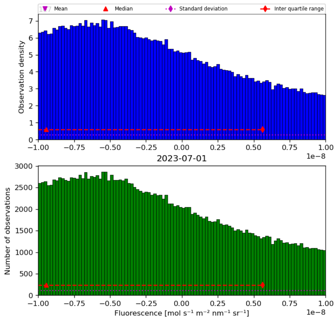
Figure 32: Histogram of “Fluorescence” for 2023-06-30 to 2023-07-02
