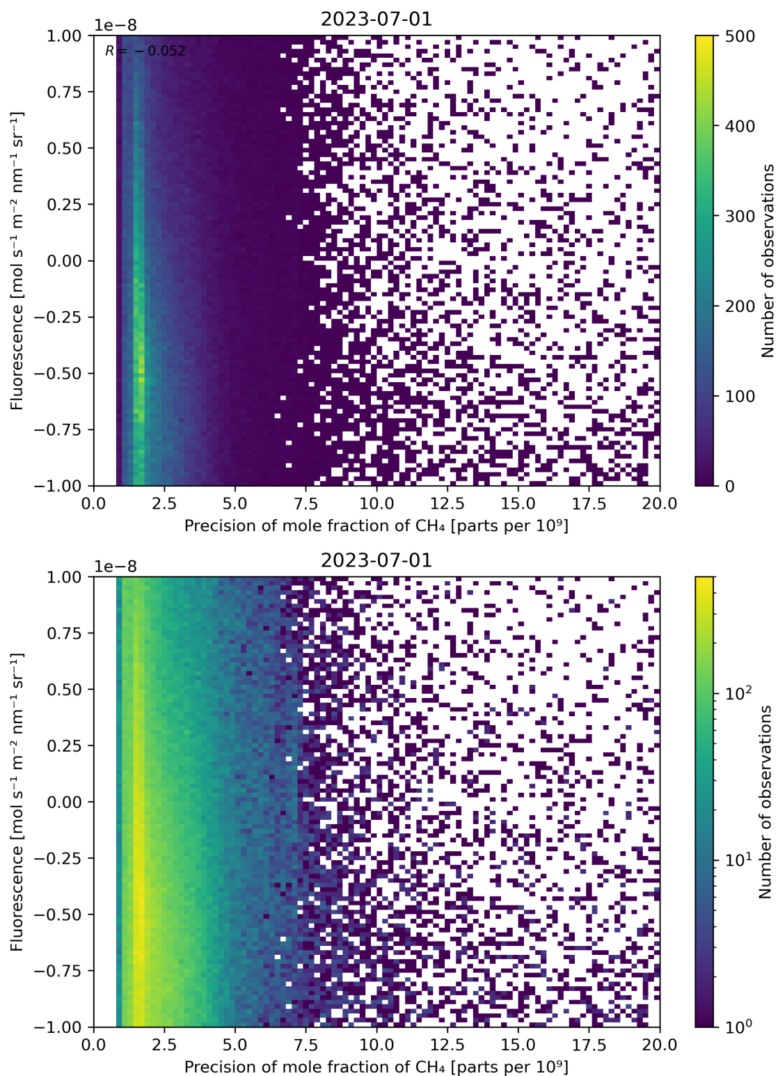
Figure 81: Scatter density plot of “Precision of mole fraction of \text{CH}_4 ” against “Fluorescence” for 2023-06-30 to 2023-07-02.
