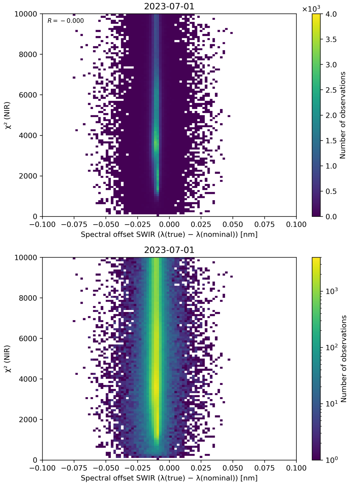
Figure 117: Scatter density plot of “Spectral offset SWIR ( \lambda(\text{true}) - \lambda(\text{nominal}) )” against “ \chi^2 (NIR)” for 2023-06-30 to 2023-07-02.
