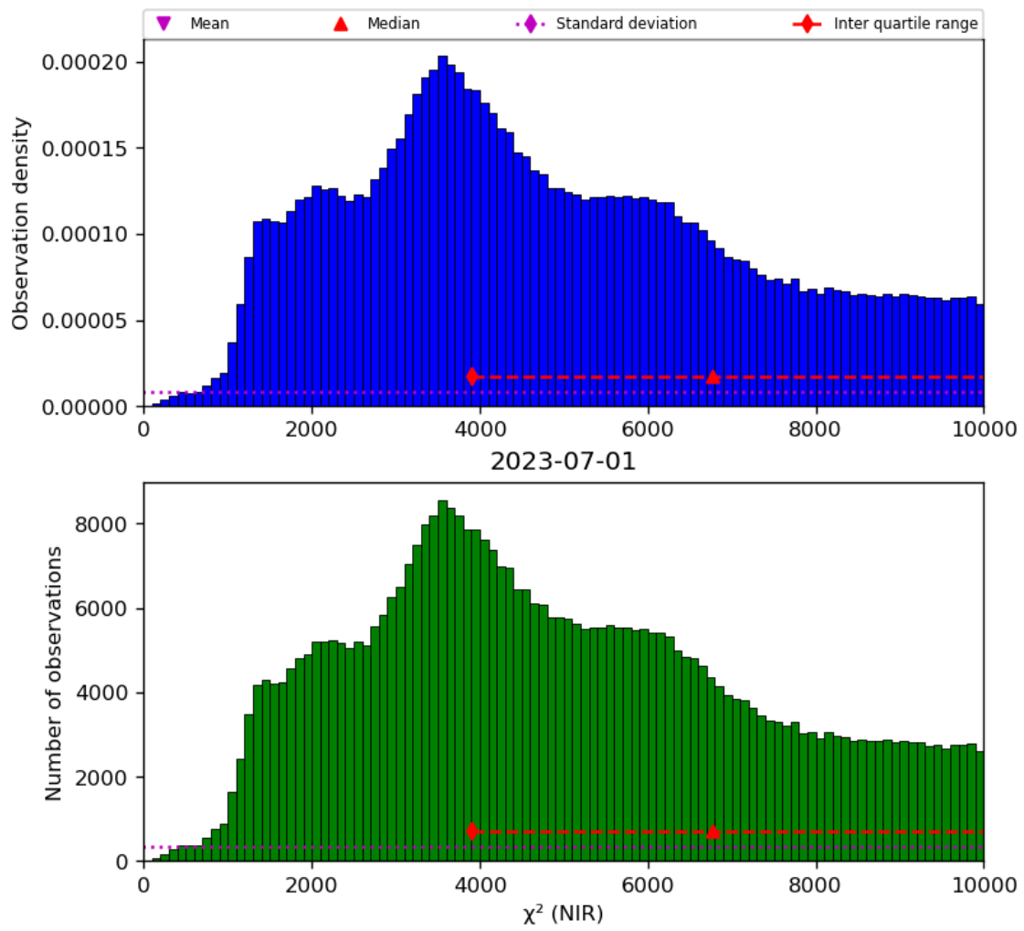
Figure 29: Histogram of “ \chi^2 (NIR)” for 2023-06-30 to 2023-07-02
