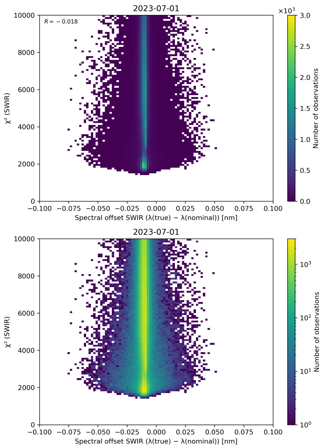
Figure 118: Scatter density plot of “Spectral offset SWIR ( \lambda(\text{true}) - \lambda(\text{nominal}) )” against “ \chi^2 (SWIR)” for 2023-06-30 to 2023-07-02.
