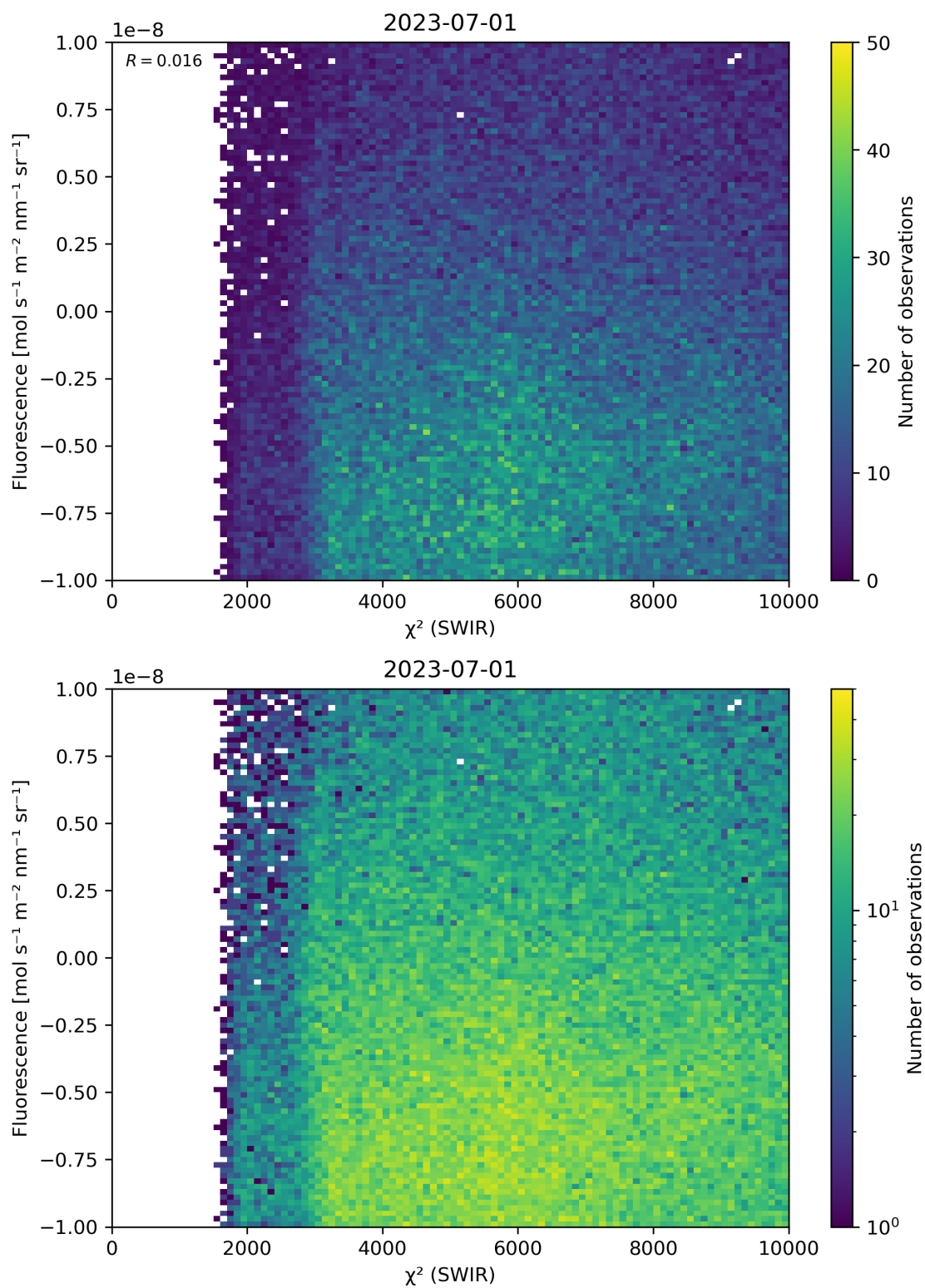
Figure 49: Scatter density plot of “ \chi^2 (SWIR)” against “Fluorescence” for 2023-06-30 to 2023-07-02.
