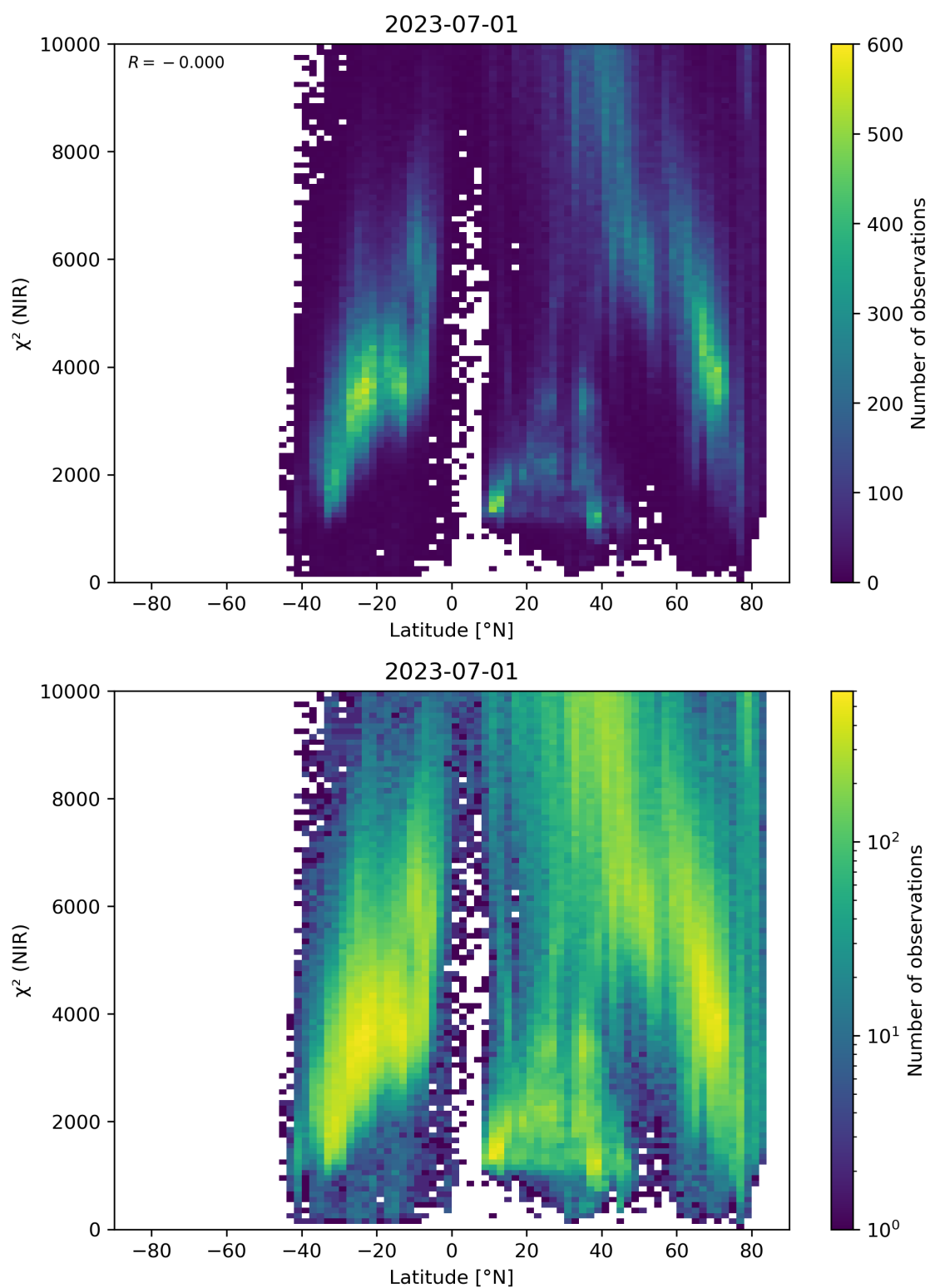
Figure 53: Scatter density plot of “Latitude” against “ \chi^2 (NIR)” for 2023-06-30 to 2023-07-02.
