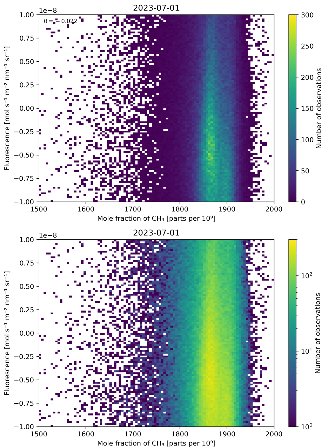
Figure 73: Scatter density plot of “Mole fraction of \text{CH}_4 ” against “Fluorescence” for 2023-06-30 to 2023-07-02.
