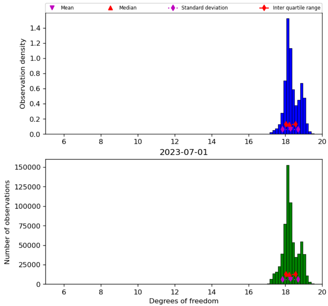
Figure 30: Histogram of “Degrees of freedom” for 2023-06-30 to 2023-07-02
