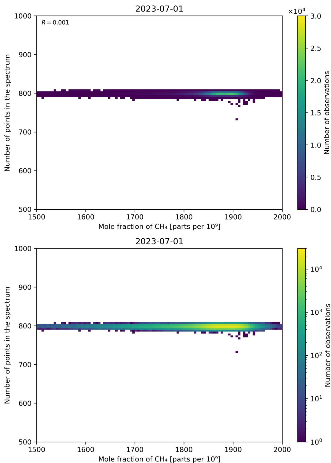
Figure 77: Scatter density plot of “Mole fraction of CH 4 ” against “Number of points in the spectrum” for 2023-06-30 to 2023-07-02.
