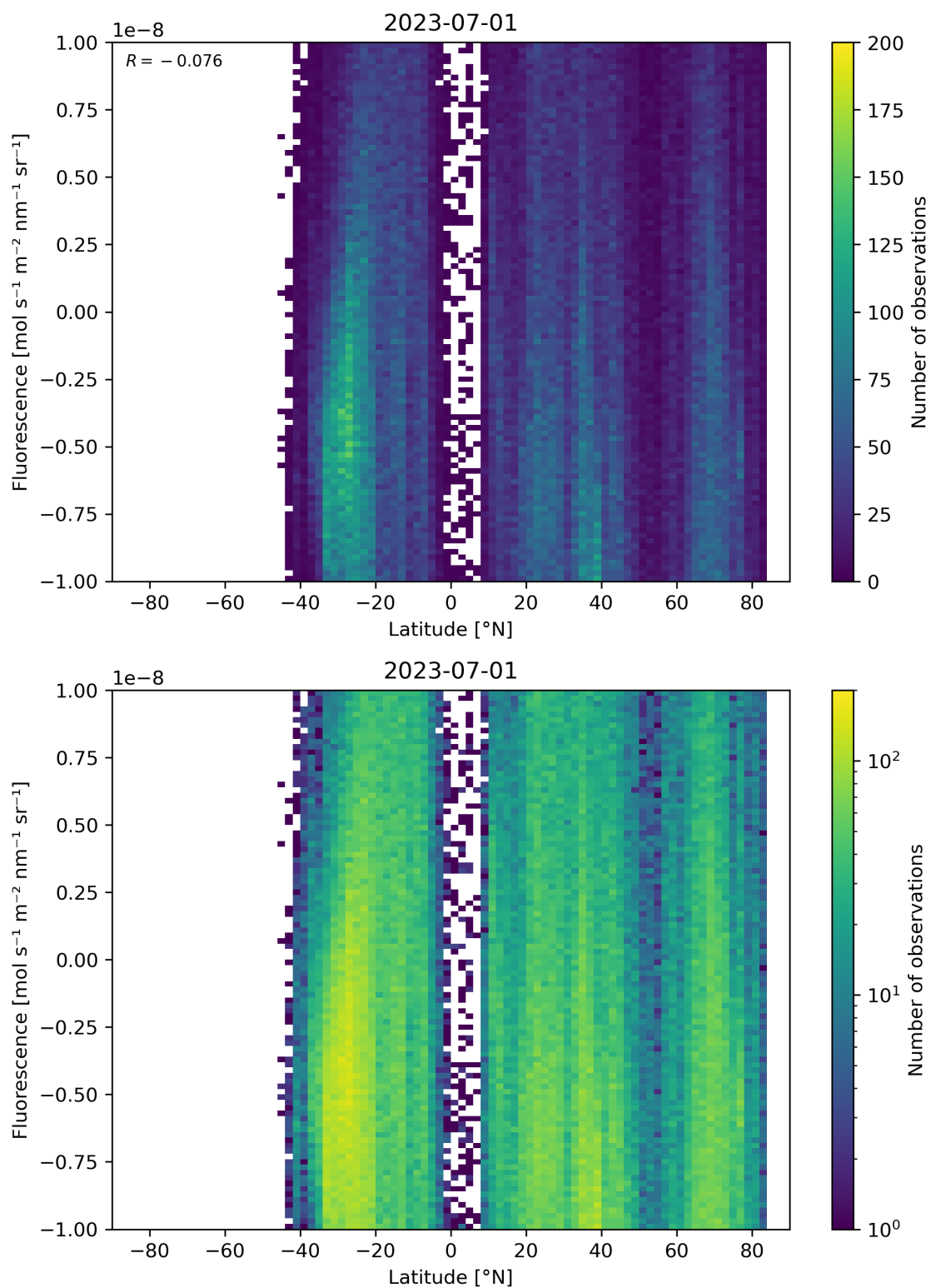
Figure 56: Scatter density plot of “Latitude” against “Fluorescence” for 2023-06-30 to 2023-07-02.
