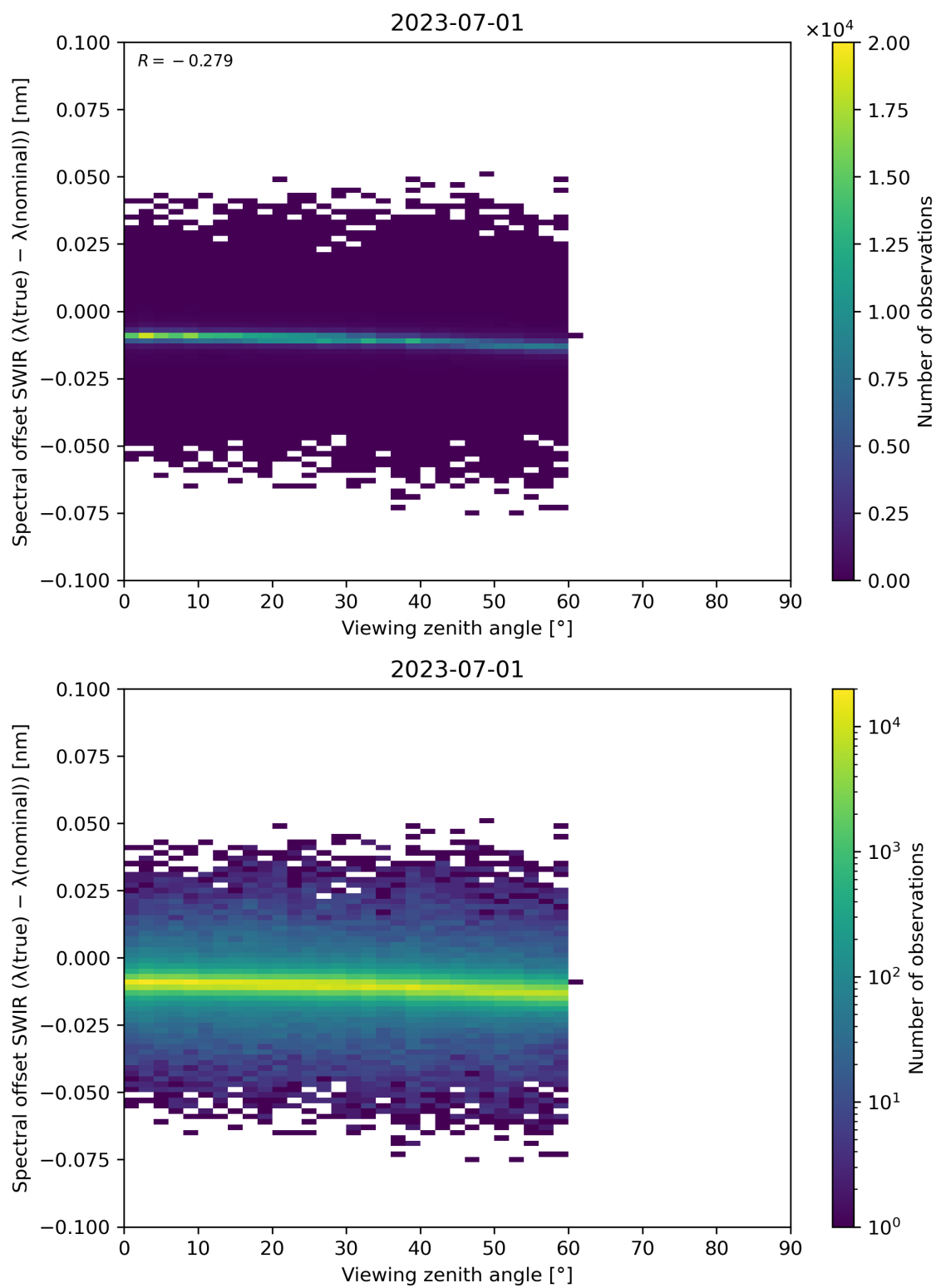
Figure 116: Scatter density plot of “Viewing zenith angle” against “Spectral offset SWIR ( \lambda(\text{true}) - \lambda(\text{nominal}) )” for 2023-06-30 to 2023-07-02.
