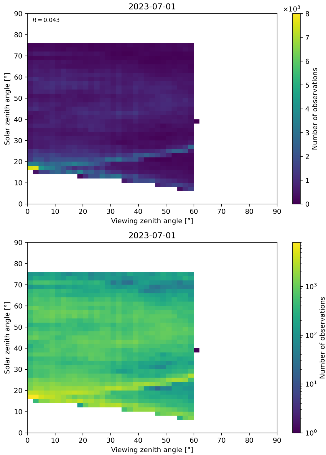
Figure 115: Scatter density plot of “Viewing zenith angle” against “Solar zenith angle” for 2023-06-30 to 2023-07-02.
