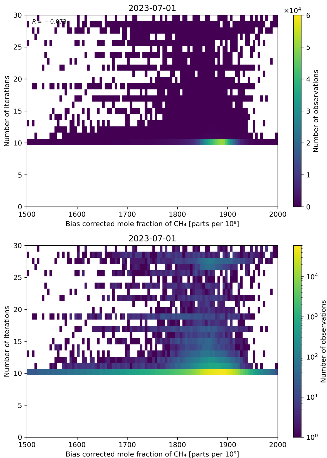
Figure 67: Scatter density plot of “Bias corrected mole fraction of CH 4 ” against “Number of iterations” for 2023-06-30 to 2023-07-02.
