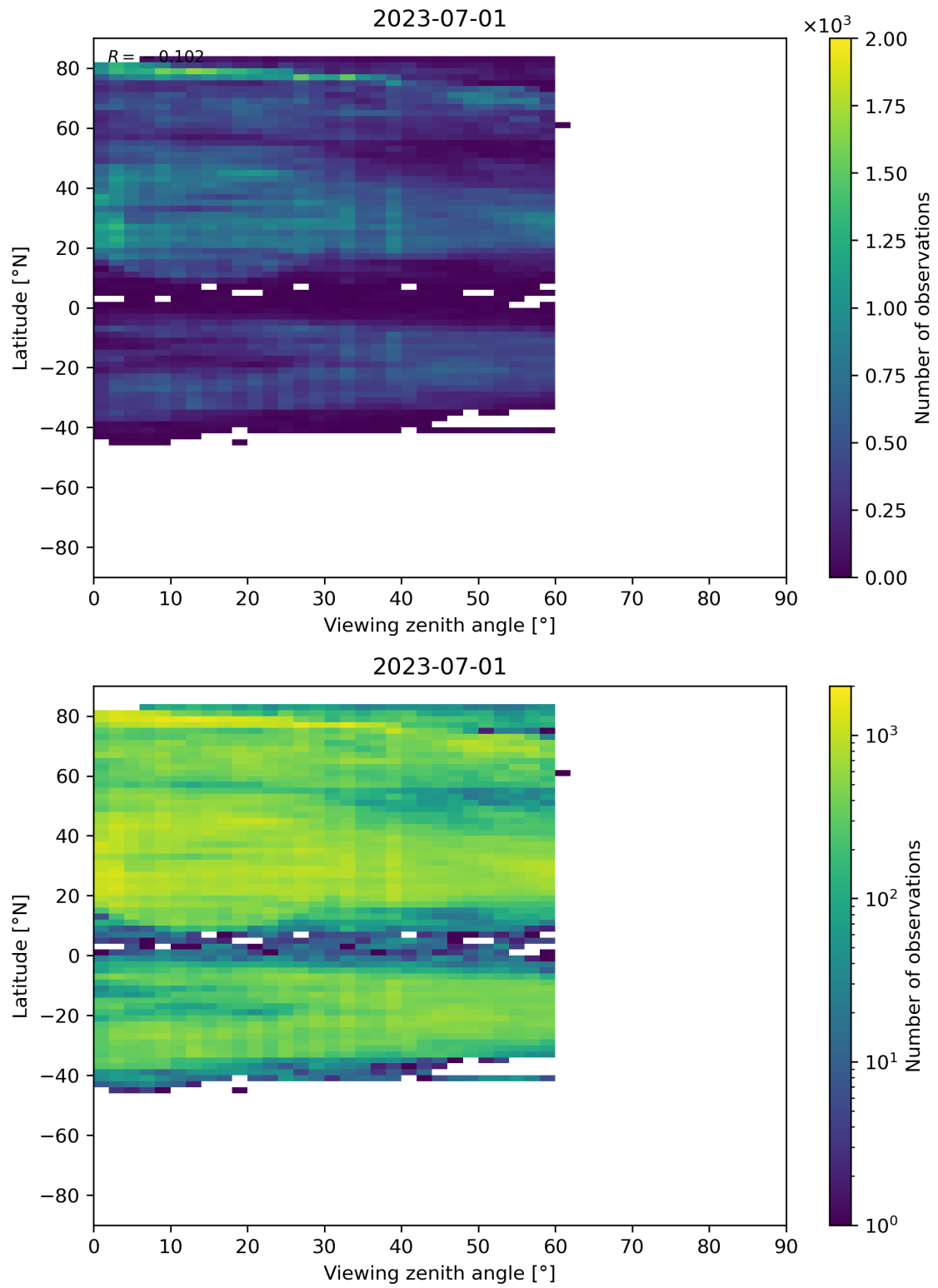
Figure 109: Scatter density plot of “Viewing zenith angle” against “Latitude” for 2023-06-30 to 2023-07-02.
