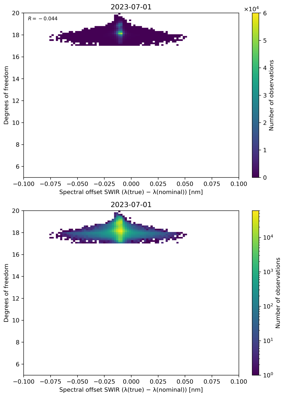
Figure 119: Scatter density plot of “Spectral offset SWIR ( \lambda(\text{true}) - \lambda(\text{nominal}) )” against “Degrees of freedom” for 2023-06-30 to 2023-07-02.
