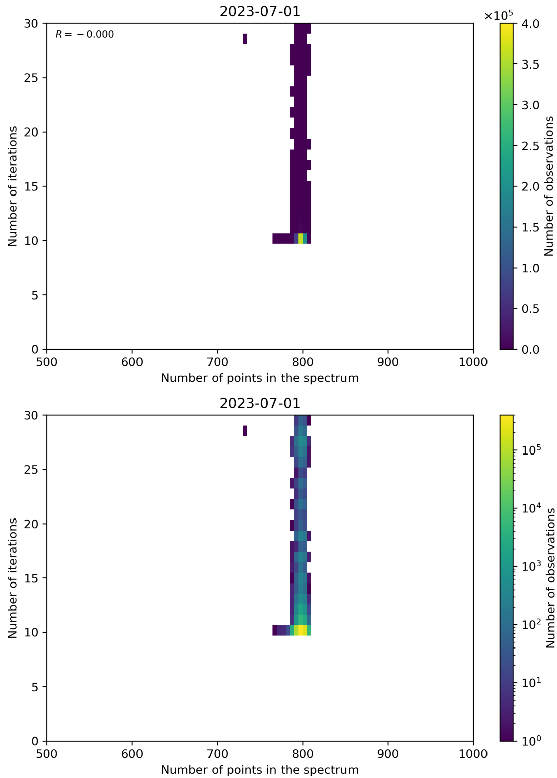
Figure 92: Scatter density plot of “Number of points in the spectrum” against “Number of iterations” for 2023-06-30 to 2023-07-02.
