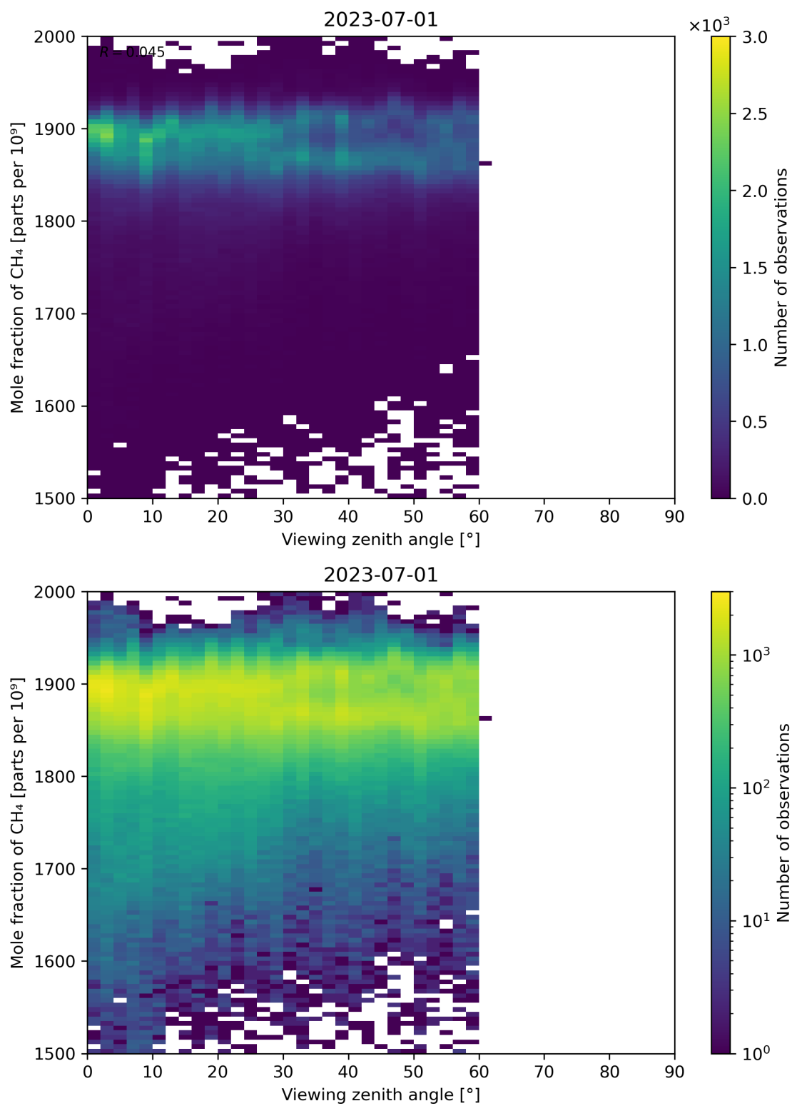
Figure 110: Scatter density plot of “Viewing zenith angle” against “Mole fraction of CH 4 ” for 2023-06-30 to 2023-07-02.
