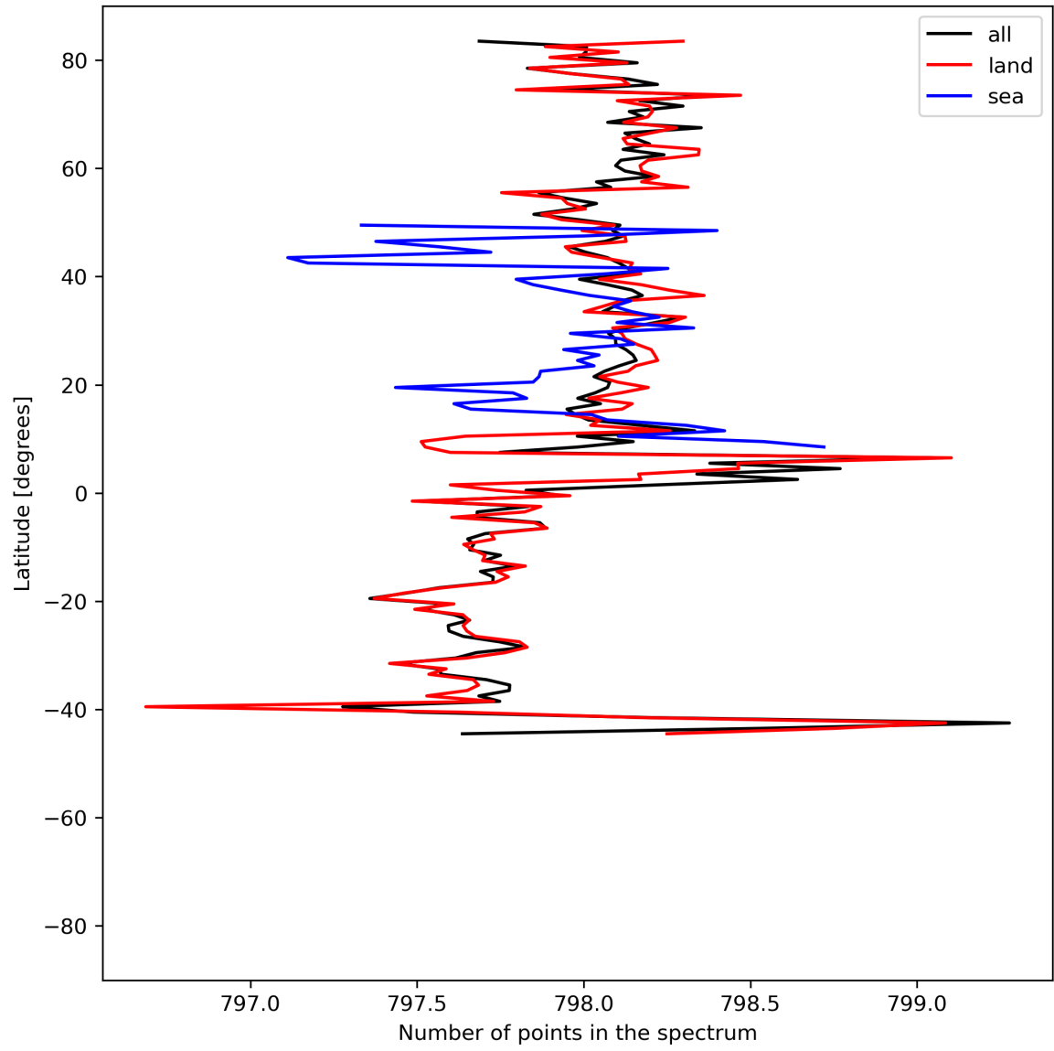
Figure 15: Zonal average of “Number of points in the spectrum” for 2023-06-30 to 2023-07-02.
