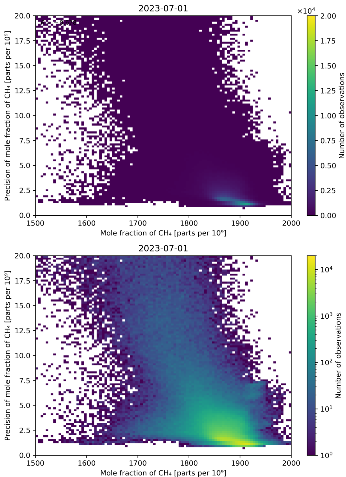
Figure 75: Scatter density plot of “Mole fraction of CH 4 ” against “Precision of mole fraction of CH 4 ” for 2023-06-30 to 2023-07-02.
