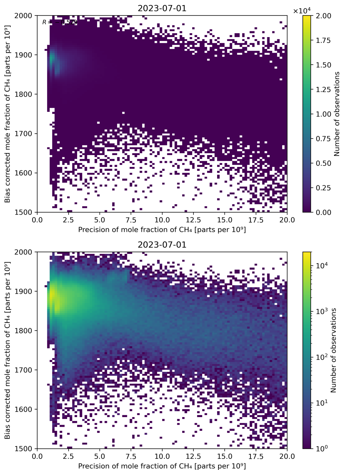
Figure 82: Scatter density plot of “Precision of mole fraction of CH 4 ” against “Bias corrected mole fraction of CH 4 ” for 2023-06-30 to 2023-07-02.
