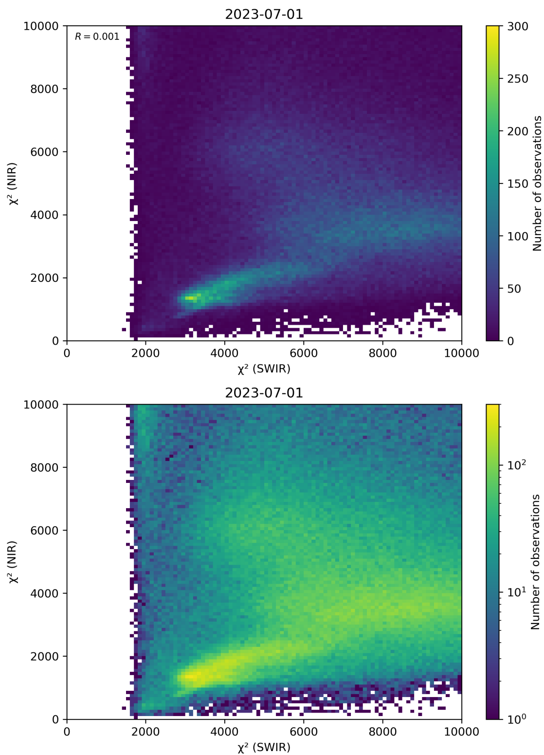
Figure 47: Scatter density plot of “ \chi^2 (SWIR)” against “ \chi^2 (NIR)” for 2023-06-30 to 2023-07-02.
