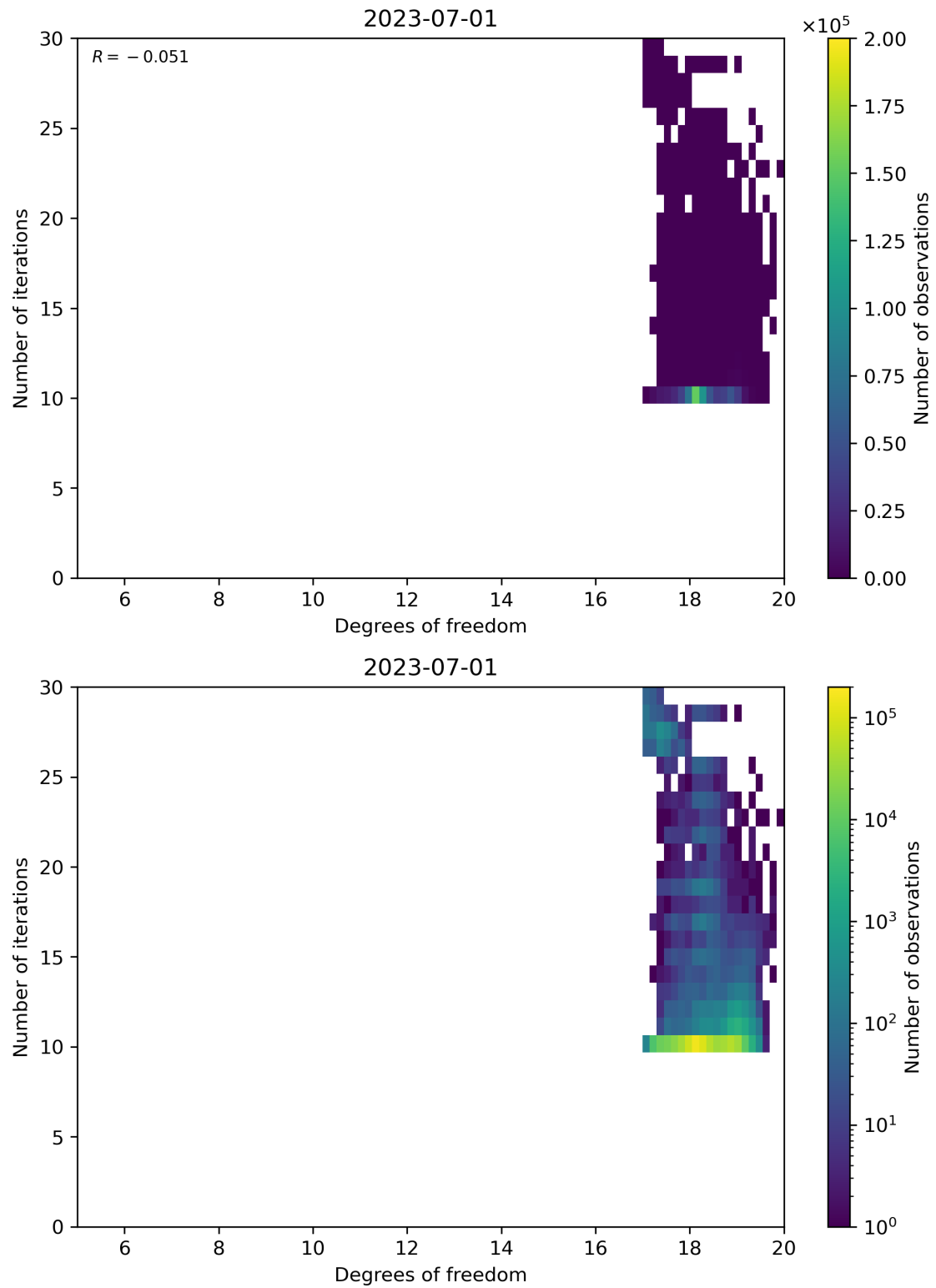
Figure 52: Scatter density plot of “Degrees of freedom” against “Number of iterations” for 2023-06-30 to 2023-07-02.
