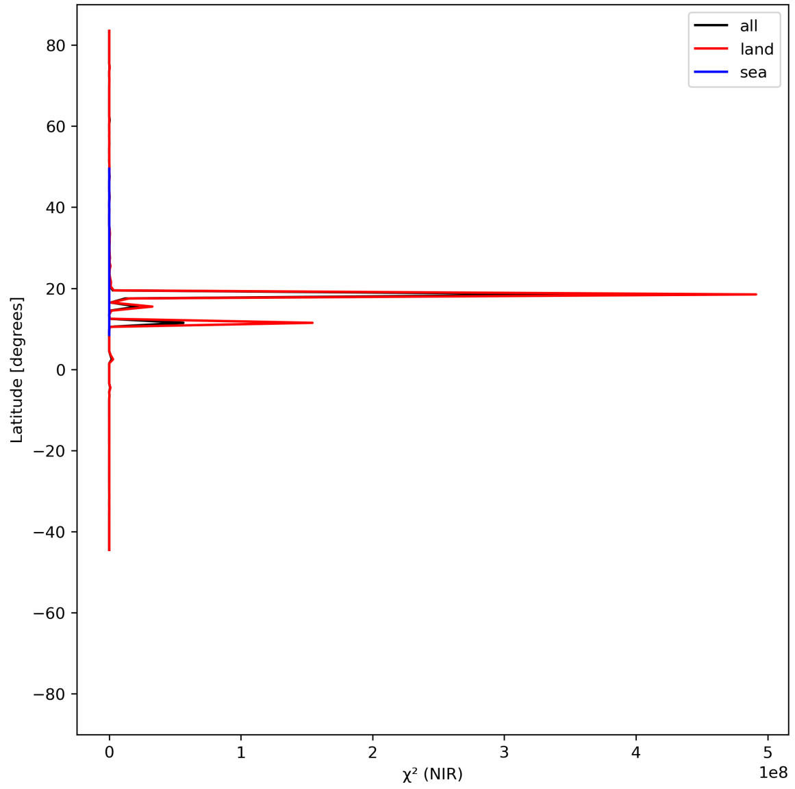
Figure 18: Zonal average of “ \chi^2 (NIR)” for 2023-06-30 to 2023-07-02.
