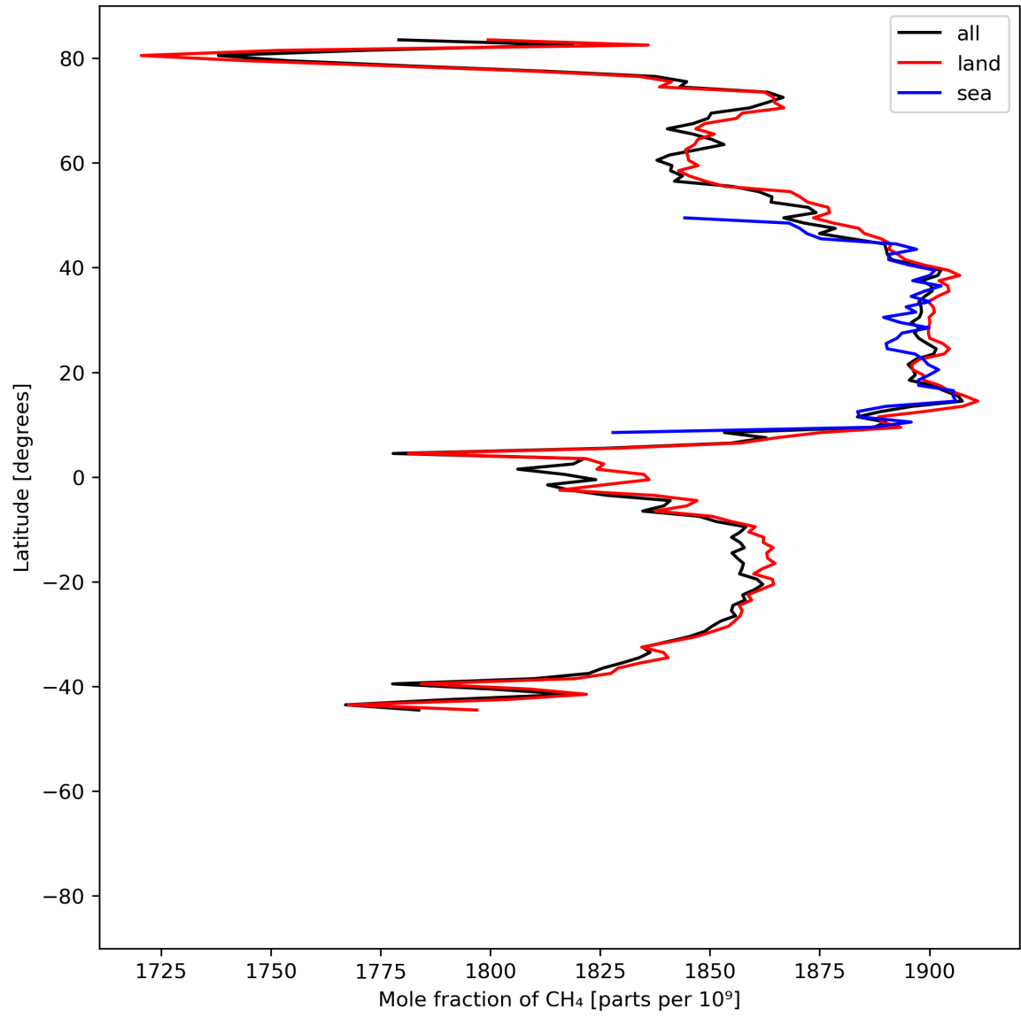
Figure 12: Zonal average of “Mole fraction of \text{CH}_4 ” for 2023-06-30 to 2023-07-02.
