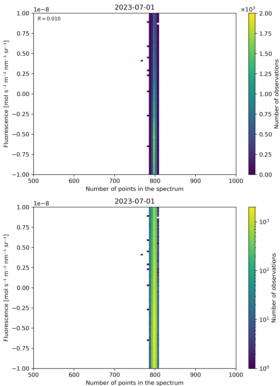
Figure 91: Scatter density plot of “Number of points in the spectrum” against “Fluorescence” for 2023-06-30 to 2023-07-02.
