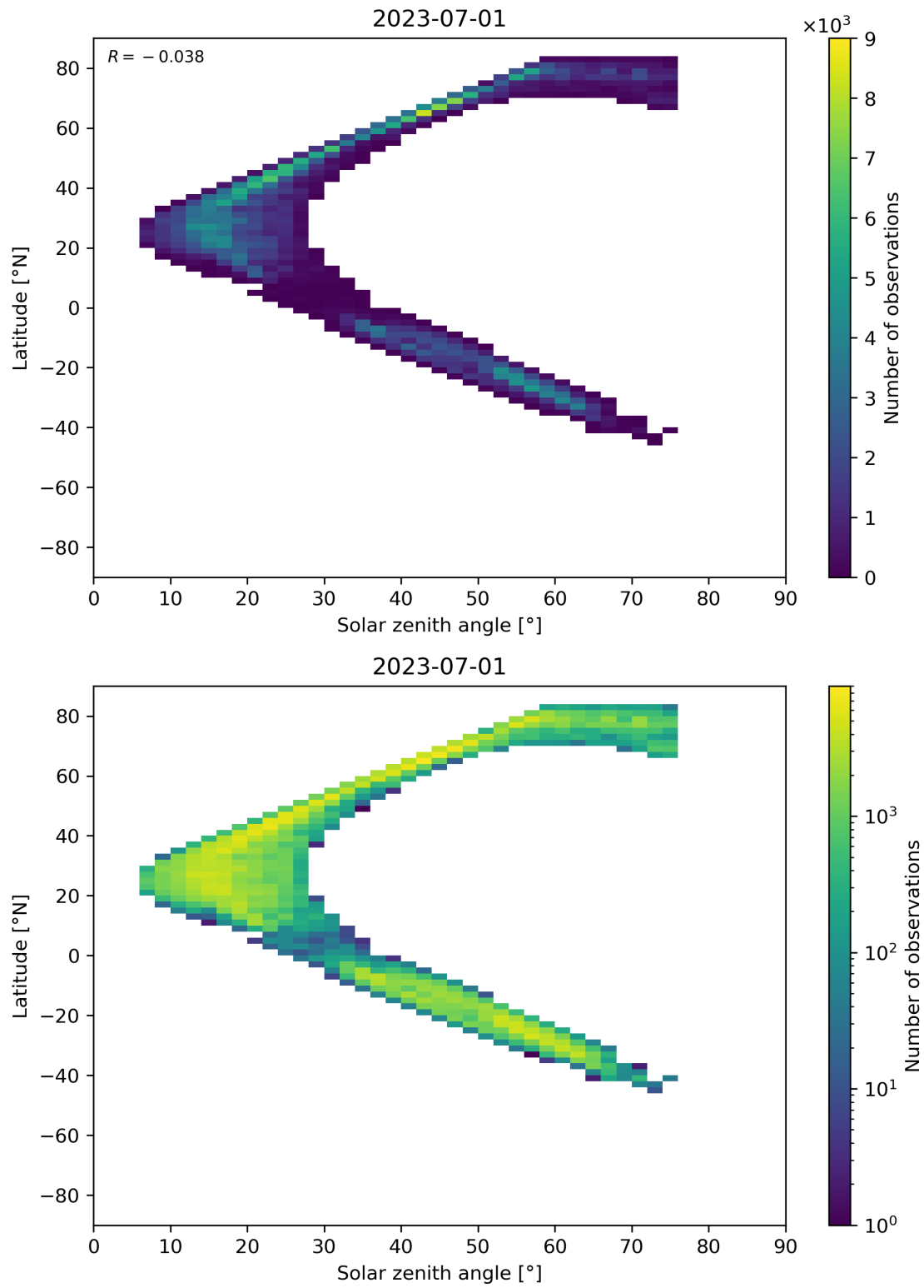
Figure 98: Scatter density plot of “Solar zenith angle” against “Latitude” for 2023-06-30 to 2023-07-02.
