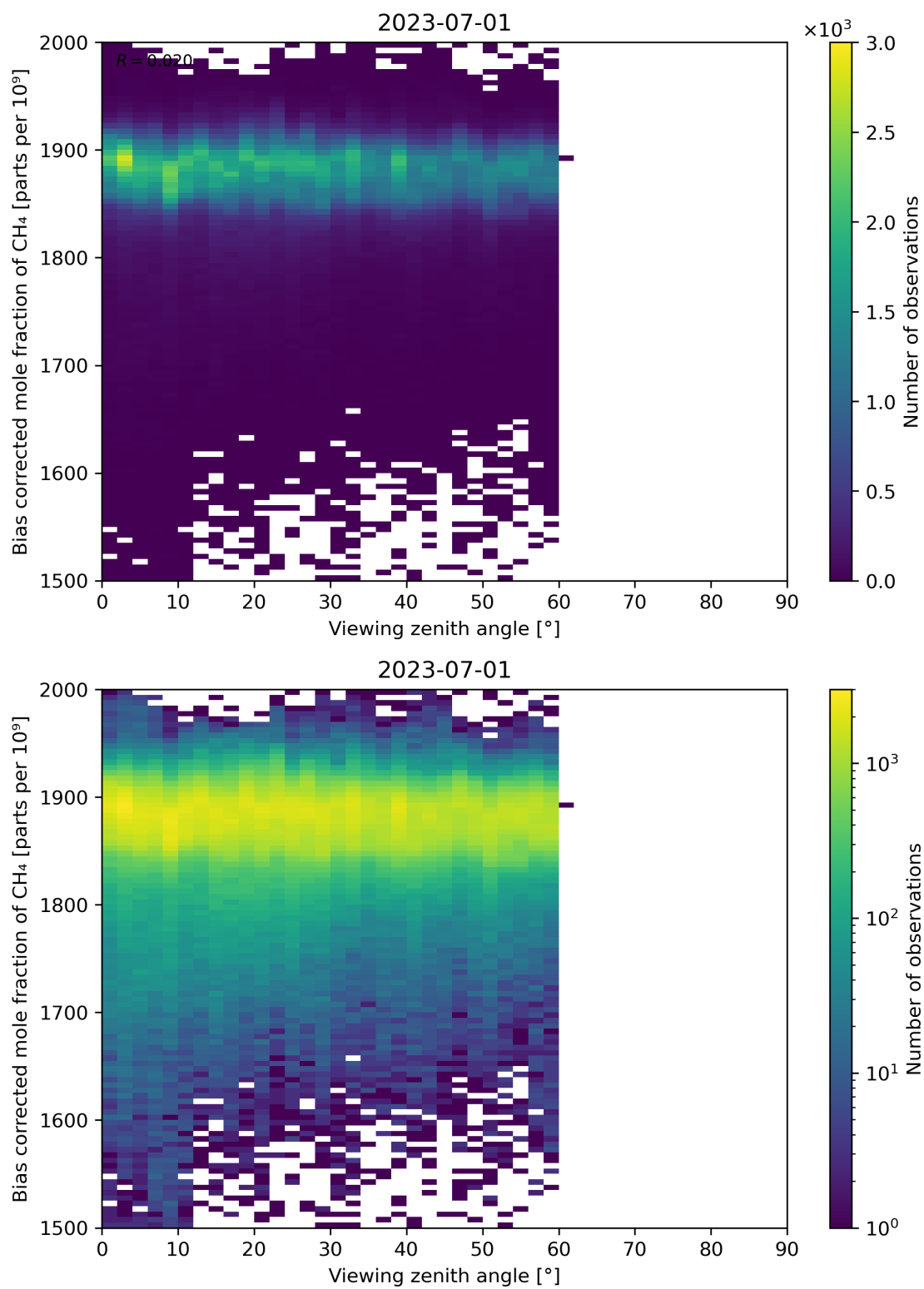
Figure 111: Scatter density plot of “Viewing zenith angle” against “Bias corrected mole fraction of CH 4 ” for 2023-06-30 to 2023-07-02.
