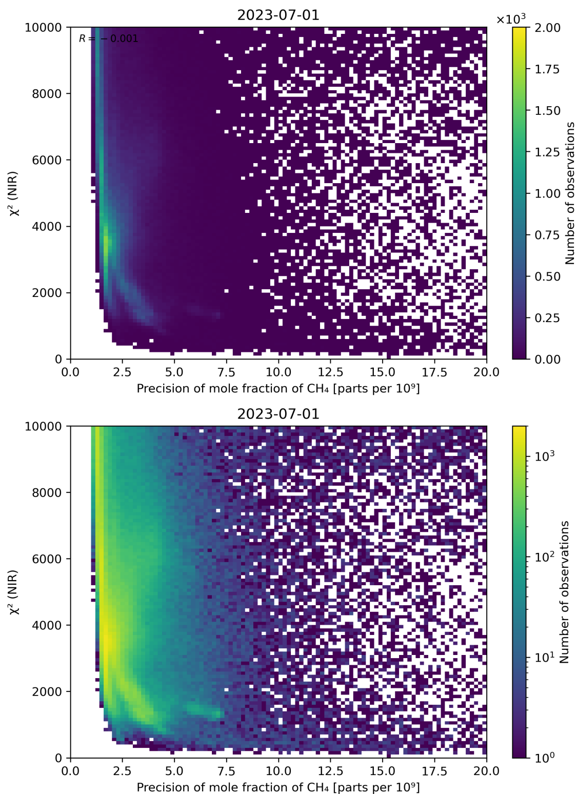
Figure 78: Scatter density plot of “Precision of mole fraction of CH 4 ” against “ \chi^2 (NIR)” for 2023-06-30 to 2023-07-02.
