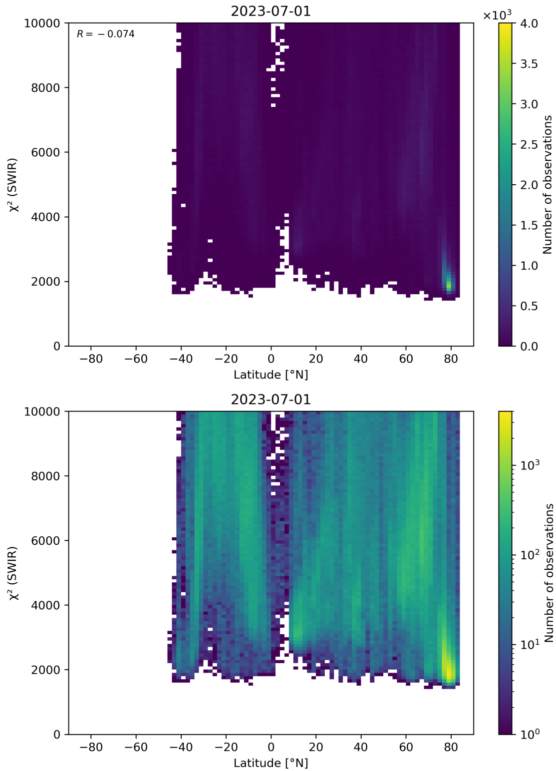
Figure 54: Scatter density plot of “Latitude” against “ \chi^2 (SWIR)” for 2023-06-30 to 2023-07-02.
