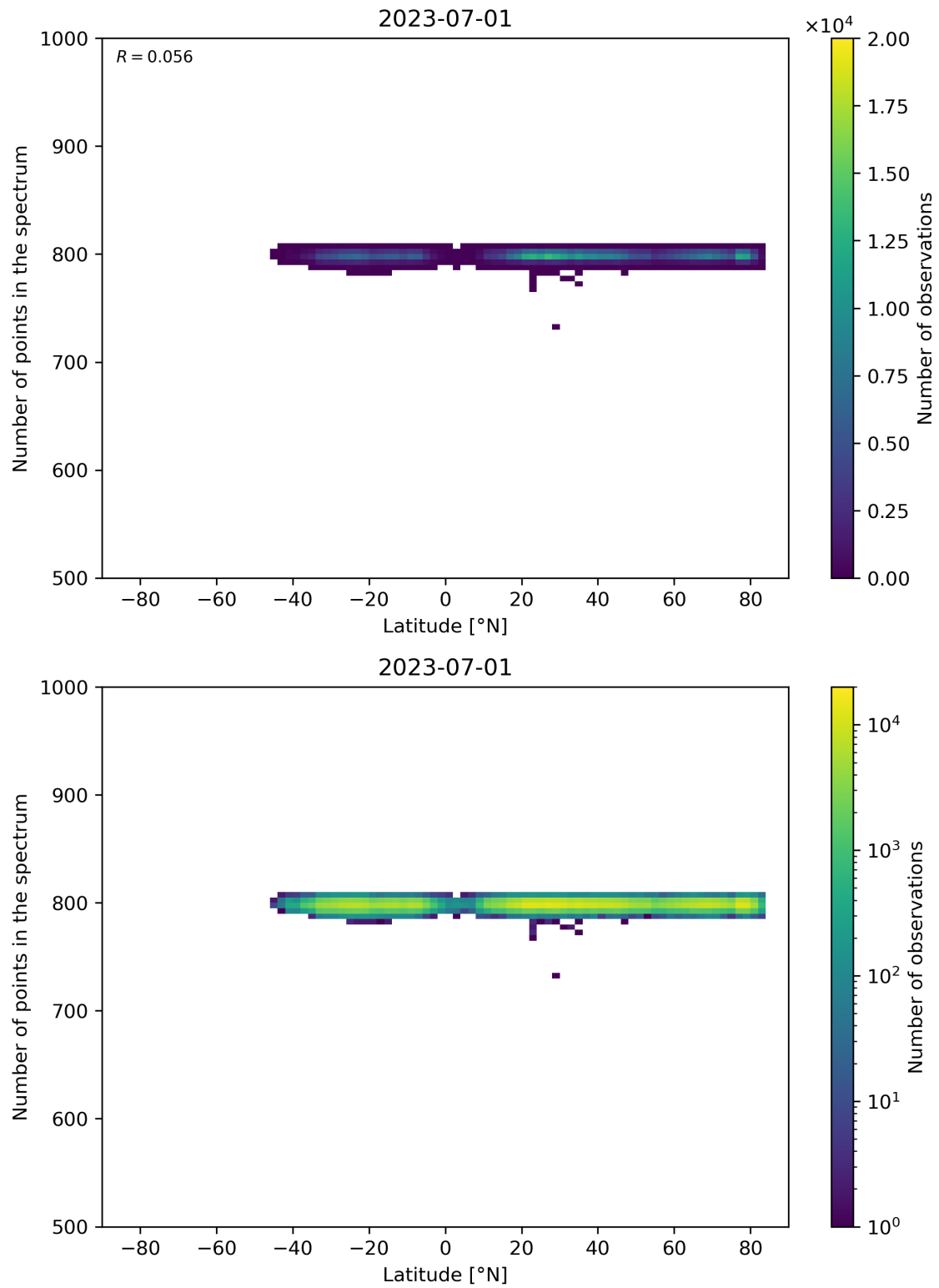
Figure 61: Scatter density plot of “Latitude” against “Number of points in the spectrum” for 2023-06-30 to 2023-07-02.
