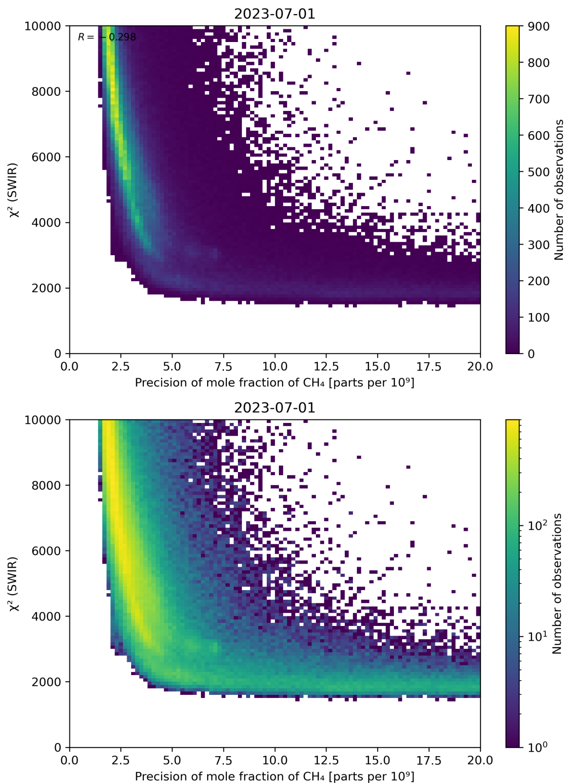
Figure 79: Scatter density plot of “Precision of mole fraction of \text{CH}_4 ” against “ \chi^2 (SWIR)” for 2023-06-30 to 2023-07-02.
