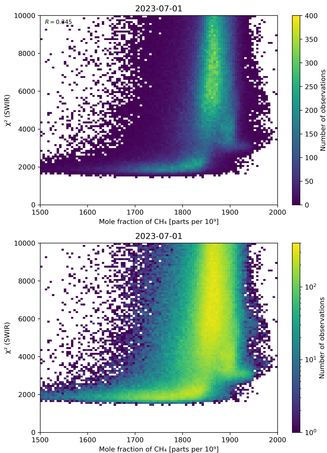
Figure 71: Scatter density plot of “Mole fraction of \text{CH}_4 ” against “ \chi^2 (SWIR)” for 2023-06-30 to 2023-07-02.
