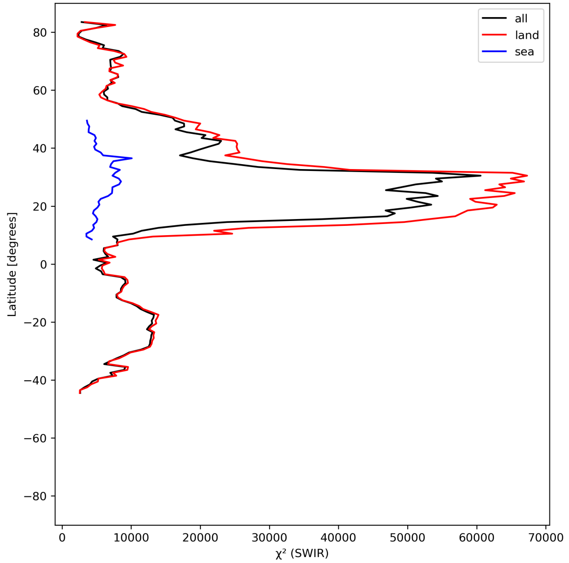
Figure 17: Zonal average of “ \chi^2 (SWIR)” for 2023-06-30 to 2023-07-02.
