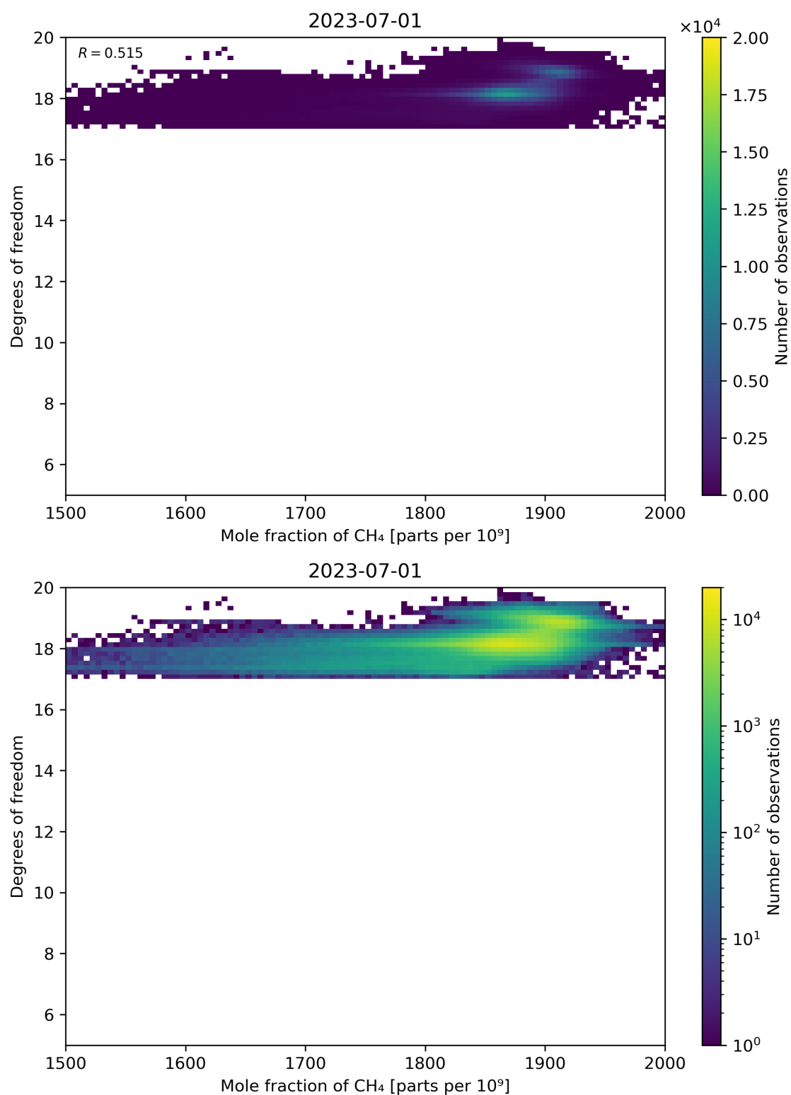
Figure 72: Scatter density plot of “Mole fraction of CH 4 ” against “Degrees of freedom” for 2023-06-30 to 2023-07-02.
