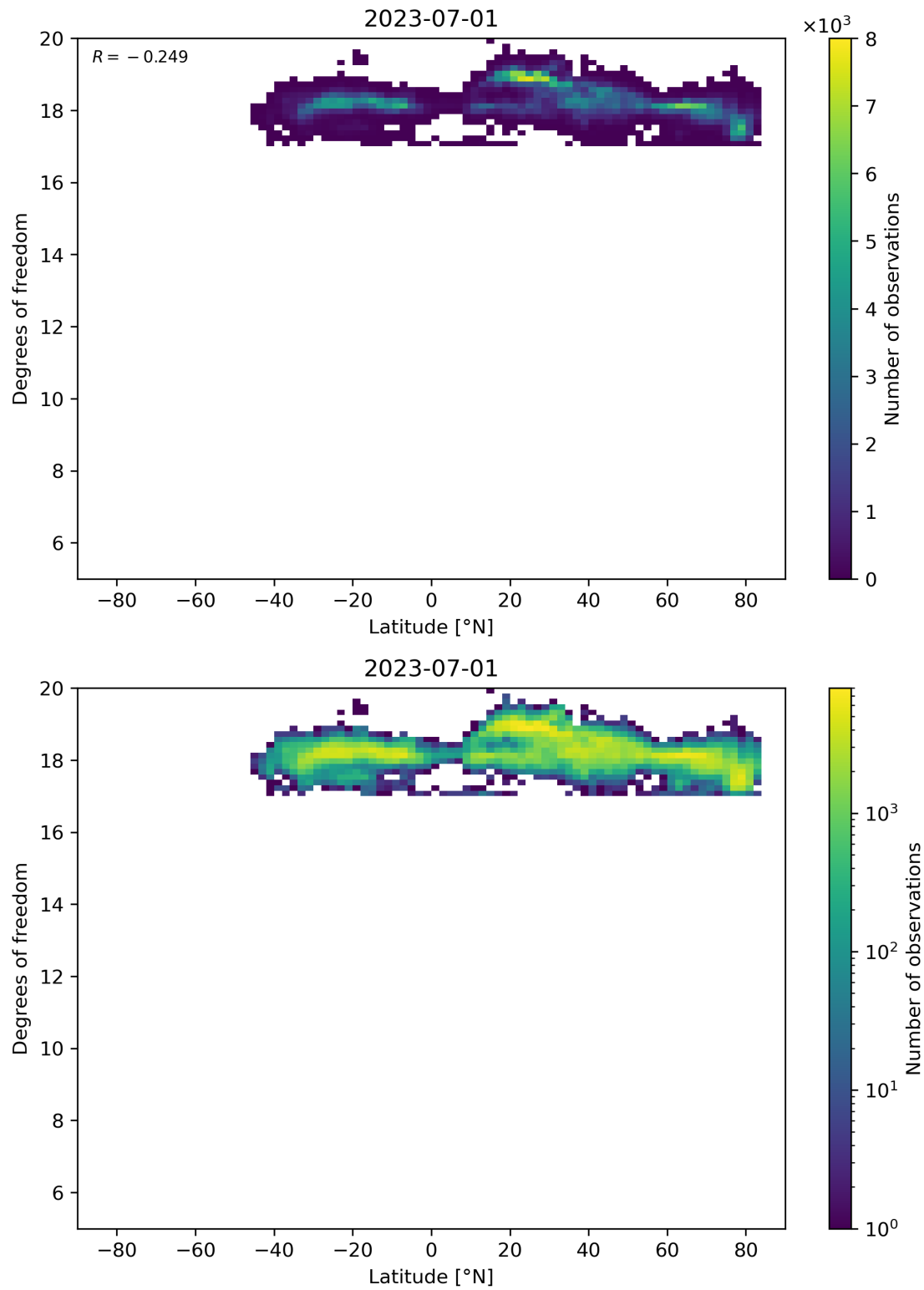
Figure 55: Scatter density plot of “Latitude” against “Degrees of freedom” for 2023-06-30 to 2023-07-02.
