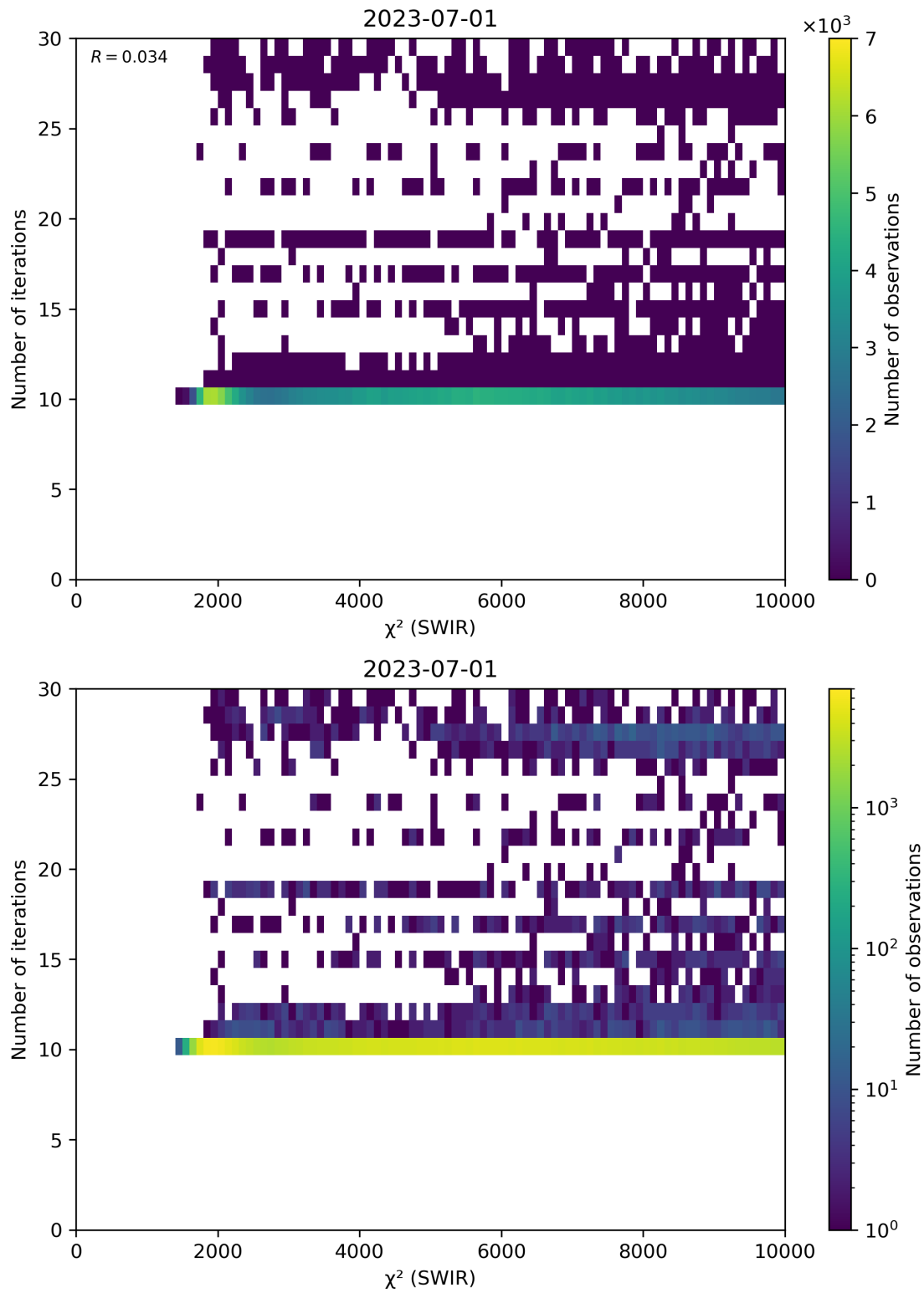
Figure 50: Scatter density plot of “ \chi^2 (SWIR)” against “Number of iterations” for 2023-06-30 to 2023-07-02.
