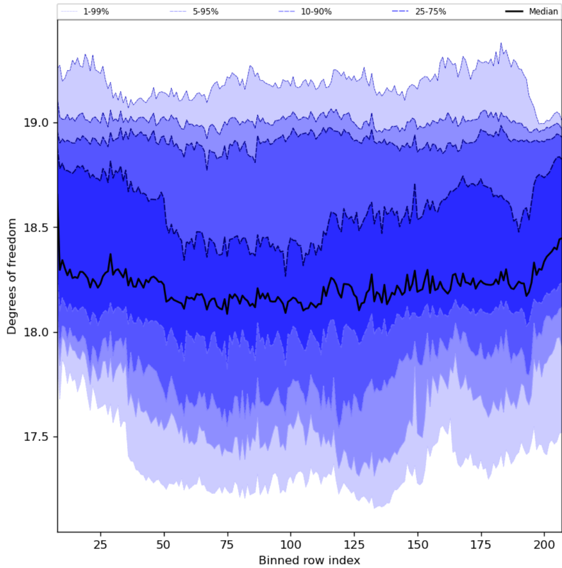
Figure 41: Along track statistics of “Degrees of freedom” for 2023-06-30 to 2023-07-02
