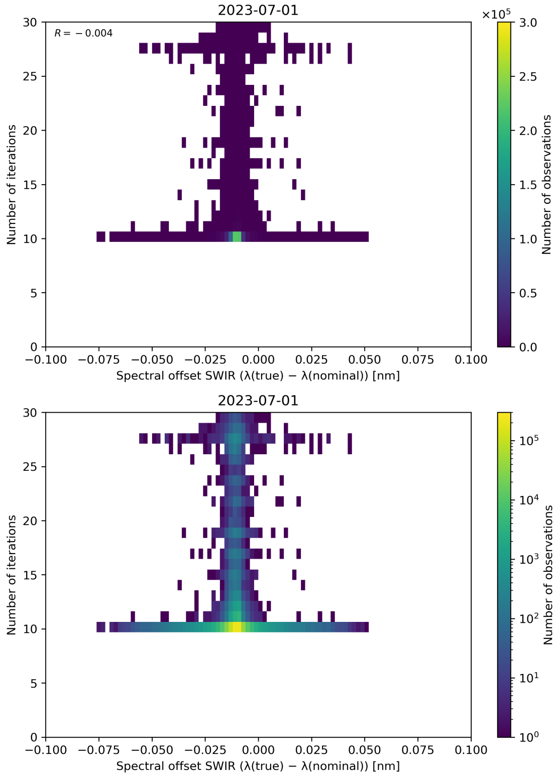
Figure 121: Scatter density plot of “Spectral offset SWIR ( \lambda(\text{true}) - \lambda(\text{nominal}) )” against “Number of iterations” for 2023-06-30 to 2023-07-02.
