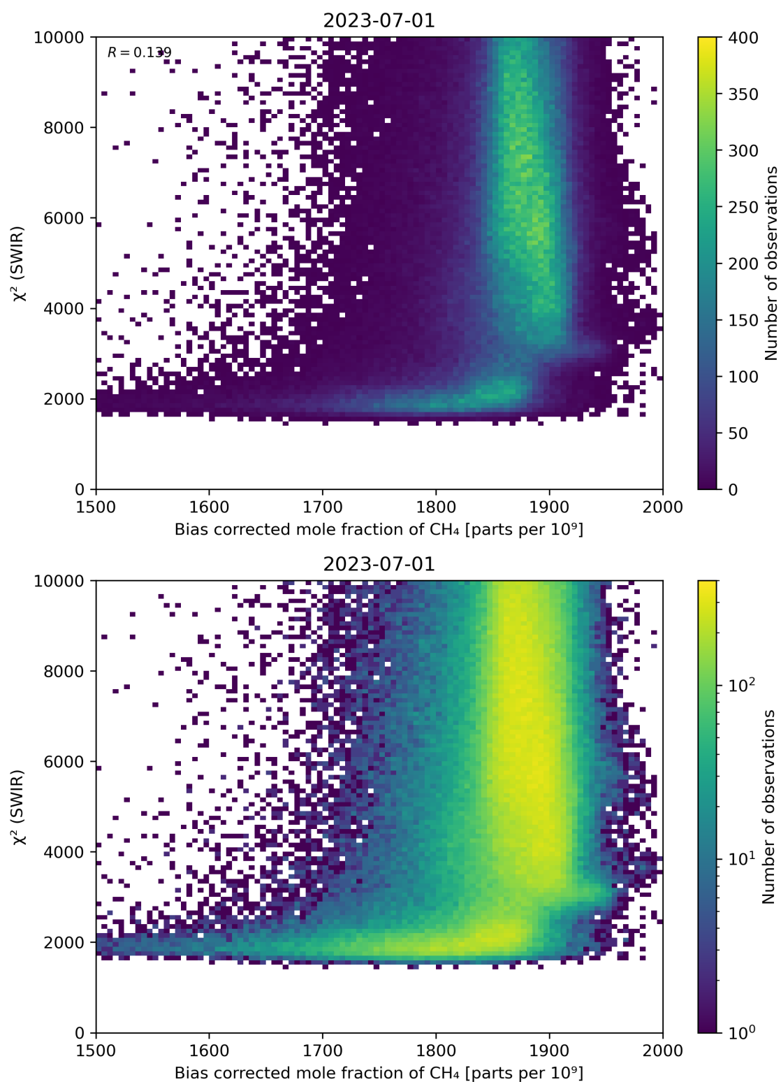
Figure 64: Scatter density plot of “Bias corrected mole fraction of CH 4 ” against “ \chi^2 (SWIR)” for 2023-06-30 to 2023-07-02.
