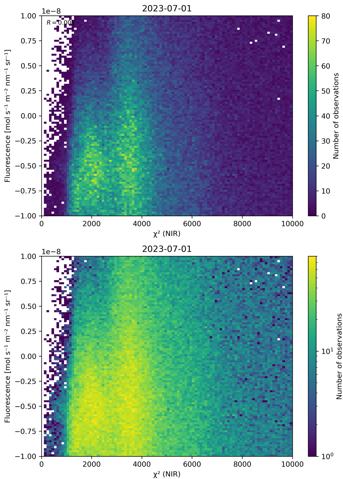
Figure 45: Scatter density plot of “ \chi^2 (NIR)” against “Fluorescence” for 2023-06-30 to 2023-07-02.
