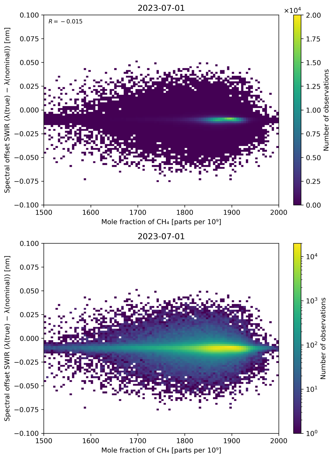
Figure 86: Scatter density plot of “Mole fraction of CH 4 ” against “Spectral offset SWIR ( \lambda(\text{true}) - \lambda(\text{nominal}) )” for 2023-06-30 to 2023-07-02.
