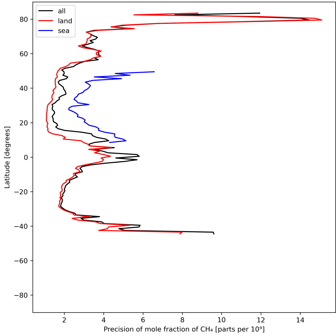
Figure 13: Zonal average of “Precision of mole fraction of CH 4 ” for 2023-06-30 to 2023-07-02.
