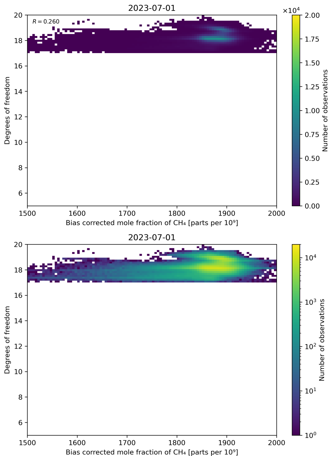
Figure 65: Scatter density plot of “Bias corrected mole fraction of CH 4 ” against “Degrees of freedom” for 2023-06-30 to 2023-07-02.
