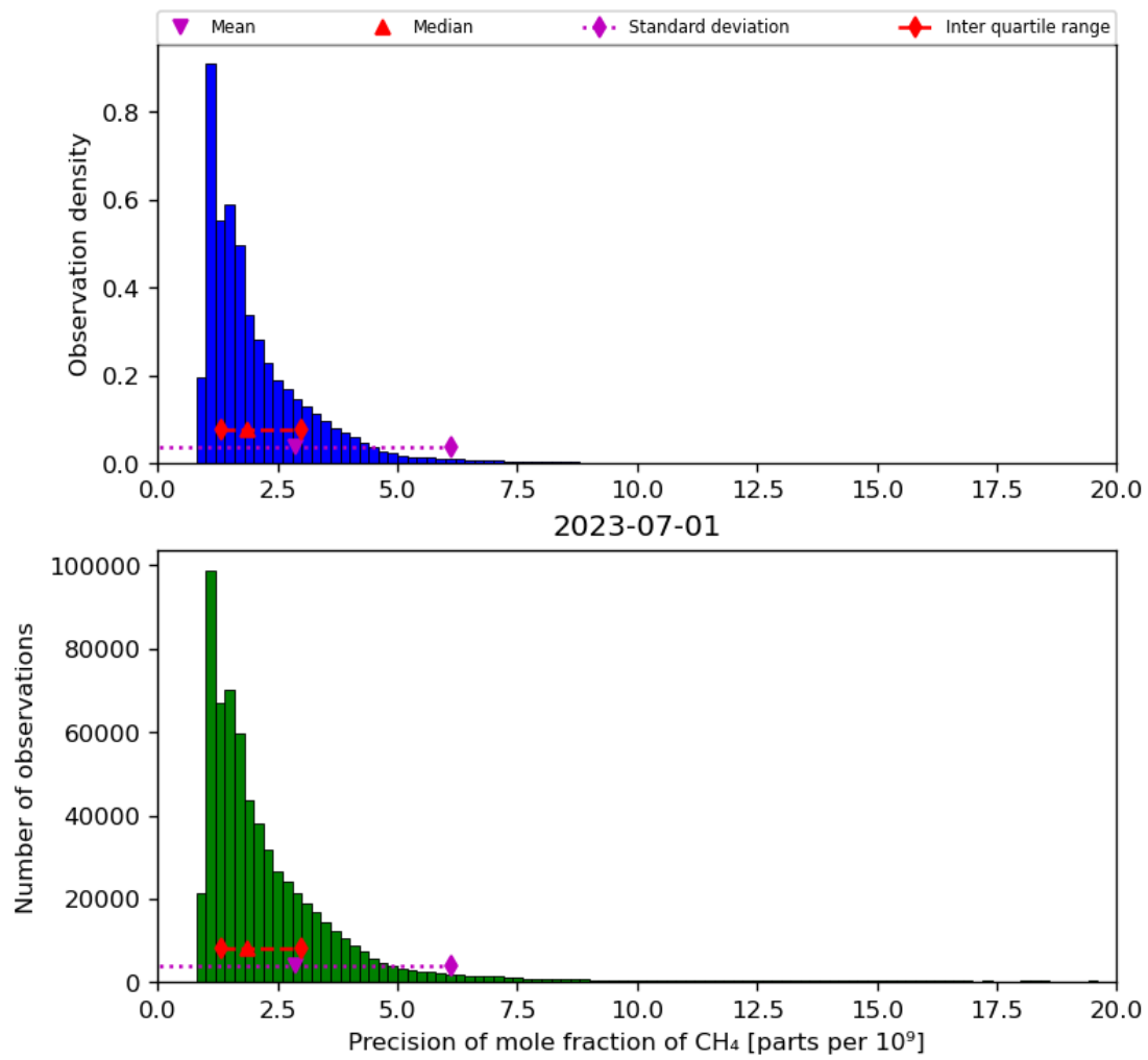
Figure 24: Histogram of “Precision of mole fraction of CH 4 ” for 2023-06-30 to 2023-07-02
