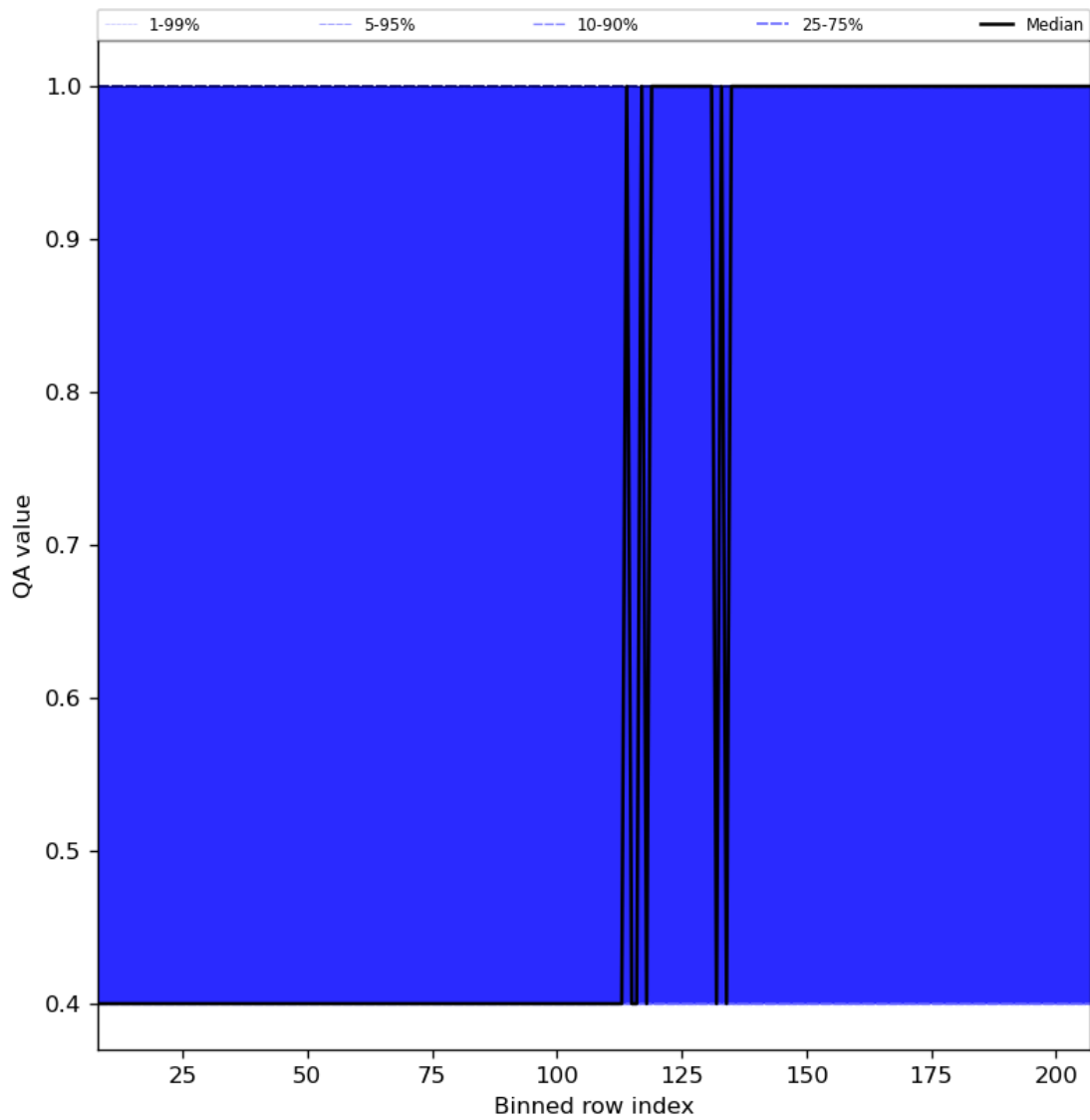
Figure 33: Along track statistics of “QA value” for 2023-06-30 to 2023-07-02
