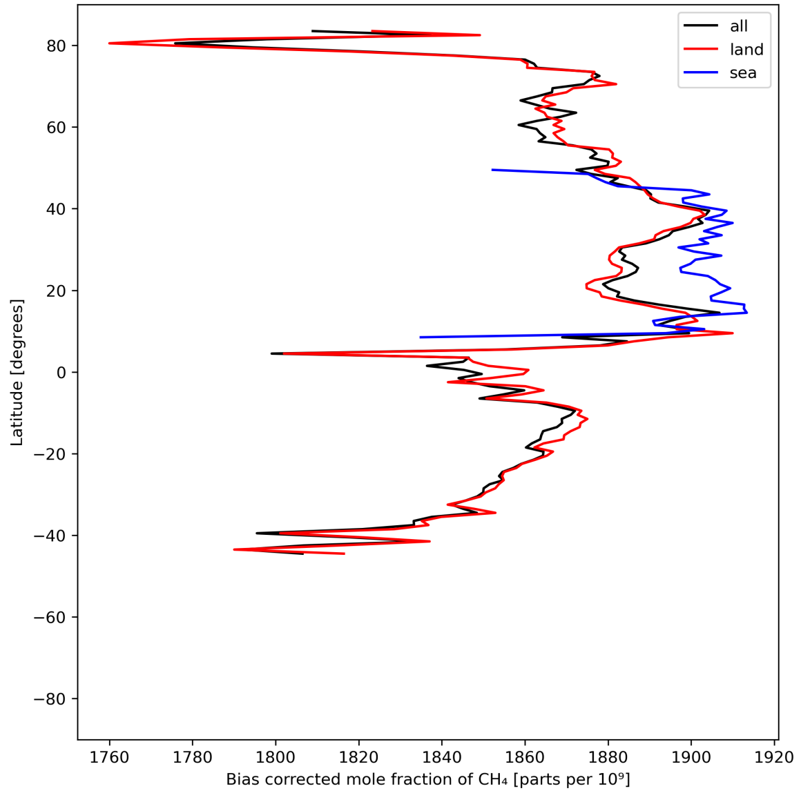
Figure 14: Zonal average of “Bias corrected mole fraction of CH 4 ” for 2023-06-30 to 2023-07-02.
