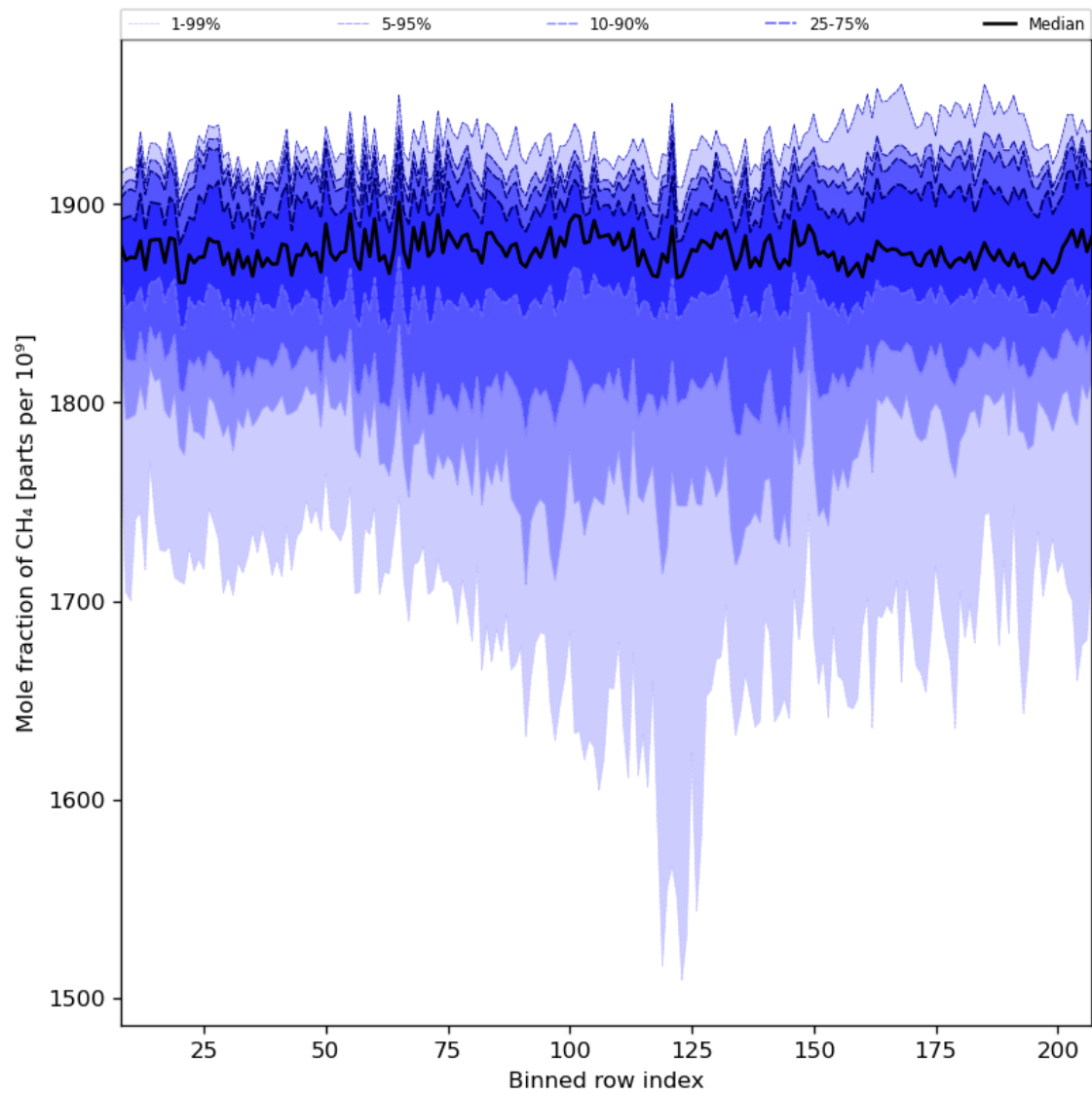
Figure 34: Along track statistics of “Mole fraction of CH 4 ” for 2023-06-30 to 2023-07-02
