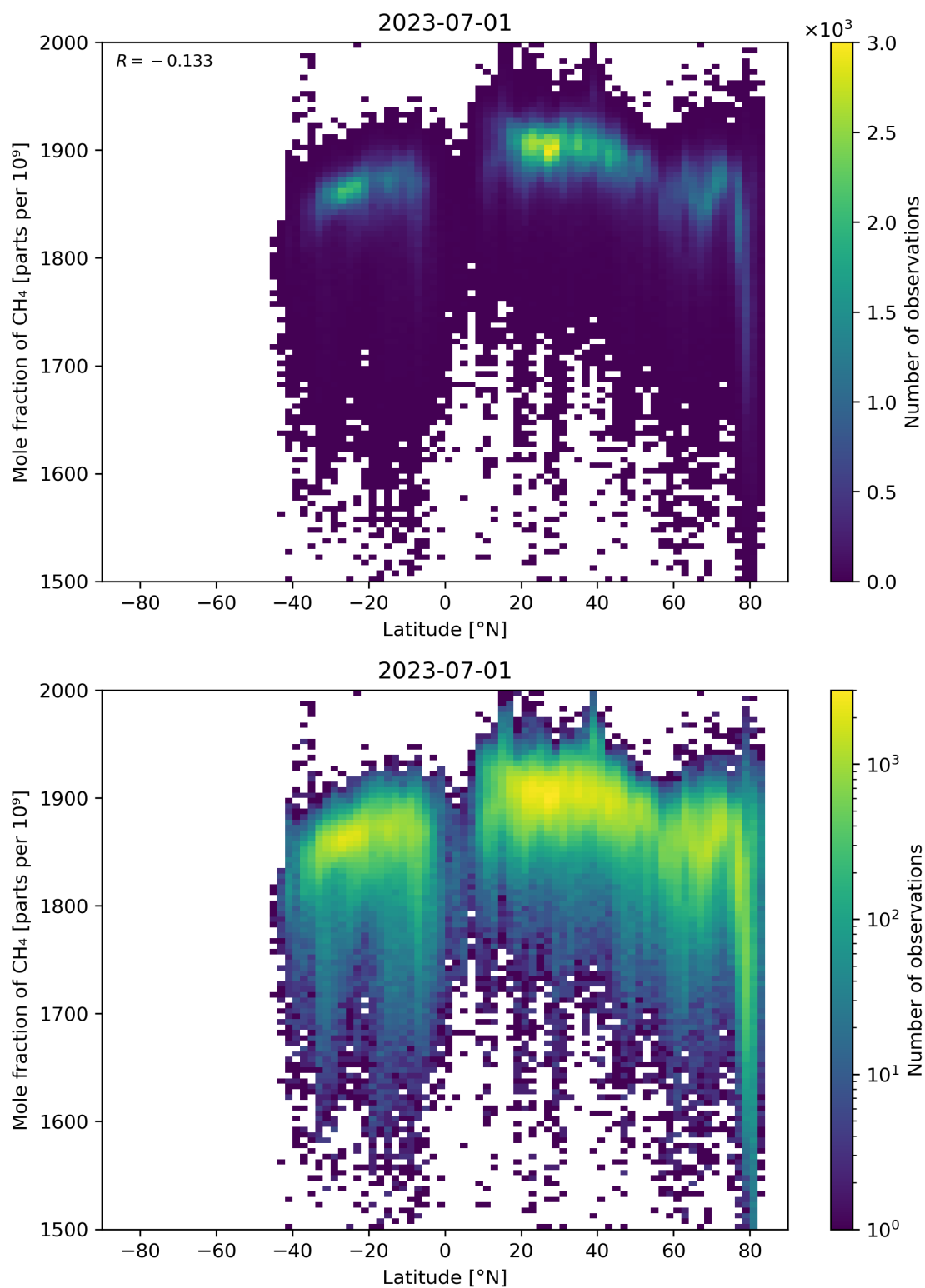
Figure 57: Scatter density plot of “Latitude” against “Mole fraction of CH 4 ” for 2023-06-30 to 2023-07-02.
