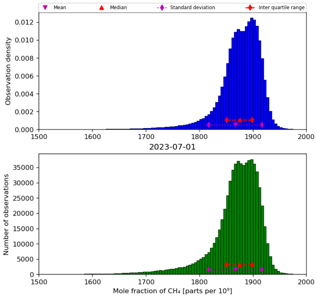
Figure 23: Histogram of “Mole fraction of CH 4 ” for 2023-06-30 to 2023-07-02
