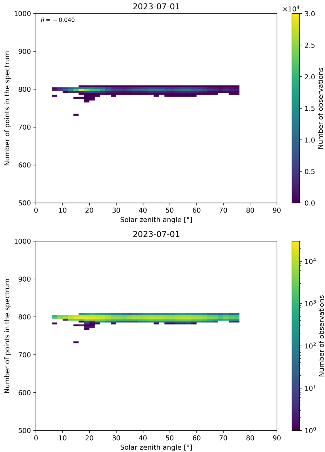
Figure 103: Scatter density plot of “Solar zenith angle” against “Number of points in the spectrum” for 2023-06-30 to 2023-07-02.
