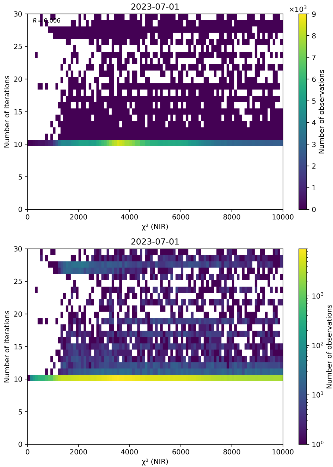
Figure 46: Scatter density plot of “ \chi^2 (NIR)” against “Number of iterations” for 2023-06-30 to 2023-07-02.
