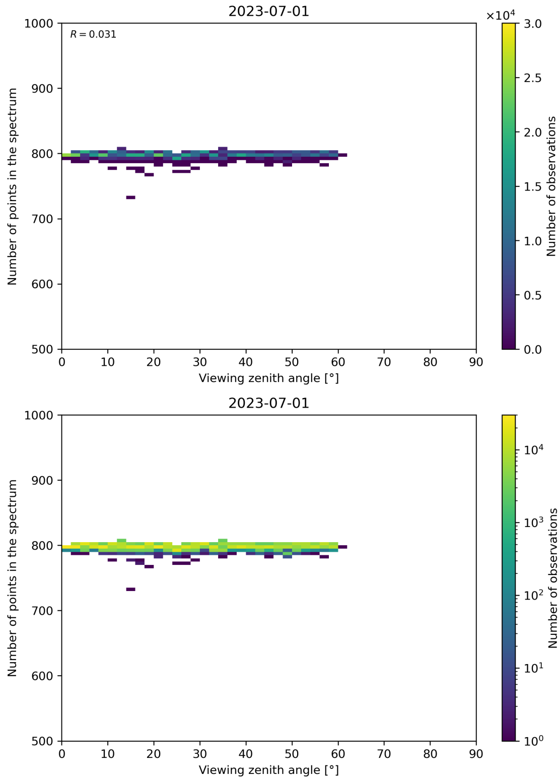
Figure 114: Scatter density plot of “Viewing zenith angle” against “Number of points in the spectrum” for 2023-06-30 to 2023-07-02.
