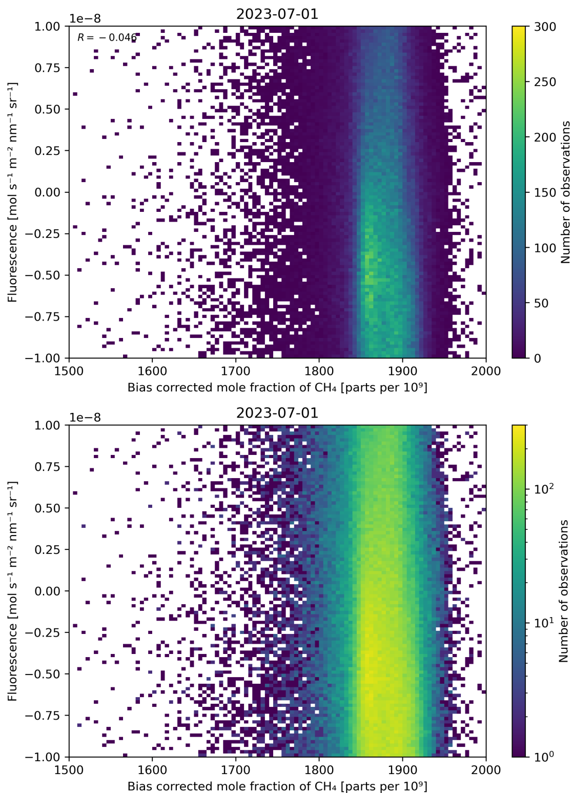
Figure 66: Scatter density plot of “Bias corrected mole fraction of \text{CH}_4 ” against “Fluorescence” for 2023-06-30 to 2023-07-02.
