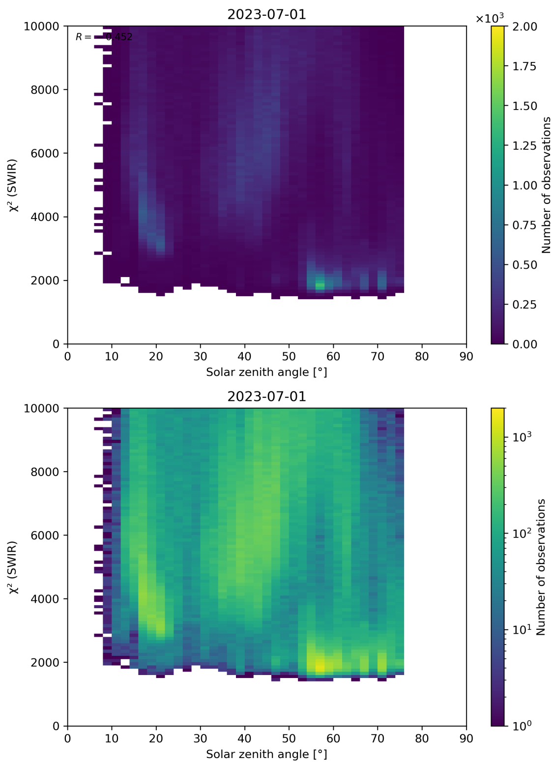
Figure 95: Scatter density plot of “Solar zenith angle” against “ \chi^2 (SWIR)” for 2023-06-30 to 2023-07-02.
