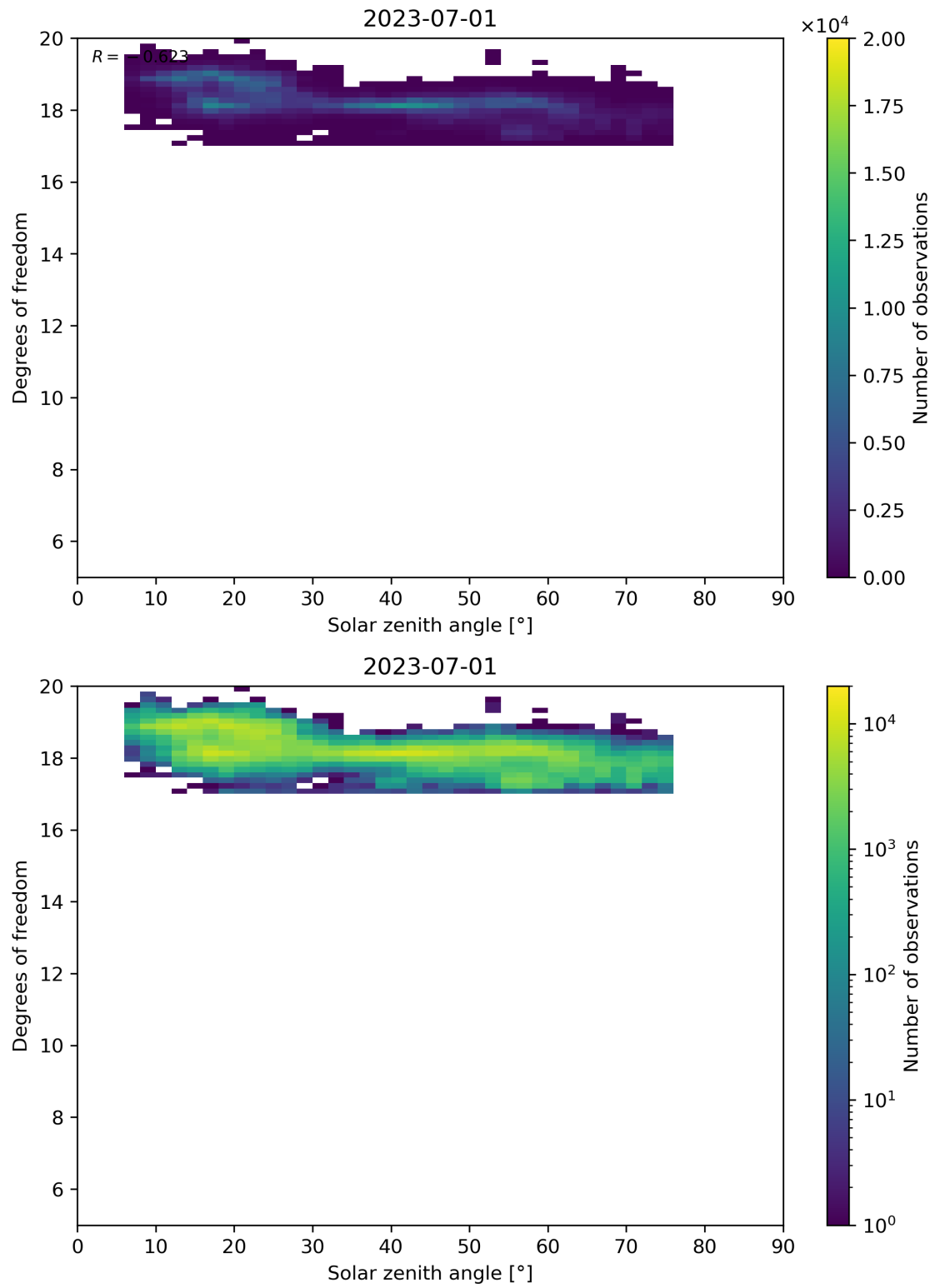
Figure 96: Scatter density plot of “Solar zenith angle” against “Degrees of freedom” for 2023-06-30 to 2023-07-02.
