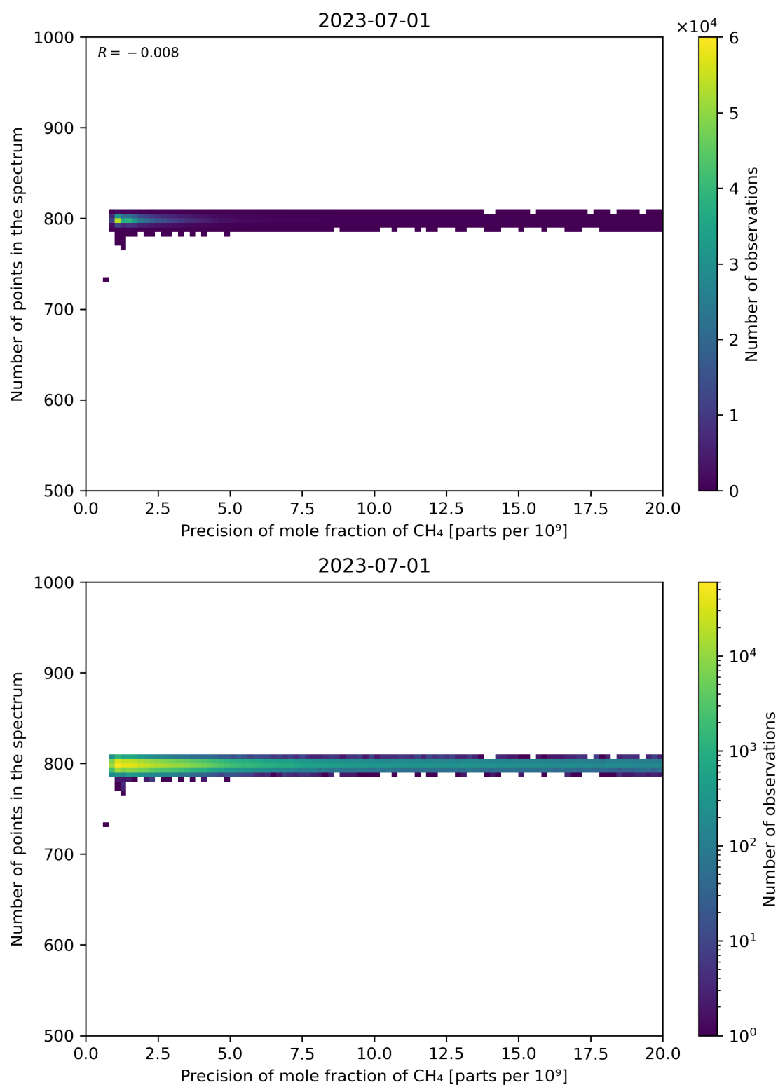
Figure 84: Scatter density plot of “Precision of mole fraction of CH 4 ” against “Number of points in the spectrum” for 2023-06-30 to 2023-07-02.
