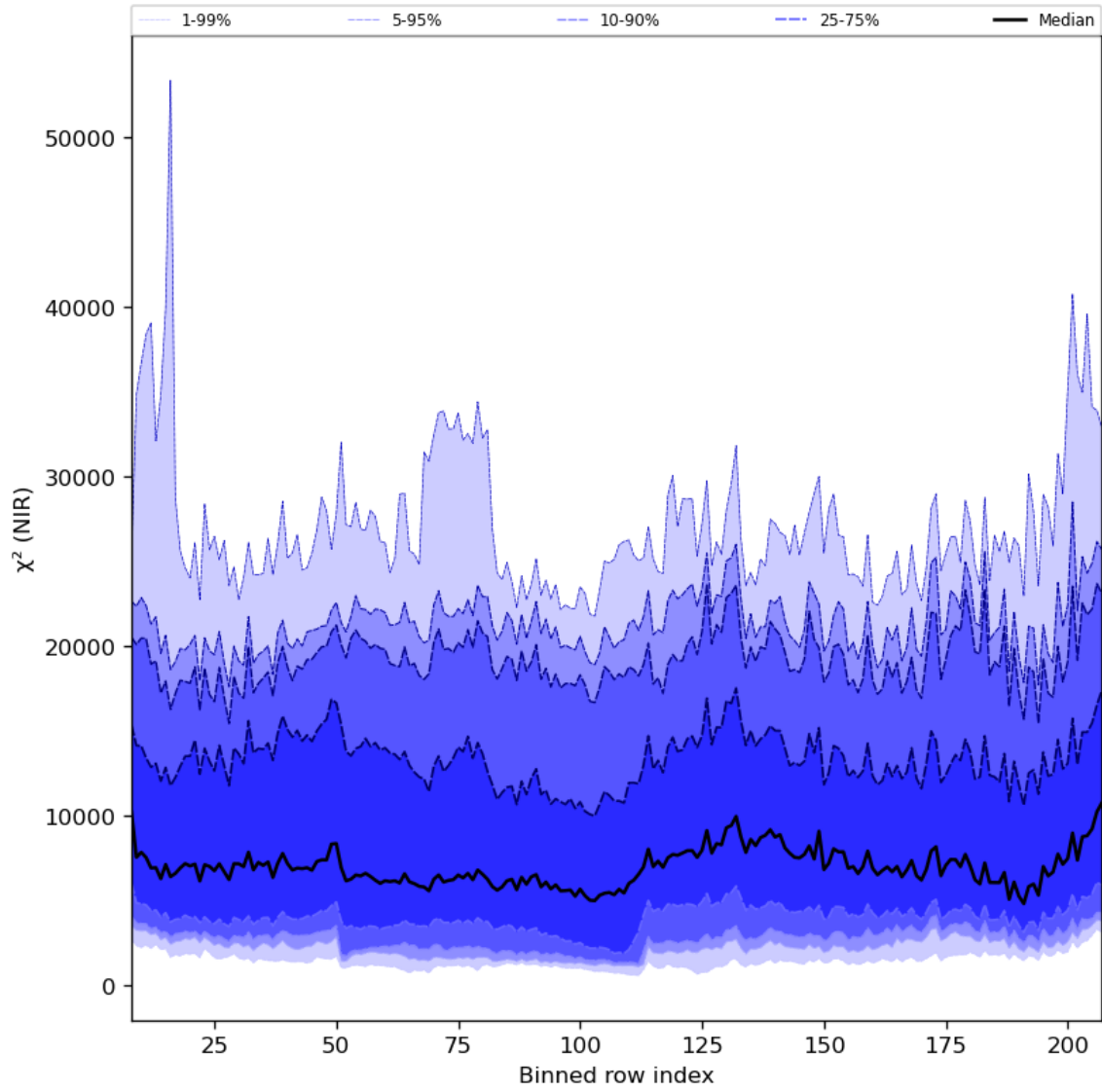
Figure 40: Along track statistics of " \chi^2 (NIR)" for 2023-06-30 to 2023-07-02
