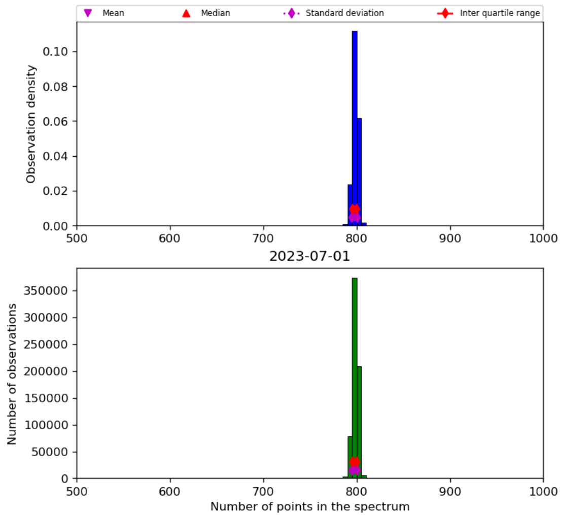
Figure 26: Histogram of “Number of points in the spectrum” for 2023-06-30 to 2023-07-02
