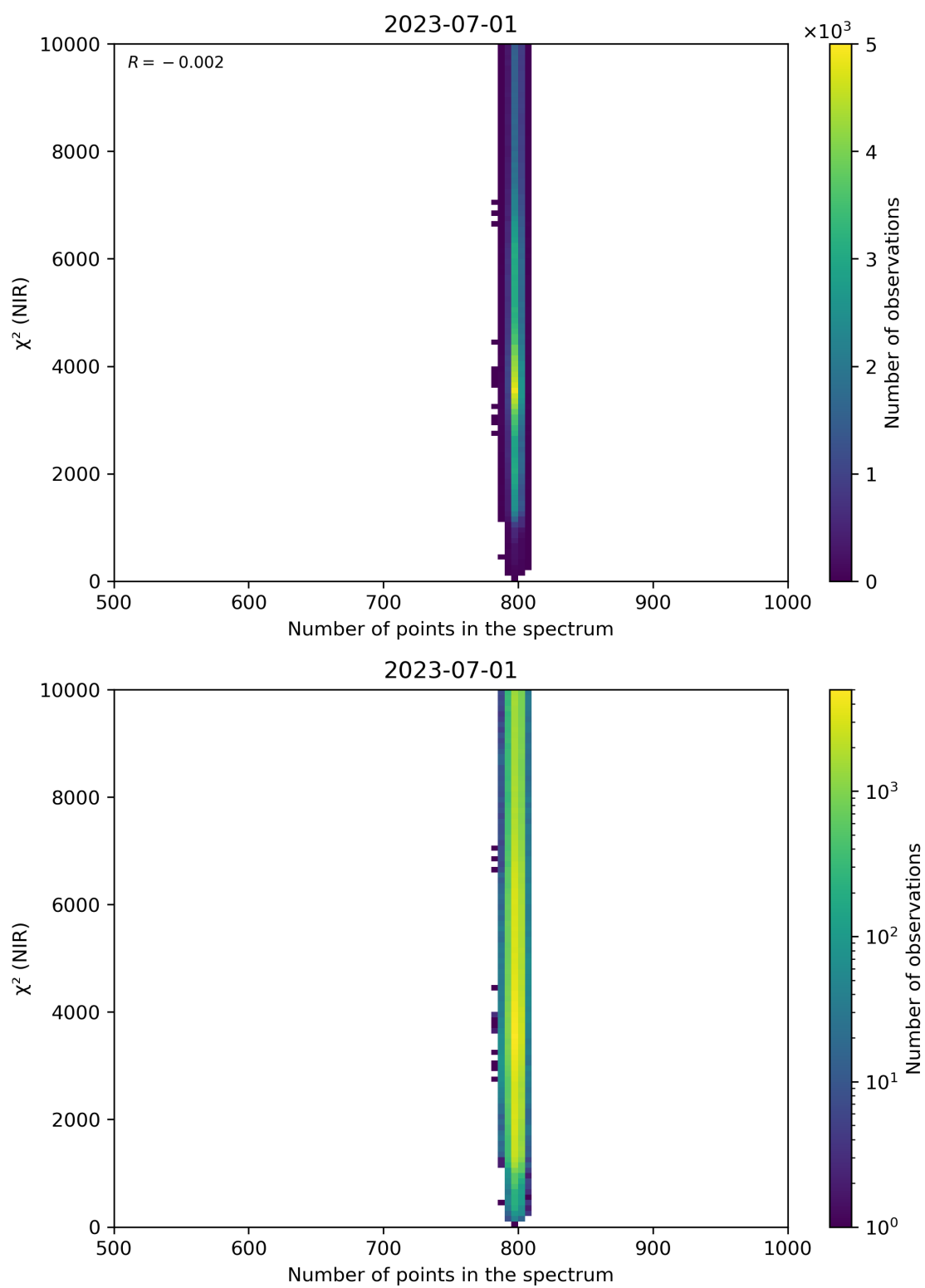
Figure 88: Scatter density plot of “Number of points in the spectrum” against “ \chi^2 (NIR)” for 2023-06-30 to 2023-07-02.
