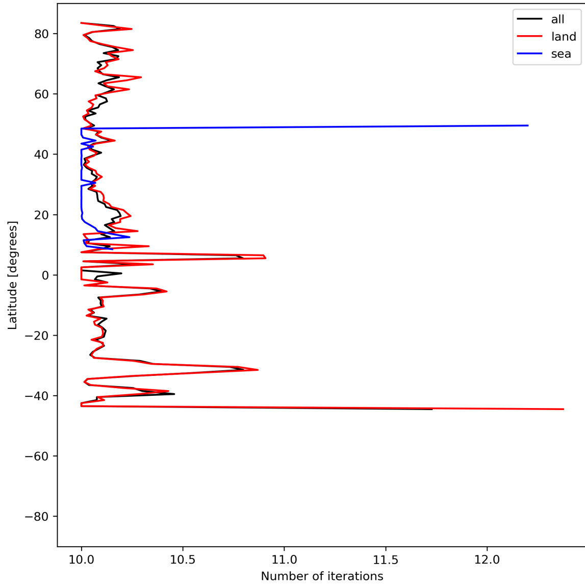
Figure 20: Zonal average of “Number of iterations” for 2023-06-30 to 2023-07-02.
