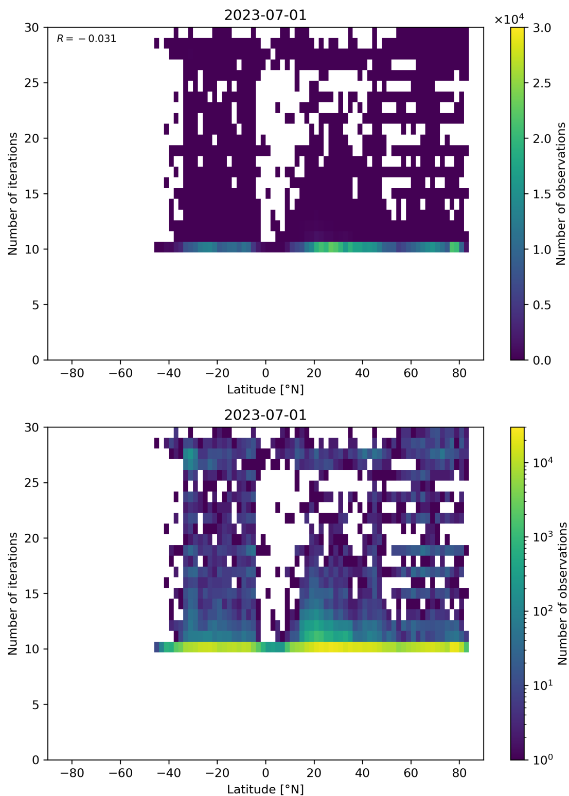
Figure 60: Scatter density plot of “Latitude” against “Number of iterations” for 2023-06-30 to 2023-07-02.
