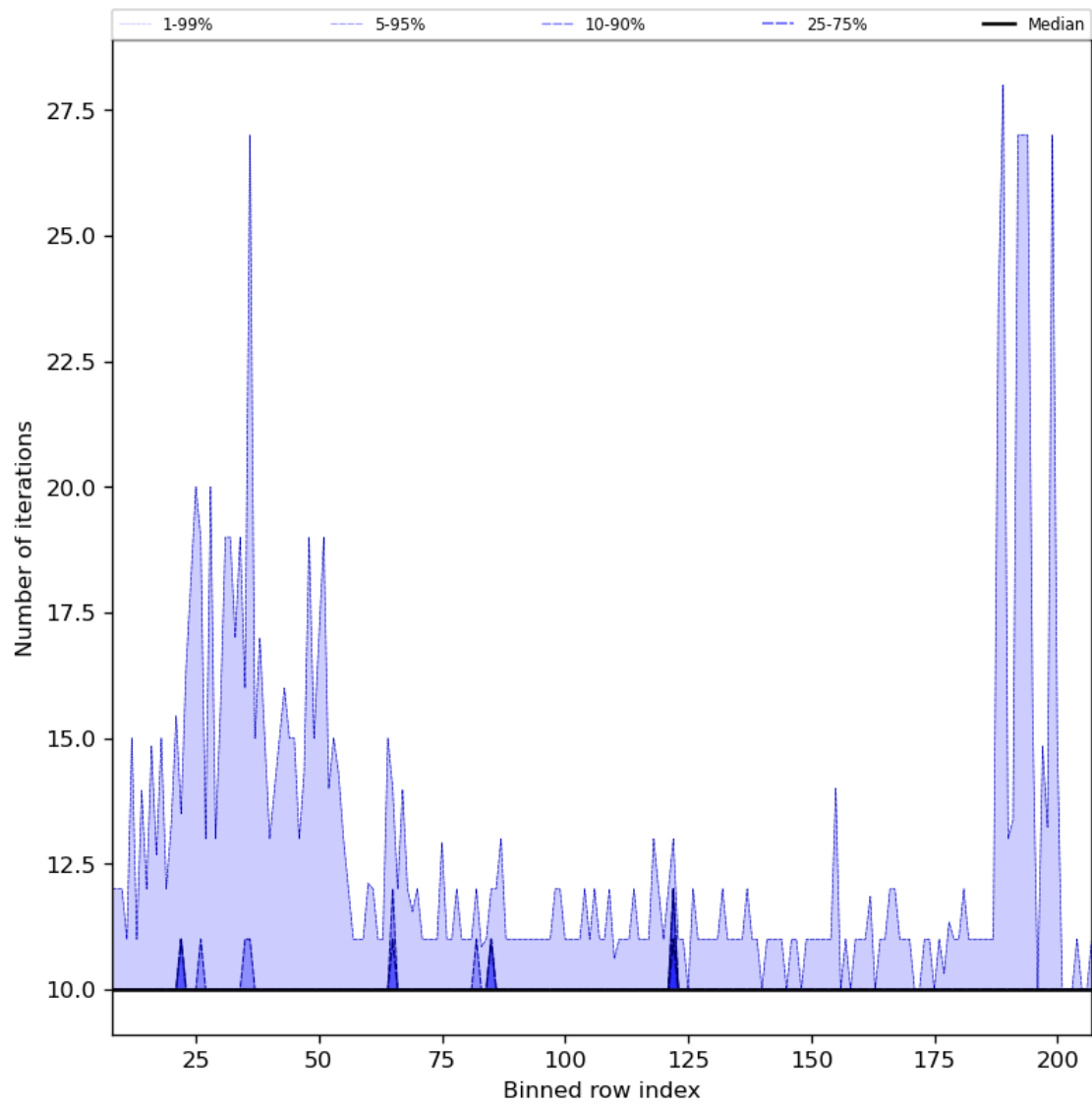
Figure 42: Along track statistics of “Number of iterations” for 2023-06-30 to 2023-07-02
