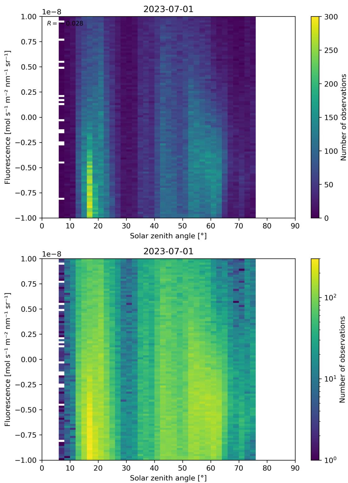
Figure 97: Scatter density plot of “Solar zenith angle” against “Fluorescence” for 2023-06-30 to 2023-07-02.
