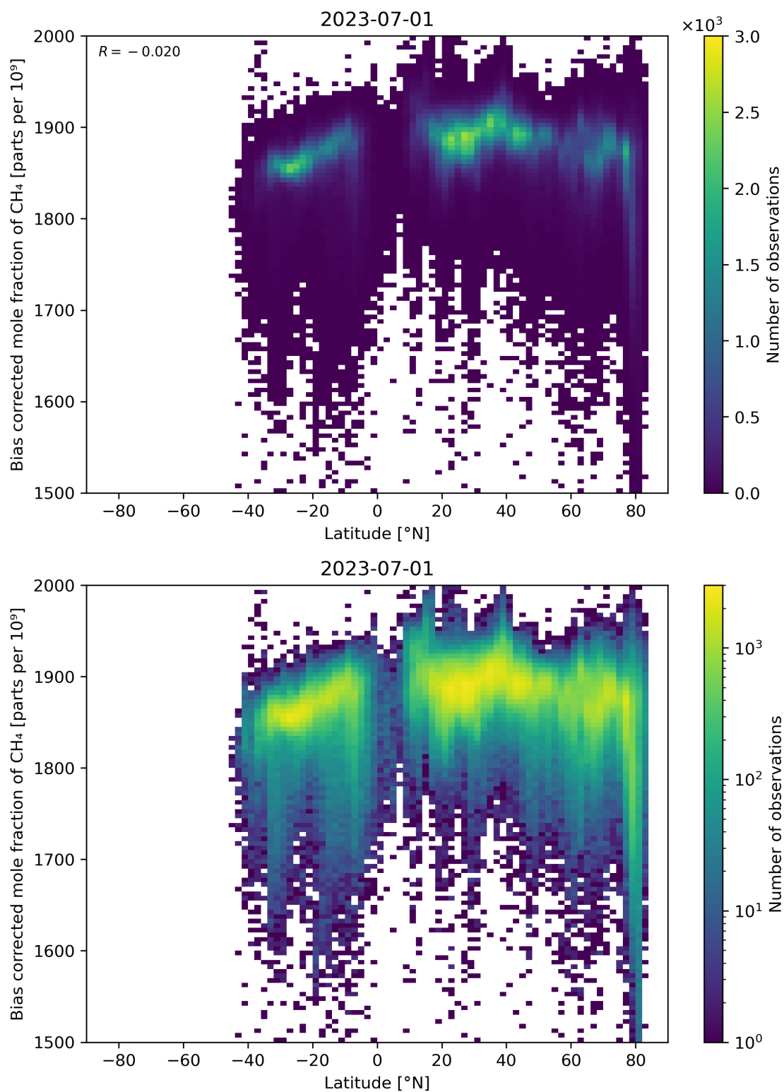
Figure 58: Scatter density plot of “Latitude” against “Bias corrected mole fraction of \text{CH}_4 ” for 2023-06-30 to 2023-07-02.
