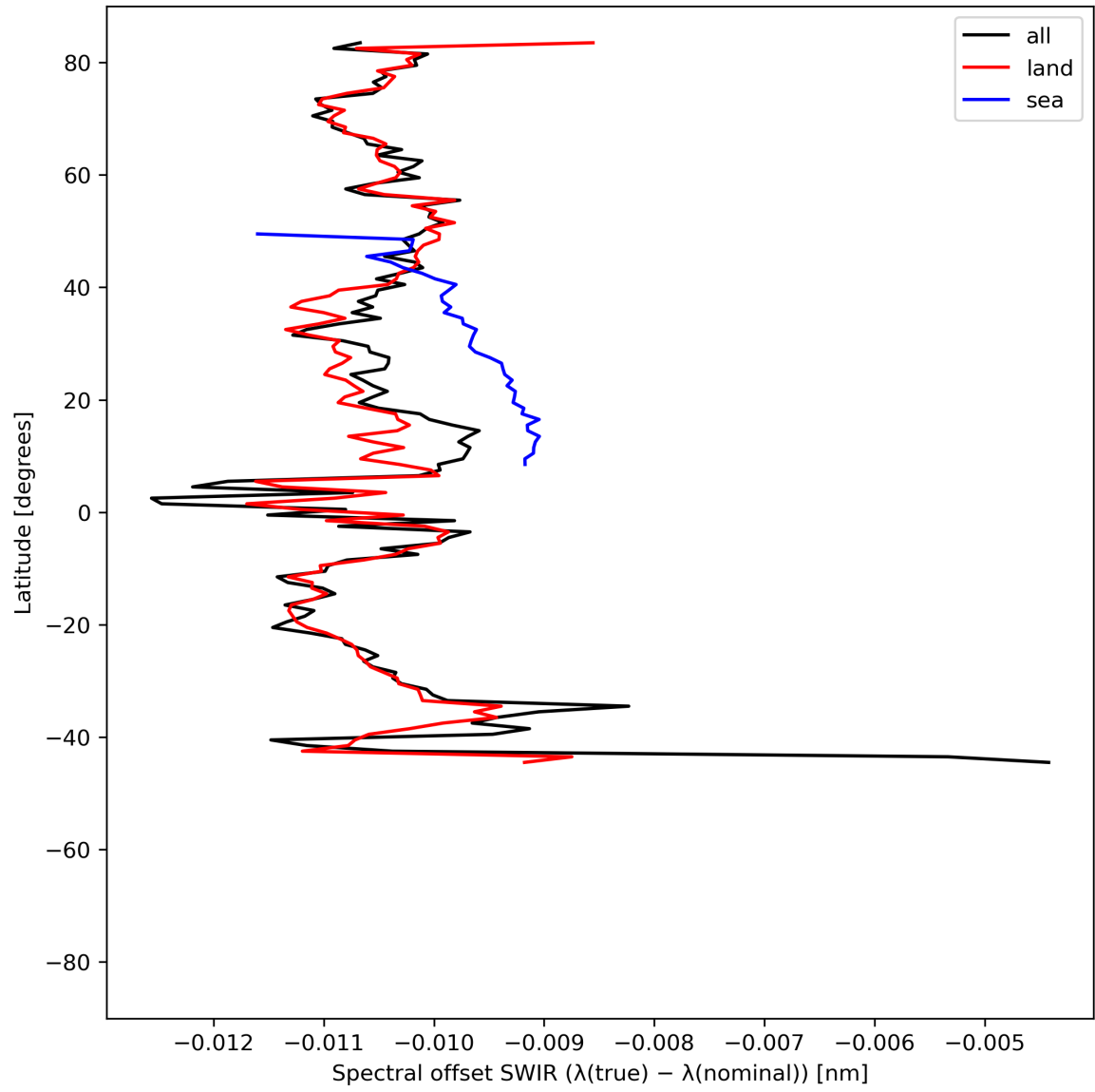
Figure 16: Zonal average of “Spectral offset SWIR ( \lambda(\text{true}) - \lambda(\text{nominal}) )” for 2023-06-30 to 2023-07-02.
