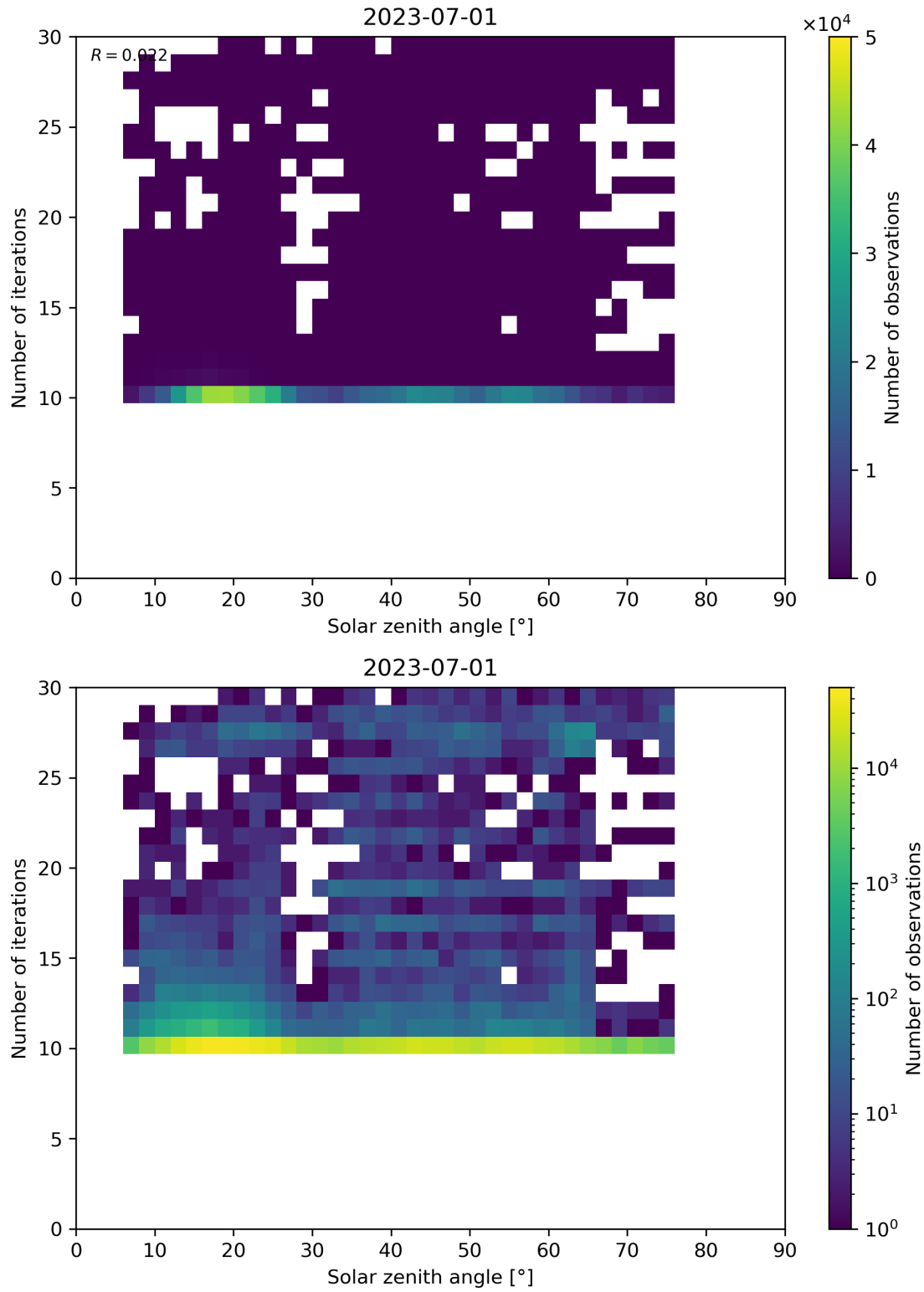
Figure 102: Scatter density plot of “Solar zenith angle” against “Number of iterations” for 2023-06-30 to 2023-07-02.
