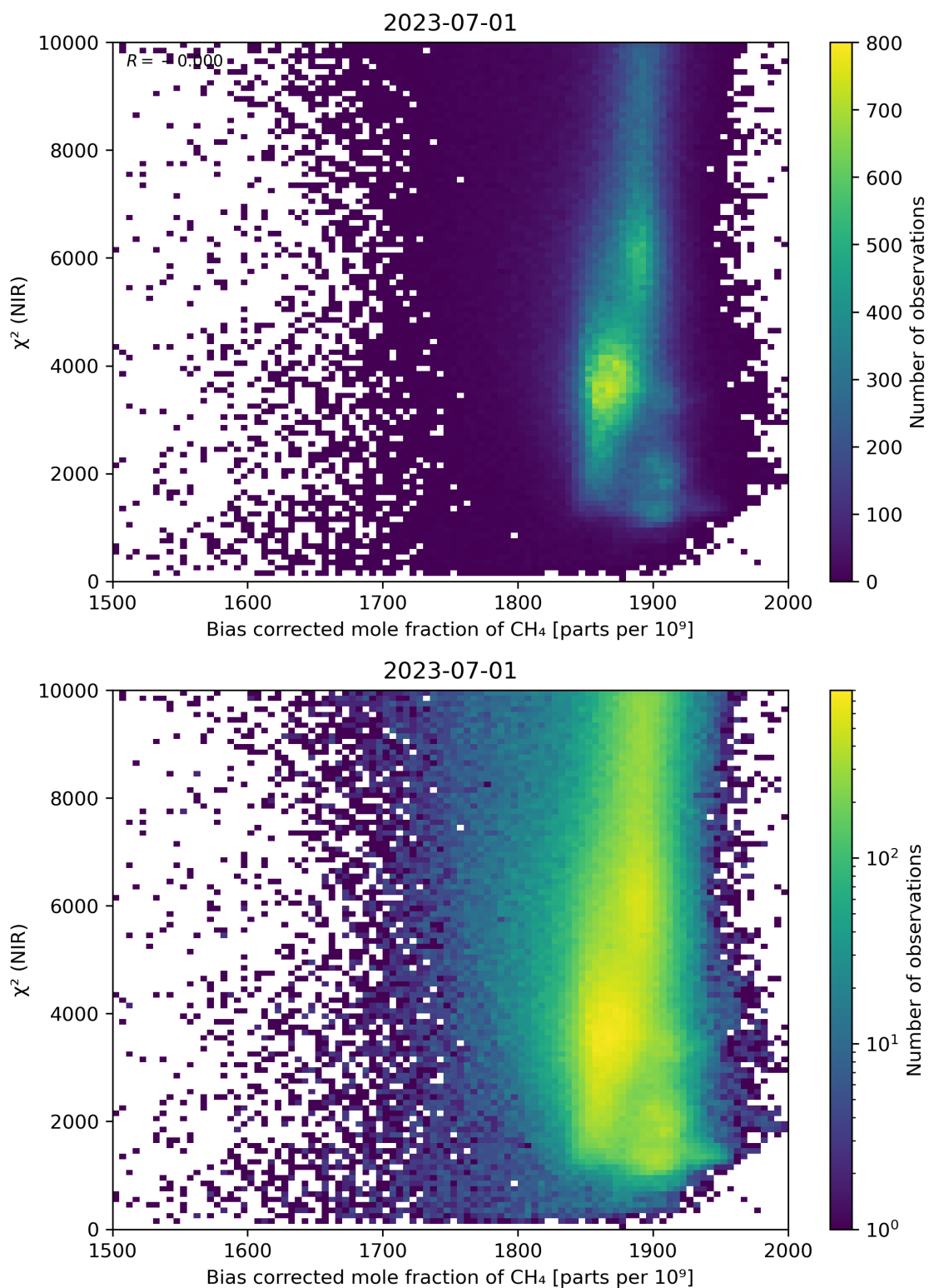
Figure 63: Scatter density plot of “Bias corrected mole fraction of CH 4 ” against “ \chi^2 (NIR)” for 2023-06-30 to 2023-07-02.
