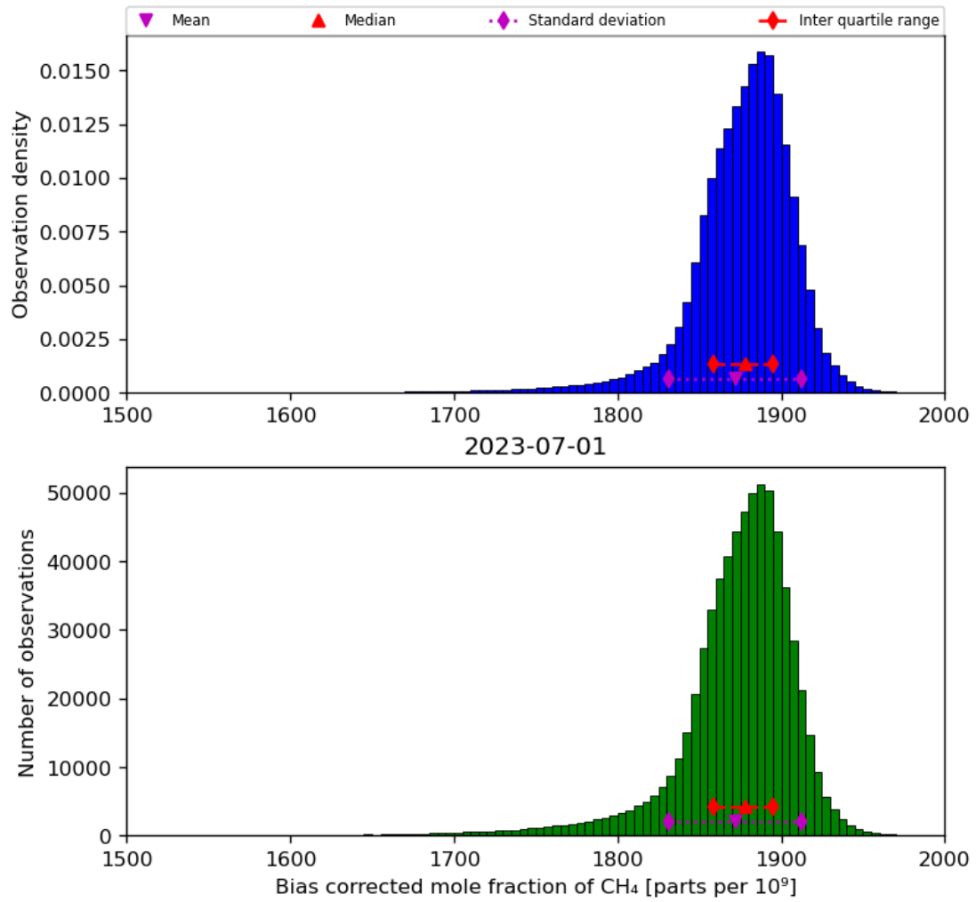
Figure 25: Histogram of “Bias corrected mole fraction of CH 4 ” for 2023-06-30 to 2023-07-02
