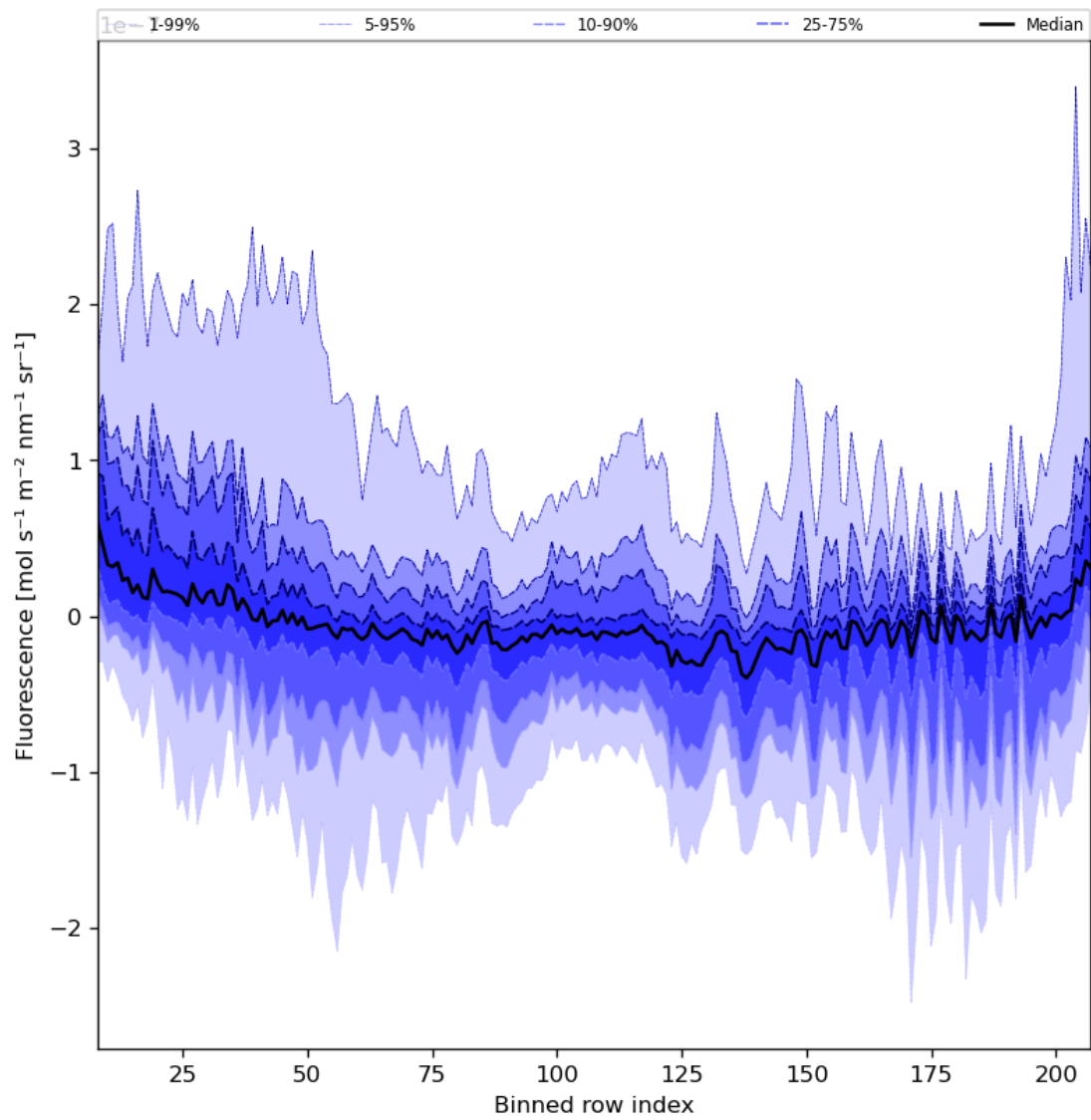
Figure 43: Along track statistics of “Fluorescence” for 2023-06-30 to 2023-07-02
