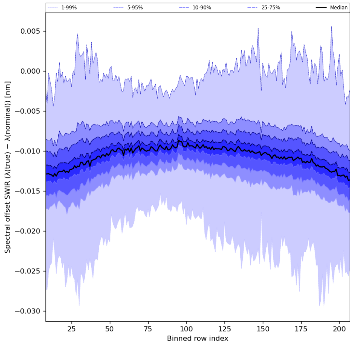
Figure 38: Along track statistics of “Spectral offset SWIR ( \lambda(\text{true}) - \lambda(\text{nominal}) )” for 2023-07-01 to 2023-07-03
