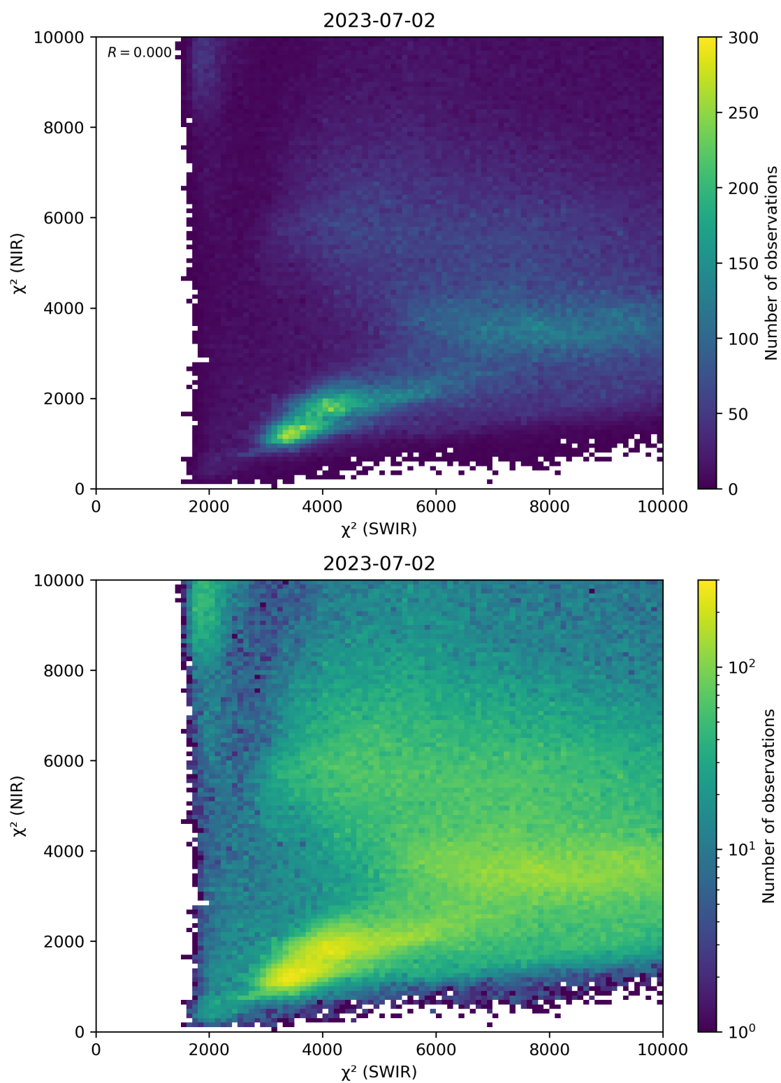
Figure 47: Scatter density plot of “ \chi^2 (SWIR)” against “ \chi^2 (NIR)” for 2023-07-01 to 2023-07-03.
