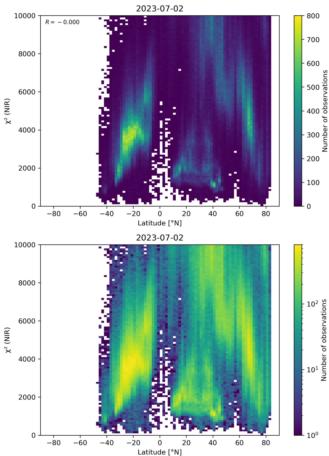
Figure 53: Scatter density plot of “Latitude” against “ \chi^2 (NIR)” for 2023-07-01 to 2023-07-03.
