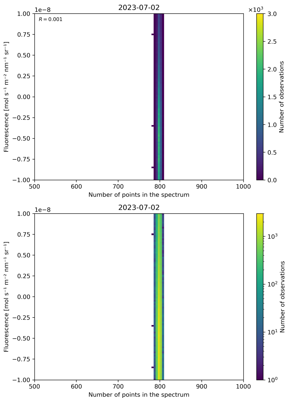
Figure 91: Scatter density plot of “Number of points in the spectrum” against “Fluorescence” for 2023-07-01 to 2023-07-03.
