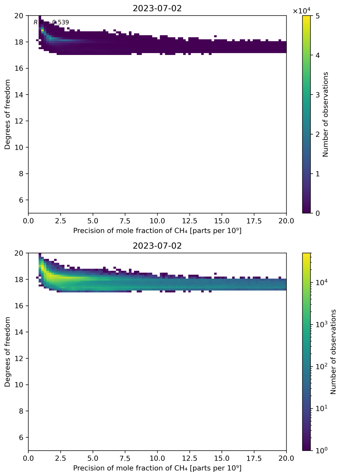
Figure 80: Scatter density plot of “Precision of mole fraction of CH 4 ” against “Degrees of freedom” for 2023-07-01 to 2023-07-03.
