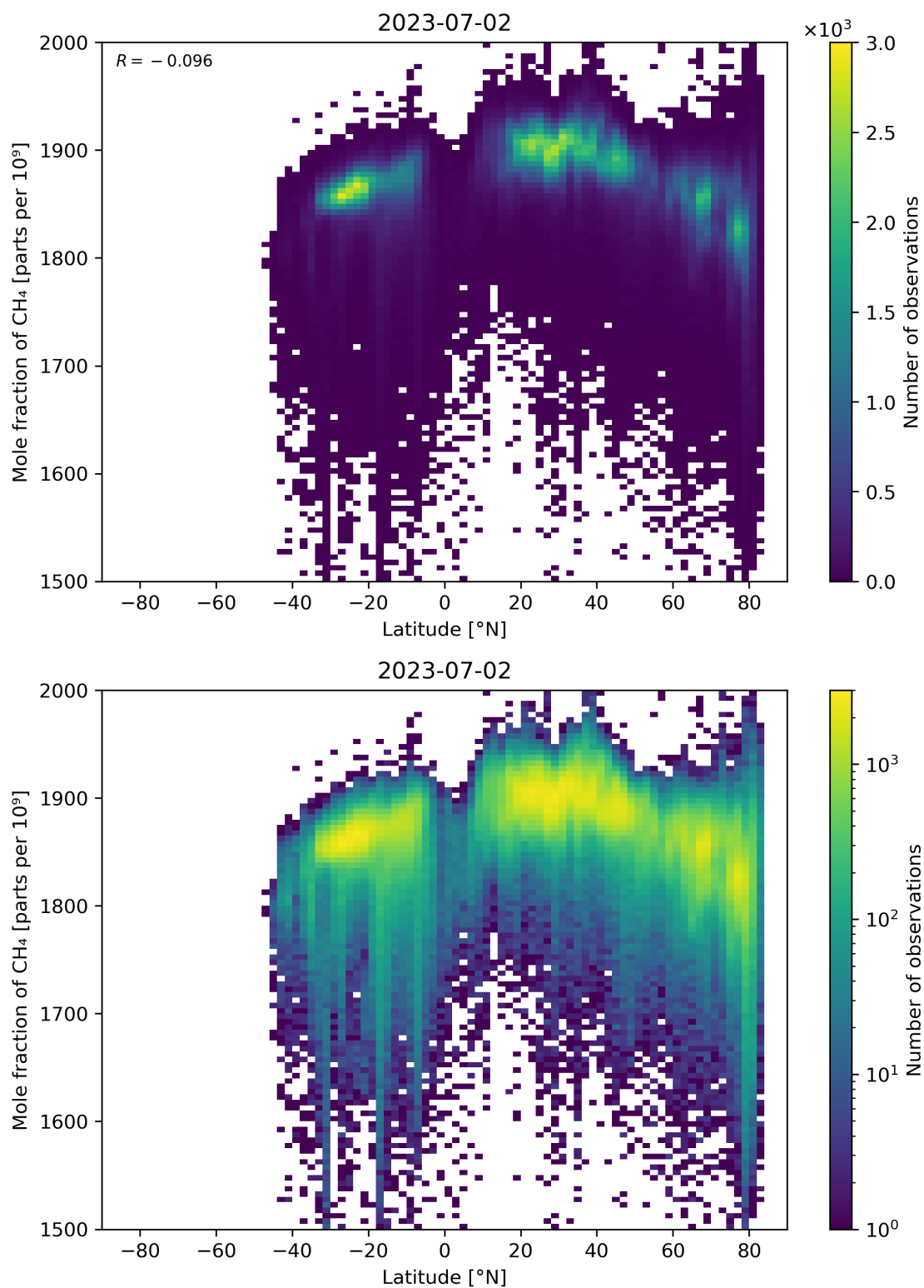
Figure 57: Scatter density plot of “Latitude” against “Mole fraction of CH 4 ” for 2023-07-01 to 2023-07-03.
