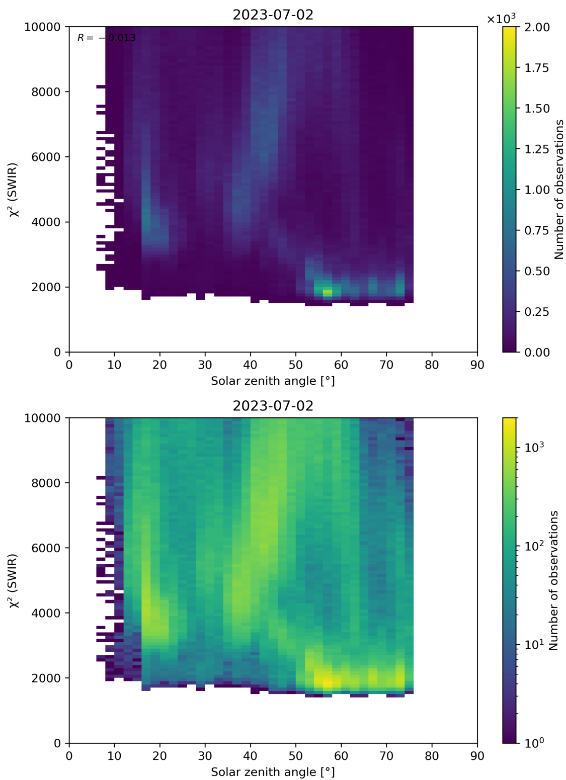
Figure 95: Scatter density plot of “Solar zenith angle” against “ \chi^2 (SWIR)” for 2023-07-01 to 2023-07-03.
