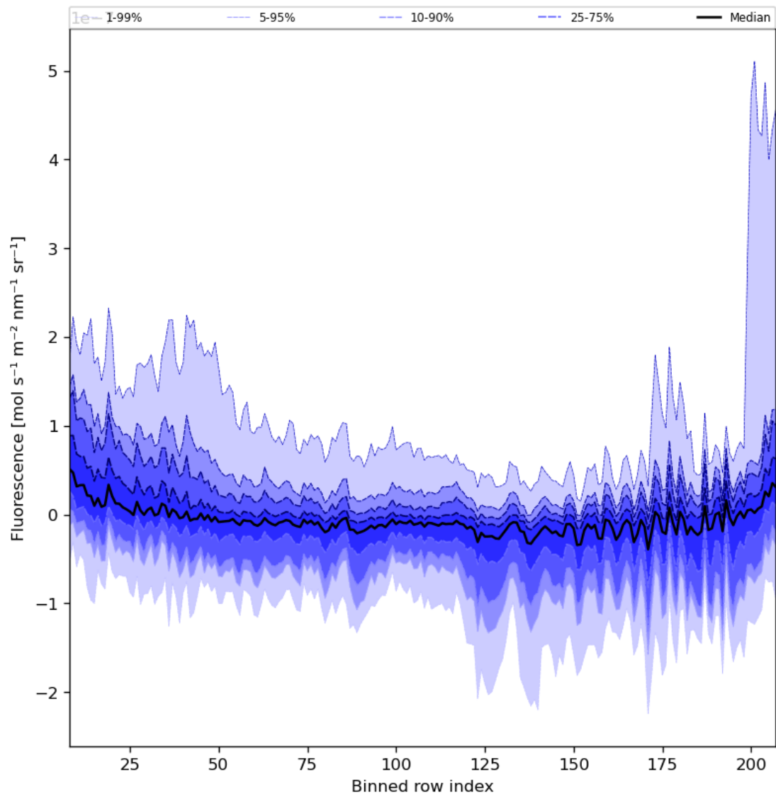
Figure 43: Along track statistics of “Fluorescence” for 2023-07-01 to 2023-07-03
