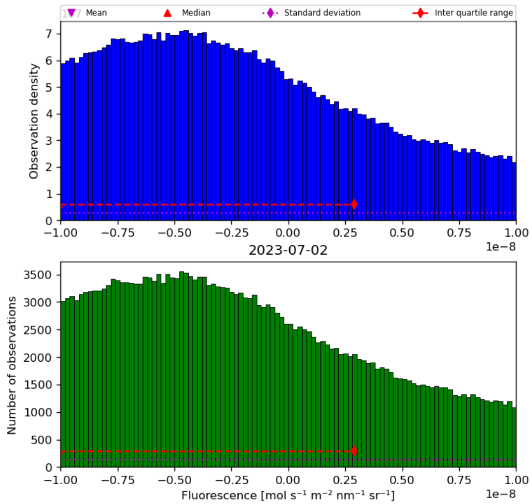
Figure 32: Histogram of “Fluorescence” for 2023-07-01 to 2023-07-03
