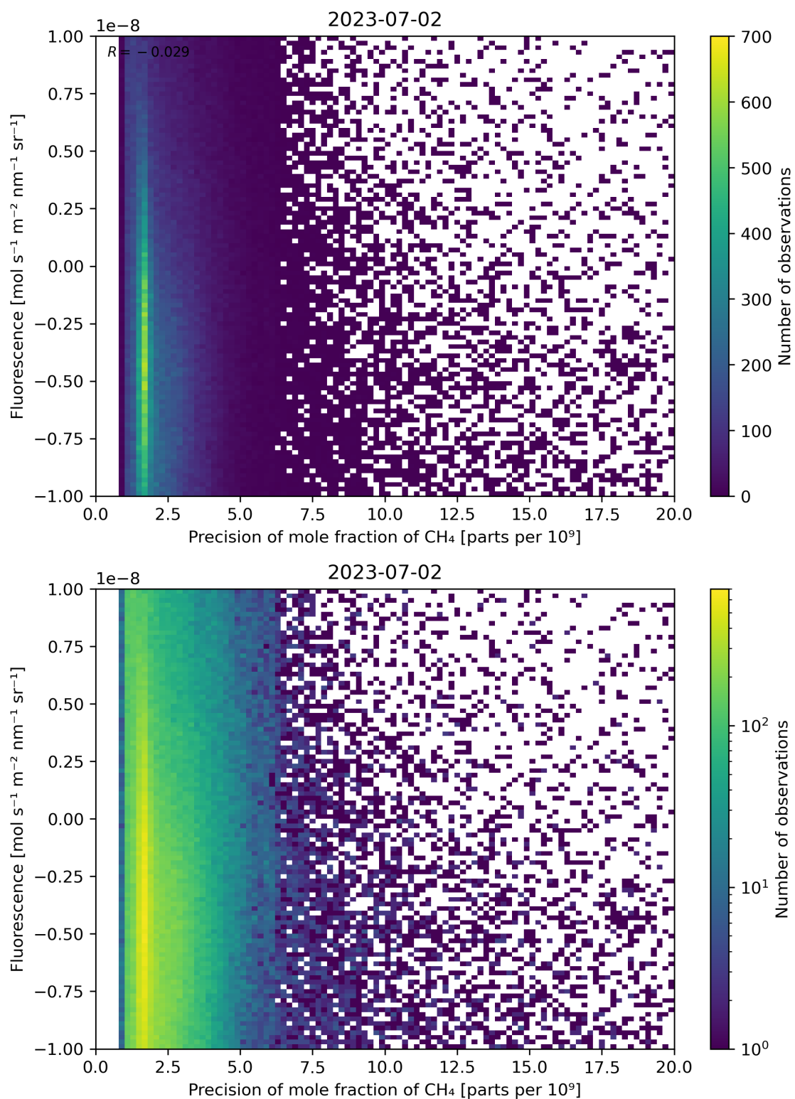
Figure 81: Scatter density plot of “Precision of mole fraction of \text{CH}_4 ” against “Fluorescence” for 2023-07-01 to 2023-07-03.
