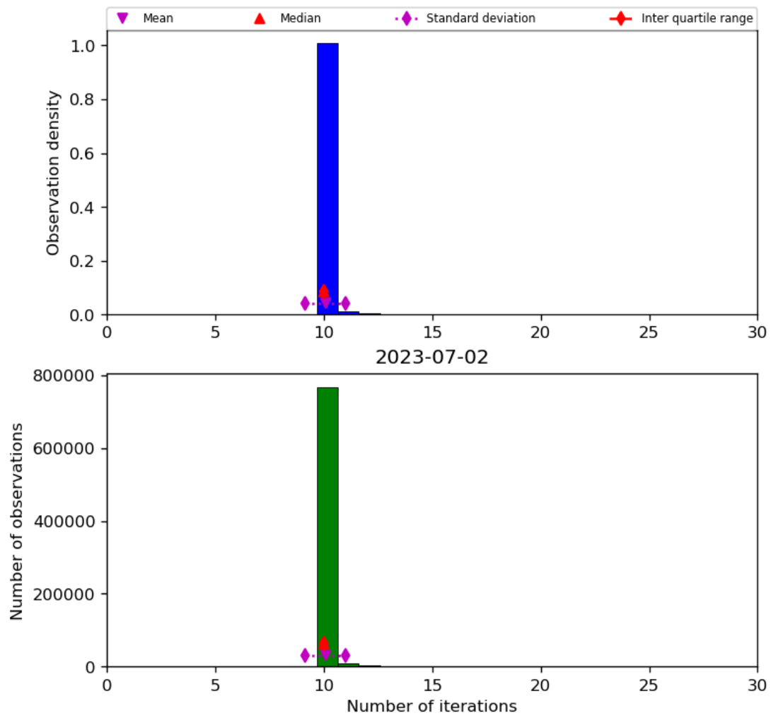
Figure 31: Histogram of “Number of iterations” for 2023-07-01 to 2023-07-03
