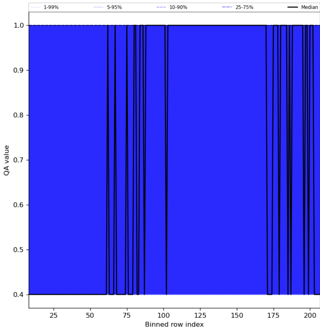
Figure 33: Along track statistics of “QA value” for 2023-07-01 to 2023-07-03
