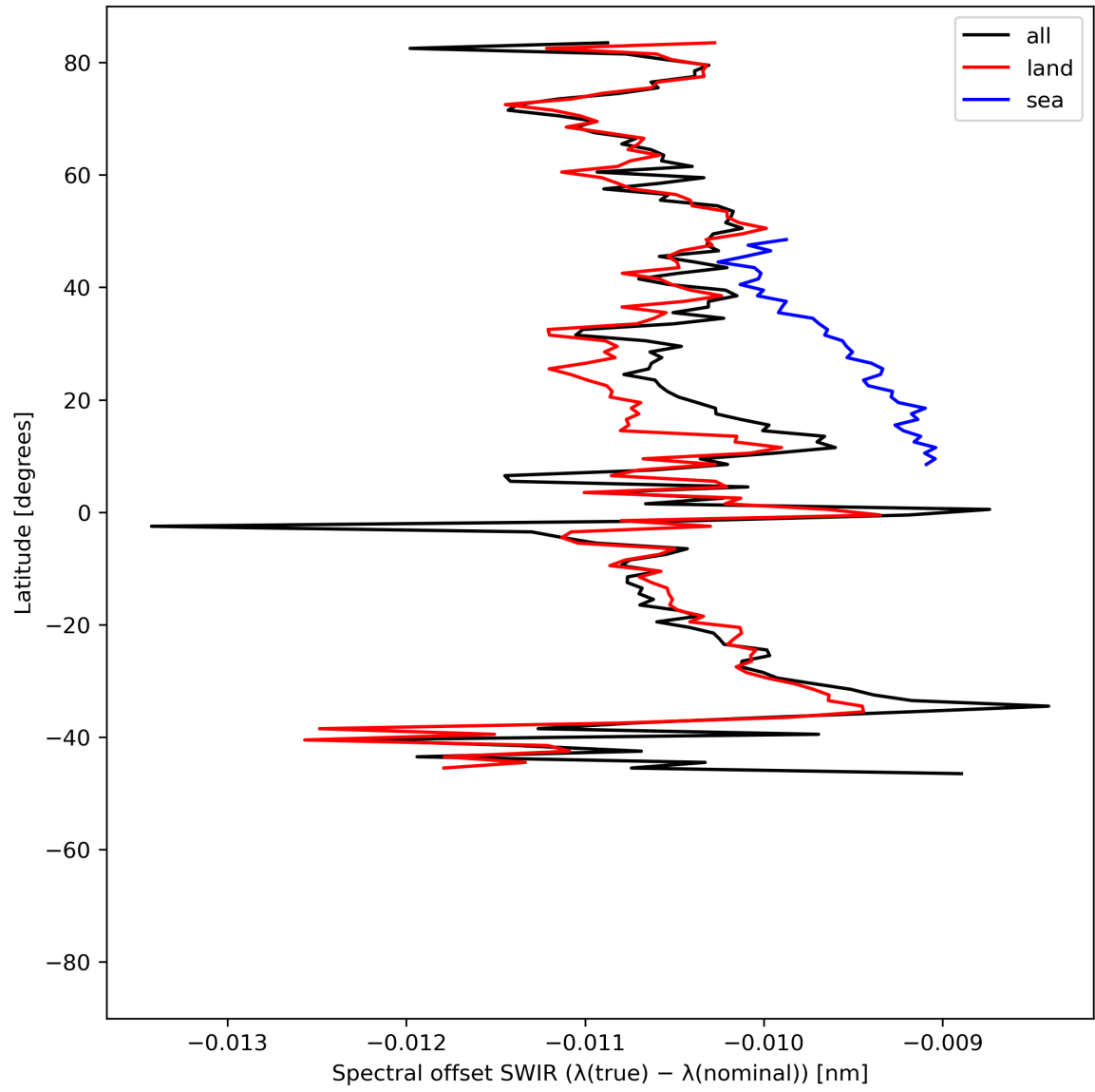
Figure 16: Zonal average of “Spectral offset SWIR ( \lambda(\text{true}) - \lambda(\text{nominal}) )” for 2023-07-01 to 2023-07-03.
