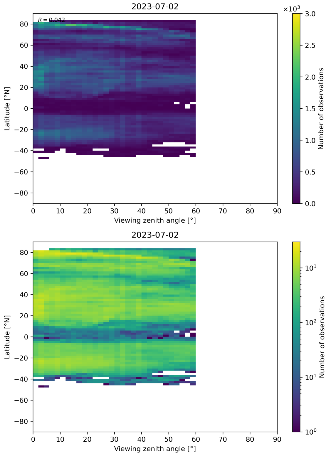
Figure 109: Scatter density plot of “Viewing zenith angle” against “Latitude” for 2023-07-01 to 2023-07-03.
