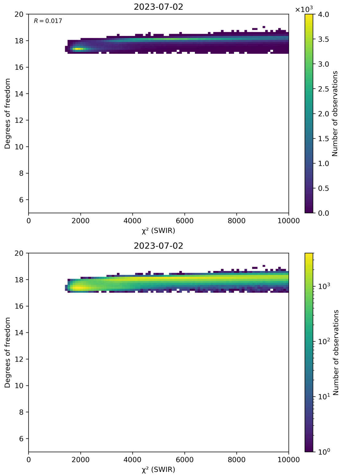
Figure 48: Scatter density plot of “ \chi^2 (SWIR)” against “Degrees of freedom” for 2023-07-01 to 2023-07-03.
