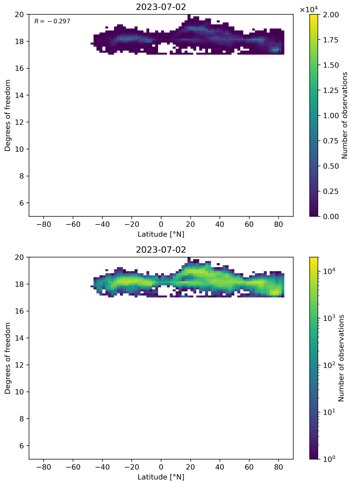
Figure 55: Scatter density plot of “Latitude” against “Degrees of freedom” for 2023-07-01 to 2023-07-03.
