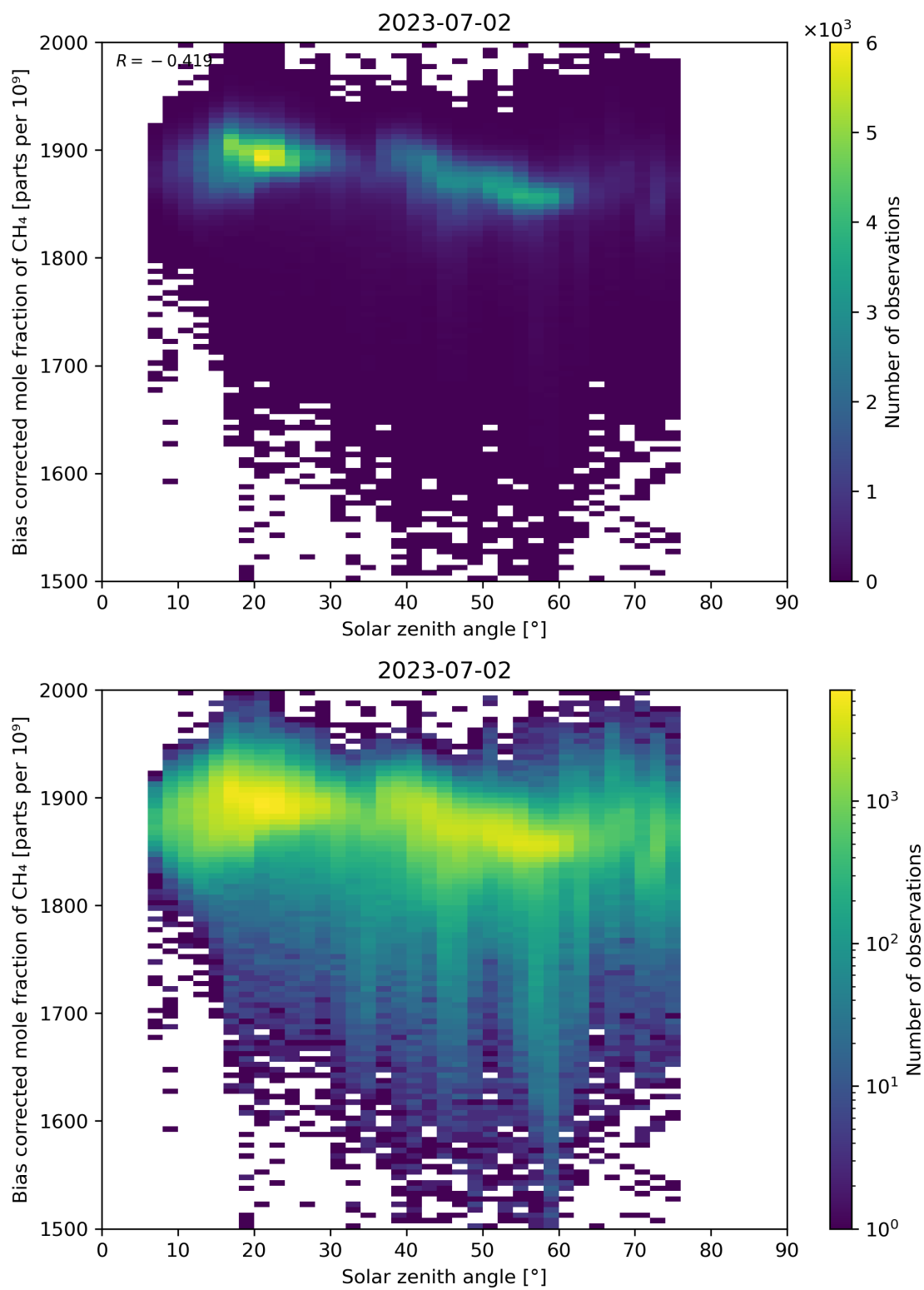
Figure 100: Scatter density plot of “Solar zenith angle” against “Bias corrected mole fraction of CH 4 ” for 2023-07-01 to 2023-07-03.
