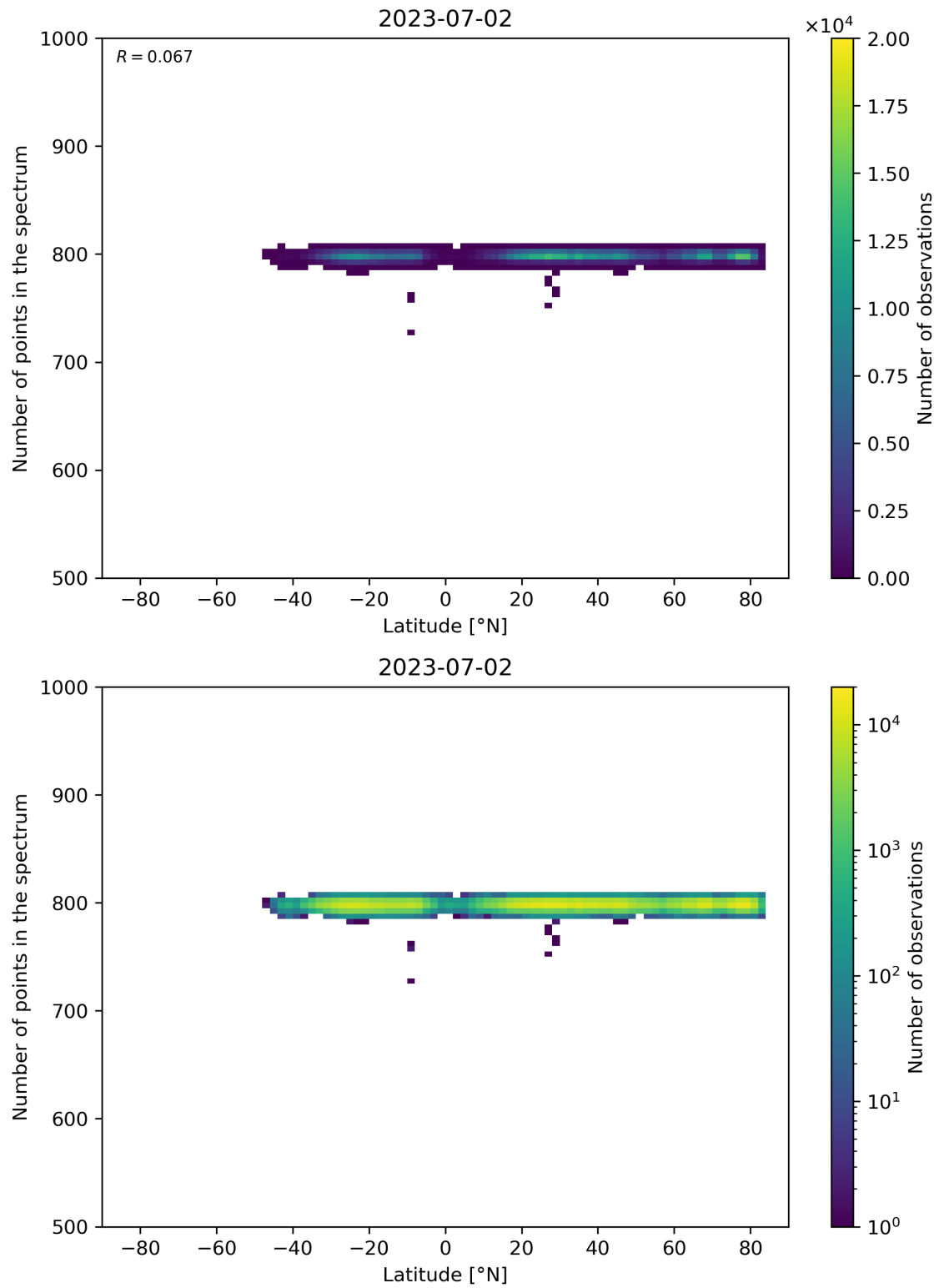
Figure 61: Scatter density plot of “Latitude” against “Number of points in the spectrum” for 2023-07-01 to 2023-07-03.
