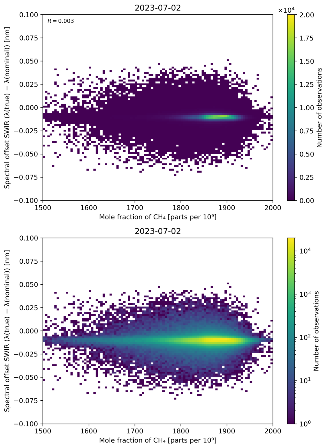
Figure 86: Scatter density plot of “Mole fraction of CH 4 ” against “Spectral offset SWIR ( \lambda(\text{true}) - \lambda(\text{nominal}) )” for 2023-07-01 to 2023-07-03.
