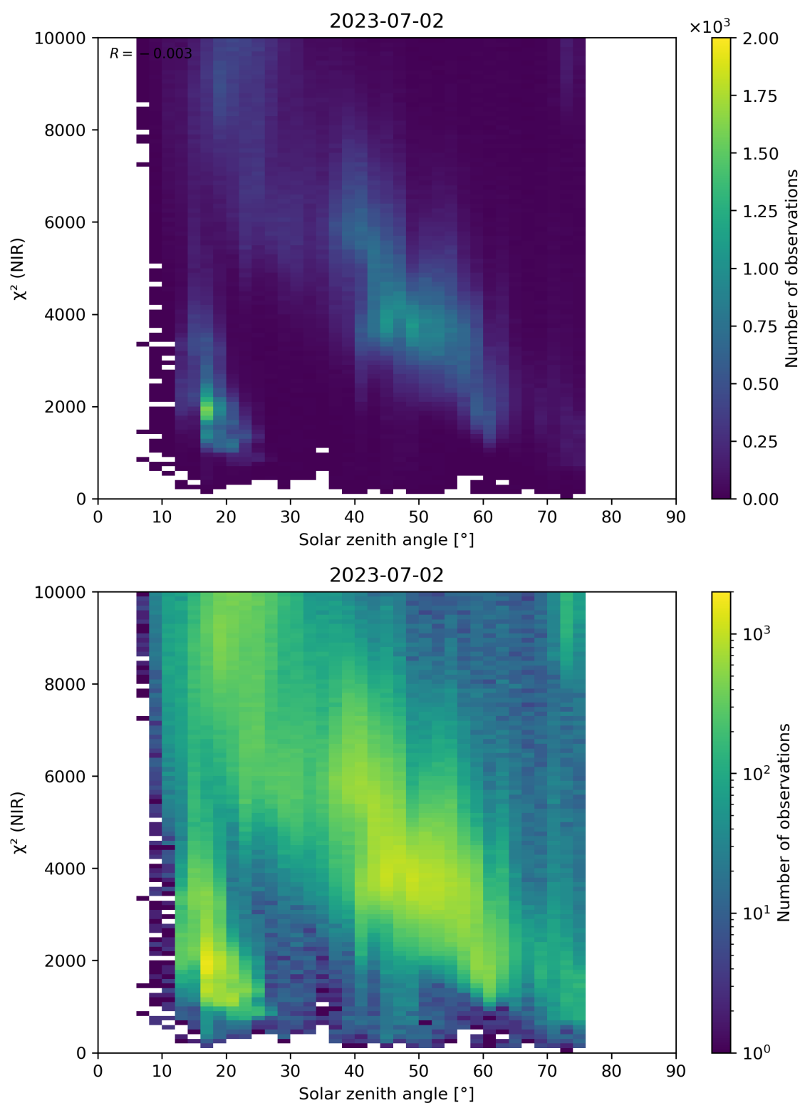
Figure 94: Scatter density plot of “Solar zenith angle” against “ \chi^2 (NIR)” for 2023-07-01 to 2023-07-03.
