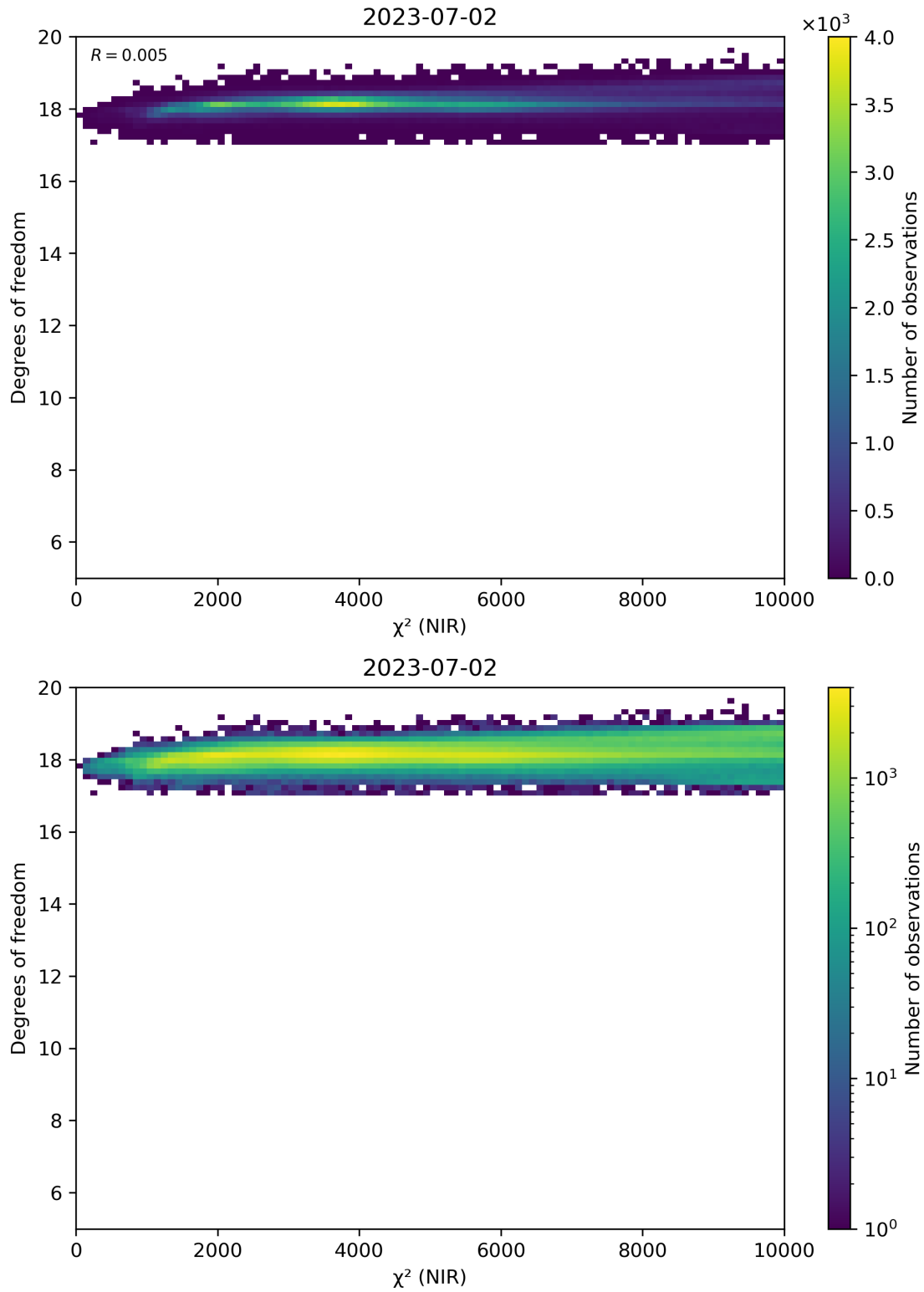
Figure 44: Scatter density plot of “ \chi^2 (NIR)” against “Degrees of freedom” for 2023-07-01 to 2023-07-03.
