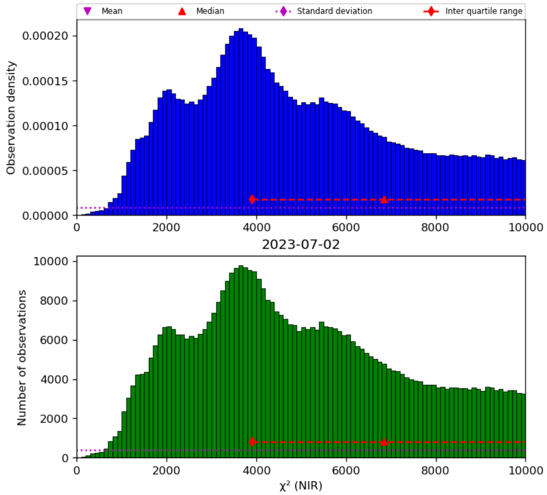
Figure 29: Histogram of “ \chi^2 (NIR)” for 2023-07-01 to 2023-07-03
