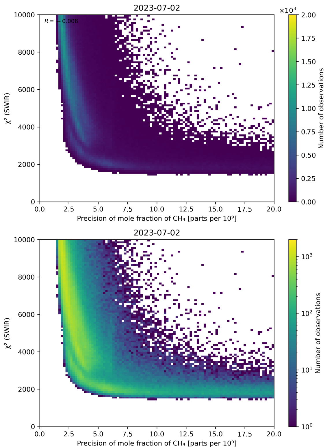
Figure 79: Scatter density plot of “Precision of mole fraction of CH 4 ” against “ \chi^2 (SWIR)” for 2023-07-01 to 2023-07-03.
