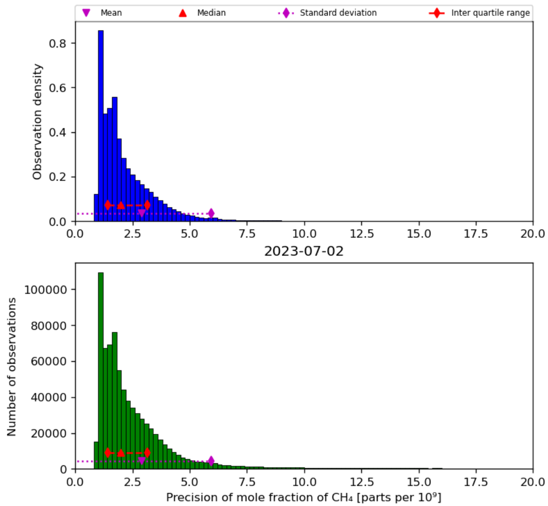
Figure 24: Histogram of “Precision of mole fraction of CH 4 ” for 2023-07-01 to 2023-07-03
