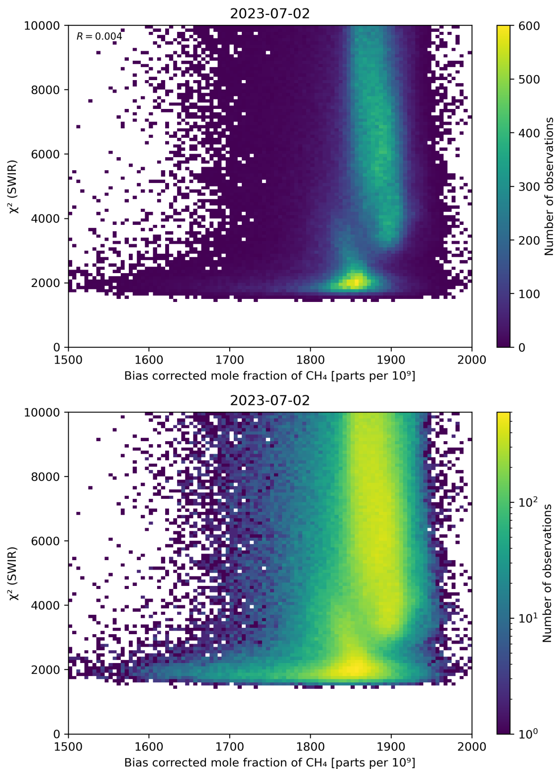
Figure 64: Scatter density plot of “Bias corrected mole fraction of CH 4 ” against “ \chi^2 (SWIR)” for 2023-07-01 to 2023-07-03.
