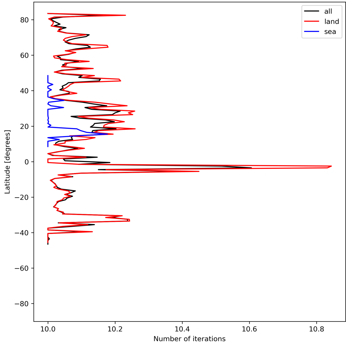
Figure 20: Zonal average of “Number of iterations” for 2023-07-01 to 2023-07-03.
