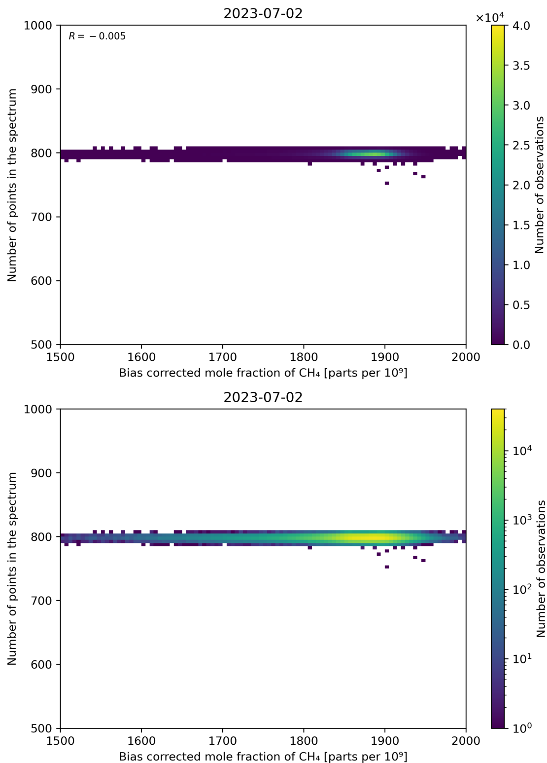
Figure 68: Scatter density plot of “Bias corrected mole fraction of CH 4 ” against “Number of points in the spectrum” for 2023-07-01 to 2023-07-03.
