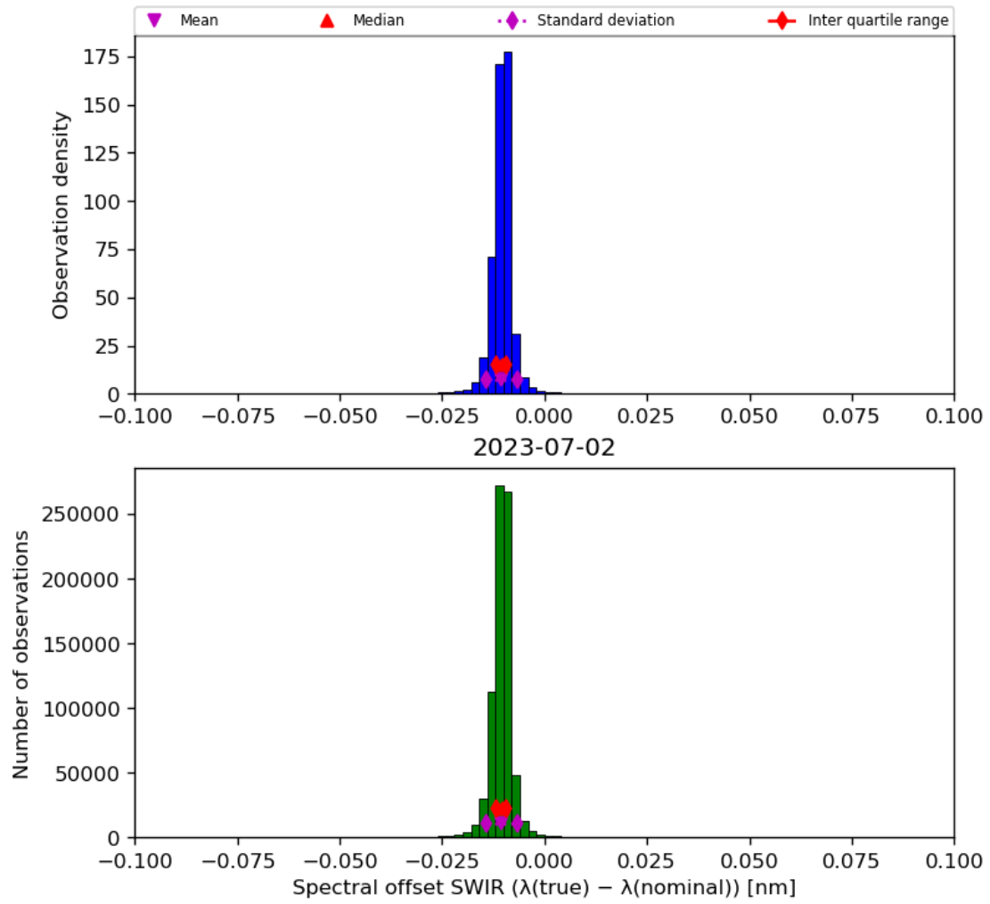
Figure 27: Histogram of “Spectral offset SWIR ( \lambda(\text{true}) - \lambda(\text{nominal}) )” for 2023-07-01 to 2023-07-03
