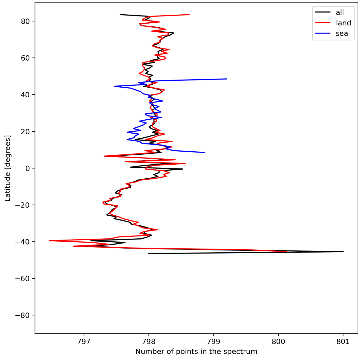
Figure 15: Zonal average of “Number of points in the spectrum” for 2023-07-01 to 2023-07-03.
