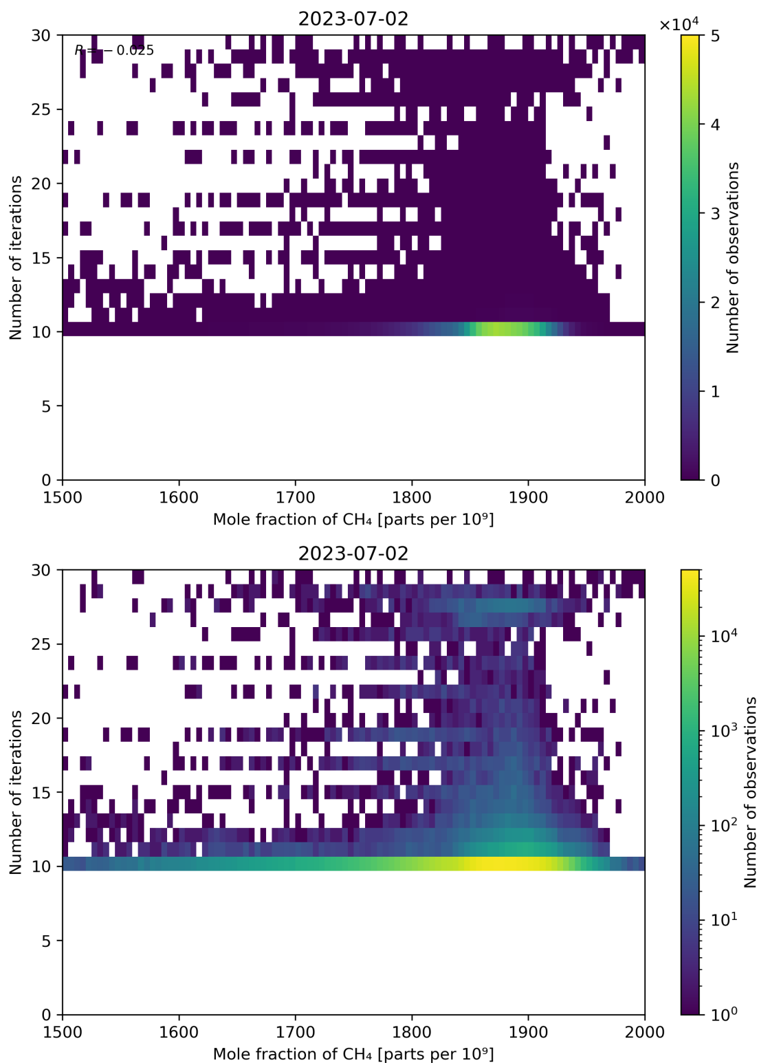
Figure 76: Scatter density plot of “Mole fraction of CH 4 ” against “Number of iterations” for 2023-07-01 to 2023-07-03.
