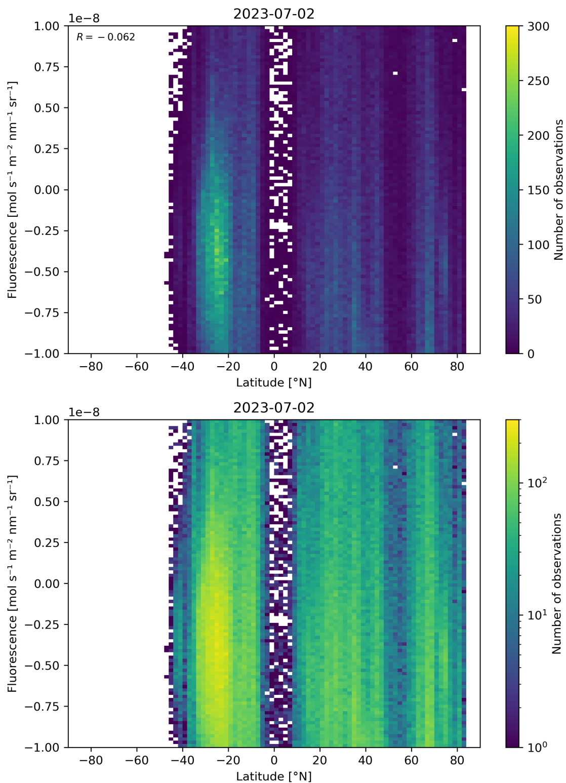
Figure 56: Scatter density plot of “Latitude” against “Fluorescence” for 2023-07-01 to 2023-07-03.
