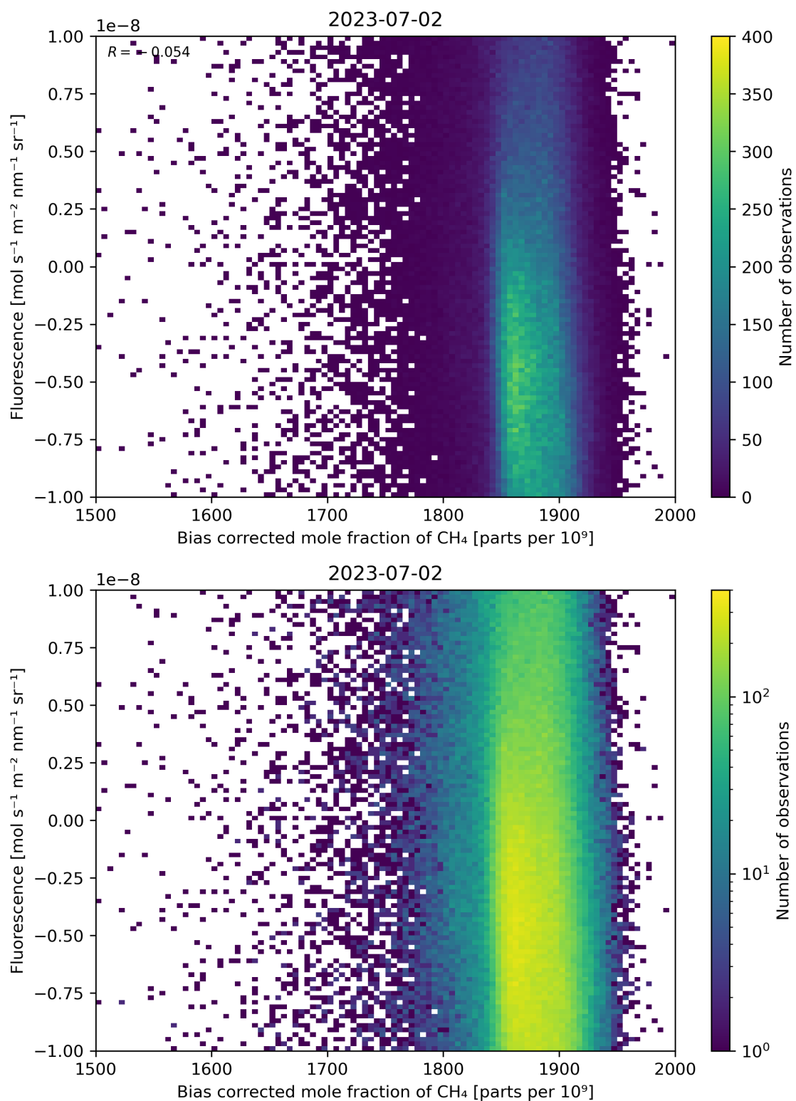
Figure 66: Scatter density plot of “Bias corrected mole fraction of \text{CH}_4 ” against “Fluorescence” for 2023-07-01 to 2023-07-03.
