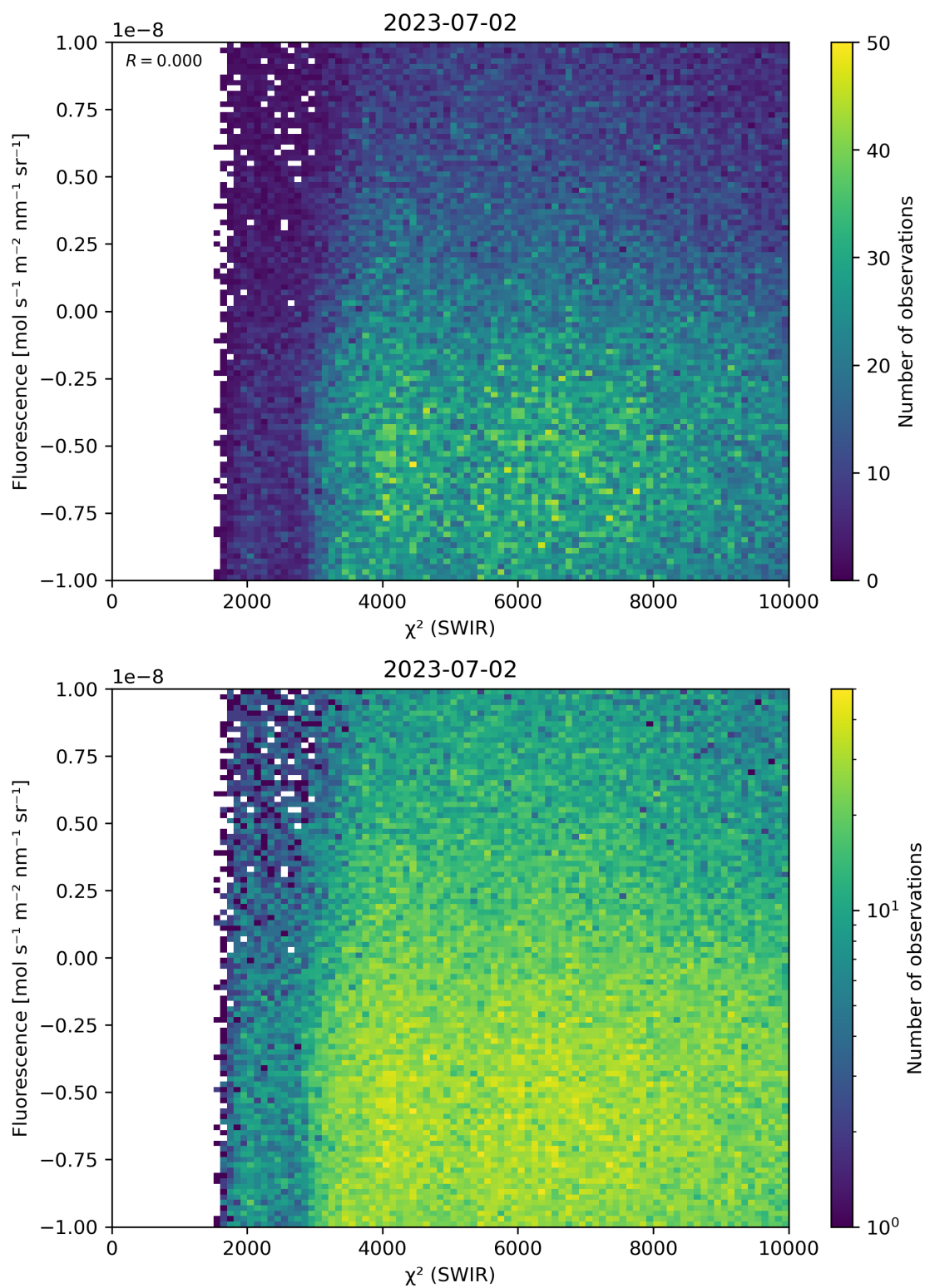
Figure 49: Scatter density plot of “ \chi^2 (SWIR)” against “Fluorescence” for 2023-07-01 to 2023-07-03.
