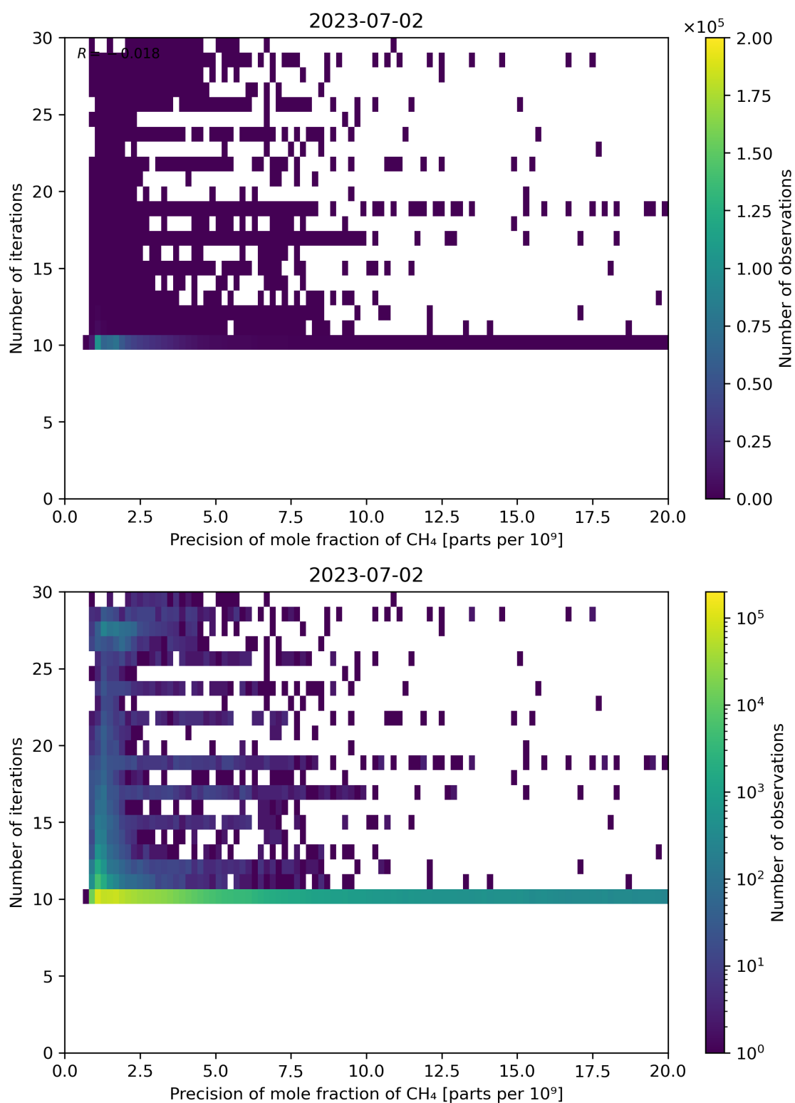
Figure 83: Scatter density plot of “Precision of mole fraction of CH 4 ” against “Number of iterations” for 2023-07-01 to 2023-07-03.
