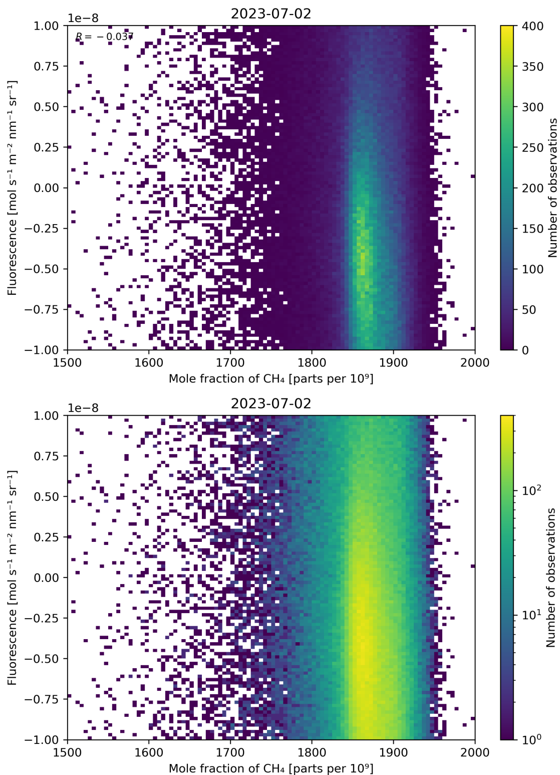
Figure 73: Scatter density plot of “Mole fraction of \text{CH}_4 ” against “Fluorescence” for 2023-07-01 to 2023-07-03.
