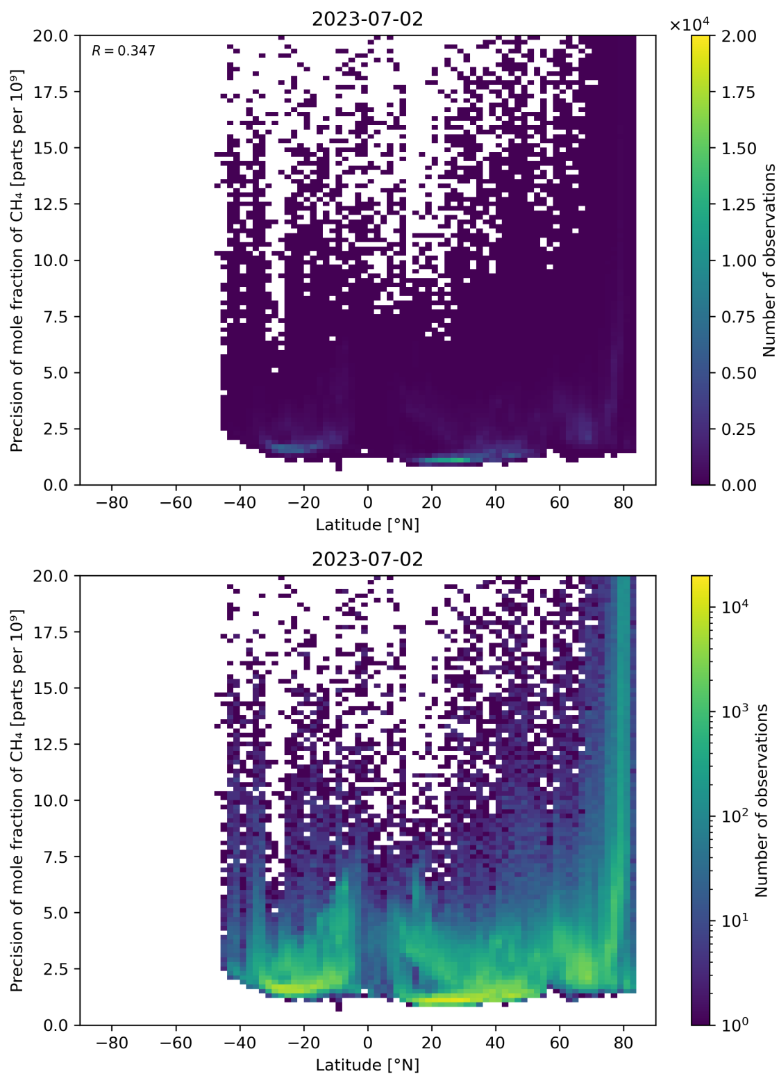
Figure 59: Scatter density plot of “Latitude” against “Precision of mole fraction of \text{CH}_4 ” for 2023-07-01 to 2023-07-03.
