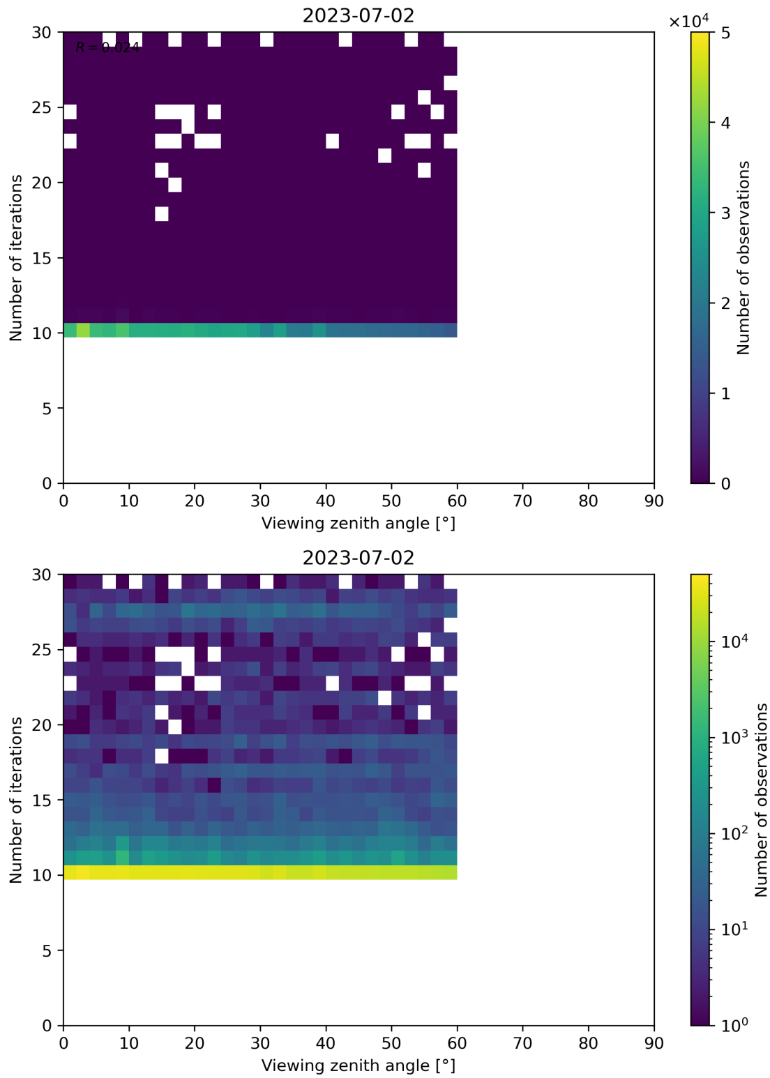
Figure 113: Scatter density plot of “Viewing zenith angle” against “Number of iterations” for 2023-07-01 to 2023-07-03.
