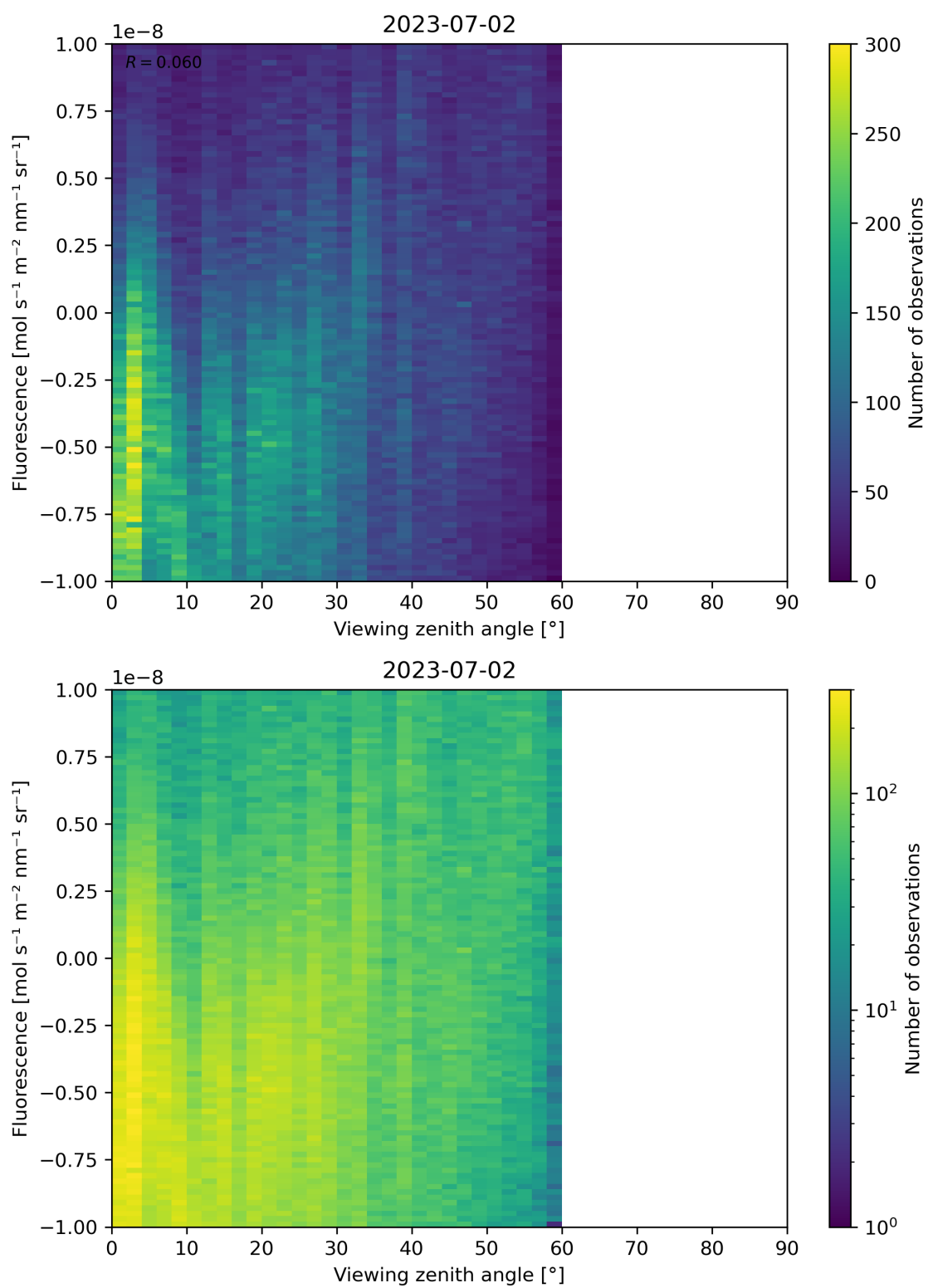
Figure 108: Scatter density plot of “Viewing zenith angle” against “Fluorescence” for 2023-07-01 to 2023-07-03.
