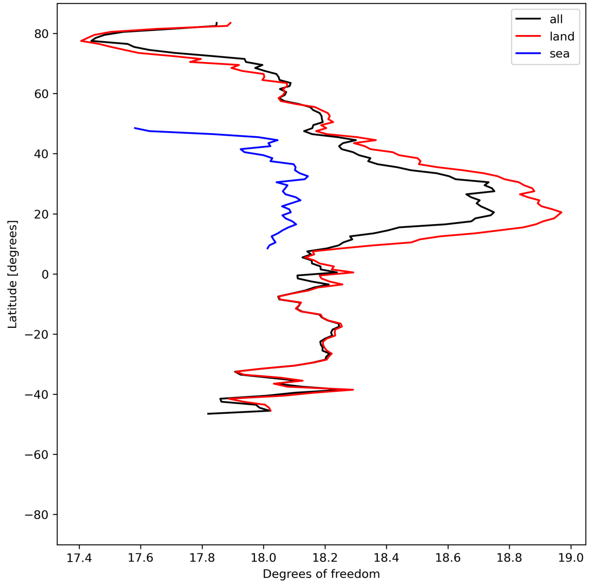
Figure 19: Zonal average of “Degrees of freedom” for 2023-07-01 to 2023-07-03.
