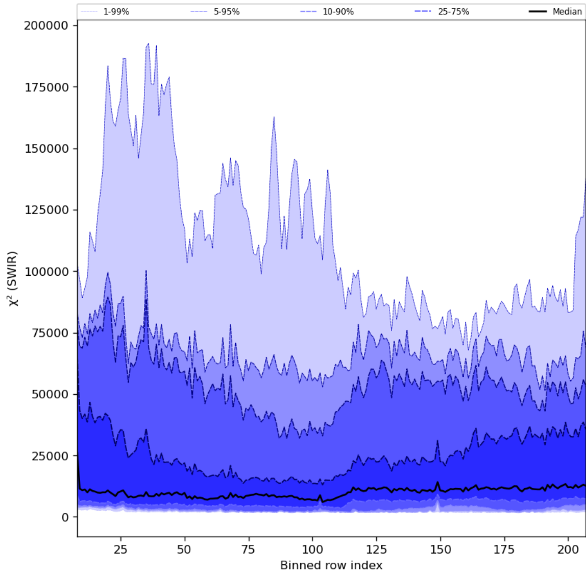
Figure 39: Along track statistics of “ \chi^2 (SWIR)” for 2023-07-01 to 2023-07-03
