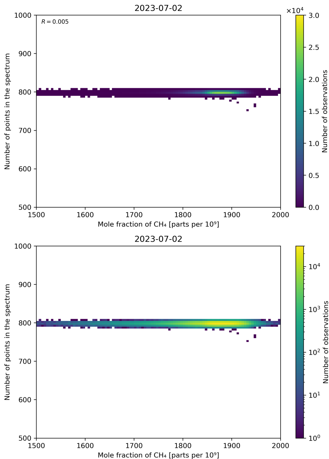
Figure 77: Scatter density plot of “Mole fraction of CH 4 ” against “Number of points in the spectrum” for 2023-07-01 to 2023-07-03.
