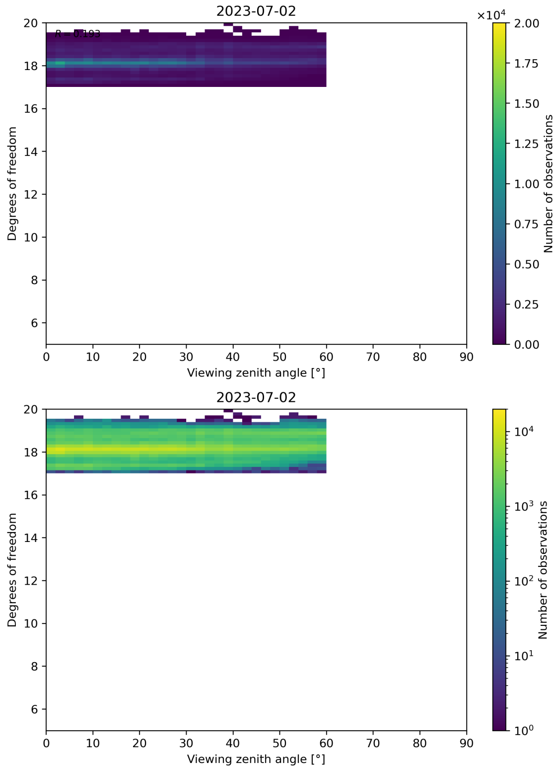
Figure 107: Scatter density plot of “Viewing zenith angle” against “Degrees of freedom” for 2023-07-01 to 2023-07-03.
