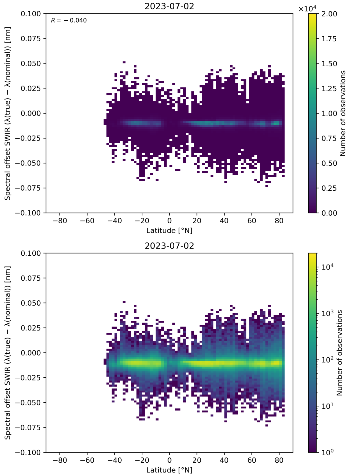
Figure 62: Scatter density plot of “Latitude” against “Spectral offset SWIR ( \lambda(\text{true}) - \lambda(\text{nominal}) )” for 2023-07-01 to 2023-07-03.
