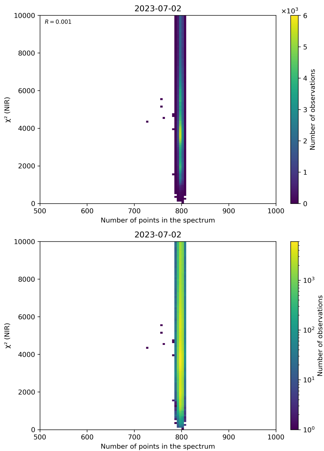
Figure 88: Scatter density plot of “Number of points in the spectrum” against “ \chi^2 (NIR)” for 2023-07-01 to 2023-07-03.
