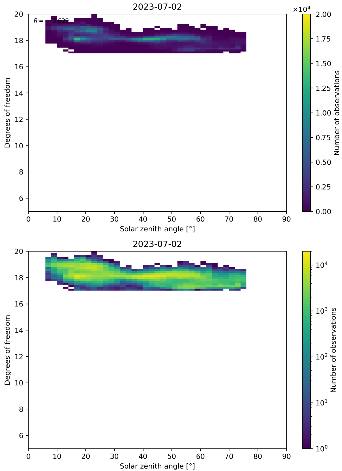
Figure 96: Scatter density plot of “Solar zenith angle” against “Degrees of freedom” for 2023-07-01 to 2023-07-03.
