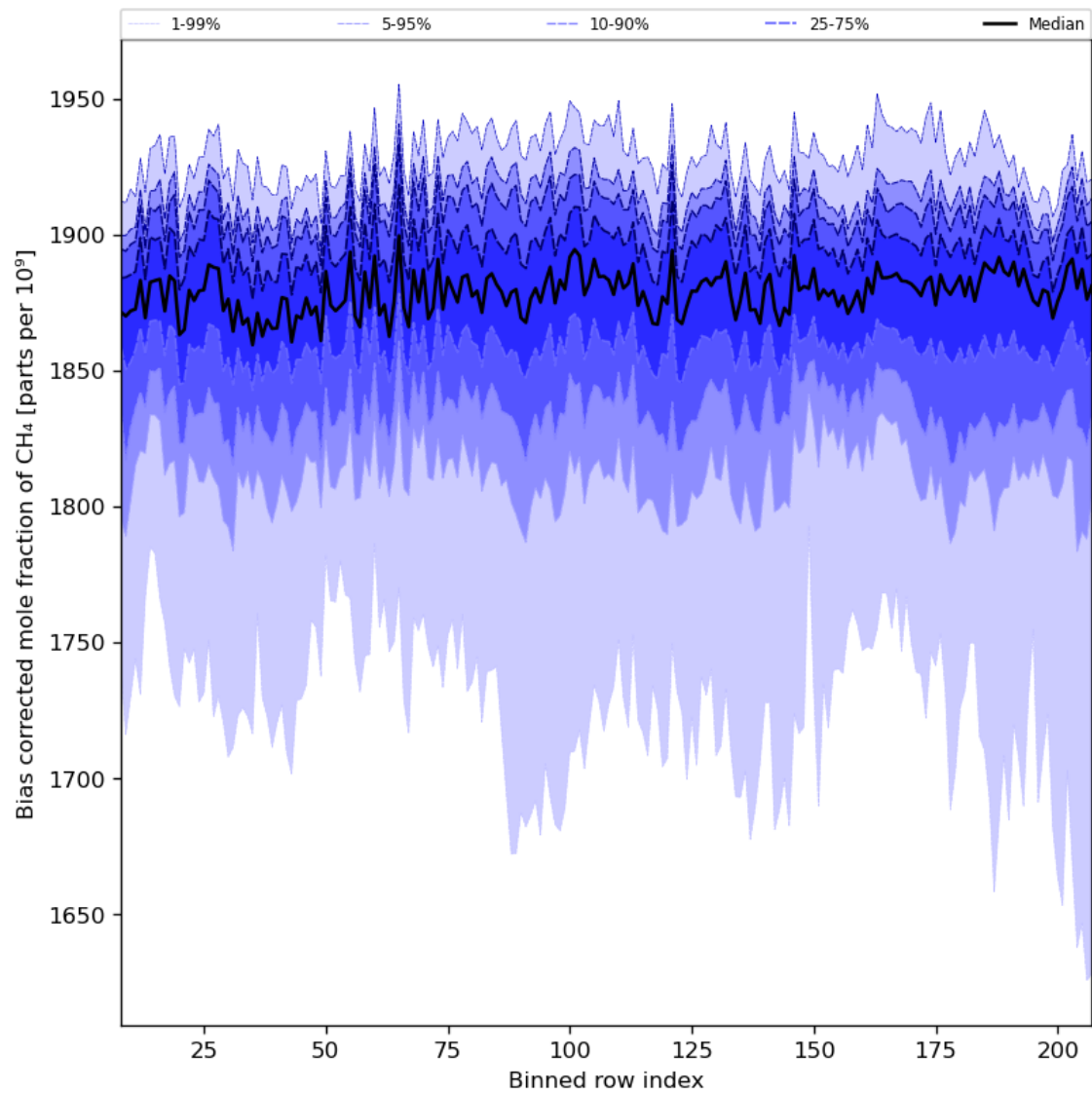
Figure 36: Along track statistics of “Bias corrected mole fraction of CH 4 ” for 2023-07-01 to 2023-07-03
