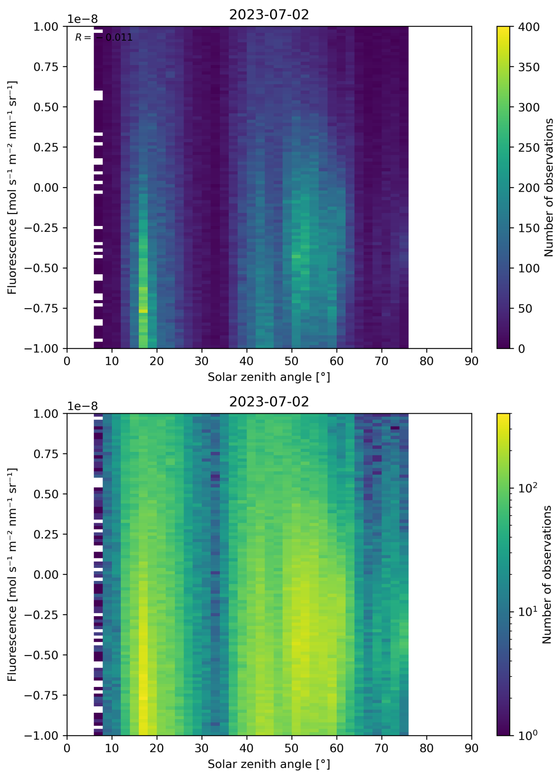
Figure 97: Scatter density plot of “Solar zenith angle” against “Fluorescence” for 2023-07-01 to 2023-07-03.
