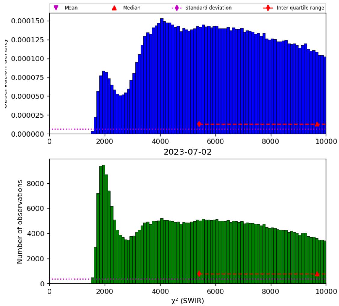
Figure 28: Histogram of “ \chi^2 (SWIR)” for 2023-07-01 to 2023-07-03
