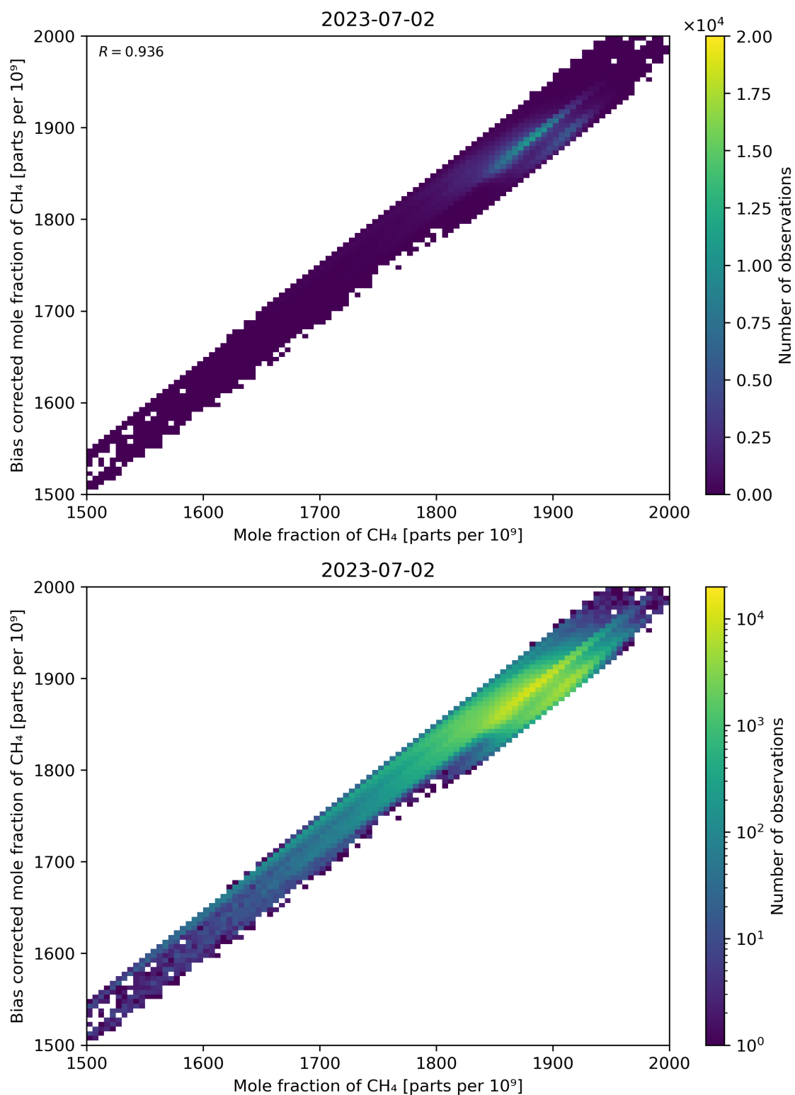
Figure 74: Scatter density plot of “Mole fraction of CH 4 ” against “Bias corrected mole fraction of CH 4 ” for 2023-07-01 to 2023-07-03.
