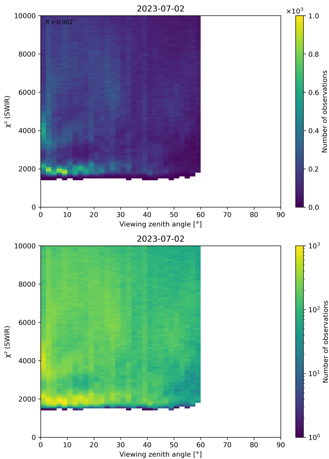
Figure 106: Scatter density plot of “Viewing zenith angle” against “ \chi^2 (SWIR)” for 2023-07-01 to 2023-07-03.
