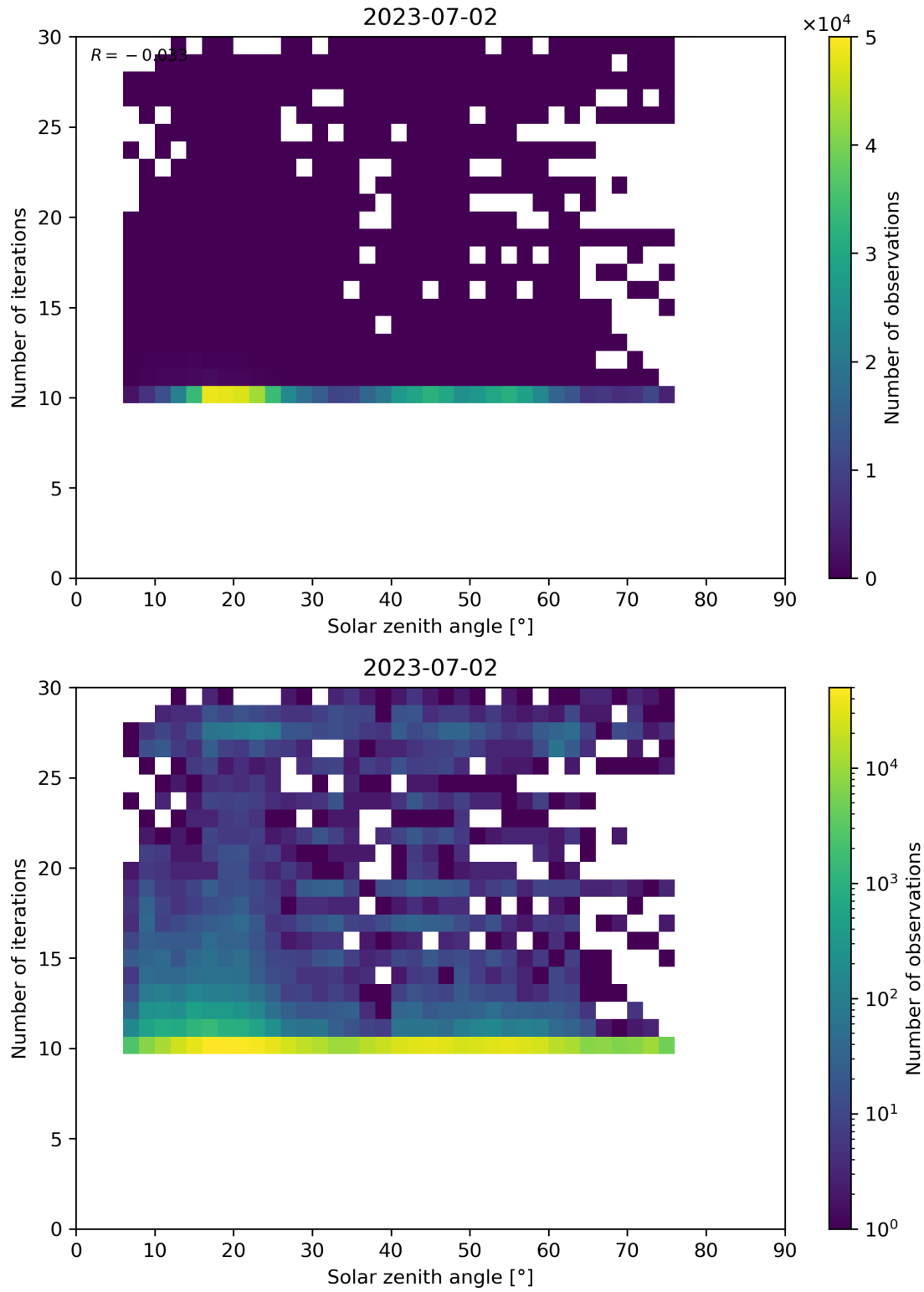
Figure 102: Scatter density plot of “Solar zenith angle” against “Number of iterations” for 2023-07-01 to 2023-07-03.
