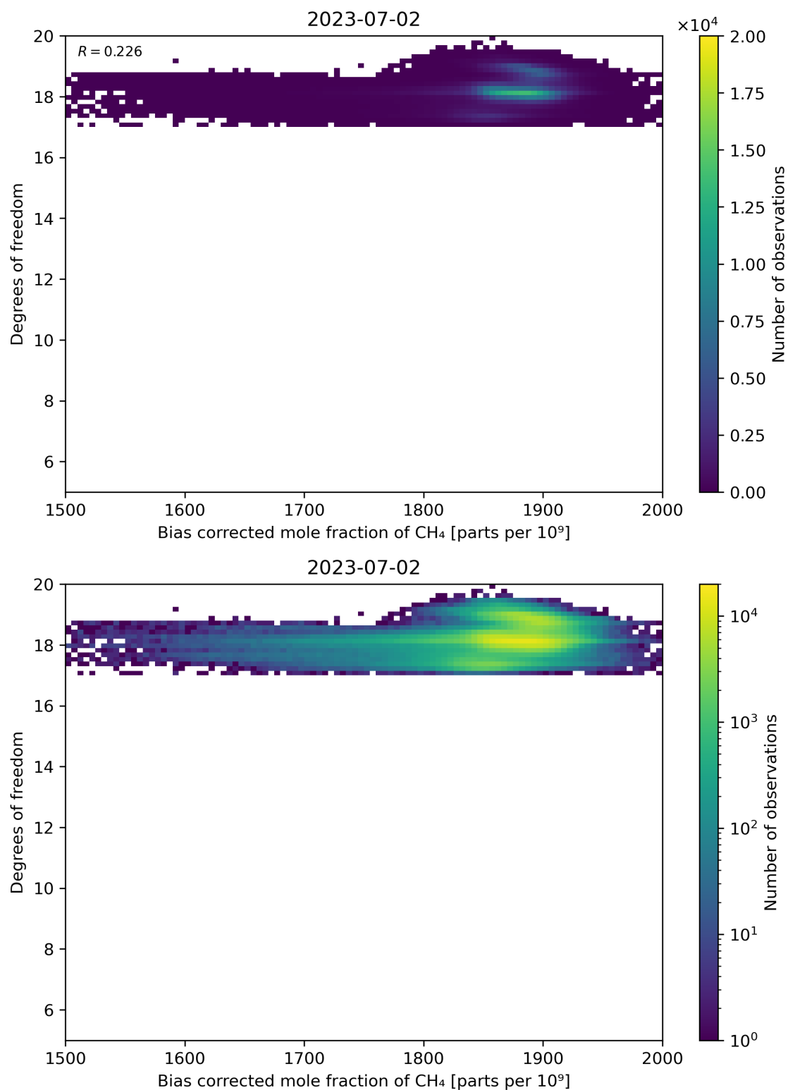
Figure 65: Scatter density plot of “Bias corrected mole fraction of CH 4 ” against “Degrees of freedom” for 2023-07-01 to 2023-07-03.
