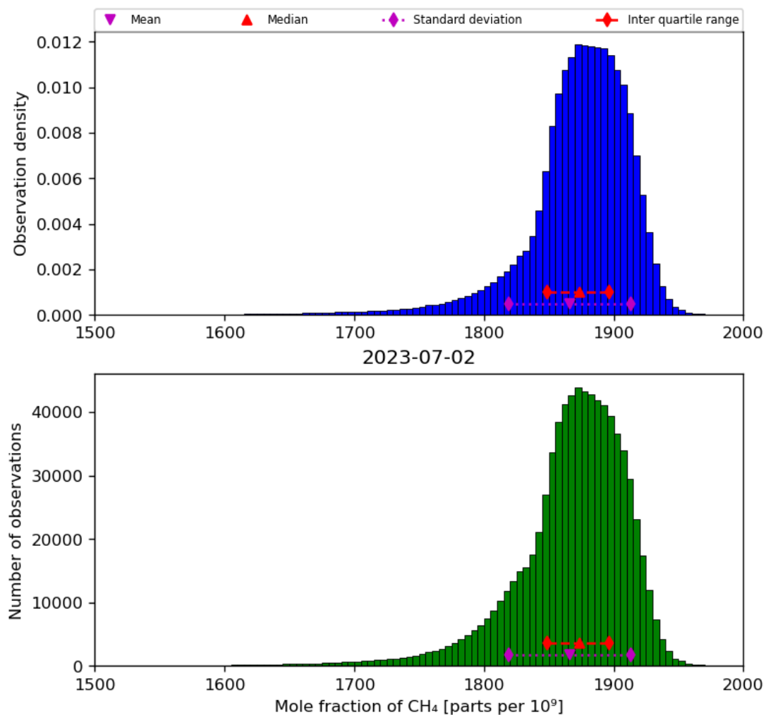
Figure 23: Histogram of “Mole fraction of CH 4 ” for 2023-07-01 to 2023-07-03
