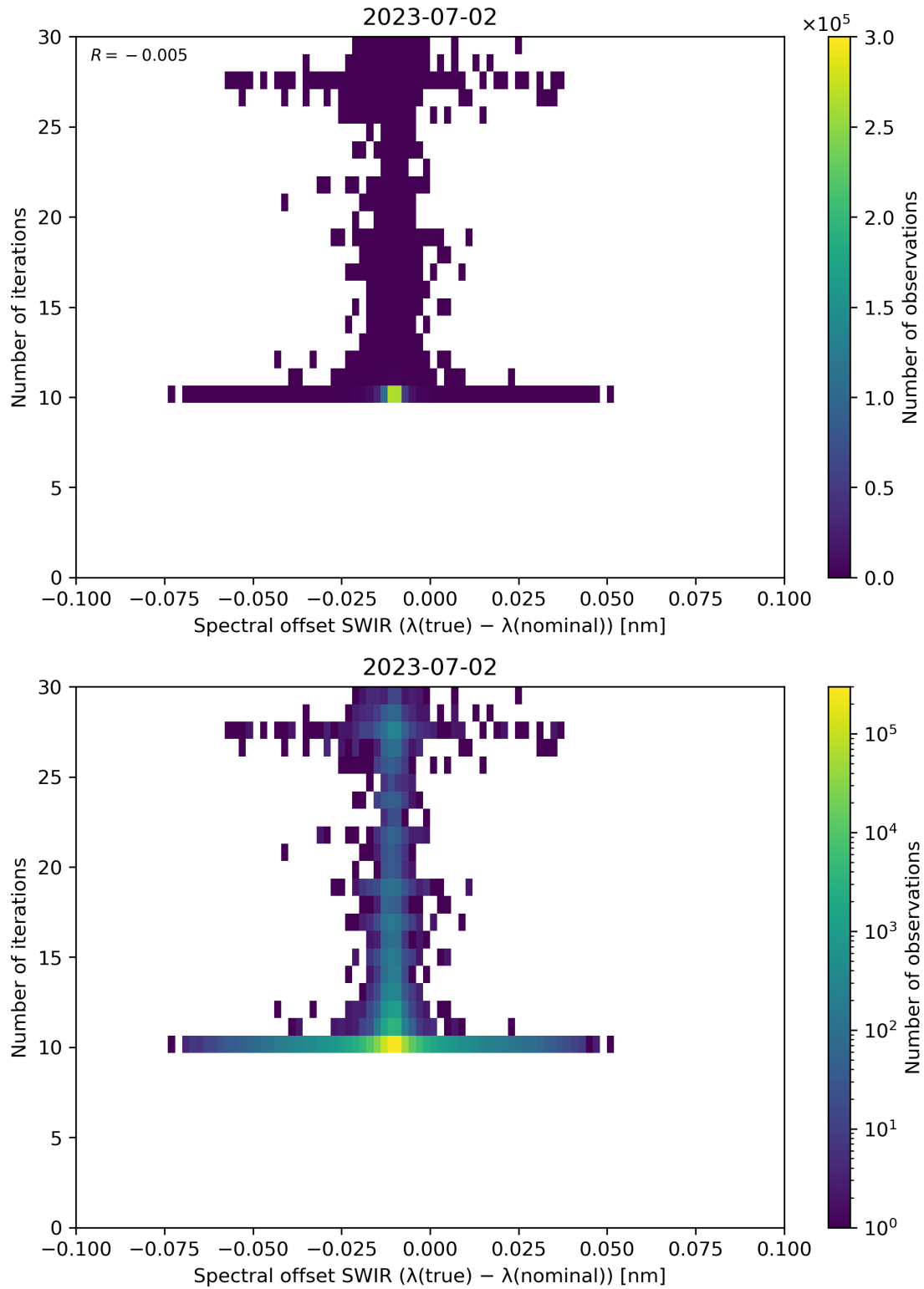
Figure 121: Scatter density plot of “Spectral offset SWIR ( \lambda(\text{true}) - \lambda(\text{nominal}) )” against “Number of iterations” for 2023-07-01 to 2023-07-03.
