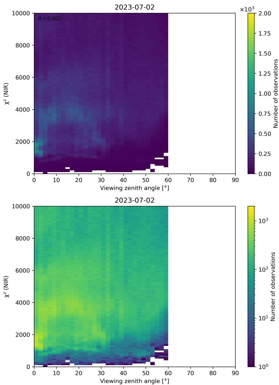
Figure 105: Scatter density plot of “Viewing zenith angle” against “ \chi^2 (NIR)” for 2023-07-01 to 2023-07-03.
