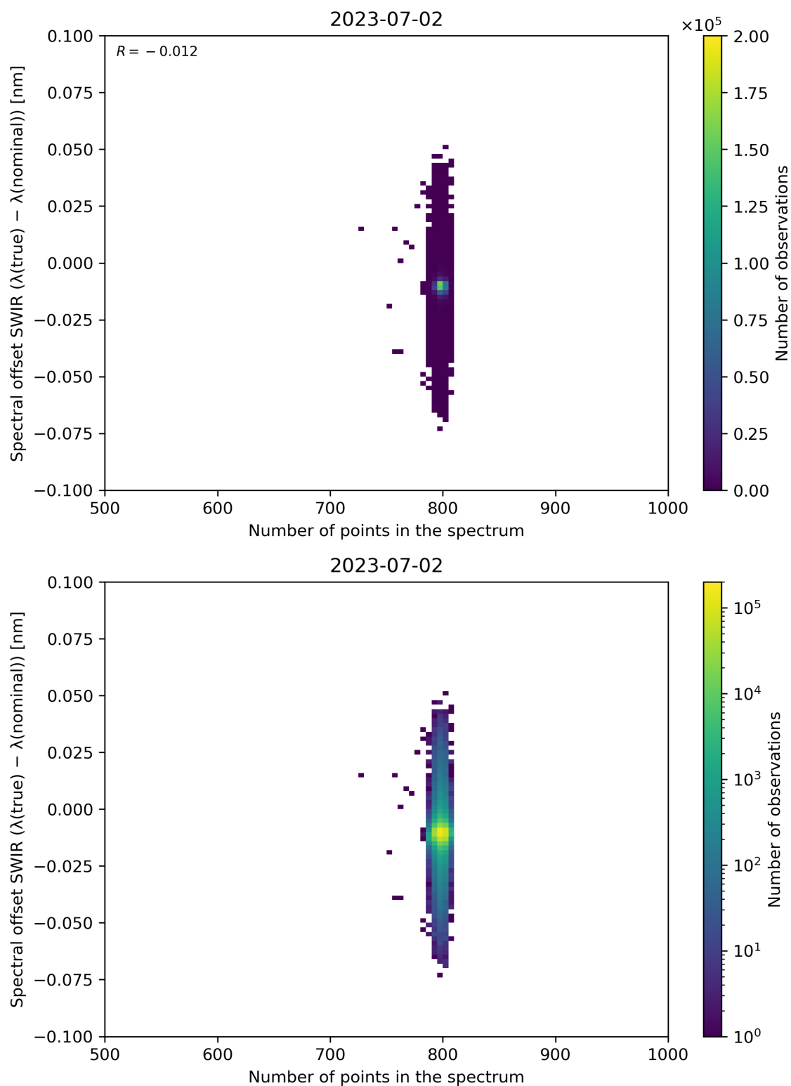
Figure 93: Scatter density plot of “Number of points in the spectrum” against “Spectral offset SWIR ( \lambda(\text{true}) - \lambda(\text{nominal}) )” for 2023-07-01 to 2023-07-03.
