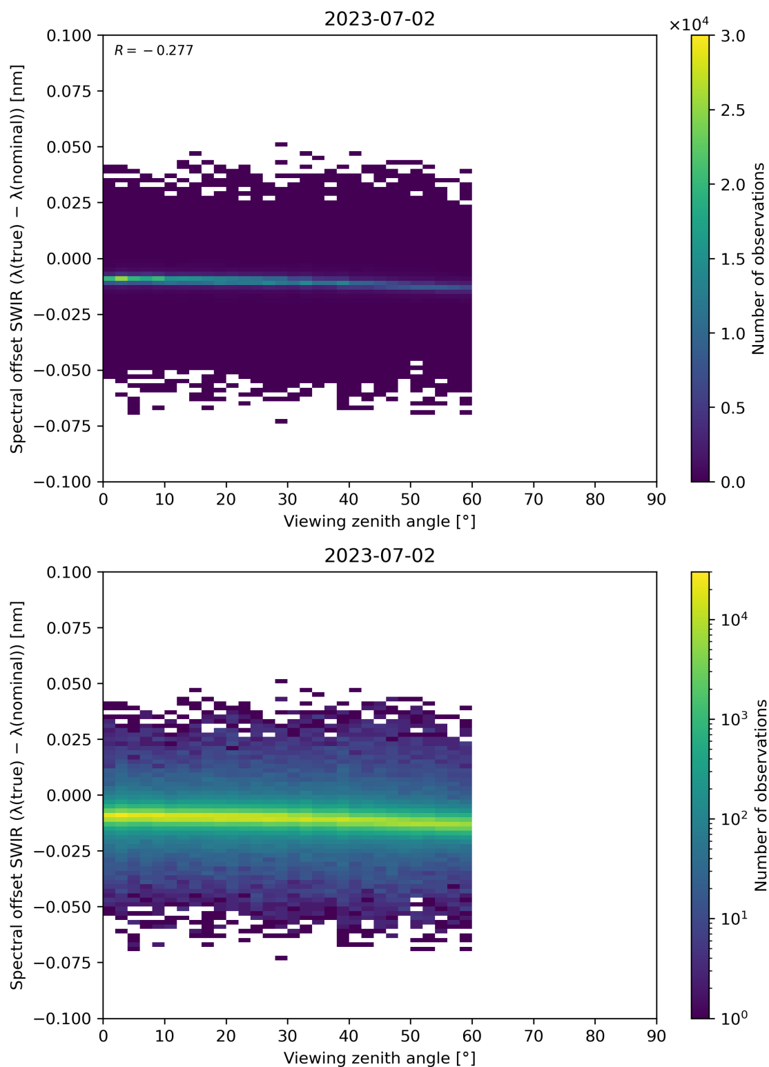
Figure 116: Scatter density plot of “Viewing zenith angle” against “Spectral offset SWIR ( \lambda(\text{true}) - \lambda(\text{nominal}) )” for 2023-07-01 to 2023-07-03.
