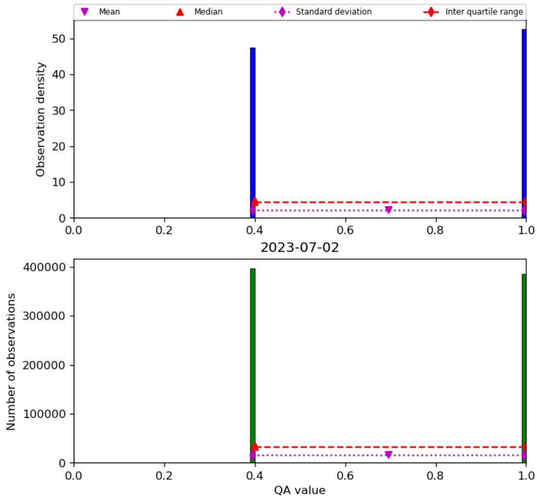
Figure 22: Histogram of “QA value” for 2023-07-01 to 2023-07-03
