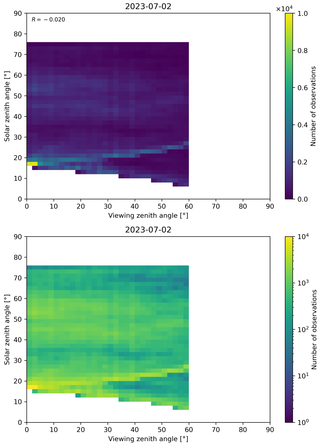
Figure 115: Scatter density plot of “Viewing zenith angle” against “Solar zenith angle” for 2023-07-01 to 2023-07-03.
