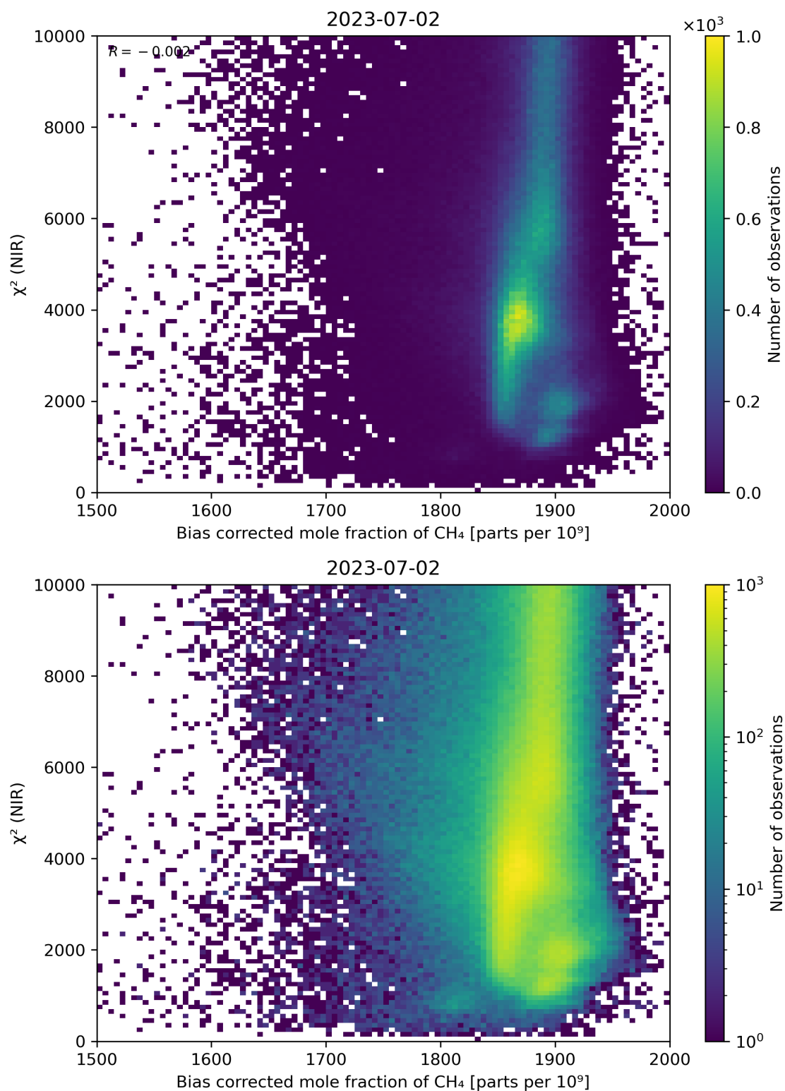
Figure 63: Scatter density plot of “Bias corrected mole fraction of CH 4 ” against “ \chi^2 (NIR)” for 2023-07-01 to 2023-07-03.
