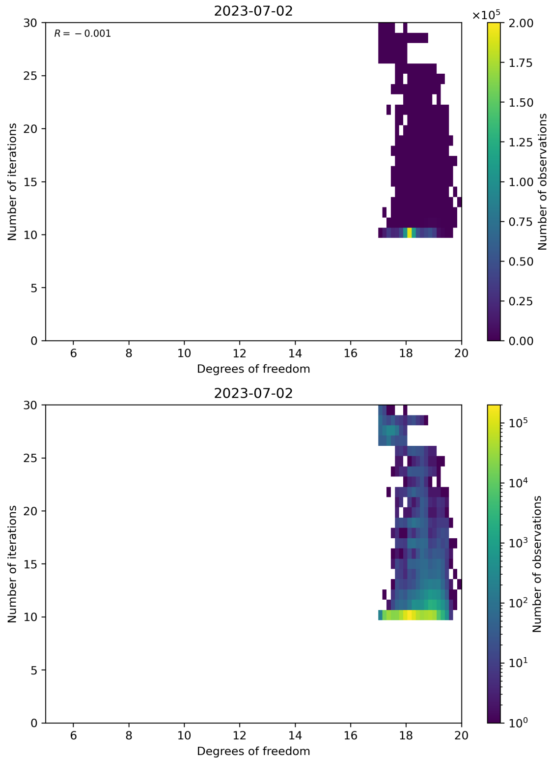
Figure 52: Scatter density plot of “Degrees of freedom” against “Number of iterations” for 2023-07-01 to 2023-07-03.
