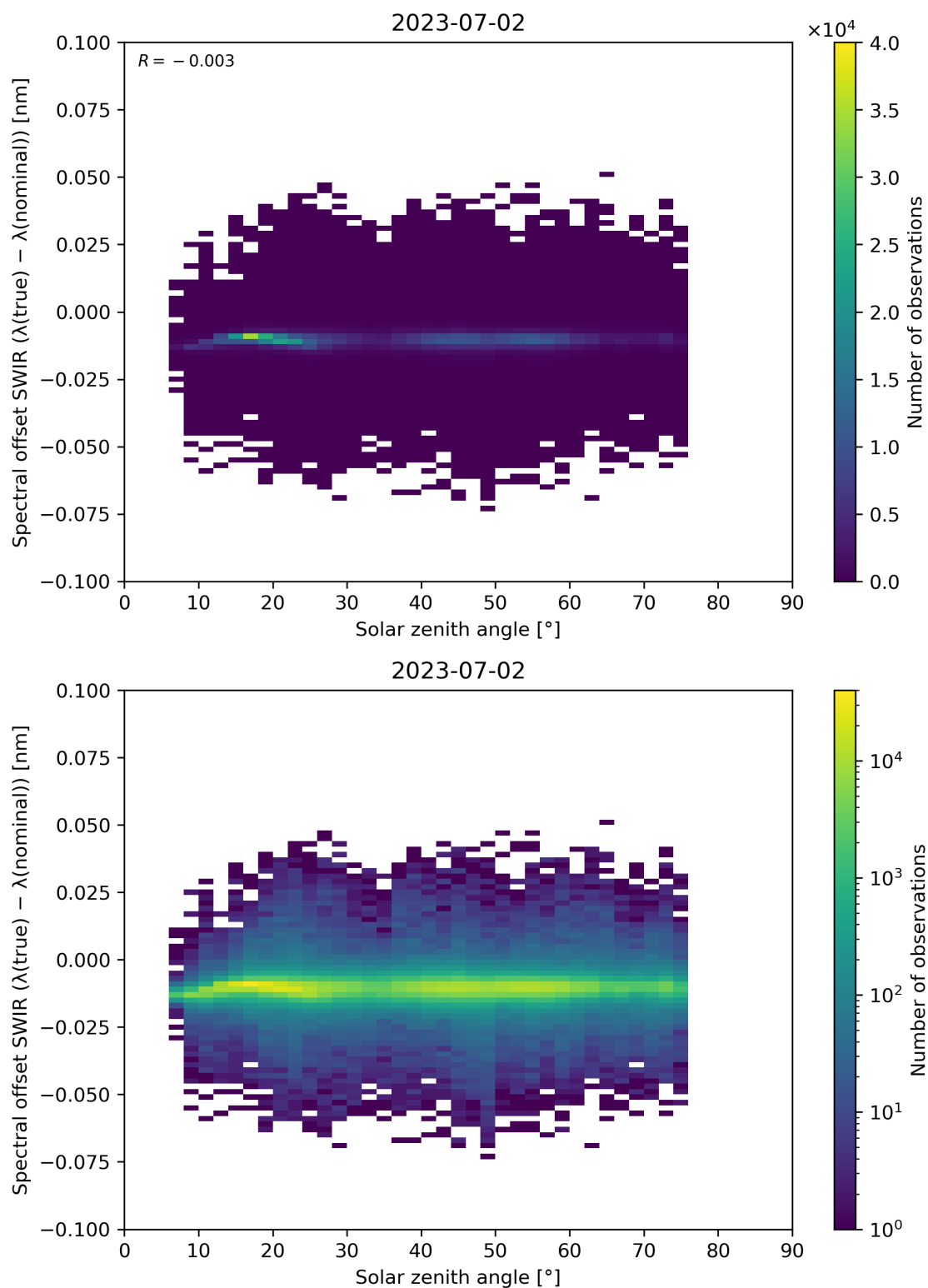
Figure 104: Scatter density plot of “Solar zenith angle” against “Spectral offset SWIR ( \lambda(\text{true}) - \lambda(\text{nominal}) )” for 2023-07-01 to 2023-07-03.
