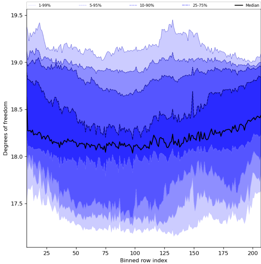
Figure 41: Along track statistics of “Degrees of freedom” for 2023-07-01 to 2023-07-03
