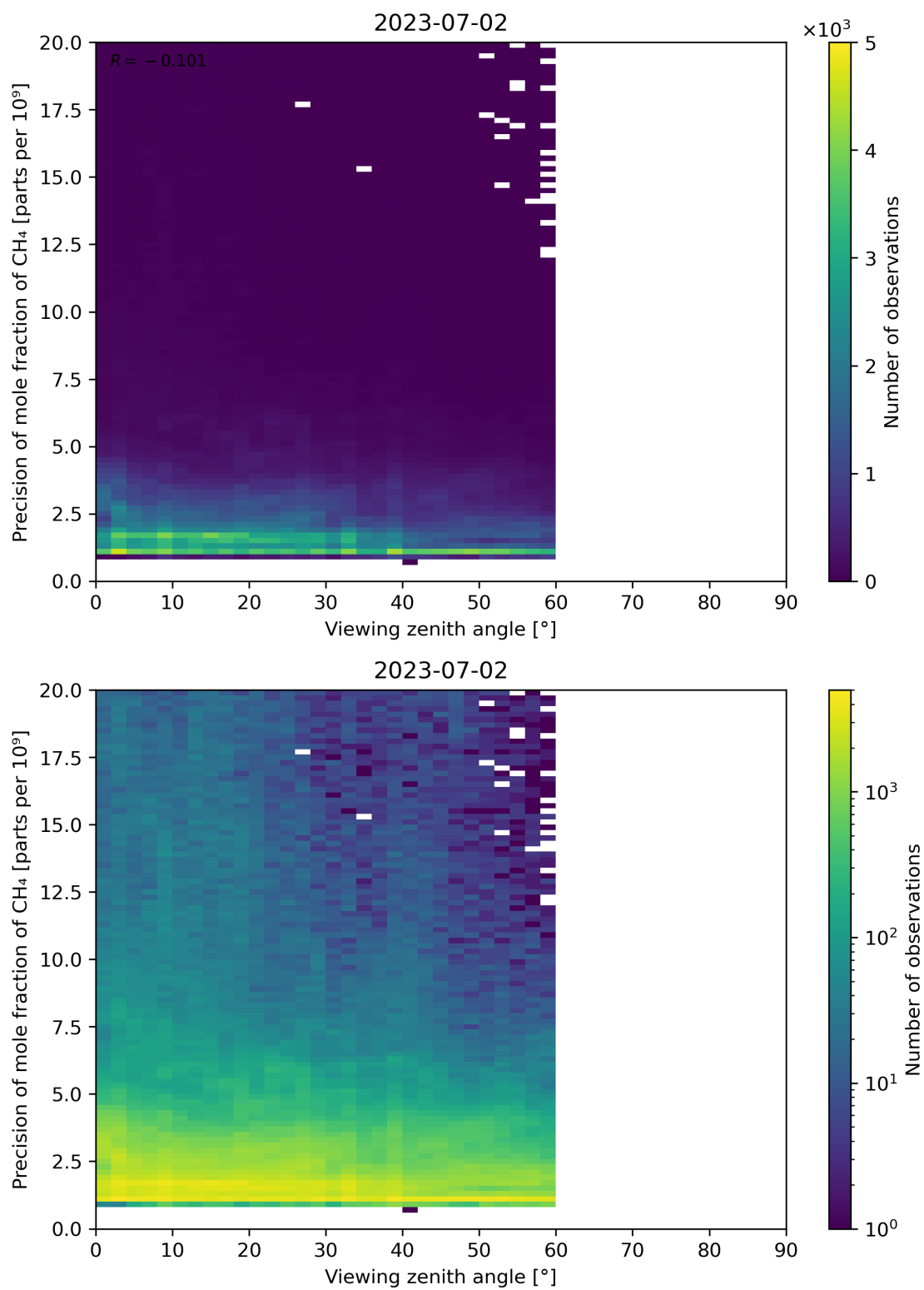
Figure 112: Scatter density plot of “Viewing zenith angle” against “Precision of mole fraction of CH 4 ” for 2023-07-01 to 2023-07-03.
