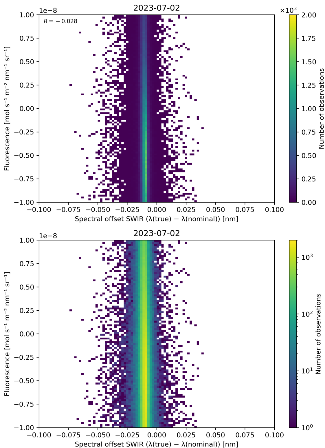
Figure 120: Scatter density plot of “Spectral offset SWIR ( \lambda(\text{true}) - \lambda(\text{nominal}) )” against “Fluorescence” for 2023-07-01 to 2023-07-03.
