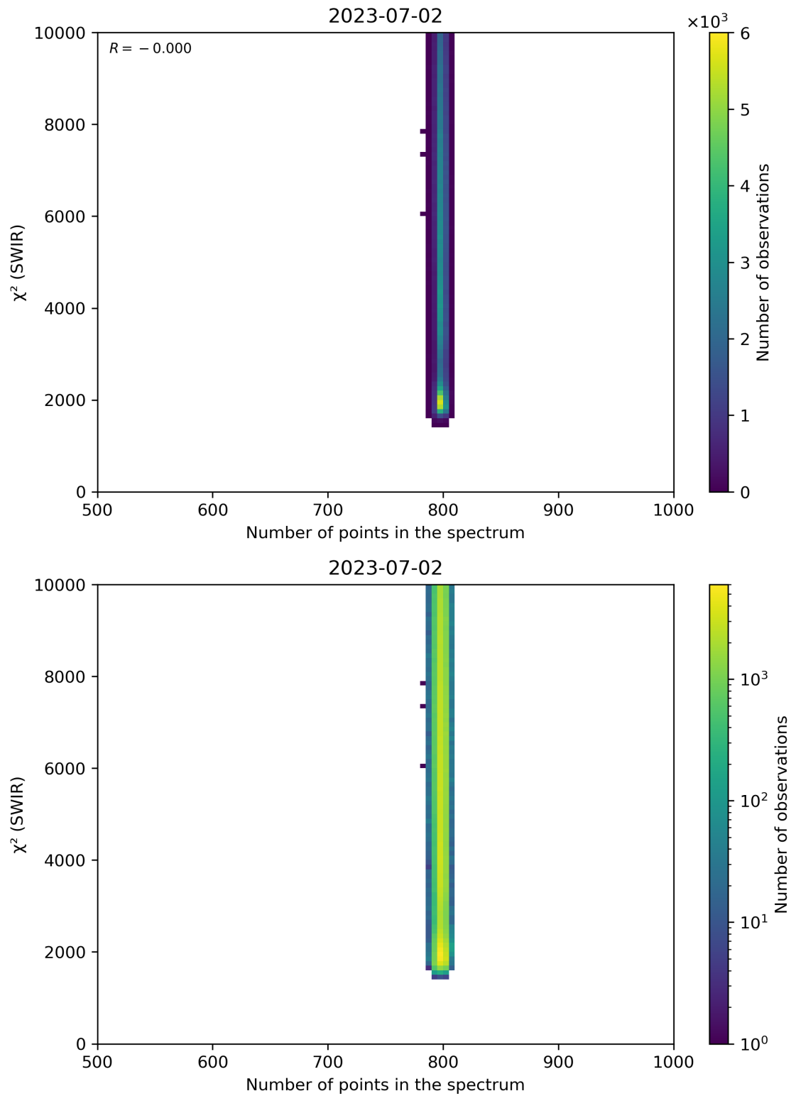
Figure 89: Scatter density plot of “Number of points in the spectrum” against “ \chi^2 (SWIR)” for 2023-07-01 to 2023-07-03.
