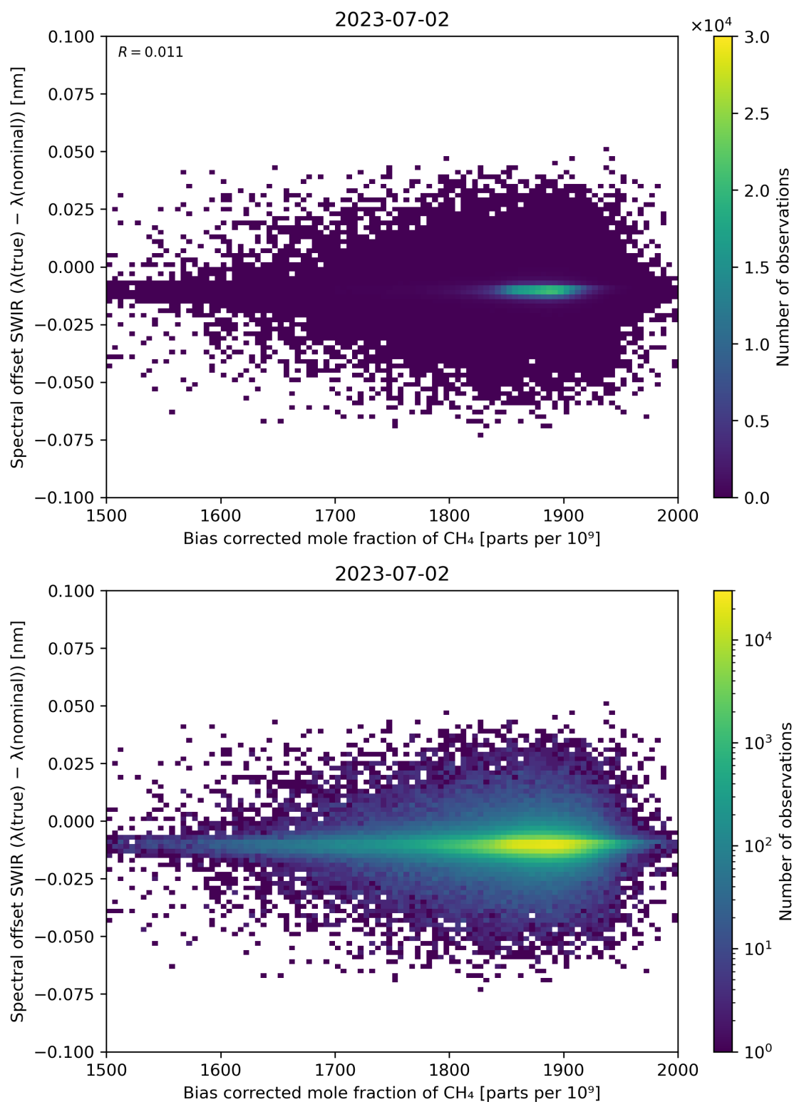
Figure 69: Scatter density plot of “Bias corrected mole fraction of \text{CH}_4 ” against “Spectral offset SWIR ( \lambda(\text{true}) - \lambda(\text{nominal}) )” for 2023-07-01 to 2023-07-03.
