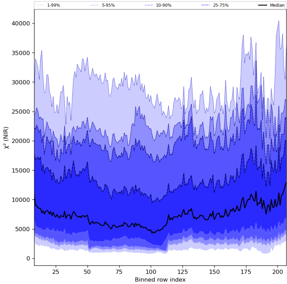
Figure 40: Along track statistics of “ \chi^2 (NIR)” for 2023-07-01 to 2023-07-03
