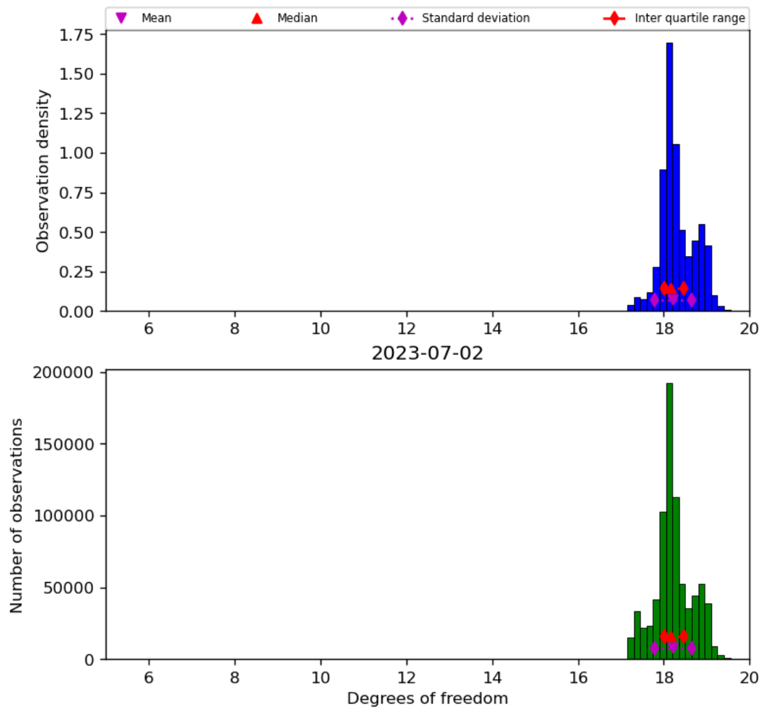
Figure 30: Histogram of “Degrees of freedom” for 2023-07-01 to 2023-07-03
