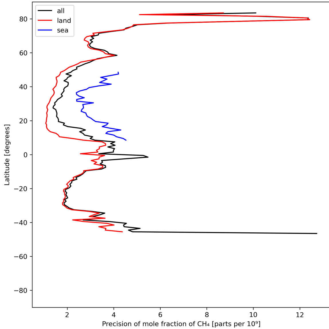
Figure 13: Zonal average of “Precision of mole fraction of CH 4 ” for 2023-07-01 to 2023-07-03.
