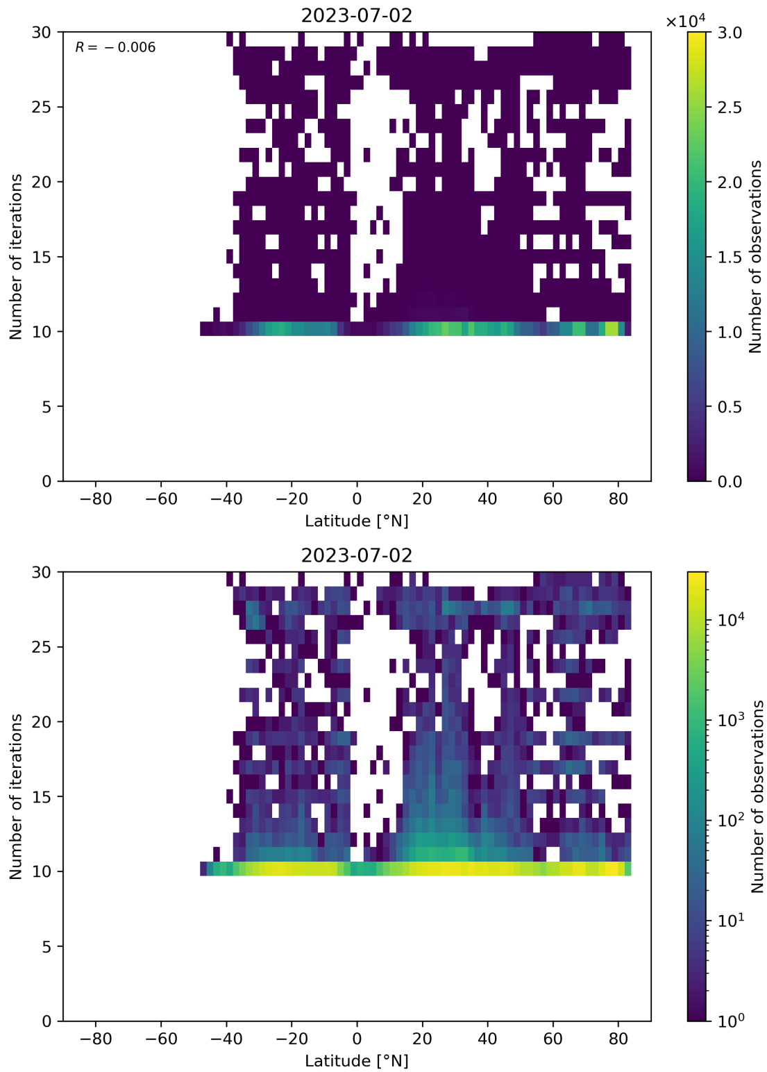
Figure 60: Scatter density plot of “Latitude” against “Number of iterations” for 2023-07-01 to 2023-07-03.
