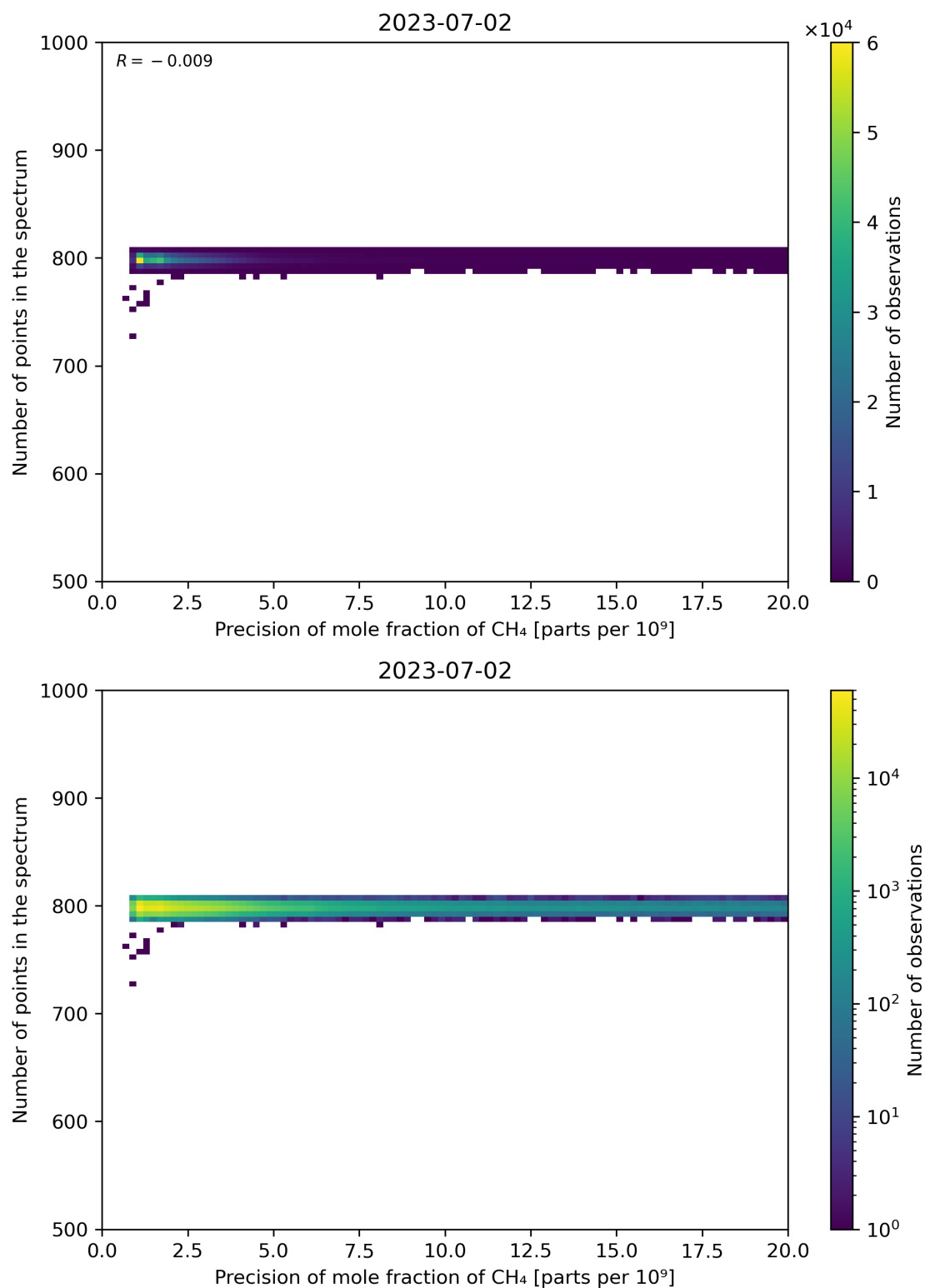
Figure 84: Scatter density plot of “Precision of mole fraction of CH 4 ” against “Number of points in the spectrum” for 2023-07-01 to 2023-07-03.
