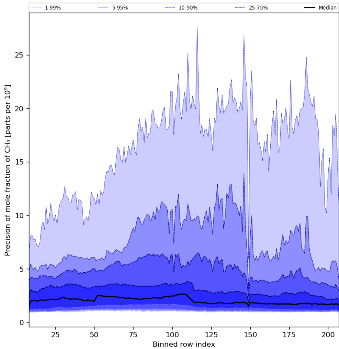
Figure 35: Along track statistics of “Precision of mole fraction of CH 4 ” for 2023-07-01 to 2023-07-03
