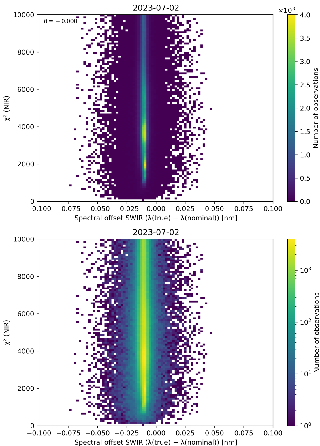
Figure 117: Scatter density plot of “Spectral offset SWIR ( \lambda(\text{true}) - \lambda(\text{nominal}) )” against “ \chi^2 (NIR)” for 2023-07-01 to 2023-07-03.
