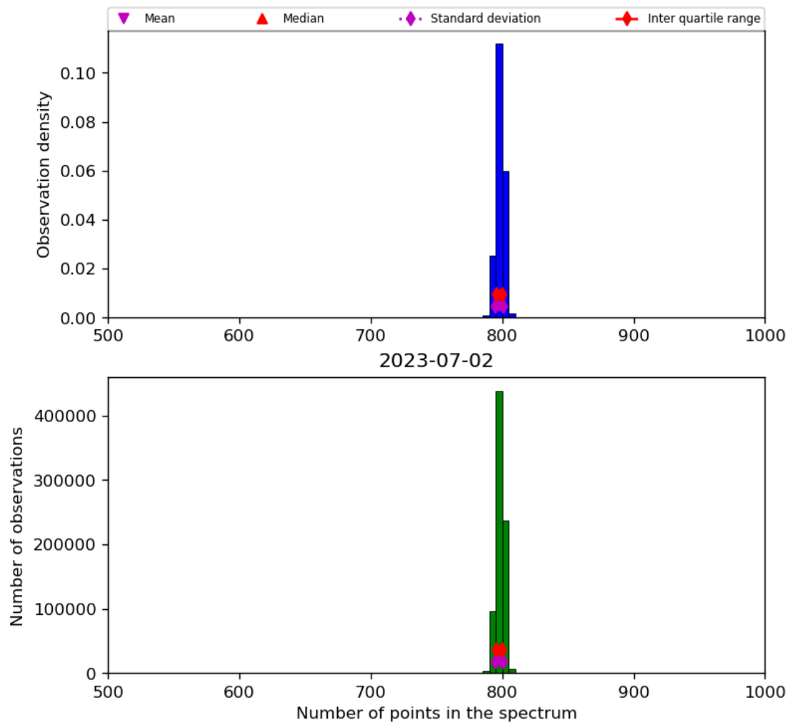
Figure 26: Histogram of “Number of points in the spectrum” for 2023-07-01 to 2023-07-03
