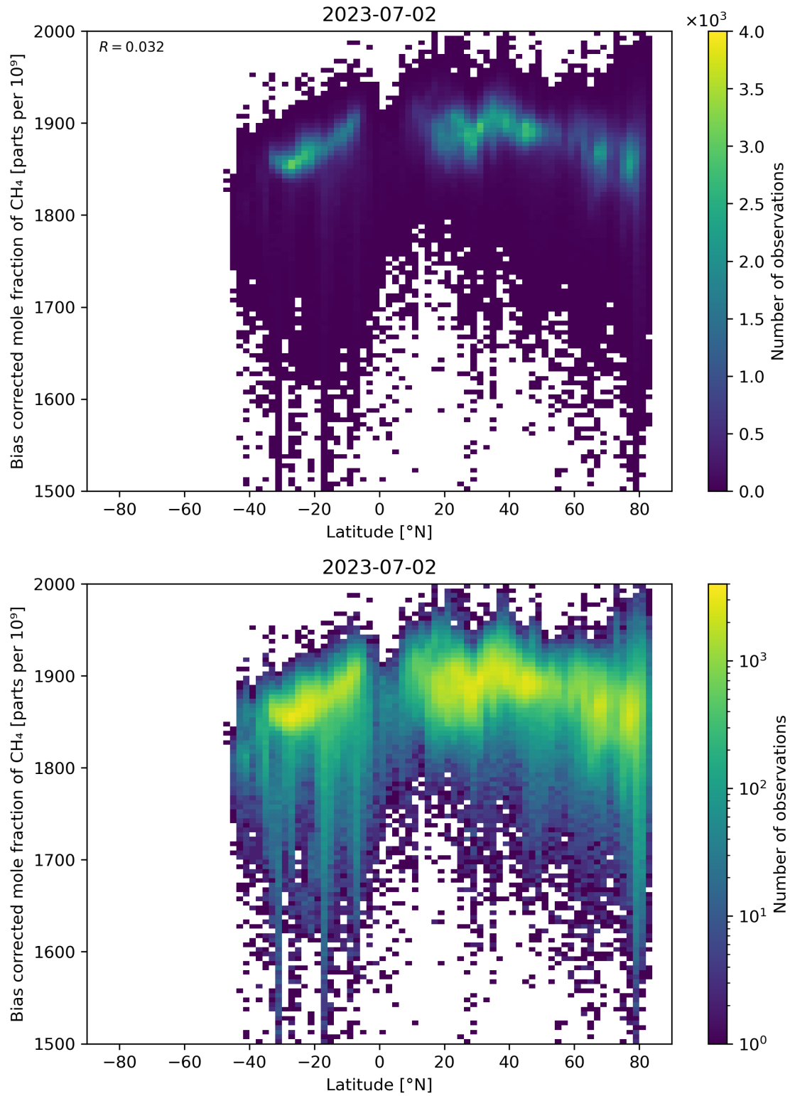
Figure 58: Scatter density plot of “Latitude” against “Bias corrected mole fraction of CH 4 ” for 2023-07-01 to 2023-07-03.
