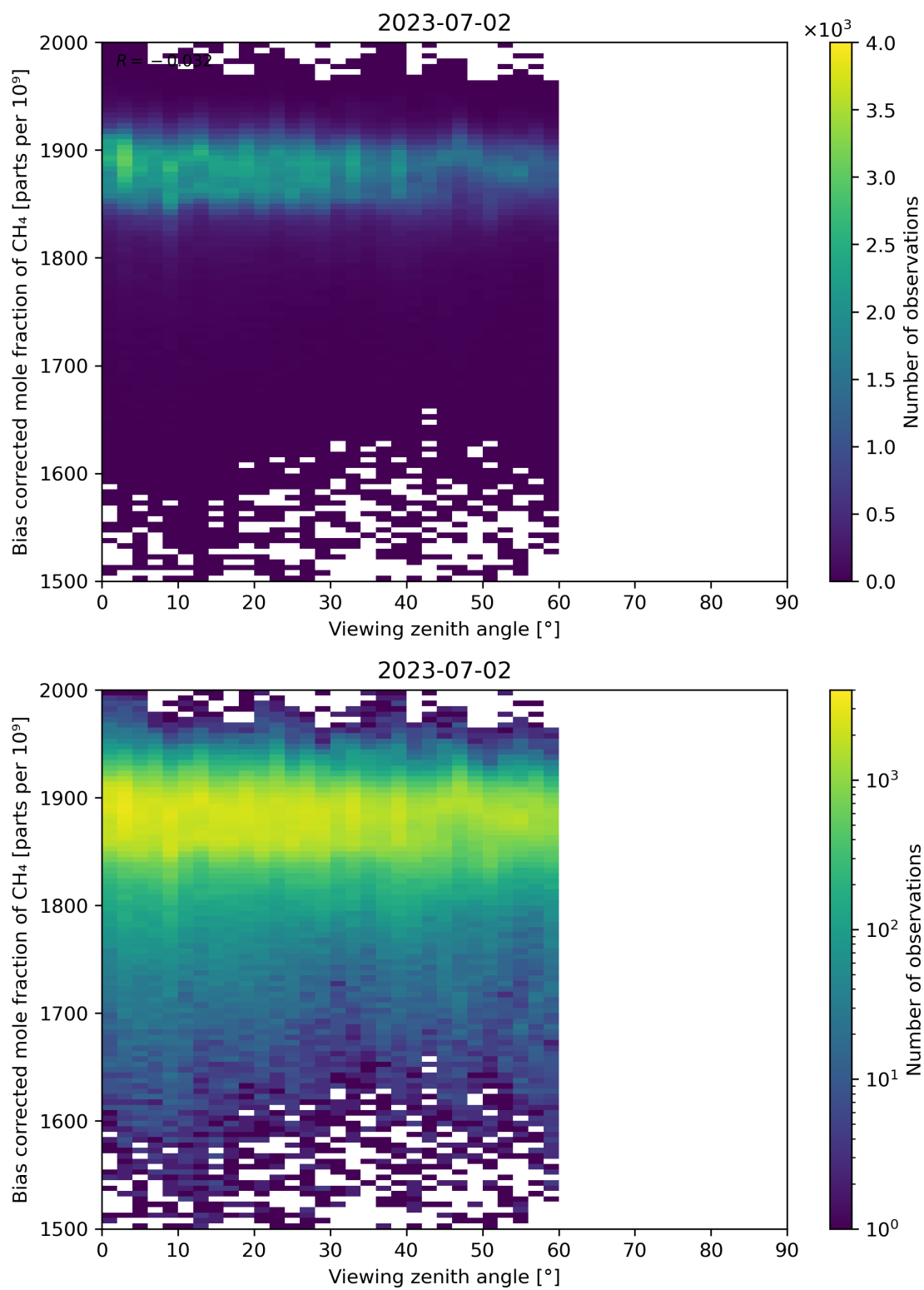
Figure 111: Scatter density plot of “Viewing zenith angle” against “Bias corrected mole fraction of CH 4 ” for 2023-07-01 to 2023-07-03.
