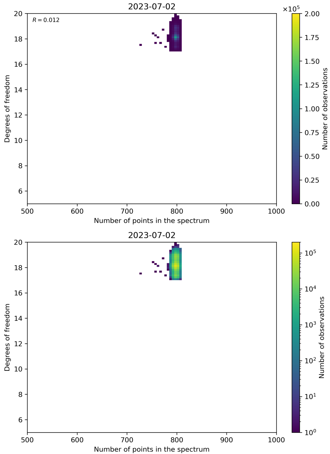
Figure 90: Scatter density plot of “Number of points in the spectrum” against “Degrees of freedom” for 2023-07-01 to 2023-07-03.
