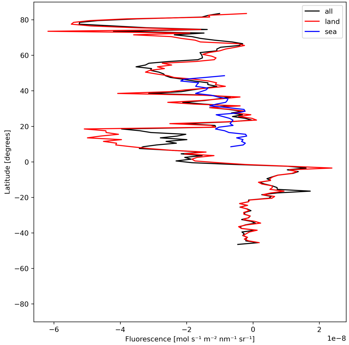
Figure 21: Zonal average of “Fluorescence” for 2023-07-01 to 2023-07-03.
