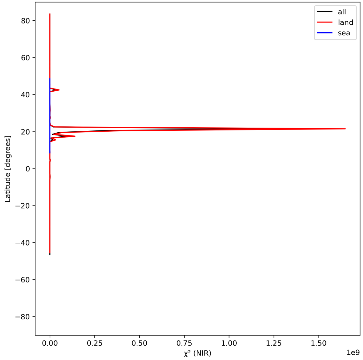
Figure 18: Zonal average of “ \chi^2 (NIR)” for 2023-07-01 to 2023-07-03.
