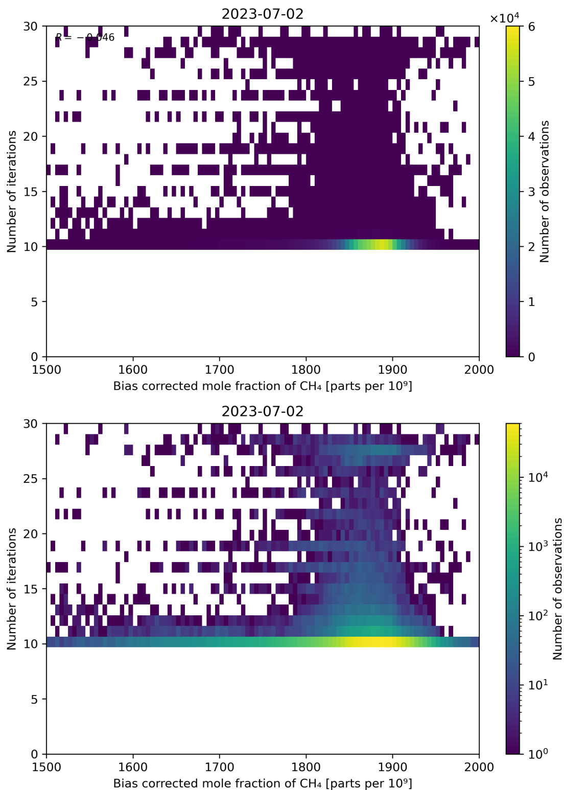
Figure 67: Scatter density plot of “Bias corrected mole fraction of CH 4 ” against “Number of iterations” for 2023-07-01 to 2023-07-03.
