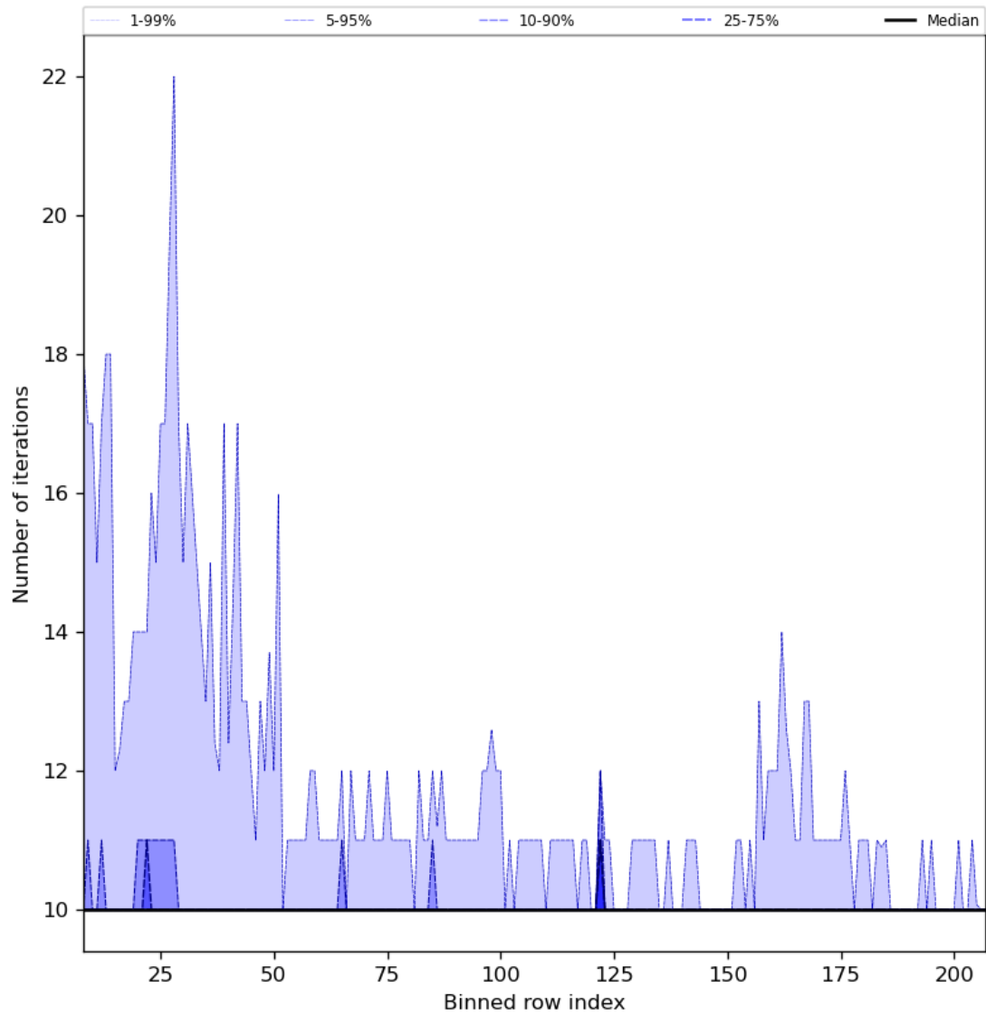
Figure 42: Along track statistics of “Number of iterations” for 2023-07-01 to 2023-07-03
