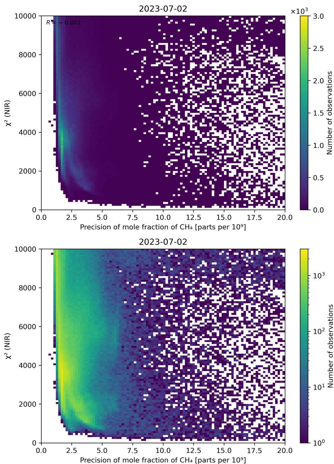
Figure 78: Scatter density plot of “Precision of mole fraction of CH 4 ” against “ \chi^2 (NIR)” for 2023-07-01 to 2023-07-03.
