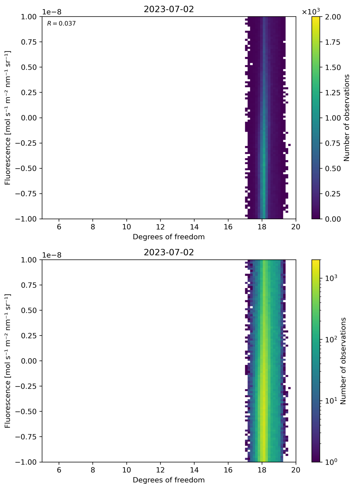
Figure 51: Scatter density plot of “Degrees of freedom” against “Fluorescence” for 2023-07-01 to 2023-07-03.
