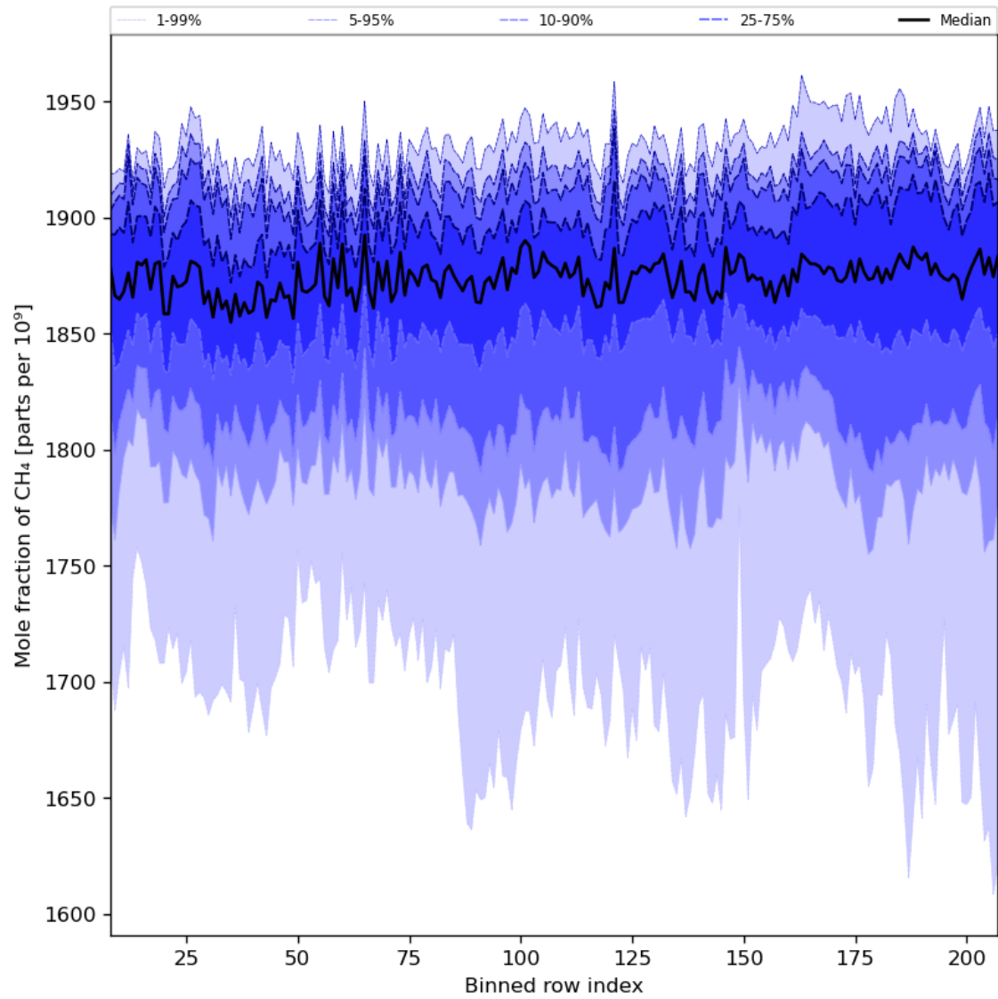
Figure 34: Along track statistics of “Mole fraction of CH 4 ” for 2023-07-01 to 2023-07-03
