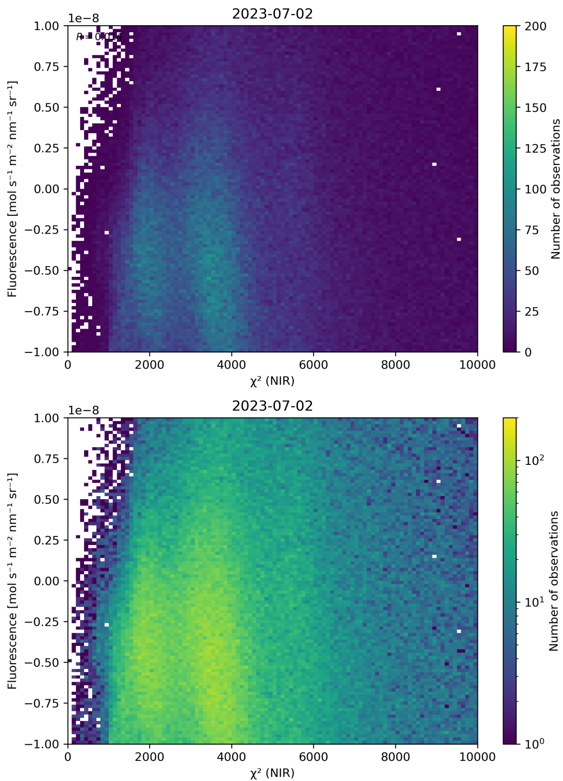
Figure 45: Scatter density plot of “ \chi^2 (NIR)” against “Fluorescence” for 2023-07-01 to 2023-07-03.
