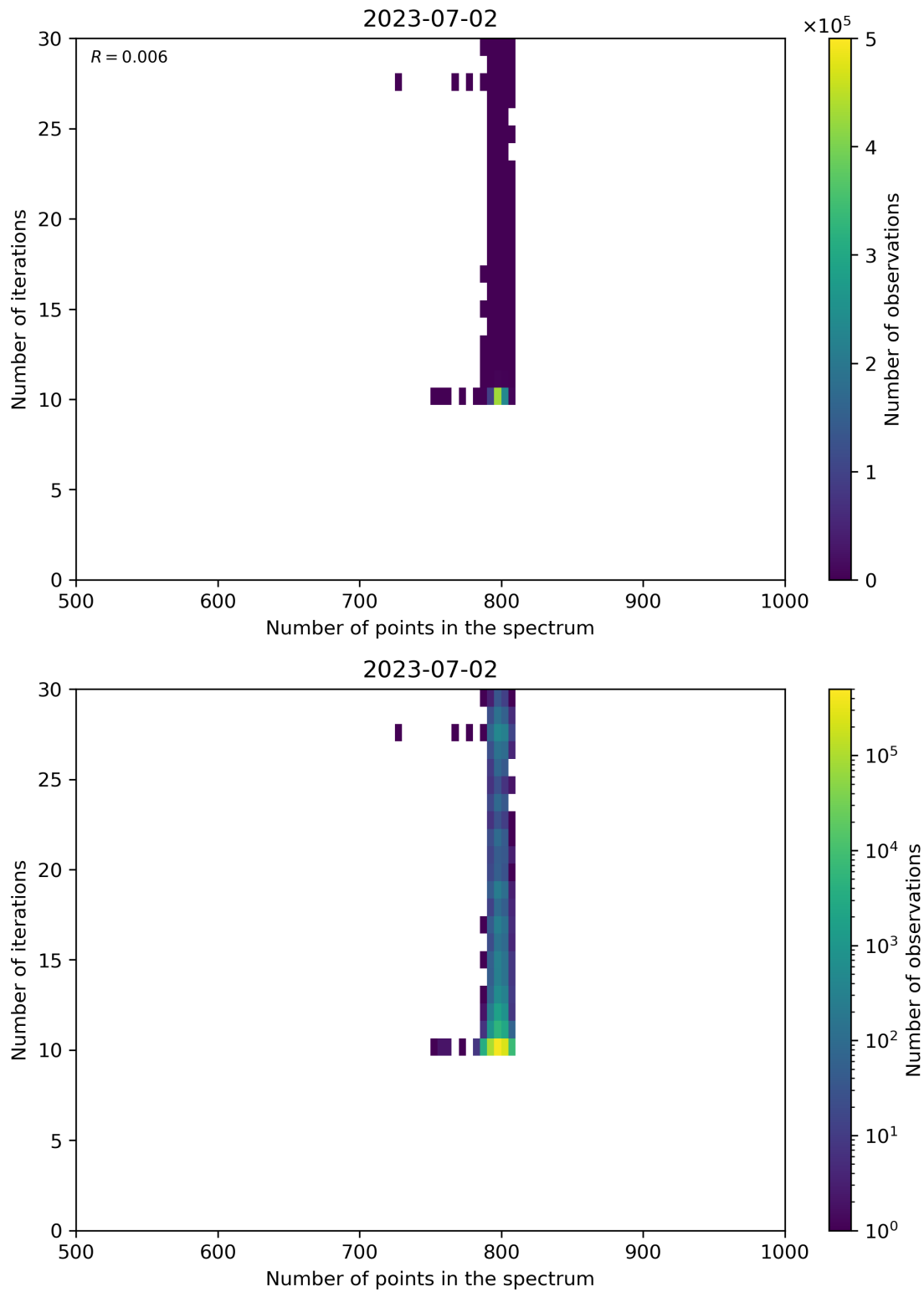
Figure 92: Scatter density plot of “Number of points in the spectrum” against “Number of iterations” for 2023-07-01 to 2023-07-03.
