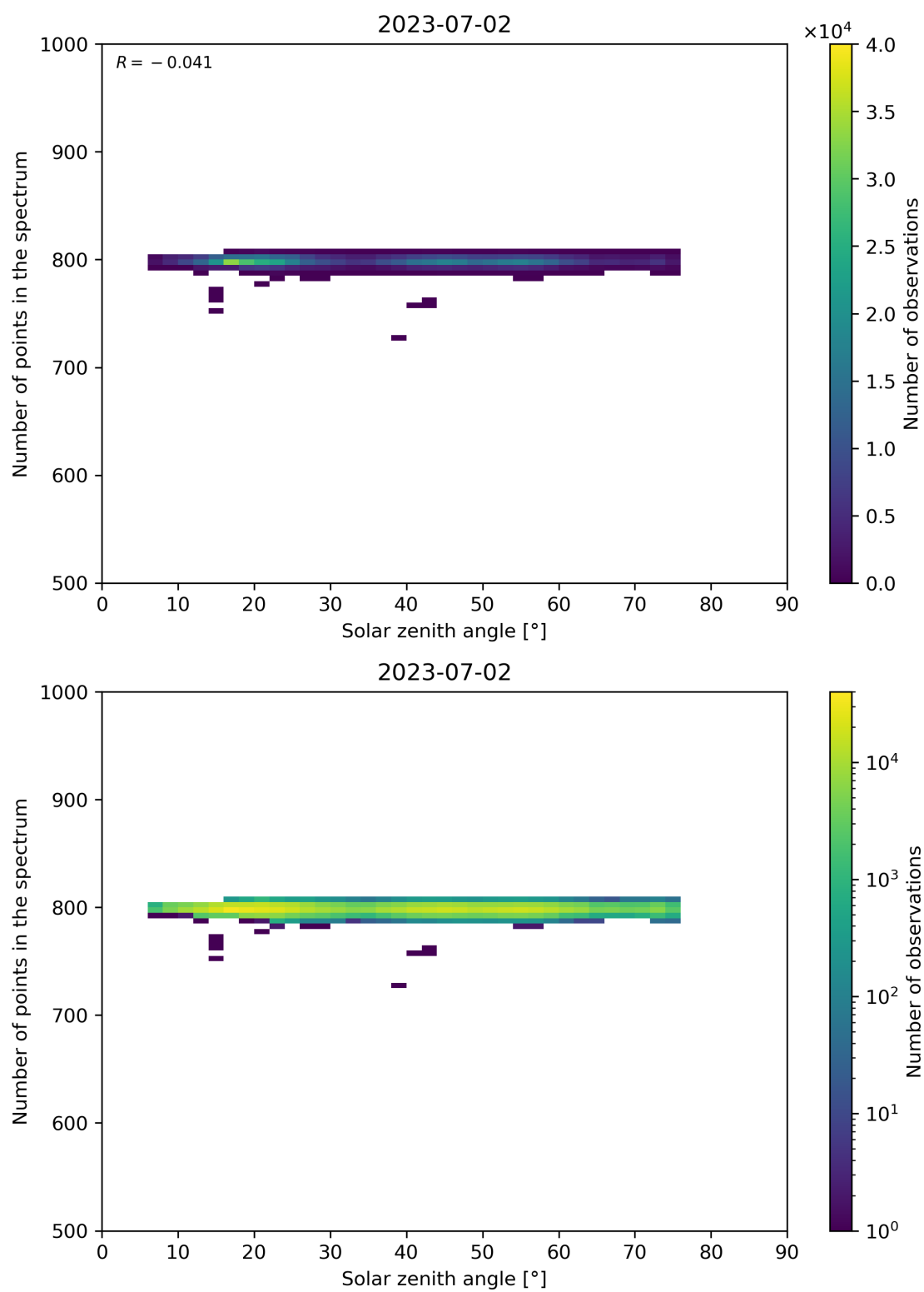
Figure 103: Scatter density plot of “Solar zenith angle” against “Number of points in the spectrum” for 2023-07-01 to 2023-07-03.
