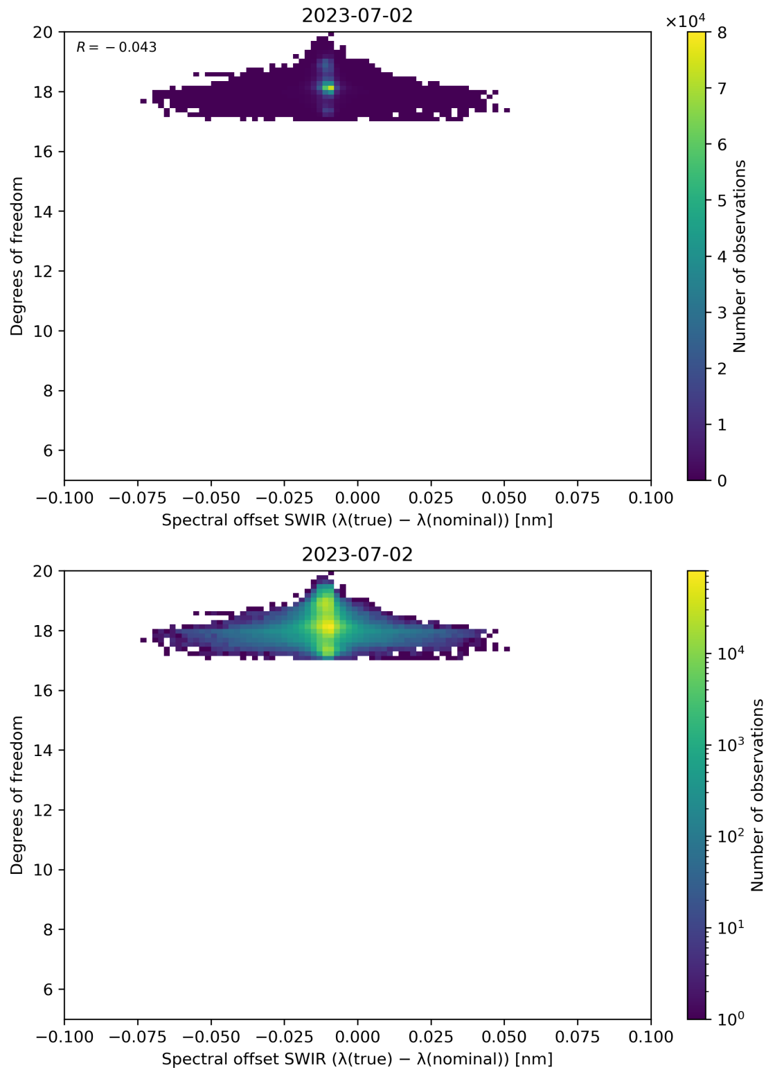
Figure 119: Scatter density plot of “Spectral offset SWIR ( \lambda(\text{true}) - \lambda(\text{nominal}) )” against “Degrees of freedom” for 2023-07-01 to 2023-07-03.
