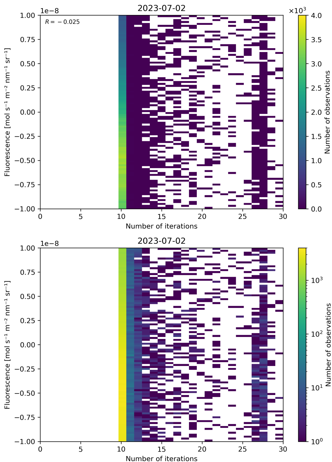
Figure 87: Scatter density plot of “Number of iterations” against “Fluorescence” for 2023-07-01 to 2023-07-03.
