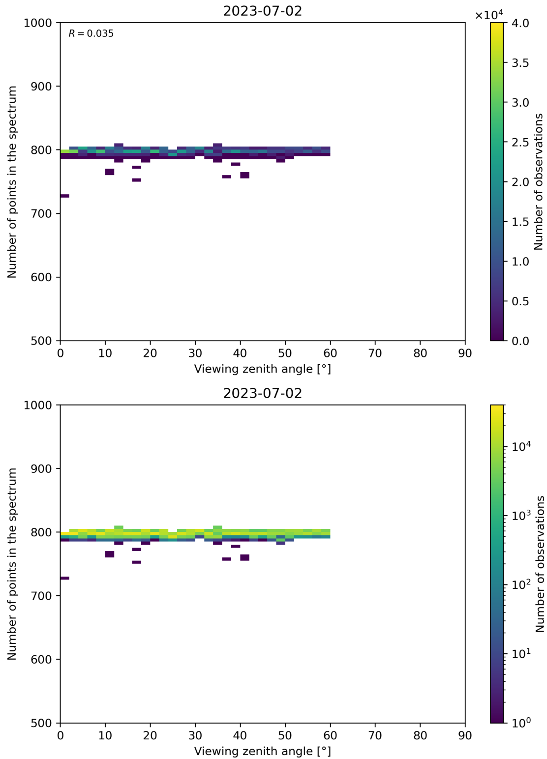
Figure 114: Scatter density plot of “Viewing zenith angle” against “Number of points in the spectrum” for 2023-07-01 to 2023-07-03.
