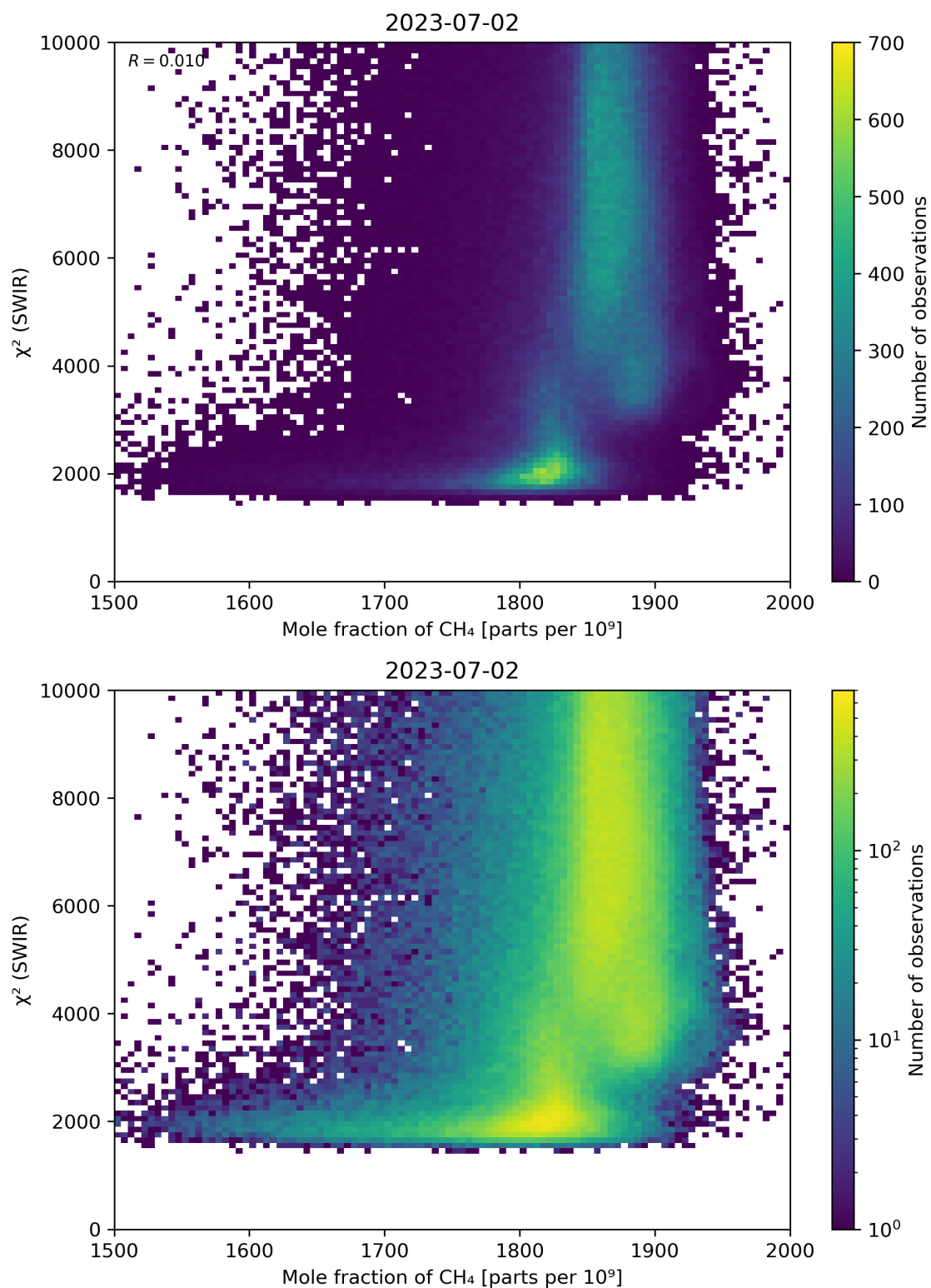
Figure 71: Scatter density plot of “Mole fraction of \text{CH}_4 ” against “ \chi^2 (SWIR)” for 2023-07-01 to 2023-07-03.
