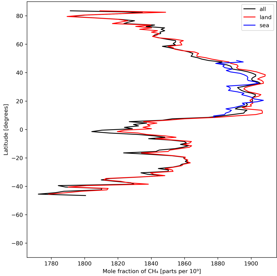
Figure 12: Zonal average of “Mole fraction of CH 4 ” for 2023-07-01 to 2023-07-03.
