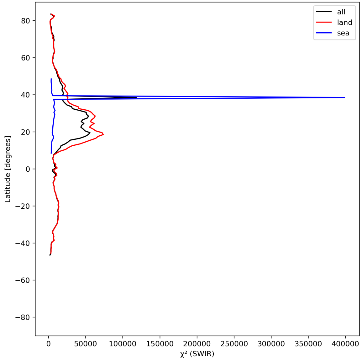
Figure 17: Zonal average of “ \chi^2 (SWIR)” for 2023-07-01 to 2023-07-03.
