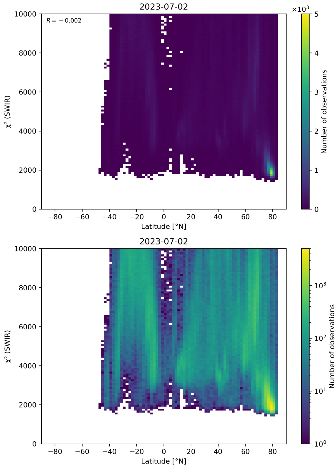
Figure 54: Scatter density plot of “Latitude” against “ \chi^2 (SWIR)” for 2023-07-01 to 2023-07-03.
