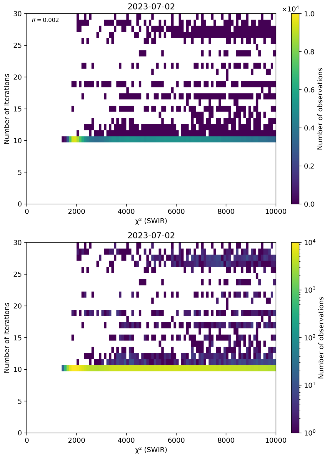
Figure 50: Scatter density plot of “ \chi^2 (SWIR)” against “Number of iterations” for 2023-07-01 to 2023-07-03.
