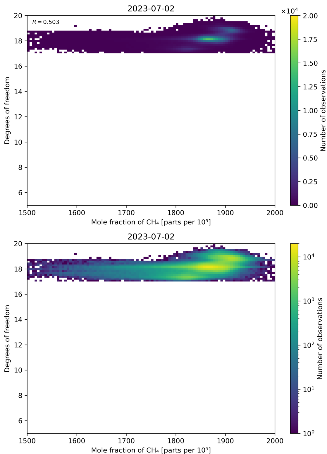
Figure 72: Scatter density plot of “Mole fraction of CH 4 ” against “Degrees of freedom” for 2023-07-01 to 2023-07-03.
