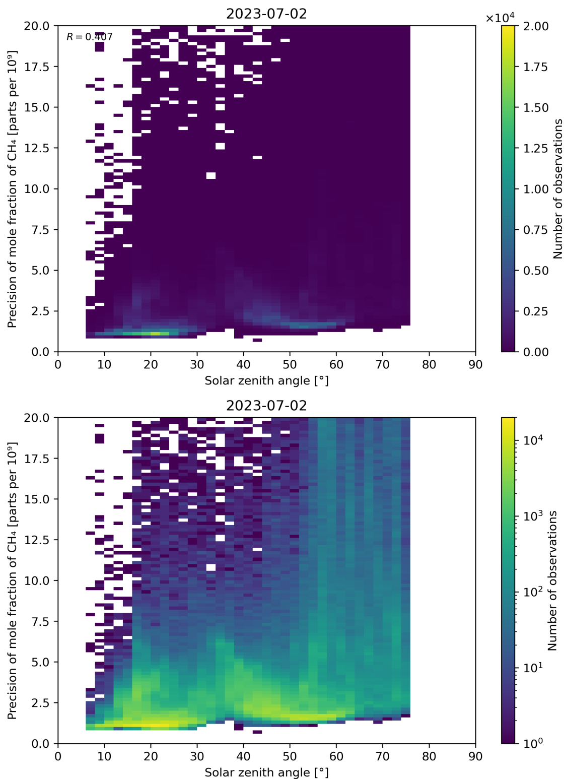
Figure 101: Scatter density plot of “Solar zenith angle” against “Precision of mole fraction of CH 4 ” for 2023-07-01 to 2023-07-03.
