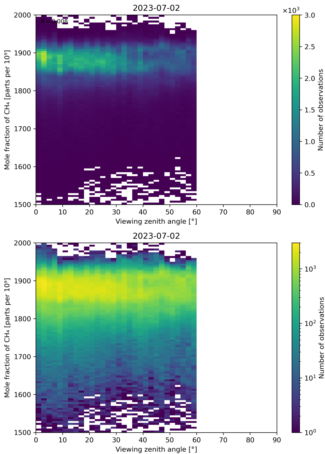
Figure 110: Scatter density plot of “Viewing zenith angle” against “Mole fraction of CH 4 ” for 2023-07-01 to 2023-07-03.
