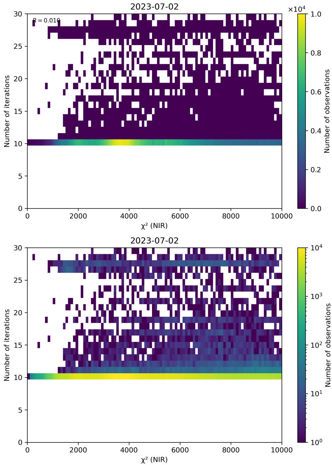
Figure 46: Scatter density plot of “ \chi^2 (NIR)” against “Number of iterations” for 2023-07-01 to 2023-07-03.
