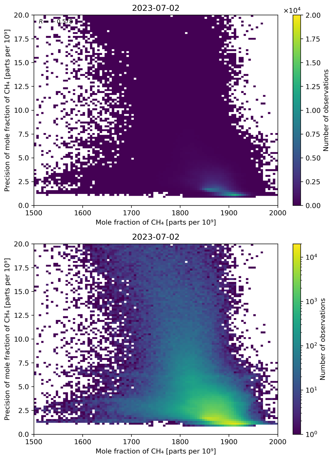
Figure 75: Scatter density plot of “Mole fraction of CH 4 ” against “Precision of mole fraction of CH 4 ” for 2023-07-01 to 2023-07-03.
