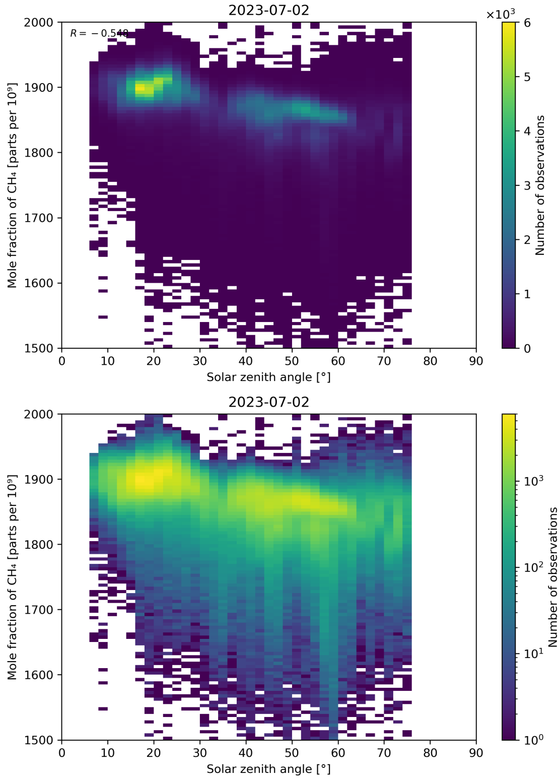
Figure 99: Scatter density plot of “Solar zenith angle” against “Mole fraction of CH 4 ” for 2023-07-01 to 2023-07-03.
