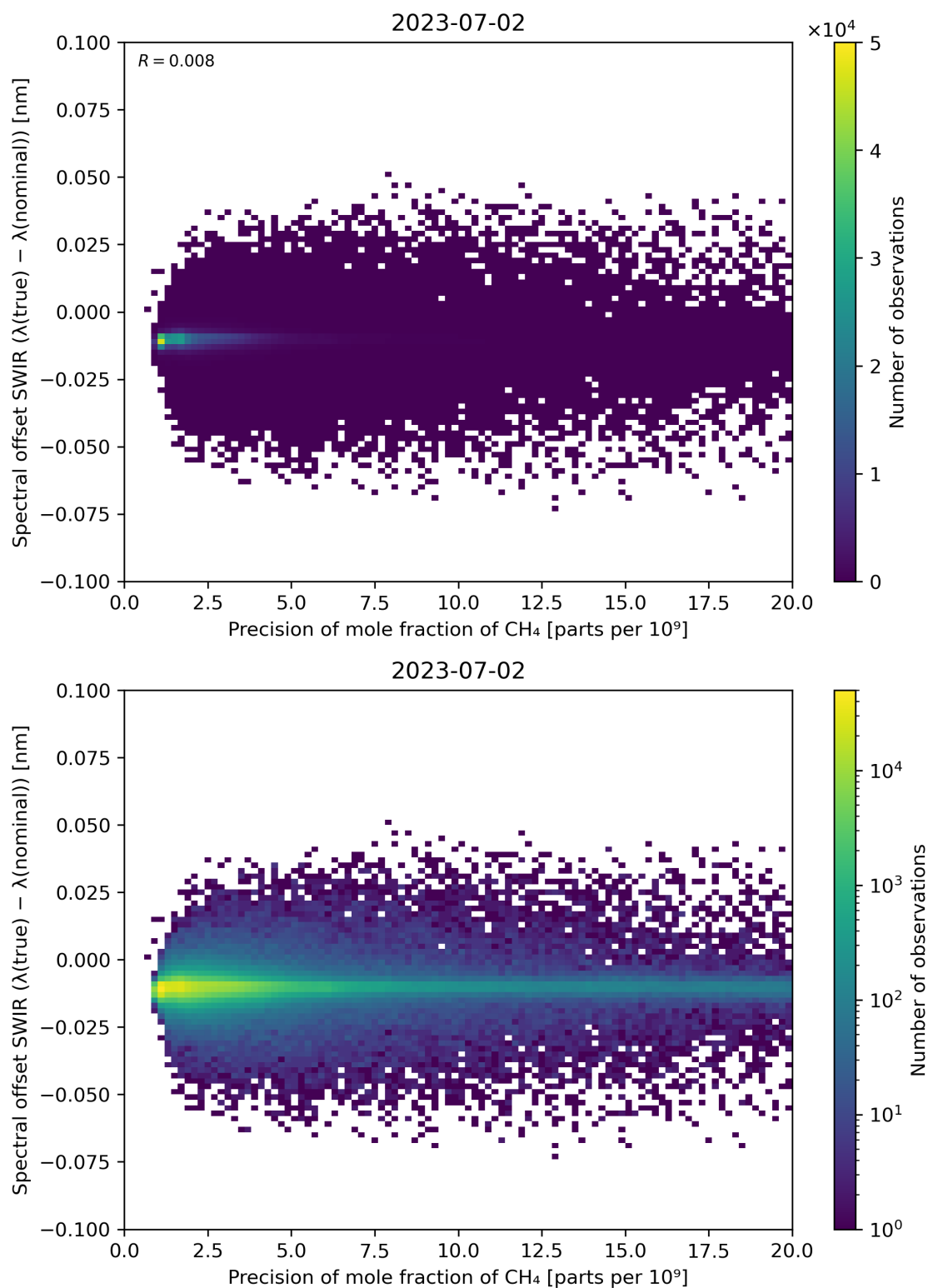
Figure 85: Scatter density plot of “Precision of mole fraction of CH 4 ” against “Spectral offset SWIR ( \lambda(\text{true}) - \lambda(\text{nominal}) )” for 2023-07-01 to 2023-07-03.
