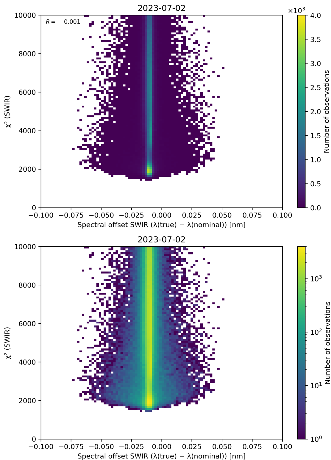
Figure 118: Scatter density plot of “Spectral offset SWIR ( \lambda(\text{true}) - \lambda(\text{nominal}) )” against “ \chi^2 (SWIR)” for 2023-07-01 to 2023-07-03.
