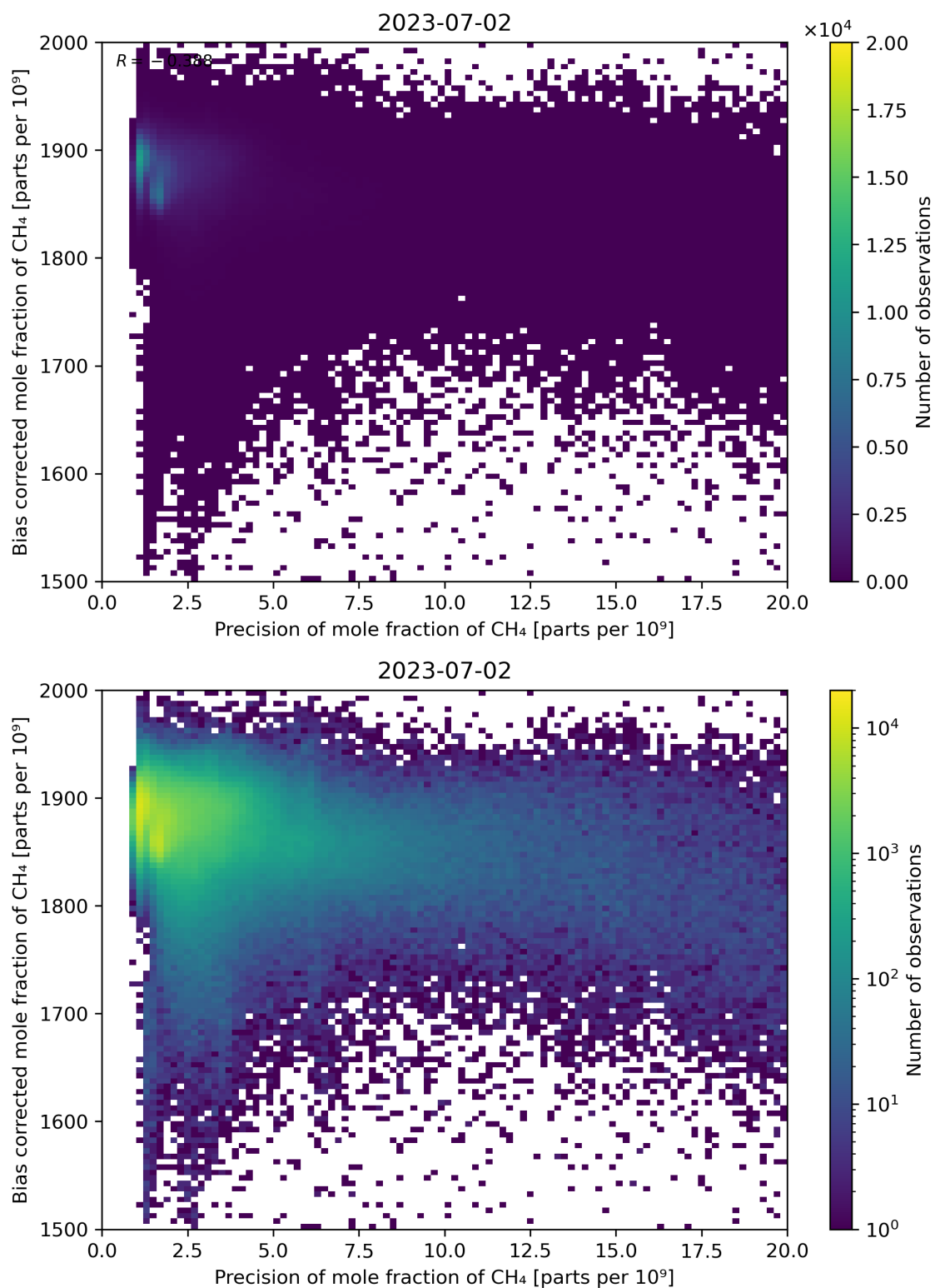
Figure 82: Scatter density plot of “Precision of mole fraction of \text{CH}_4 ” against “Bias corrected mole fraction of \text{CH}_4 ” for 2023-07-01 to 2023-07-03.
