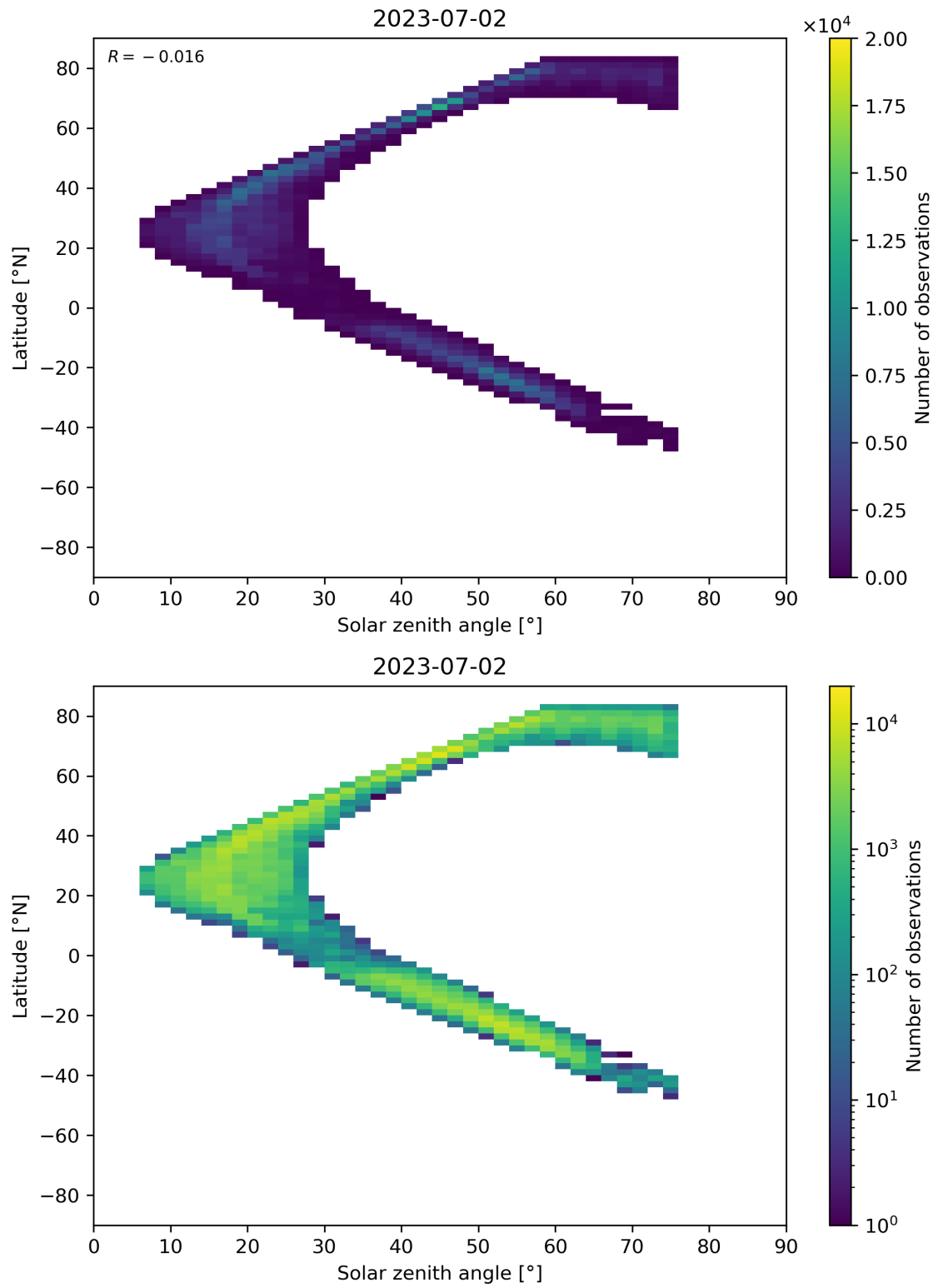
Figure 98: Scatter density plot of “Solar zenith angle” against “Latitude” for 2023-07-01 to 2023-07-03.
