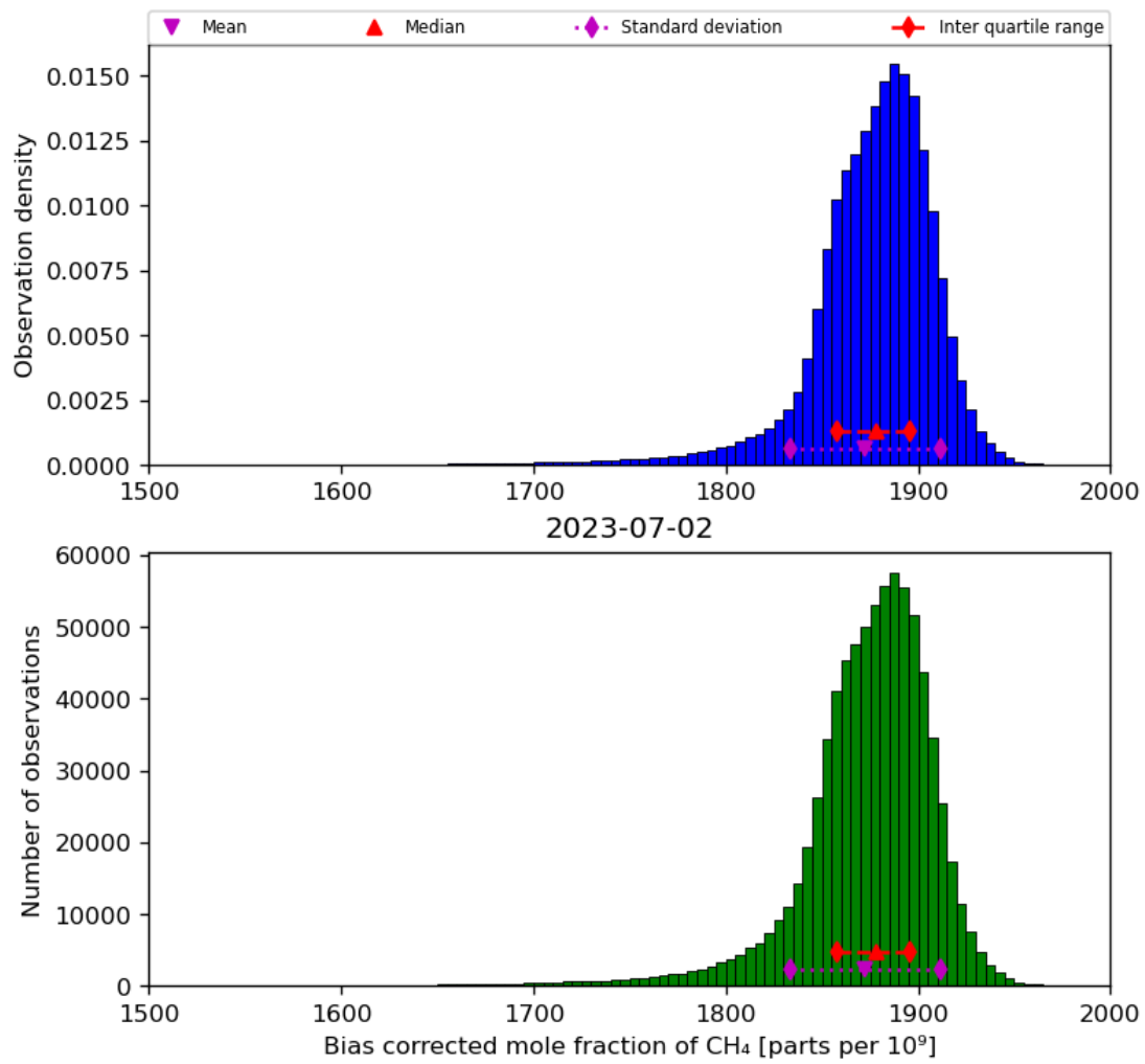
Figure 25: Histogram of “Bias corrected mole fraction of CH 4 ” for 2023-07-01 to 2023-07-03
