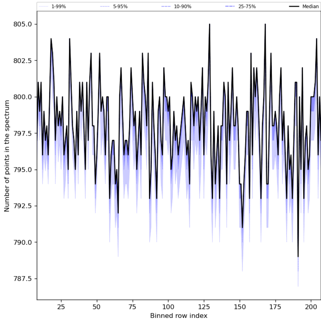
Figure 37: Along track statistics of “Number of points in the spectrum” for 2023-07-01 to 2023-07-03
