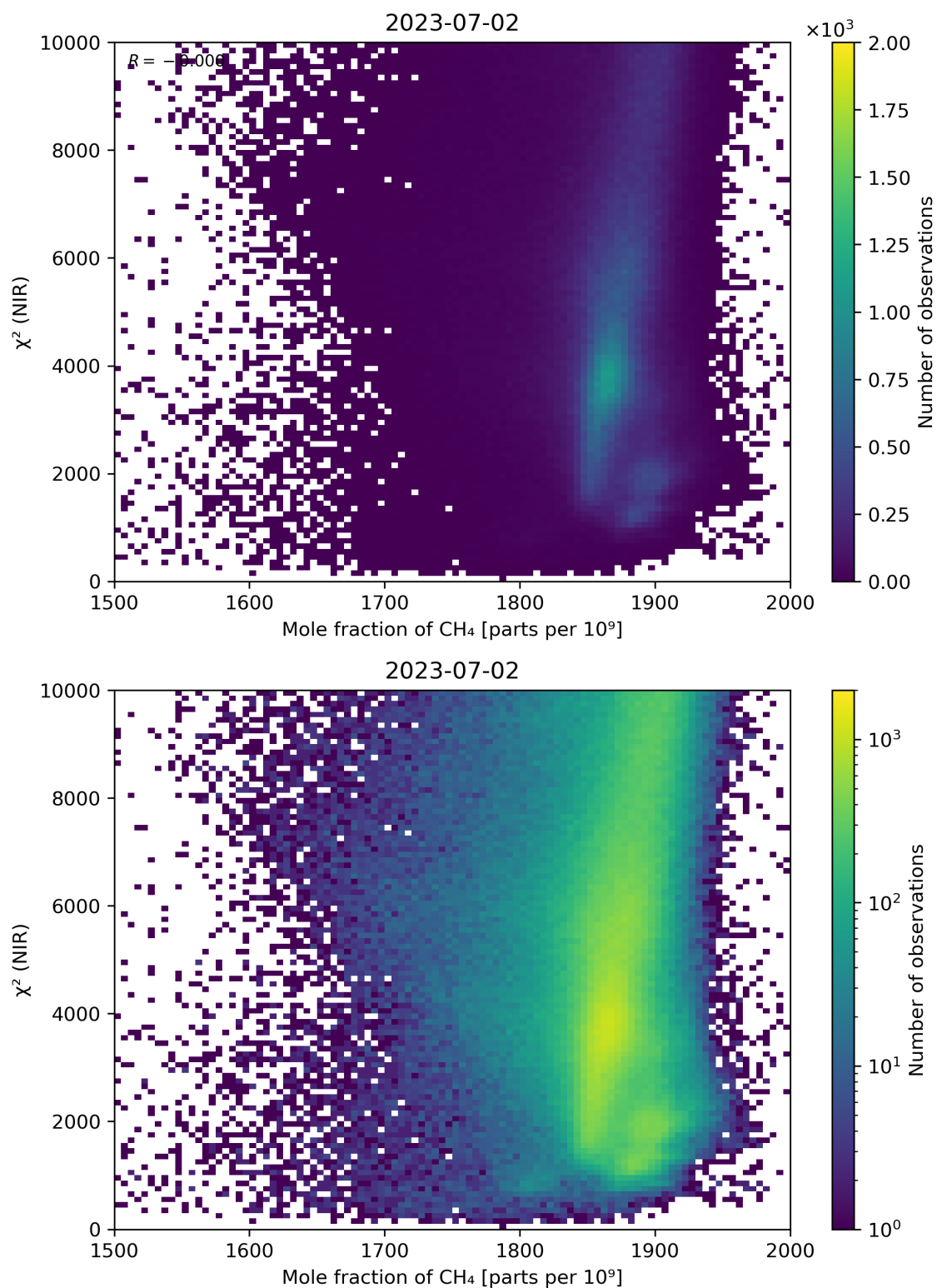
Figure 70: Scatter density plot of “Mole fraction of CH 4 ” against “ \chi^2 (NIR)” for 2023-07-01 to 2023-07-03.
