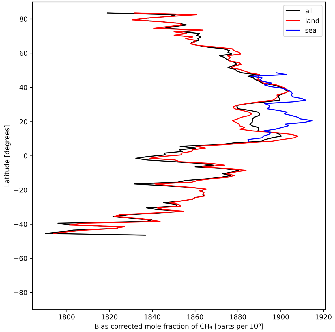
Figure 14: Zonal average of “Bias corrected mole fraction of CH 4 ” for 2023-07-01 to 2023-07-03.
