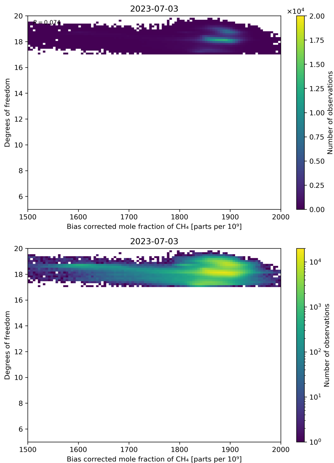
Figure 65: Scatter density plot of “Bias corrected mole fraction of \text{CH}_4 ” against “Degrees of freedom” for 2023-07-03 to 2023-07-04.
