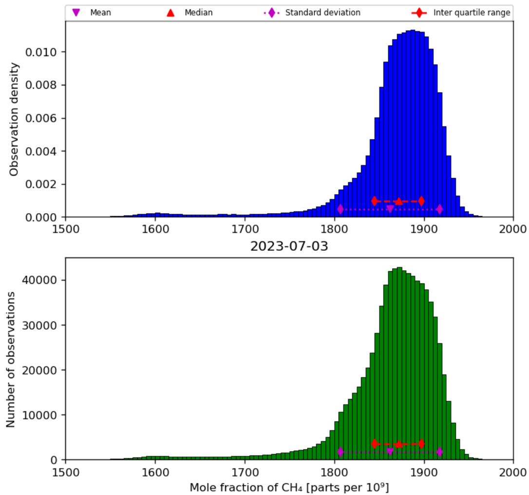
Figure 23: Histogram of “Mole fraction of CH 4 ” for 2023-07-03 to 2023-07-04
