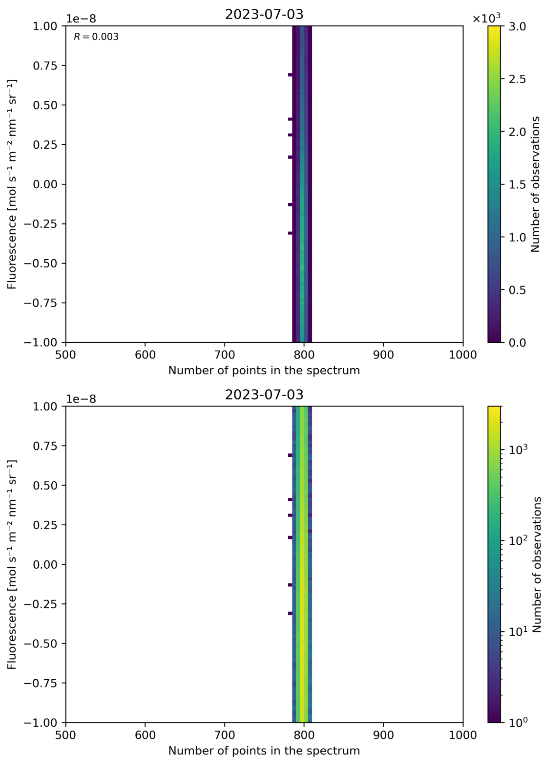
Figure 91: Scatter density plot of “Number of points in the spectrum” against “Fluorescence” for 2023-07-03 to 2023-07-04.
