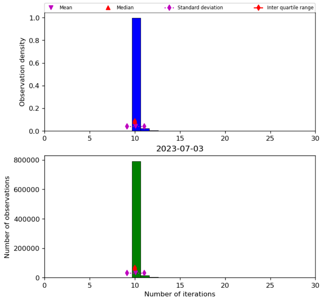
Figure 31: Histogram of “Number of iterations” for 2023-07-03 to 2023-07-04
