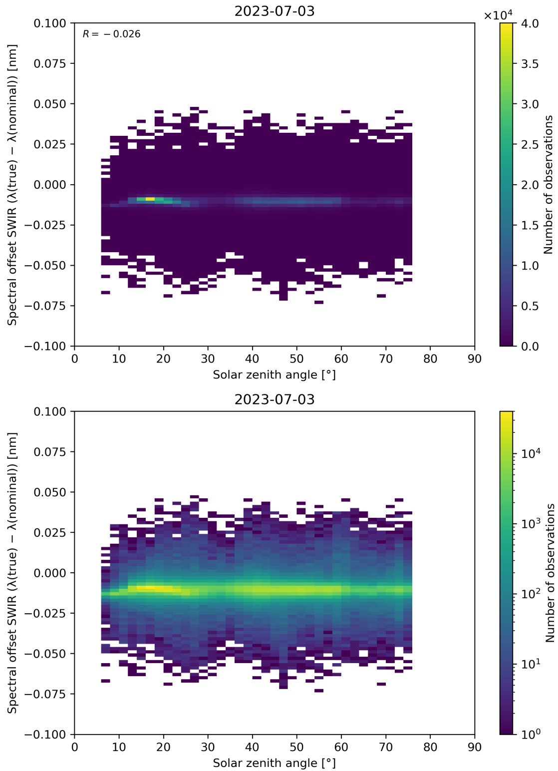
Figure 104: Scatter density plot of “Solar zenith angle” against “Spectral offset SWIR ( \lambda(\text{true}) - \lambda(\text{nominal}) )” for 2023-07-03 to 2023-07-04.
