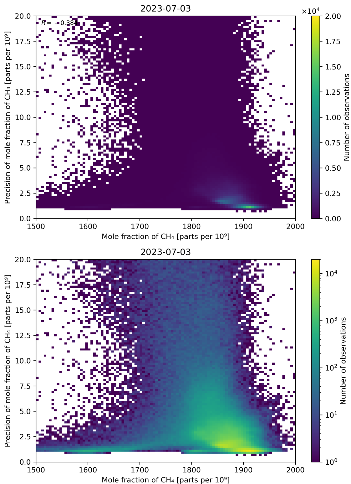
Figure 75: Scatter density plot of “Mole fraction of CH 4 ” against “Precision of mole fraction of CH 4 ” for 2023-07-03 to 2023-07-04.
