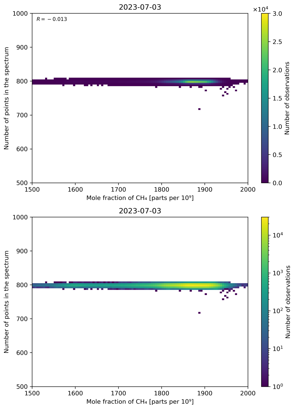
Figure 77: Scatter density plot of “Mole fraction of CH 4 ” against “Number of points in the spectrum” for 2023-07-03 to 2023-07-04.
