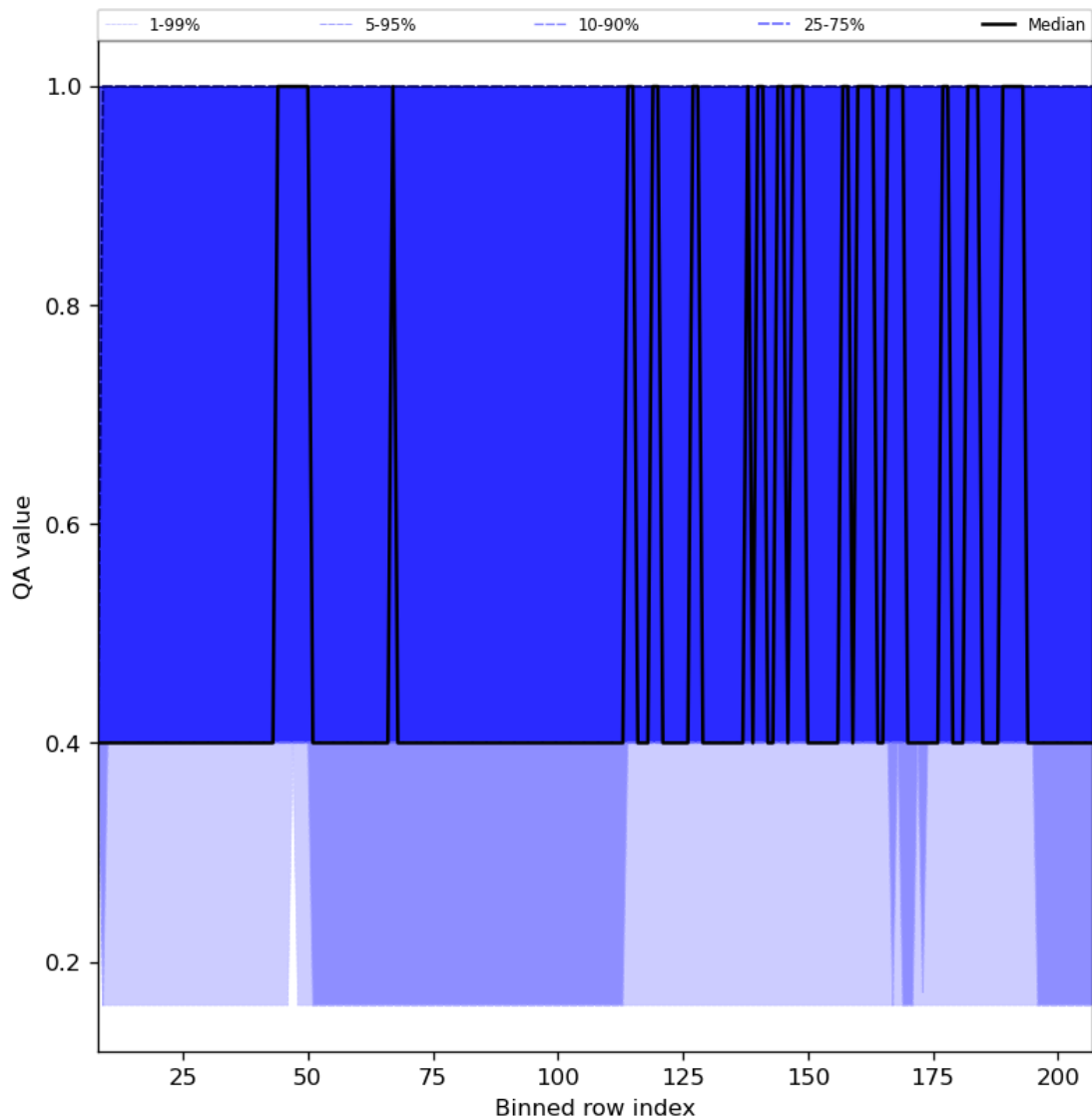
Figure 33: Along track statistics of “QA value” for 2023-07-03 to 2023-07-04
