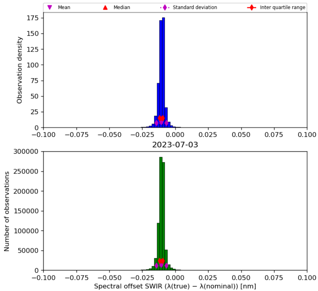
Figure 27: Histogram of “Spectral offset SWIR ( \lambda(\text{true}) - \lambda(\text{nominal}) )” for 2023-07-03 to 2023-07-04
