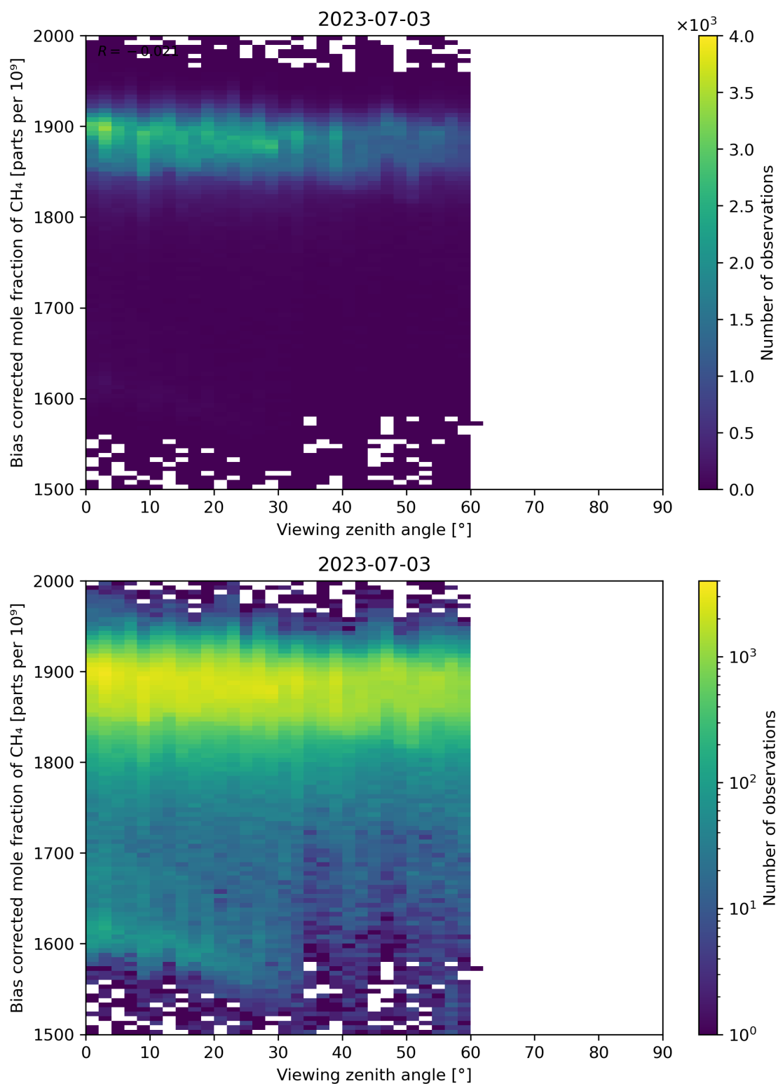
Figure 111: Scatter density plot of “Viewing zenith angle” against “Bias corrected mole fraction of CH 4 ” for 2023-07-03 to 2023-07-04.
