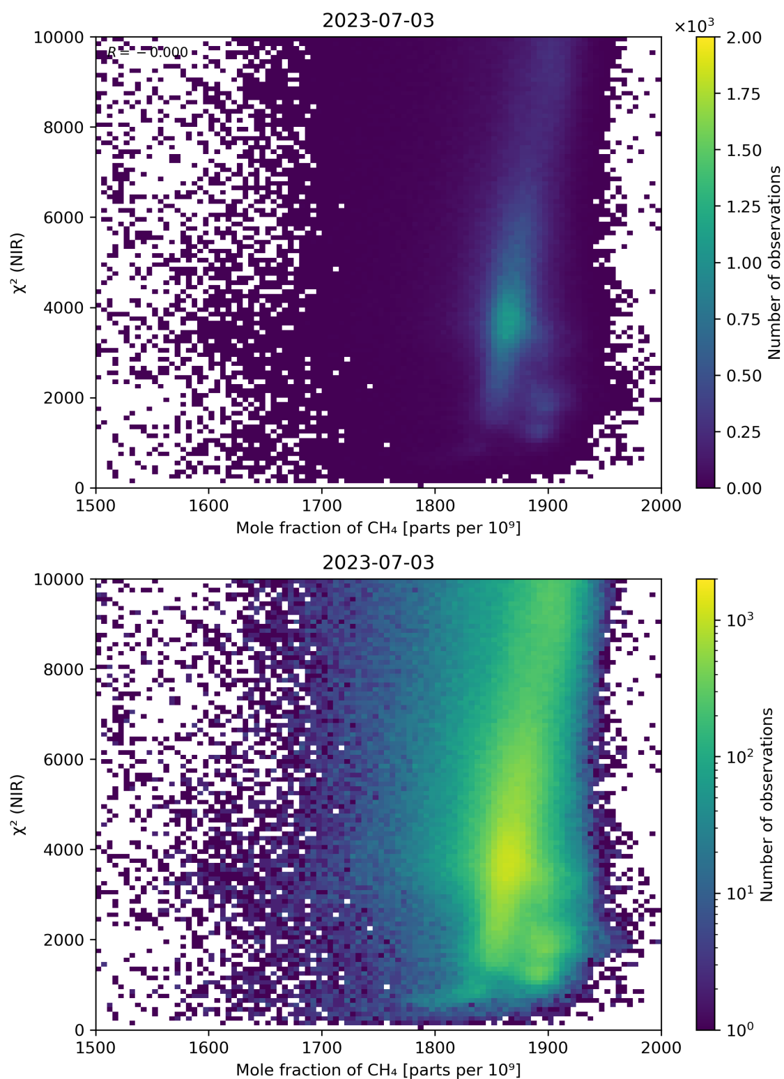
Figure 70: Scatter density plot of “Mole fraction of \text{CH}_4 ” against “ \chi^2 (NIR)” for 2023-07-03 to 2023-07-04.
