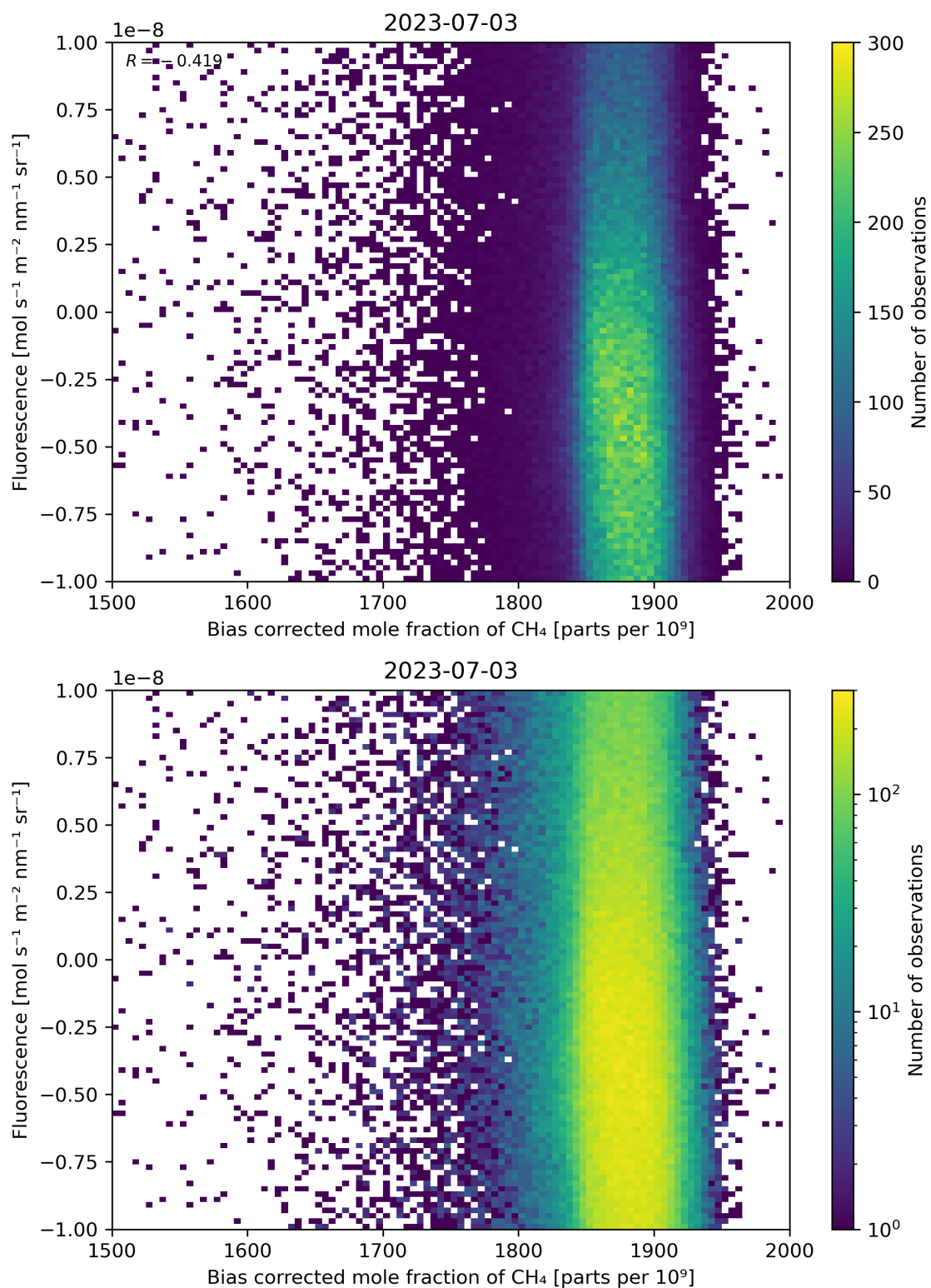
Figure 66: Scatter density plot of “Bias corrected mole fraction of \text{CH}_4 ” against “Fluorescence” for 2023-07-03 to 2023-07-04.
