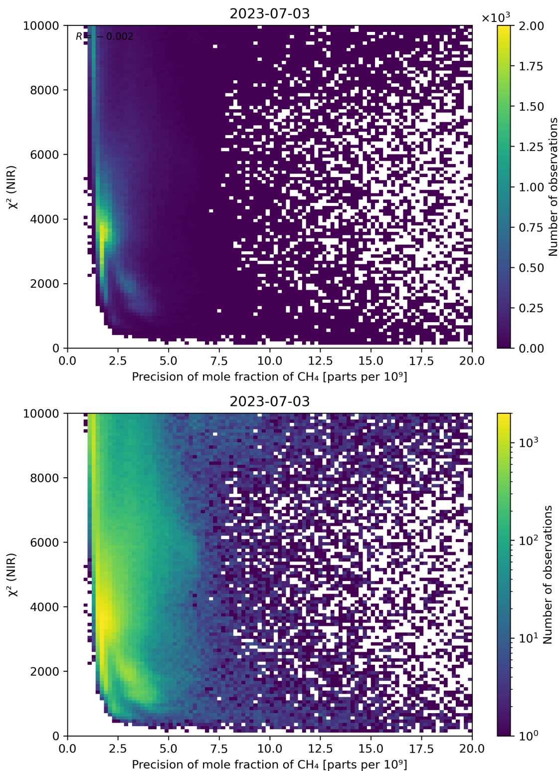
Figure 78: Scatter density plot of “Precision of mole fraction of CH 4 ” against “ \chi^2 (NIR)” for 2023-07-03 to 2023-07-04.
