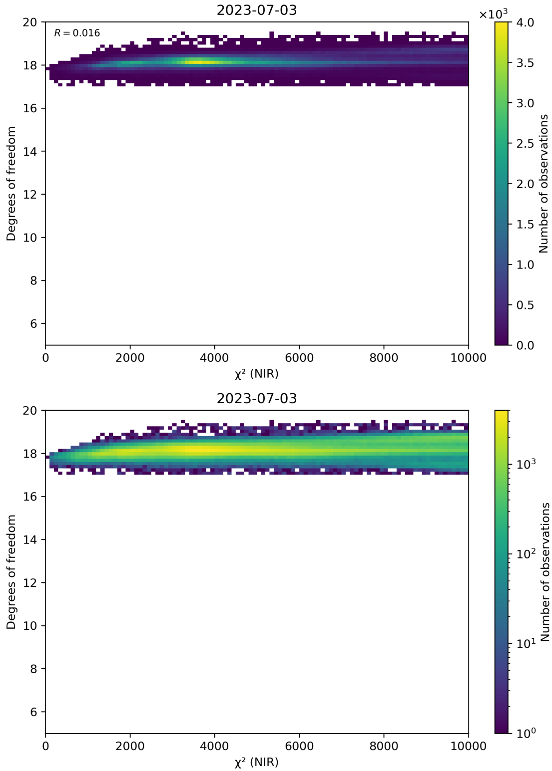
Figure 44: Scatter density plot of “ \chi^2 (NIR)” against “Degrees of freedom” for 2023-07-03 to 2023-07-04.
