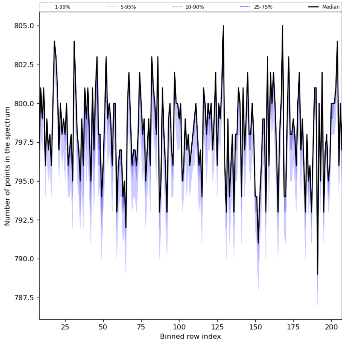
Figure 37: Along track statistics of “Number of points in the spectrum” for 2023-07-03 to 2023-07-04
