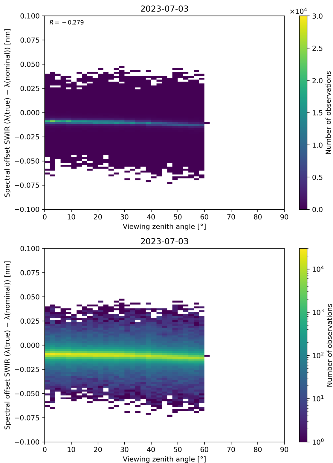
Figure 116: Scatter density plot of “Viewing zenith angle” against “Spectral offset SWIR ( \lambda(\text{true}) - \lambda(\text{nominal}) )” for 2023-07-03 to 2023-07-04.
