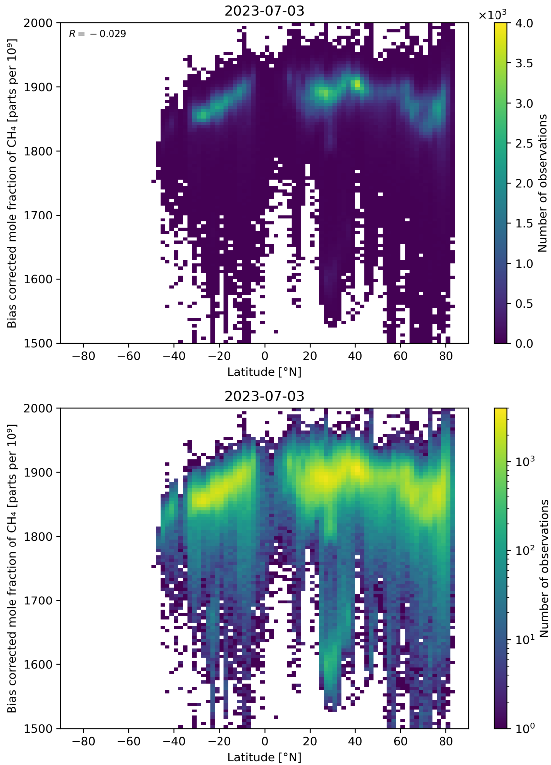
Figure 58: Scatter density plot of “Latitude” against “Bias corrected mole fraction of \text{CH}_4 ” for 2023-07-03 to 2023-07-04.
