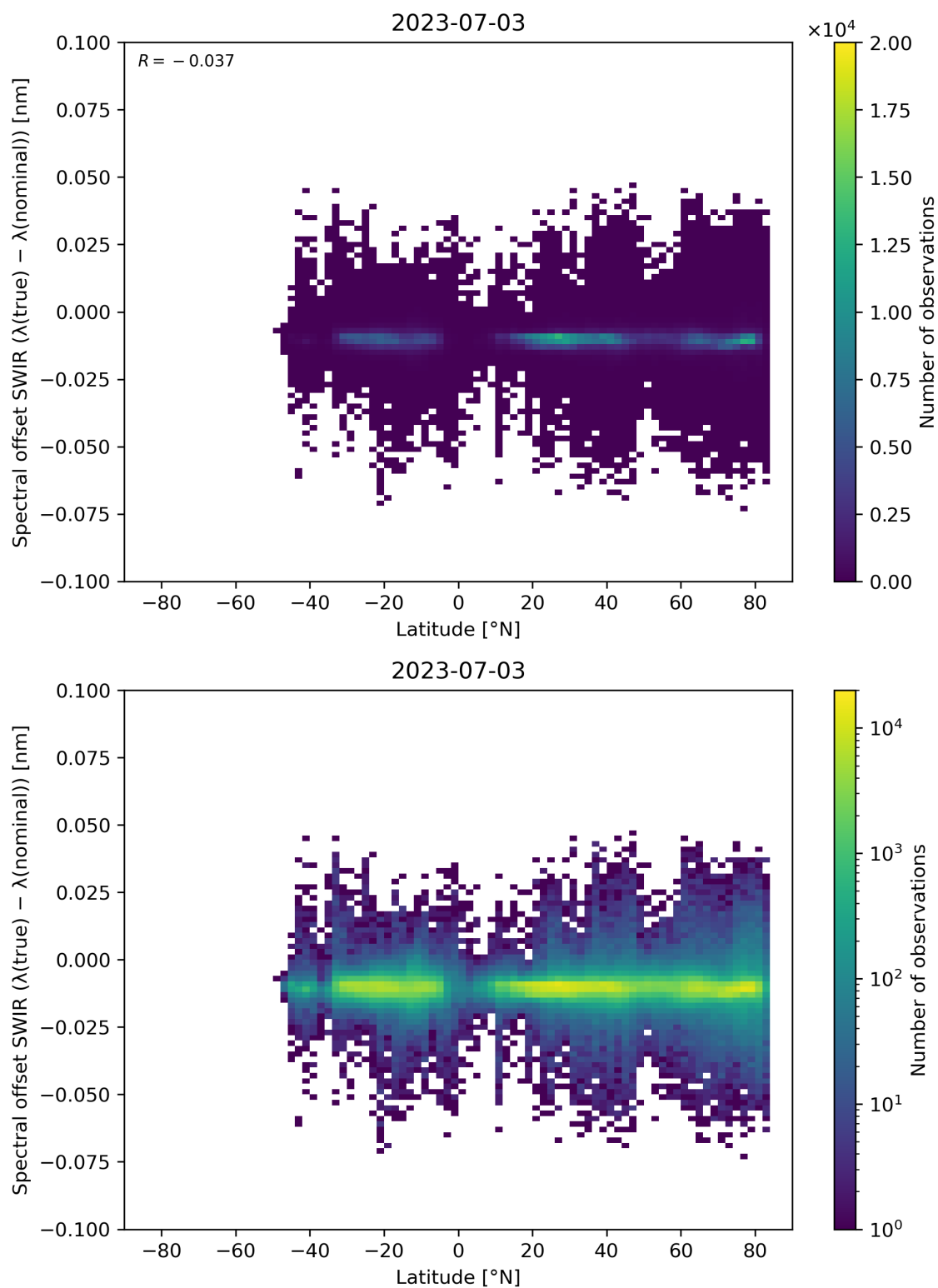
Figure 62: Scatter density plot of “Latitude” against “Spectral offset SWIR ( \lambda(\text{true}) - \lambda(\text{nominal}) )” for 2023-07-03 to 2023-07-04.
