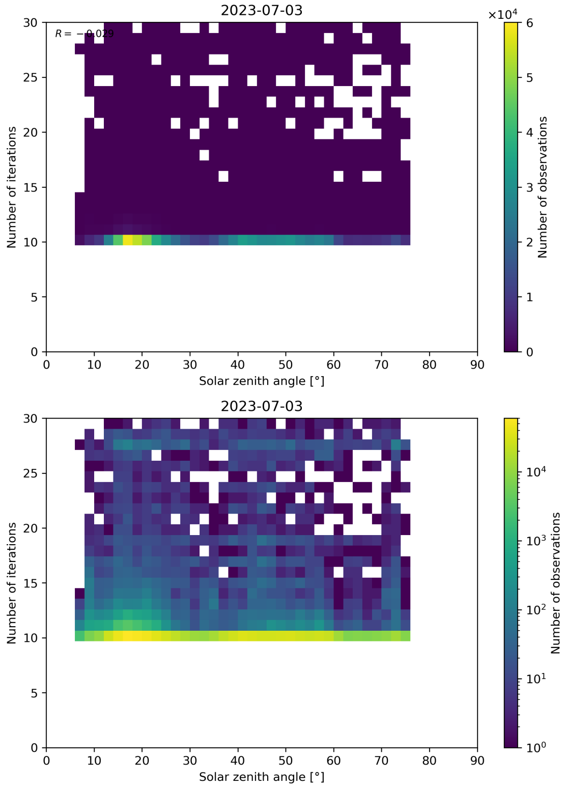
Figure 102: Scatter density plot of “Solar zenith angle” against “Number of iterations” for 2023-07-03 to 2023-07-04.
