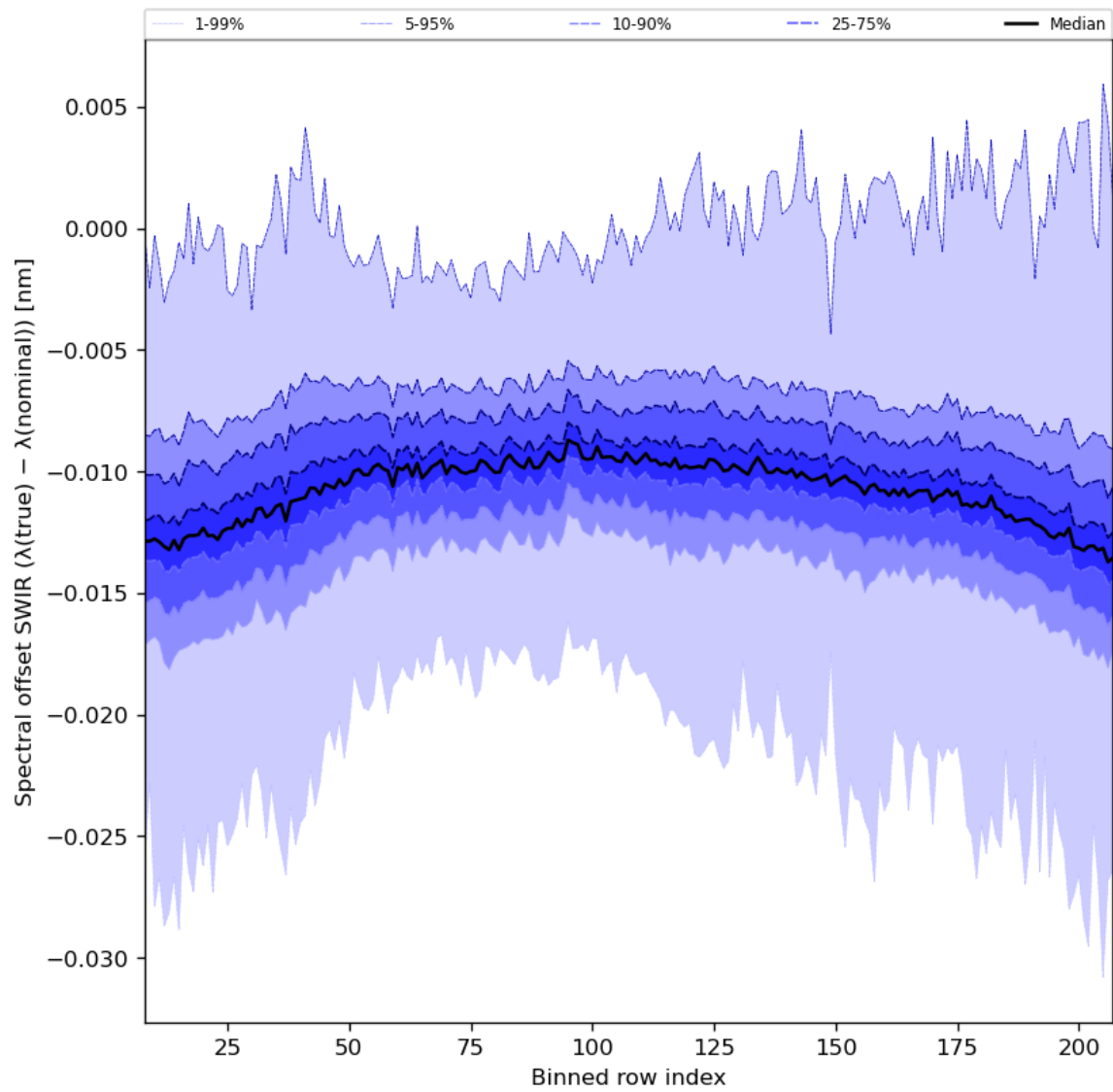
Figure 38: Along track statistics of “Spectral offset SWIR ( \lambda(\text{true}) - \lambda(\text{nominal}) )” for 2023-07-03 to 2023-07-04
