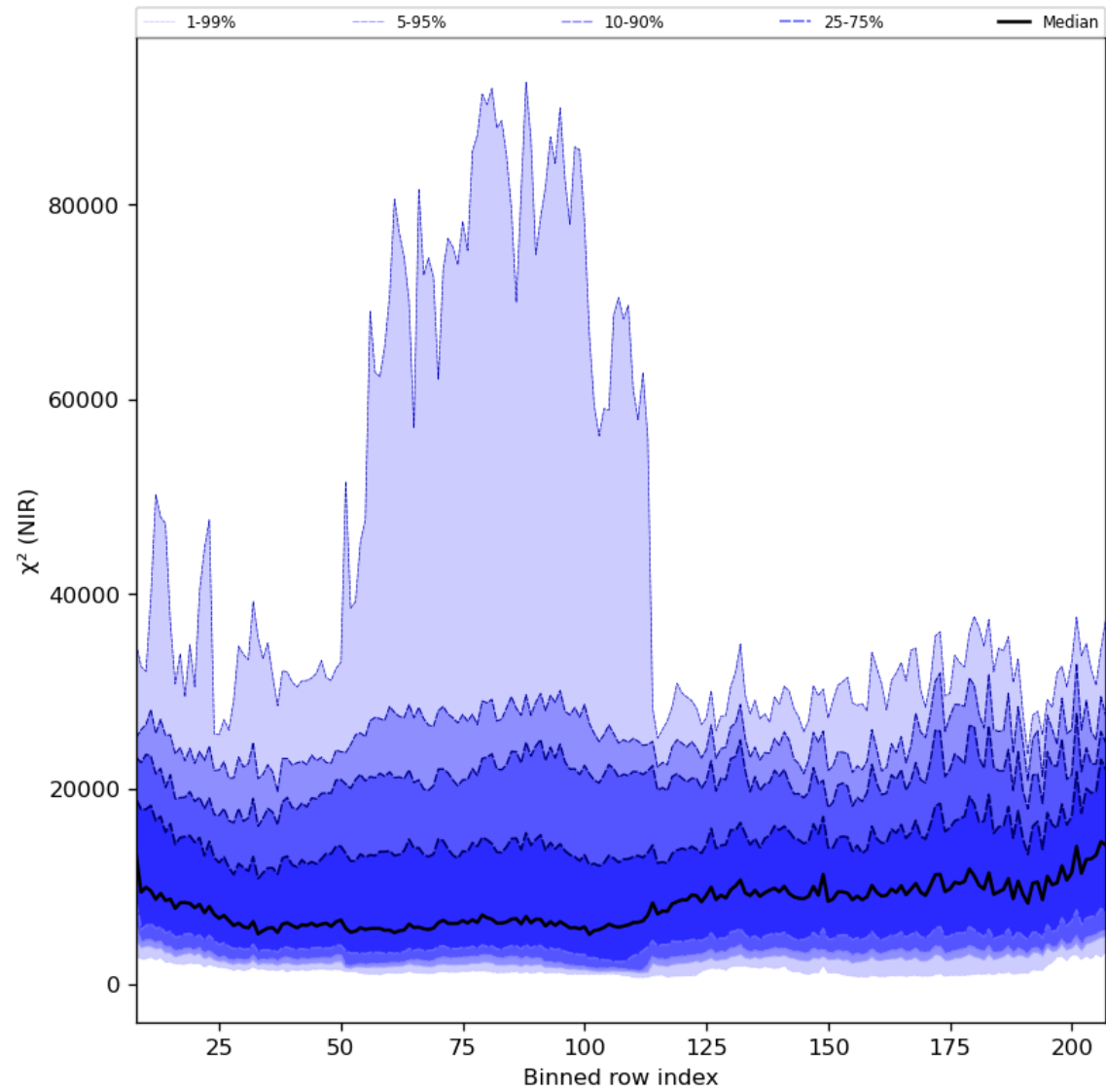
Figure 40: Along track statistics of " \chi^2 (NIR)" for 2023-07-03 to 2023-07-04
