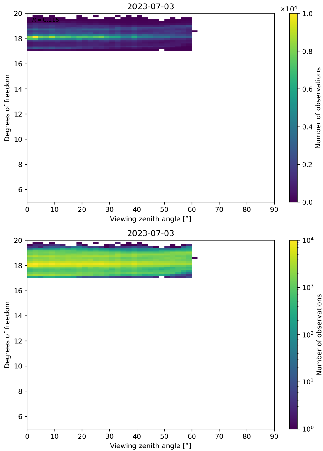
Figure 107: Scatter density plot of “Viewing zenith angle” against “Degrees of freedom” for 2023-07-03 to 2023-07-04.
