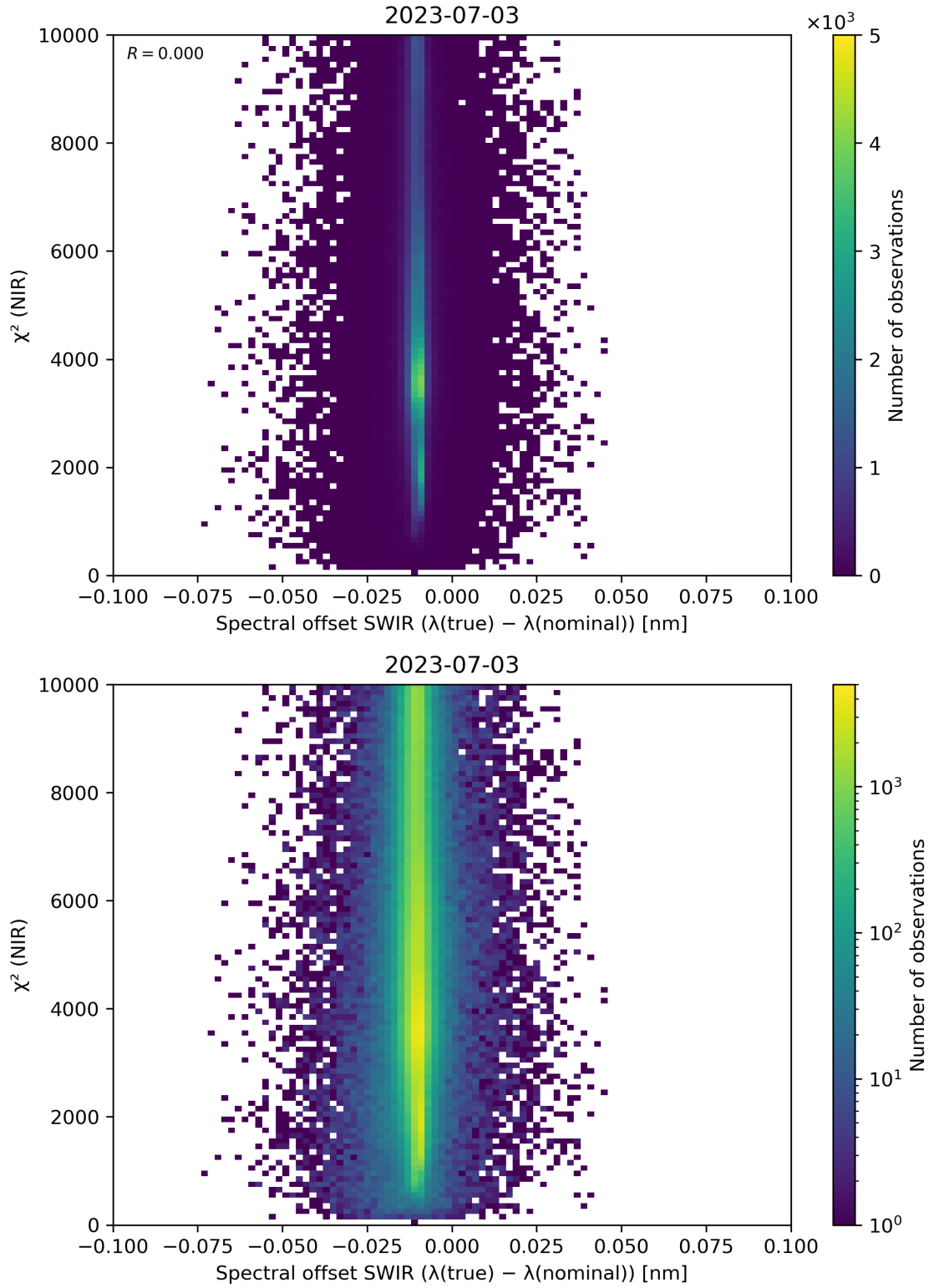
Figure 117: Scatter density plot of “Spectral offset SWIR ( \lambda(\text{true}) - \lambda(\text{nominal}) )” against “ \chi^2 (NIR)” for 2023-07-03 to 2023-07-04.
