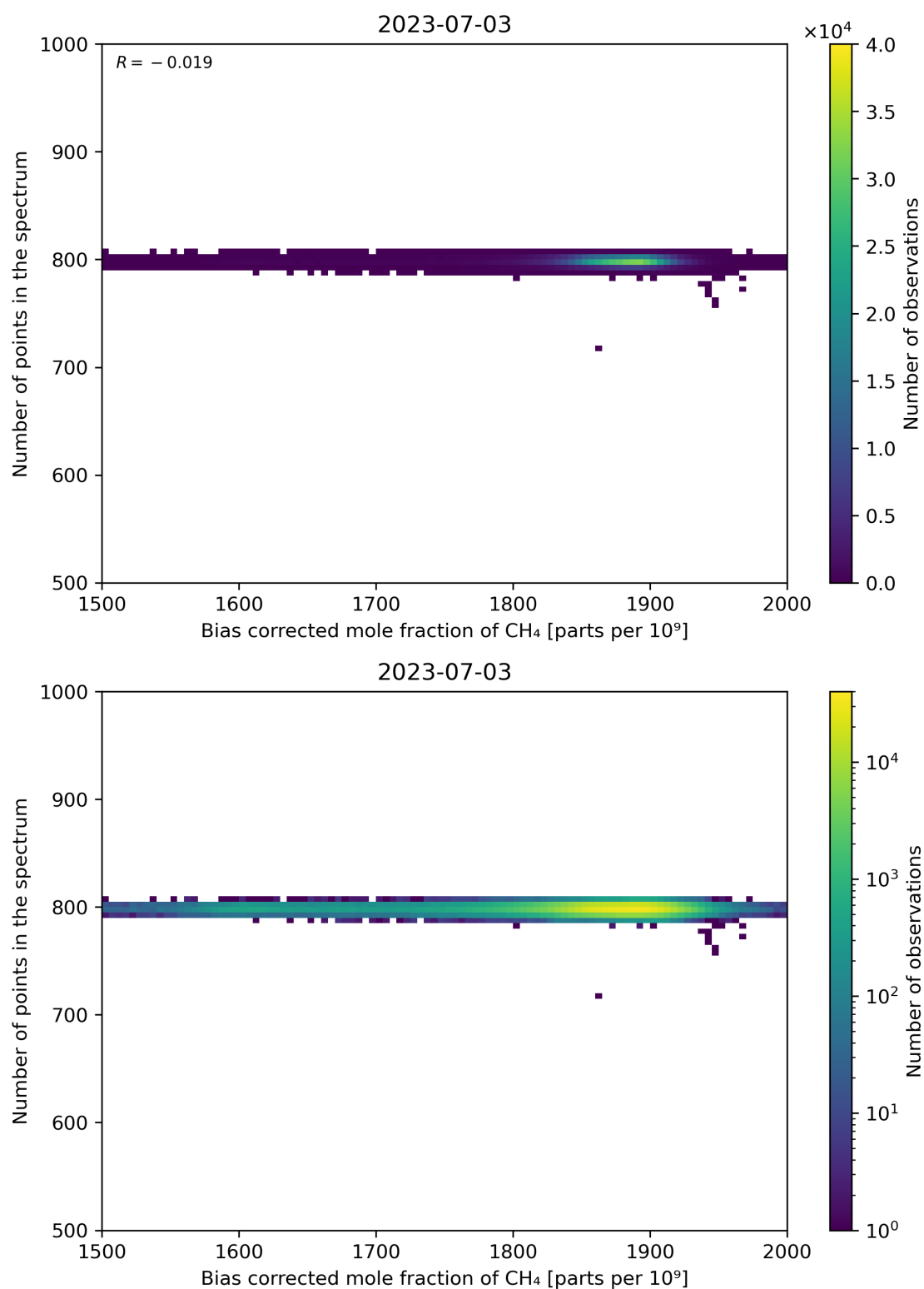
Figure 68: Scatter density plot of “Bias corrected mole fraction of CH 4 ” against “Number of points in the spectrum” for 2023-07-03 to 2023-07-04.
