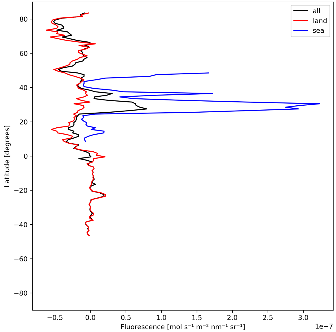
Figure 21: Zonal average of “Fluorescence” for 2023-07-03 to 2023-07-04.
