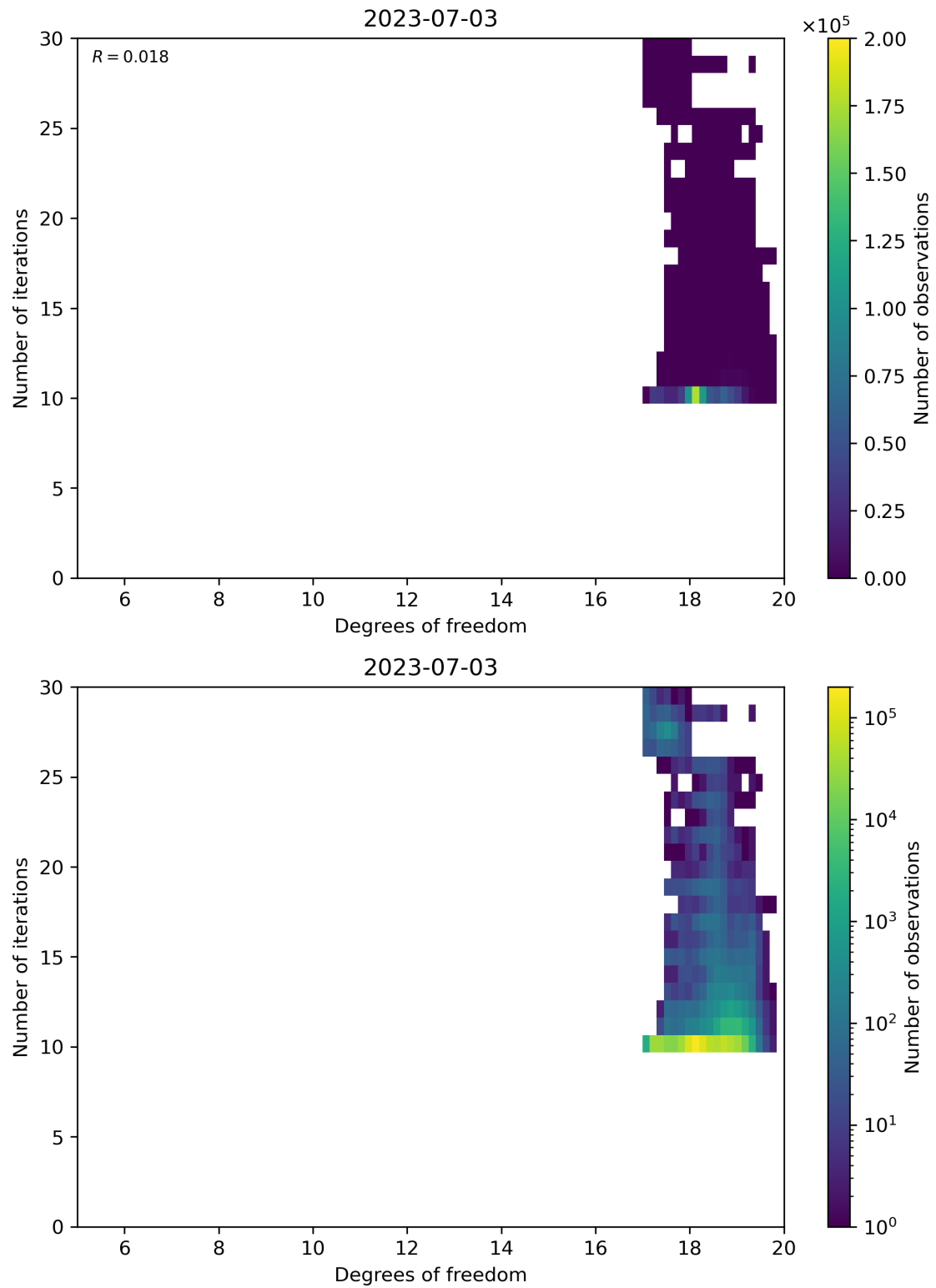
Figure 52: Scatter density plot of “Degrees of freedom” against “Number of iterations” for 2023-07-03 to 2023-07-04.
