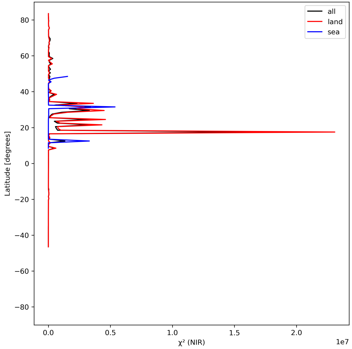
Figure 18: Zonal average of “ \chi^2 (NIR)” for 2023-07-03 to 2023-07-04.
