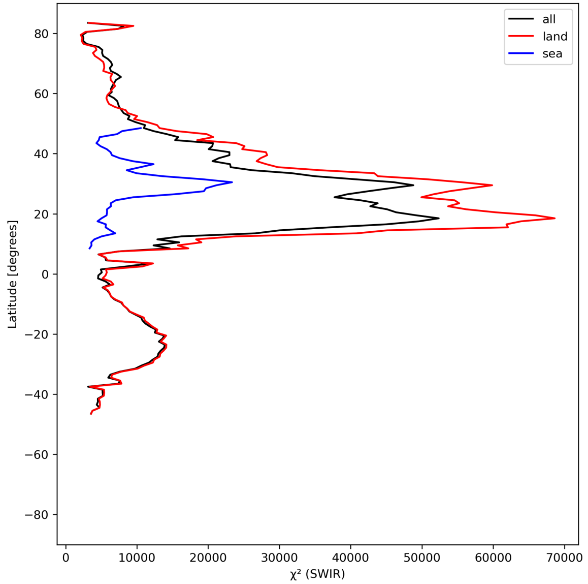
Figure 17: Zonal average of “ \chi^2 (SWIR)” for 2023-07-03 to 2023-07-04.
