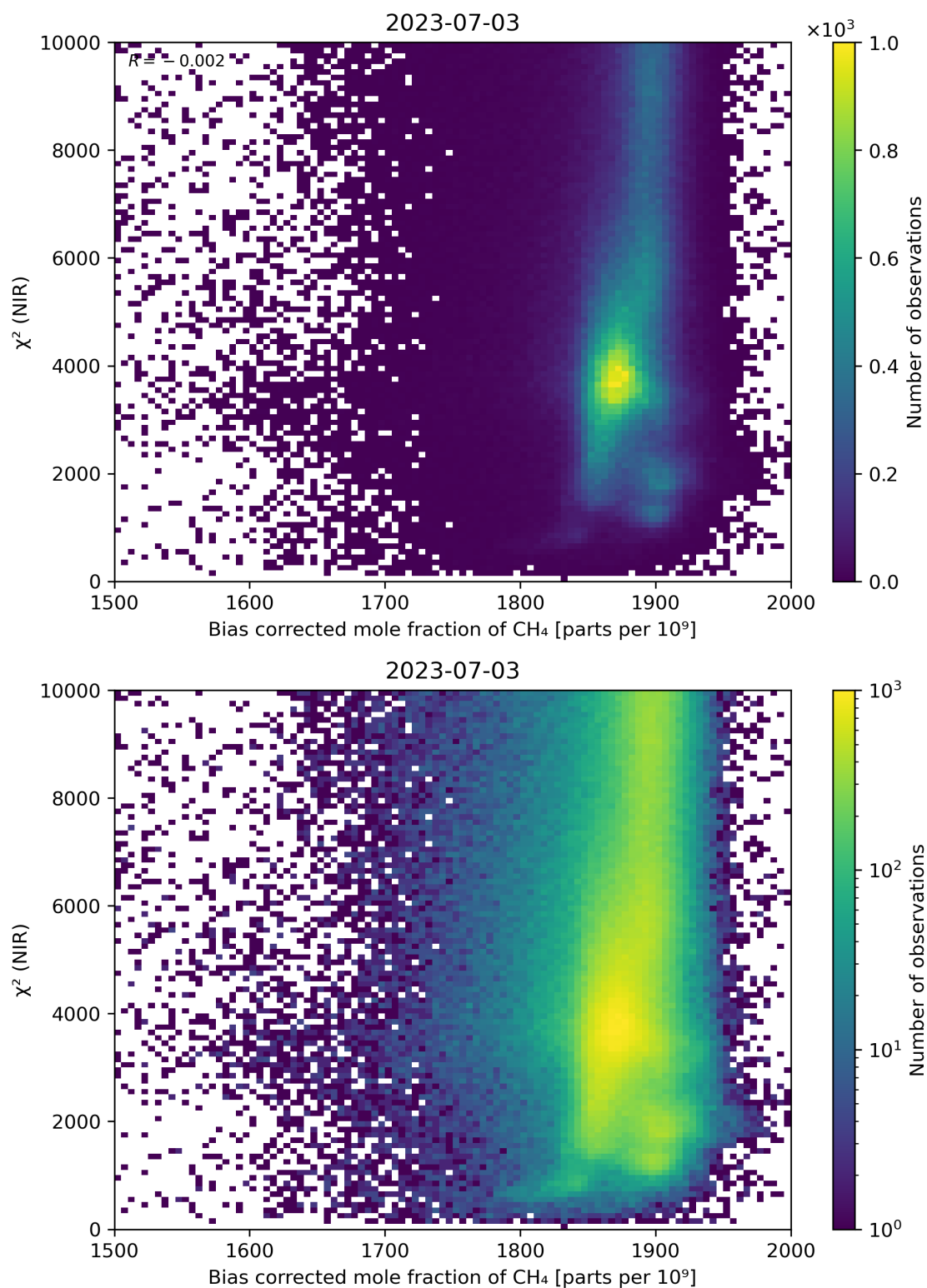
Figure 63: Scatter density plot of “Bias corrected mole fraction of CH 4 ” against “ \chi^2 (NIR)” for 2023-07-03 to 2023-07-04.
