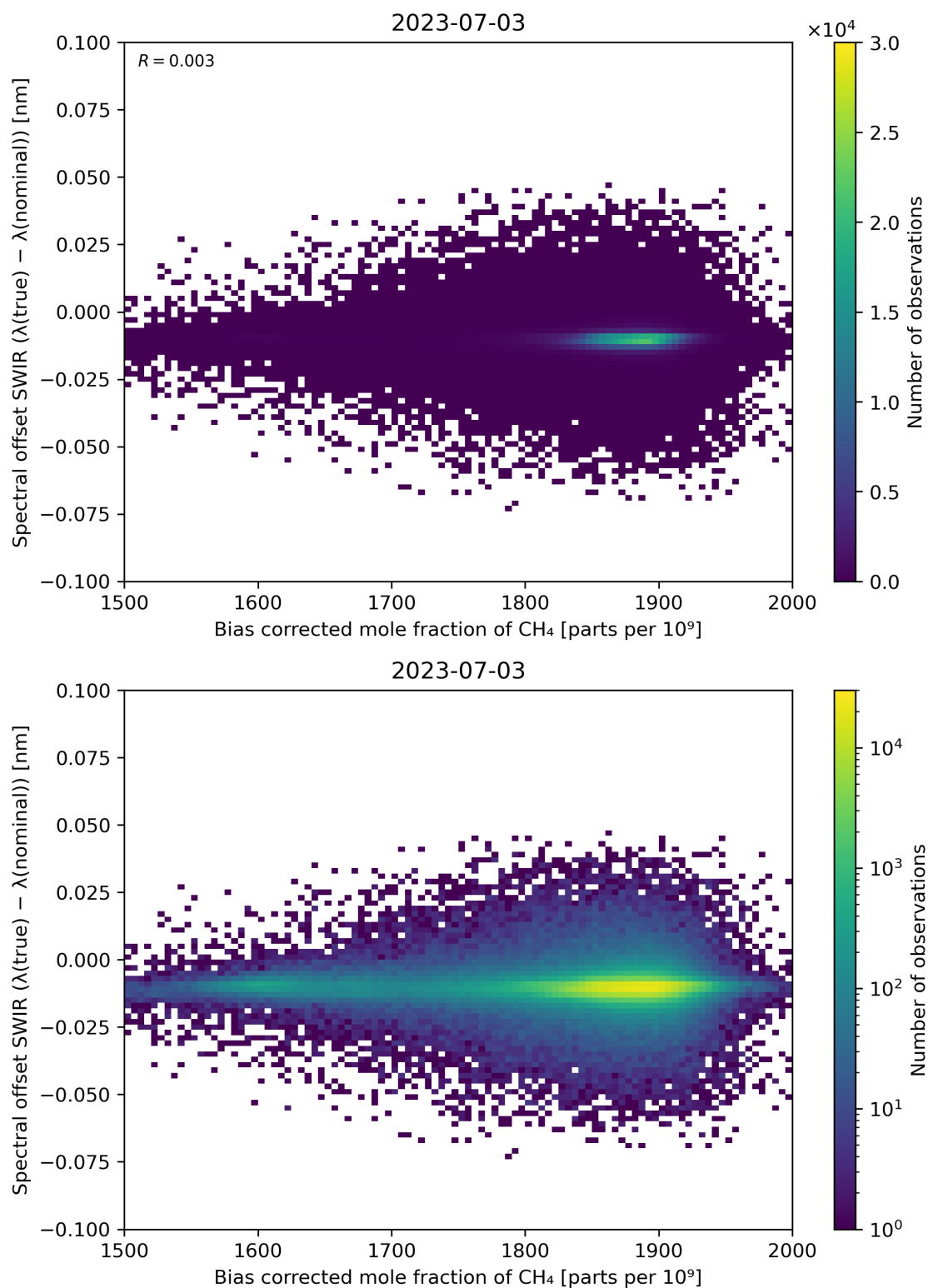
Figure 69: Scatter density plot of “Bias corrected mole fraction of \text{CH}_4 ” against “Spectral offset SWIR ( \lambda(\text{true}) - \lambda(\text{nominal}) )” for 2023-07-03 to 2023-07-04.
