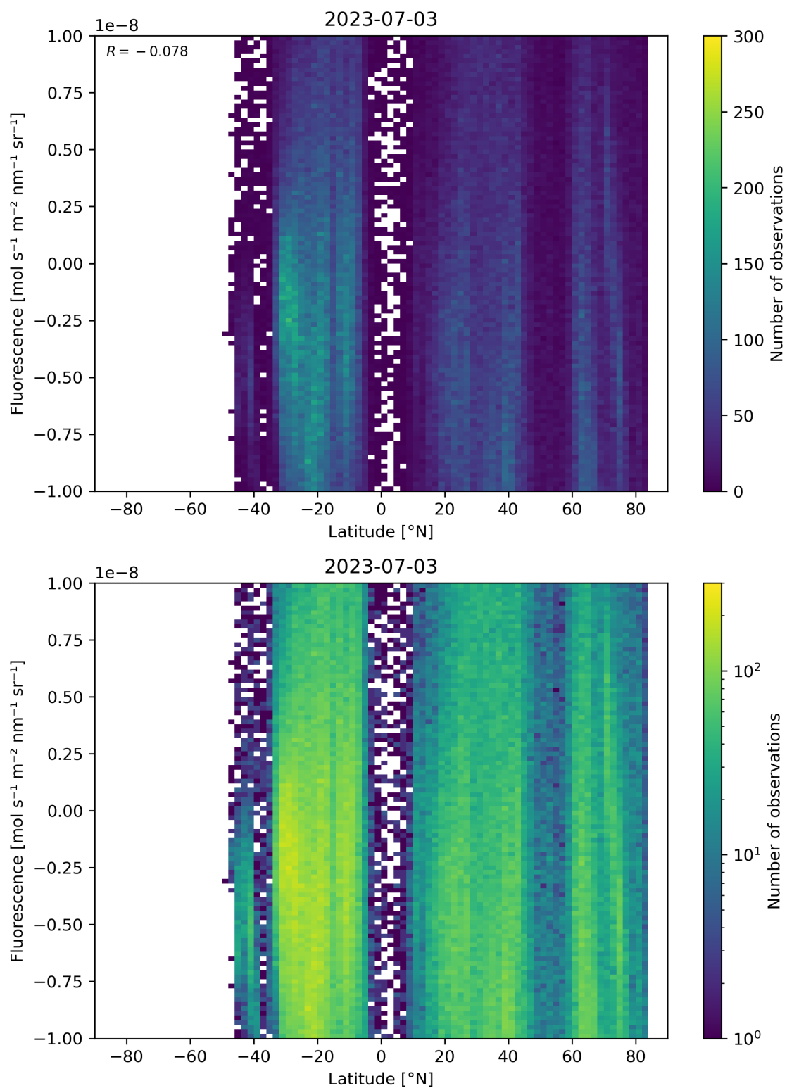
Figure 56: Scatter density plot of “Latitude” against “Fluorescence” for 2023-07-03 to 2023-07-04.
