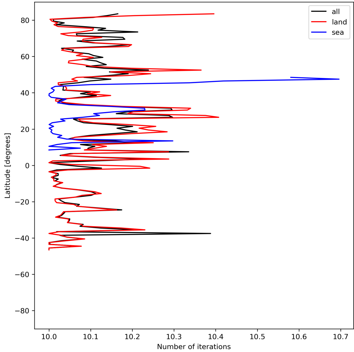
Figure 20: Zonal average of “Number of iterations” for 2023-07-03 to 2023-07-04.
