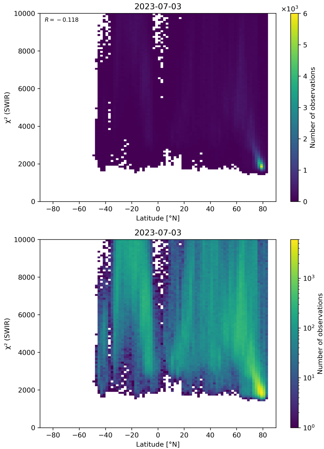
Figure 54: Scatter density plot of “Latitude” against “ \chi^2 (SWIR)” for 2023-07-03 to 2023-07-04.
