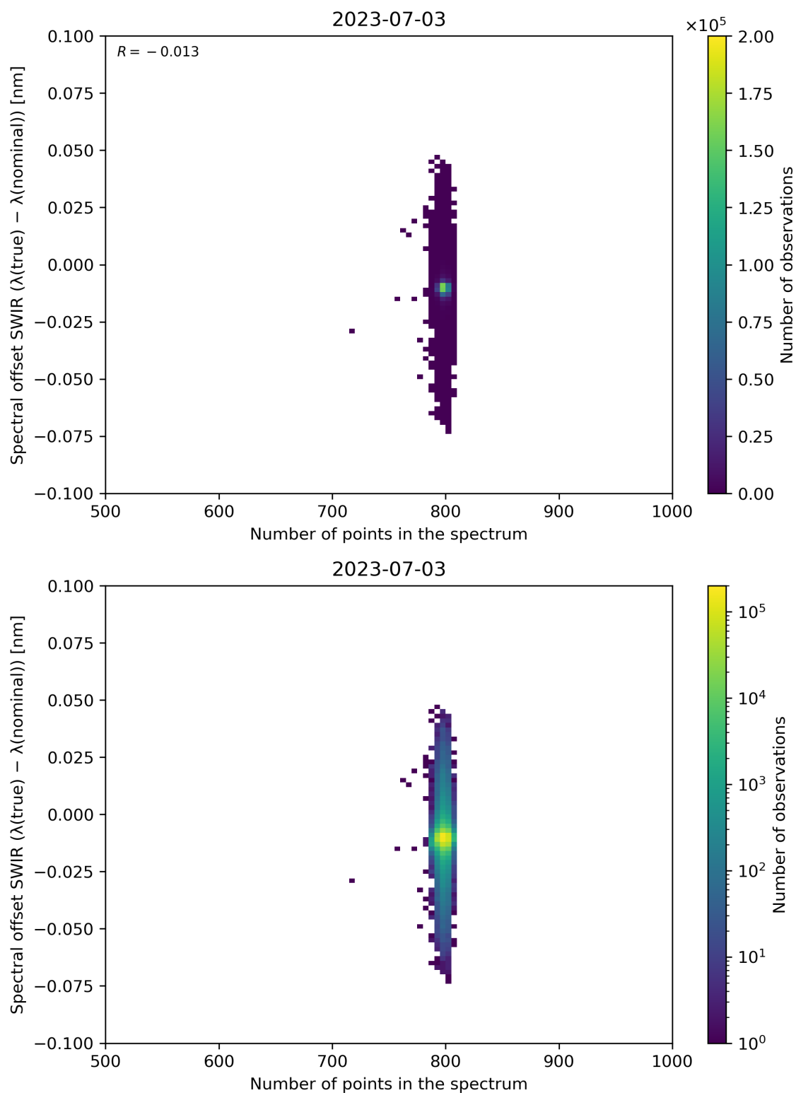
Figure 93: Scatter density plot of “Number of points in the spectrum” against “Spectral offset SWIR ( \lambda(\text{true}) - \lambda(\text{nominal}) )” for 2023-07-03 to 2023-07-04.
