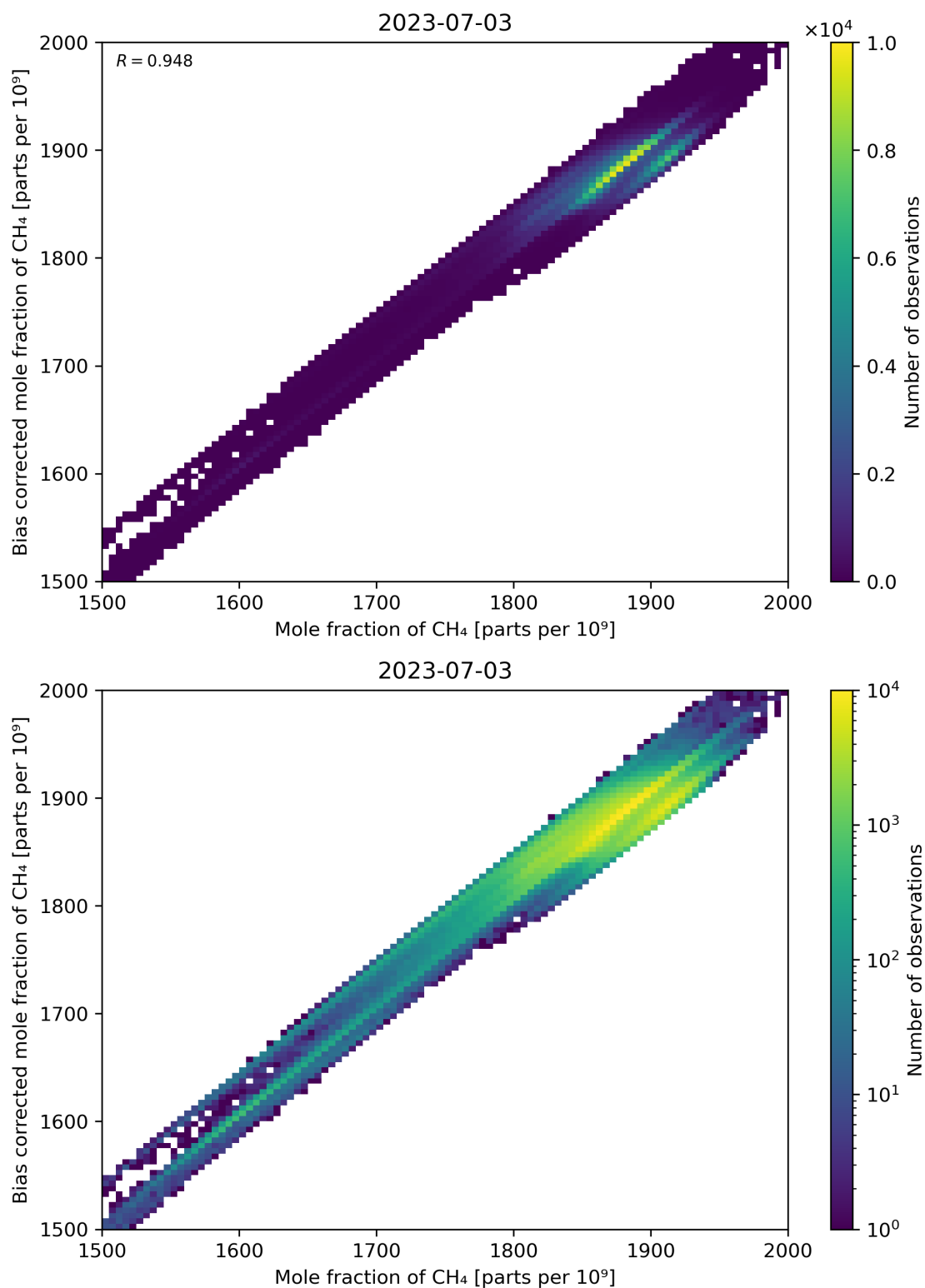
Figure 74: Scatter density plot of “Mole fraction of CH 4 ” against “Bias corrected mole fraction of CH 4 ” for 2023-07-03 to 2023-07-04.
