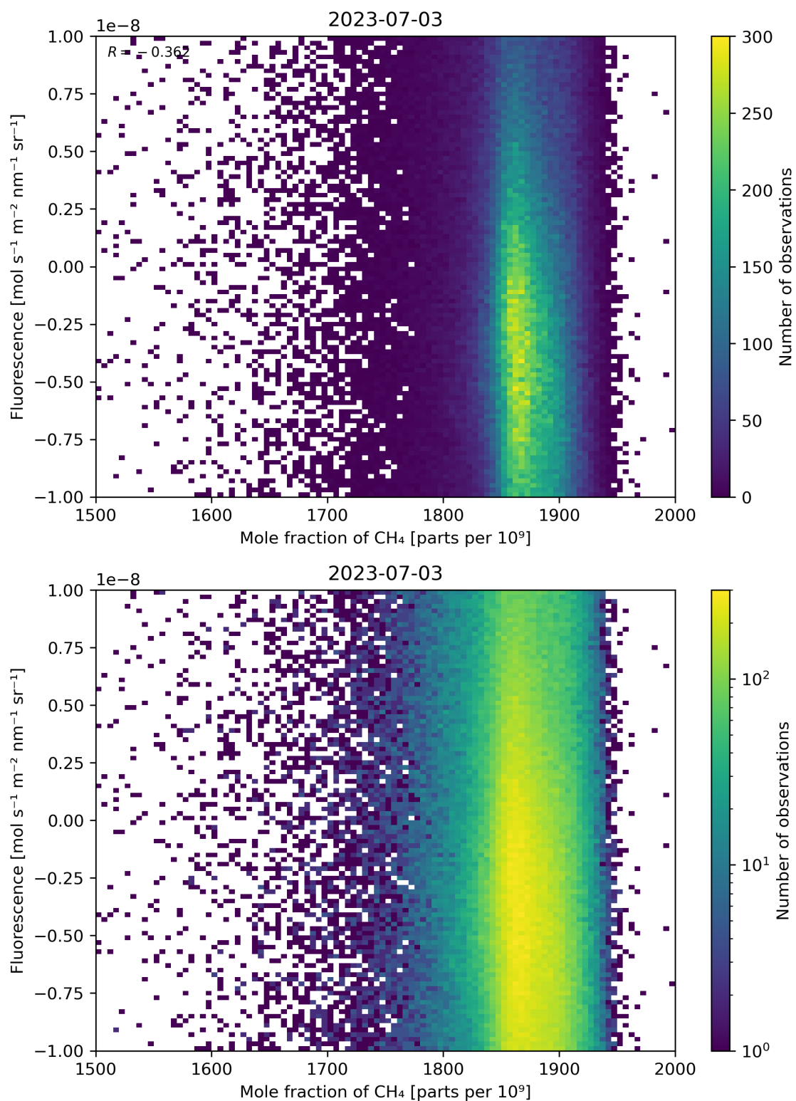
Figure 73: Scatter density plot of “Mole fraction of \text{CH}_4 ” against “Fluorescence” for 2023-07-03 to 2023-07-04.
