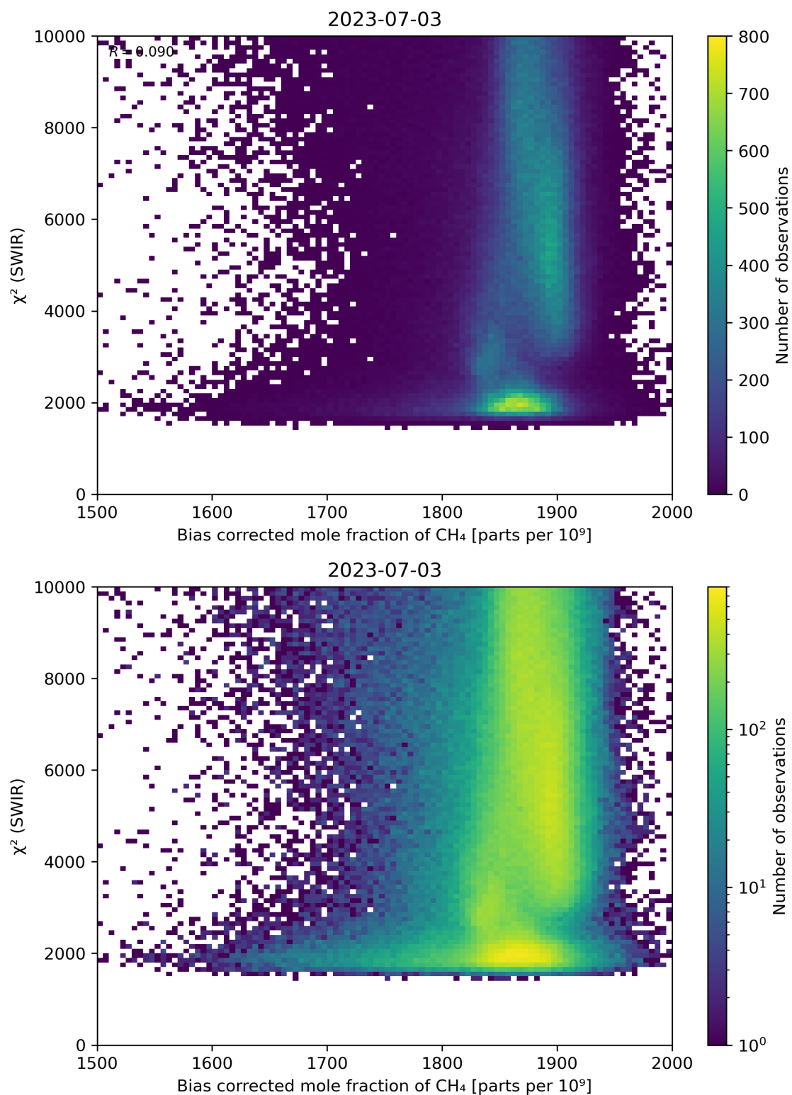
Figure 64: Scatter density plot of “Bias corrected mole fraction of CH 4 ” against “ \chi^2 (SWIR)” for 2023-07-03 to 2023-07-04.
