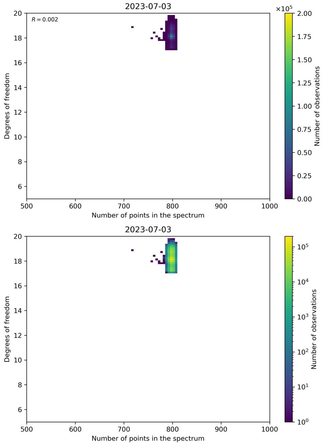
Figure 90: Scatter density plot of “Number of points in the spectrum” against “Degrees of freedom” for 2023-07-03 to 2023-07-04.
