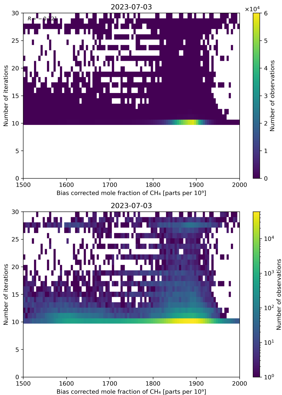
Figure 67: Scatter density plot of “Bias corrected mole fraction of CH 4 ” against “Number of iterations” for 2023-07-03 to 2023-07-04.
