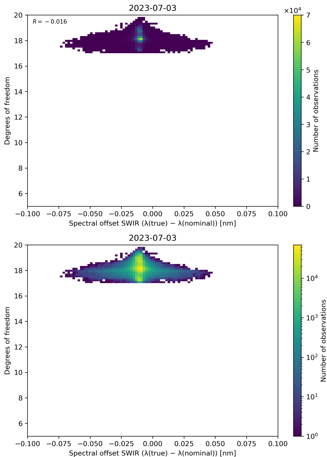
Figure 119: Scatter density plot of “Spectral offset SWIR ( \lambda(\text{true}) - \lambda(\text{nominal}) )” against “Degrees of freedom” for 2023-07-03 to 2023-07-04.
