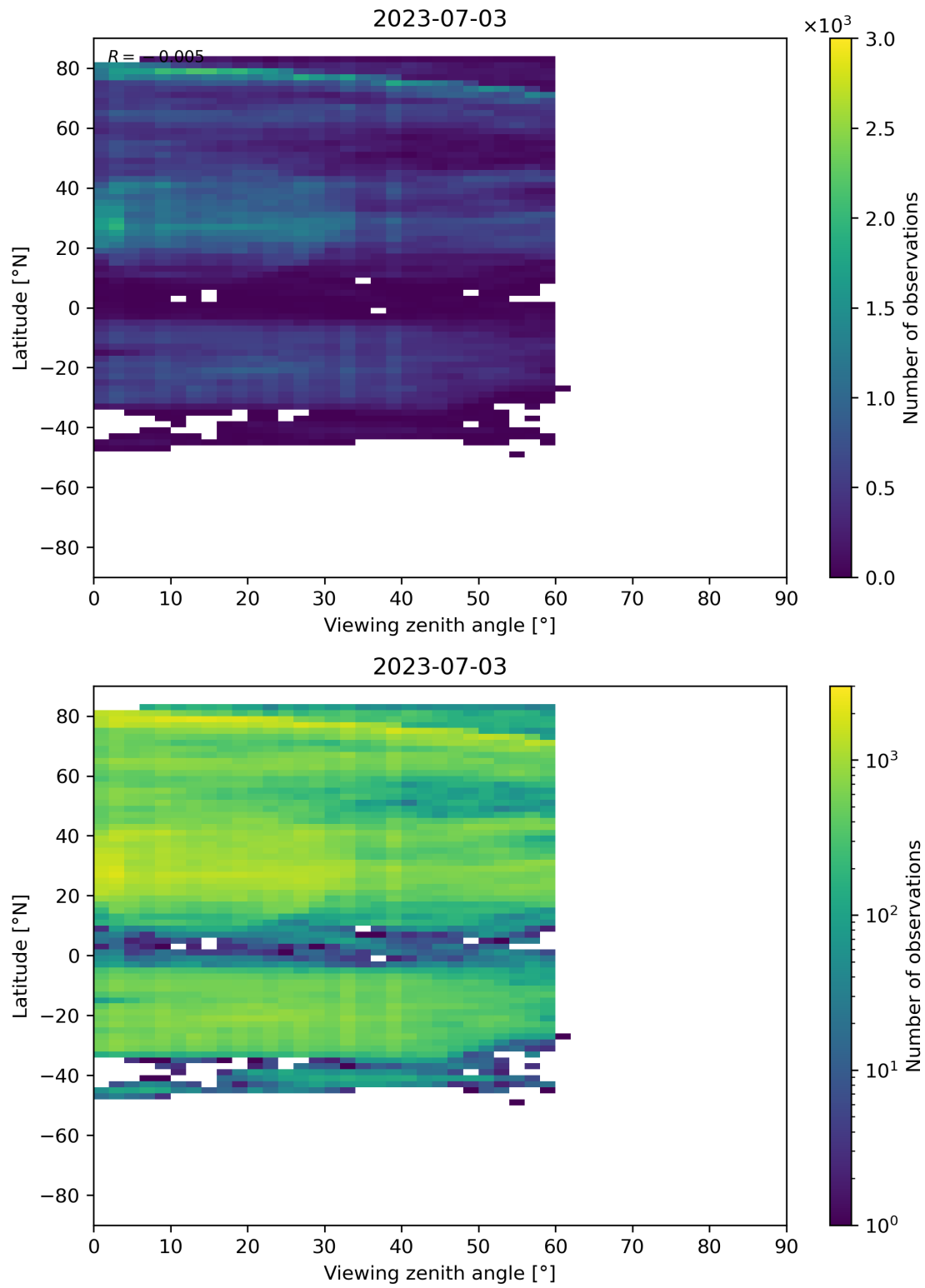
Figure 109: Scatter density plot of “Viewing zenith angle” against “Latitude” for 2023-07-03 to 2023-07-04.
