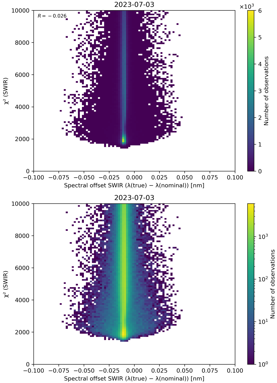
Figure 118: Scatter density plot of “Spectral offset SWIR ( \lambda(\text{true}) - \lambda(\text{nominal}) )” against “ \chi^2 (SWIR)” for 2023-07-03 to 2023-07-04.
