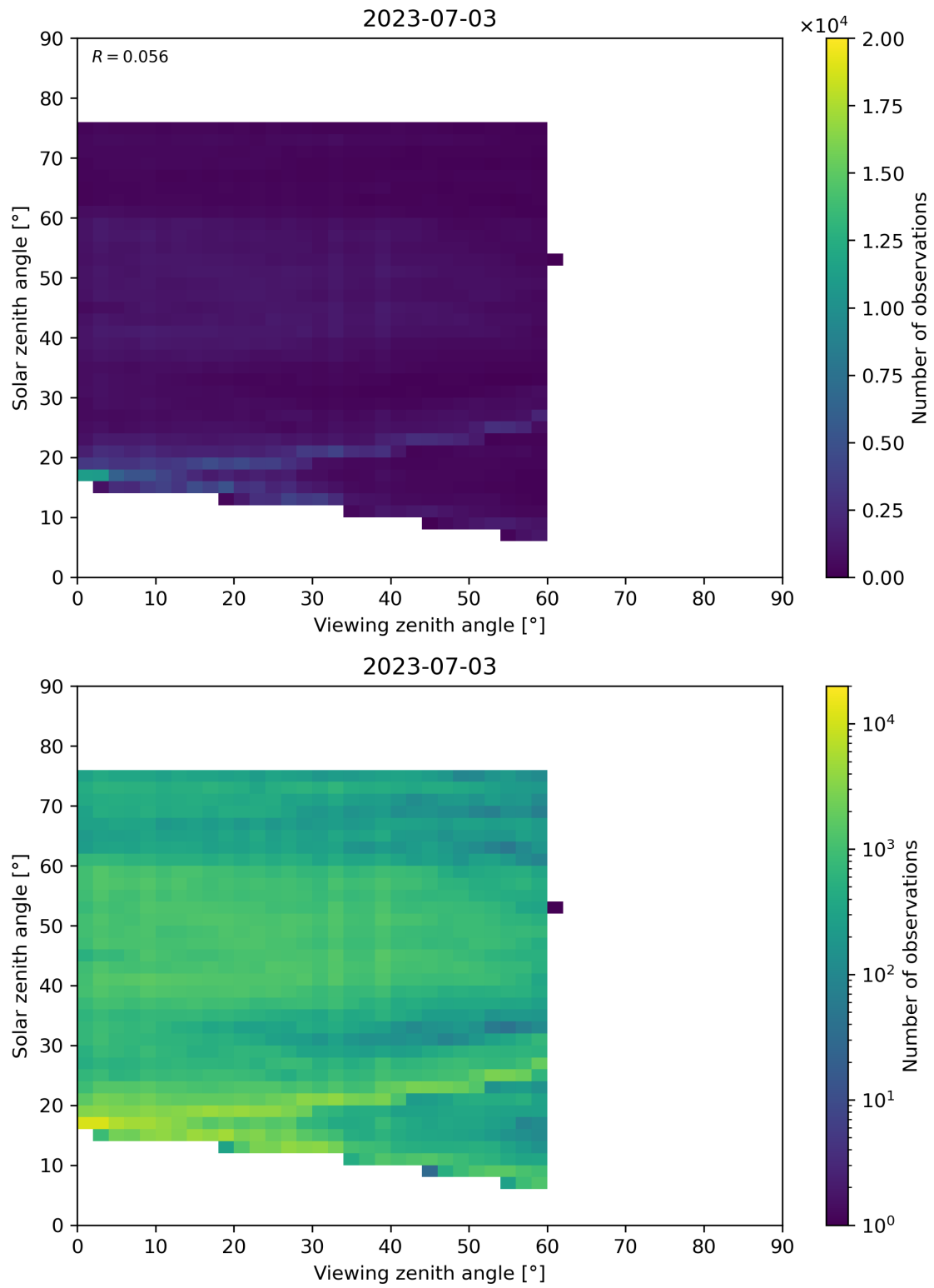
Figure 115: Scatter density plot of “Viewing zenith angle” against “Solar zenith angle” for 2023-07-03 to 2023-07-04.
