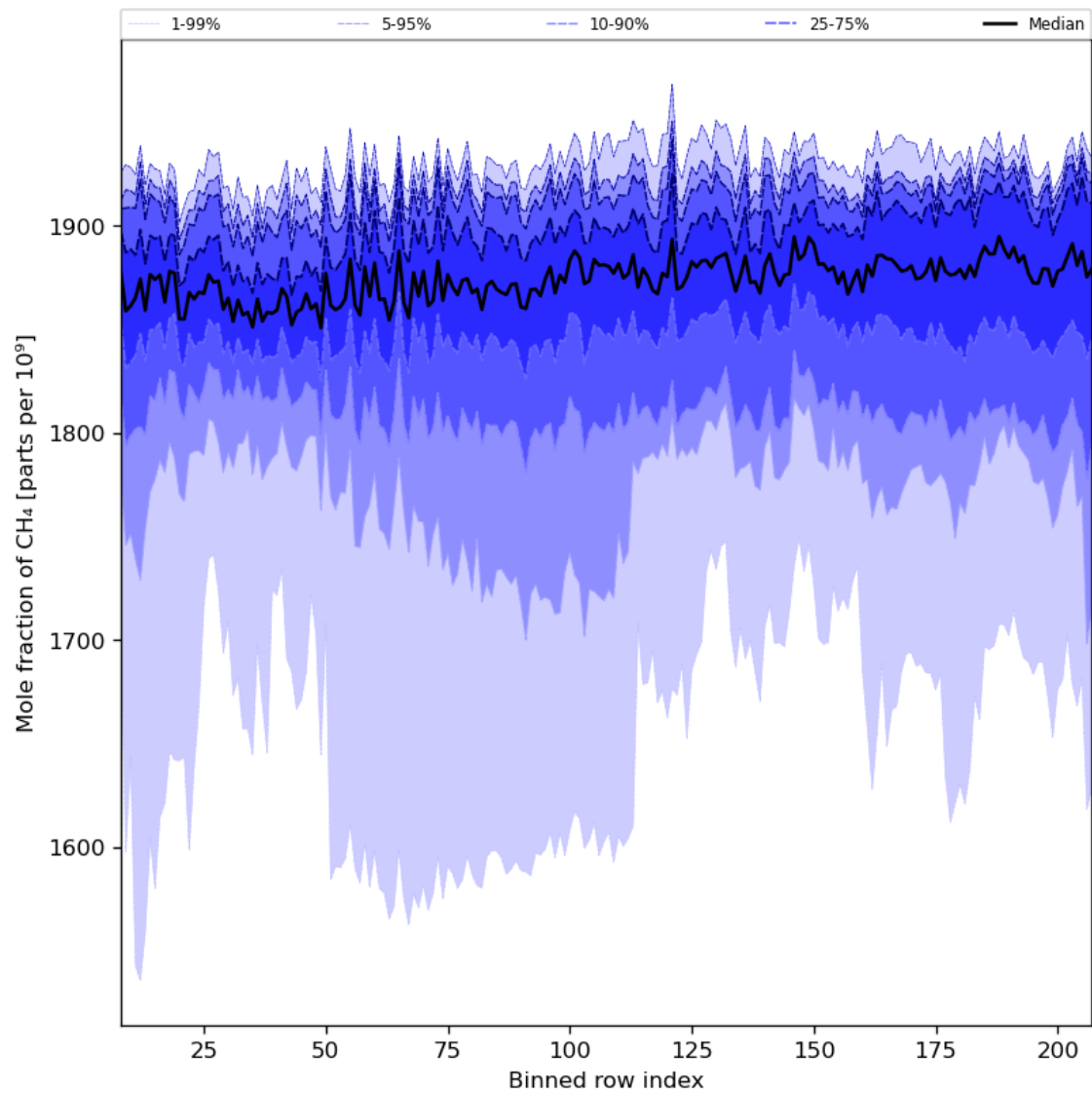
Figure 34: Along track statistics of “Mole fraction of CH 4 ” for 2023-07-03 to 2023-07-04
