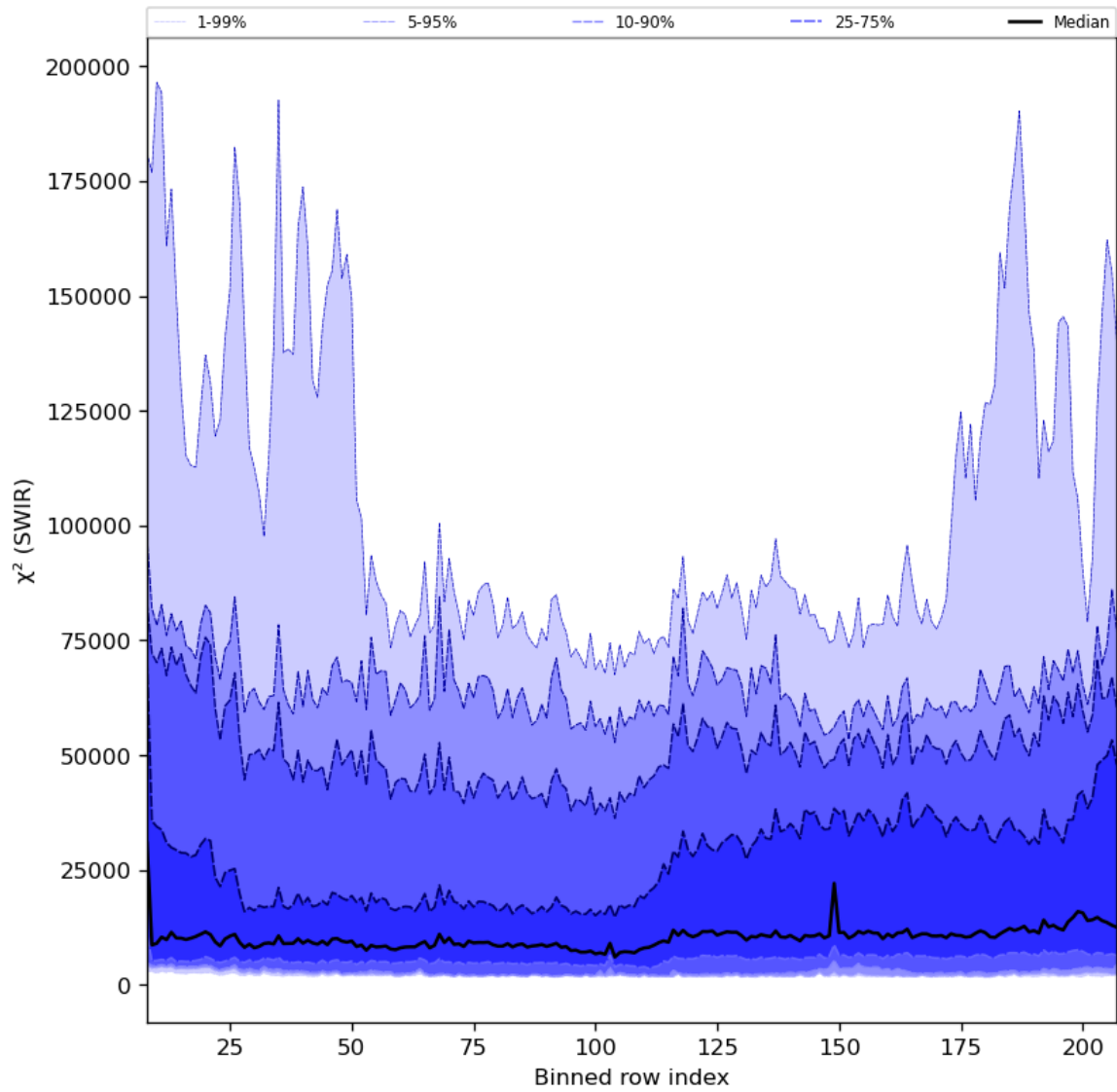
Figure 39: Along track statistics of " \chi^2 (SWIR)" for 2023-07-03 to 2023-07-04
