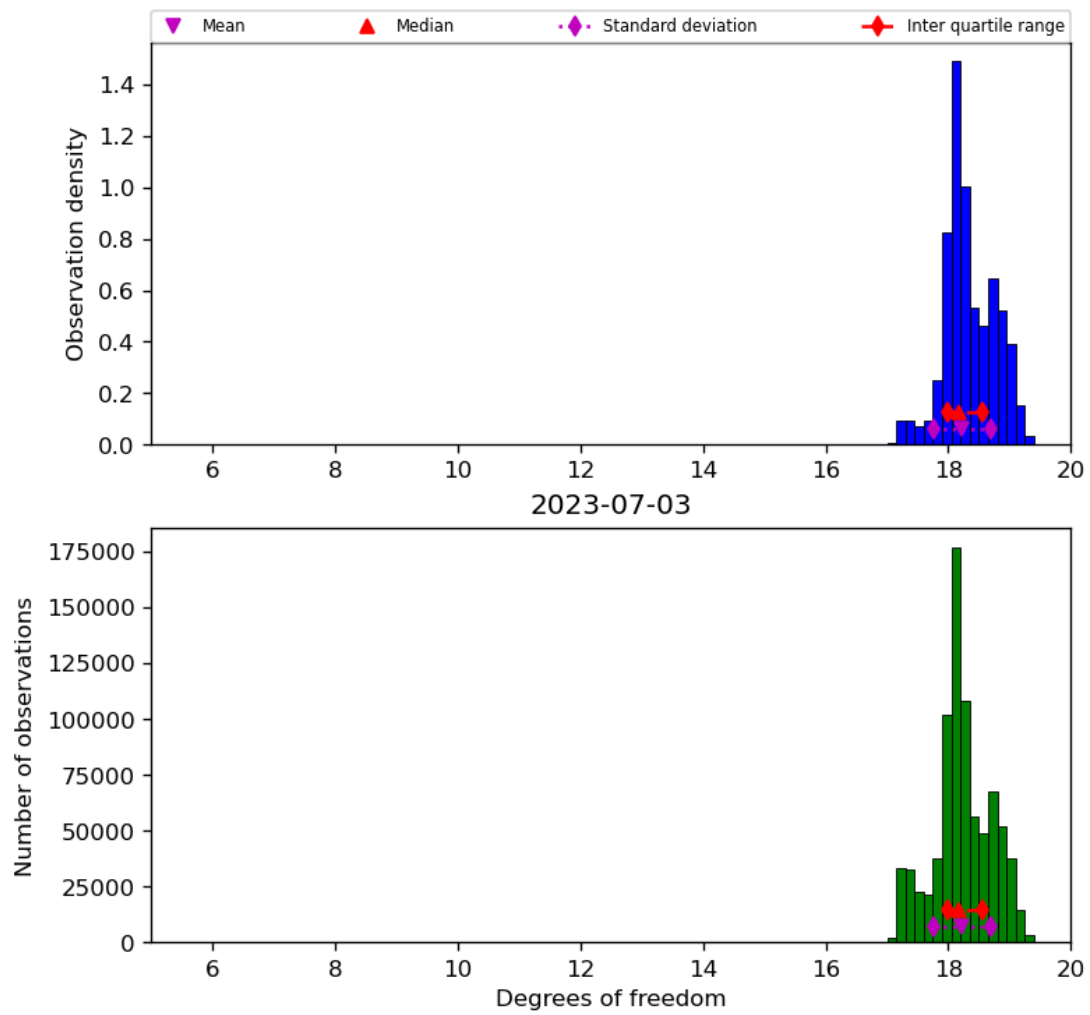
Figure 30: Histogram of “Degrees of freedom” for 2023-07-03 to 2023-07-04
