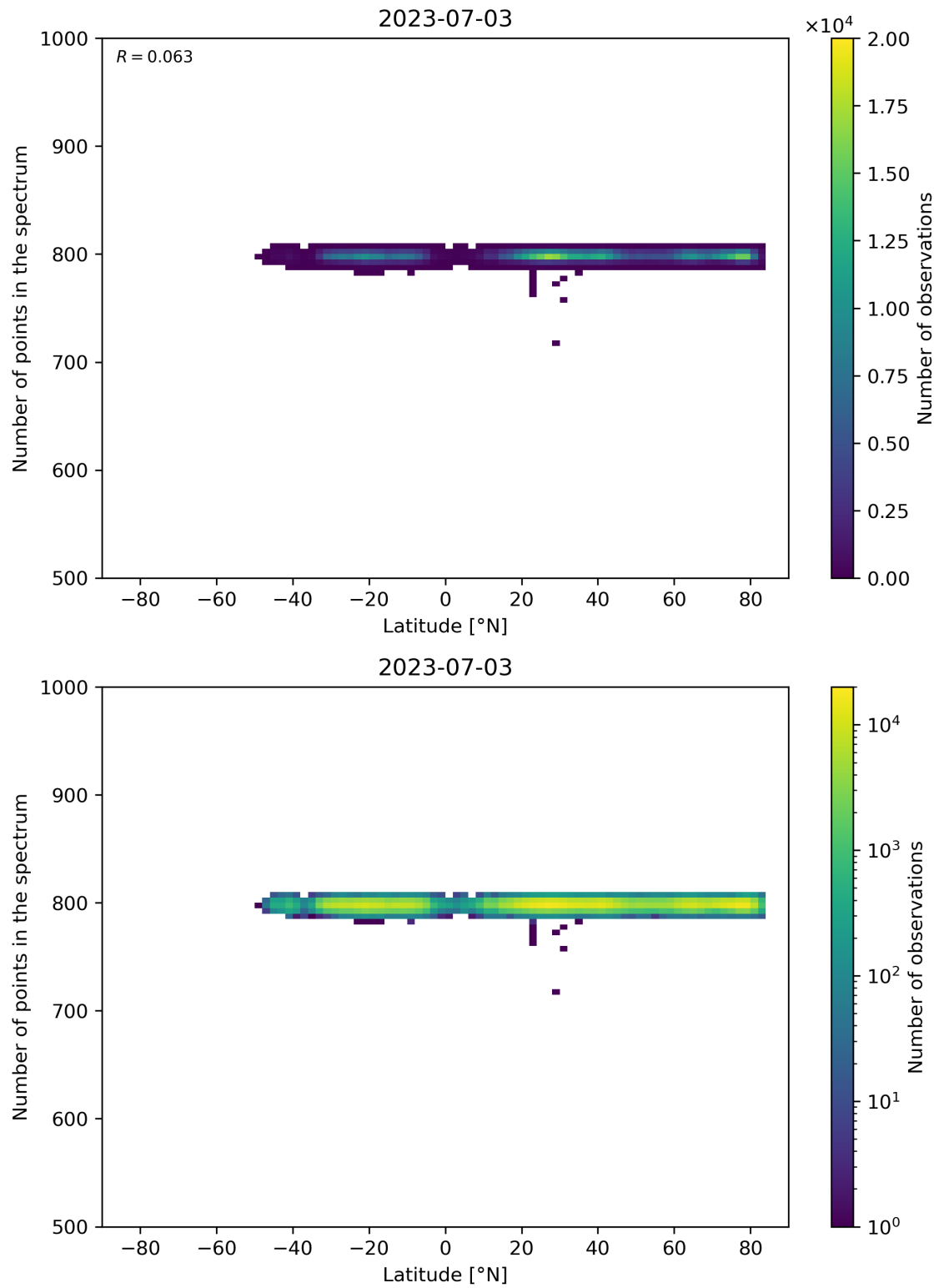
Figure 61: Scatter density plot of “Latitude” against “Number of points in the spectrum” for 2023-07-03 to 2023-07-04.
