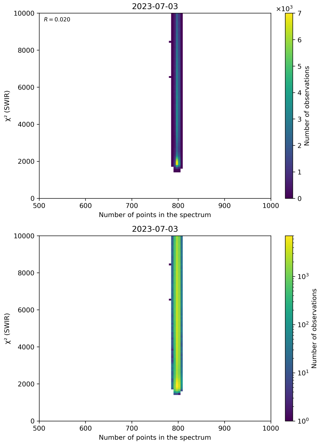
Figure 89: Scatter density plot of “Number of points in the spectrum” against “ \chi^2 (SWIR)” for 2023-07-03 to 2023-07-04.
