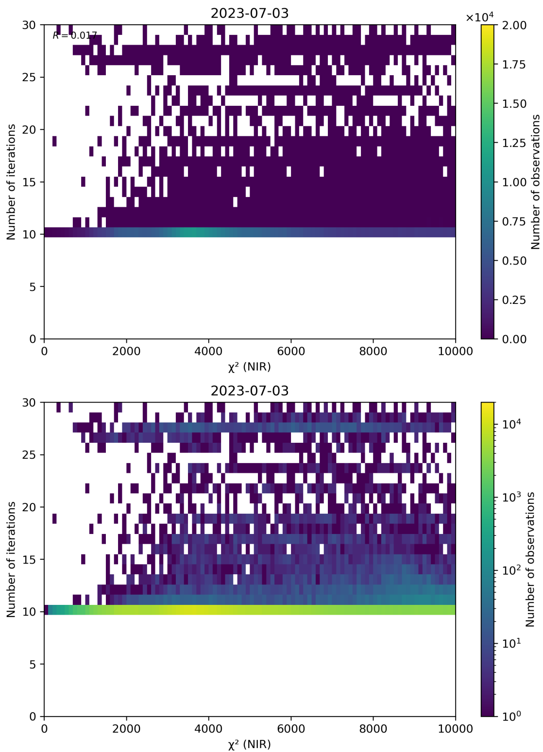
Figure 46: Scatter density plot of “ \chi^2 (NIR)” against “Number of iterations” for 2023-07-03 to 2023-07-04.
