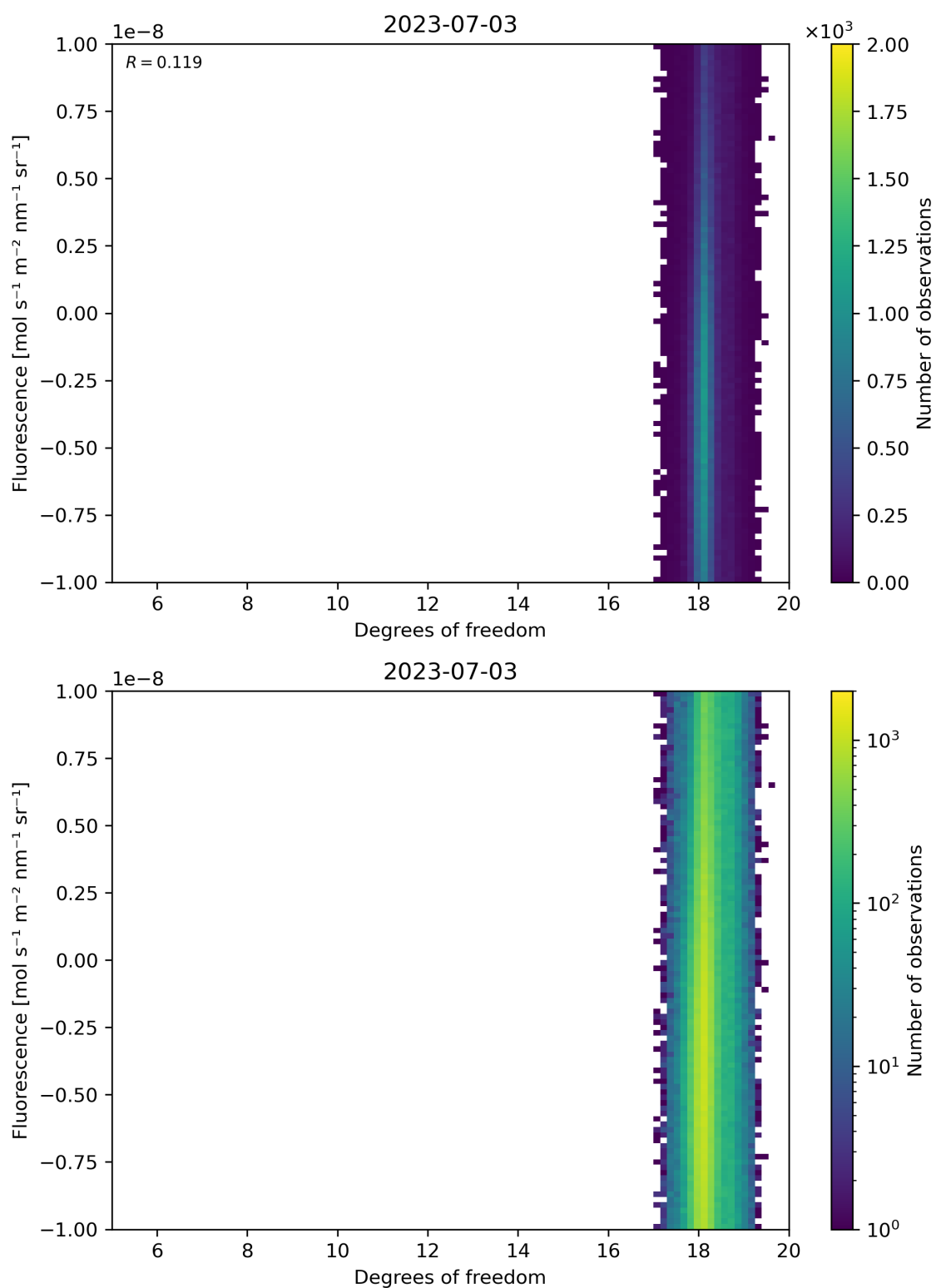
Figure 51: Scatter density plot of “Degrees of freedom” against “Fluorescence” for 2023-07-03 to 2023-07-04.
