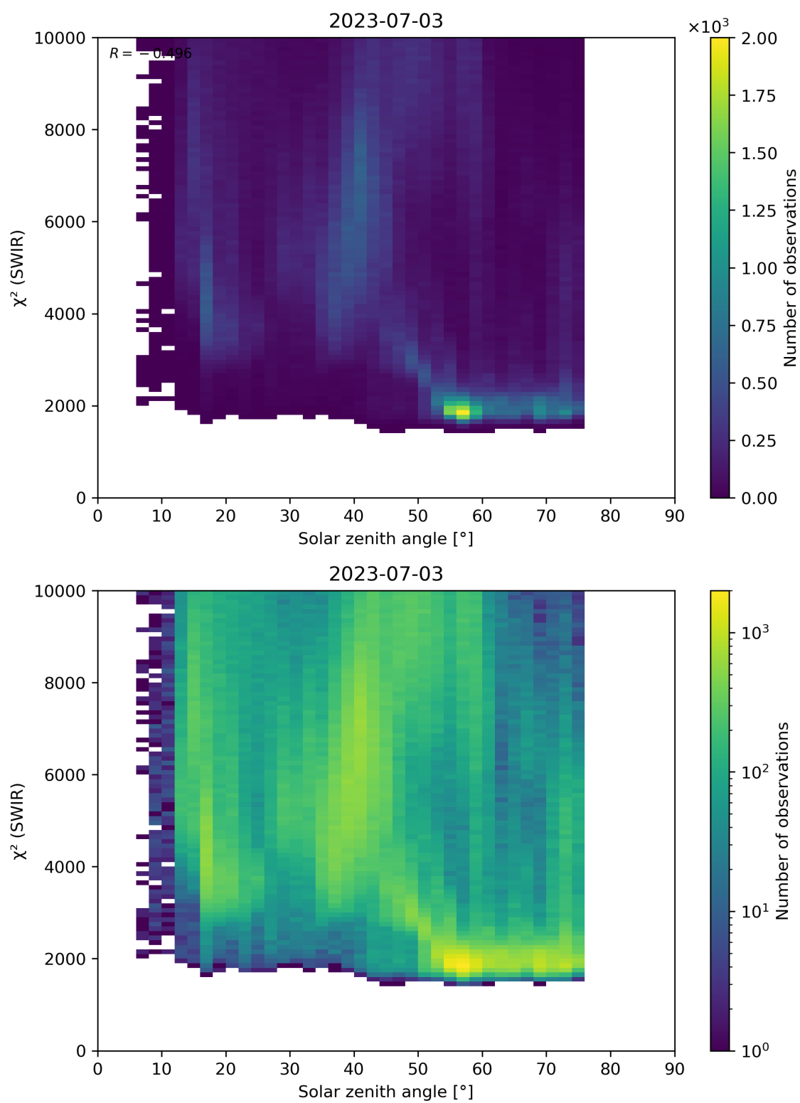
Figure 95: Scatter density plot of “Solar zenith angle” against “ \chi^2 (SWIR)” for 2023-07-03 to 2023-07-04.
