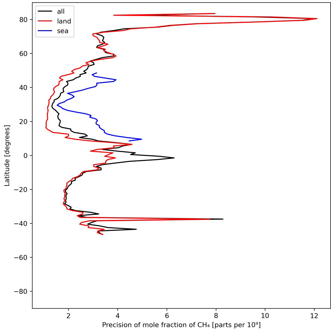
Figure 13: Zonal average of “Precision of mole fraction of CH 4 ” for 2023-07-03 to 2023-07-04.
