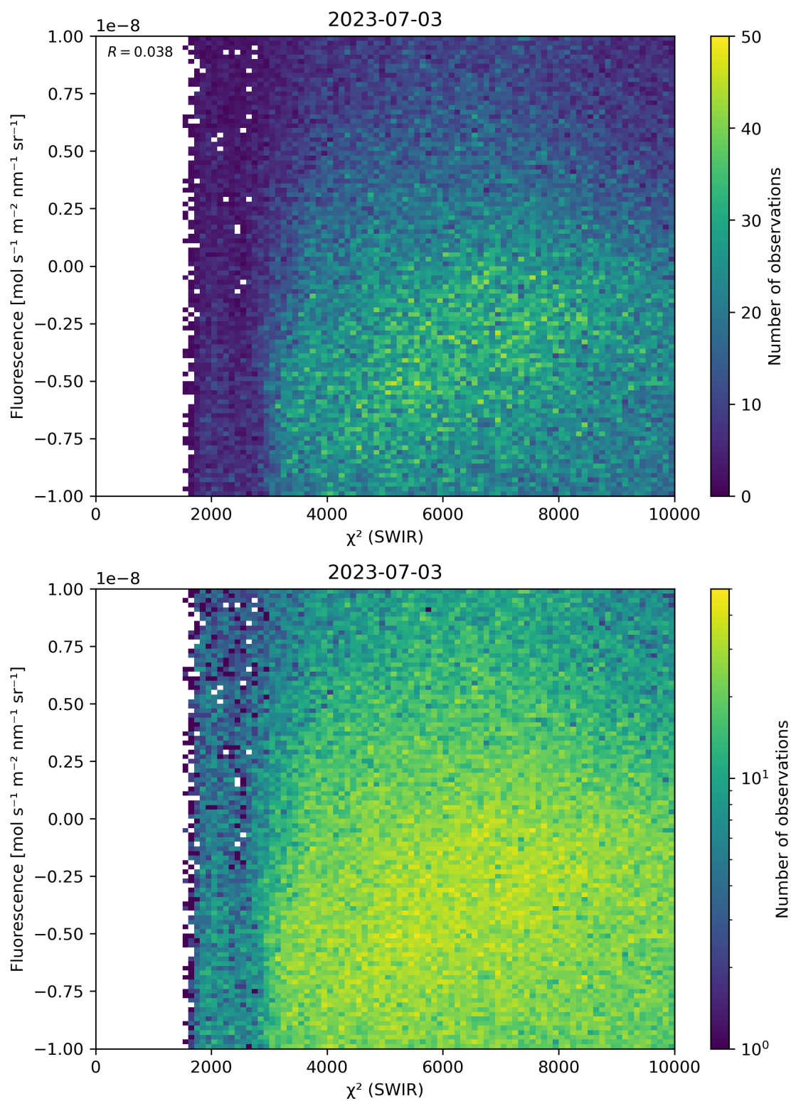
Figure 49: Scatter density plot of “ \chi^2 (SWIR)” against “Fluorescence” for 2023-07-03 to 2023-07-04.
