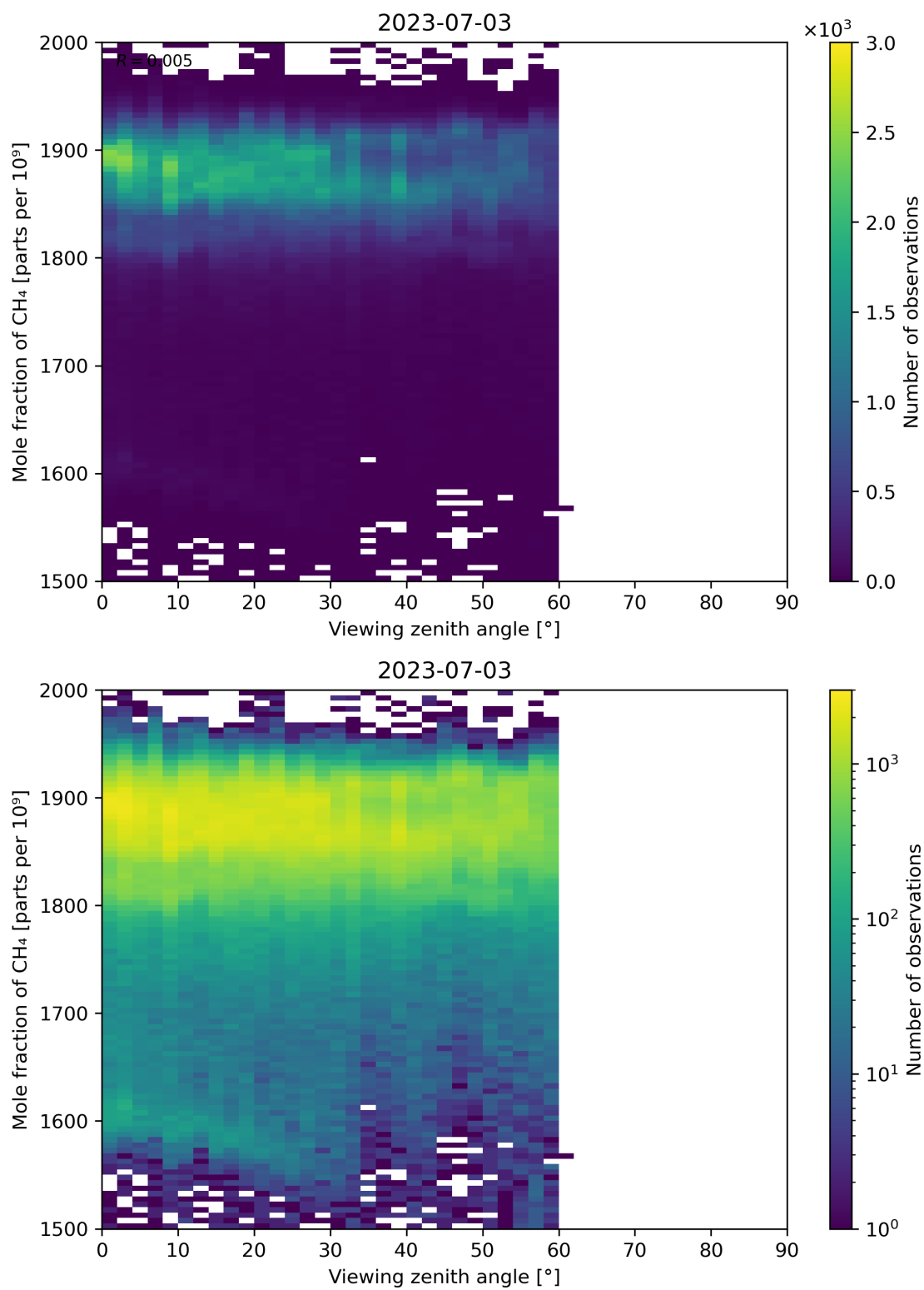
Figure 110: Scatter density plot of “Viewing zenith angle” against “Mole fraction of CH 4 ” for 2023-07-03 to 2023-07-04.
