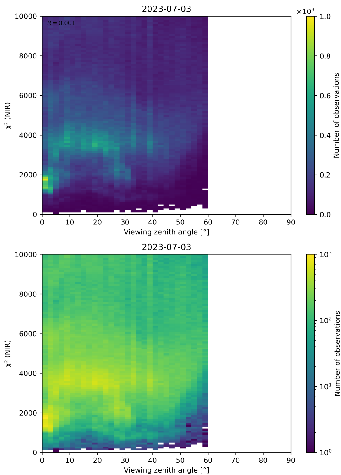
Figure 105: Scatter density plot of “Viewing zenith angle” against “ \chi^2 (NIR)” for 2023-07-03 to 2023-07-04.
