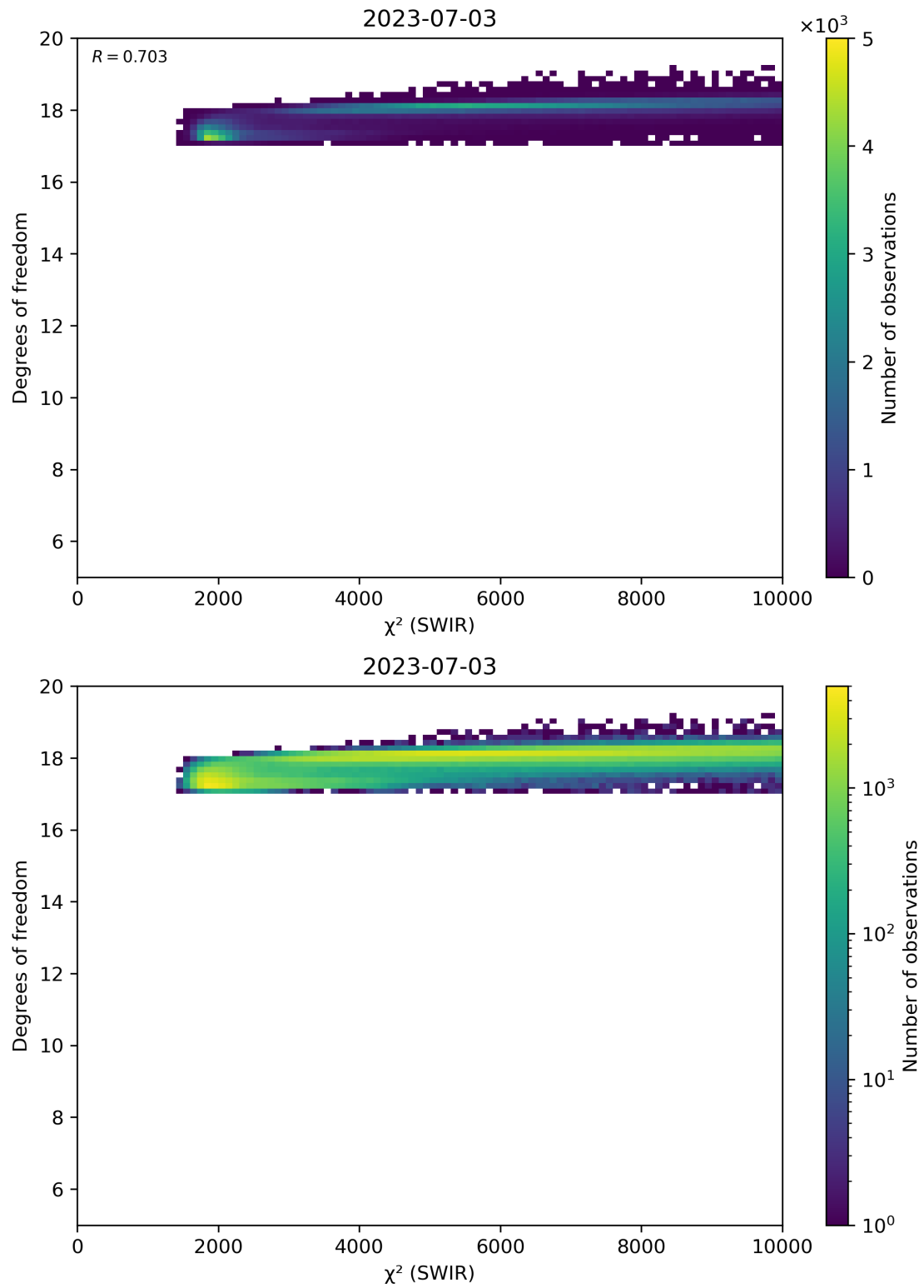
Figure 48: Scatter density plot of “ \chi^2 (SWIR)” against “Degrees of freedom” for 2023-07-03 to 2023-07-04.
