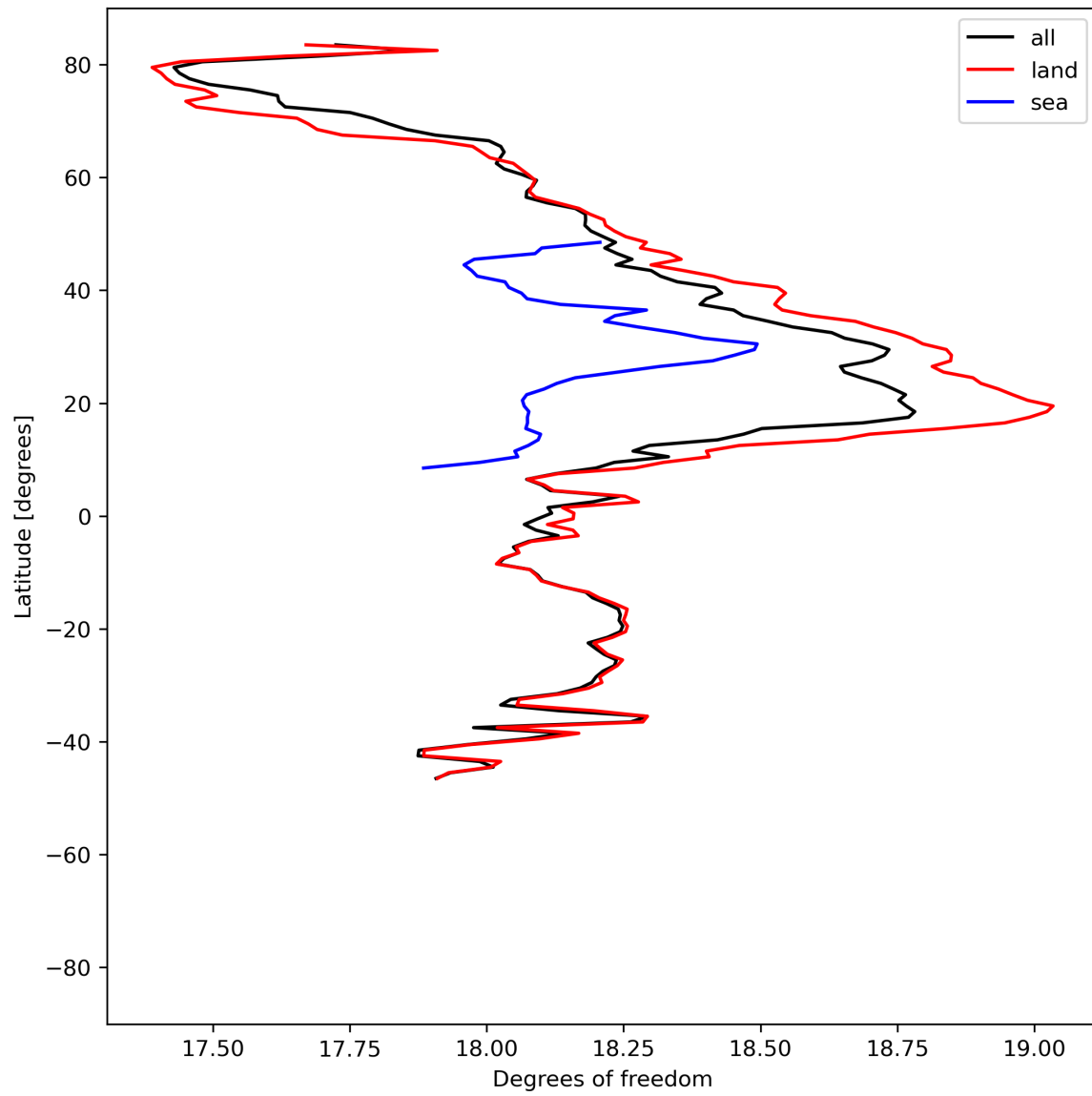
Figure 19: Zonal average of “Degrees of freedom” for 2023-07-03 to 2023-07-04.
