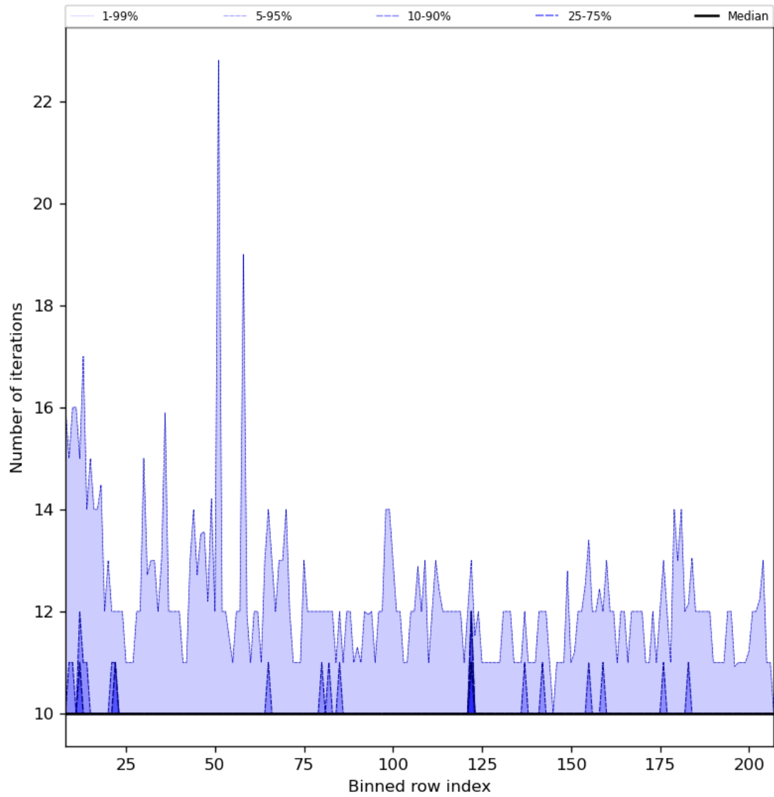
Figure 42: Along track statistics of “Number of iterations” for 2023-07-03 to 2023-07-04
