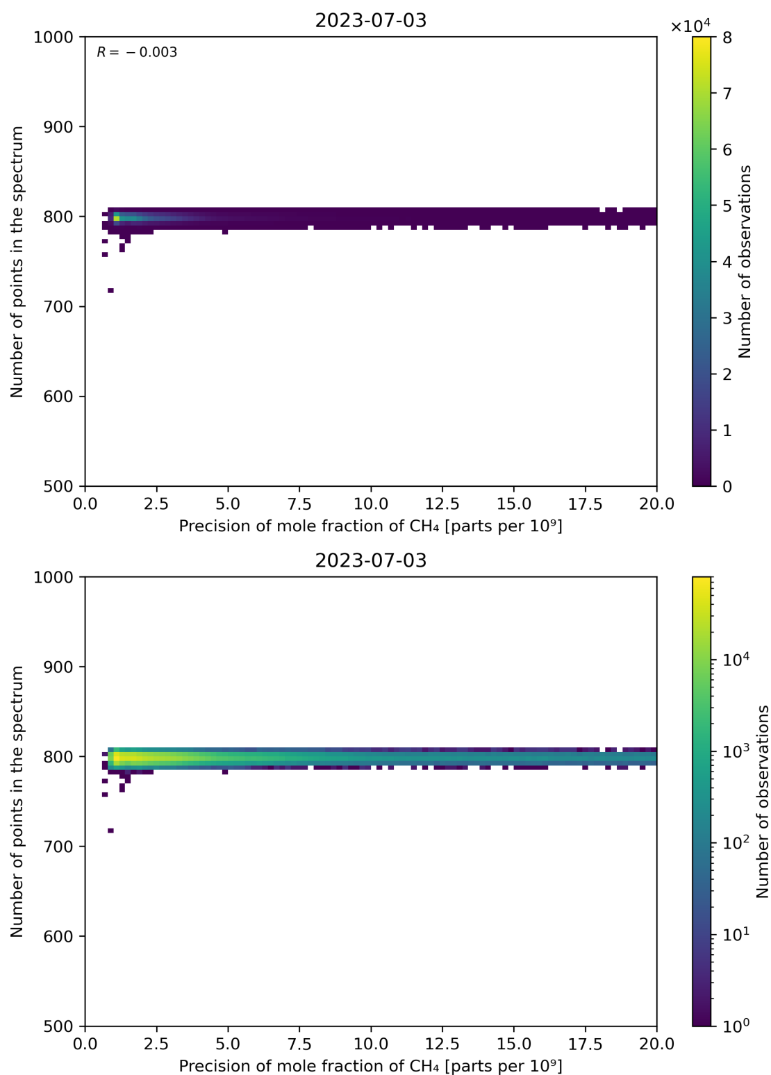
Figure 84: Scatter density plot of “Precision of mole fraction of CH 4 ” against “Number of points in the spectrum” for 2023-07-03 to 2023-07-04.
