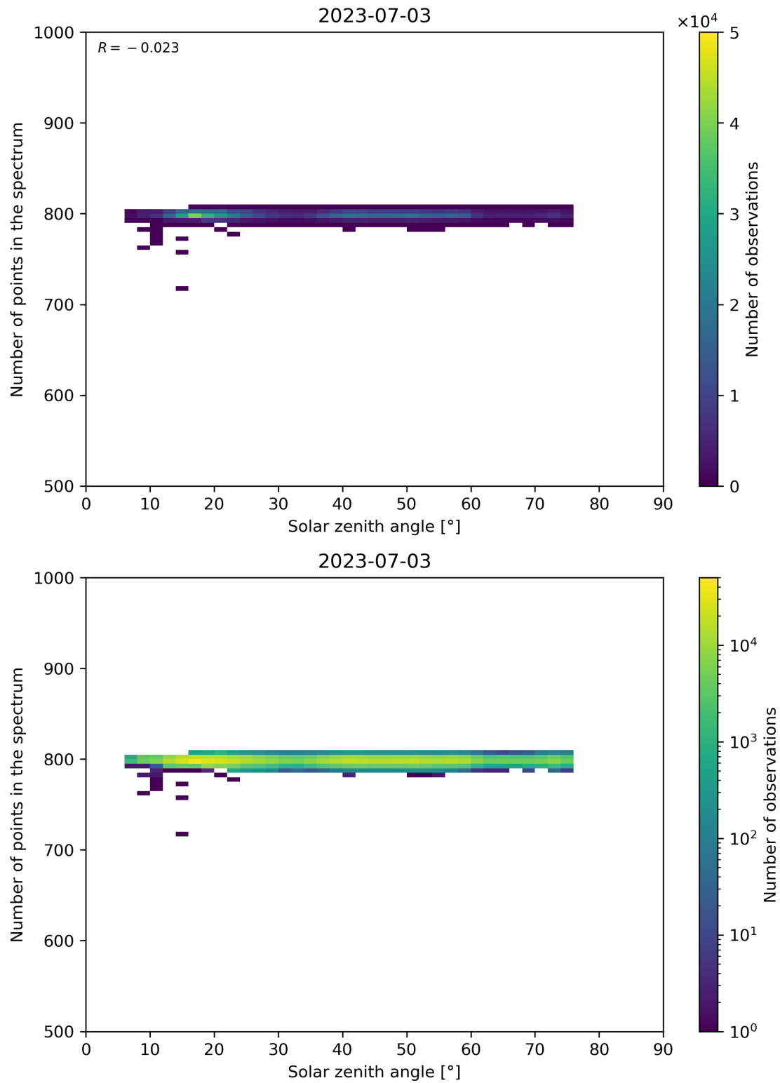
Figure 103: Scatter density plot of “Solar zenith angle” against “Number of points in the spectrum” for 2023-07-03 to 2023-07-04.
