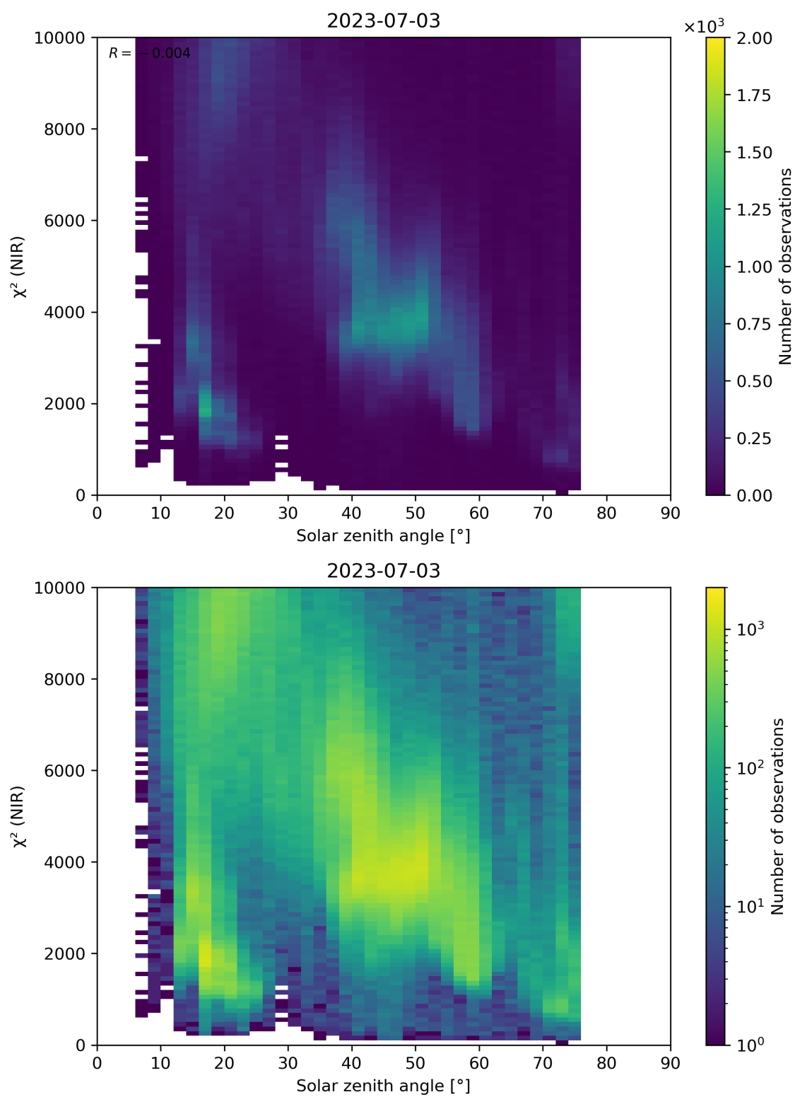
Figure 94: Scatter density plot of “Solar zenith angle” against “ \chi^2 (NIR)” for 2023-07-03 to 2023-07-04.
