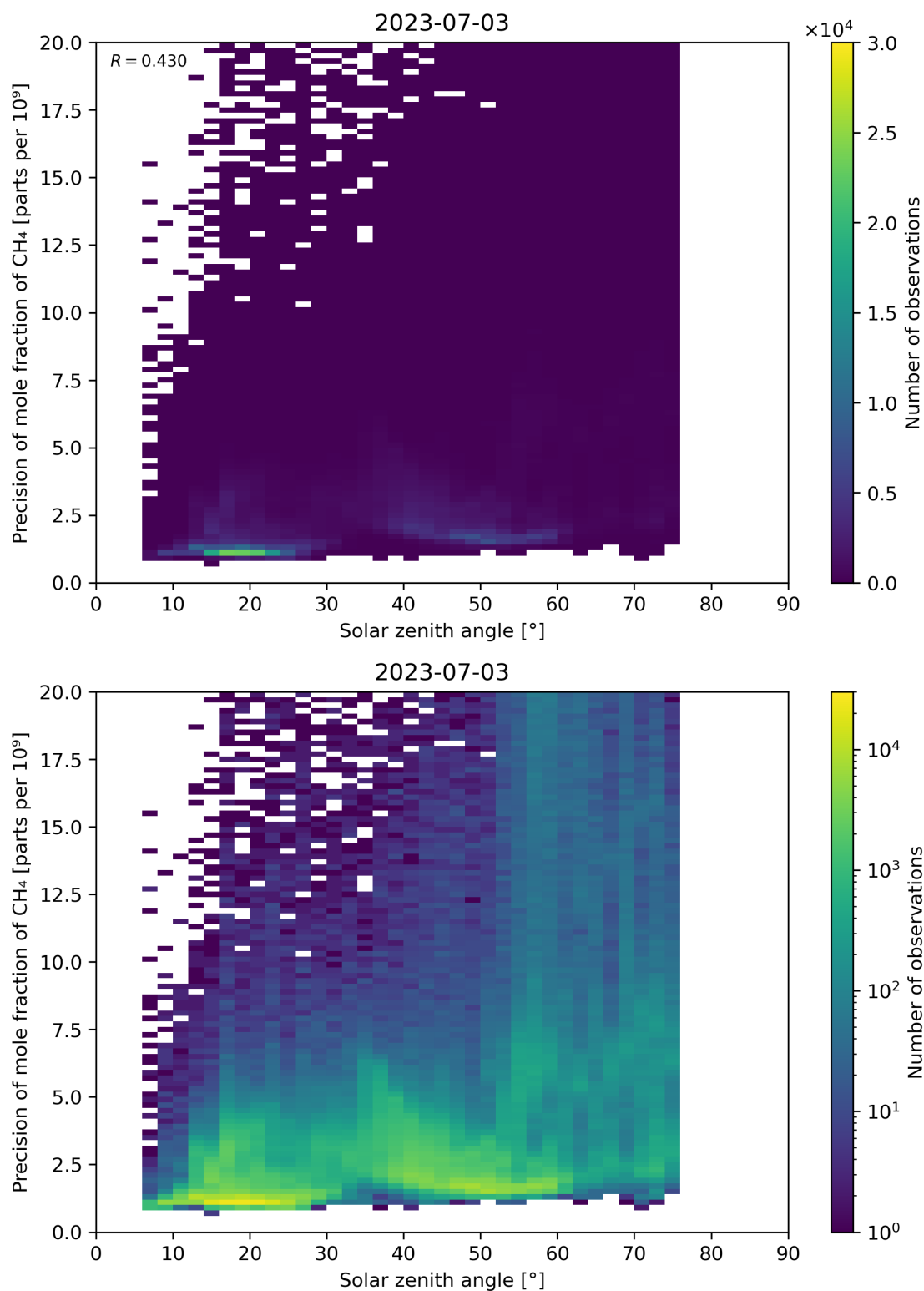
Figure 101: Scatter density plot of “Solar zenith angle” against “Precision of mole fraction of CH 4 ” for 2023-07-03 to 2023-07-04.
