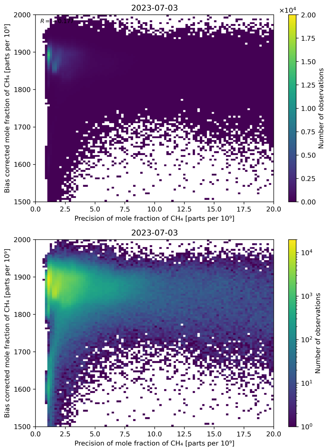
Figure 82: Scatter density plot of “Precision of mole fraction of CH 4 ” against “Bias corrected mole fraction of CH 4 ” for 2023-07-03 to 2023-07-04.
