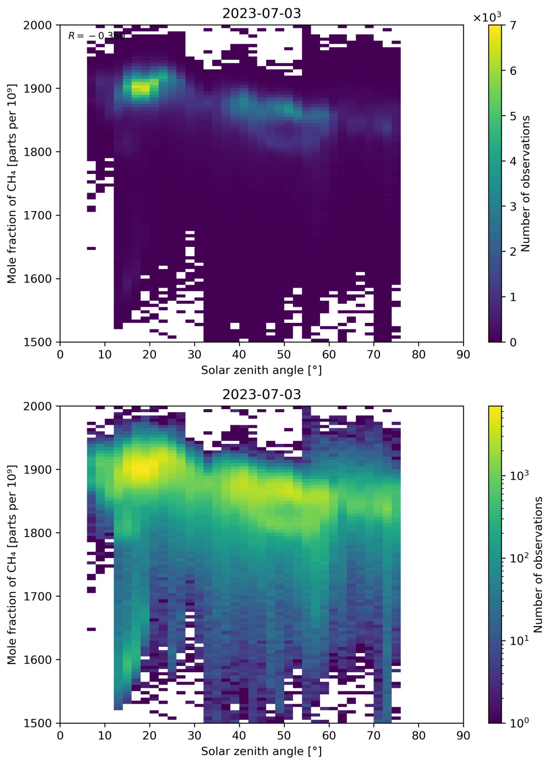
Figure 99: Scatter density plot of “Solar zenith angle” against “Mole fraction of CH 4 ” for 2023-07-03 to 2023-07-04.
