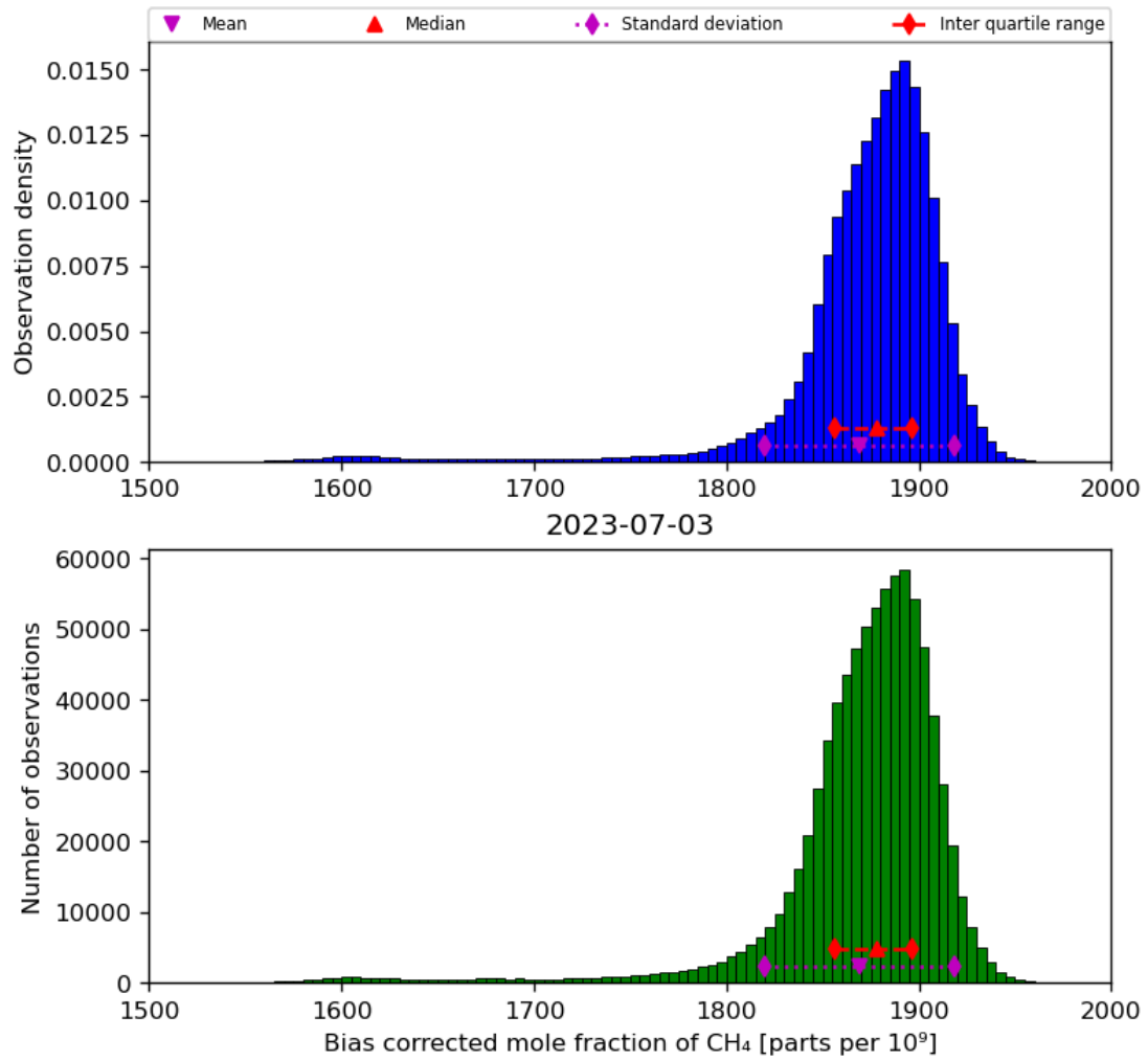
Figure 25: Histogram of “Bias corrected mole fraction of CH 4 ” for 2023-07-03 to 2023-07-04
