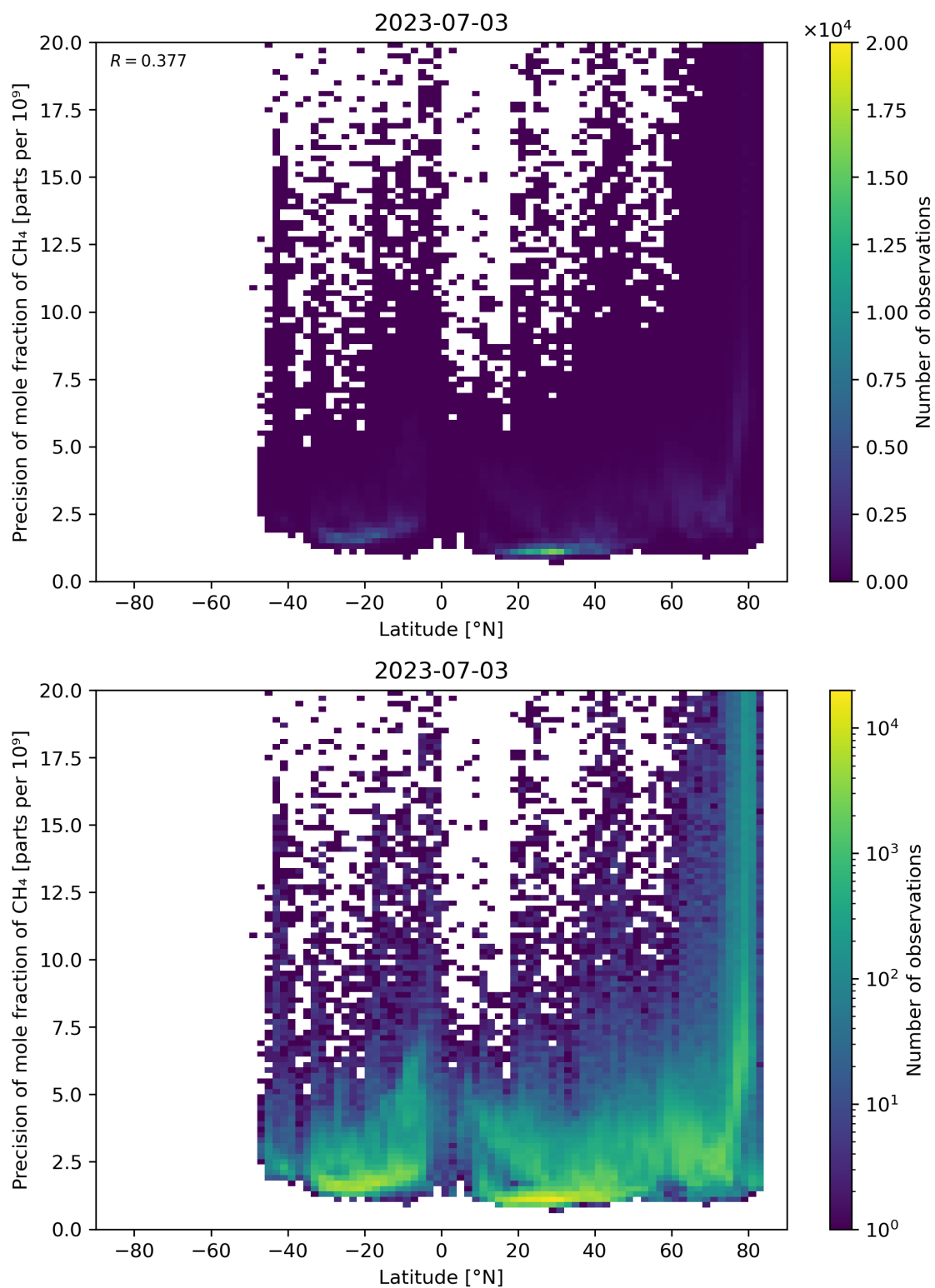
Figure 59: Scatter density plot of “Latitude” against “Precision of mole fraction of \text{CH}_4 ” for 2023-07-03 to 2023-07-04.
