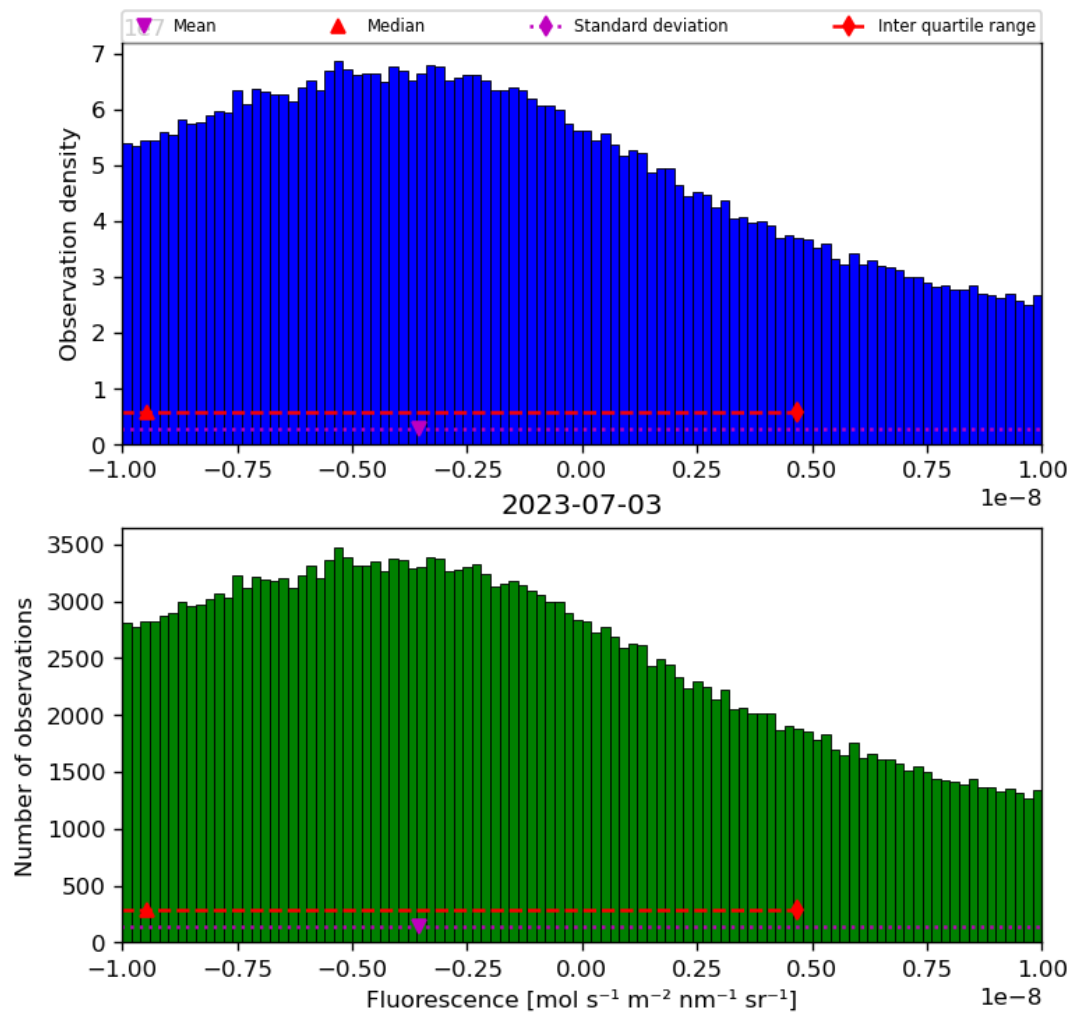
Figure 32: Histogram of “Fluorescence” for 2023-07-03 to 2023-07-04
