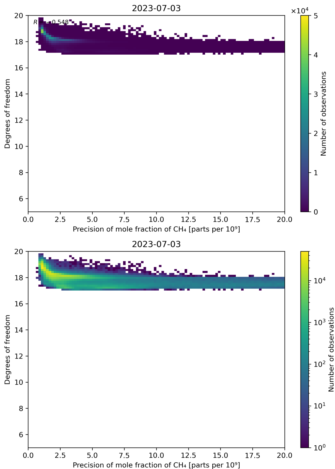
Figure 80: Scatter density plot of “Precision of mole fraction of CH 4 ” against “Degrees of freedom” for 2023-07-03 to 2023-07-04.
