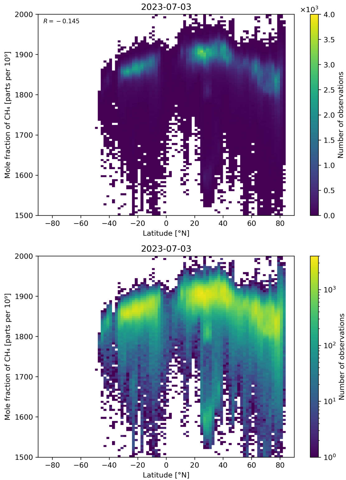
Figure 57: Scatter density plot of “Latitude” against “Mole fraction of \text{CH}_4 ” for 2023-07-03 to 2023-07-04.
