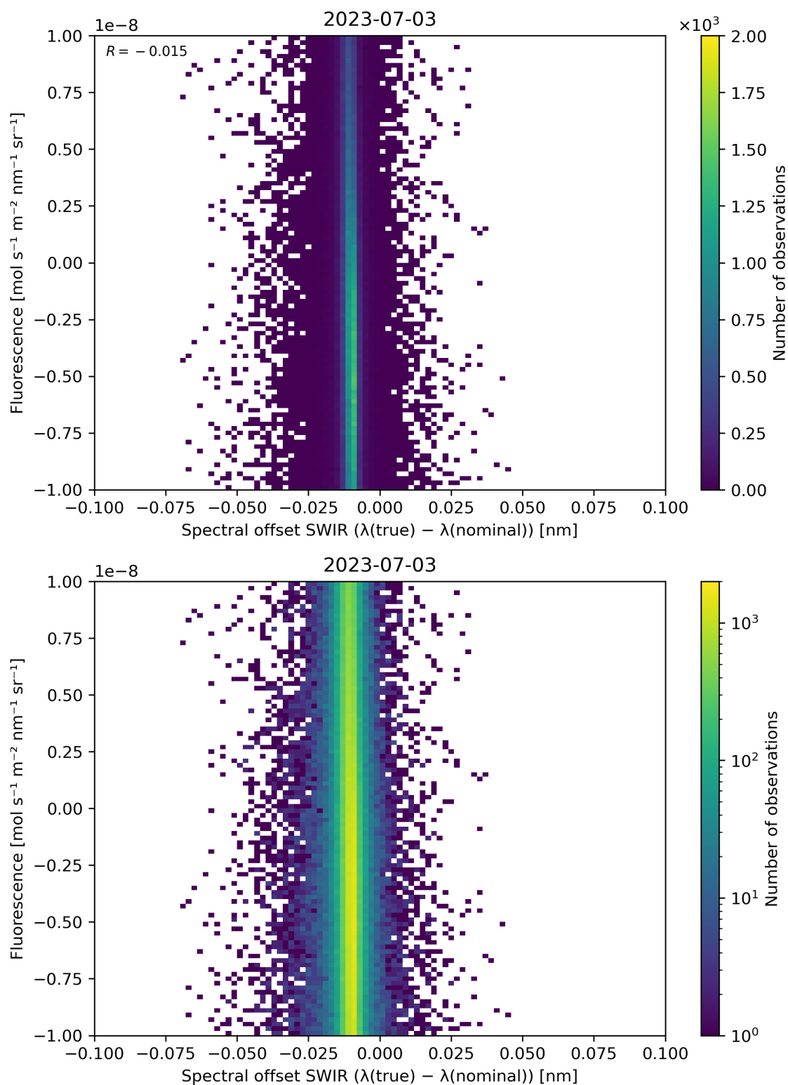
Figure 120: Scatter density plot of “Spectral offset SWIR ( \lambda(\text{true}) - \lambda(\text{nominal}) )” against “Fluorescence” for 2023-07-03 to 2023-07-04.
