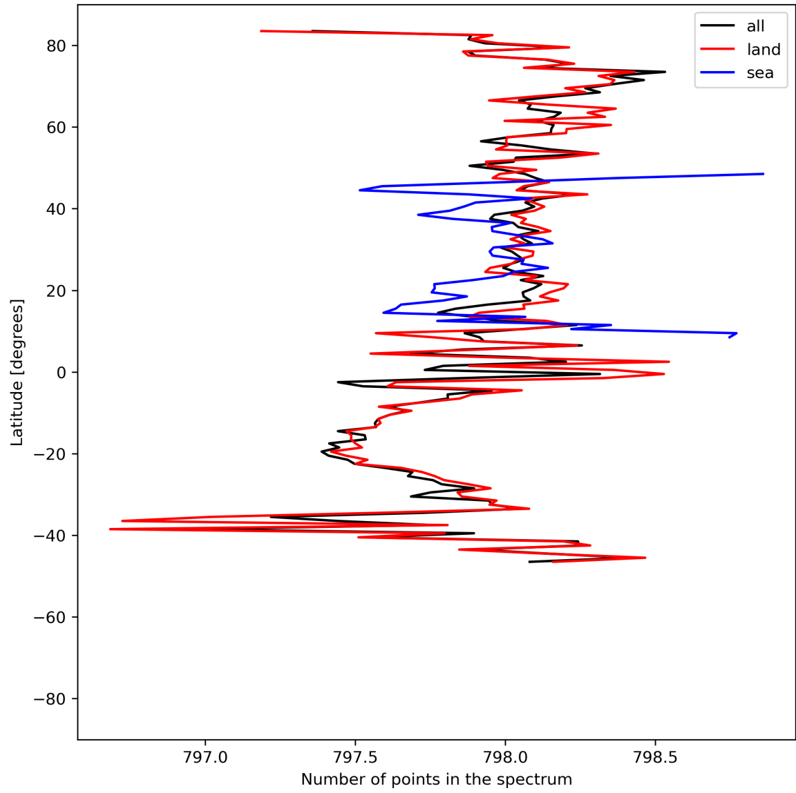
Figure 15: Zonal average of “Number of points in the spectrum” for 2023-07-03 to 2023-07-04.
