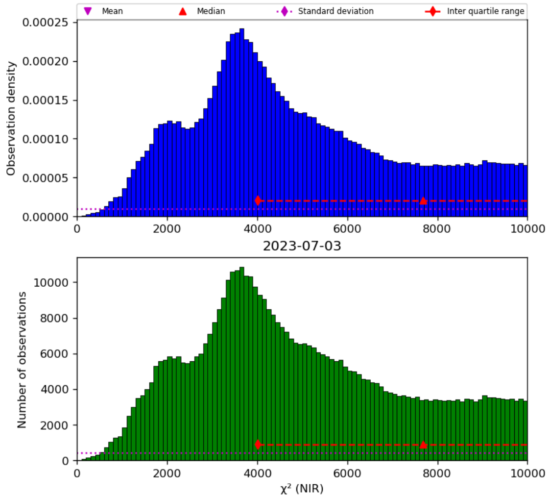
Figure 29: Histogram of “ \chi^2 (NIR)” for 2023-07-03 to 2023-07-04
