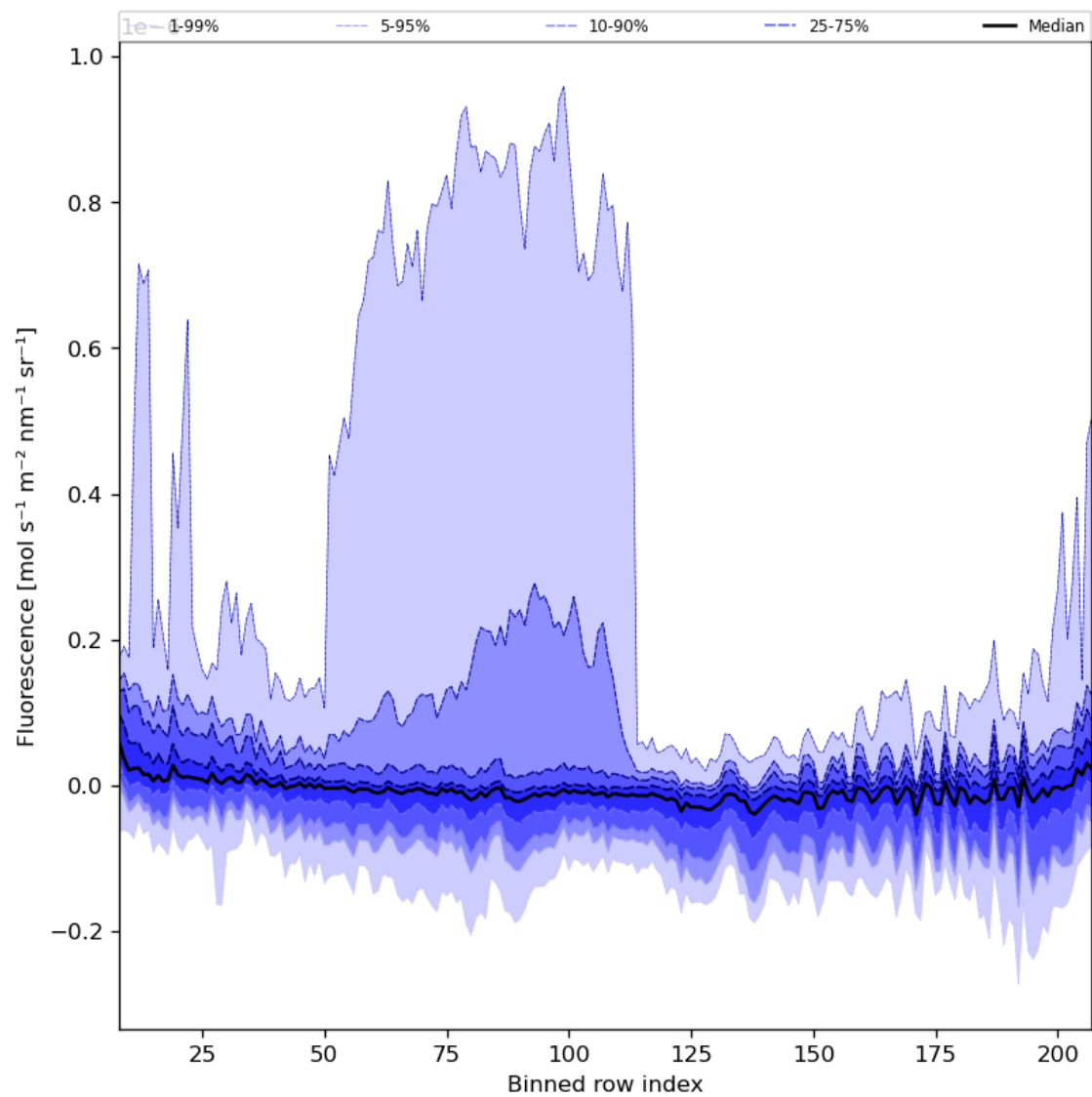
Figure 43: Along track statistics of “Fluorescence” for 2023-07-03 to 2023-07-04
