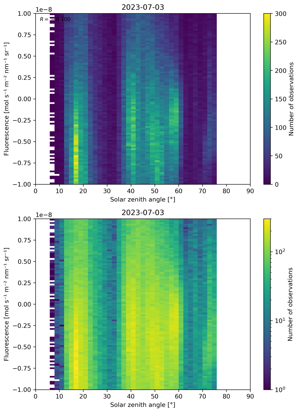
Figure 97: Scatter density plot of “Solar zenith angle” against “Fluorescence” for 2023-07-03 to 2023-07-04.
