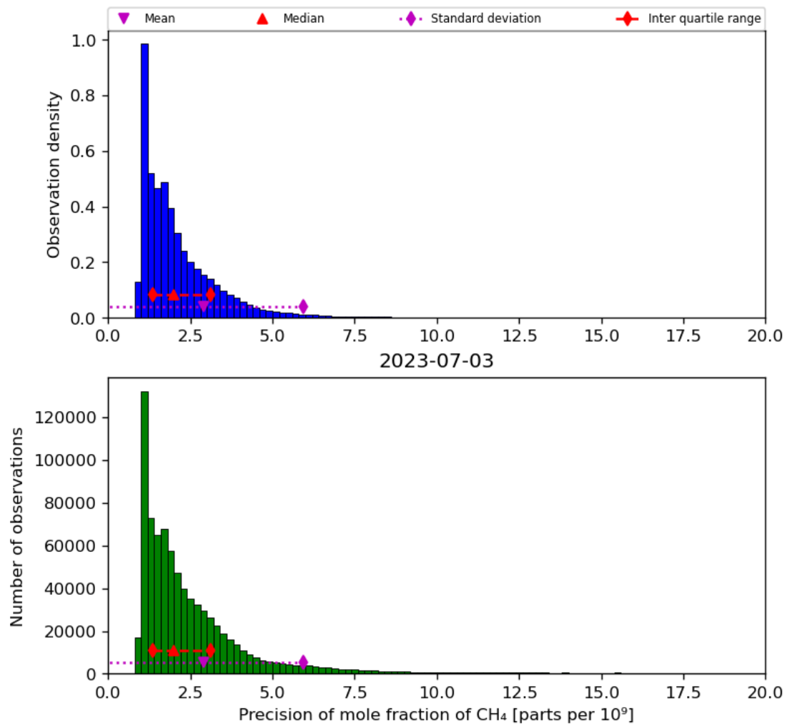
Figure 24: Histogram of “Precision of mole fraction of CH 4 ” for 2023-07-03 to 2023-07-04
