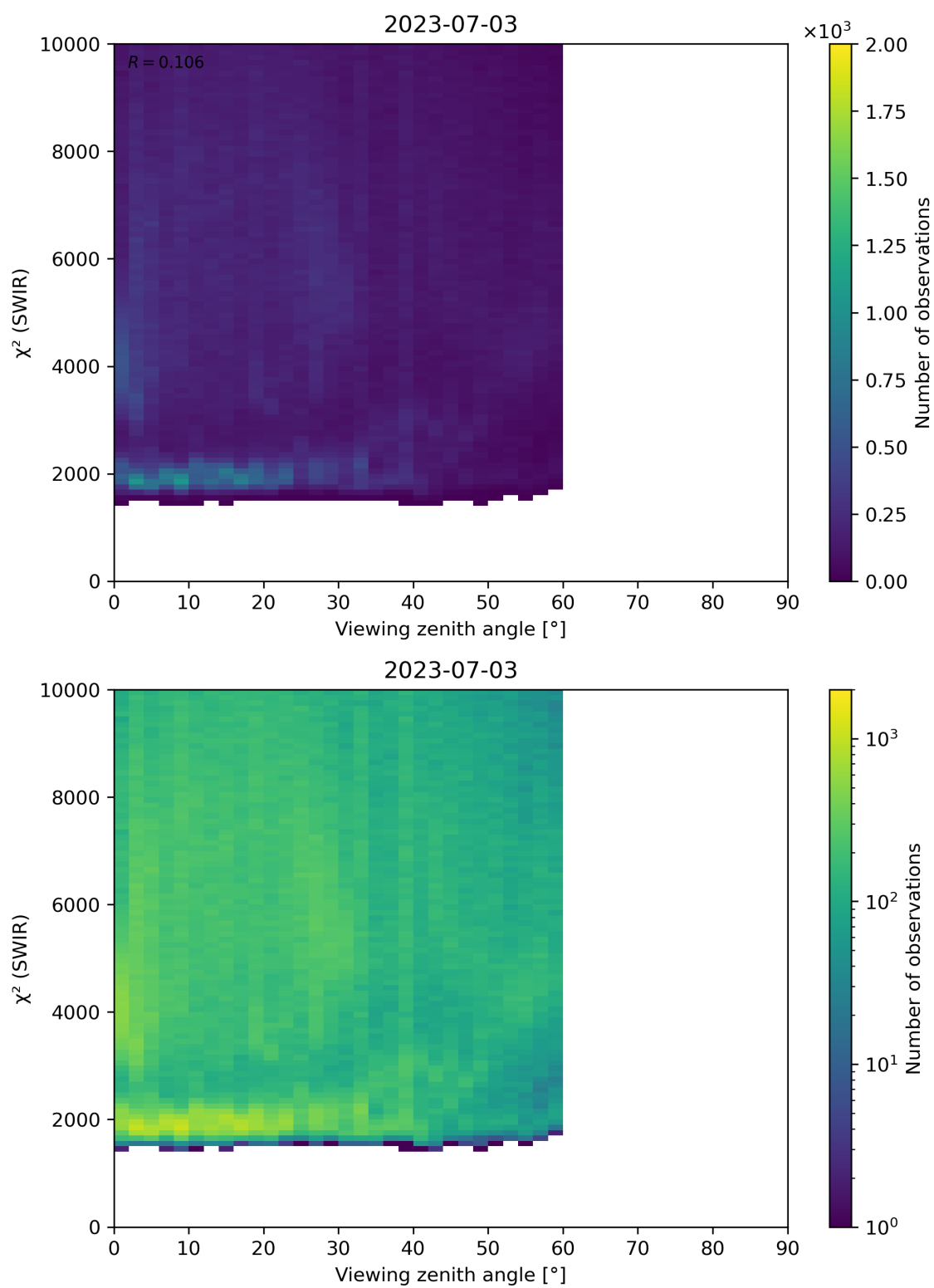
Figure 106: Scatter density plot of “Viewing zenith angle” against “ \chi^2 (SWIR)” for 2023-07-03 to 2023-07-04.
