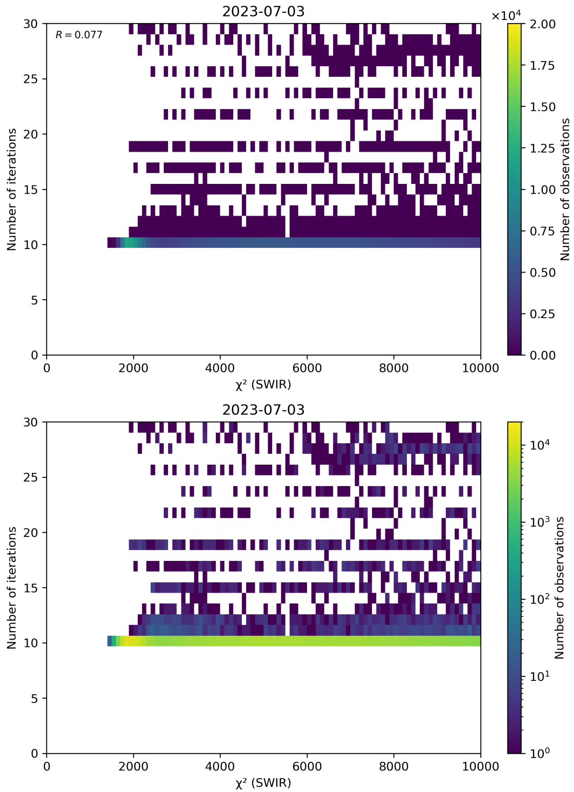
Figure 50: Scatter density plot of “ \chi^2 (SWIR)” against “Number of iterations” for 2023-07-03 to 2023-07-04.
