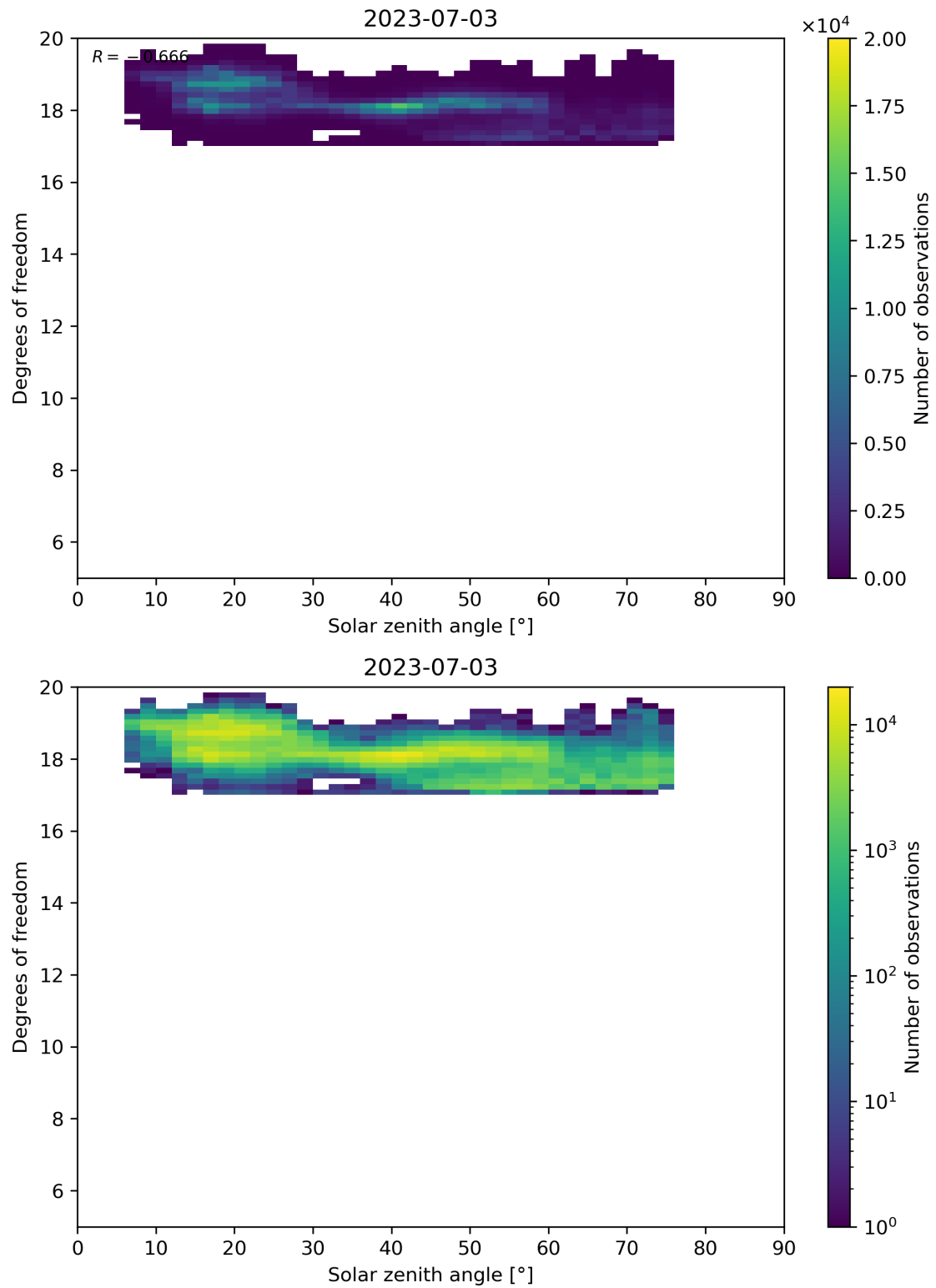
Figure 96: Scatter density plot of “Solar zenith angle” against “Degrees of freedom” for 2023-07-03 to 2023-07-04.
