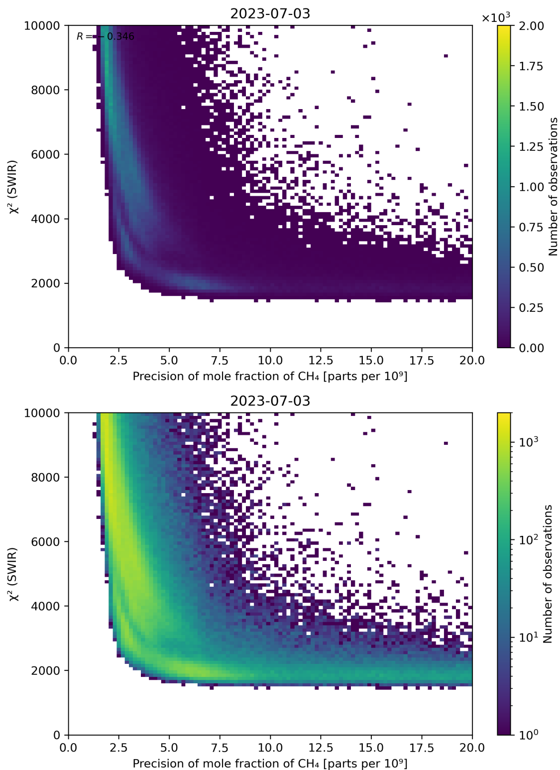
Figure 79: Scatter density plot of “Precision of mole fraction of CH 4 ” against “ \chi^2 (SWIR)” for 2023-07-03 to 2023-07-04.
