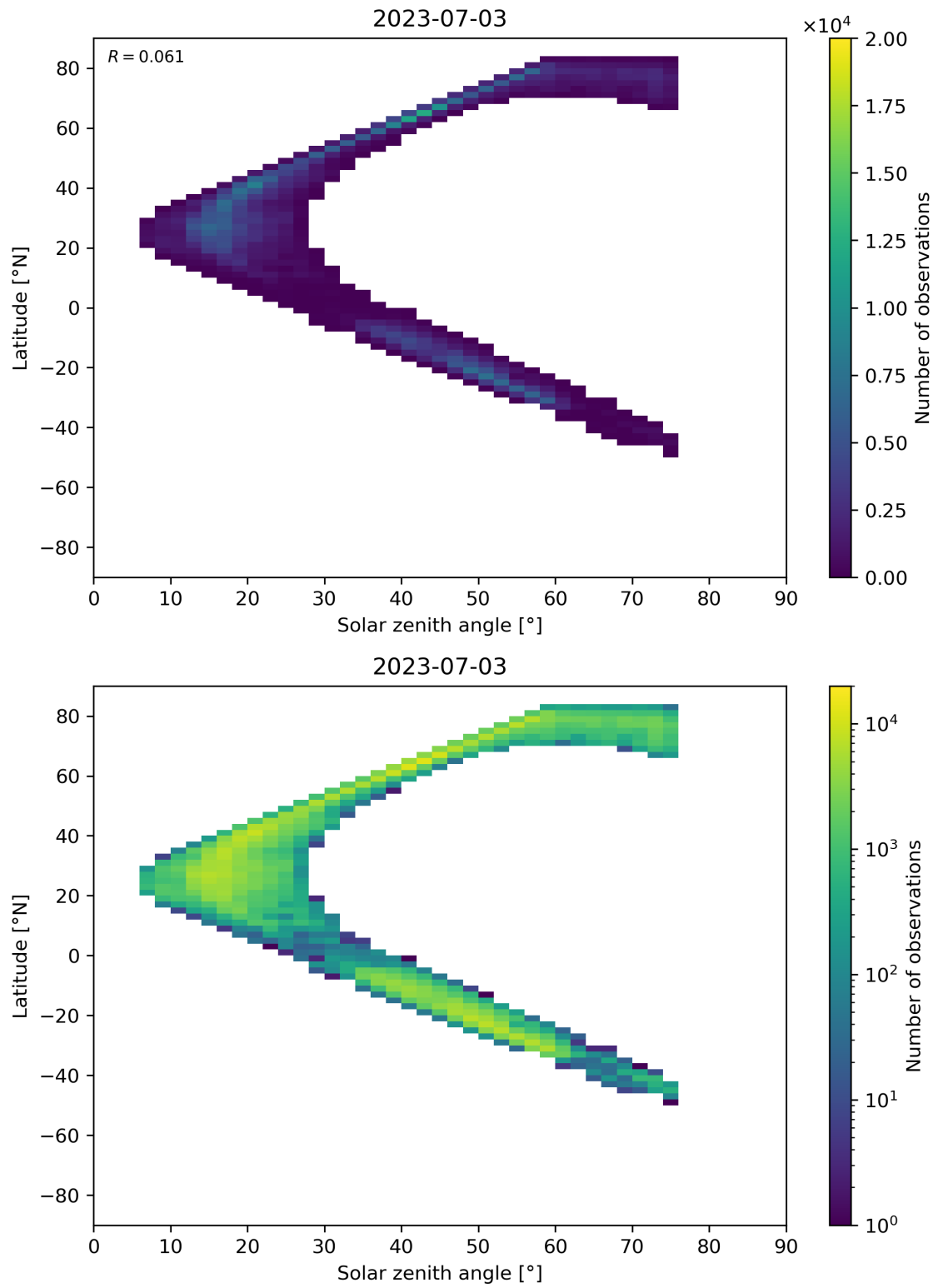
Figure 98: Scatter density plot of “Solar zenith angle” against “Latitude” for 2023-07-03 to 2023-07-04.
