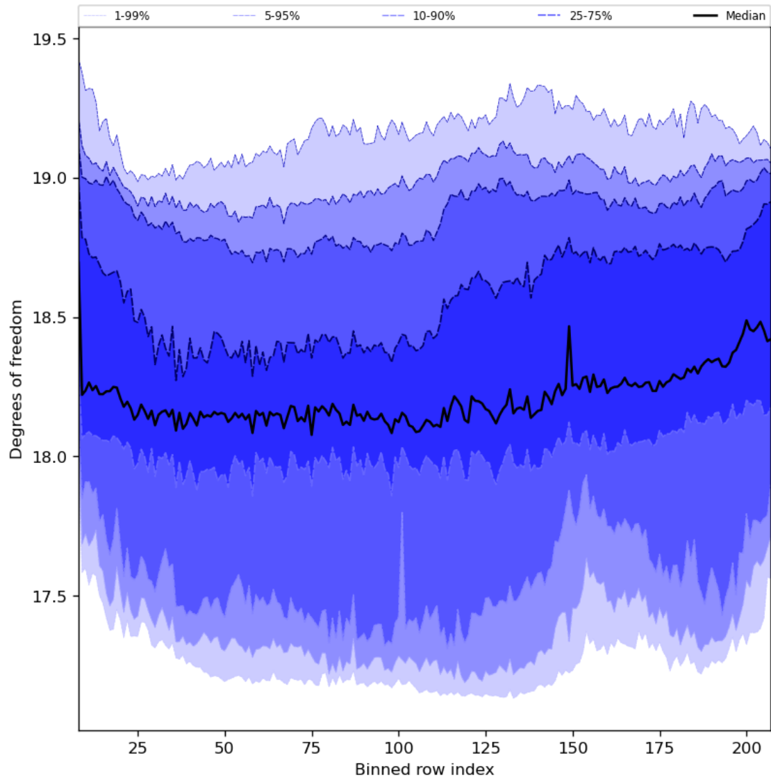
Figure 41: Along track statistics of “Degrees of freedom” for 2023-07-03 to 2023-07-04
