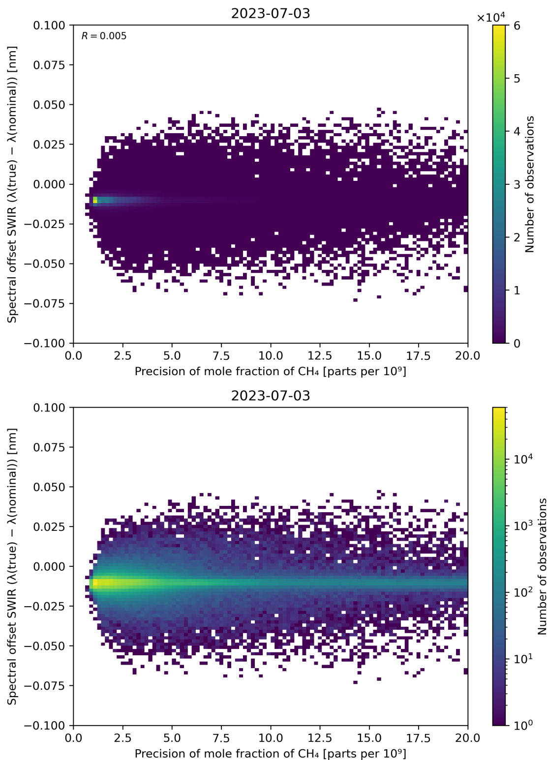
Figure 85: Scatter density plot of “Precision of mole fraction of CH 4 ” against “Spectral offset SWIR ( \lambda(\text{true}) - \lambda(\text{nominal}) )” for 2023-07-03 to 2023-07-04.
