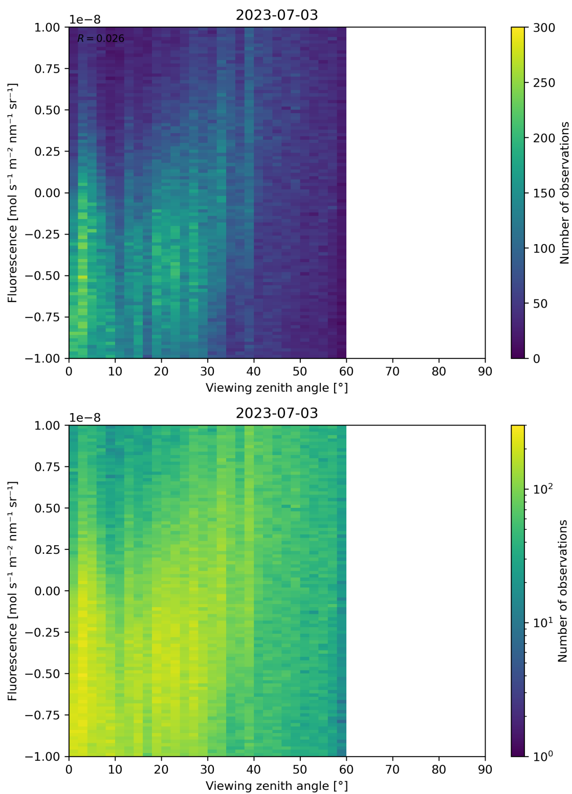
Figure 108: Scatter density plot of “Viewing zenith angle” against “Fluorescence” for 2023-07-03 to 2023-07-04.
