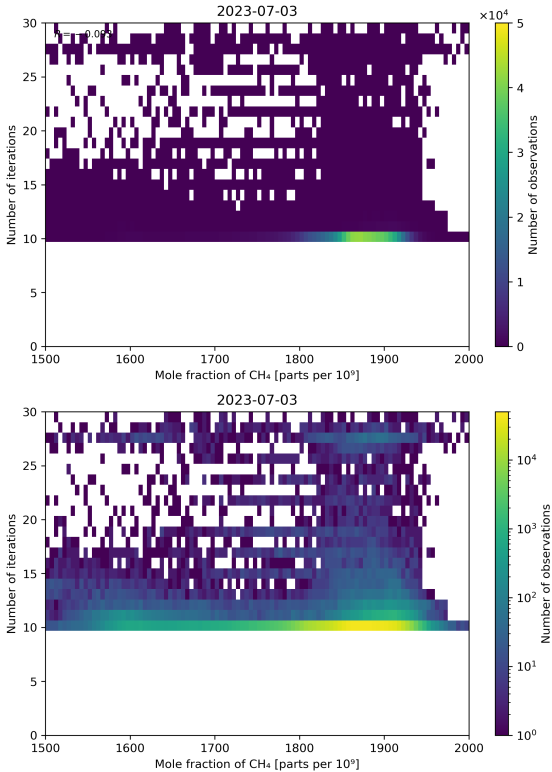
Figure 76: Scatter density plot of “Mole fraction of CH 4 ” against “Number of iterations” for 2023-07-03 to 2023-07-04.
