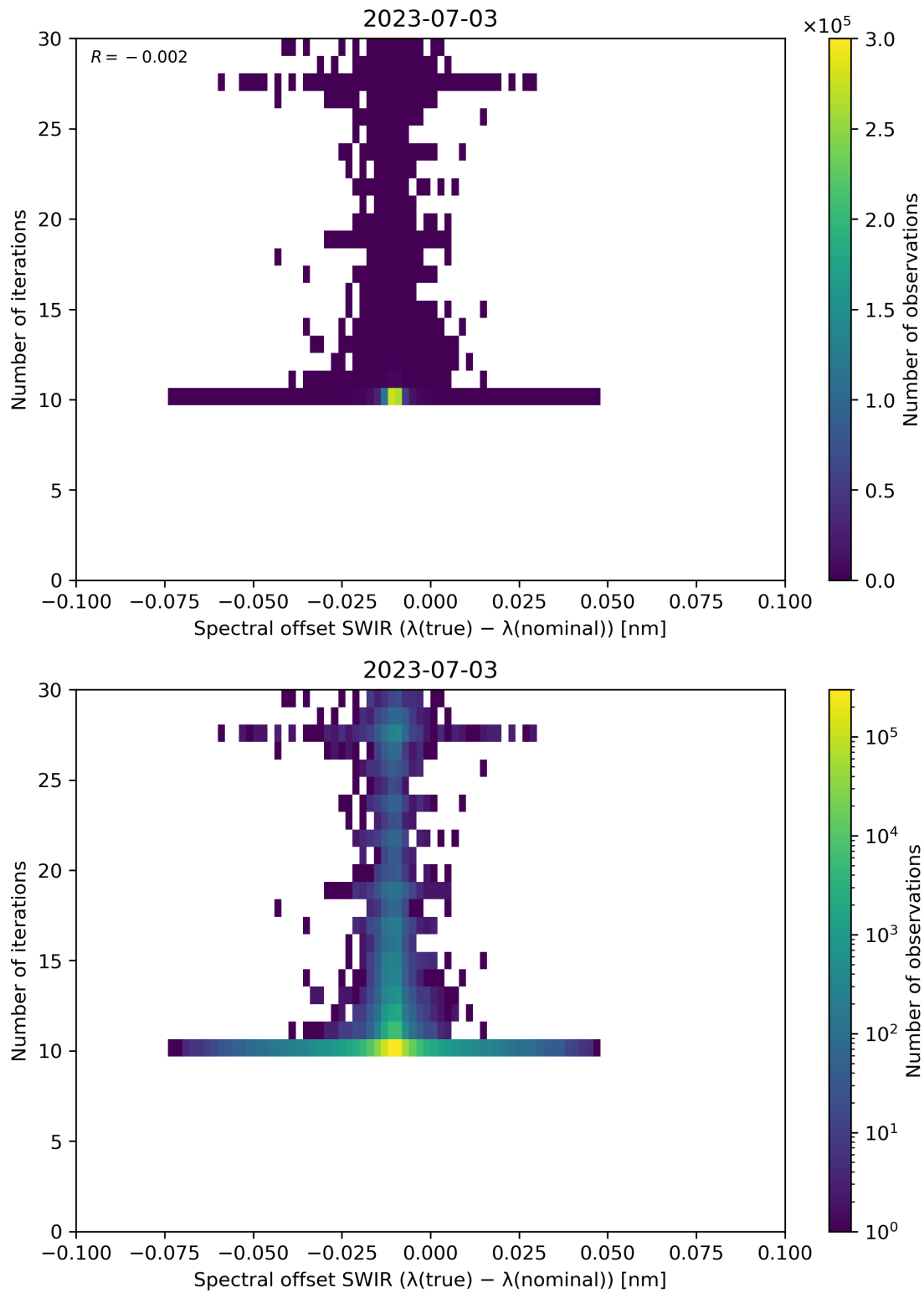
Figure 121: Scatter density plot of “Spectral offset SWIR ( \lambda(\text{true}) - \lambda(\text{nominal}) )” against “Number of iterations” for 2023-07-03 to 2023-07-04.
