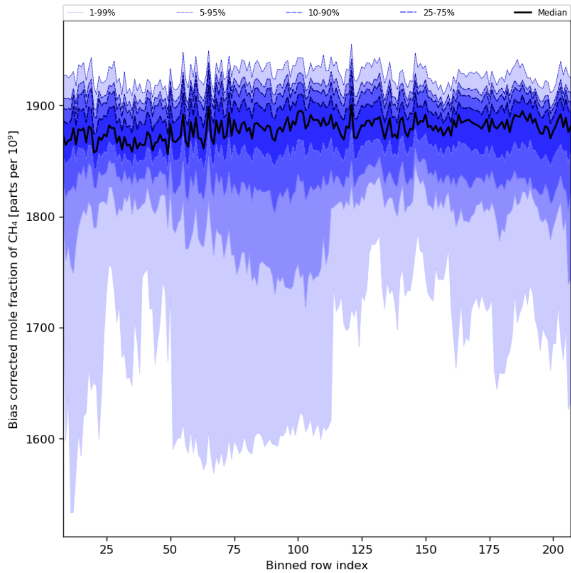
Figure 36: Along track statistics of “Bias corrected mole fraction of CH 4 ” for 2023-07-03 to 2023-07-04
