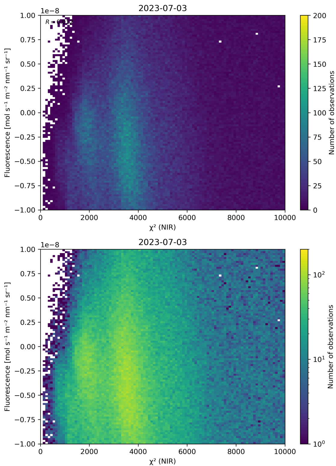
Figure 45: Scatter density plot of “ \chi^2 (NIR)” against “Fluorescence” for 2023-07-03 to 2023-07-04.
