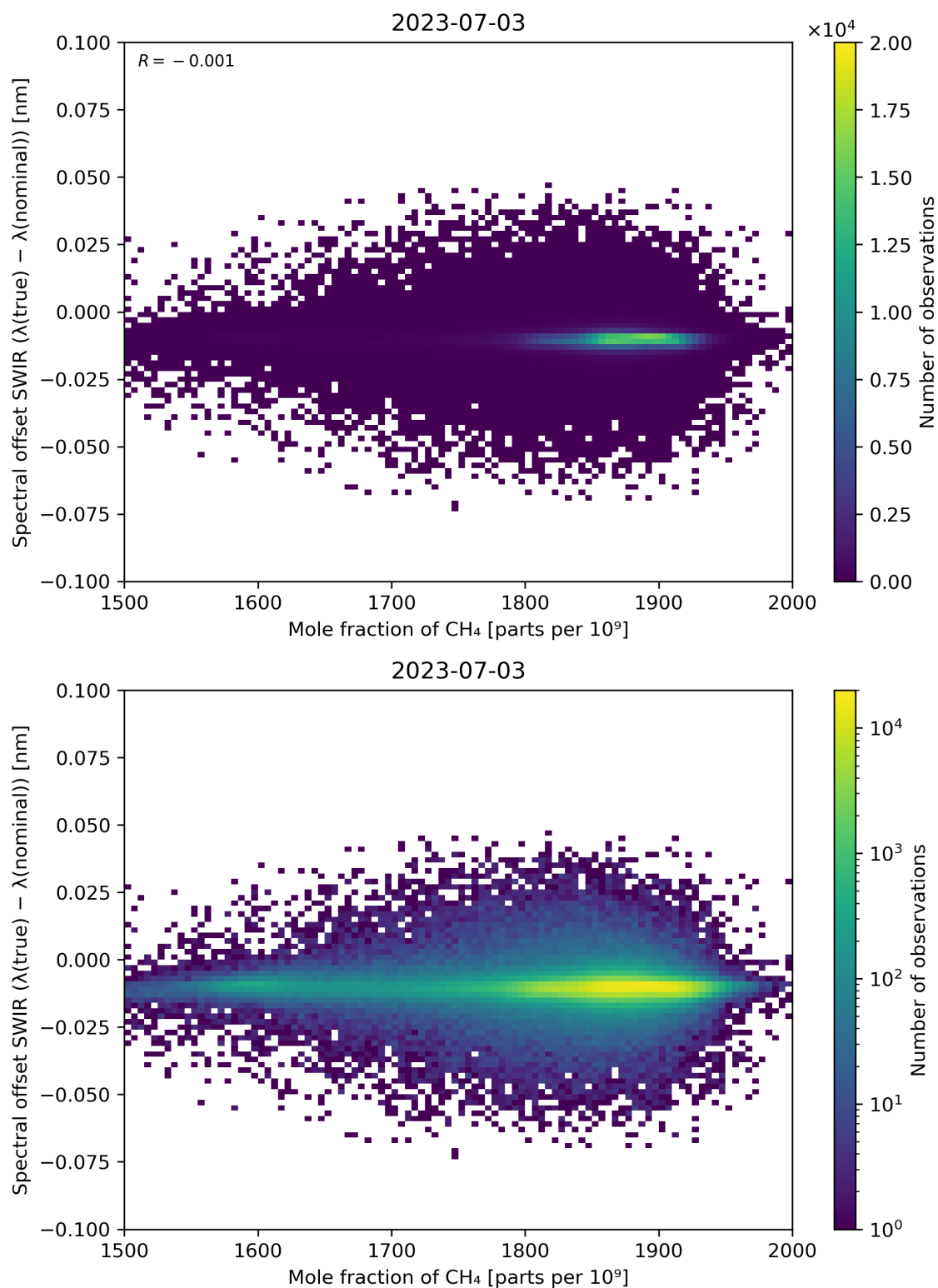
Figure 86: Scatter density plot of “Mole fraction of CH 4 ” against “Spectral offset SWIR ( \lambda(\text{true}) - \lambda(\text{nominal}) )” for 2023-07-03 to 2023-07-04.
