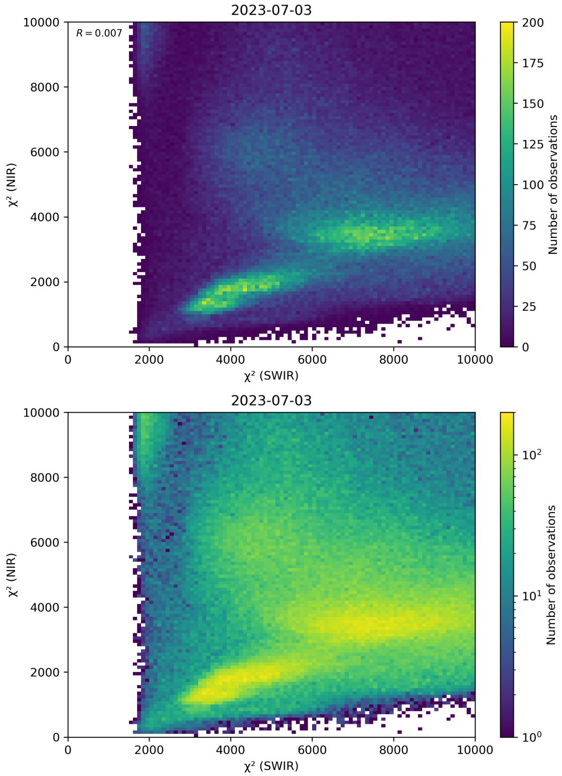
Figure 47: Scatter density plot of “ \chi^2 (SWIR)” against “ \chi^2 (NIR)” for 2023-07-03 to 2023-07-04.
