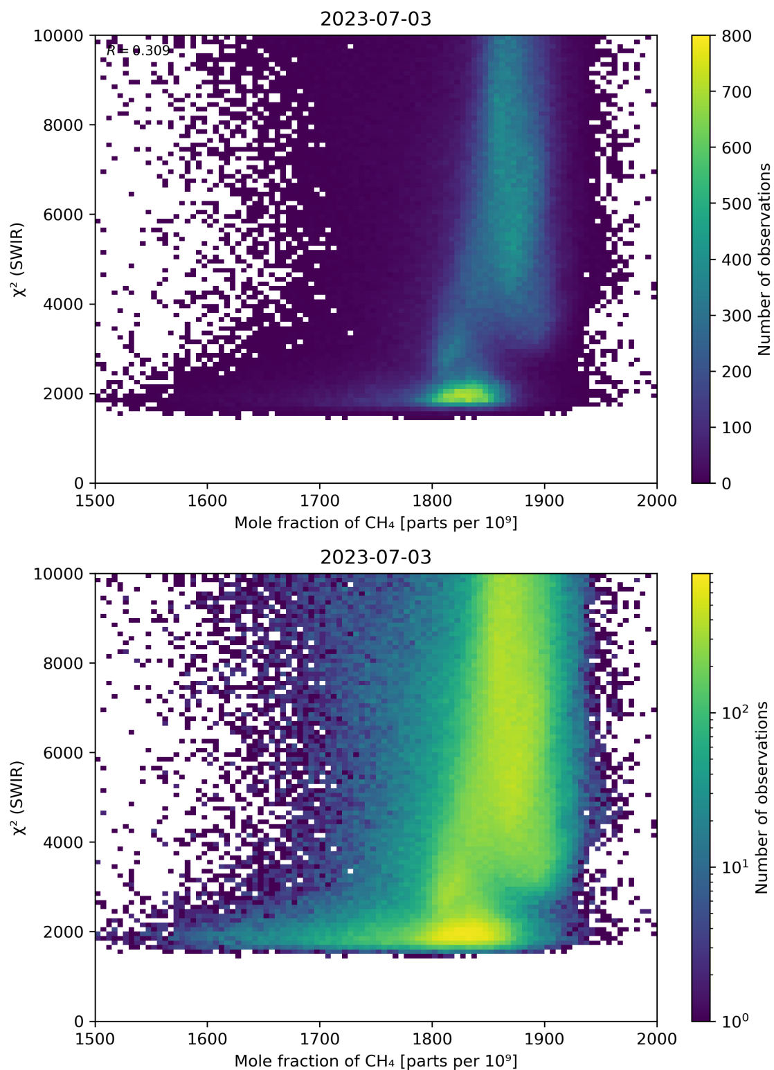
Figure 71: Scatter density plot of “Mole fraction of \text{CH}_4 ” against “ \chi^2 (SWIR)” for 2023-07-03 to 2023-07-04.
