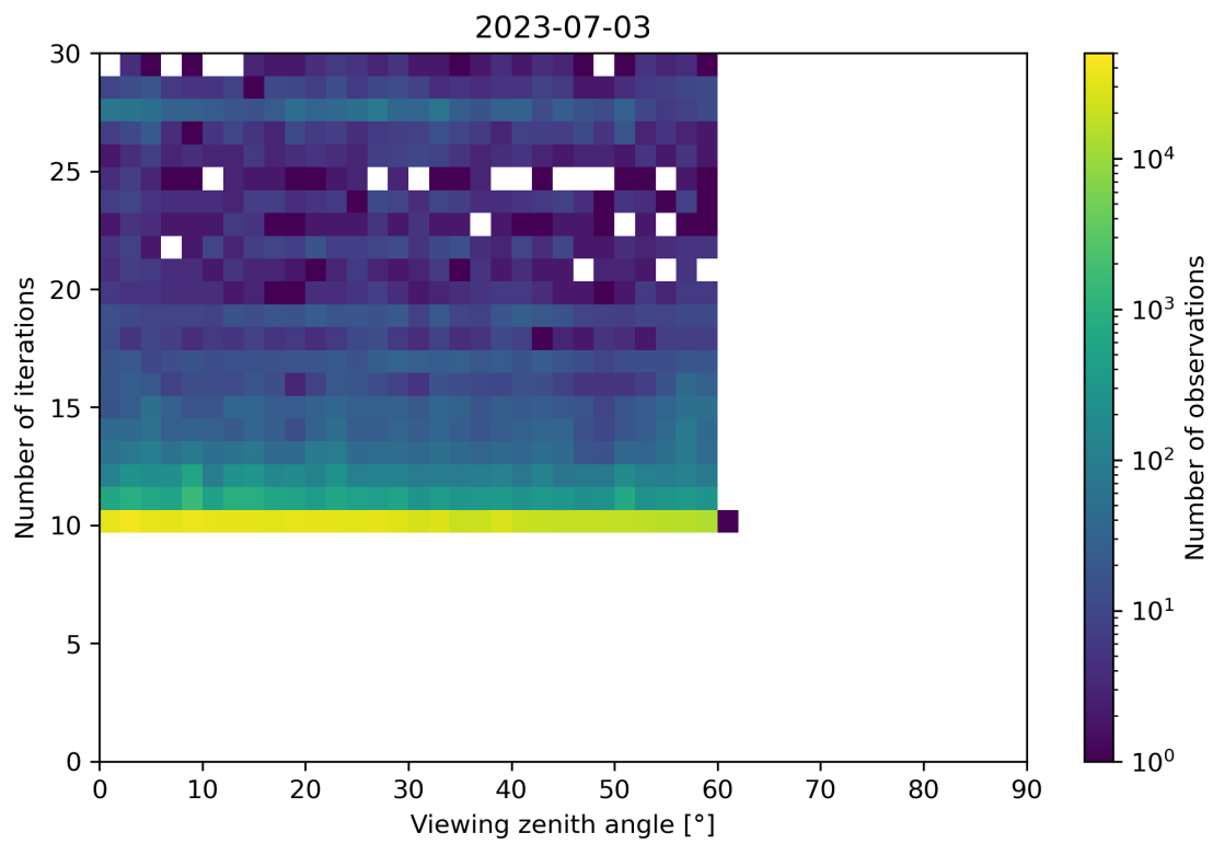
Figure 113: Scatter density plot of “Viewing zenith angle” against “Number of iterations” for 2023-07-03 to 2023-07-04.
