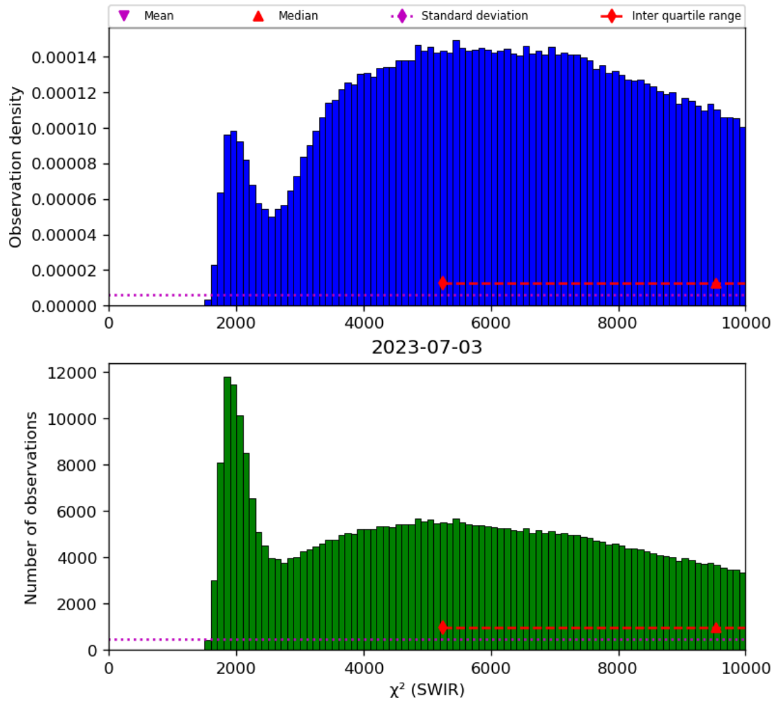
Figure 28: Histogram of “ \chi^2 (SWIR)” for 2023-07-03 to 2023-07-04
