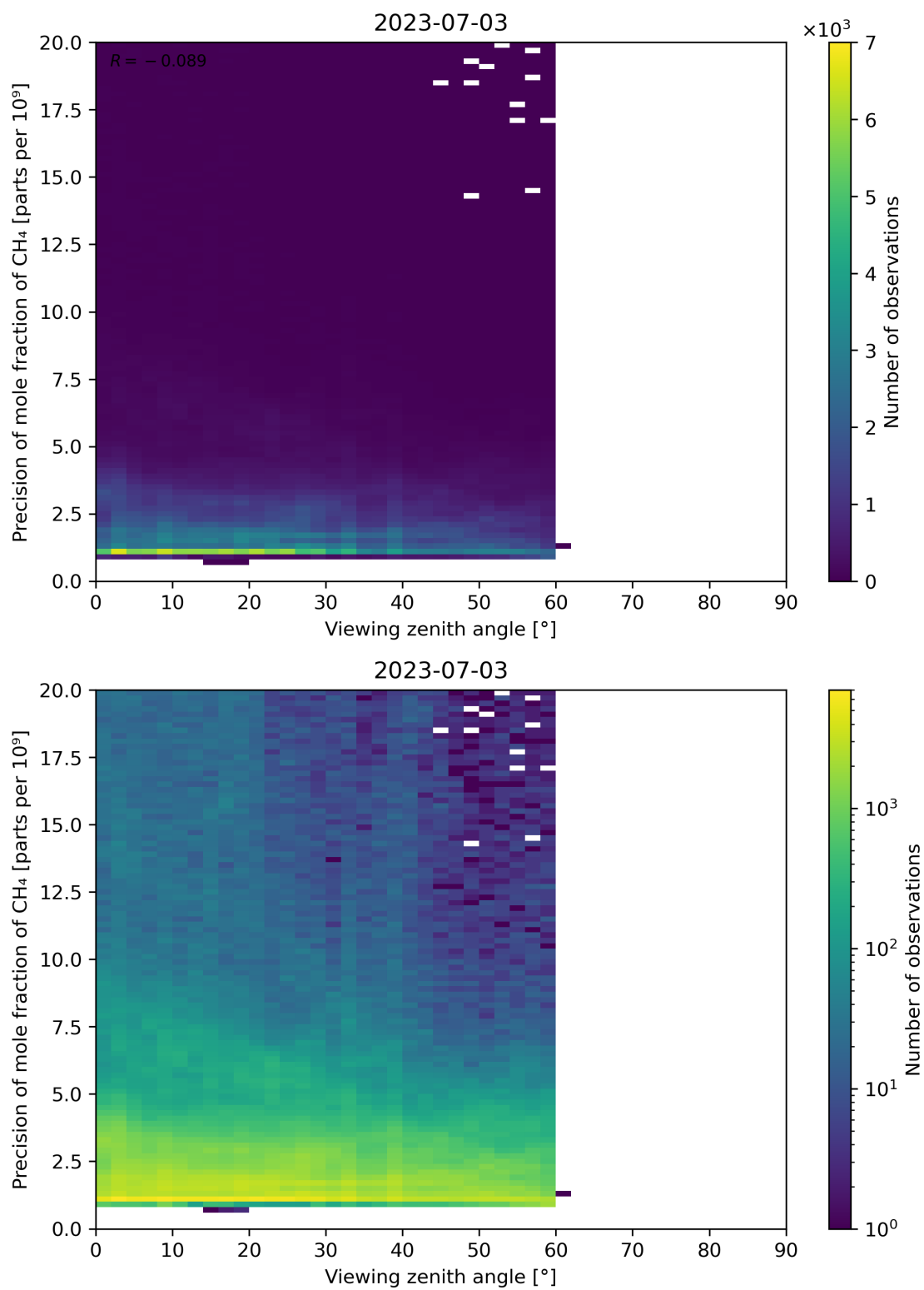
Figure 112: Scatter density plot of “Viewing zenith angle” against “Precision of mole fraction of CH 4 ” for 2023-07-03 to 2023-07-04.
