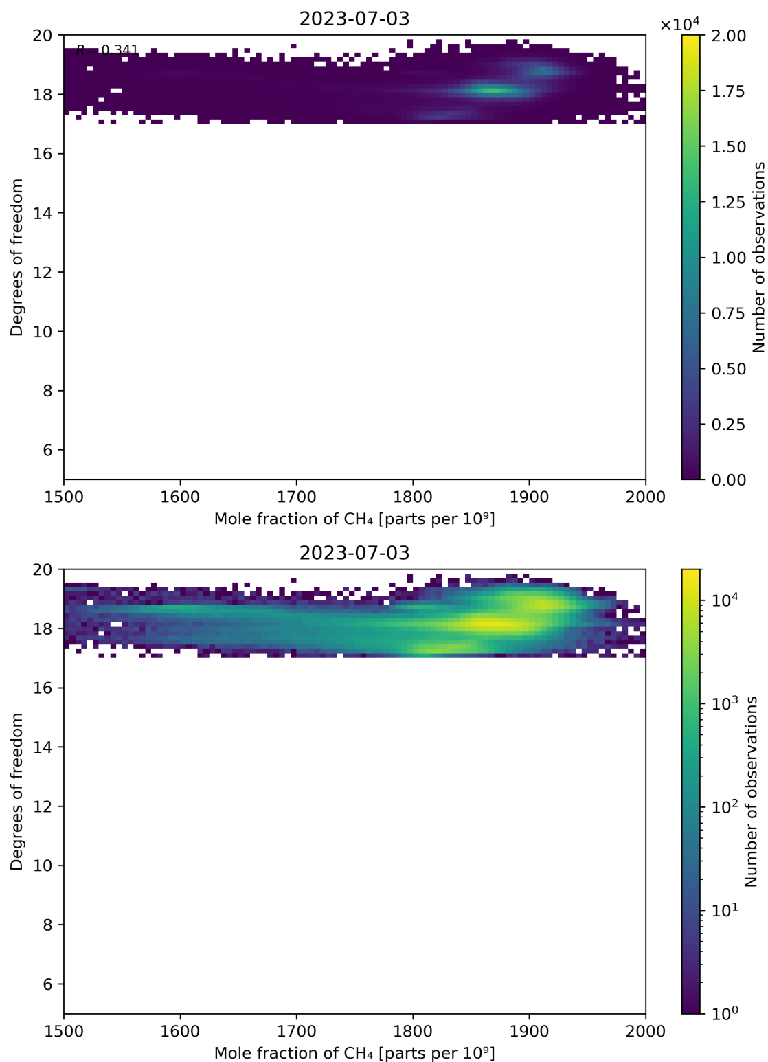
Figure 72: Scatter density plot of “Mole fraction of CH 4 ” against “Degrees of freedom” for 2023-07-03 to 2023-07-04.
