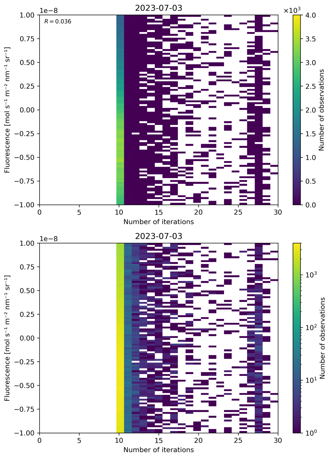
Figure 87: Scatter density plot of “Number of iterations” against “Fluorescence” for 2023-07-03 to 2023-07-04.
