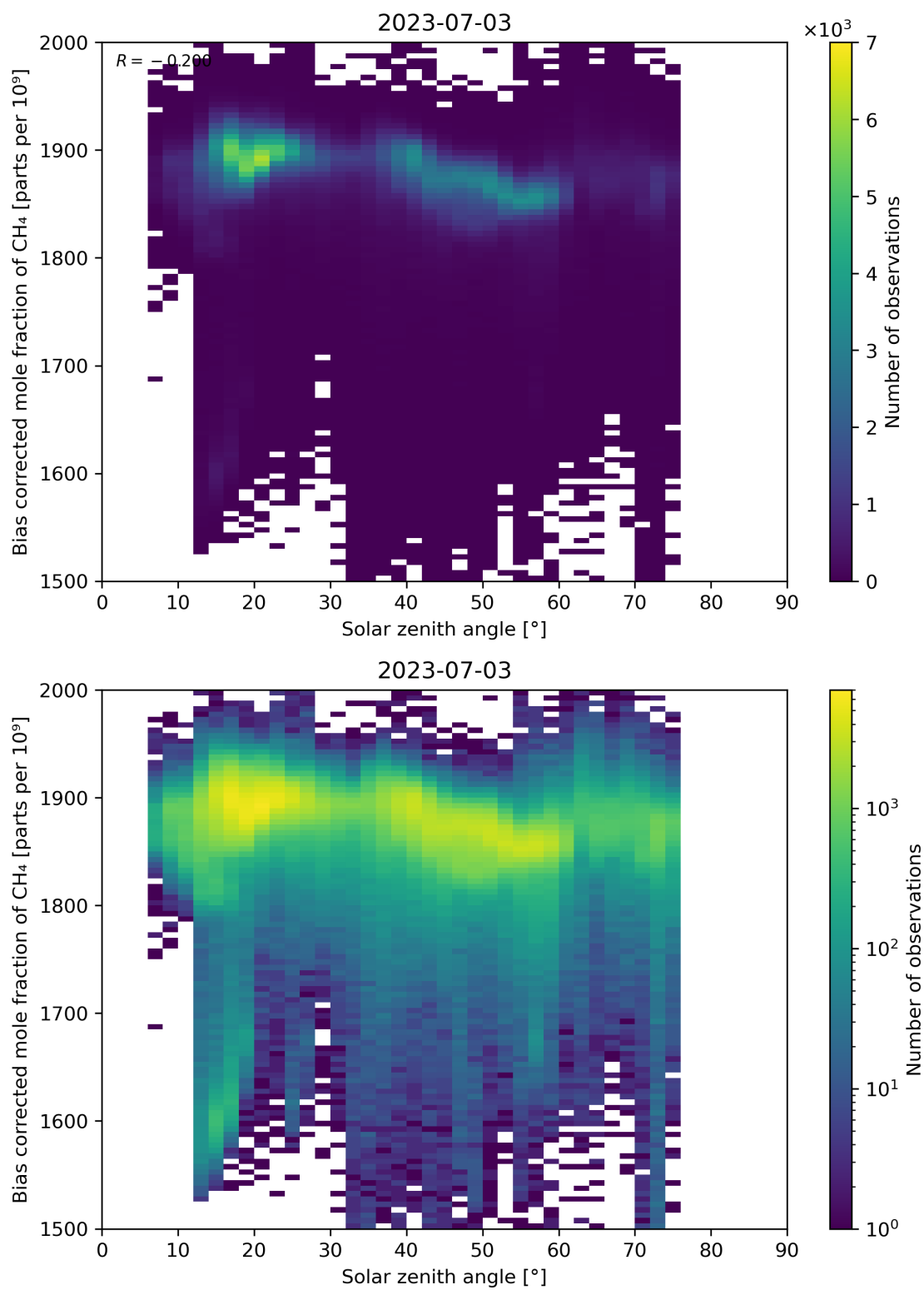
Figure 100: Scatter density plot of “Solar zenith angle” against “Bias corrected mole fraction of CH 4 ” for 2023-07-03 to 2023-07-04.
