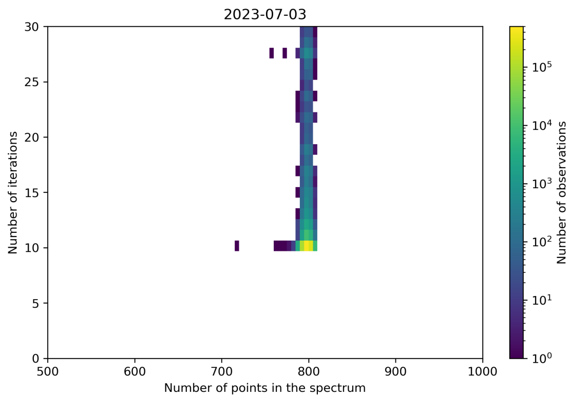
Figure 92: Scatter density plot of “Number of points in the spectrum” against “Number of iterations” for 2023-07-03 to 2023-07-04.
