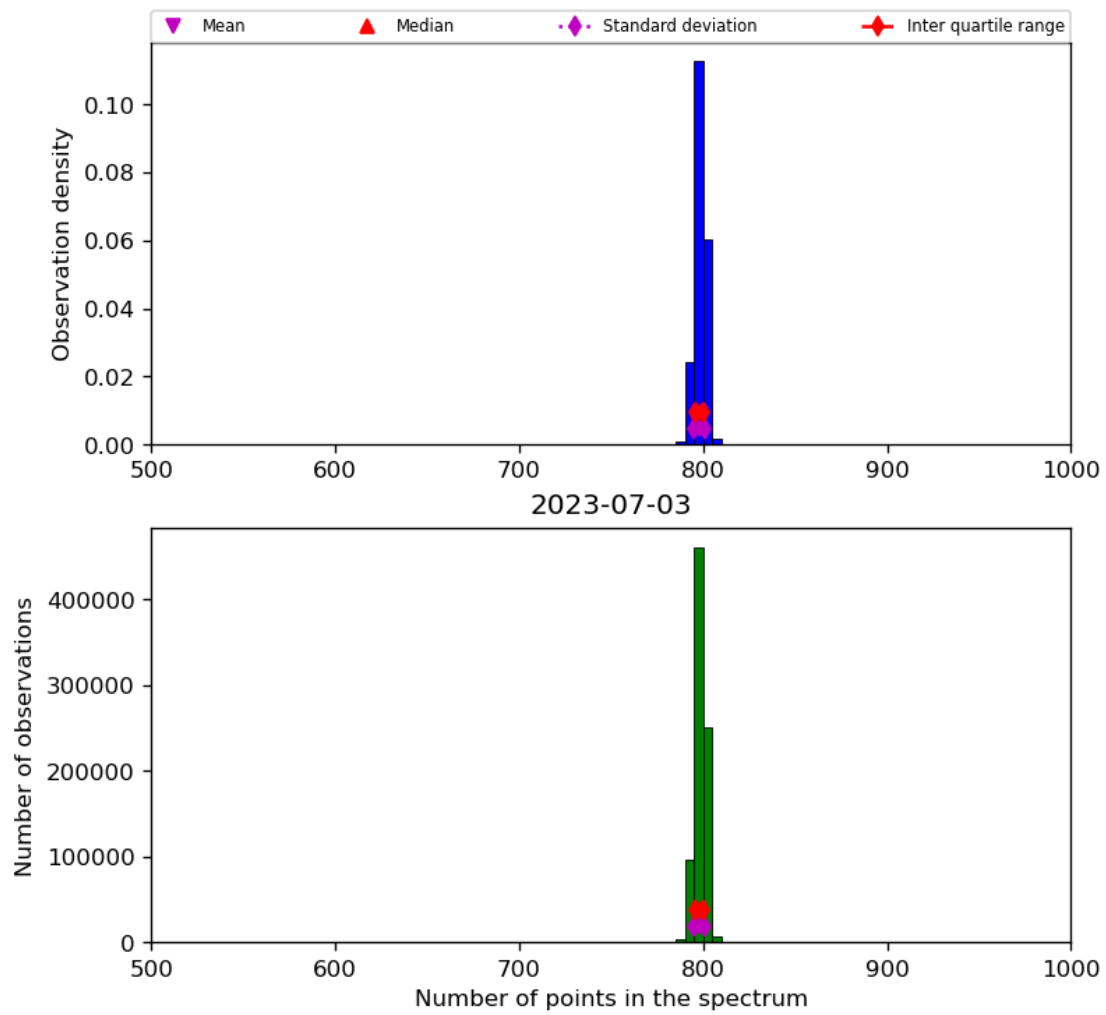
Figure 26: Histogram of “Number of points in the spectrum” for 2023-07-03 to 2023-07-04
