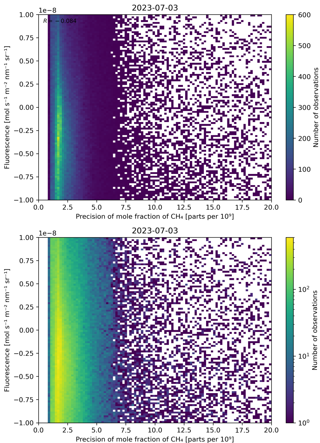
Figure 81: Scatter density plot of “Precision of mole fraction of CH 4 ” against “Fluorescence” for 2023-07-03 to 2023-07-04.
