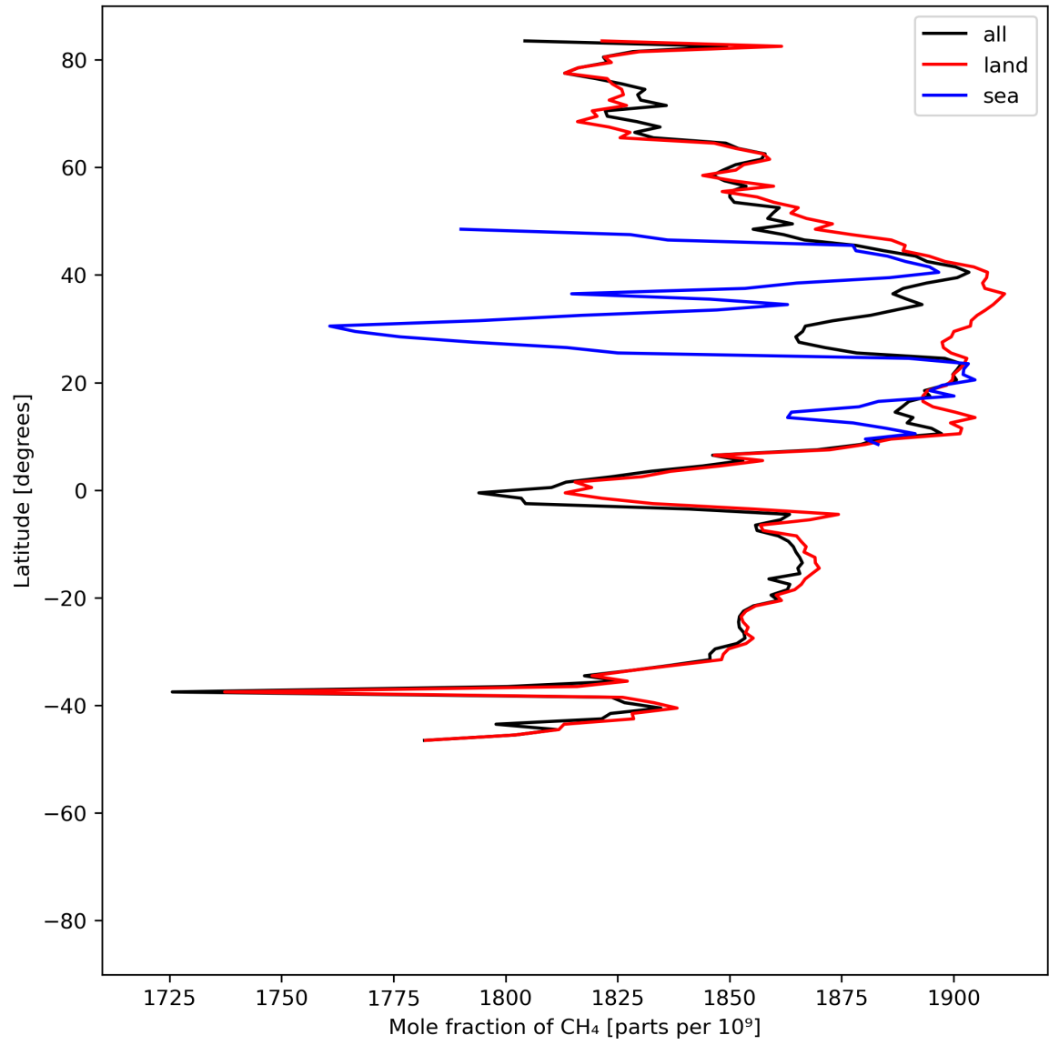
Figure 12: Zonal average of “Mole fraction of \text{CH}_4 ” for 2023-07-03 to 2023-07-04.
