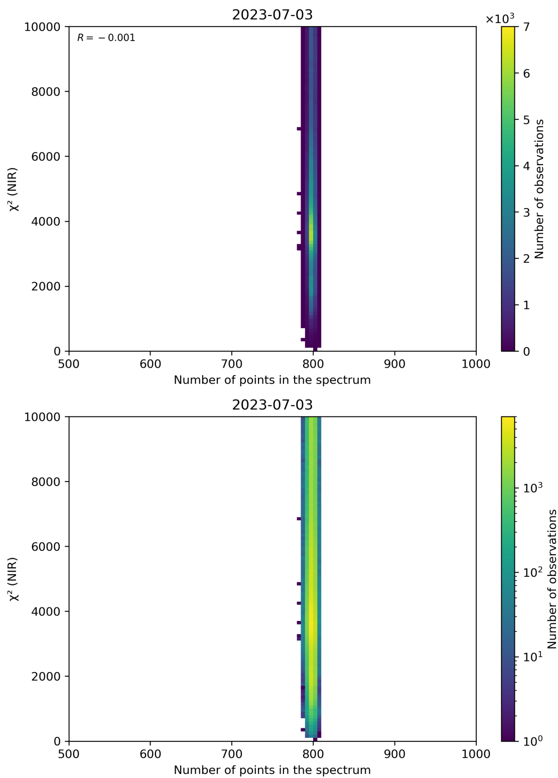
Figure 88: Scatter density plot of “Number of points in the spectrum” against “ \chi^2 (NIR)” for 2023-07-03 to 2023-07-04.
