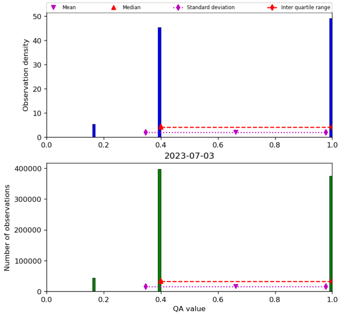
Figure 22: Histogram of “QA value” for 2023-07-03 to 2023-07-04
