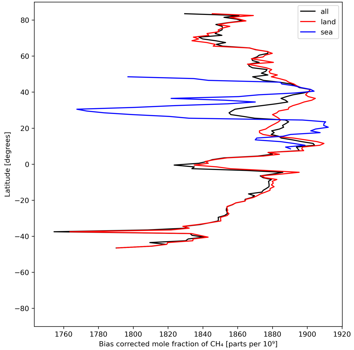
Figure 14: Zonal average of “Bias corrected mole fraction of CH 4 ” for 2023-07-03 to 2023-07-04.
