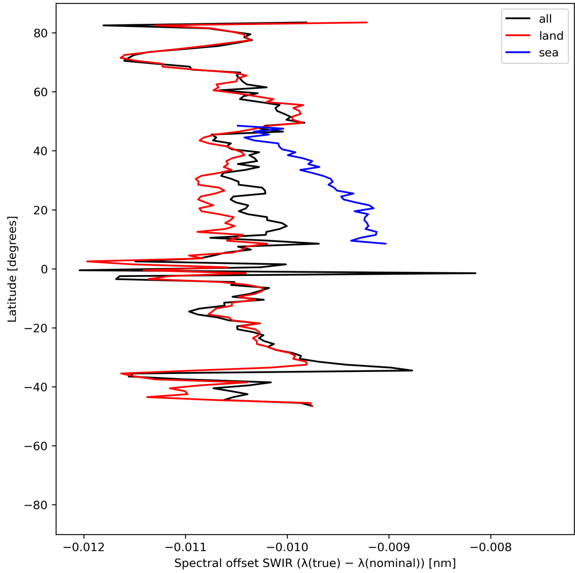
Figure 16: Zonal average of “Spectral offset SWIR ( \lambda(\text{true}) - \lambda(\text{nominal}) )” for 2023-07-03 to 2023-07-04.
