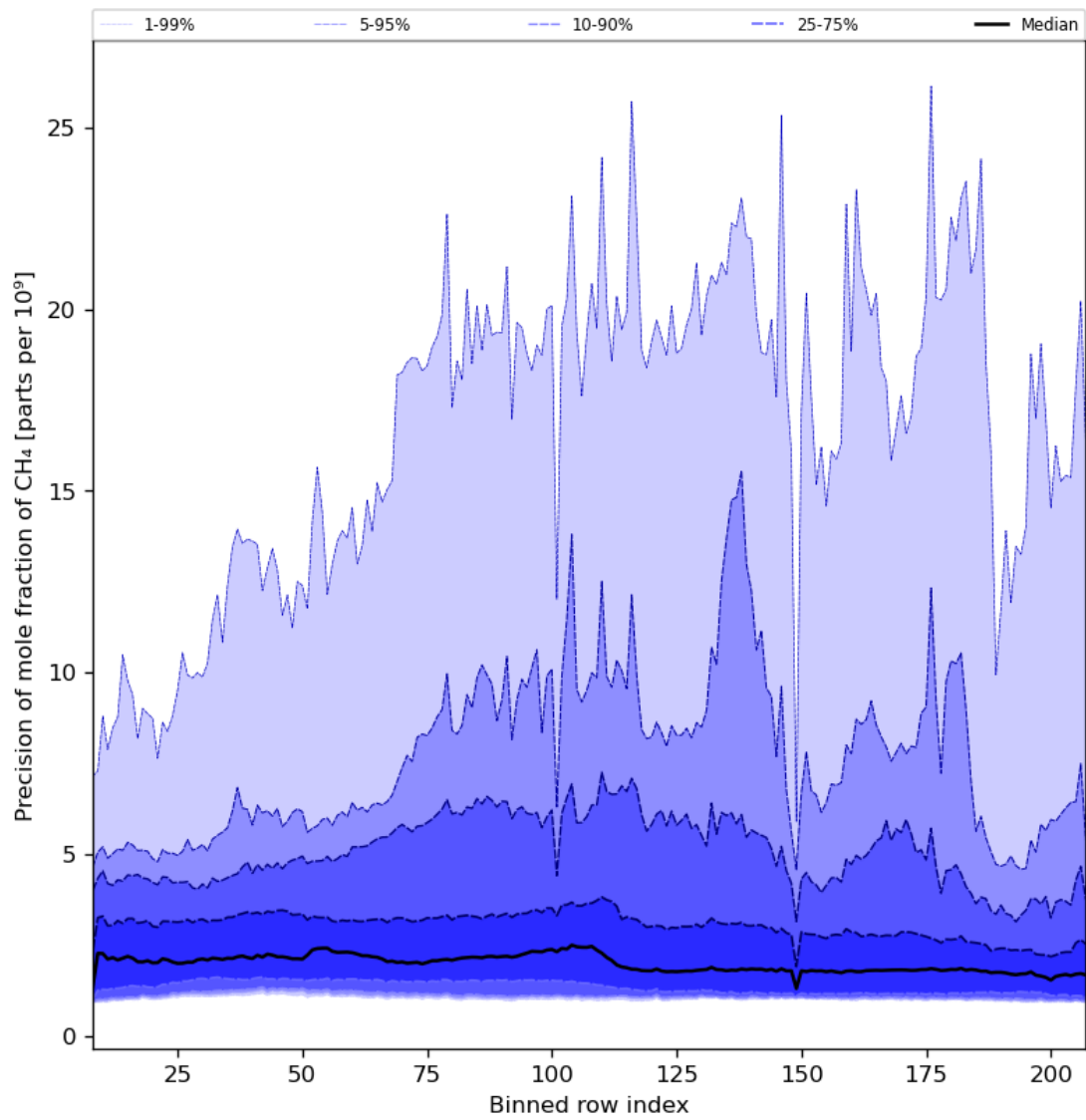
Figure 35: Along track statistics of "Precision of mole fraction of CH 4 " for 2023-07-03 to 2023-07-04
