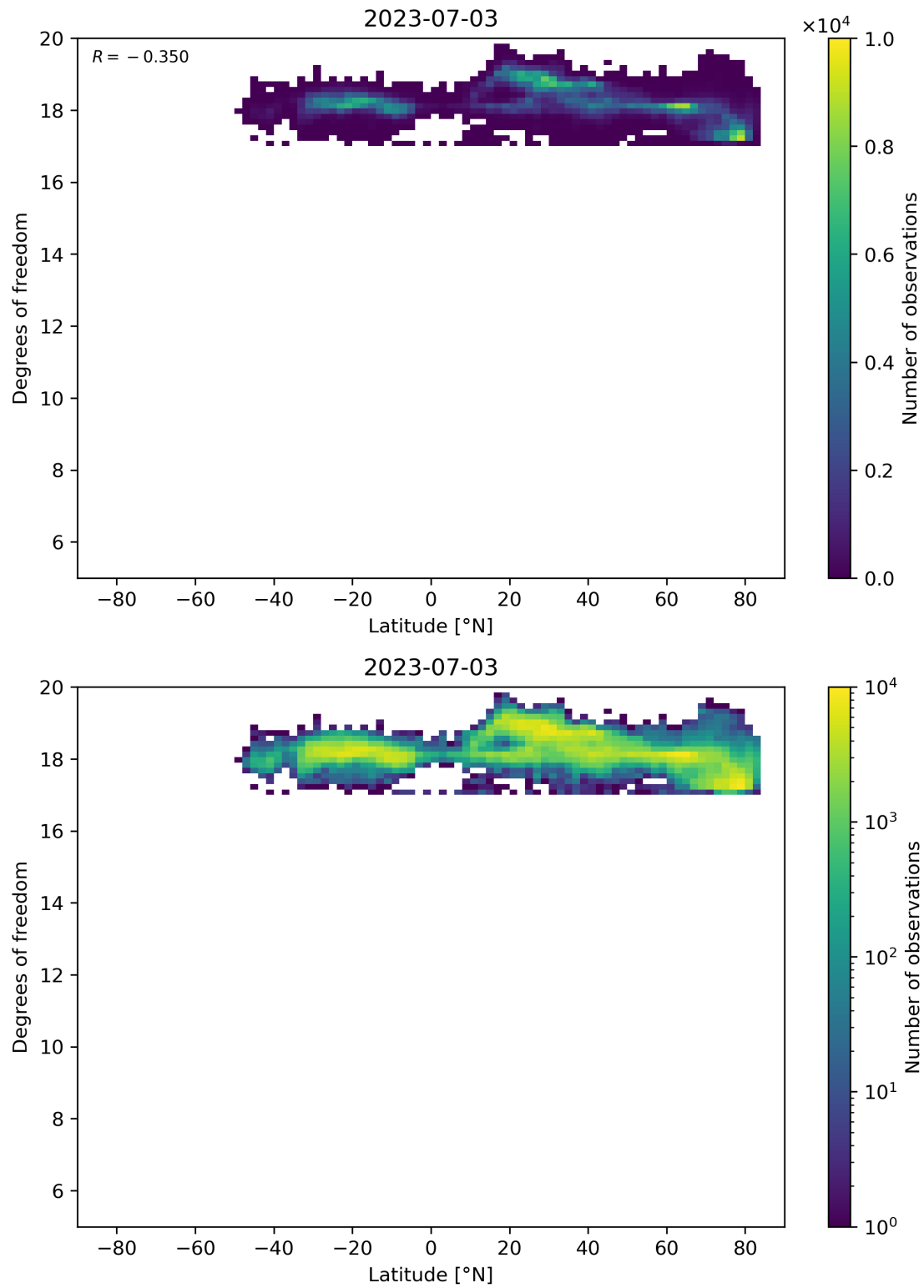
Figure 55: Scatter density plot of “Latitude” against “Degrees of freedom” for 2023-07-03 to 2023-07-04.
