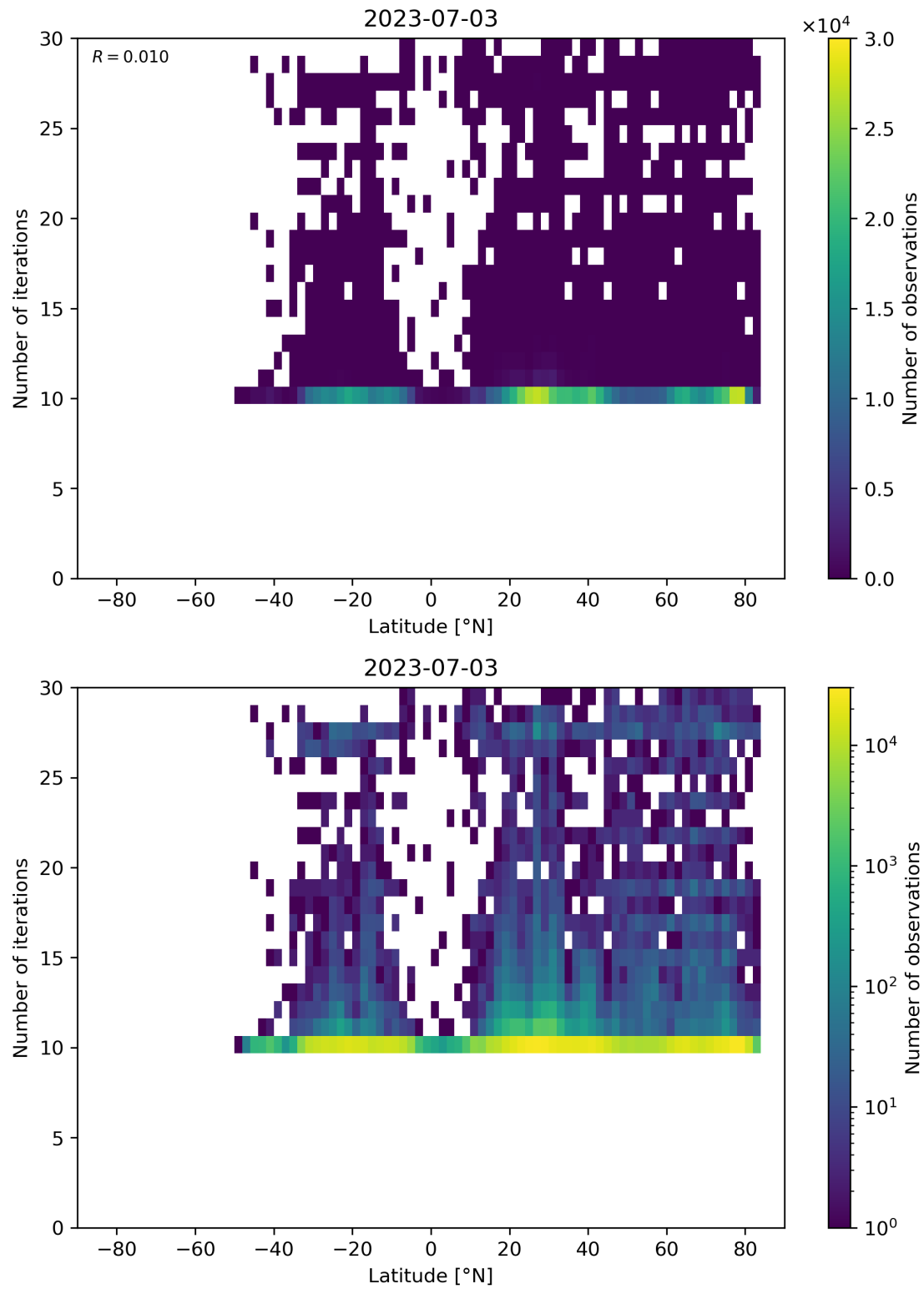
Figure 60: Scatter density plot of “Latitude” against “Number of iterations” for 2023-07-03 to 2023-07-04.
