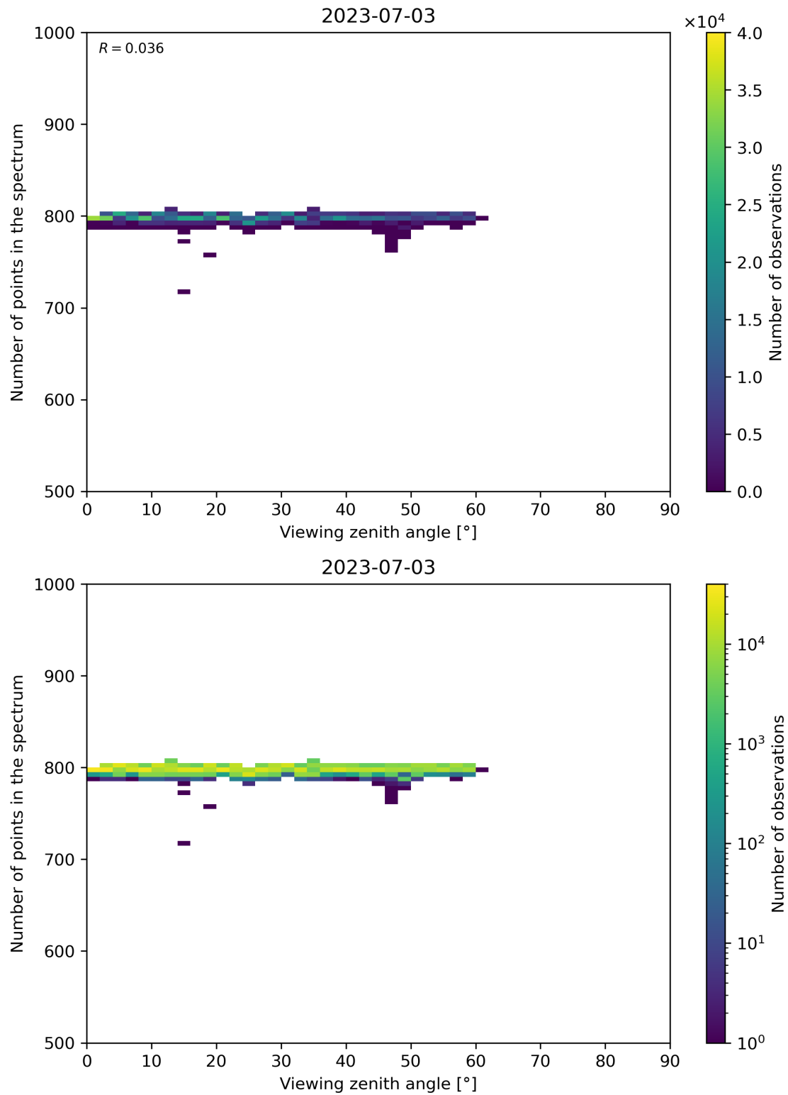
Figure 114: Scatter density plot of “Viewing zenith angle” against “Number of points in the spectrum” for 2023-07-03 to 2023-07-04.
