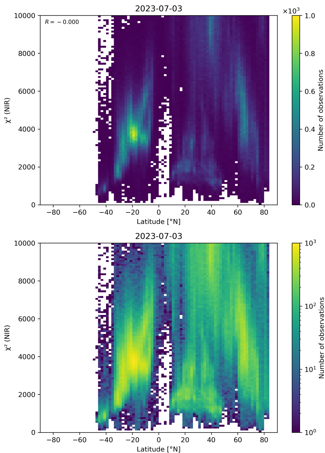
Figure 53: Scatter density plot of “Latitude” against “ \chi^2 (NIR)” for 2023-07-03 to 2023-07-04.
