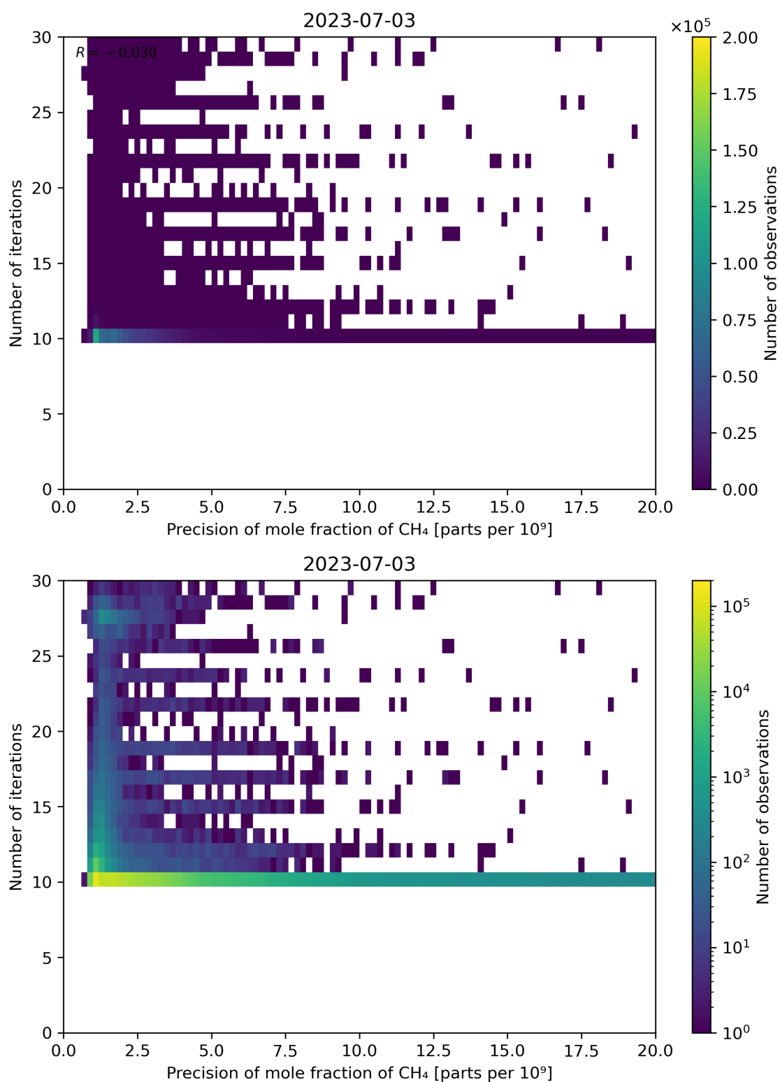
Figure 83: Scatter density plot of “Precision of mole fraction of CH 4 ” against “Number of iterations” for 2023-07-03 to 2023-07-04.
