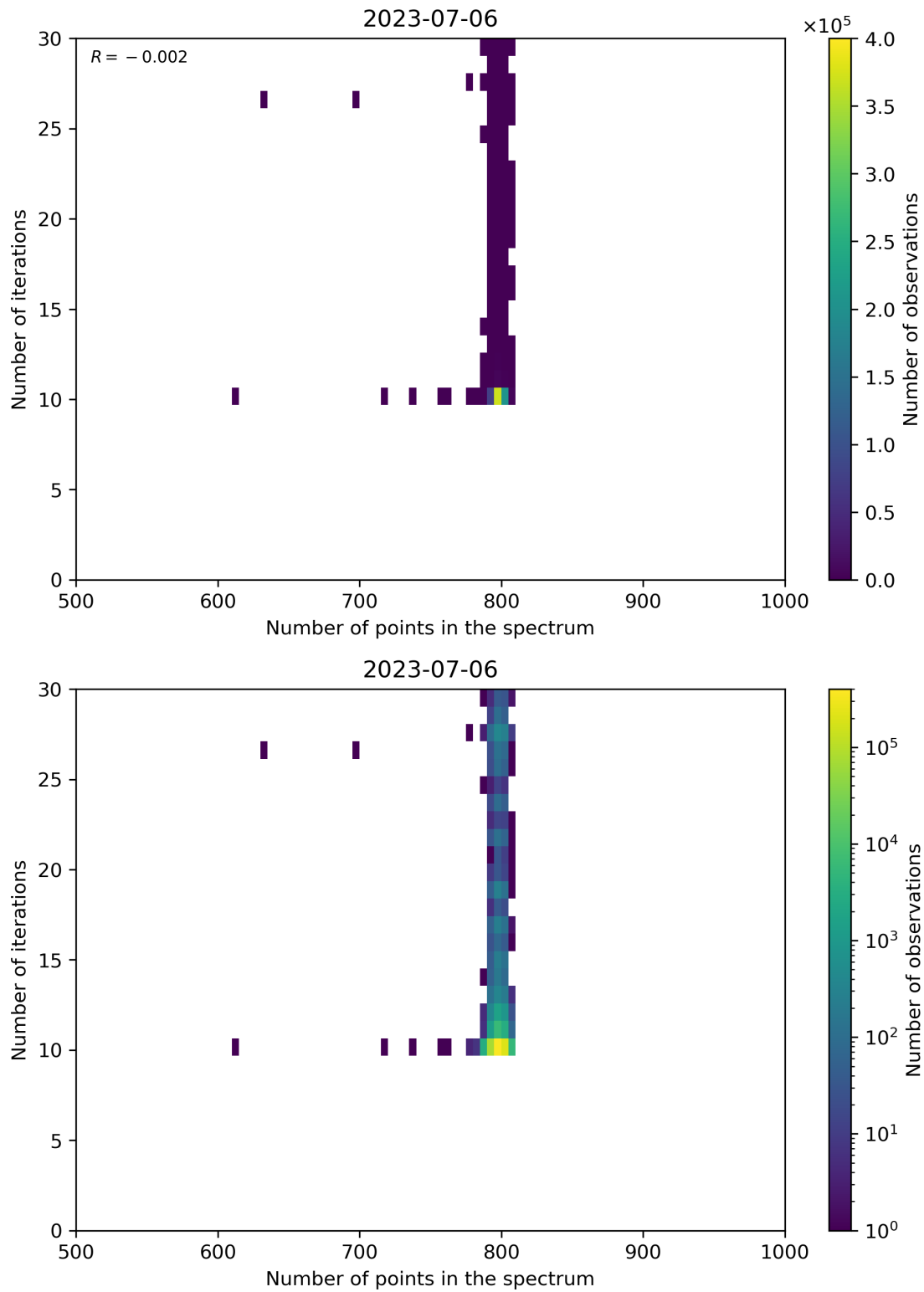
Figure 92: Scatter density plot of “Number of points in the spectrum” against “Number of iterations” for 2023-07-05 to 2023-07-07.
