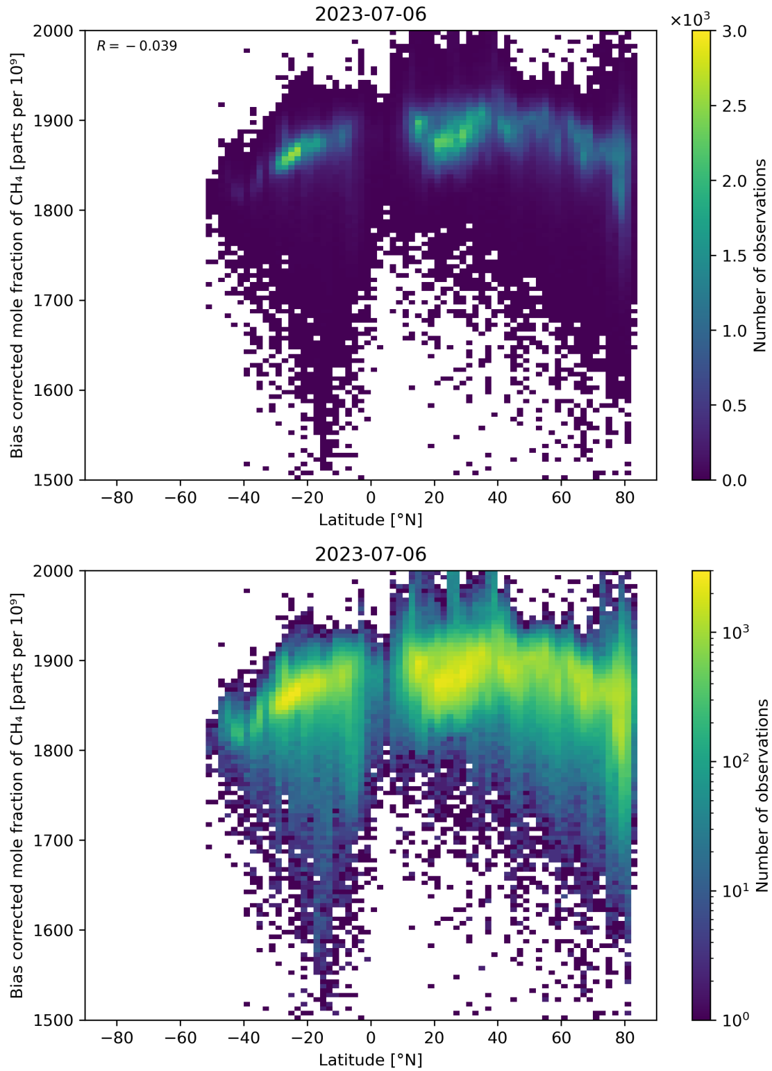
Figure 58: Scatter density plot of “Latitude” against “Bias corrected mole fraction of \text{CH}_4 ” for 2023-07-05 to 2023-07-07.
