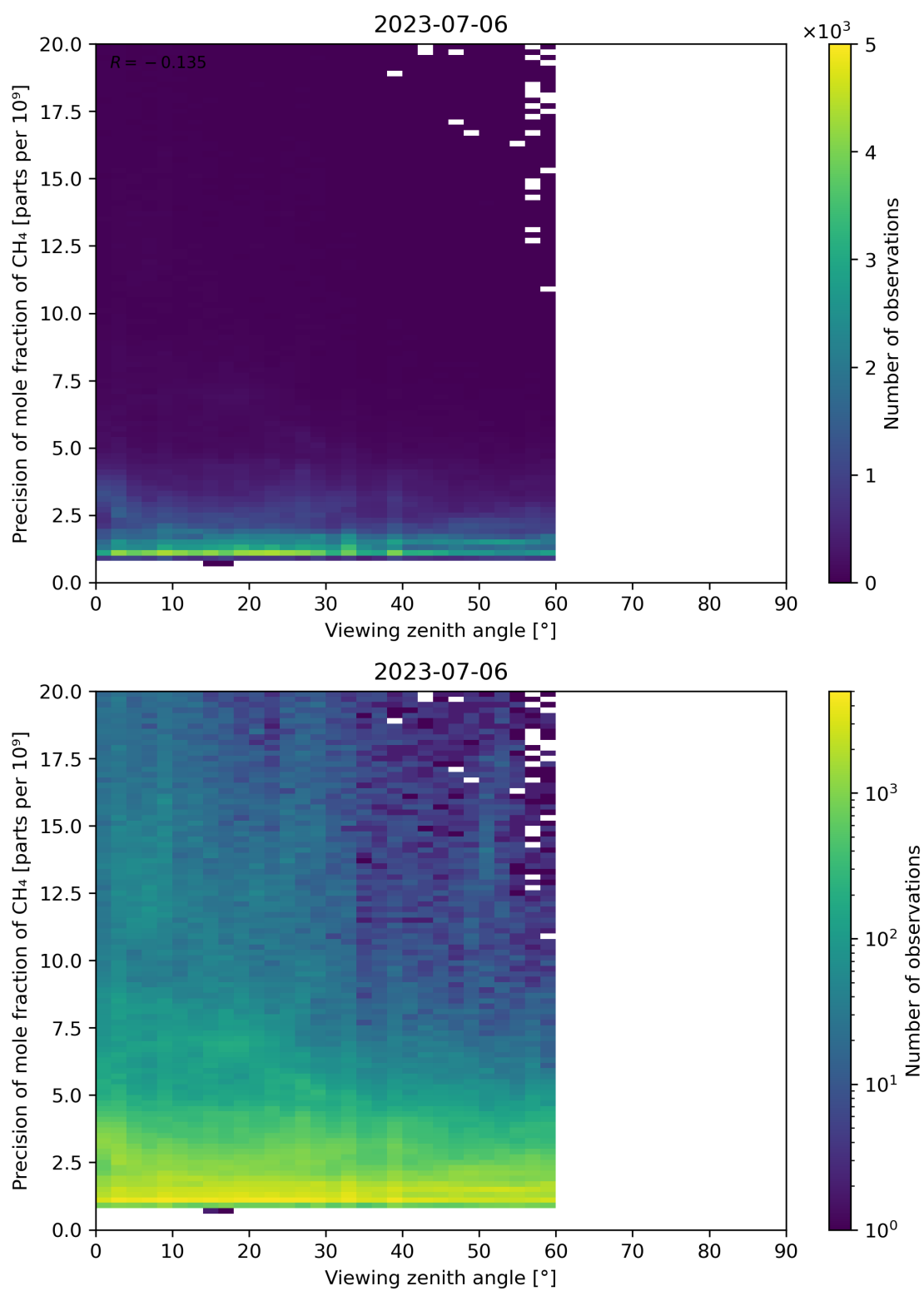
Figure 112: Scatter density plot of “Viewing zenith angle” against “Precision of mole fraction of CH 4 ” for 2023-07-05 to 2023-07-07.
