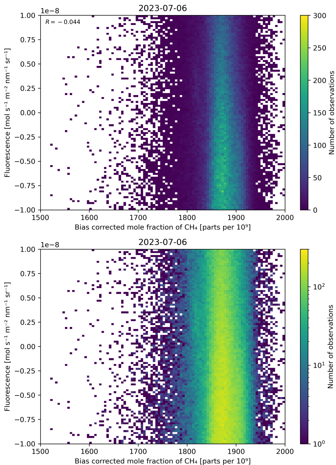
Figure 66: Scatter density plot of “Bias corrected mole fraction of \text{CH}_4 ” against “Fluorescence” for 2023-07-05 to 2023-07-07.
