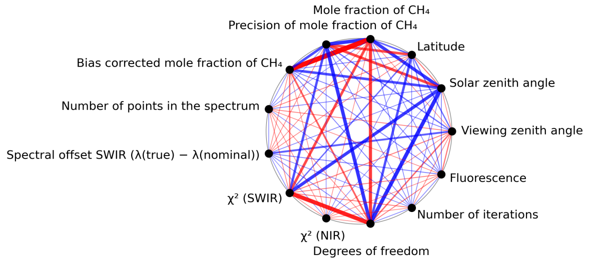
Figure 1: Map of correlation graph for 2023-07-05 to 2023-07-07.
