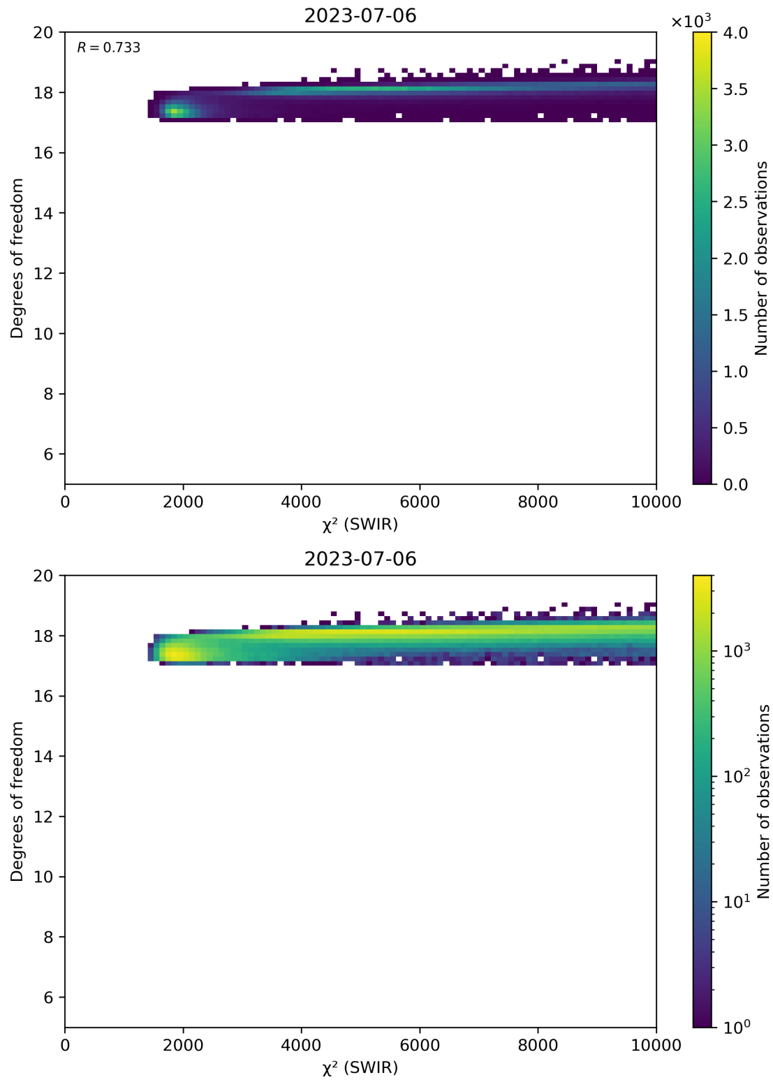
Figure 48: Scatter density plot of “ \chi^2 (SWIR)” against “Degrees of freedom” for 2023-07-05 to 2023-07-07.
