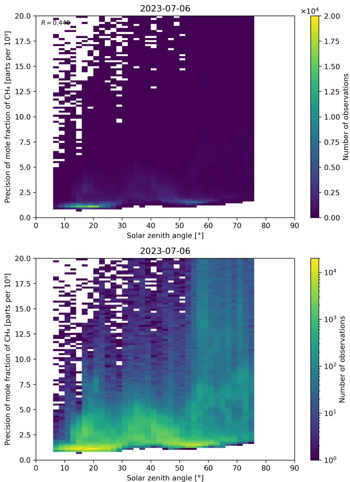
Figure 101: Scatter density plot of “Solar zenith angle” against “Precision of mole fraction of CH 4 ” for 2023-07-05 to 2023-07-07.
