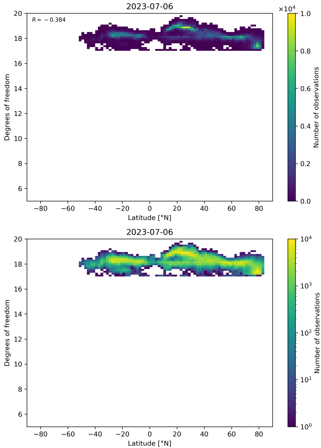
Figure 55: Scatter density plot of “Latitude” against “Degrees of freedom” for 2023-07-05 to 2023-07-07.
