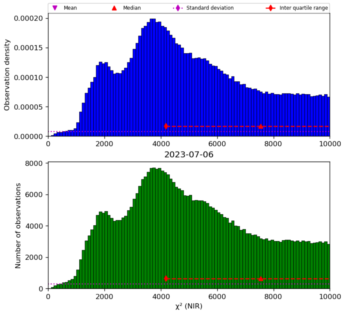
Figure 29: Histogram of " \chi^2 (NIR)" for 2023-07-05 to 2023-07-07
