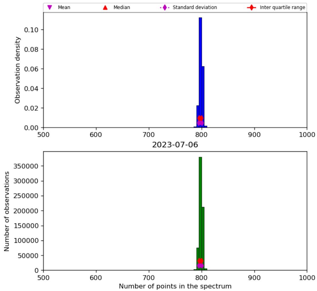
Figure 26: Histogram of “Number of points in the spectrum” for 2023-07-05 to 2023-07-07
