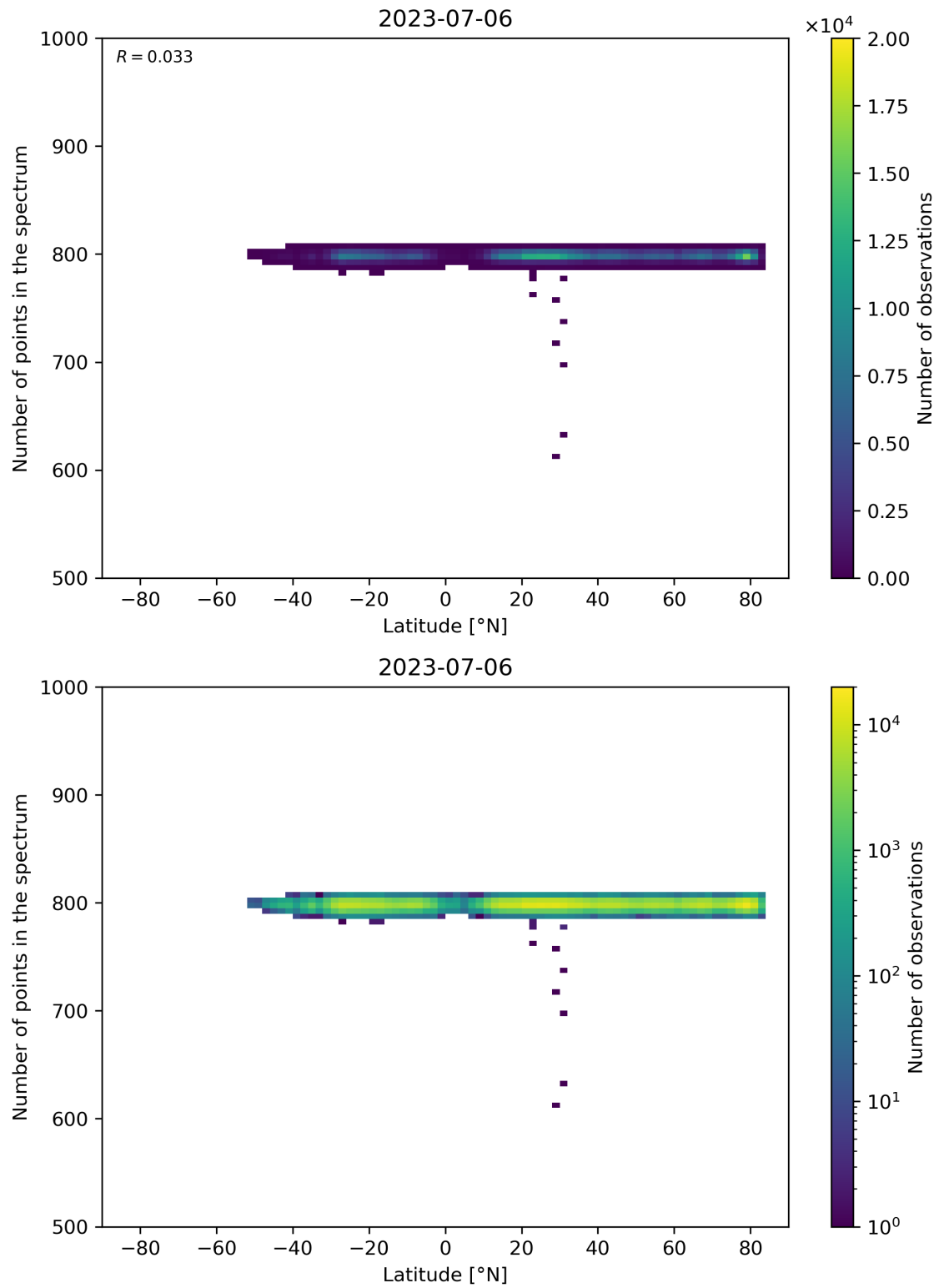
Figure 61: Scatter density plot of “Latitude” against “Number of points in the spectrum” for 2023-07-05 to 2023-07-07.
