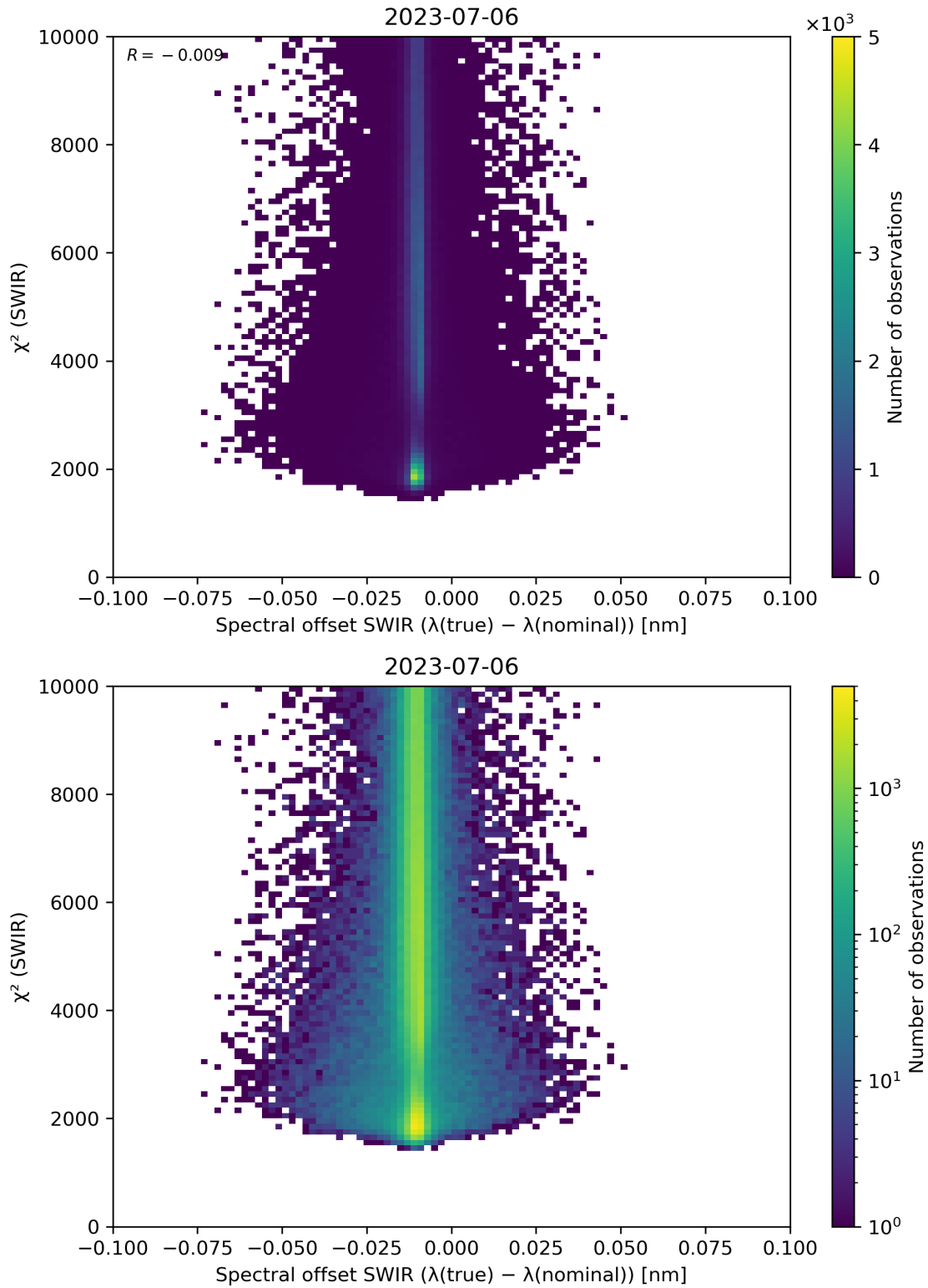
Figure 118: Scatter density plot of “Spectral offset SWIR ( \lambda(\text{true}) - \lambda(\text{nominal}) )” against “ \chi^2 (SWIR)” for 2023-07-05 to 2023-07-07.
