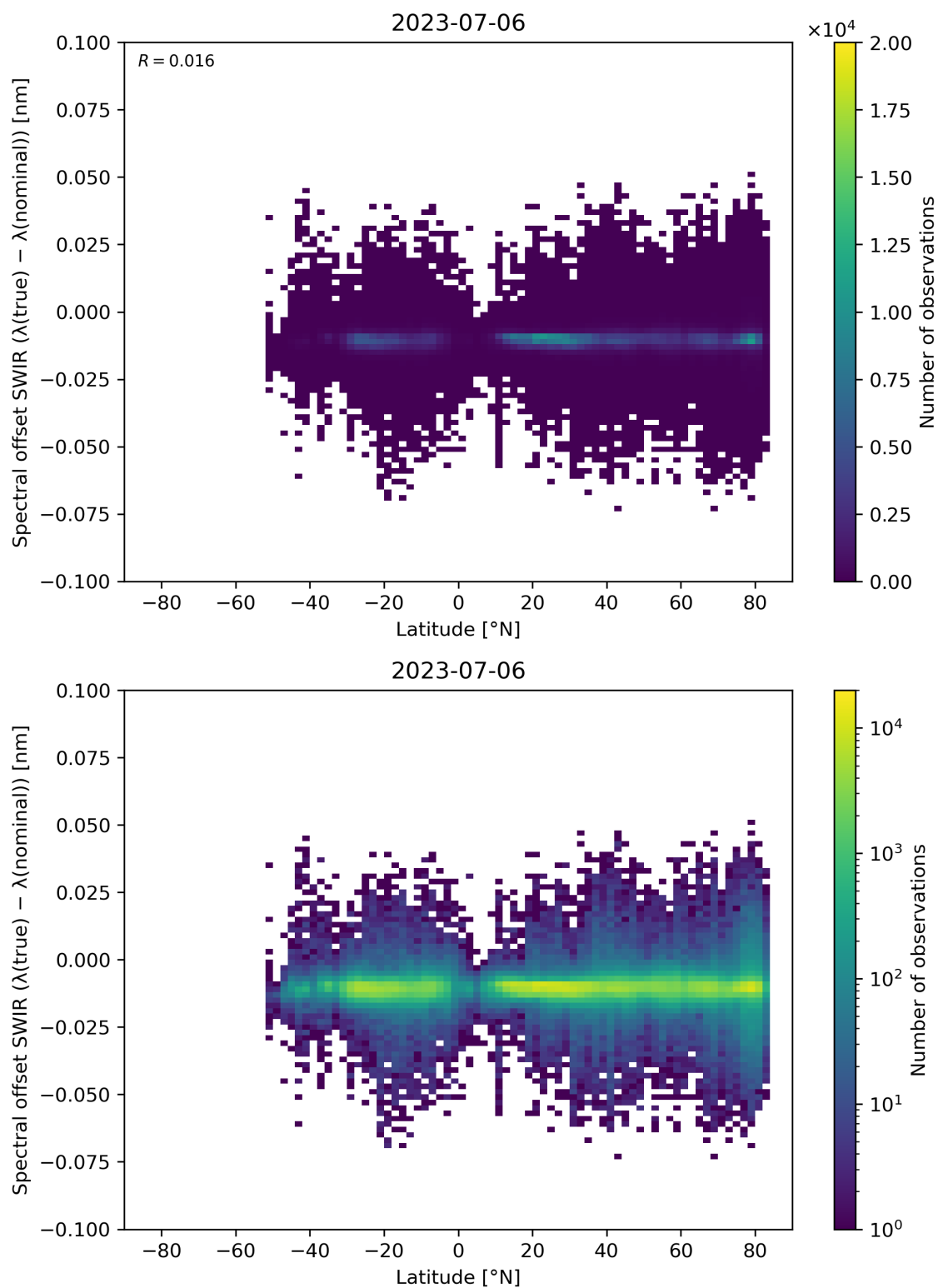
Figure 62: Scatter density plot of “Latitude” against “Spectral offset SWIR ( \lambda(\text{true}) - \lambda(\text{nominal}) )” for 2023-07-05 to 2023-07-07.
