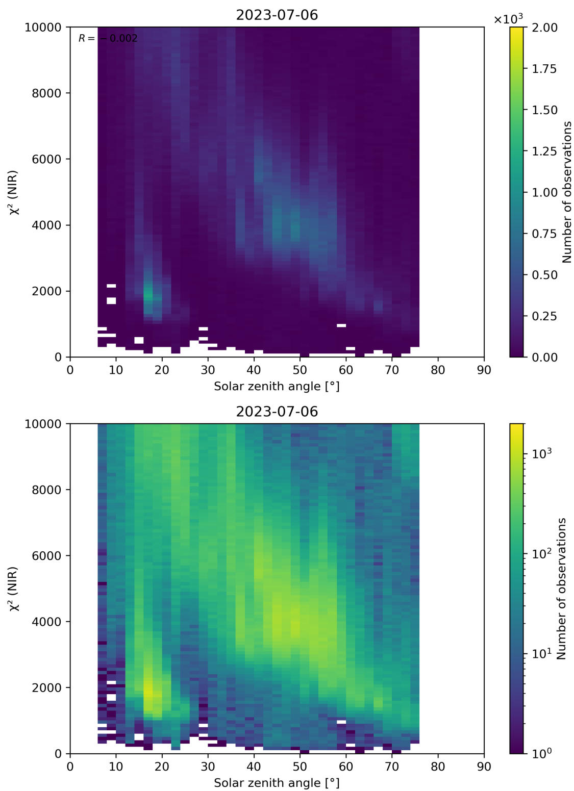
Figure 94: Scatter density plot of “Solar zenith angle” against “ \chi^2 (NIR)” for 2023-07-05 to 2023-07-07.
