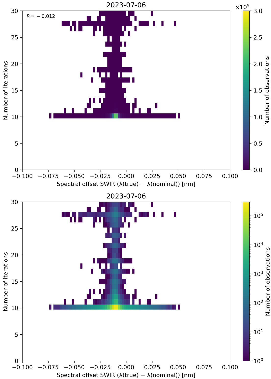
Figure 121: Scatter density plot of “Spectral offset SWIR ( \lambda(\text{true}) - \lambda(\text{nominal}) )” against “Number of iterations” for 2023-07-05 to 2023-07-07.
