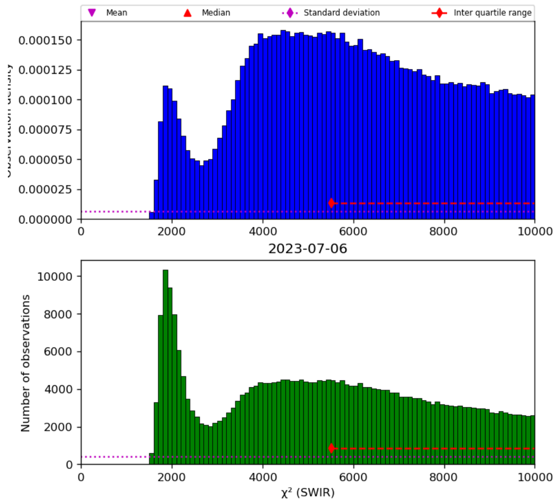
Figure 28: Histogram of “ \chi^2 (SWIR)” for 2023-07-05 to 2023-07-07
