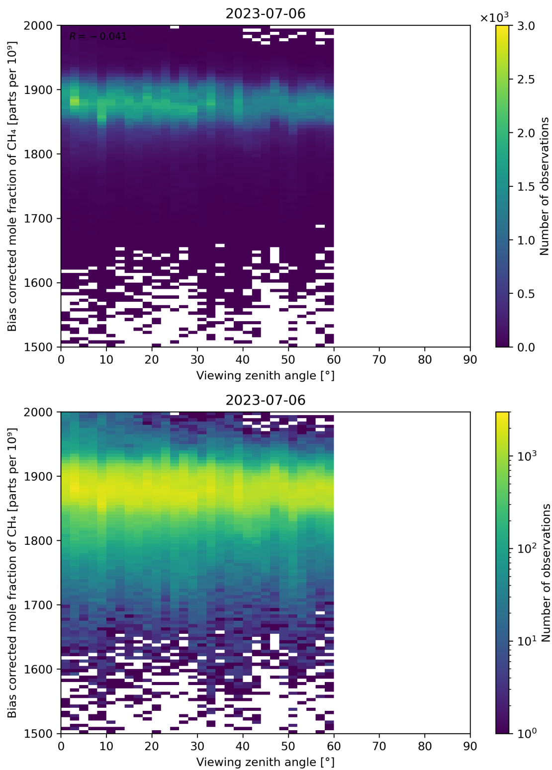
Figure 111: Scatter density plot of “Viewing zenith angle” against “Bias corrected mole fraction of CH 4 ” for 2023-07-05 to 2023-07-07.
