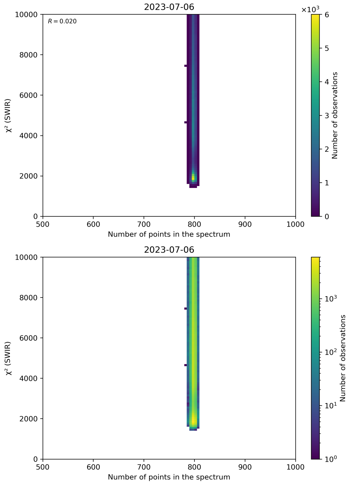
Figure 89: Scatter density plot of “Number of points in the spectrum” against “ \chi^2 (SWIR)” for 2023-07-05 to 2023-07-07.
