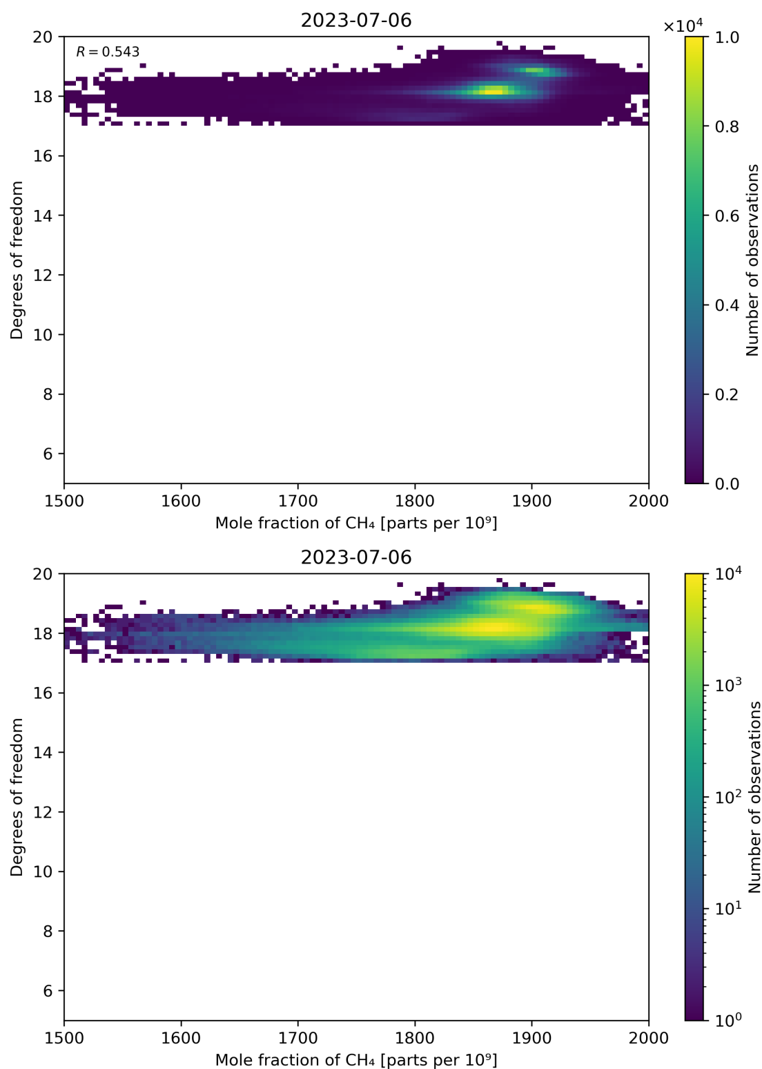
Figure 72: Scatter density plot of “Mole fraction of CH 4 ” against “Degrees of freedom” for 2023-07-05 to 2023-07-07.
