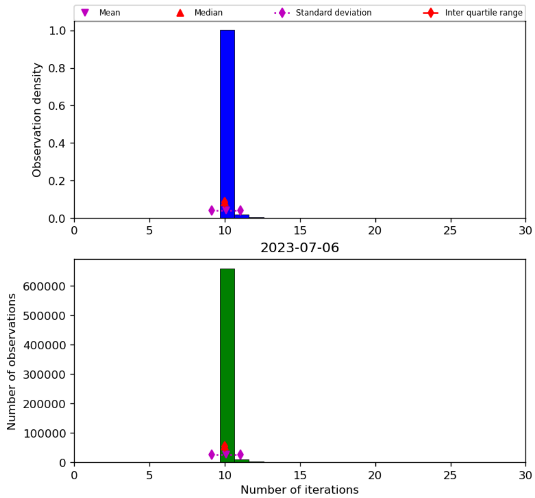
Figure 31: Histogram of “Number of iterations” for 2023-07-05 to 2023-07-07
