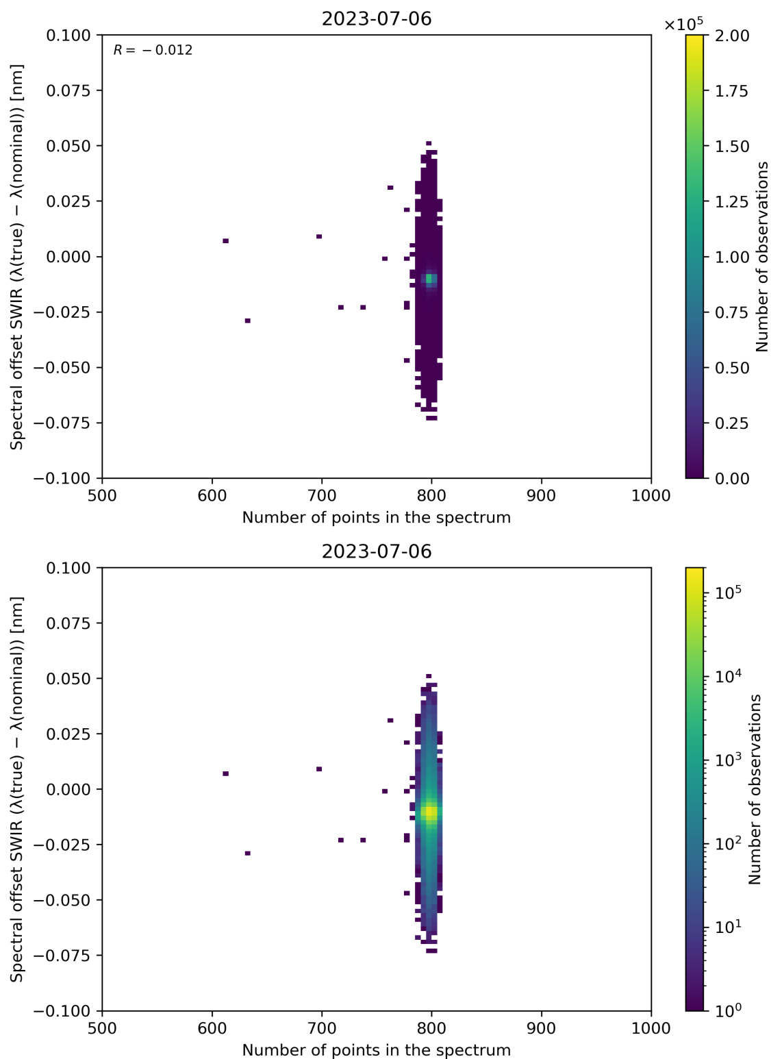
Figure 93: Scatter density plot of “Number of points in the spectrum” against “Spectral offset SWIR ( \lambda(\text{true}) - \lambda(\text{nominal}) )” for 2023-07-05 to 2023-07-07.
