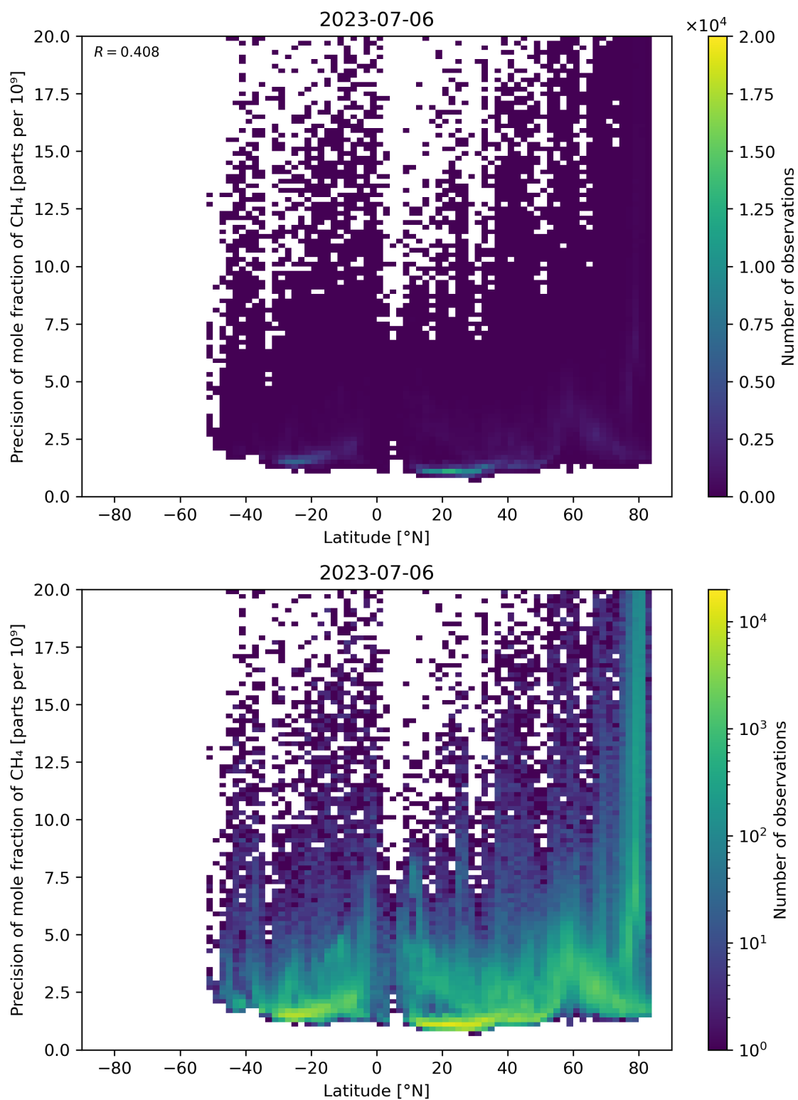
Figure 59: Scatter density plot of “Latitude” against “Precision of mole fraction of CH 4 ” for 2023-07-05 to 2023-07-07.
