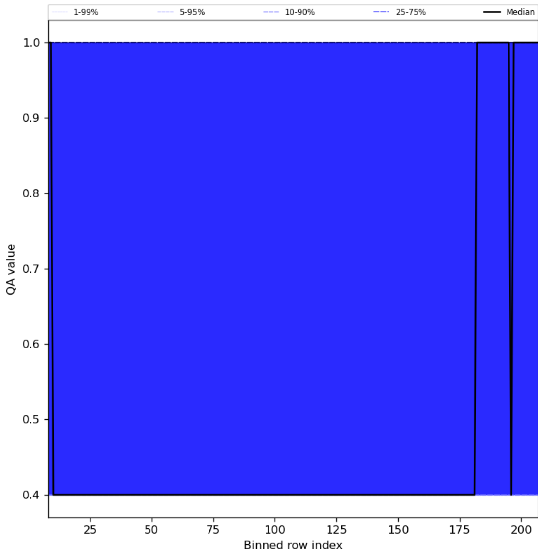
Figure 33: Along track statistics of “QA value” for 2023-07-05 to 2023-07-07
