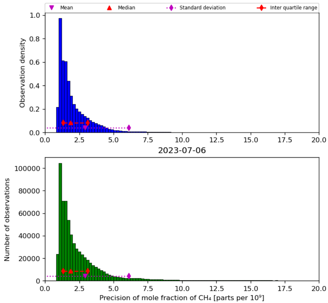
Figure 24: Histogram of “Precision of mole fraction of CH 4 ” for 2023-07-05 to 2023-07-07
