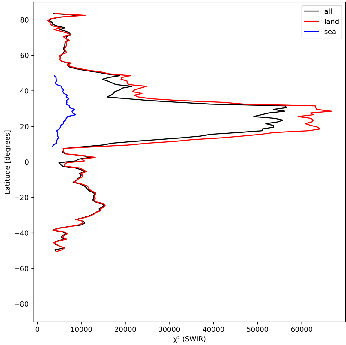
Figure 17: Zonal average of “ \chi^2 (SWIR)” for 2023-07-05 to 2023-07-07.
