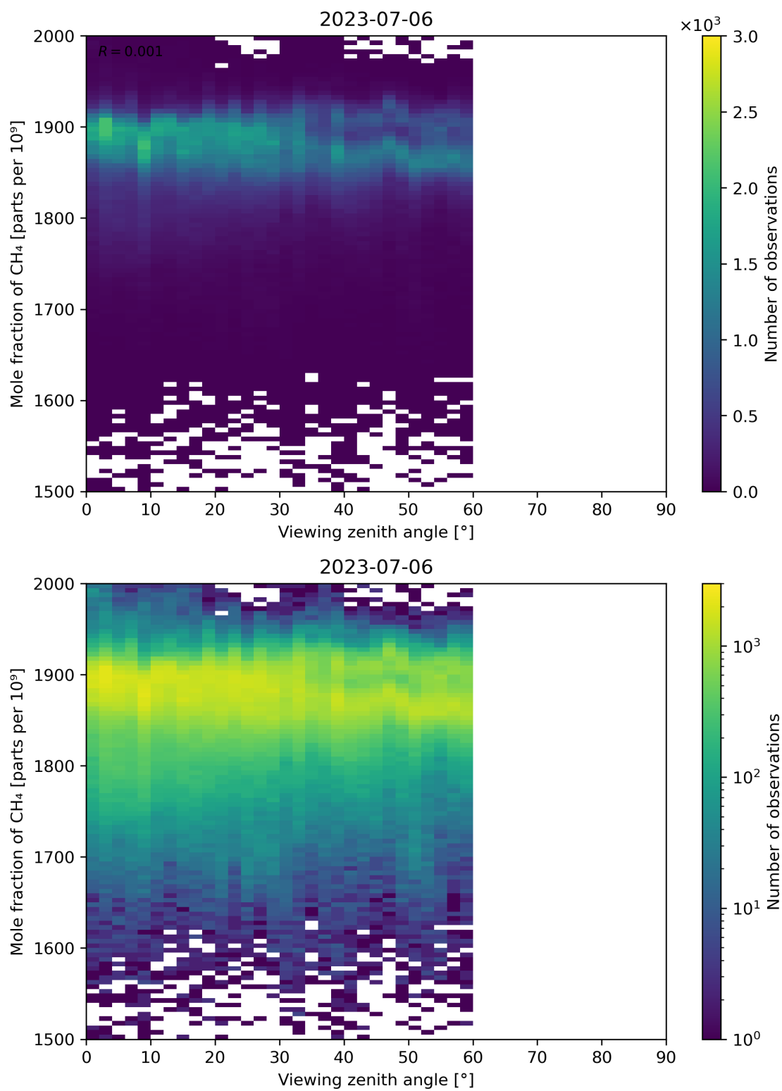
Figure 110: Scatter density plot of “Viewing zenith angle” against “Mole fraction of CH 4 ” for 2023-07-05 to 2023-07-07.
