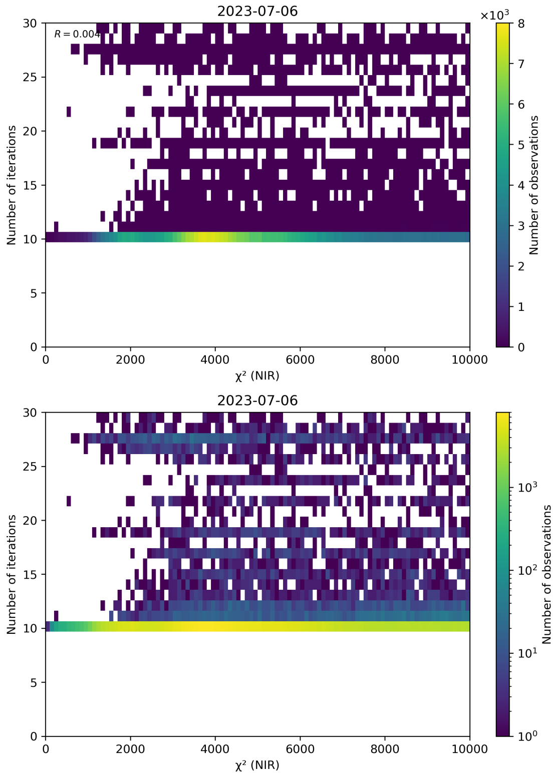
Figure 46: Scatter density plot of “ \chi^2 (NIR)” against “Number of iterations” for 2023-07-05 to 2023-07-07.
