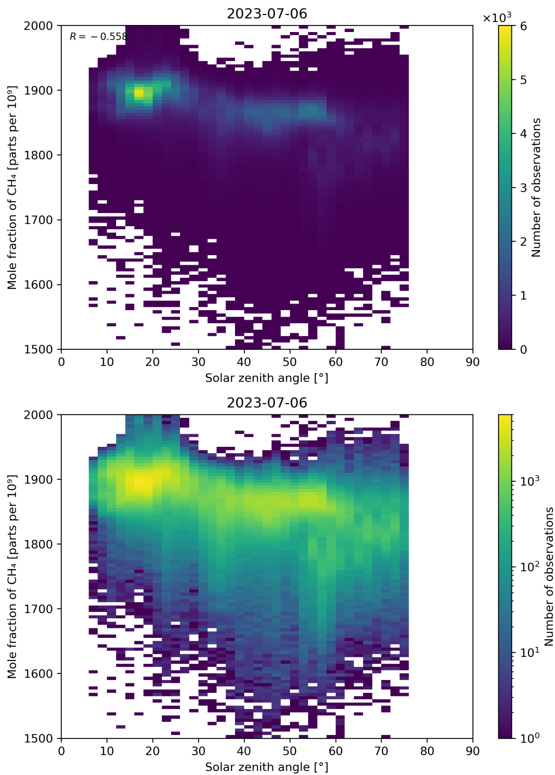
Figure 99: Scatter density plot of “Solar zenith angle” against “Mole fraction of \text{CH}_4 ” for 2023-07-05 to 2023-07-07.
