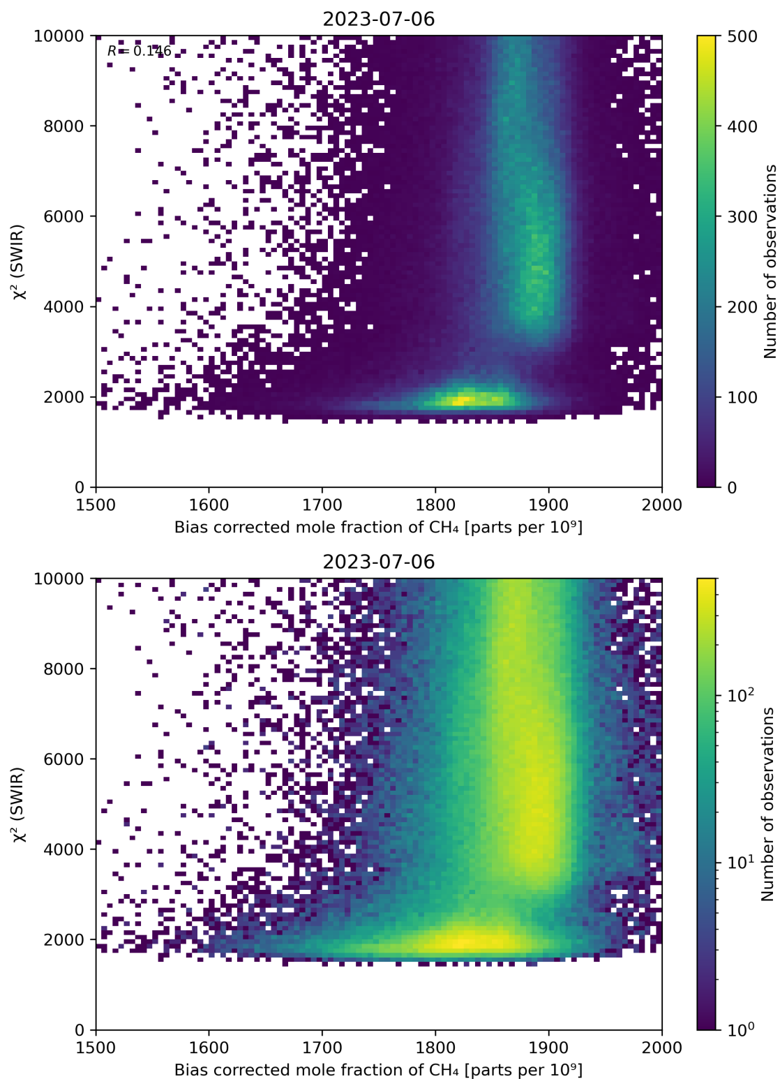
Figure 64: Scatter density plot of “Bias corrected mole fraction of CH 4 ” against “ \chi^2 (SWIR)” for 2023-07-05 to 2023-07-07.
