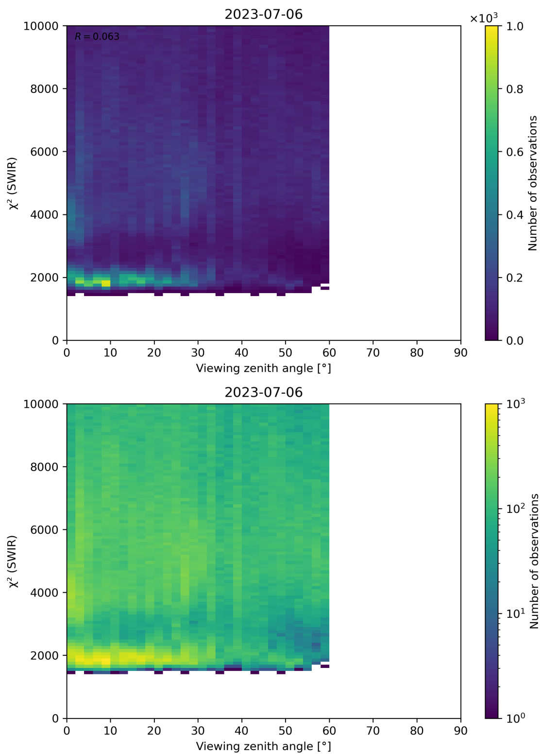
Figure 106: Scatter density plot of “Viewing zenith angle” against “ \chi^2 (SWIR)” for 2023-07-05 to 2023-07-07.
