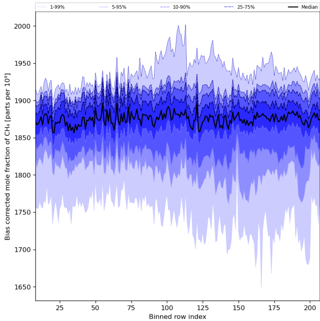
Figure 36: Along track statistics of “Bias corrected mole fraction of CH 4 ” for 2023-07-05 to 2023-07-07
