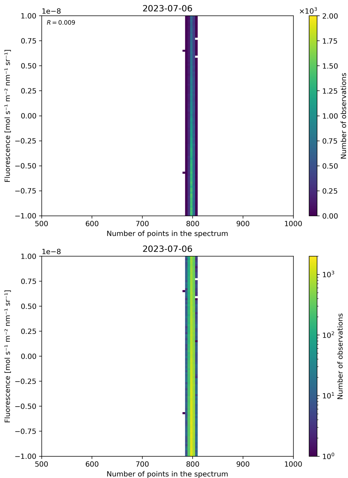
Figure 91: Scatter density plot of “Number of points in the spectrum” against “Fluorescence” for 2023-07-05 to 2023-07-07.
