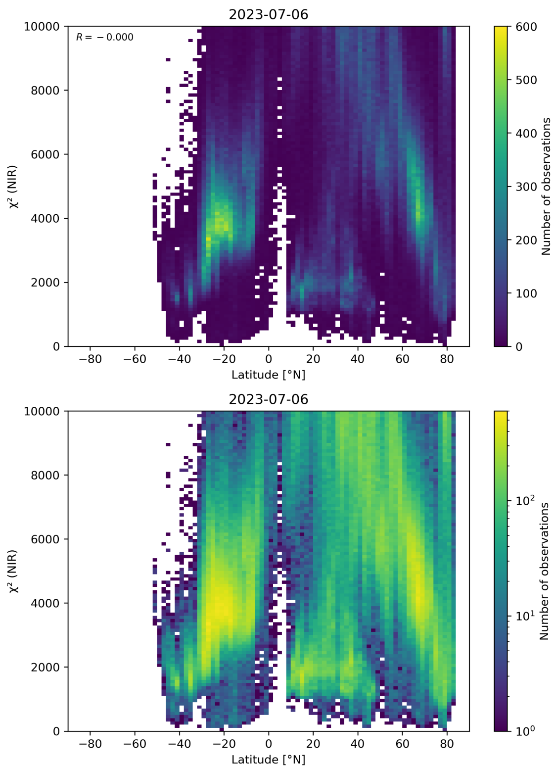
Figure 53: Scatter density plot of “Latitude” against “ \chi^2 (NIR)” for 2023-07-05 to 2023-07-07.
