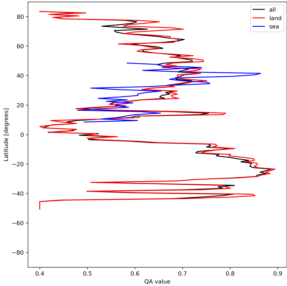
Figure 11: Zonal average of “QA value” for 2023-07-05 to 2023-07-07.
