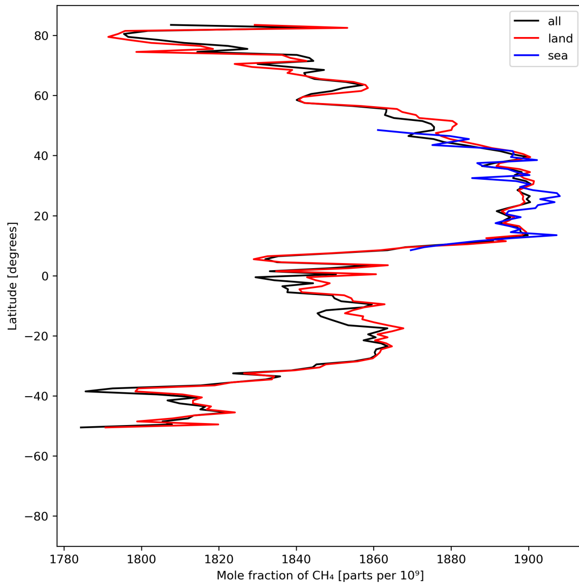
Figure 12: Zonal average of “Mole fraction of \text{CH}_4 ” for 2023-07-05 to 2023-07-07.
