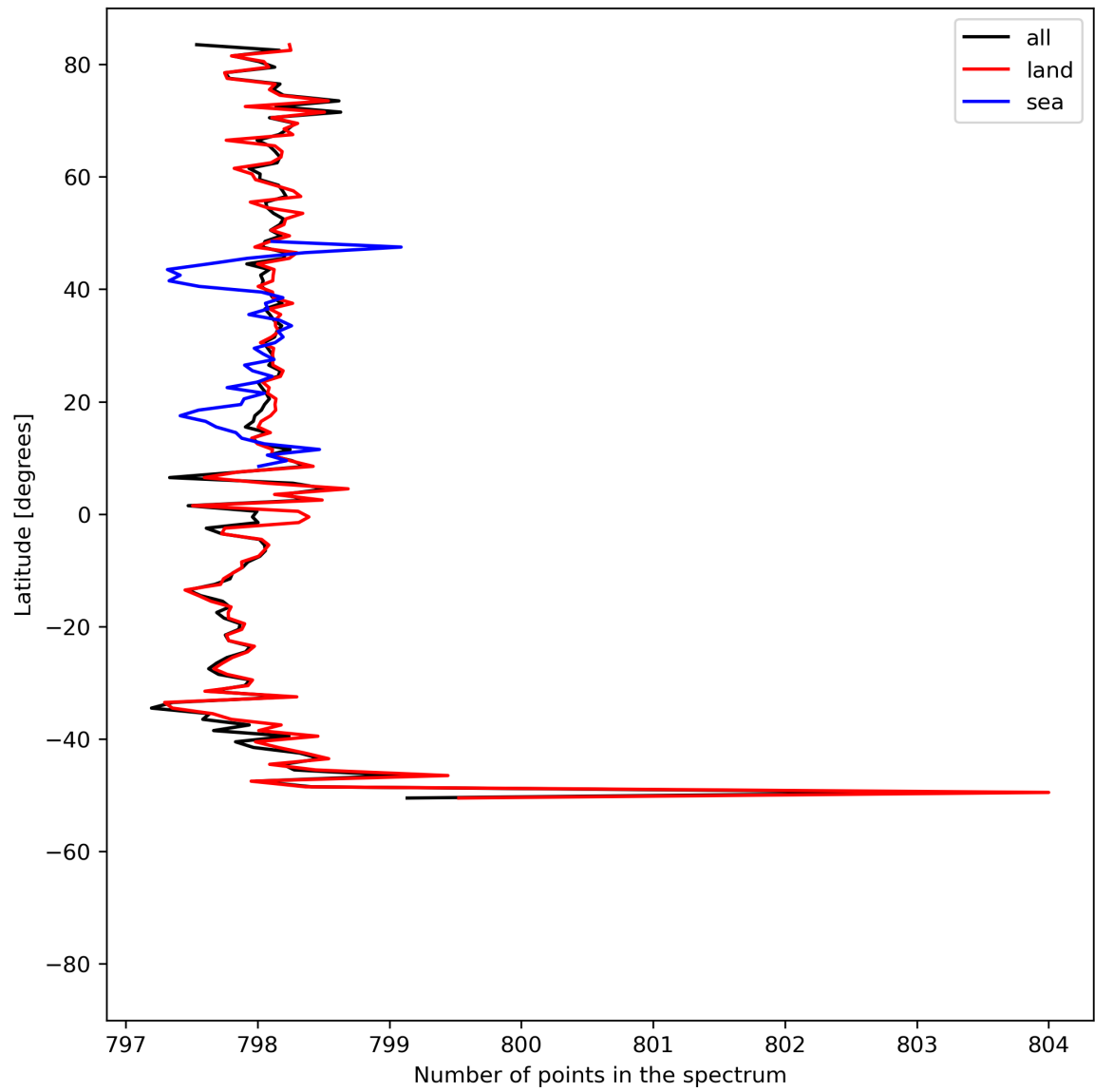
Figure 15: Zonal average of “Number of points in the spectrum” for 2023-07-05 to 2023-07-07.
