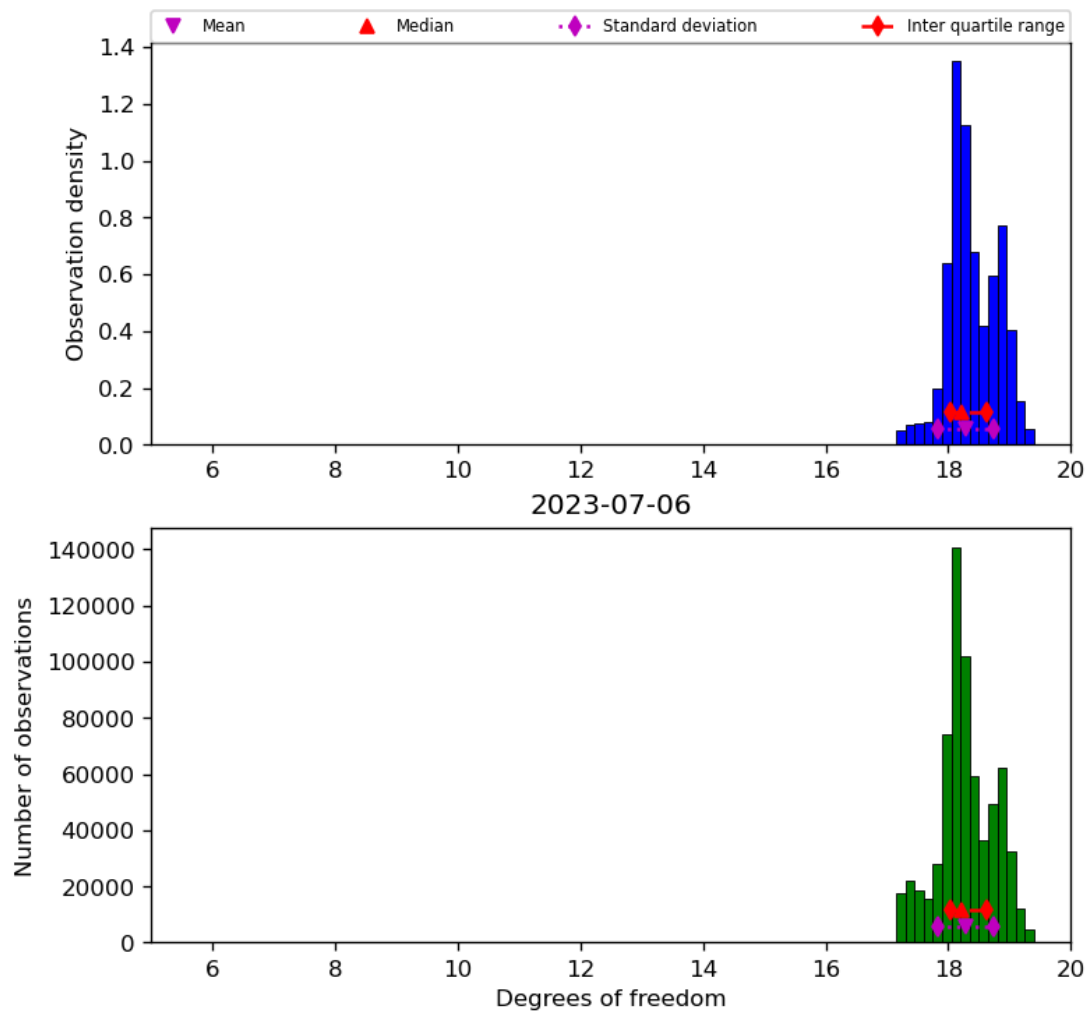
Figure 30: Histogram of “Degrees of freedom” for 2023-07-05 to 2023-07-07
