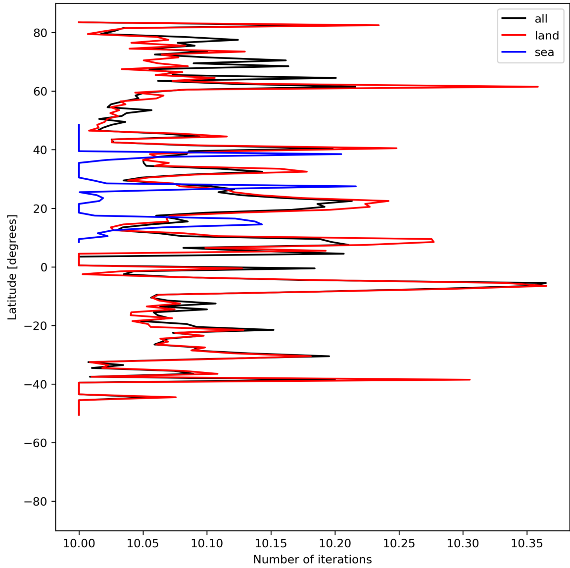
Figure 20: Zonal average of “Number of iterations” for 2023-07-05 to 2023-07-07.
