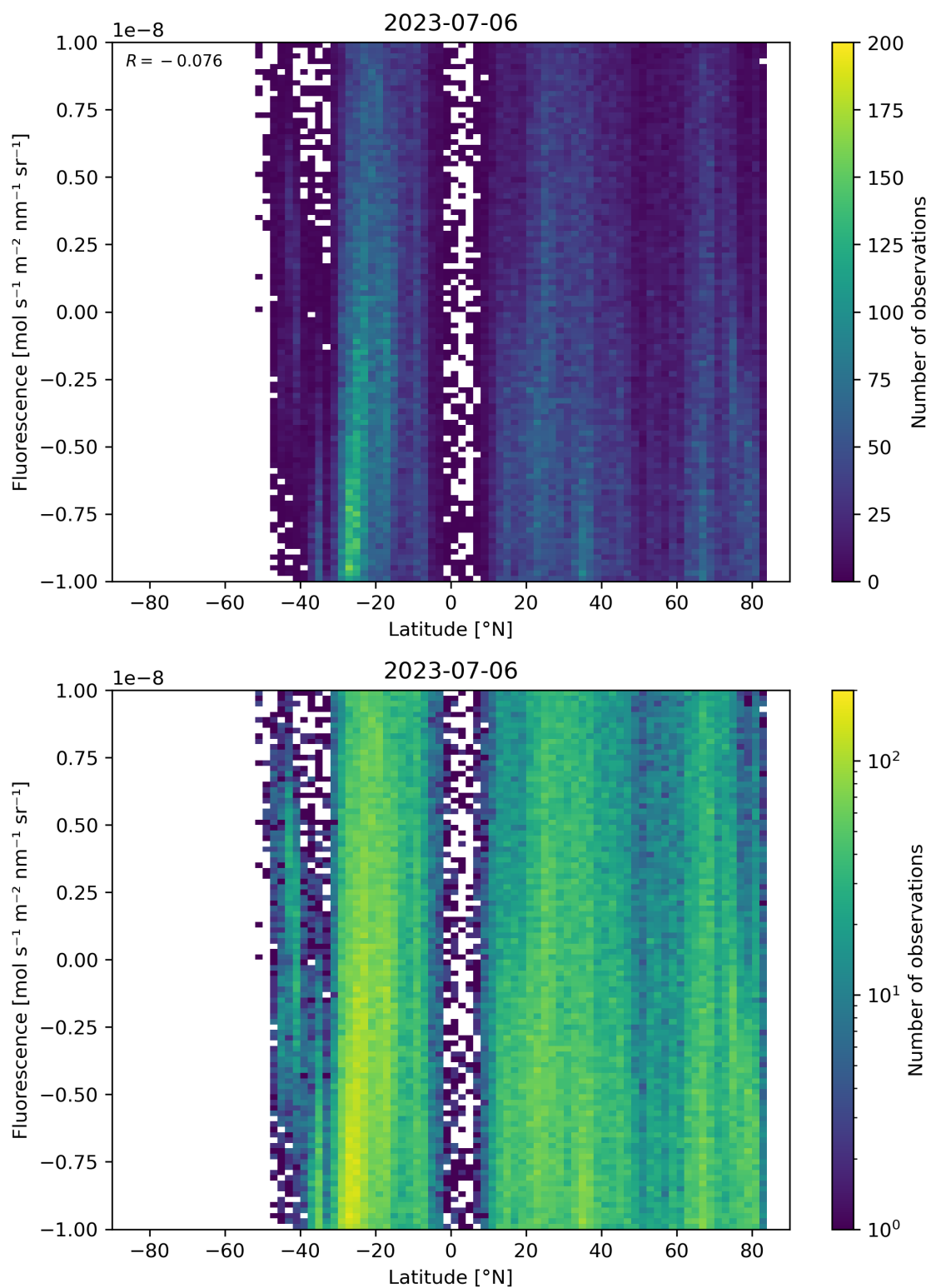
Figure 56: Scatter density plot of “Latitude” against “Fluorescence” for 2023-07-05 to 2023-07-07.
