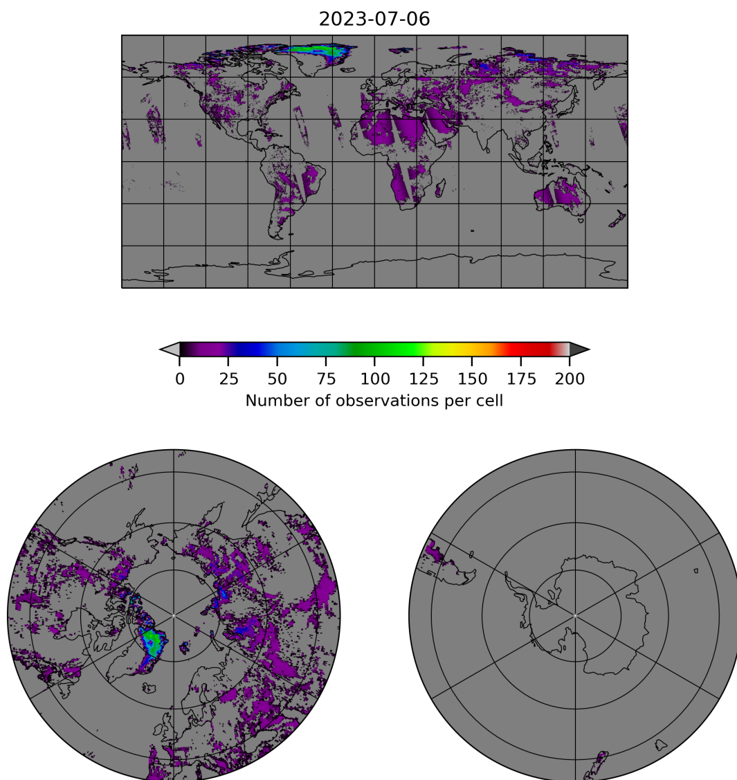
Figure 10: Map of the number of observations for 2023-07-05 to 2023-07-07
