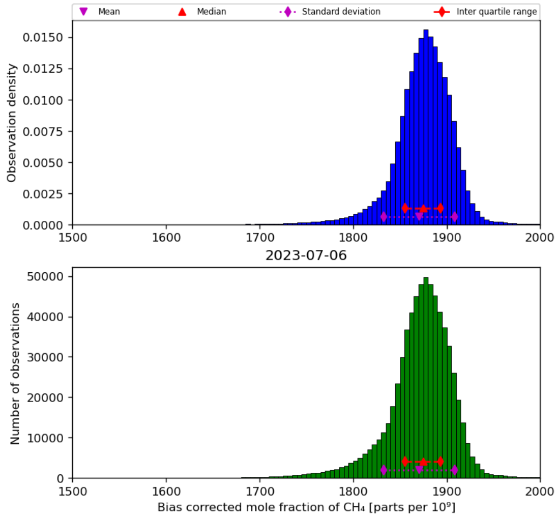
Figure 25: Histogram of “Bias corrected mole fraction of CH 4 ” for 2023-07-05 to 2023-07-07
