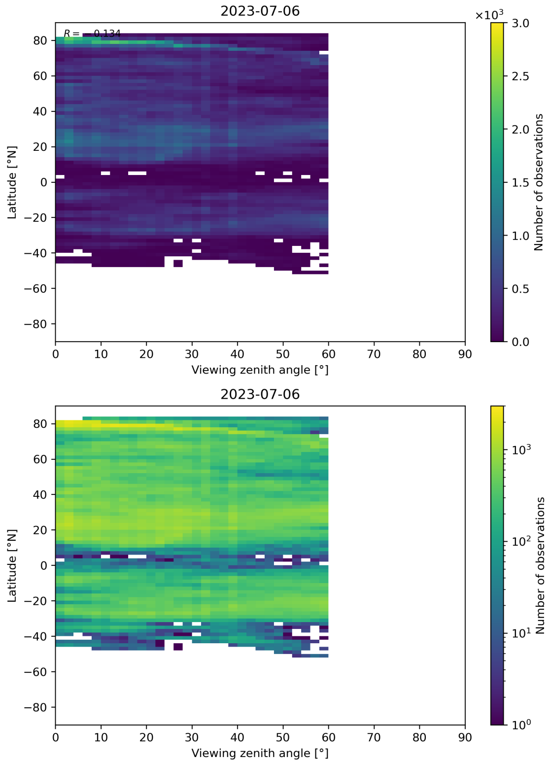
Figure 109: Scatter density plot of “Viewing zenith angle” against “Latitude” for 2023-07-05 to 2023-07-07.
