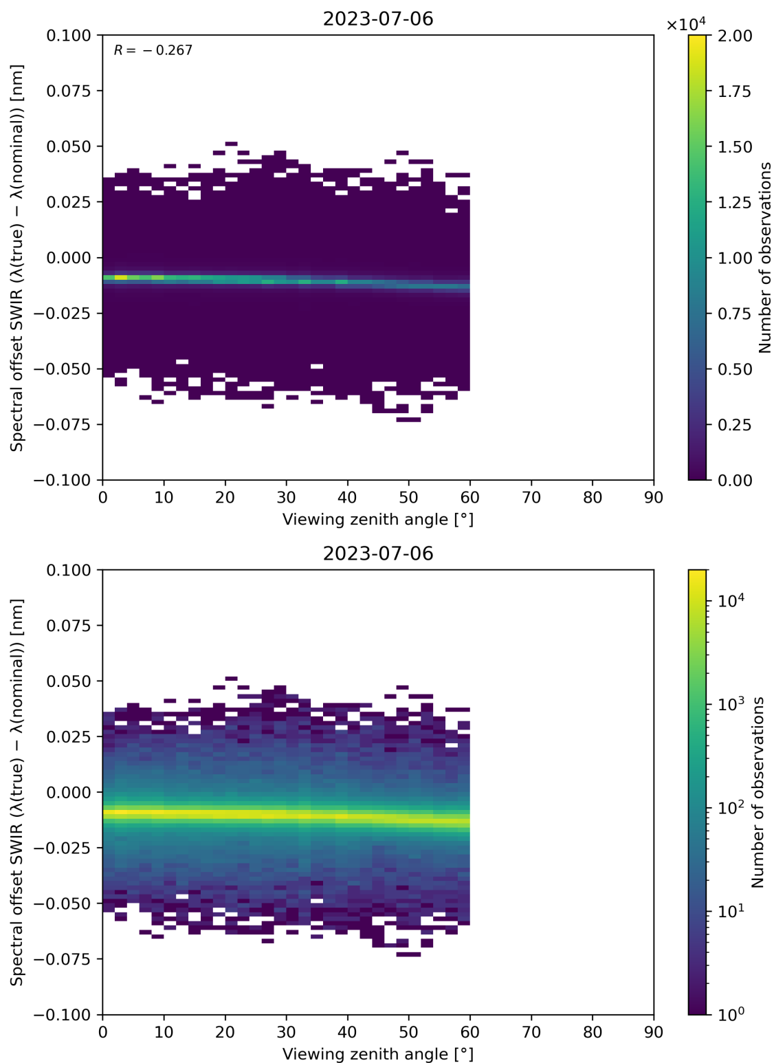
Figure 116: Scatter density plot of “Viewing zenith angle” against “Spectral offset SWIR ( \lambda(\text{true}) - \lambda(\text{nominal}) )” for 2023-07-05 to 2023-07-07.
