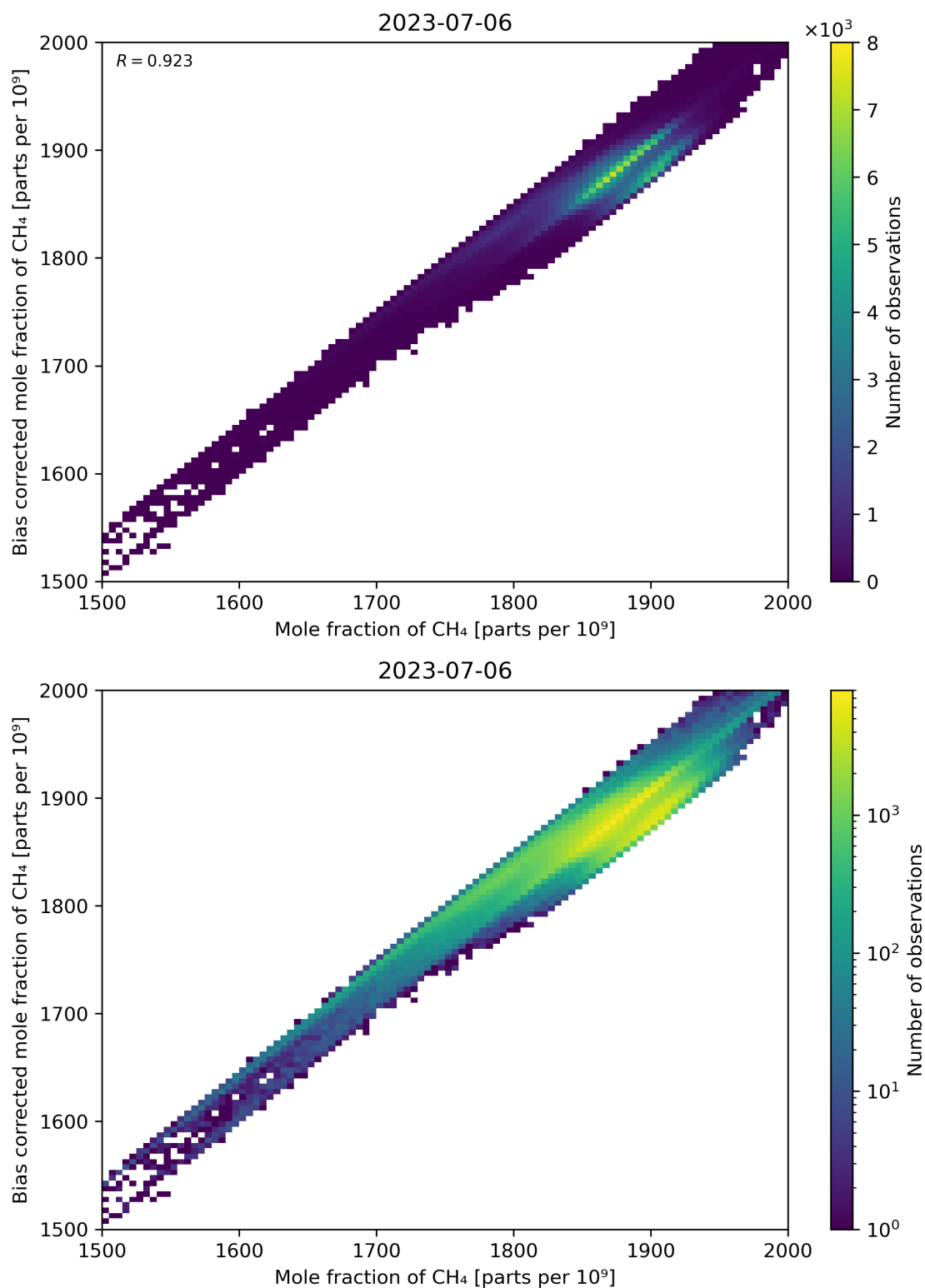
Figure 74: Scatter density plot of “Mole fraction of CH 4 ” against “Bias corrected mole fraction of CH 4 ” for 2023-07-05 to 2023-07-07.
