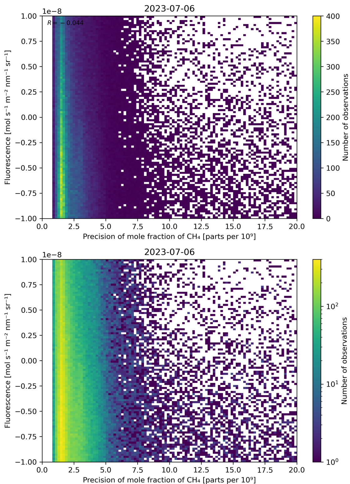
Figure 81: Scatter density plot of “Precision of mole fraction of \text{CH}_4 ” against “Fluorescence” for 2023-07-05 to 2023-07-07.
