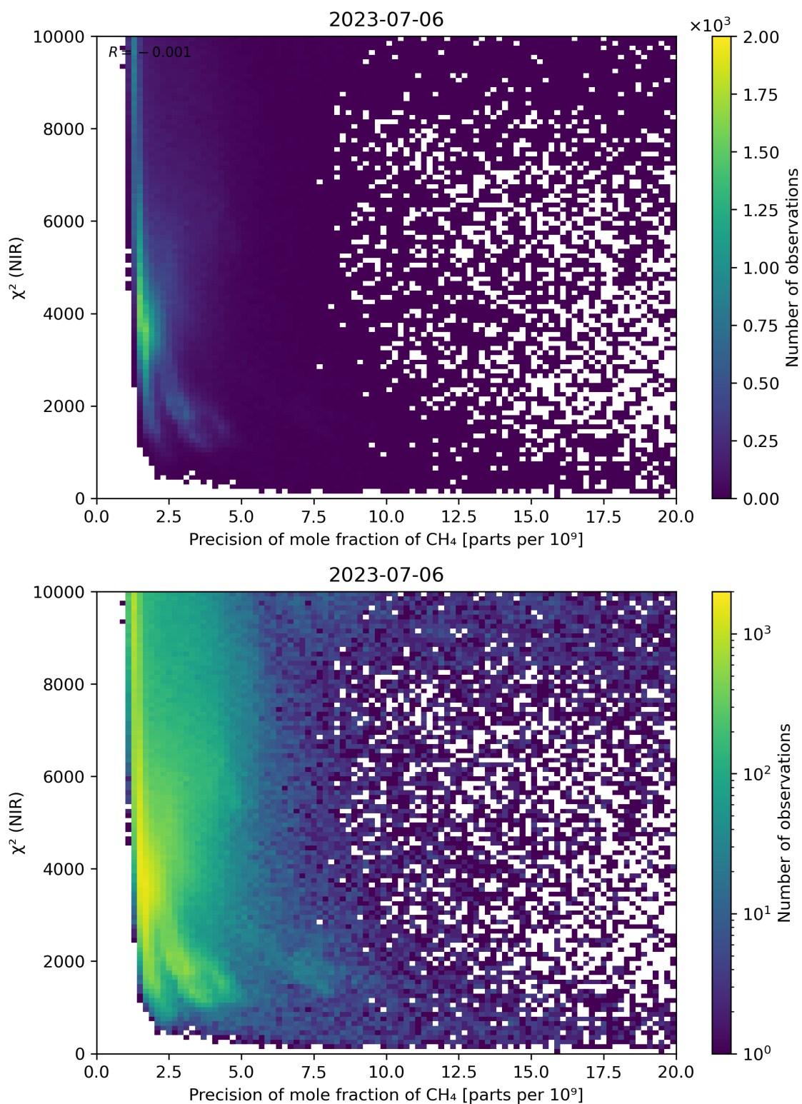
Figure 78: Scatter density plot of “Precision of mole fraction of CH 4 ” against “ \chi^2 (NIR)” for 2023-07-05 to 2023-07-07.
