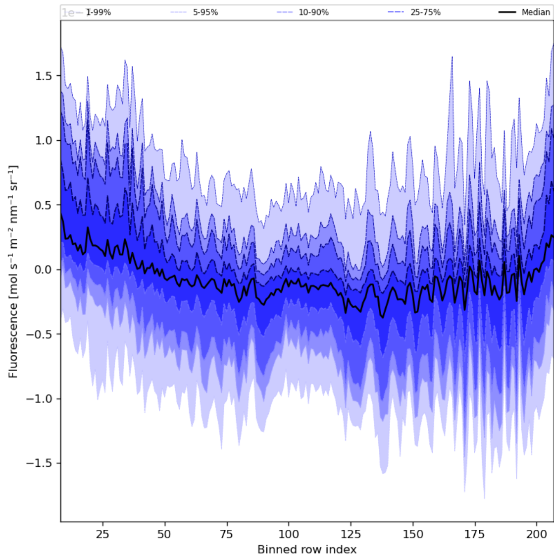
Figure 43: Along track statistics of “Fluorescence” for 2023-07-05 to 2023-07-07
