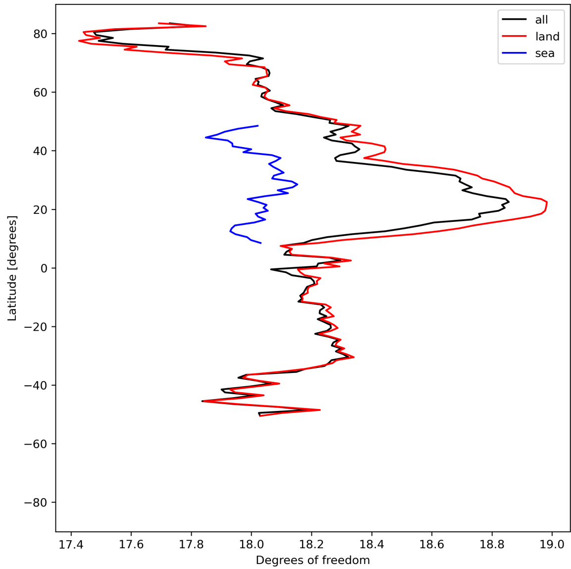
Figure 19: Zonal average of “Degrees of freedom” for 2023-07-05 to 2023-07-07.
