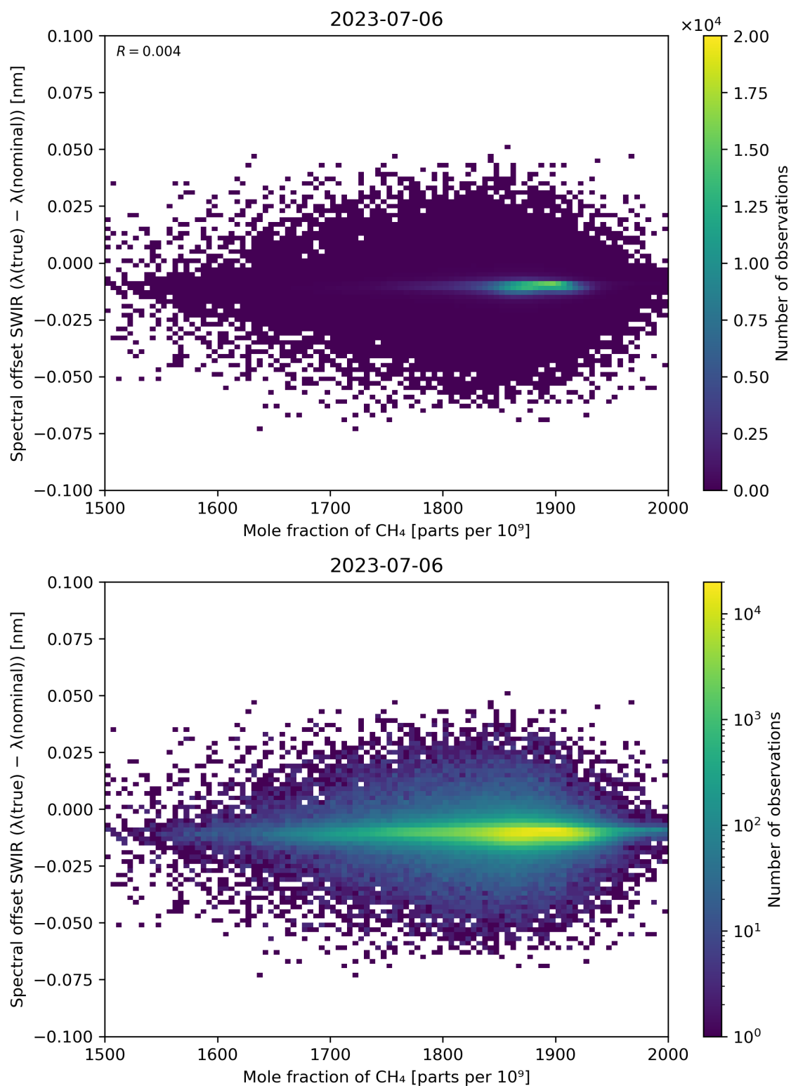
Figure 86: Scatter density plot of “Mole fraction of CH 4 ” against “Spectral offset SWIR ( \lambda(\text{true}) - \lambda(\text{nominal}) )” for 2023-07-05 to 2023-07-07.
