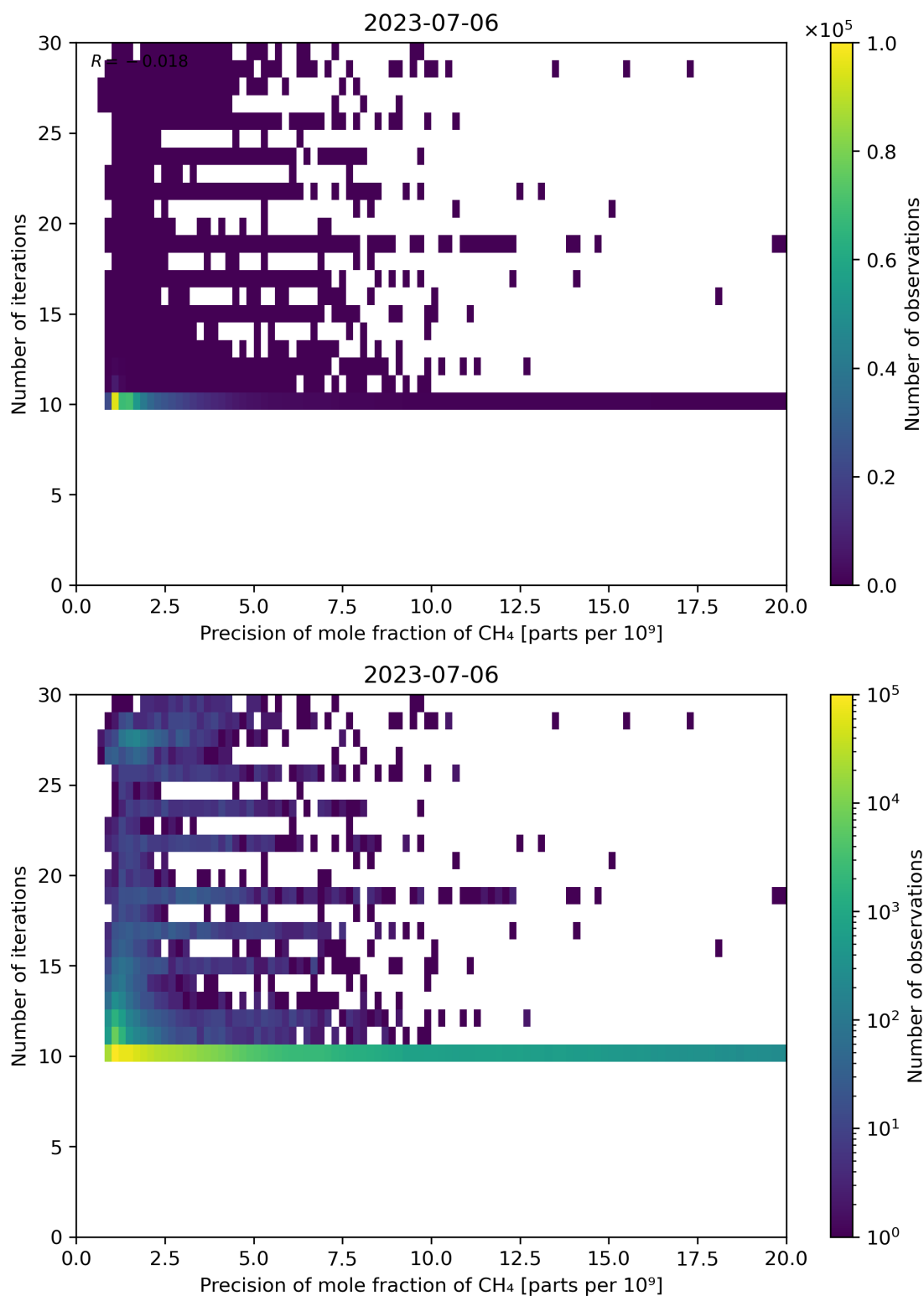
Figure 83: Scatter density plot of “Precision of mole fraction of CH 4 ” against “Number of iterations” for 2023-07-05 to 2023-07-07.
