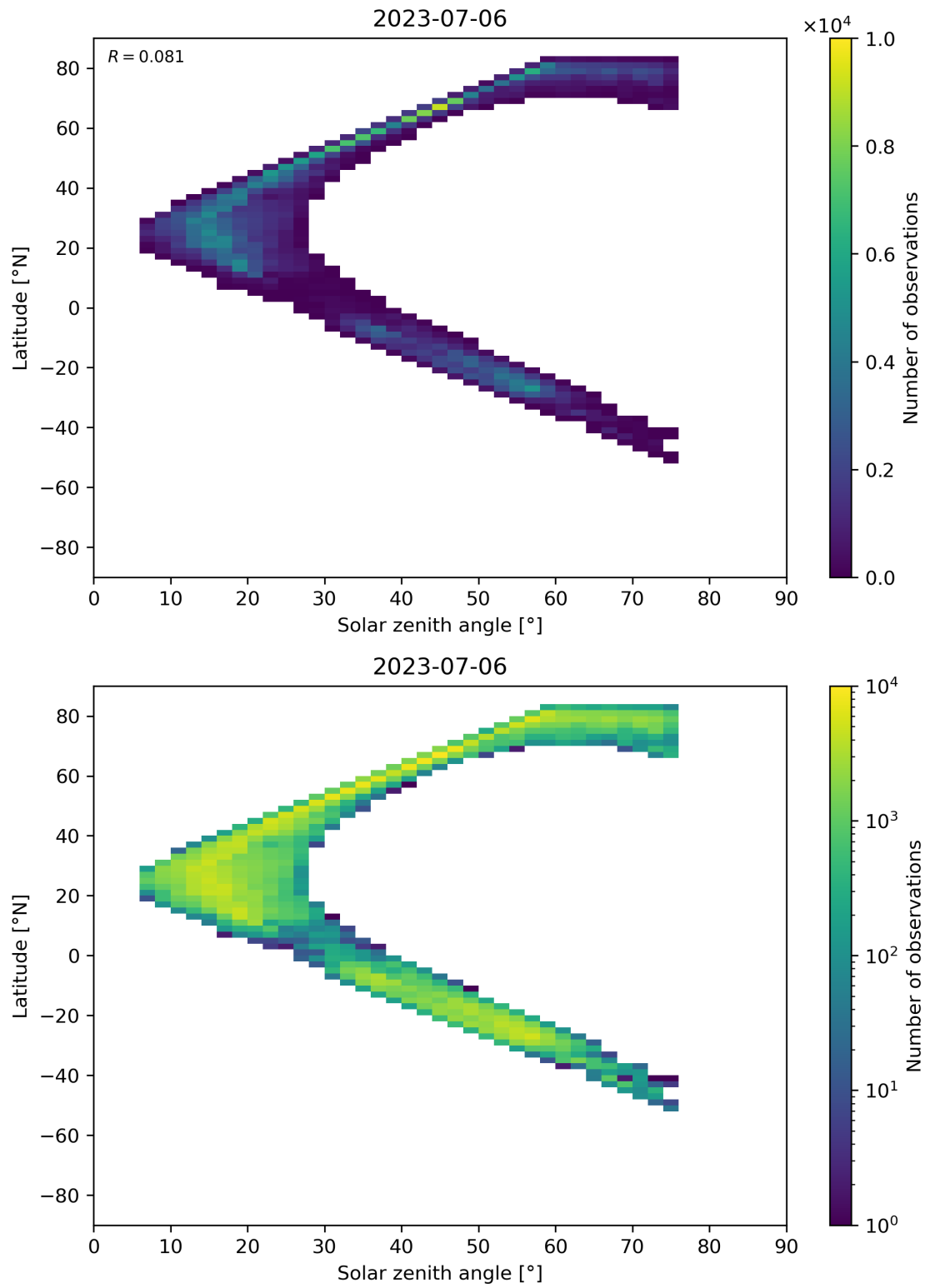
Figure 98: Scatter density plot of “Solar zenith angle” against “Latitude” for 2023-07-05 to 2023-07-07.
