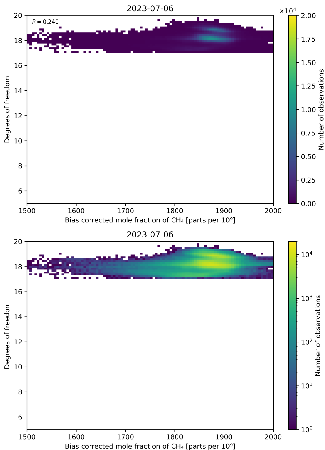
Figure 65: Scatter density plot of “Bias corrected mole fraction of CH 4 ” against “Degrees of freedom” for 2023-07-05 to 2023-07-07.
