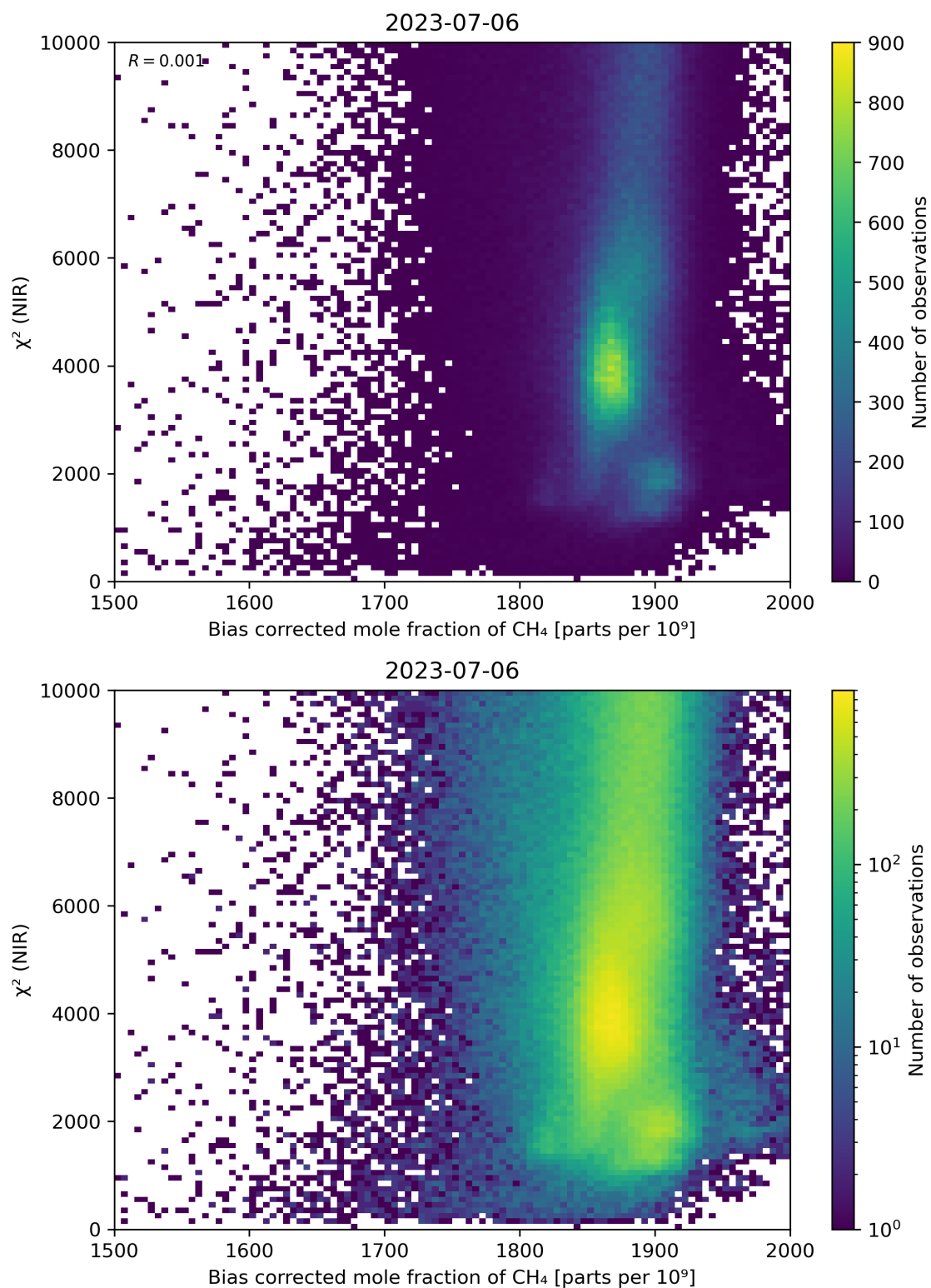
Figure 63: Scatter density plot of “Bias corrected mole fraction of CH 4 ” against “ \chi^2 (NIR)” for 2023-07-05 to 2023-07-07.
