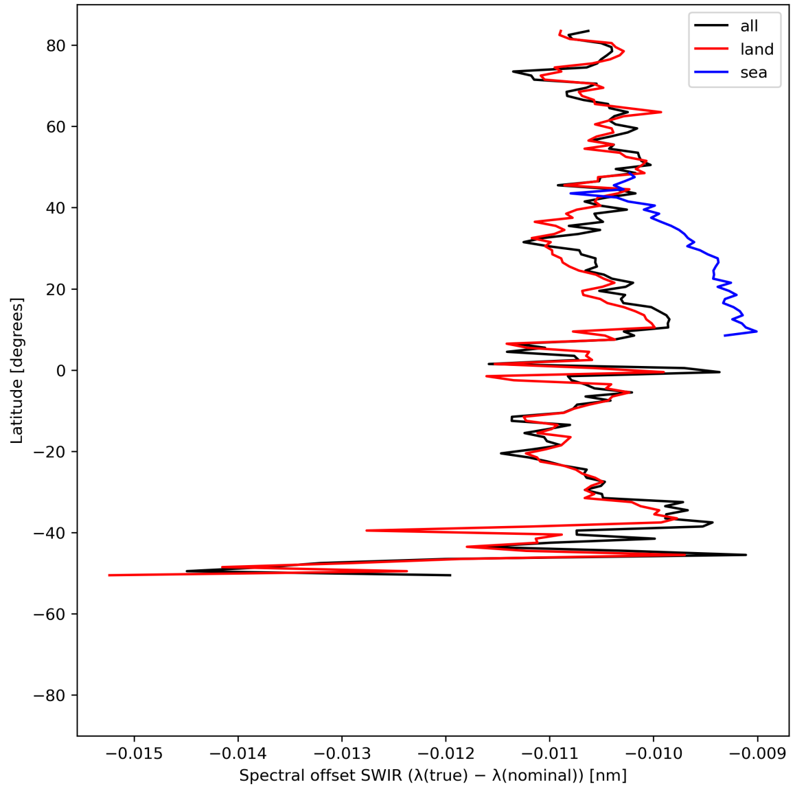
Figure 16: Zonal average of “Spectral offset SWIR ( \lambda(\text{true}) - \lambda(\text{nominal}) )” for 2023-07-05 to 2023-07-07.
