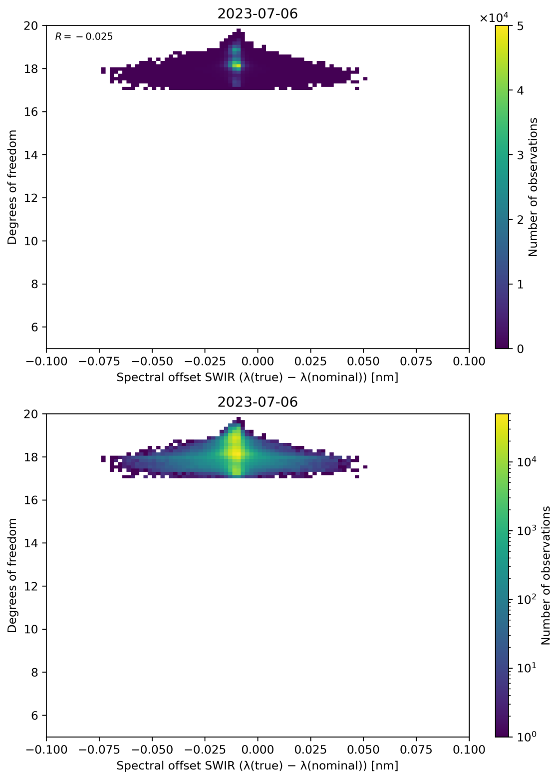
Figure 119: Scatter density plot of “Spectral offset SWIR ( \lambda(\text{true}) - \lambda(\text{nominal}) )” against “Degrees of freedom” for 2023-07-05 to 2023-07-07.
