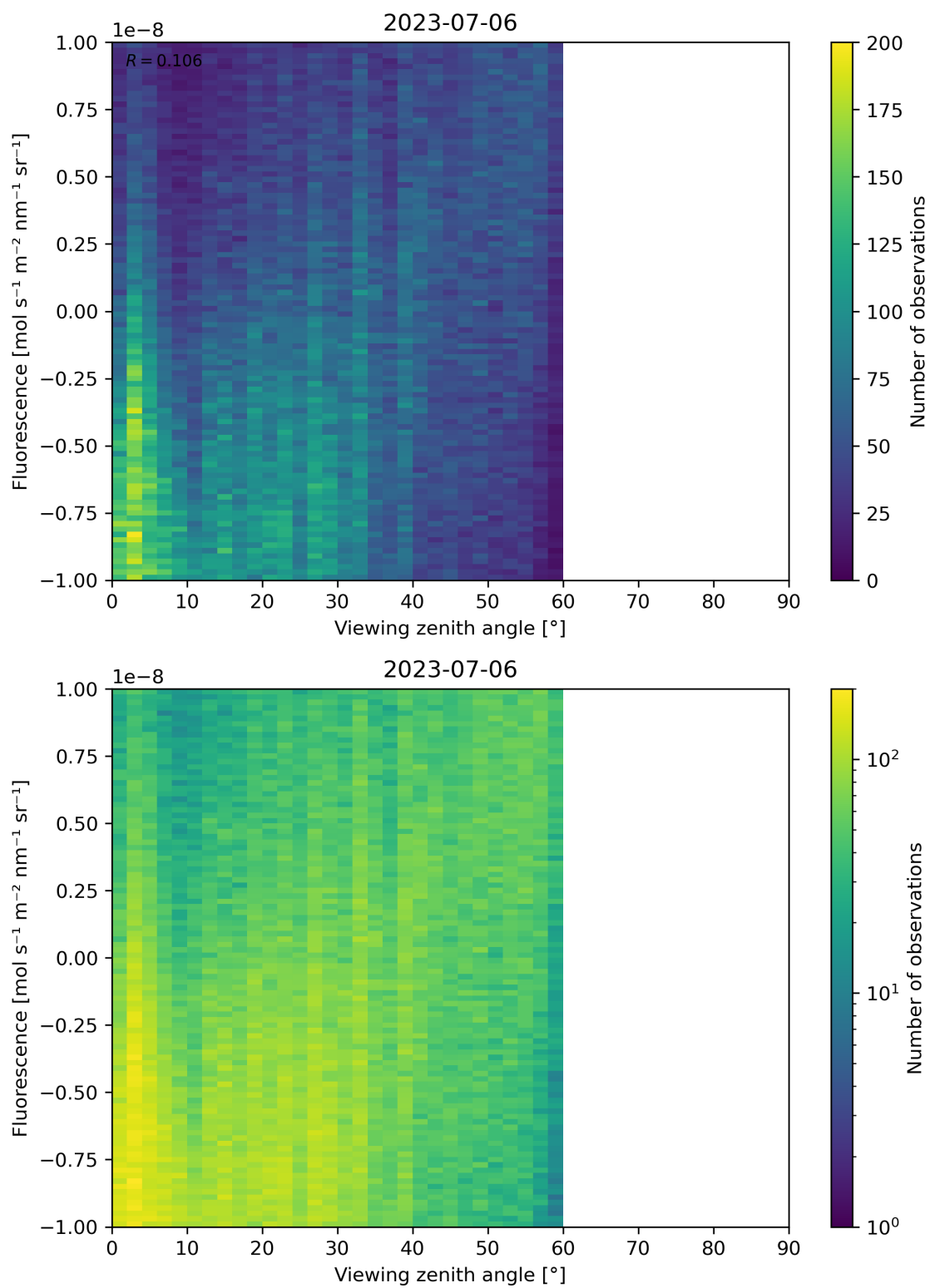
Figure 108: Scatter density plot of “Viewing zenith angle” against “Fluorescence” for 2023-07-05 to 2023-07-07.
