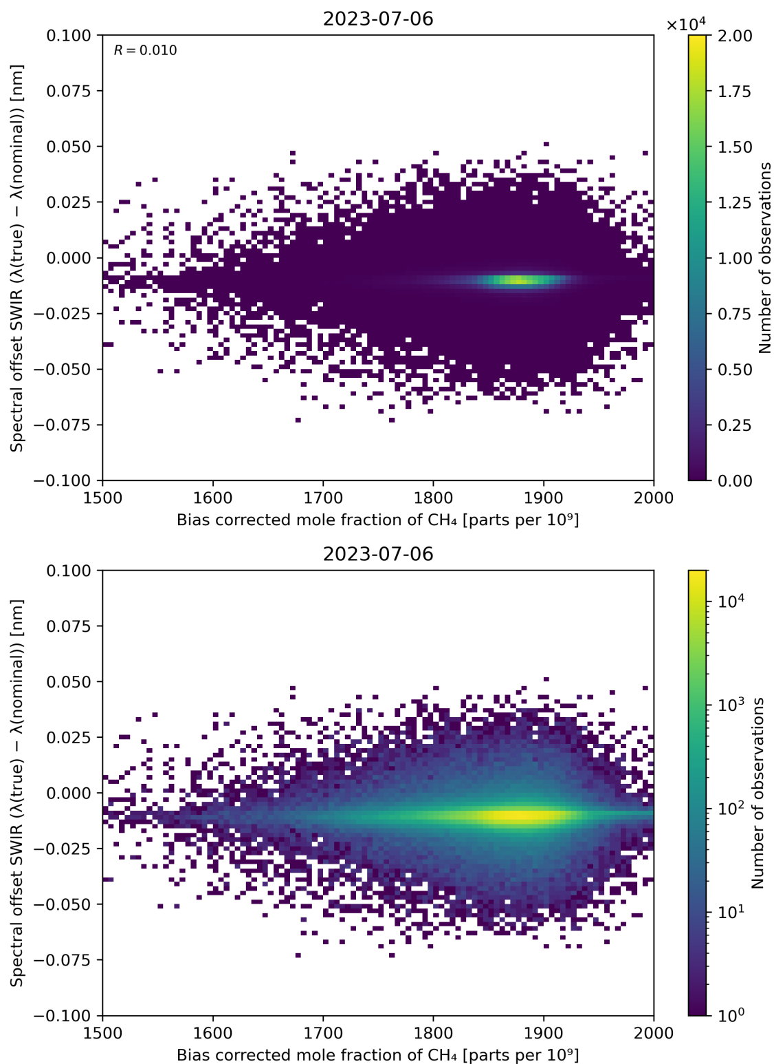
Figure 69: Scatter density plot of “Bias corrected mole fraction of \text{CH}_4 ” against “Spectral offset SWIR ( \lambda(\text{true}) - \lambda(\text{nominal}) )” for 2023-07-05 to 2023-07-07.
