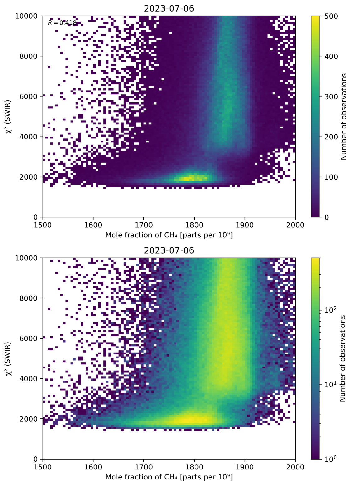
Figure 71: Scatter density plot of “Mole fraction of CH 4 ” against “ \chi^2 (SWIR)” for 2023-07-05 to 2023-07-07.
