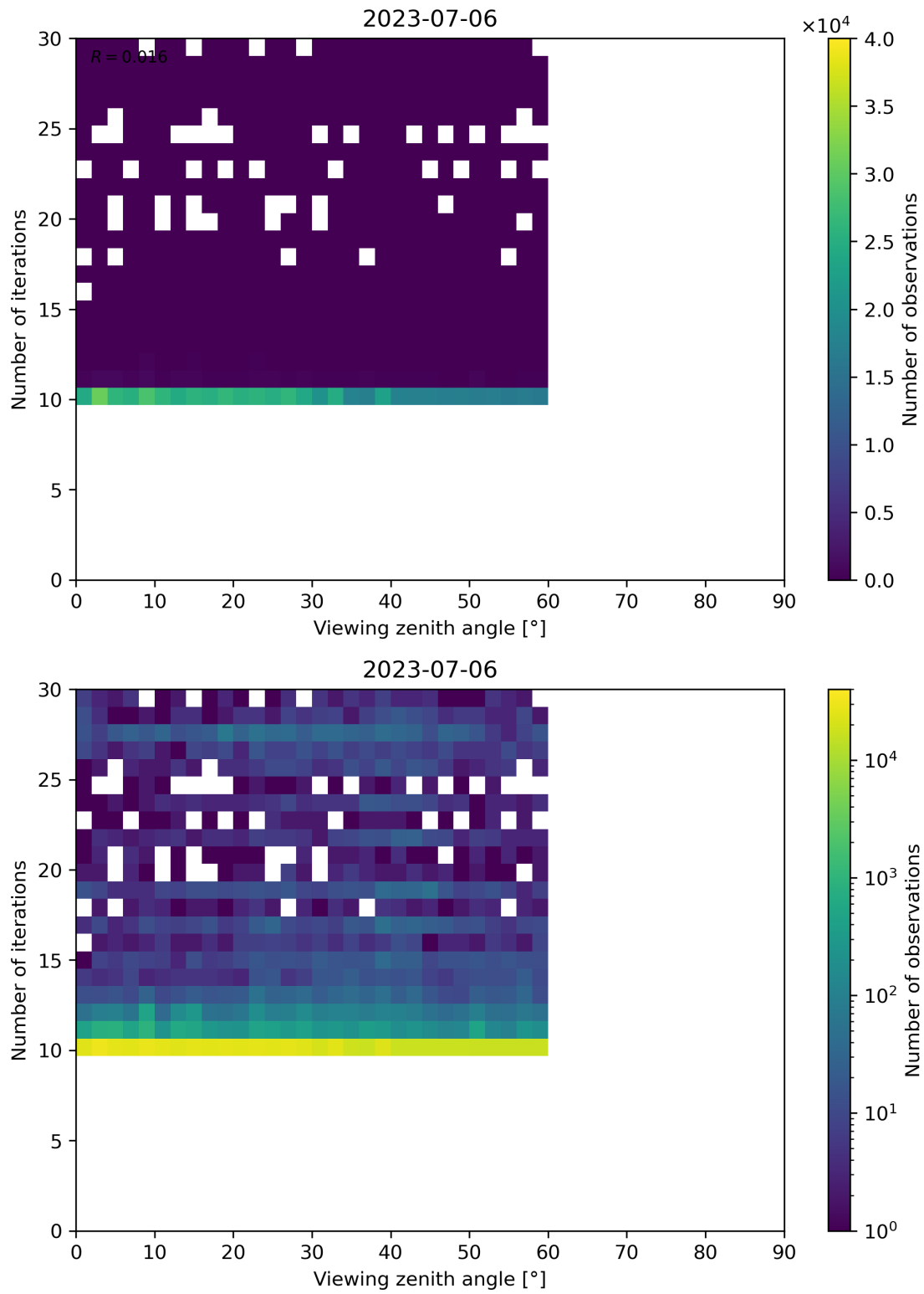
Figure 113: Scatter density plot of “Viewing zenith angle” against “Number of iterations” for 2023-07-05 to 2023-07-07.
