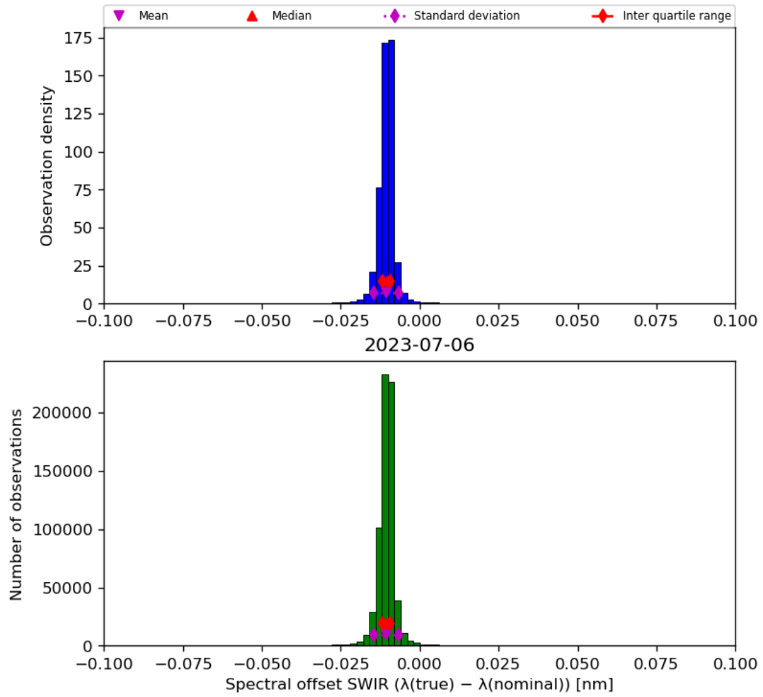
Figure 27: Histogram of “Spectral offset SWIR ( \lambda(\text{true}) - \lambda(\text{nominal}) )” for 2023-07-05 to 2023-07-07
