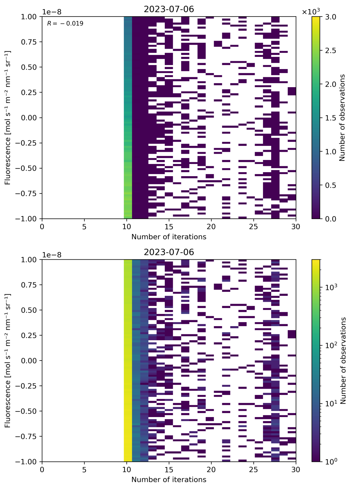
Figure 87: Scatter density plot of “Number of iterations” against “Fluorescence” for 2023-07-05 to 2023-07-07.
