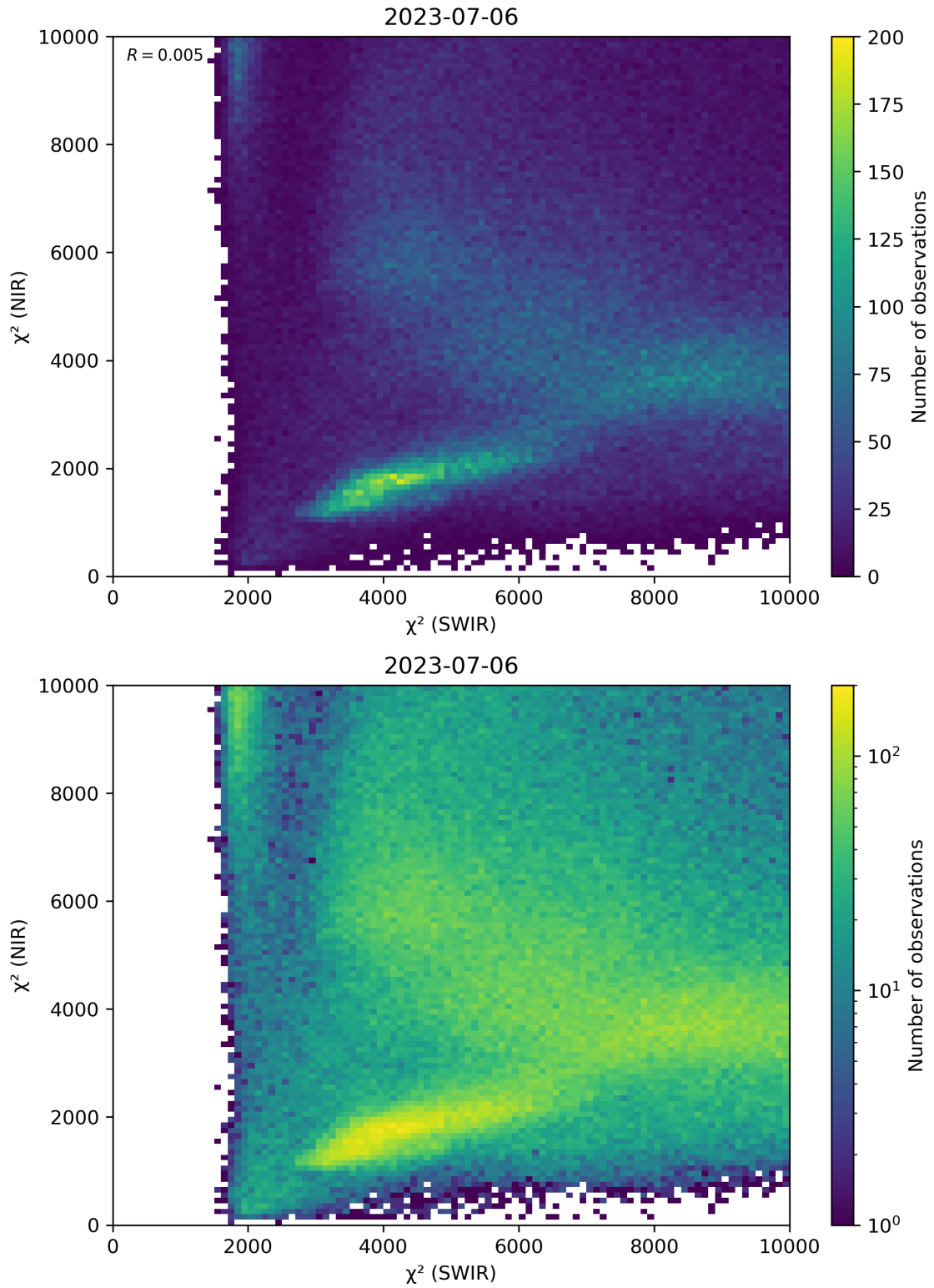
Figure 47: Scatter density plot of “ \chi^2 (SWIR)” against “ \chi^2 (NIR)” for 2023-07-05 to 2023-07-07.
