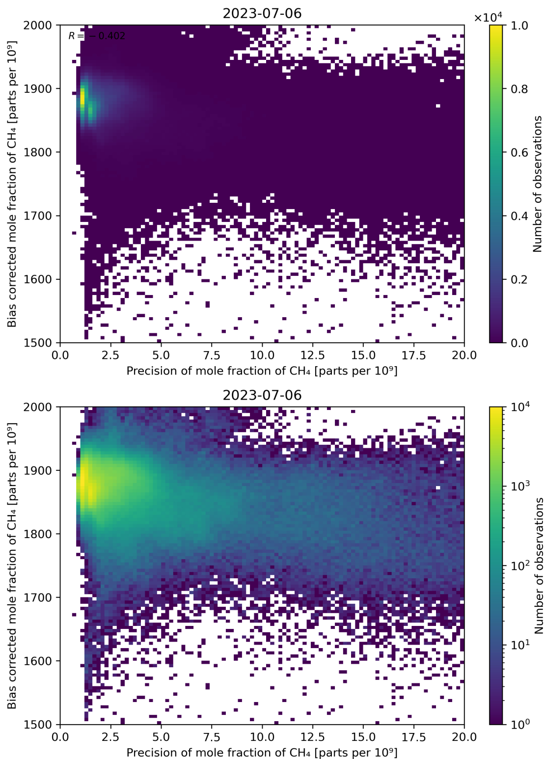
Figure 82: Scatter density plot of “Precision of mole fraction of CH 4 ” against “Bias corrected mole fraction of CH 4 ” for 2023-07-05 to 2023-07-07.
