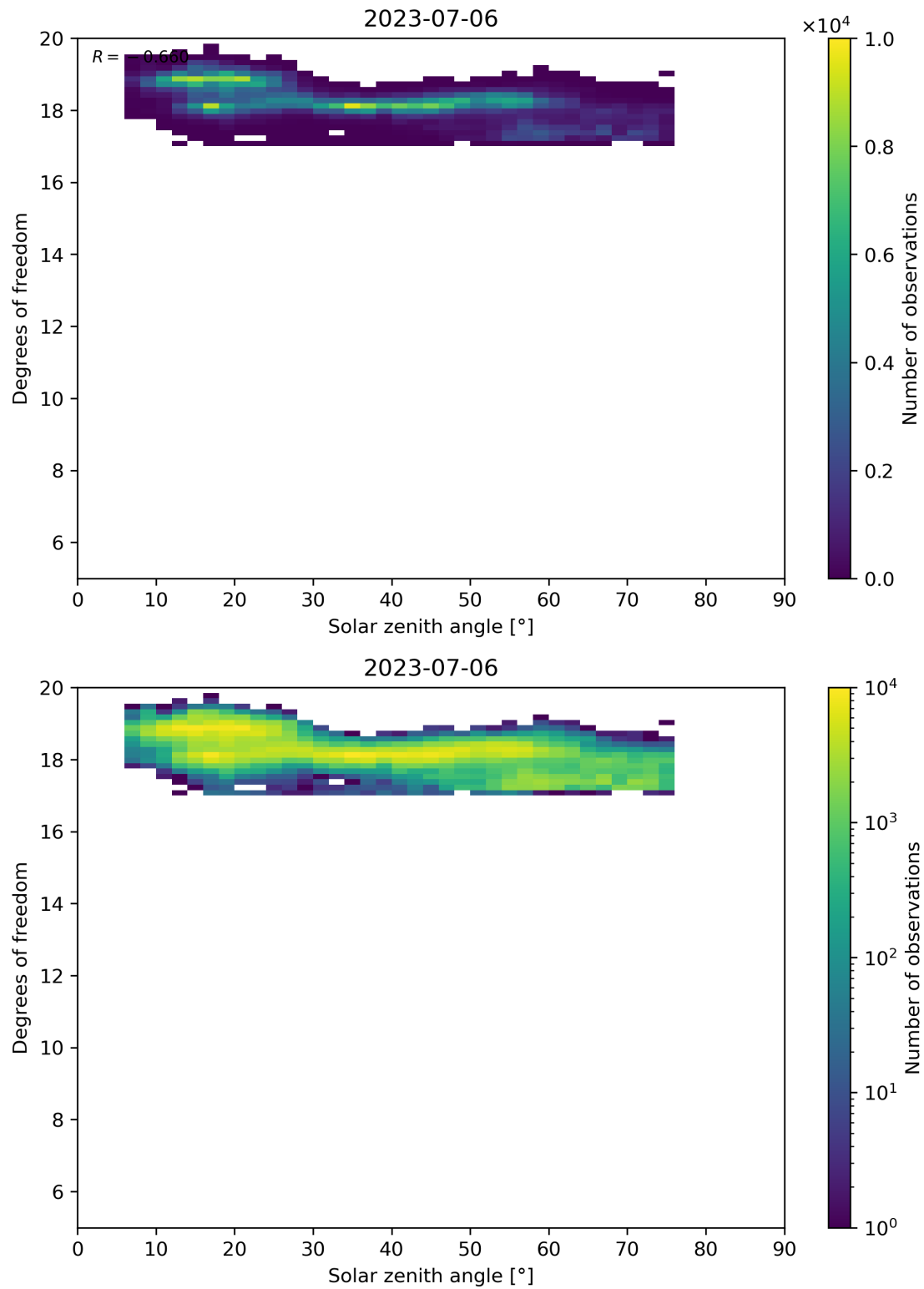
Figure 96: Scatter density plot of “Solar zenith angle” against “Degrees of freedom” for 2023-07-05 to 2023-07-07.
