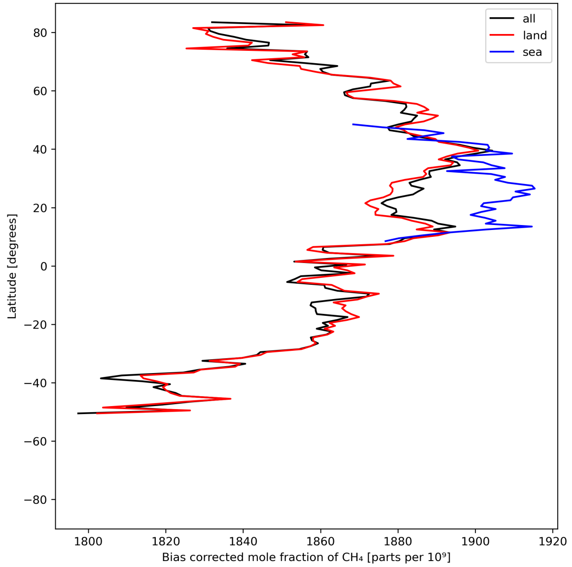
Figure 14: Zonal average of “Bias corrected mole fraction of CH 4 ” for 2023-07-05 to 2023-07-07.
