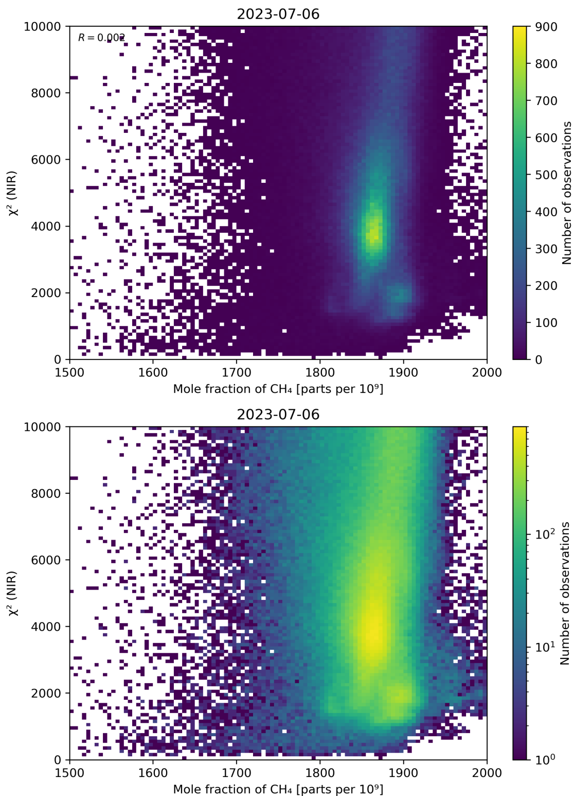
Figure 70: Scatter density plot of “Mole fraction of CH 4 ” against “ \chi^2 (NIR)” for 2023-07-05 to 2023-07-07.
