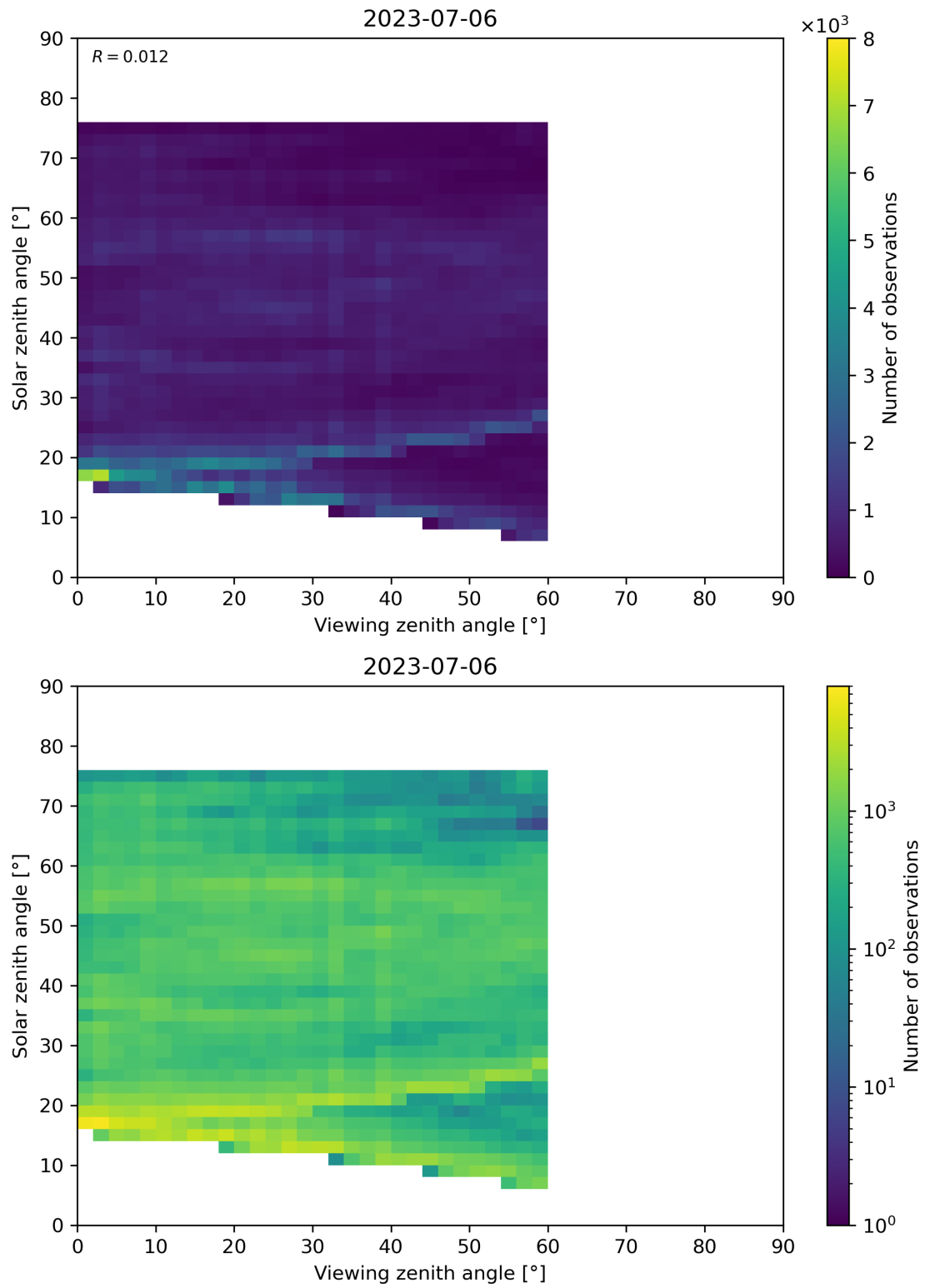
Figure 115: Scatter density plot of “Viewing zenith angle” against “Solar zenith angle” for 2023-07-05 to 2023-07-07.
