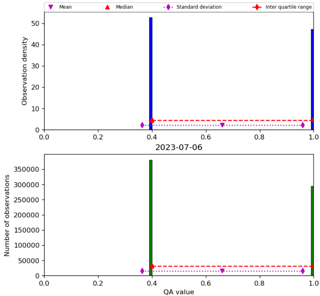
Figure 22: Histogram of “QA value” for 2023-07-05 to 2023-07-07
