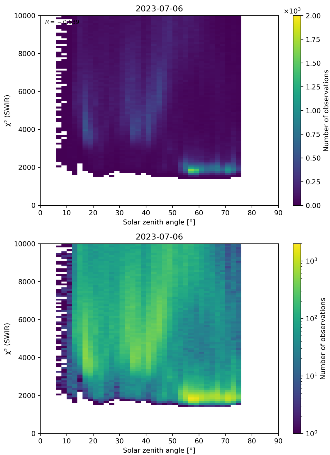
Figure 95: Scatter density plot of “Solar zenith angle” against “ \chi^2 (SWIR)” for 2023-07-05 to 2023-07-07.
