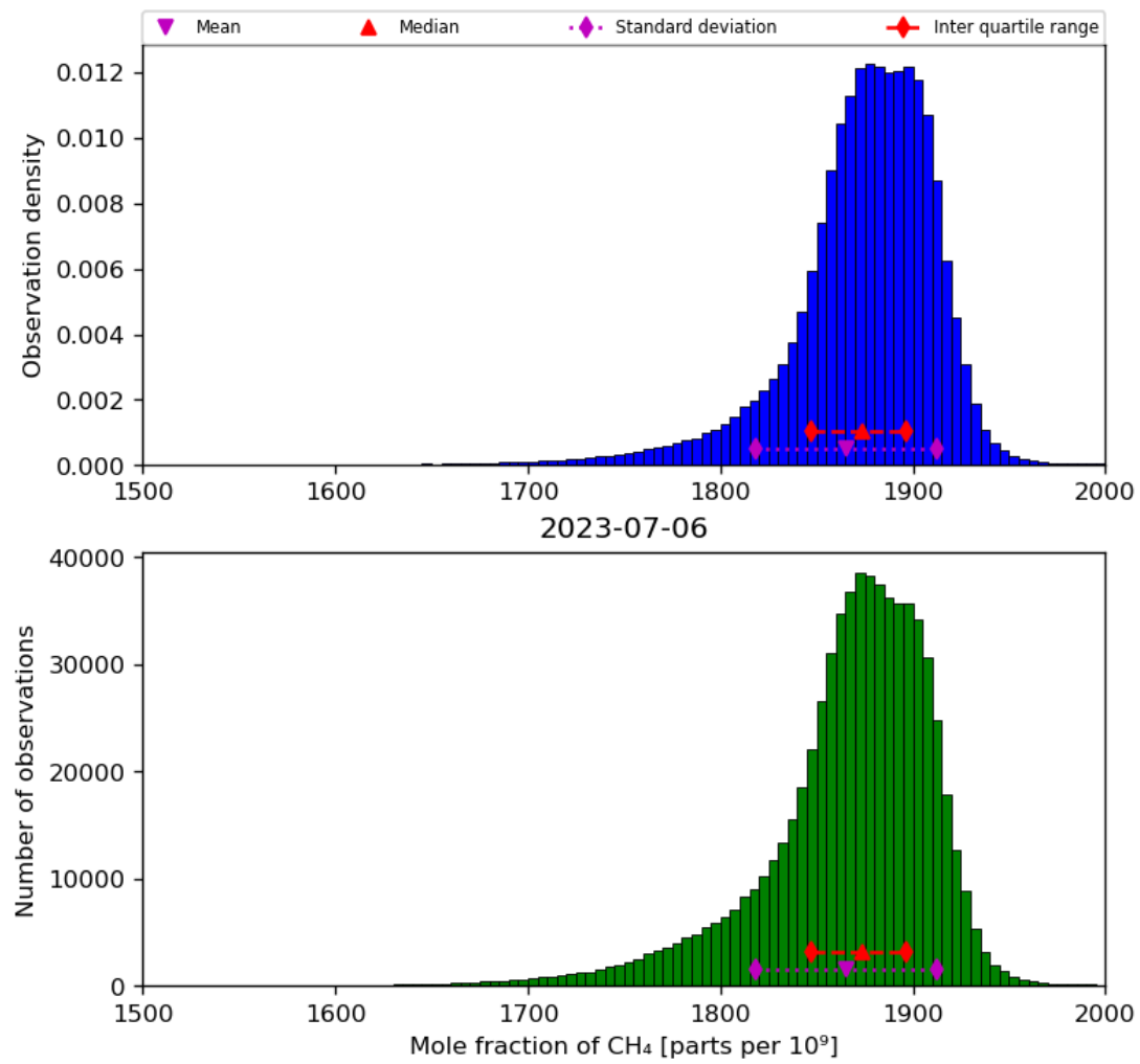
Figure 23: Histogram of “Mole fraction of CH 4 ” for 2023-07-05 to 2023-07-07
