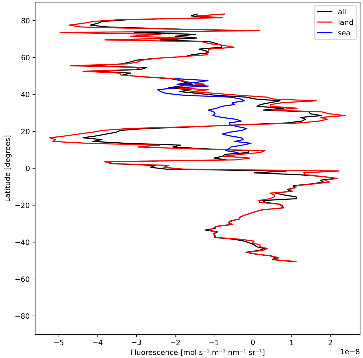
Figure 21: Zonal average of “Fluorescence” for 2023-07-05 to 2023-07-07.
