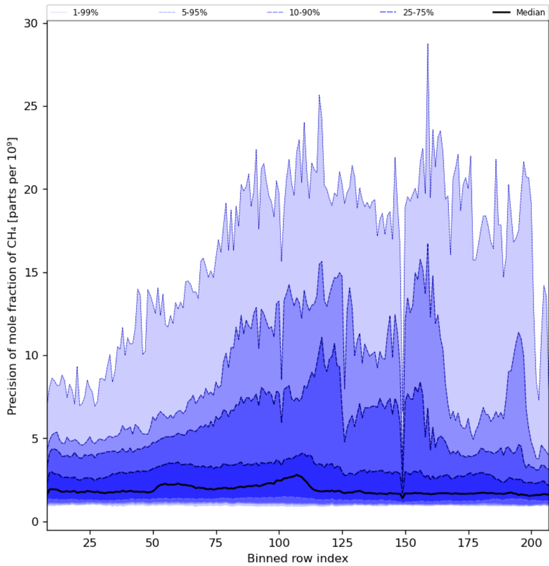
Figure 35: Along track statistics of “Precision of mole fraction of CH 4 ” for 2023-07-05 to 2023-07-07
