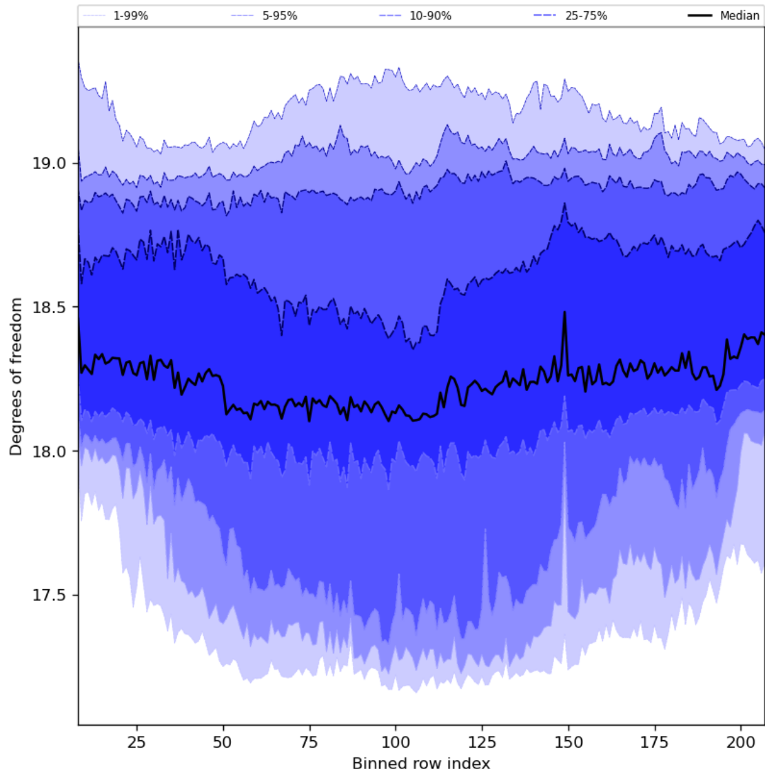
Figure 41: Along track statistics of “Degrees of freedom” for 2023-07-05 to 2023-07-07
