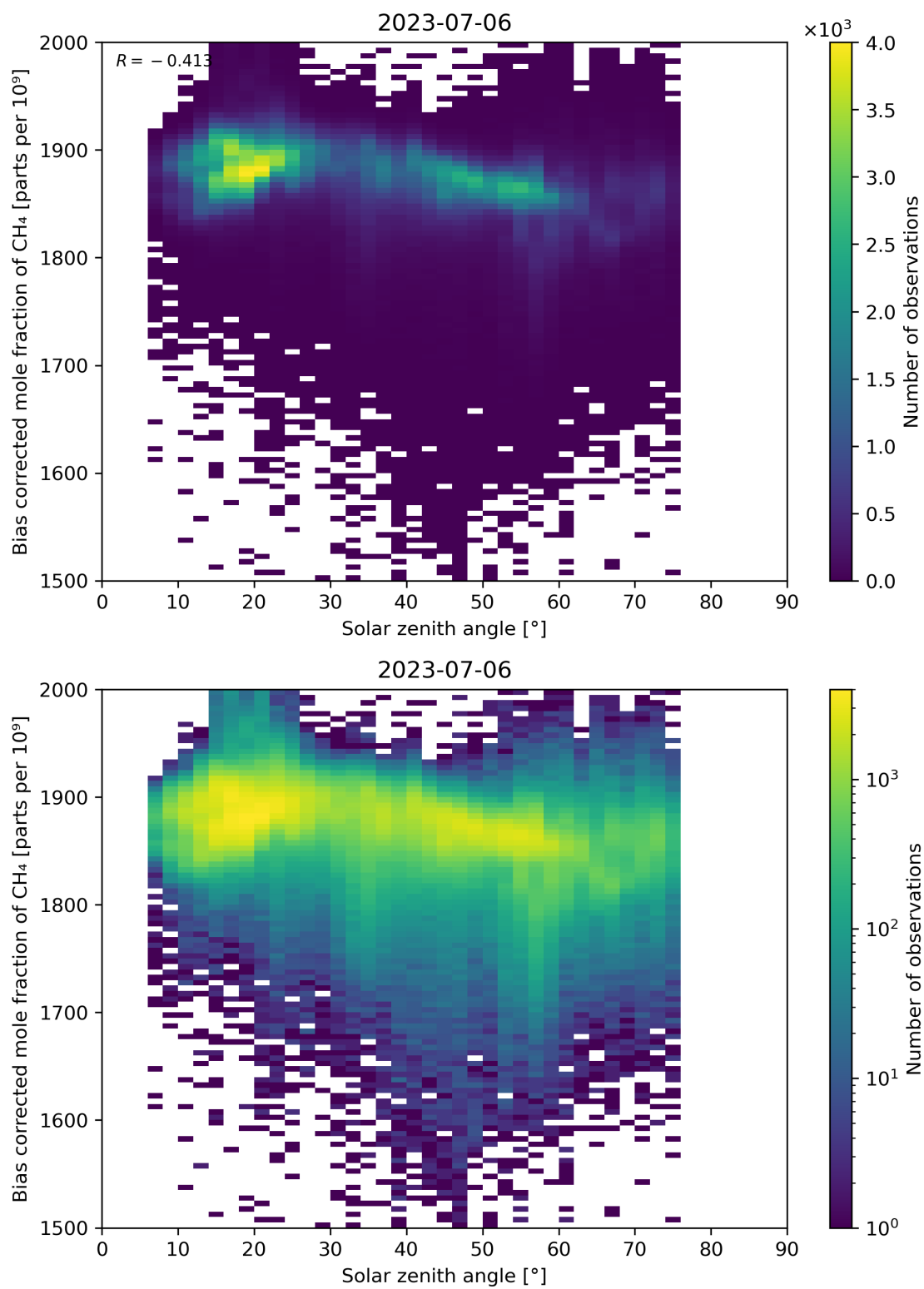
Figure 100: Scatter density plot of “Solar zenith angle” against “Bias corrected mole fraction of \text{CH}_4 ” for 2023-07-05 to 2023-07-07.
