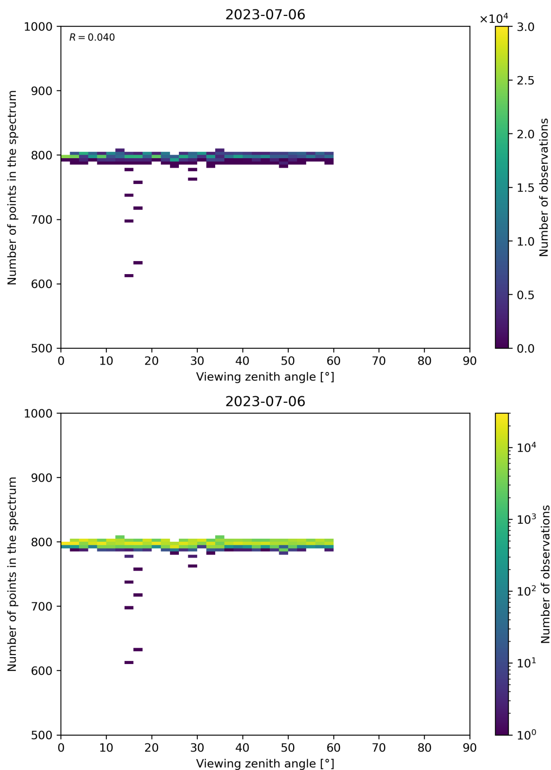
Figure 114: Scatter density plot of “Viewing zenith angle” against “Number of points in the spectrum” for 2023-07-05 to 2023-07-07.
