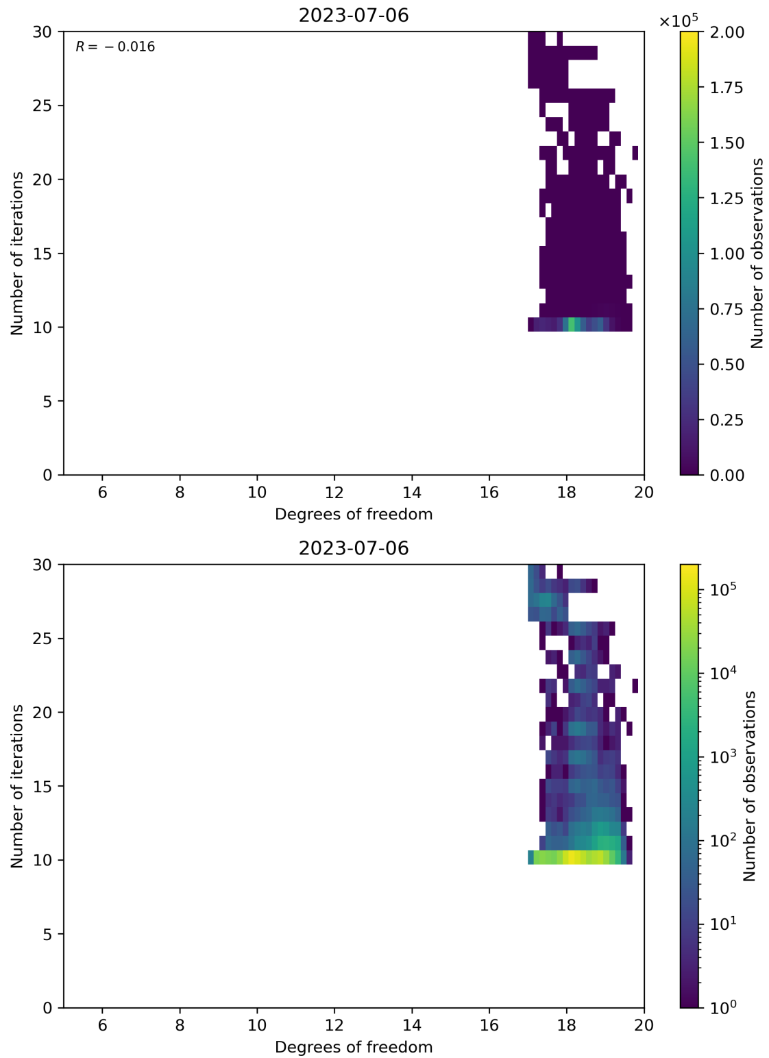
Figure 52: Scatter density plot of “Degrees of freedom” against “Number of iterations” for 2023-07-05 to 2023-07-07.
