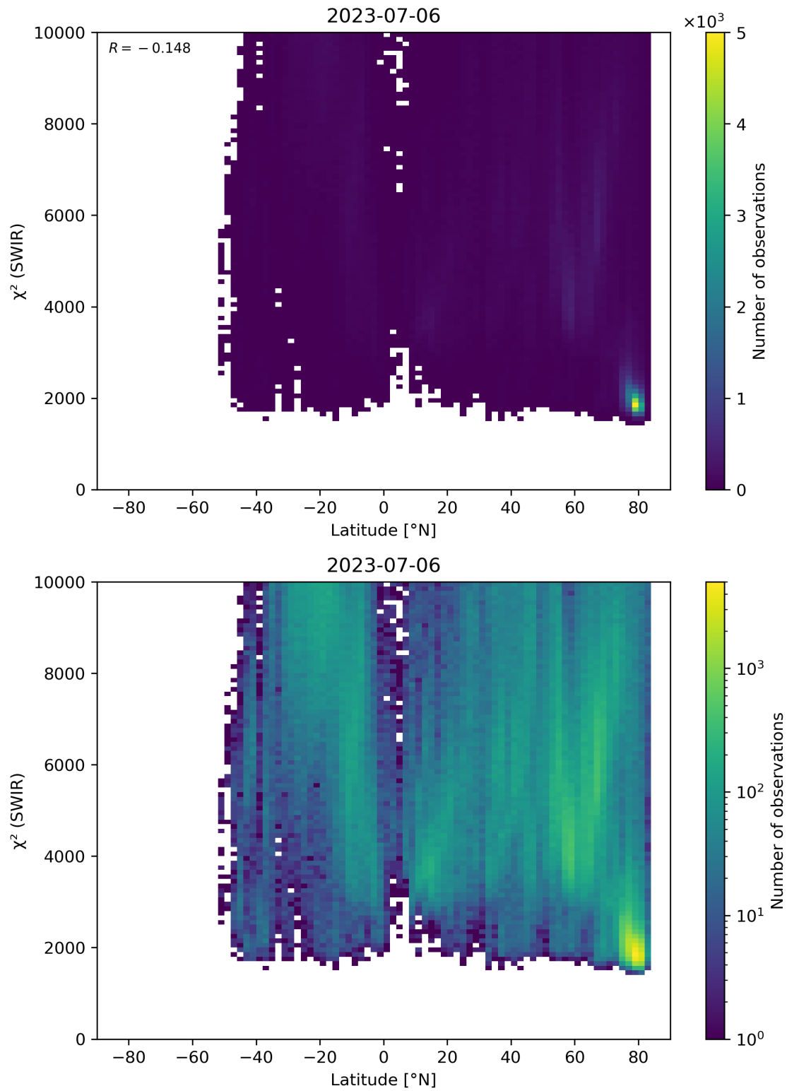
Figure 54: Scatter density plot of “Latitude” against “ \chi^2 (SWIR)” for 2023-07-05 to 2023-07-07.
