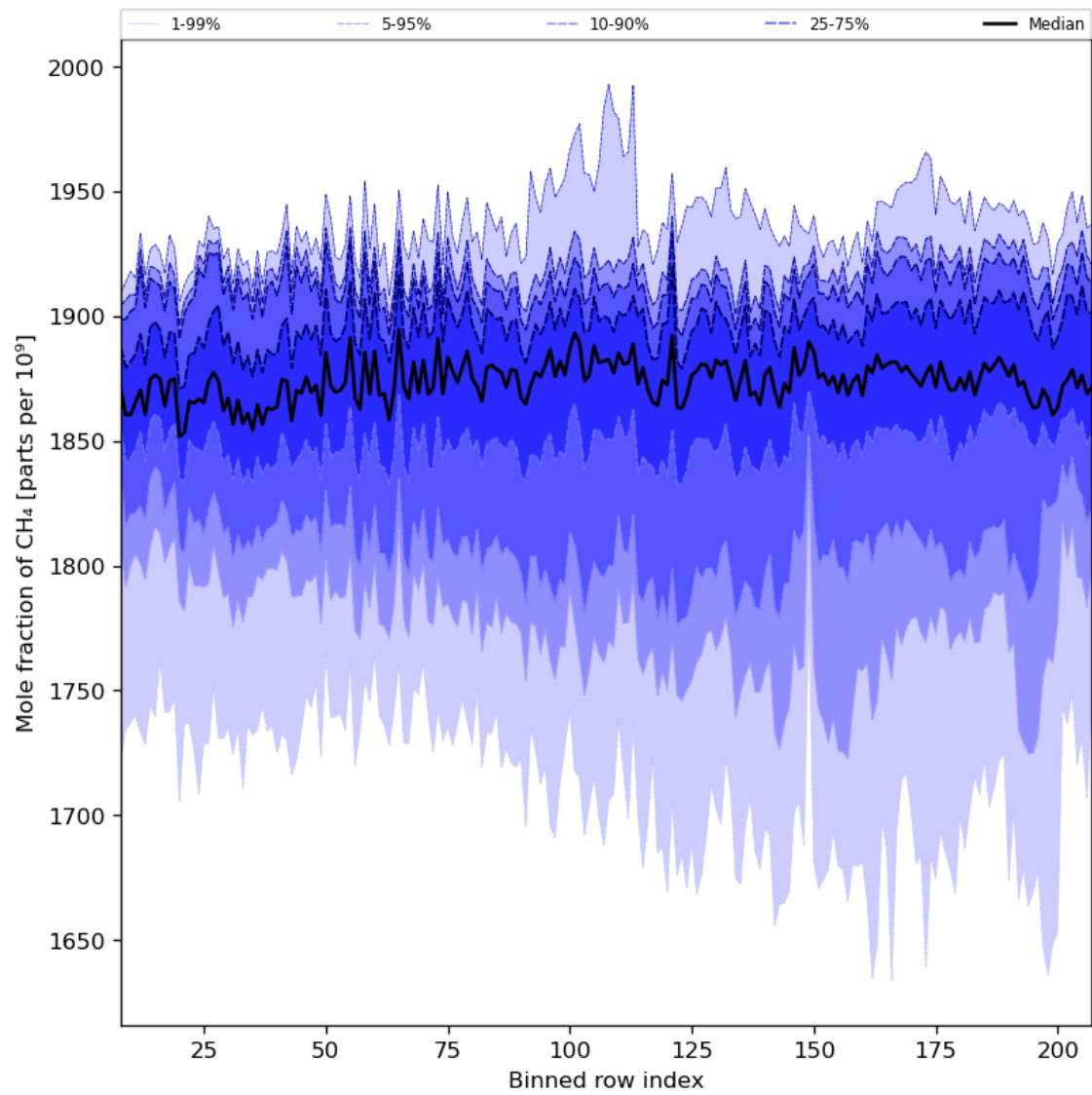
Figure 34: Along track statistics of “Mole fraction of CH 4 ” for 2023-07-05 to 2023-07-07
