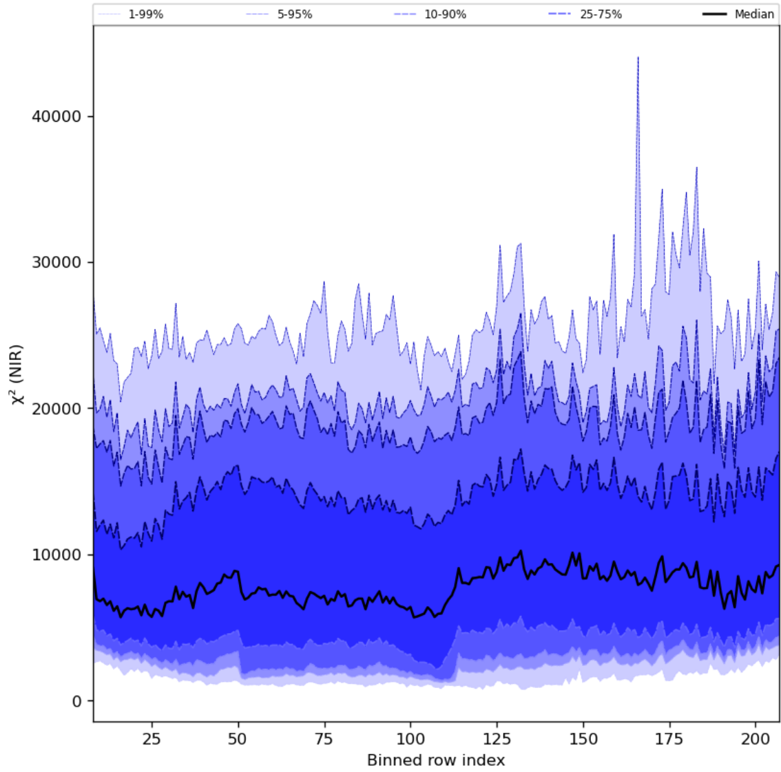
Figure 40: Along track statistics of “ \chi^2 (NIR)” for 2023-07-05 to 2023-07-07
