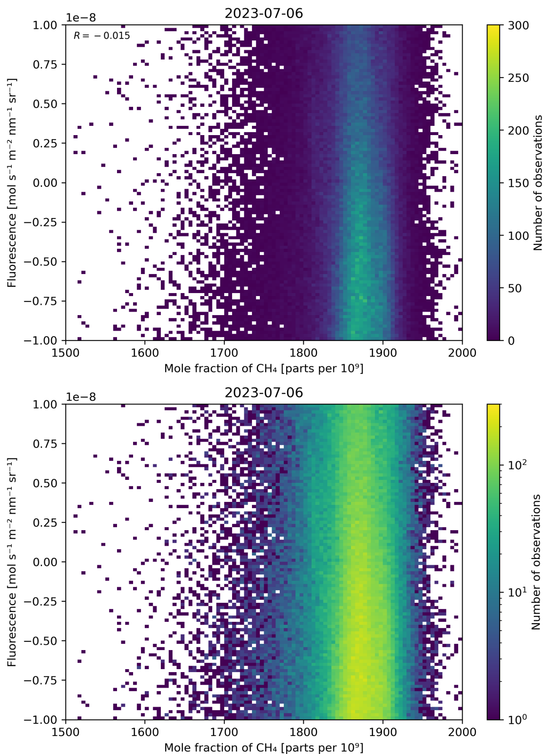
Figure 73: Scatter density plot of “Mole fraction of \text{CH}_4 ” against “Fluorescence” for 2023-07-05 to 2023-07-07.
