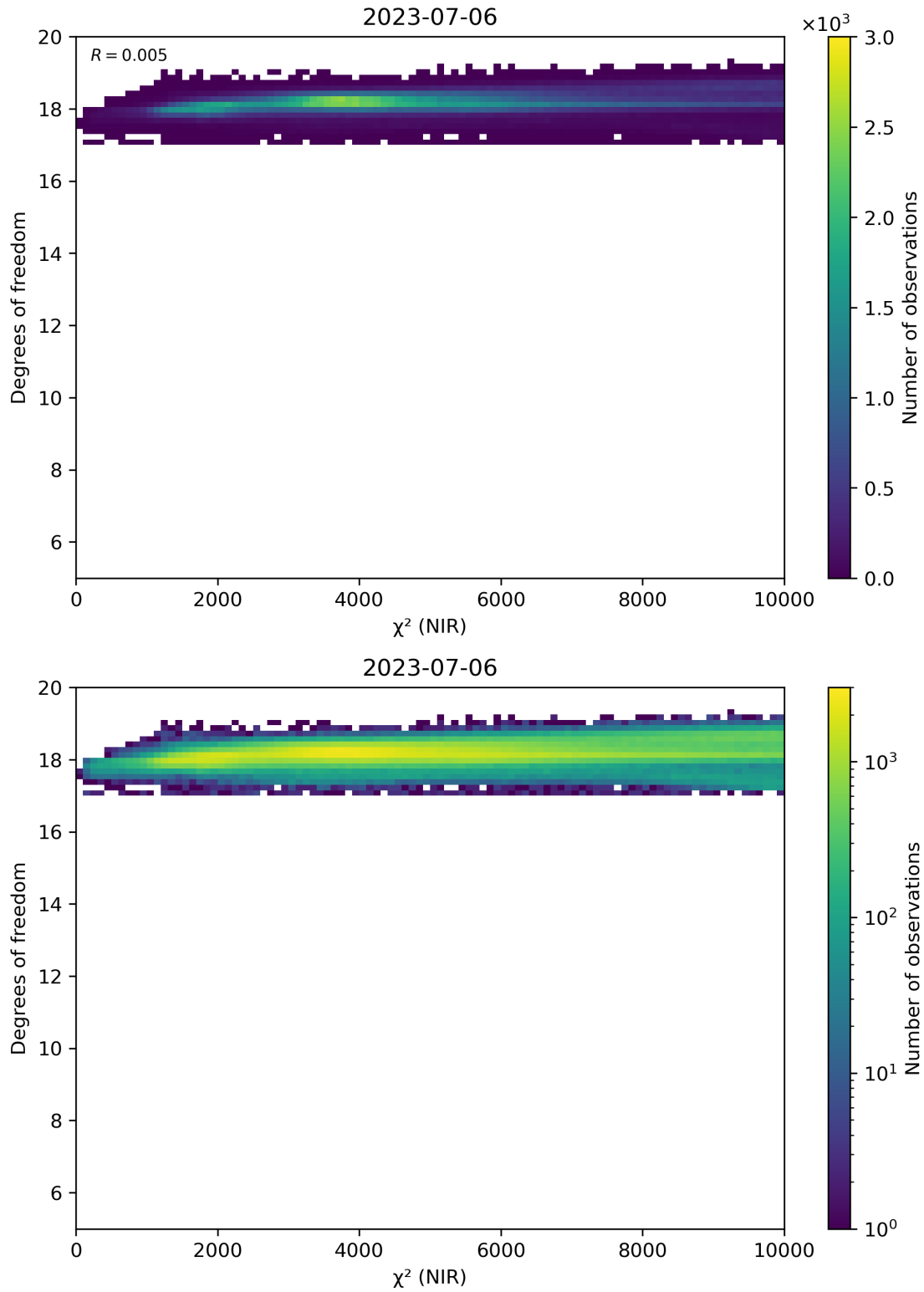
Figure 44: Scatter density plot of “ \chi^2 (NIR)” against “Degrees of freedom” for 2023-07-05 to 2023-07-07.
