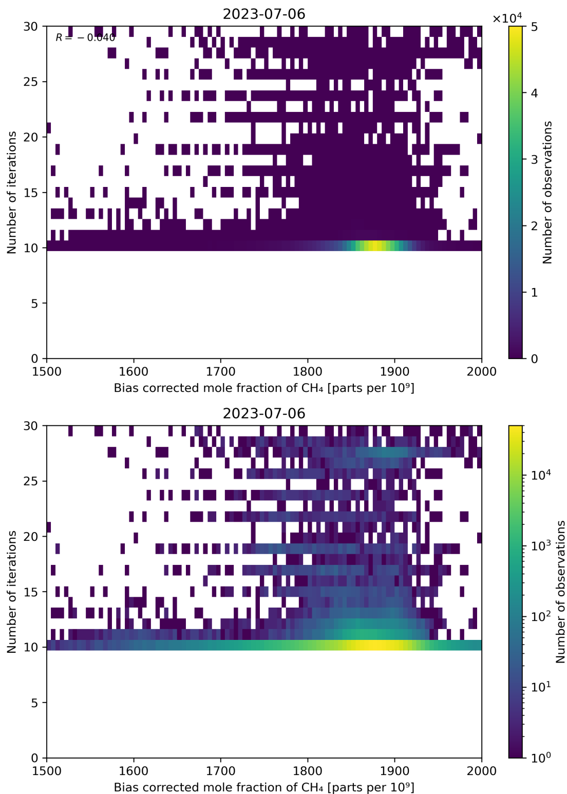
Figure 67: Scatter density plot of “Bias corrected mole fraction of CH 4 ” against “Number of iterations” for 2023-07-05 to 2023-07-07.
