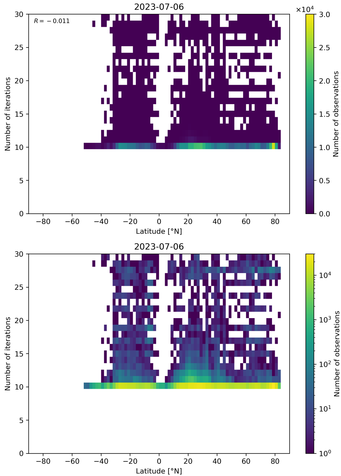
Figure 60: Scatter density plot of “Latitude” against “Number of iterations” for 2023-07-05 to 2023-07-07.
