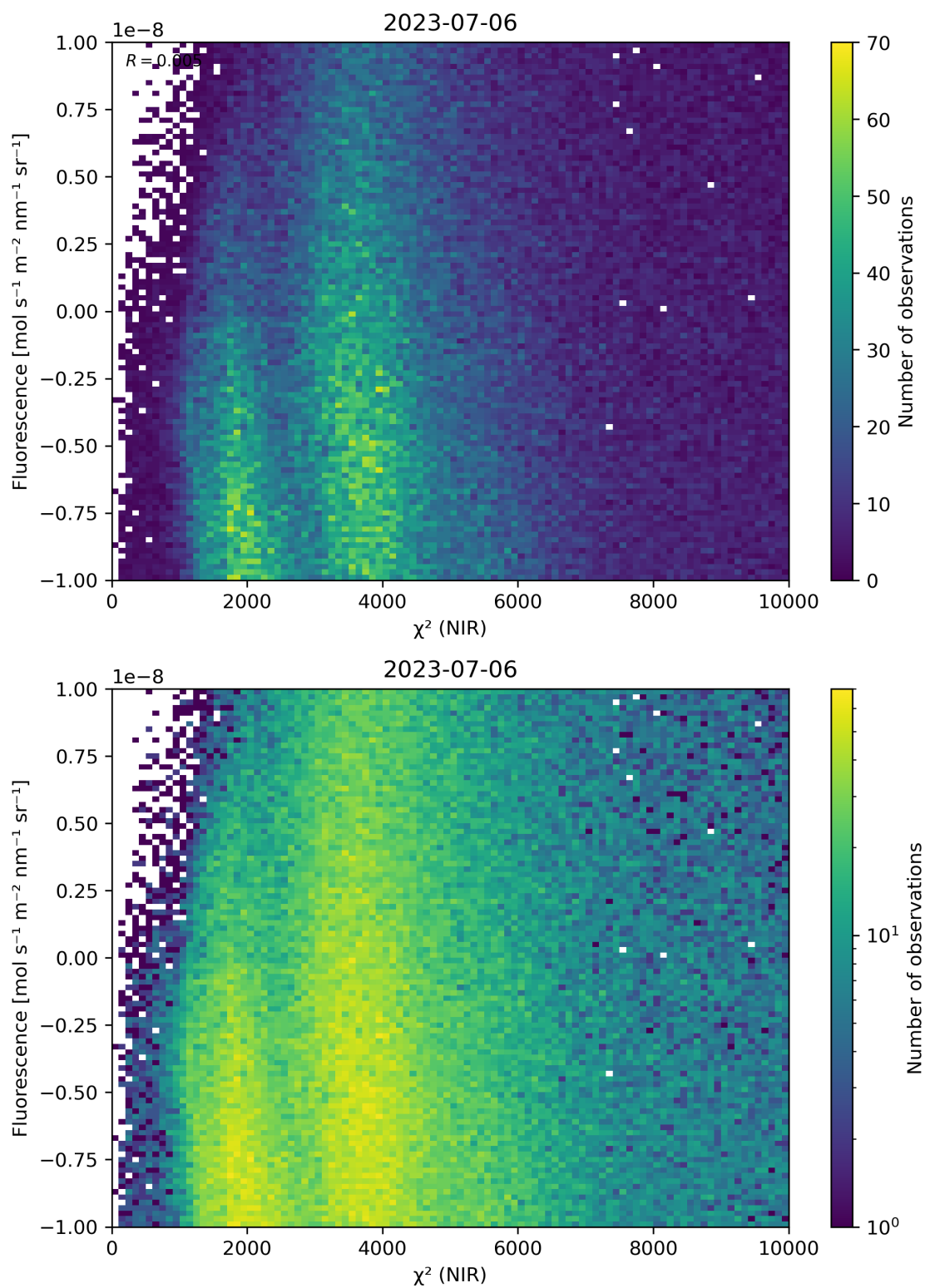
Figure 45: Scatter density plot of “ \chi^2 (NIR)” against “Fluorescence” for 2023-07-05 to 2023-07-07.
