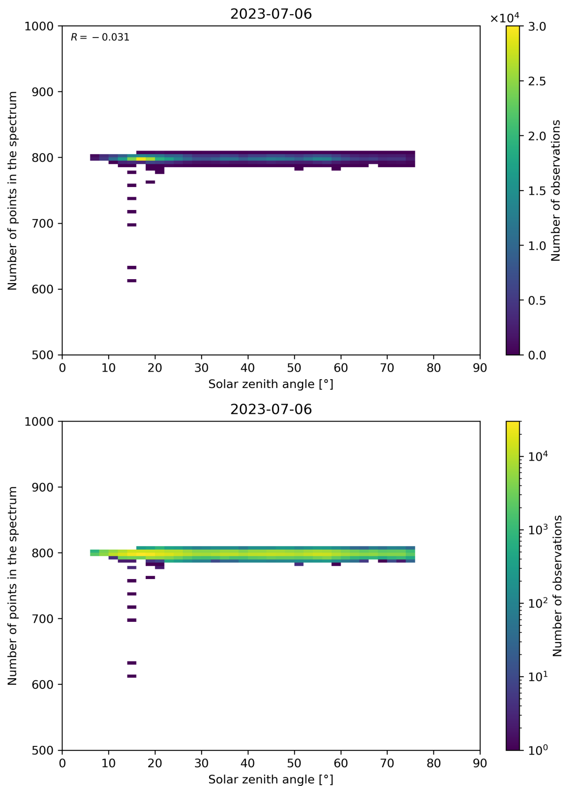
Figure 103: Scatter density plot of “Solar zenith angle” against “Number of points in the spectrum” for 2023-07-05 to 2023-07-07.
