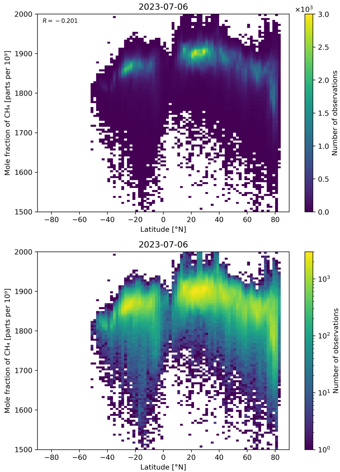
Figure 57: Scatter density plot of “Latitude” against “Mole fraction of CH 4 ” for 2023-07-05 to 2023-07-07.
