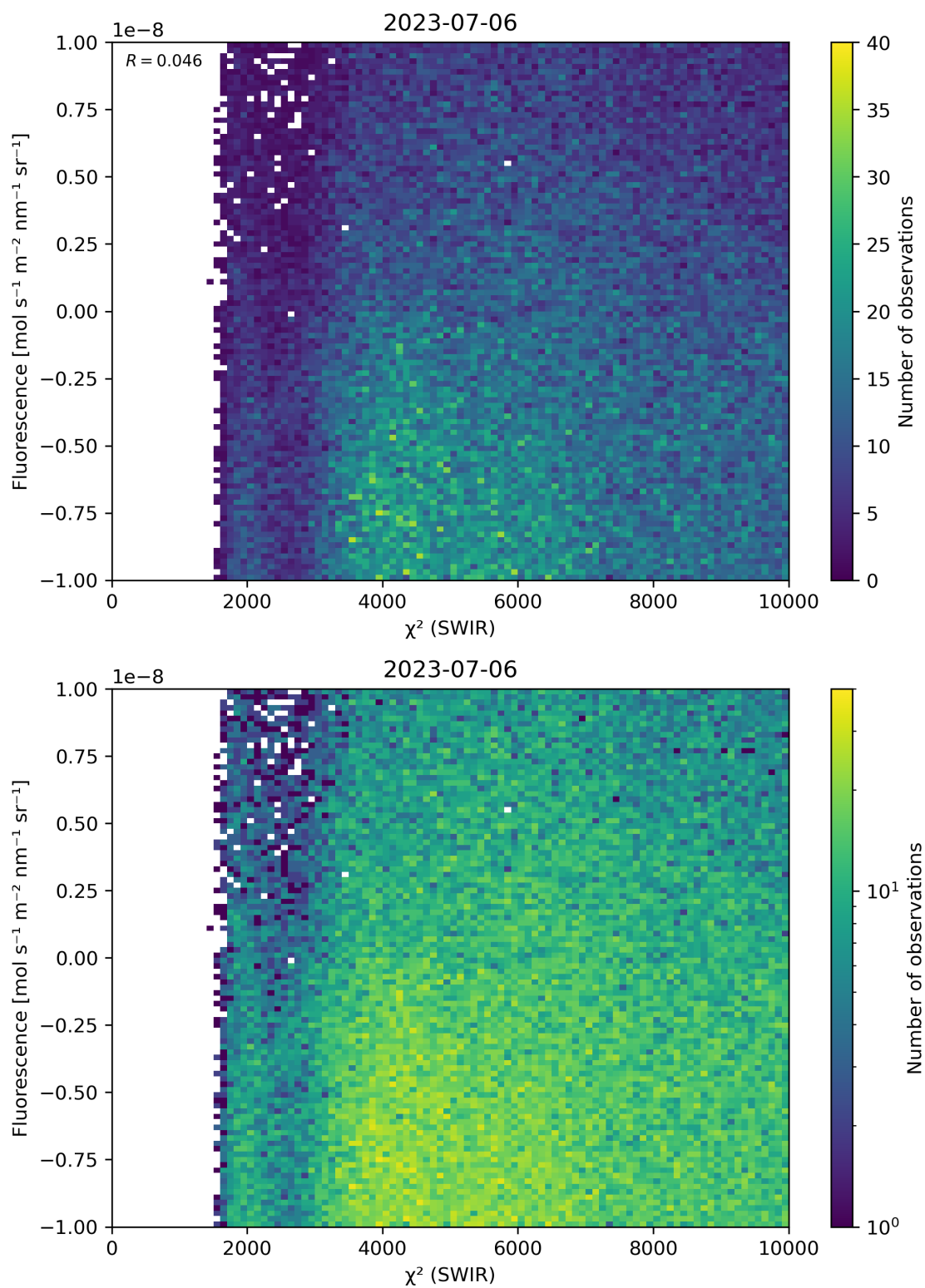
Figure 49: Scatter density plot of “ \chi^2 (SWIR)” against “Fluorescence” for 2023-07-05 to 2023-07-07.
