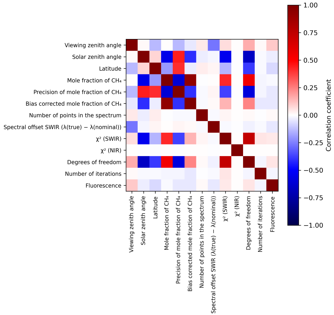
Figure 2: Map of correlation matrix for 2023-07-05 to 2023-07-07.
