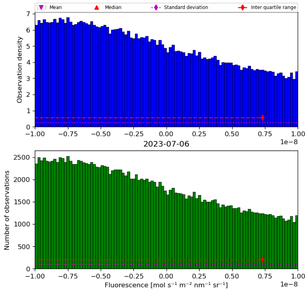
Figure 32: Histogram of “Fluorescence” for 2023-07-05 to 2023-07-07
