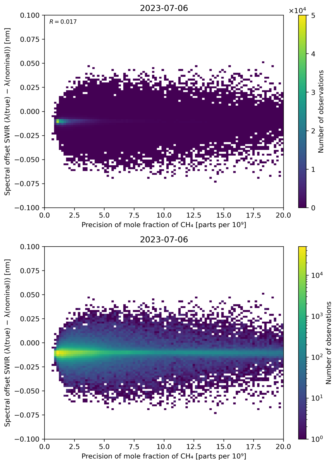
Figure 85: Scatter density plot of “Precision of mole fraction of CH 4 ” against “Spectral offset SWIR ( \lambda(\text{true}) - \lambda(\text{nominal}) )” for 2023-07-05 to 2023-07-07.
