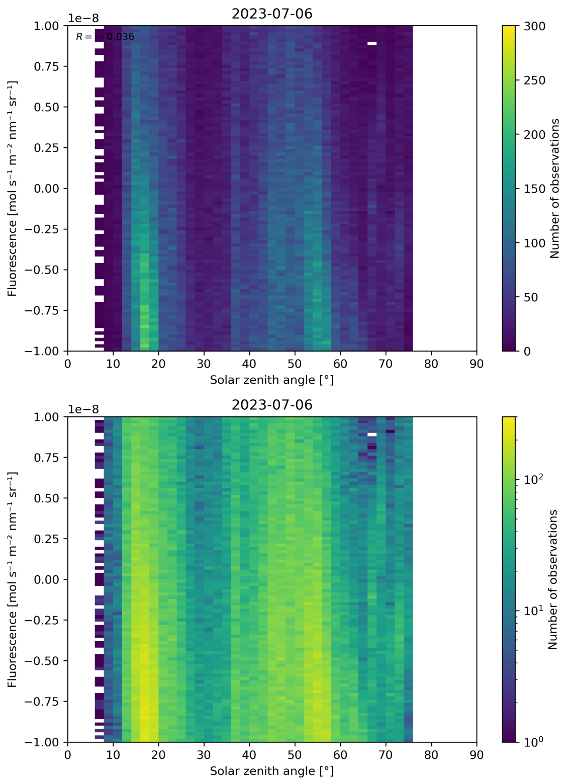
Figure 97: Scatter density plot of “Solar zenith angle” against “Fluorescence” for 2023-07-05 to 2023-07-07.
