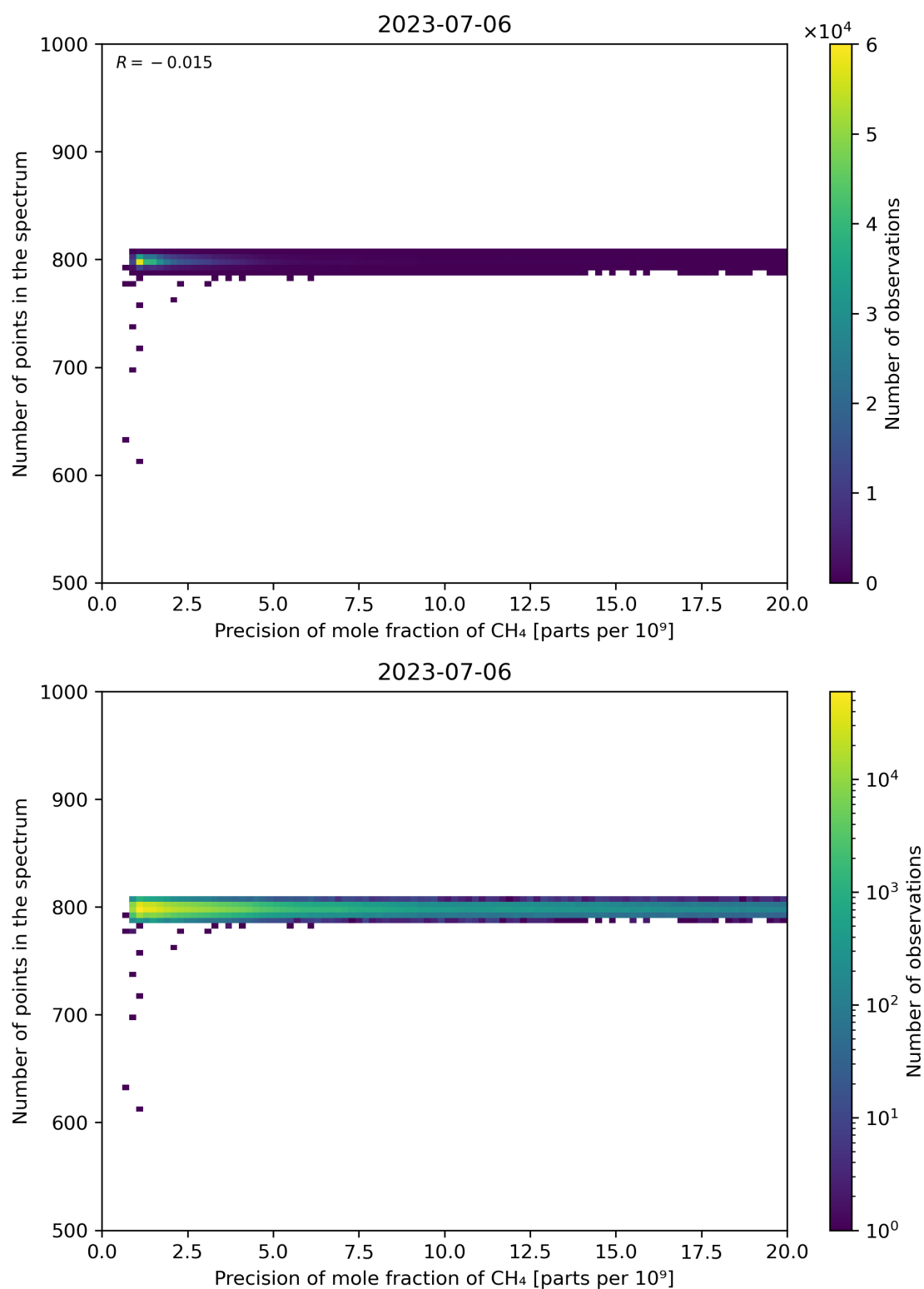
Figure 84: Scatter density plot of “Precision of mole fraction of CH 4 ” against “Number of points in the spectrum” for 2023-07-05 to 2023-07-07.
