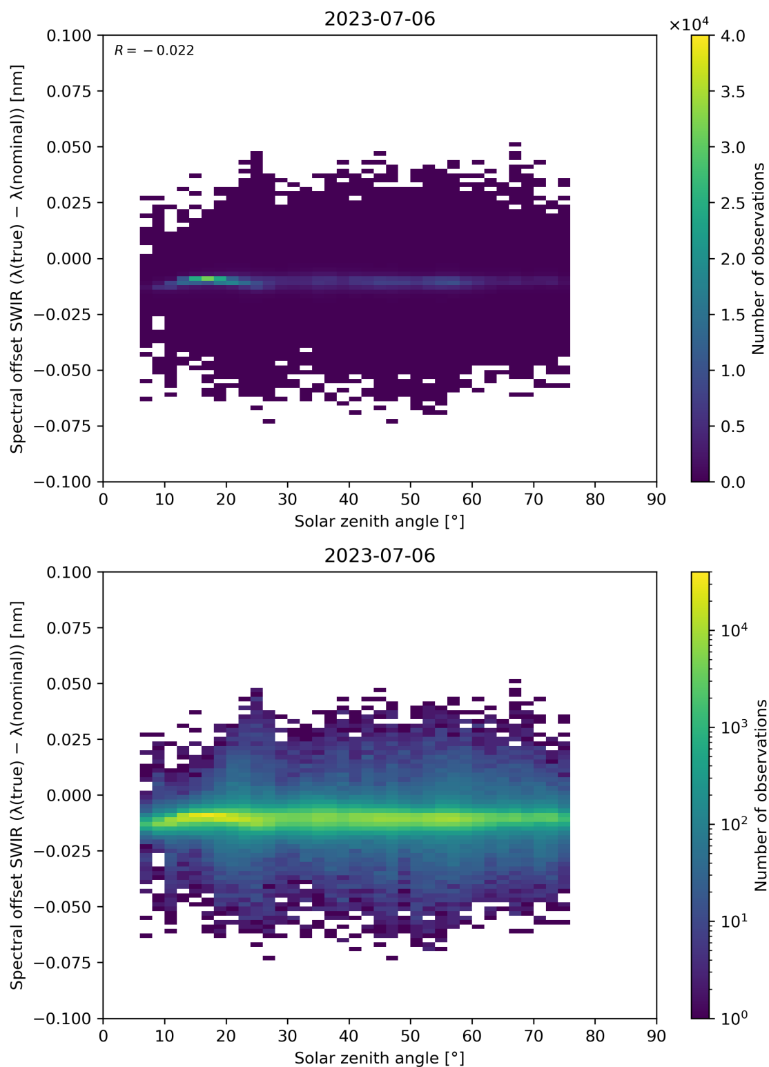
Figure 104: Scatter density plot of “Solar zenith angle” against “Spectral offset SWIR ( \lambda(\text{true}) - \lambda(\text{nominal}) )” for 2023-07-05 to 2023-07-07.
