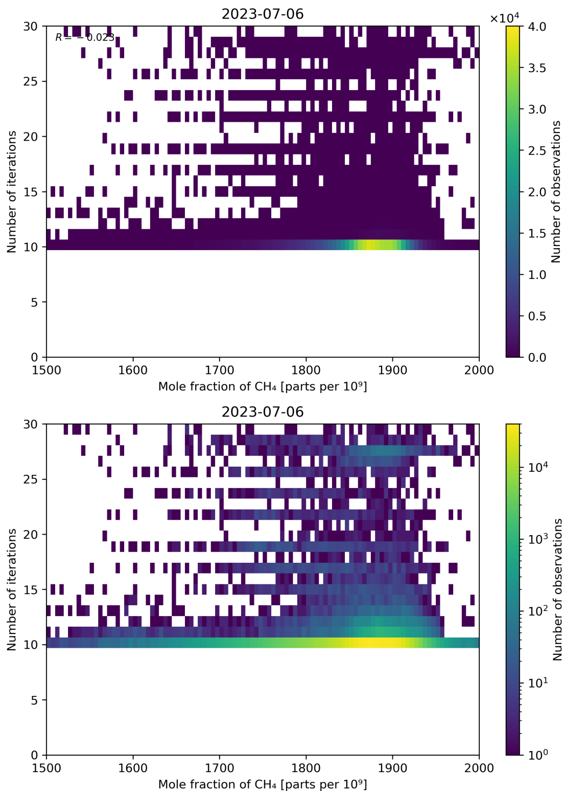
Figure 76: Scatter density plot of “Mole fraction of CH 4 ” against “Number of iterations” for 2023-07-05 to 2023-07-07.
