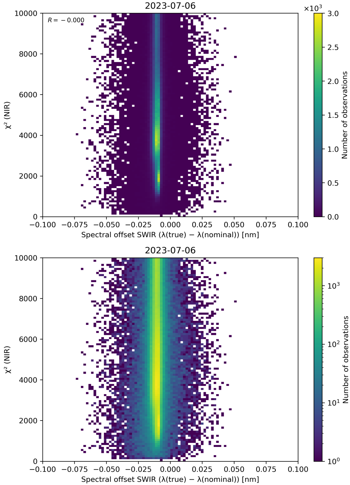
Figure 117: Scatter density plot of “Spectral offset SWIR ( \lambda(\text{true}) - \lambda(\text{nominal}) )” against “ \chi^2 (NIR)” for 2023-07-05 to 2023-07-07.
