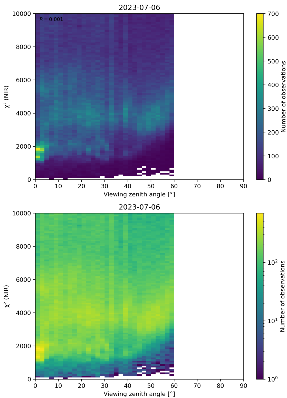
Figure 105: Scatter density plot of “Viewing zenith angle” against “ \chi^2 (NIR)” for 2023-07-05 to 2023-07-07.
