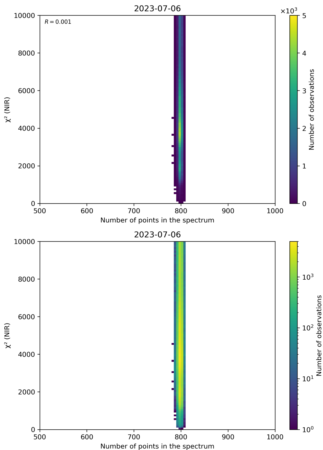
Figure 88: Scatter density plot of “Number of points in the spectrum” against “ \chi^2 (NIR)” for 2023-07-05 to 2023-07-07.
