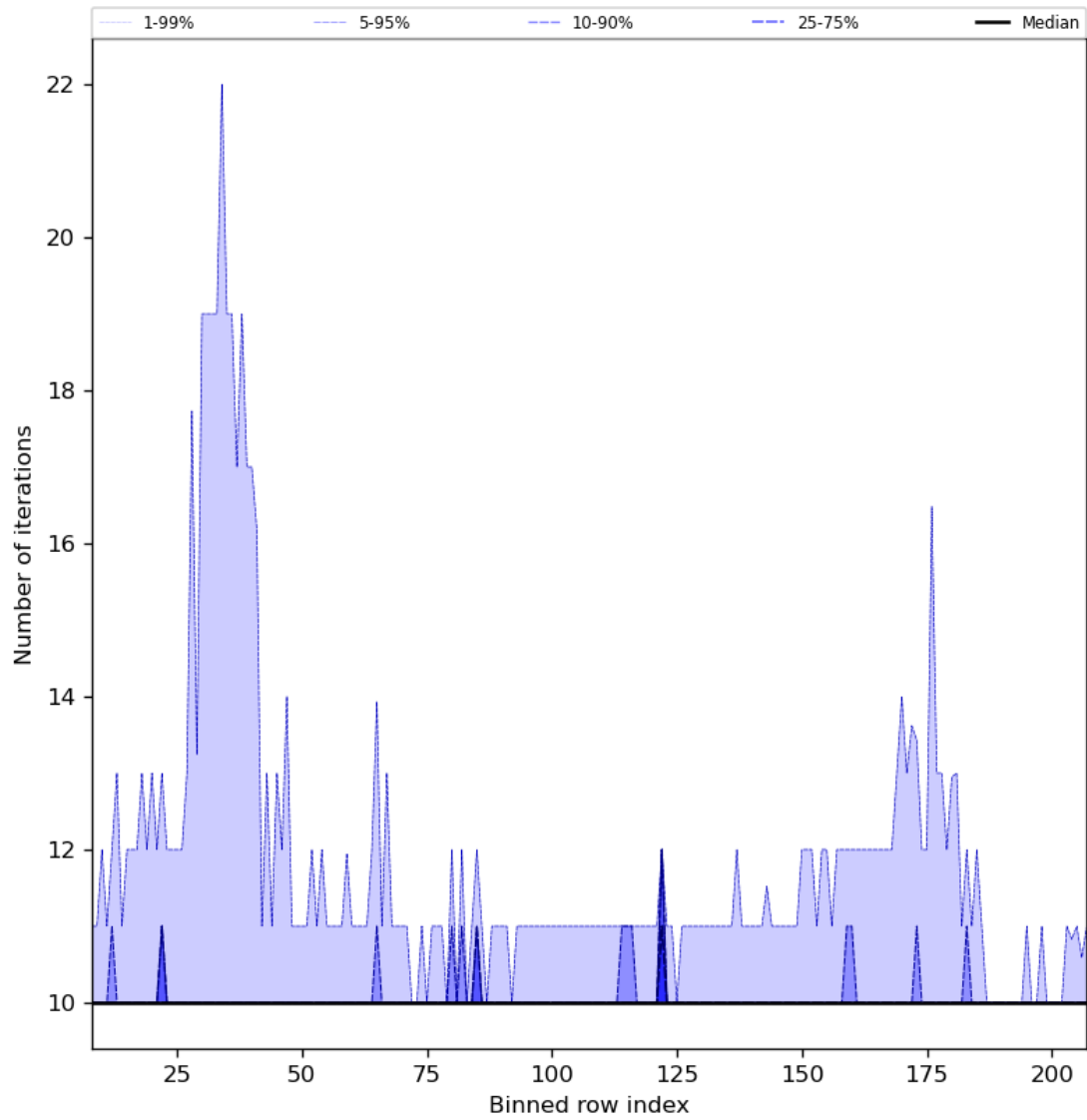
Figure 42: Along track statistics of “Number of iterations” for 2023-07-05 to 2023-07-07
