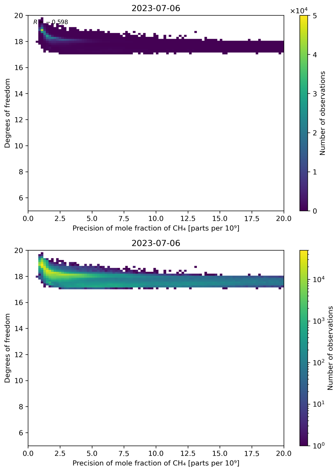
Figure 80: Scatter density plot of “Precision of mole fraction of CH 4 ” against “Degrees of freedom” for 2023-07-05 to 2023-07-07.
