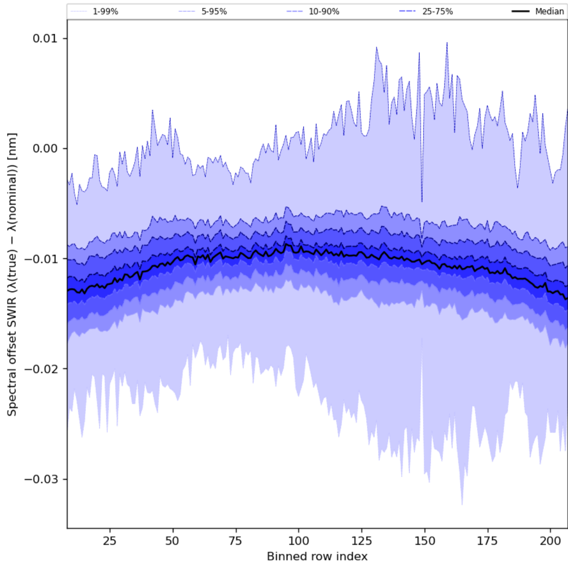
Figure 38: Along track statistics of “Spectral offset SWIR ( \lambda(\text{true}) - \lambda(\text{nominal}) )” for 2023-07-05 to 2023-07-07
