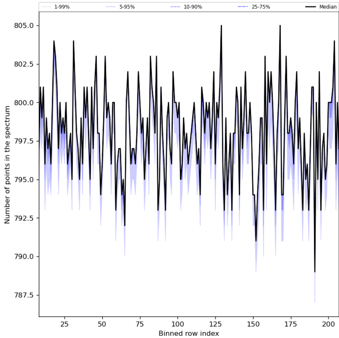
Figure 37: Along track statistics of “Number of points in the spectrum” for 2023-07-05 to 2023-07-07
