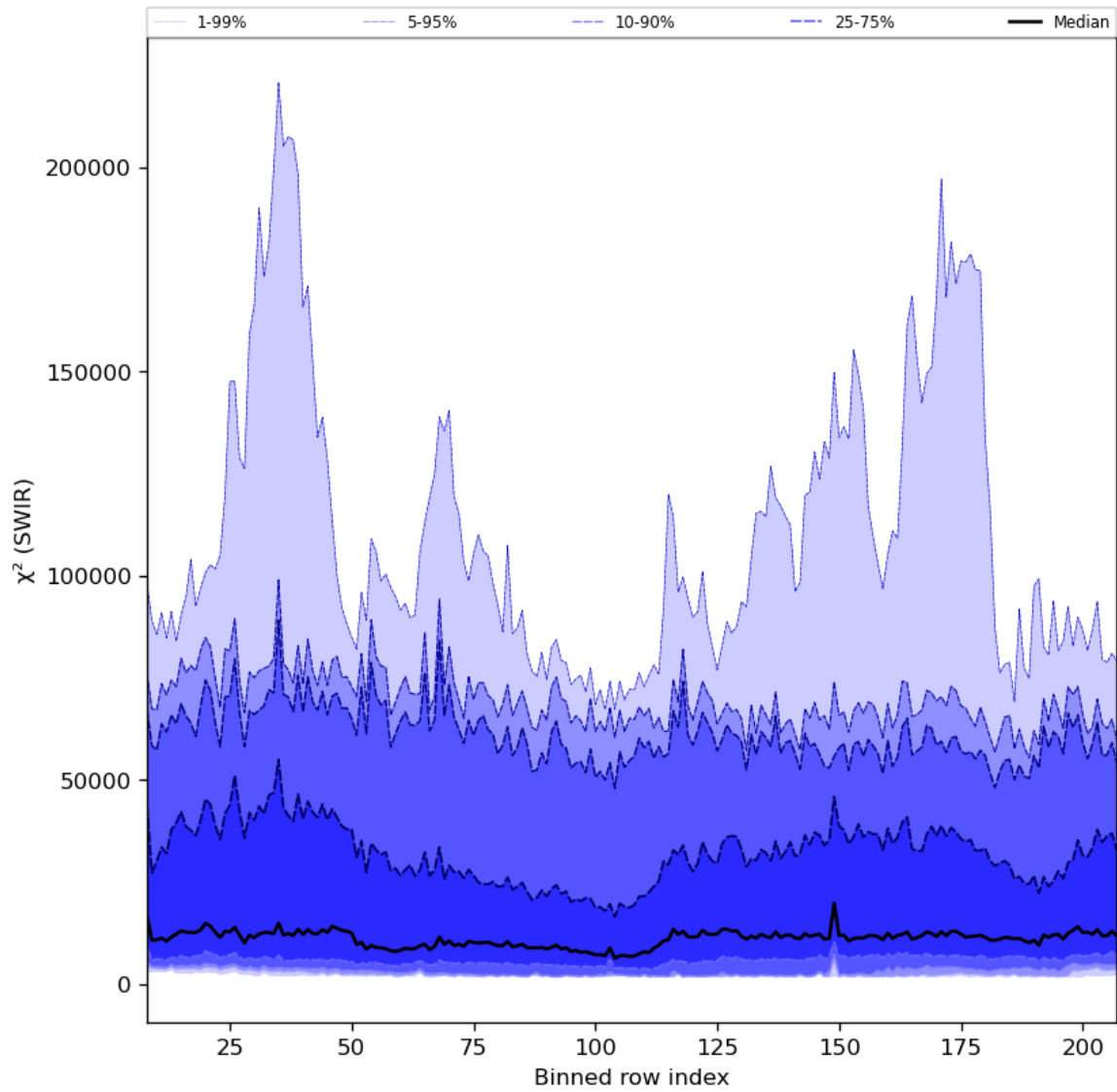
Figure 39: Along track statistics of “ \chi^2 (SWIR)” for 2023-07-05 to 2023-07-07
