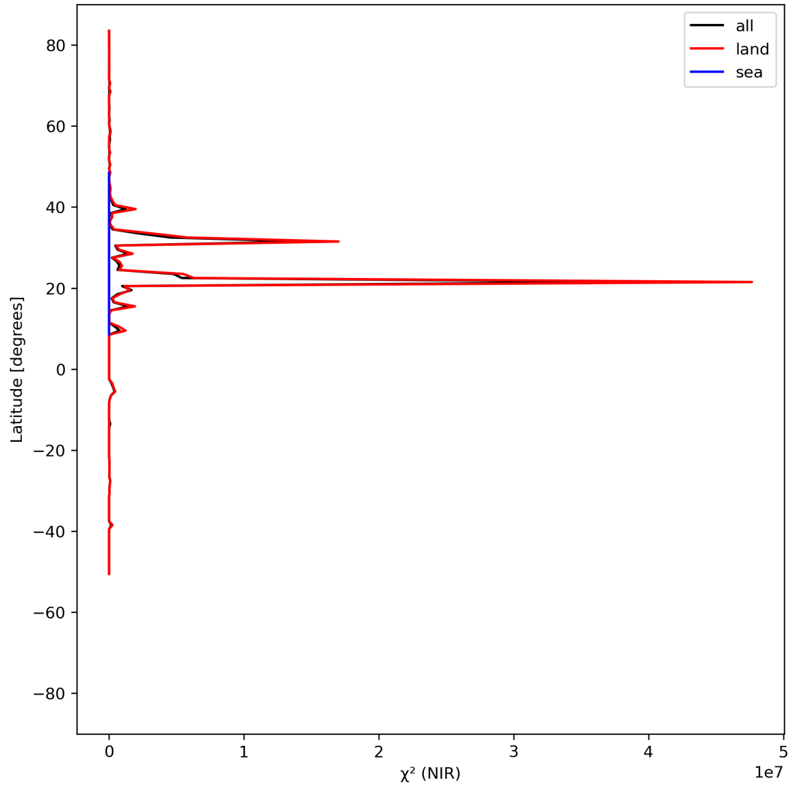
Figure 18: Zonal average of “ \chi^2 (NIR)” for 2023-07-05 to 2023-07-07.
