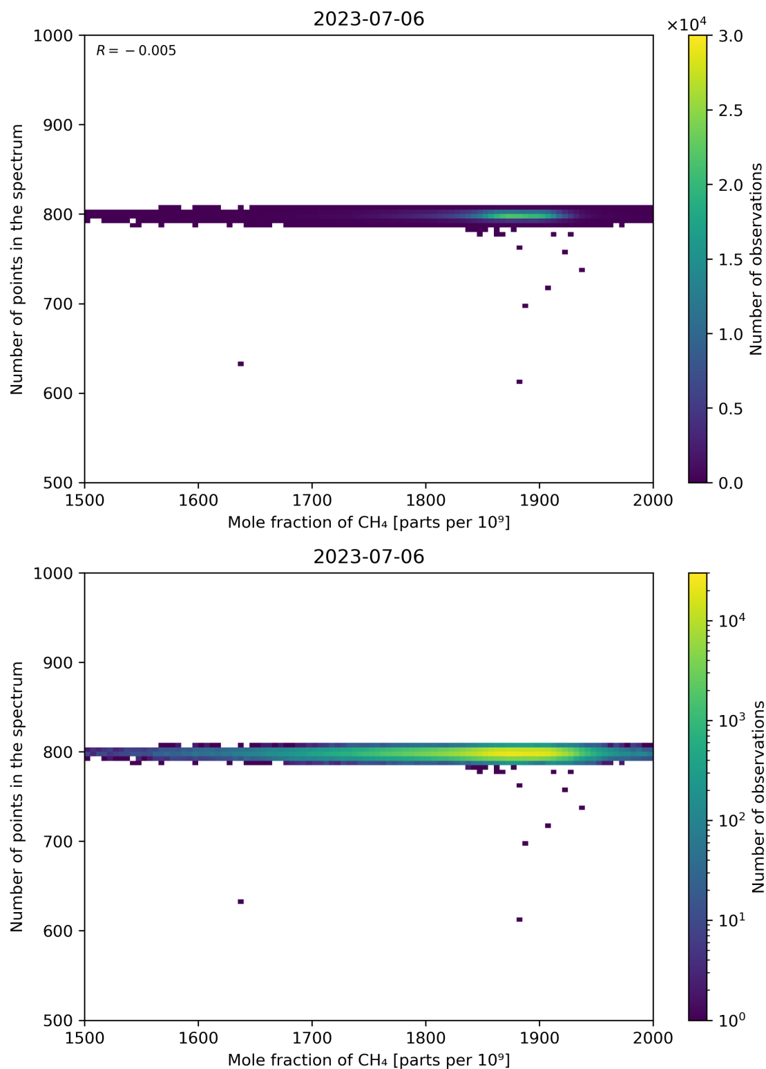
Figure 77: Scatter density plot of “Mole fraction of CH 4 ” against “Number of points in the spectrum” for 2023-07-05 to 2023-07-07.
