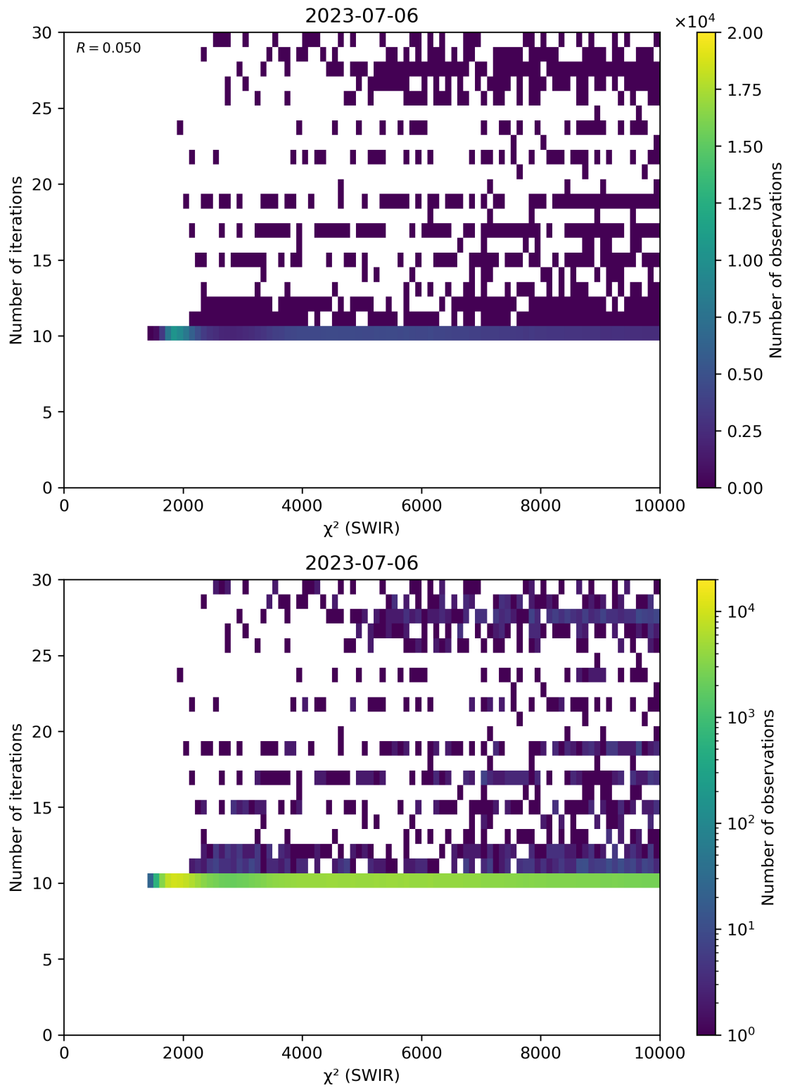
Figure 50: Scatter density plot of " \chi^2 (SWIR)" against "Number of iterations" for 2023-07-05 to 2023-07-07.
