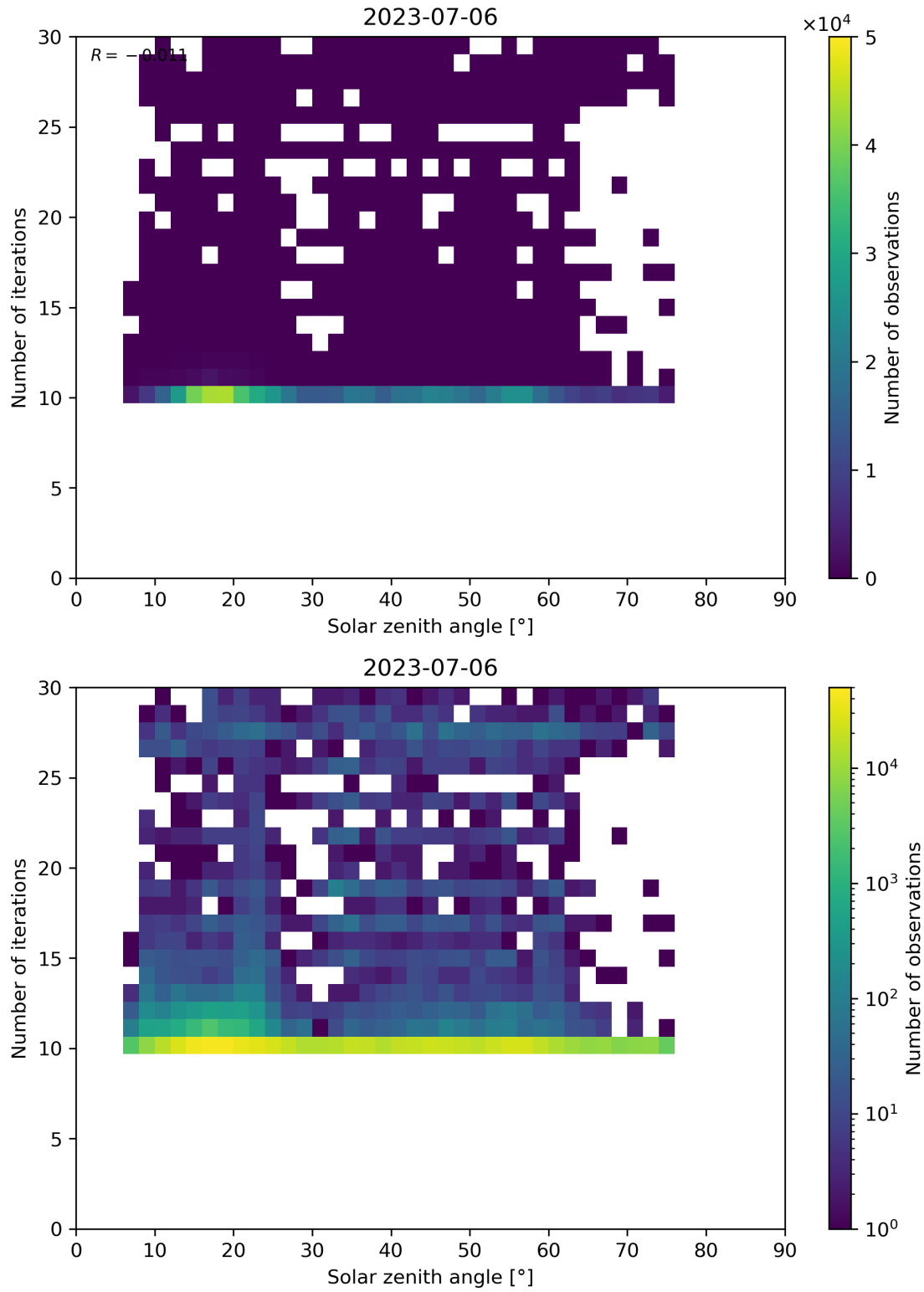
Figure 102: Scatter density plot of “Solar zenith angle” against “Number of iterations” for 2023-07-05 to 2023-07-07.
