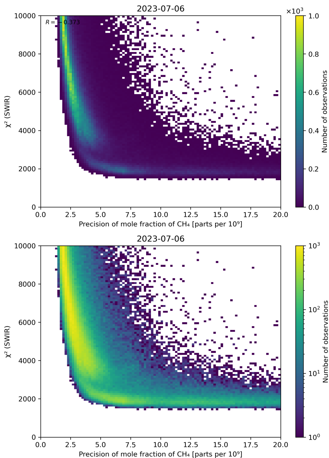
Figure 79: Scatter density plot of “Precision of mole fraction of CH 4 ” against “ \chi^2 (SWIR)” for 2023-07-05 to 2023-07-07.
