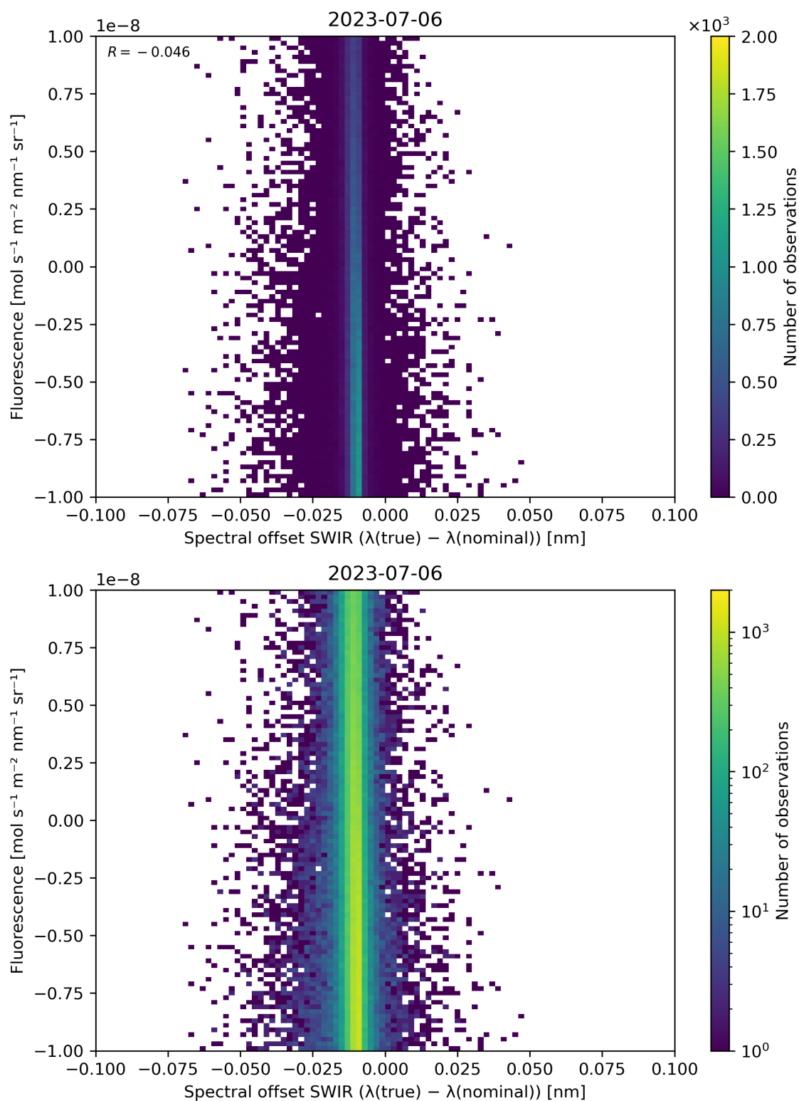
Figure 120: Scatter density plot of “Spectral offset SWIR ( \lambda(\text{true}) - \lambda(\text{nominal}) )” against “Fluorescence” for 2023-07-05 to 2023-07-07.
