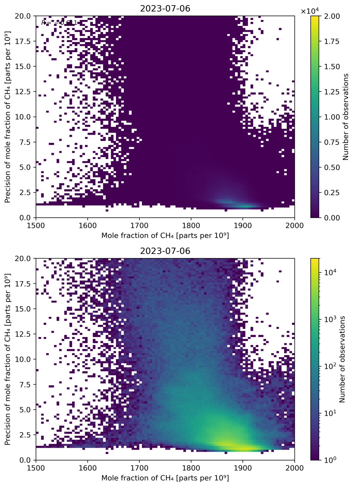
Figure 75: Scatter density plot of “Mole fraction of CH 4 ” against “Precision of mole fraction of CH 4 ” for 2023-07-05 to 2023-07-07.
