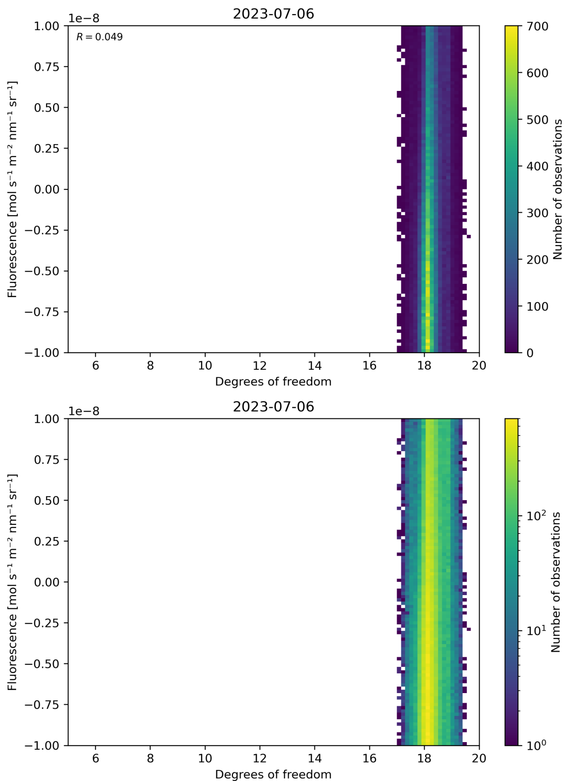
Figure 51: Scatter density plot of “Degrees of freedom” against “Fluorescence” for 2023-07-05 to 2023-07-07.
