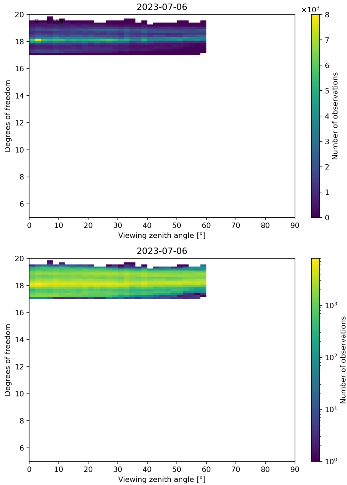
Figure 107: Scatter density plot of “Viewing zenith angle” against “Degrees of freedom” for 2023-07-05 to 2023-07-07.
