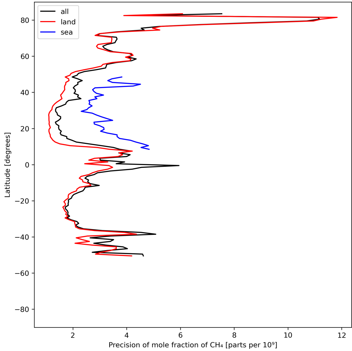
Figure 13: Zonal average of “Precision of mole fraction of CH 4 ” for 2023-07-05 to 2023-07-07.
