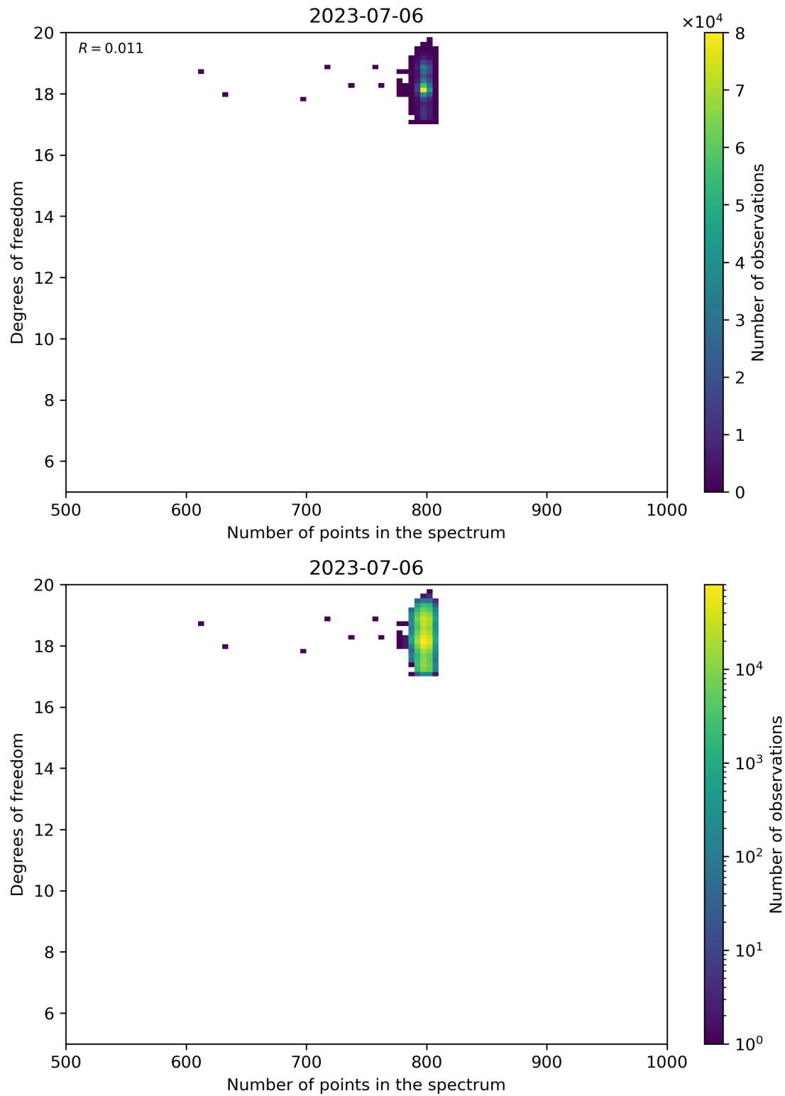
Figure 90: Scatter density plot of “Number of points in the spectrum” against “Degrees of freedom” for 2023-07-05 to 2023-07-07.
