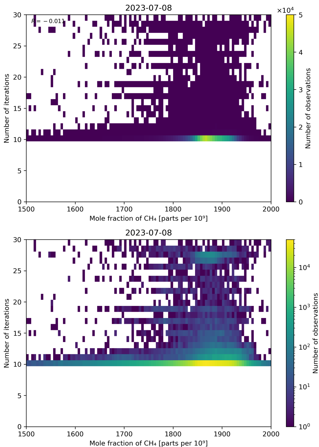
Figure 76: Scatter density plot of “Mole fraction of CH 4 ” against “Number of iterations” for 2023-07-08 to 2023-07-09.
