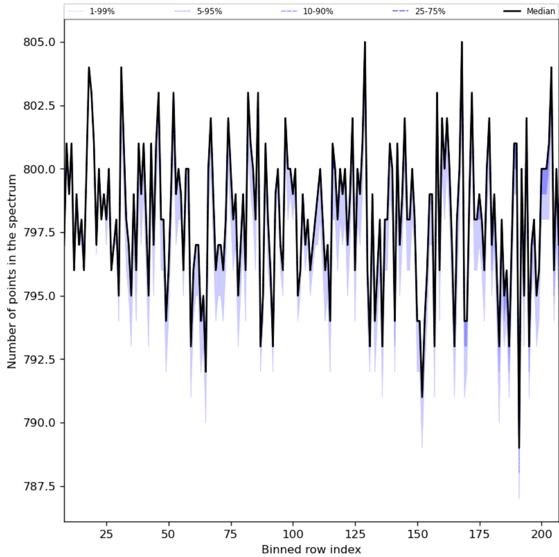
Figure 37: Along track statistics of “Number of points in the spectrum” for 2023-07-08 to 2023-07-09
