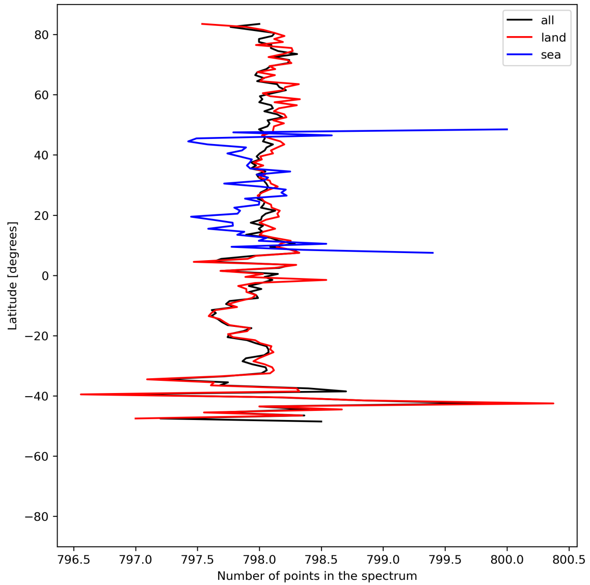
Figure 15: Zonal average of “Number of points in the spectrum” for 2023-07-08 to 2023-07-09.
