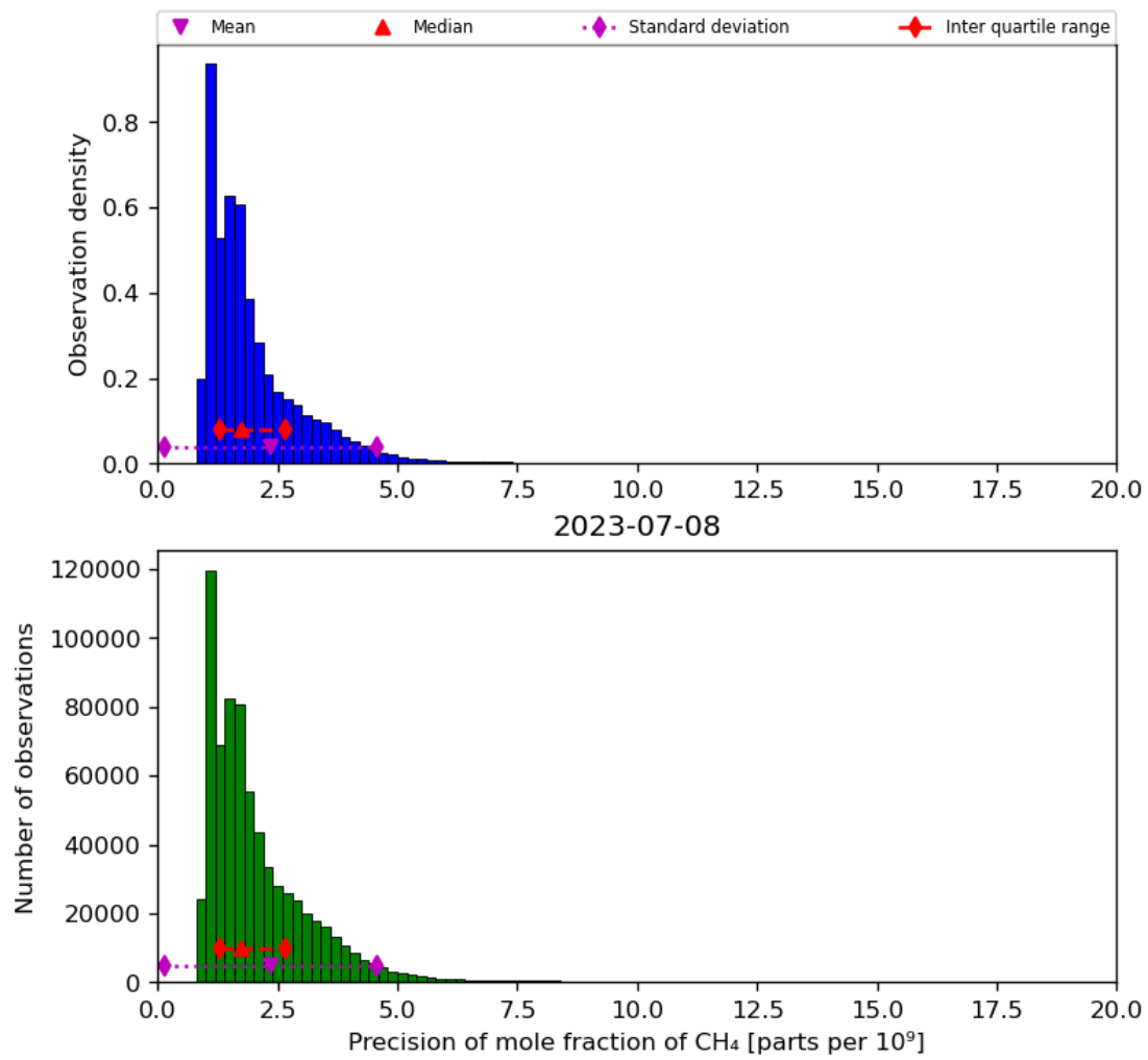
Figure 24: Histogram of “Precision of mole fraction of CH 4 ” for 2023-07-08 to 2023-07-09
