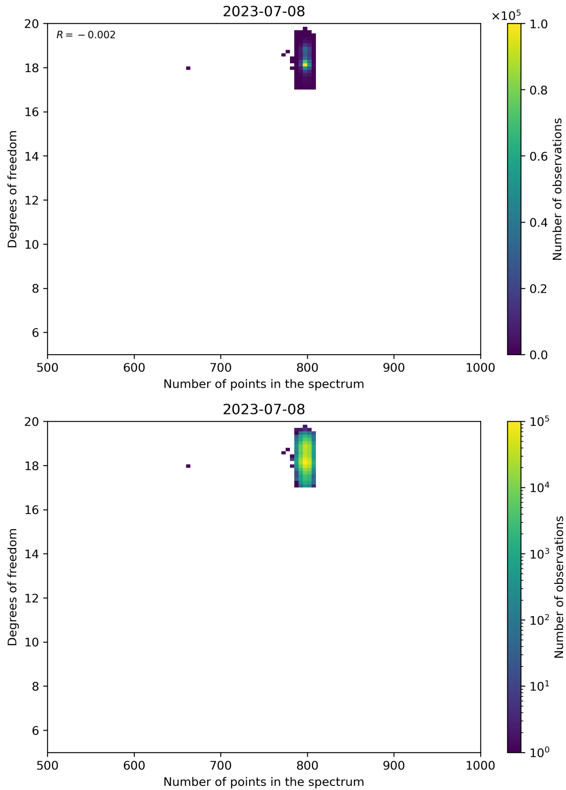
Figure 90: Scatter density plot of “Number of points in the spectrum” against “Degrees of freedom” for 2023-07-08 to 2023-07-09.
