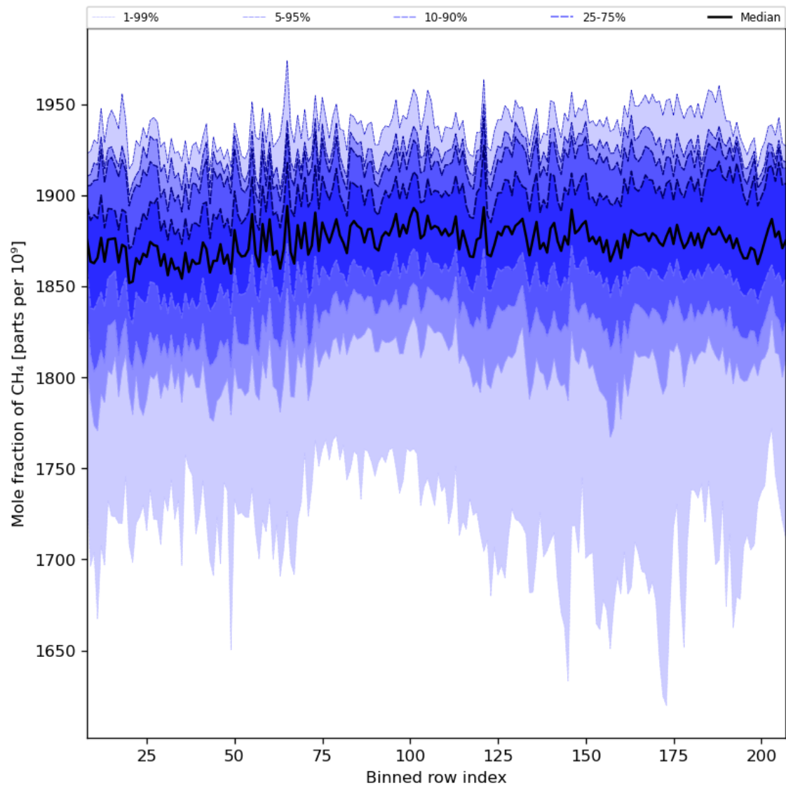
Figure 34: Along track statistics of “Mole fraction of CH 4 ” for 2023-07-08 to 2023-07-09
