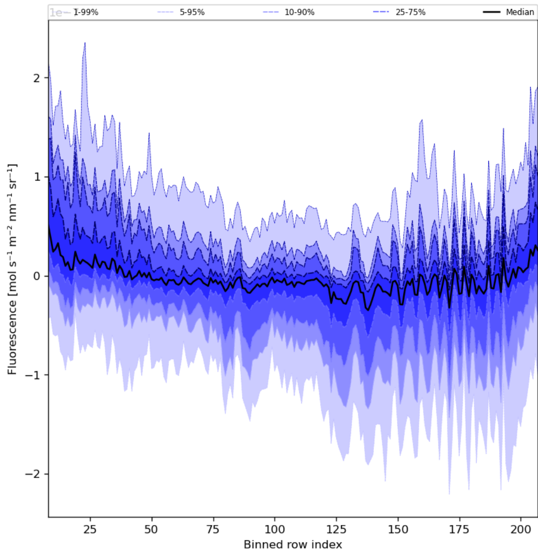
Figure 43: Along track statistics of “Fluorescence” for 2023-07-08 to 2023-07-09
