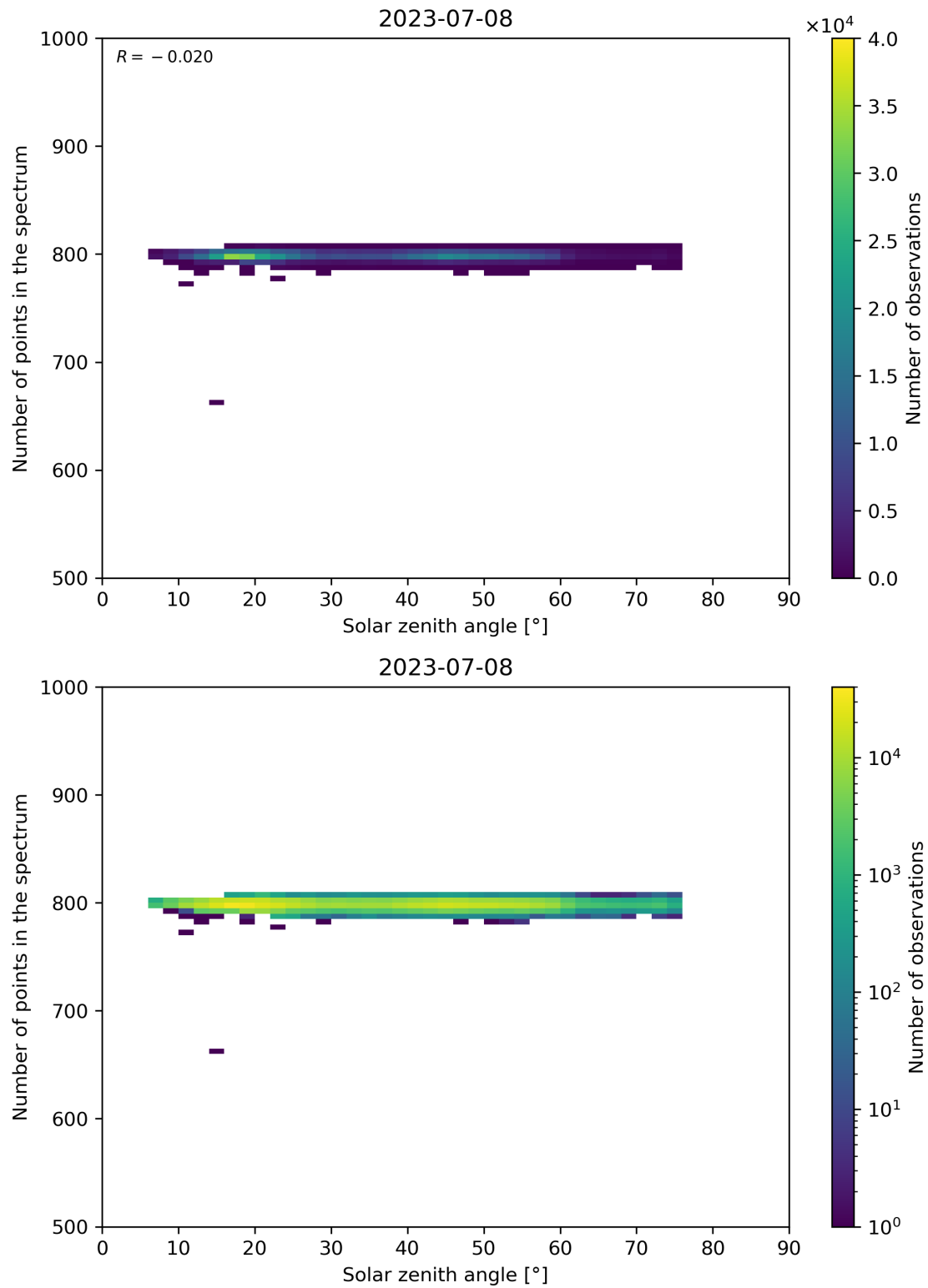
Figure 103: Scatter density plot of “Solar zenith angle” against “Number of points in the spectrum” for 2023-07-08 to 2023-07-09.
