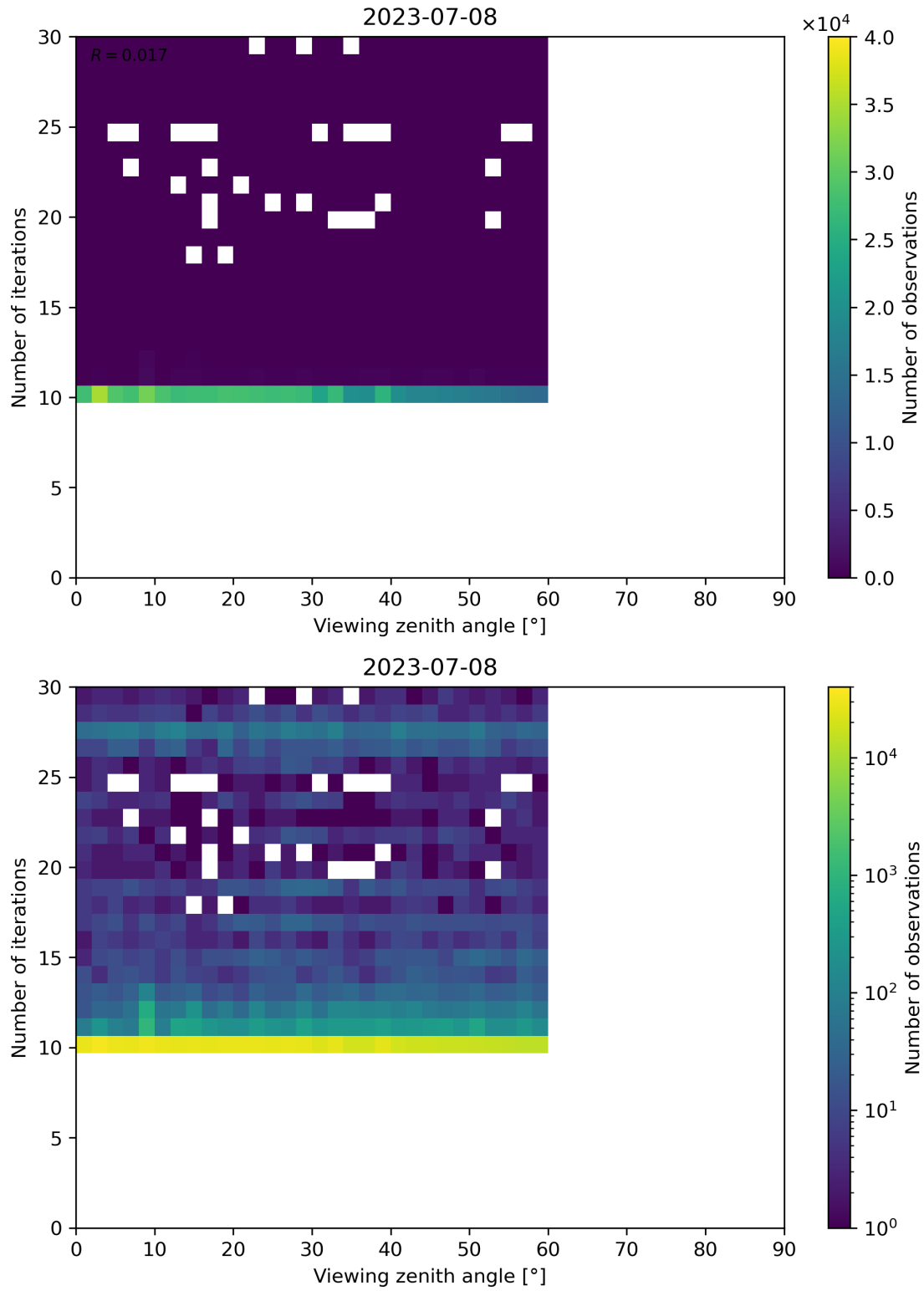
Figure 113: Scatter density plot of “Viewing zenith angle” against “Number of iterations” for 2023-07-08 to 2023-07-09.
