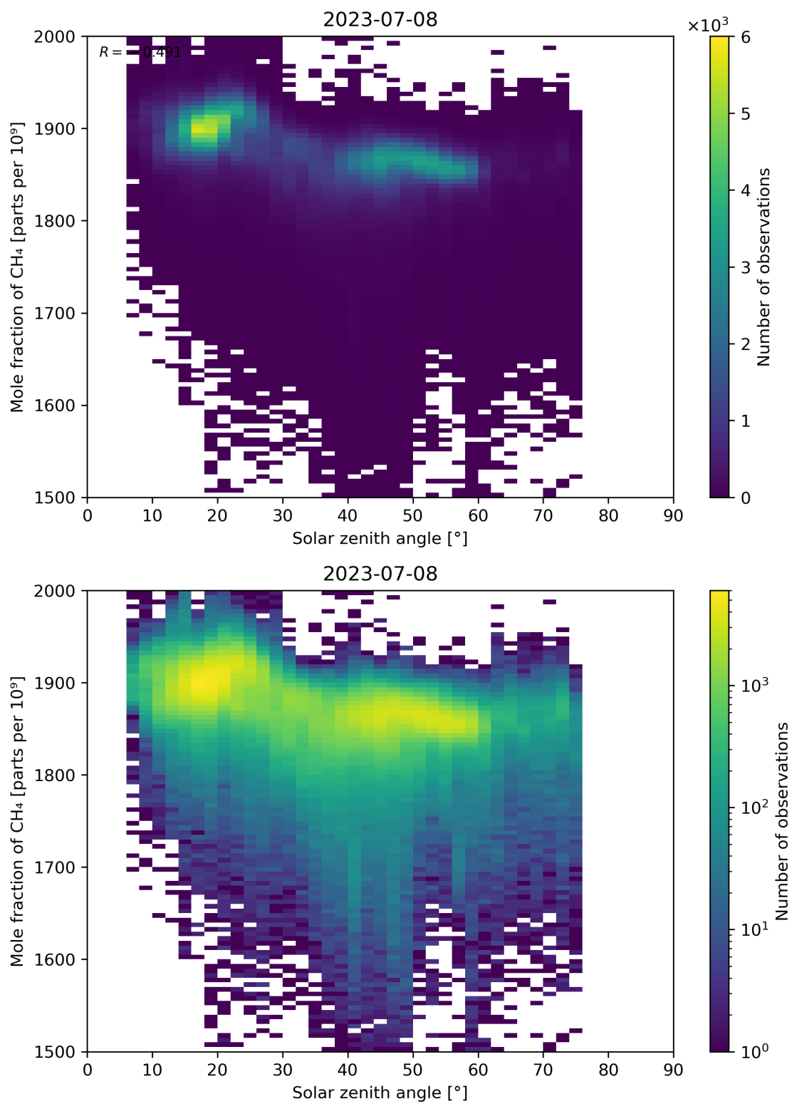
Figure 99: Scatter density plot of “Solar zenith angle” against “Mole fraction of CH 4 ” for 2023-07-08 to 2023-07-09.
