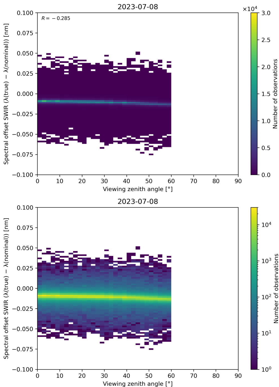
Figure 116: Scatter density plot of “Viewing zenith angle” against “Spectral offset SWIR ( \lambda(\text{true}) - \lambda(\text{nominal}) )” for 2023-07-08 to 2023-07-09.
