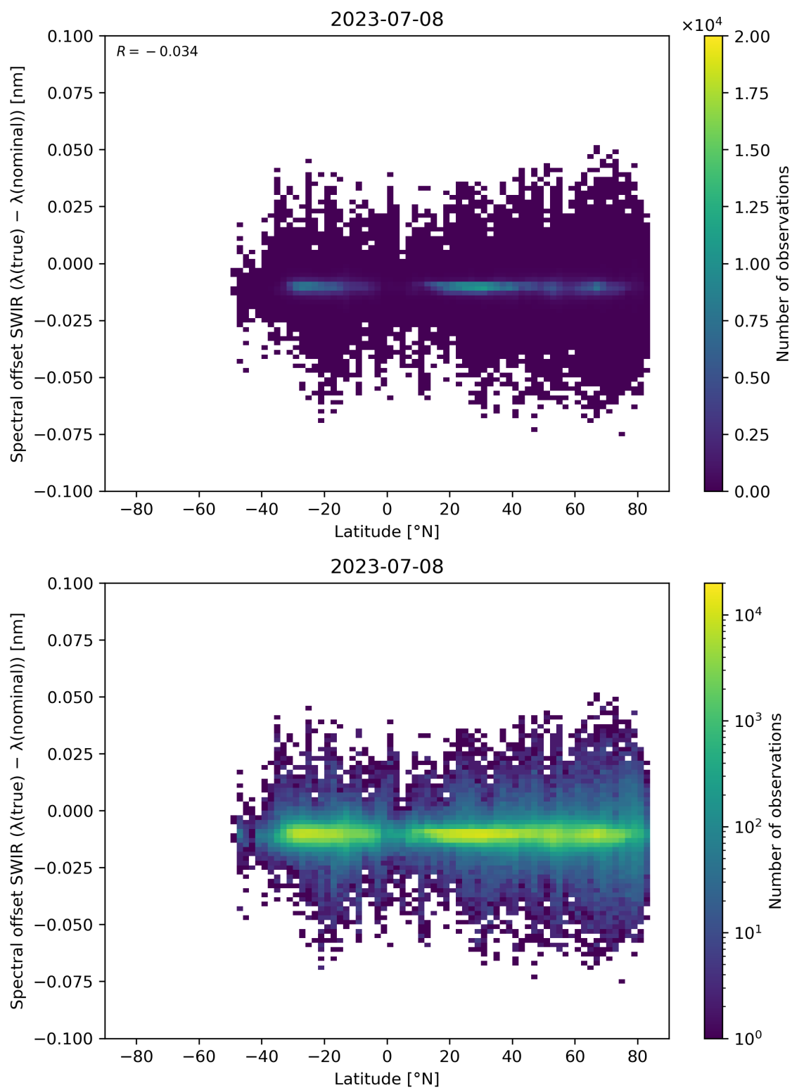
Figure 62: Scatter density plot of “Latitude” against “Spectral offset SWIR ( \lambda(\text{true}) - \lambda(\text{nominal}) )” for 2023-07-08 to 2023-07-09.
