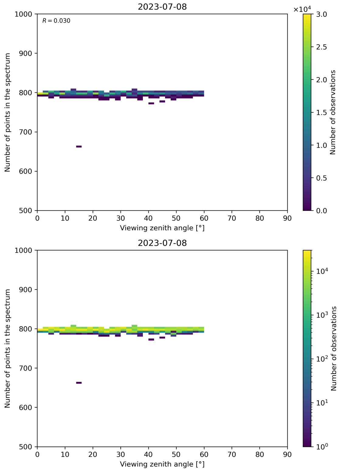
Figure 114: Scatter density plot of “Viewing zenith angle” against “Number of points in the spectrum” for 2023-07-08 to 2023-07-09.
