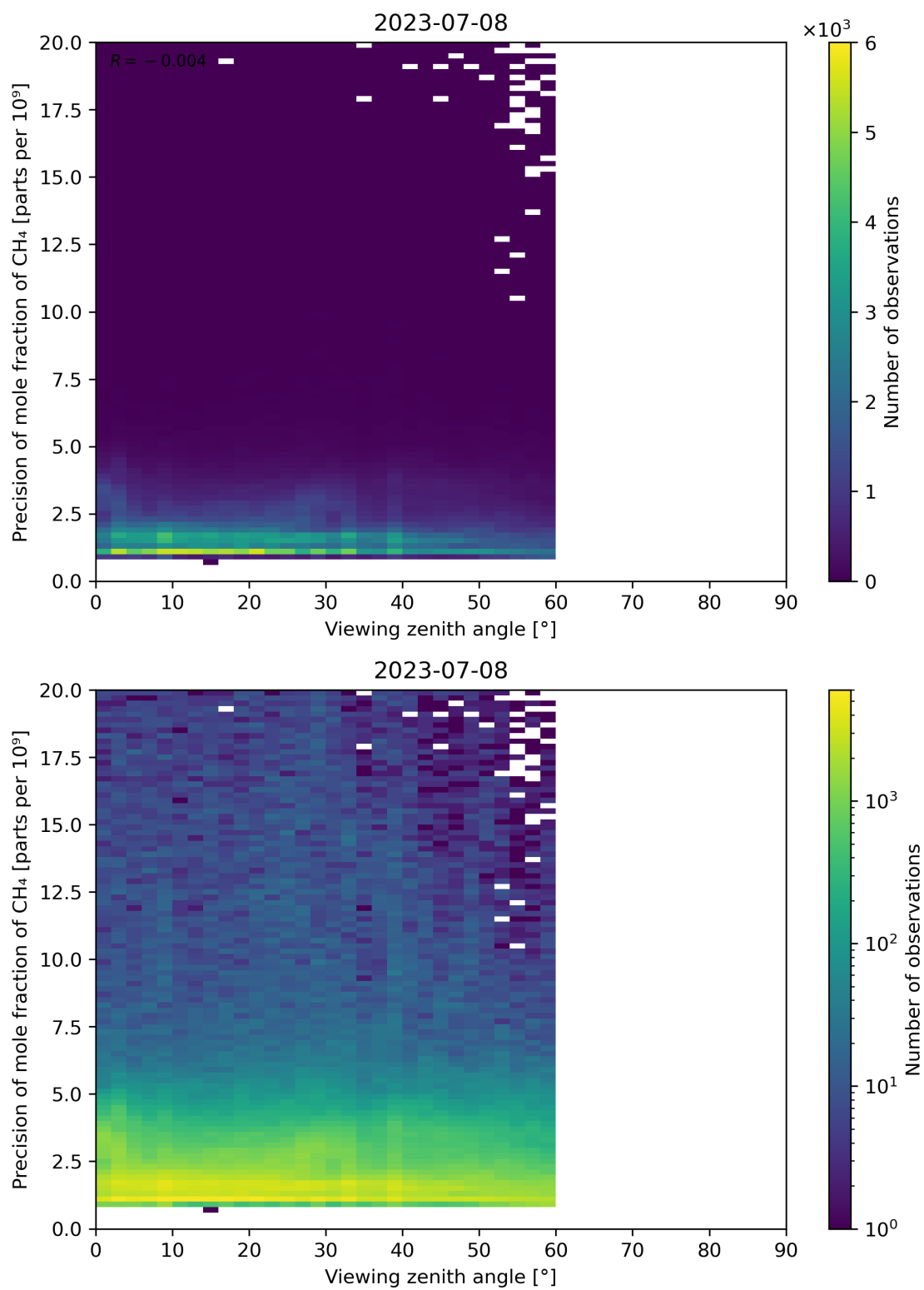
Figure 112: Scatter density plot of “Viewing zenith angle” against “Precision of mole fraction of CH 4 ” for 2023-07-08 to 2023-07-09.
