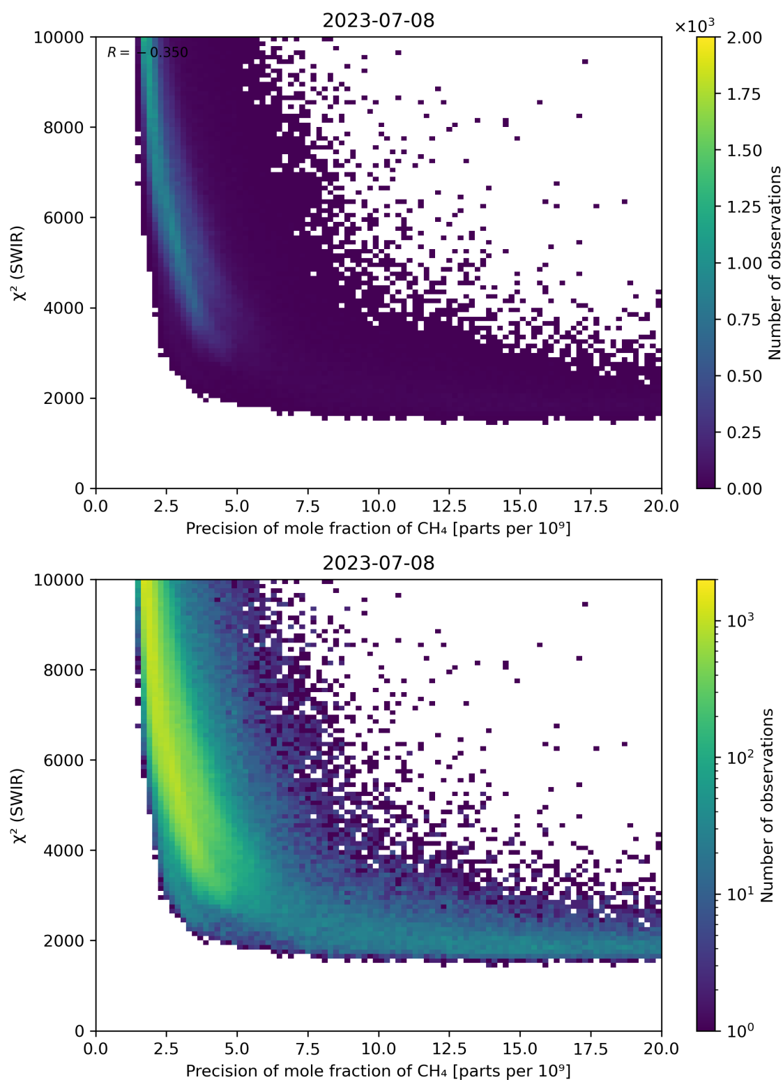
Figure 79: Scatter density plot of “Precision of mole fraction of \text{CH}_4 ” against “ \chi^2 (SWIR)” for 2023-07-08 to 2023-07-09.
