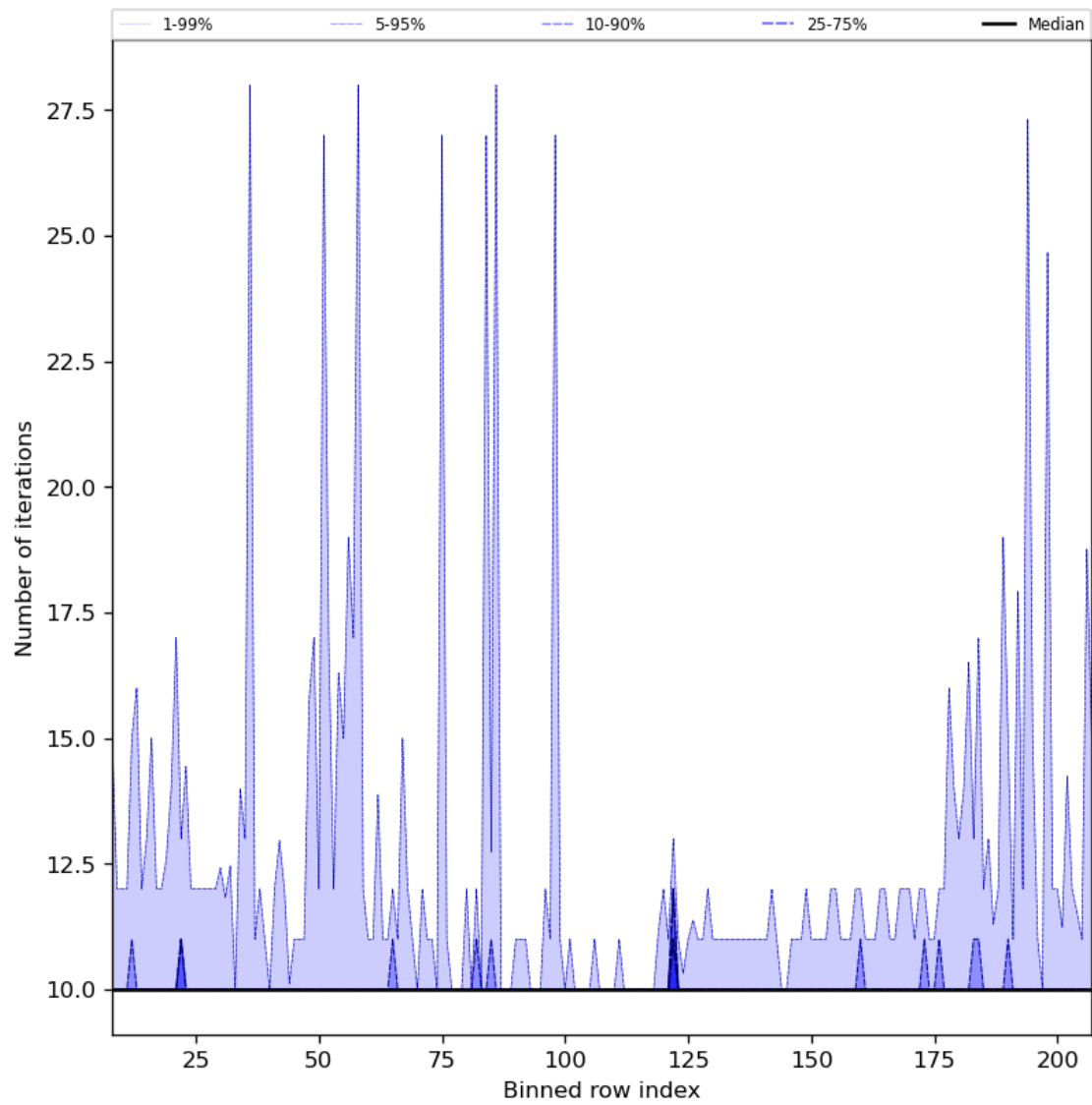
Figure 42: Along track statistics of “Number of iterations” for 2023-07-08 to 2023-07-09
