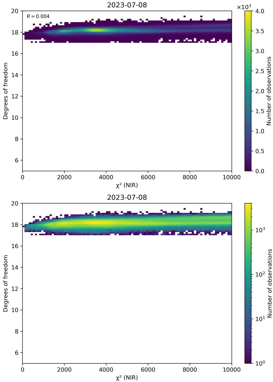
Figure 44: Scatter density plot of “ \chi^2 (NIR)” against “Degrees of freedom” for 2023-07-08 to 2023-07-09.
