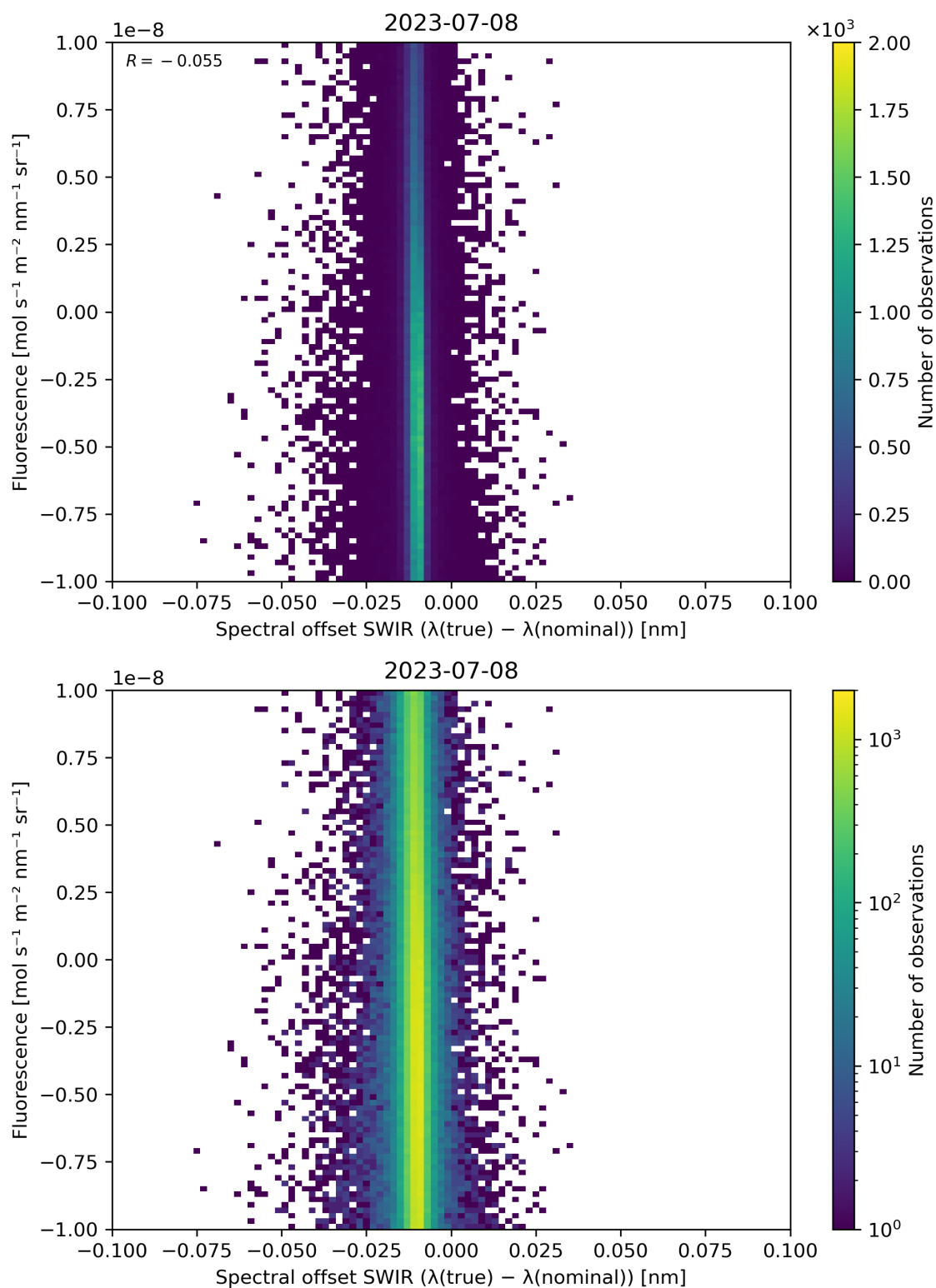
Figure 120: Scatter density plot of “Spectral offset SWIR ( \lambda(\text{true}) - \lambda(\text{nominal}) )” against “Fluorescence” for 2023-07-08 to 2023-07-09.
