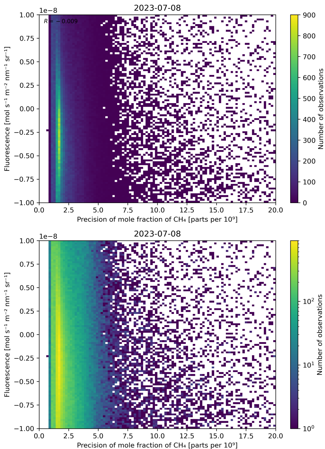
Figure 81: Scatter density plot of “Precision of mole fraction of \text{CH}_4 ” against “Fluorescence” for 2023-07-08 to 2023-07-09.
