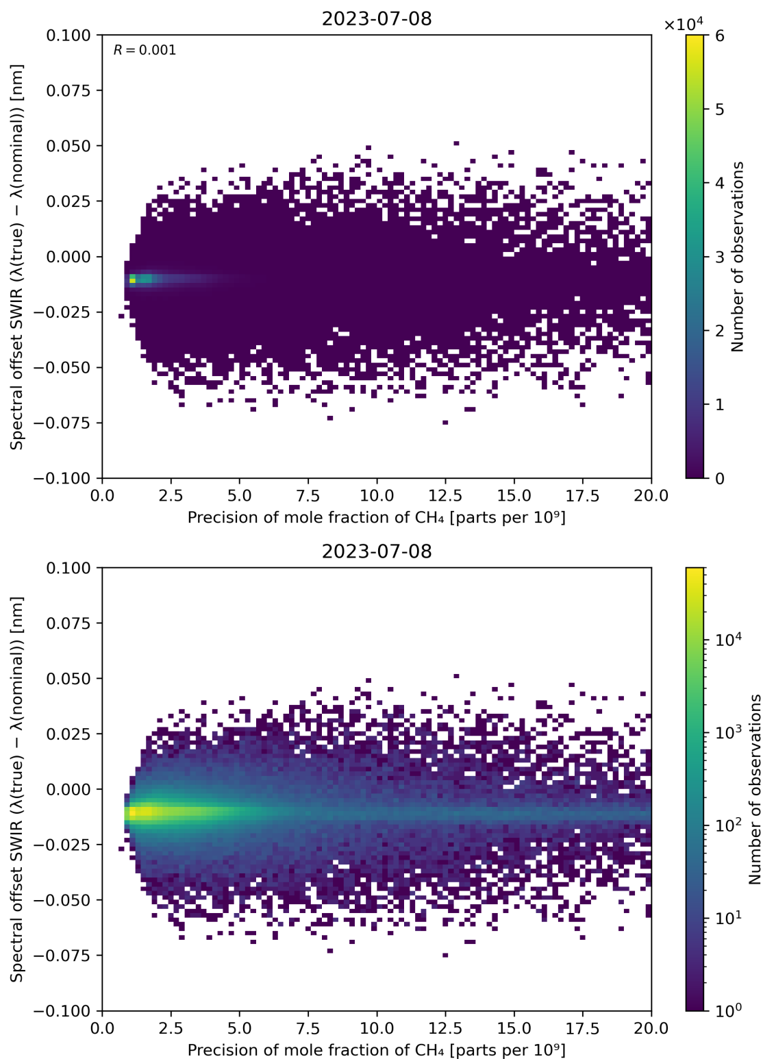
Figure 85: Scatter density plot of “Precision of mole fraction of CH 4 ” against “Spectral offset SWIR ( \lambda(\text{true}) - \lambda(\text{nominal}) )” for 2023-07-08 to 2023-07-09.
