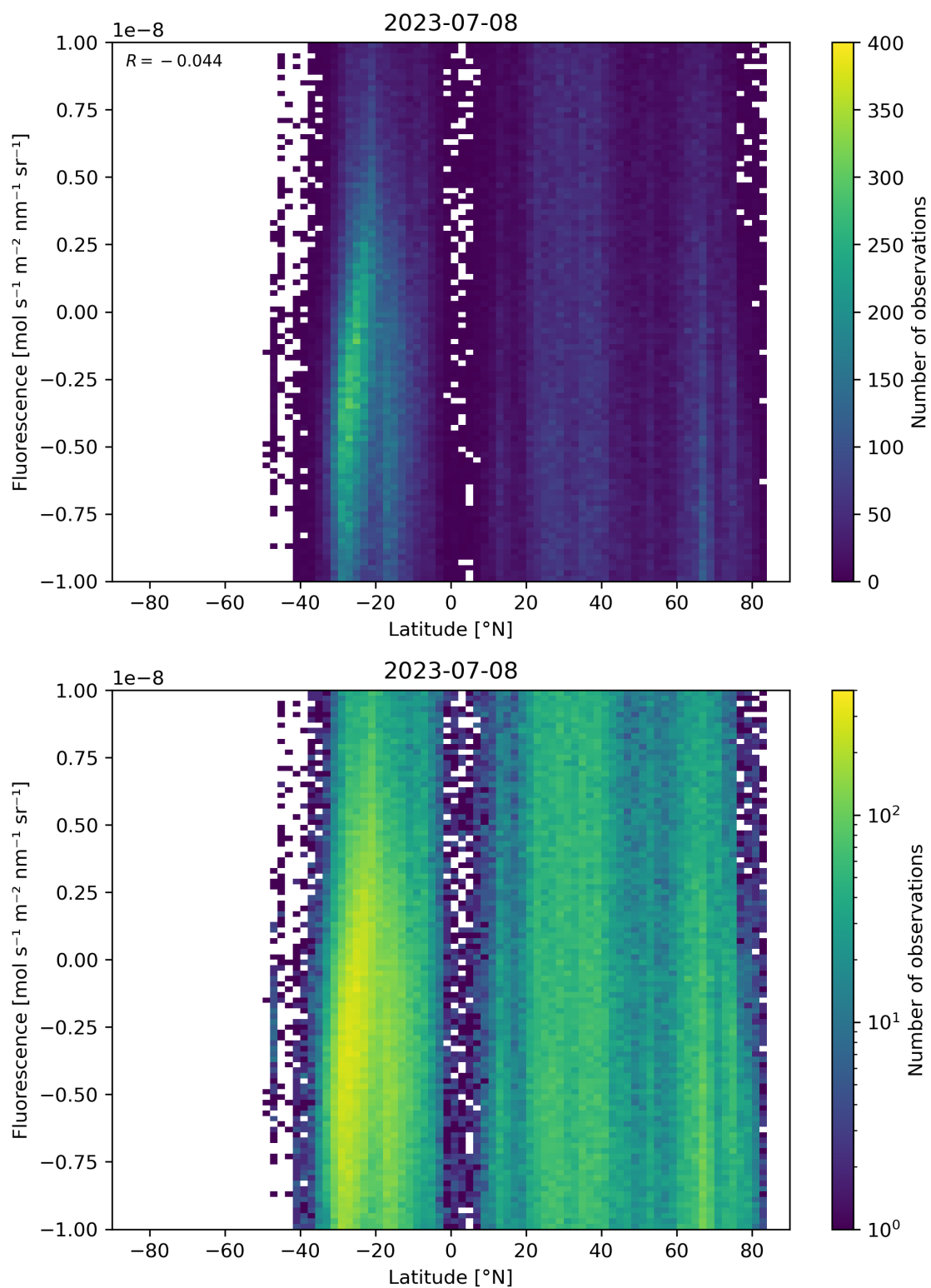
Figure 56: Scatter density plot of “Latitude” against “Fluorescence” for 2023-07-08 to 2023-07-09.
