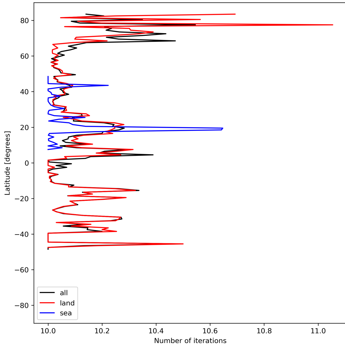
Figure 20: Zonal average of “Number of iterations” for 2023-07-08 to 2023-07-09.
