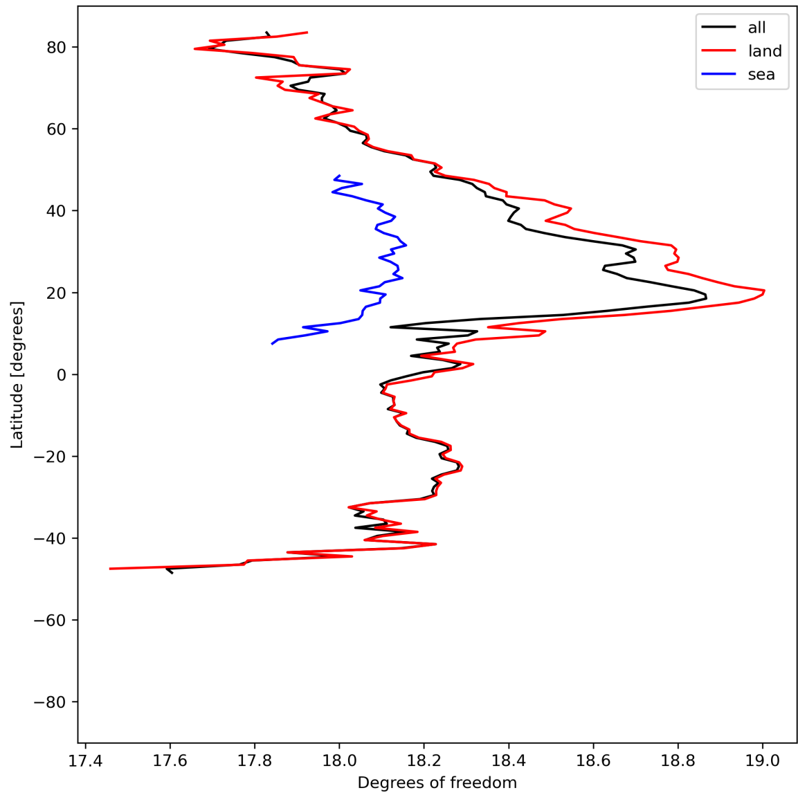
Figure 19: Zonal average of “Degrees of freedom” for 2023-07-08 to 2023-07-09.
