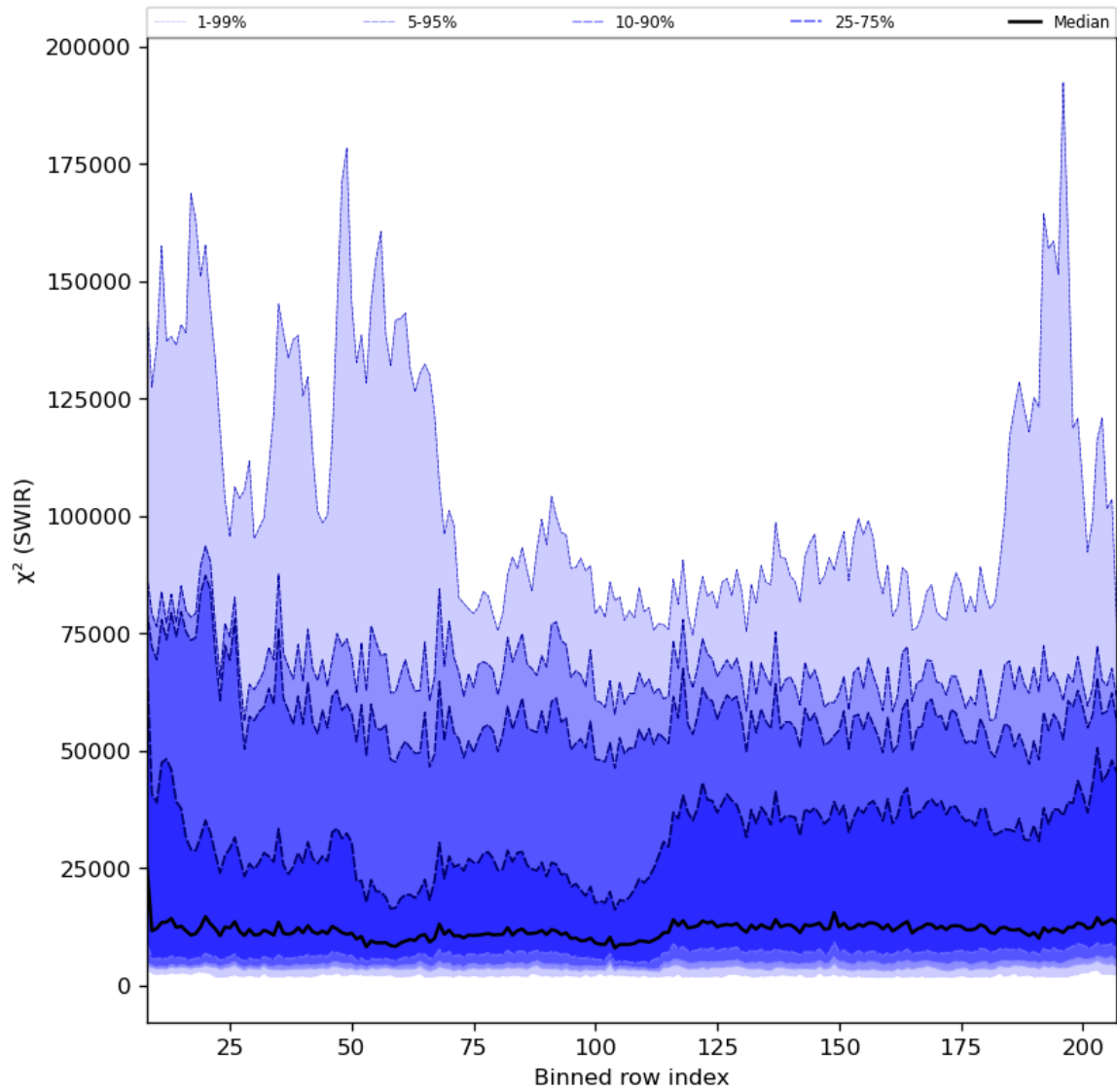
Figure 39: Along track statistics of “ \chi^2 (SWIR)” for 2023-07-08 to 2023-07-09
