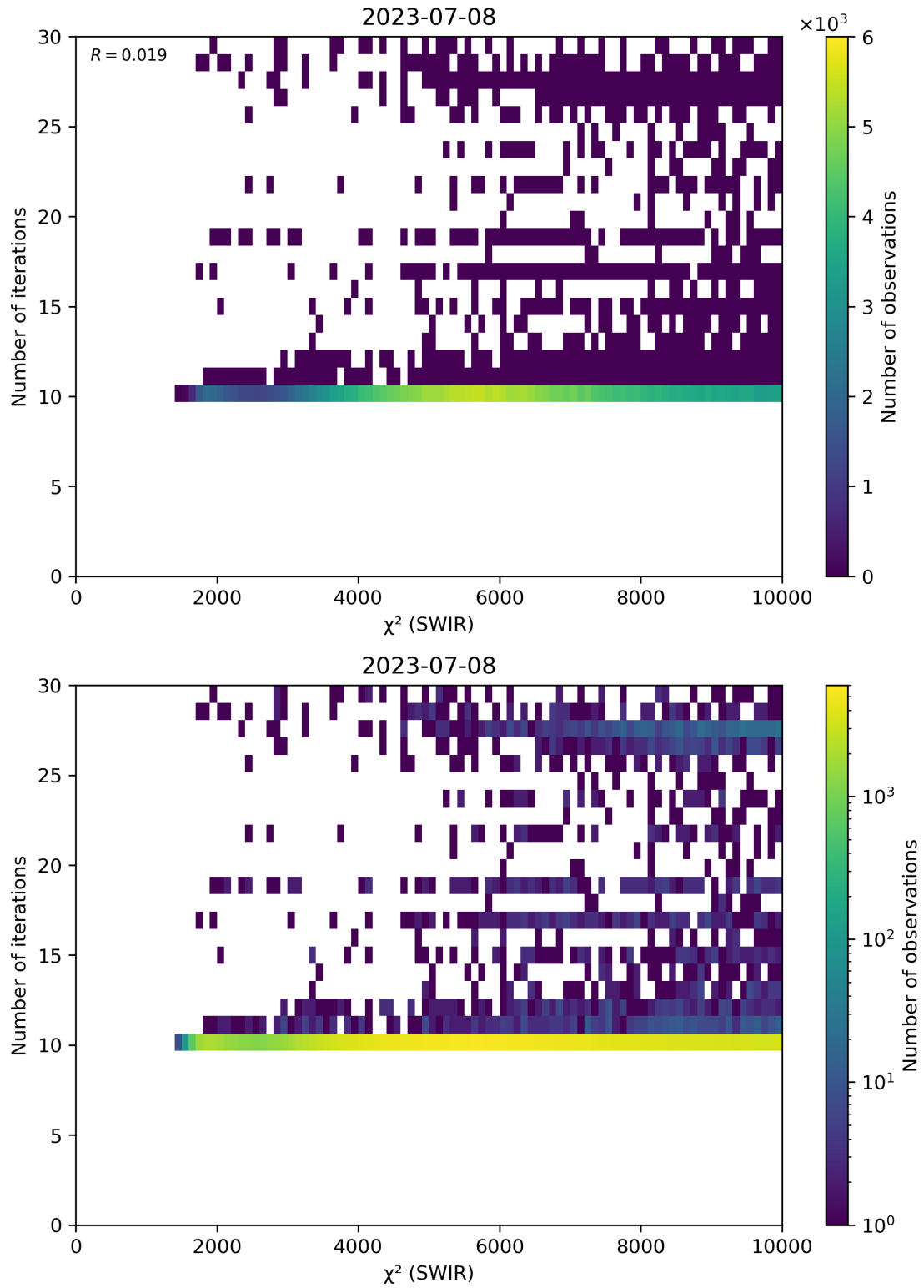
Figure 50: Scatter density plot of “ \chi^2 (SWIR)” against “Number of iterations” for 2023-07-08 to 2023-07-09.
