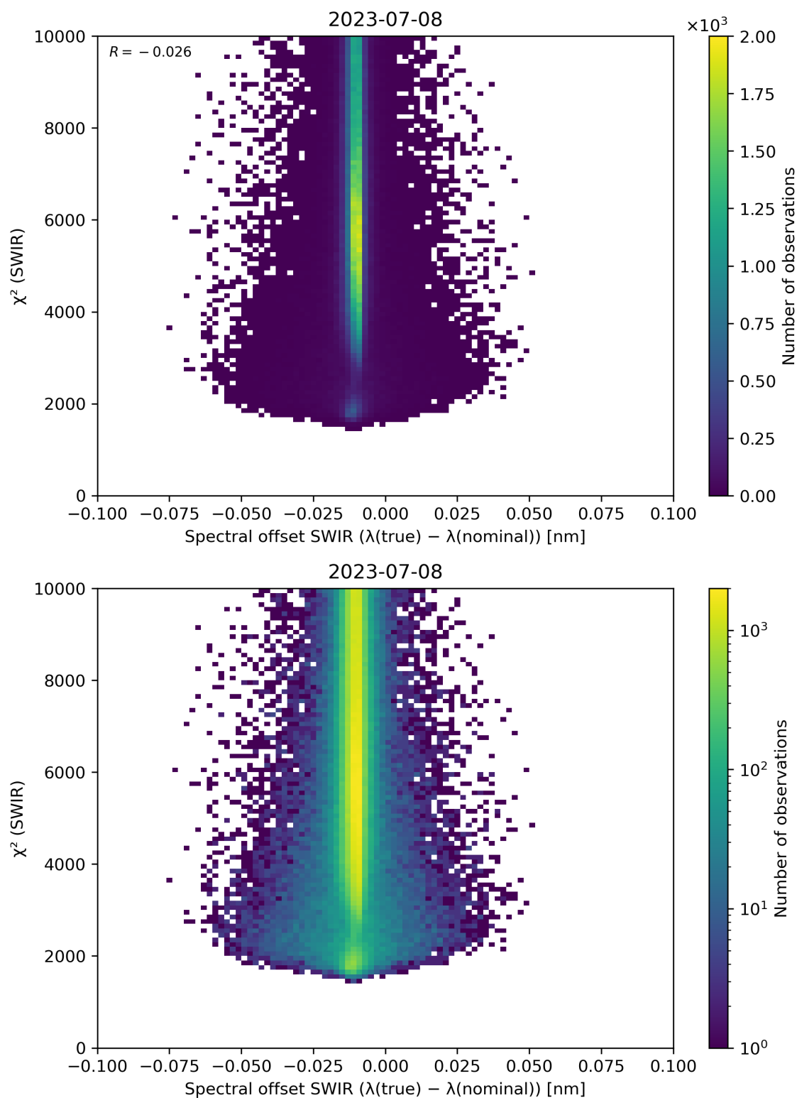
Figure 118: Scatter density plot of “Spectral offset SWIR ( \lambda(\text{true}) - \lambda(\text{nominal}) )” against “ \chi^2 (SWIR)” for 2023-07-08 to 2023-07-09.
