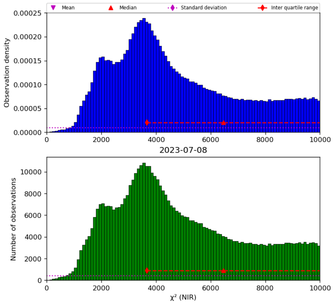
Figure 29: Histogram of “ \chi^2 (NIR)” for 2023-07-08 to 2023-07-09
