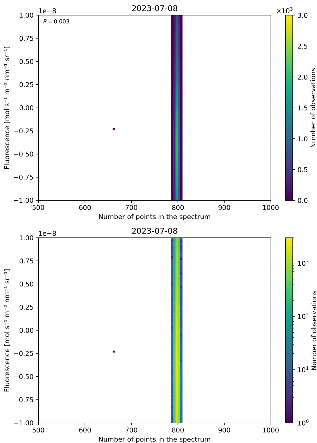
Figure 91: Scatter density plot of “Number of points in the spectrum” against “Fluorescence” for 2023-07-08 to 2023-07-09.
