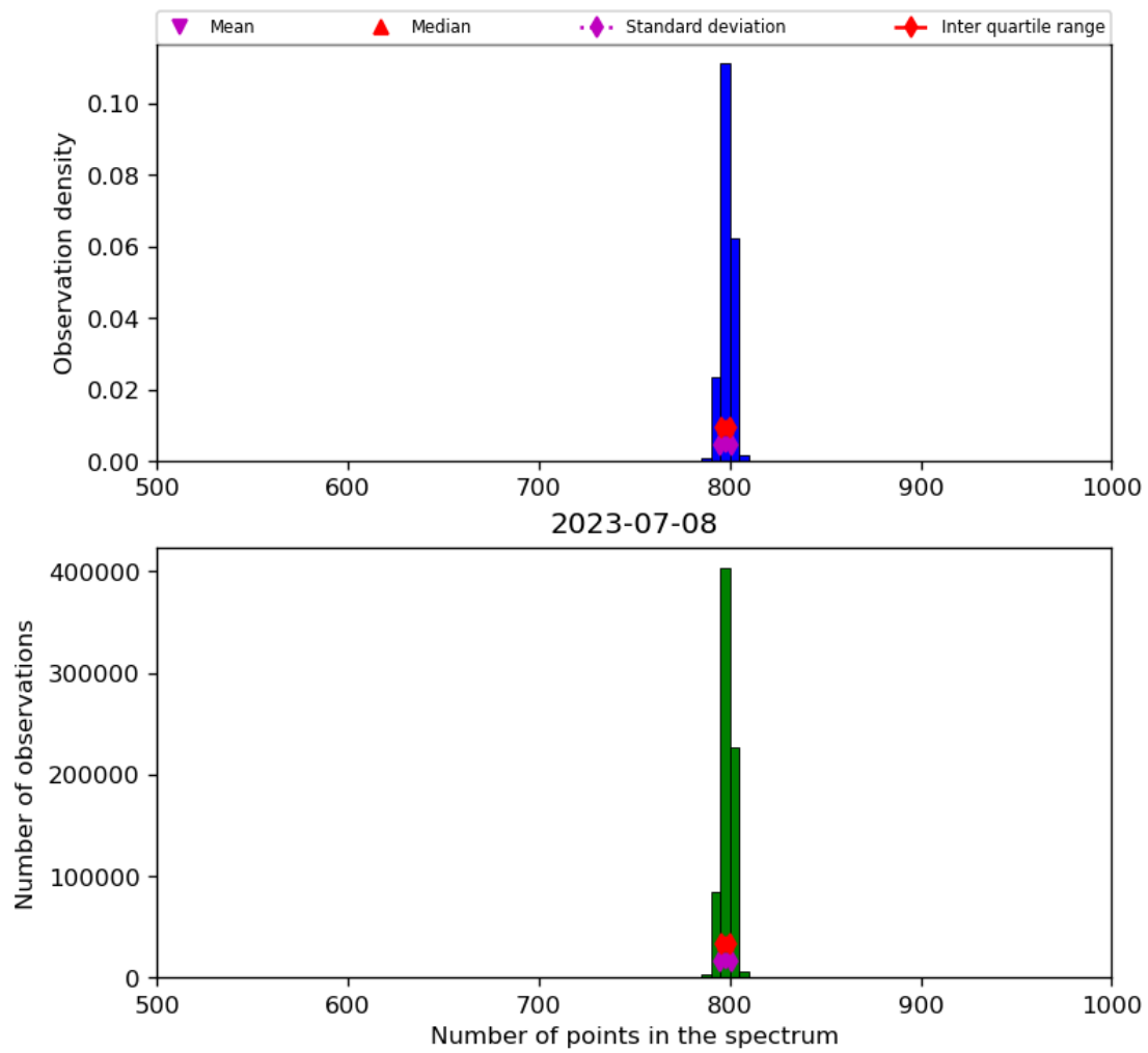
Figure 26: Histogram of “Number of points in the spectrum” for 2023-07-08 to 2023-07-09
