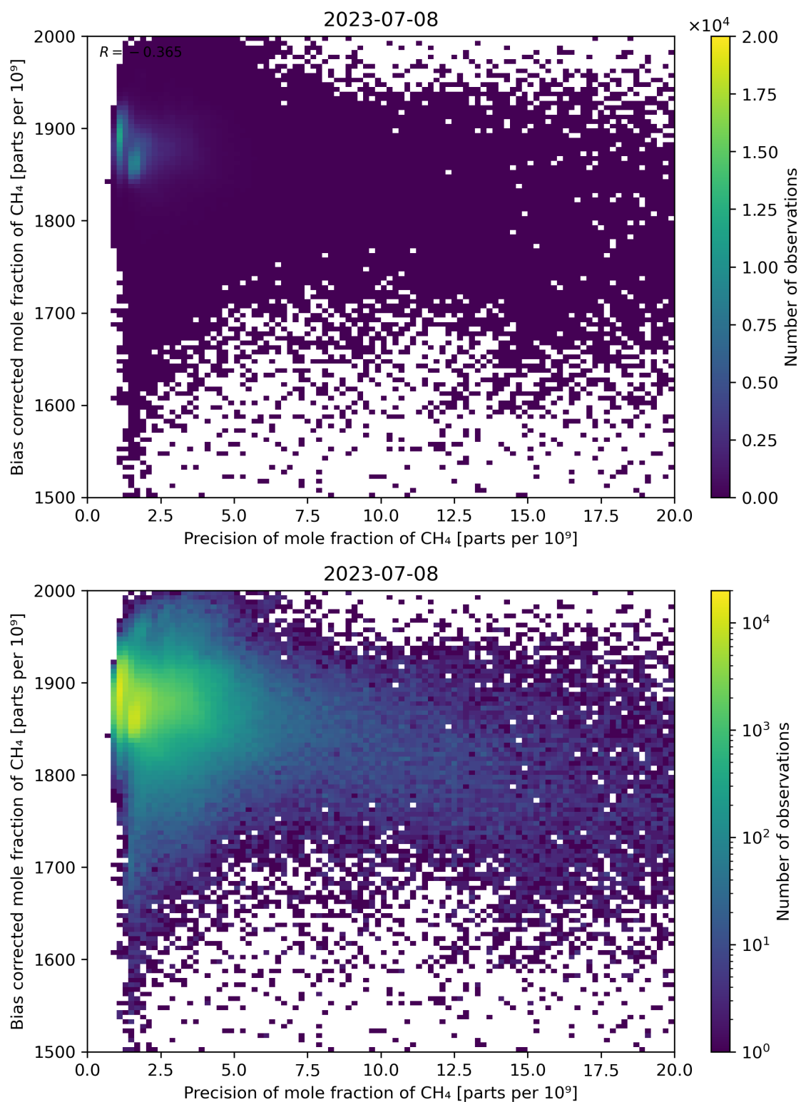
Figure 82: Scatter density plot of “Precision of mole fraction of CH 4 ” against “Bias corrected mole fraction of CH 4 ” for 2023-07-08 to 2023-07-09.
