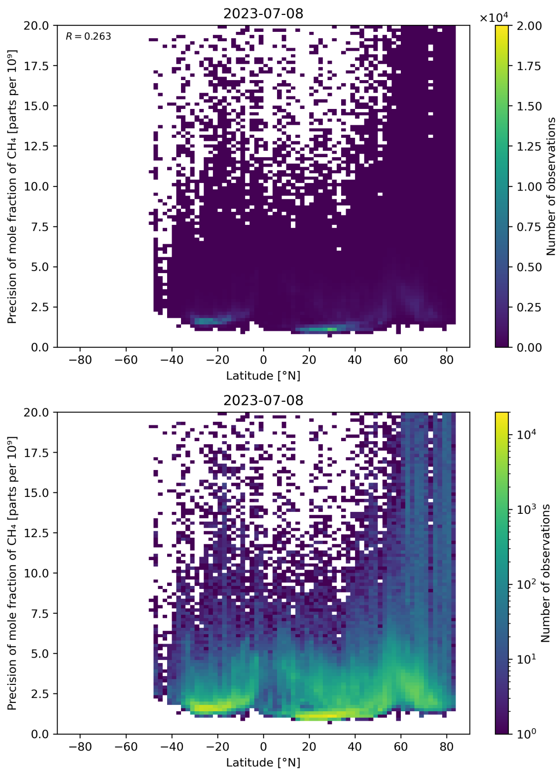
Figure 59: Scatter density plot of “Latitude” against “Precision of mole fraction of CH 4 ” for 2023-07-08 to 2023-07-09.
