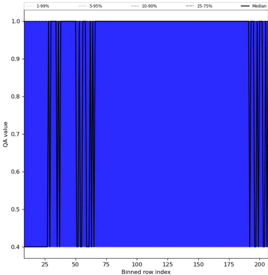
Figure 33: Along track statistics of “QA value” for 2023-07-08 to 2023-07-09
