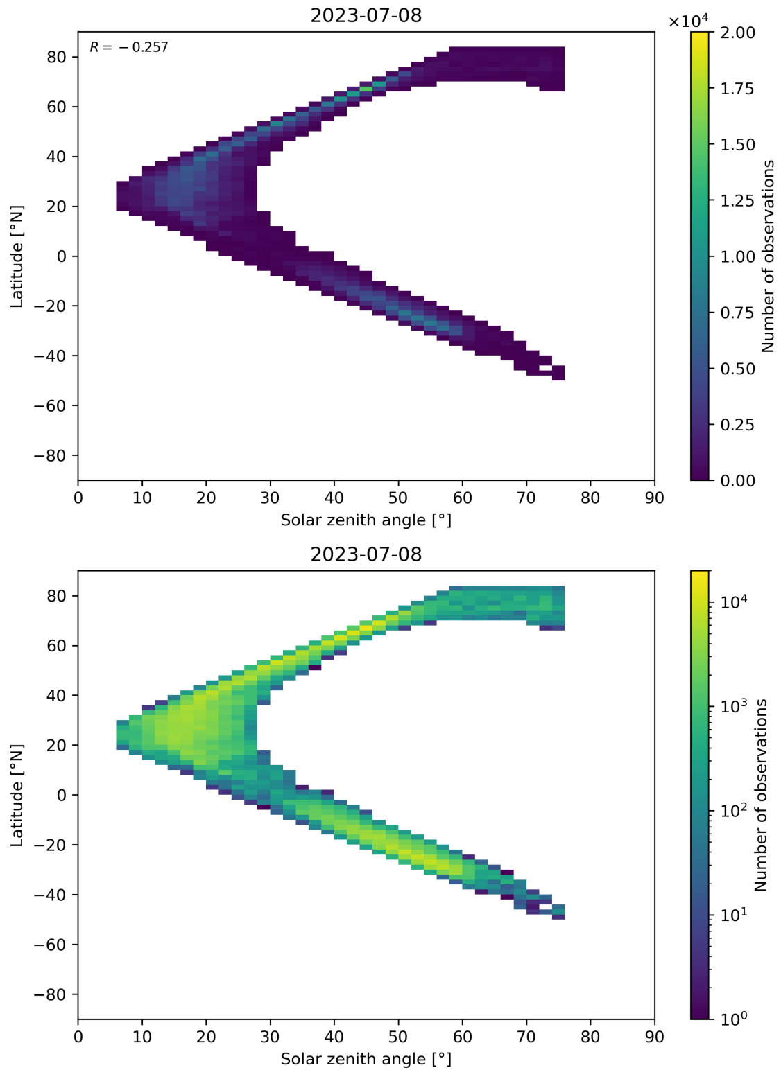
Figure 98: Scatter density plot of “Solar zenith angle” against “Latitude” for 2023-07-08 to 2023-07-09.
