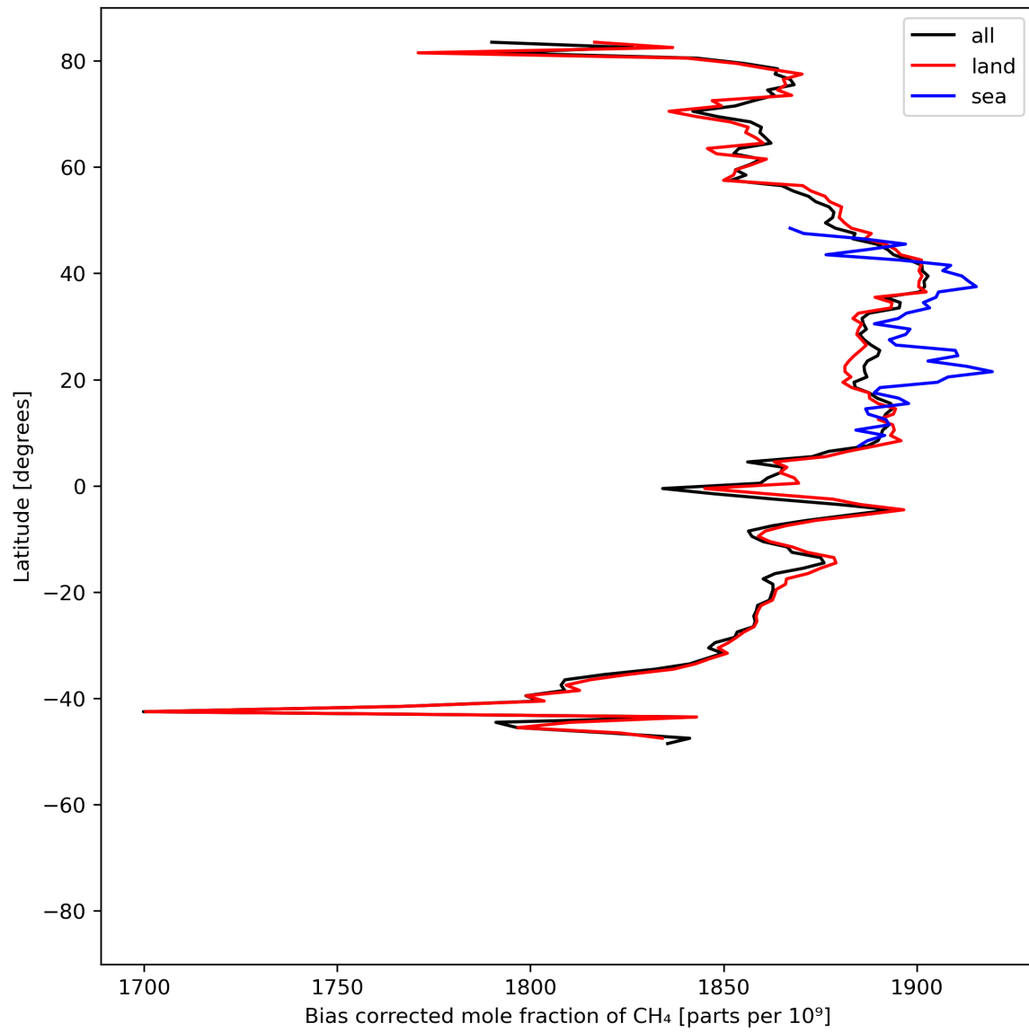
Figure 14: Zonal average of “Bias corrected mole fraction of CH 4 ” for 2023-07-08 to 2023-07-09.
