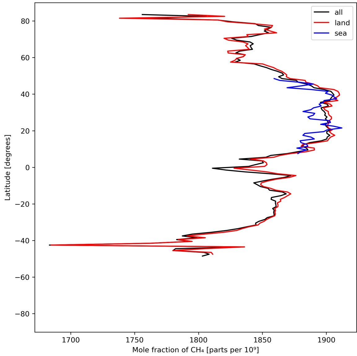
Figure 12: Zonal average of “Mole fraction of \text{CH}_4 ” for 2023-07-08 to 2023-07-09.
