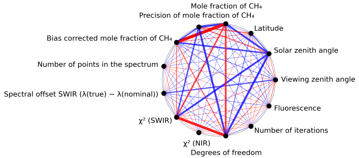
Figure 1: Map of correlation graph for 2023-07-08 to 2023-07-09.
