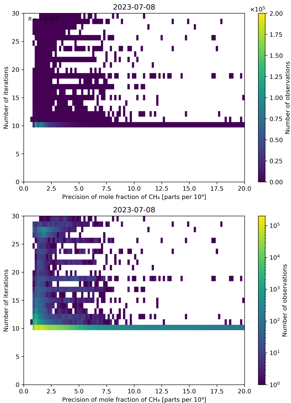
Figure 83: Scatter density plot of “Precision of mole fraction of CH 4 ” against “Number of iterations” for 2023-07-08 to 2023-07-09.
