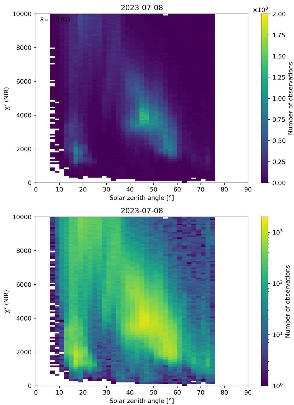
Figure 94: Scatter density plot of “Solar zenith angle” against “ \chi^2 (NIR)” for 2023-07-08 to 2023-07-09.
