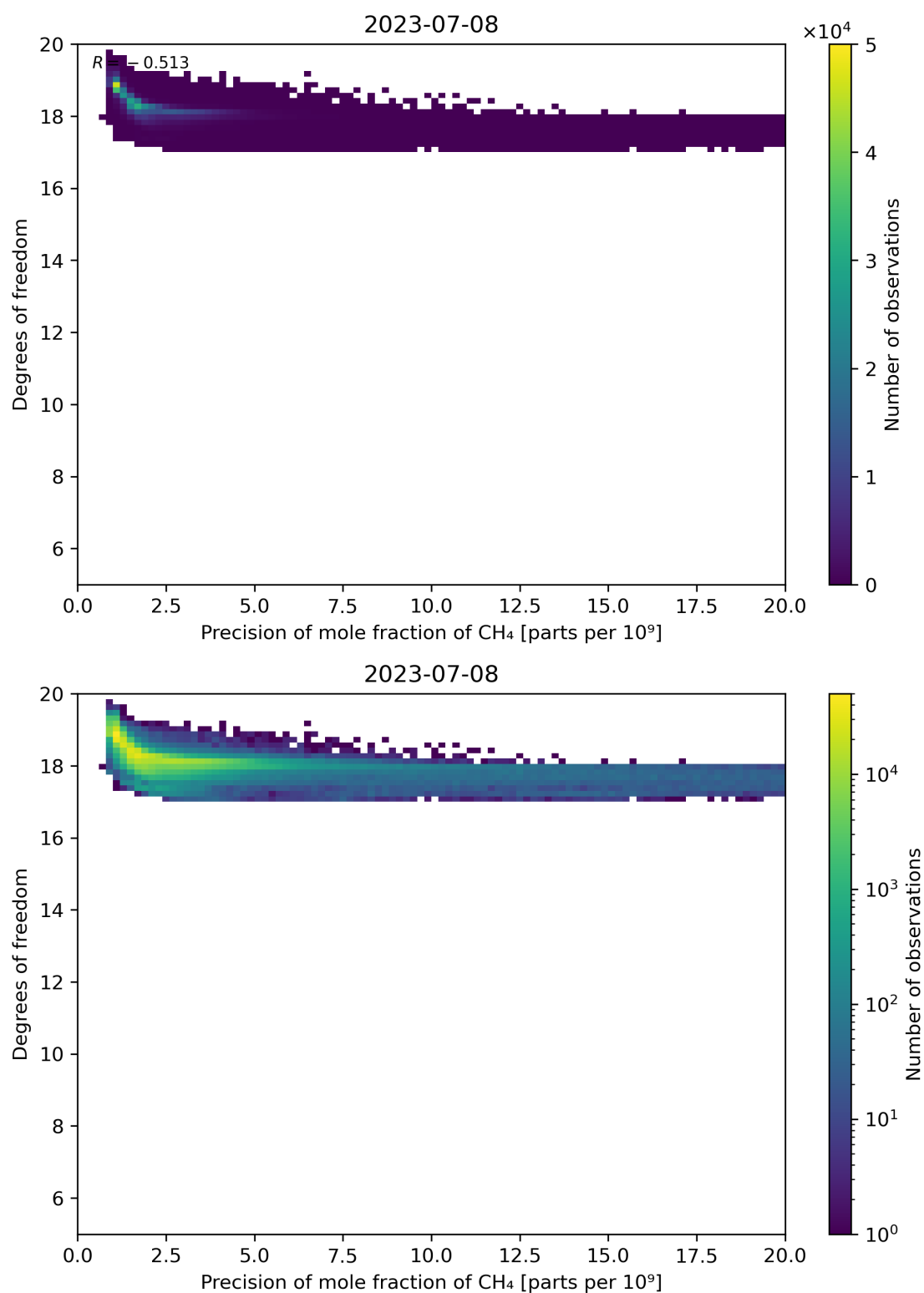
Figure 80: Scatter density plot of “Precision of mole fraction of CH 4 ” against “Degrees of freedom” for 2023-07-08 to 2023-07-09.
