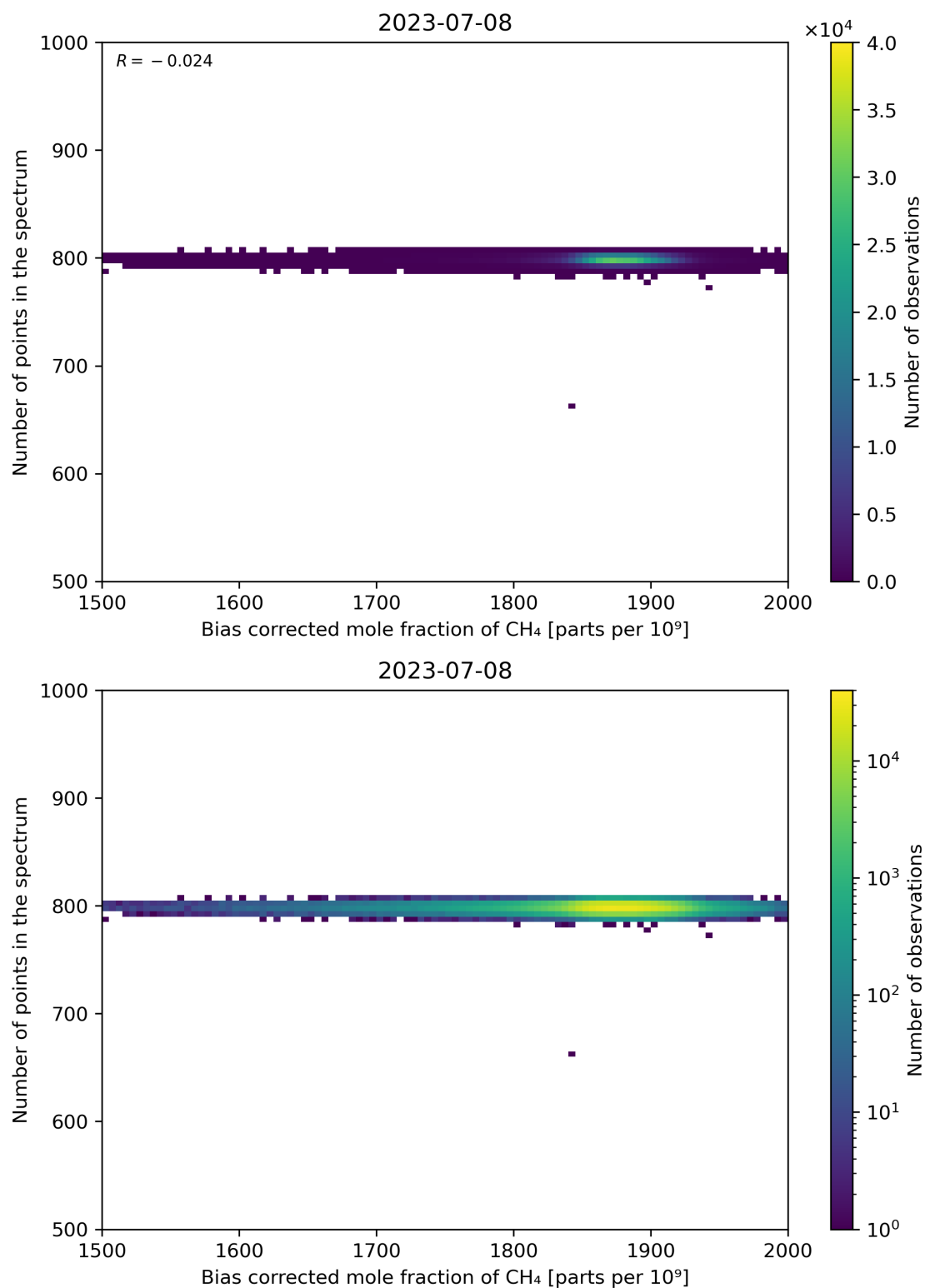
Figure 68: Scatter density plot of “Bias corrected mole fraction of CH 4 ” against “Number of points in the spectrum” for 2023-07-08 to 2023-07-09.
