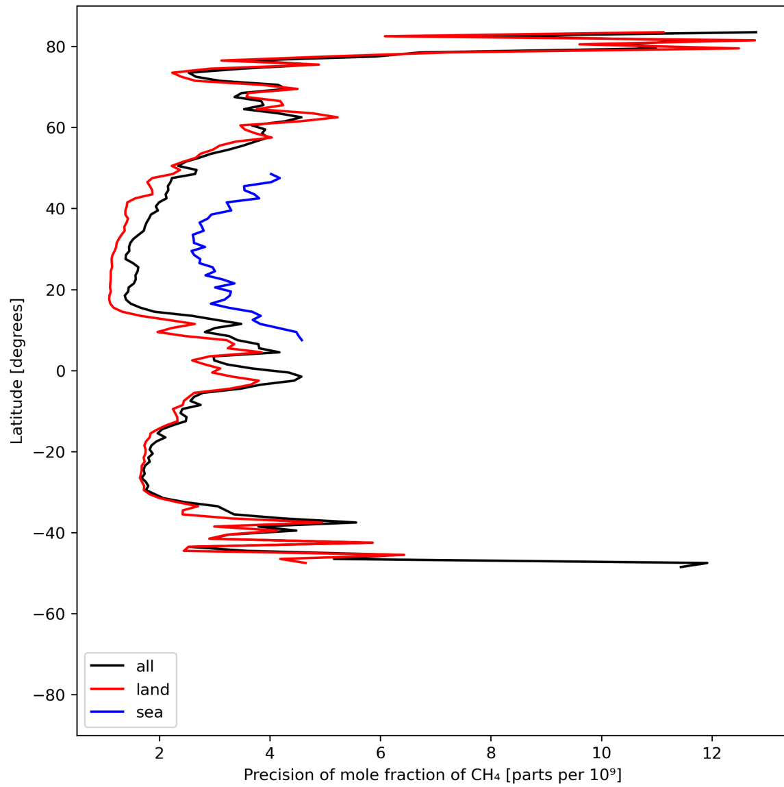
Figure 13: Zonal average of “Precision of mole fraction of CH 4 ” for 2023-07-08 to 2023-07-09.
