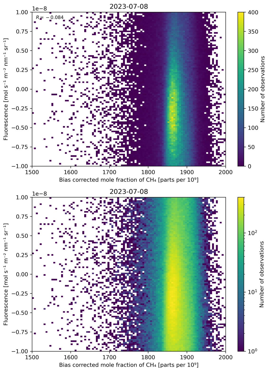
Figure 66: Scatter density plot of “Bias corrected mole fraction of \text{CH}_4 ” against “Fluorescence” for 2023-07-08 to 2023-07-09.
