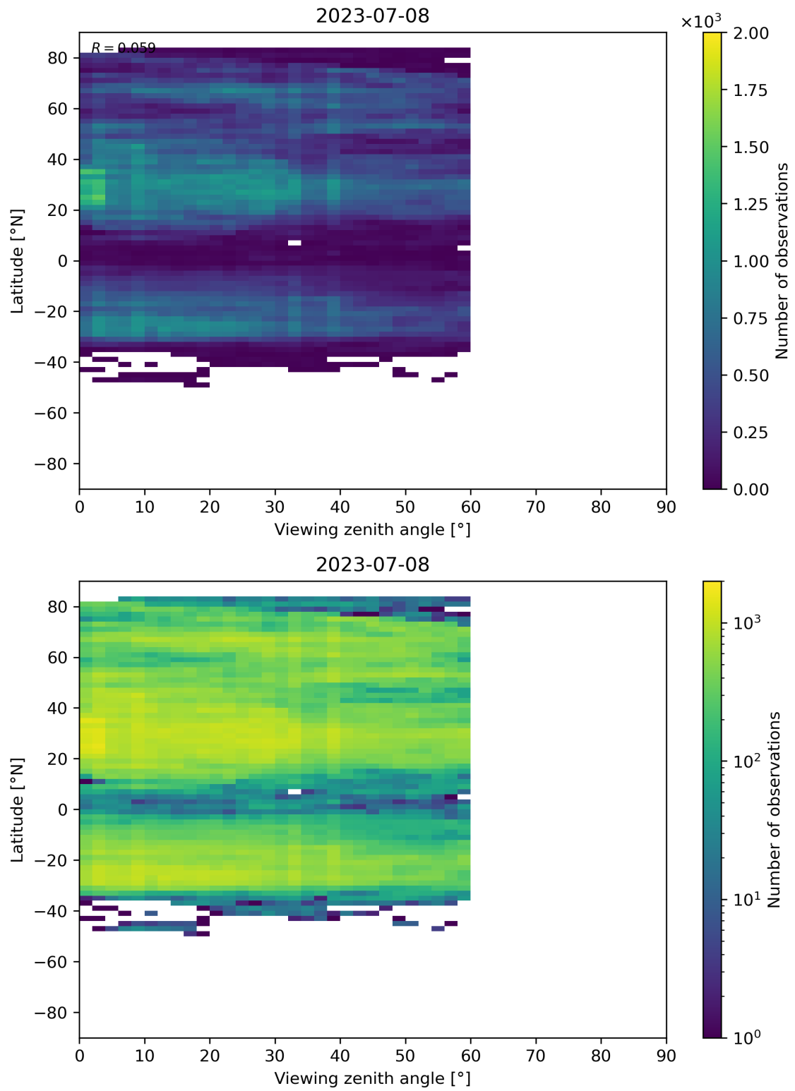
Figure 109: Scatter density plot of “Viewing zenith angle” against “Latitude” for 2023-07-08 to 2023-07-09.
