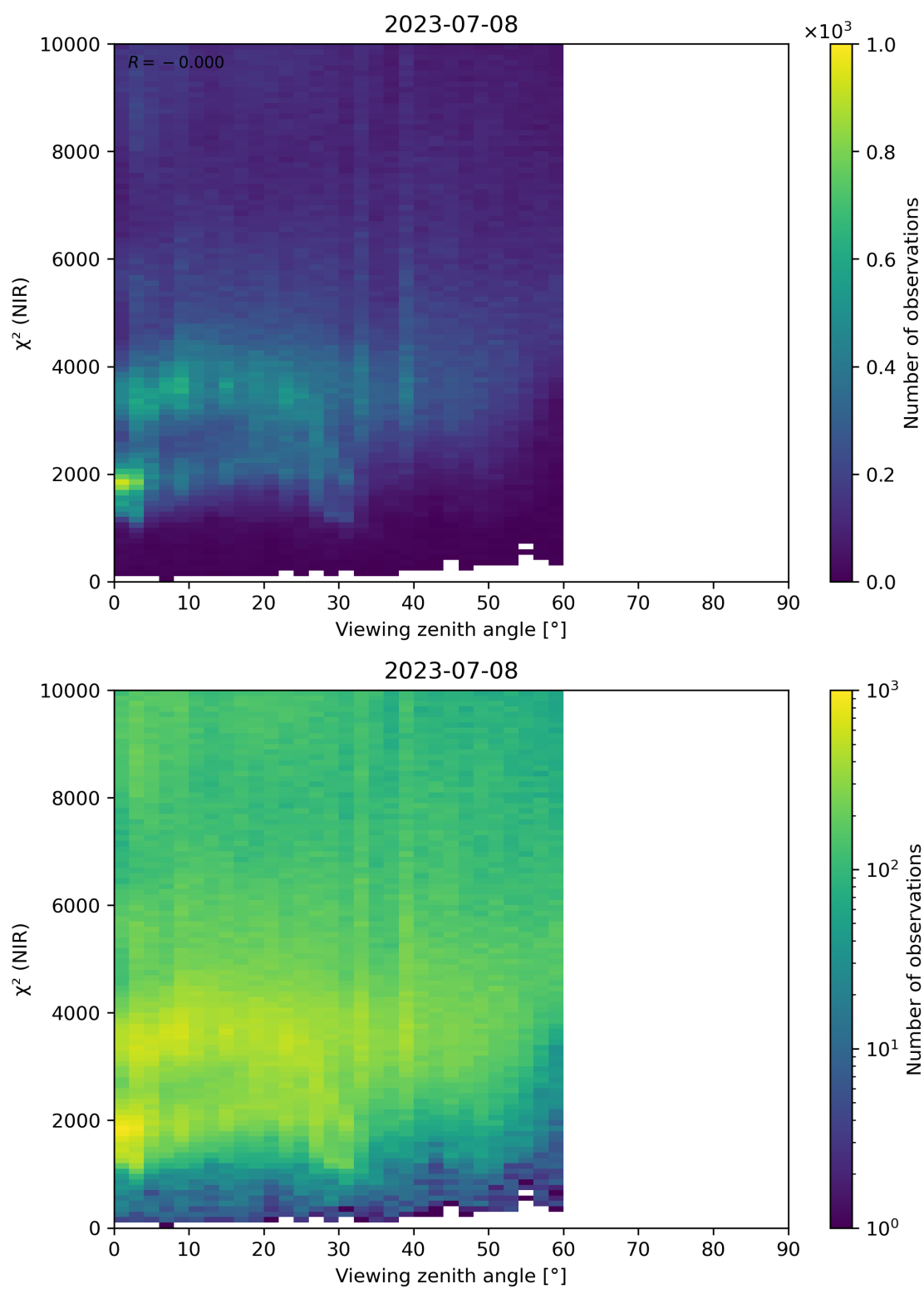
Figure 105: Scatter density plot of “Viewing zenith angle” against “ \chi^2 (NIR)” for 2023-07-08 to 2023-07-09.
