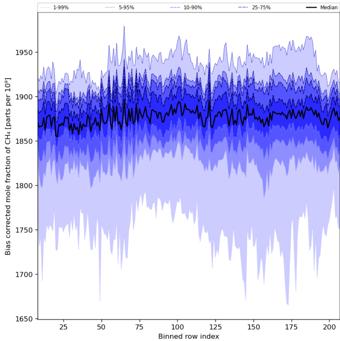
Figure 36: Along track statistics of “Bias corrected mole fraction of CH 4 ” for 2023-07-08 to 2023-07-09
