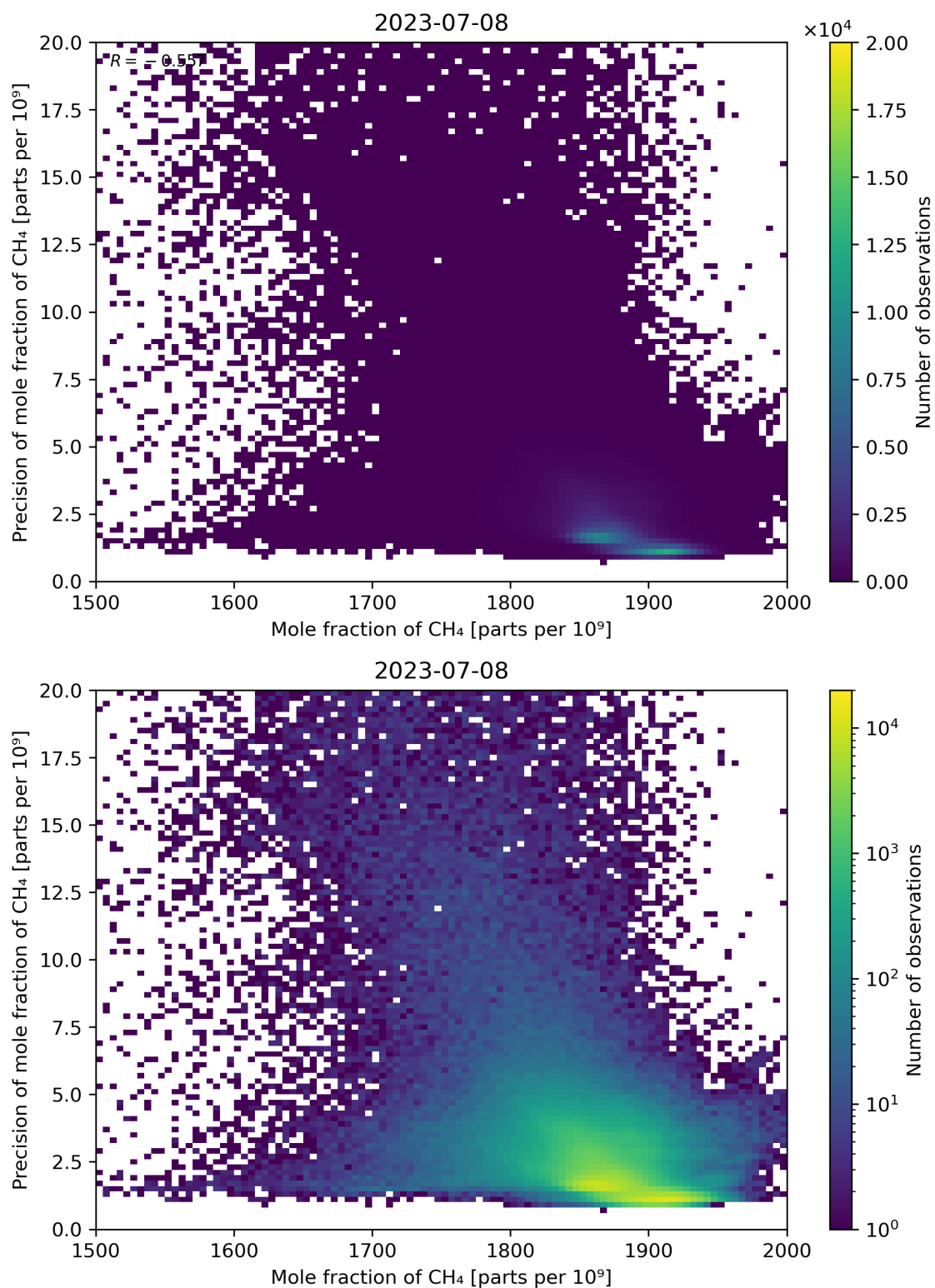
Figure 75: Scatter density plot of “Mole fraction of CH 4 ” against “Precision of mole fraction of CH 4 ” for 2023-07-08 to 2023-07-09.
