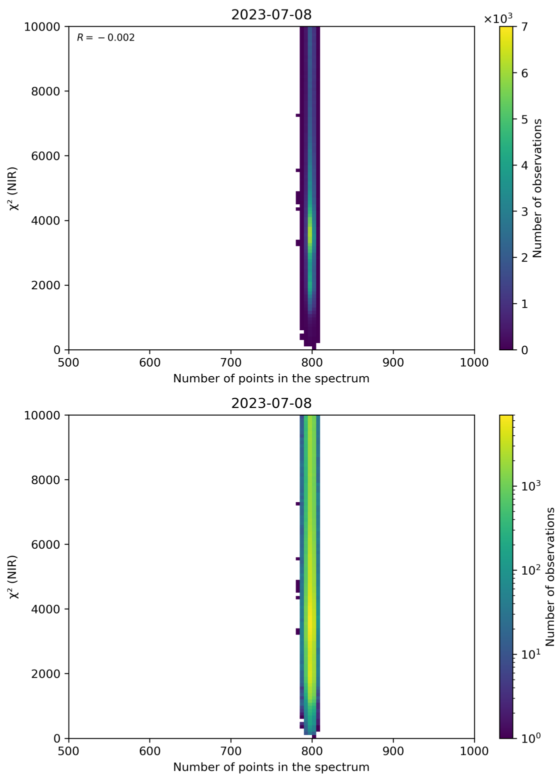
Figure 88: Scatter density plot of “Number of points in the spectrum” against “ \chi^2 (NIR)” for 2023-07-08 to 2023-07-09.
