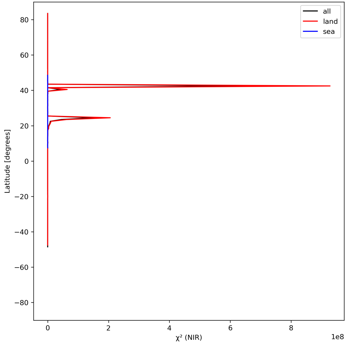
Figure 18: Zonal average of “ \chi^2 (NIR)” for 2023-07-08 to 2023-07-09.
