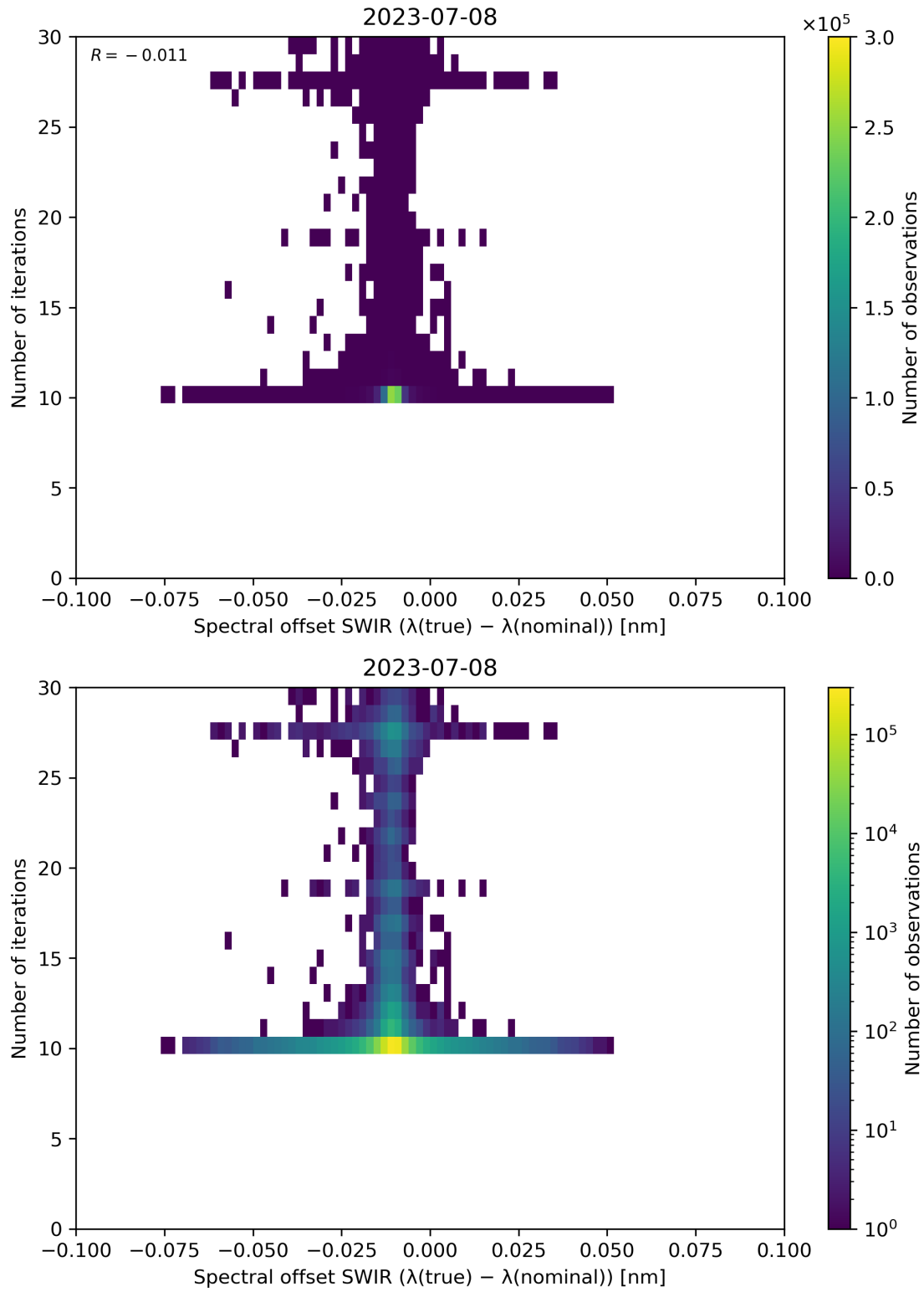
Figure 121: Scatter density plot of “Spectral offset SWIR ( \lambda(\text{true}) - \lambda(\text{nominal}) )” against “Number of iterations” for 2023-07-08 to 2023-07-09.
