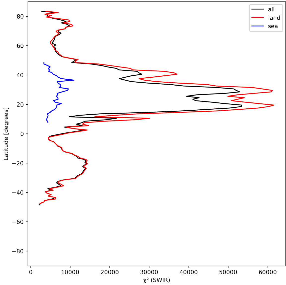
Figure 17: Zonal average of “ \chi^2 (SWIR)” for 2023-07-08 to 2023-07-09.
