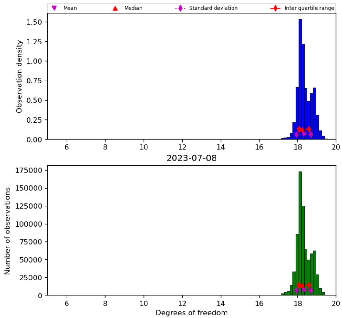
Figure 30: Histogram of “Degrees of freedom” for 2023-07-08 to 2023-07-09
