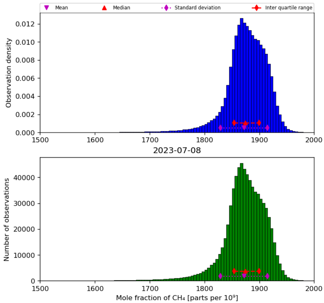
Figure 23: Histogram of "Mole fraction of CH 4 " for 2023-07-08 to 2023-07-09
