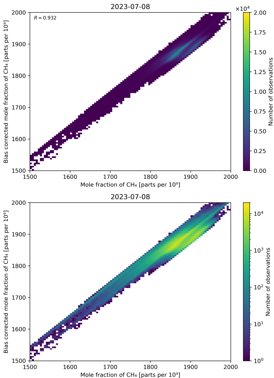
Figure 74: Scatter density plot of “Mole fraction of CH 4 ” against “Bias corrected mole fraction of CH 4 ” for 2023-07-08 to 2023-07-09.
