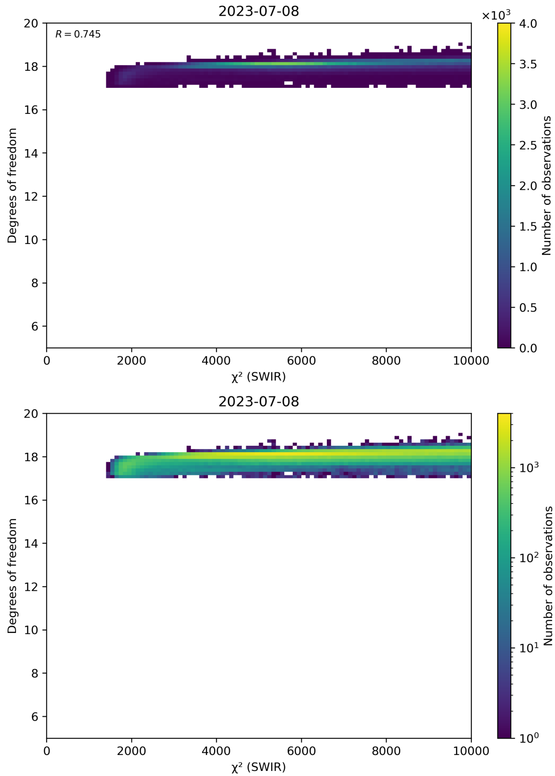
Figure 48: Scatter density plot of “ \chi^2 (SWIR)” against “Degrees of freedom” for 2023-07-08 to 2023-07-09.
