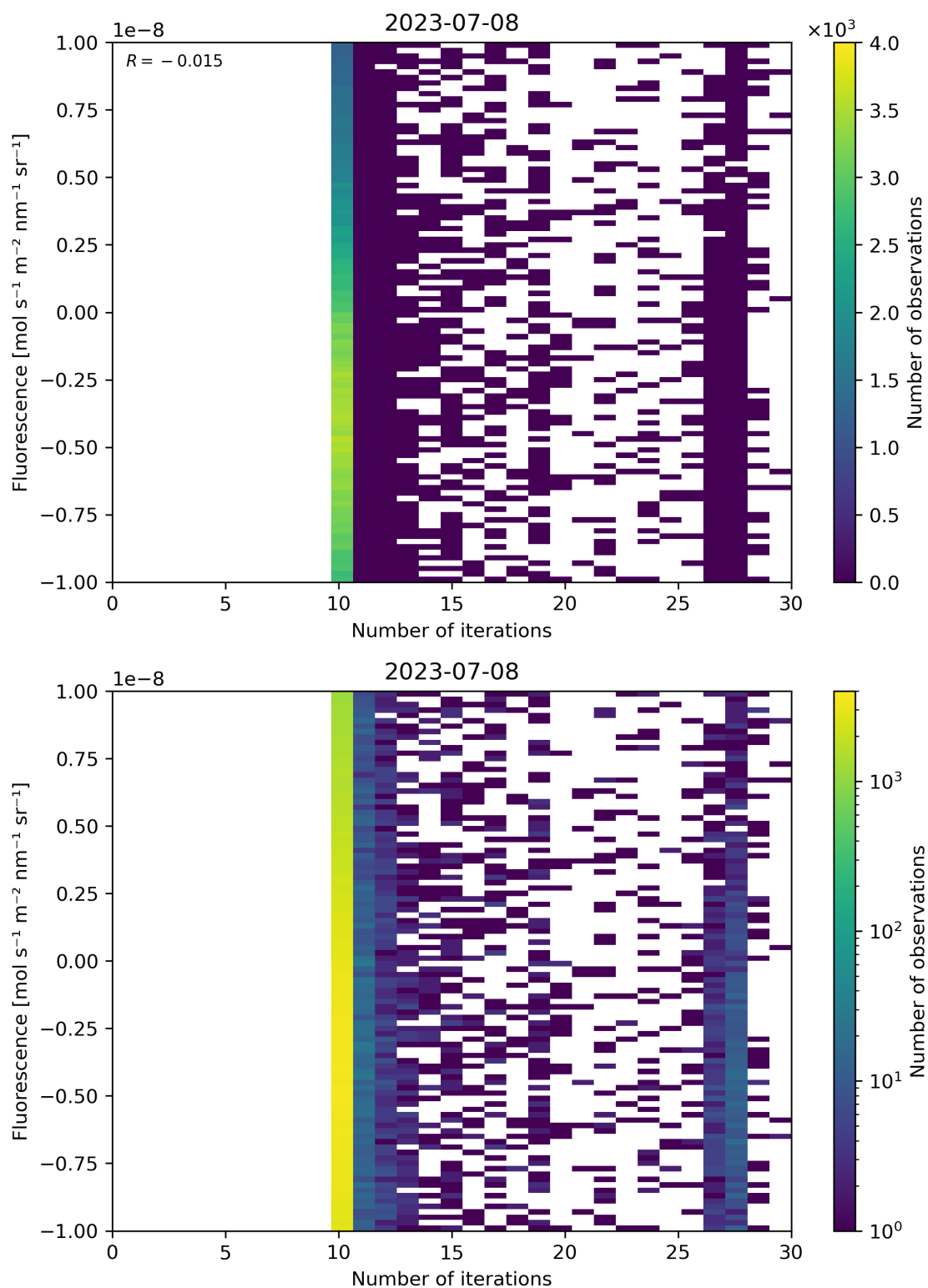
Figure 87: Scatter density plot of “Number of iterations” against “Fluorescence” for 2023-07-08 to 2023-07-09.
