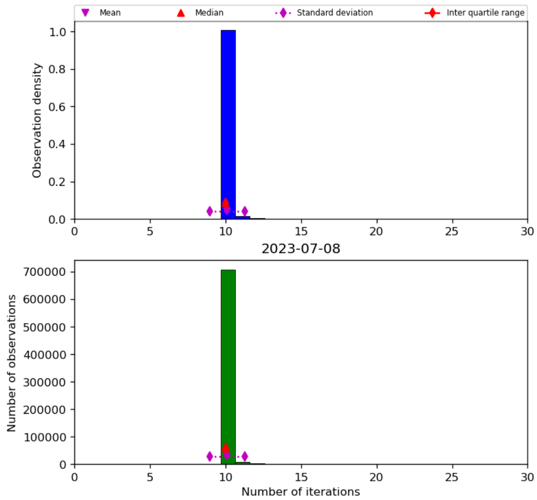
Figure 31: Histogram of “Number of iterations” for 2023-07-08 to 2023-07-09
