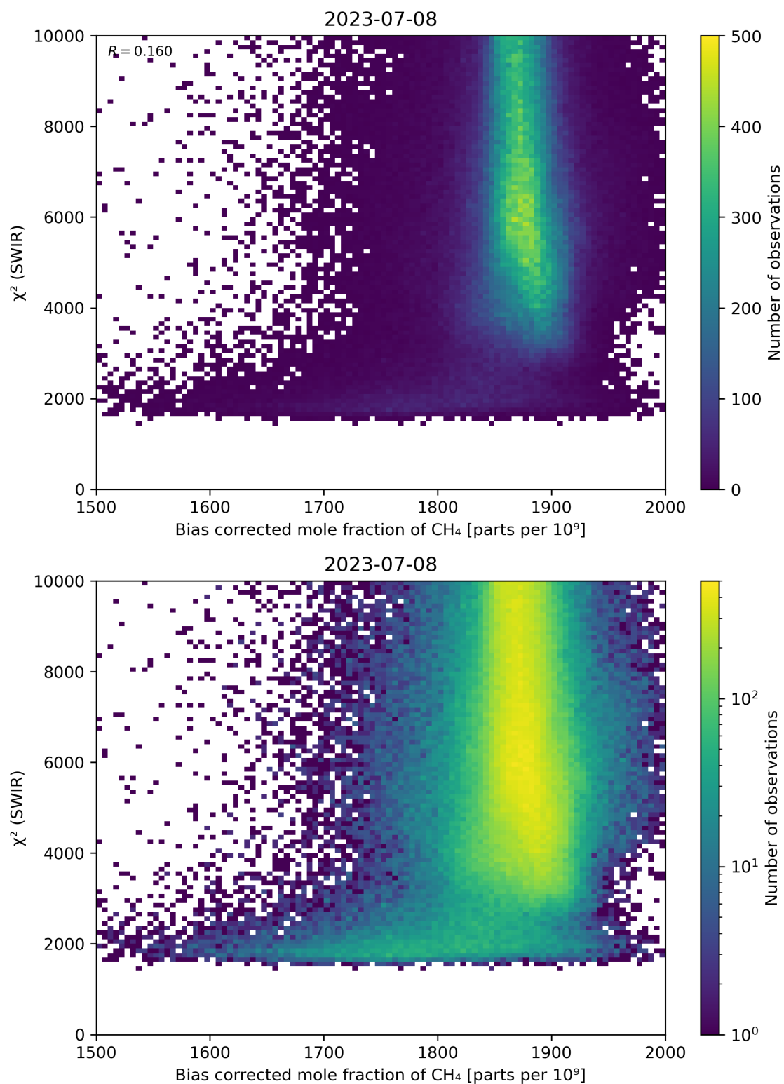
Figure 64: Scatter density plot of “Bias corrected mole fraction of CH 4 ” against “ \chi^2 (SWIR)” for 2023-07-08 to 2023-07-09.
