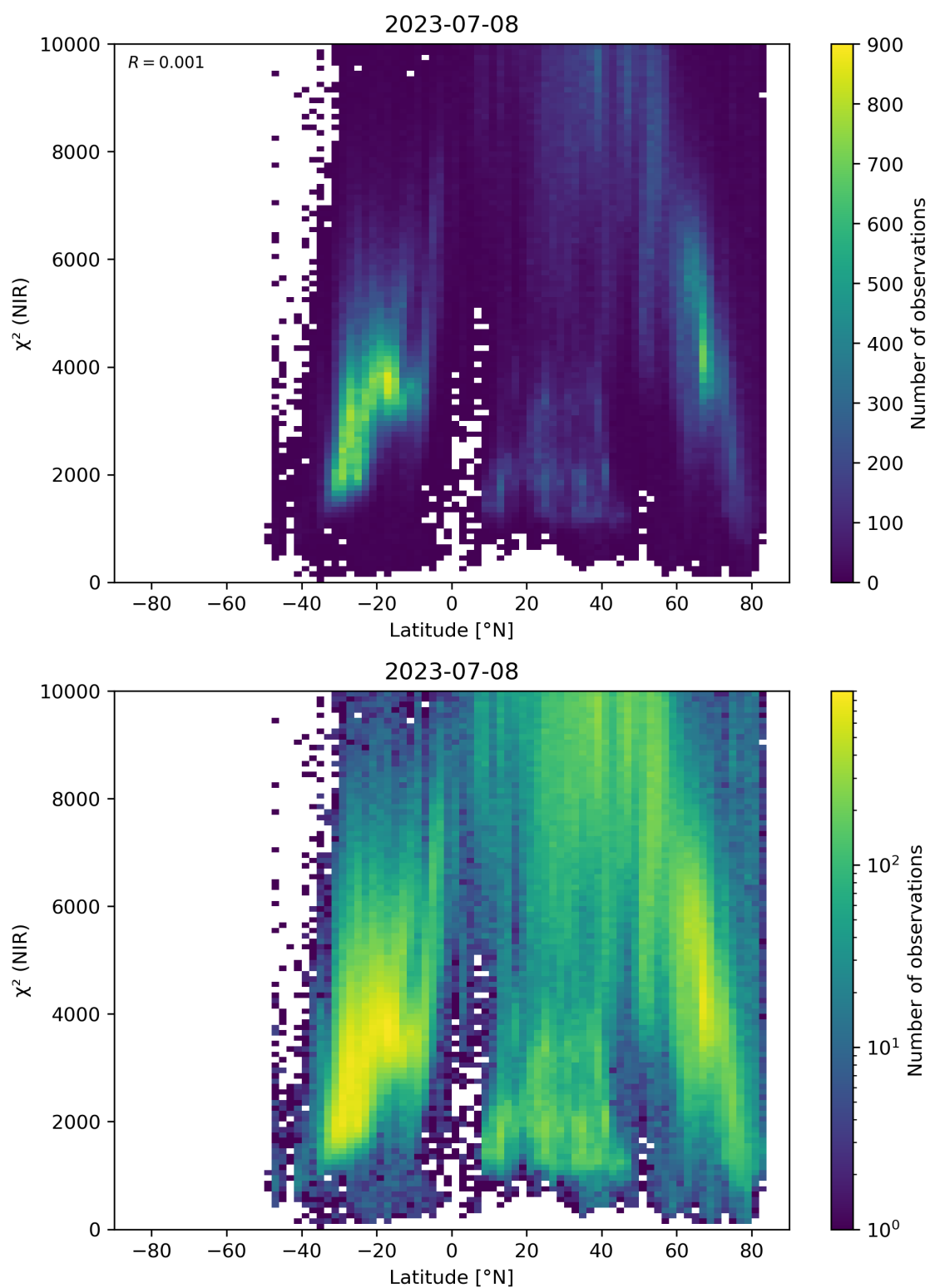
Figure 53: Scatter density plot of “Latitude” against “ \chi^2 (NIR)” for 2023-07-08 to 2023-07-09.
