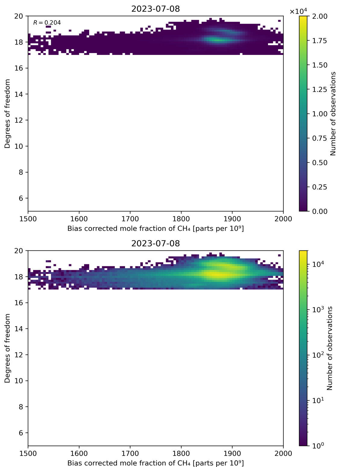
Figure 65: Scatter density plot of “Bias corrected mole fraction of CH 4 ” against “Degrees of freedom” for 2023-07-08 to 2023-07-09.
