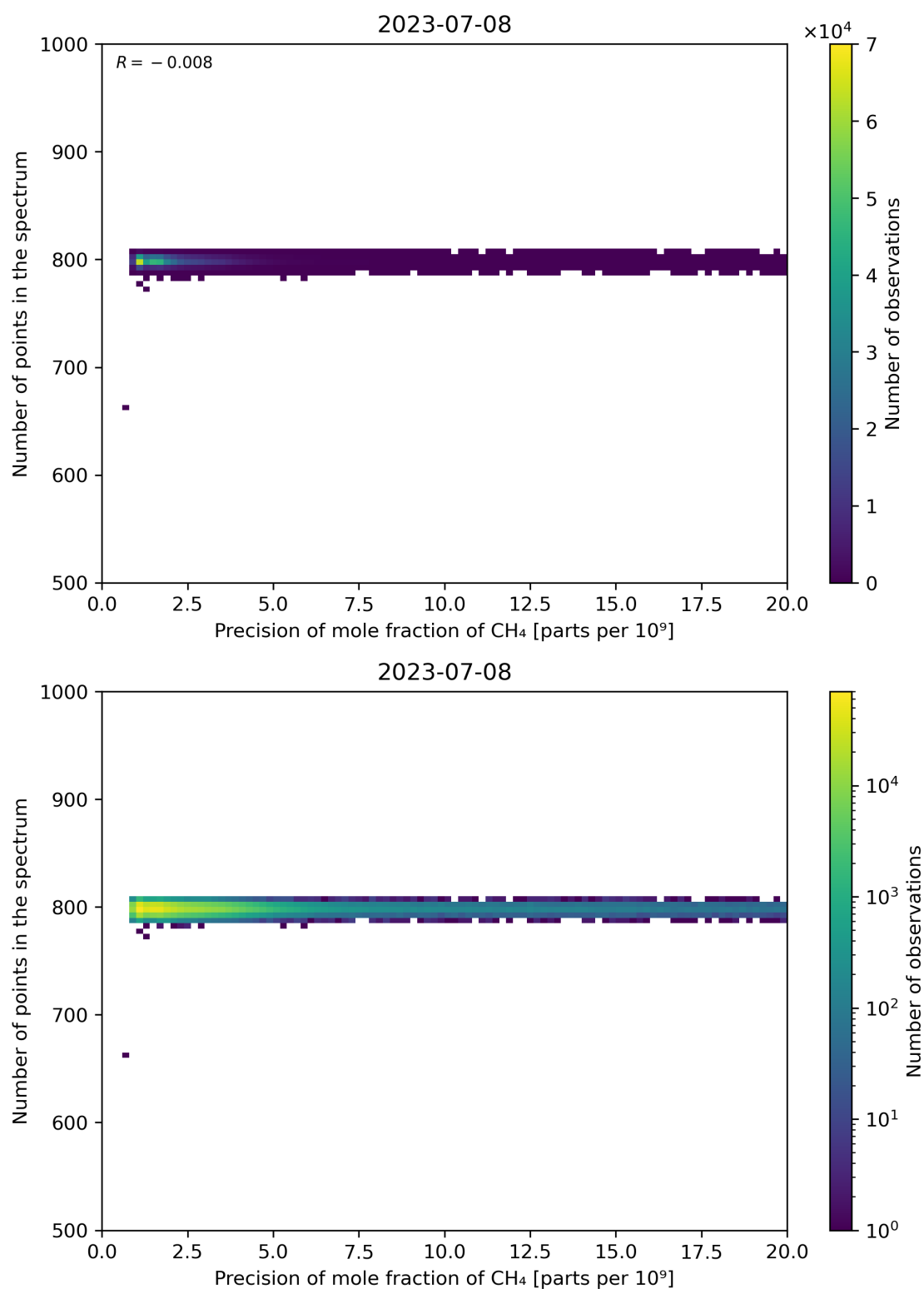
Figure 84: Scatter density plot of “Precision of mole fraction of CH 4 ” against “Number of points in the spectrum” for 2023-07-08 to 2023-07-09.
