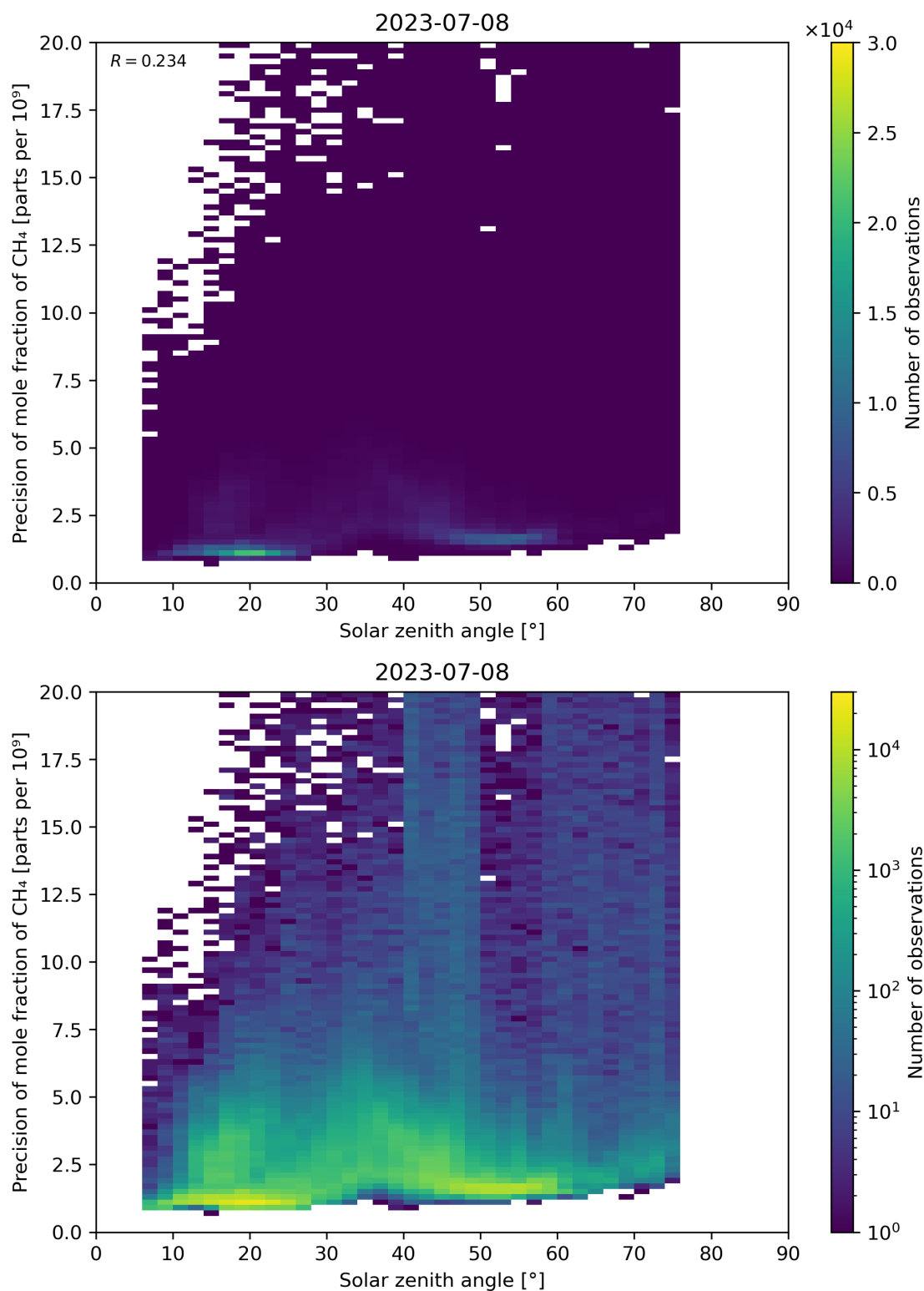
Figure 101: Scatter density plot of “Solar zenith angle” against “Precision of mole fraction of CH 4 ” for 2023-07-08 to 2023-07-09.
