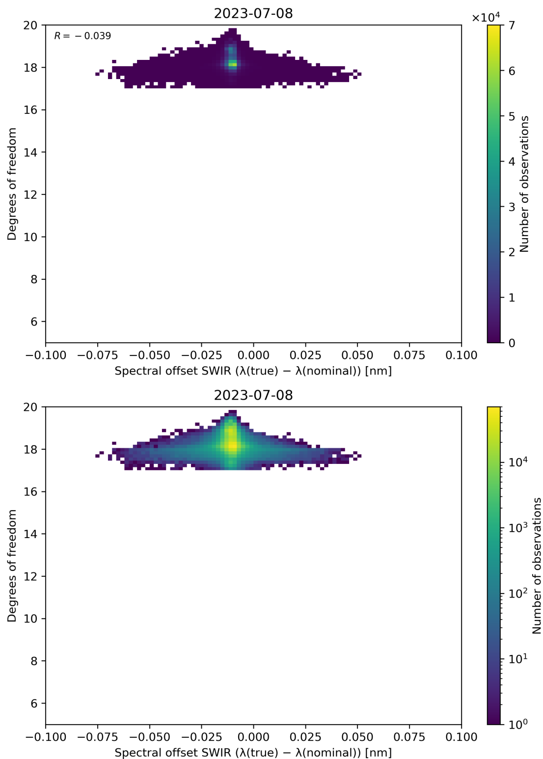
Figure 119: Scatter density plot of “Spectral offset SWIR ( \lambda(\text{true}) - \lambda(\text{nominal}) )” against “Degrees of freedom” for 2023-07-08 to 2023-07-09.
