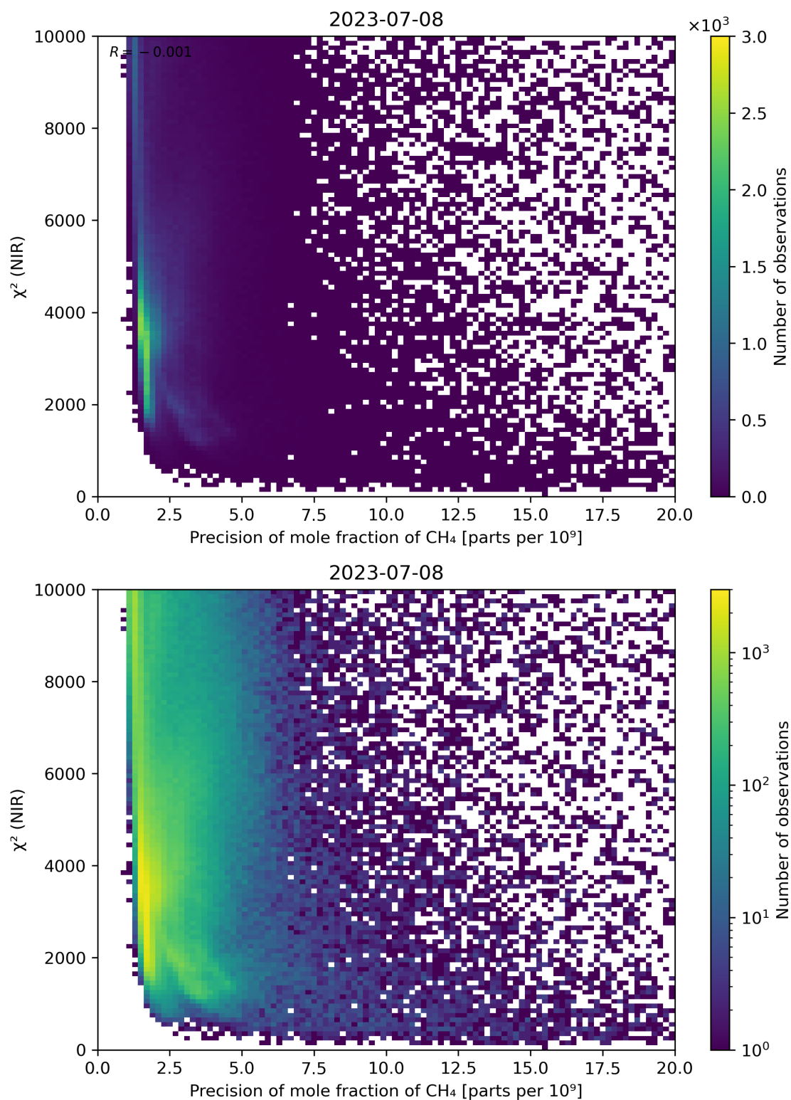
Figure 78: Scatter density plot of “Precision of mole fraction of CH 4 ” against “ \chi^2 (NIR)” for 2023-07-08 to 2023-07-09.
