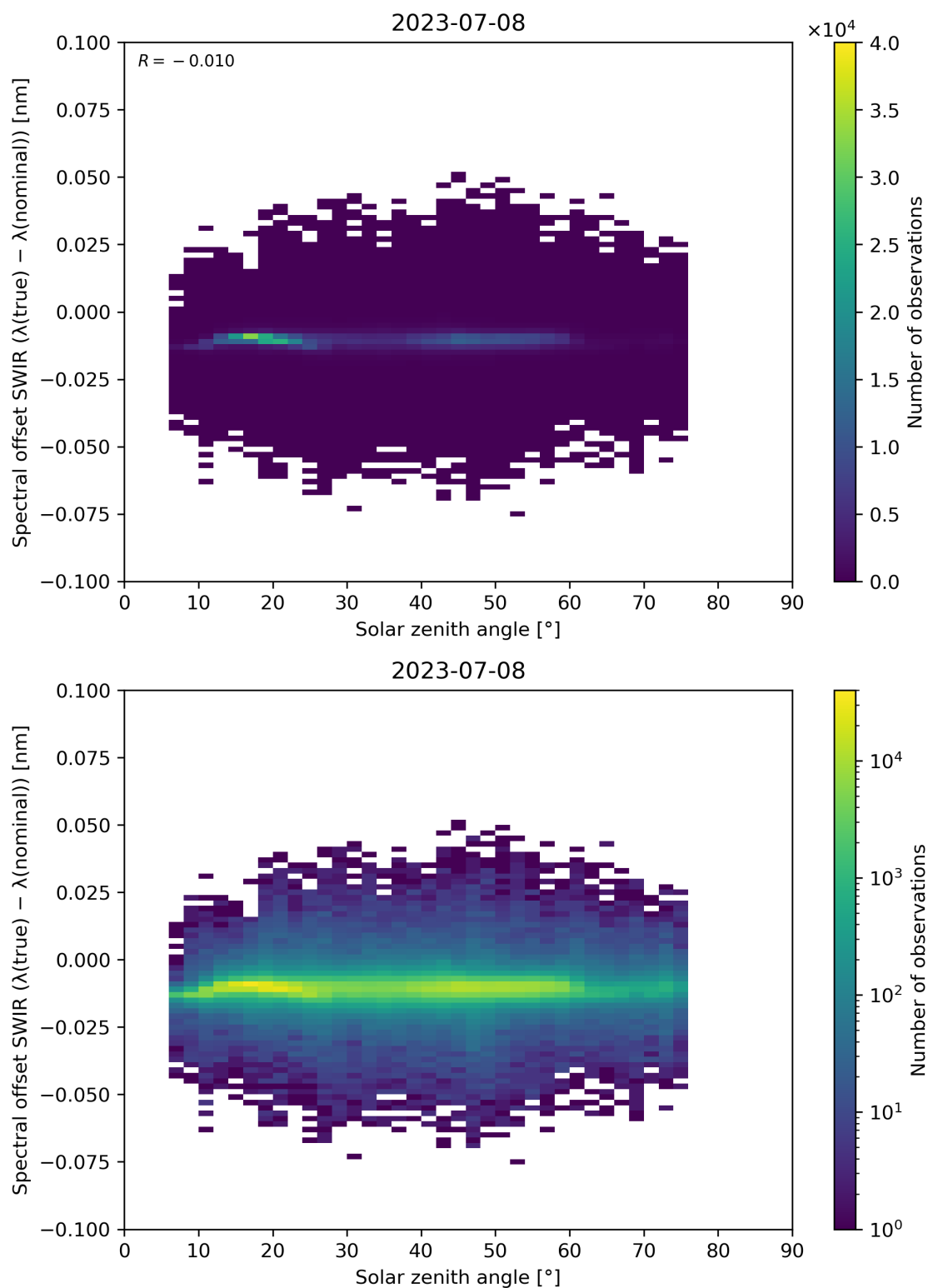
Figure 104: Scatter density plot of “Solar zenith angle” against “Spectral offset SWIR ( \lambda(\text{true}) - \lambda(\text{nominal}) )” for 2023-07-08 to 2023-07-09.
