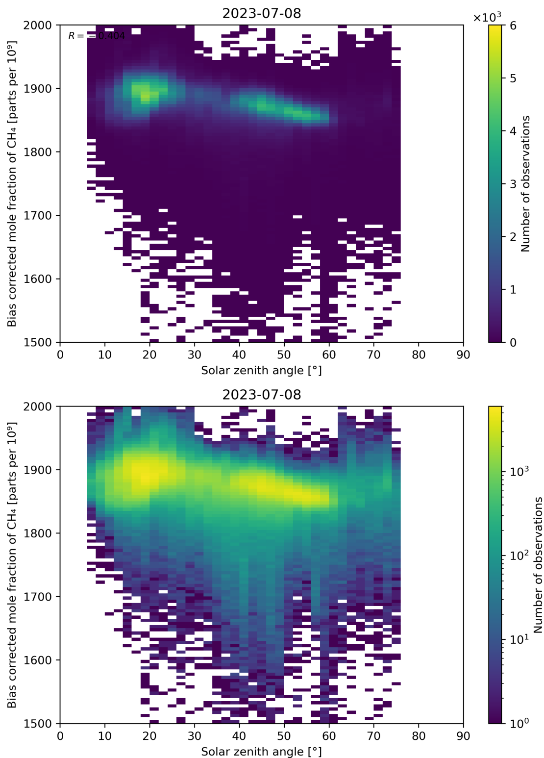
Figure 100: Scatter density plot of “Solar zenith angle” against “Bias corrected mole fraction of CH 4 ” for 2023-07-08 to 2023-07-09.
