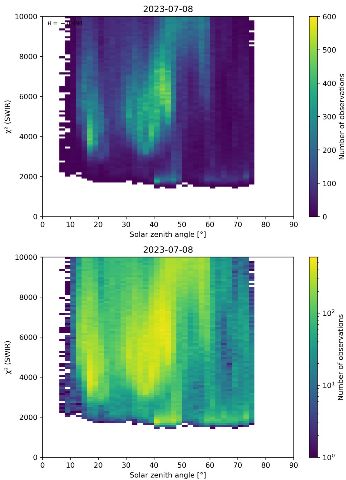
Figure 95: Scatter density plot of “Solar zenith angle” against “ \chi^2 (SWIR)” for 2023-07-08 to 2023-07-09.
