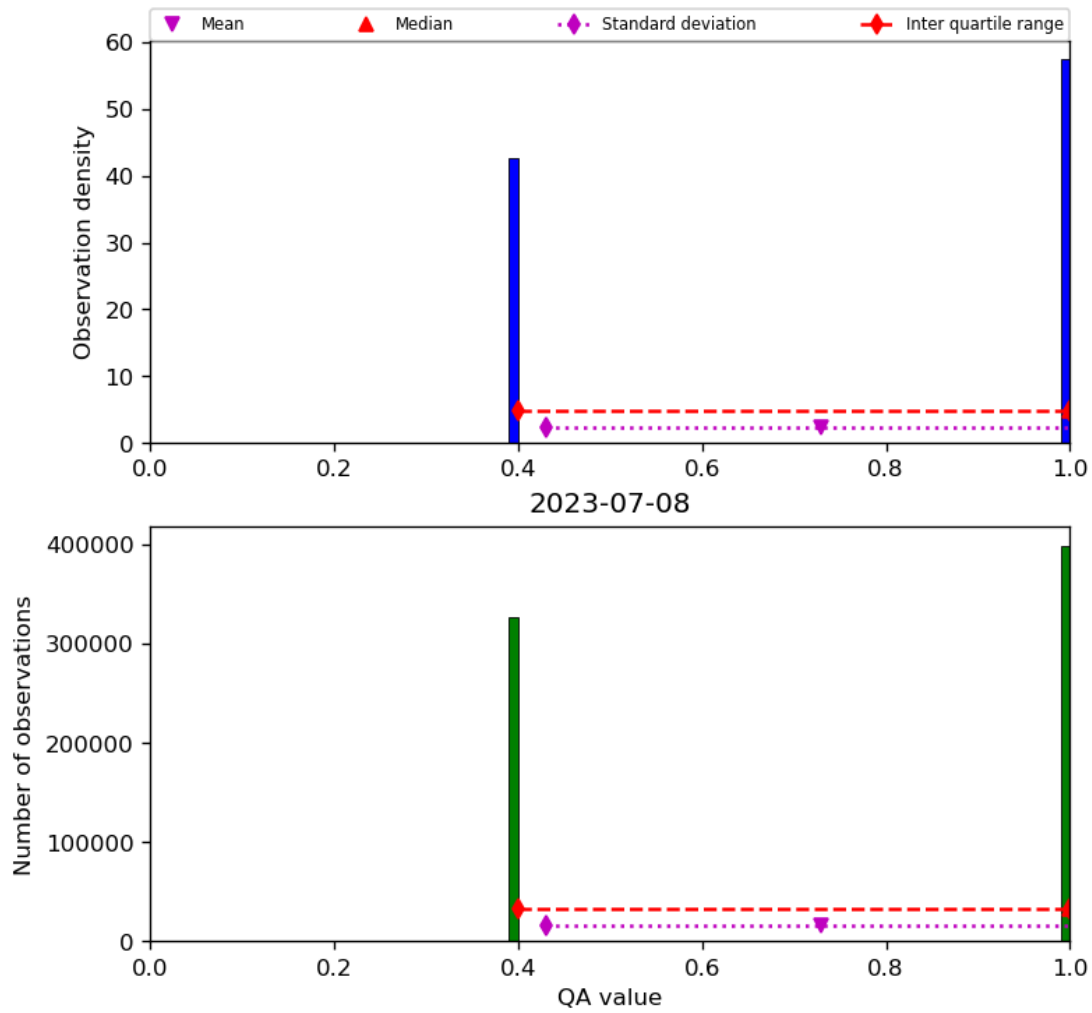
Figure 22: Histogram of “QA value” for 2023-07-08 to 2023-07-09
