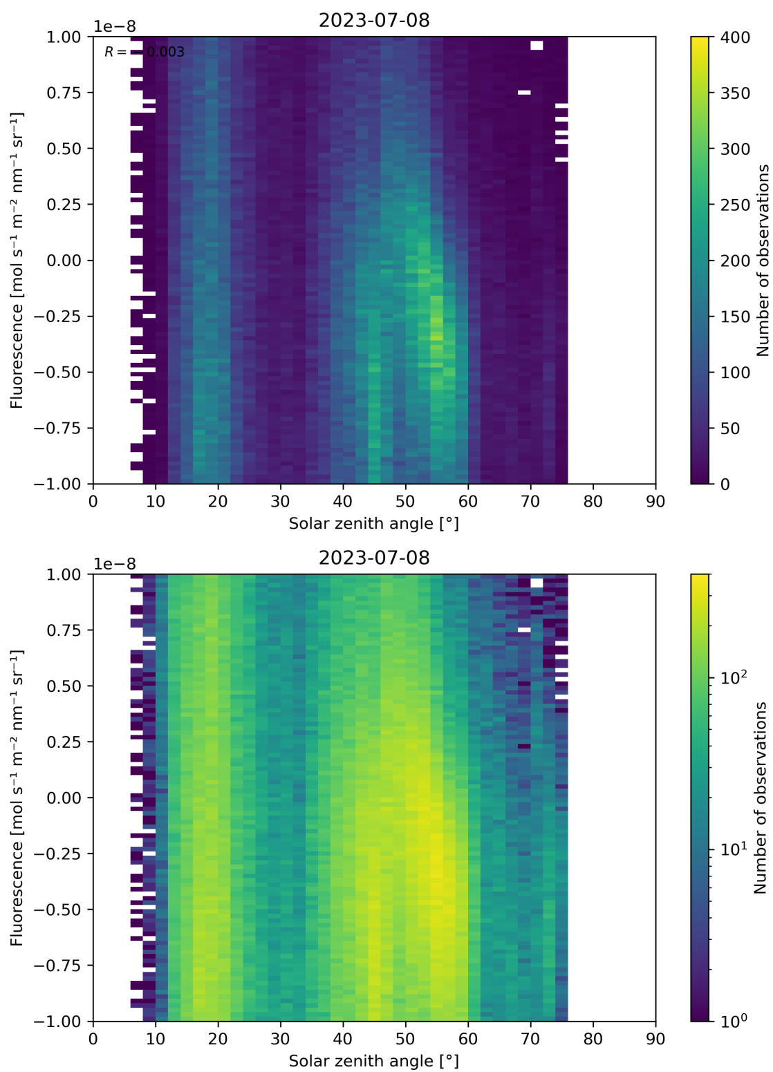
Figure 97: Scatter density plot of “Solar zenith angle” against “Fluorescence” for 2023-07-08 to 2023-07-09.
