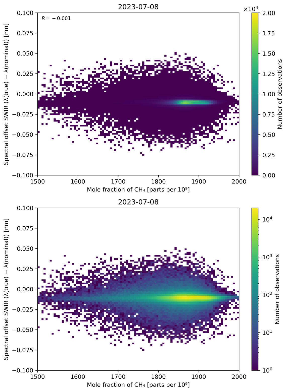
Figure 86: Scatter density plot of “Mole fraction of CH 4 ” against “Spectral offset SWIR ( \lambda(\text{true}) - \lambda(\text{nominal}) )” for 2023-07-08 to 2023-07-09.
