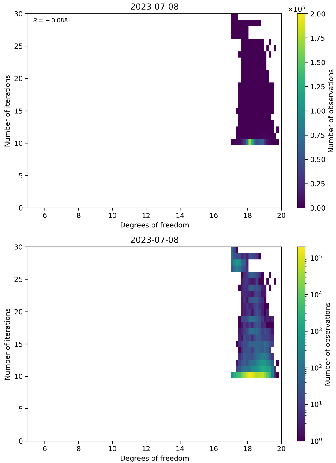
Figure 52: Scatter density plot of “Degrees of freedom” against “Number of iterations” for 2023-07-08 to 2023-07-09.
