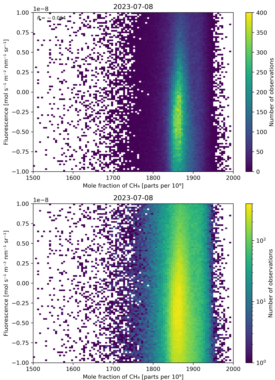
Figure 73: Scatter density plot of “Mole fraction of \text{CH}_4 ” against “Fluorescence” for 2023-07-08 to 2023-07-09.
