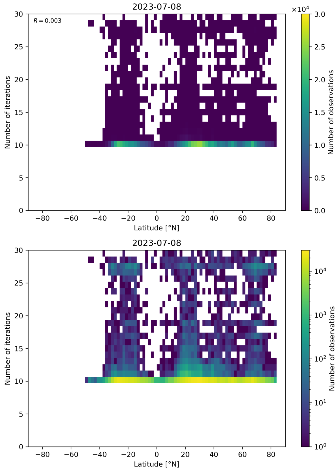
Figure 60: Scatter density plot of “Latitude” against “Number of iterations” for 2023-07-08 to 2023-07-09.
