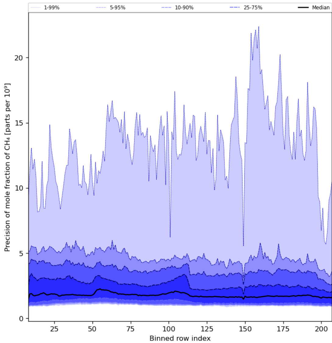
Figure 35: Along track statistics of “Precision of mole fraction of CH 4 ” for 2023-07-08 to 2023-07-09
