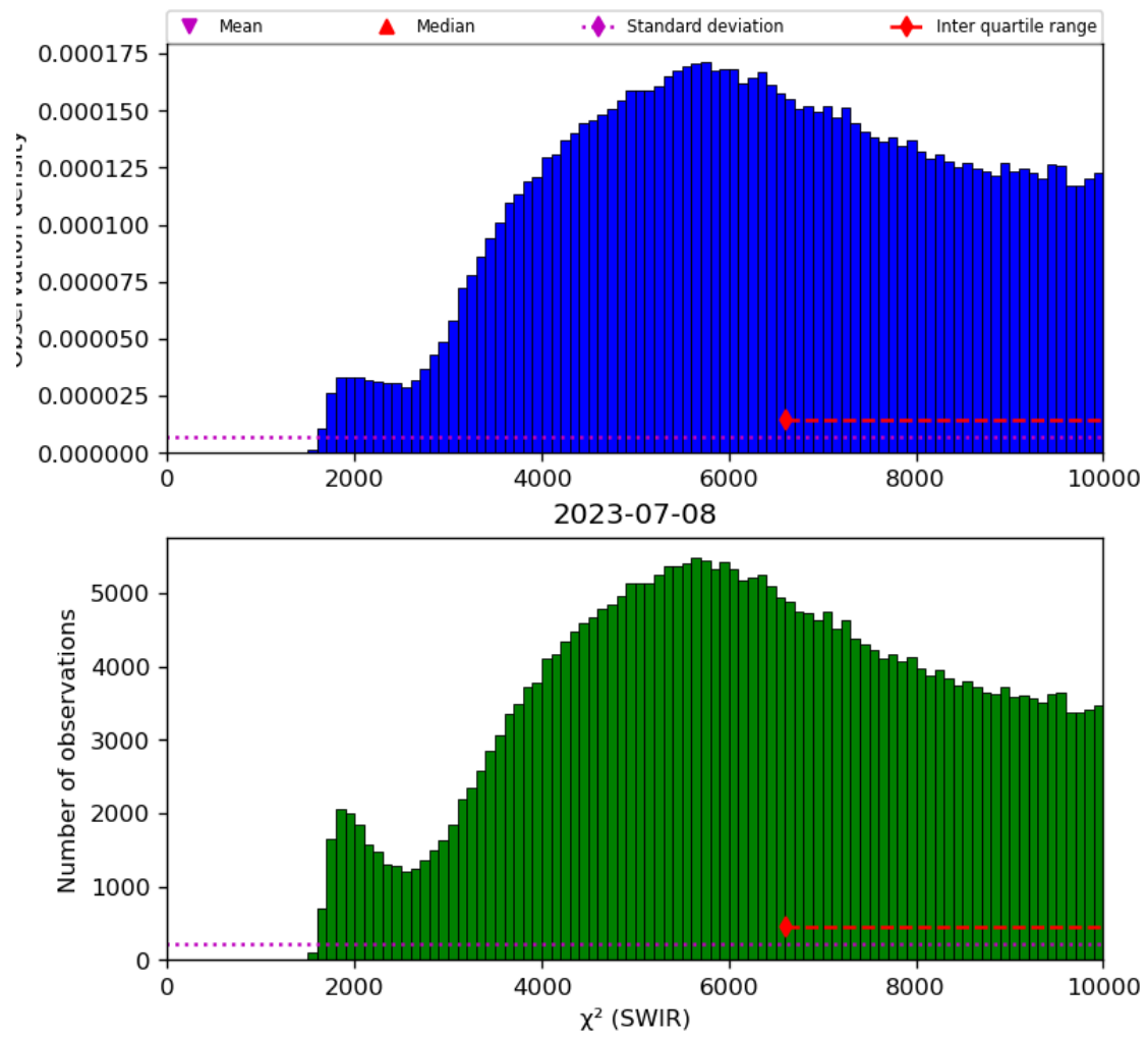
Figure 28: Histogram of “ \chi^2 (SWIR)” for 2023-07-08 to 2023-07-09
