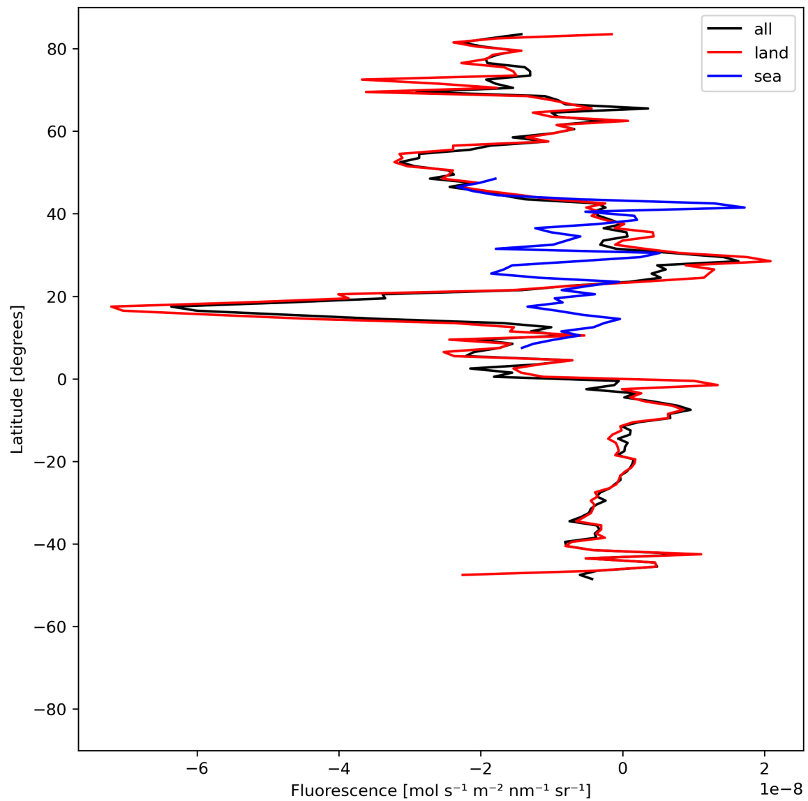
Figure 21: Zonal average of “Fluorescence” for 2023-07-08 to 2023-07-09.
