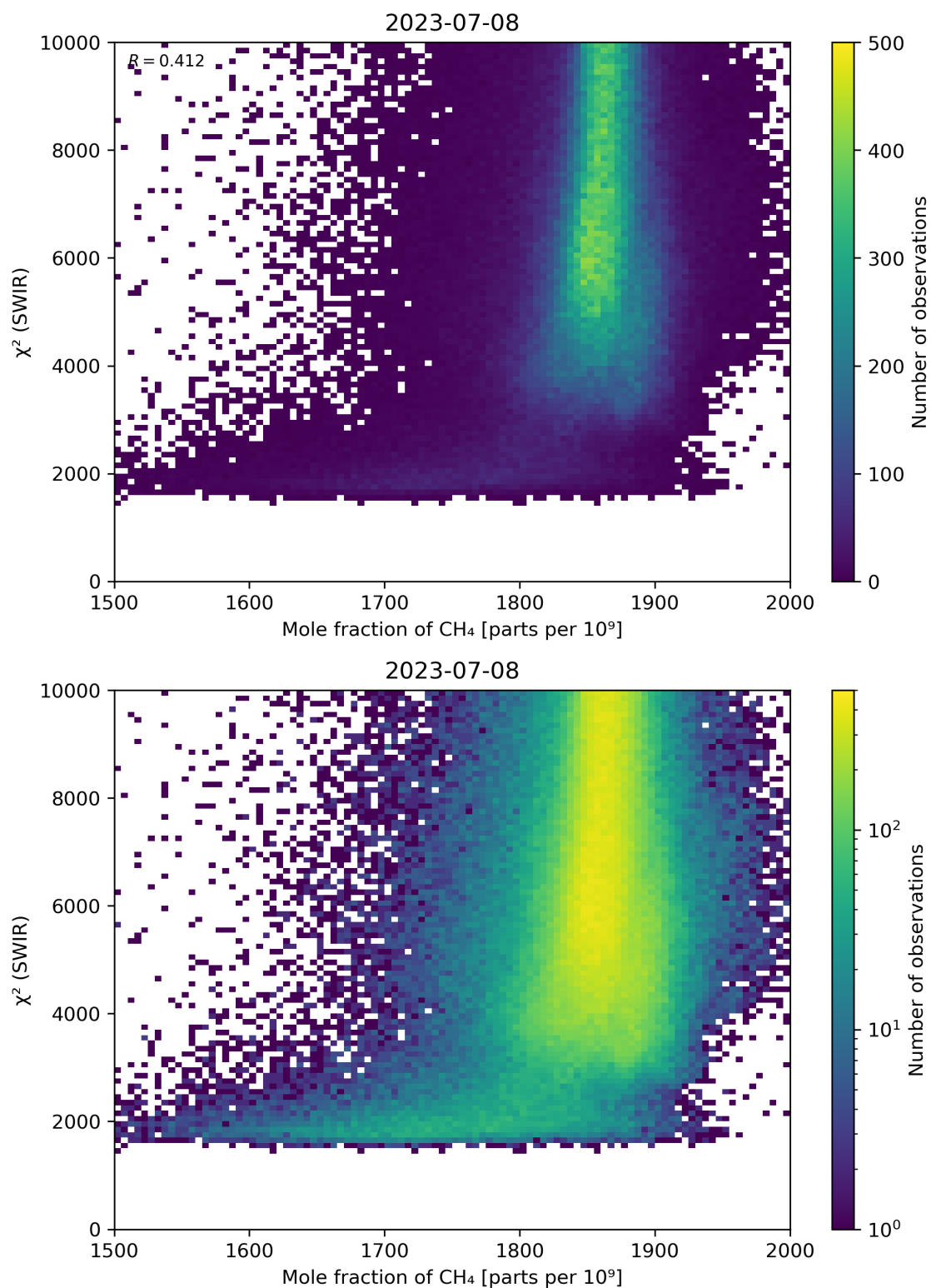
Figure 71: Scatter density plot of “Mole fraction of \text{CH}_4 ” against “ \chi^2 (SWIR)” for 2023-07-08 to 2023-07-09.
