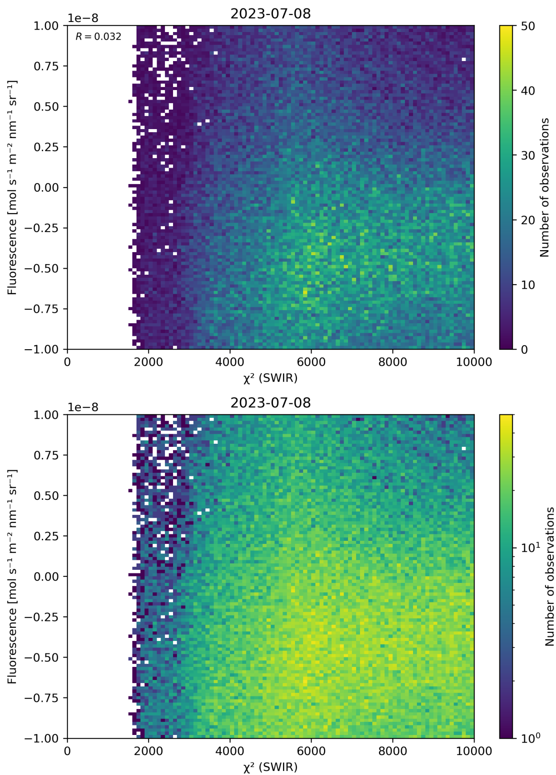
Figure 49: Scatter density plot of “ \chi^2 (SWIR)” against “Fluorescence” for 2023-07-08 to 2023-07-09.
