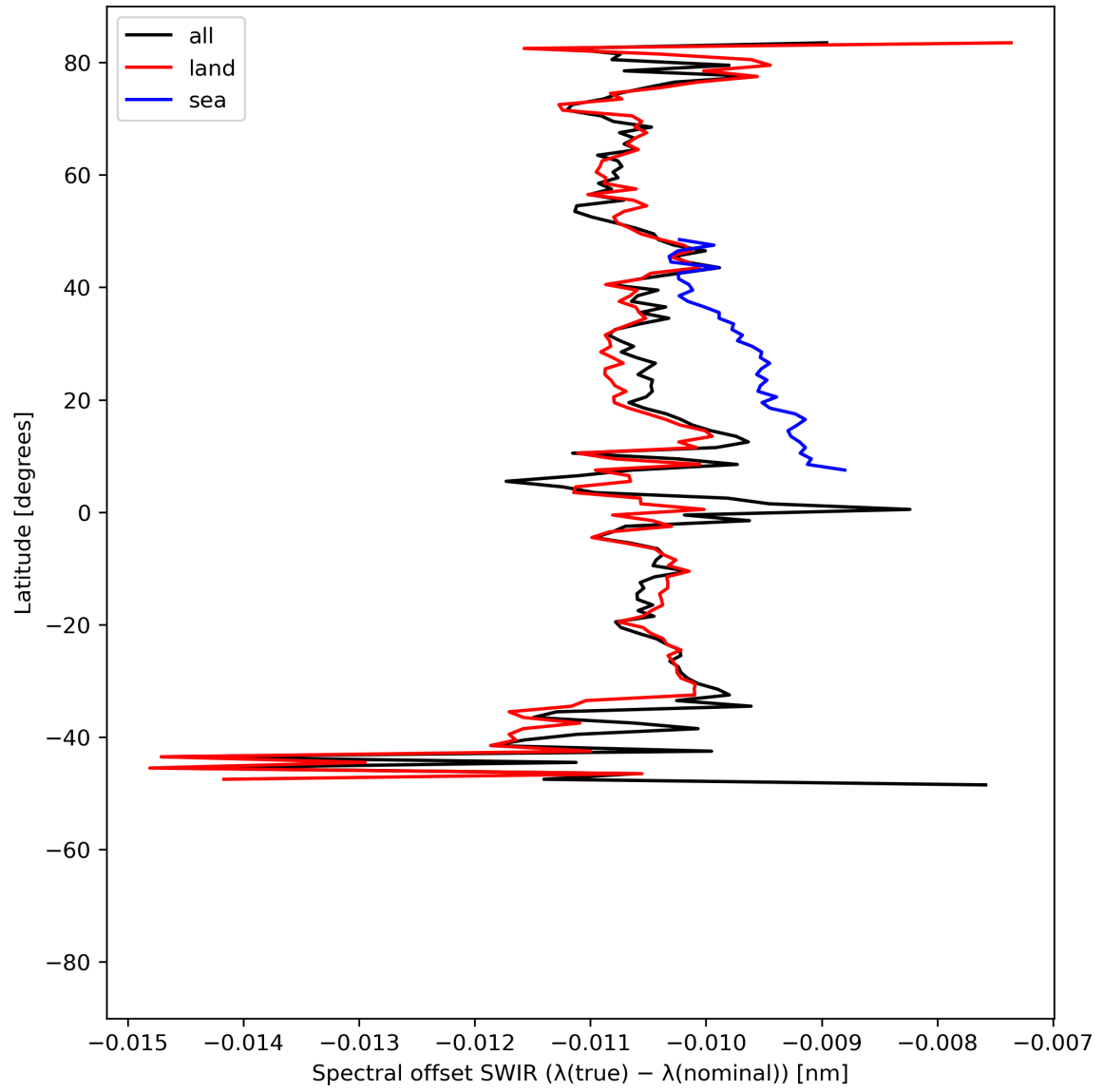
Figure 16: Zonal average of “Spectral offset SWIR ( \lambda(\text{true}) - \lambda(\text{nominal}) )” for 2023-07-08 to 2023-07-09.
