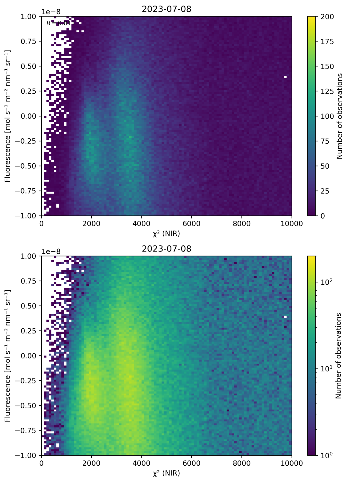
Figure 45: Scatter density plot of “ \chi^2 (NIR)” against “Fluorescence” for 2023-07-08 to 2023-07-09.
