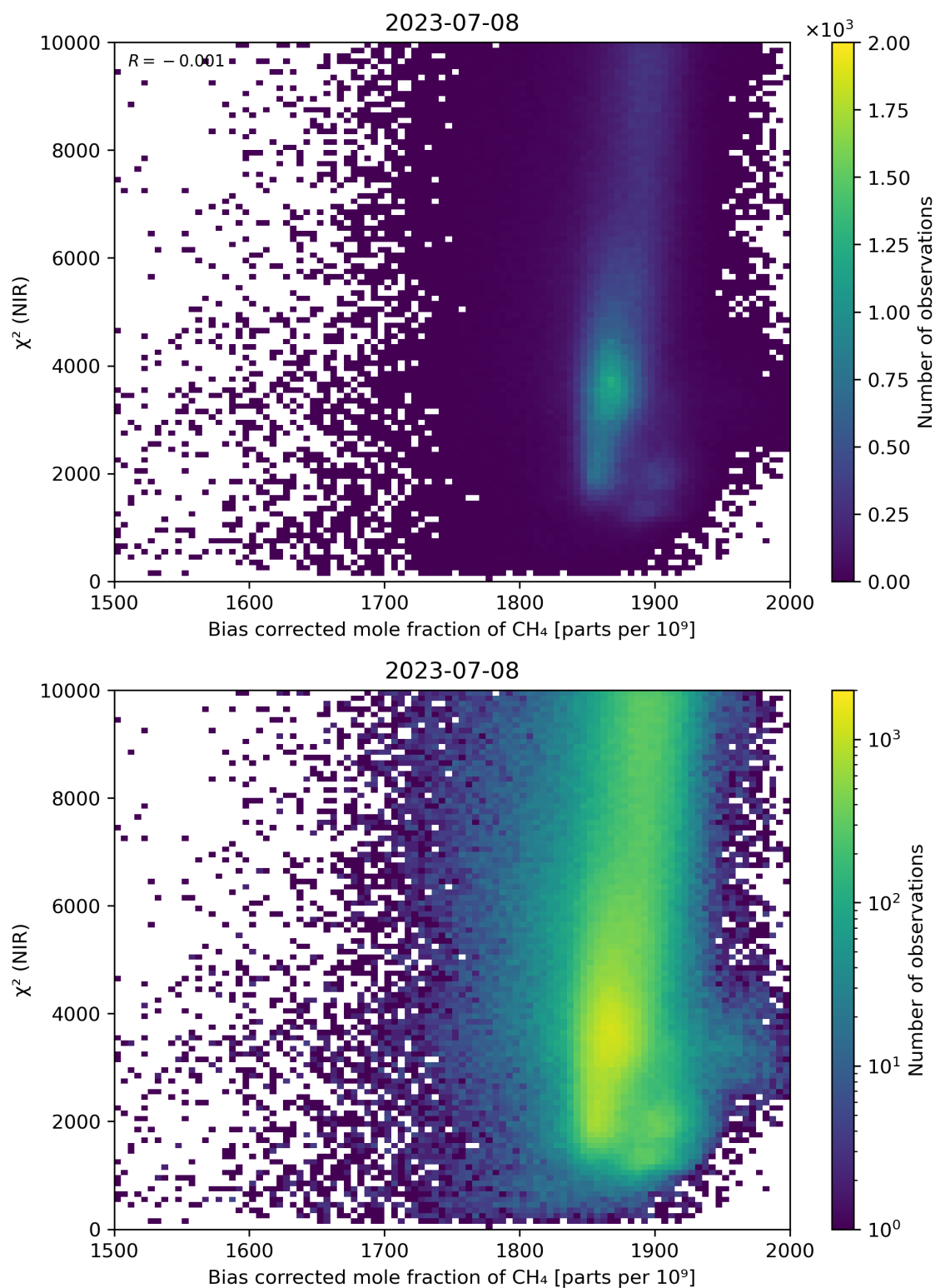
Figure 63: Scatter density plot of “Bias corrected mole fraction of \text{CH}_4 ” against “ \chi^2 (NIR)” for 2023-07-08 to 2023-07-09.
