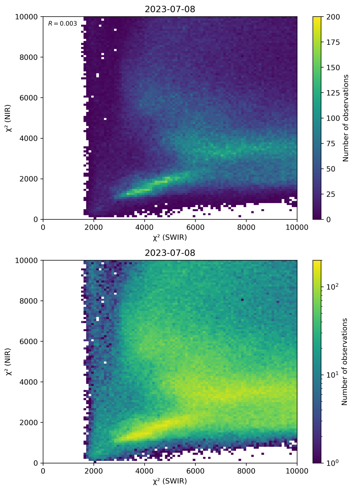
Figure 47: Scatter density plot of “ \chi^2 (SWIR)” against “ \chi^2 (NIR)” for 2023-07-08 to 2023-07-09.
