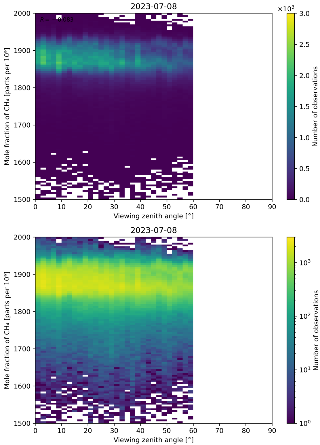
Figure 110: Scatter density plot of “Viewing zenith angle” against “Mole fraction of CH 4 ” for 2023-07-08 to 2023-07-09.
