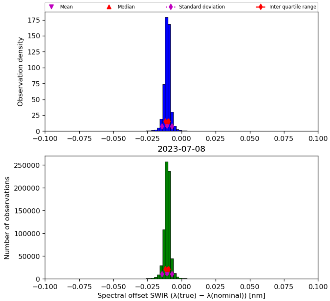
Figure 27: Histogram of “Spectral offset SWIR ( \lambda(\text{true}) - \lambda(\text{nominal}) )” for 2023-07-08 to 2023-07-09
