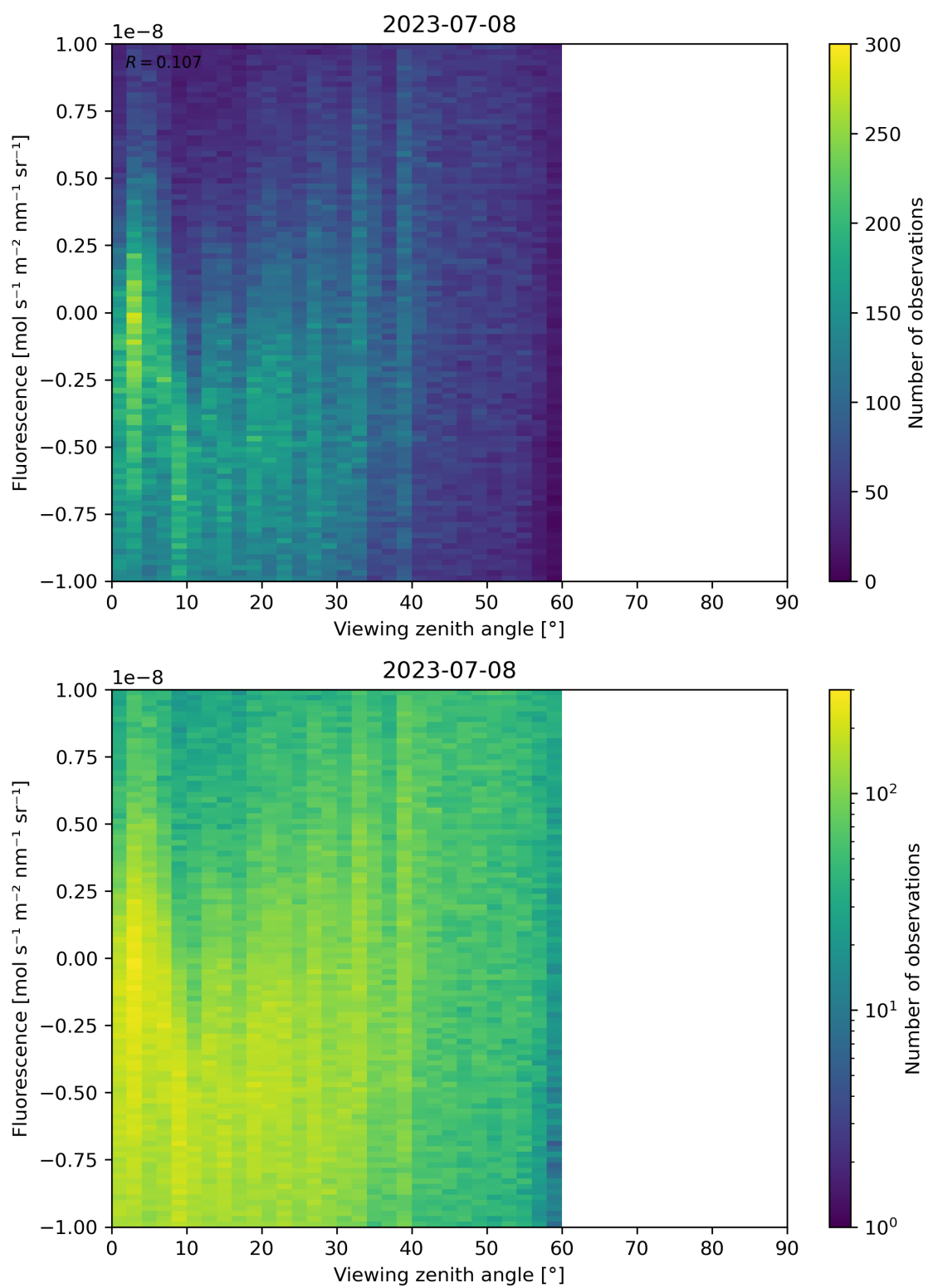
Figure 108: Scatter density plot of “Viewing zenith angle” against “Fluorescence” for 2023-07-08 to 2023-07-09.
