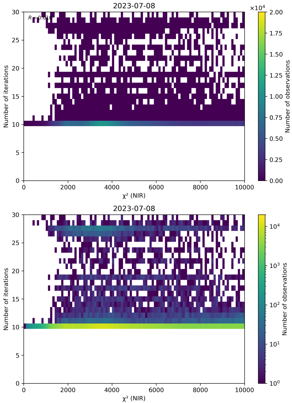
Figure 46: Scatter density plot of “ \chi^2 (NIR)” against “Number of iterations” for 2023-07-08 to 2023-07-09.
