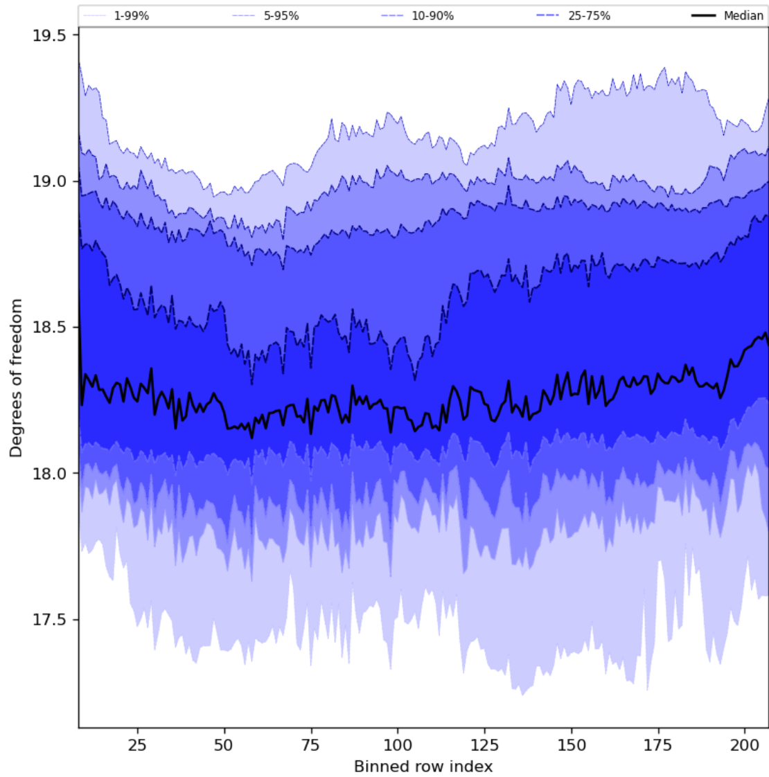
Figure 41: Along track statistics of “Degrees of freedom” for 2023-07-08 to 2023-07-09
