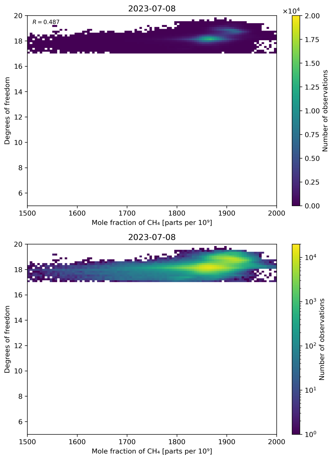
Figure 72: Scatter density plot of “Mole fraction of CH 4 ” against “Degrees of freedom” for 2023-07-08 to 2023-07-09.
