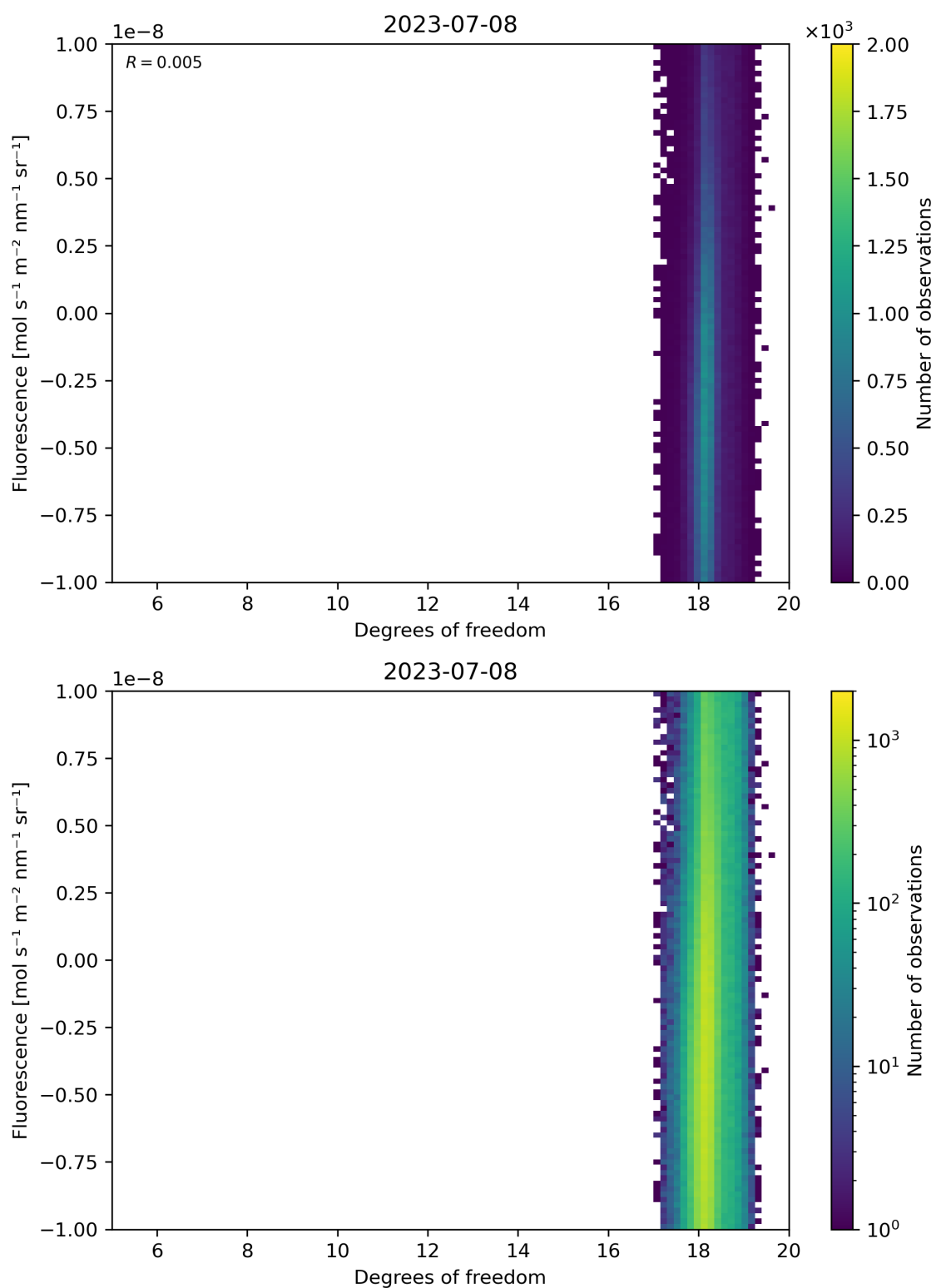
Figure 51: Scatter density plot of “Degrees of freedom” against “Fluorescence” for 2023-07-08 to 2023-07-09.
