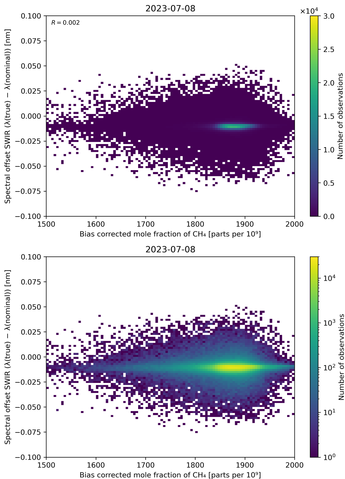
Figure 69: Scatter density plot of “Bias corrected mole fraction of \text{CH}_4 ” against “Spectral offset SWIR ( \lambda(\text{true}) - \lambda(\text{nominal}) )” for 2023-07-08 to 2023-07-09.
