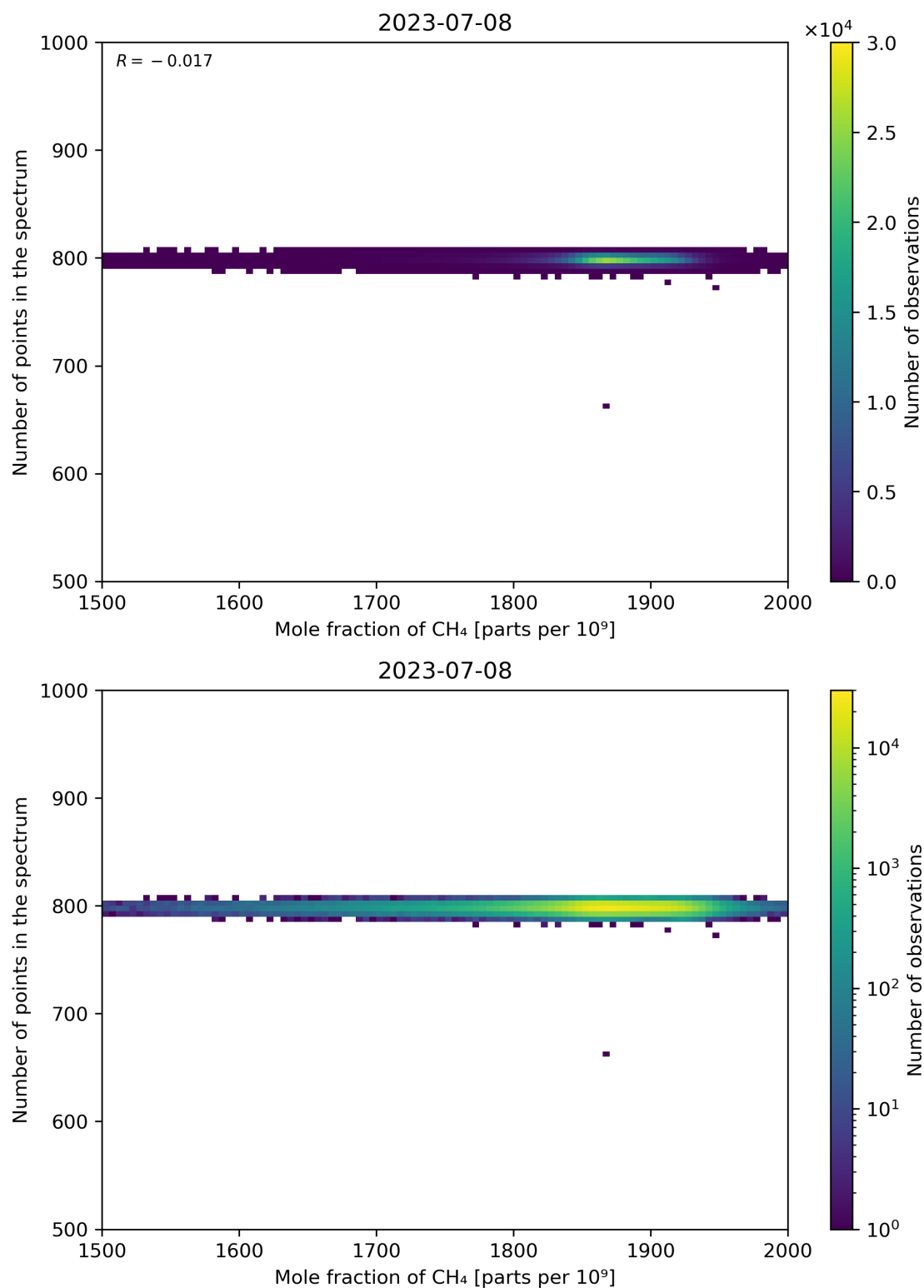
Figure 77: Scatter density plot of “Mole fraction of CH 4 ” against “Number of points in the spectrum” for 2023-07-08 to 2023-07-09.
