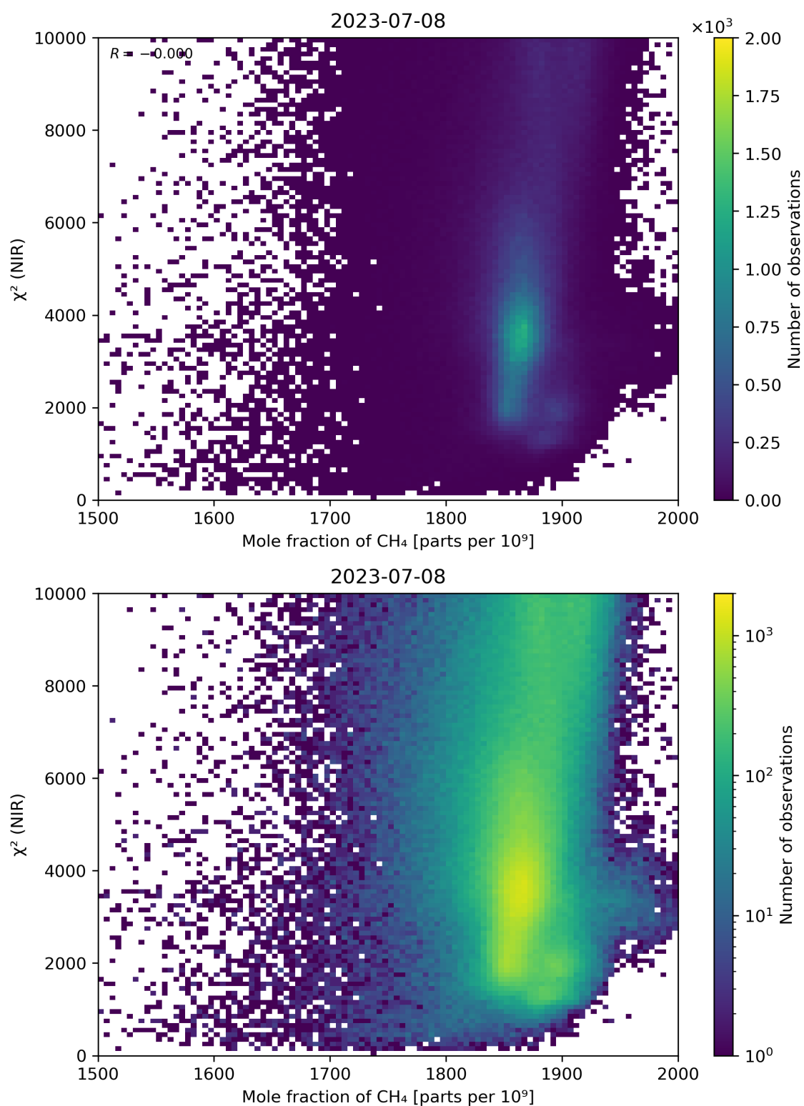
Figure 70: Scatter density plot of “Mole fraction of \text{CH}_4 ” against “ \chi^2 (NIR)” for 2023-07-08 to 2023-07-09.
