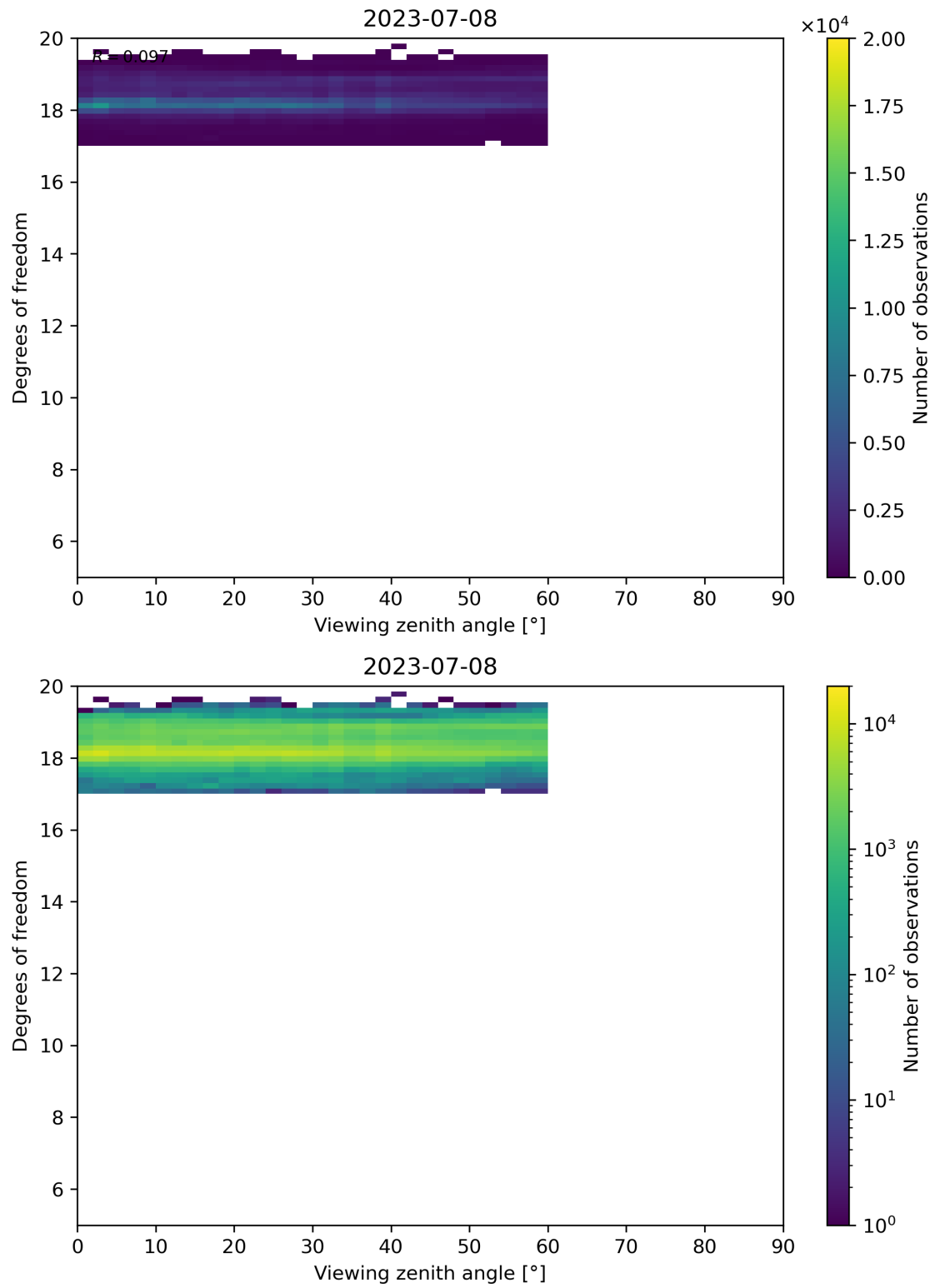
Figure 107: Scatter density plot of “Viewing zenith angle” against “Degrees of freedom” for 2023-07-08 to 2023-07-09.
