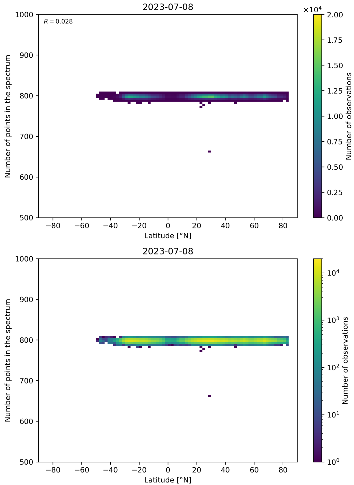
Figure 61: Scatter density plot of “Latitude” against “Number of points in the spectrum” for 2023-07-08 to 2023-07-09.
