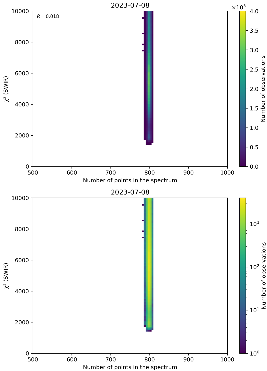
Figure 89: Scatter density plot of “Number of points in the spectrum” against “ \chi^2 (SWIR)” for 2023-07-08 to 2023-07-09.
