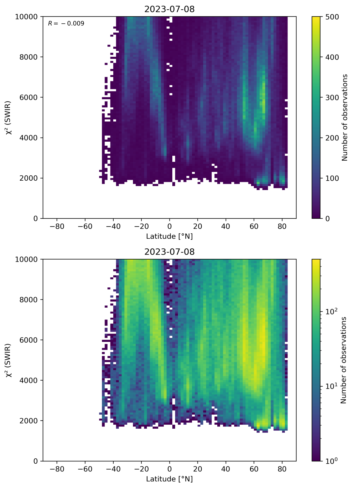
Figure 54: Scatter density plot of “Latitude” against “ \chi^2 (SWIR)” for 2023-07-08 to 2023-07-09.
