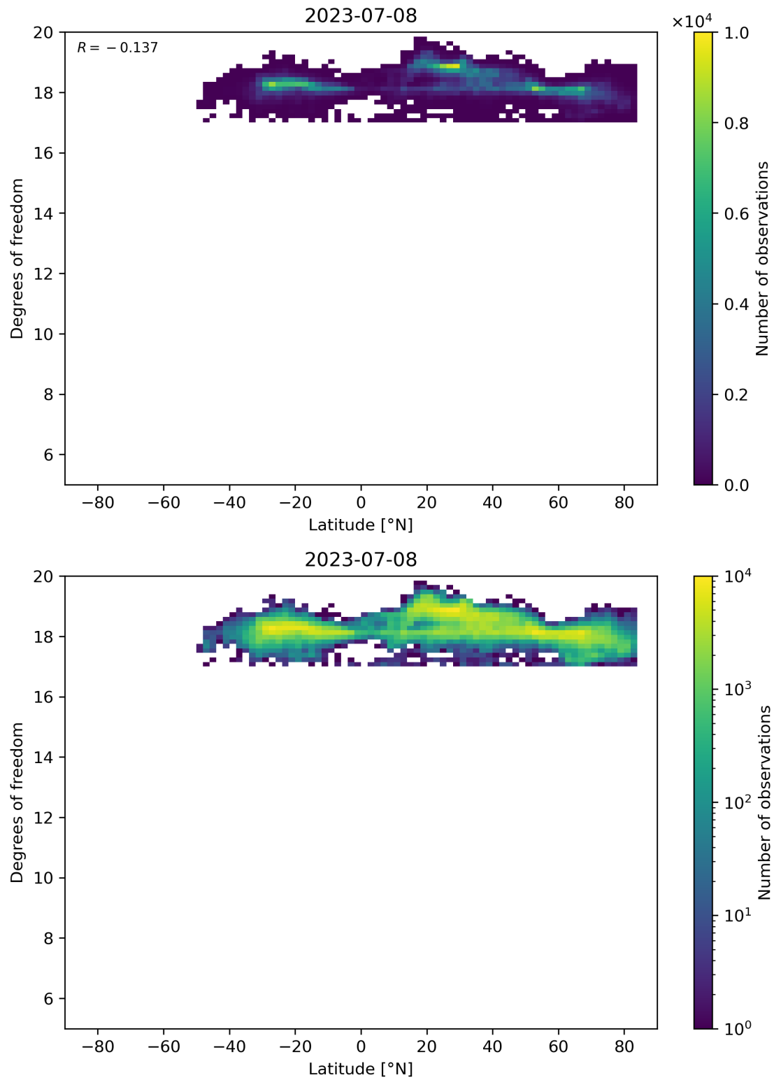
Figure 55: Scatter density plot of “Latitude” against “Degrees of freedom” for 2023-07-08 to 2023-07-09.
