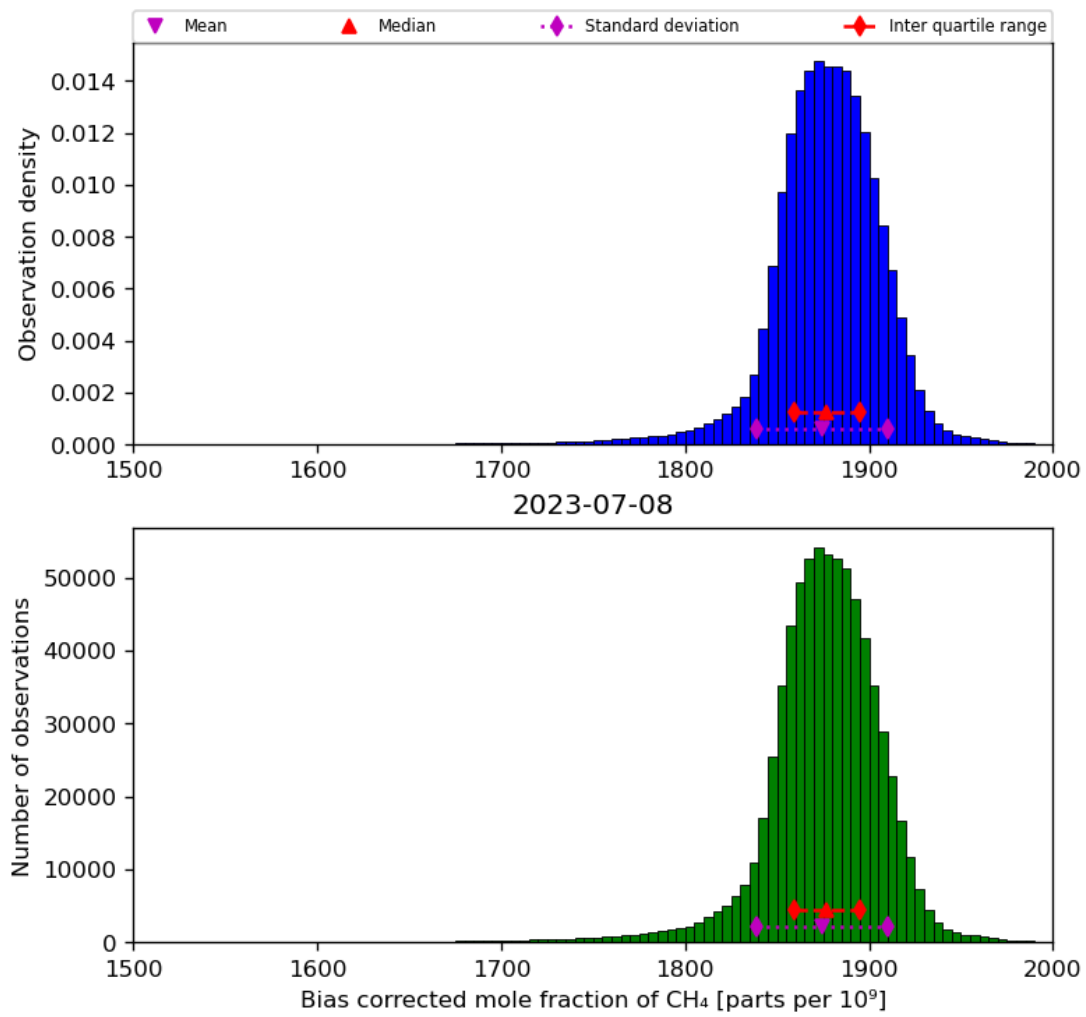
Figure 25: Histogram of “Bias corrected mole fraction of CH 4 ” for 2023-07-08 to 2023-07-09
