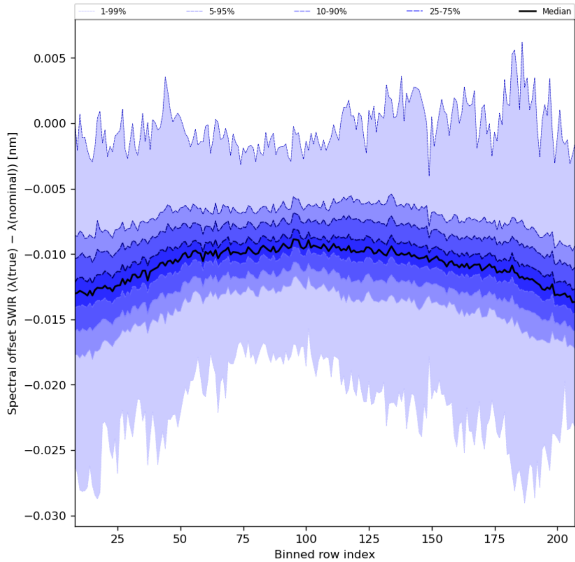
Figure 38: Along track statistics of “Spectral offset SWIR ( \lambda(\text{true}) - \lambda(\text{nominal}) )” for 2023-07-08 to 2023-07-09
