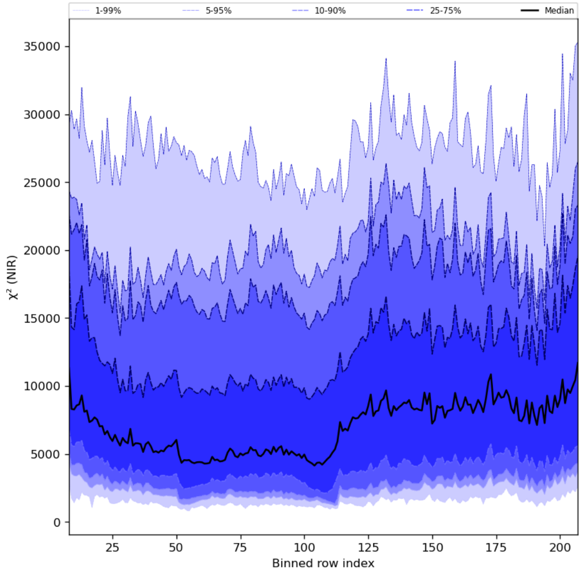
Figure 40: Along track statistics of “ \chi^2 (NIR)” for 2023-07-08 to 2023-07-09
