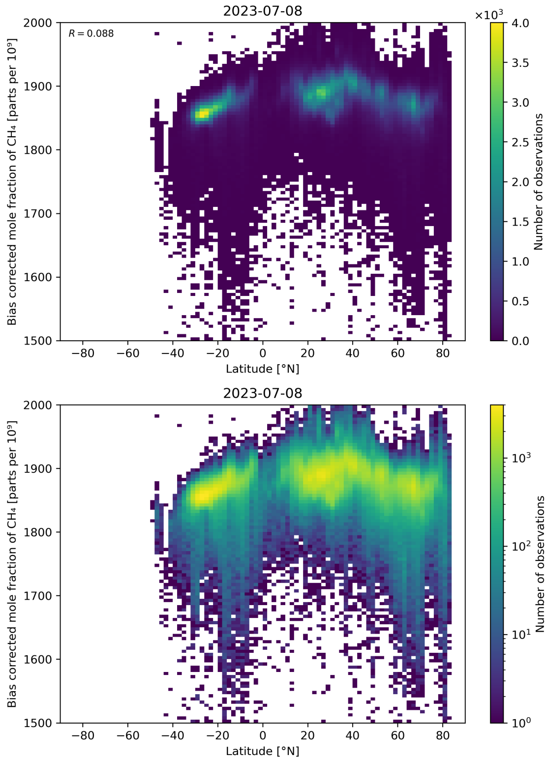
Figure 58: Scatter density plot of “Latitude” against “Bias corrected mole fraction of \text{CH}_4 ” for 2023-07-08 to 2023-07-09.
