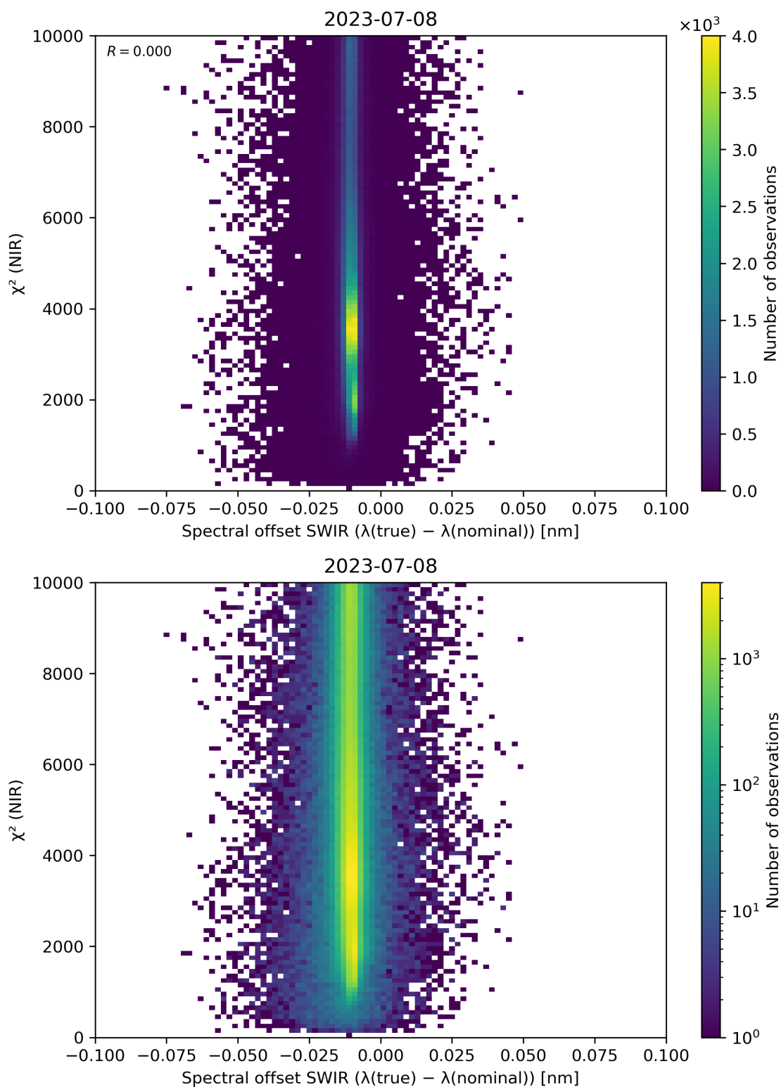
Figure 117: Scatter density plot of “Spectral offset SWIR ( \lambda(\text{true}) - \lambda(\text{nominal}) )” against “ \chi^2 (NIR)” for 2023-07-08 to 2023-07-09.
