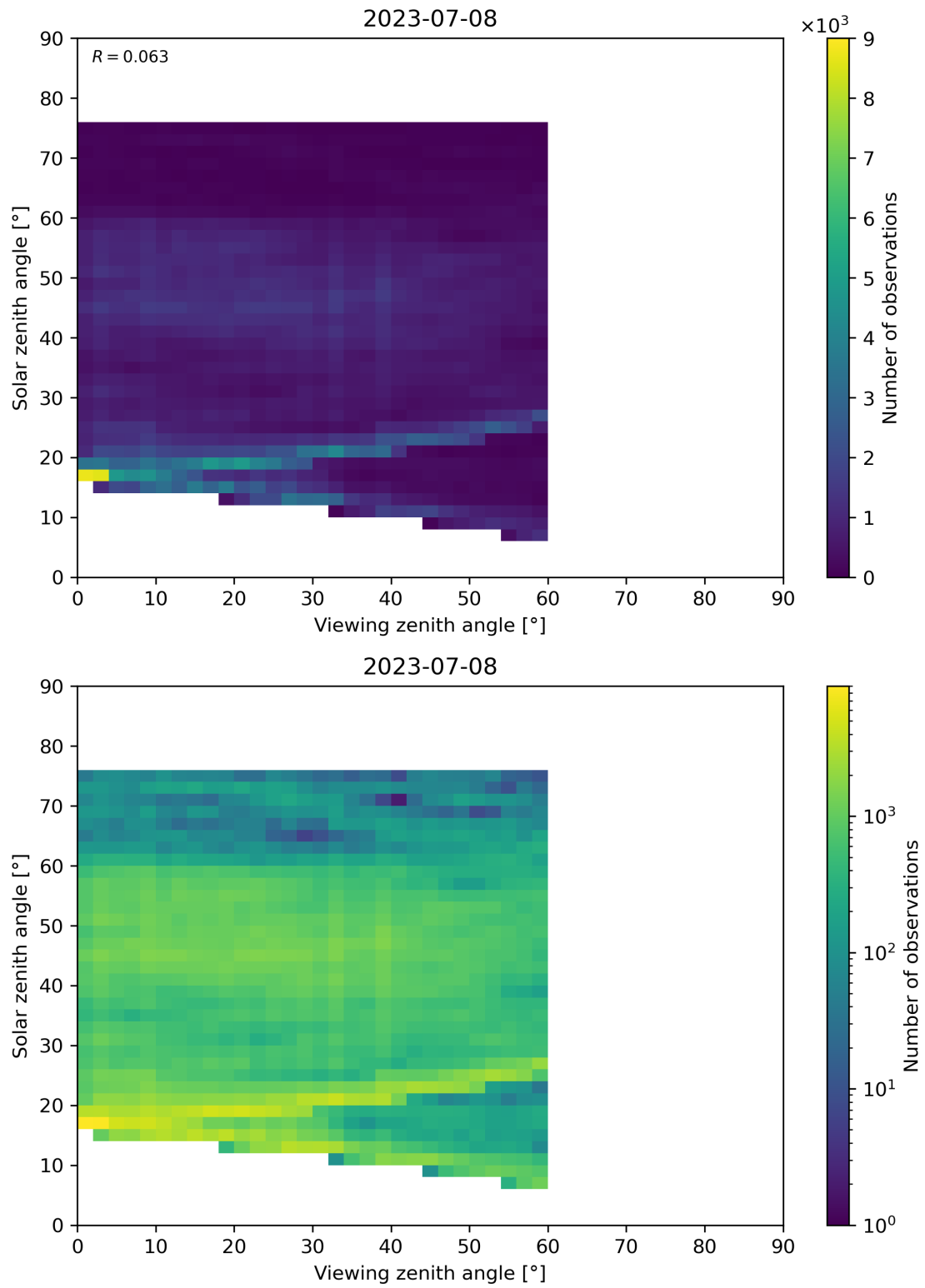
Figure 115: Scatter density plot of “Viewing zenith angle” against “Solar zenith angle” for 2023-07-08 to 2023-07-09.
