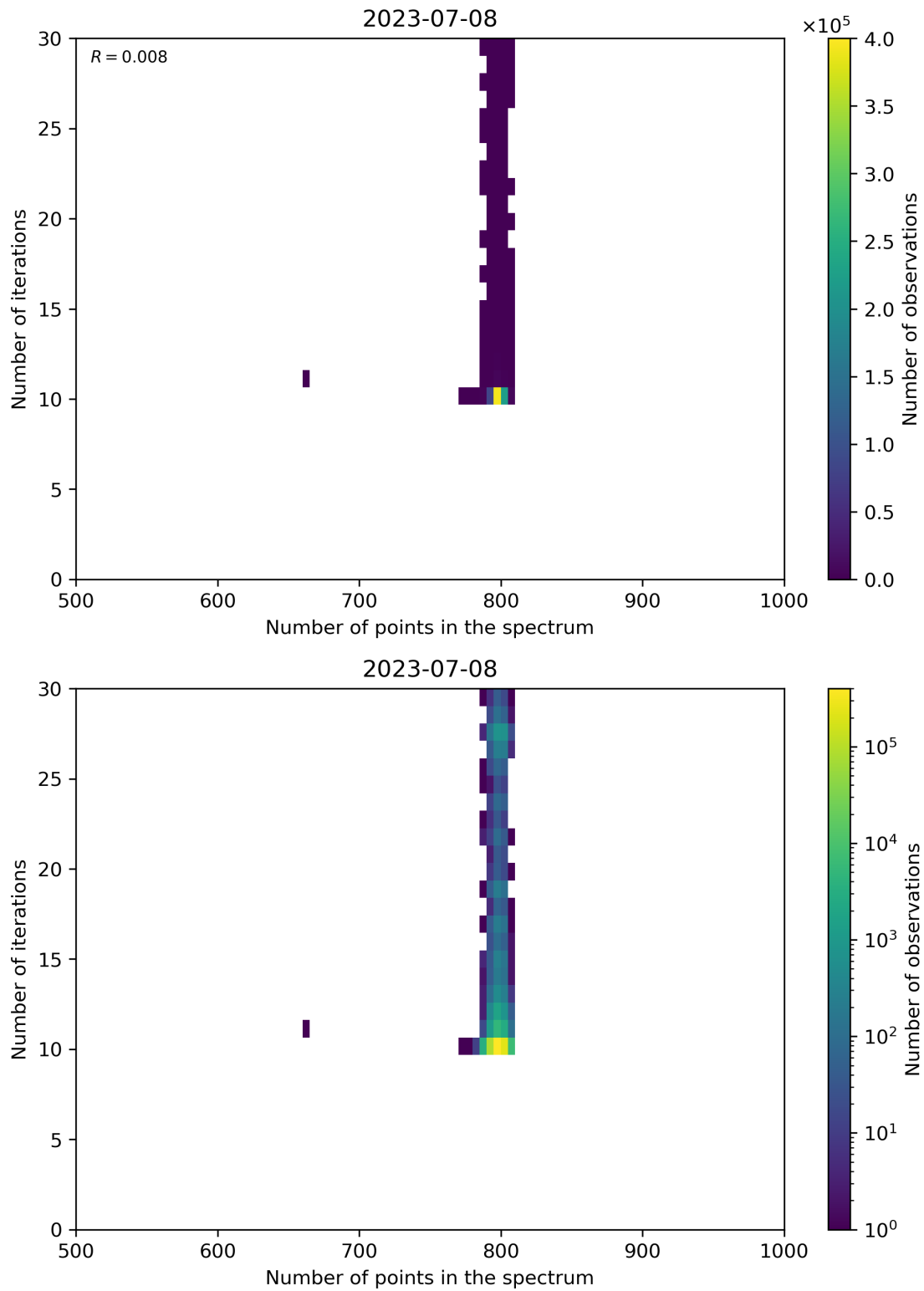
Figure 92: Scatter density plot of “Number of points in the spectrum” against “Number of iterations” for 2023-07-08 to 2023-07-09.
