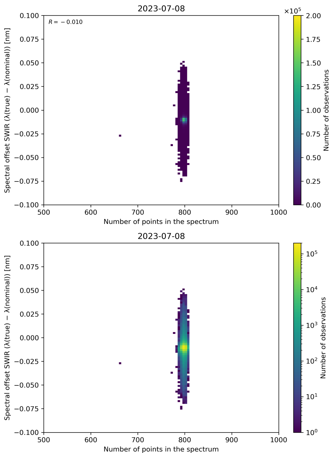
Figure 93: Scatter density plot of “Number of points in the spectrum” against “Spectral offset SWIR ( \lambda(\text{true}) - \lambda(\text{nominal}) )” for 2023-07-08 to 2023-07-09.
