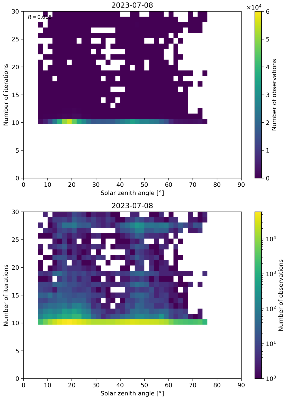
Figure 102: Scatter density plot of “Solar zenith angle” against “Number of iterations” for 2023-07-08 to 2023-07-09.
