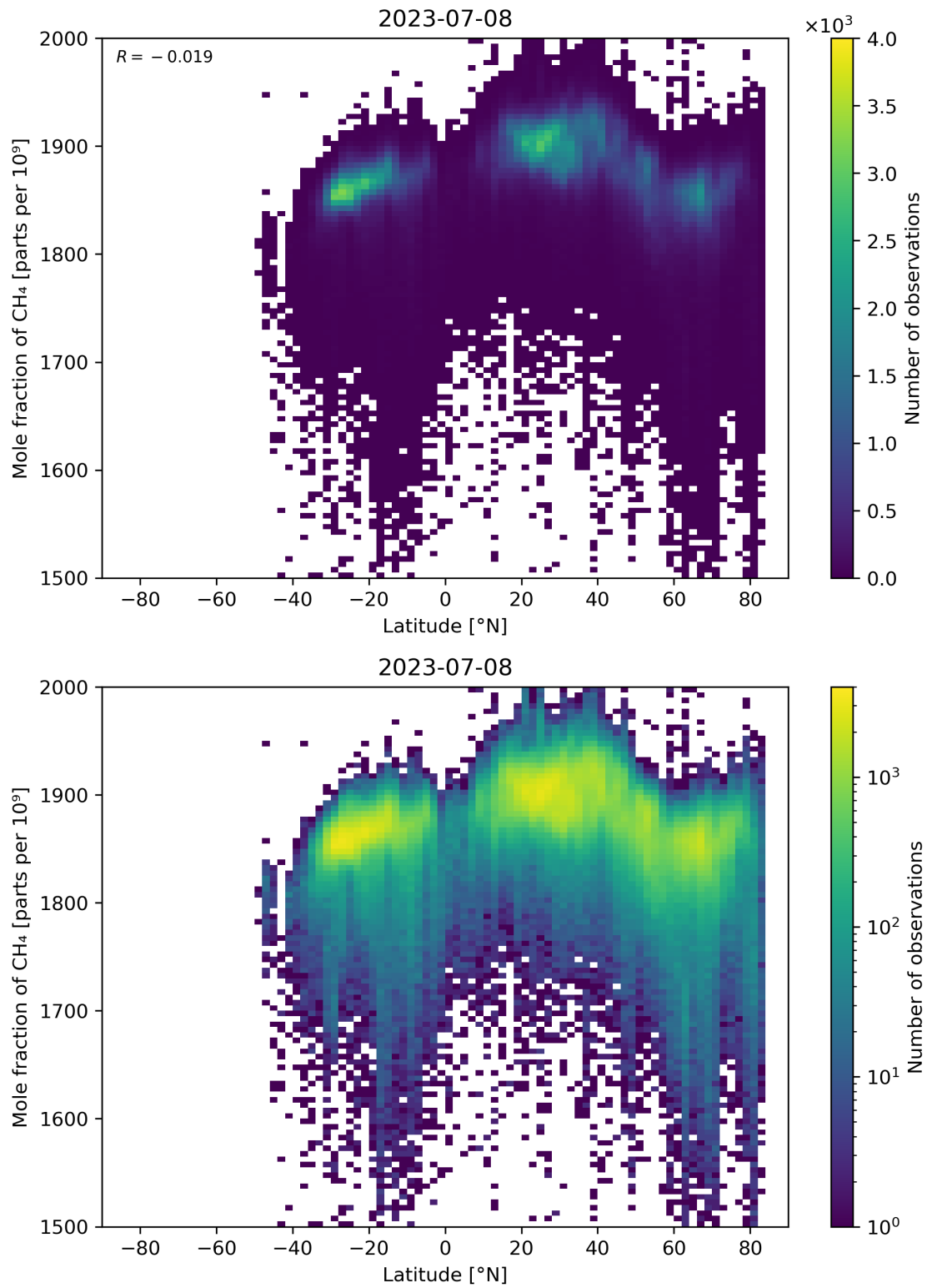
Figure 57: Scatter density plot of “Latitude” against “Mole fraction of \text{CH}_4 ” for 2023-07-08 to 2023-07-09.
