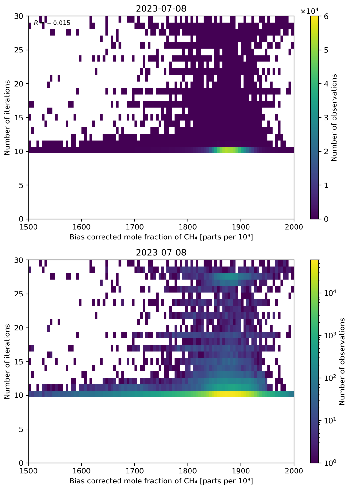
Figure 67: Scatter density plot of “Bias corrected mole fraction of CH 4 ” against “Number of iterations” for 2023-07-08 to 2023-07-09.
