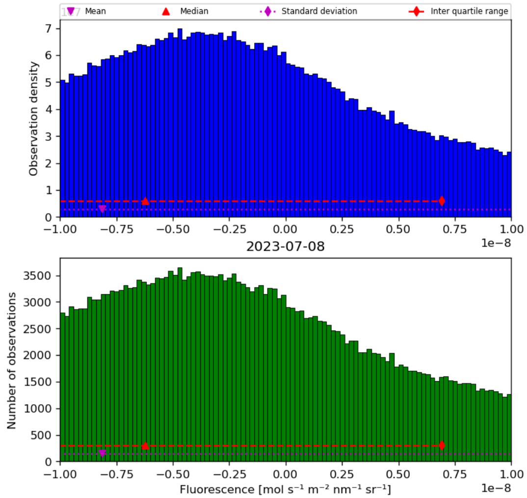
Figure 32: Histogram of “Fluorescence” for 2023-07-08 to 2023-07-09
