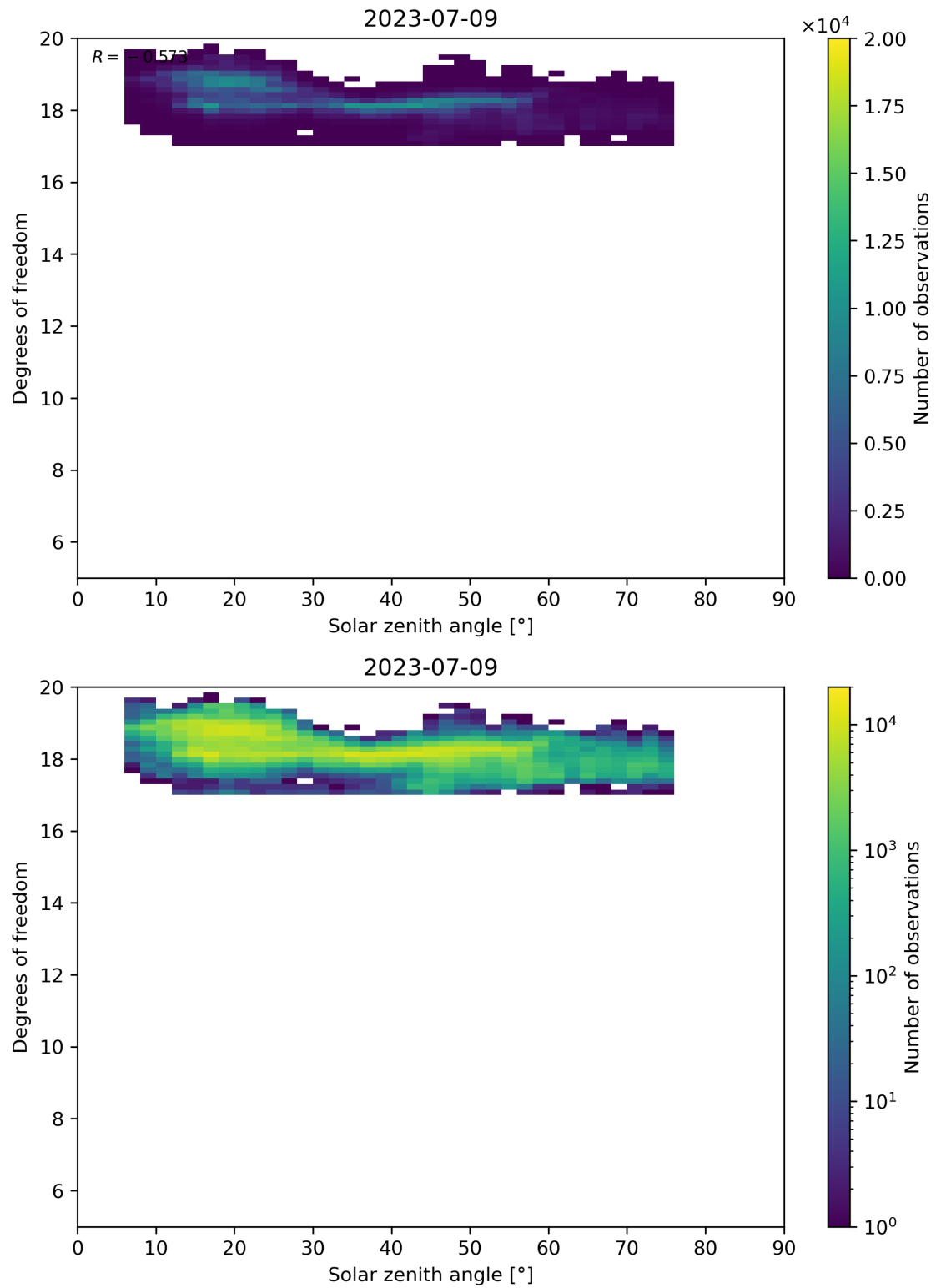
Figure 96: Scatter density plot of “Solar zenith angle” against “Degrees of freedom” for 2023-07-08 to 2023-07-10.
