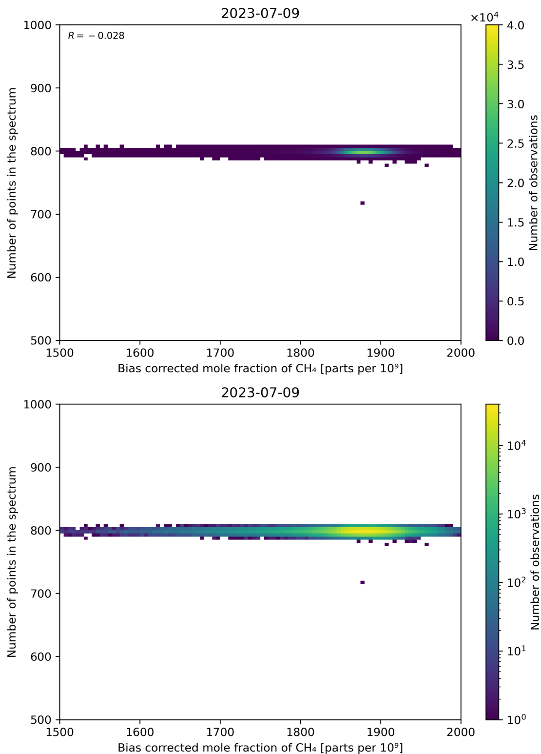
Figure 68: Scatter density plot of “Bias corrected mole fraction of CH 4 ” against “Number of points in the spectrum” for 2023-07-08 to 2023-07-10.
