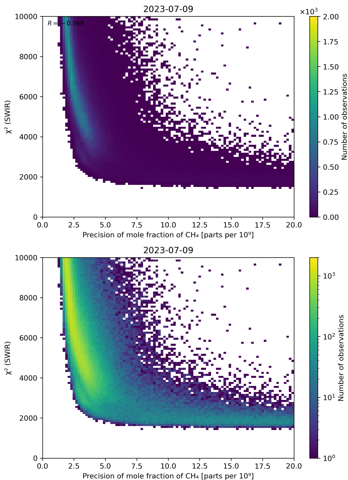
Figure 79: Scatter density plot of “Precision of mole fraction of CH 4 ” against “ \chi^2 (SWIR)” for 2023-07-08 to 2023-07-10.
