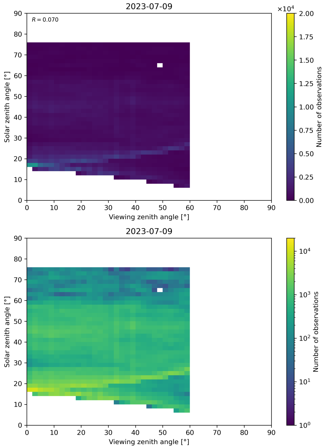
Figure 115: Scatter density plot of “Viewing zenith angle” against “Solar zenith angle” for 2023-07-08 to 2023-07-10.
