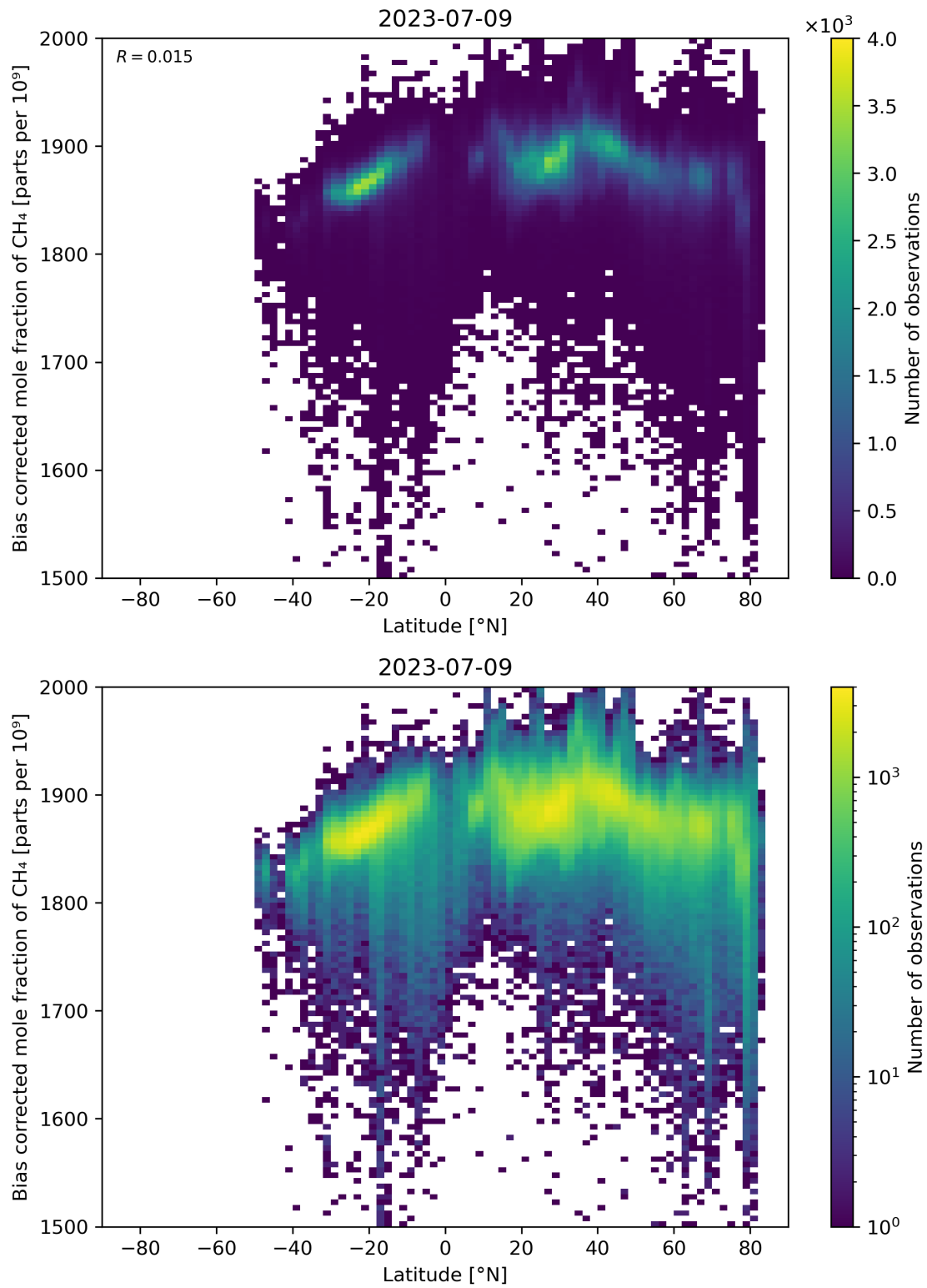
Figure 58: Scatter density plot of “Latitude” against “Bias corrected mole fraction of \text{CH}_4 ” for 2023-07-08 to 2023-07-10.
