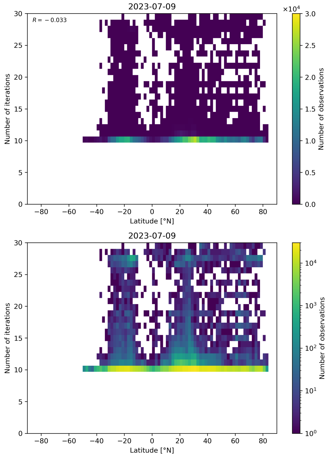
Figure 60: Scatter density plot of “Latitude” against “Number of iterations” for 2023-07-08 to 2023-07-10.
