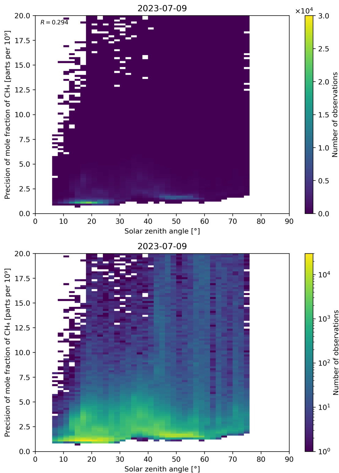
Figure 101: Scatter density plot of “Solar zenith angle” against “Precision of mole fraction of CH 4 ” for 2023-07-08 to 2023-07-10.
