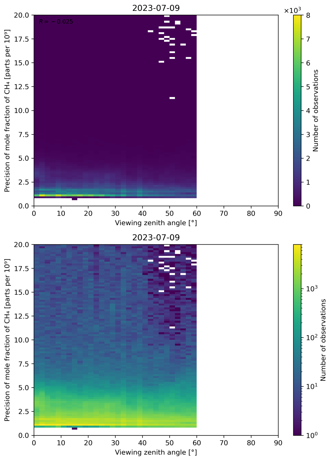
Figure 112: Scatter density plot of “Viewing zenith angle” against “Precision of mole fraction of CH 4 ” for 2023-07-08 to 2023-07-10.
