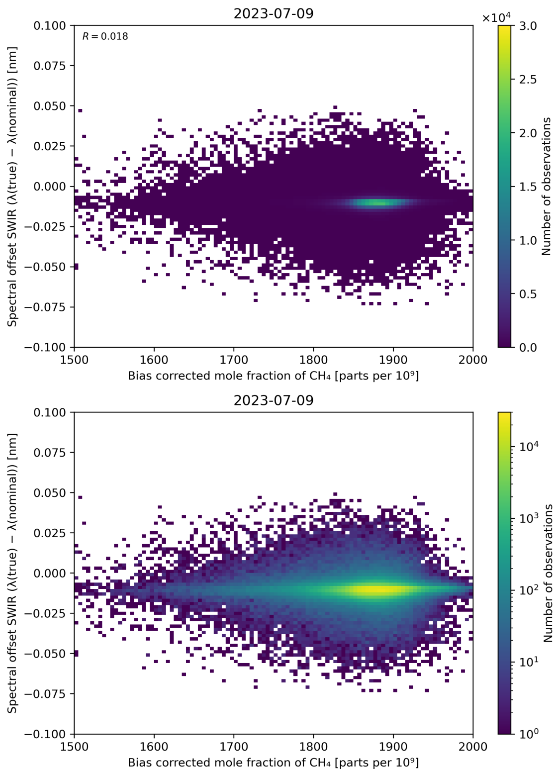
Figure 69: Scatter density plot of “Bias corrected mole fraction of \text{CH}_4 ” against “Spectral offset SWIR ( \lambda(\text{true}) - \lambda(\text{nominal}) )” for 2023-07-08 to 2023-07-10.
