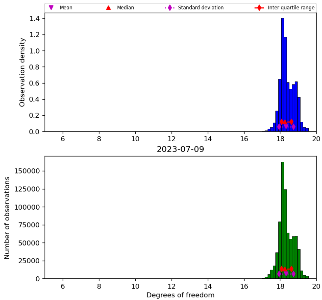
Figure 30: Histogram of “Degrees of freedom” for 2023-07-08 to 2023-07-10
