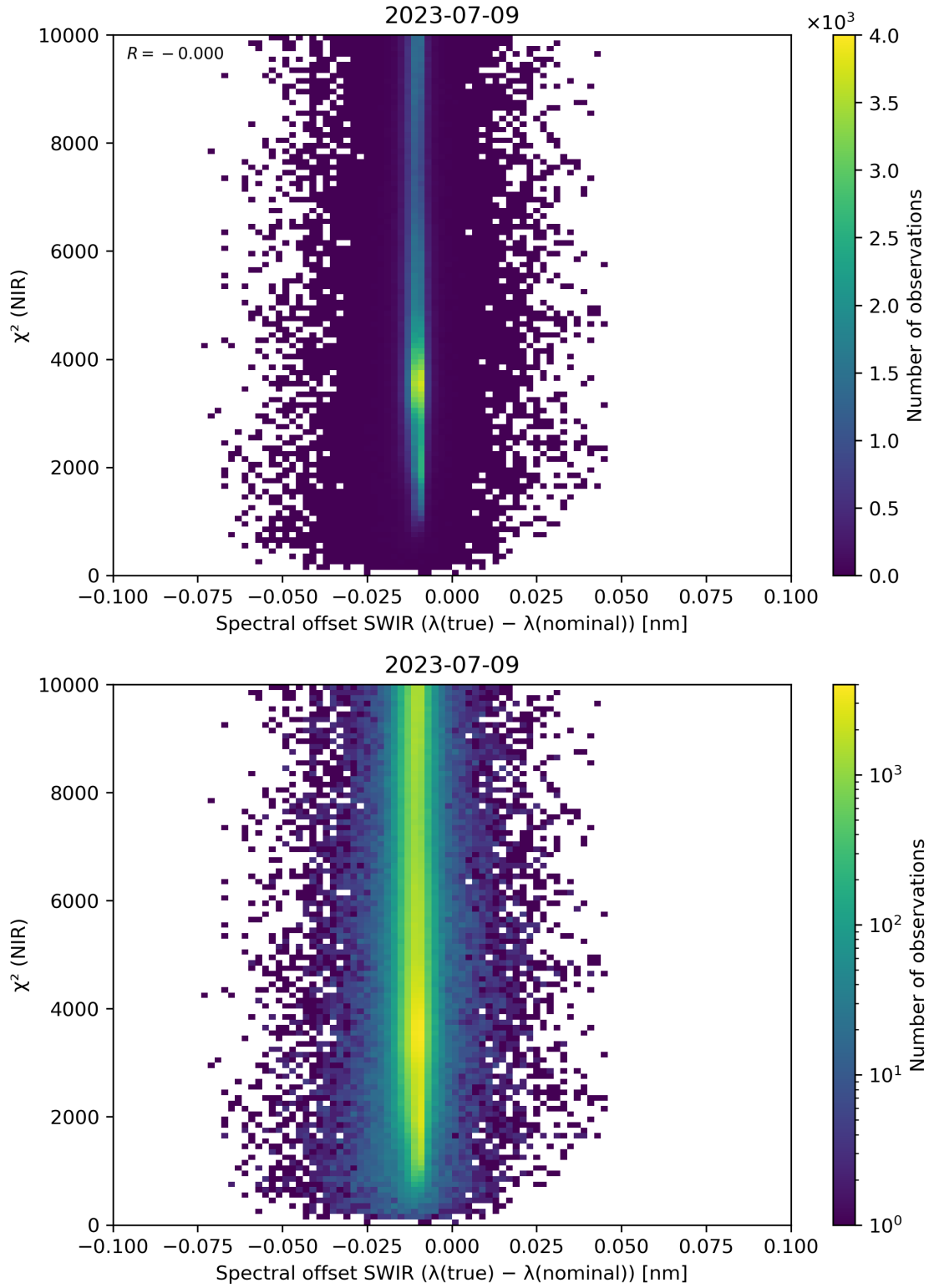
Figure 117: Scatter density plot of “Spectral offset SWIR ( \lambda(\text{true}) - \lambda(\text{nominal}) )” against “ \chi^2 (NIR)” for 2023-07-08 to 2023-07-10.
