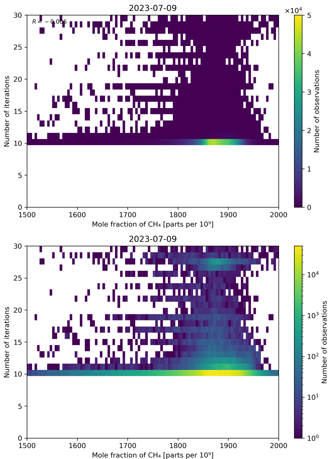
Figure 76: Scatter density plot of “Mole fraction of CH 4 ” against “Number of iterations” for 2023-07-08 to 2023-07-10.
