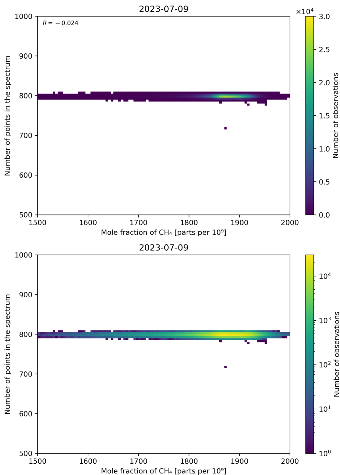
Figure 77: Scatter density plot of “Mole fraction of CH 4 ” against “Number of points in the spectrum” for 2023-07-08 to 2023-07-10.
