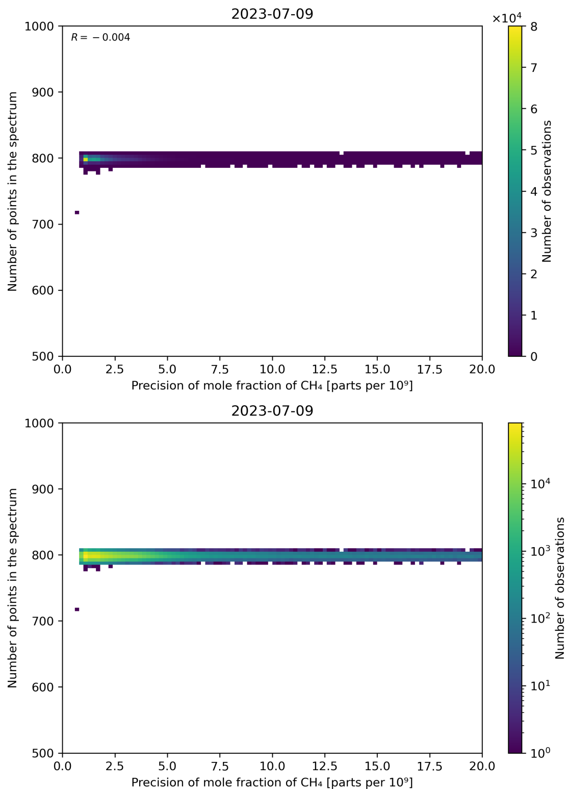
Figure 84: Scatter density plot of “Precision of mole fraction of CH 4 ” against “Number of points in the spectrum” for 2023-07-08 to 2023-07-10.
