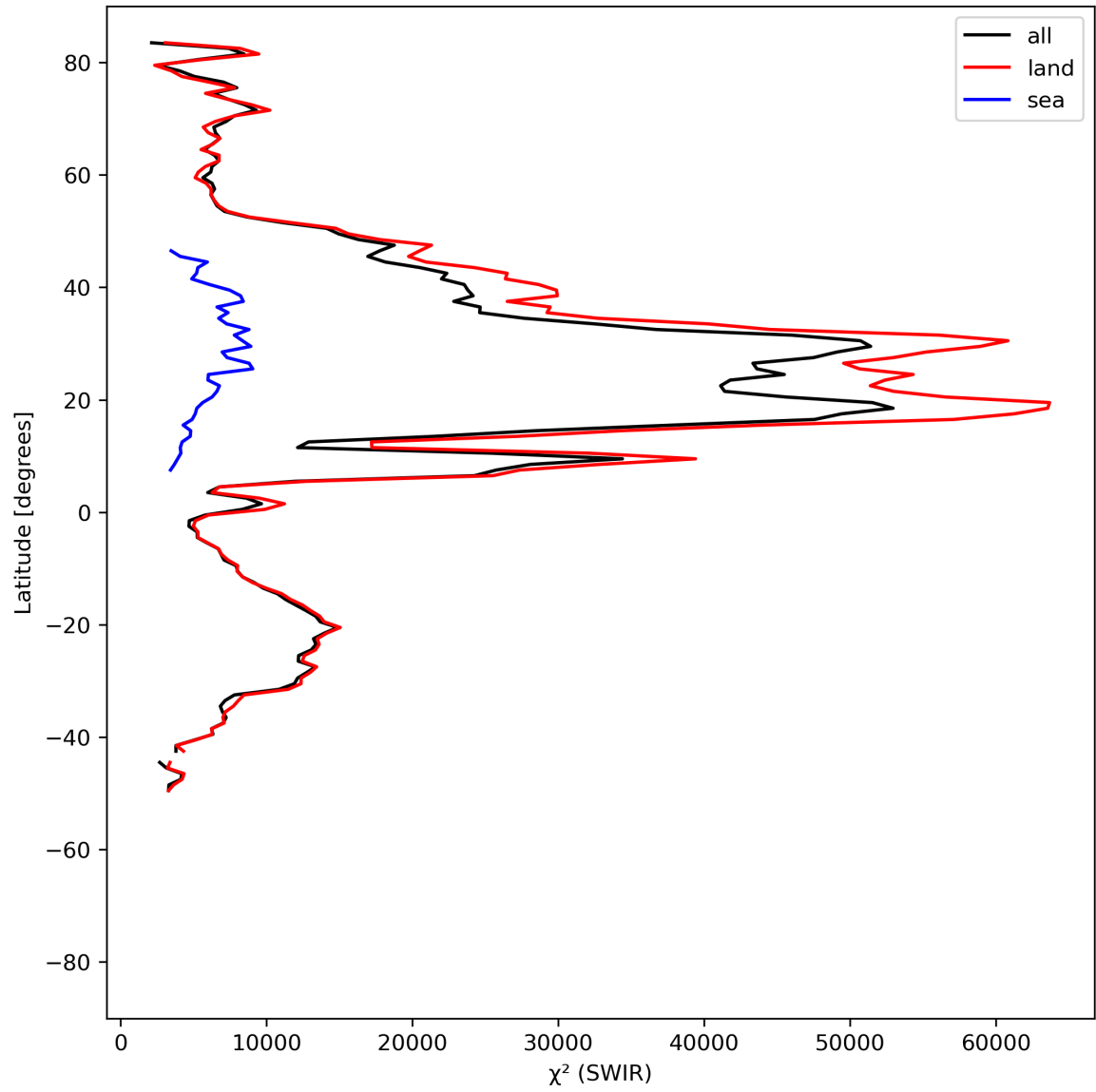
Figure 17: Zonal average of “ \chi^2 (SWIR)” for 2023-07-08 to 2023-07-10.
