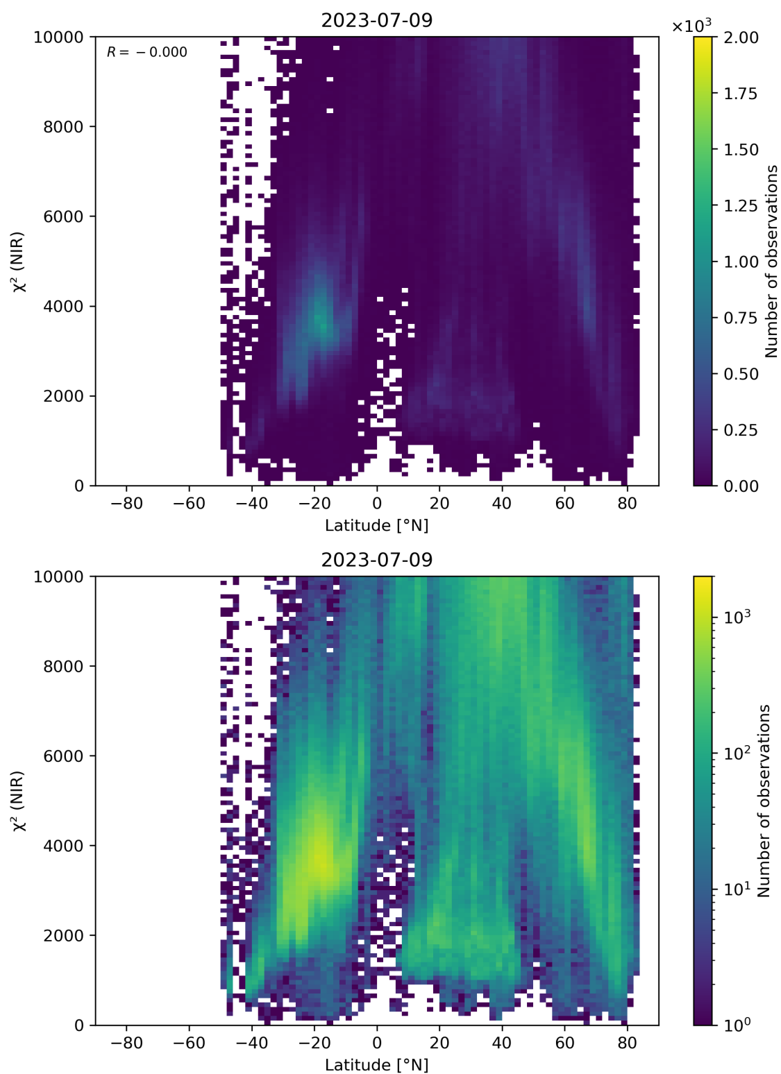
Figure 53: Scatter density plot of “Latitude” against “ \chi^2 (NIR)” for 2023-07-08 to 2023-07-10.
