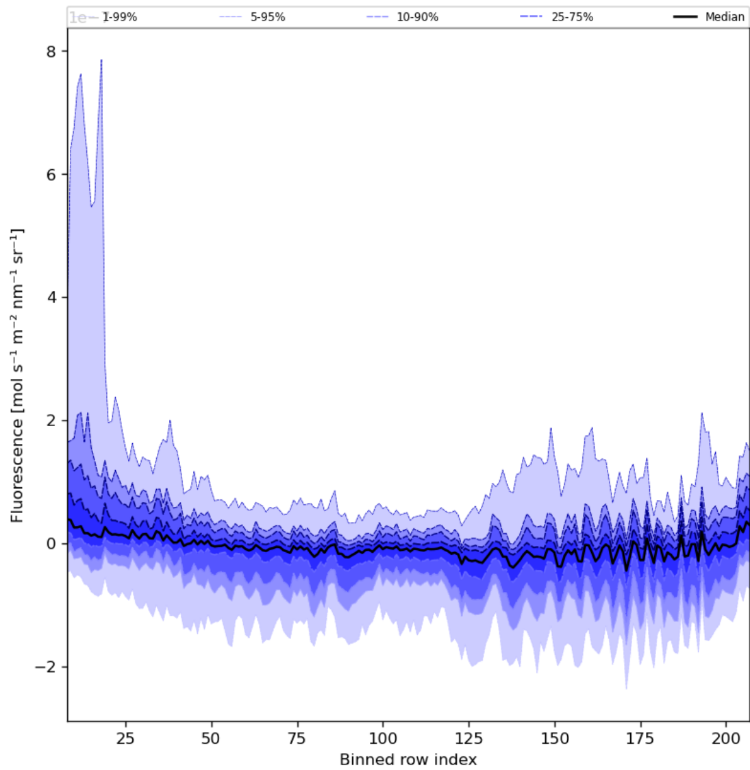
Figure 43: Along track statistics of “Fluorescence” for 2023-07-08 to 2023-07-10
