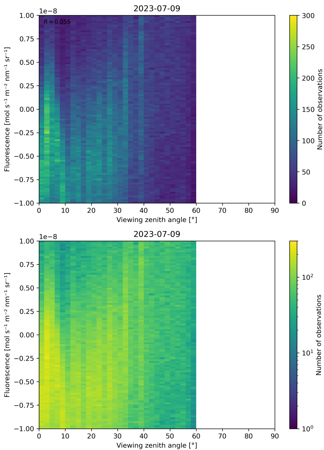
Figure 108: Scatter density plot of “Viewing zenith angle” against “Fluorescence” for 2023-07-08 to 2023-07-10.
