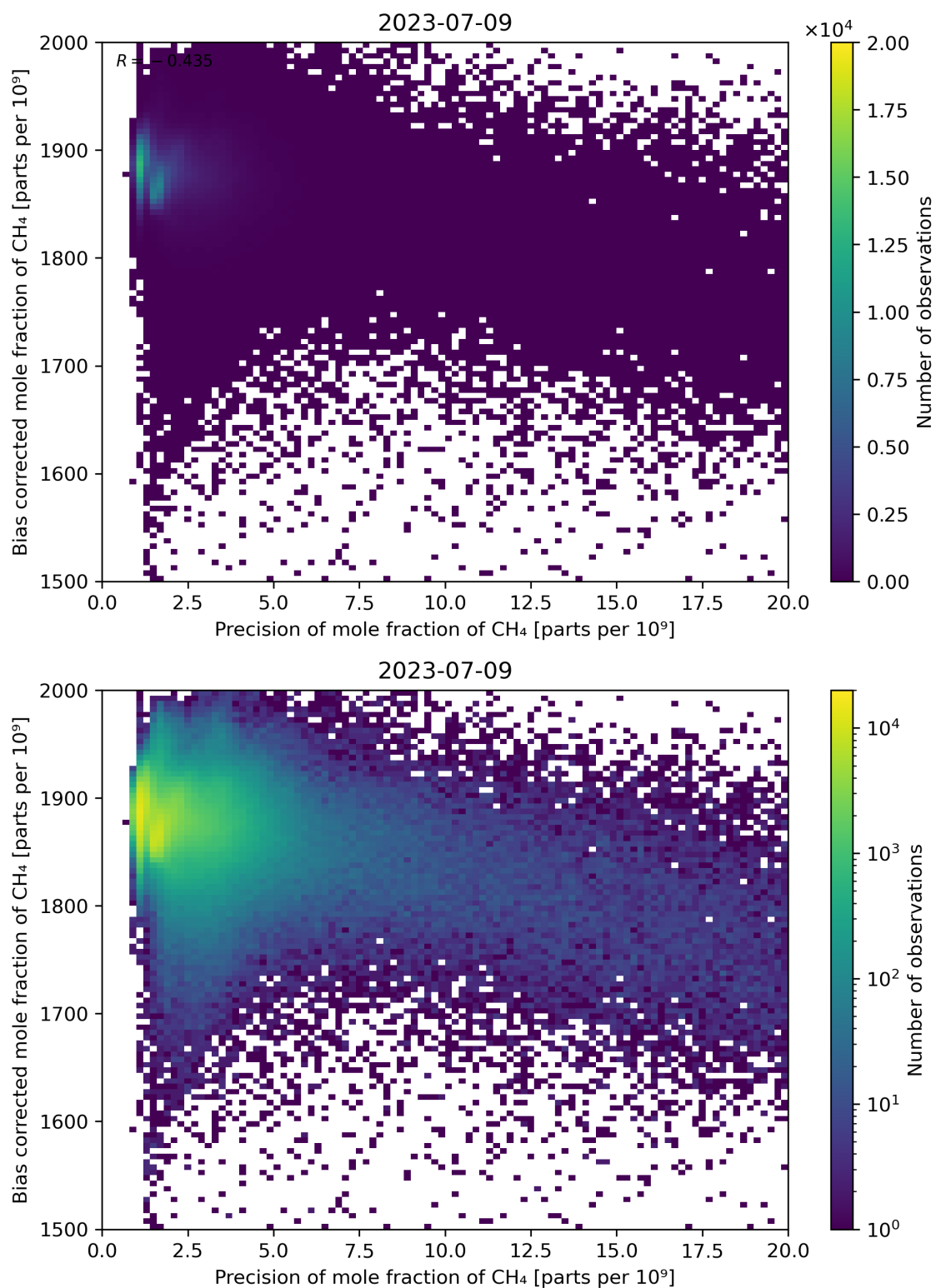
Figure 82: Scatter density plot of “Precision of mole fraction of CH 4 ” against “Bias corrected mole fraction of CH 4 ” for 2023-07-08 to 2023-07-10.
