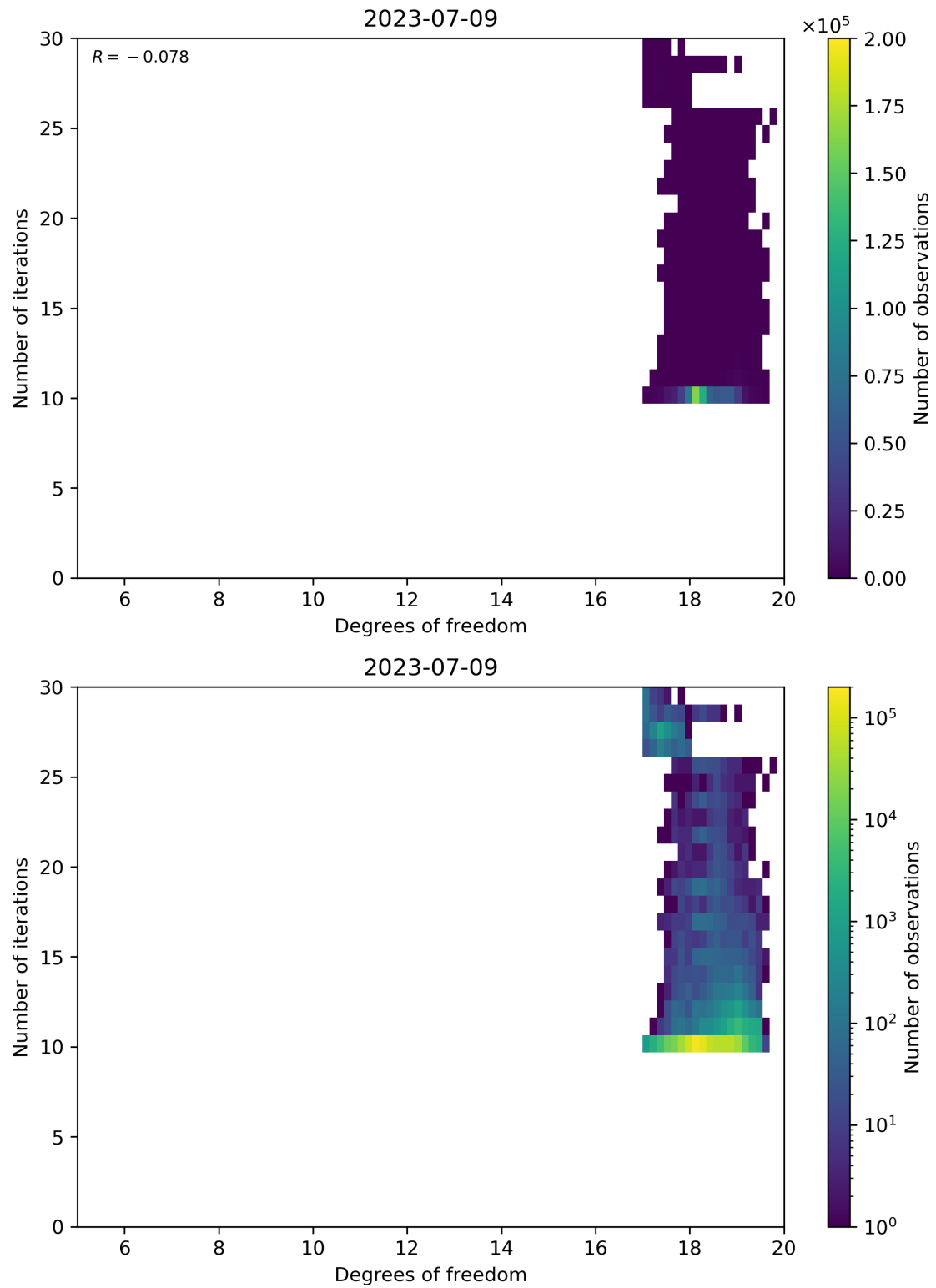
Figure 52: Scatter density plot of “Degrees of freedom” against “Number of iterations” for 2023-07-08 to 2023-07-10.
