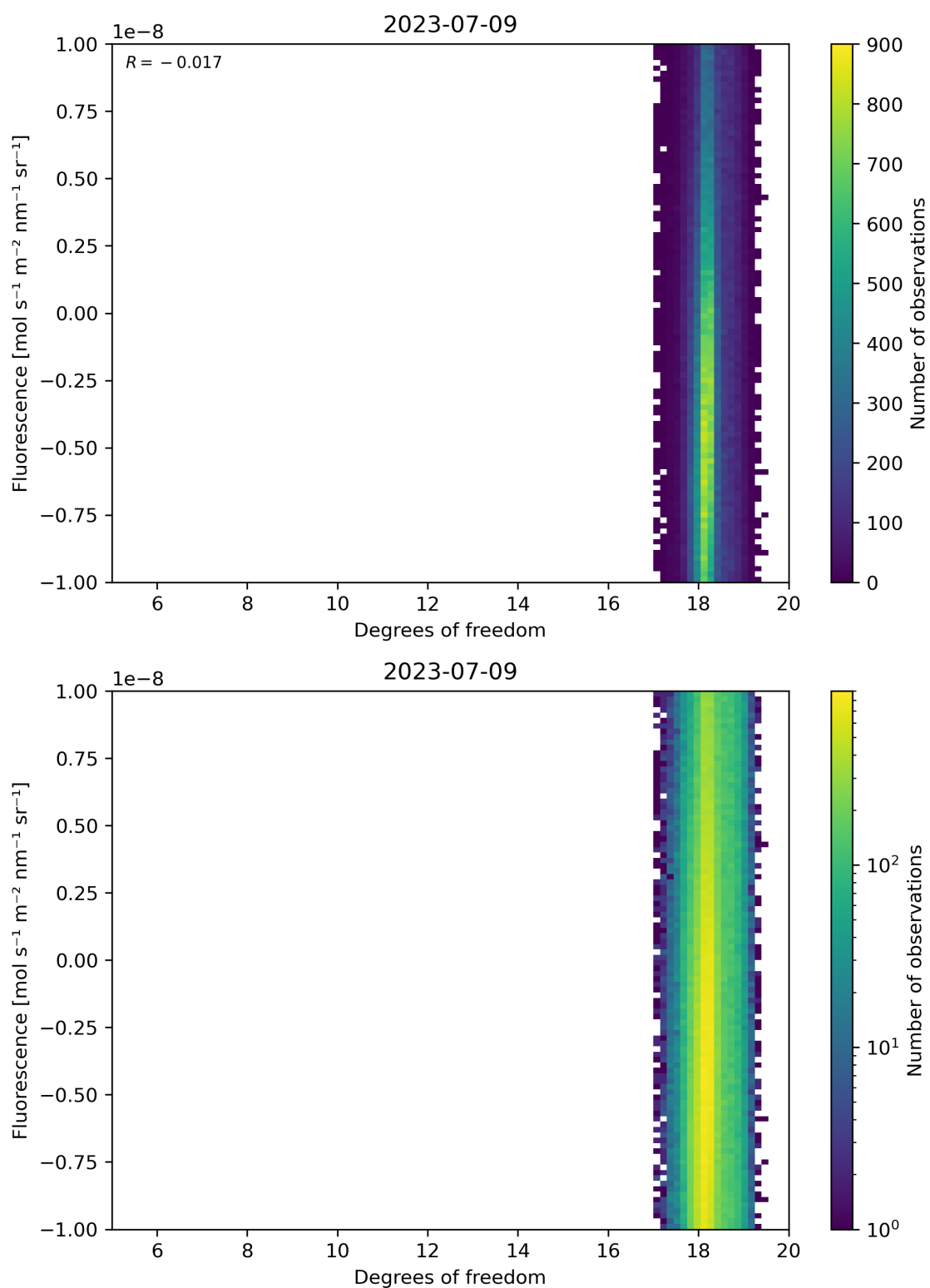
Figure 51: Scatter density plot of “Degrees of freedom” against “Fluorescence” for 2023-07-08 to 2023-07-10.
