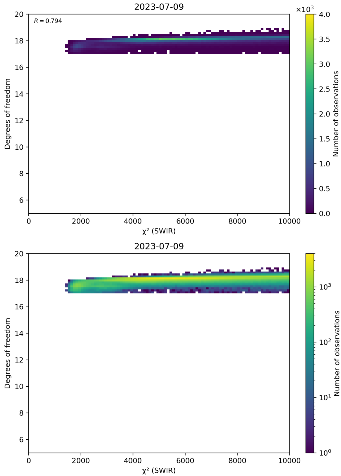
Figure 48: Scatter density plot of “ \chi^2 (SWIR)” against “Degrees of freedom” for 2023-07-08 to 2023-07-10.
