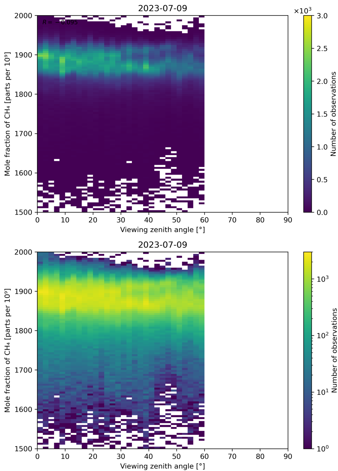
Figure 110: Scatter density plot of “Viewing zenith angle” against “Mole fraction of CH 4 ” for 2023-07-08 to 2023-07-10.
