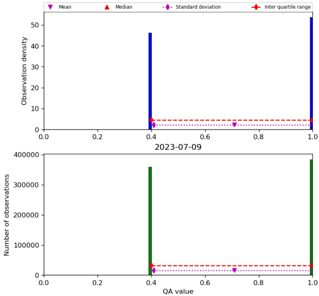
Figure 22: Histogram of “QA value” for 2023-07-08 to 2023-07-10
