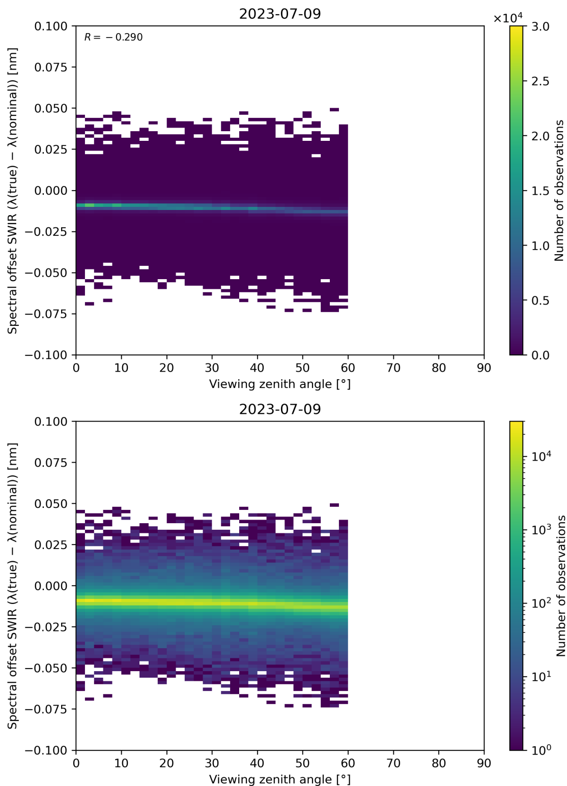
Figure 116: Scatter density plot of “Viewing zenith angle” against “Spectral offset SWIR ( \lambda(\text{true}) - \lambda(\text{nominal}) )” for 2023-07-08 to 2023-07-10.
