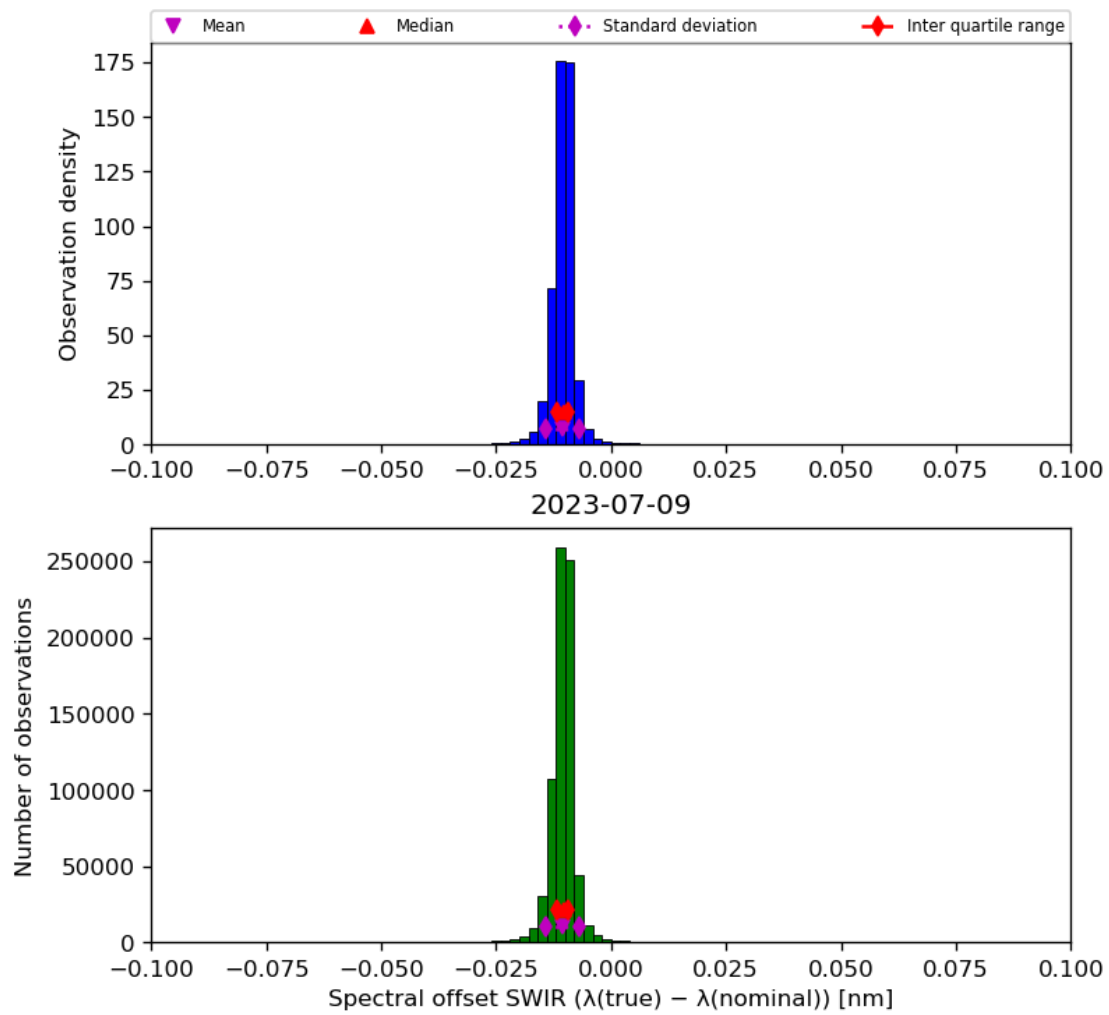
Figure 27: Histogram of “Spectral offset SWIR ( \lambda(\text{true}) - \lambda(\text{nominal}) )” for 2023-07-08 to 2023-07-10
