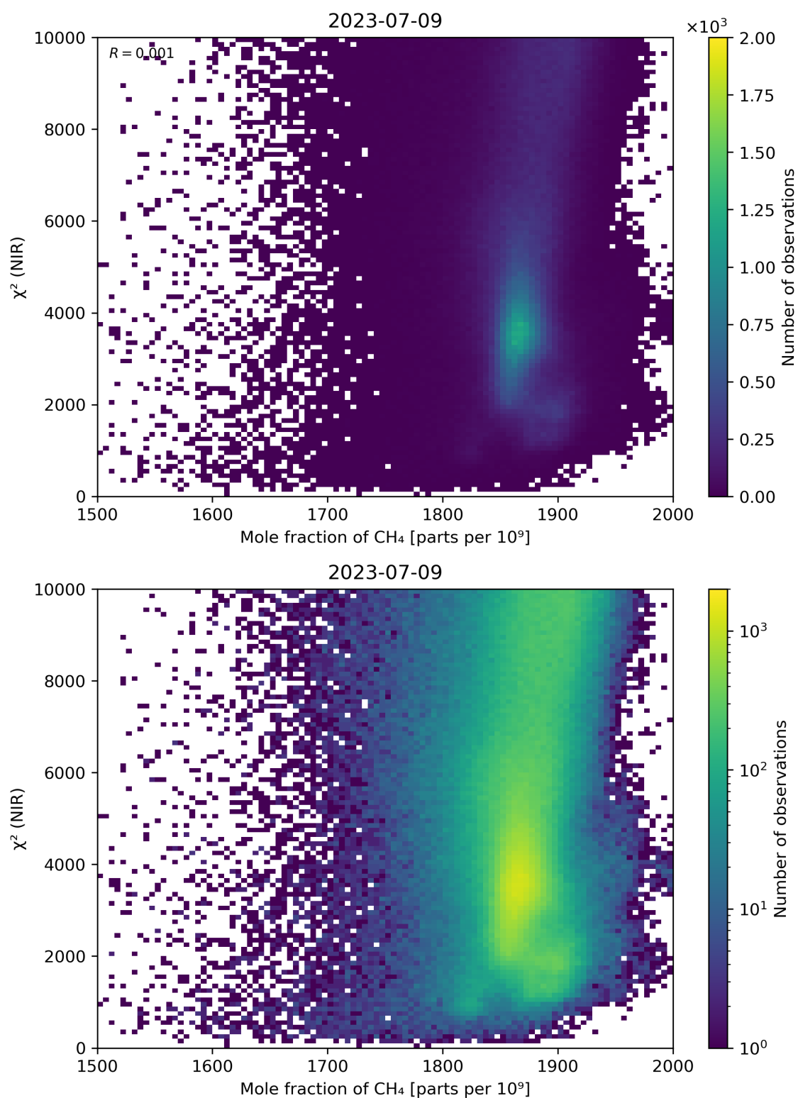
Figure 70: Scatter density plot of “Mole fraction of CH 4 ” against “ \chi^2 (NIR)” for 2023-07-08 to 2023-07-10.
