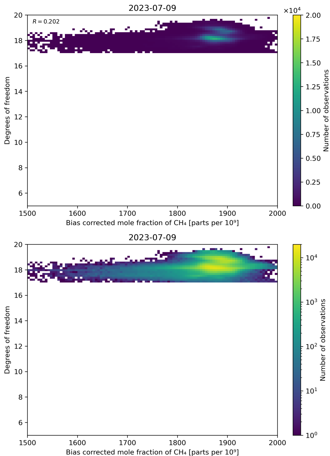
Figure 65: Scatter density plot of “Bias corrected mole fraction of CH 4 ” against “Degrees of freedom” for 2023-07-08 to 2023-07-10.
