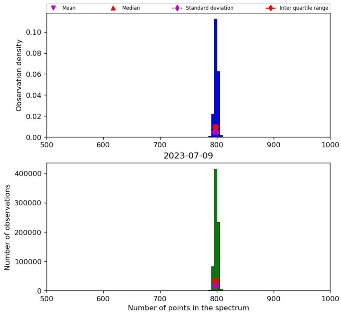
Figure 26: Histogram of “Number of points in the spectrum” for 2023-07-08 to 2023-07-10
