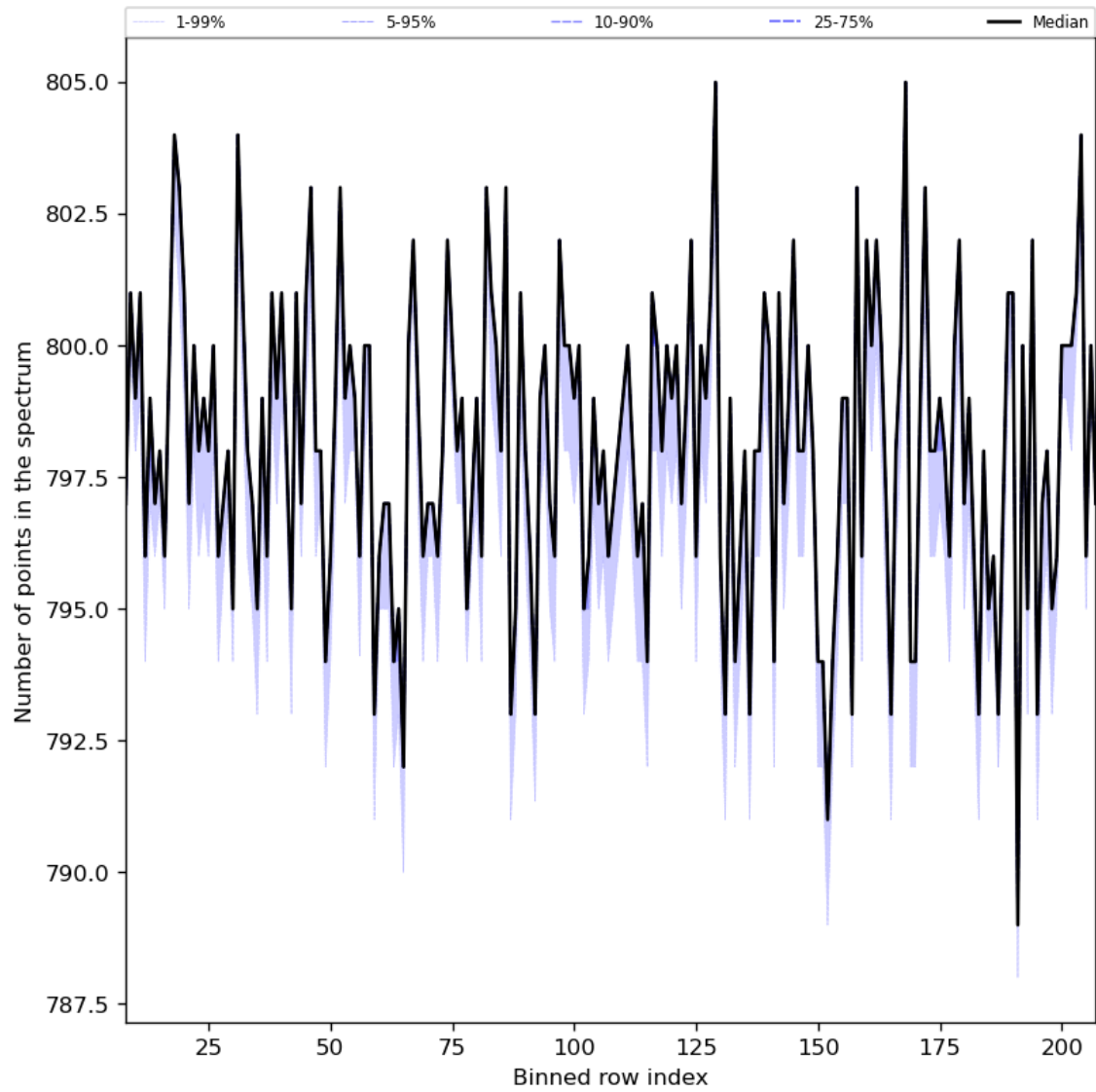
Figure 37: Along track statistics of “Number of points in the spectrum” for 2023-07-08 to 2023-07-10
