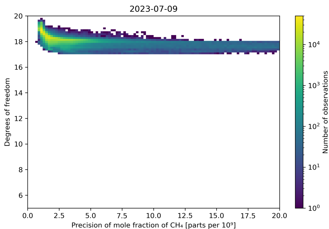
Figure 80: Scatter density plot of “Precision of mole fraction of CH 4 ” against “Degrees of freedom” for 2023-07-08 to 2023-07-10.
