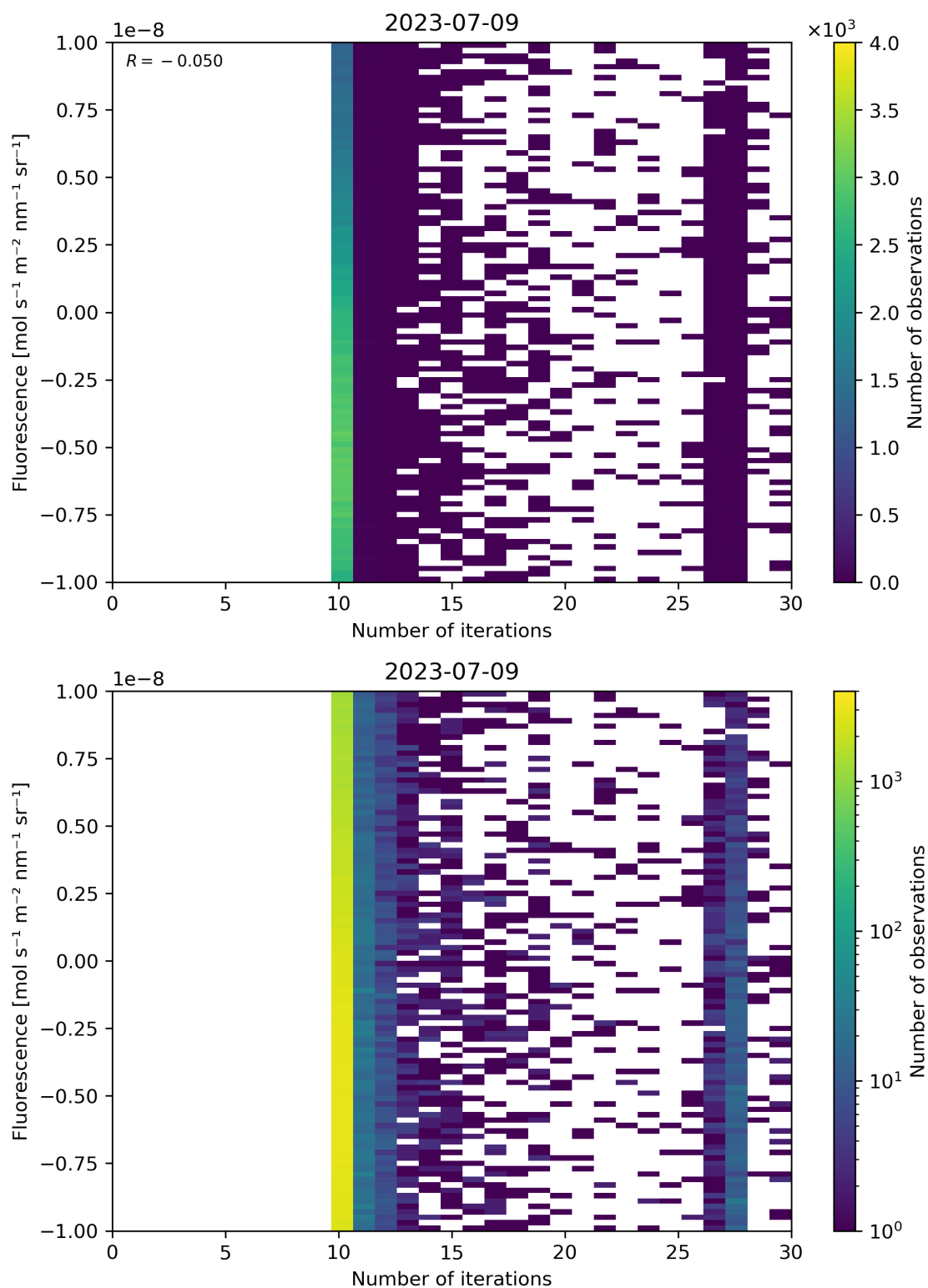
Figure 87: Scatter density plot of “Number of iterations” against “Fluorescence” for 2023-07-08 to 2023-07-10.
