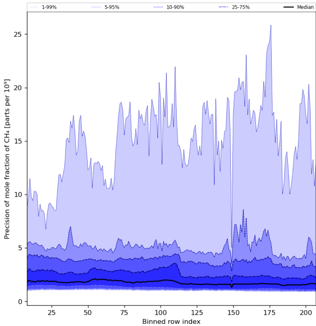
Figure 35: Along track statistics of "Precision of mole fraction of CH 4 " for 2023-07-08 to 2023-07-10
