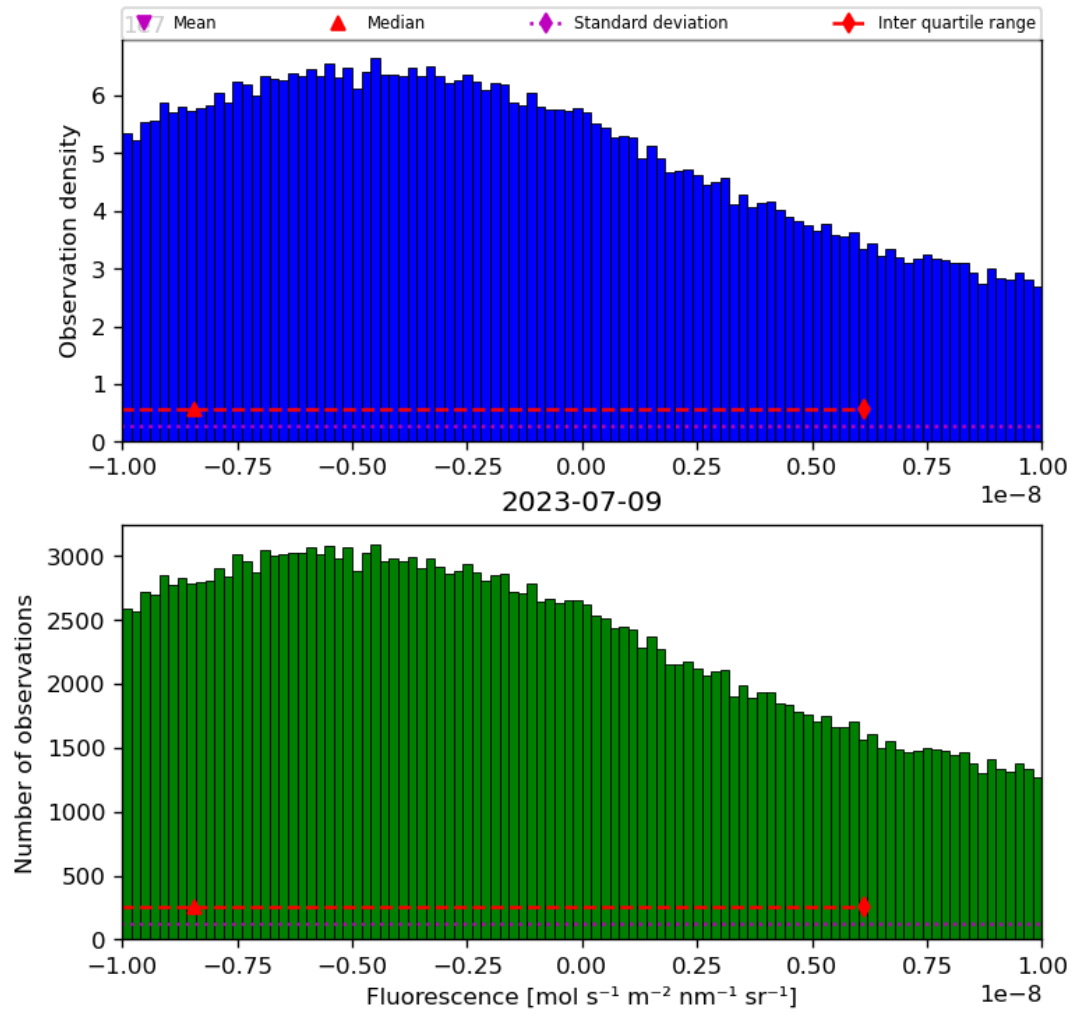
Figure 32: Histogram of “Fluorescence” for 2023-07-08 to 2023-07-10
