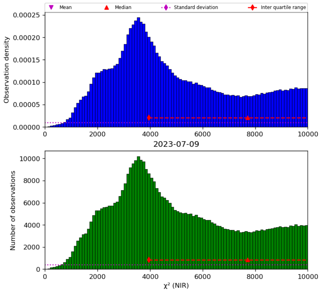
Figure 29: Histogram of “ \chi^2 (NIR)” for 2023-07-08 to 2023-07-10
