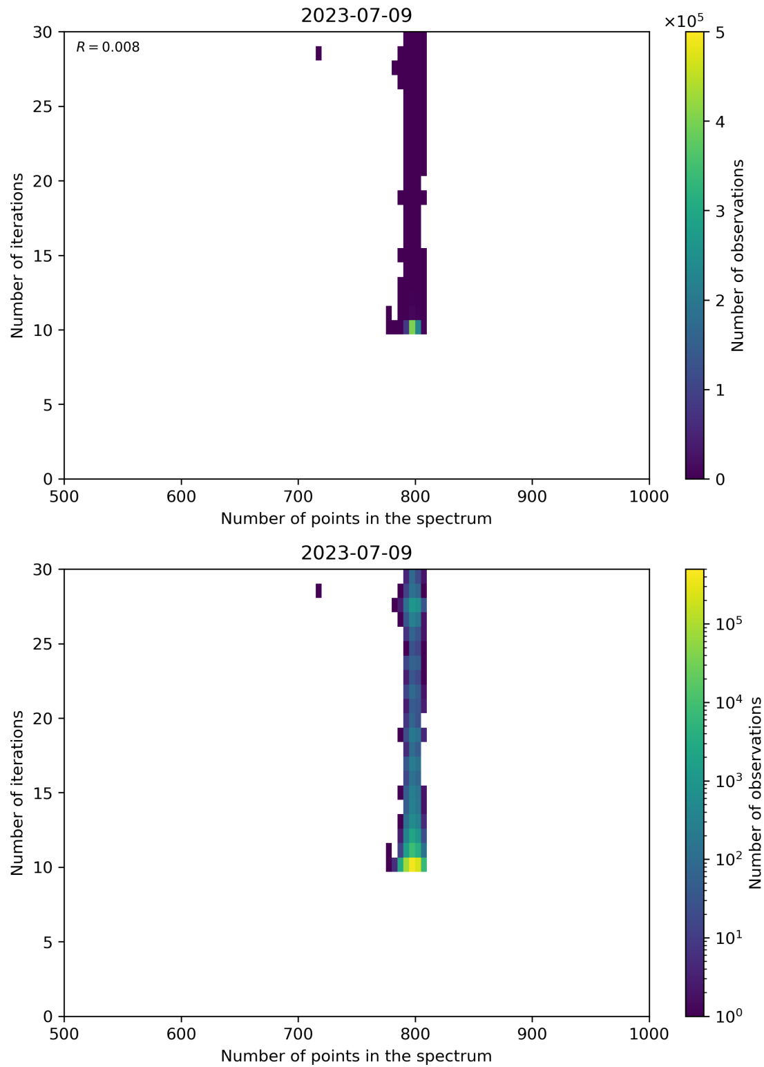
Figure 92: Scatter density plot of “Number of points in the spectrum” against “Number of iterations” for 2023-07-08 to 2023-07-10.
