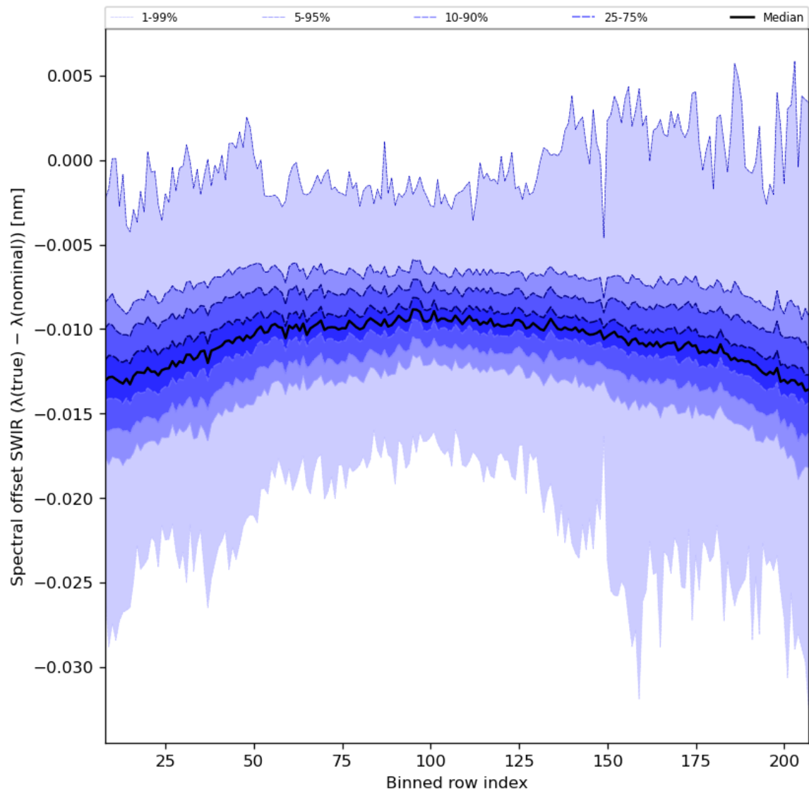
Figure 38: Along track statistics of “Spectral offset SWIR ( \lambda(\text{true}) - \lambda(\text{nominal}) )” for 2023-07-08 to 2023-07-10
