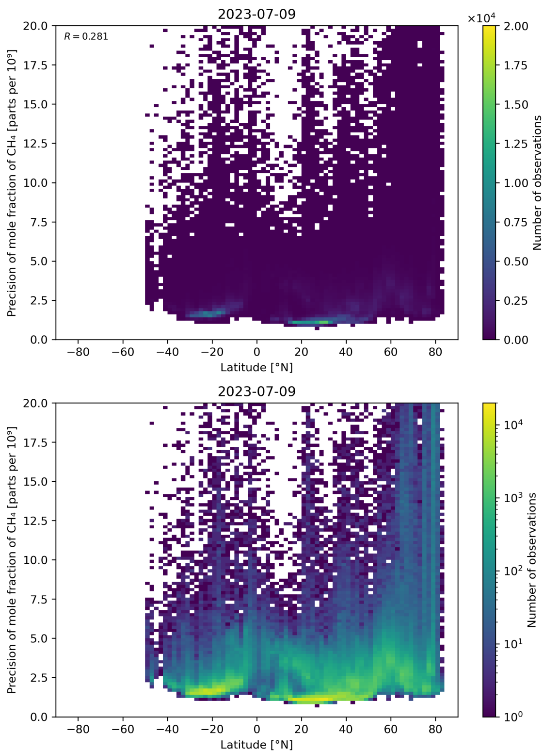
Figure 59: Scatter density plot of “Latitude” against “Precision of mole fraction of \text{CH}_4 ” for 2023-07-08 to 2023-07-10.
