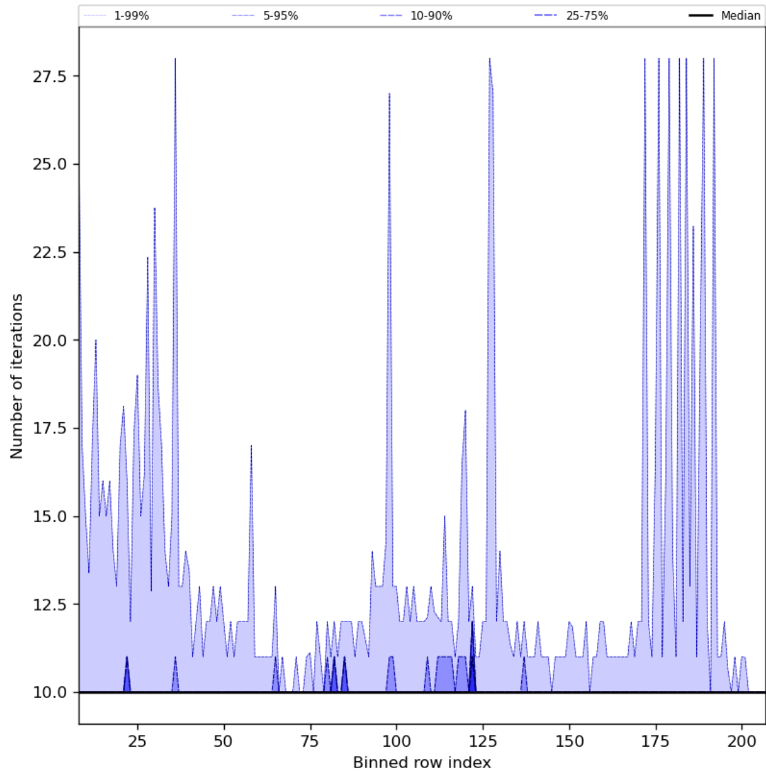
Figure 42: Along track statistics of “Number of iterations” for 2023-07-08 to 2023-07-10
