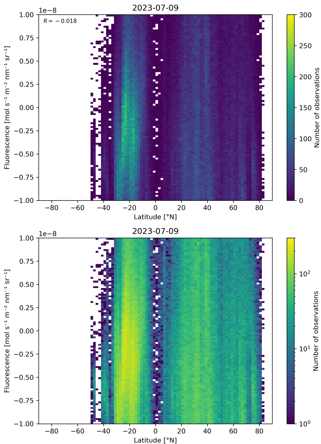
Figure 56: Scatter density plot of “Latitude” against “Fluorescence” for 2023-07-08 to 2023-07-10.
