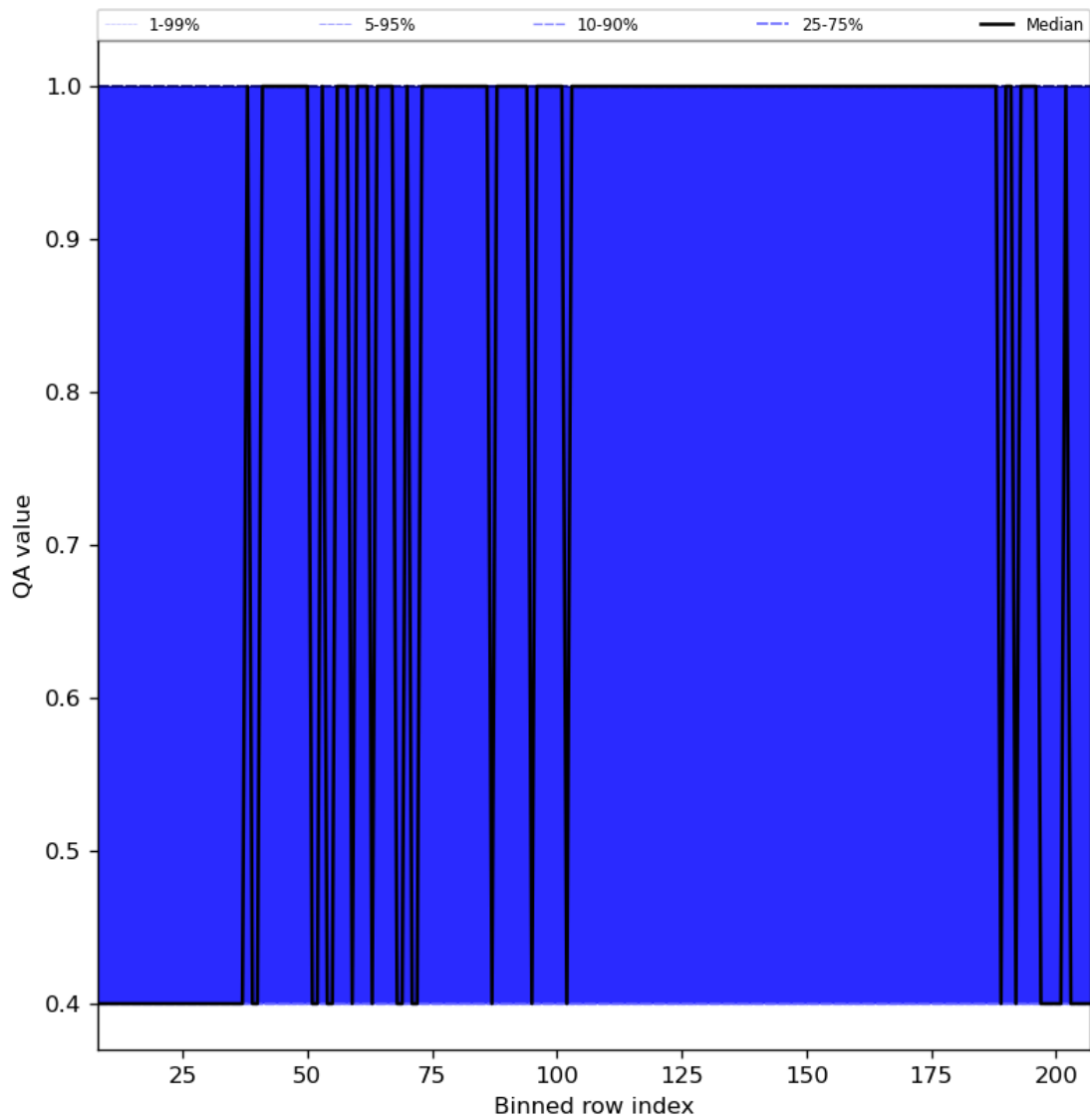
Figure 33: Along track statistics of “QA value” for 2023-07-08 to 2023-07-10
