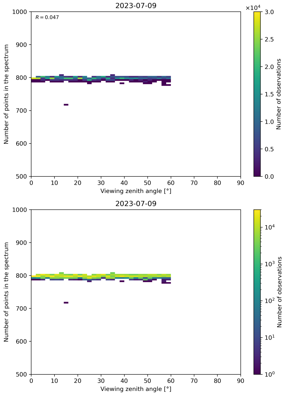
Figure 114: Scatter density plot of “Viewing zenith angle” against “Number of points in the spectrum” for 2023-07-08 to 2023-07-10.
