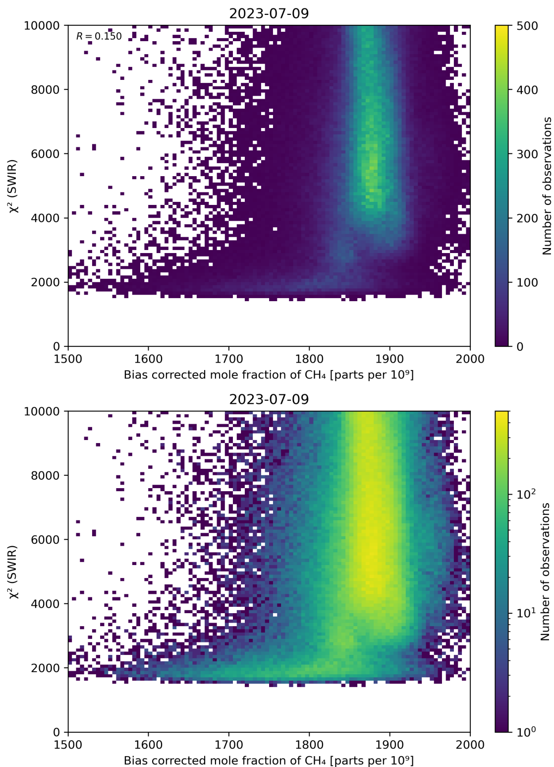
Figure 64: Scatter density plot of “Bias corrected mole fraction of CH 4 ” against “ \chi^2 (SWIR)” for 2023-07-08 to 2023-07-10.
