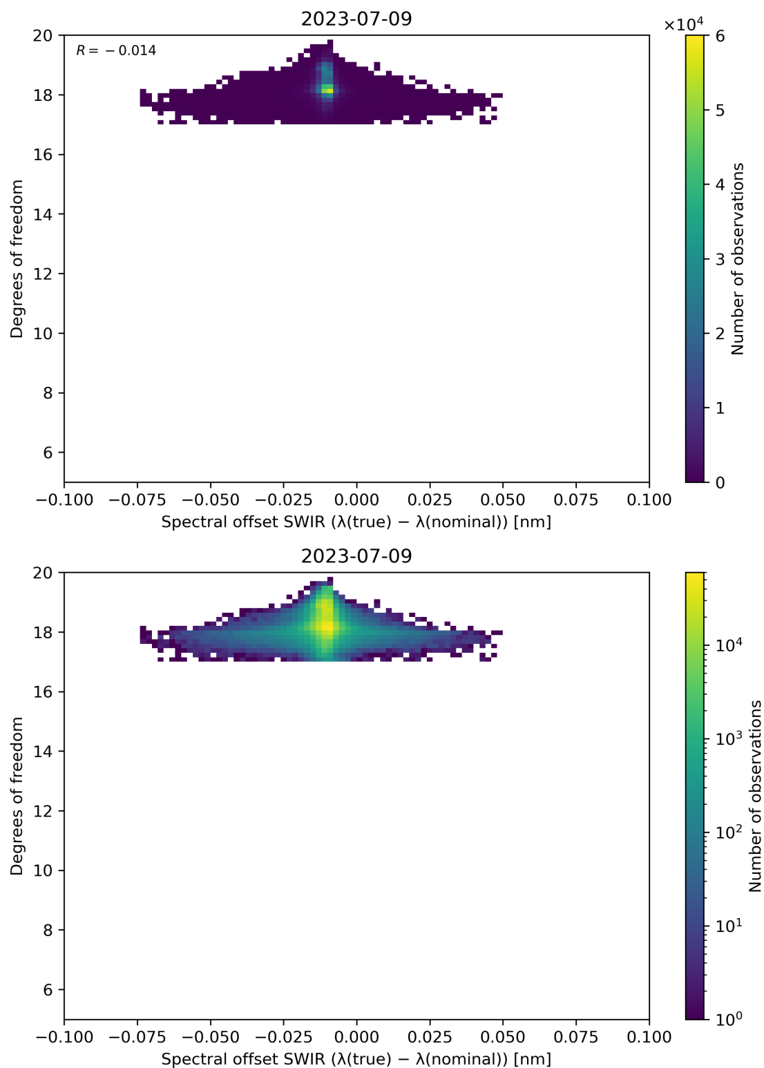
Figure 119: Scatter density plot of “Spectral offset SWIR ( \lambda(\text{true}) - \lambda(\text{nominal}) )” against “Degrees of freedom” for 2023-07-08 to 2023-07-10.
