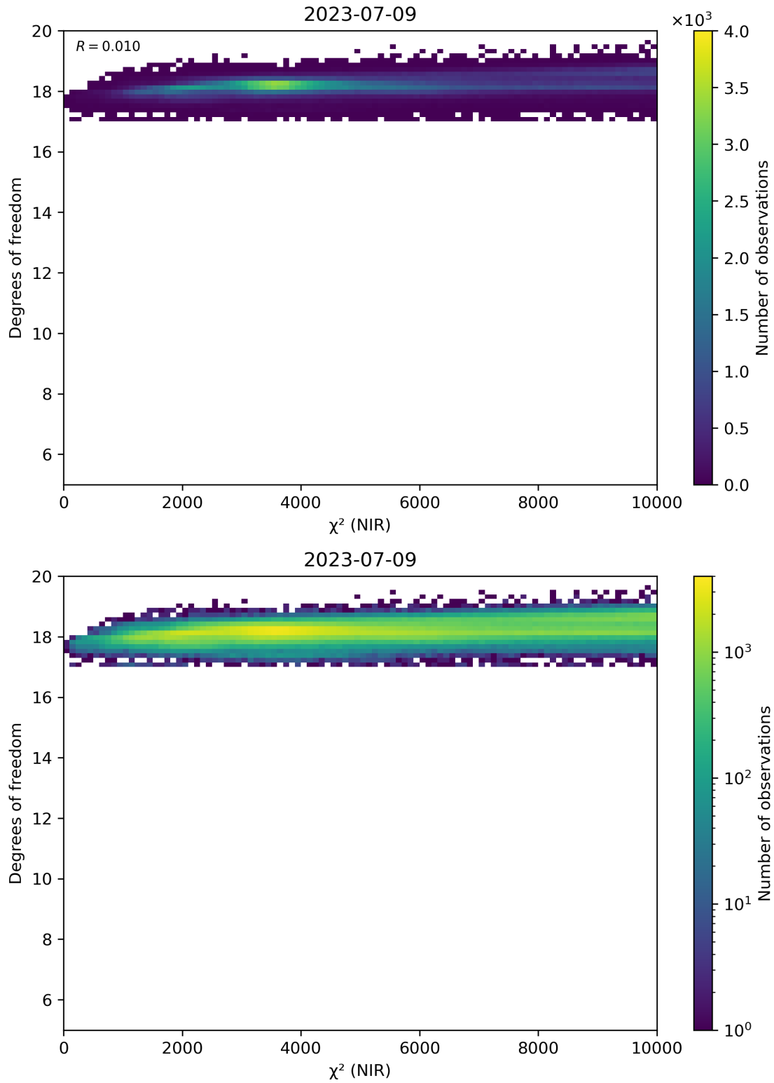
Figure 44: Scatter density plot of “ \chi^2 (NIR)” against “Degrees of freedom” for 2023-07-08 to 2023-07-10.
