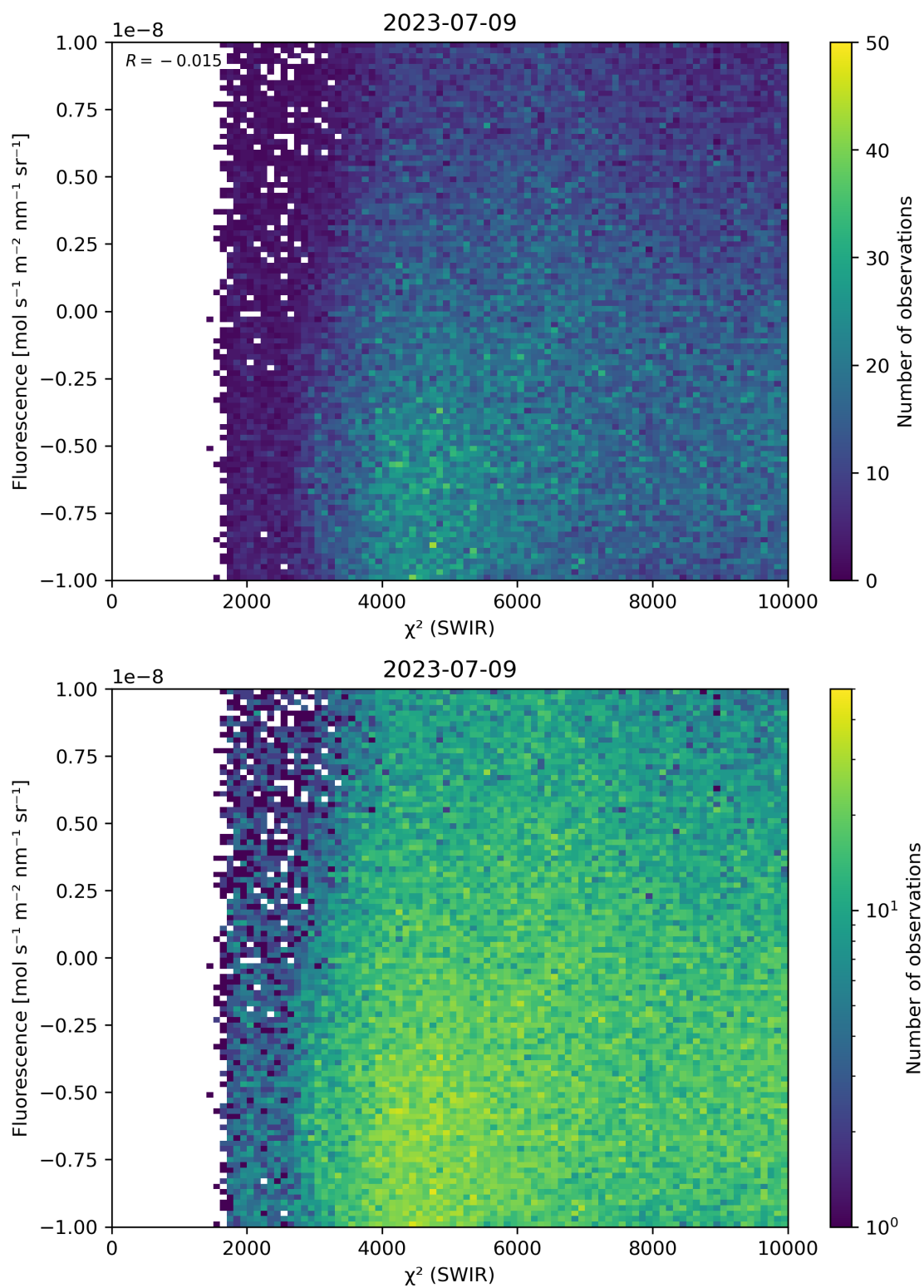
Figure 49: Scatter density plot of “ \chi^2 (SWIR)” against “Fluorescence” for 2023-07-08 to 2023-07-10.
