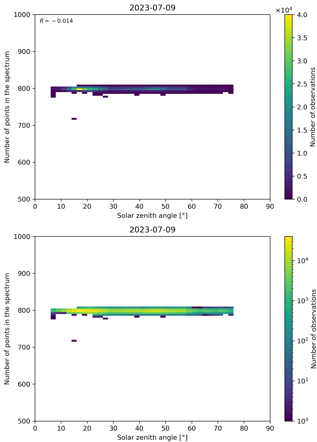
Figure 103: Scatter density plot of “Solar zenith angle” against “Number of points in the spectrum” for 2023-07-08 to 2023-07-10.
