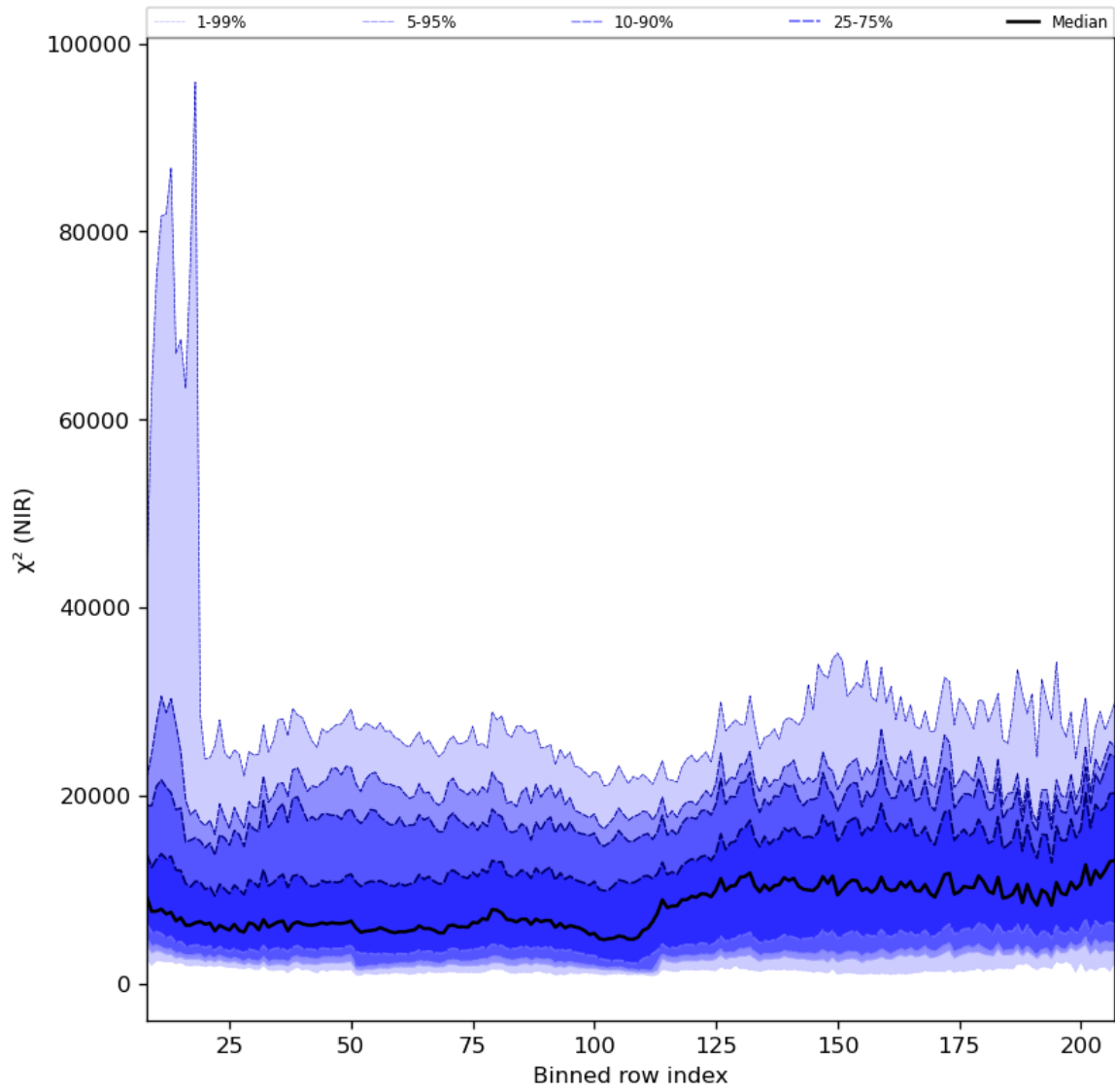
Figure 40: Along track statistics of “ \chi^2 (NIR)” for 2023-07-08 to 2023-07-10
