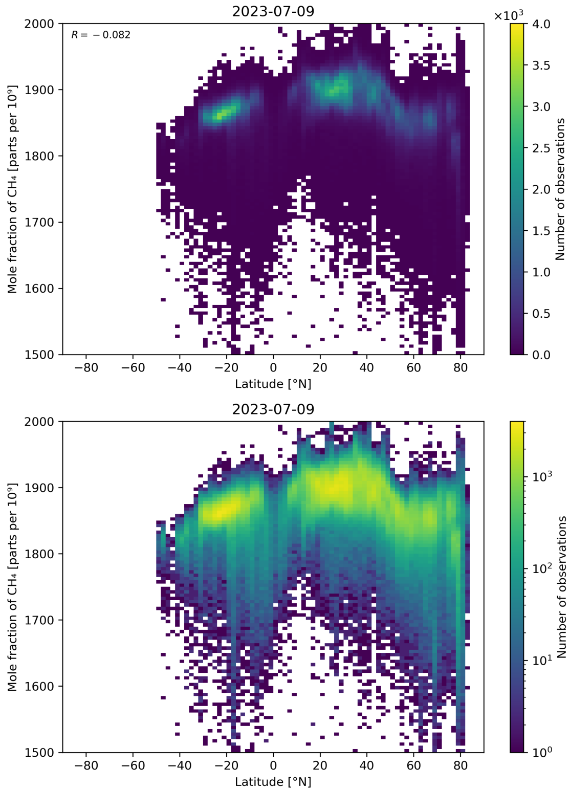
Figure 57: Scatter density plot of “Latitude” against “Mole fraction of CH 4 ” for 2023-07-08 to 2023-07-10.
