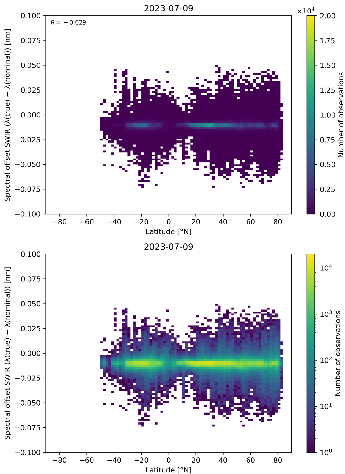
Figure 62: Scatter density plot of “Latitude” against “Spectral offset SWIR ( \lambda(\text{true}) - \lambda(\text{nominal}) )” for 2023-07-08 to 2023-07-10.
