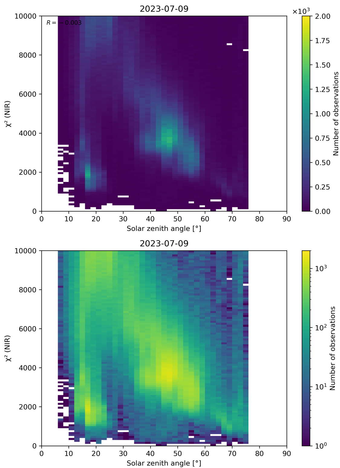
Figure 94: Scatter density plot of “Solar zenith angle” against “ \chi^2 (NIR)” for 2023-07-08 to 2023-07-10.
