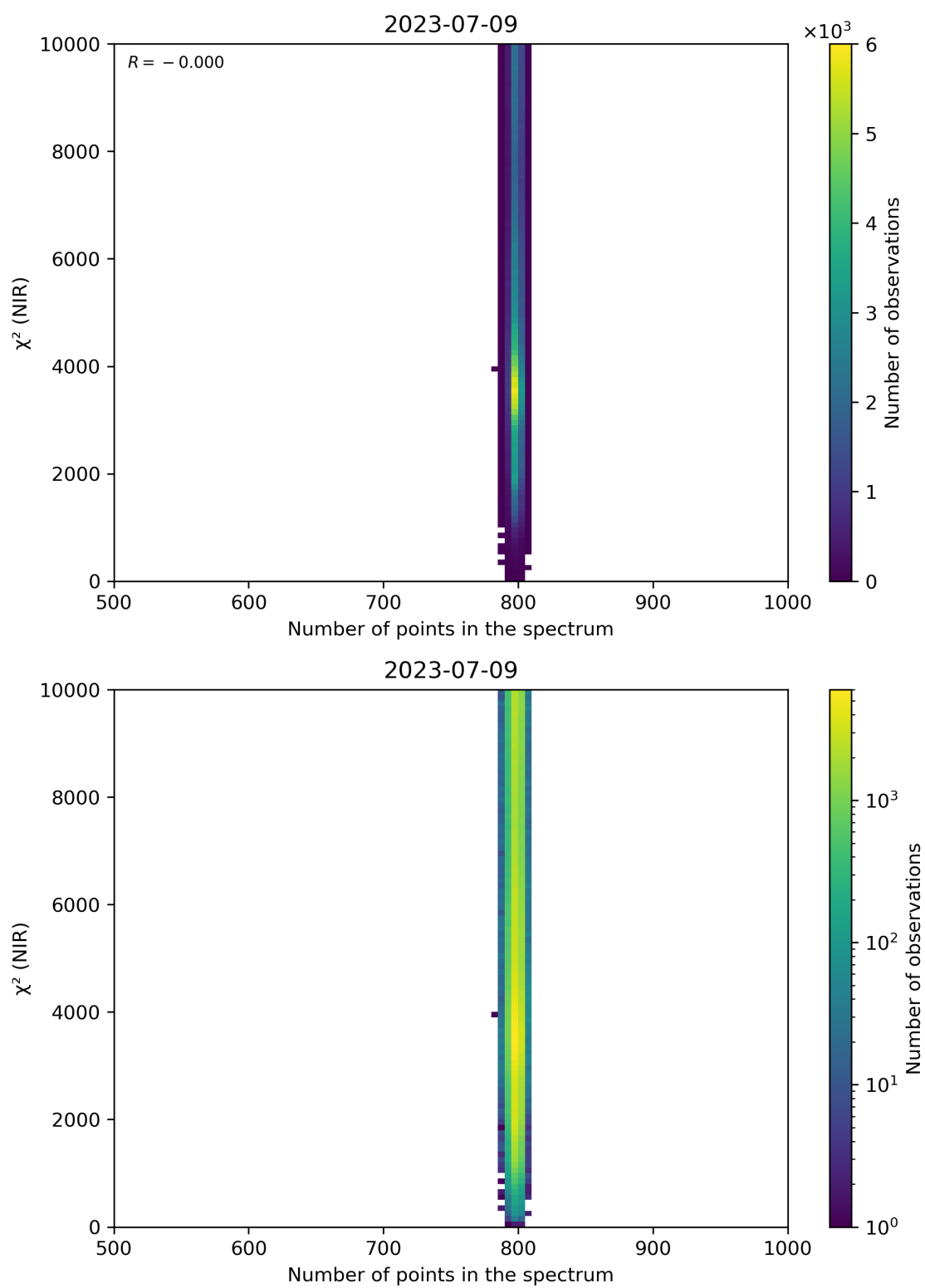
Figure 88: Scatter density plot of “Number of points in the spectrum” against “ \chi^2 (NIR)” for 2023-07-08 to 2023-07-10.
