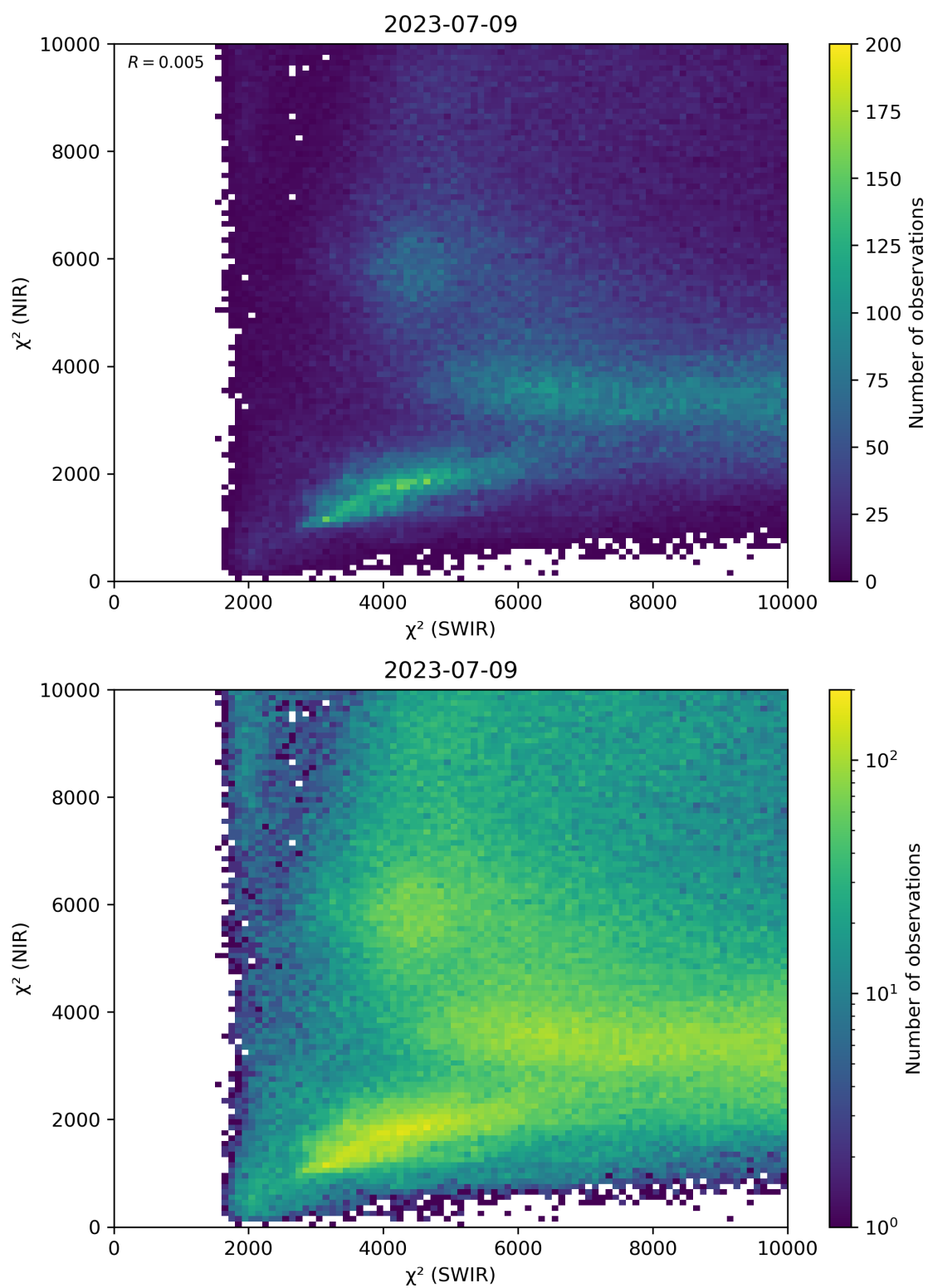
Figure 47: Scatter density plot of “ \chi^2 (SWIR)” against “ \chi^2 (NIR)” for 2023-07-08 to 2023-07-10.
