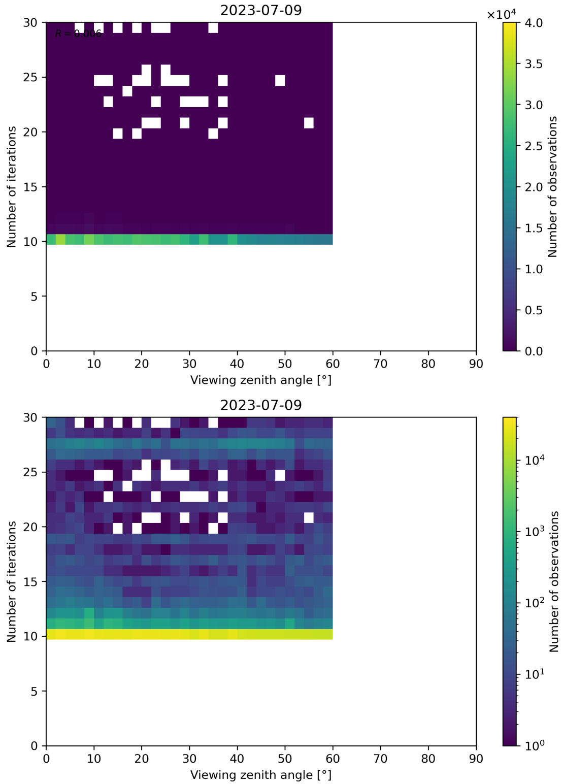
Figure 113: Scatter density plot of “Viewing zenith angle” against “Number of iterations” for 2023-07-08 to 2023-07-10.
