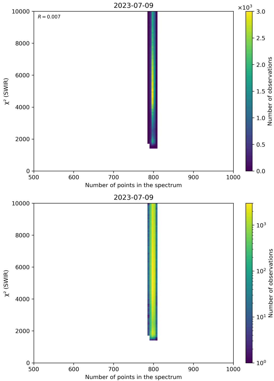
Figure 89: Scatter density plot of “Number of points in the spectrum” against “ \chi^2 (SWIR)” for 2023-07-08 to 2023-07-10.
