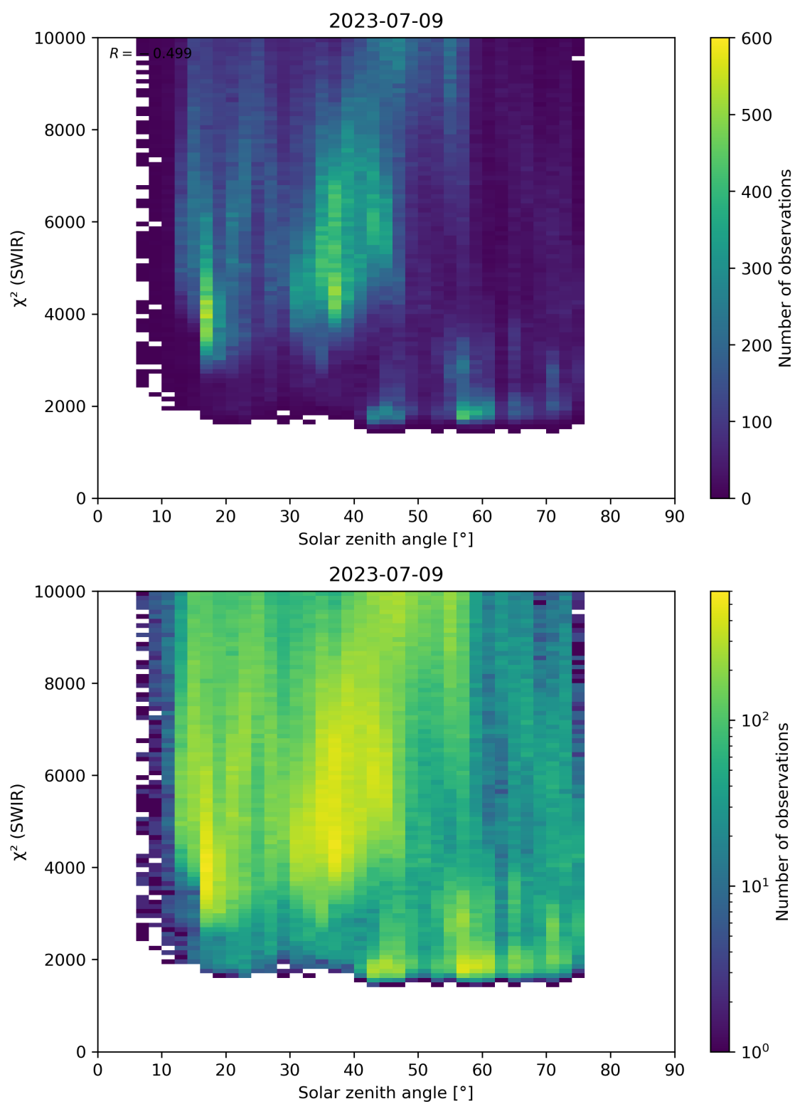
Figure 95: Scatter density plot of “Solar zenith angle” against “ \chi^2 (SWIR)” for 2023-07-08 to 2023-07-10.
