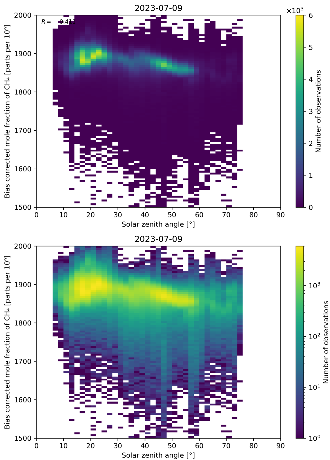
Figure 100: Scatter density plot of “Solar zenith angle” against “Bias corrected mole fraction of CH 4 ” for 2023-07-08 to 2023-07-10.
