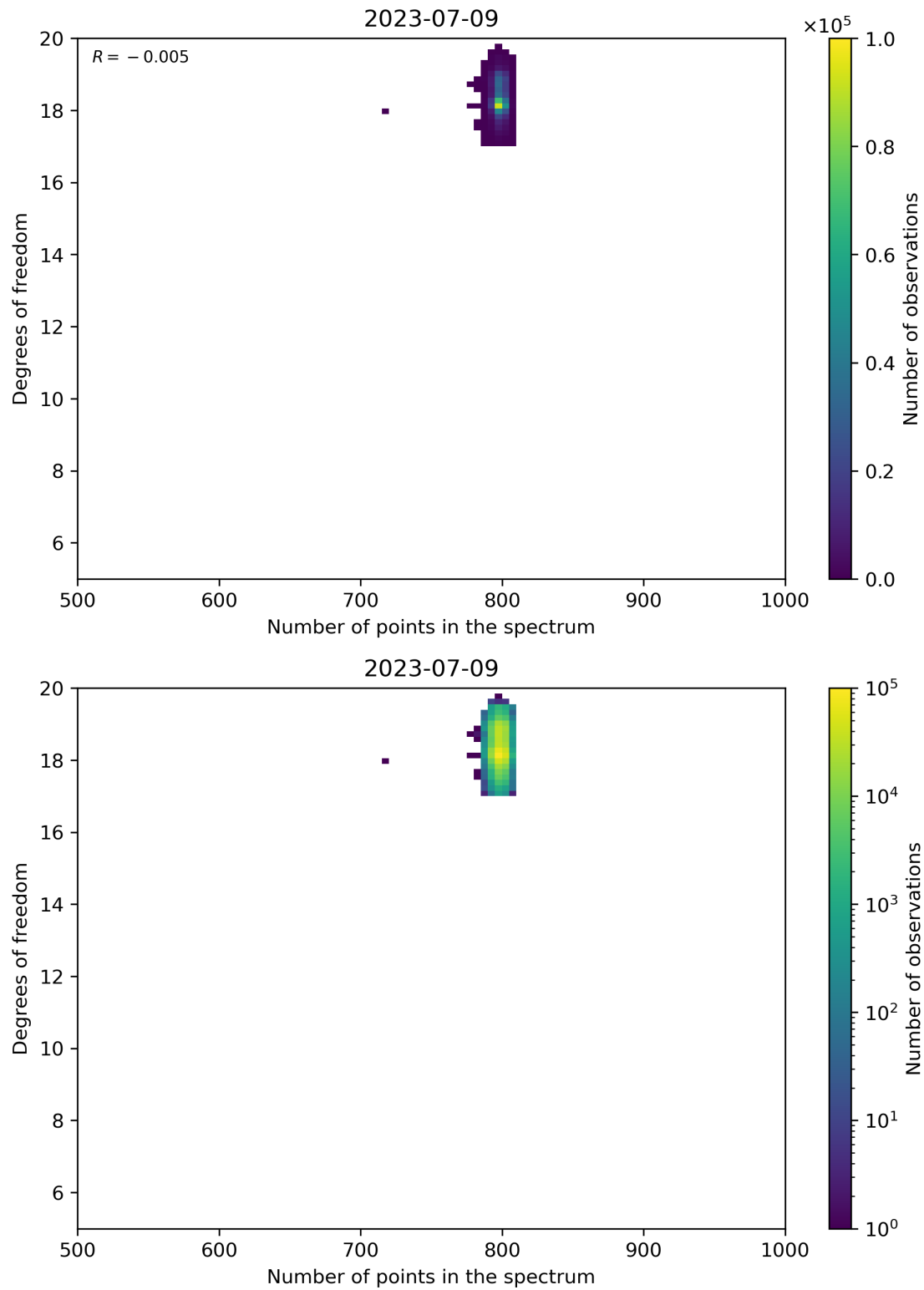
Figure 90: Scatter density plot of “Number of points in the spectrum” against “Degrees of freedom” for 2023-07-08 to 2023-07-10.
