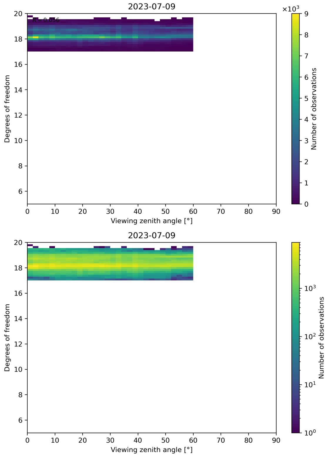
Figure 107: Scatter density plot of “Viewing zenith angle” against “Degrees of freedom” for 2023-07-08 to 2023-07-10.
