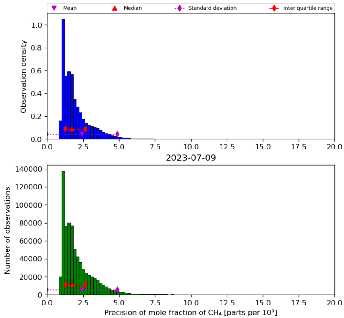
Figure 24: Histogram of “Precision of mole fraction of CH 4 ” for 2023-07-08 to 2023-07-10
