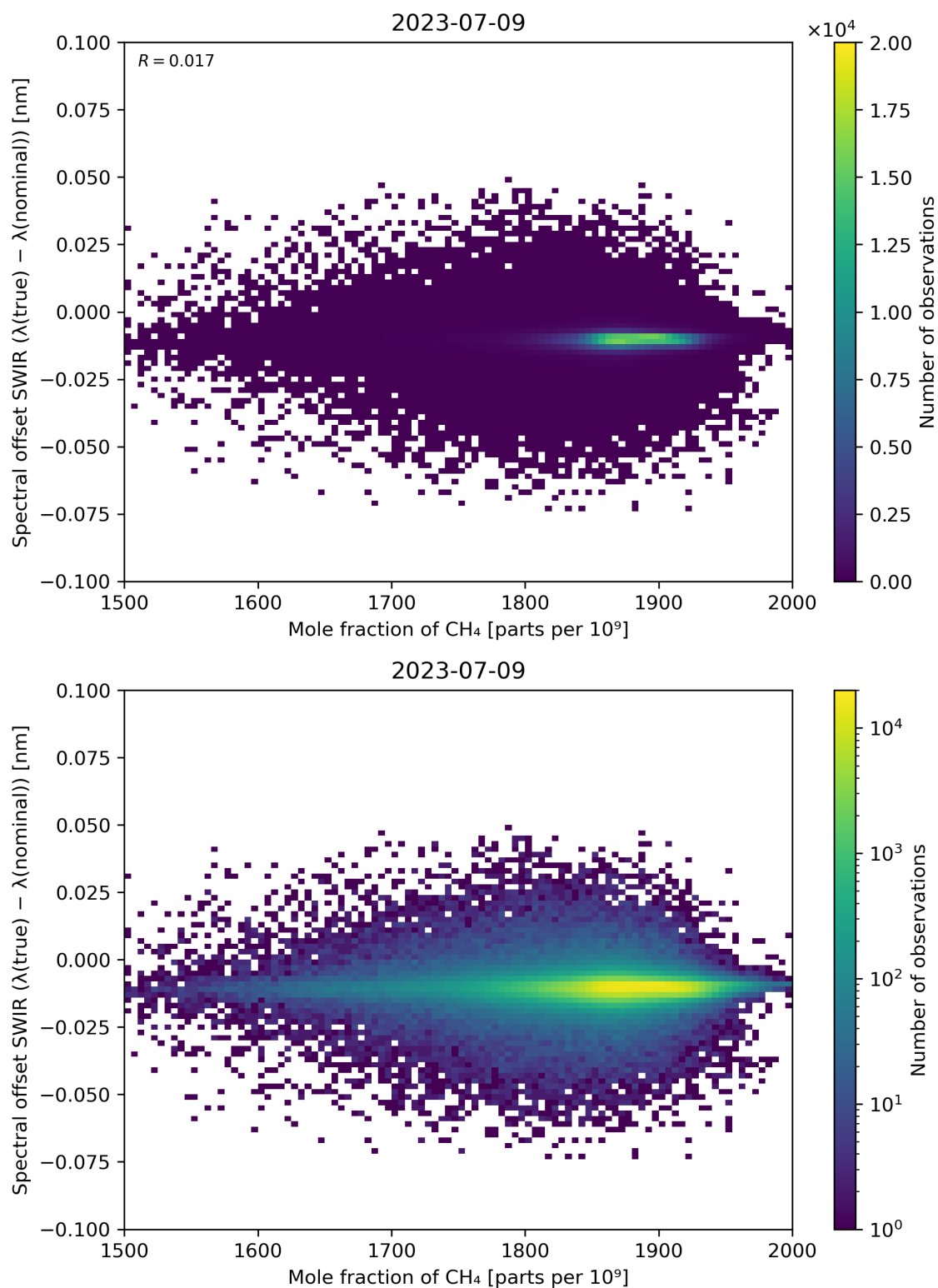
Figure 86: Scatter density plot of “Mole fraction of CH 4 ” against “Spectral offset SWIR ( \lambda(\text{true}) - \lambda(\text{nominal}) )” for 2023-07-08 to 2023-07-10.
