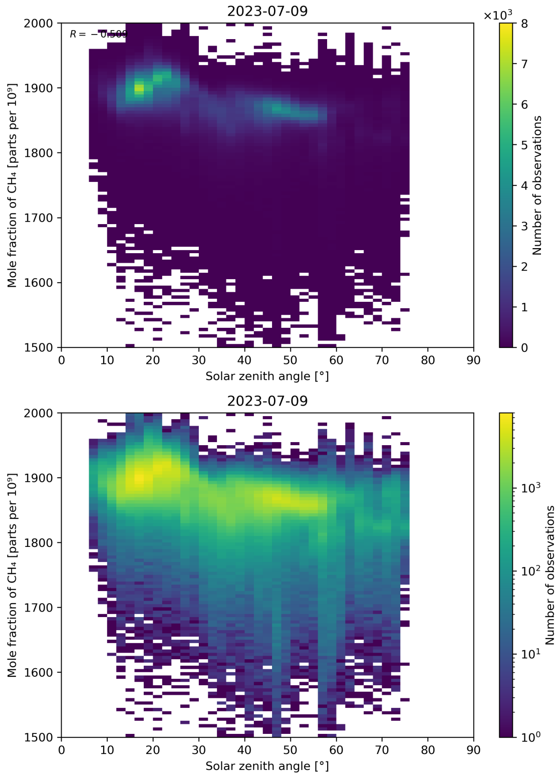
Figure 99: Scatter density plot of “Solar zenith angle” against “Mole fraction of CH 4 ” for 2023-07-08 to 2023-07-10.
