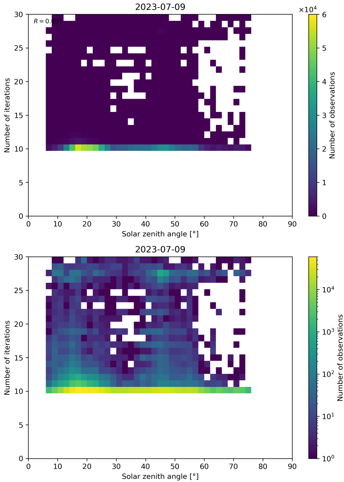
Figure 102: Scatter density plot of “Solar zenith angle” against “Number of iterations” for 2023-07-08 to 2023-07-10.
