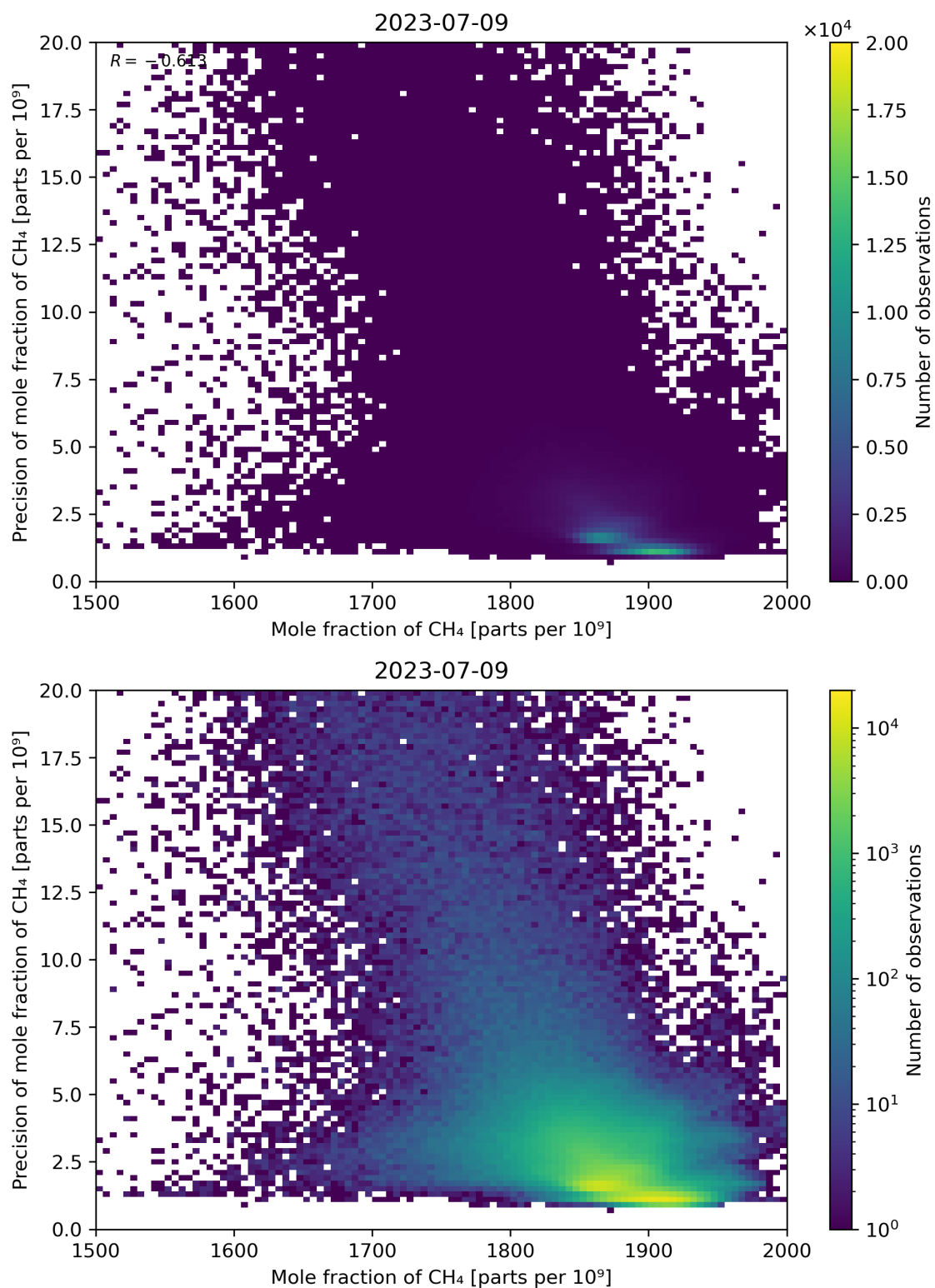
Figure 75: Scatter density plot of “Mole fraction of CH 4 ” against “Precision of mole fraction of CH 4 ” for 2023-07-08 to 2023-07-10.
