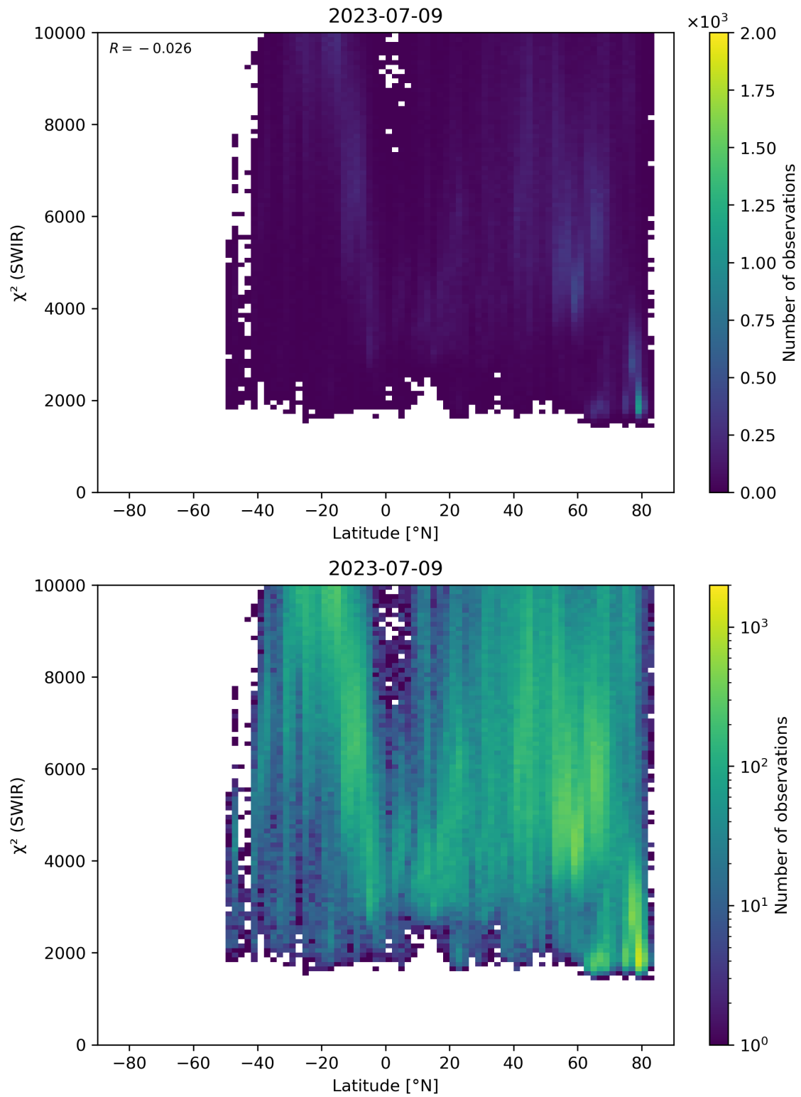
Figure 54: Scatter density plot of “Latitude” against “ \chi^2 (SWIR)” for 2023-07-08 to 2023-07-10.
