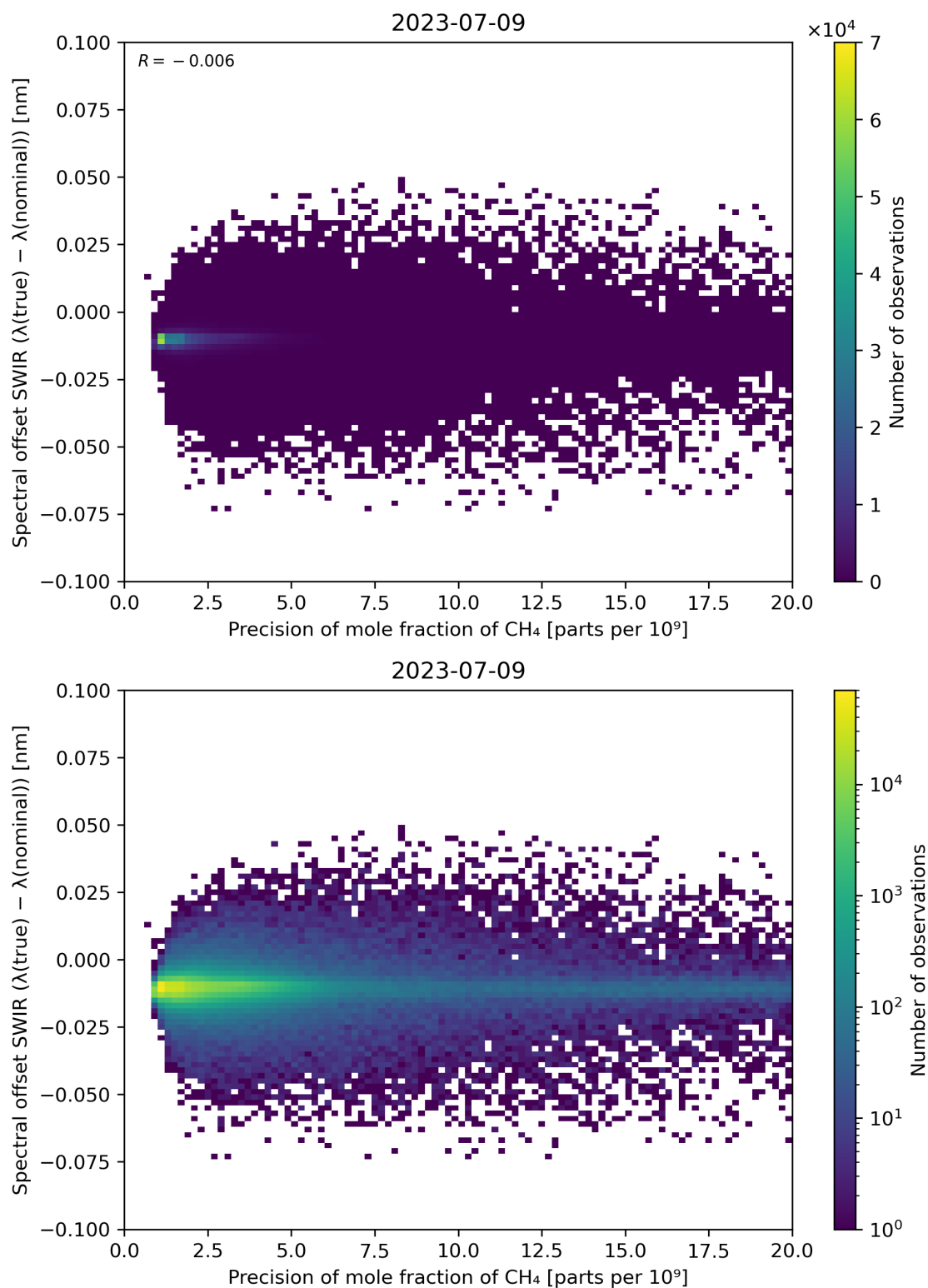
Figure 85: Scatter density plot of “Precision of mole fraction of CH 4 ” against “Spectral offset SWIR ( \lambda(\text{true}) - \lambda(\text{nominal}) )” for 2023-07-08 to 2023-07-10.
