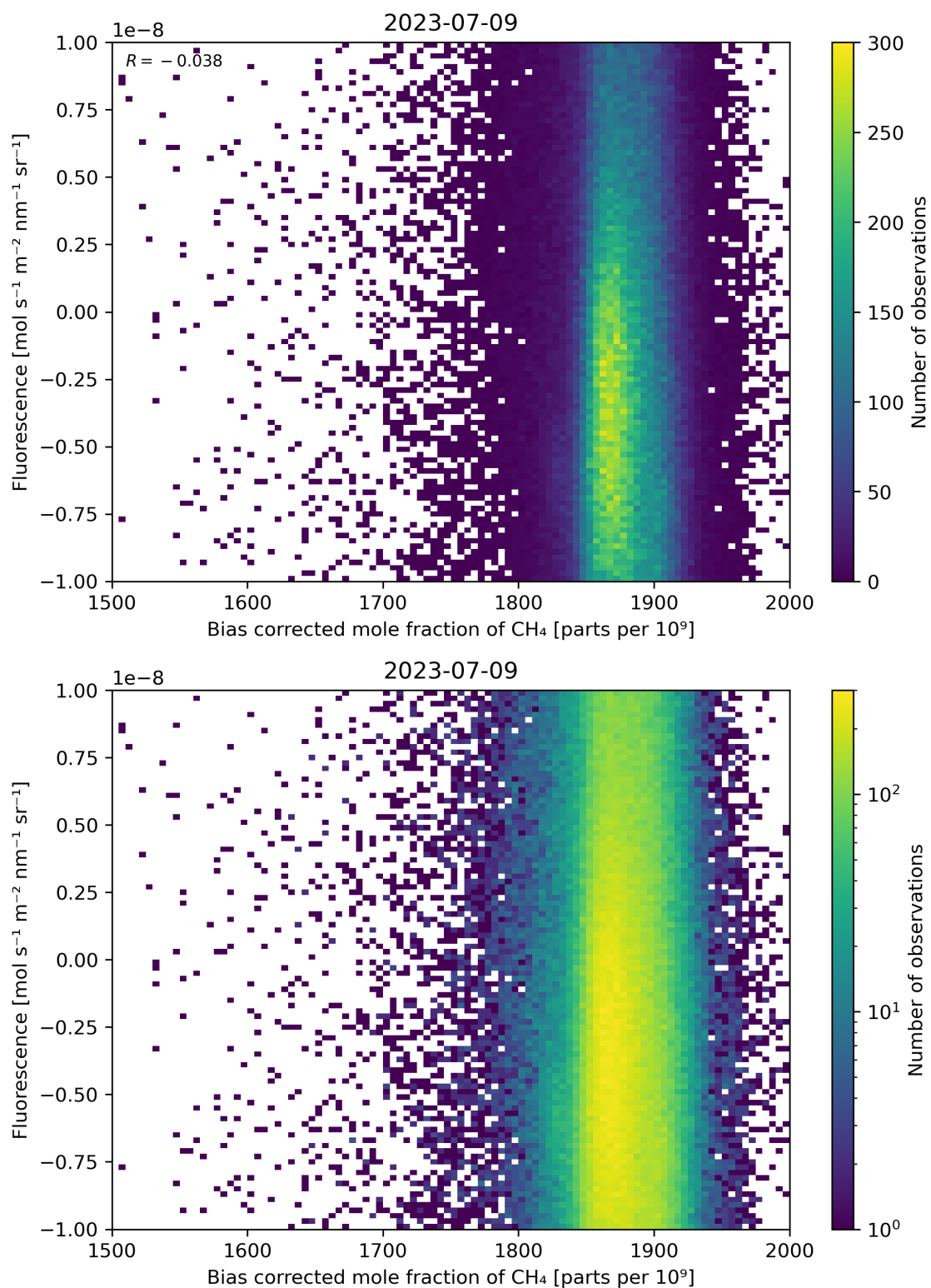
Figure 66: Scatter density plot of “Bias corrected mole fraction of \text{CH}_4 ” against “Fluorescence” for 2023-07-08 to 2023-07-10.
