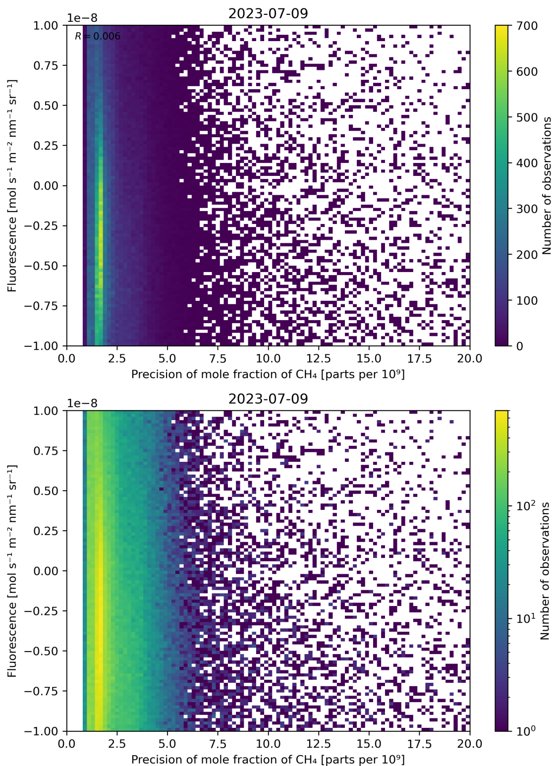
Figure 81: Scatter density plot of “Precision of mole fraction of \text{CH}_4 ” against “Fluorescence” for 2023-07-08 to 2023-07-10.
