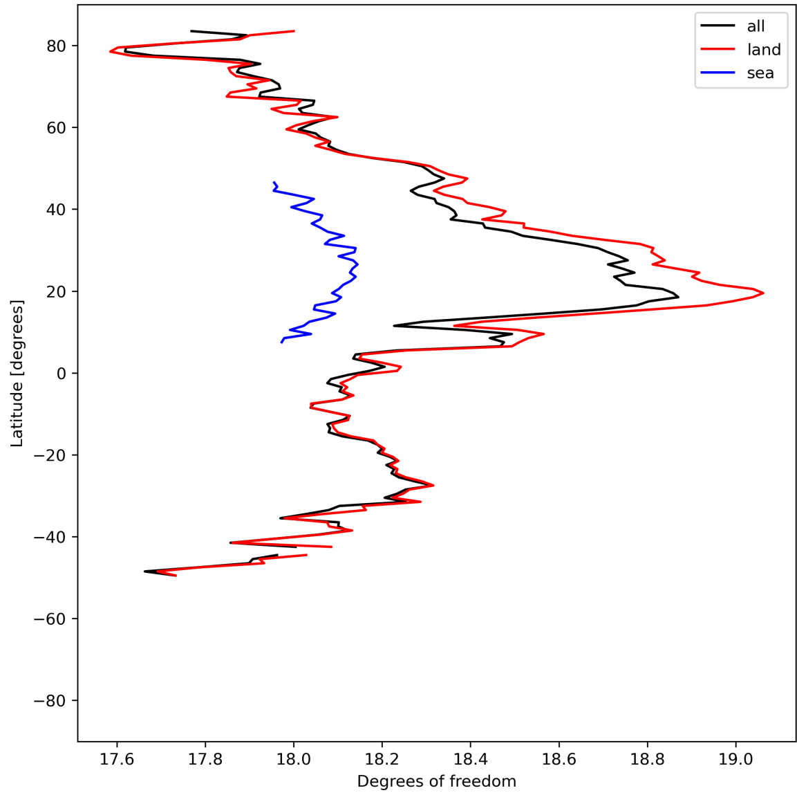
Figure 19: Zonal average of “Degrees of freedom” for 2023-07-08 to 2023-07-10.
