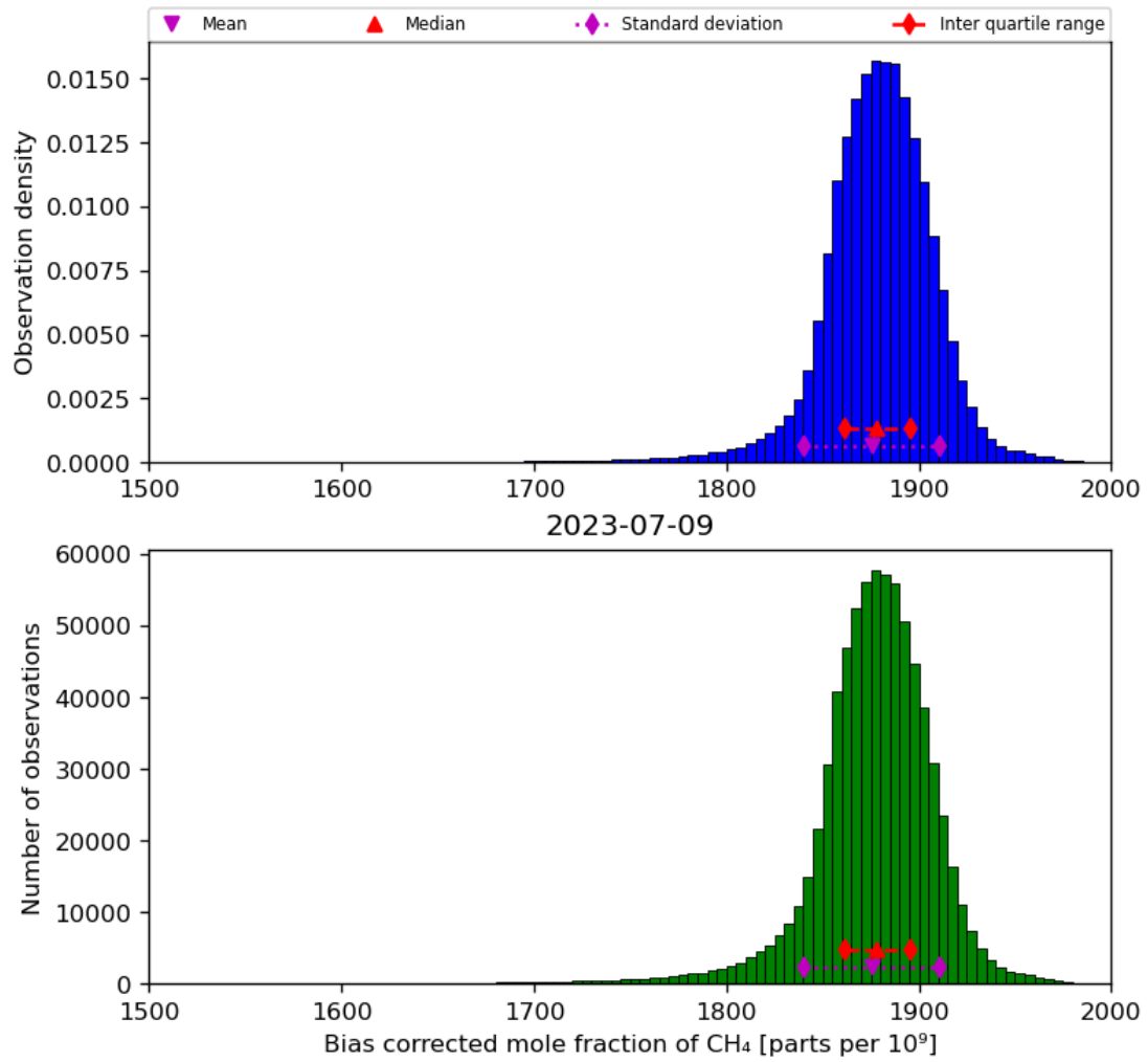
Figure 25: Histogram of “Bias corrected mole fraction of CH 4 ” for 2023-07-08 to 2023-07-10
