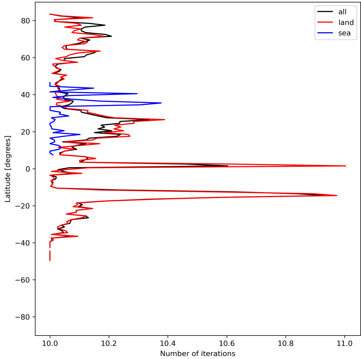
Figure 20: Zonal average of “Number of iterations” for 2023-07-08 to 2023-07-10.
