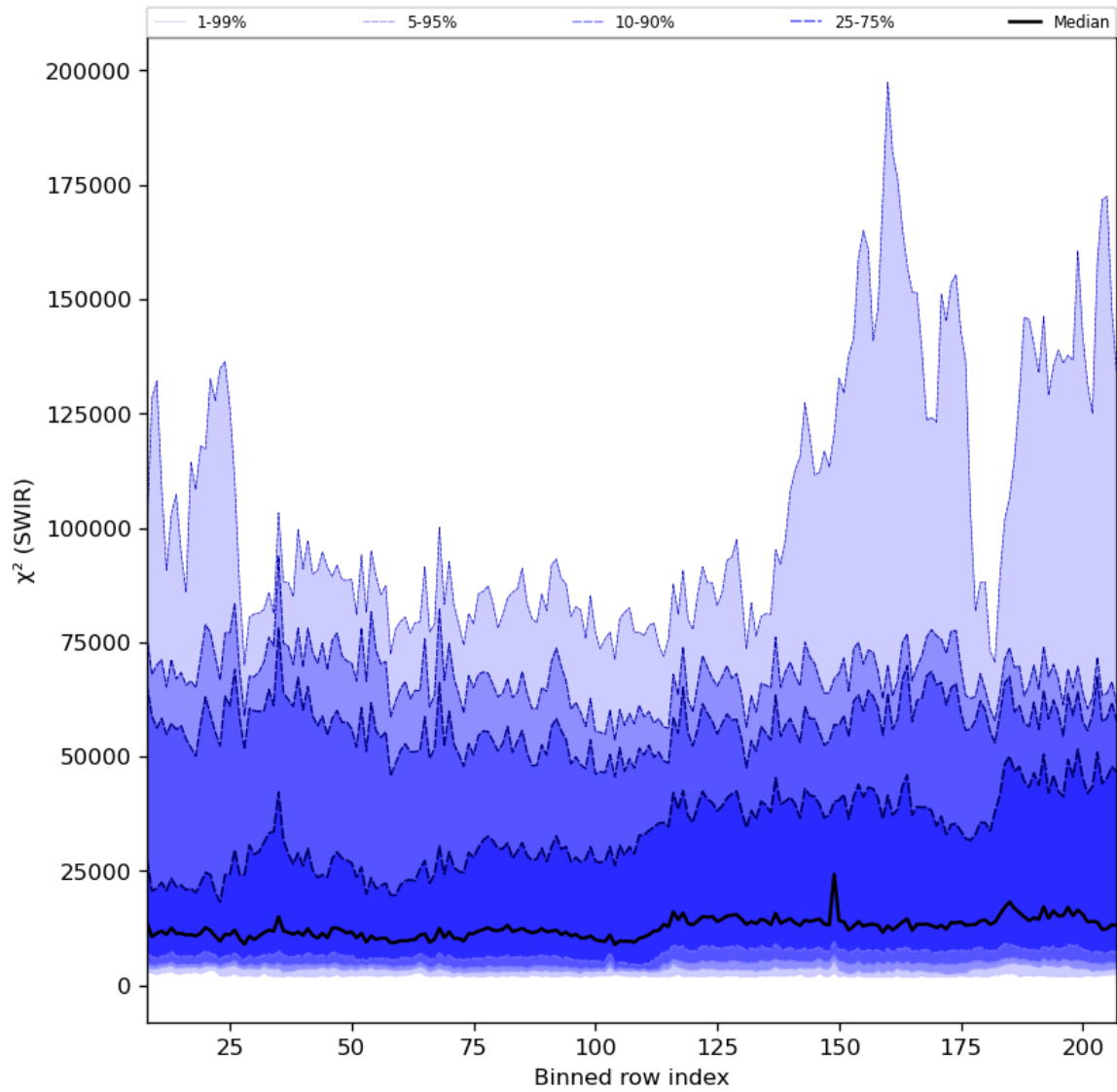
Figure 39: Along track statistics of " \chi^2 (SWIR)" for 2023-07-08 to 2023-07-10
