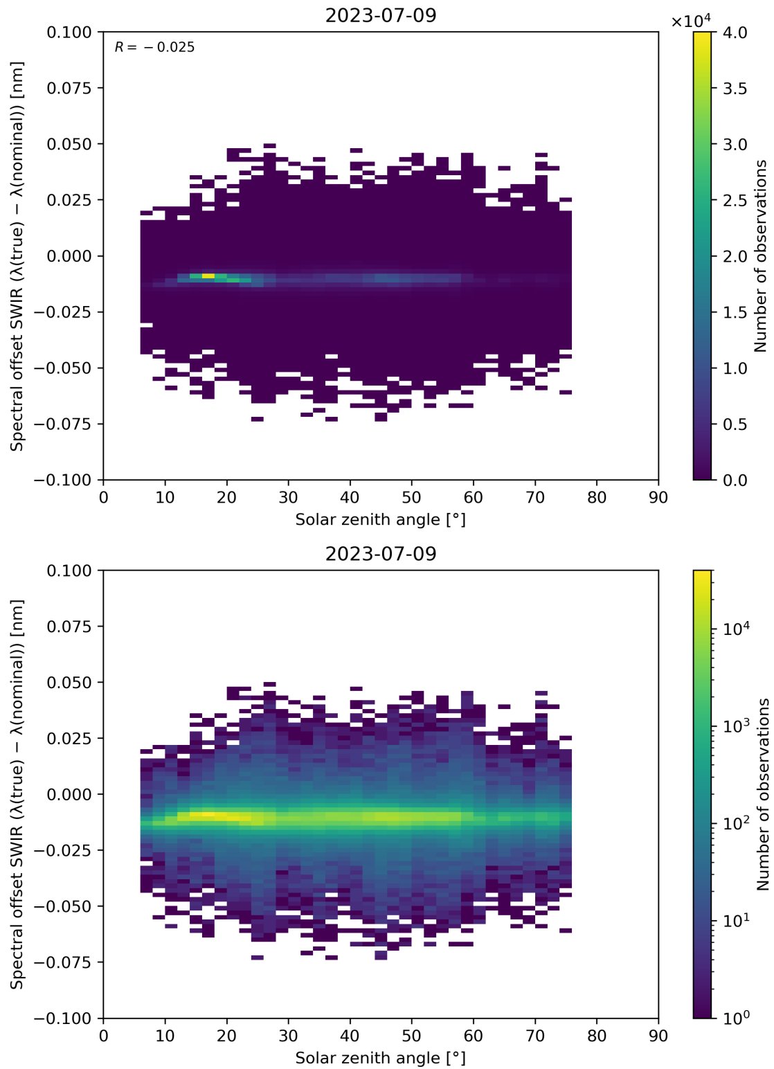
Figure 104: Scatter density plot of “Solar zenith angle” against “Spectral offset SWIR ( \lambda(\text{true}) - \lambda(\text{nominal}) )” for 2023-07-08 to 2023-07-10.
