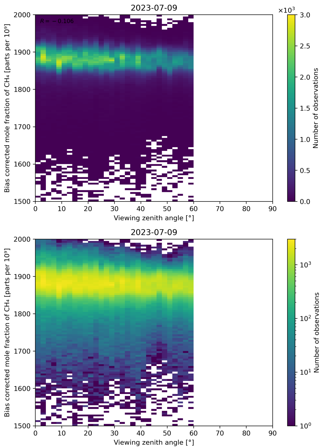
Figure 111: Scatter density plot of “Viewing zenith angle” against “Bias corrected mole fraction of CH 4 ” for 2023-07-08 to 2023-07-10.
