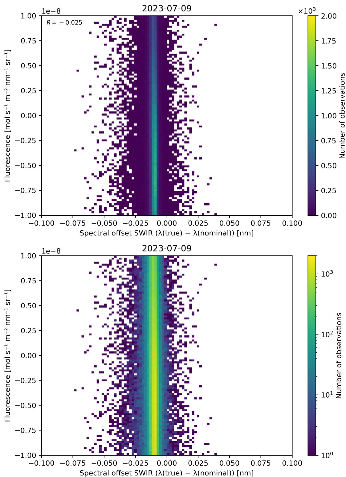
Figure 120: Scatter density plot of “Spectral offset SWIR ( \lambda(\text{true}) - \lambda(\text{nominal}) )” against “Fluorescence” for 2023-07-08 to 2023-07-10.
