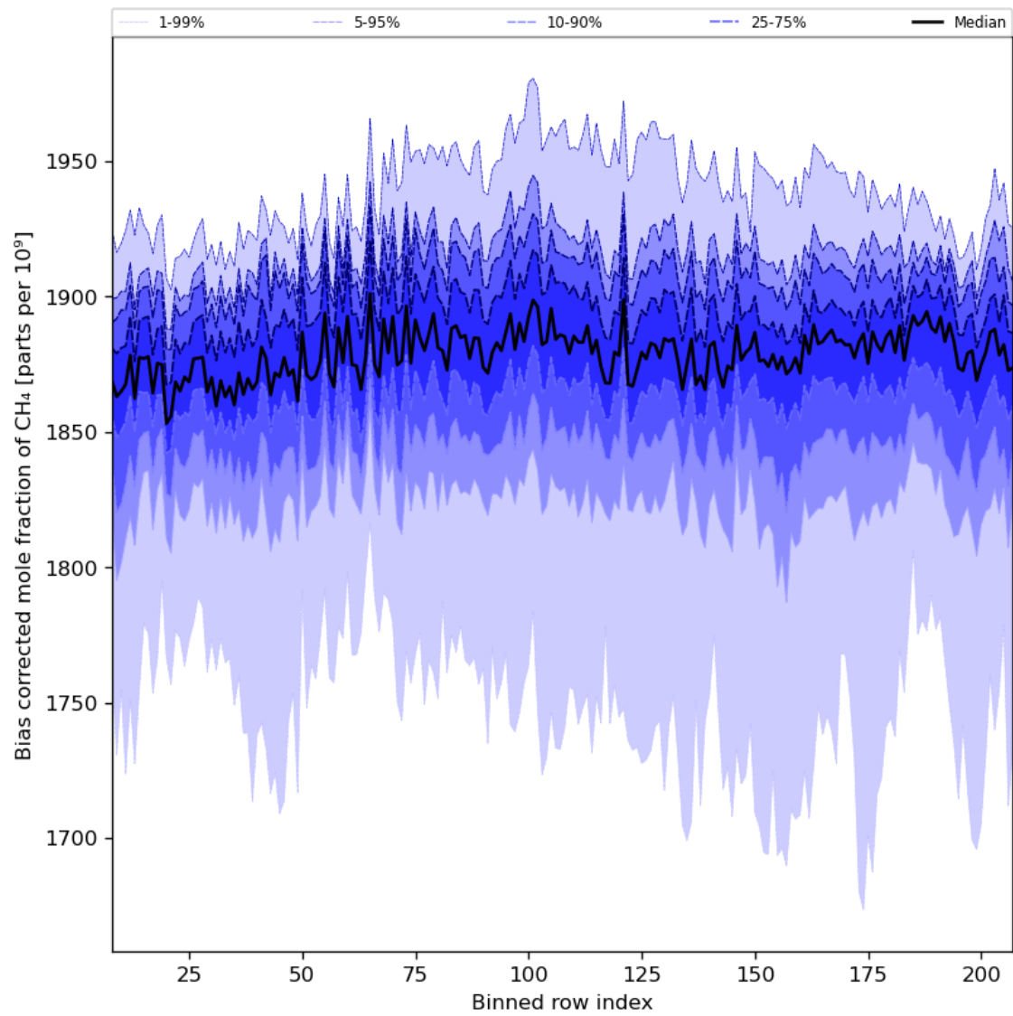
Figure 36: Along track statistics of “Bias corrected mole fraction of CH 4 ” for 2023-07-08 to 2023-07-10
