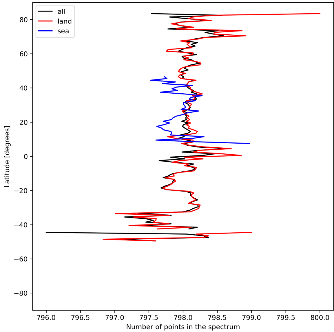
Figure 15: Zonal average of “Number of points in the spectrum” for 2023-07-08 to 2023-07-10.
