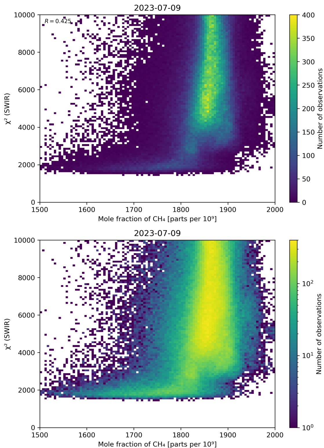
Figure 71: Scatter density plot of “Mole fraction of \text{CH}_4 ” against “ \chi^2 (SWIR)” for 2023-07-08 to 2023-07-10.
