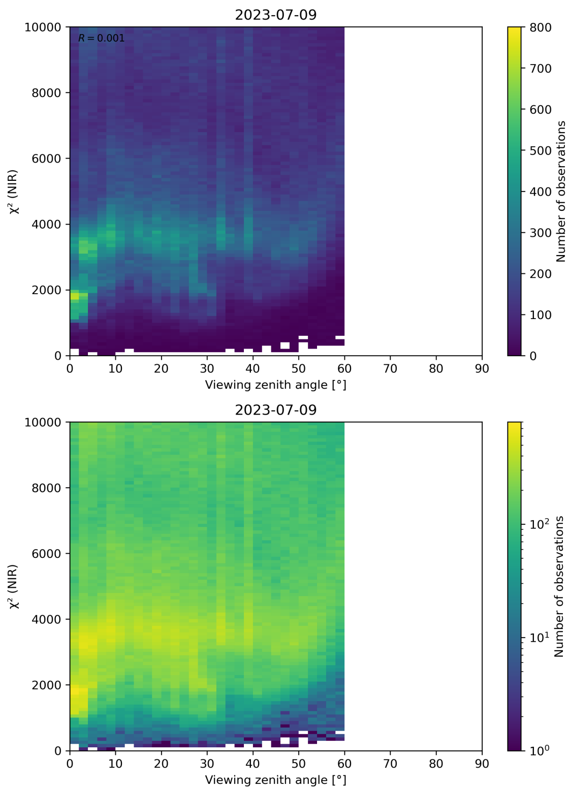
Figure 105: Scatter density plot of “Viewing zenith angle” against “ \chi^2 (NIR)” for 2023-07-08 to 2023-07-10.
