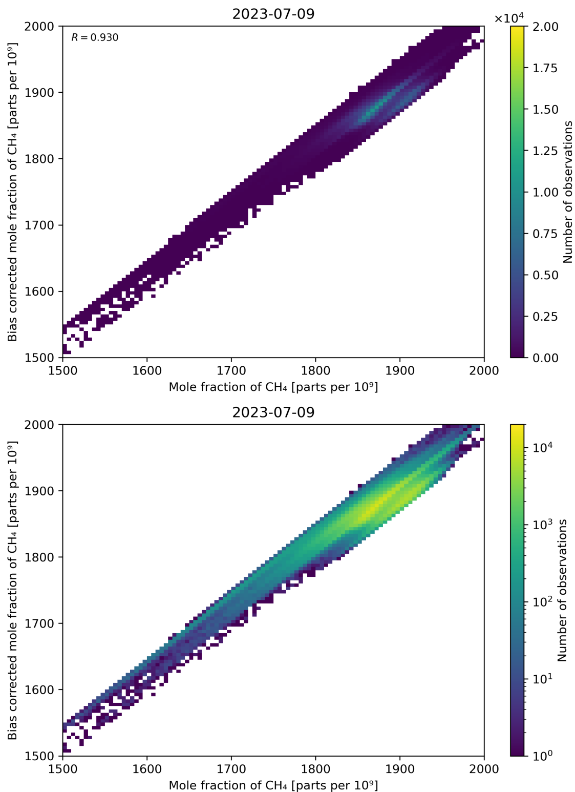
Figure 74: Scatter density plot of “Mole fraction of CH 4 ” against “Bias corrected mole fraction of CH 4 ” for 2023-07-08 to 2023-07-10.
