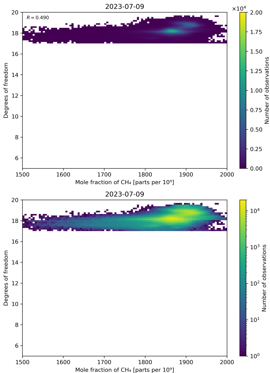
Figure 72: Scatter density plot of “Mole fraction of CH 4 ” against “Degrees of freedom” for 2023-07-08 to 2023-07-10.
