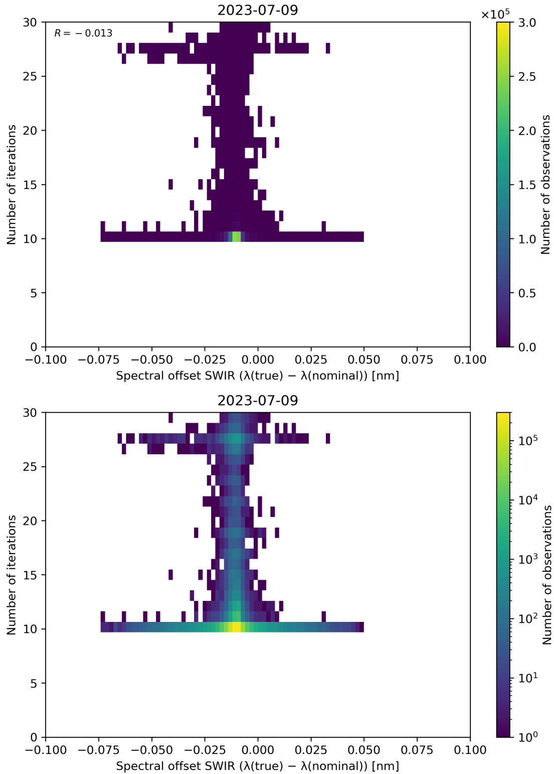
Figure 121: Scatter density plot of “Spectral offset SWIR ( \lambda(\text{true}) - \lambda(\text{nominal}) )” against “Number of iterations” for 2023-07-08 to 2023-07-10.
