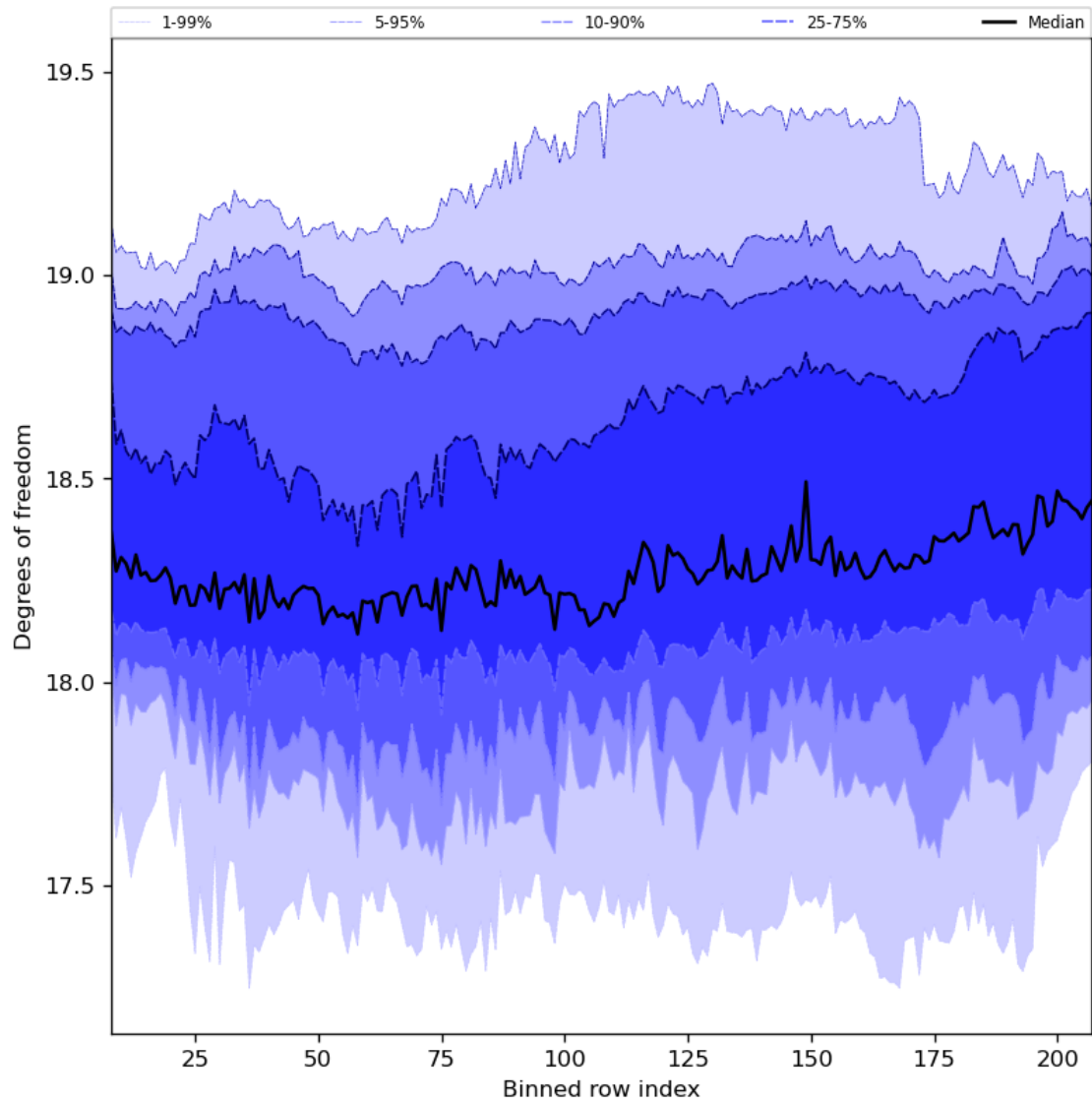
Figure 41: Along track statistics of “Degrees of freedom” for 2023-07-08 to 2023-07-10
