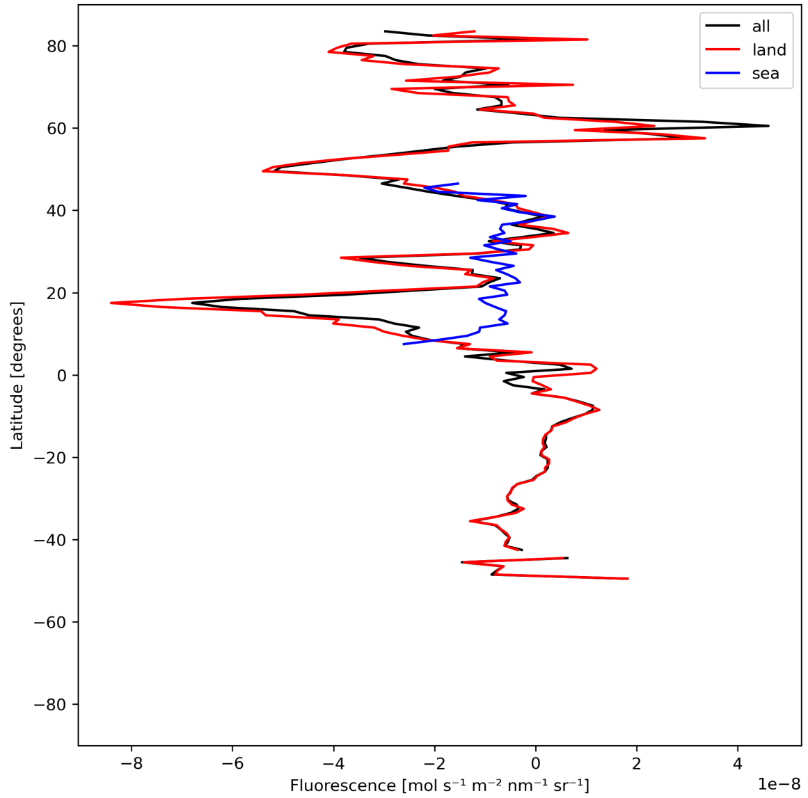
Figure 21: Zonal average of “Fluorescence” for 2023-07-08 to 2023-07-10.
