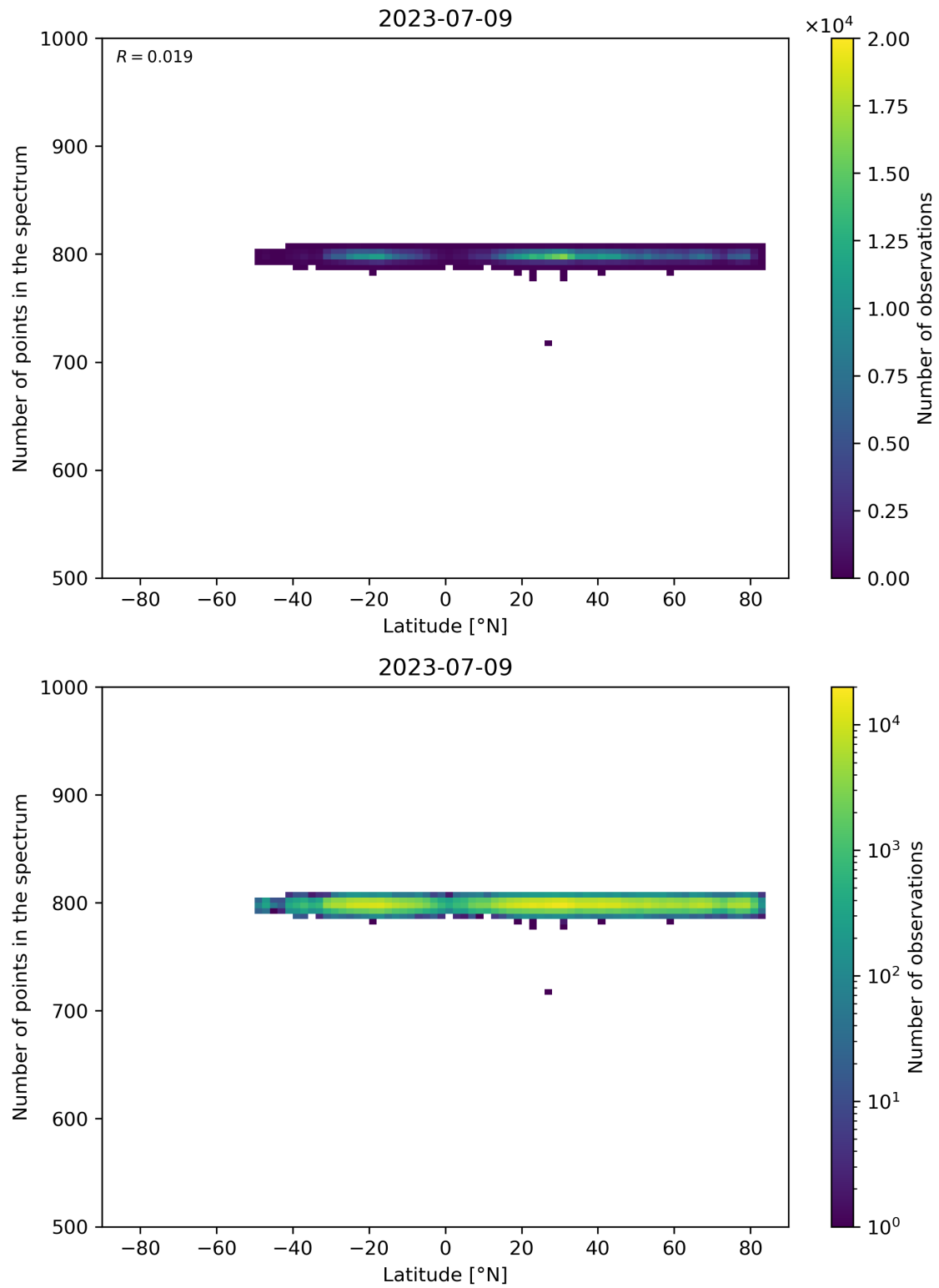
Figure 61: Scatter density plot of “Latitude” against “Number of points in the spectrum” for 2023-07-08 to 2023-07-10.
