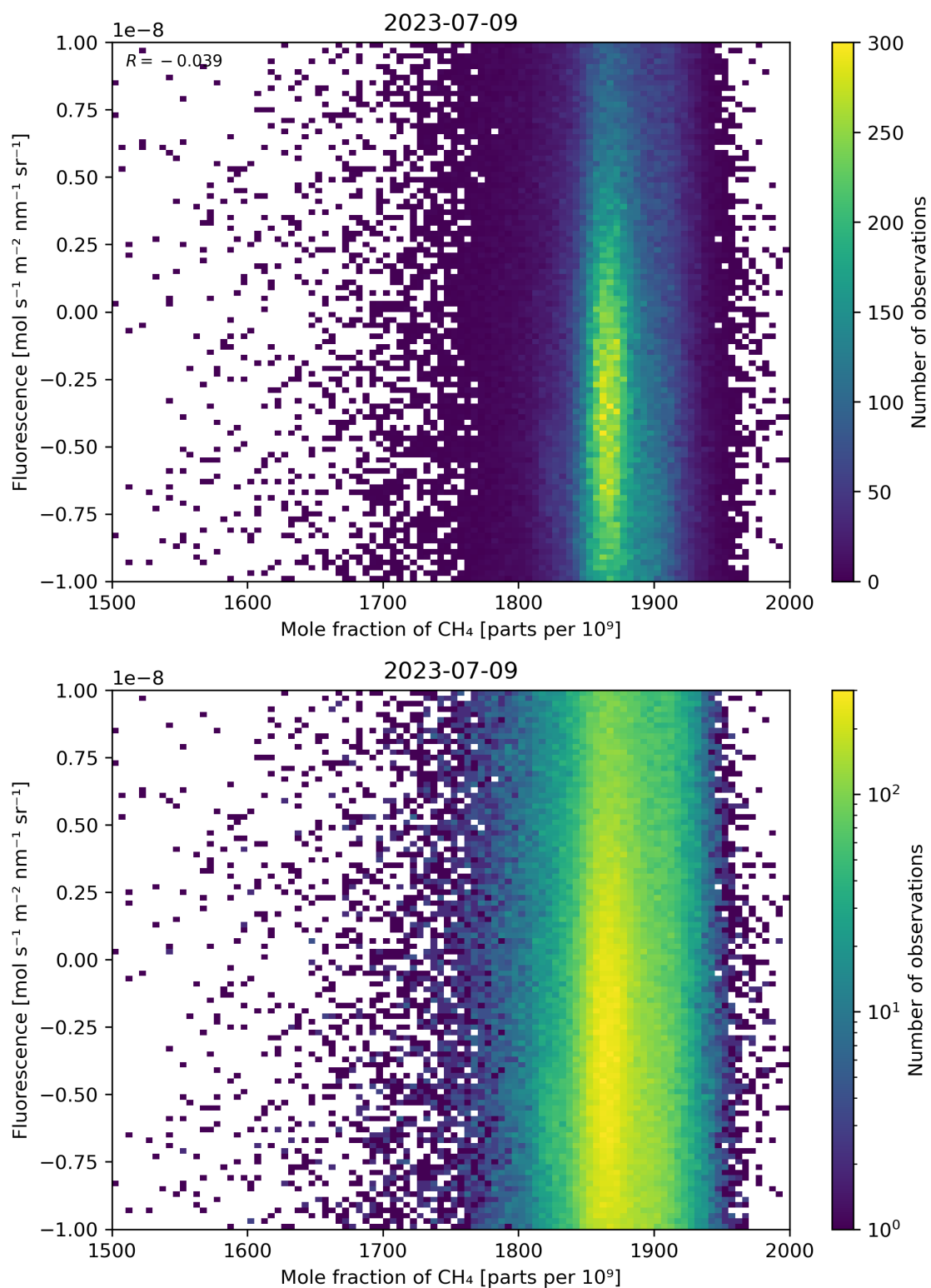
Figure 73: Scatter density plot of “Mole fraction of \text{CH}_4 ” against “Fluorescence” for 2023-07-08 to 2023-07-10.
