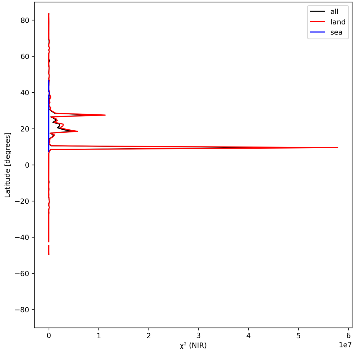
Figure 18: Zonal average of “ \chi^2 (NIR)” for 2023-07-08 to 2023-07-10.
