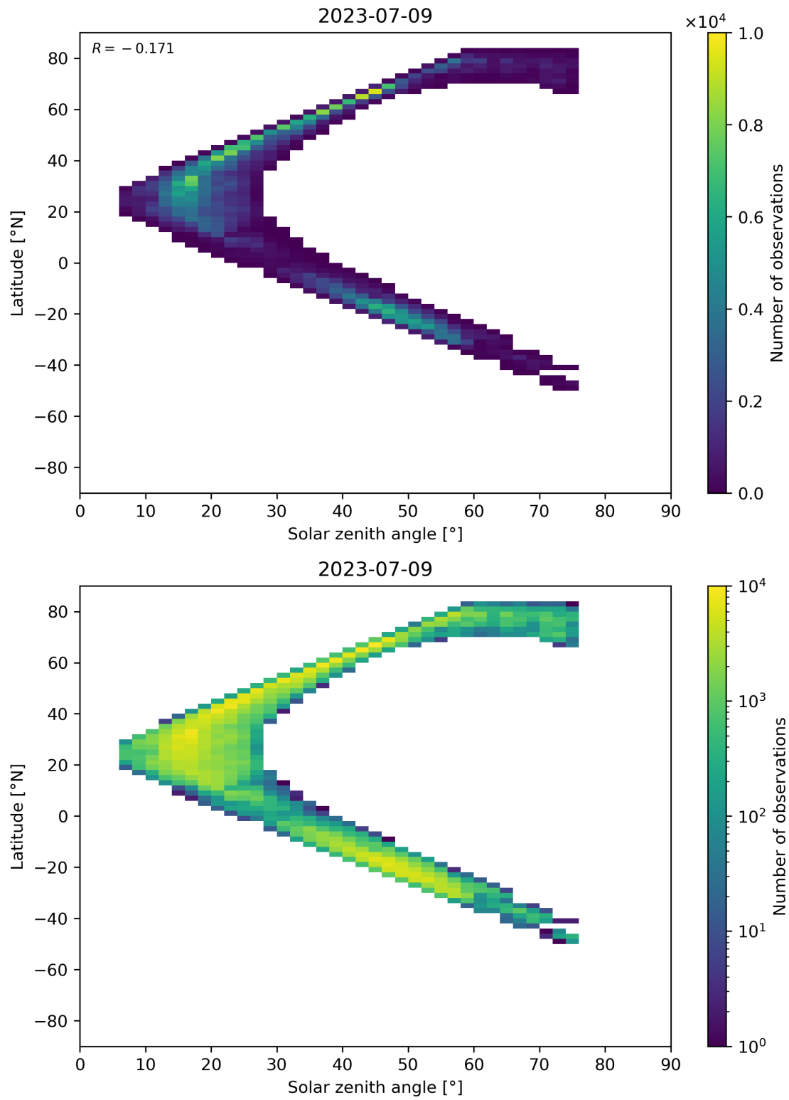
Figure 98: Scatter density plot of “Solar zenith angle” against “Latitude” for 2023-07-08 to 2023-07-10.
