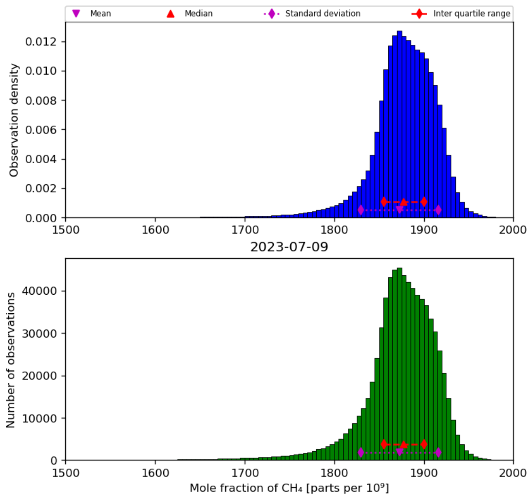
Figure 23: Histogram of “Mole fraction of CH 4 ” for 2023-07-08 to 2023-07-10
