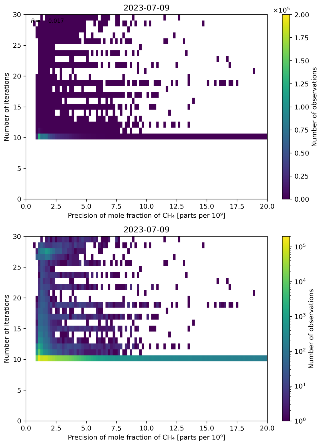
Figure 83: Scatter density plot of “Precision of mole fraction of CH 4 ” against “Number of iterations” for 2023-07-08 to 2023-07-10.
