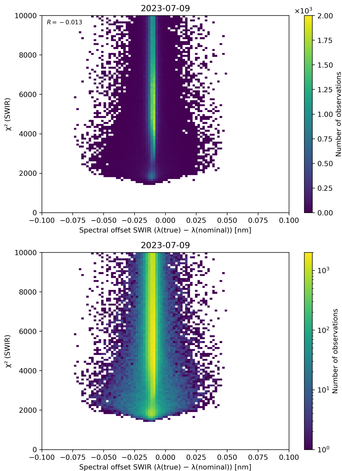
Figure 118: Scatter density plot of “Spectral offset SWIR ( \lambda(\text{true}) - \lambda(\text{nominal}) )” against “ \chi^2 (SWIR)” for 2023-07-08 to 2023-07-10.
