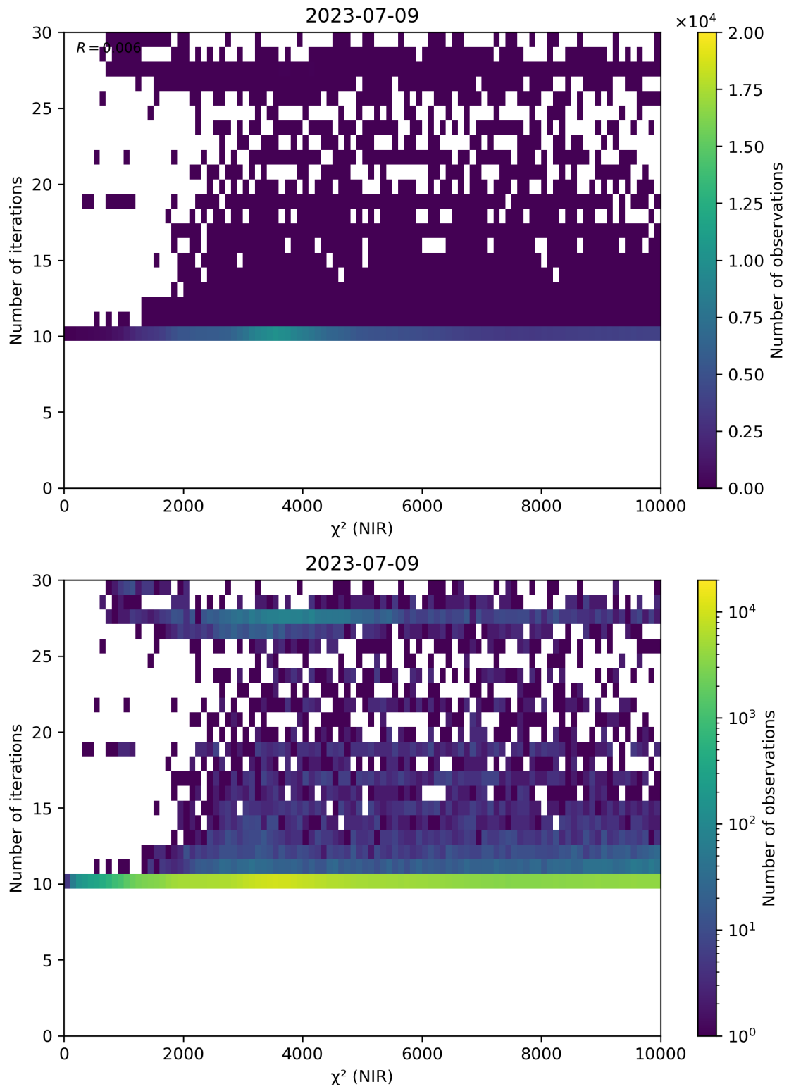
Figure 46: Scatter density plot of “ \chi^2 (NIR)” against “Number of iterations” for 2023-07-08 to 2023-07-10.
