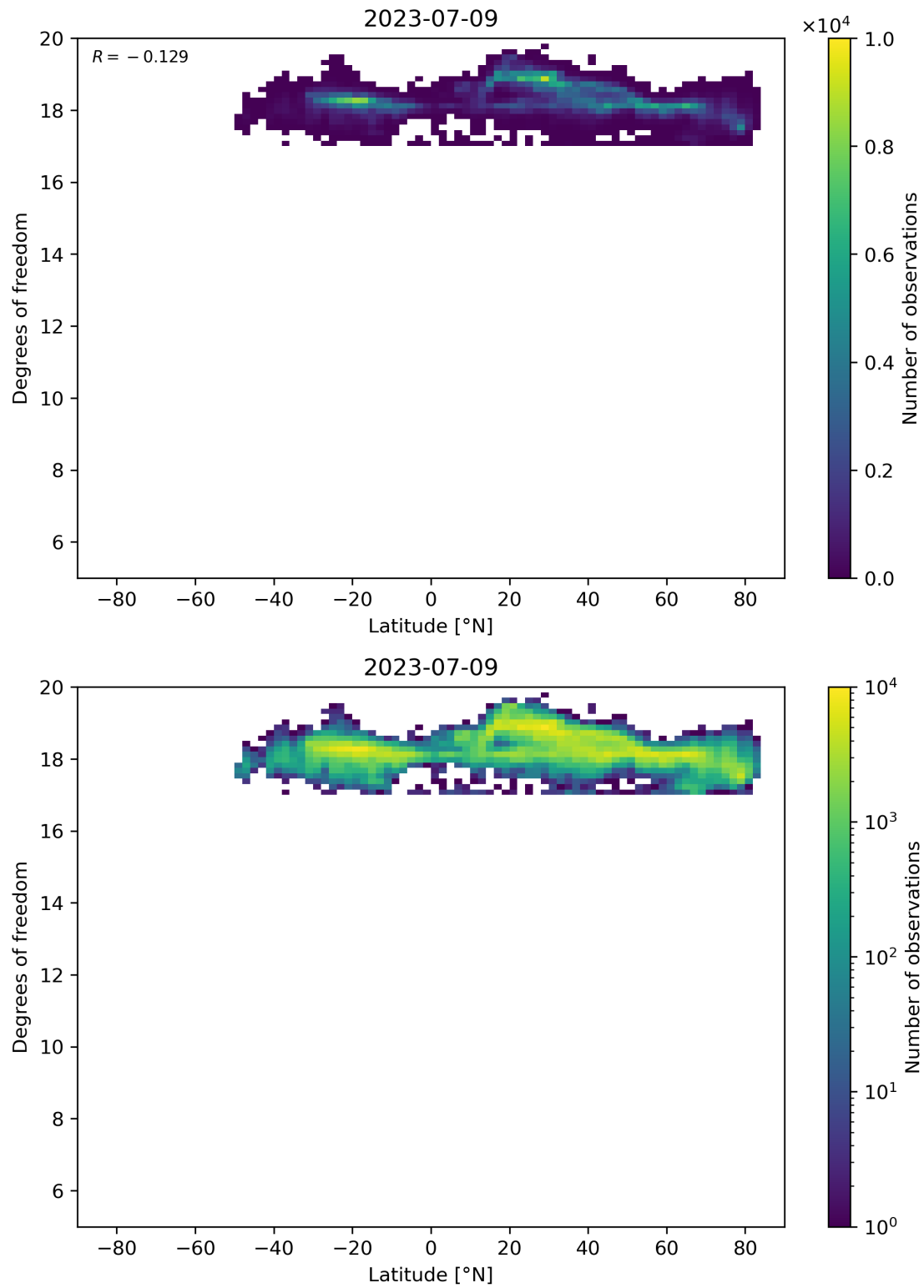
Figure 55: Scatter density plot of “Latitude” against “Degrees of freedom” for 2023-07-08 to 2023-07-10.
