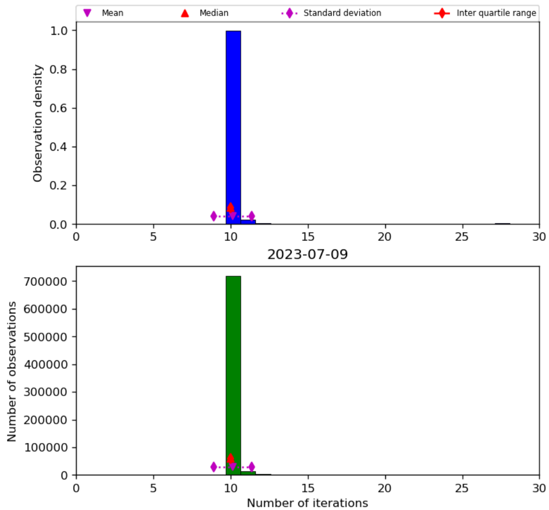
Figure 31: Histogram of “Number of iterations” for 2023-07-08 to 2023-07-10
