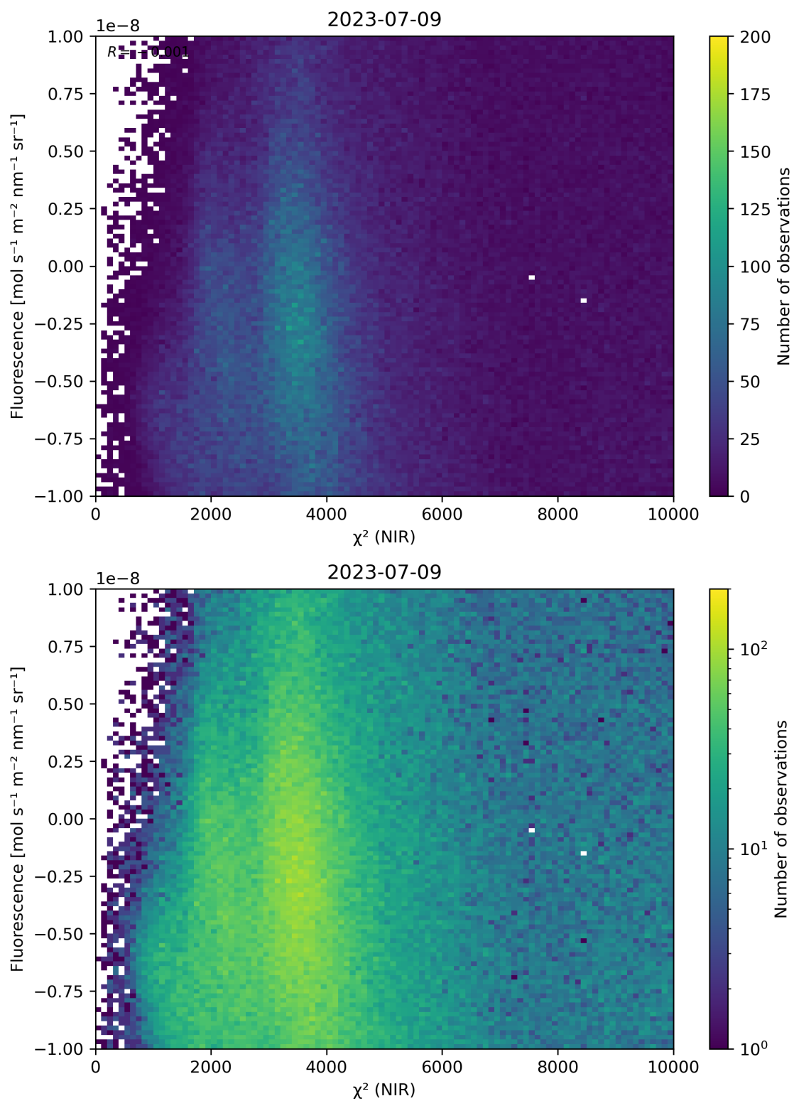
Figure 45: Scatter density plot of “ \chi^2 (NIR)” against “Fluorescence” for 2023-07-08 to 2023-07-10.
