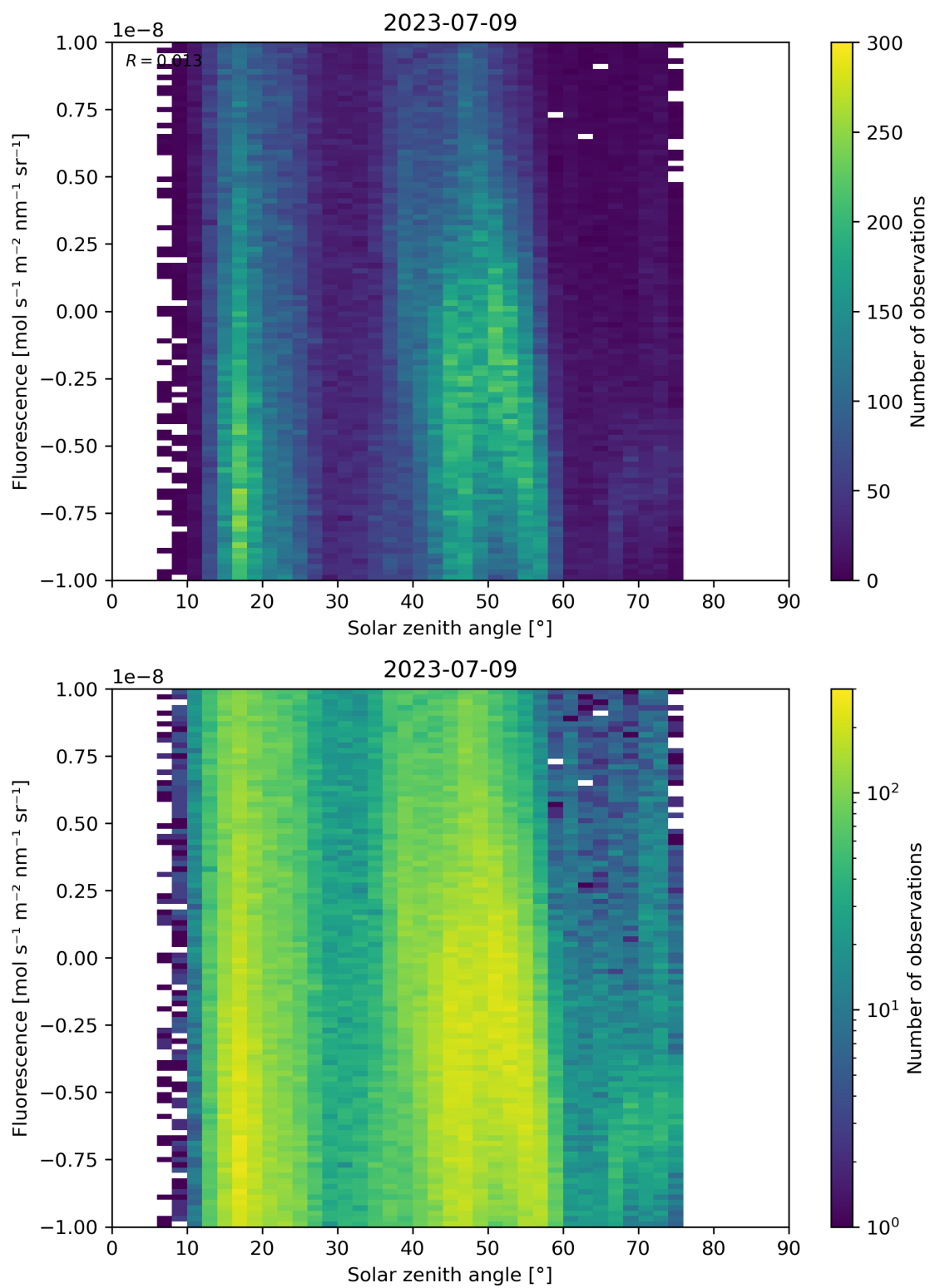
Figure 97: Scatter density plot of “Solar zenith angle” against “Fluorescence” for 2023-07-08 to 2023-07-10.
