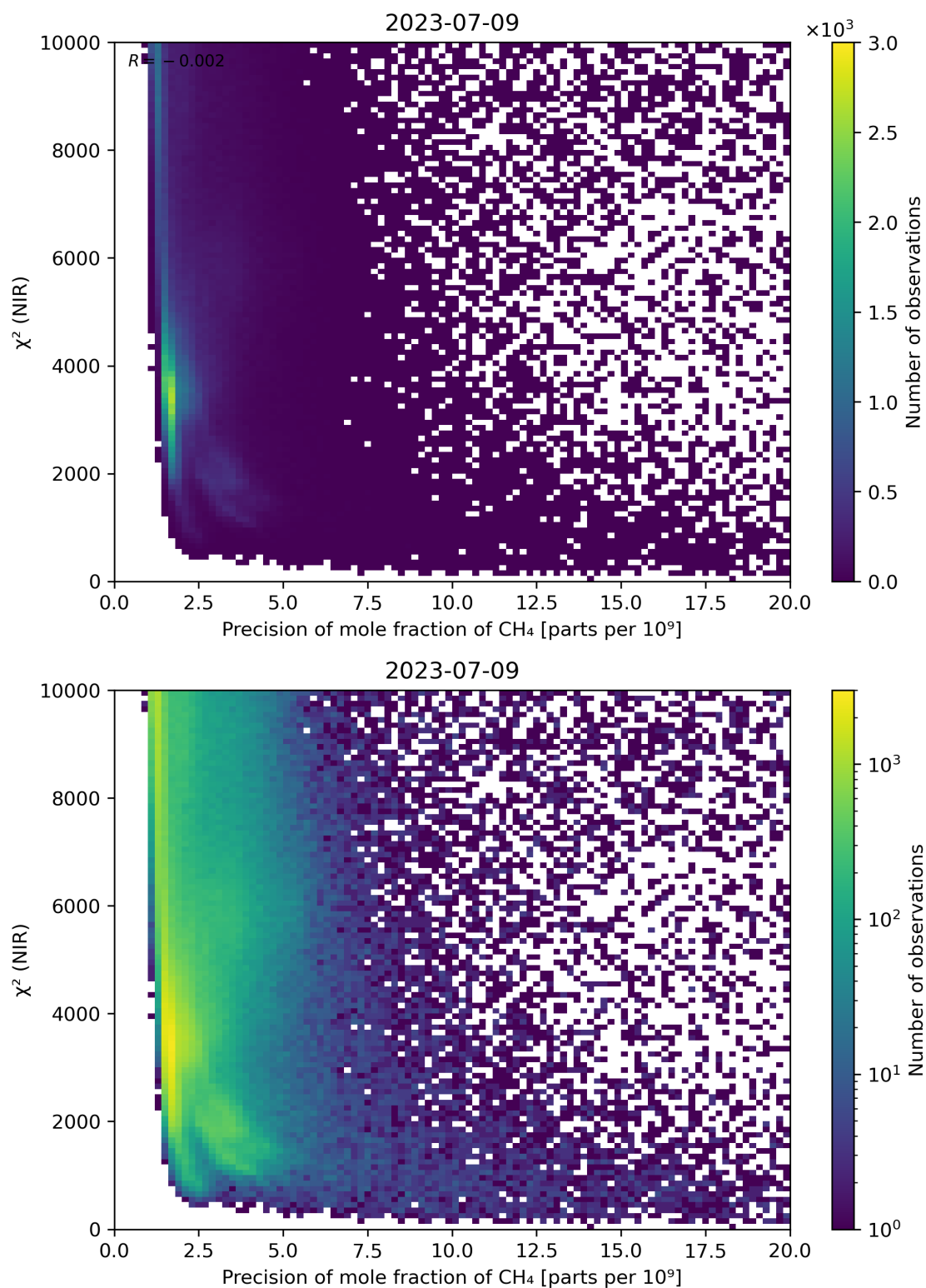
Figure 78: Scatter density plot of “Precision of mole fraction of \text{CH}_4 ” against “ \chi^2 (NIR)” for 2023-07-08 to 2023-07-10.
