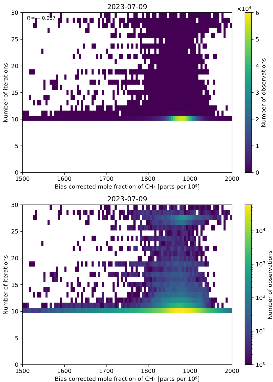
Figure 67: Scatter density plot of “Bias corrected mole fraction of CH 4 ” against “Number of iterations” for 2023-07-08 to 2023-07-10.
