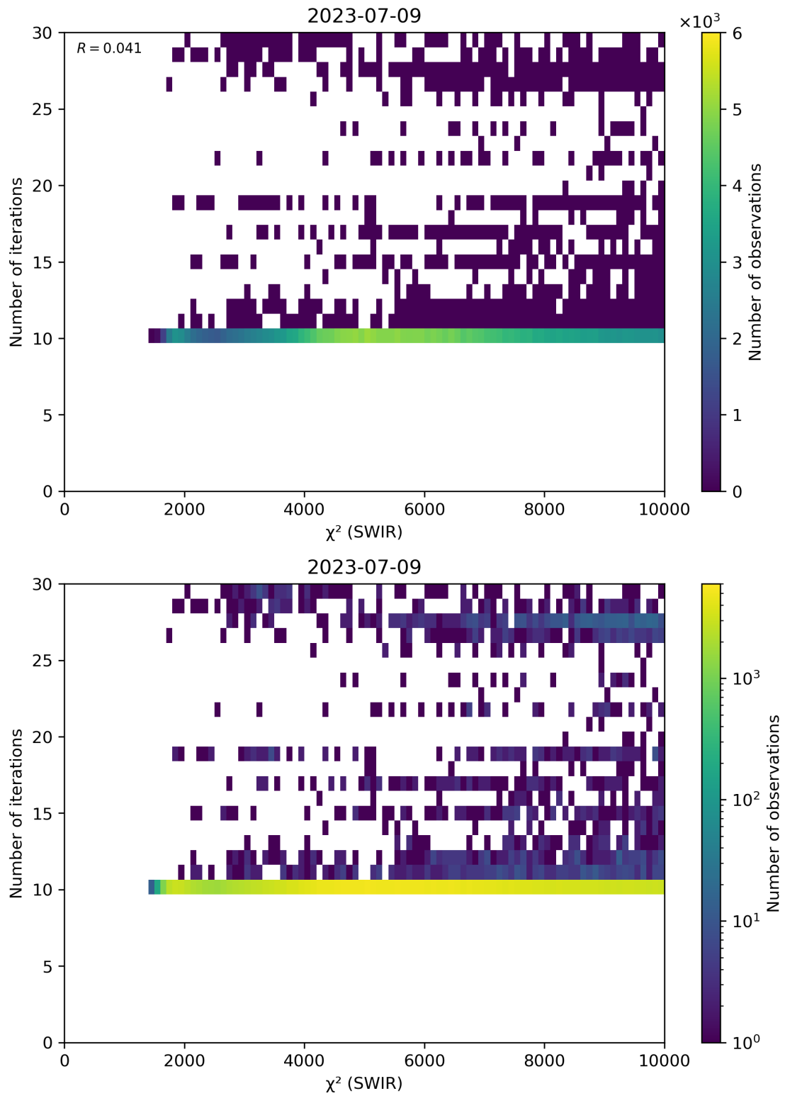
Figure 50: Scatter density plot of “ \chi^2 (SWIR)” against “Number of iterations” for 2023-07-08 to 2023-07-10.
