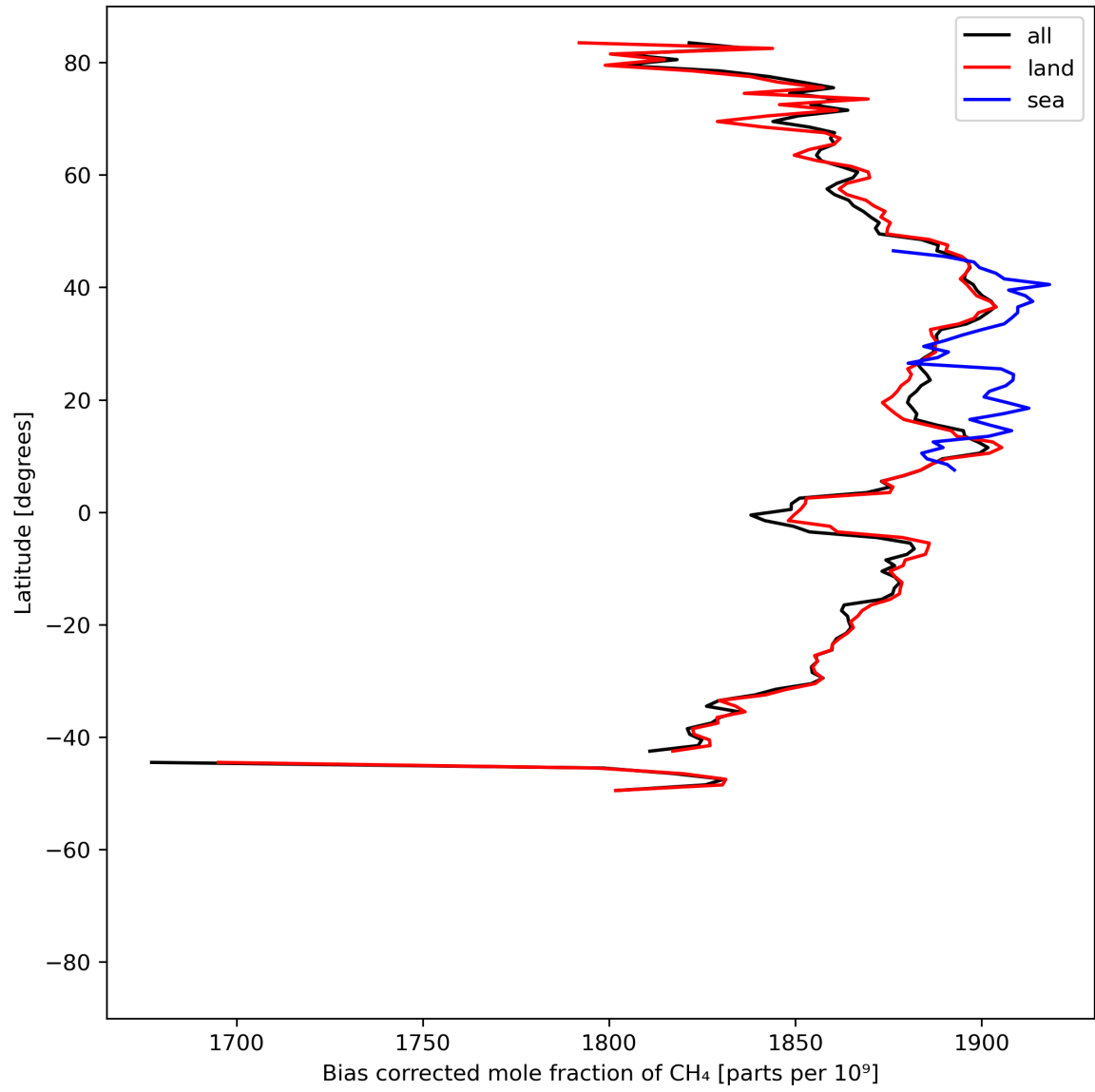
Figure 14: Zonal average of “Bias corrected mole fraction of CH 4 ” for 2023-07-08 to 2023-07-10.
