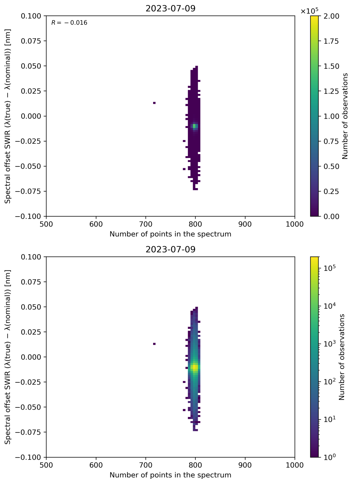
Figure 93: Scatter density plot of “Number of points in the spectrum” against “Spectral offset SWIR ( \lambda(\text{true}) - \lambda(\text{nominal}) )” for 2023-07-08 to 2023-07-10.
