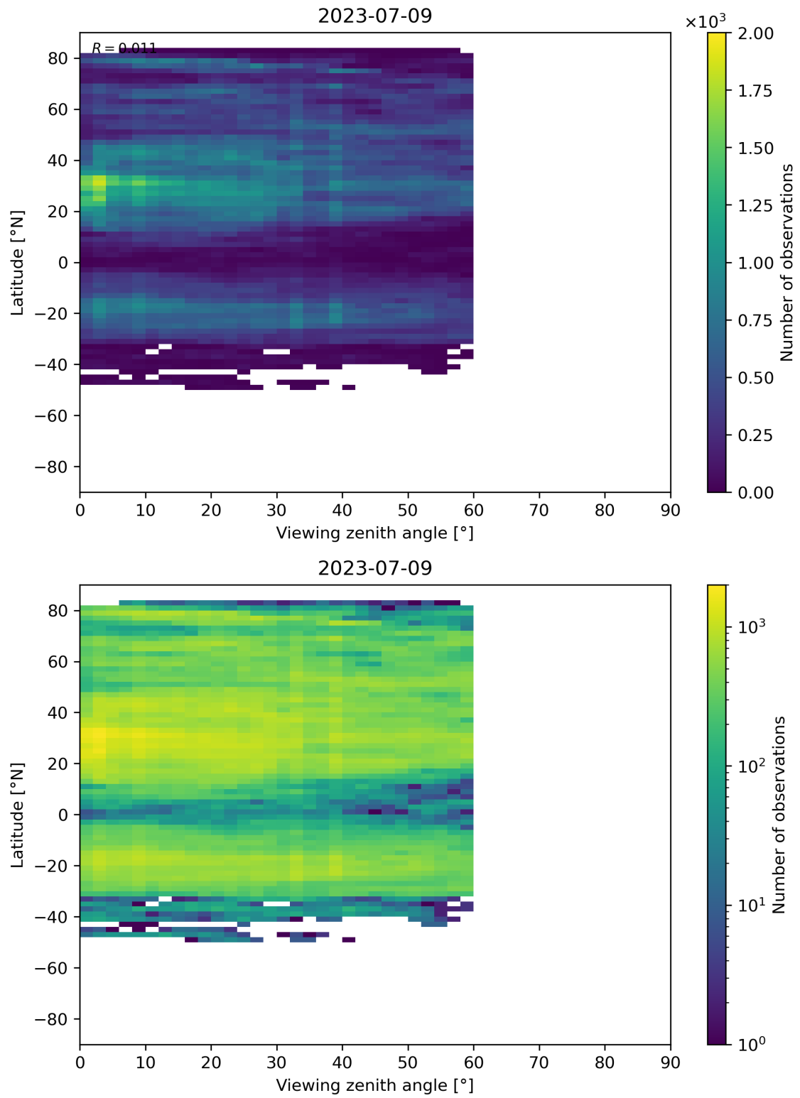
Figure 109: Scatter density plot of “Viewing zenith angle” against “Latitude” for 2023-07-08 to 2023-07-10.
