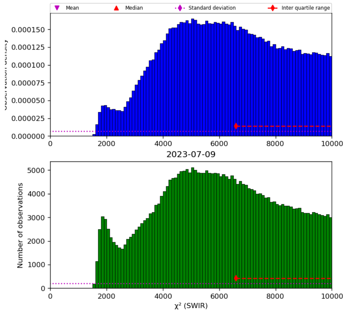
Figure 28: Histogram of “ \chi^2 (SWIR)” for 2023-07-08 to 2023-07-10
