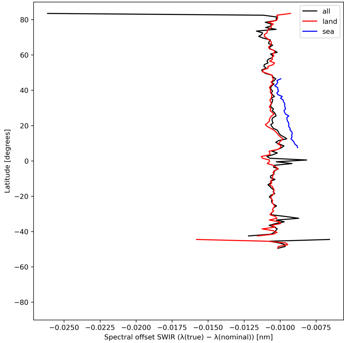
Figure 16: Zonal average of “Spectral offset SWIR ( \lambda(\text{true}) - \lambda(\text{nominal}) )” for 2023-07-08 to 2023-07-10.
