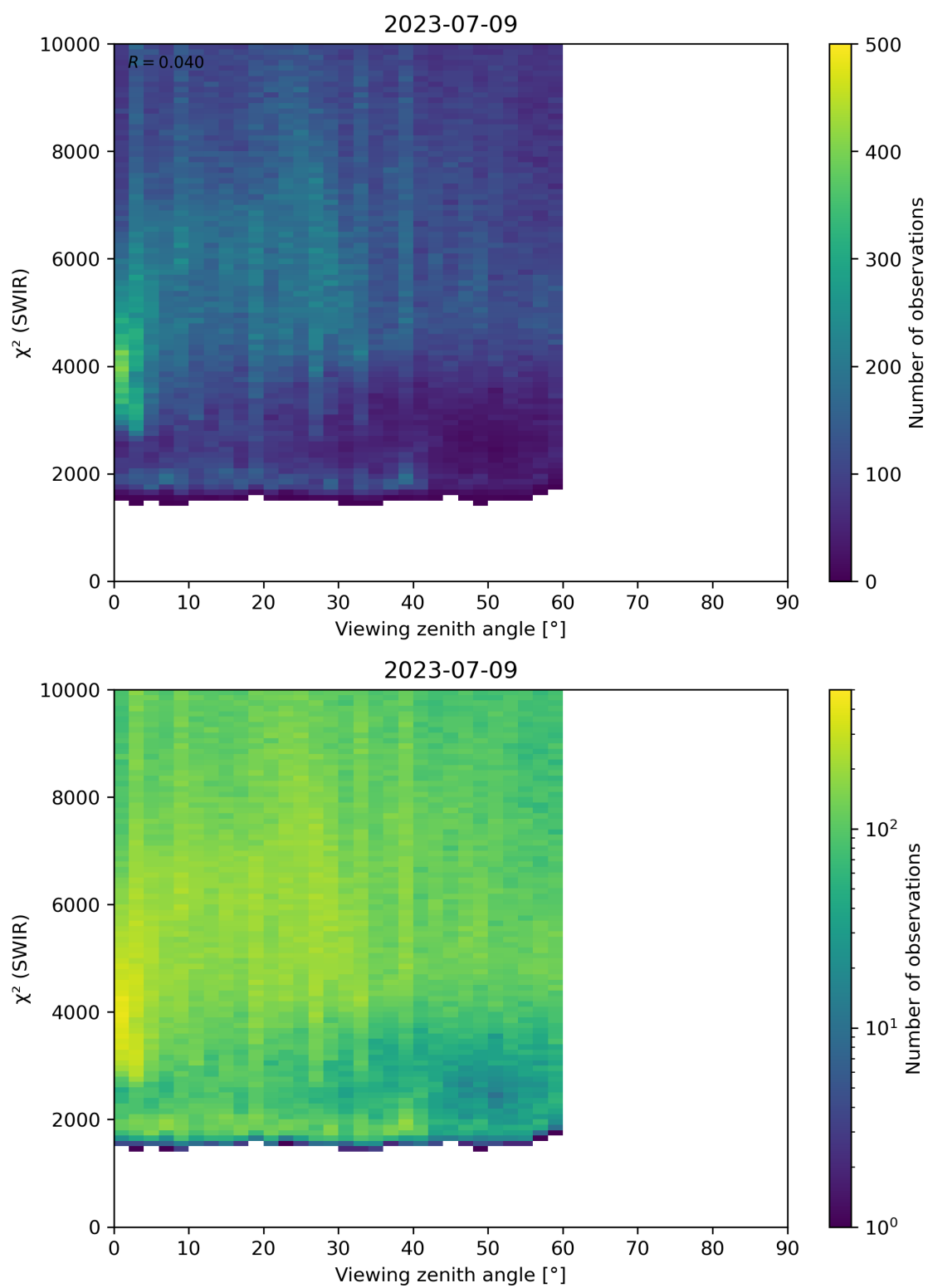
Figure 106: Scatter density plot of “Viewing zenith angle” against “ \chi^2 (SWIR)” for 2023-07-08 to 2023-07-10.
