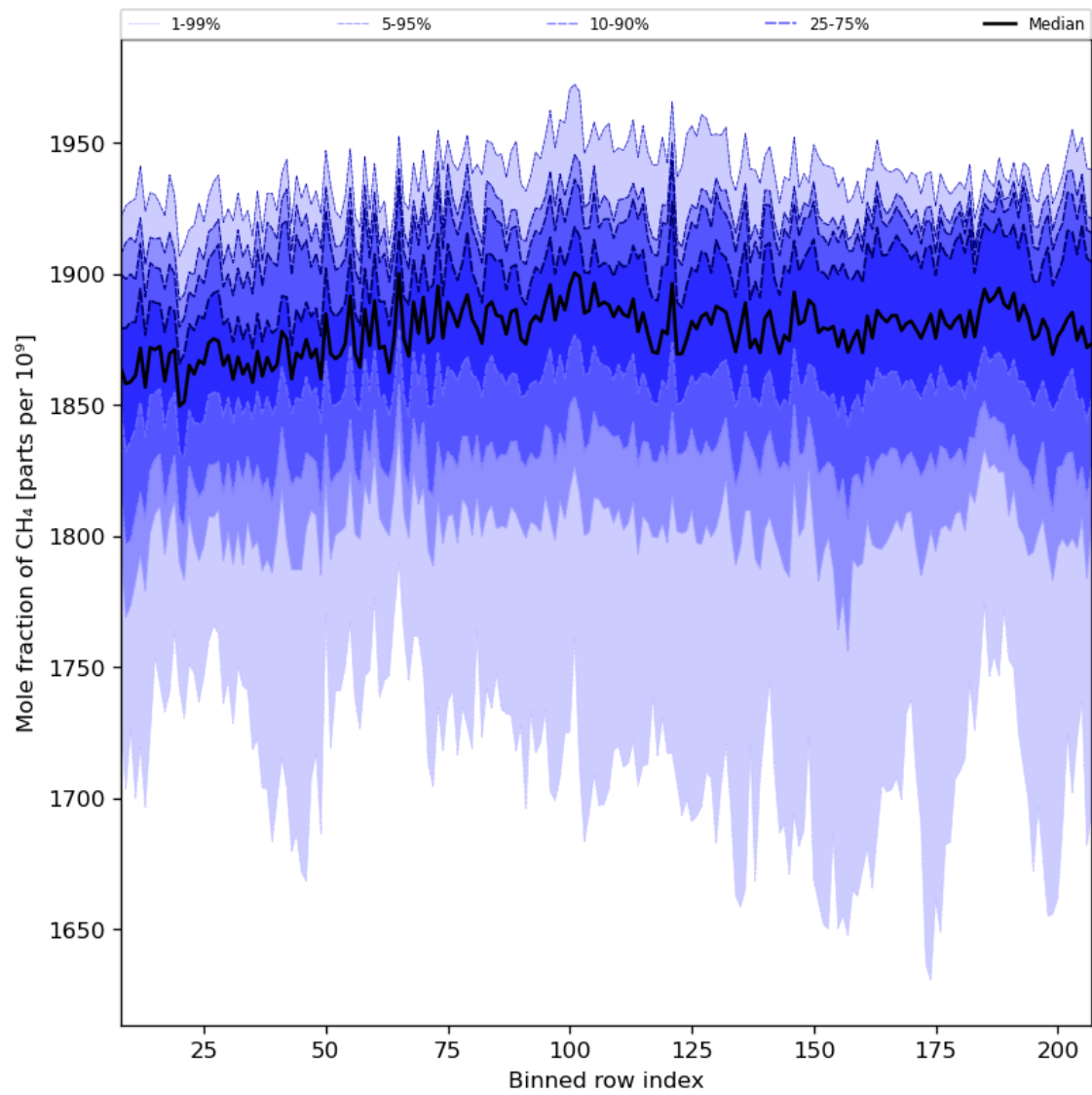
Figure 34: Along track statistics of “Mole fraction of CH 4 ” for 2023-07-08 to 2023-07-10
