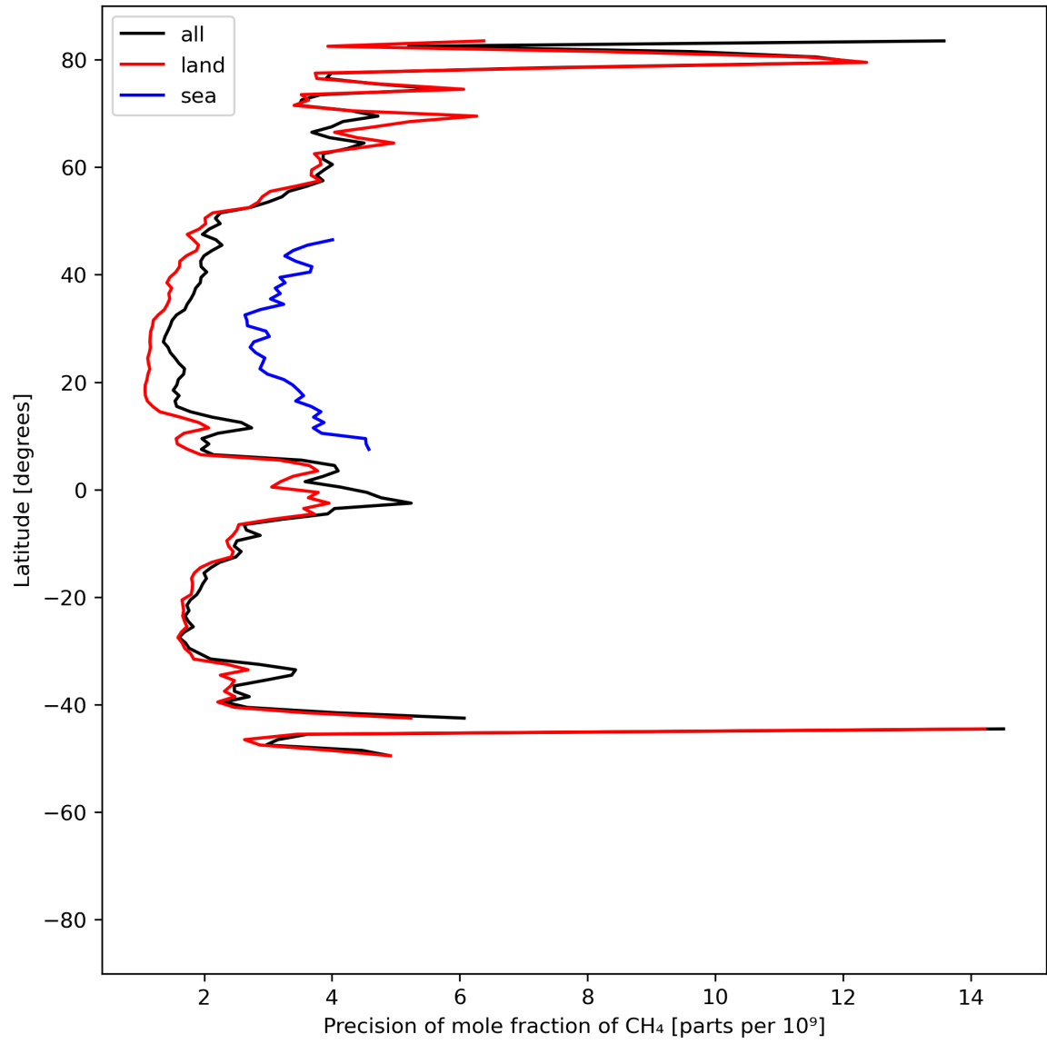
Figure 13: Zonal average of “Precision of mole fraction of CH 4 ” for 2023-07-08 to 2023-07-10.
