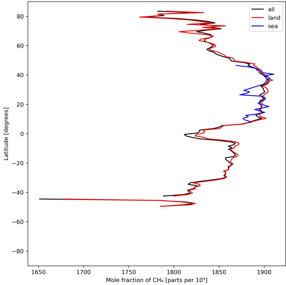
Figure 12: Zonal average of “Mole fraction of \text{CH}_4 ” for 2023-07-08 to 2023-07-10.
