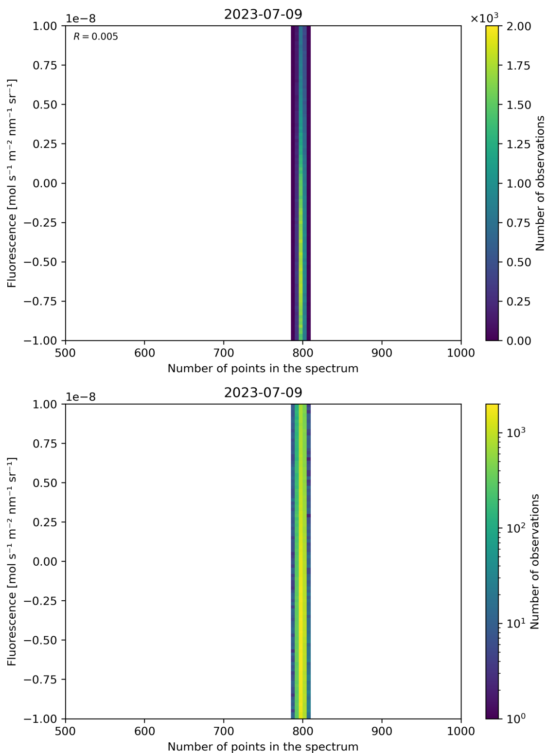
Figure 91: Scatter density plot of “Number of points in the spectrum” against “Fluorescence” for 2023-07-08 to 2023-07-10.
