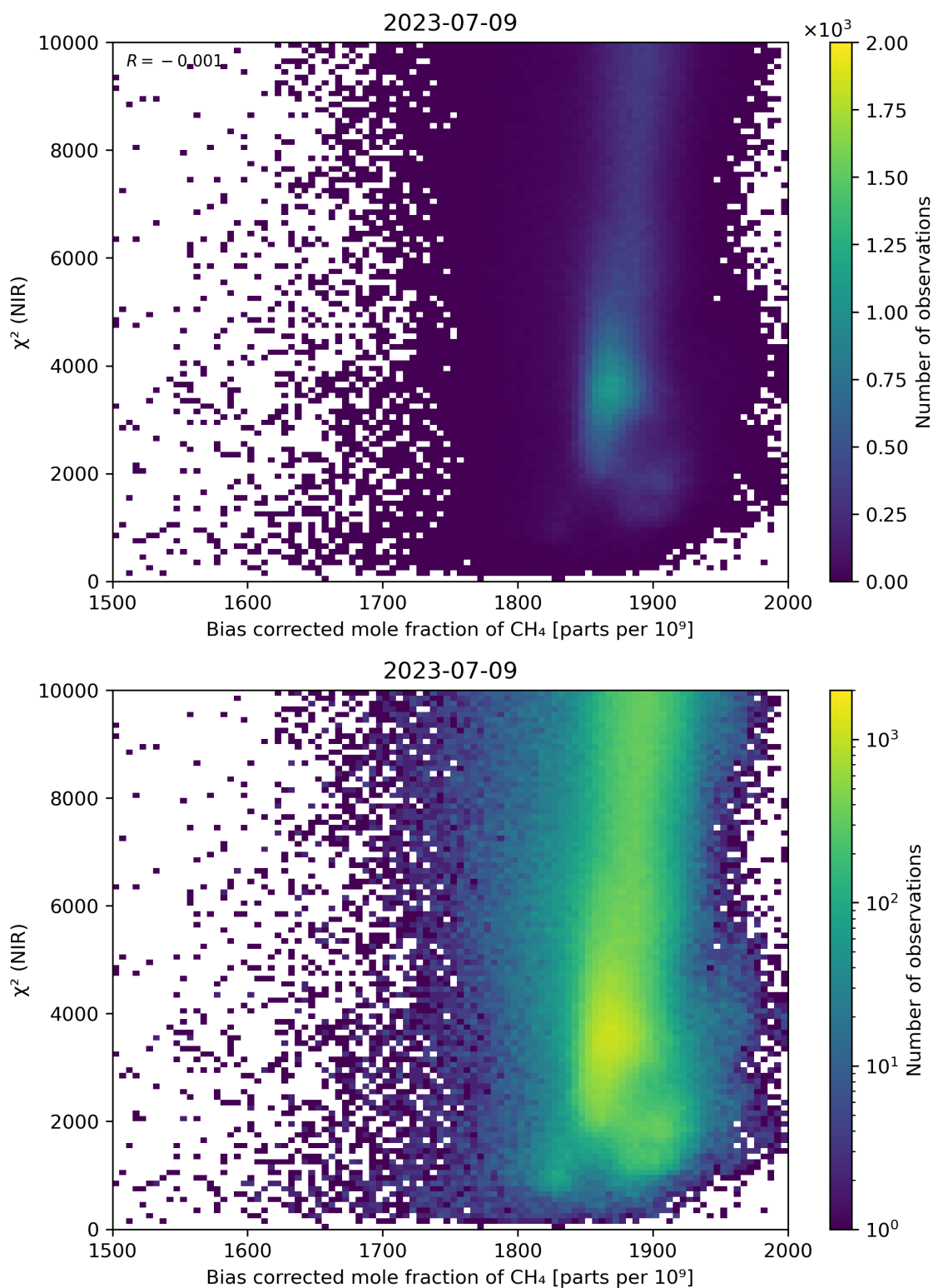
Figure 63: Scatter density plot of “Bias corrected mole fraction of CH 4 ” against “ \chi^2 (NIR)” for 2023-07-08 to 2023-07-10.
