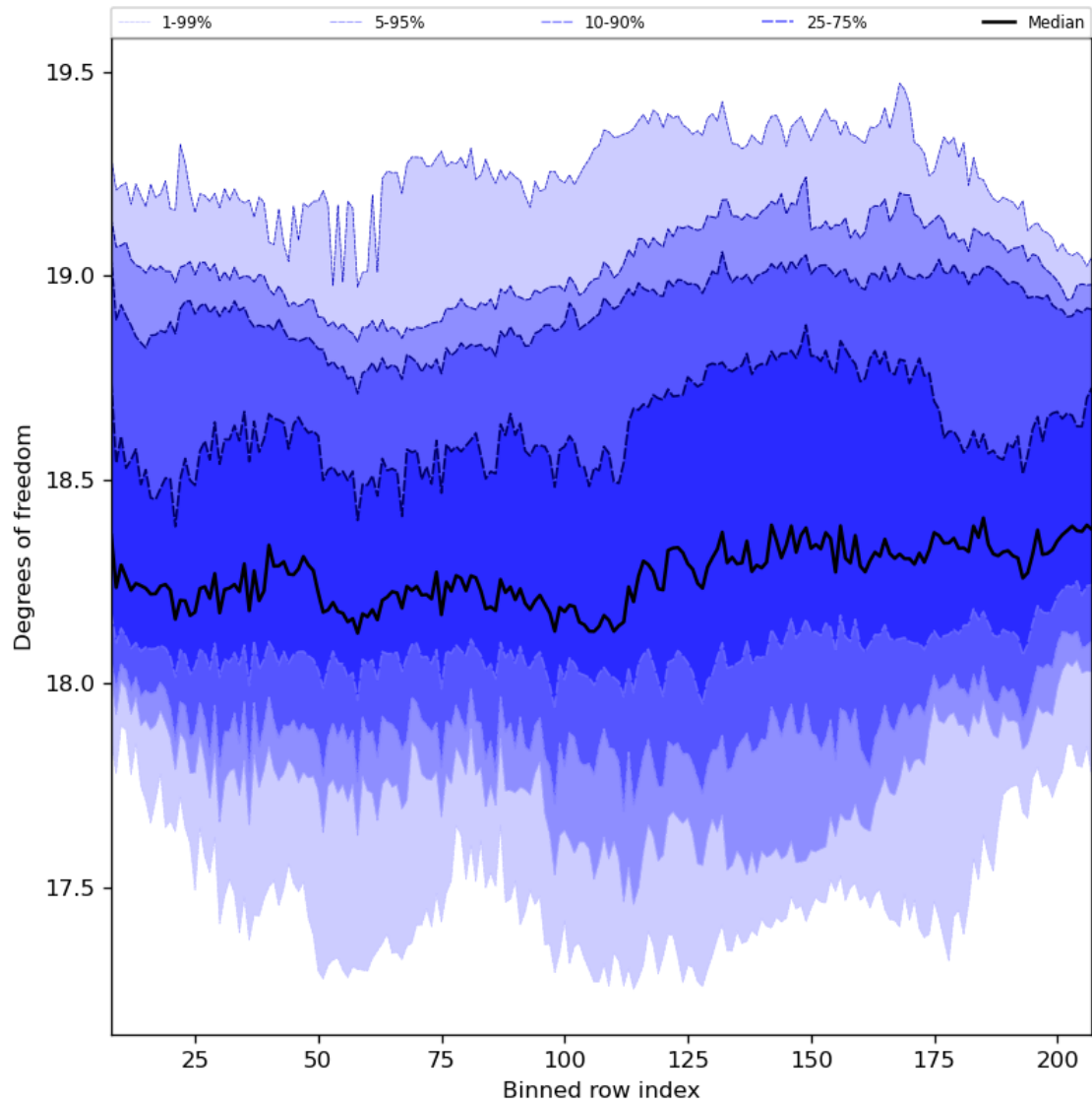
Figure 41: Along track statistics of “Degrees of freedom” for 2023-07-09 to 2023-07-11
