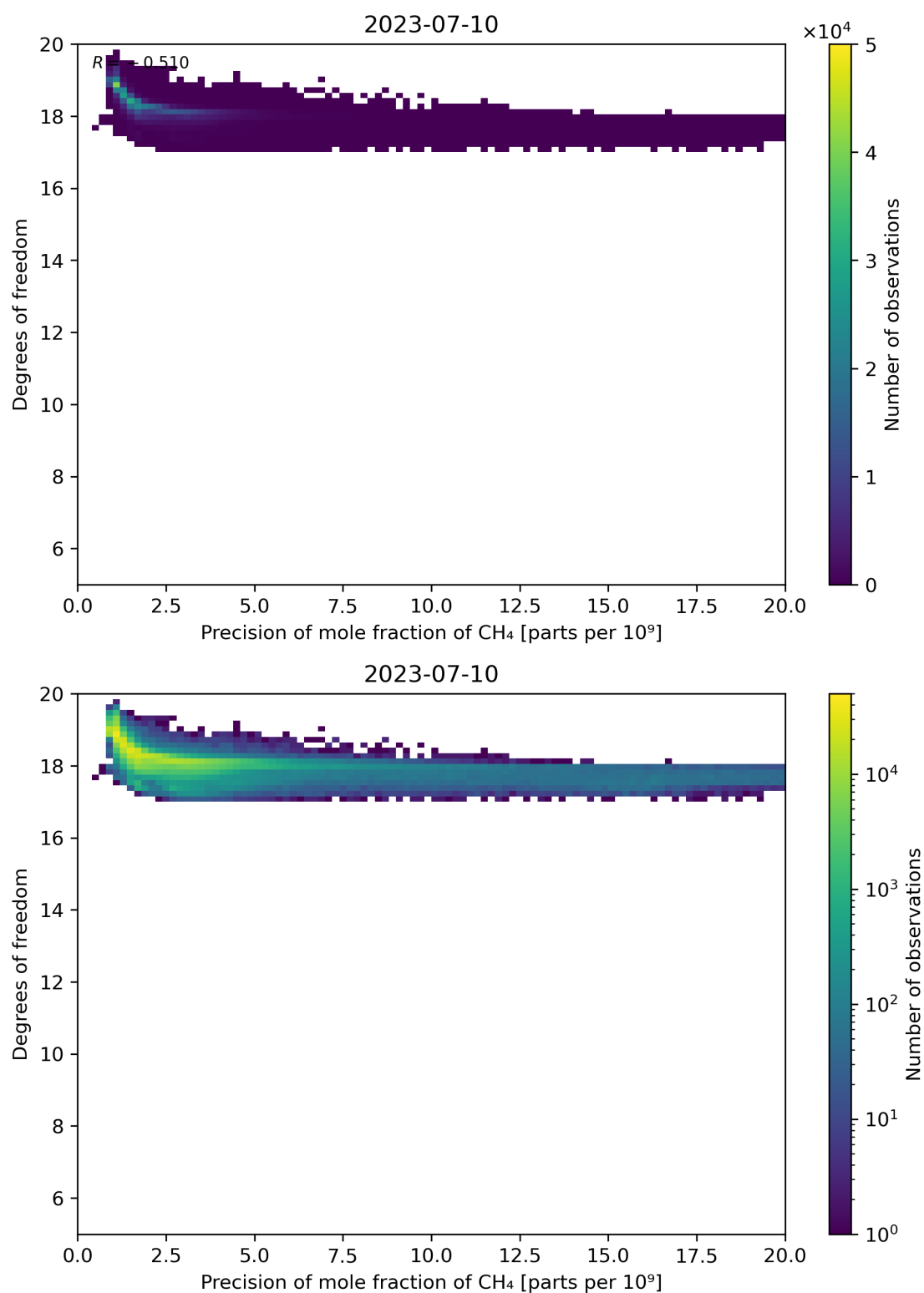
Figure 80: Scatter density plot of “Precision of mole fraction of CH 4 ” against “Degrees of freedom” for 2023-07-09 to 2023-07-11.
