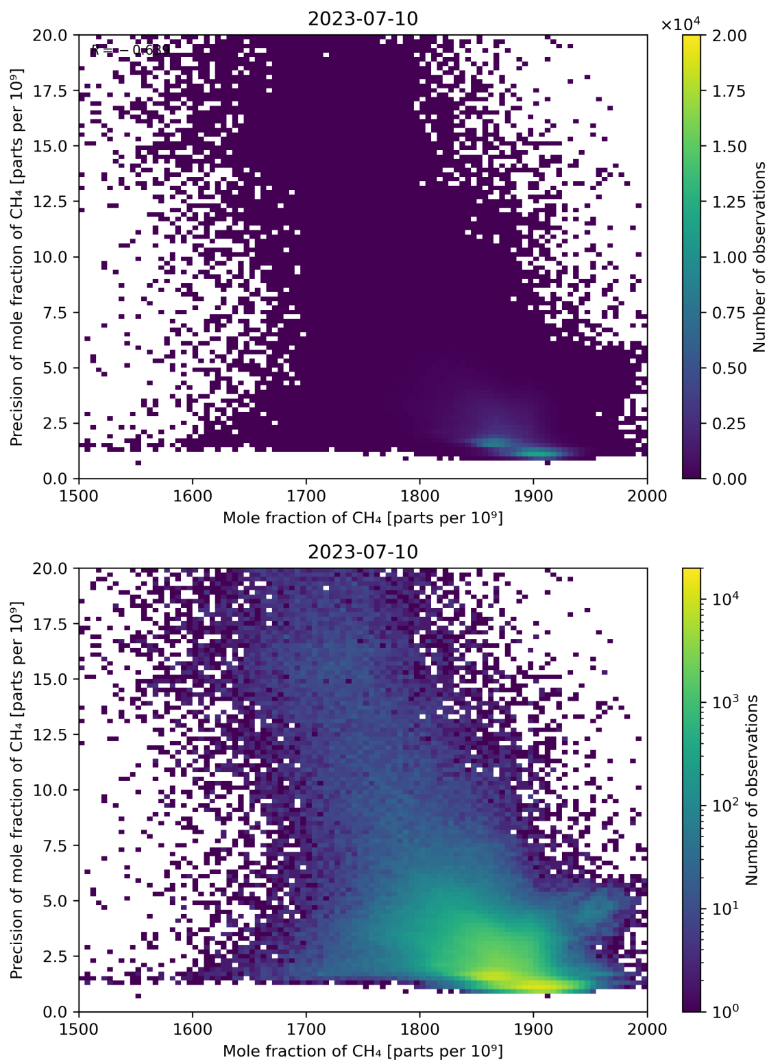
Figure 75: Scatter density plot of “Mole fraction of CH 4 ” against “Precision of mole fraction of CH 4 ” for 2023-07-09 to 2023-07-11.
