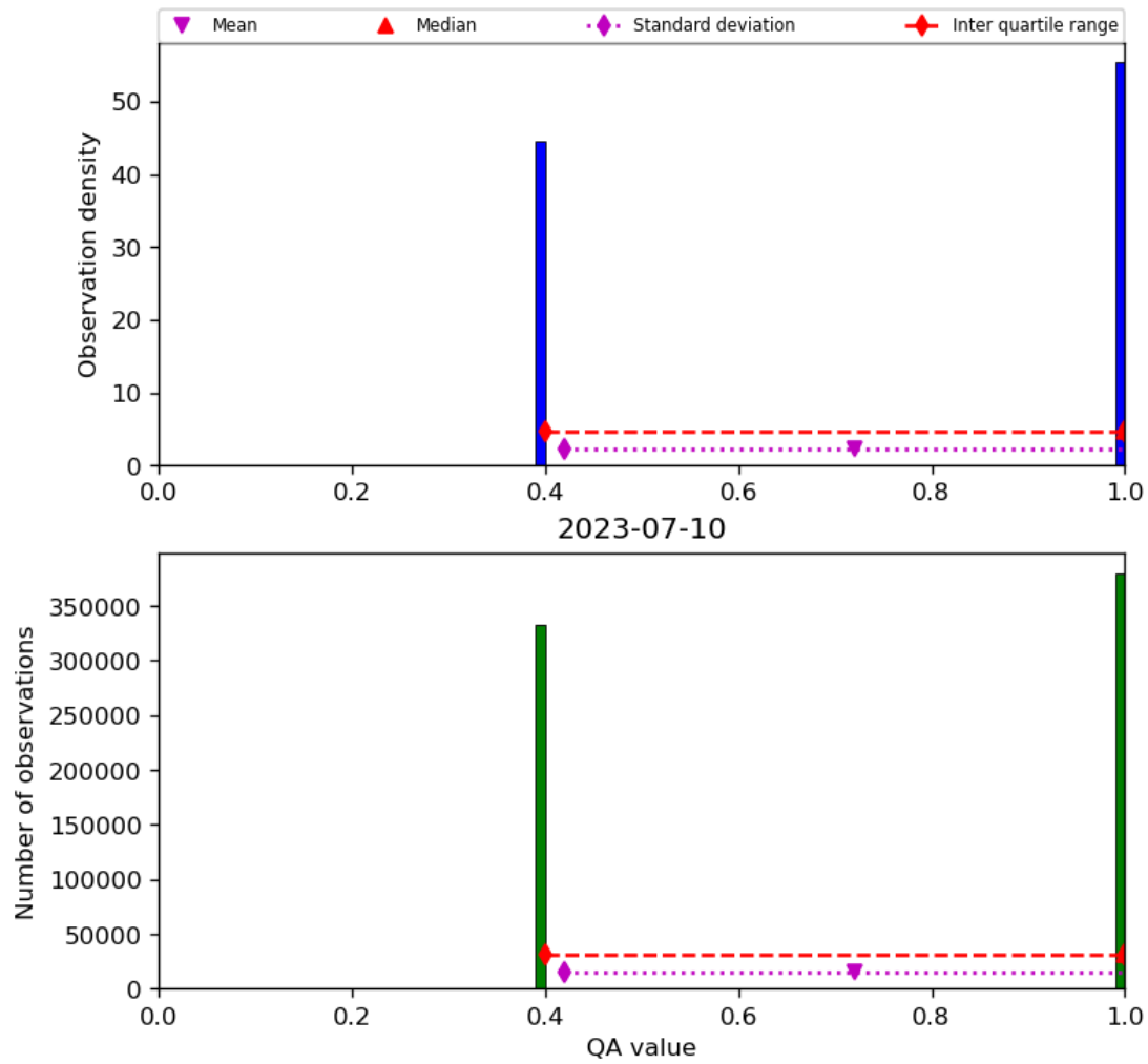
Figure 22: Histogram of “QA value” for 2023-07-09 to 2023-07-11
