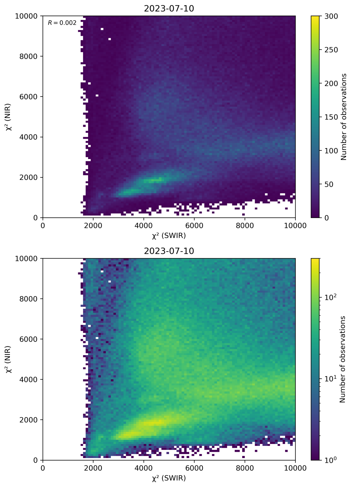
Figure 47: Scatter density plot of “ \chi^2 (SWIR)” against “ \chi^2 (NIR)” for 2023-07-09 to 2023-07-11.
