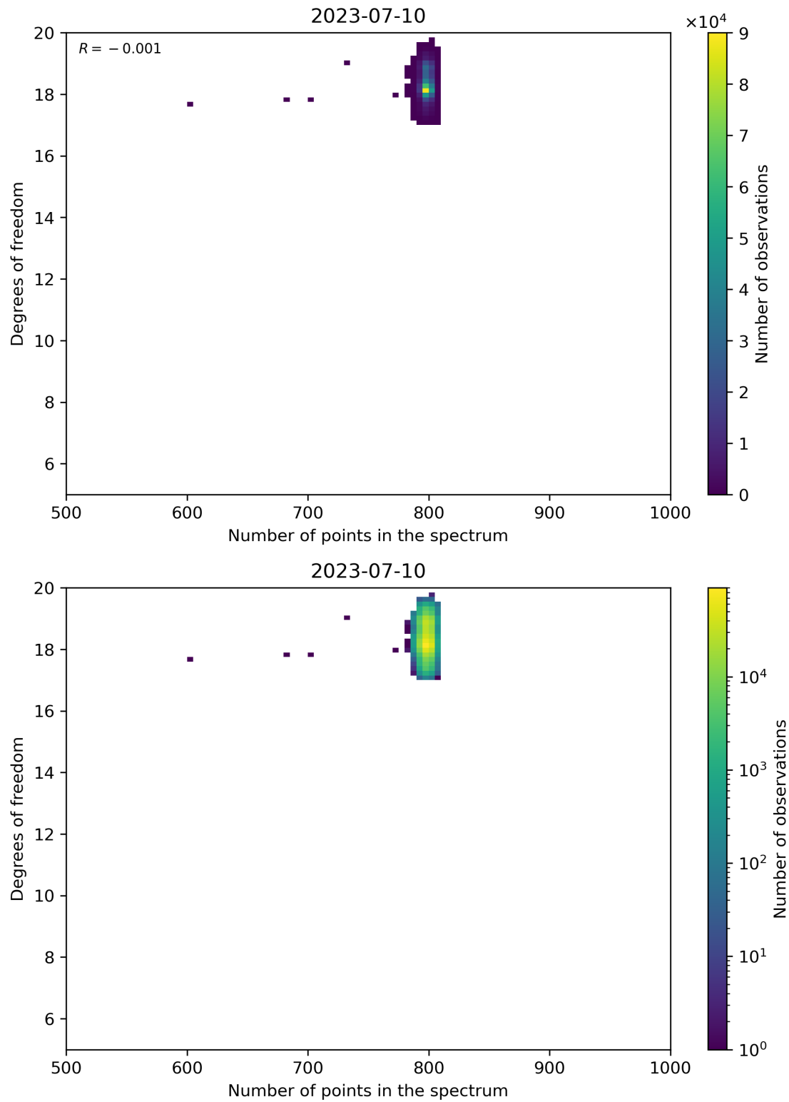
Figure 90: Scatter density plot of “Number of points in the spectrum” against “Degrees of freedom” for 2023-07-09 to 2023-07-11.
