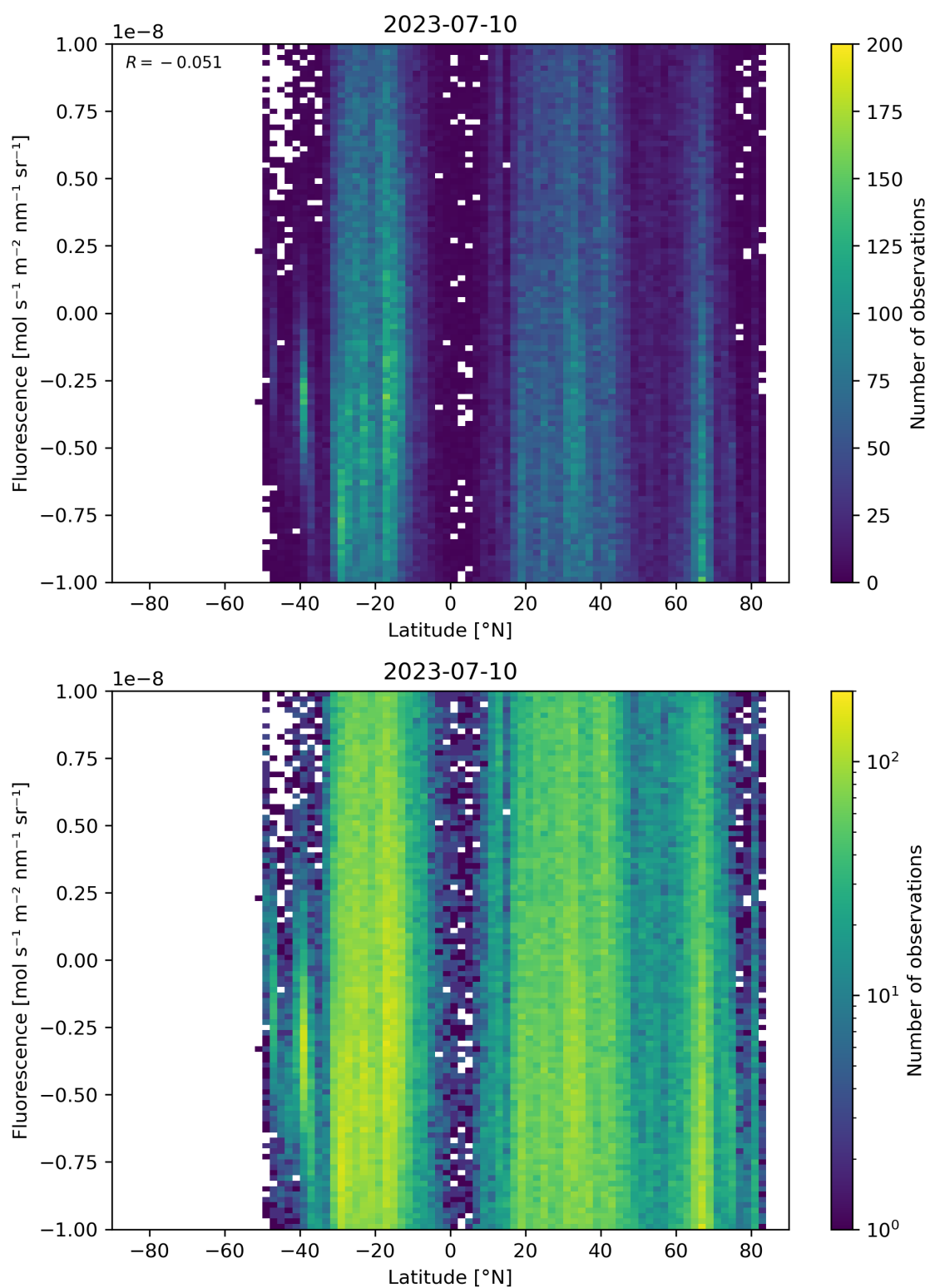
Figure 56: Scatter density plot of “Latitude” against “Fluorescence” for 2023-07-09 to 2023-07-11.
