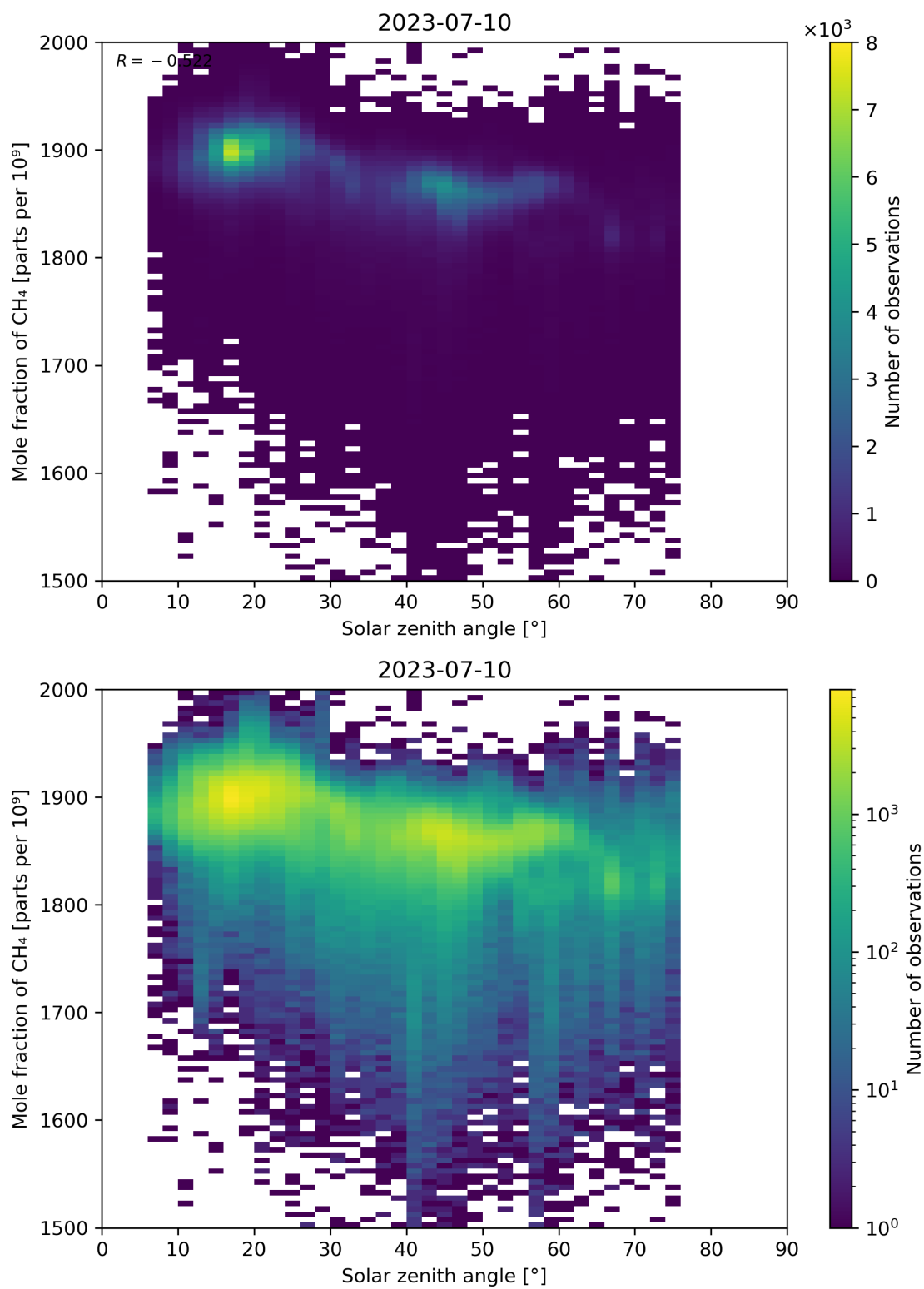
Figure 99: Scatter density plot of “Solar zenith angle” against “Mole fraction of CH 4 ” for 2023-07-09 to 2023-07-11.
