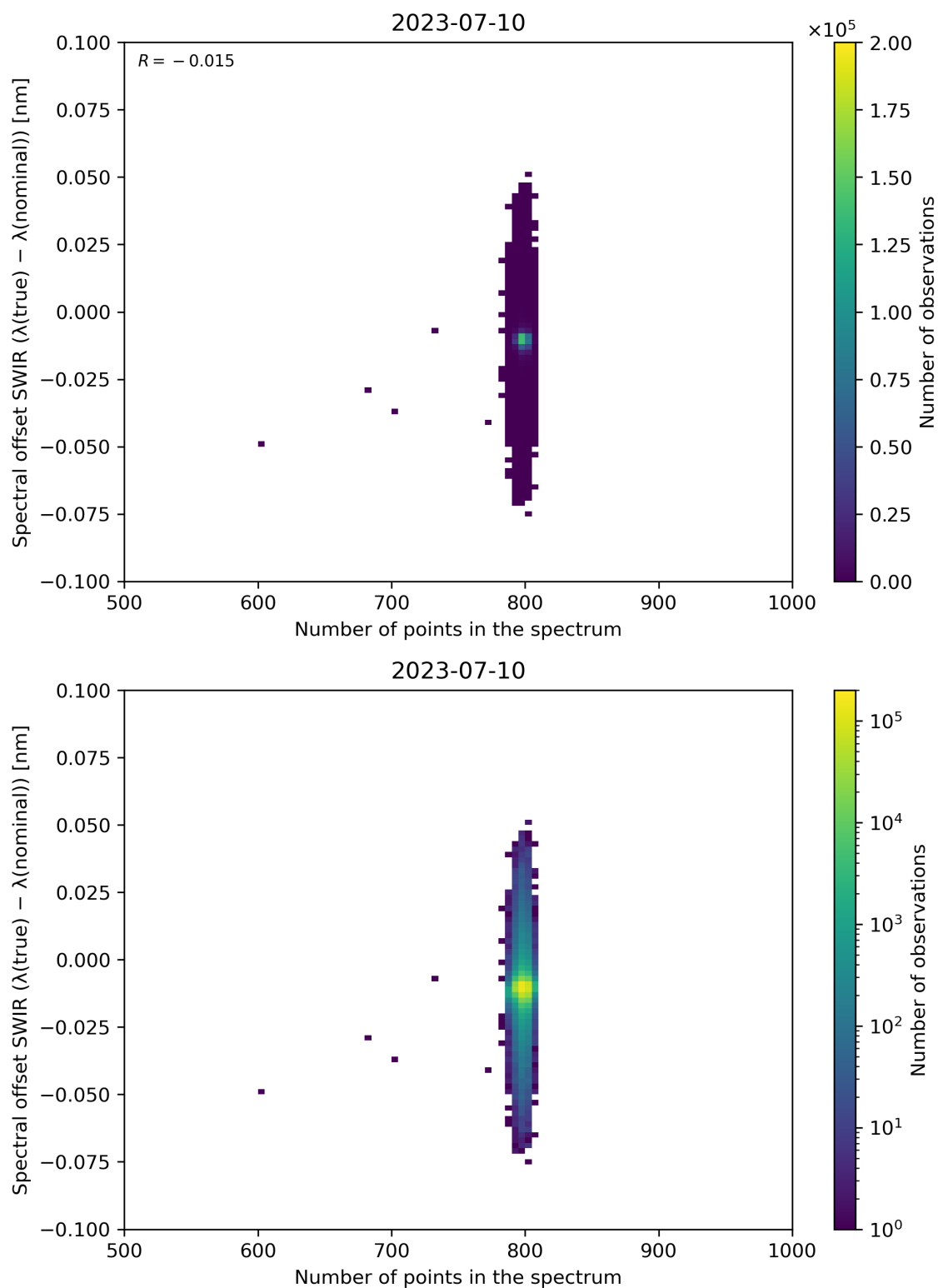
Figure 93: Scatter density plot of “Number of points in the spectrum” against “Spectral offset SWIR ( \lambda(\text{true}) - \lambda(\text{nominal}) )” for 2023-07-09 to 2023-07-11.
