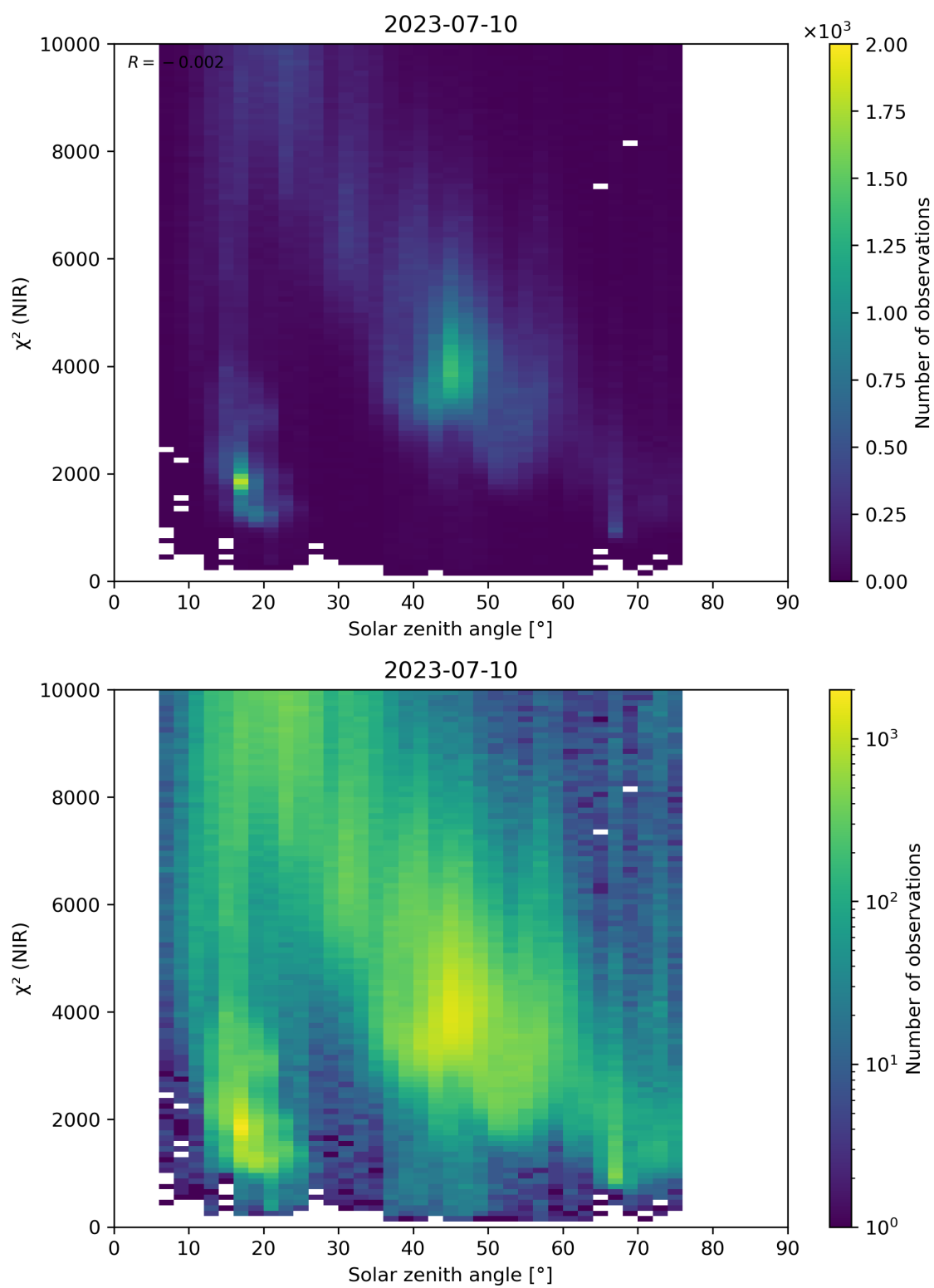
Figure 94: Scatter density plot of “Solar zenith angle” against “ \chi^2 (NIR)” for 2023-07-09 to 2023-07-11.
