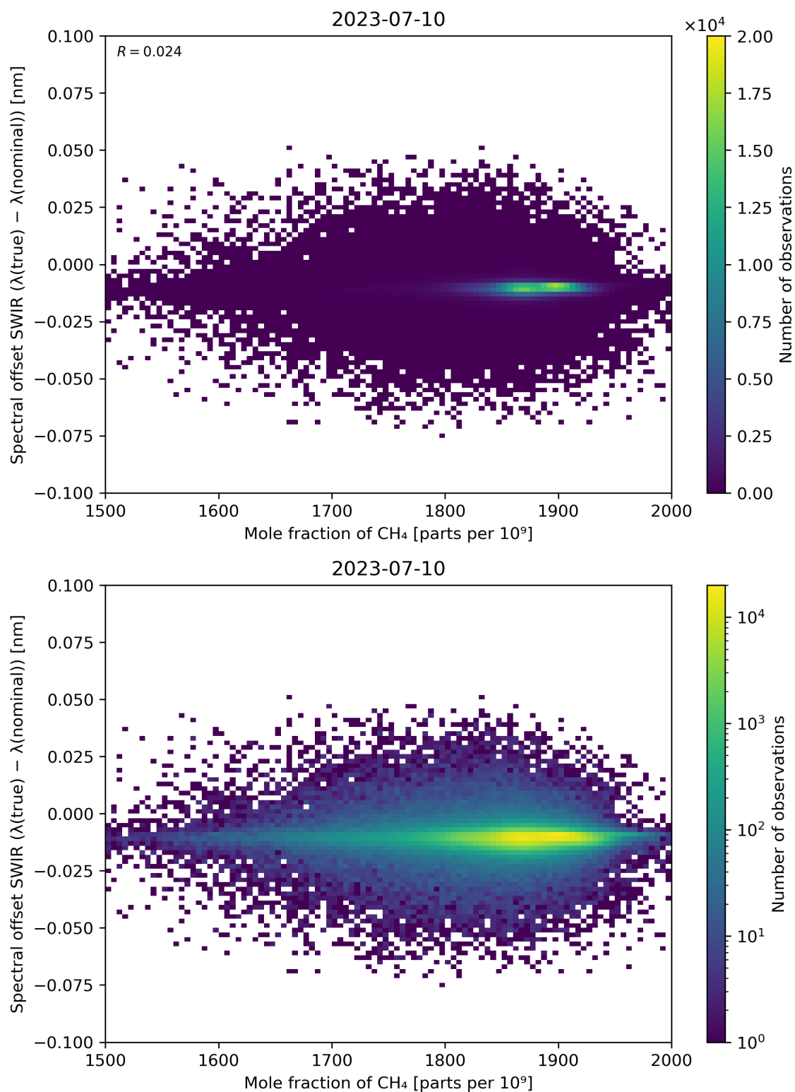
Figure 86: Scatter density plot of “Mole fraction of CH 4 ” against “Spectral offset SWIR ( \lambda(\text{true}) - \lambda(\text{nominal}) )” for 2023-07-09 to 2023-07-11.
