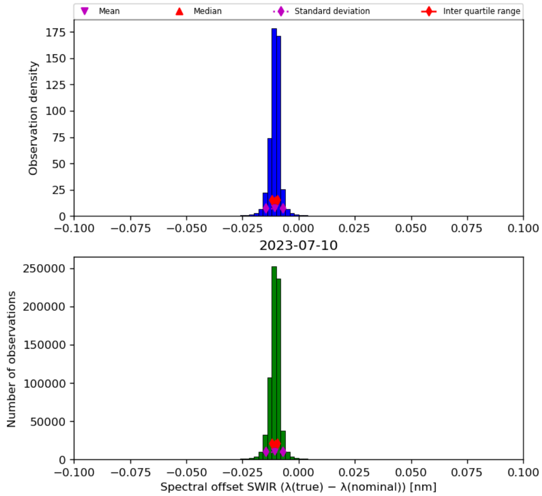
Figure 27: Histogram of “Spectral offset SWIR ( \lambda(\text{true}) - \lambda(\text{nominal}) )” for 2023-07-09 to 2023-07-11
