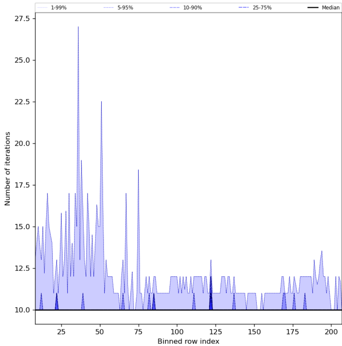
Figure 42: Along track statistics of “Number of iterations” for 2023-07-09 to 2023-07-11
