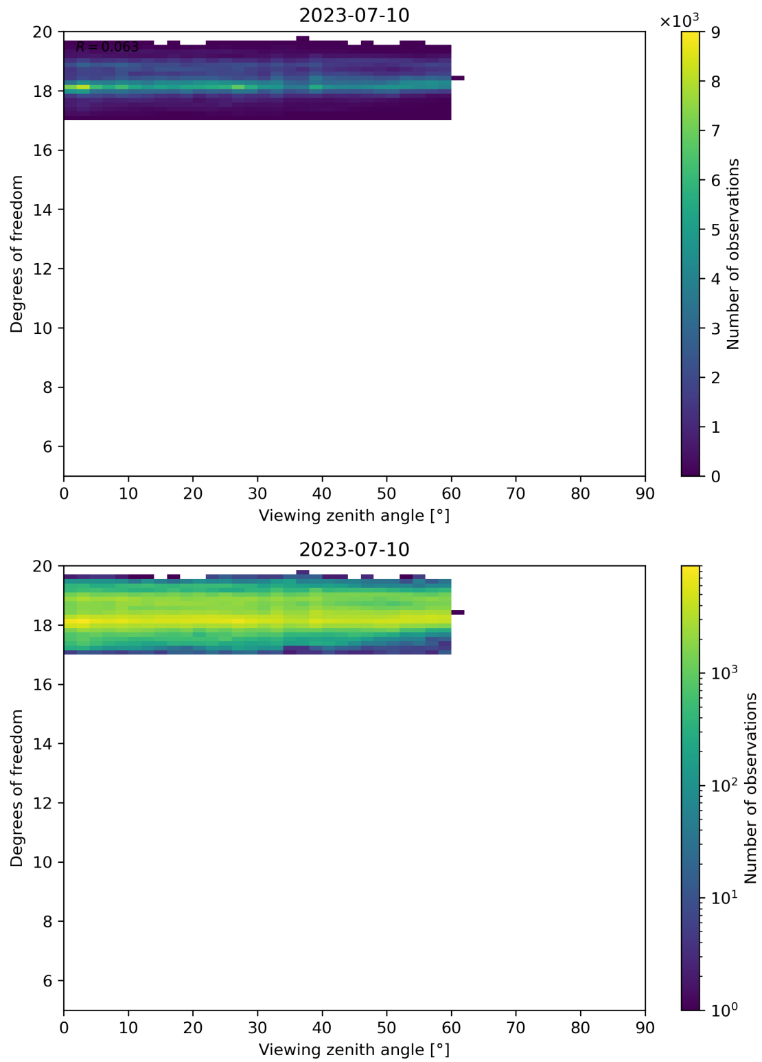
Figure 107: Scatter density plot of “Viewing zenith angle” against “Degrees of freedom” for 2023-07-09 to 2023-07-11.
