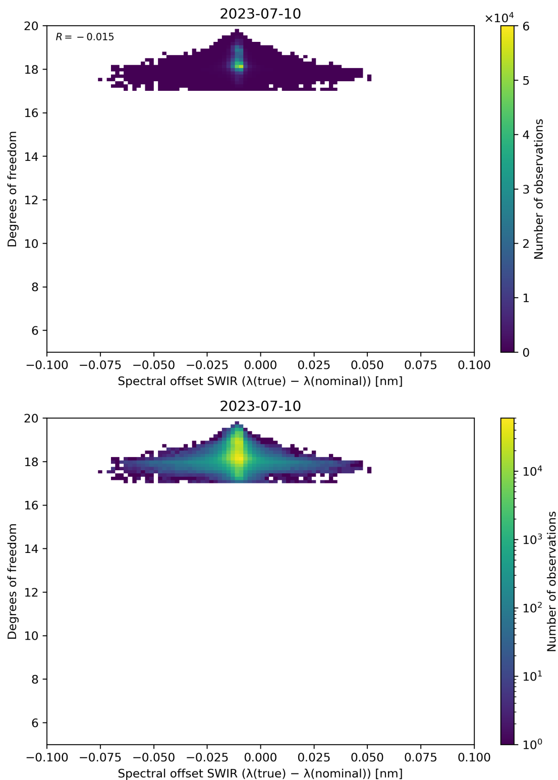
Figure 119: Scatter density plot of “Spectral offset SWIR ( \lambda(\text{true}) - \lambda(\text{nominal}) )” against “Degrees of freedom” for 2023-07-09 to 2023-07-11.
