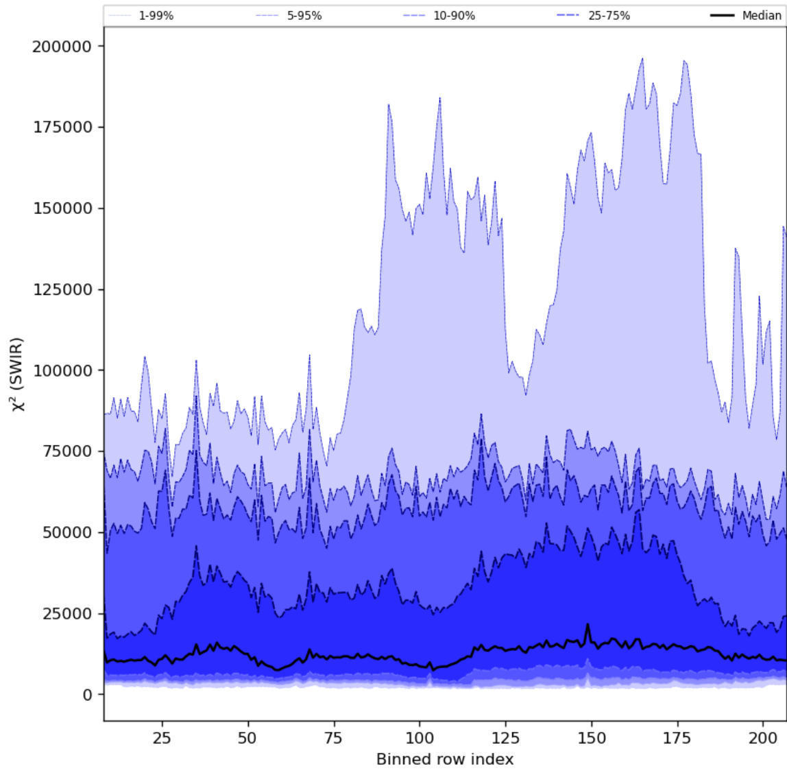
Figure 39: Along track statistics of “ \chi^2 (SWIR)” for 2023-07-09 to 2023-07-11
