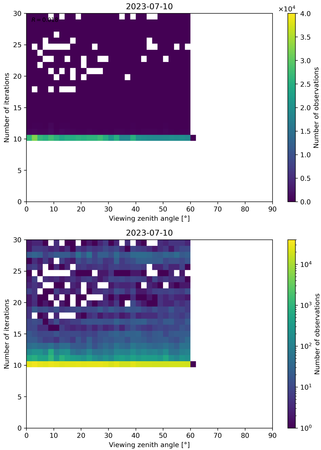
Figure 113: Scatter density plot of “Viewing zenith angle” against “Number of iterations” for 2023-07-09 to 2023-07-11.
