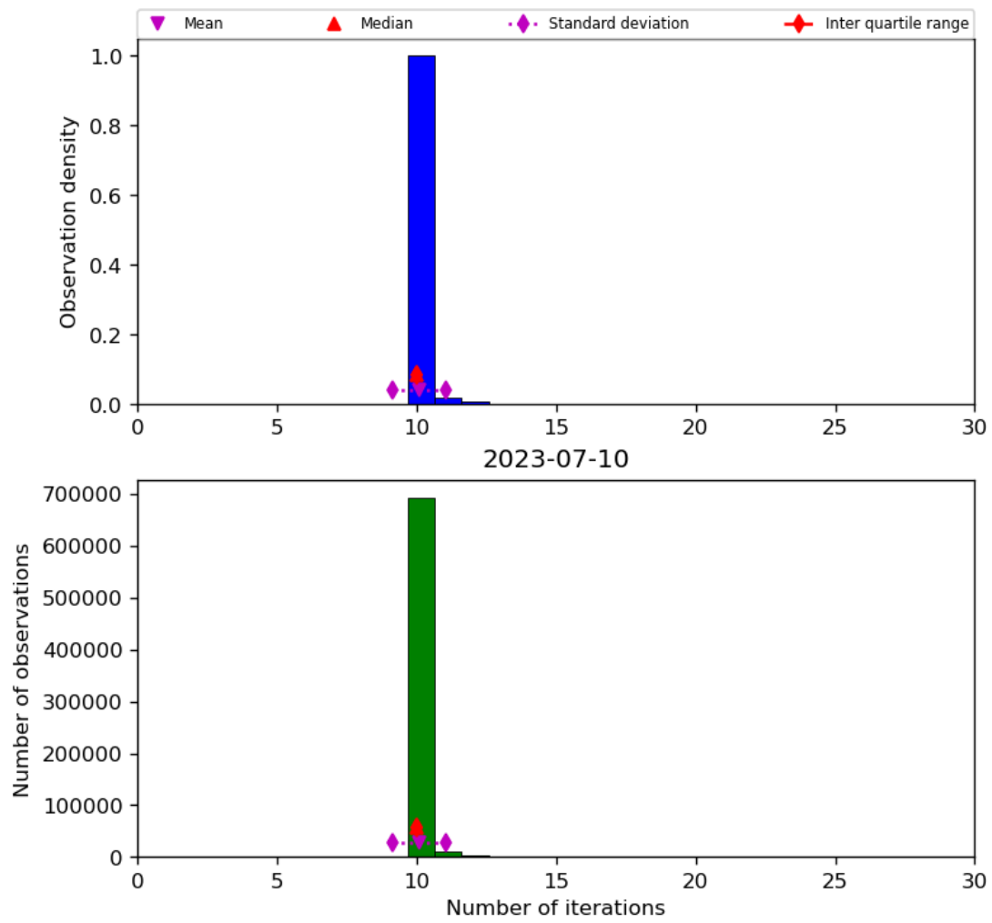
Figure 31: Histogram of “Number of iterations” for 2023-07-09 to 2023-07-11
