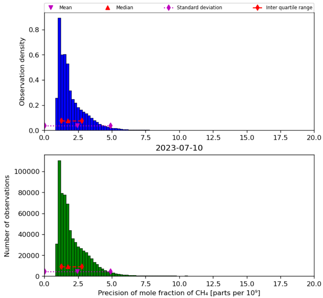
Figure 24: Histogram of “Precision of mole fraction of CH 4 ” for 2023-07-09 to 2023-07-11
