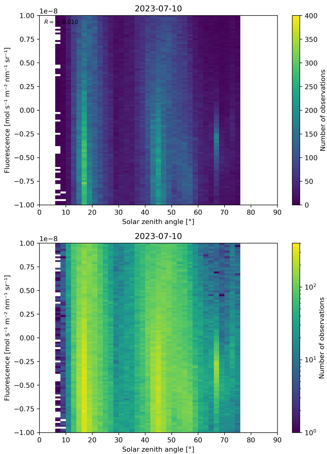
Figure 97: Scatter density plot of “Solar zenith angle” against “Fluorescence” for 2023-07-09 to 2023-07-11.
