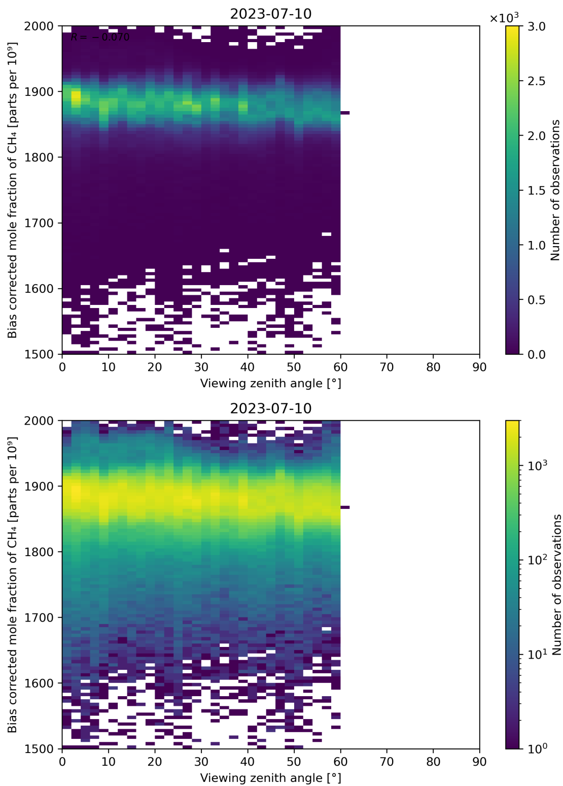
Figure 111: Scatter density plot of “Viewing zenith angle” against “Bias corrected mole fraction of CH 4 ” for 2023-07-09 to 2023-07-11.
