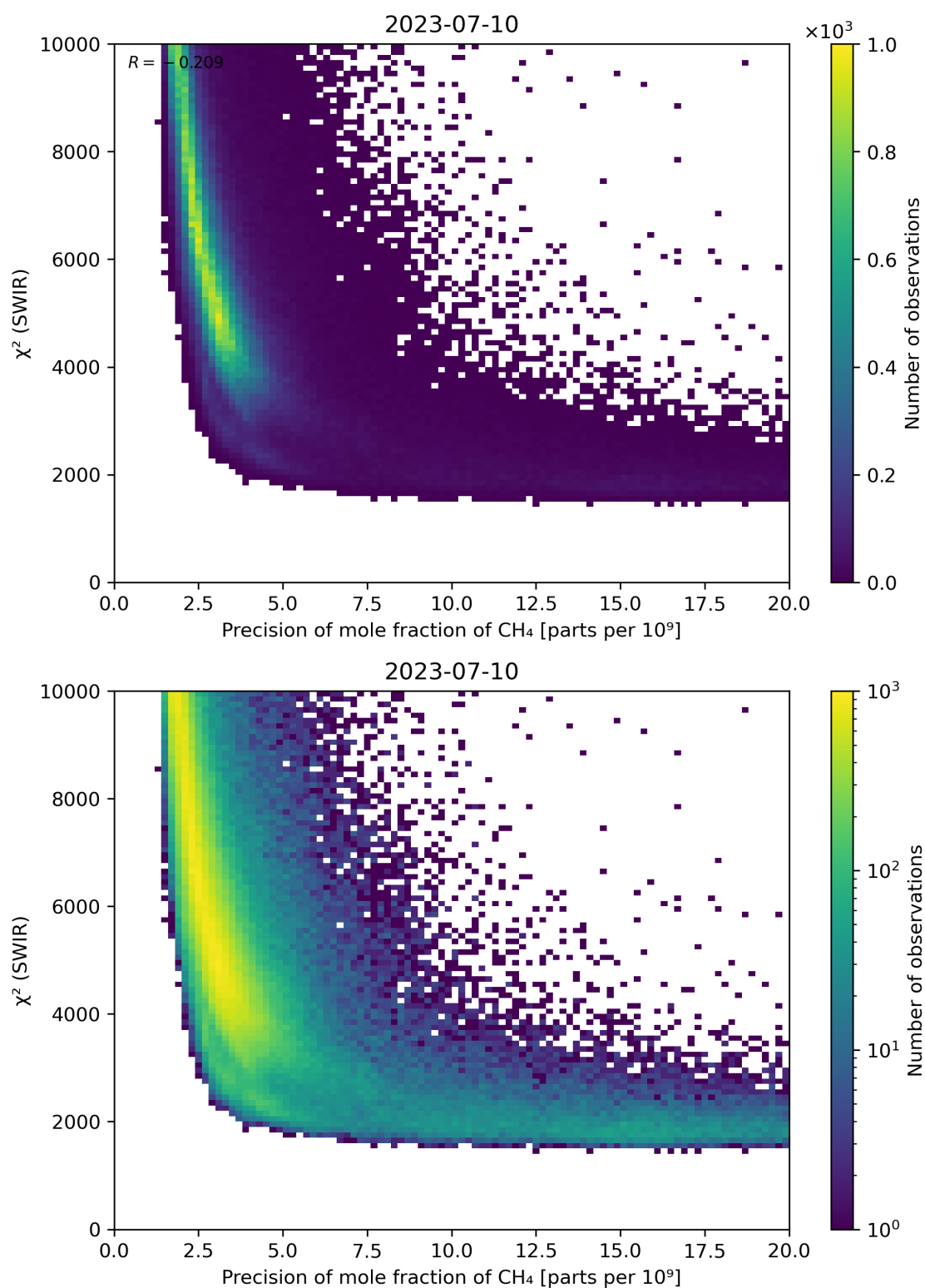
Figure 79: Scatter density plot of “Precision of mole fraction of \text{CH}_4 ” against “ \chi^2 (SWIR)” for 2023-07-09 to 2023-07-11.
