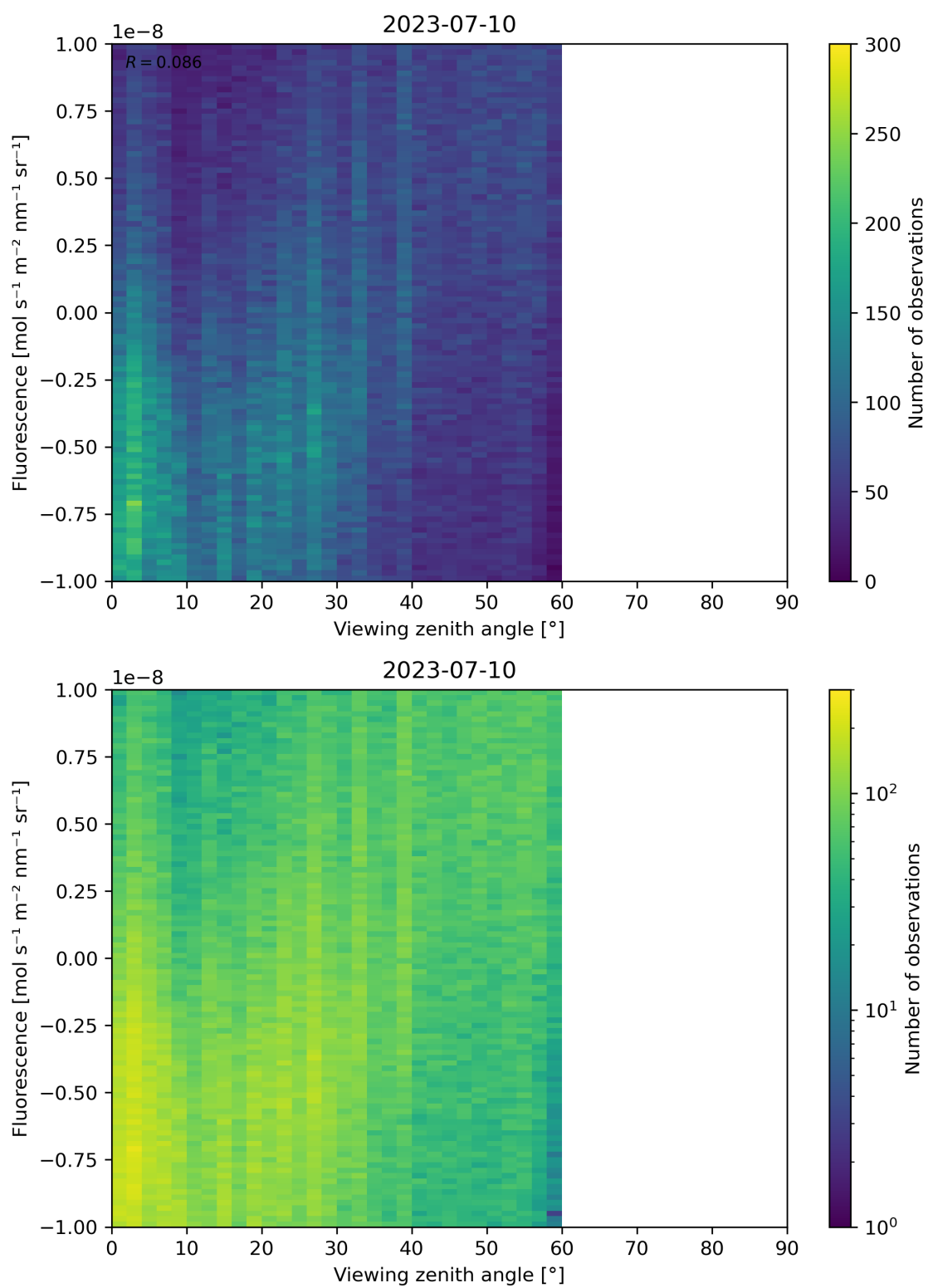
Figure 108: Scatter density plot of “Viewing zenith angle” against “Fluorescence” for 2023-07-09 to 2023-07-11.
