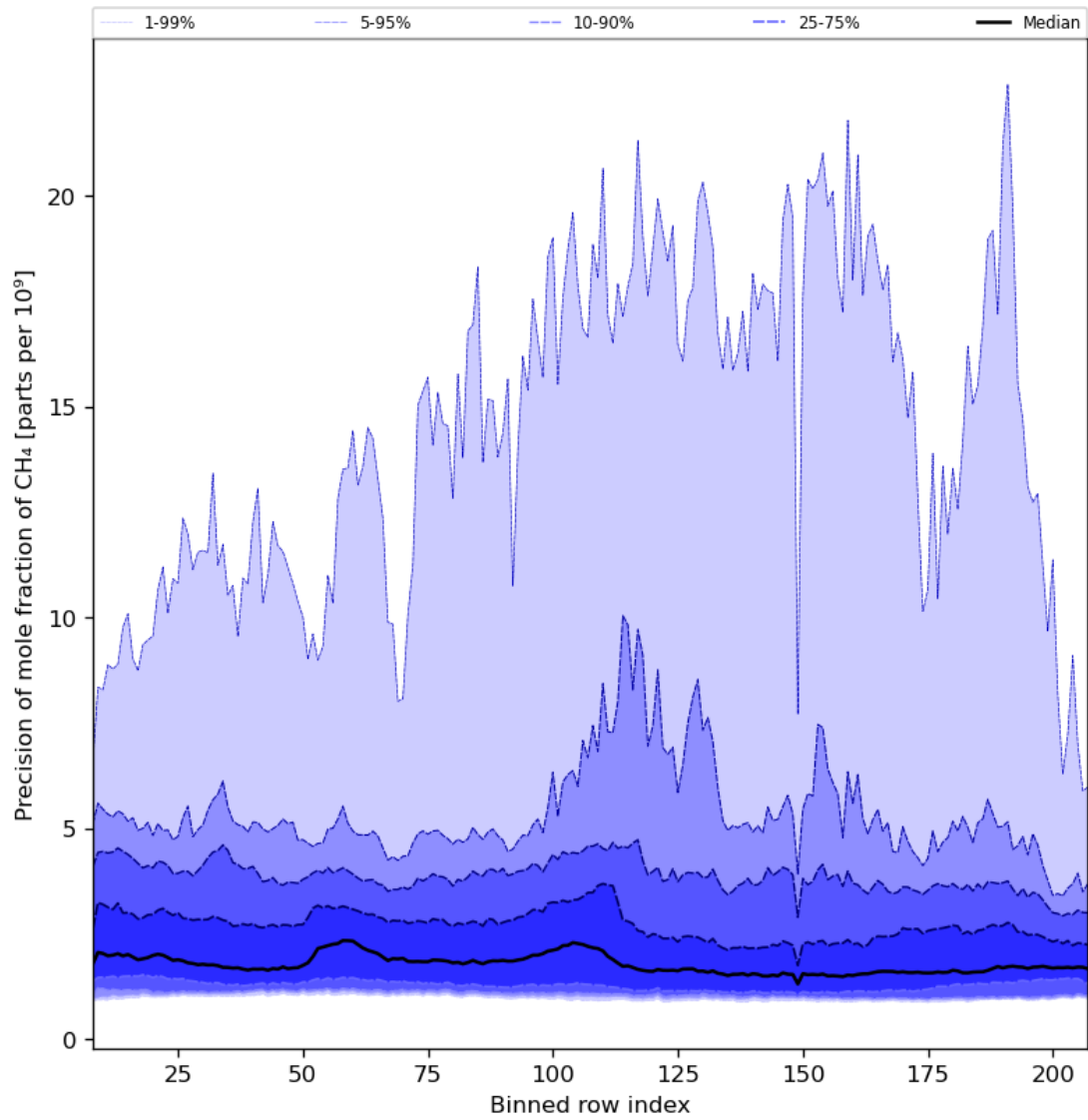
Figure 35: Along track statistics of “Precision of mole fraction of CH 4 ” for 2023-07-09 to 2023-07-11
