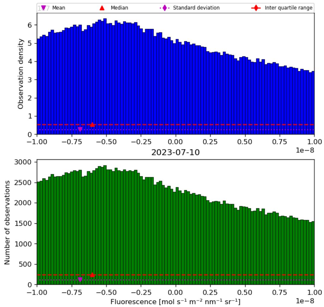
Figure 32: Histogram of “Fluorescence” for 2023-07-09 to 2023-07-11
