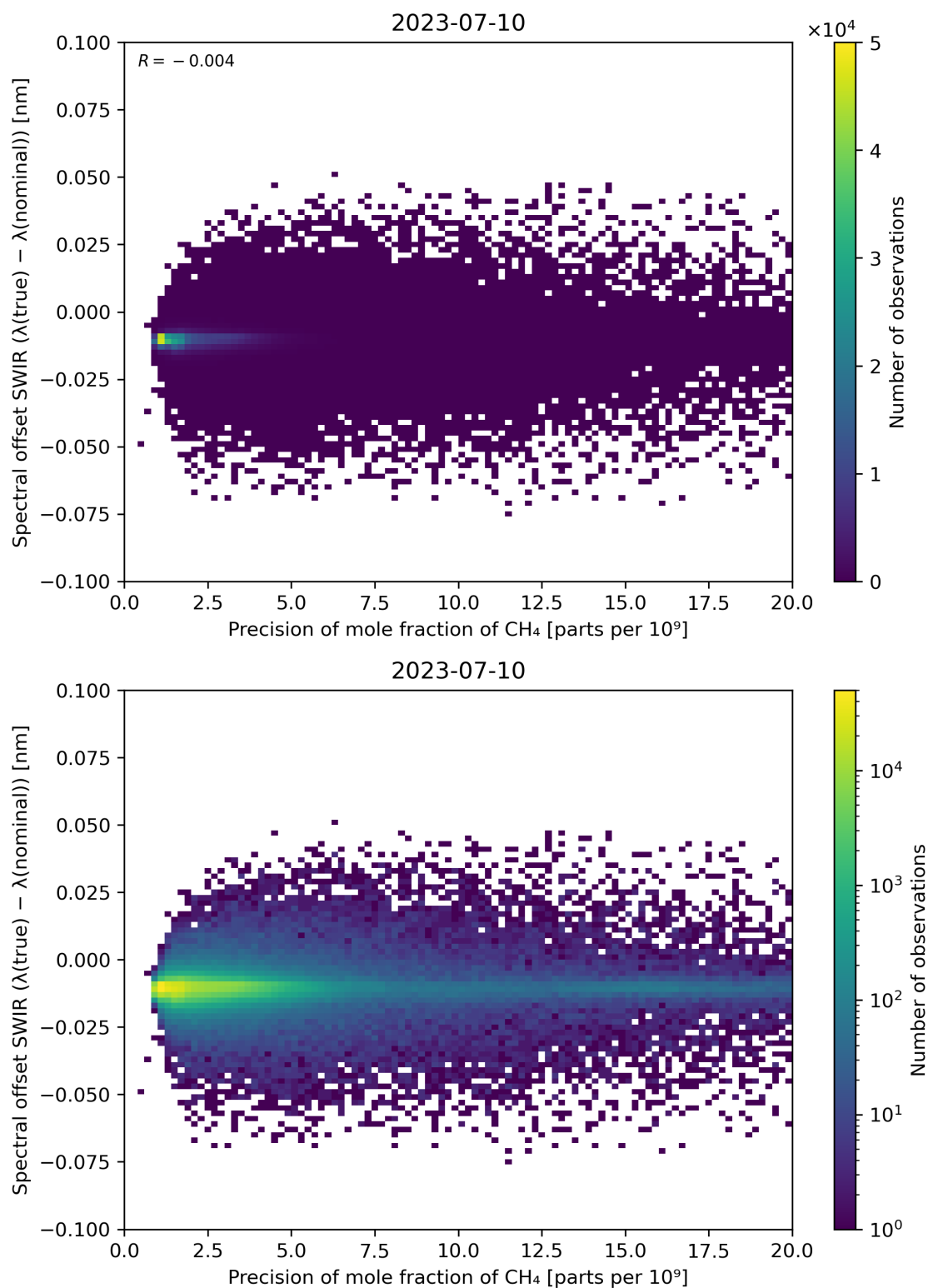
Figure 85: Scatter density plot of “Precision of mole fraction of CH 4 ” against “Spectral offset SWIR ( \lambda(\text{true}) - \lambda(\text{nominal}) )” for 2023-07-09 to 2023-07-11.
