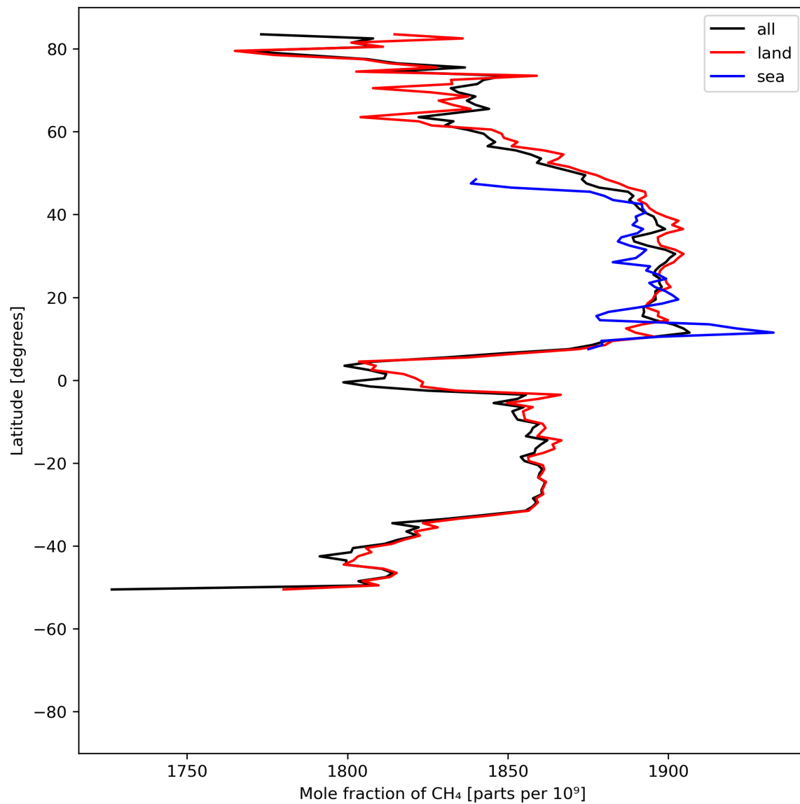
Figure 12: Zonal average of “Mole fraction of \text{CH}_4 ” for 2023-07-09 to 2023-07-11.
