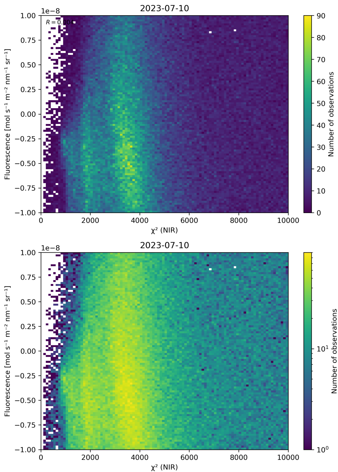
Figure 45: Scatter density plot of “ \chi^2 (NIR)” against “Fluorescence” for 2023-07-09 to 2023-07-11.
