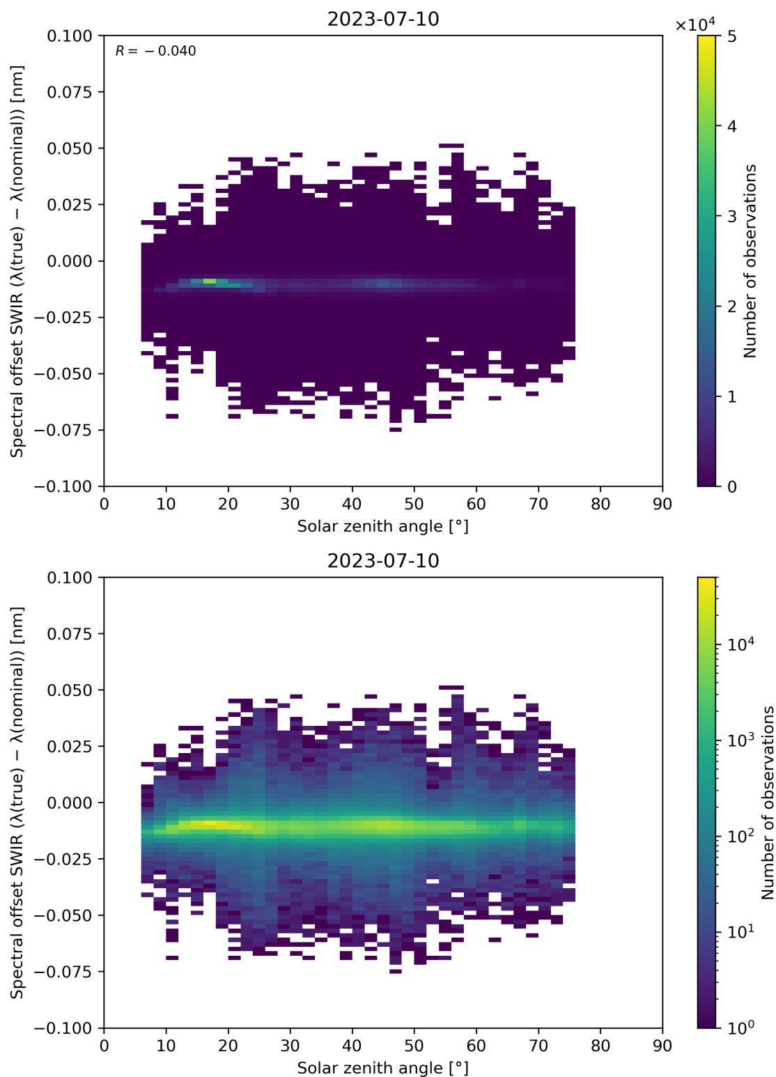
Figure 104: Scatter density plot of “Solar zenith angle” against “Spectral offset SWIR ( \lambda(\text{true}) - \lambda(\text{nominal}) )” for 2023-07-09 to 2023-07-11.
