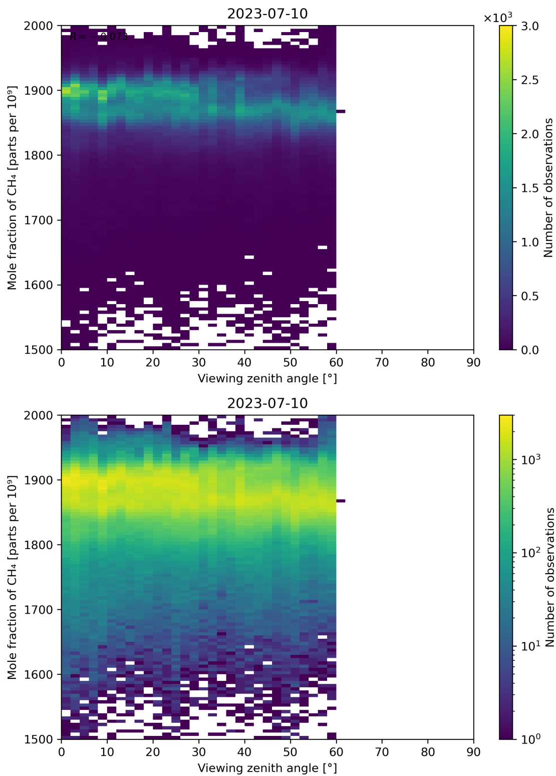
Figure 110: Scatter density plot of “Viewing zenith angle” against “Mole fraction of CH 4 ” for 2023-07-09 to 2023-07-11.
