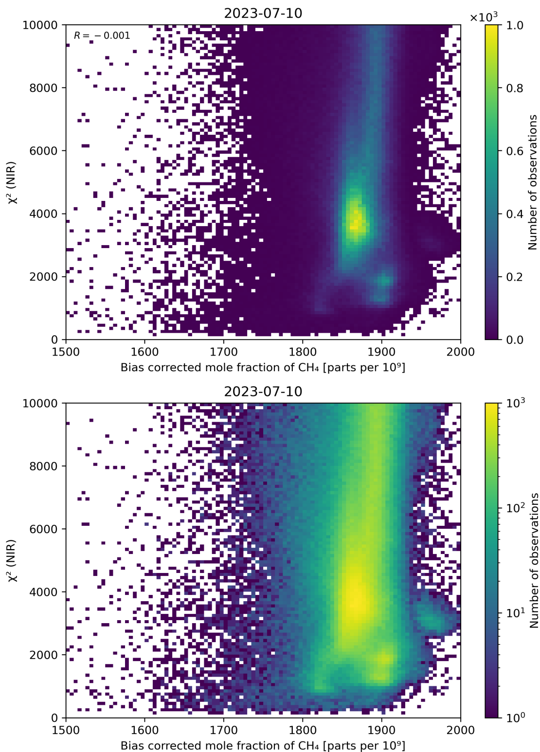
Figure 63: Scatter density plot of “Bias corrected mole fraction of CH 4 ” against “ \chi^2 (NIR)” for 2023-07-09 to 2023-07-11.
