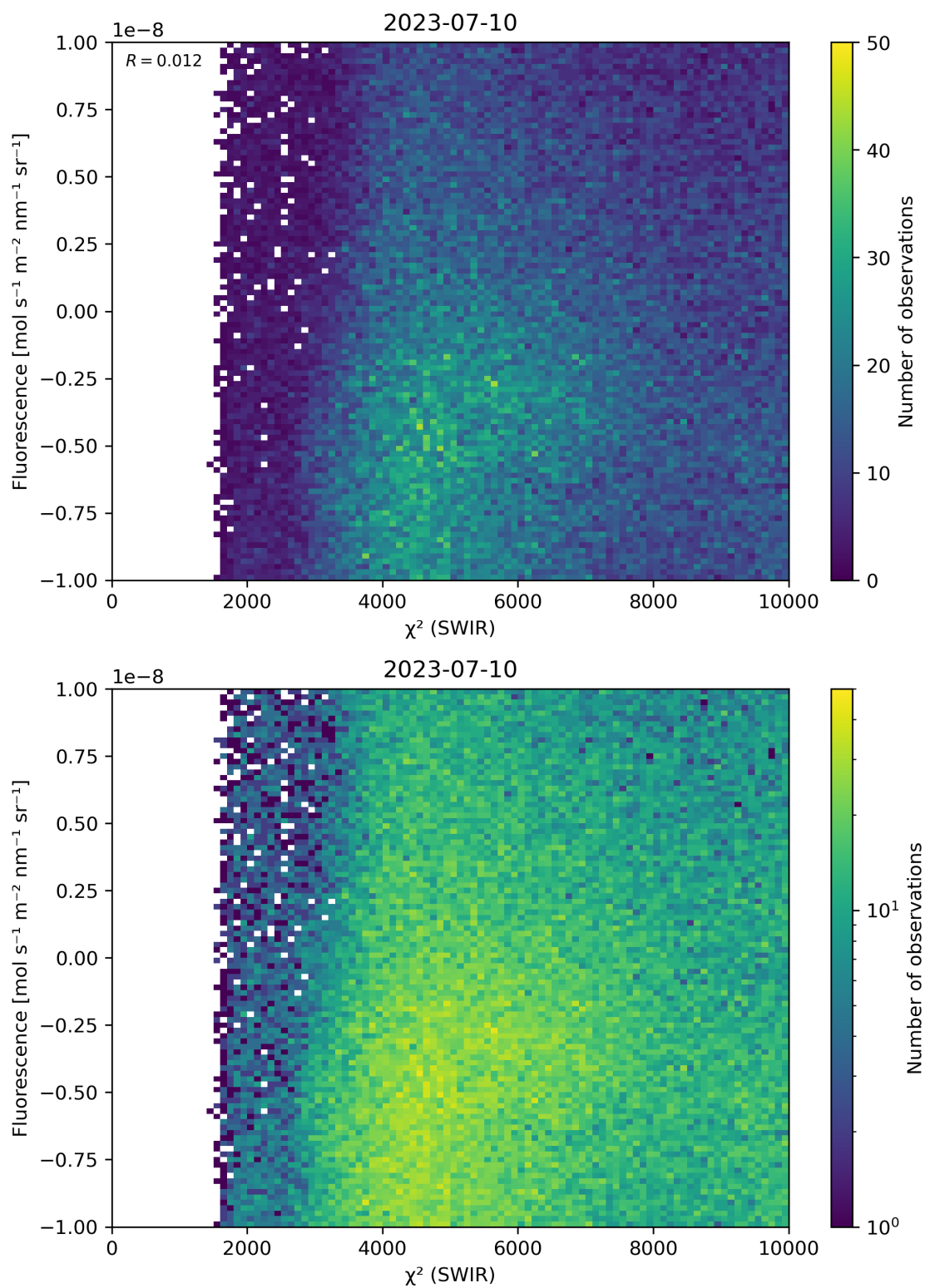
Figure 49: Scatter density plot of “ \chi^2 (SWIR)” against “Fluorescence” for 2023-07-09 to 2023-07-11.
