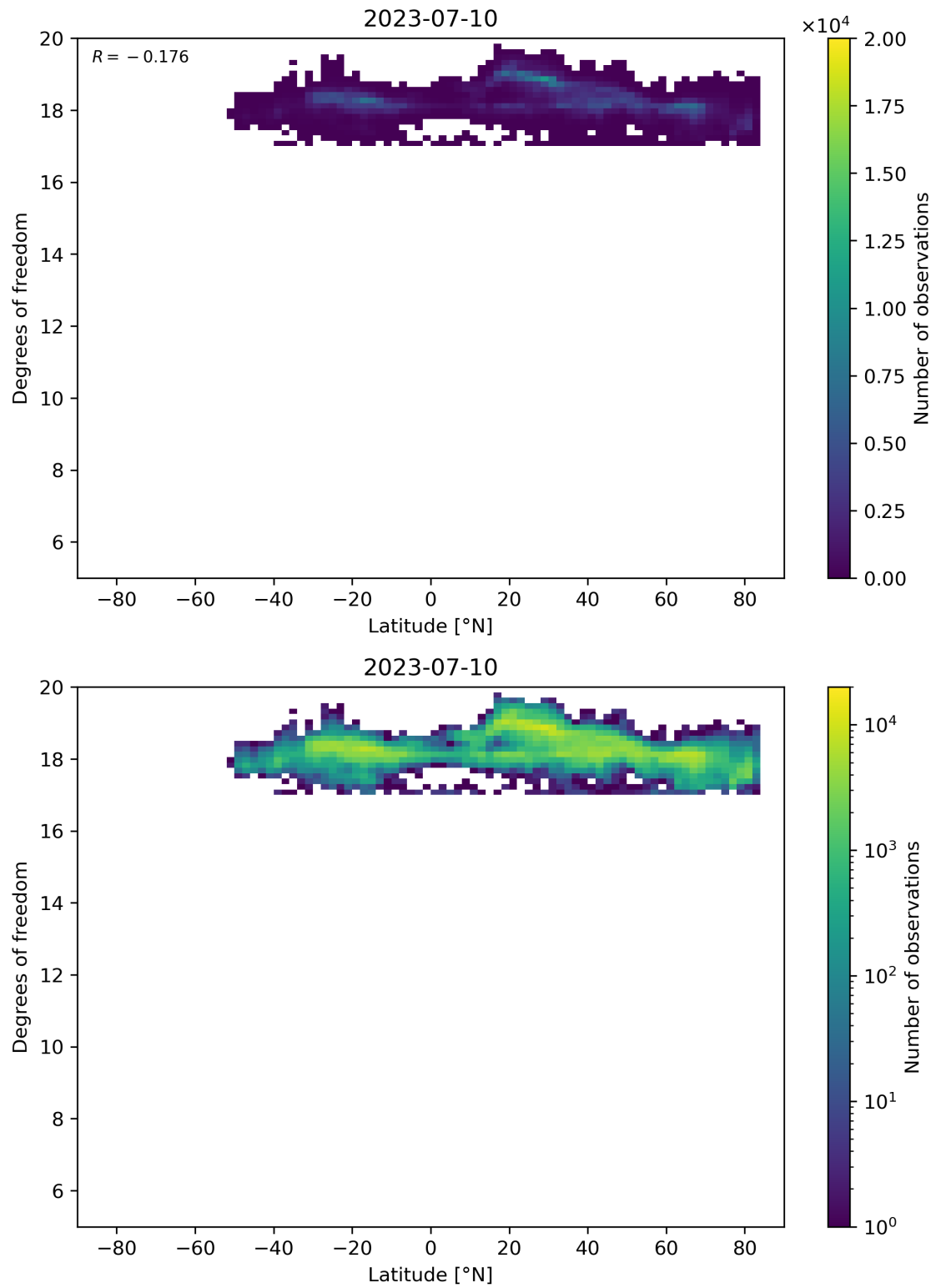
Figure 55: Scatter density plot of “Latitude” against “Degrees of freedom” for 2023-07-09 to 2023-07-11.
