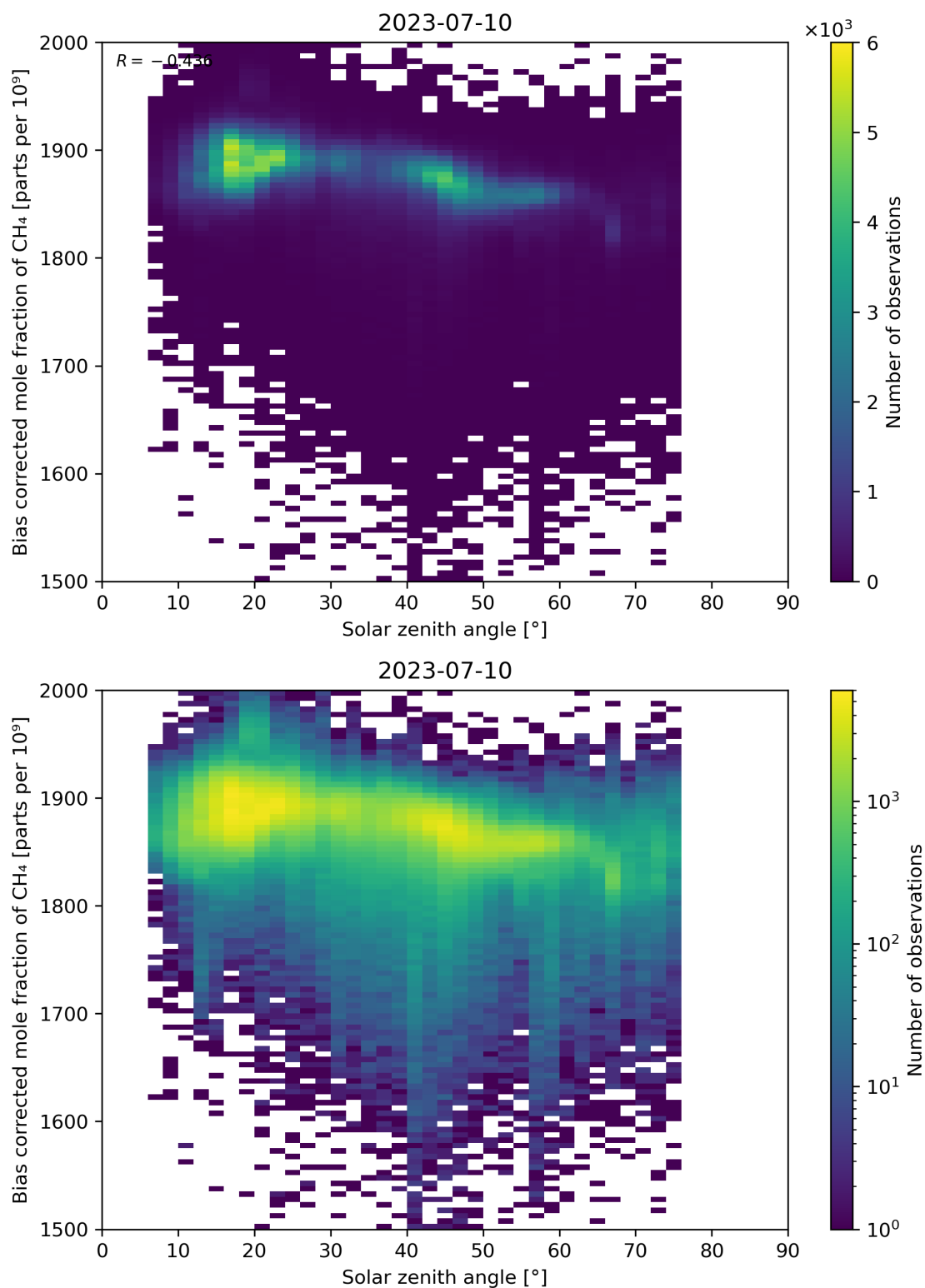
Figure 100: Scatter density plot of “Solar zenith angle” against “Bias corrected mole fraction of CH 4 ” for 2023-07-09 to 2023-07-11.
