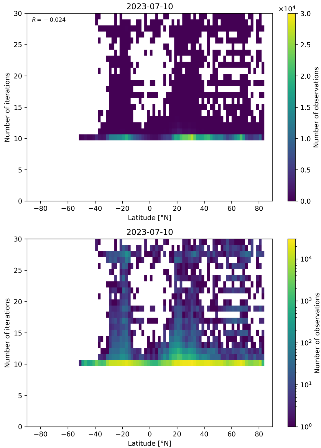
Figure 60: Scatter density plot of “Latitude” against “Number of iterations” for 2023-07-09 to 2023-07-11.
