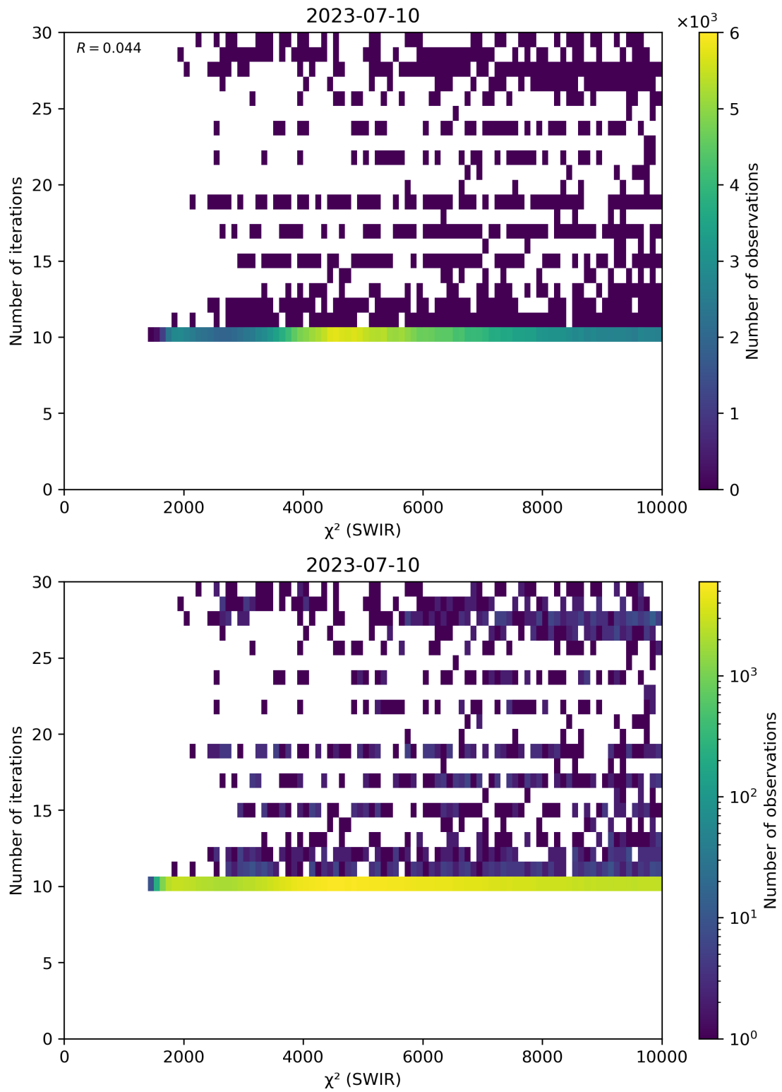
Figure 50: Scatter density plot of “ \chi^2 (SWIR)” against “Number of iterations” for 2023-07-09 to 2023-07-11.
