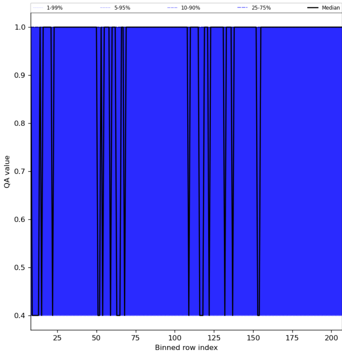
Figure 33: Along track statistics of “QA value” for 2023-07-09 to 2023-07-11
