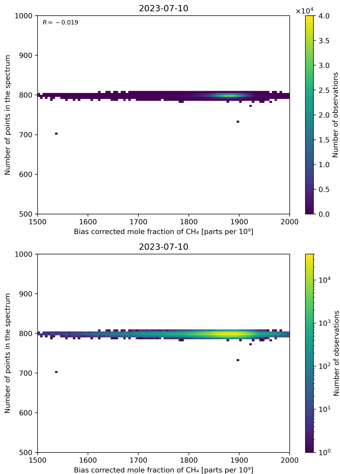
Figure 68: Scatter density plot of “Bias corrected mole fraction of CH 4 ” against “Number of points in the spectrum” for 2023-07-09 to 2023-07-11.
