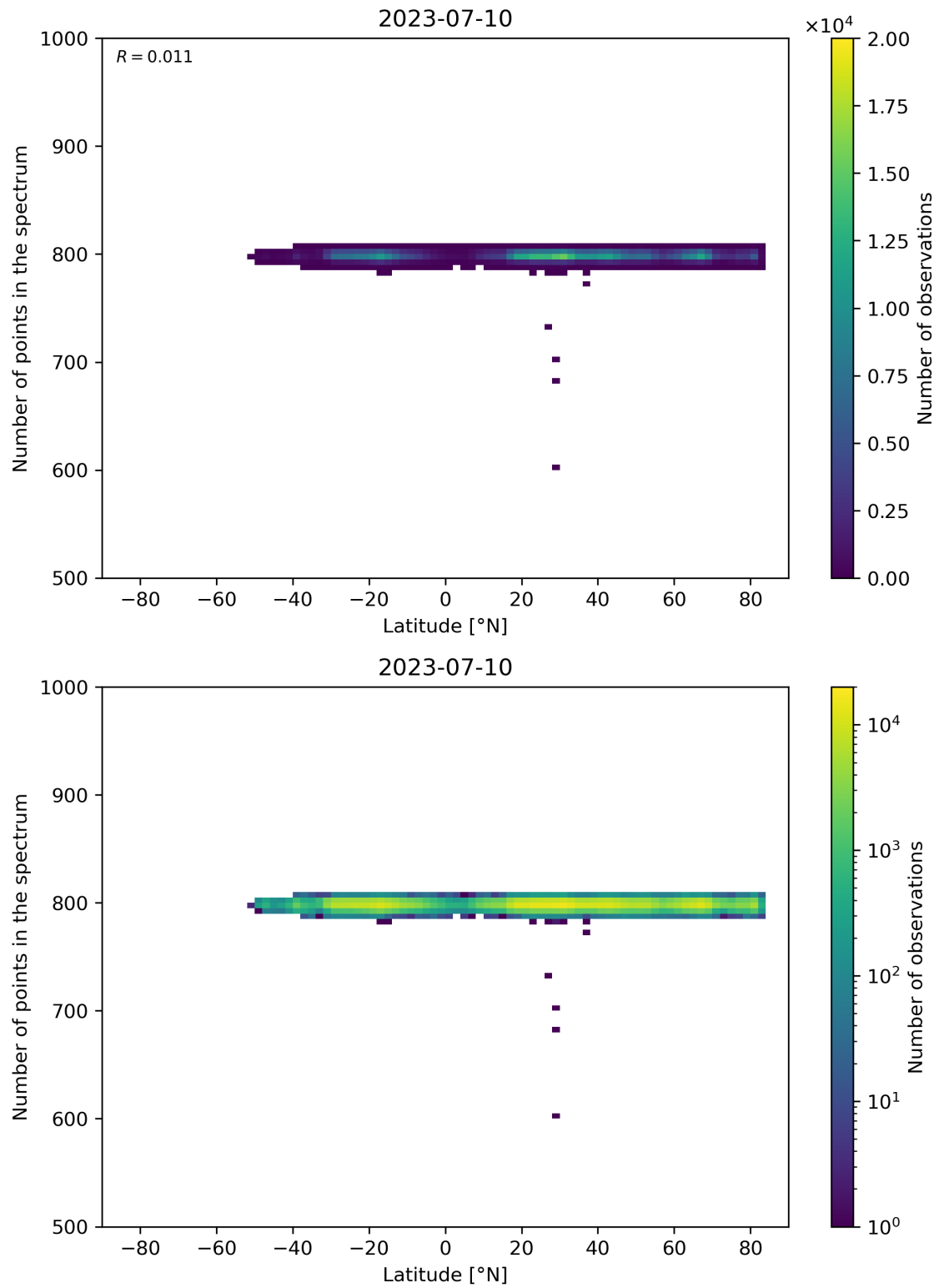
Figure 61: Scatter density plot of “Latitude” against “Number of points in the spectrum” for 2023-07-09 to 2023-07-11.
