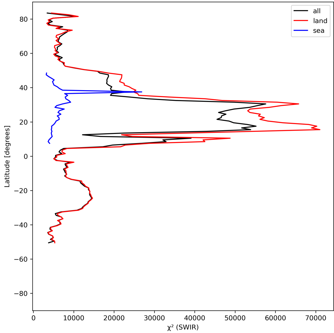
Figure 17: Zonal average of “ \chi^2 (SWIR)” for 2023-07-09 to 2023-07-11.
