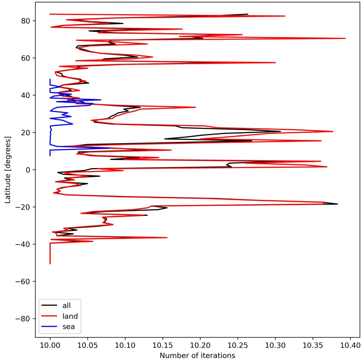
Figure 20: Zonal average of “Number of iterations” for 2023-07-09 to 2023-07-11.
