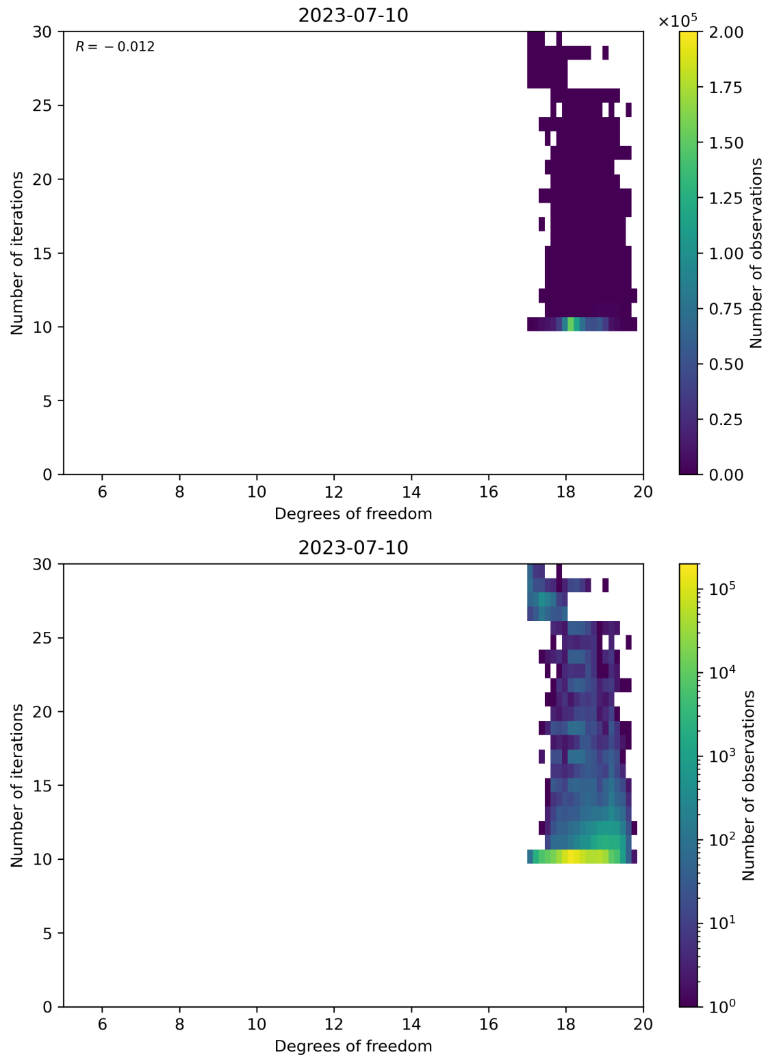
Figure 52: Scatter density plot of “Degrees of freedom” against “Number of iterations” for 2023-07-09 to 2023-07-11.
