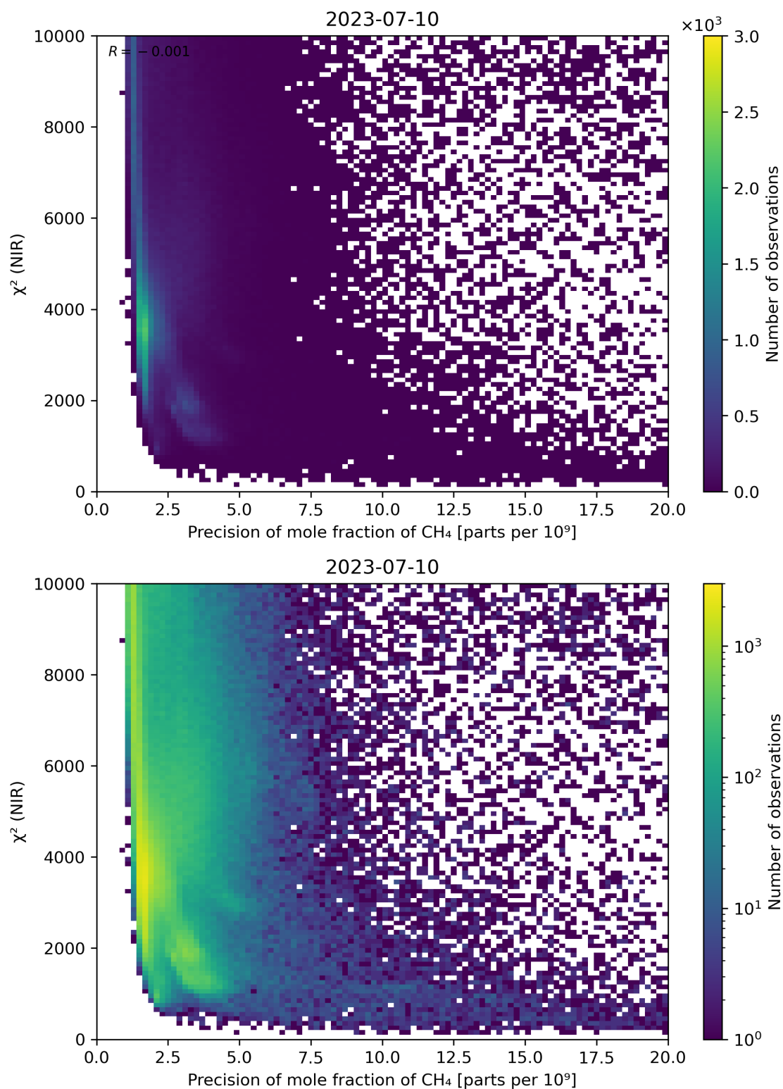
Figure 78: Scatter density plot of “Precision of mole fraction of CH 4 ” against “ \chi^2 (NIR)” for 2023-07-09 to 2023-07-11.
