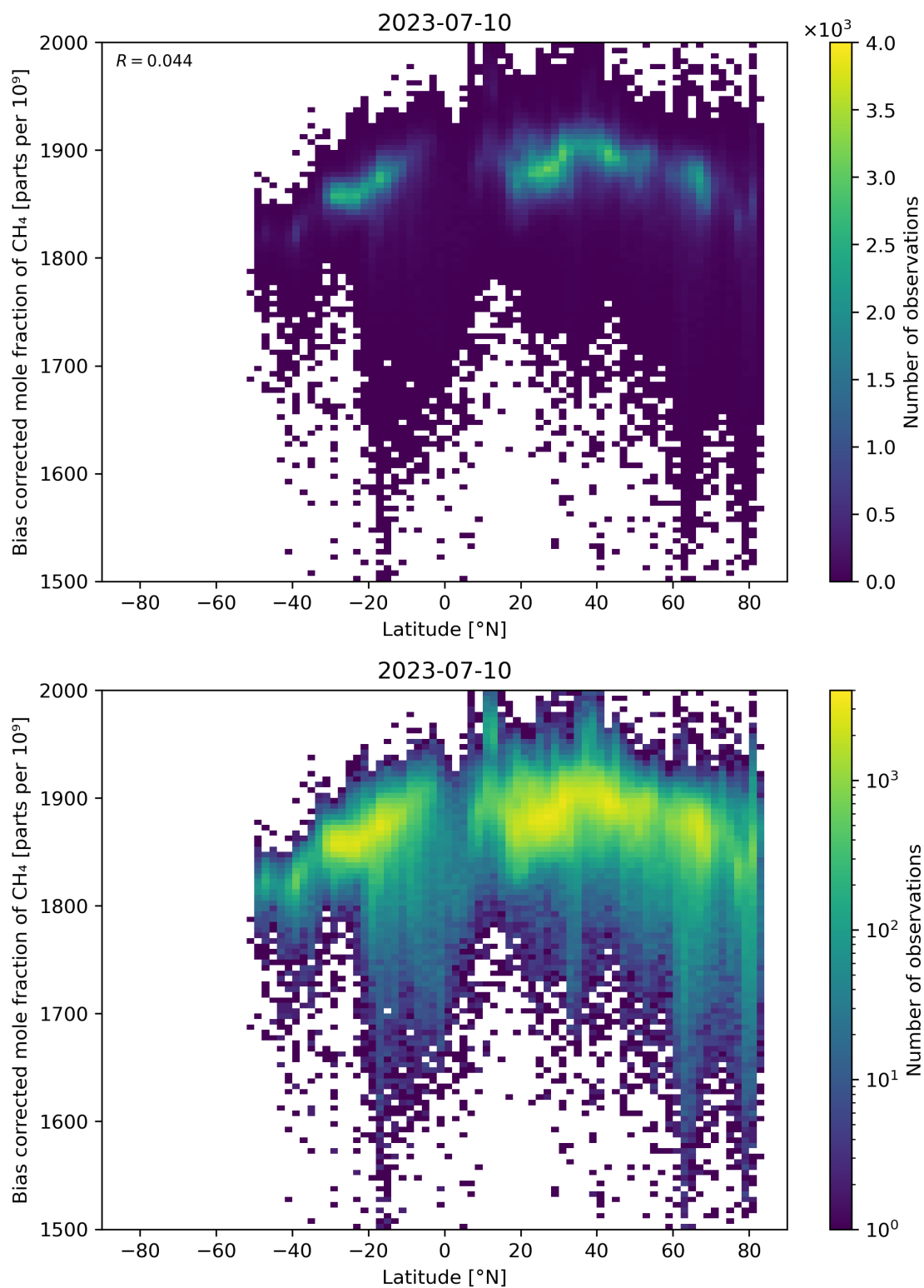
Figure 58: Scatter density plot of “Latitude” against “Bias corrected mole fraction of CH 4 ” for 2023-07-09 to 2023-07-11.
