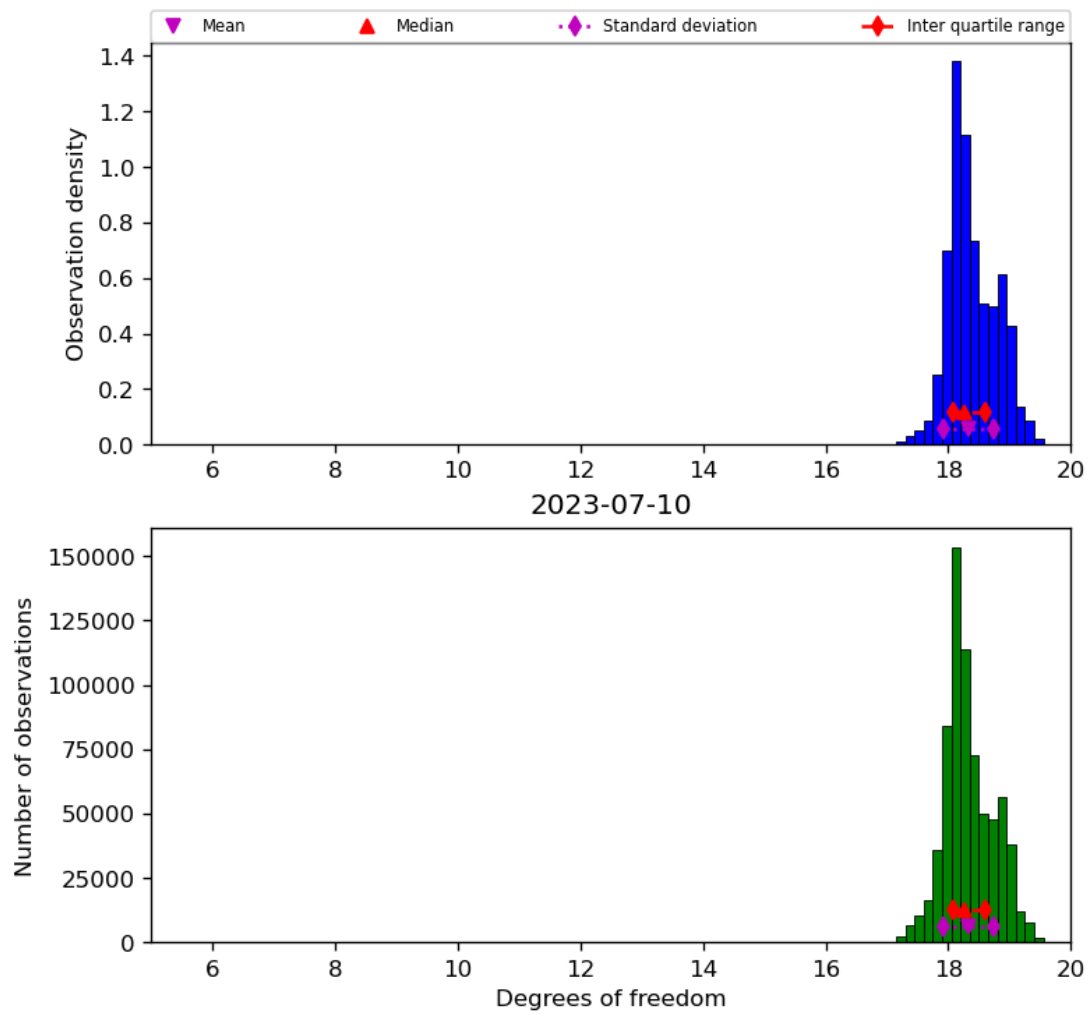
Figure 30: Histogram of “Degrees of freedom” for 2023-07-09 to 2023-07-11
