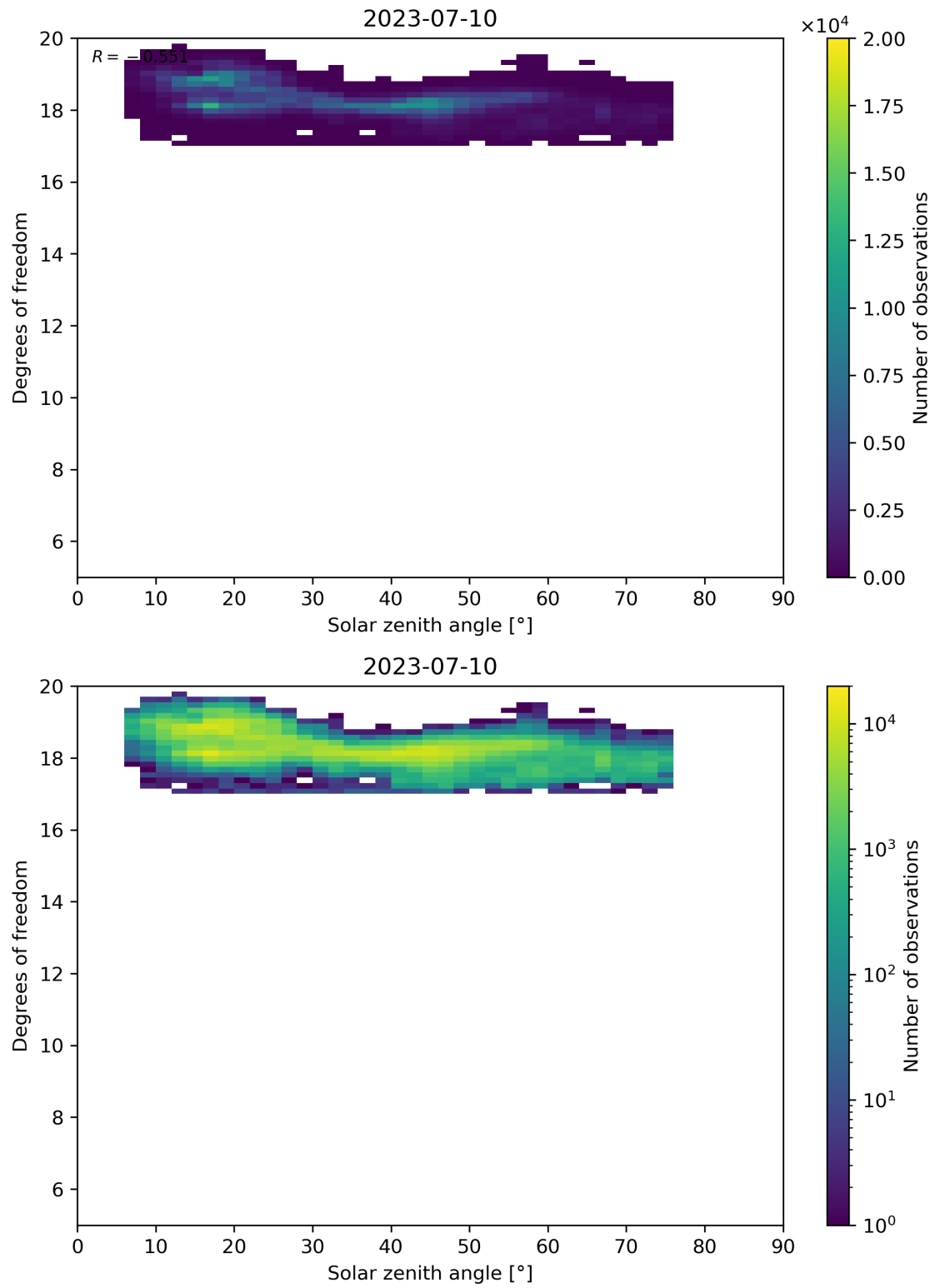
Figure 96: Scatter density plot of “Solar zenith angle” against “Degrees of freedom” for 2023-07-09 to 2023-07-11.
