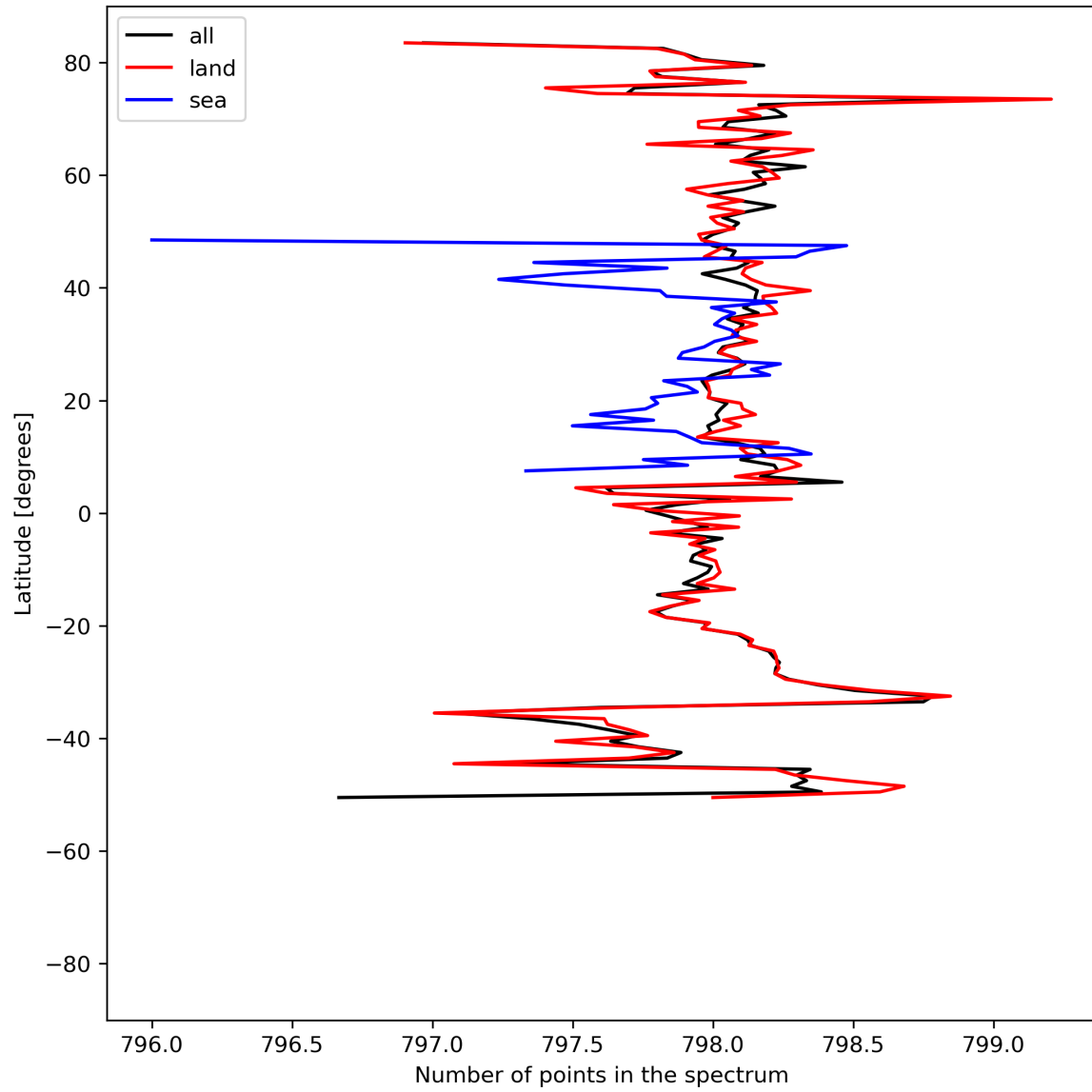
Figure 15: Zonal average of “Number of points in the spectrum” for 2023-07-09 to 2023-07-11.
