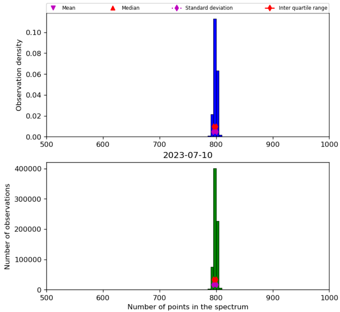
Figure 26: Histogram of “Number of points in the spectrum” for 2023-07-09 to 2023-07-11
