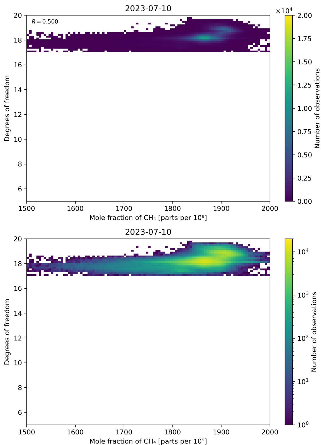
Figure 72: Scatter density plot of “Mole fraction of CH 4 ” against “Degrees of freedom” for 2023-07-09 to 2023-07-11.
