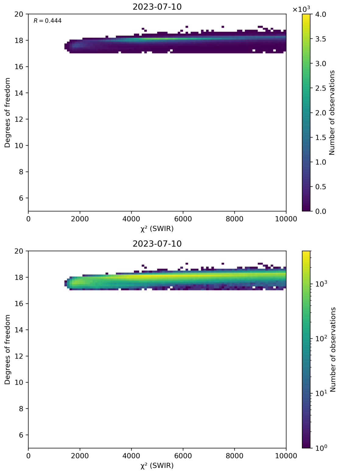
Figure 48: Scatter density plot of “ \chi^2 (SWIR)” against “Degrees of freedom” for 2023-07-09 to 2023-07-11.
