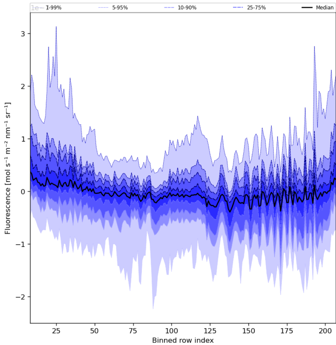
Figure 43: Along track statistics of “Fluorescence” for 2023-07-09 to 2023-07-11
