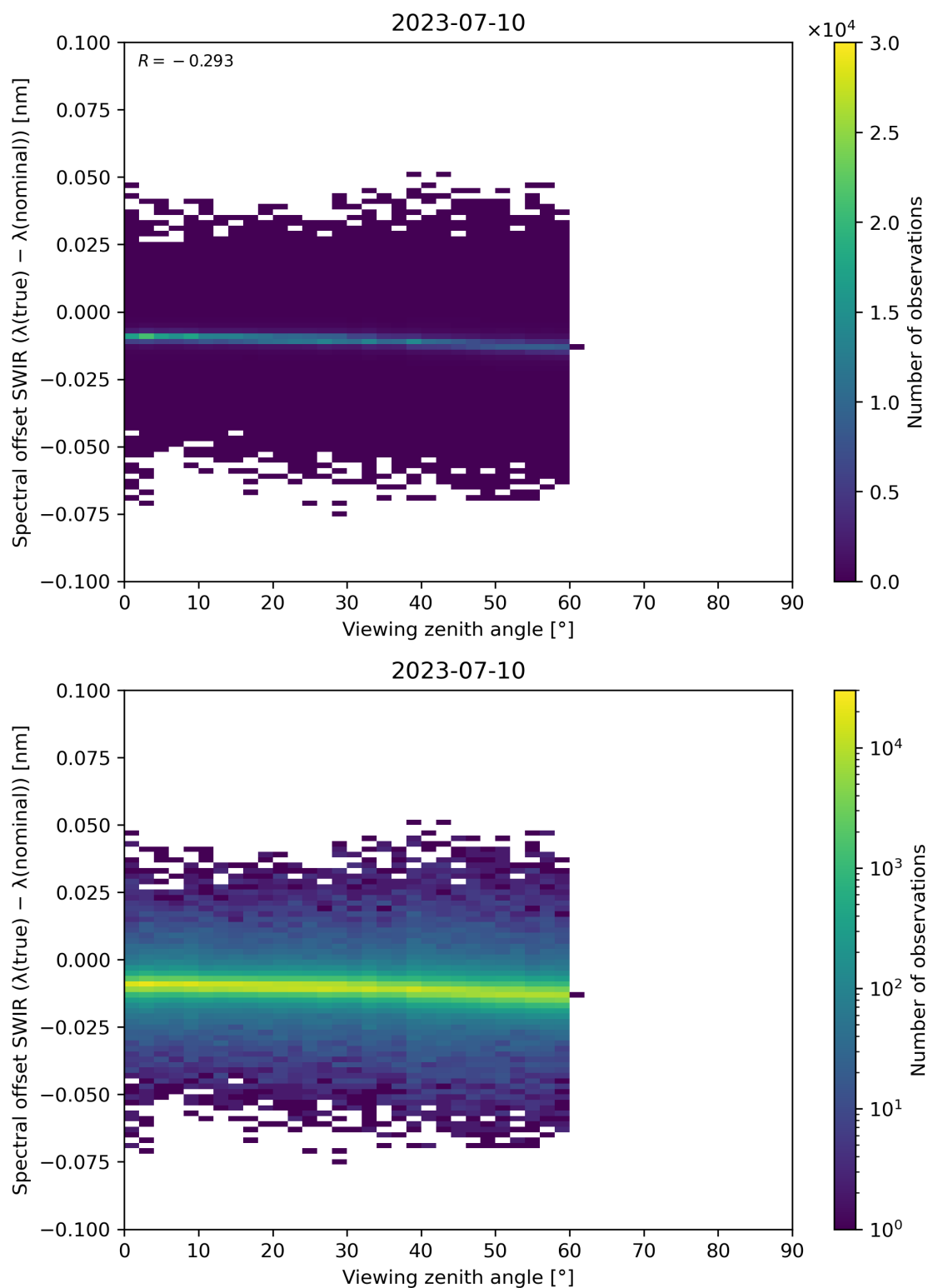
Figure 116: Scatter density plot of “Viewing zenith angle” against “Spectral offset SWIR ( \lambda(\text{true}) - \lambda(\text{nominal}) )” for 2023-07-09 to 2023-07-11.
