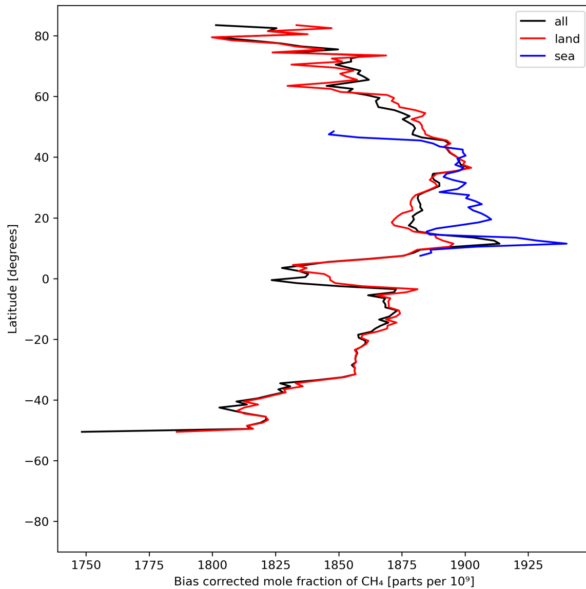
Figure 14: Zonal average of “Bias corrected mole fraction of CH 4 ” for 2023-07-09 to 2023-07-11.
