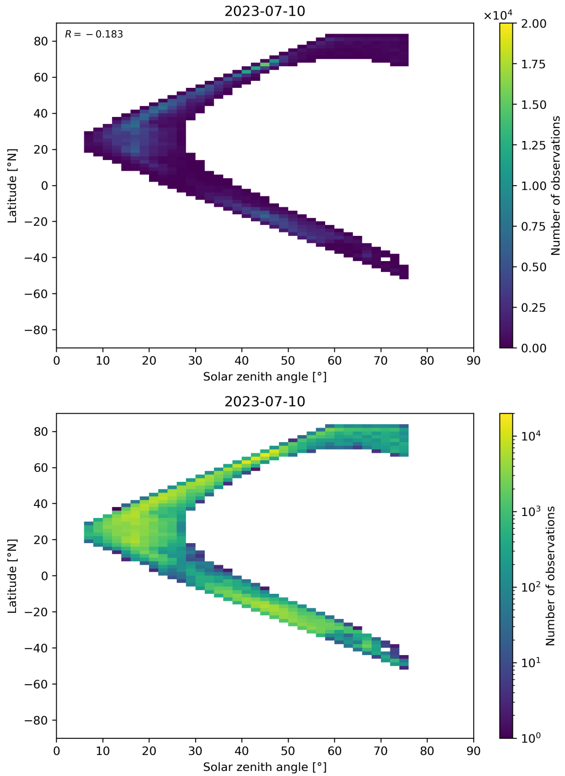
Figure 98: Scatter density plot of “Solar zenith angle” against “Latitude” for 2023-07-09 to 2023-07-11.
