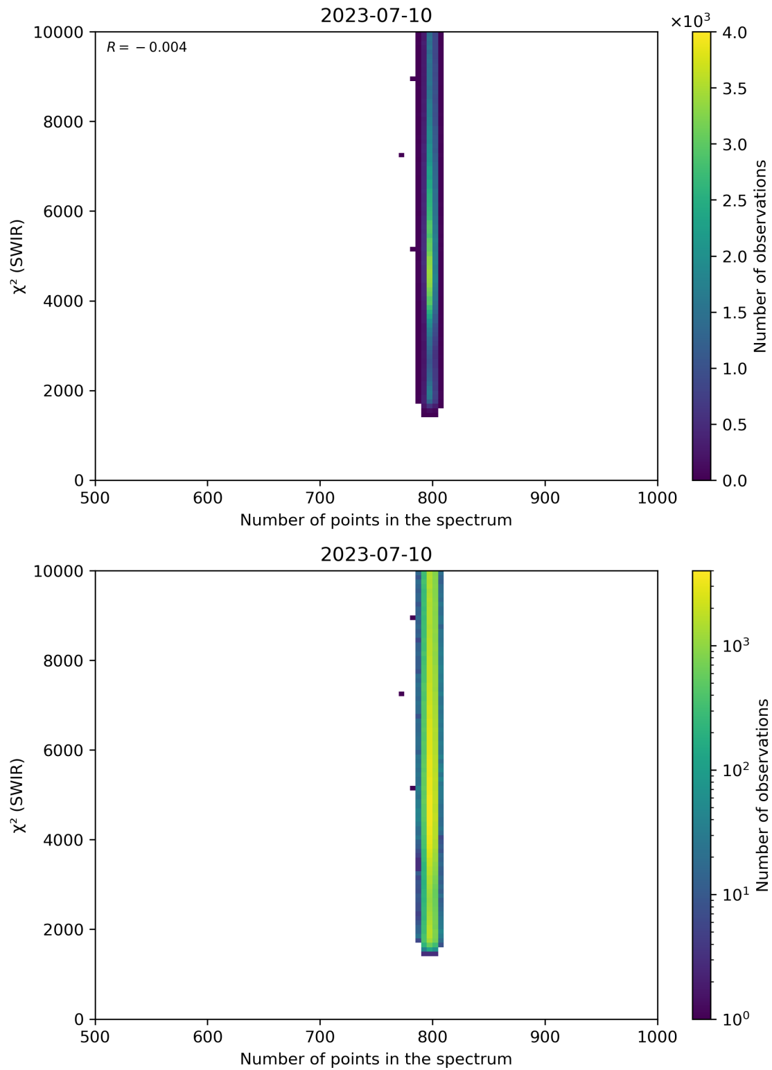
Figure 89: Scatter density plot of “Number of points in the spectrum” against “ \chi^2 (SWIR)” for 2023-07-09 to 2023-07-11.
