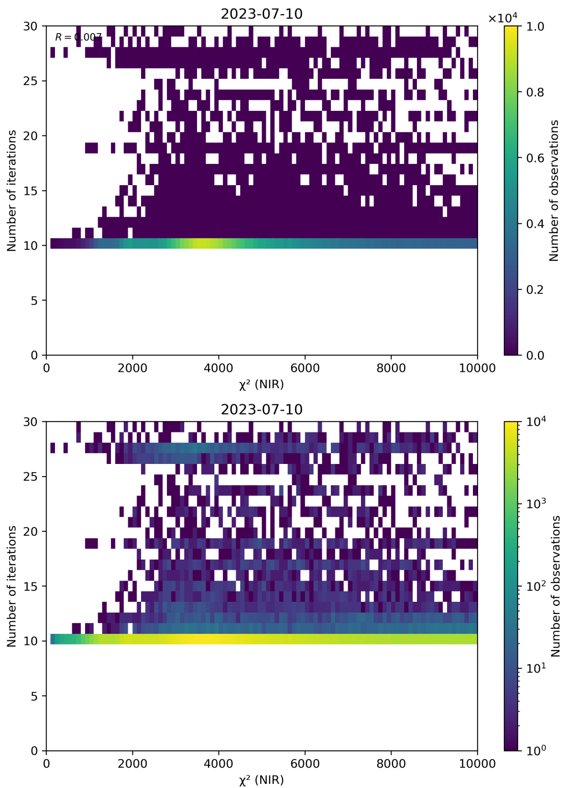
Figure 46: Scatter density plot of “ \chi^2 (NIR)” against “Number of iterations” for 2023-07-09 to 2023-07-11.
