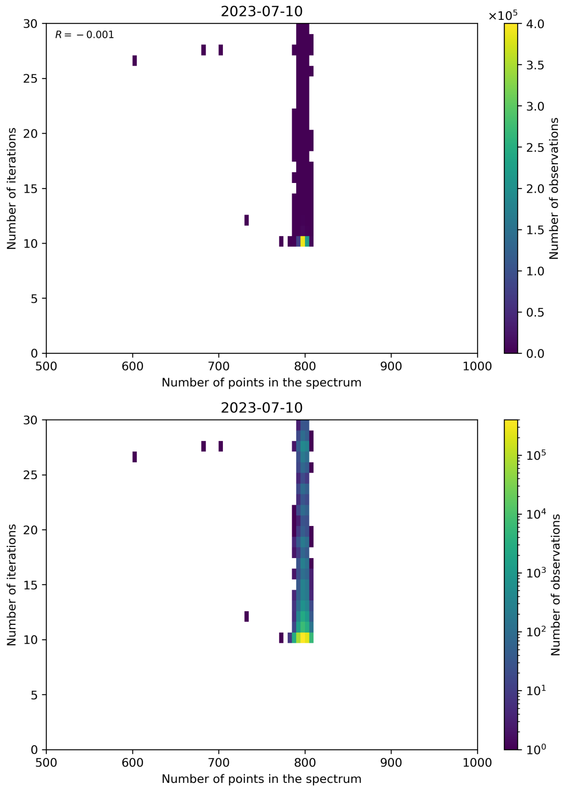
Figure 92: Scatter density plot of “Number of points in the spectrum” against “Number of iterations” for 2023-07-09 to 2023-07-11.
