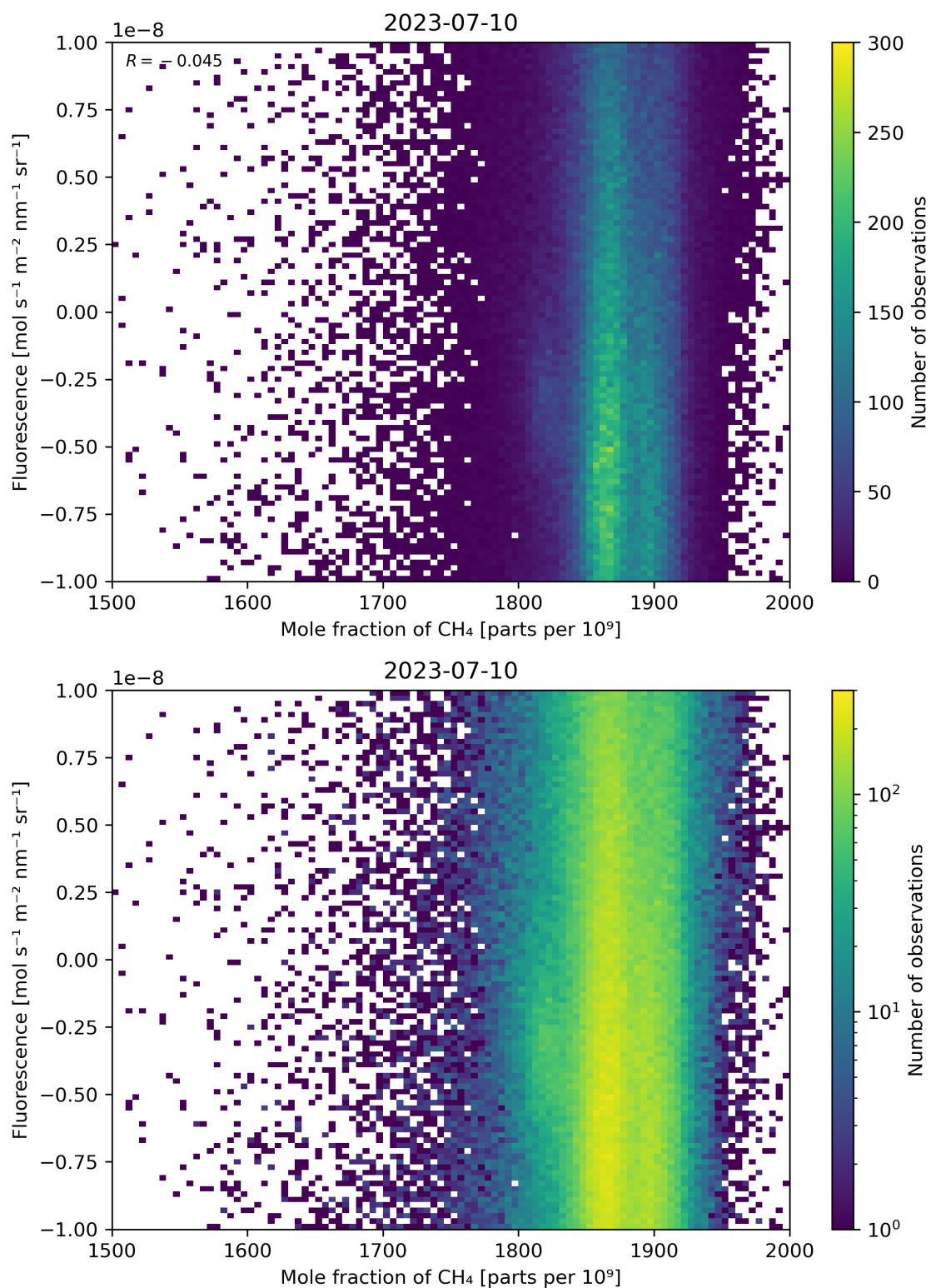
Figure 73: Scatter density plot of “Mole fraction of \text{CH}_4 ” against “Fluorescence” for 2023-07-09 to 2023-07-11.
