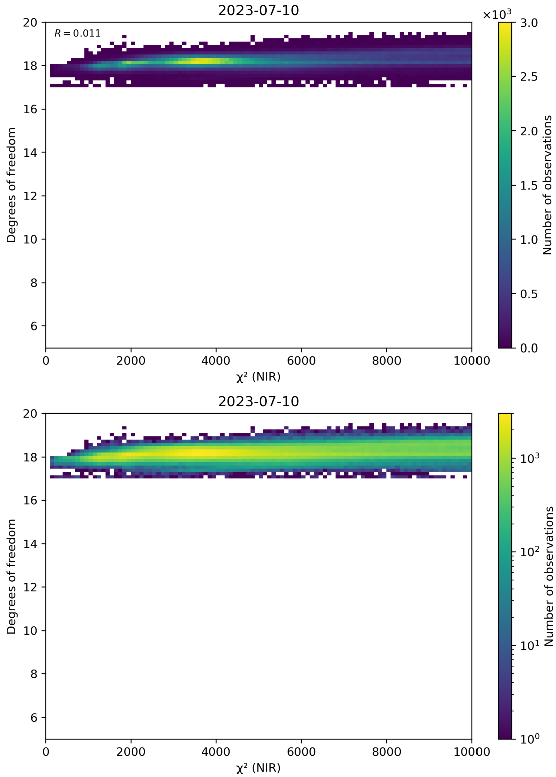
Figure 44: Scatter density plot of “ \chi^2 (NIR)” against “Degrees of freedom” for 2023-07-09 to 2023-07-11.
