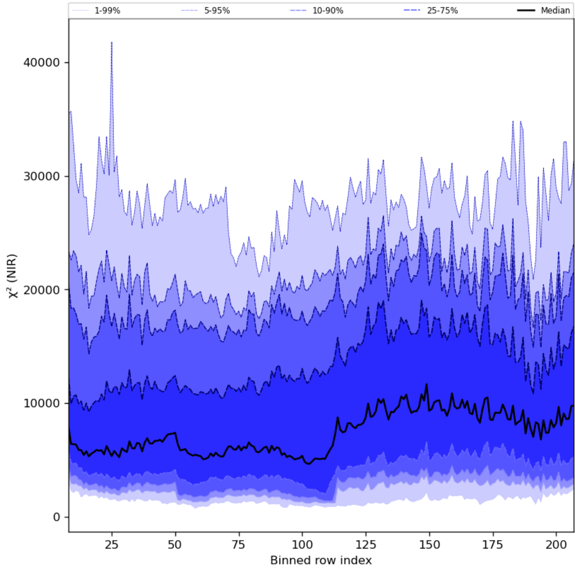
Figure 40: Along track statistics of “ \chi^2 (NIR)” for 2023-07-09 to 2023-07-11
