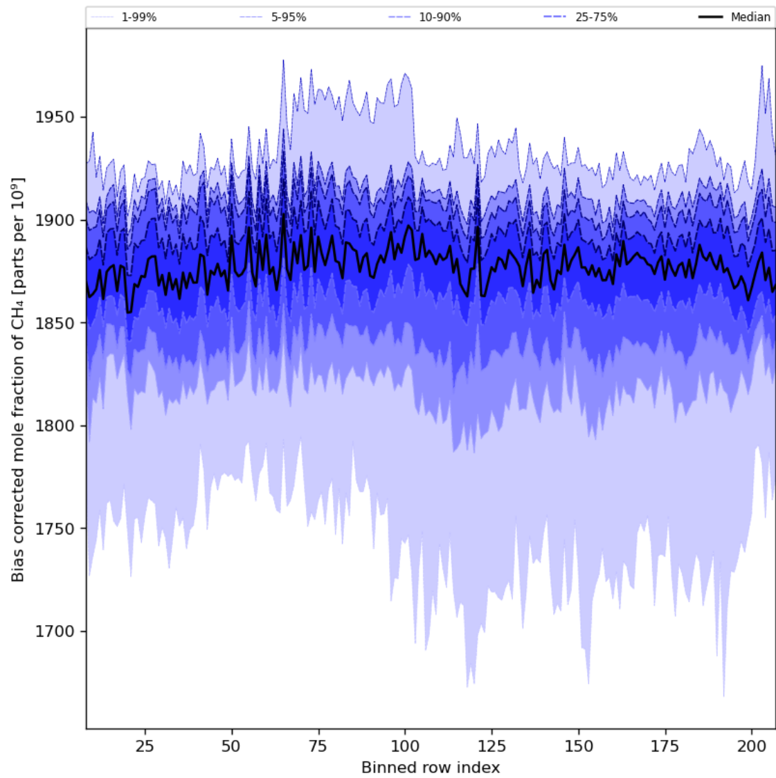
Figure 36: Along track statistics of “Bias corrected mole fraction of CH 4 ” for 2023-07-09 to 2023-07-11
