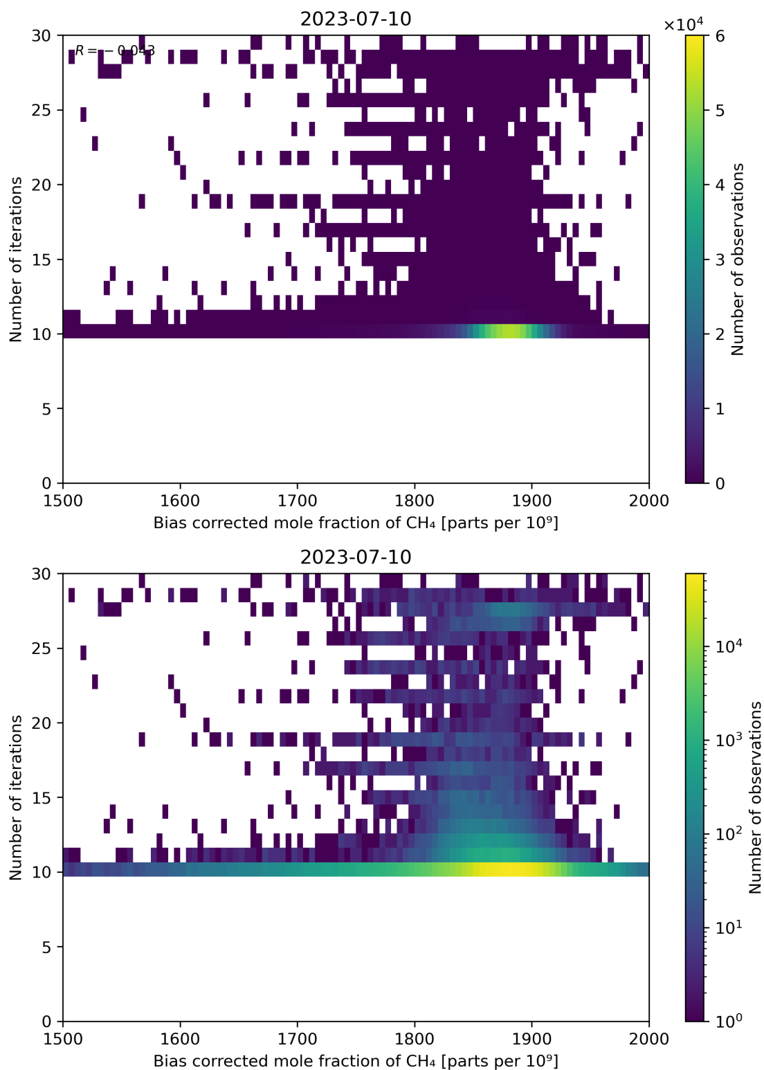
Figure 67: Scatter density plot of “Bias corrected mole fraction of CH 4 ” against “Number of iterations” for 2023-07-09 to 2023-07-11.
