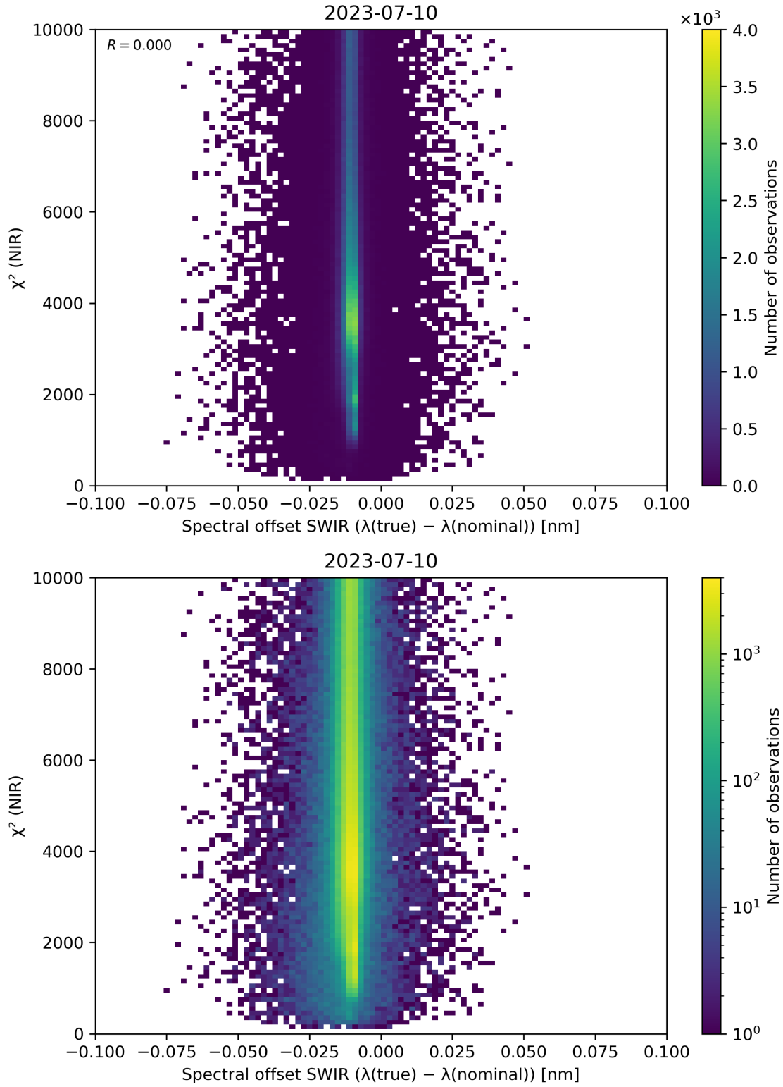
Figure 117: Scatter density plot of “Spectral offset SWIR ( \lambda(\text{true}) - \lambda(\text{nominal}) )” against “ \chi^2 (NIR)” for 2023-07-09 to 2023-07-11.
