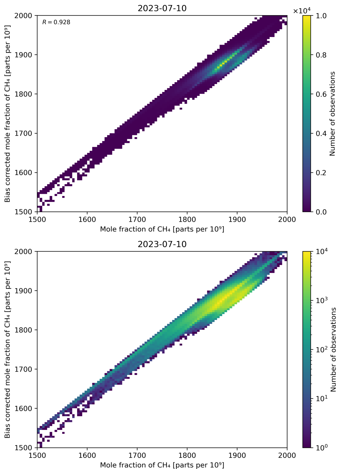
Figure 74: Scatter density plot of “Mole fraction of CH 4 ” against “Bias corrected mole fraction of CH 4 ” for 2023-07-09 to 2023-07-11.
