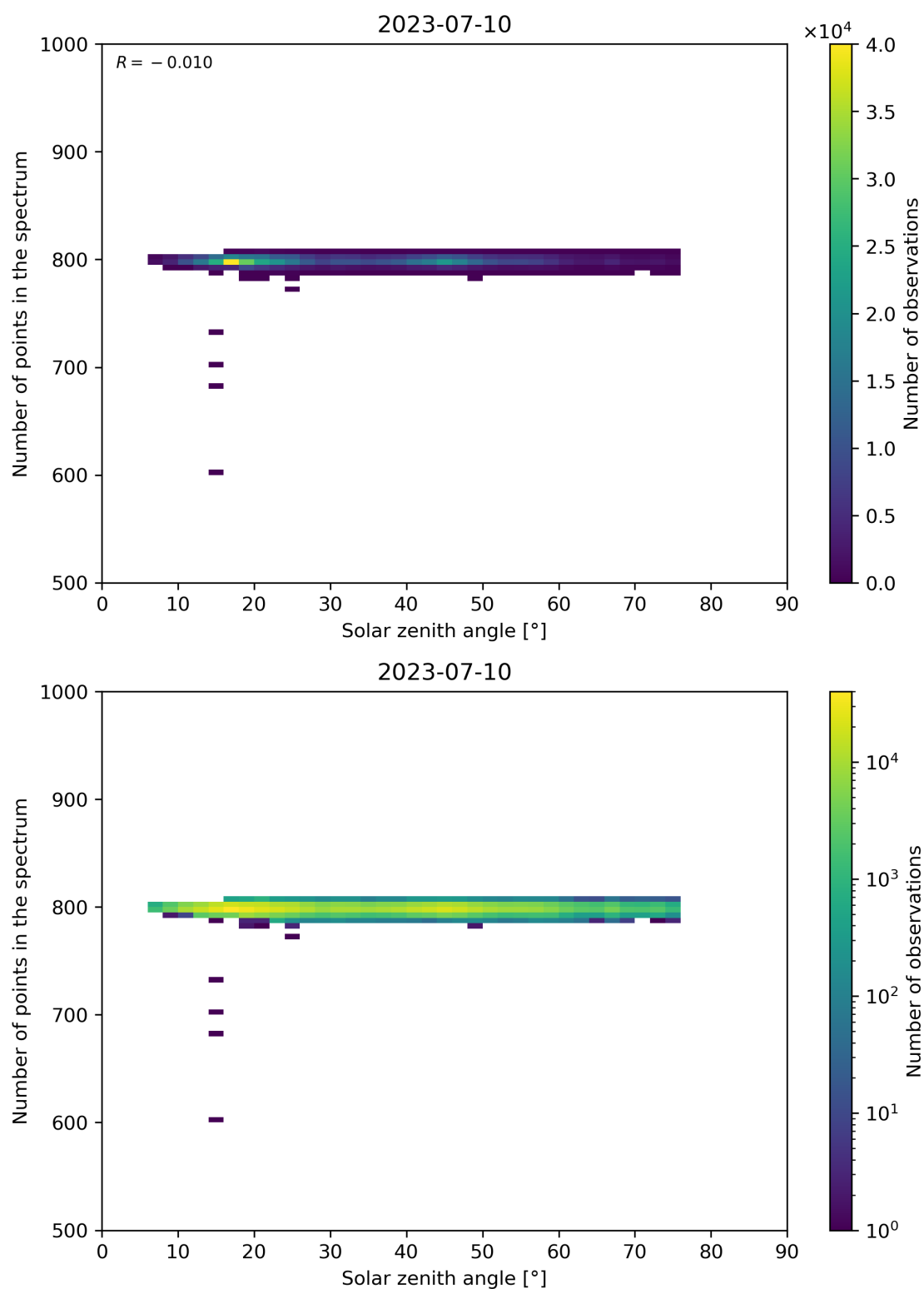
Figure 103: Scatter density plot of “Solar zenith angle” against “Number of points in the spectrum” for 2023-07-09 to 2023-07-11.
