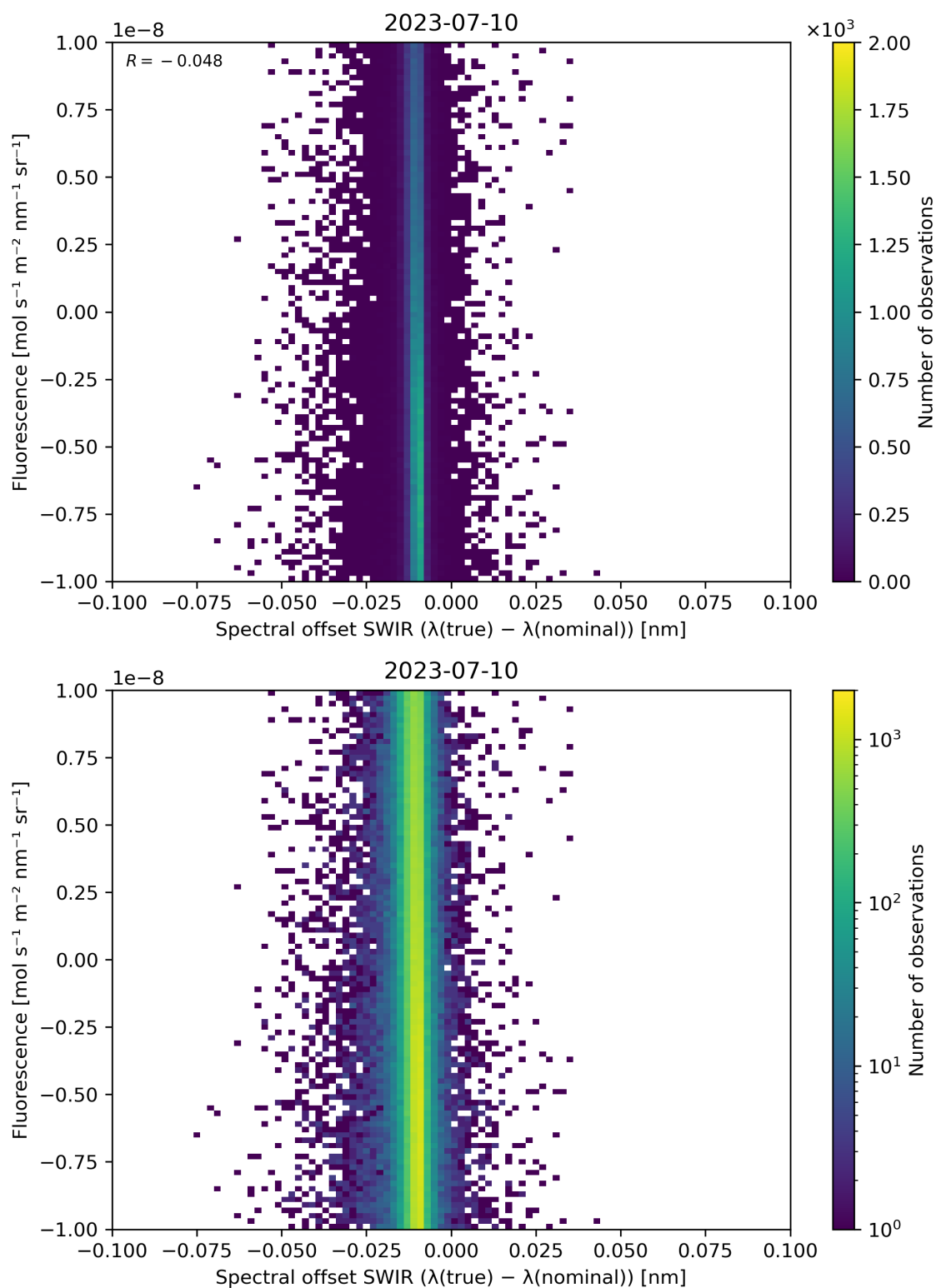
Figure 120: Scatter density plot of “Spectral offset SWIR ( \lambda(\text{true}) - \lambda(\text{nominal}) )” against “Fluorescence” for 2023-07-09 to 2023-07-11.
