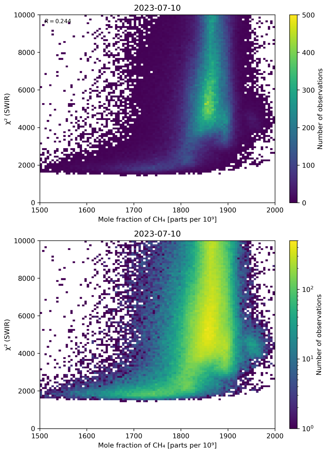
Figure 71: Scatter density plot of “Mole fraction of \text{CH}_4 ” against “ \chi^2 (SWIR)” for 2023-07-09 to 2023-07-11.
