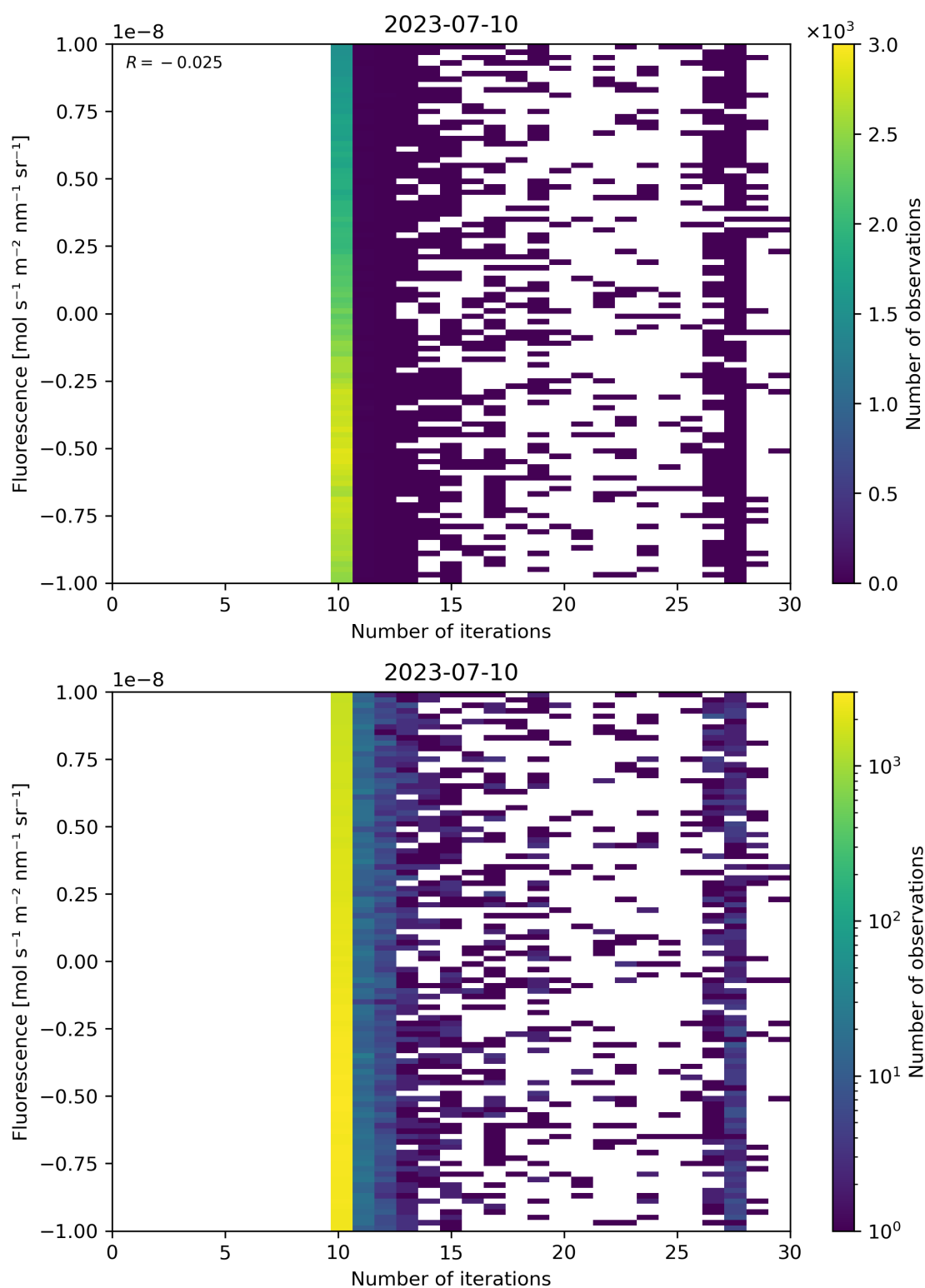
Figure 87: Scatter density plot of “Number of iterations” against “Fluorescence” for 2023-07-09 to 2023-07-11.
