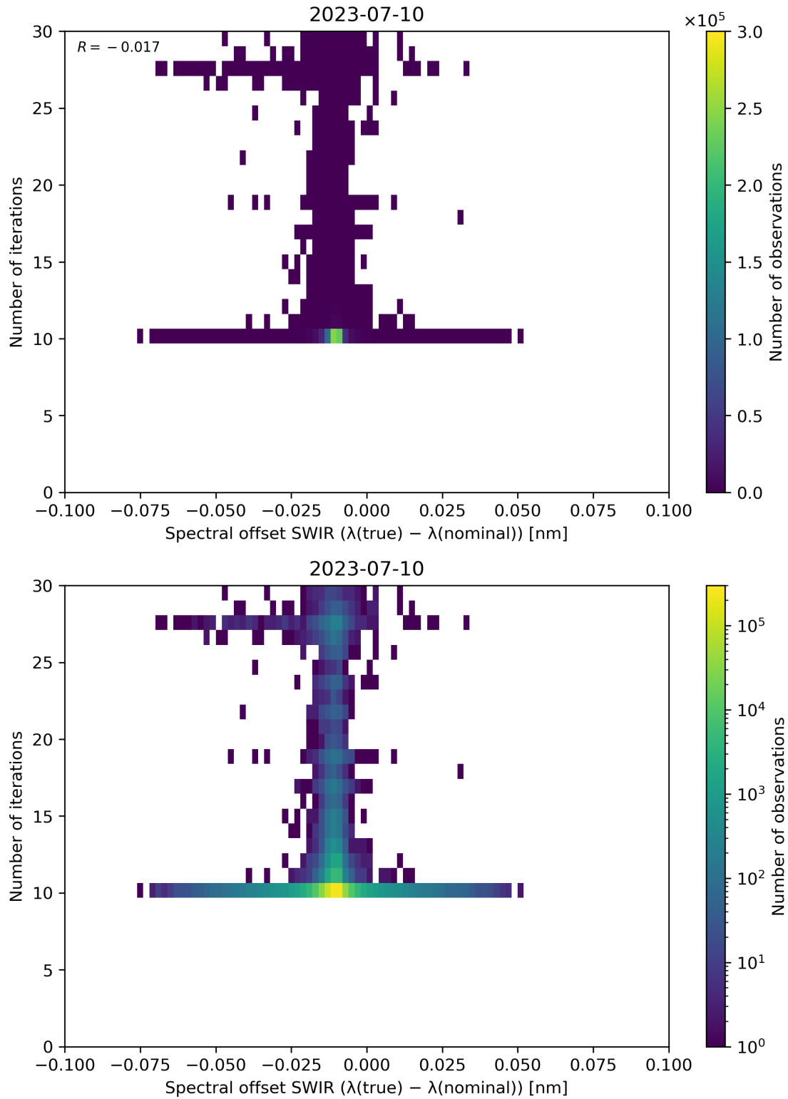
Figure 121: Scatter density plot of “Spectral offset SWIR ( \lambda(\text{true}) - \lambda(\text{nominal}) )” against “Number of iterations” for 2023-07-09 to 2023-07-11.
