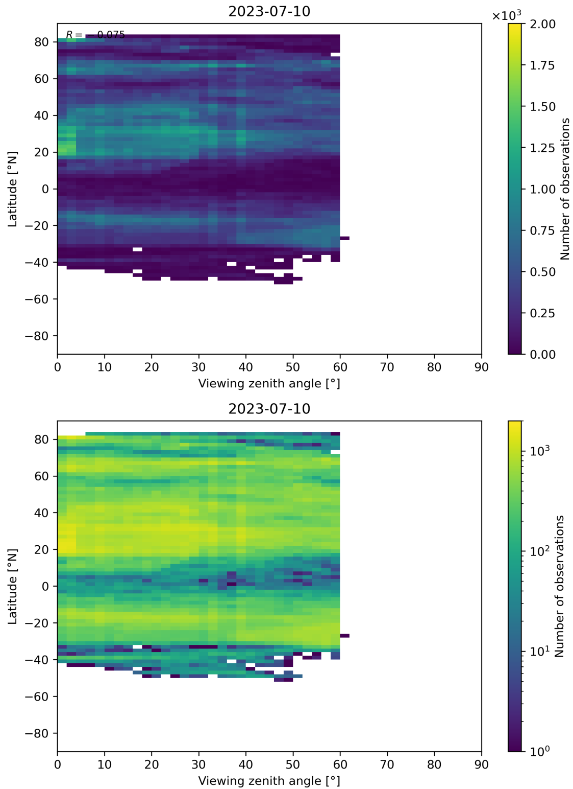
Figure 109: Scatter density plot of “Viewing zenith angle” against “Latitude” for 2023-07-09 to 2023-07-11.
