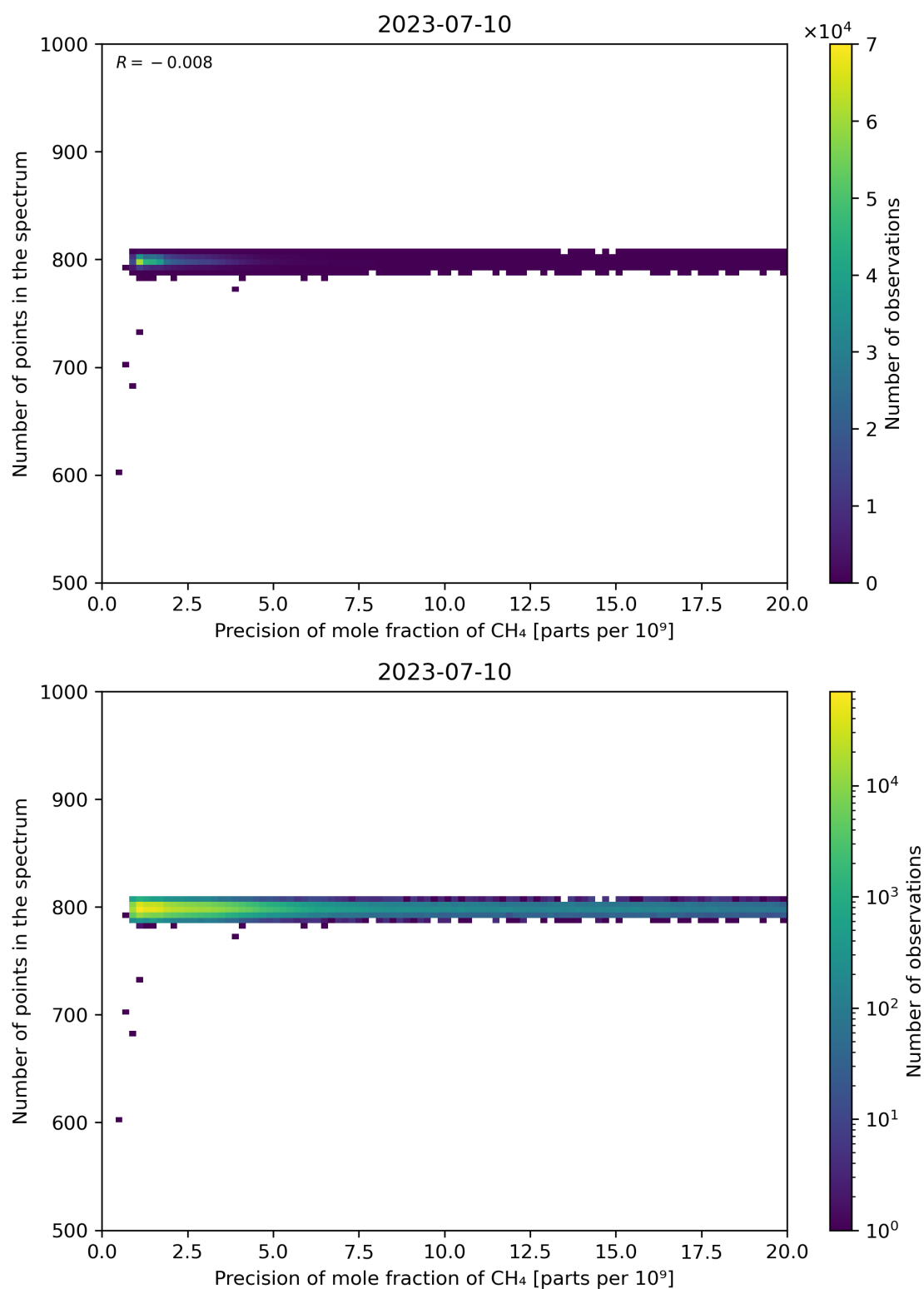
Figure 84: Scatter density plot of “Precision of mole fraction of CH 4 ” against “Number of points in the spectrum” for 2023-07-09 to 2023-07-11.
