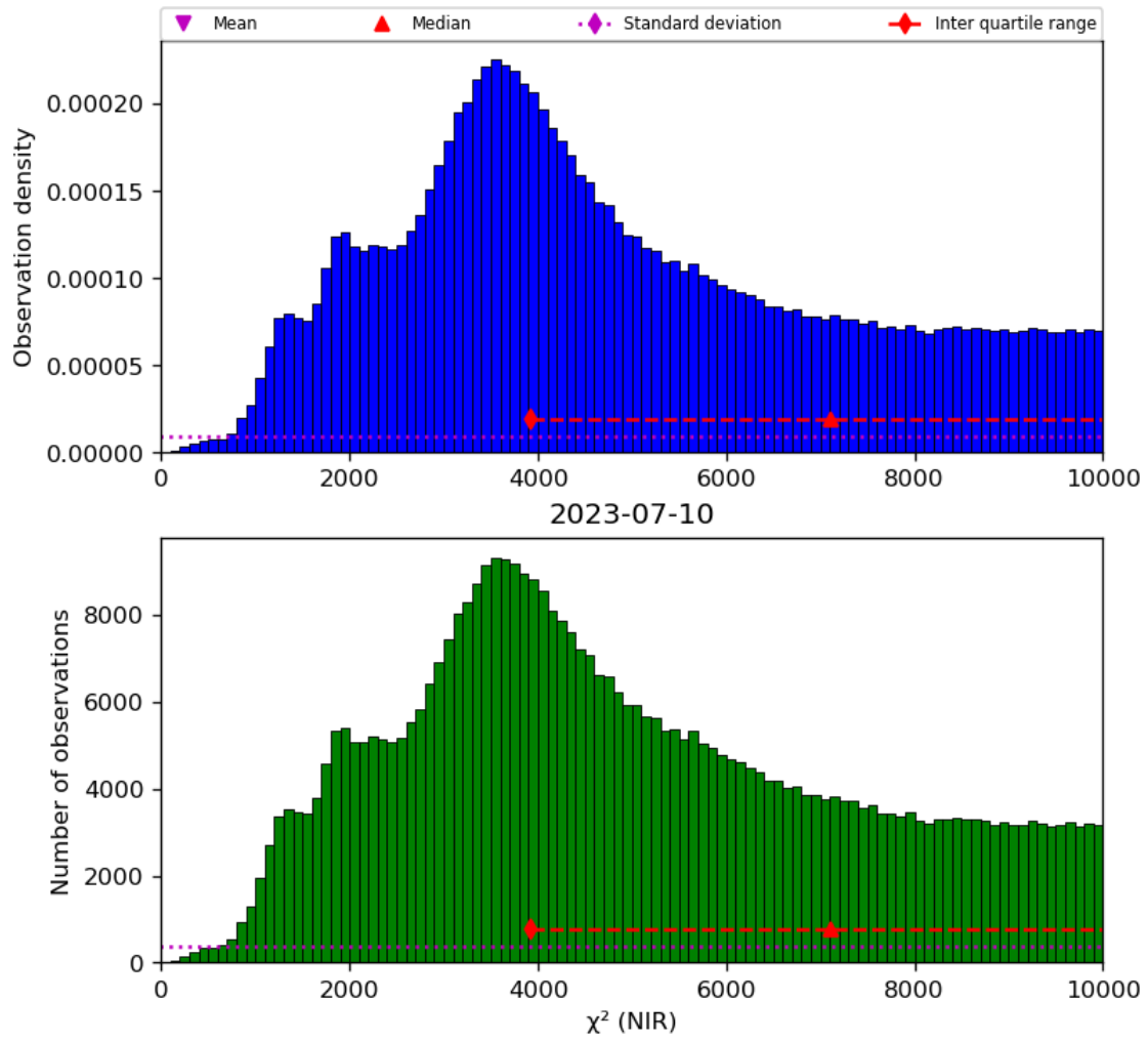
Figure 29: Histogram of “ \chi^2 (NIR)” for 2023-07-09 to 2023-07-11
