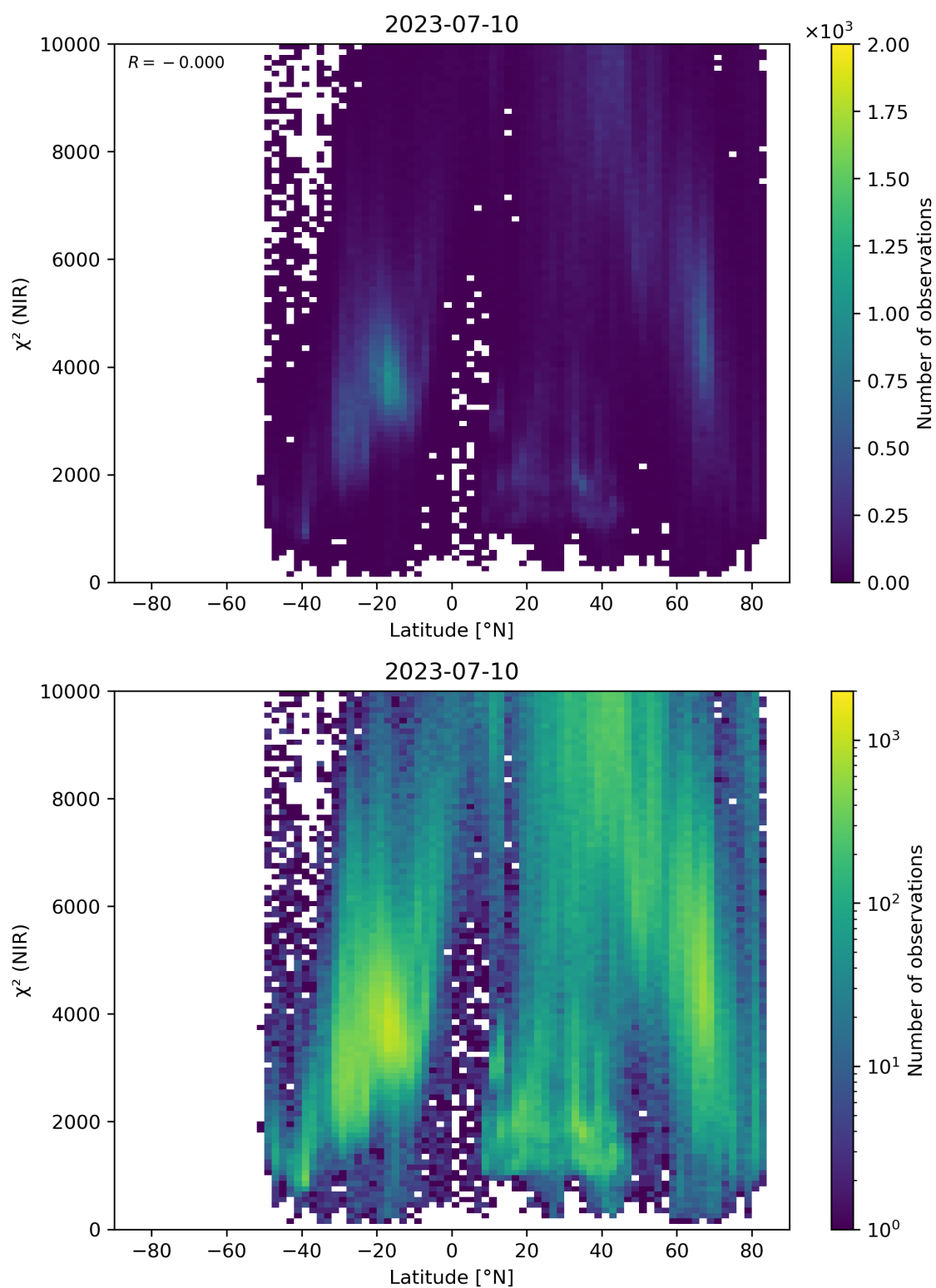
Figure 53: Scatter density plot of “Latitude” against “ \chi^2 (NIR)” for 2023-07-09 to 2023-07-11.
