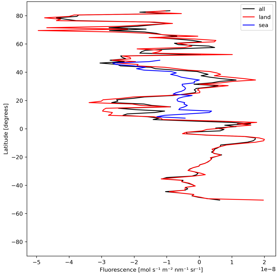
Figure 21: Zonal average of “Fluorescence” for 2023-07-09 to 2023-07-11.
