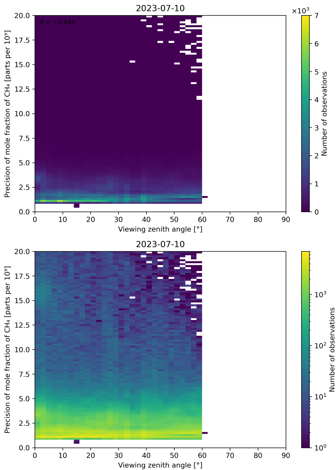
Figure 112: Scatter density plot of “Viewing zenith angle” against “Precision of mole fraction of CH 4 ” for 2023-07-09 to 2023-07-11.
