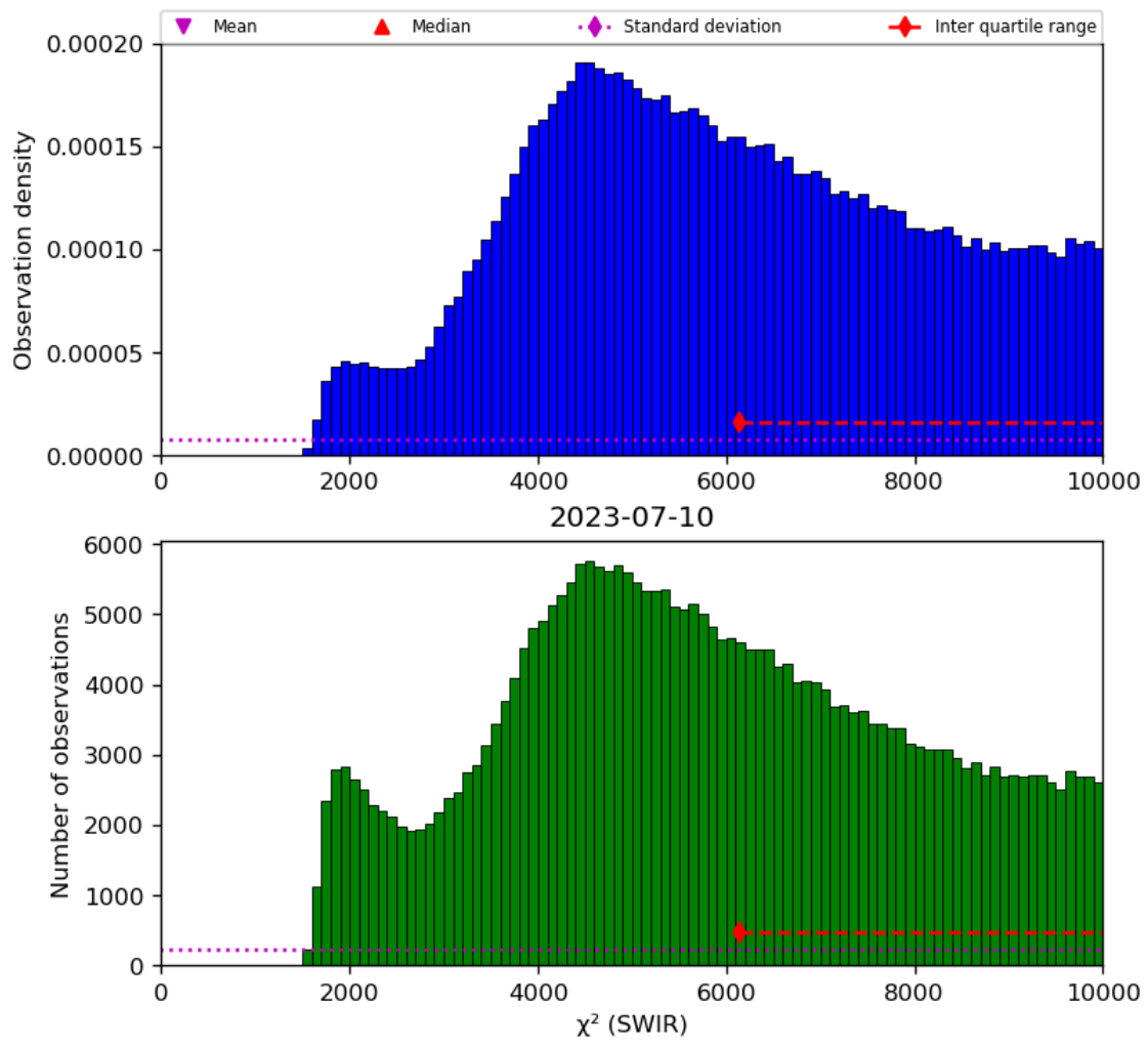
Figure 28: Histogram of “ \chi^2 (SWIR)” for 2023-07-09 to 2023-07-11
