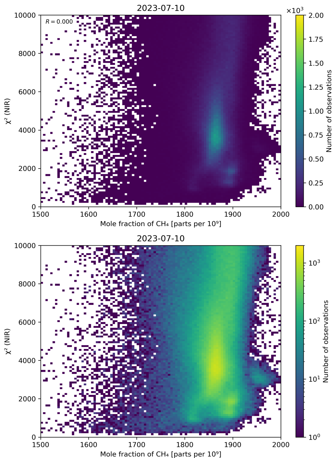
Figure 70: Scatter density plot of “Mole fraction of CH 4 ” against “ \chi^2 (NIR)” for 2023-07-09 to 2023-07-11.
