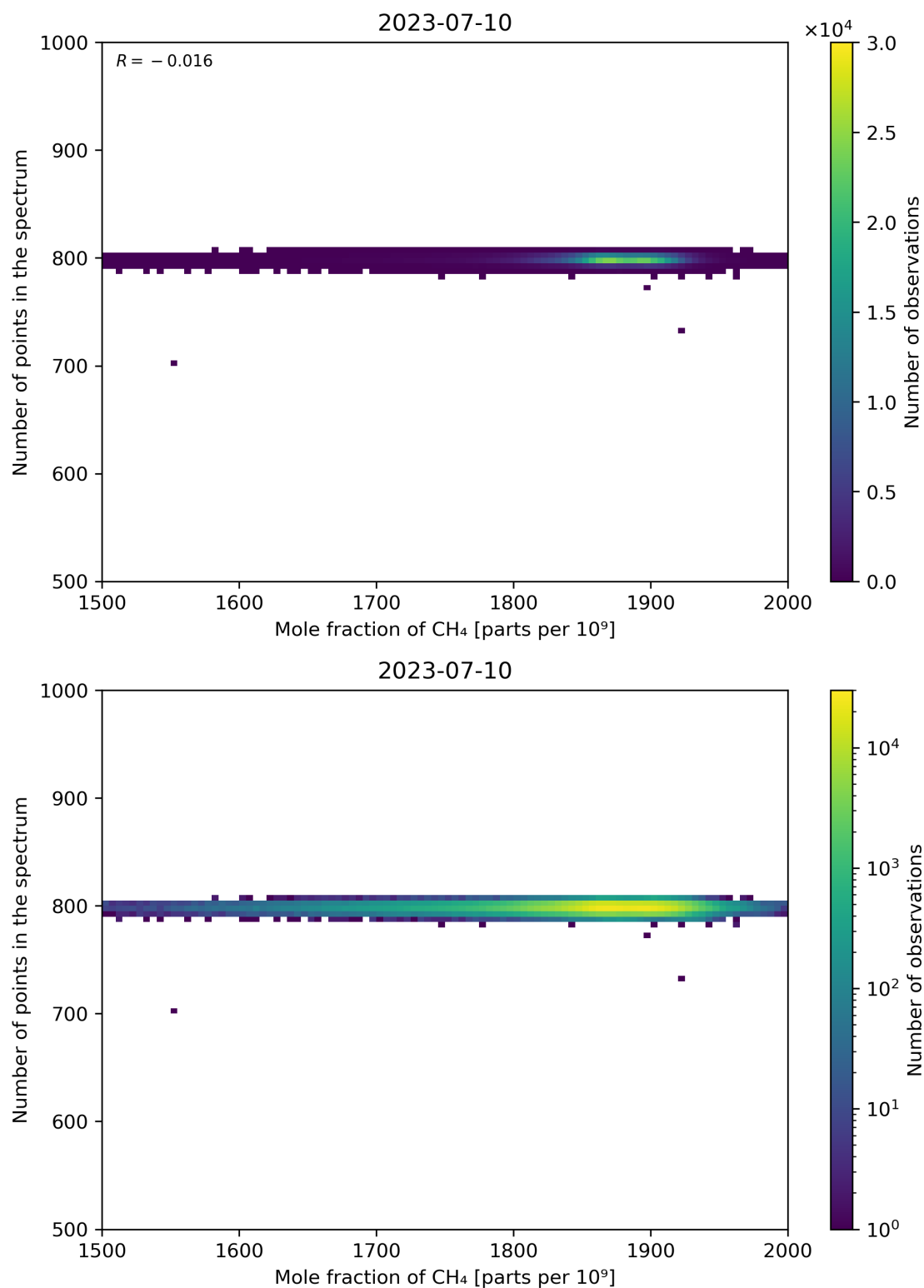
Figure 77: Scatter density plot of “Mole fraction of CH 4 ” against “Number of points in the spectrum” for 2023-07-09 to 2023-07-11.
