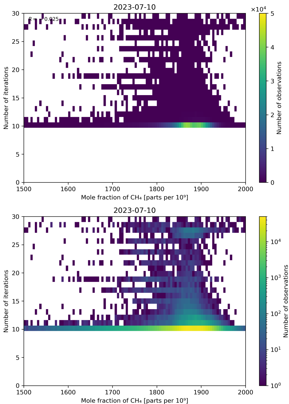
Figure 76: Scatter density plot of “Mole fraction of CH 4 ” against “Number of iterations” for 2023-07-09 to 2023-07-11.
