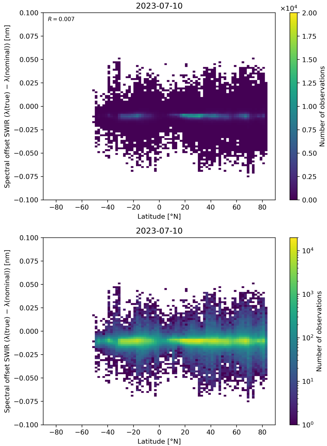
Figure 62: Scatter density plot of “Latitude” against “Spectral offset SWIR ( \lambda(\text{true}) - \lambda(\text{nominal}) )” for 2023-07-09 to 2023-07-11.
