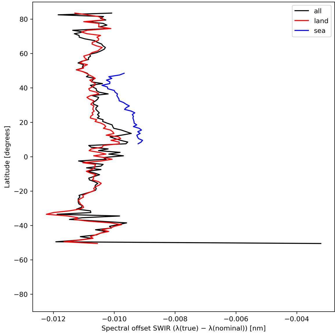
Figure 16: Zonal average of “Spectral offset SWIR ( \lambda(\text{true}) - \lambda(\text{nominal}) )” for 2023-07-09 to 2023-07-11.
