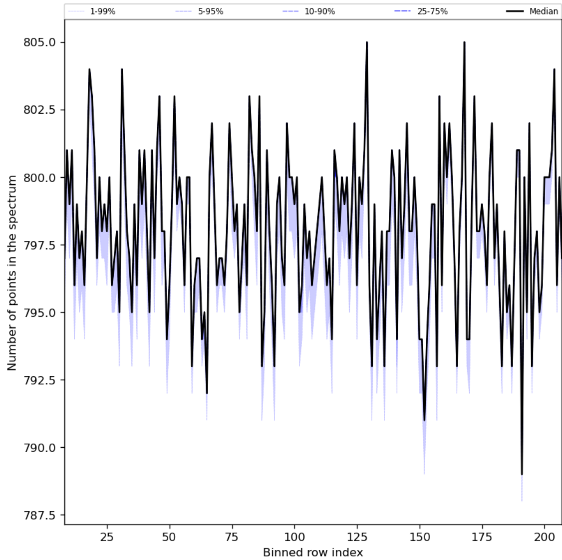
Figure 37: Along track statistics of “Number of points in the spectrum” for 2023-07-09 to 2023-07-11
