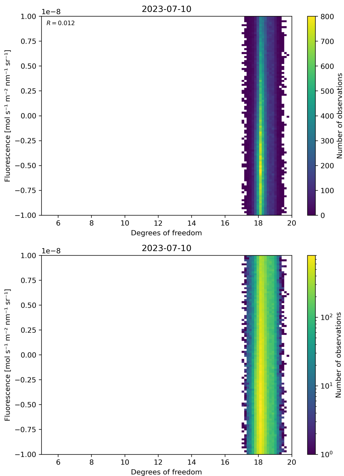
Figure 51: Scatter density plot of “Degrees of freedom” against “Fluorescence” for 2023-07-09 to 2023-07-11.
