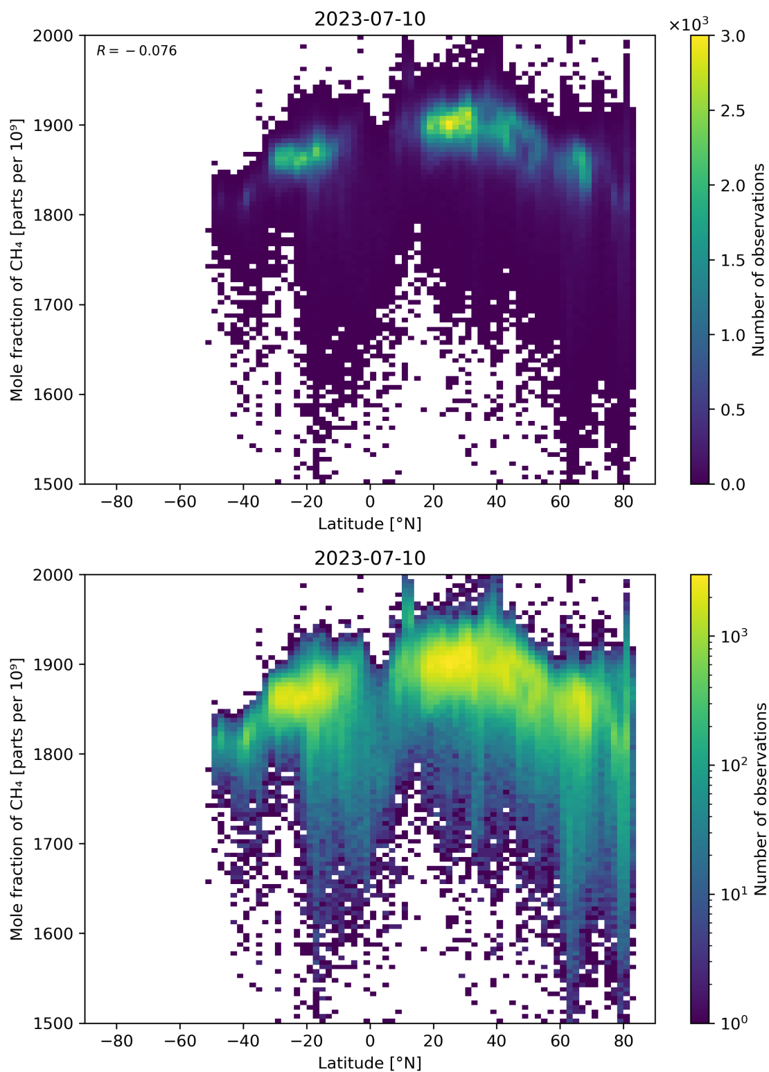
Figure 57: Scatter density plot of “Latitude” against “Mole fraction of CH 4 ” for 2023-07-09 to 2023-07-11.
