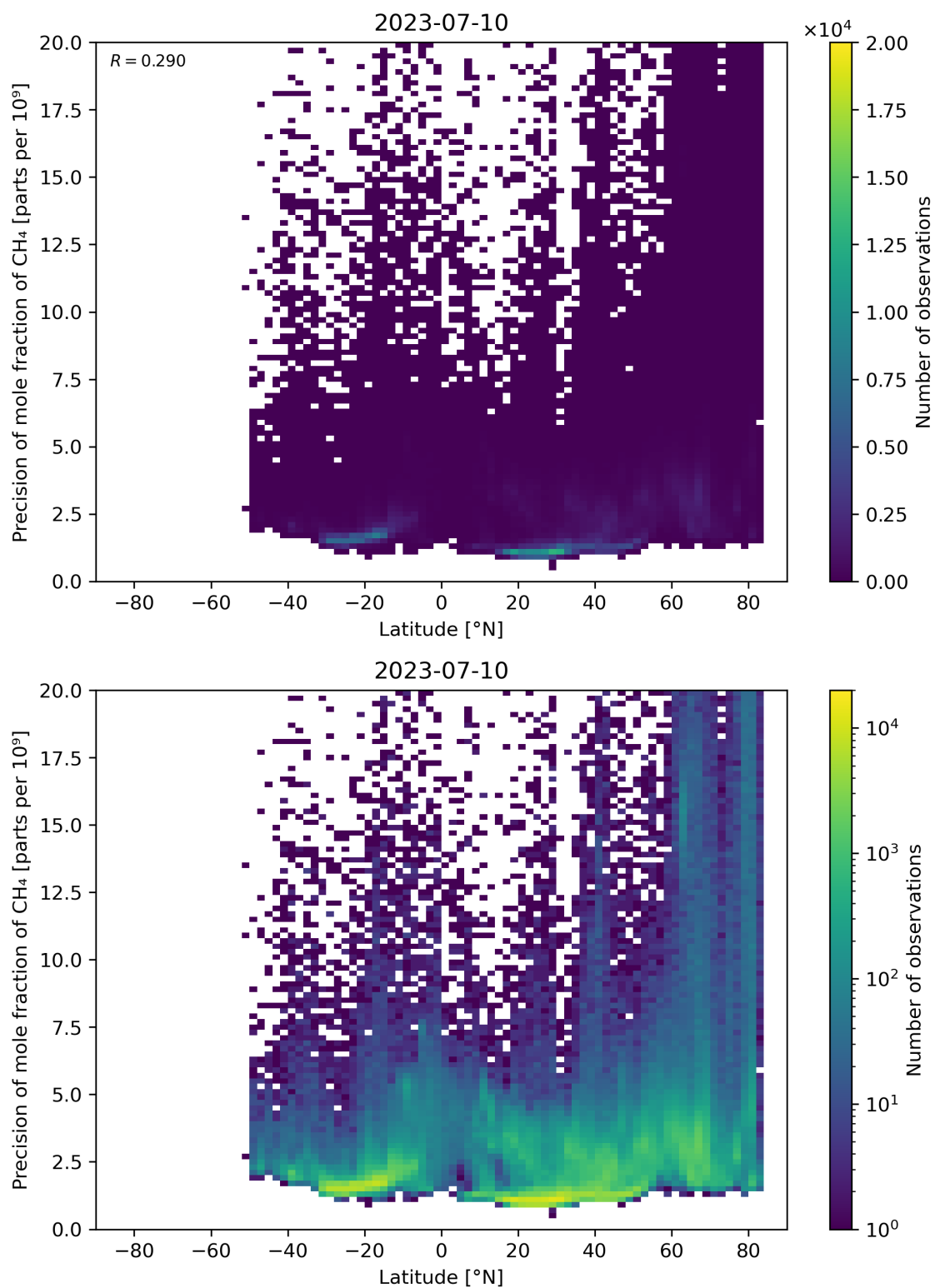
Figure 59: Scatter density plot of “Latitude” against “Precision of mole fraction of CH 4 ” for 2023-07-09 to 2023-07-11.
