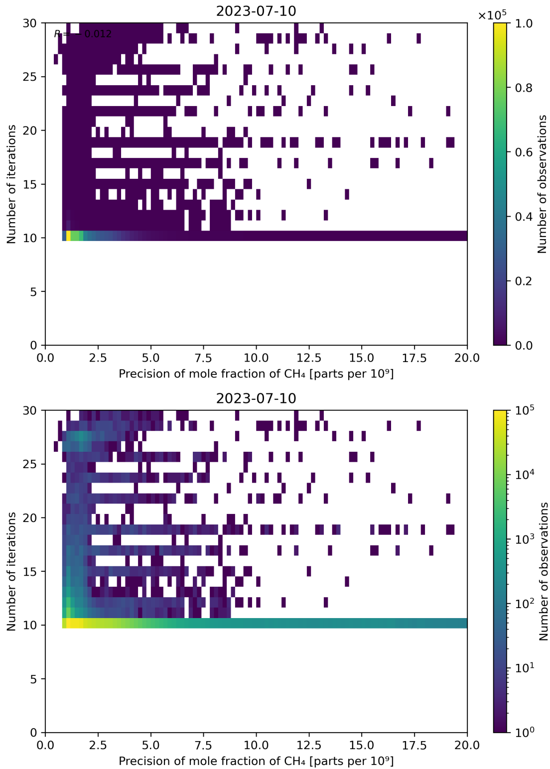
Figure 83: Scatter density plot of “Precision of mole fraction of CH 4 ” against “Number of iterations” for 2023-07-09 to 2023-07-11.
