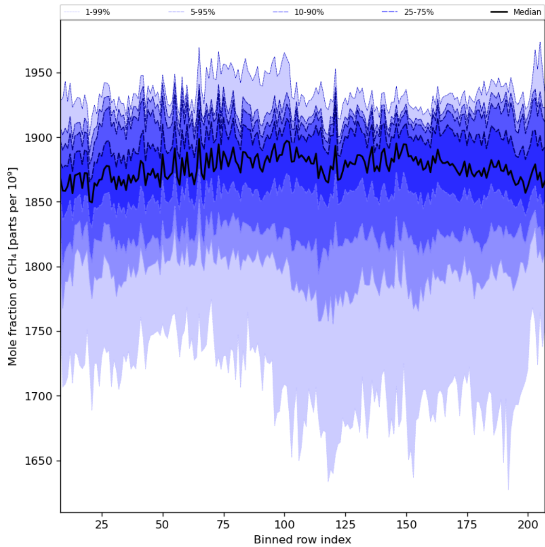
Figure 34: Along track statistics of “Mole fraction of CH 4 ” for 2023-07-09 to 2023-07-11
