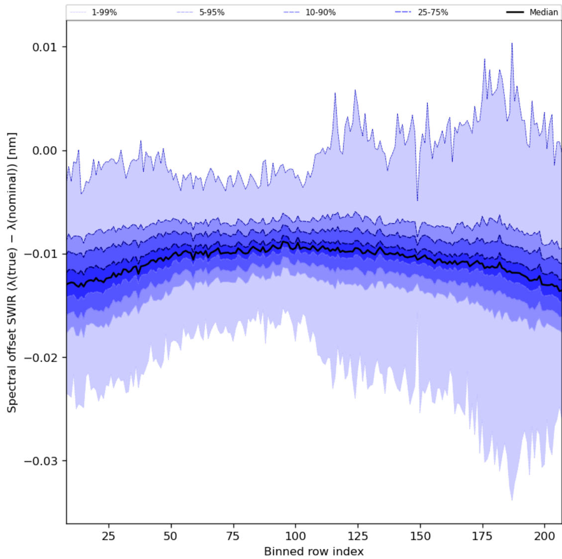
Figure 38: Along track statistics of “Spectral offset SWIR ( \lambda(\text{true}) - \lambda(\text{nominal}) )” for 2023-07-09 to 2023-07-11
