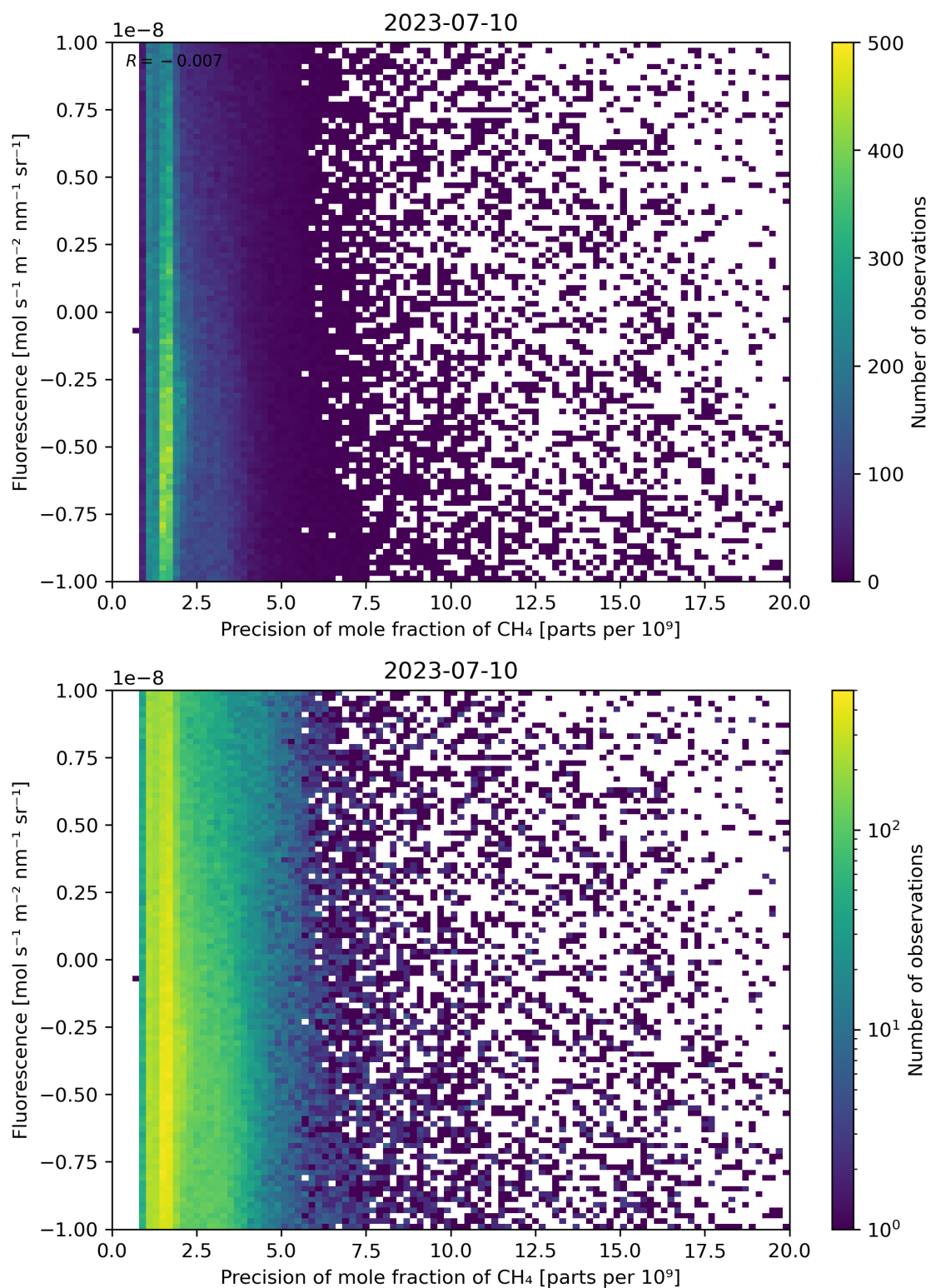
Figure 81: Scatter density plot of “Precision of mole fraction of \text{CH}_4 ” against “Fluorescence” for 2023-07-09 to 2023-07-11.
