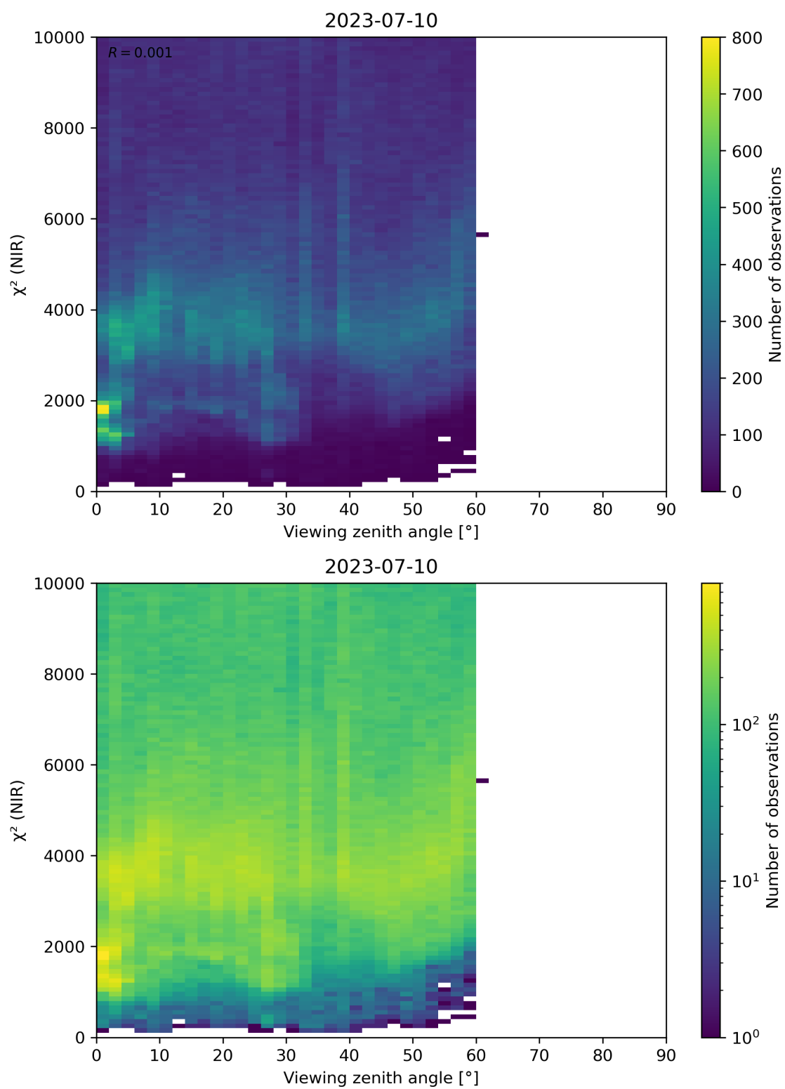
Figure 105: Scatter density plot of “Viewing zenith angle” against “ \chi^2 (NIR)” for 2023-07-09 to 2023-07-11.
