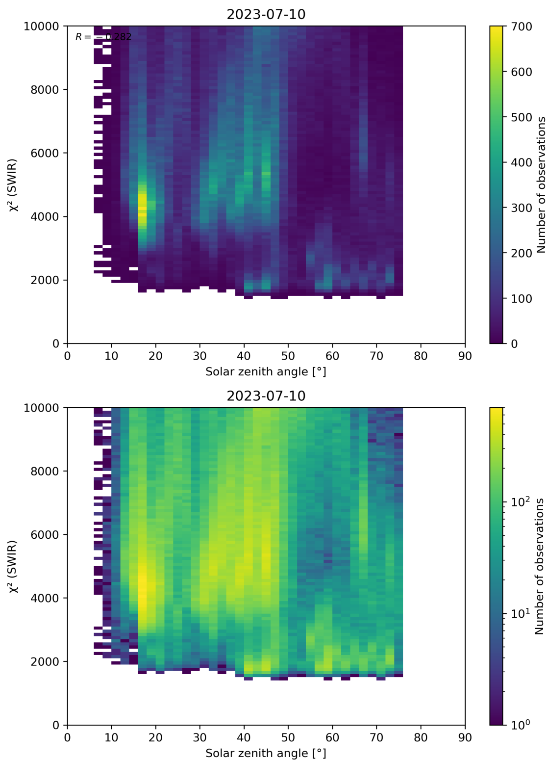
Figure 95: Scatter density plot of “Solar zenith angle” against “ \chi^2 (SWIR)” for 2023-07-09 to 2023-07-11.
