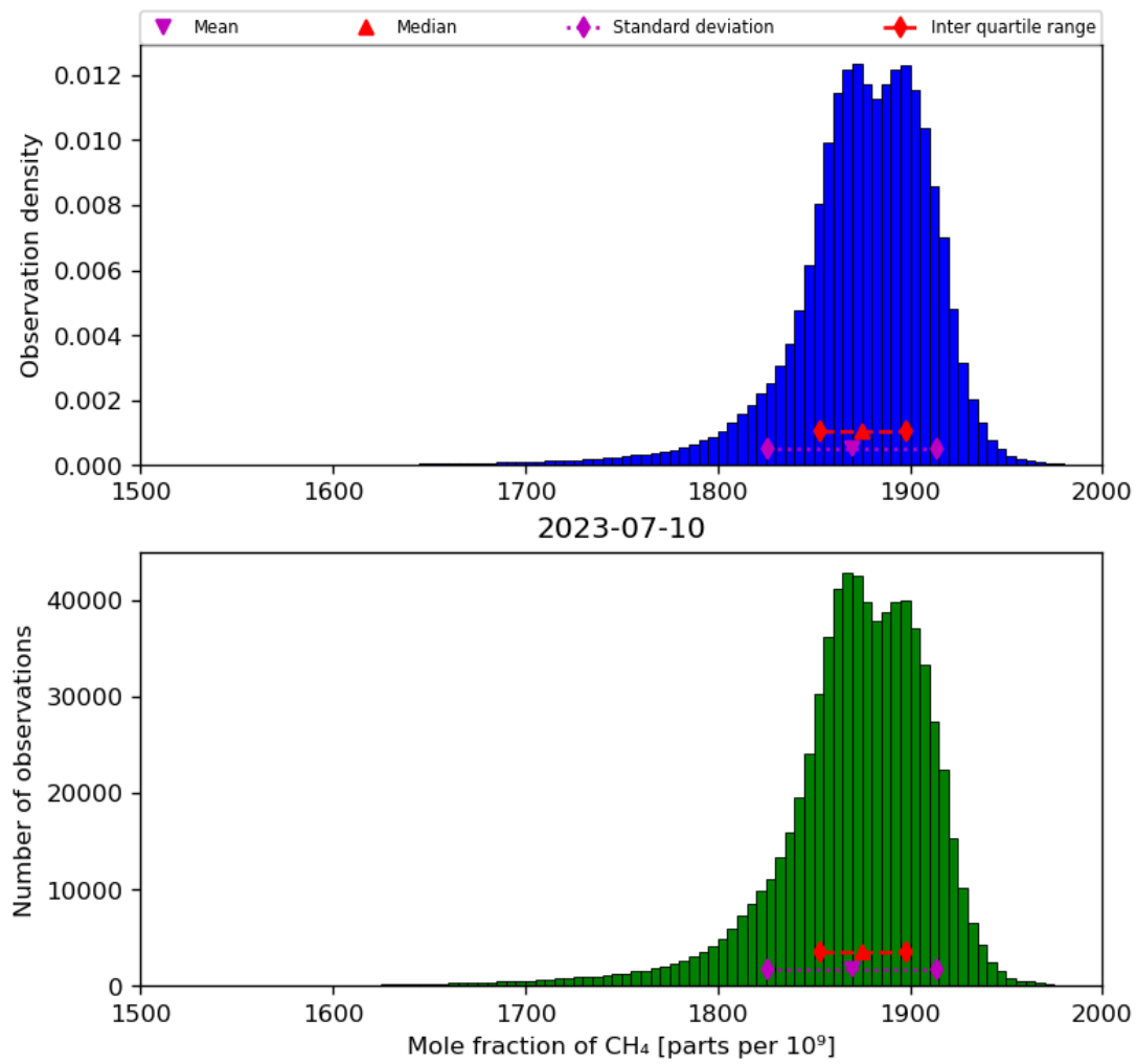
Figure 23: Histogram of “Mole fraction of CH 4 ” for 2023-07-09 to 2023-07-11
