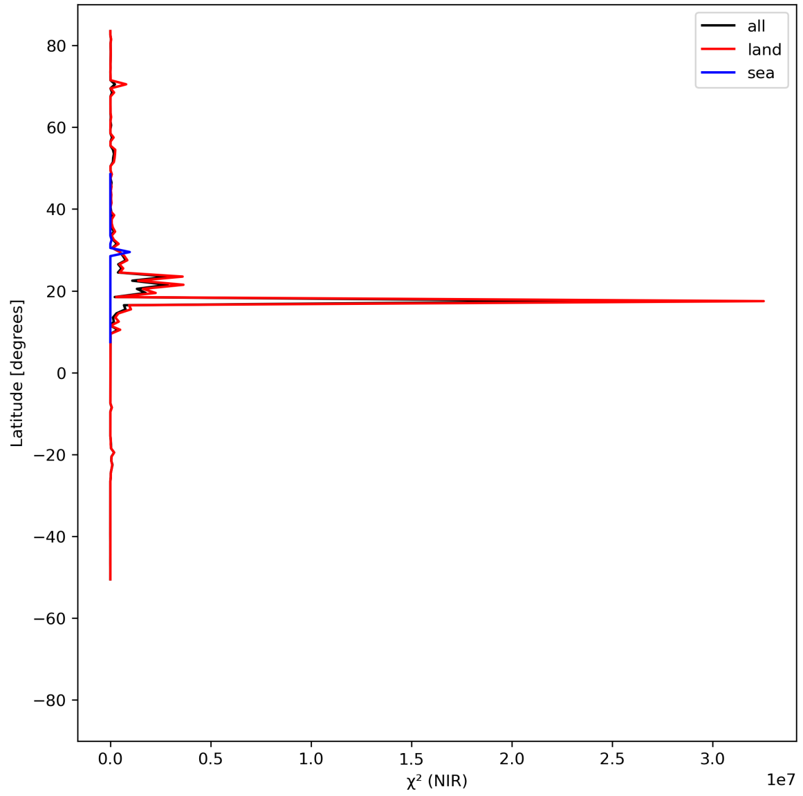
Figure 18: Zonal average of “ \chi^2 (NIR)” for 2023-07-09 to 2023-07-11.
