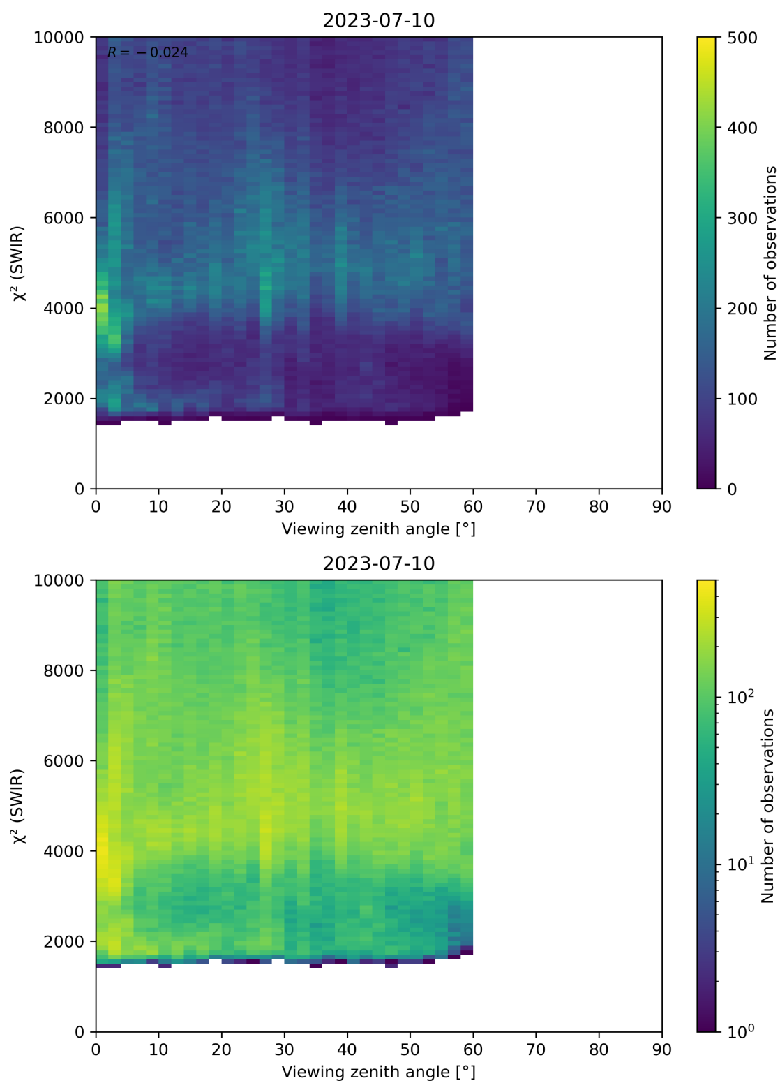
Figure 106: Scatter density plot of “Viewing zenith angle” against “ \chi^2 (SWIR)” for 2023-07-09 to 2023-07-11.
