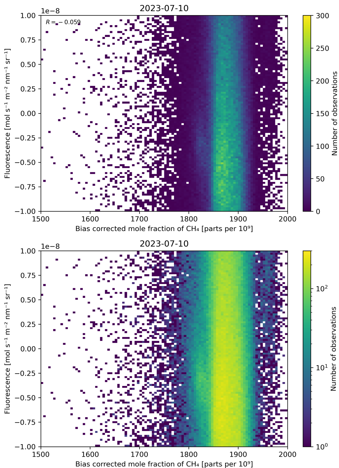
Figure 66: Scatter density plot of “Bias corrected mole fraction of \text{CH}_4 ” against “Fluorescence” for 2023-07-09 to 2023-07-11.
