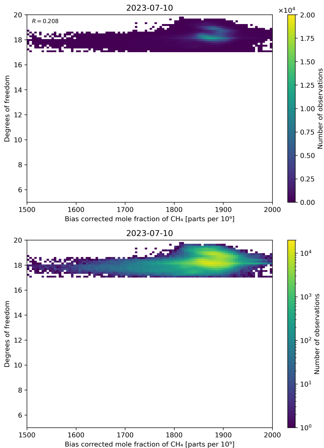
Figure 65: Scatter density plot of “Bias corrected mole fraction of CH 4 ” against “Degrees of freedom” for 2023-07-09 to 2023-07-11.
