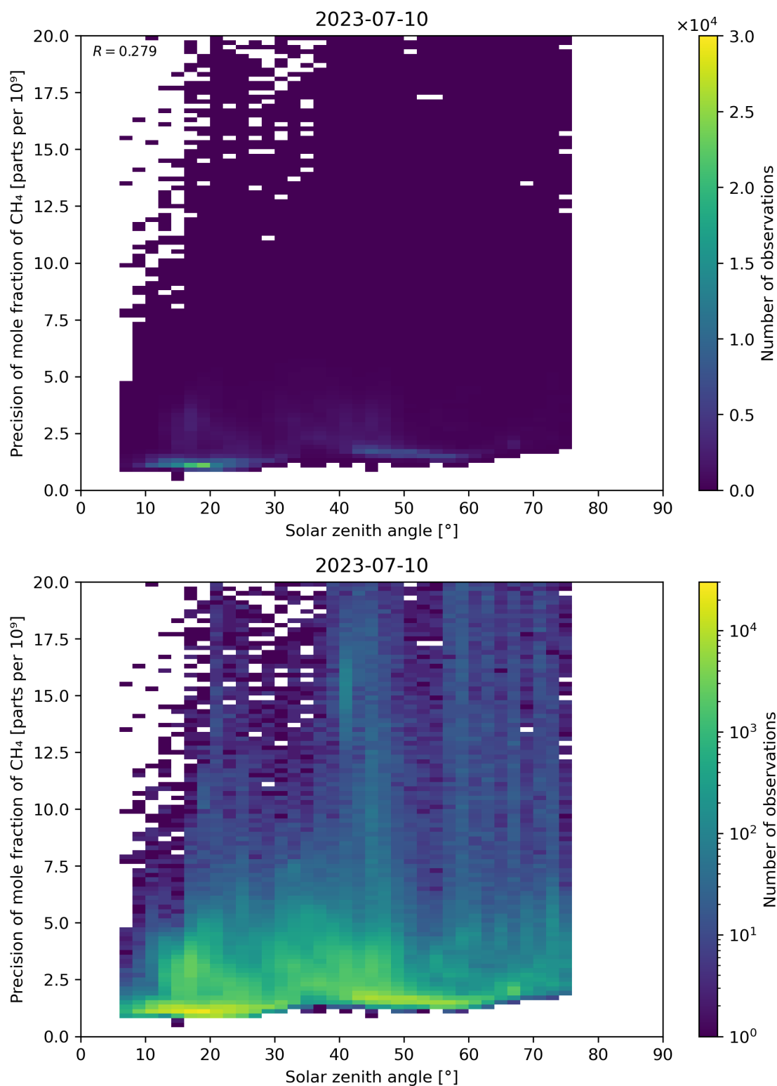
Figure 101: Scatter density plot of “Solar zenith angle” against “Precision of mole fraction of CH 4 ” for 2023-07-09 to 2023-07-11.
