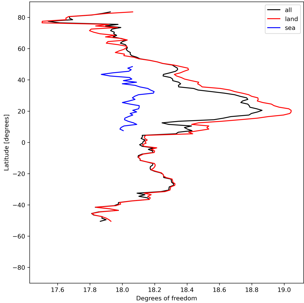
Figure 19: Zonal average of “Degrees of freedom” for 2023-07-09 to 2023-07-11.
