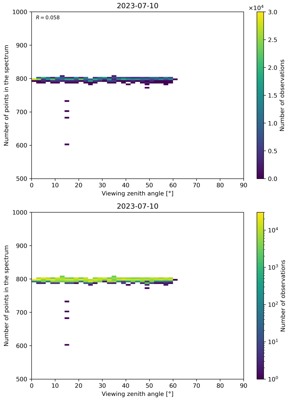
Figure 114: Scatter density plot of “Viewing zenith angle” against “Number of points in the spectrum” for 2023-07-09 to 2023-07-11.
