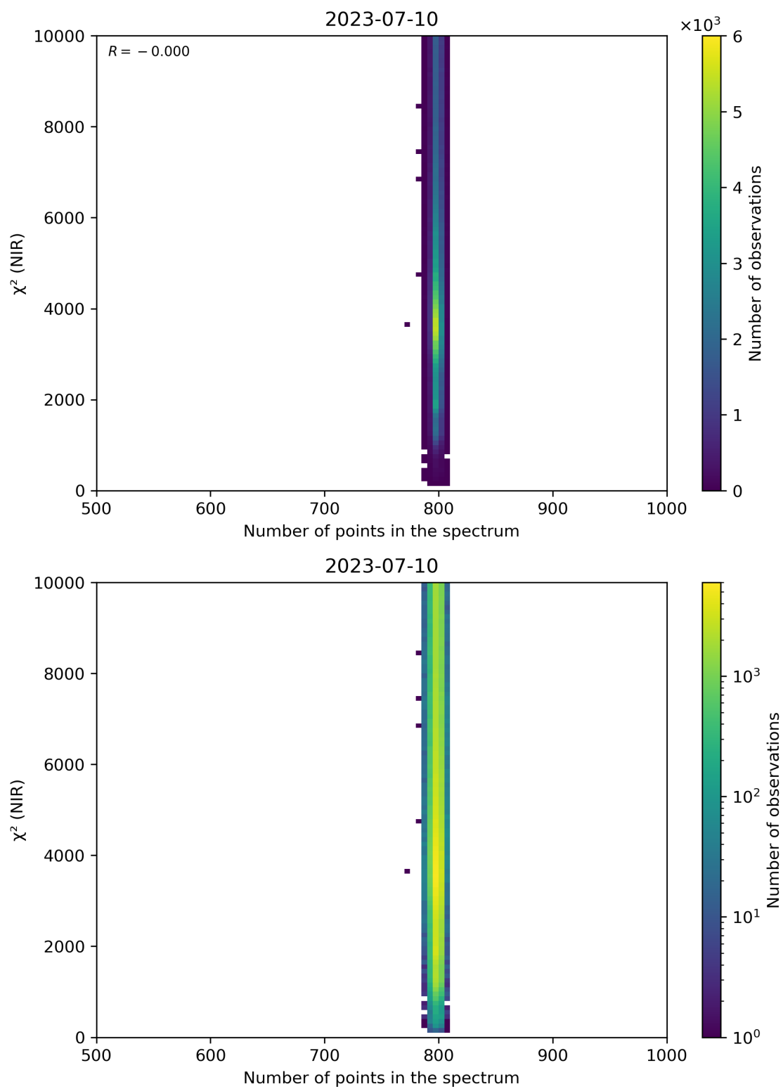
Figure 88: Scatter density plot of “Number of points in the spectrum” against “ \chi^2 (NIR)” for 2023-07-09 to 2023-07-11.
