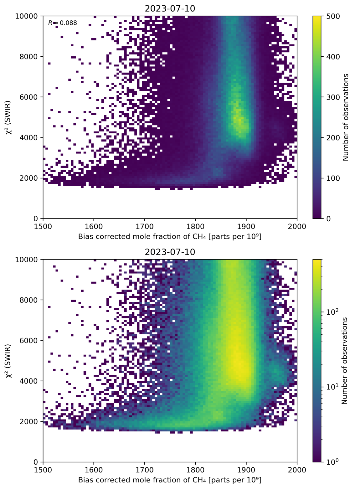
Figure 64: Scatter density plot of “Bias corrected mole fraction of CH 4 ” against “ \chi^2 (SWIR)” for 2023-07-09 to 2023-07-11.
