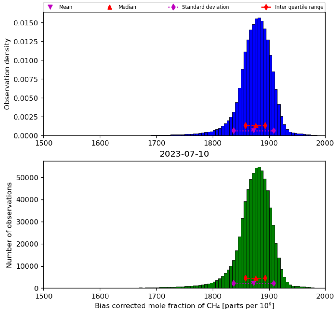
Figure 25: Histogram of “Bias corrected mole fraction of CH 4 ” for 2023-07-09 to 2023-07-11
