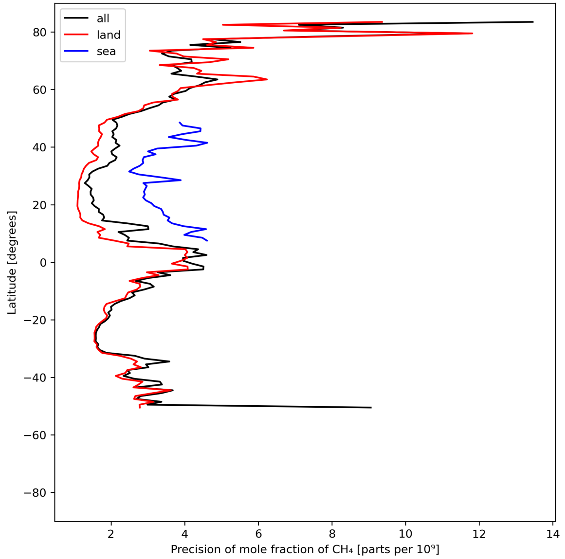
Figure 13: Zonal average of “Precision of mole fraction of \text{CH}_4 ” for 2023-07-09 to 2023-07-11.
