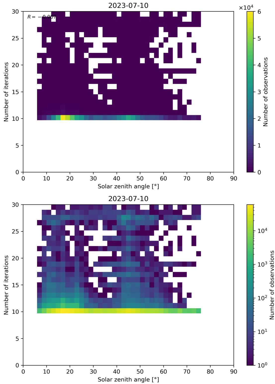
Figure 102: Scatter density plot of “Solar zenith angle” against “Number of iterations” for 2023-07-09 to 2023-07-11.
