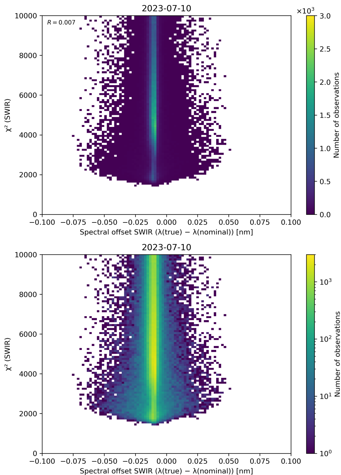
Figure 118: Scatter density plot of “Spectral offset SWIR ( \lambda(\text{true}) - \lambda(\text{nominal}) )” against “ \chi^2 (SWIR)” for 2023-07-09 to 2023-07-11.
