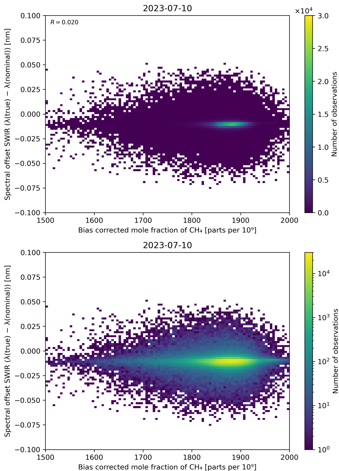
Figure 69: Scatter density plot of “Bias corrected mole fraction of \text{CH}_4 ” against “Spectral offset SWIR ( \lambda(\text{true}) - \lambda(\text{nominal}) )” for 2023-07-09 to 2023-07-11.
