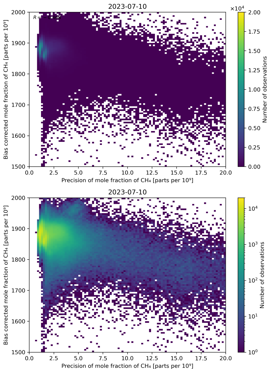
Figure 82: Scatter density plot of “Precision of mole fraction of CH 4 ” against “Bias corrected mole fraction of CH 4 ” for 2023-07-09 to 2023-07-11.
