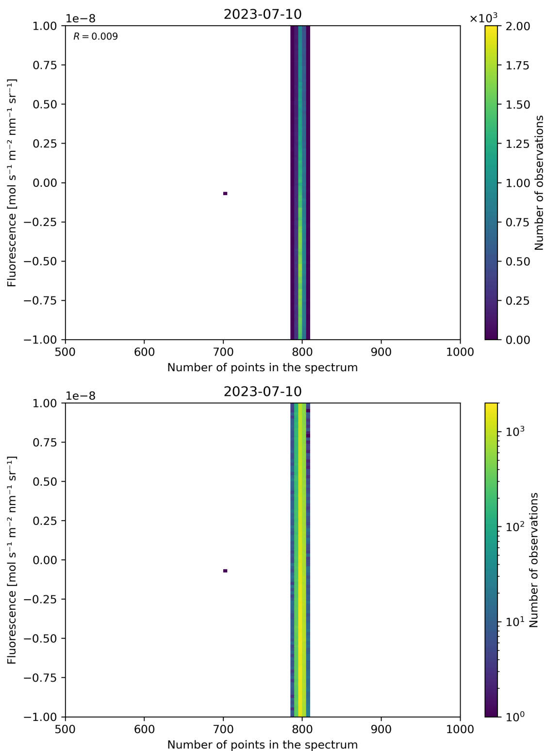
Figure 91: Scatter density plot of “Number of points in the spectrum” against “Fluorescence” for 2023-07-09 to 2023-07-11.
