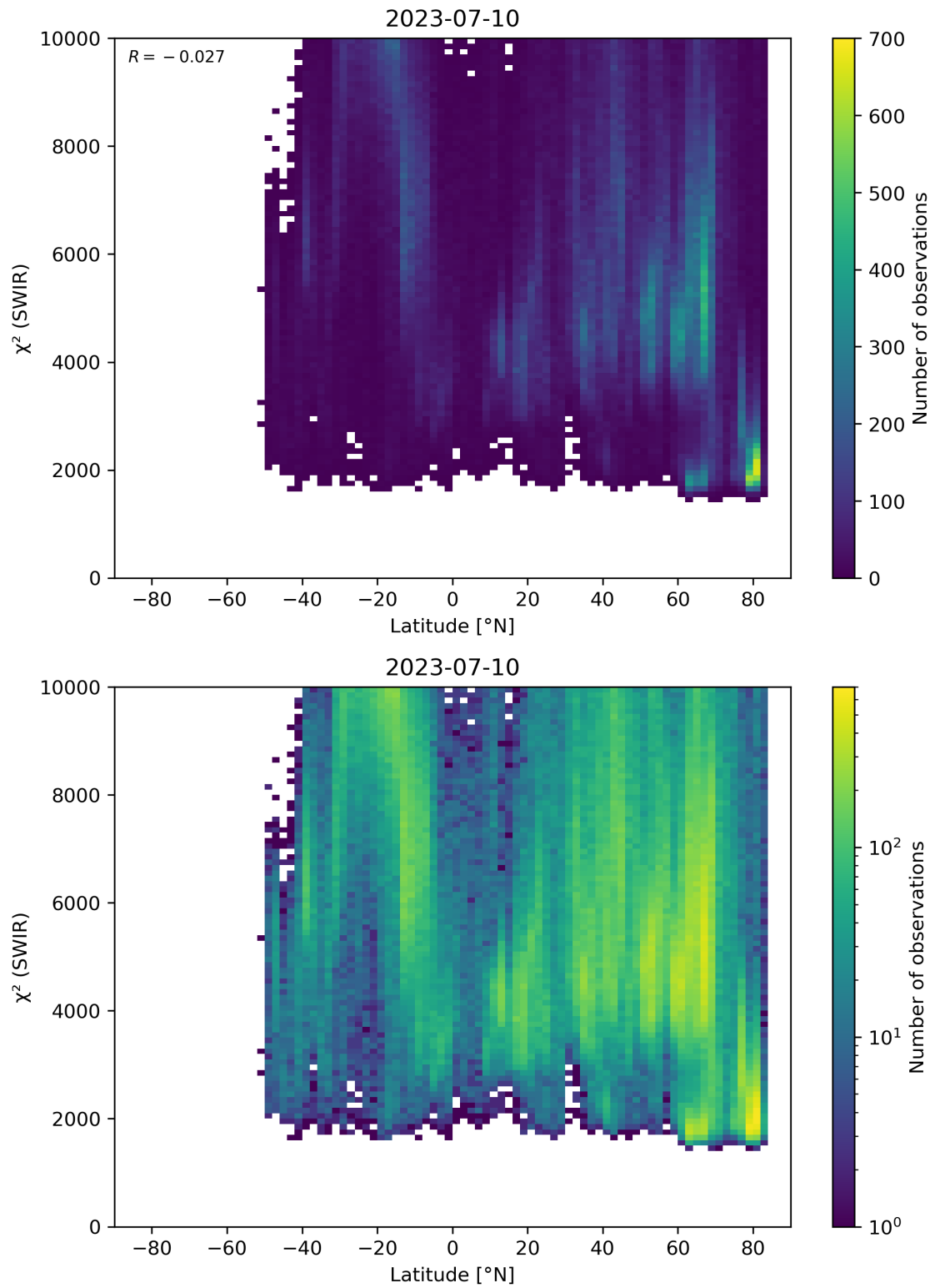
Figure 54: Scatter density plot of “Latitude” against “ \chi^2 (SWIR)” for 2023-07-09 to 2023-07-11.
