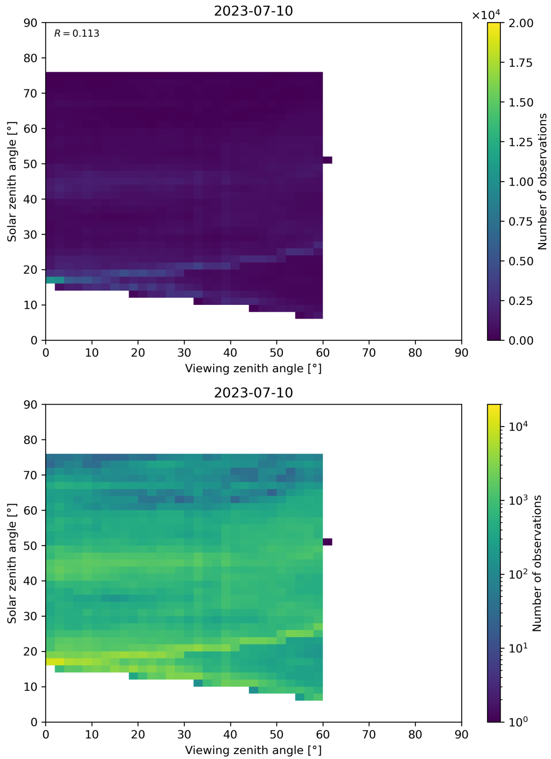
Figure 115: Scatter density plot of “Viewing zenith angle” against “Solar zenith angle” for 2023-07-09 to 2023-07-11.
