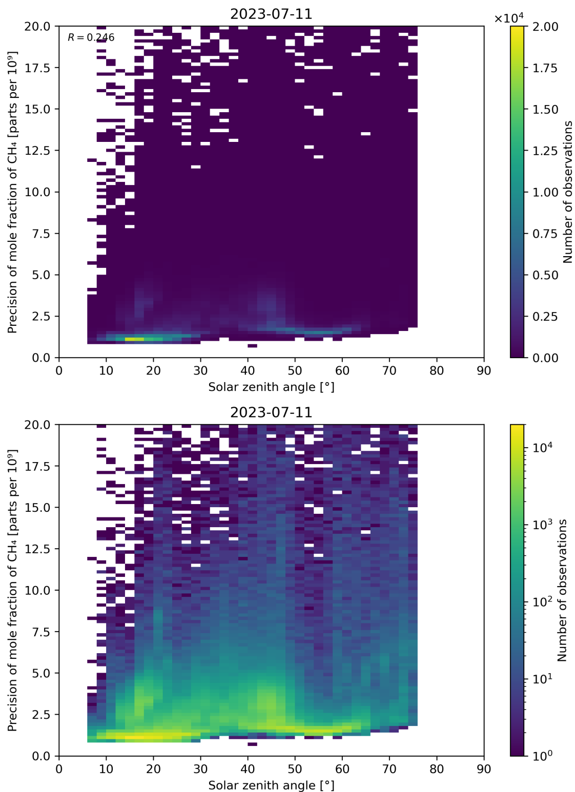
Figure 101: Scatter density plot of “Solar zenith angle” against “Precision of mole fraction of CH 4 ” for 2023-07-10 to 2023-07-12.
