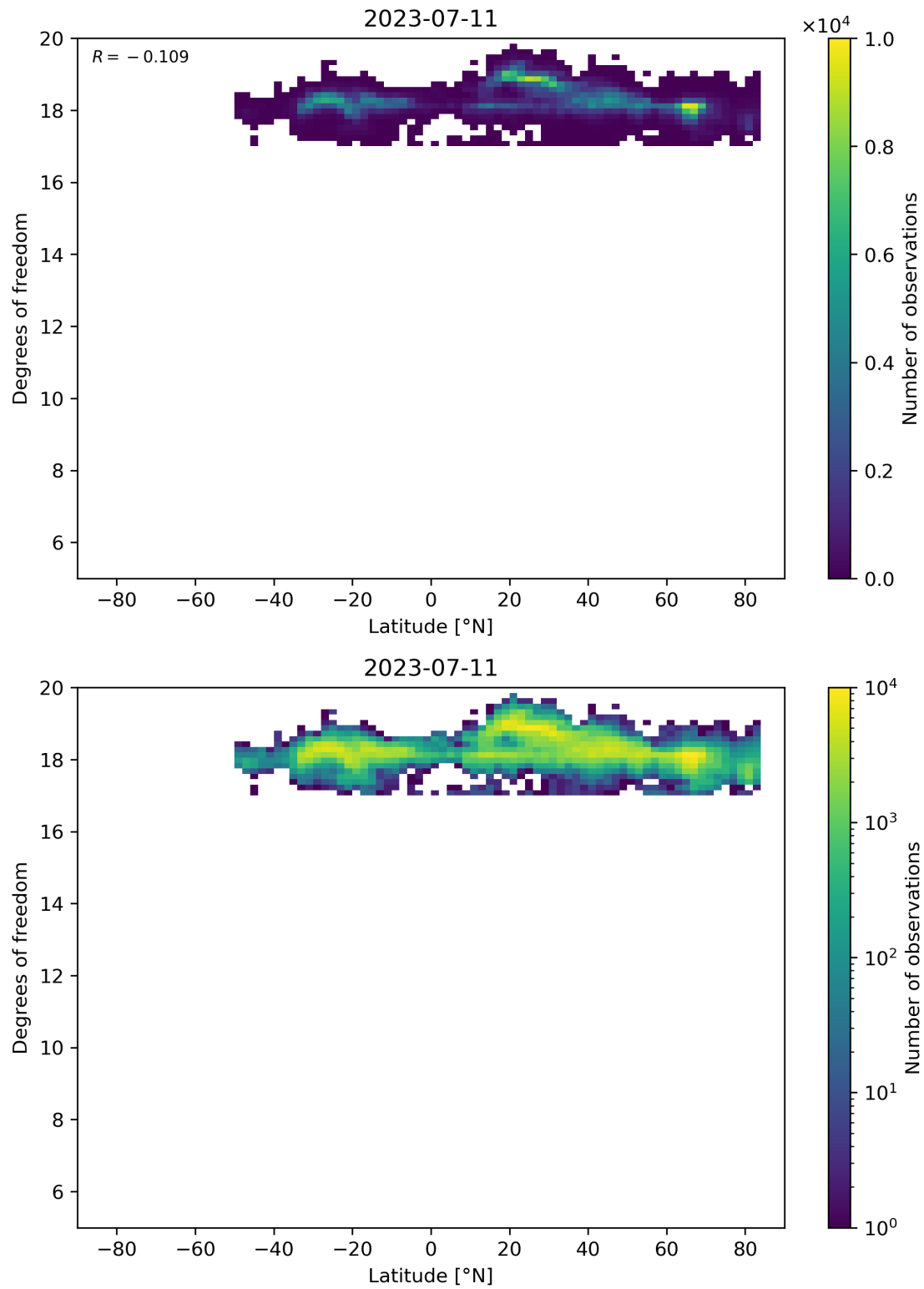
Figure 55: Scatter density plot of “Latitude” against “Degrees of freedom” for 2023-07-10 to 2023-07-12.
