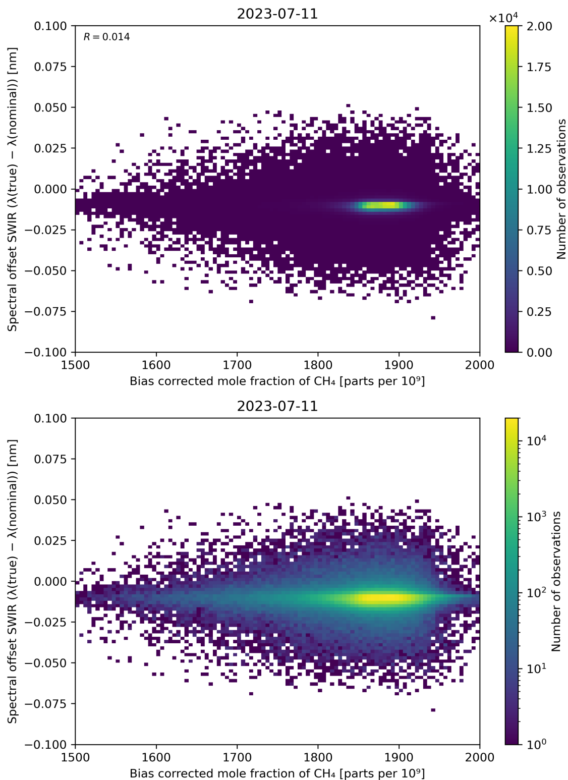
Figure 69: Scatter density plot of “Bias corrected mole fraction of \text{CH}_4 ” against “Spectral offset SWIR ( \lambda(\text{true}) - \lambda(\text{nominal}) )” for 2023-07-10 to 2023-07-12.
