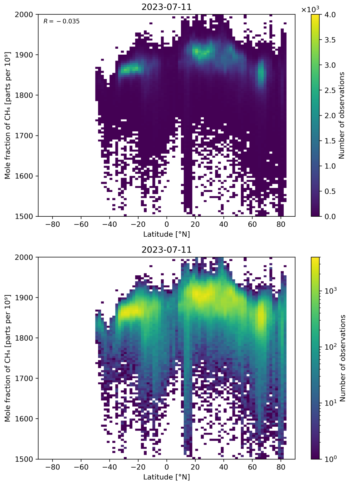
Figure 57: Scatter density plot of “Latitude” against “Mole fraction of CH 4 ” for 2023-07-10 to 2023-07-12.
