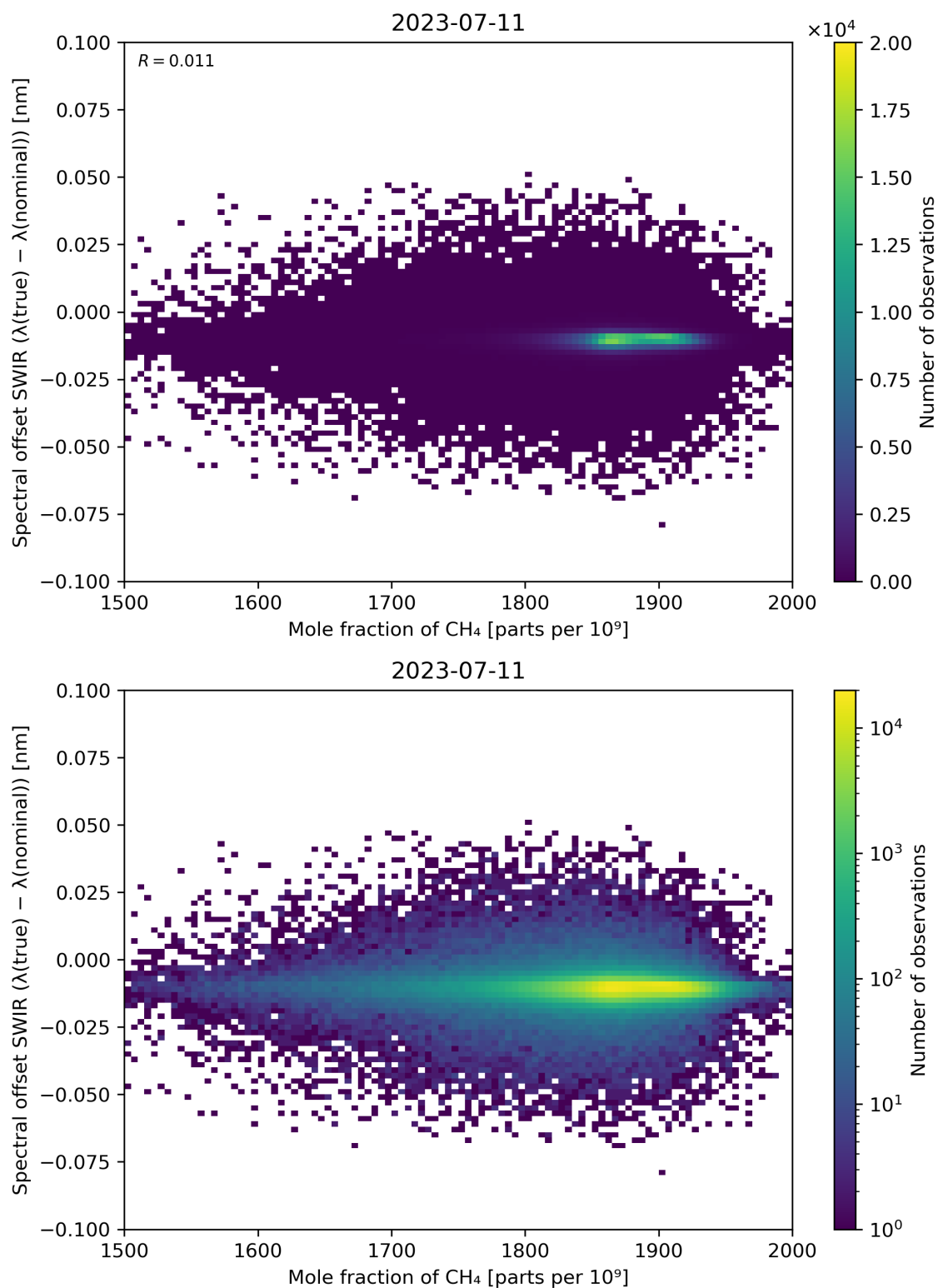
Figure 86: Scatter density plot of “Mole fraction of CH 4 ” against “Spectral offset SWIR ( \lambda(\text{true}) - \lambda(\text{nominal}) )” for 2023-07-10 to 2023-07-12.
