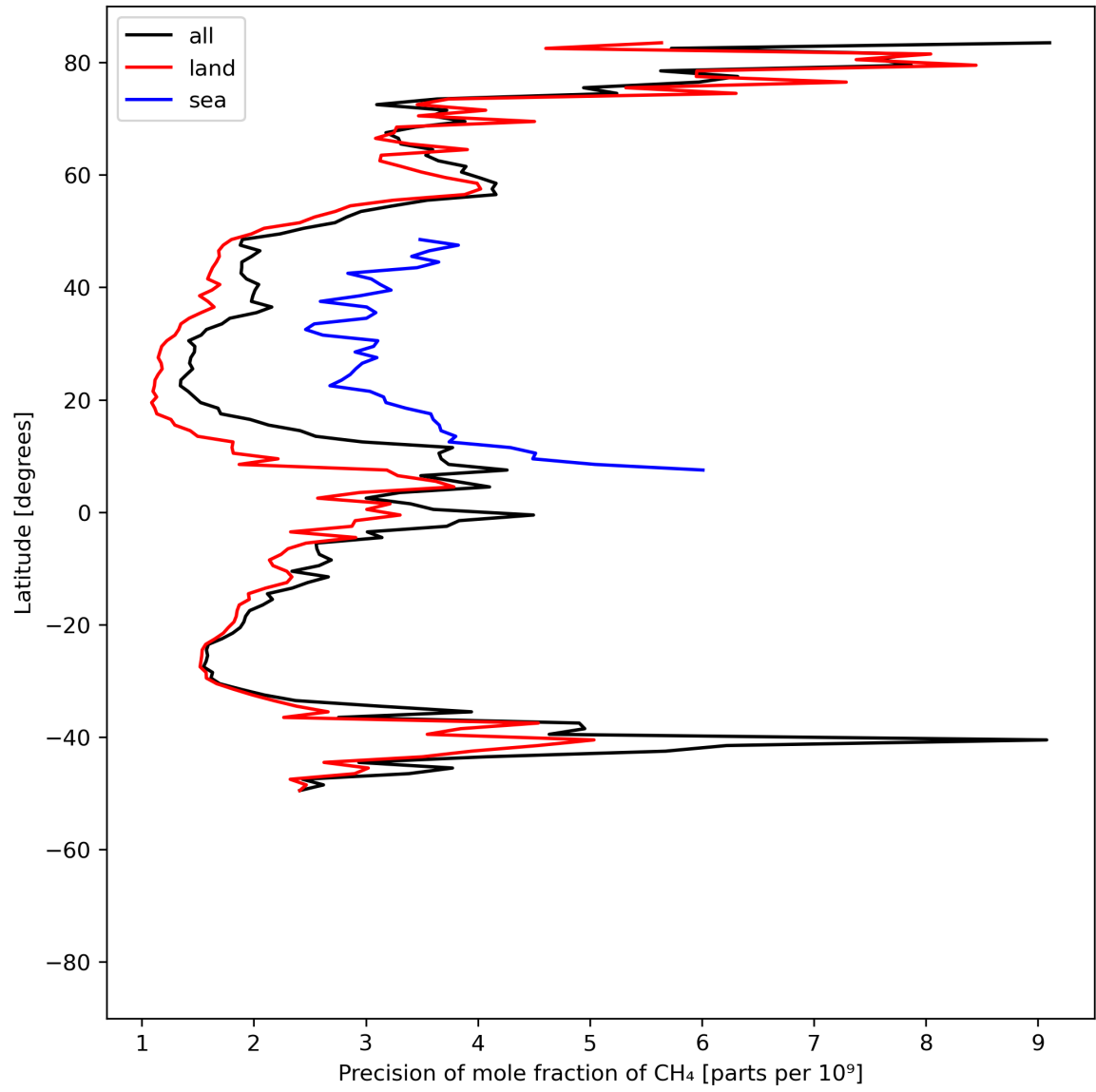
Figure 13: Zonal average of “Precision of mole fraction of \text{CH}_4 ” for 2023-07-10 to 2023-07-12.
