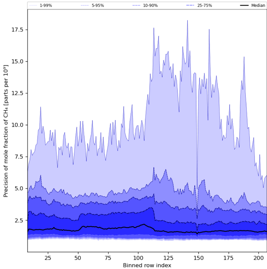
Figure 35: Along track statistics of “Precision of mole fraction of CH 4 ” for 2023-07-10 to 2023-07-12
