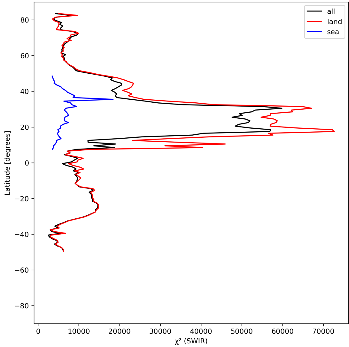
Figure 17: Zonal average of “ \chi^2 (SWIR)” for 2023-07-10 to 2023-07-12.
