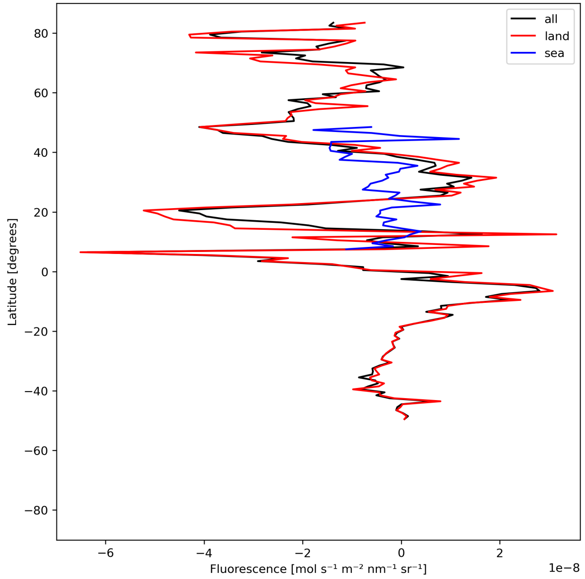
Figure 21: Zonal average of “Fluorescence” for 2023-07-10 to 2023-07-12.
