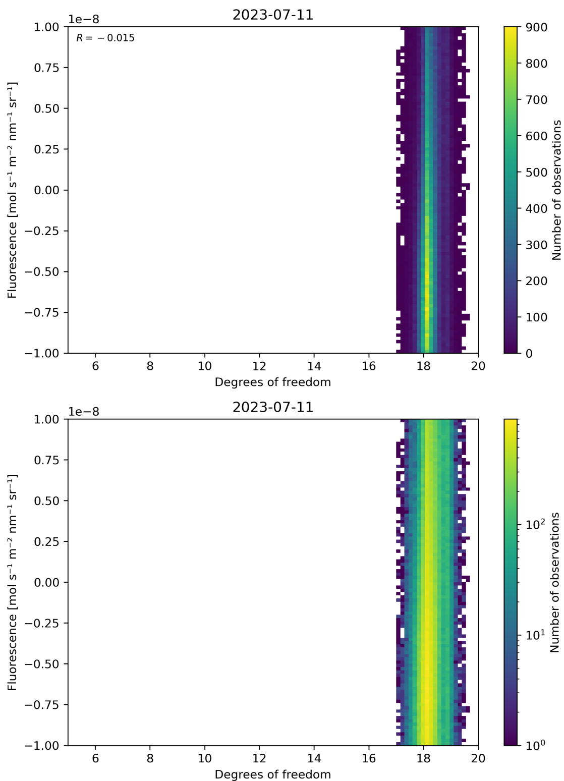
Figure 51: Scatter density plot of “Degrees of freedom” against “Fluorescence” for 2023-07-10 to 2023-07-12.
