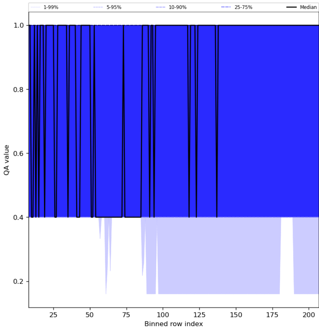
Figure 33: Along track statistics of “QA value” for 2023-07-10 to 2023-07-12
