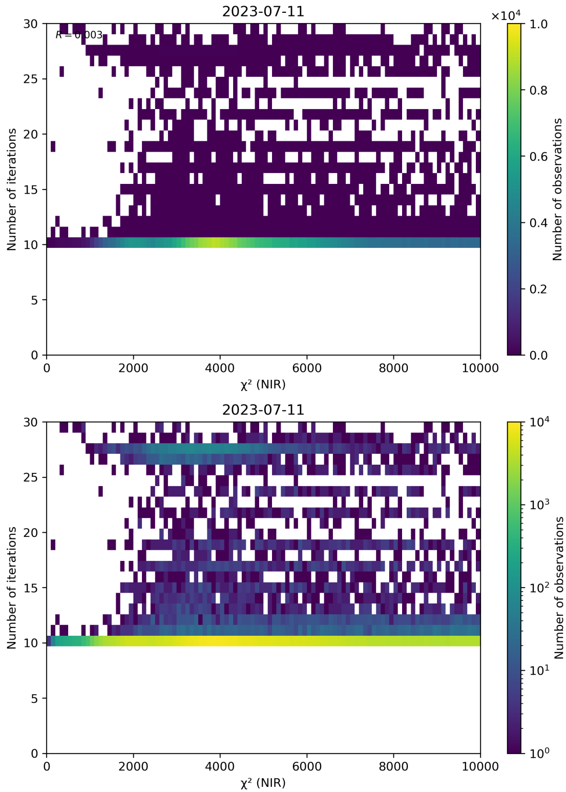
Figure 46: Scatter density plot of “ \chi^2 (NIR)” against “Number of iterations” for 2023-07-10 to 2023-07-12.
