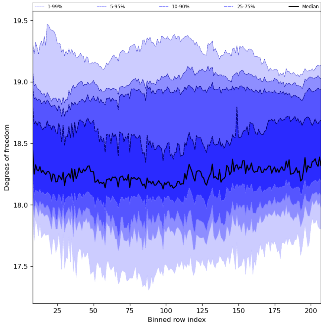
Figure 41: Along track statistics of “Degrees of freedom” for 2023-07-10 to 2023-07-12
