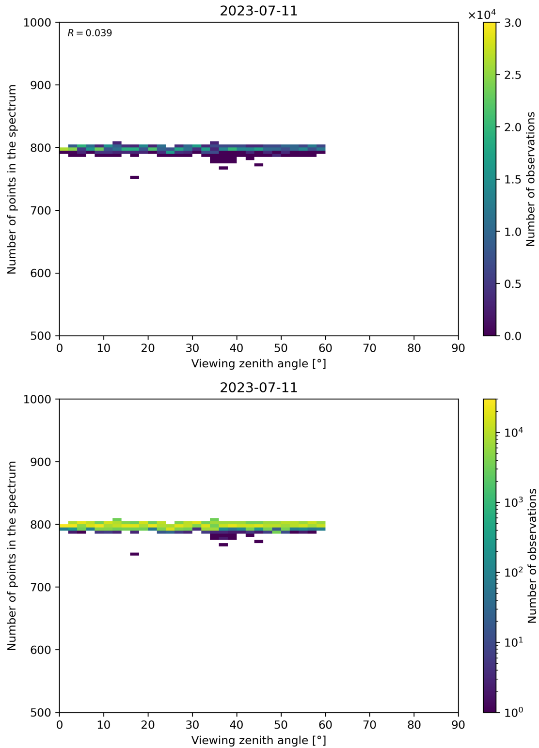
Figure 114: Scatter density plot of “Viewing zenith angle” against “Number of points in the spectrum” for 2023-07-10 to 2023-07-12.
