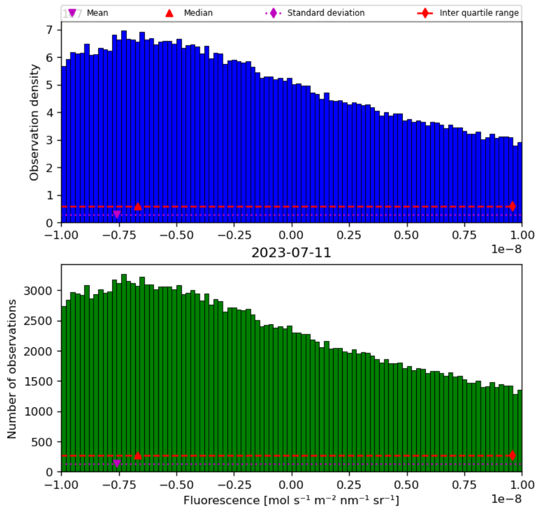
Figure 32: Histogram of “Fluorescence” for 2023-07-10 to 2023-07-12
