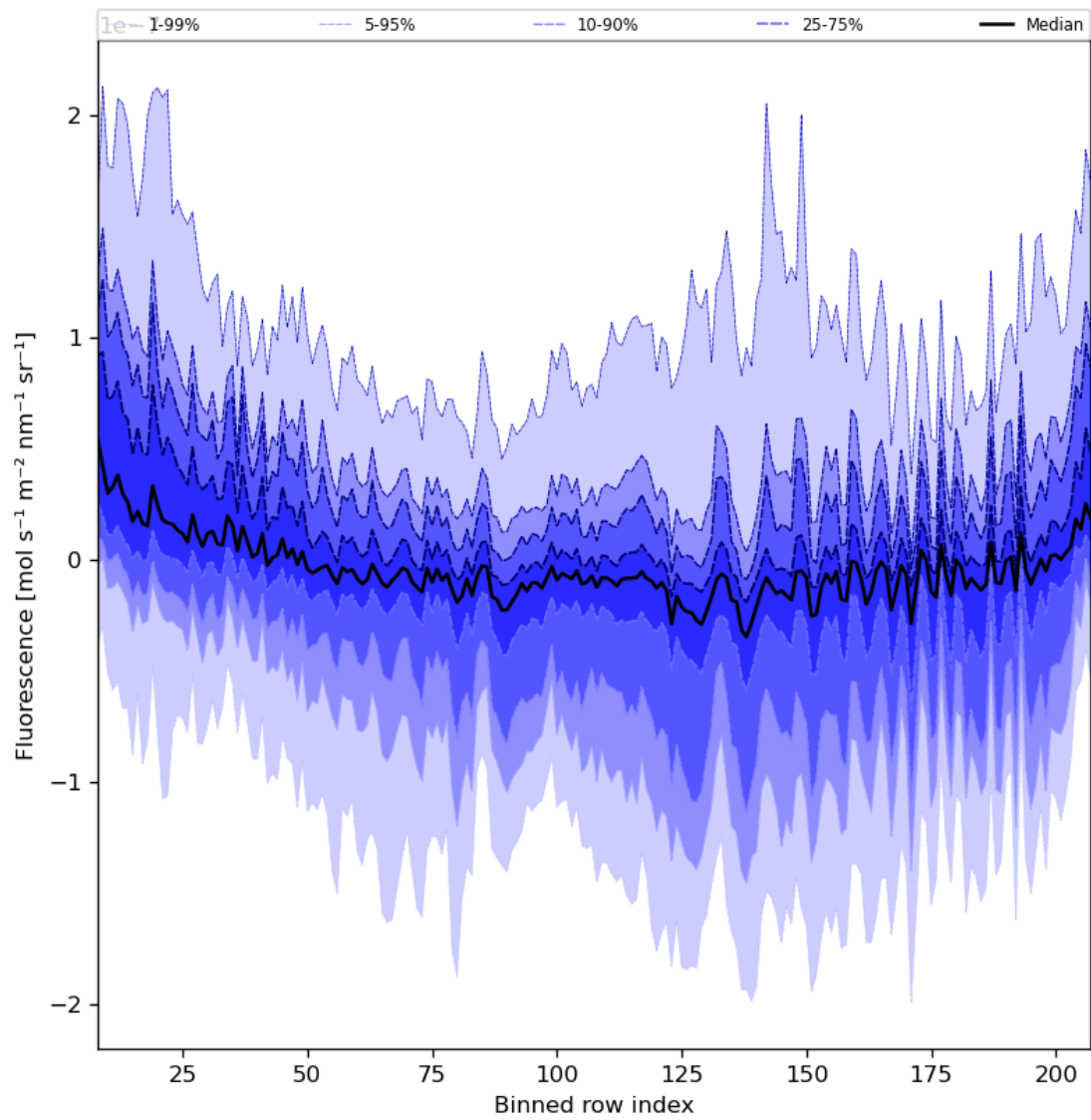
Figure 43: Along track statistics of “Fluorescence” for 2023-07-10 to 2023-07-12
