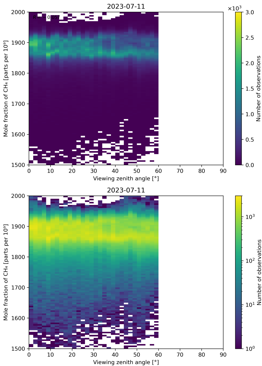
Figure 110: Scatter density plot of “Viewing zenith angle” against “Mole fraction of CH 4 ” for 2023-07-10 to 2023-07-12.
