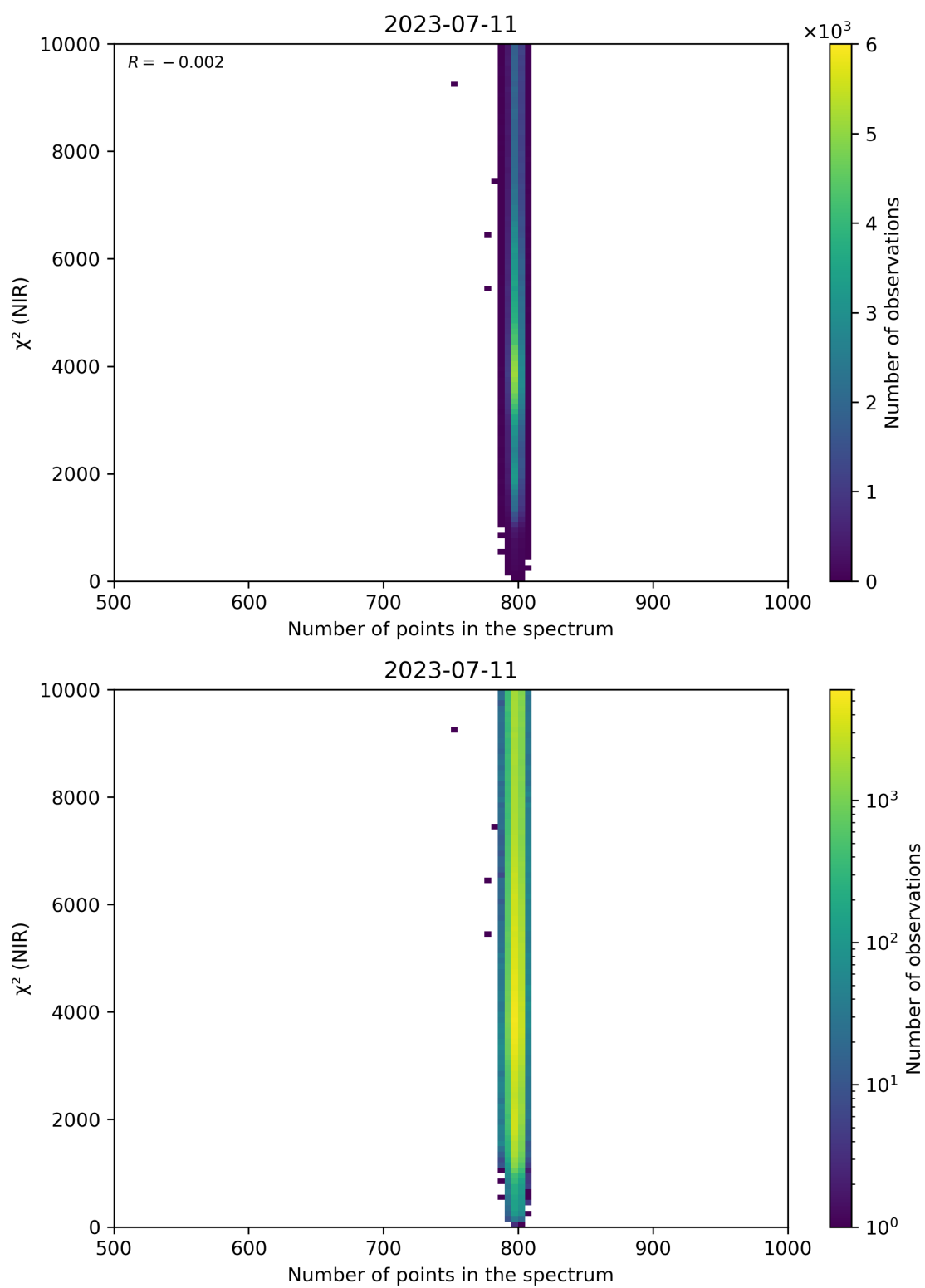
Figure 88: Scatter density plot of “Number of points in the spectrum” against “ \chi^2 (NIR)” for 2023-07-10 to 2023-07-12.
