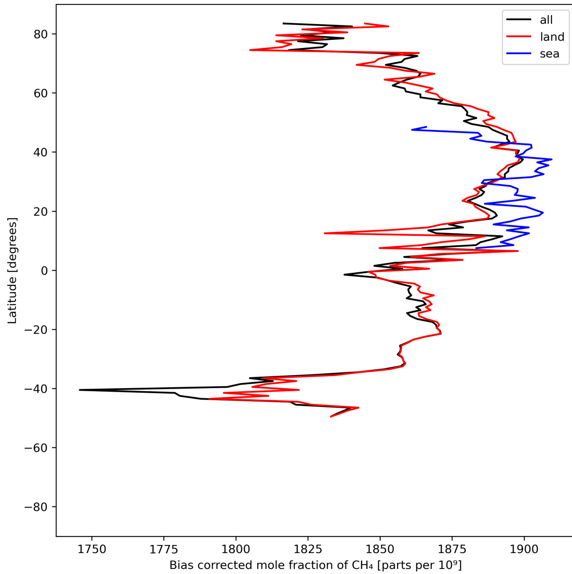
Figure 14: Zonal average of “Bias corrected mole fraction of \text{CH}_4 ” for 2023-07-10 to 2023-07-12.
