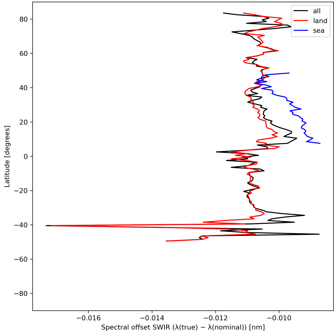
Figure 16: Zonal average of “Spectral offset SWIR ( \lambda(\text{true}) - \lambda(\text{nominal}) )” for 2023-07-10 to 2023-07-12.
