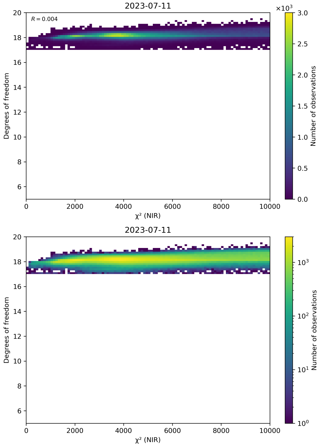
Figure 44: Scatter density plot of “ \chi^2 (NIR)” against “Degrees of freedom” for 2023-07-10 to 2023-07-12.
