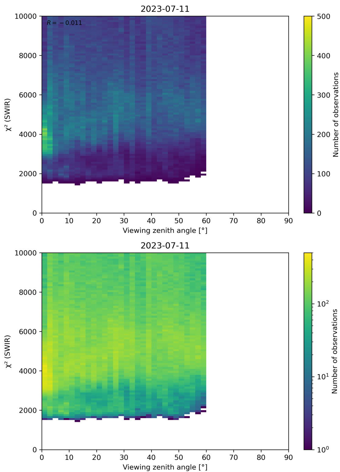
Figure 106: Scatter density plot of “Viewing zenith angle” against “ \chi^2 (SWIR)” for 2023-07-10 to 2023-07-12.
