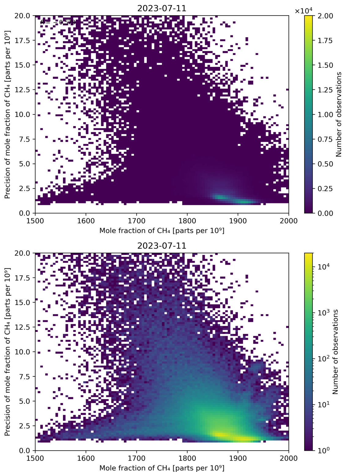
Figure 75: Scatter density plot of “Mole fraction of CH 4 ” against “Precision of mole fraction of CH 4 ” for 2023-07-10 to 2023-07-12.
