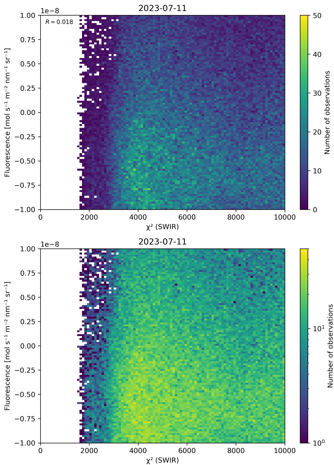
Figure 49: Scatter density plot of “ \chi^2 (SWIR)” against “Fluorescence” for 2023-07-10 to 2023-07-12.
