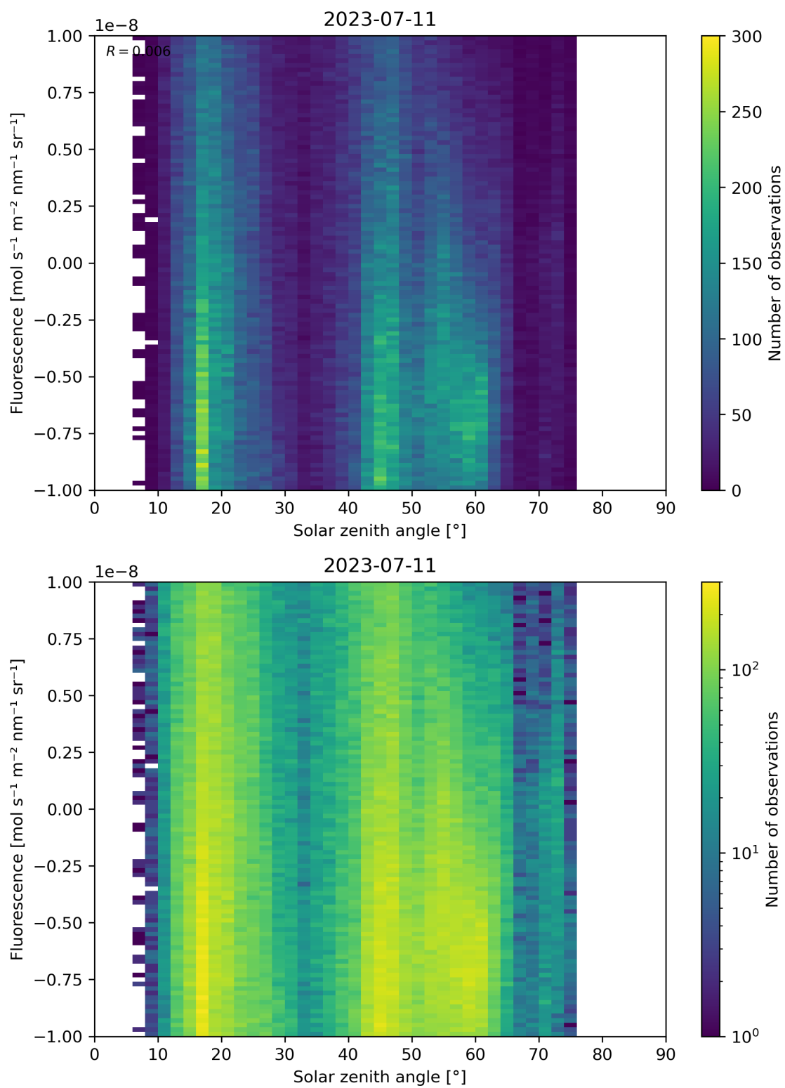
Figure 97: Scatter density plot of “Solar zenith angle” against “Fluorescence” for 2023-07-10 to 2023-07-12.
