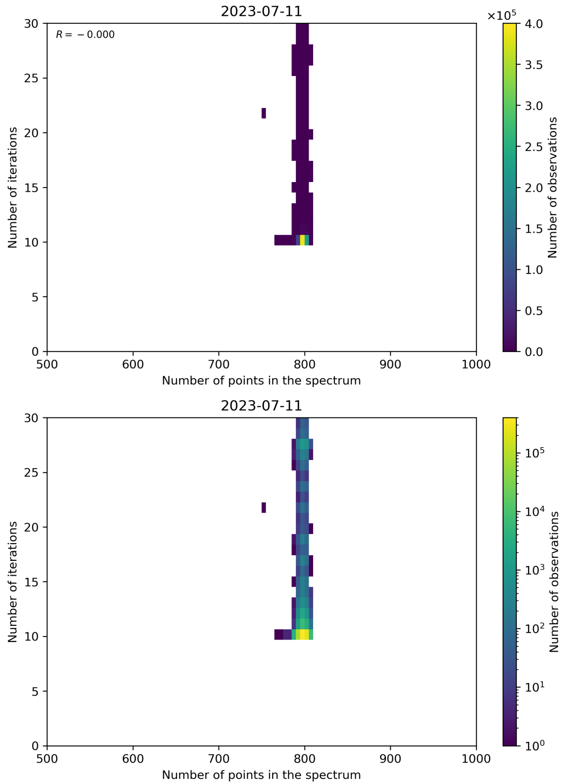
Figure 92: Scatter density plot of “Number of points in the spectrum” against “Number of iterations” for 2023-07-10 to 2023-07-12.
