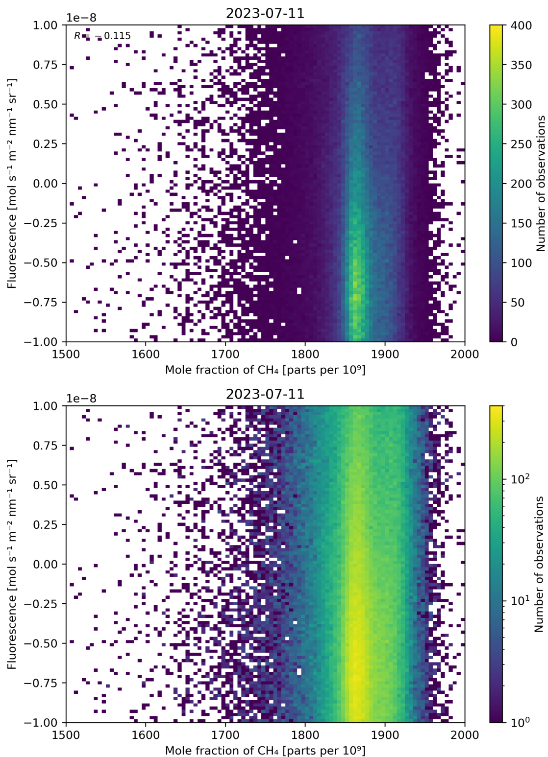
Figure 73: Scatter density plot of “Mole fraction of \text{CH}_4 ” against “Fluorescence” for 2023-07-10 to 2023-07-12.
