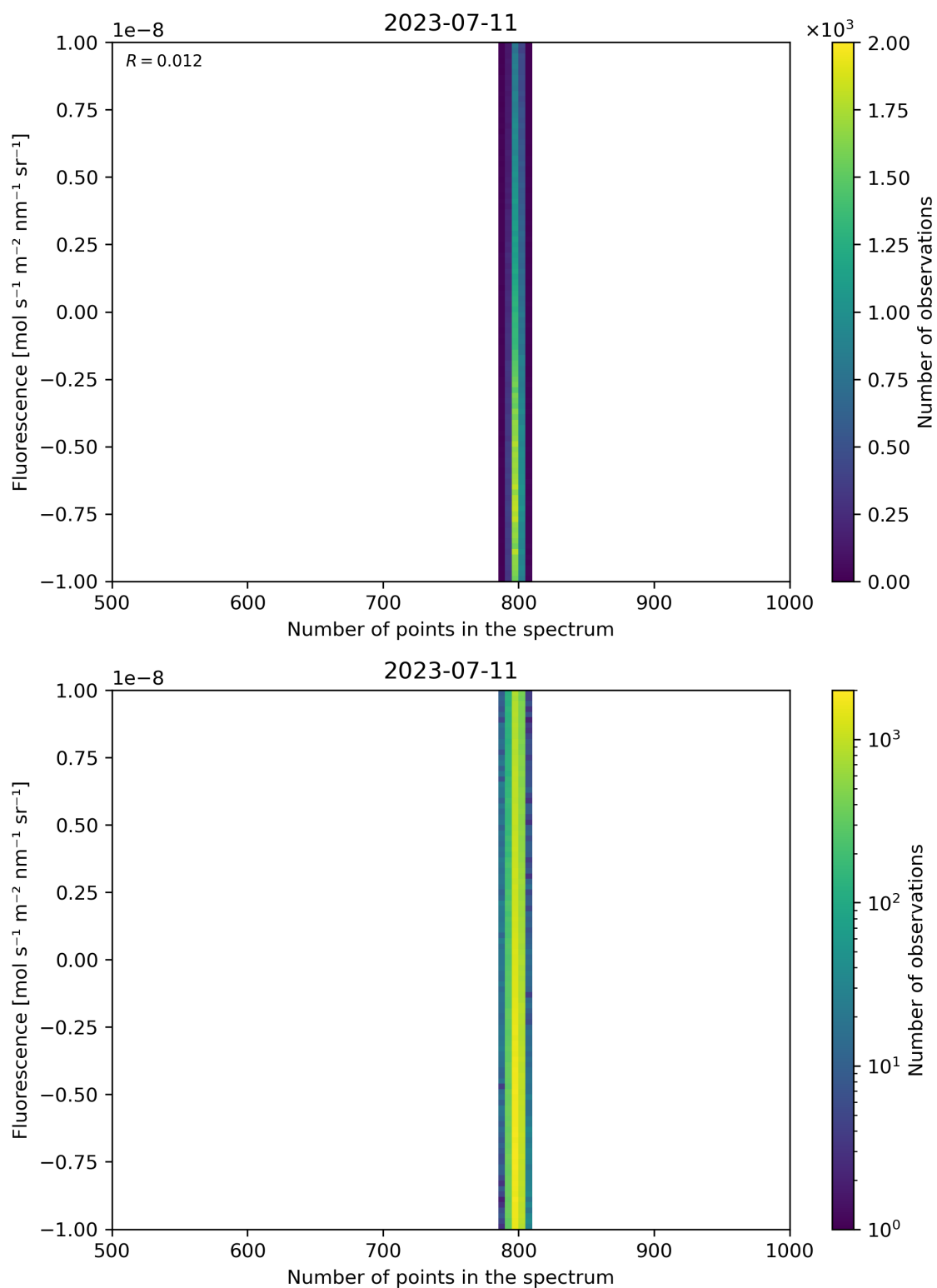
Figure 91: Scatter density plot of “Number of points in the spectrum” against “Fluorescence” for 2023-07-10 to 2023-07-12.
