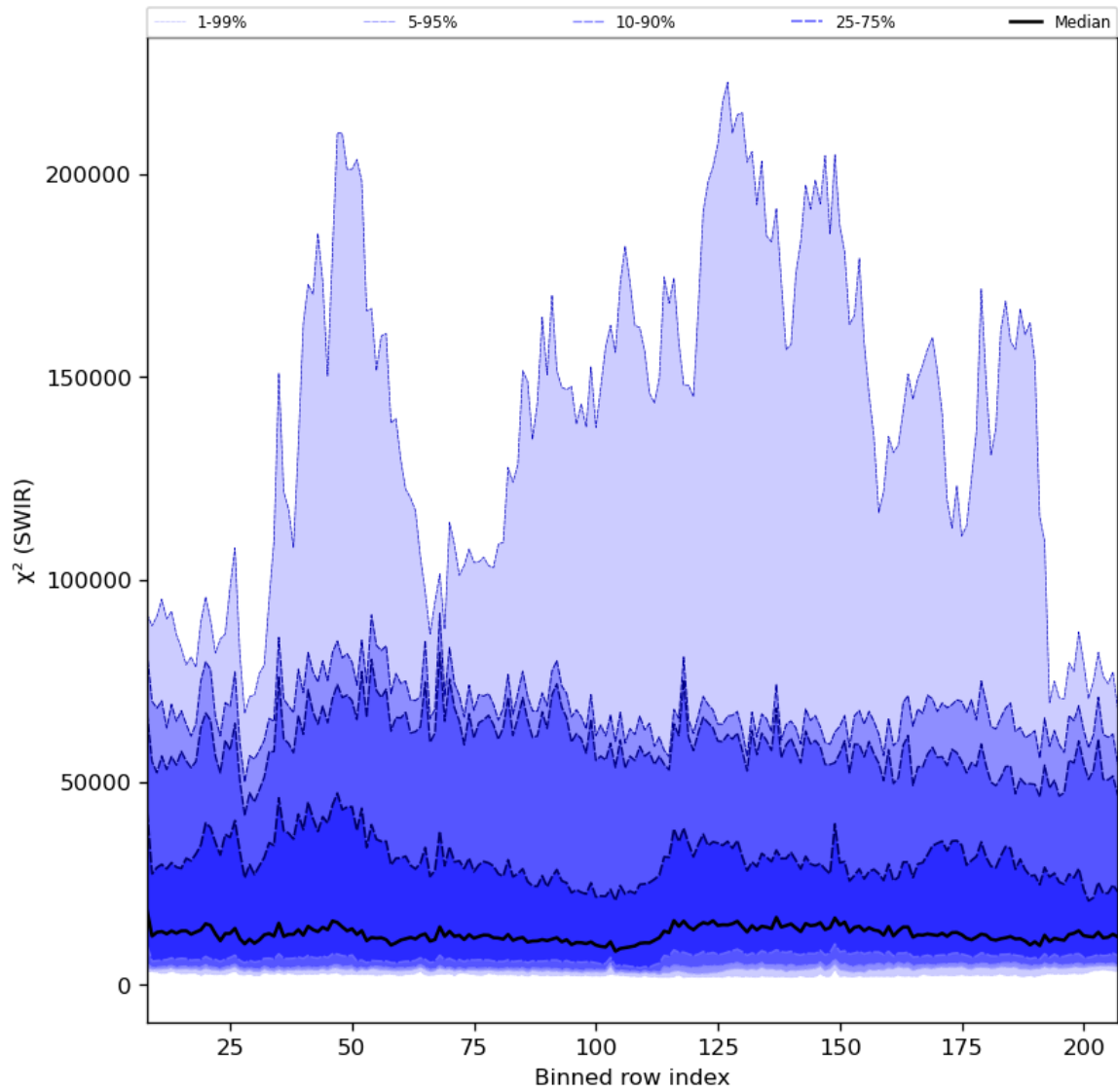
Figure 39: Along track statistics of “ \chi^2 (SWIR)” for 2023-07-10 to 2023-07-12
