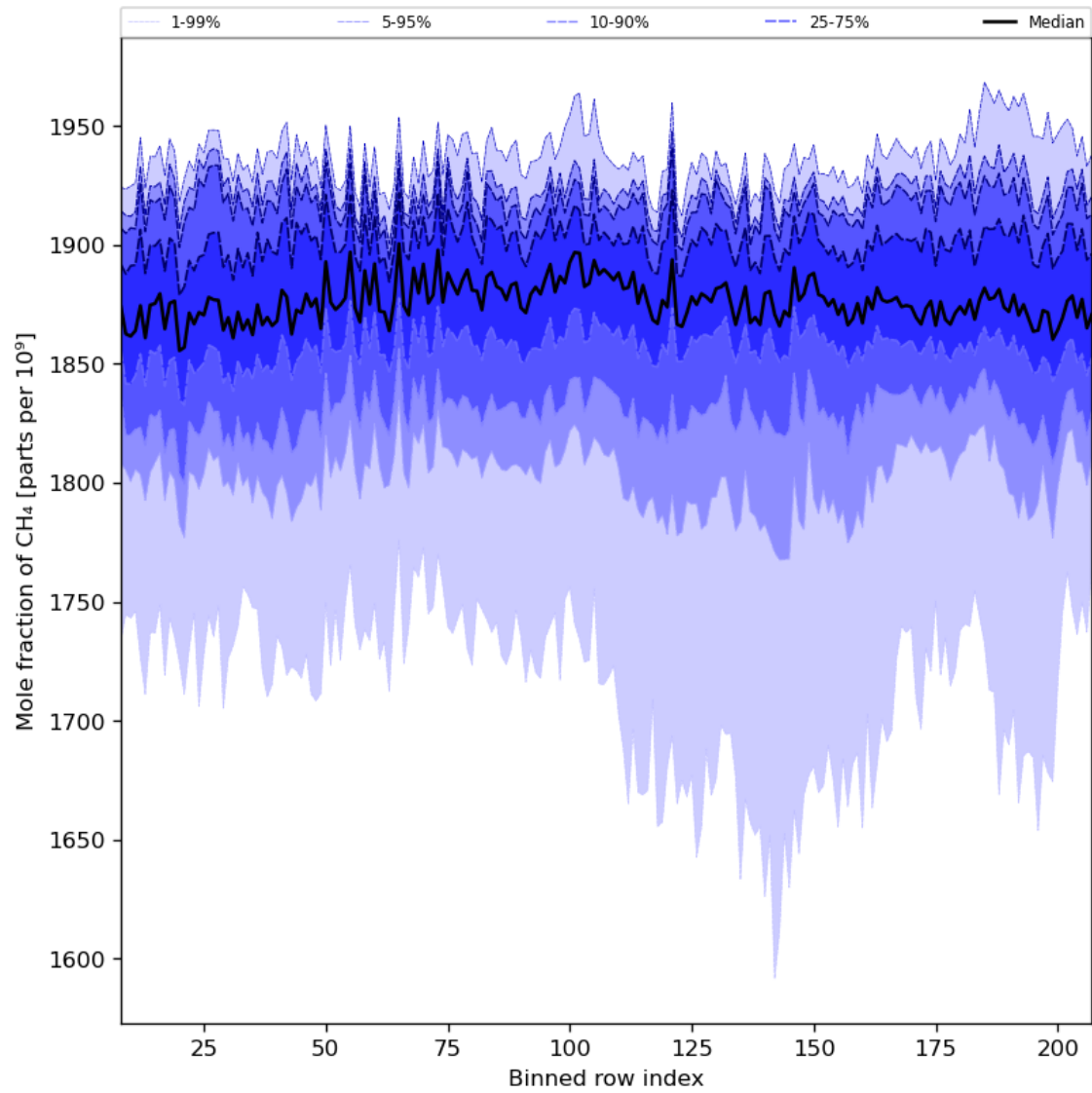
Figure 34: Along track statistics of “Mole fraction of CH 4 ” for 2023-07-10 to 2023-07-12
