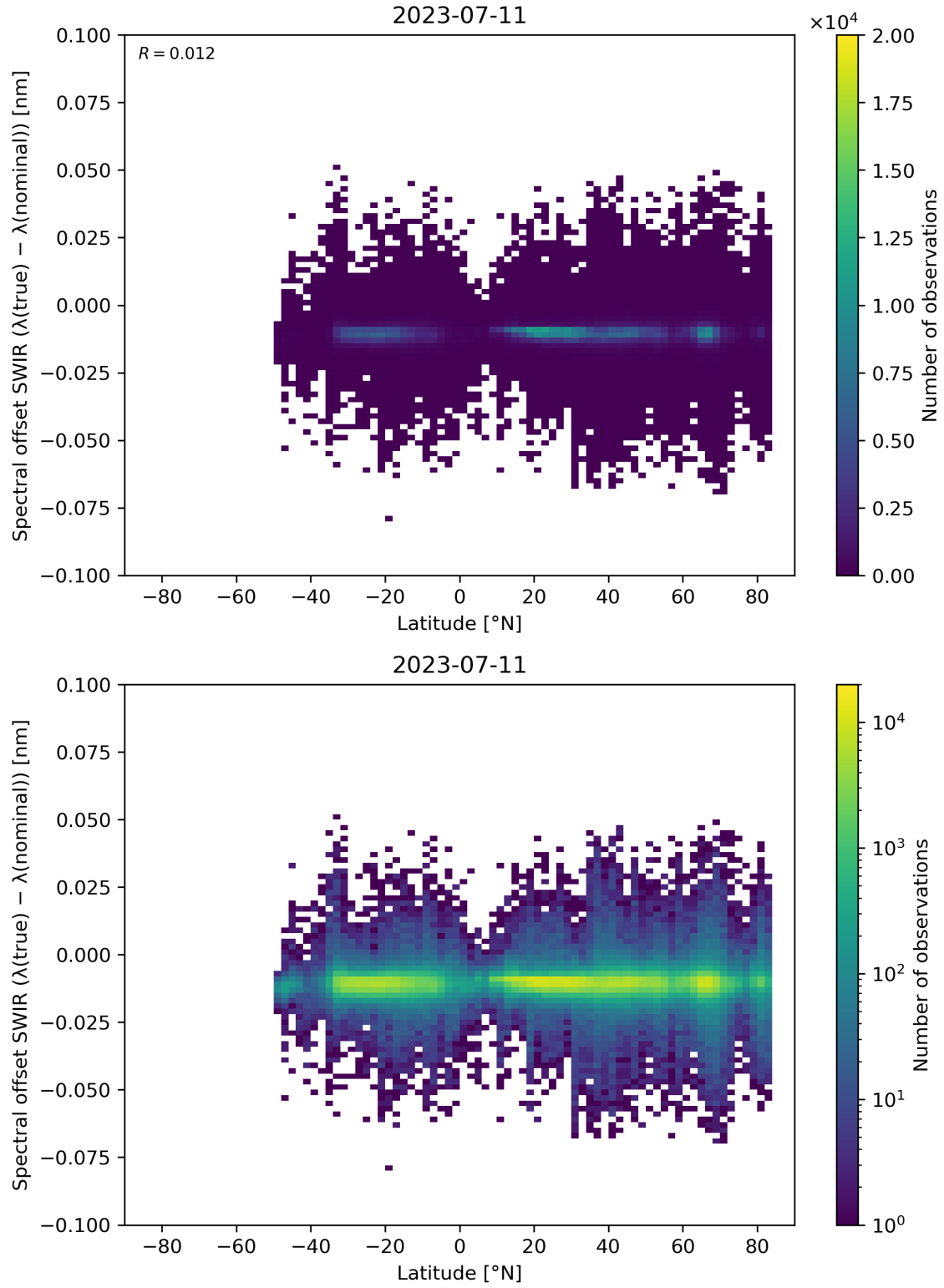
Figure 62: Scatter density plot of “Latitude” against “Spectral offset SWIR ( \lambda(\text{true}) - \lambda(\text{nominal}) )” for 2023-07-10 to 2023-07-12.
