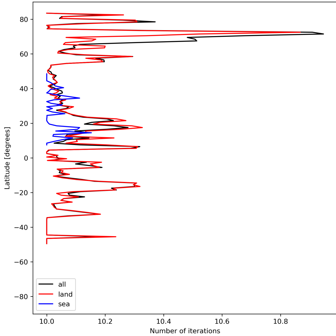
Figure 20: Zonal average of “Number of iterations” for 2023-07-10 to 2023-07-12.
