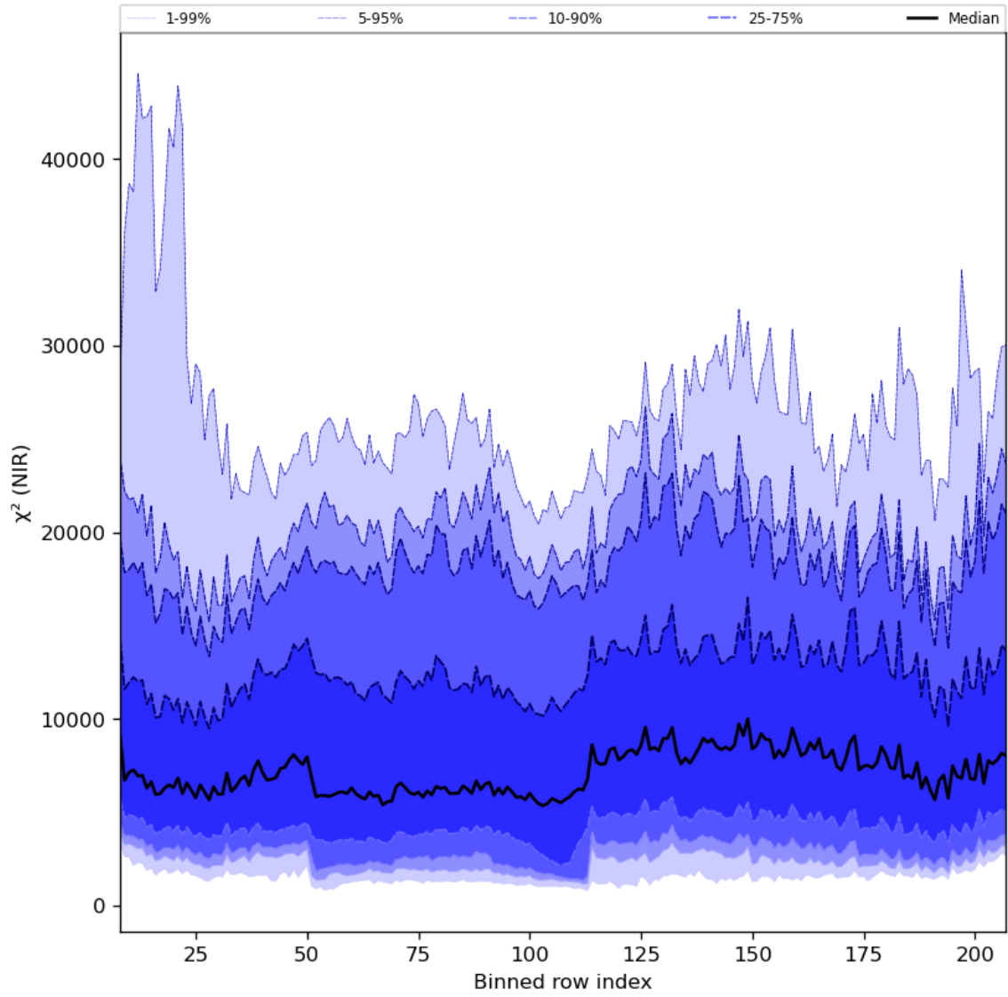
Figure 40: Along track statistics of “ \chi^2 (NIR)” for 2023-07-10 to 2023-07-12
