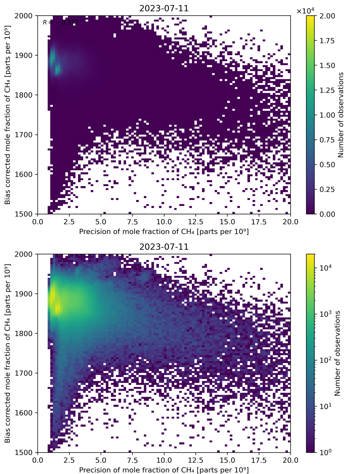
Figure 82: Scatter density plot of “Precision of mole fraction of CH 4 ” against “Bias corrected mole fraction of CH 4 ” for 2023-07-10 to 2023-07-12.
