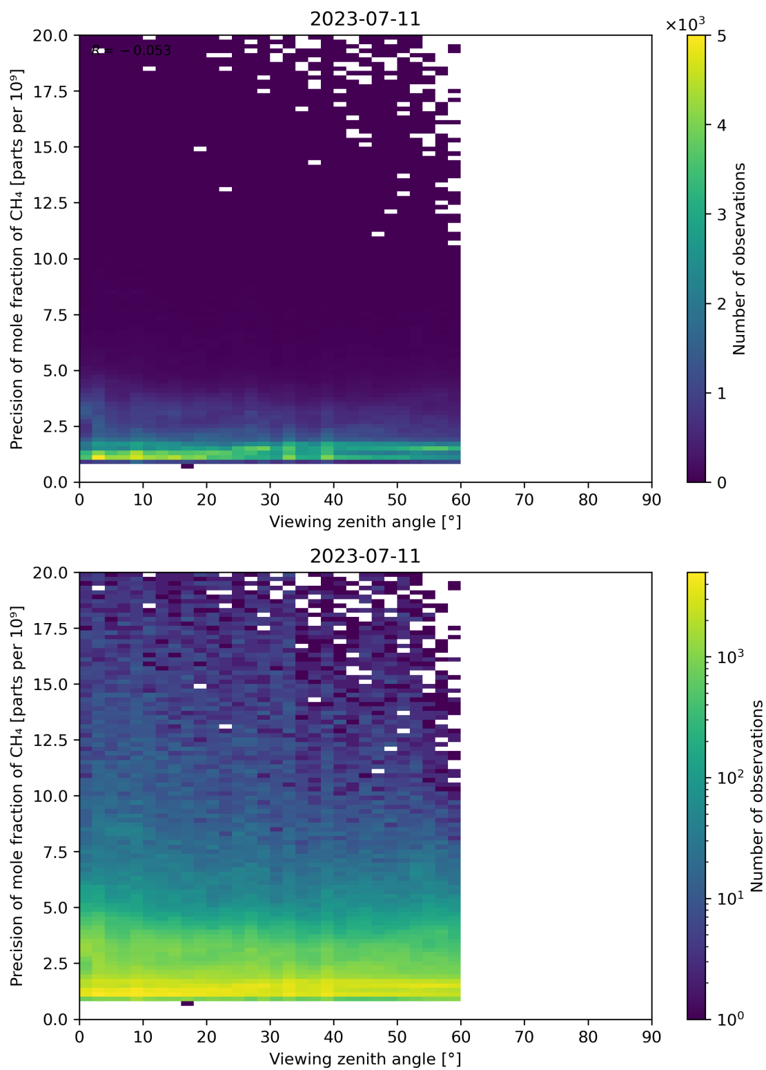
Figure 112: Scatter density plot of “Viewing zenith angle” against “Precision of mole fraction of CH 4 ” for 2023-07-10 to 2023-07-12.
