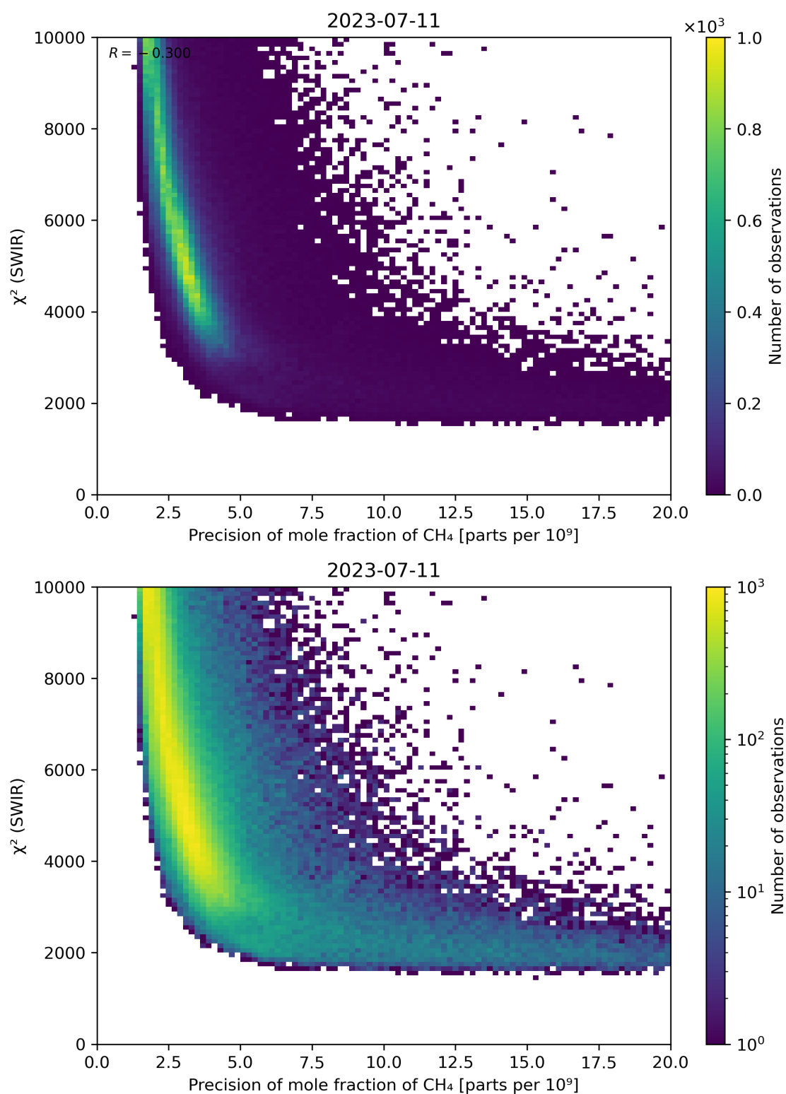
Figure 79: Scatter density plot of “Precision of mole fraction of \text{CH}_4 ” against “ \chi^2 (SWIR)” for 2023-07-10 to 2023-07-12.
