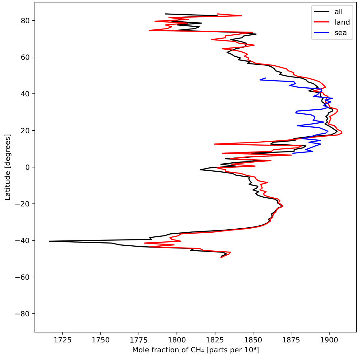
Figure 12: Zonal average of “Mole fraction of \text{CH}_4 ” for 2023-07-10 to 2023-07-12.
