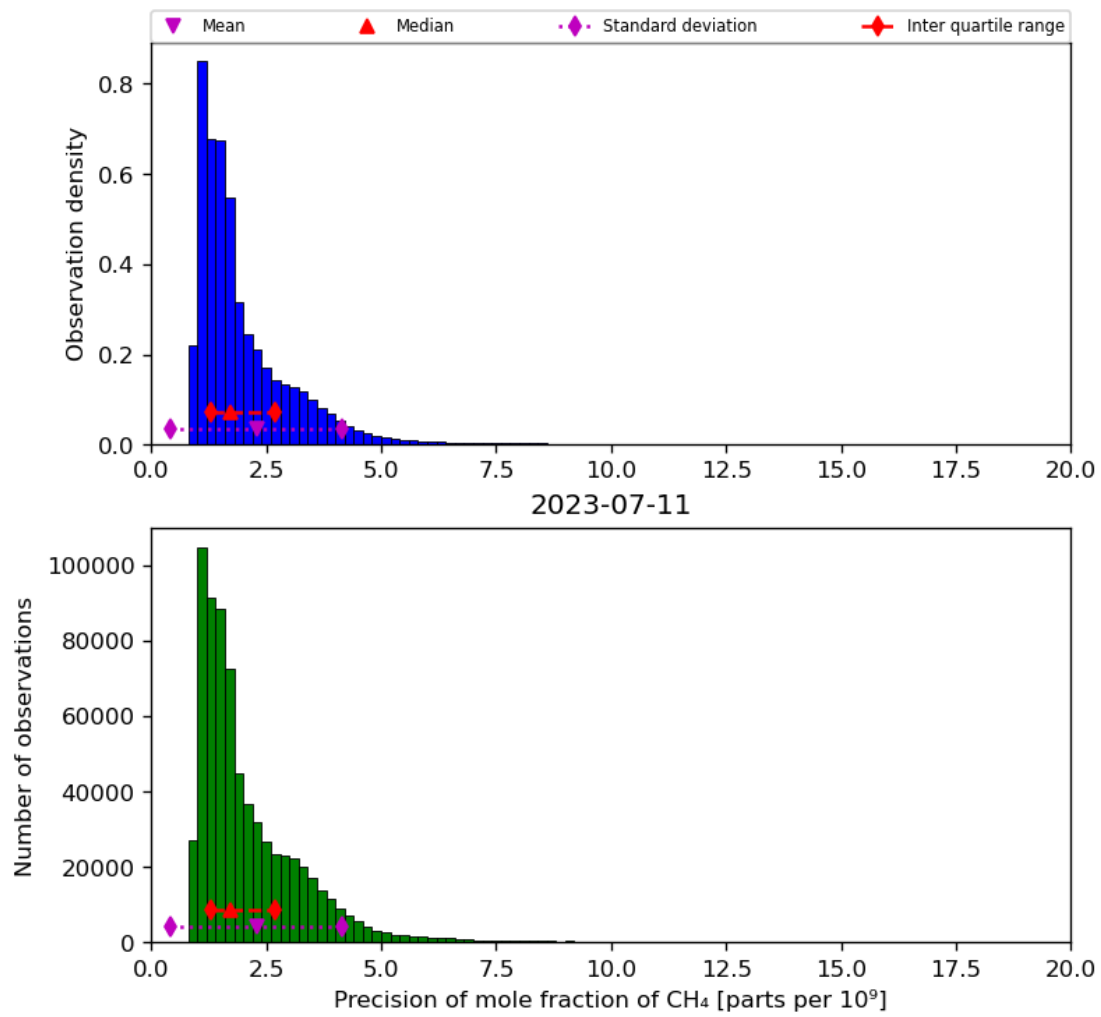
Figure 24: Histogram of “Precision of mole fraction of CH 4 ” for 2023-07-10 to 2023-07-12
