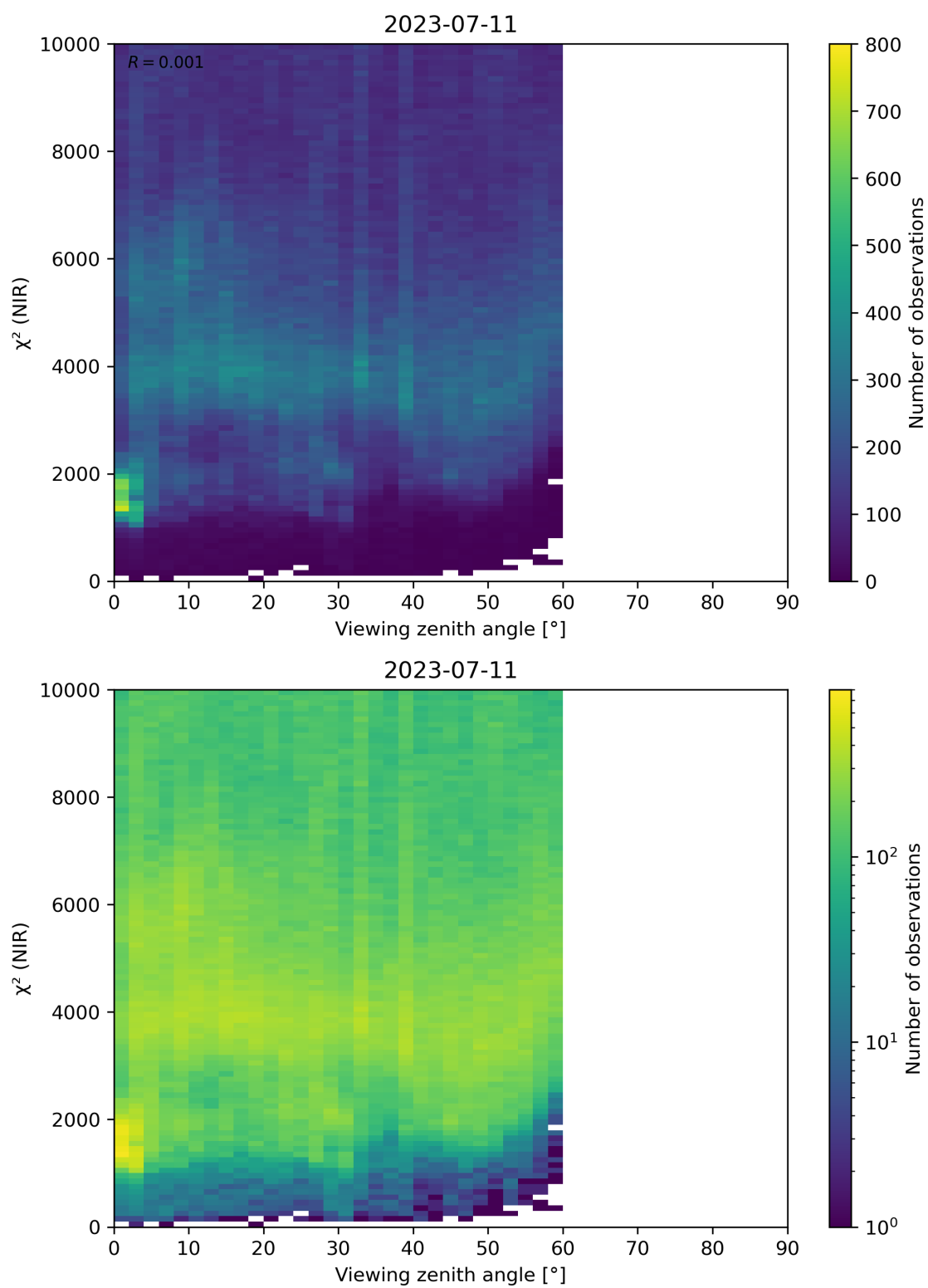
Figure 105: Scatter density plot of “Viewing zenith angle” against “ \chi^2 (NIR)” for 2023-07-10 to 2023-07-12.
