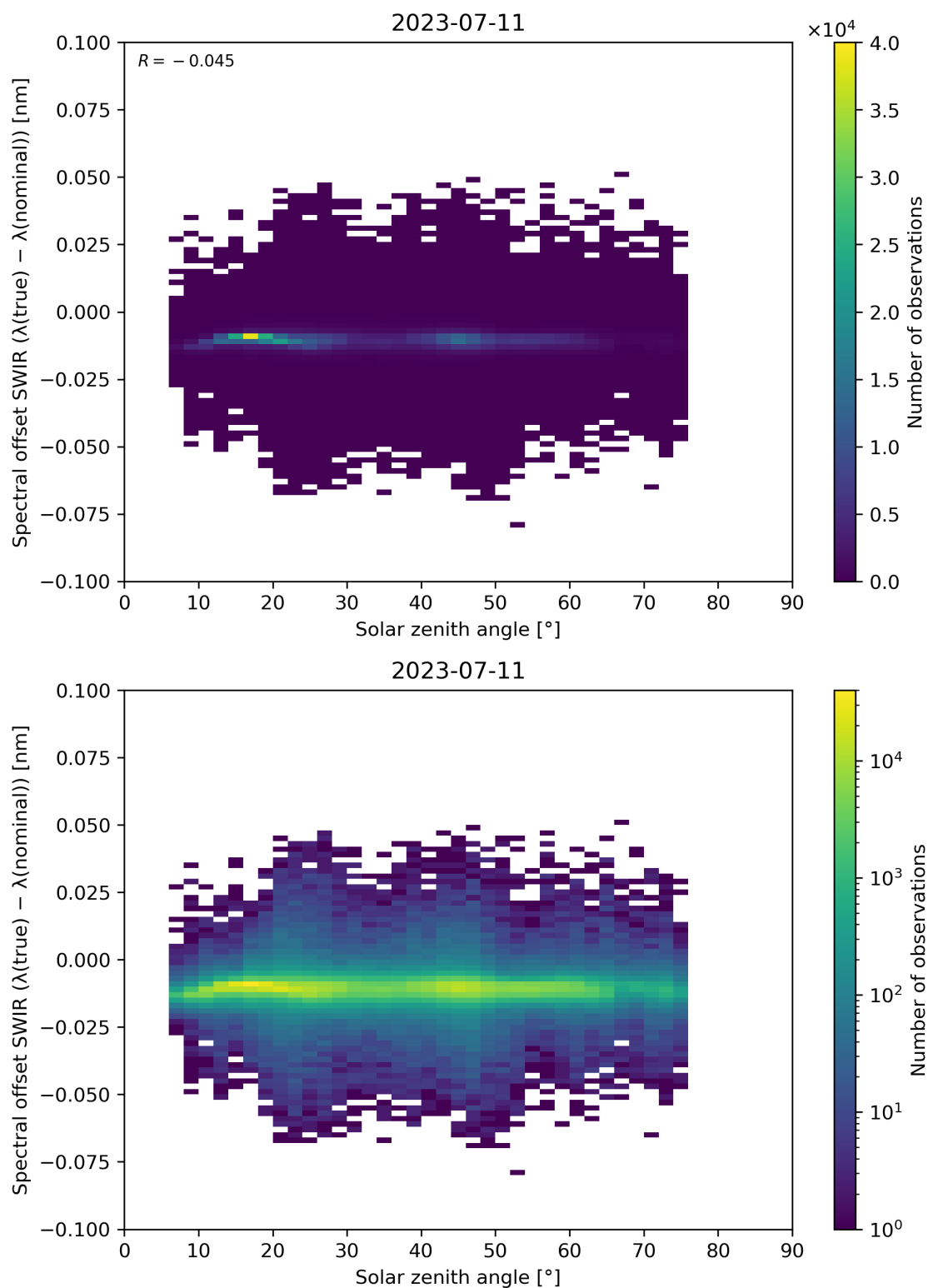
Figure 104: Scatter density plot of “Solar zenith angle” against “Spectral offset SWIR ( \lambda(\text{true}) - \lambda(\text{nominal}) )” for 2023-07-10 to 2023-07-12.
