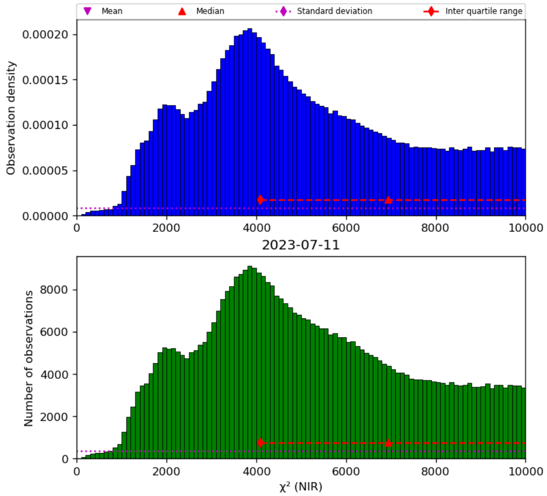
Figure 29: Histogram of “ \chi^2 (NIR)” for 2023-07-10 to 2023-07-12
