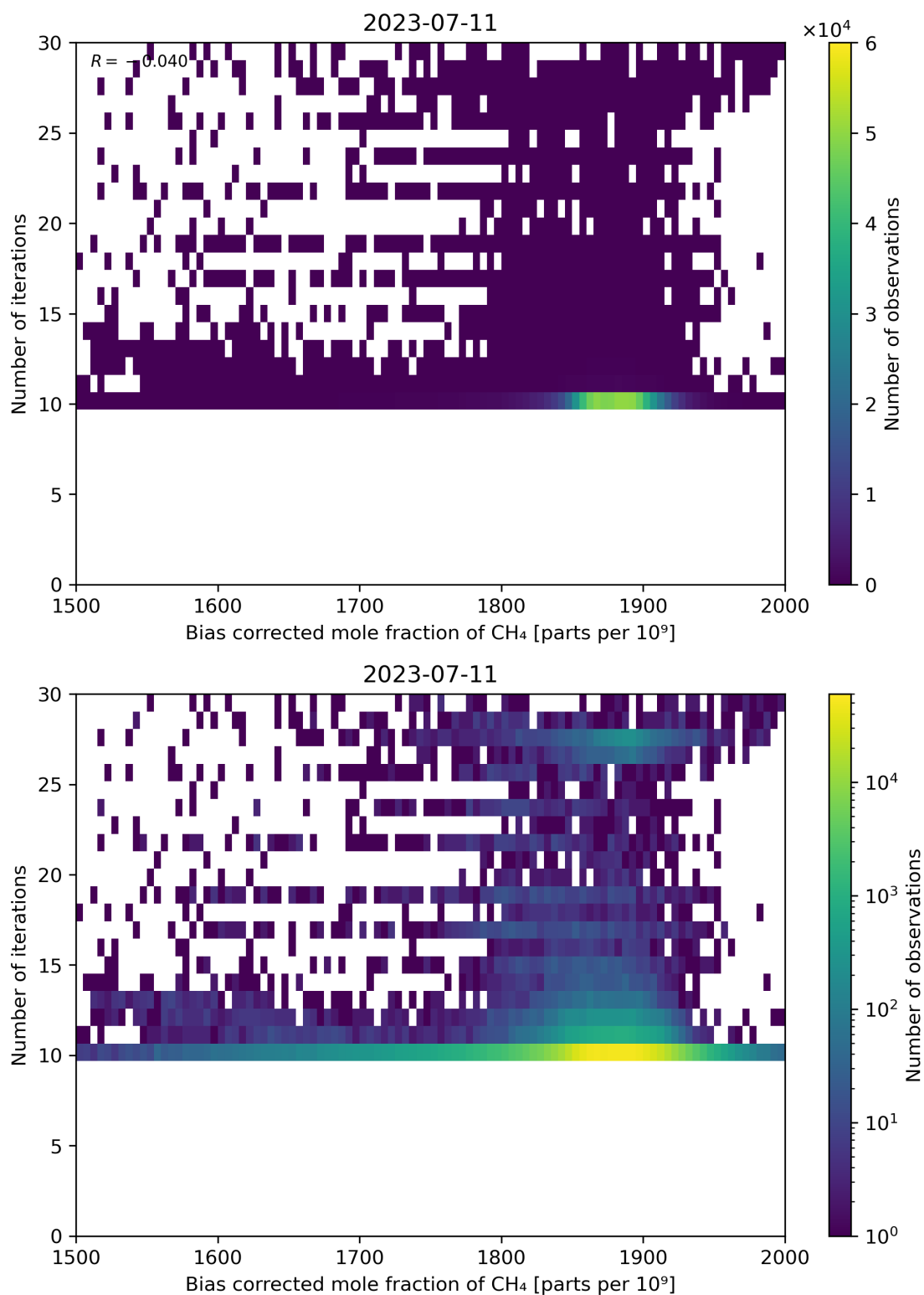
Figure 67: Scatter density plot of “Bias corrected mole fraction of CH 4 ” against “Number of iterations” for 2023-07-10 to 2023-07-12.
