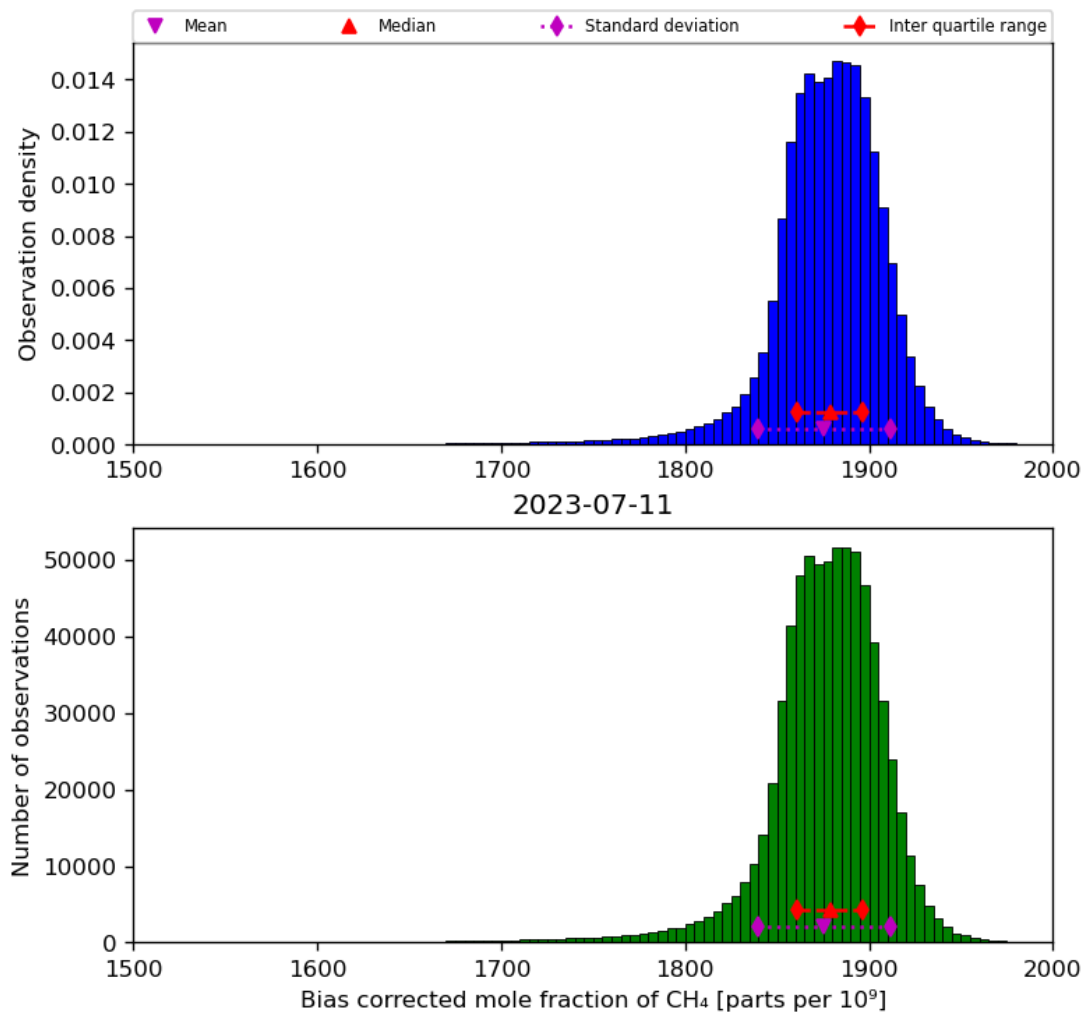
Figure 25: Histogram of “Bias corrected mole fraction of CH 4 ” for 2023-07-10 to 2023-07-12
