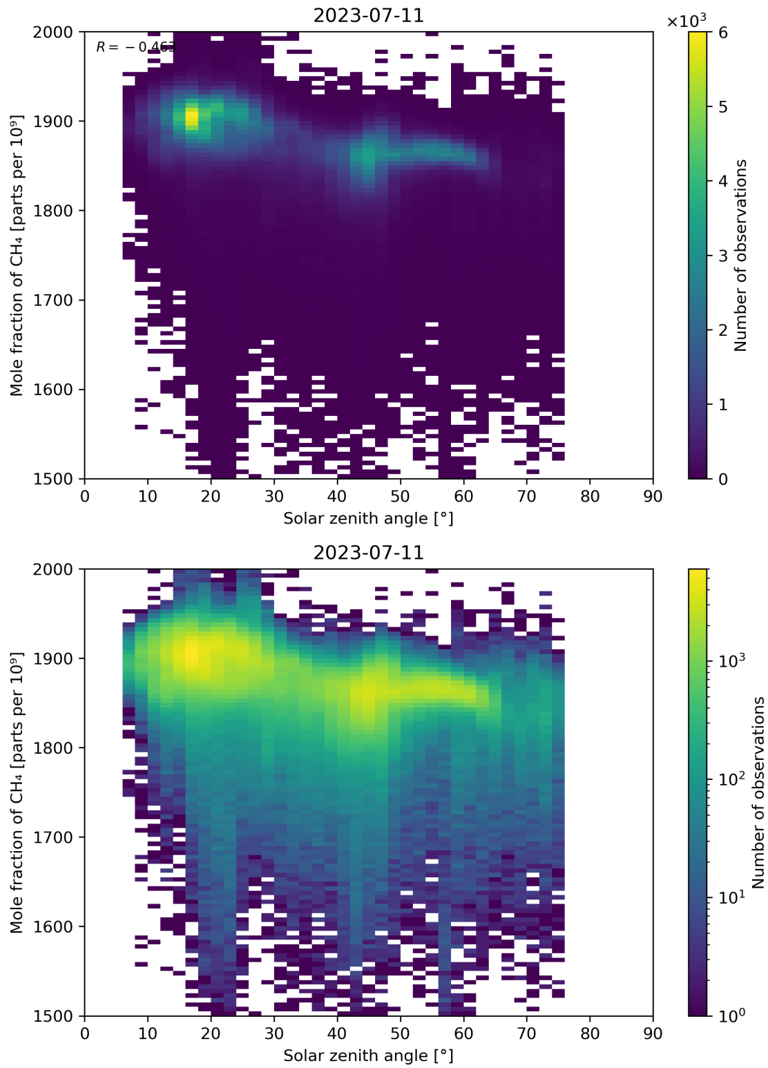
Figure 99: Scatter density plot of “Solar zenith angle” against “Mole fraction of \text{CH}_4 ” for 2023-07-10 to 2023-07-12.
