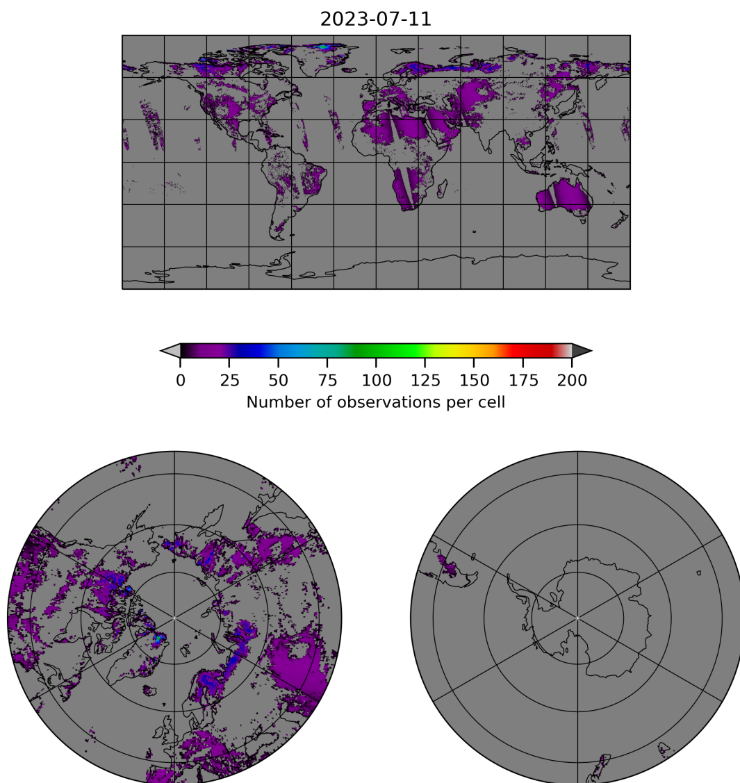
Figure 10: Map of the number of observations for 2023-07-10 to 2023-07-12
