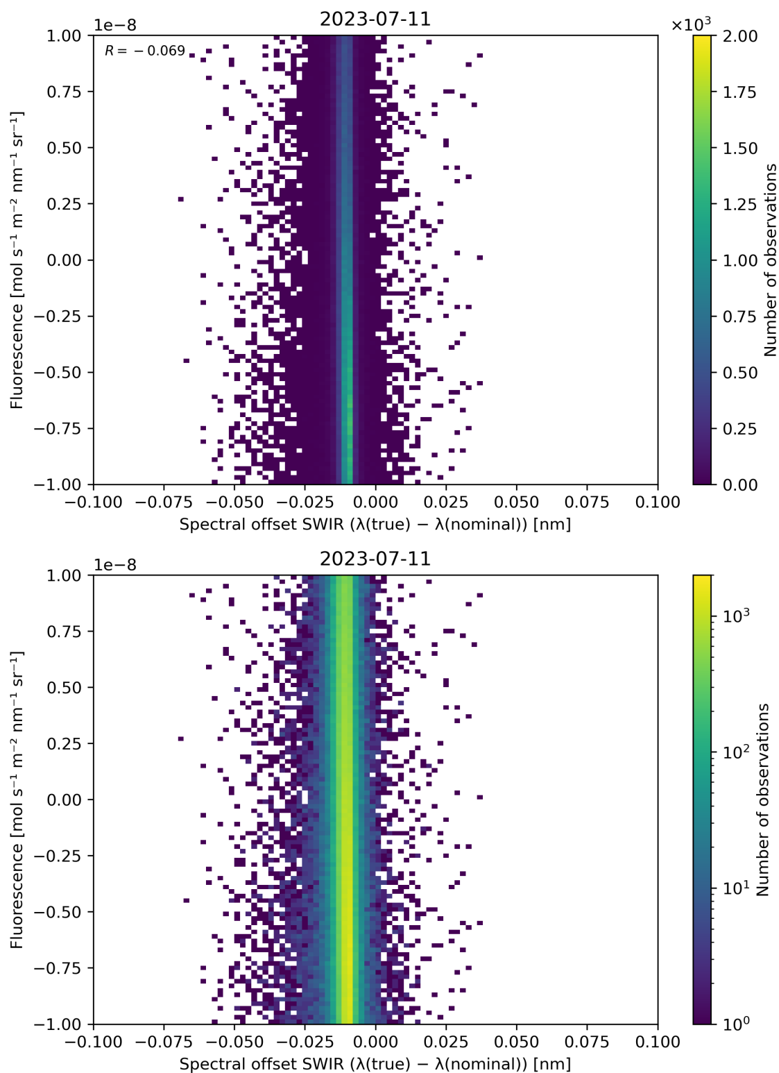
Figure 120: Scatter density plot of “Spectral offset SWIR ( \lambda(\text{true}) - \lambda(\text{nominal}) )” against “Fluorescence” for 2023-07-10 to 2023-07-12.
