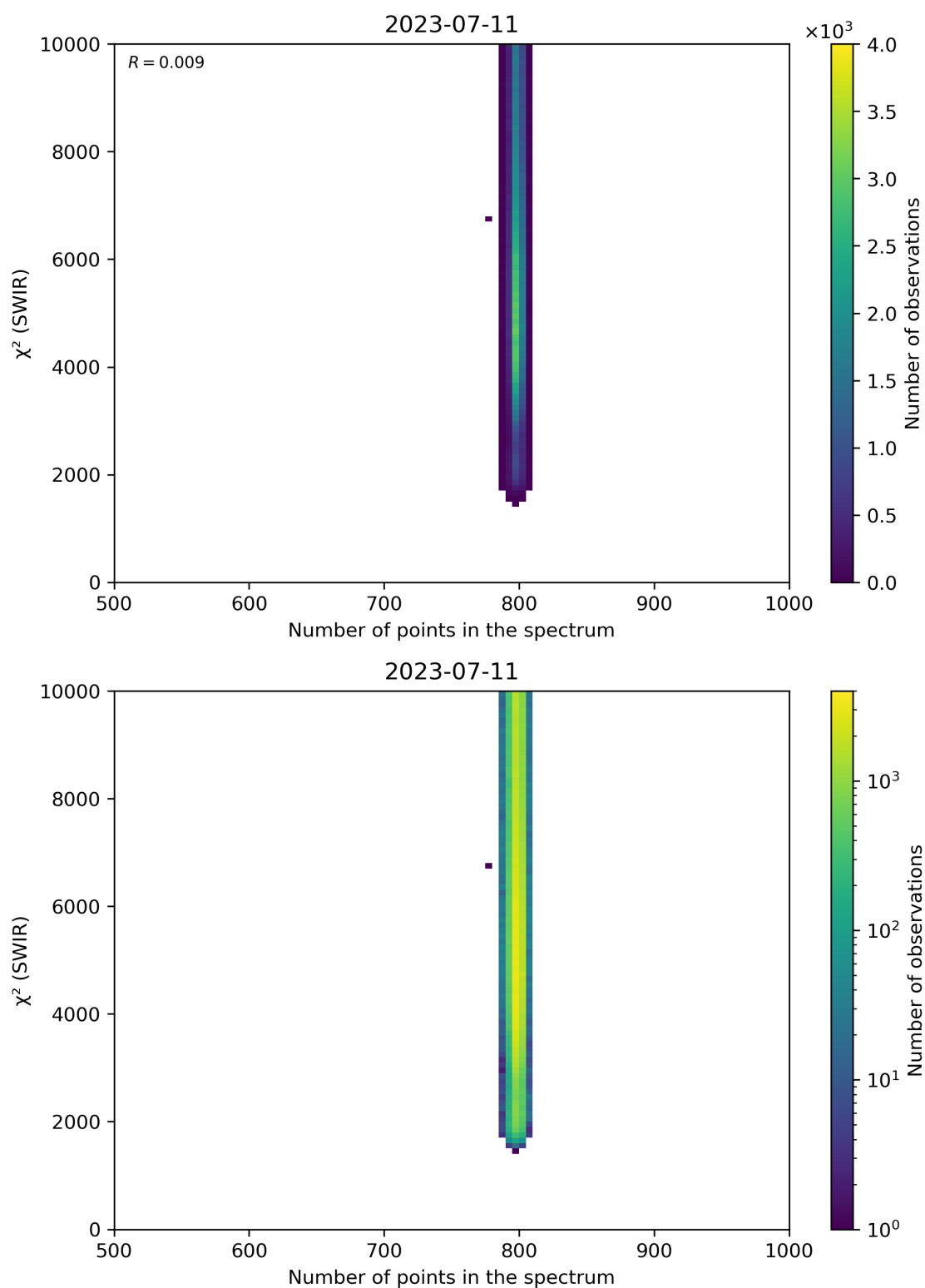
Figure 89: Scatter density plot of “Number of points in the spectrum” against “ \chi^2 (SWIR)” for 2023-07-10 to 2023-07-12.
