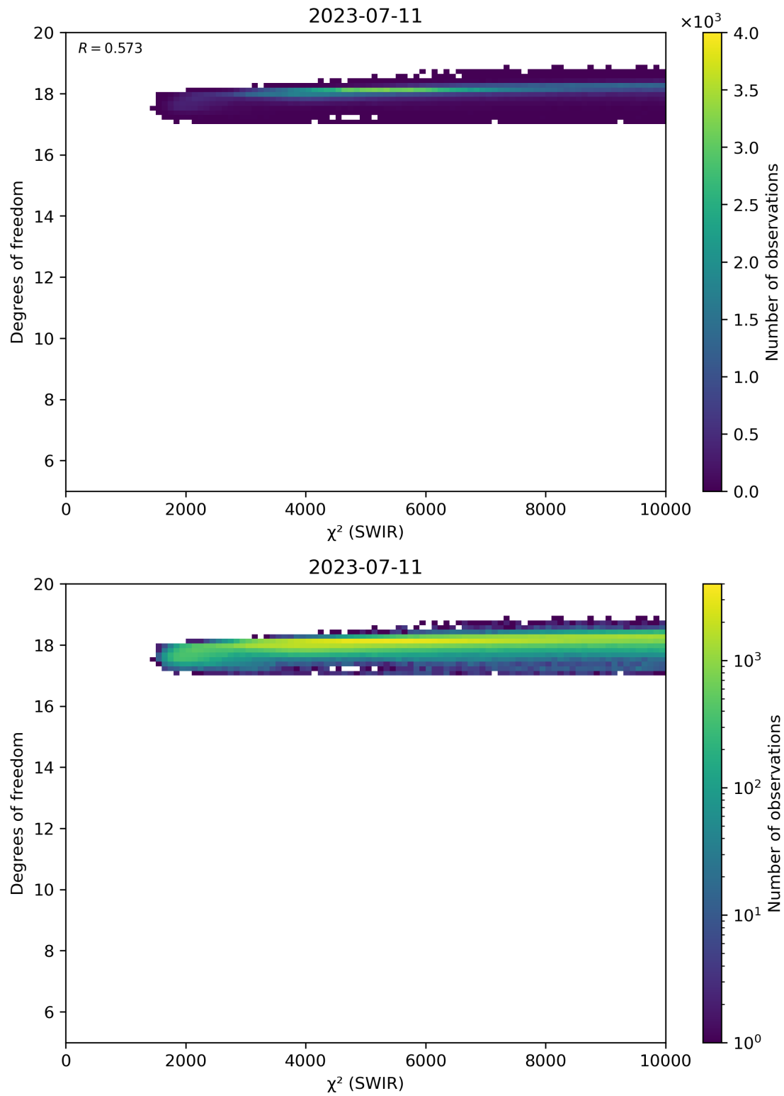
Figure 48: Scatter density plot of “ \chi^2 (SWIR)” against “Degrees of freedom” for 2023-07-10 to 2023-07-12.
