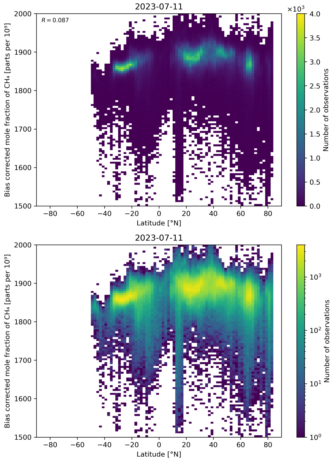
Figure 58: Scatter density plot of “Latitude” against “Bias corrected mole fraction of CH 4 ” for 2023-07-10 to 2023-07-12.
