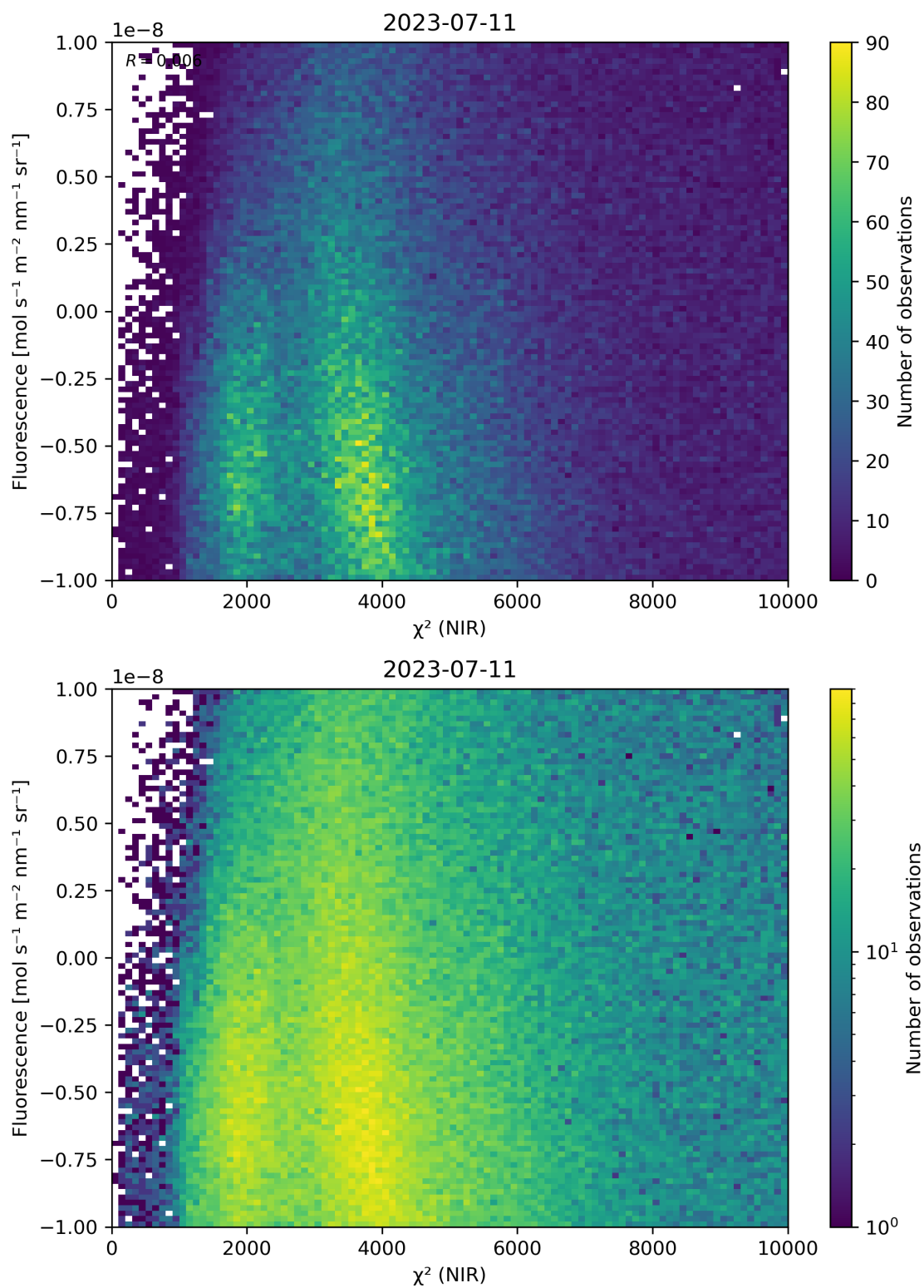
Figure 45: Scatter density plot of “ \chi^2 (NIR)” against “Fluorescence” for 2023-07-10 to 2023-07-12.
