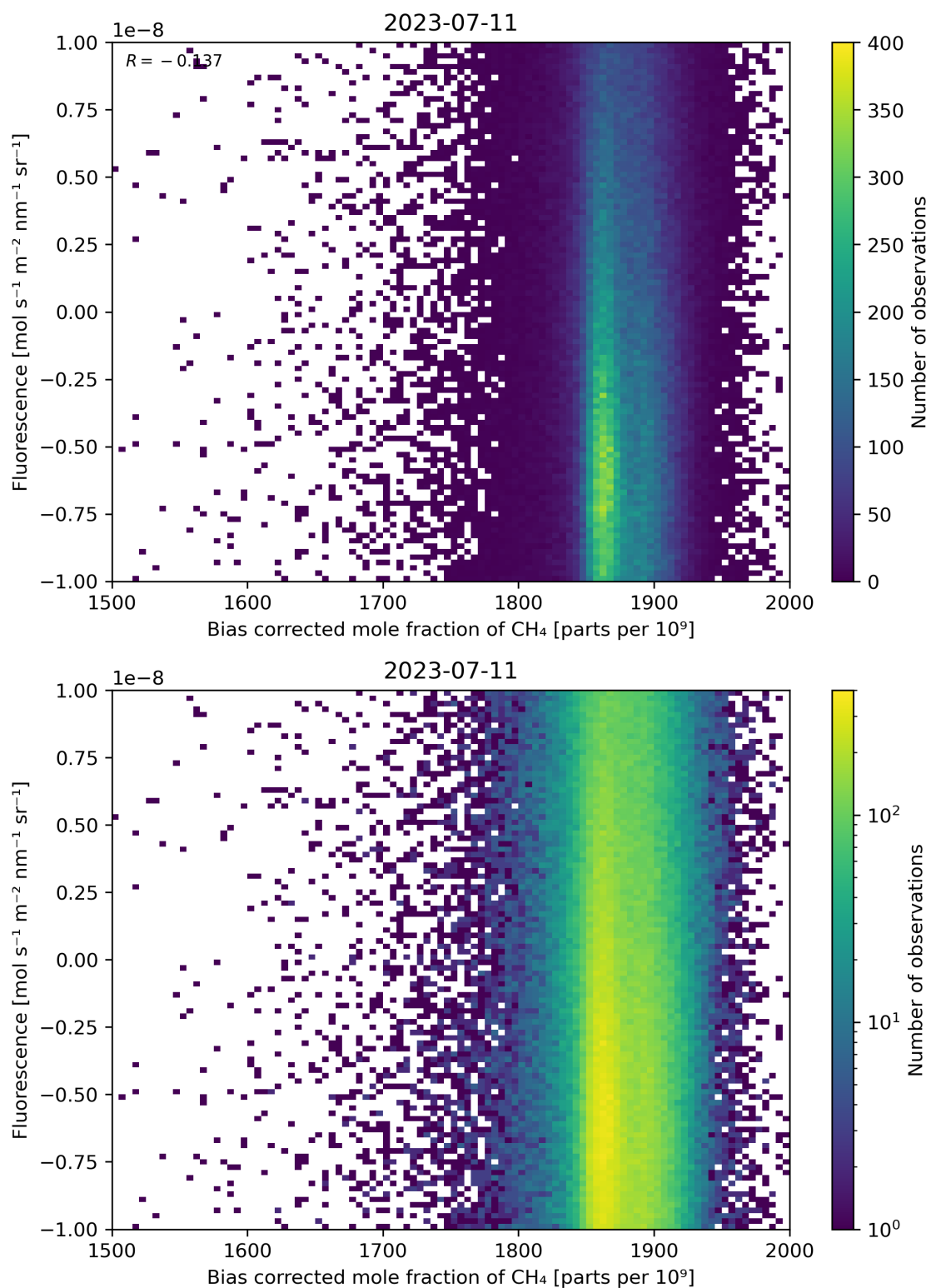
Figure 66: Scatter density plot of “Bias corrected mole fraction of \text{CH}_4 ” against “Fluorescence” for 2023-07-10 to 2023-07-12.
