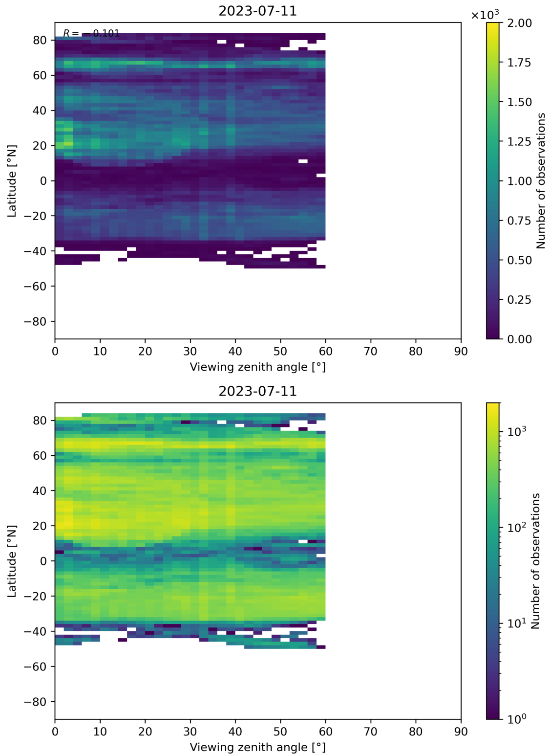
Figure 109: Scatter density plot of “Viewing zenith angle” against “Latitude” for 2023-07-10 to 2023-07-12.
