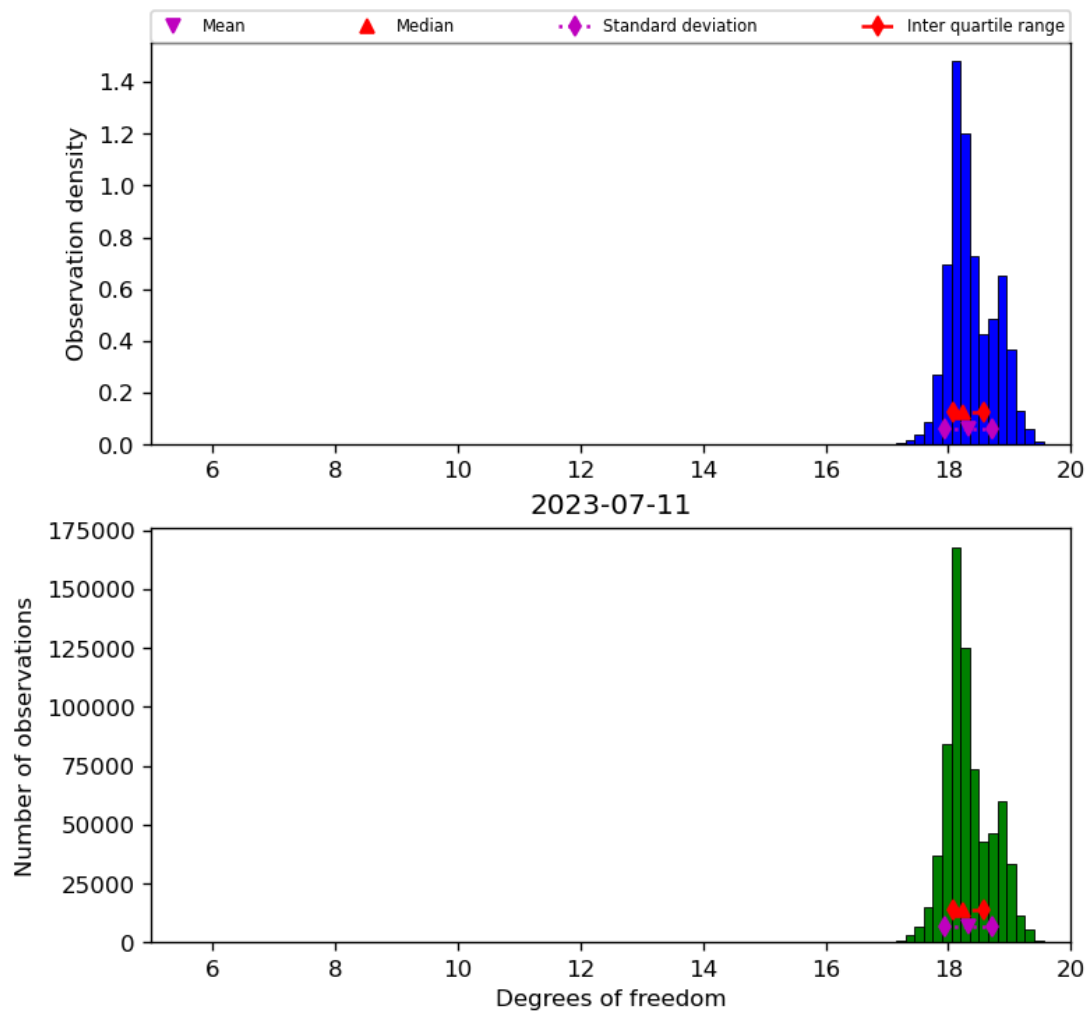
Figure 30: Histogram of “Degrees of freedom” for 2023-07-10 to 2023-07-12
