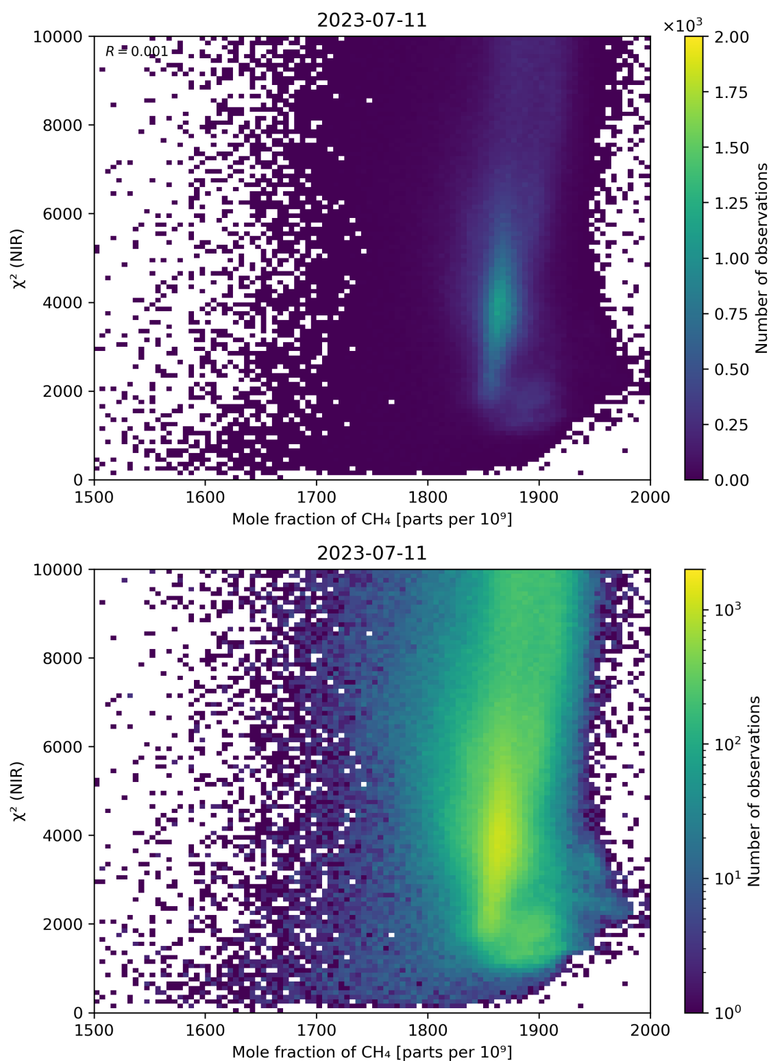
Figure 70: Scatter density plot of “Mole fraction of CH 4 ” against “ \chi^2 (NIR)” for 2023-07-10 to 2023-07-12.
