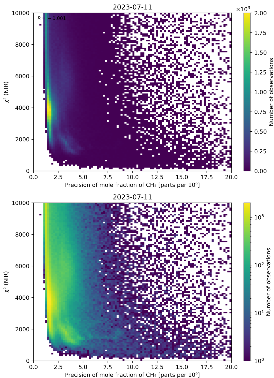
Figure 78: Scatter density plot of “Precision of mole fraction of CH 4 ” against “ \chi^2 (NIR)” for 2023-07-10 to 2023-07-12.
