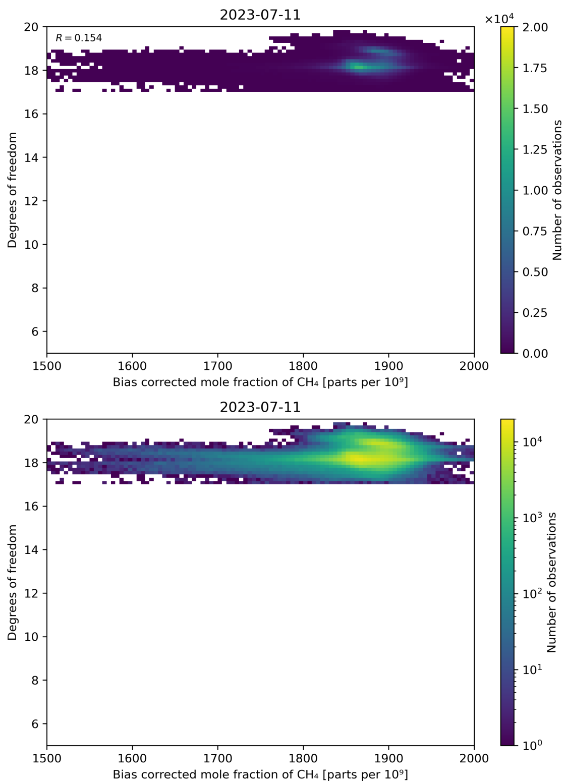
Figure 65: Scatter density plot of “Bias corrected mole fraction of CH 4 ” against “Degrees of freedom” for 2023-07-10 to 2023-07-12.
