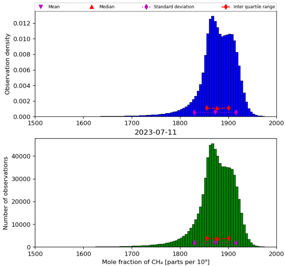
Figure 23: Histogram of “Mole fraction of CH 4 ” for 2023-07-10 to 2023-07-12
