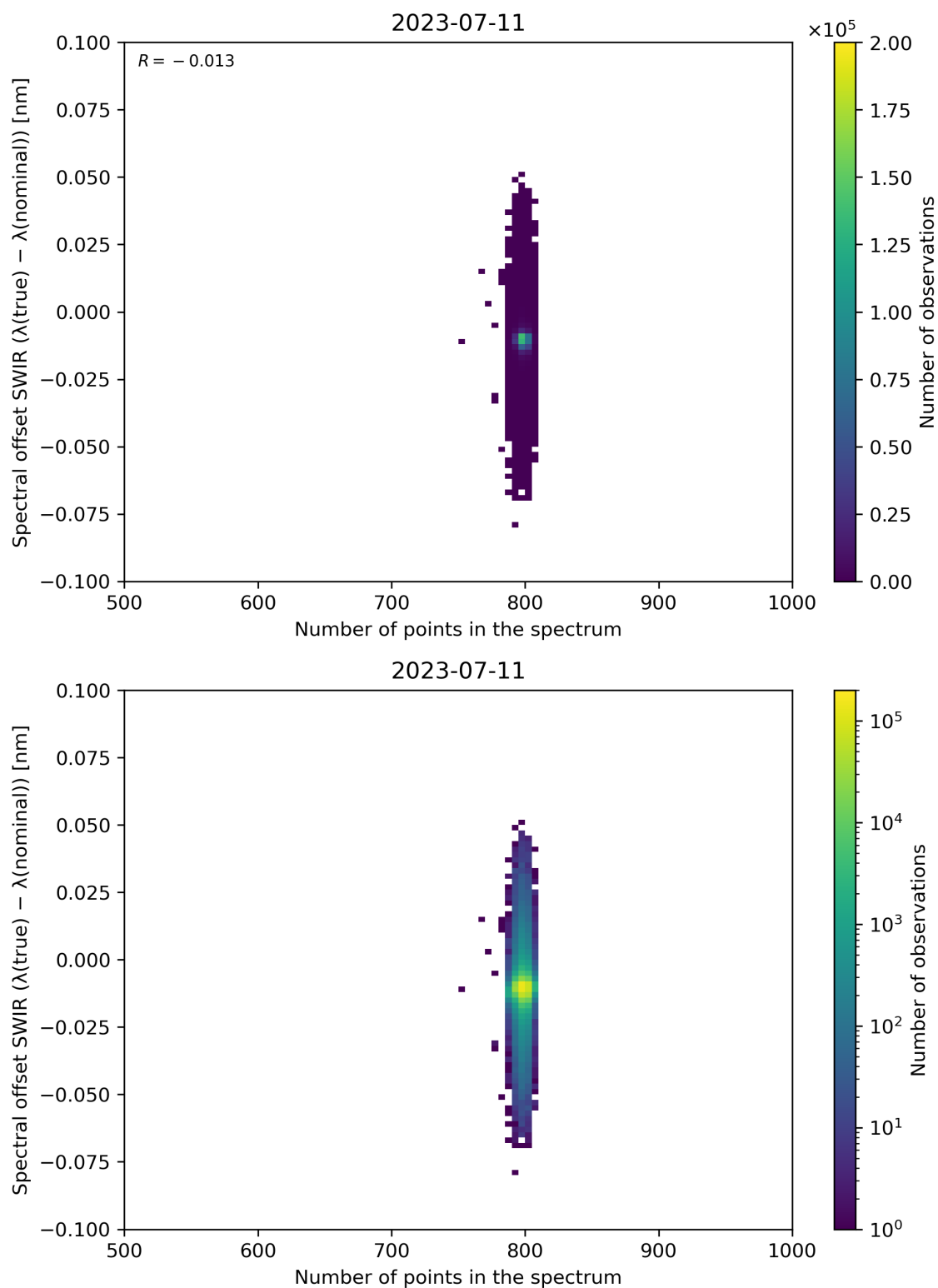
Figure 93: Scatter density plot of “Number of points in the spectrum” against “Spectral offset SWIR ( \lambda(\text{true}) - \lambda(\text{nominal}) )” for 2023-07-10 to 2023-07-12.
