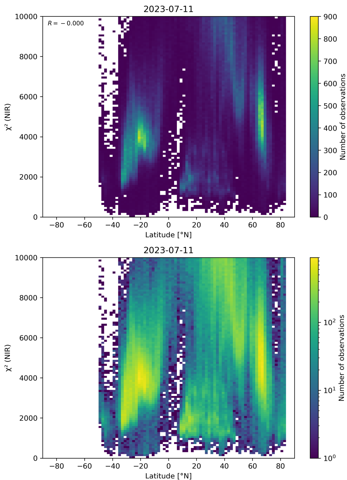
Figure 53: Scatter density plot of “Latitude” against “ \chi^2 (NIR)” for 2023-07-10 to 2023-07-12.
