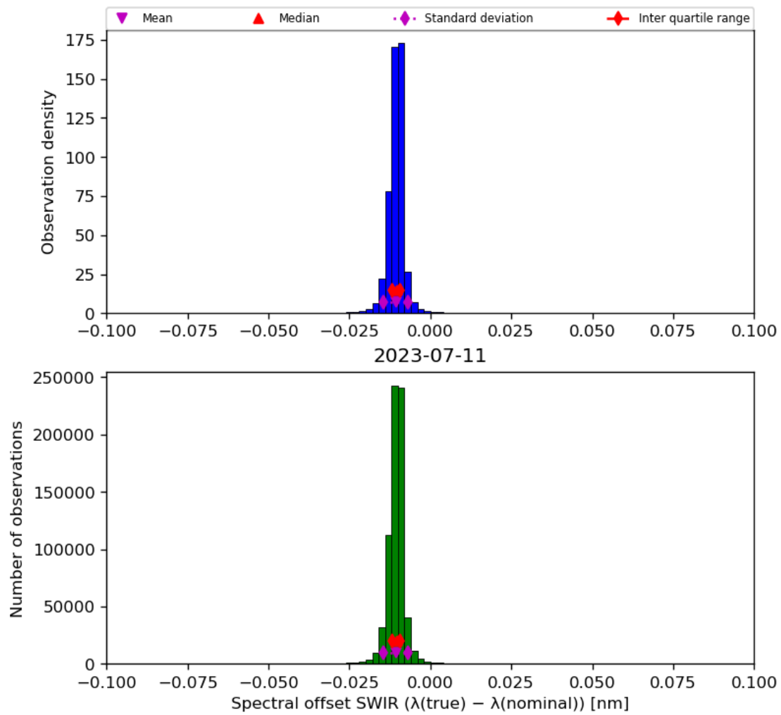
Figure 27: Histogram of “Spectral offset SWIR ( \lambda(\text{true}) - \lambda(\text{nominal}) )” for 2023-07-10 to 2023-07-12
