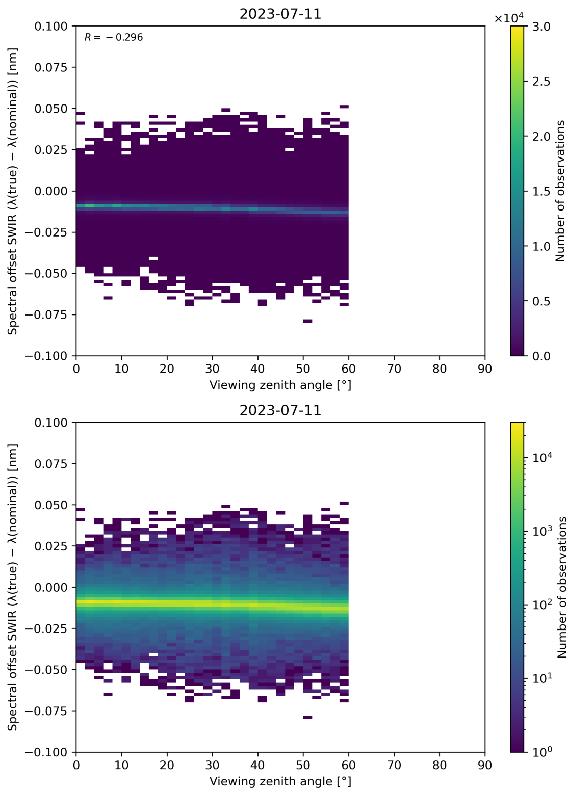
Figure 116: Scatter density plot of “Viewing zenith angle” against “Spectral offset SWIR ( \lambda(\text{true}) - \lambda(\text{nominal}) )” for 2023-07-10 to 2023-07-12.
