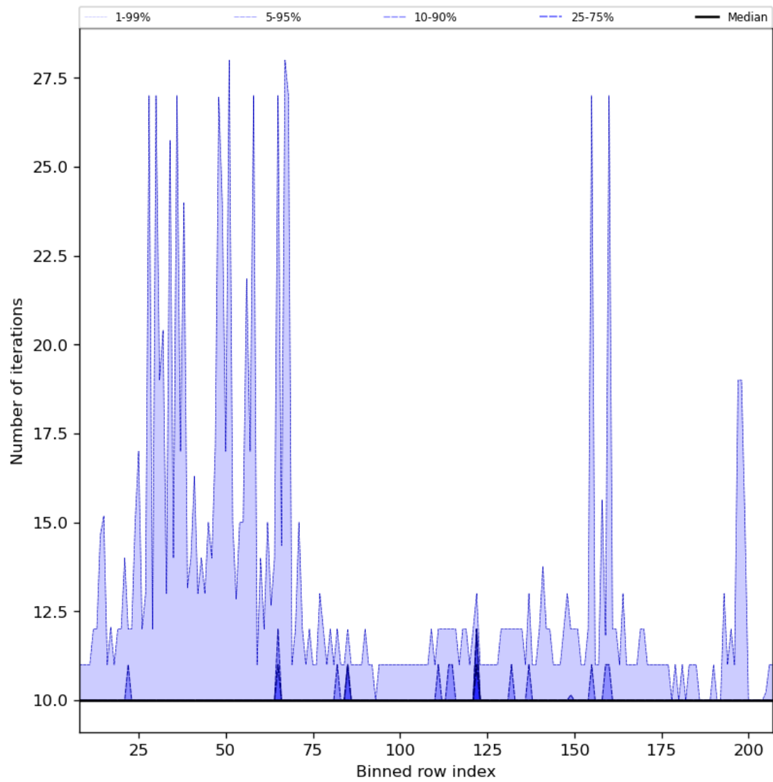
Figure 42: Along track statistics of “Number of iterations” for 2023-07-10 to 2023-07-12
