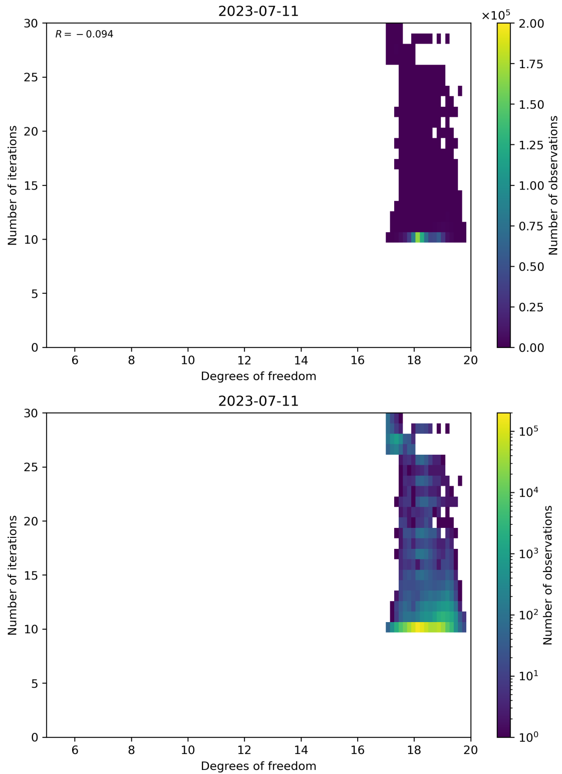
Figure 52: Scatter density plot of “Degrees of freedom” against “Number of iterations” for 2023-07-10 to 2023-07-12.
