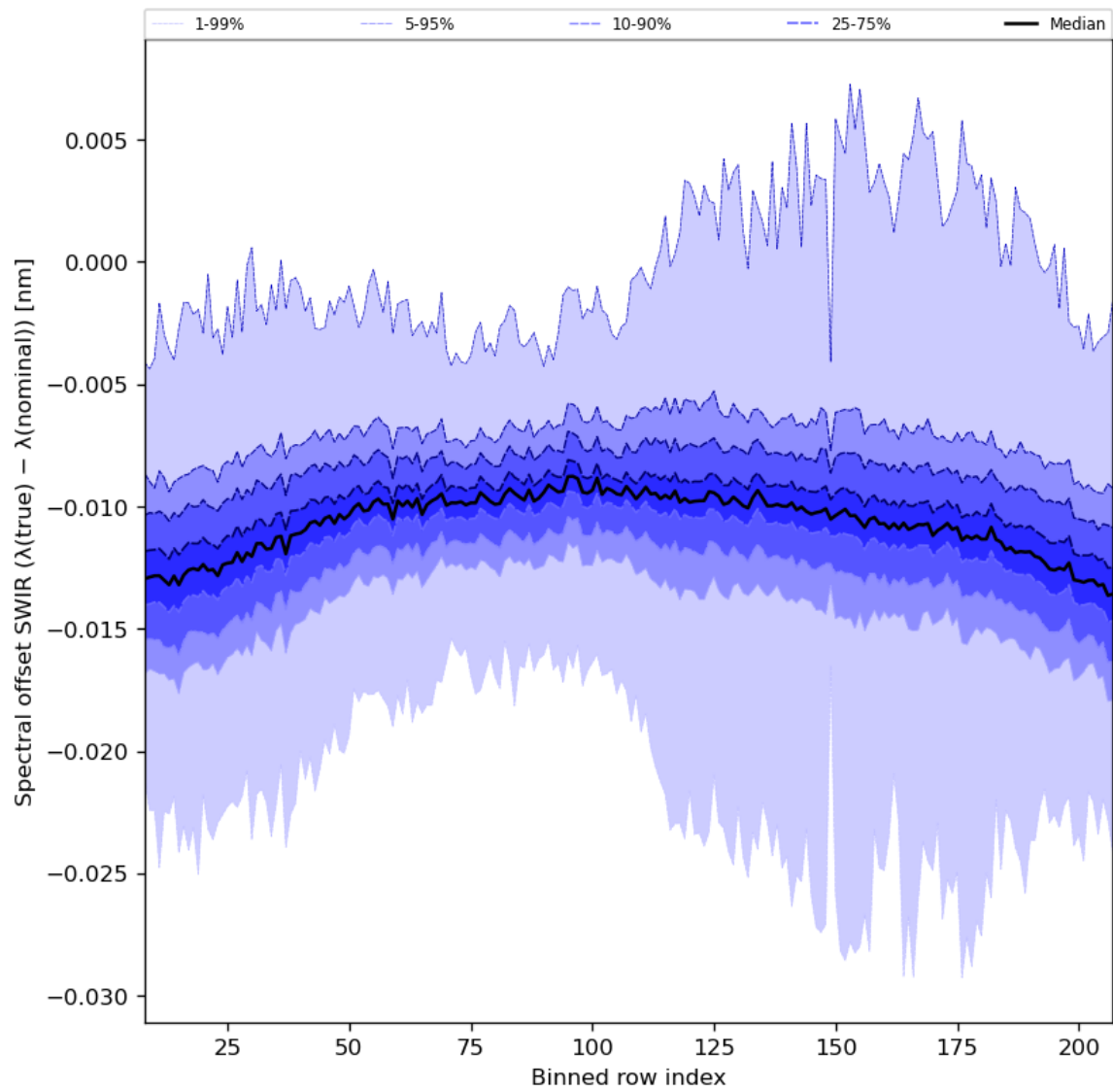
Figure 38: Along track statistics of “Spectral offset SWIR ( \lambda(\text{true}) - \lambda(\text{nominal}) )” for 2023-07-10 to 2023-07-12
