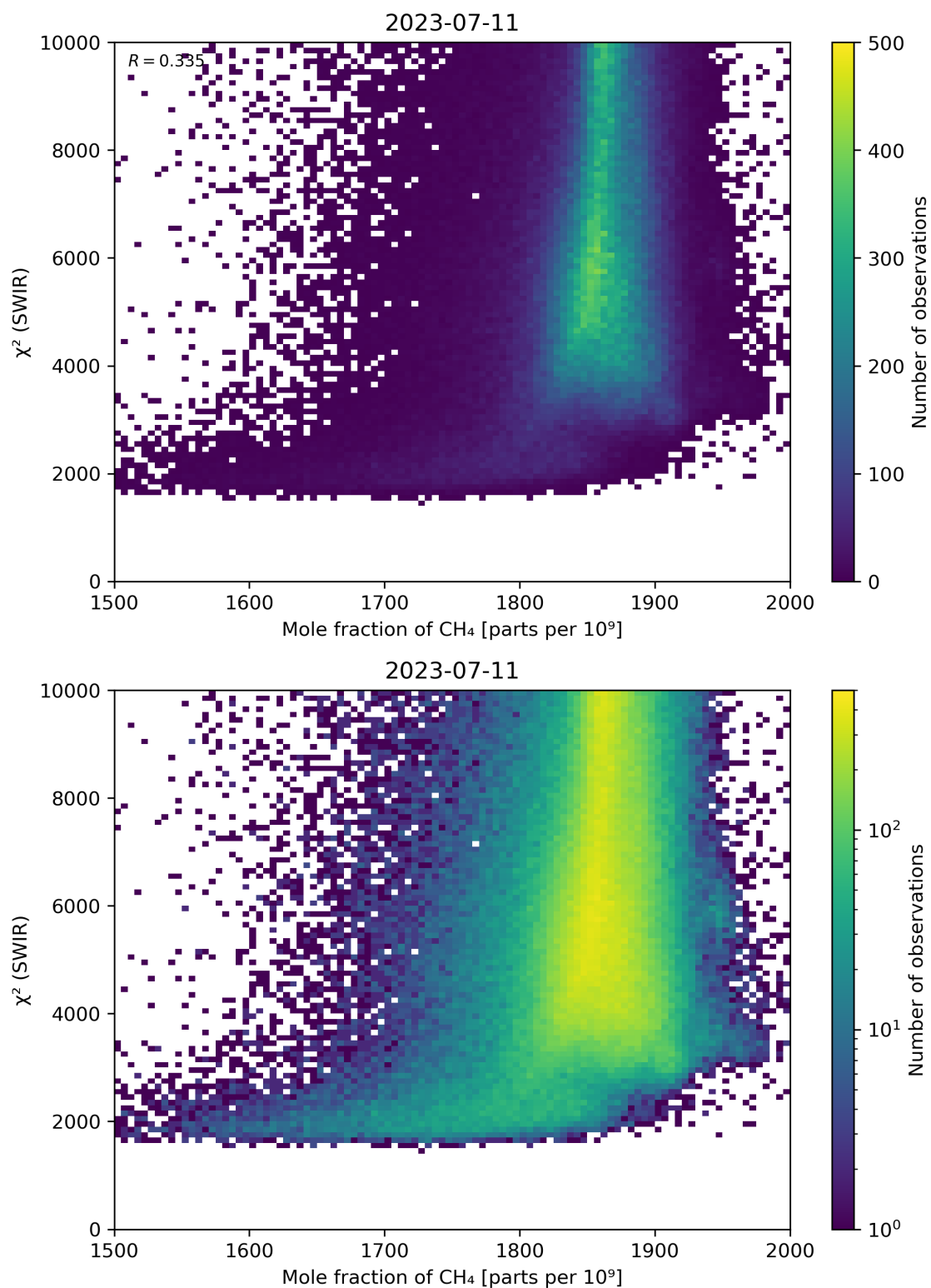
Figure 71: Scatter density plot of “Mole fraction of CH 4 ” against “ \chi^2 (SWIR)” for 2023-07-10 to 2023-07-12.
