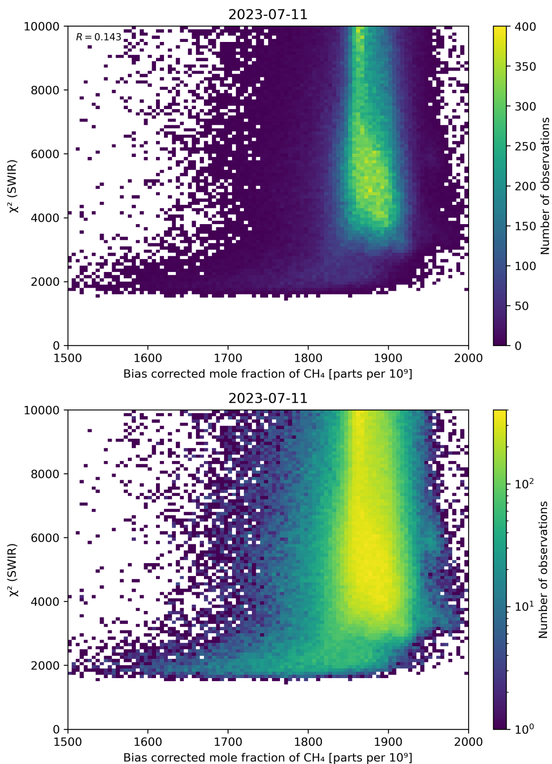
Figure 64: Scatter density plot of “Bias corrected mole fraction of \text{CH}_4 ” against “ \chi^2 (SWIR)” for 2023-07-10 to 2023-07-12.
