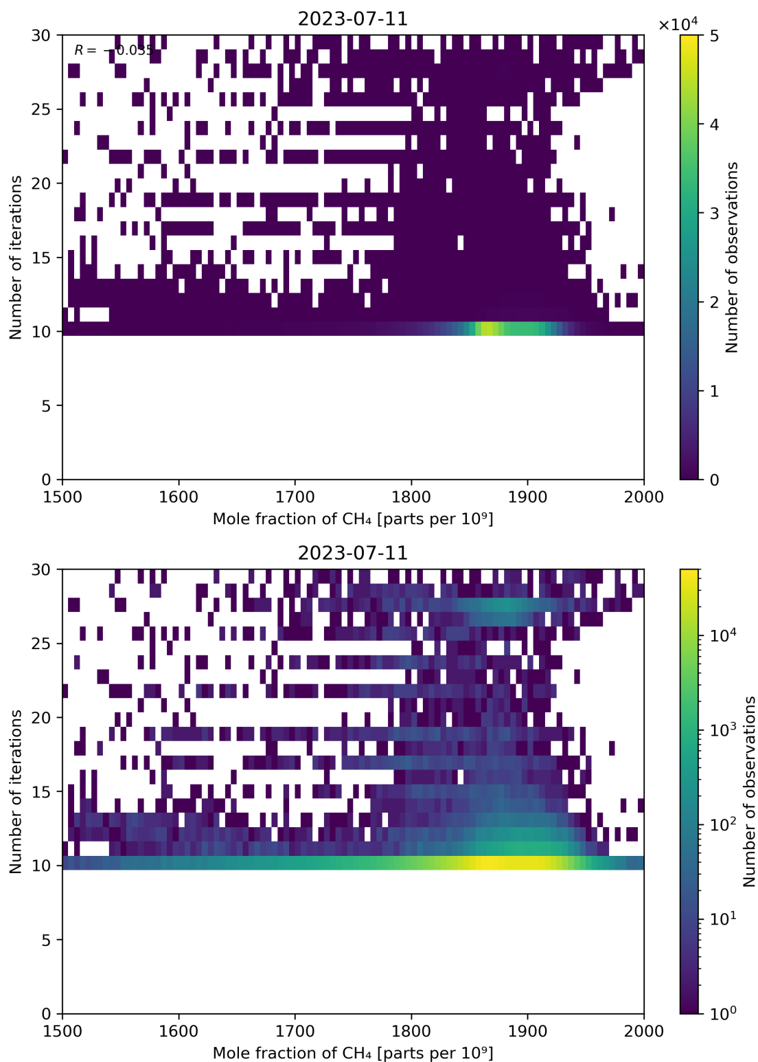
Figure 76: Scatter density plot of “Mole fraction of CH 4 ” against “Number of iterations” for 2023-07-10 to 2023-07-12.
