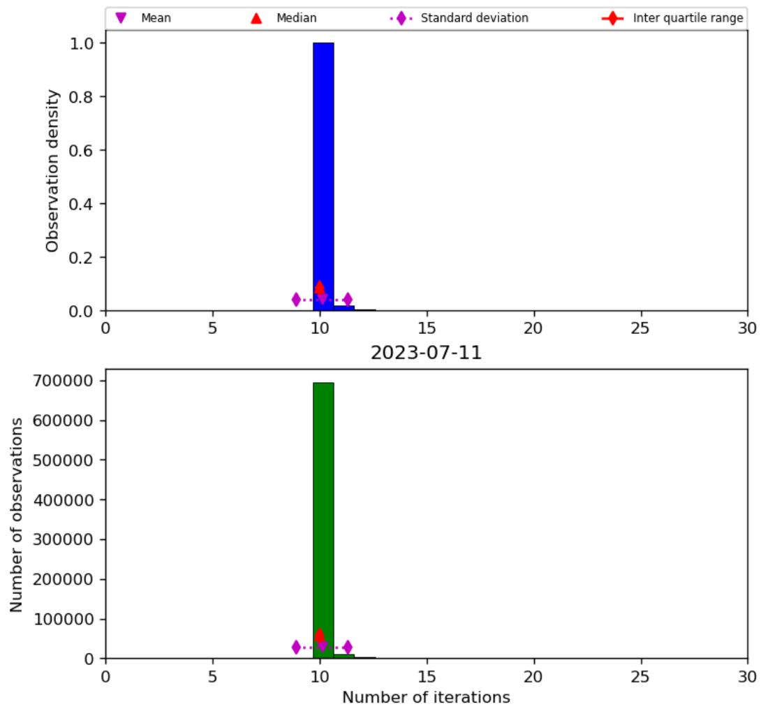
Figure 31: Histogram of “Number of iterations” for 2023-07-10 to 2023-07-12
