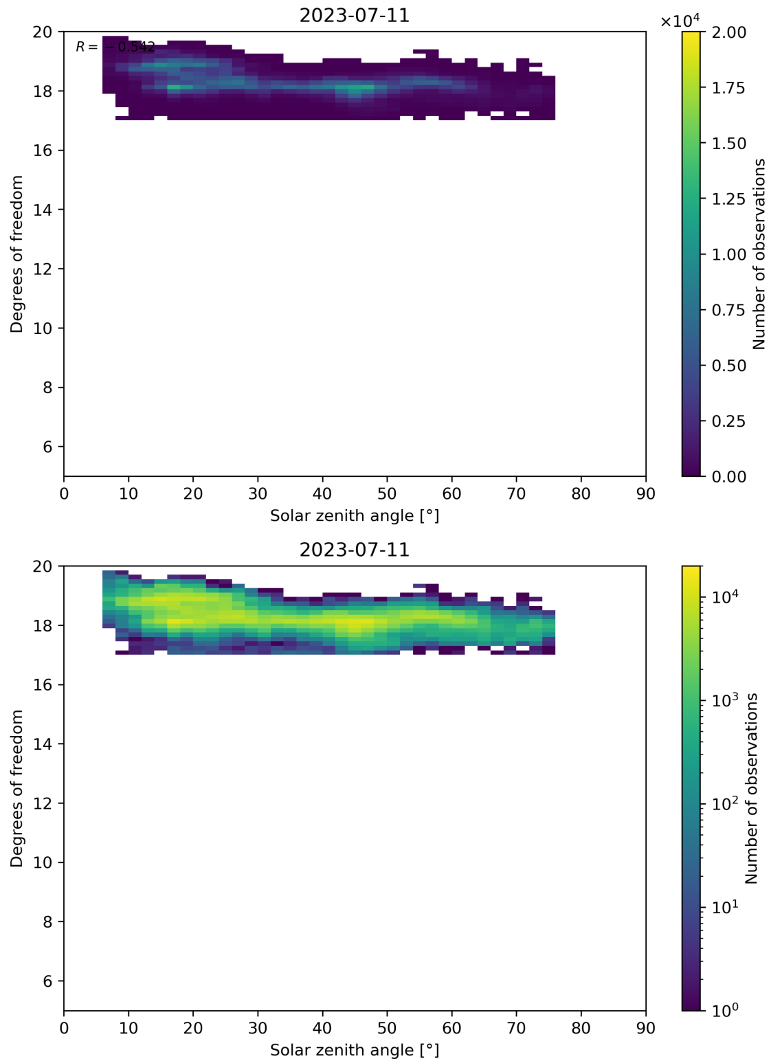
Figure 96: Scatter density plot of “Solar zenith angle” against “Degrees of freedom” for 2023-07-10 to 2023-07-12.
