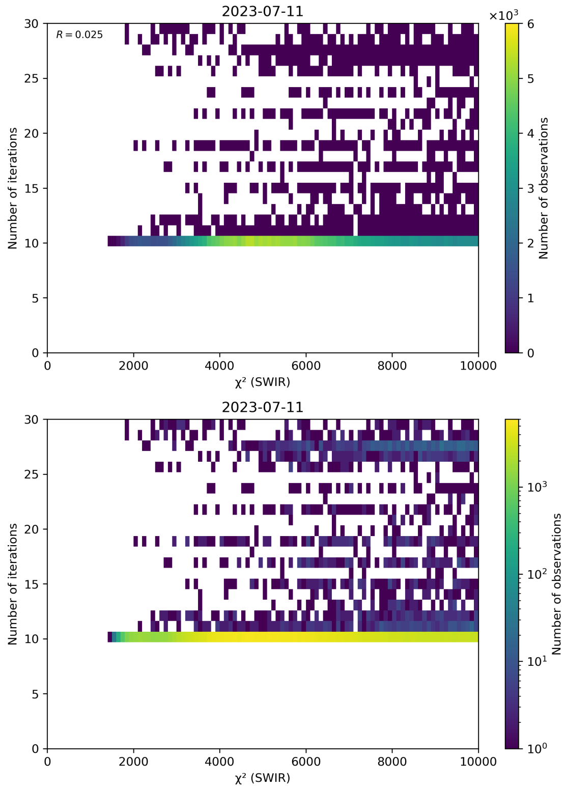
Figure 50: Scatter density plot of “ \chi^2 (SWIR)” against “Number of iterations” for 2023-07-10 to 2023-07-12.
