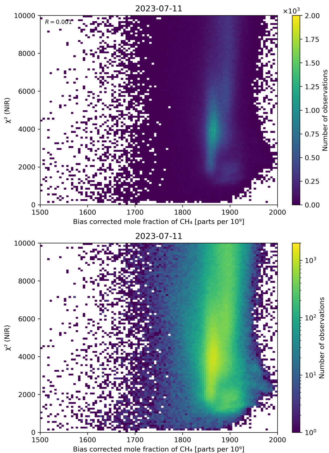
Figure 63: Scatter density plot of “Bias corrected mole fraction of CH 4 ” against “ \chi^2 (NIR)” for 2023-07-10 to 2023-07-12.
