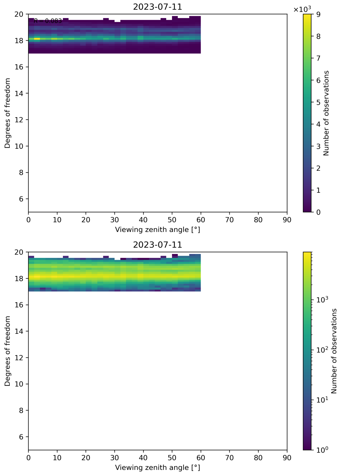
Figure 107: Scatter density plot of “Viewing zenith angle” against “Degrees of freedom” for 2023-07-10 to 2023-07-12.
