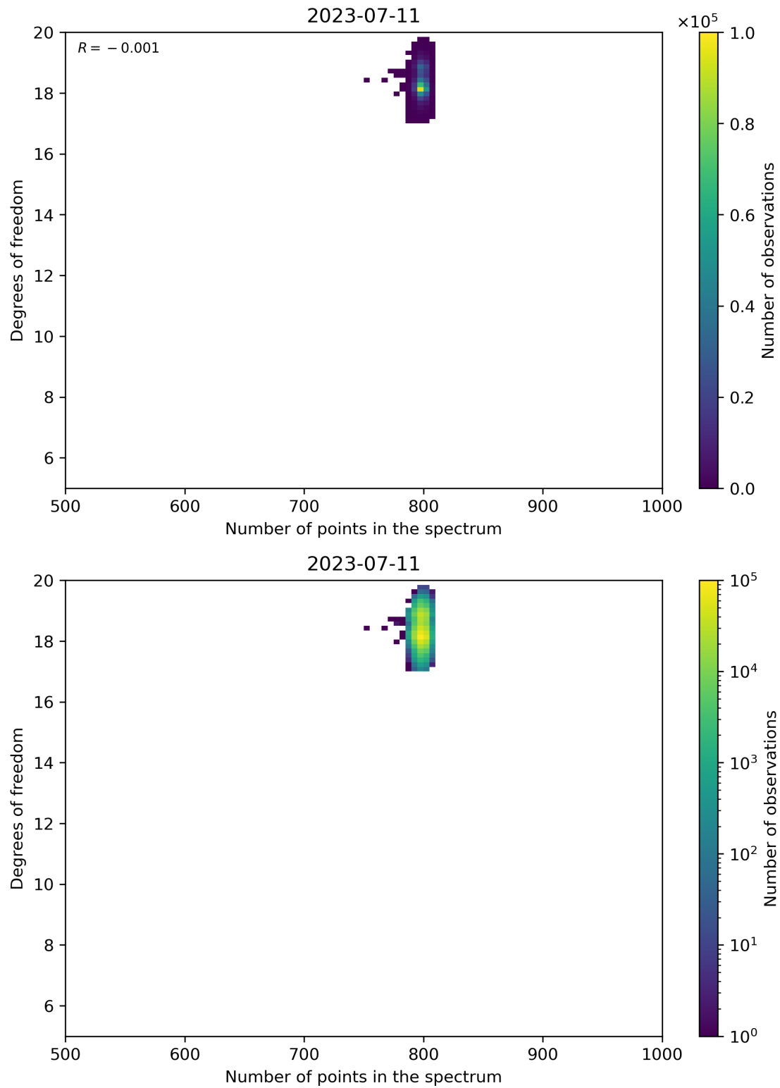
Figure 90: Scatter density plot of “Number of points in the spectrum” against “Degrees of freedom” for 2023-07-10 to 2023-07-12.
