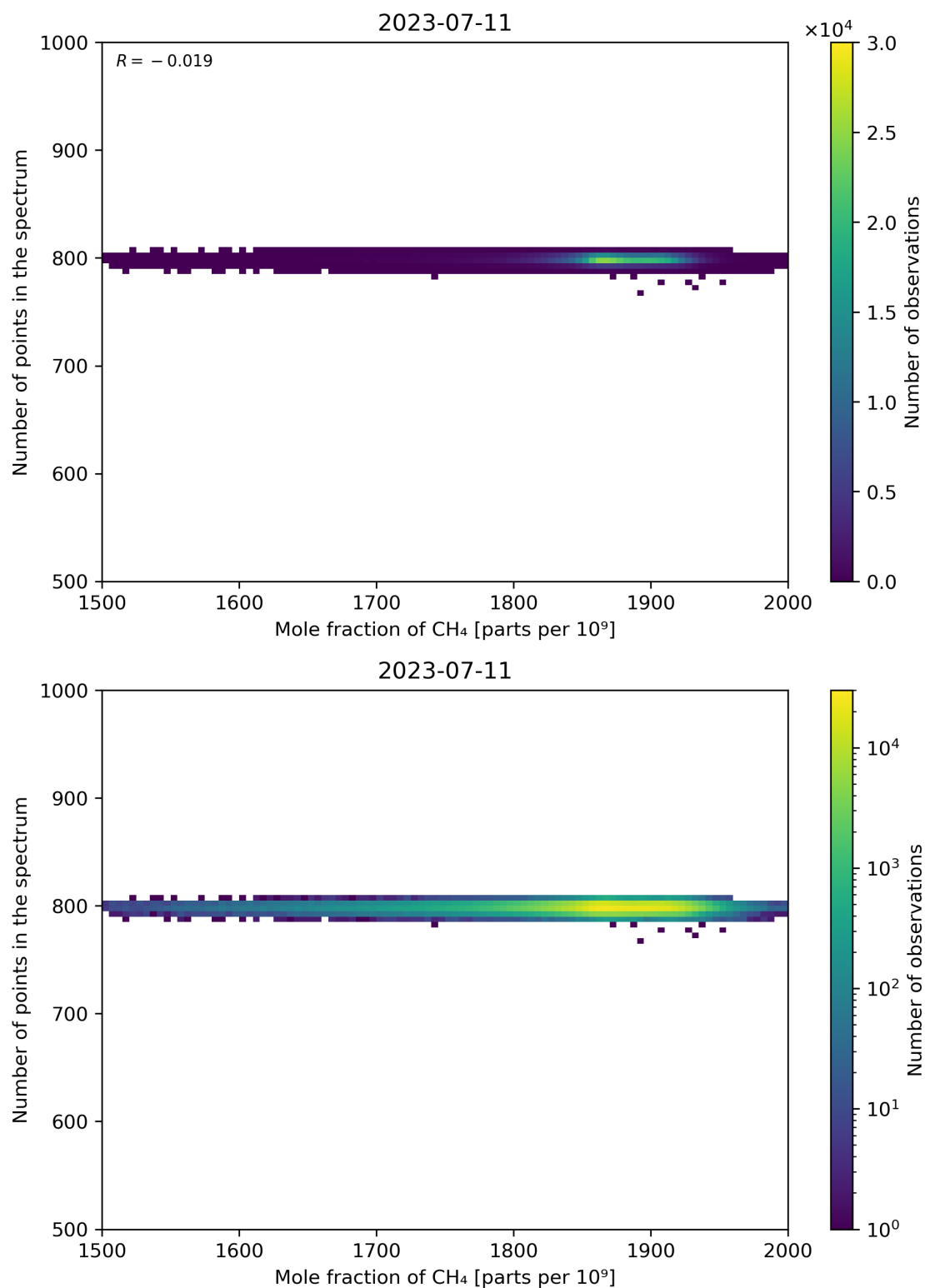
Figure 77: Scatter density plot of “Mole fraction of CH 4 ” against “Number of points in the spectrum” for 2023-07-10 to 2023-07-12.
