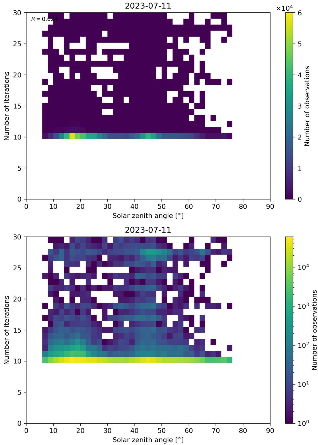
Figure 102: Scatter density plot of “Solar zenith angle” against “Number of iterations” for 2023-07-10 to 2023-07-12.
