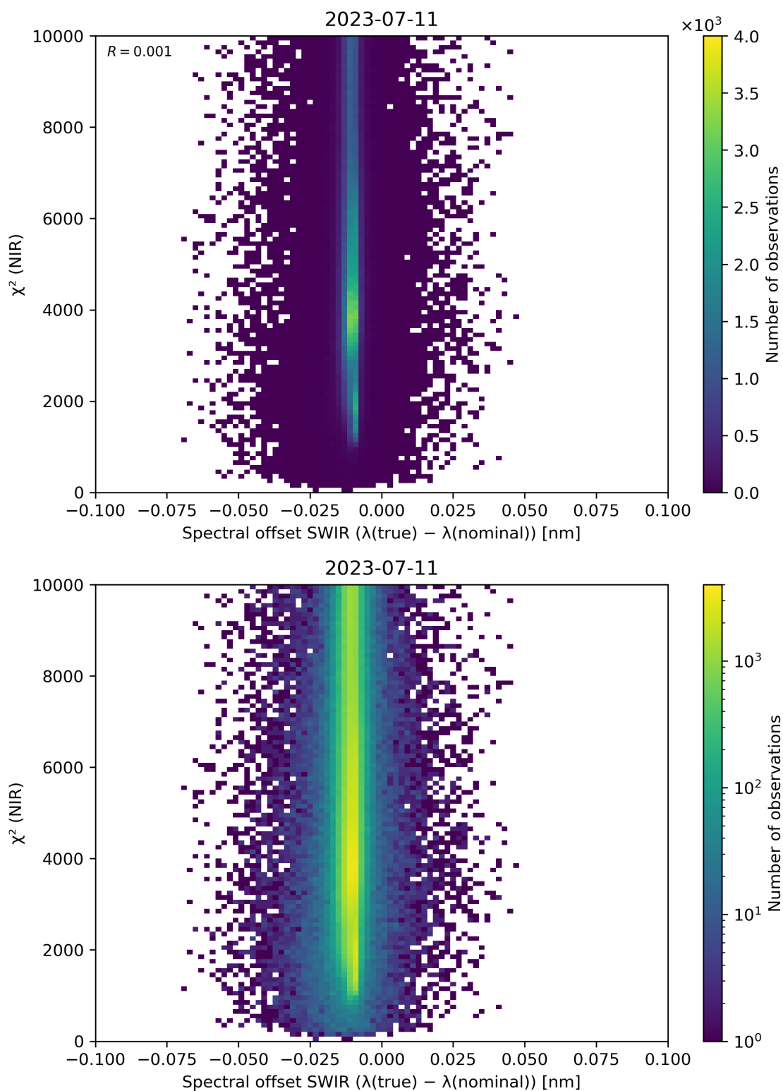
Figure 117: Scatter density plot of “Spectral offset SWIR ( \lambda(\text{true}) - \lambda(\text{nominal}) )” against “ \chi^2 (NIR)” for 2023-07-10 to 2023-07-12.
