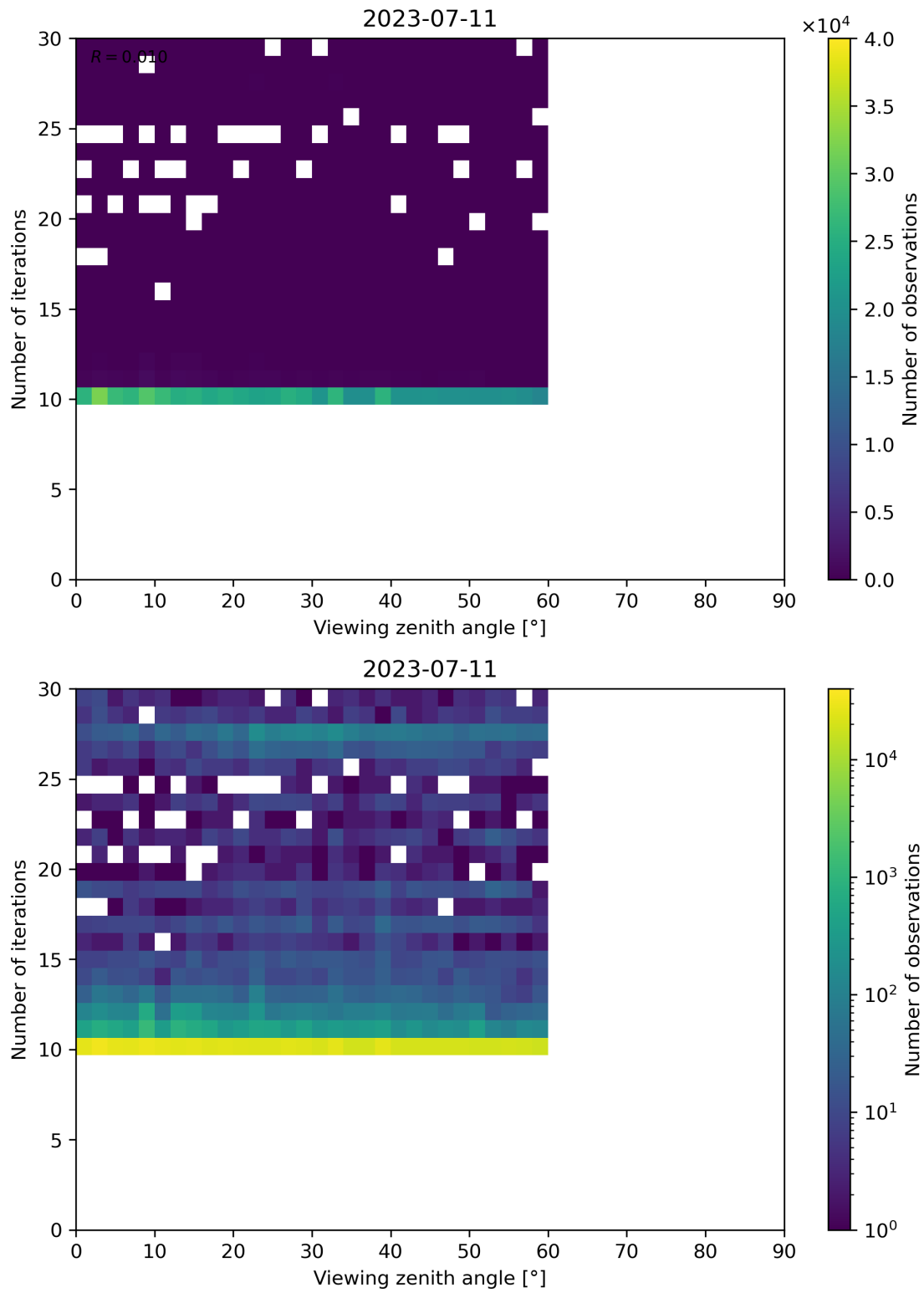
Figure 113: Scatter density plot of “Viewing zenith angle” against “Number of iterations” for 2023-07-10 to 2023-07-12.
