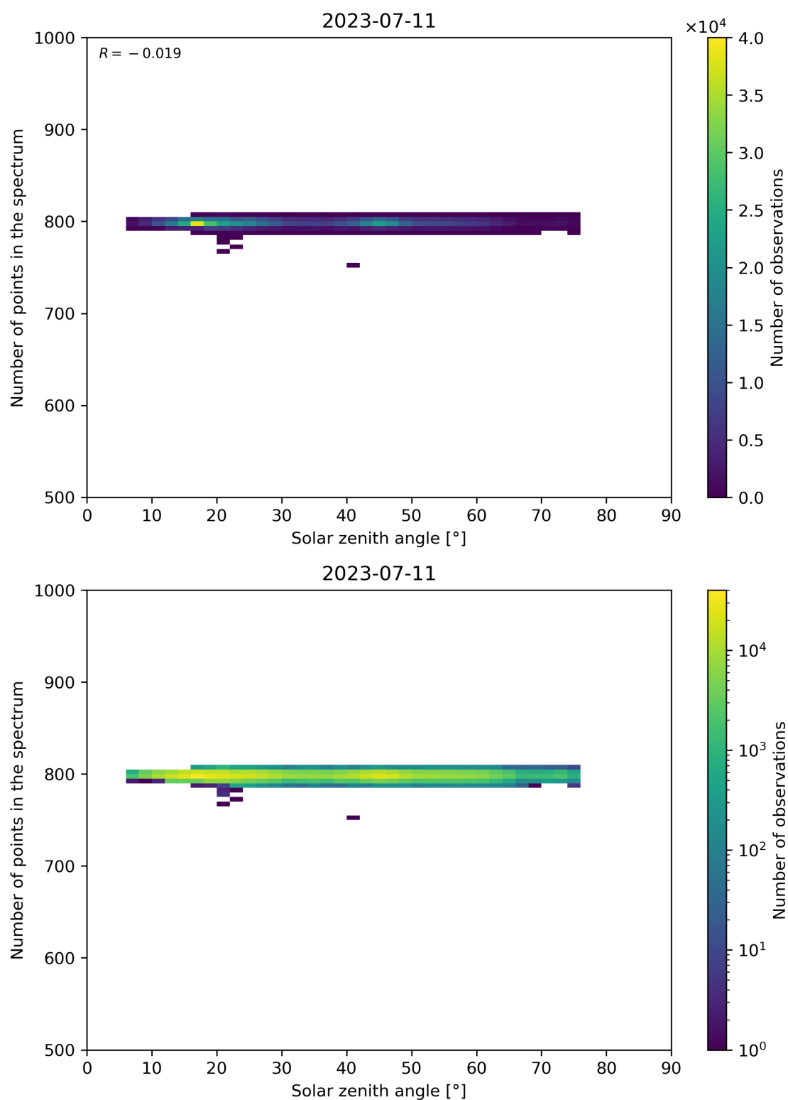
Figure 103: Scatter density plot of “Solar zenith angle” against “Number of points in the spectrum” for 2023-07-10 to 2023-07-12.
