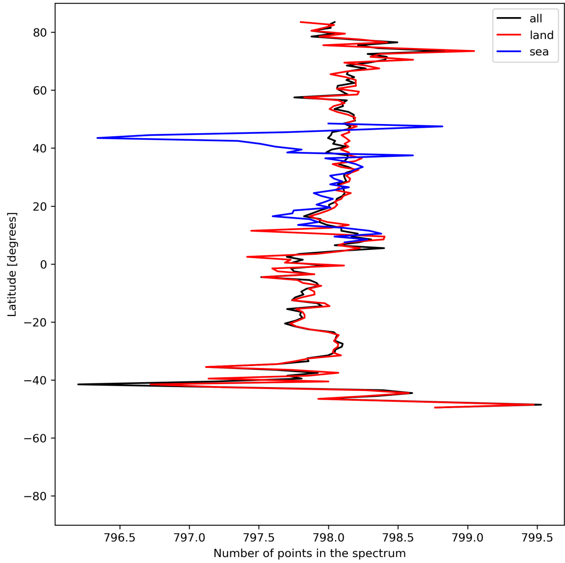
Figure 15: Zonal average of “Number of points in the spectrum” for 2023-07-10 to 2023-07-12.
