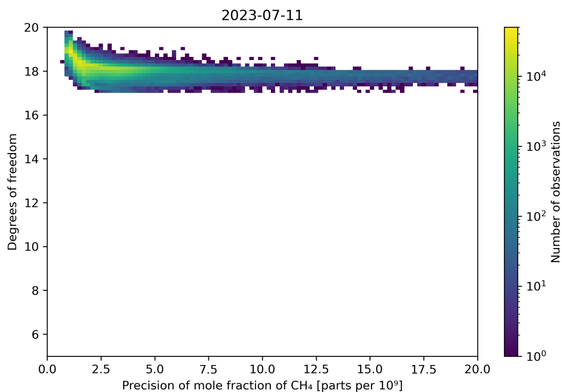
Figure 80: Scatter density plot of “Precision of mole fraction of CH 4 ” against “Degrees of freedom” for 2023-07-10 to 2023-07-12.
