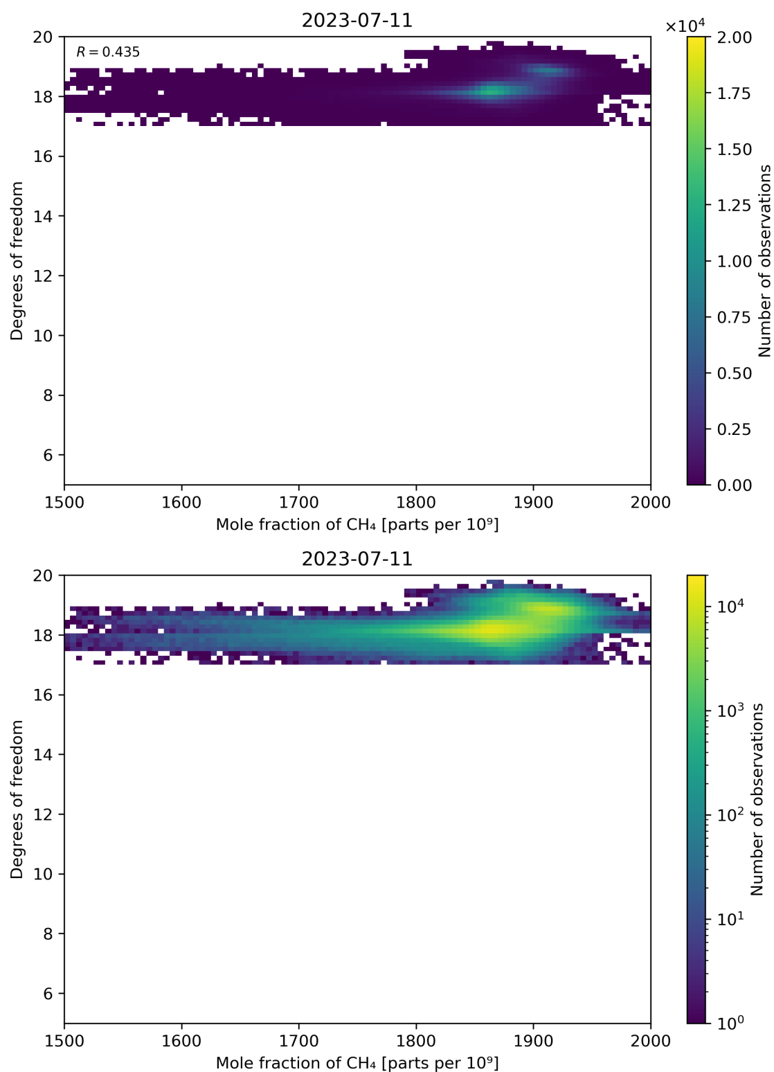
Figure 72: Scatter density plot of “Mole fraction of CH 4 ” against “Degrees of freedom” for 2023-07-10 to 2023-07-12.
