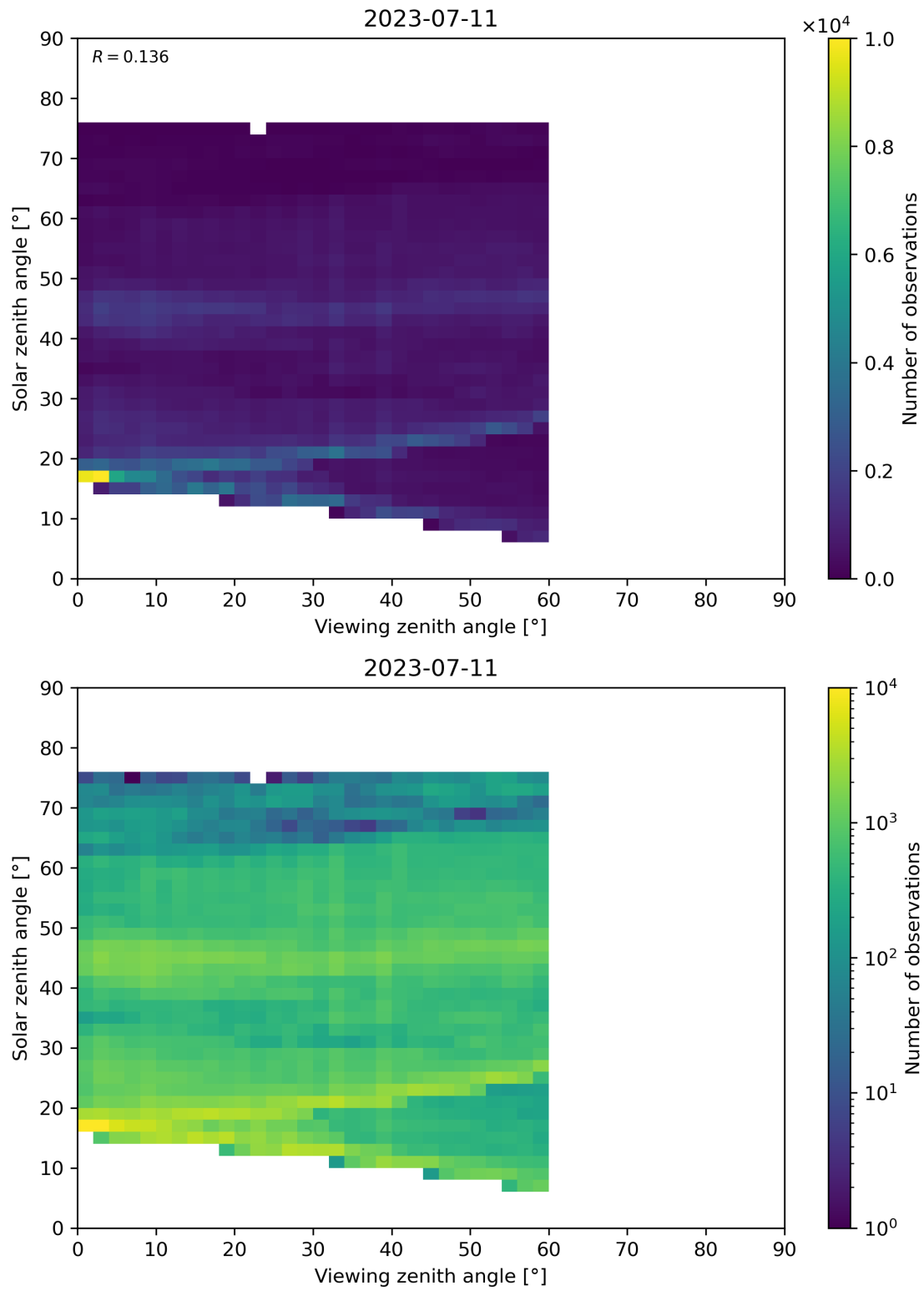
Figure 115: Scatter density plot of “Viewing zenith angle” against “Solar zenith angle” for 2023-07-10 to 2023-07-12.
