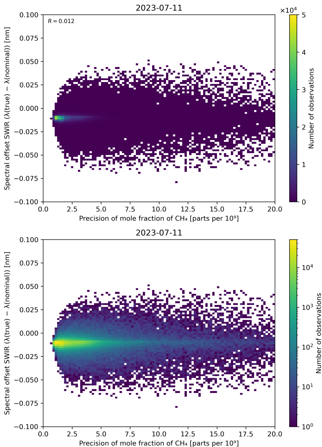
Figure 85: Scatter density plot of “Precision of mole fraction of CH 4 ” against “Spectral offset SWIR ( \lambda(\text{true}) - \lambda(\text{nominal}) )” for 2023-07-10 to 2023-07-12.
