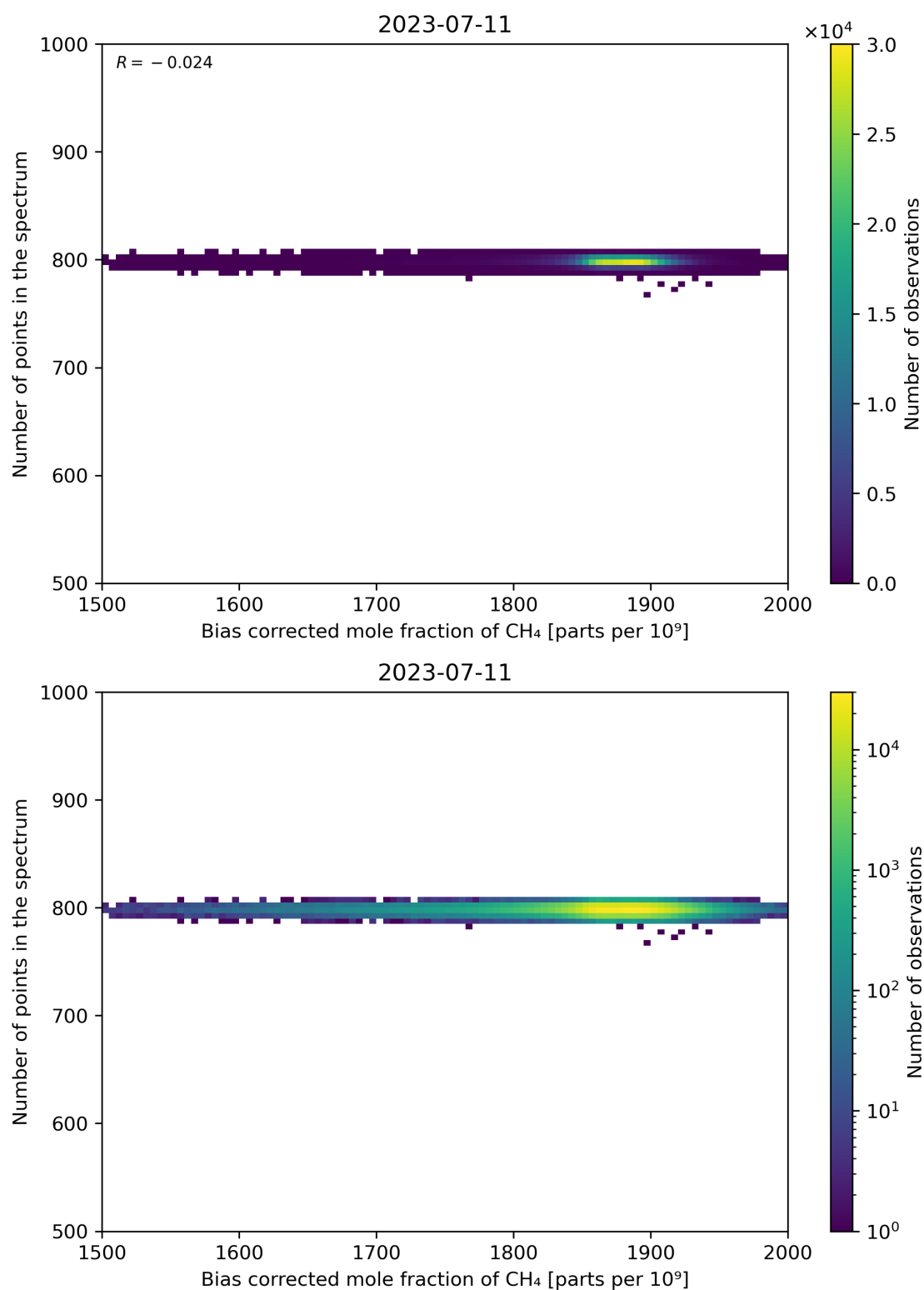
Figure 68: Scatter density plot of “Bias corrected mole fraction of CH 4 ” against “Number of points in the spectrum” for 2023-07-10 to 2023-07-12.
