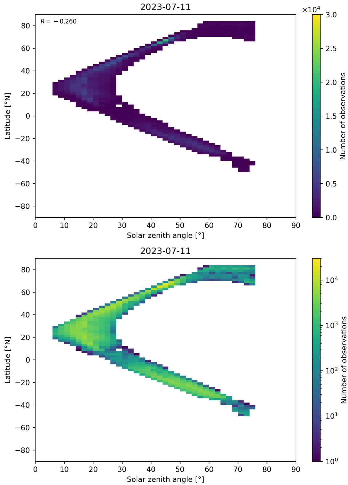
Figure 98: Scatter density plot of “Solar zenith angle” against “Latitude” for 2023-07-10 to 2023-07-12.
