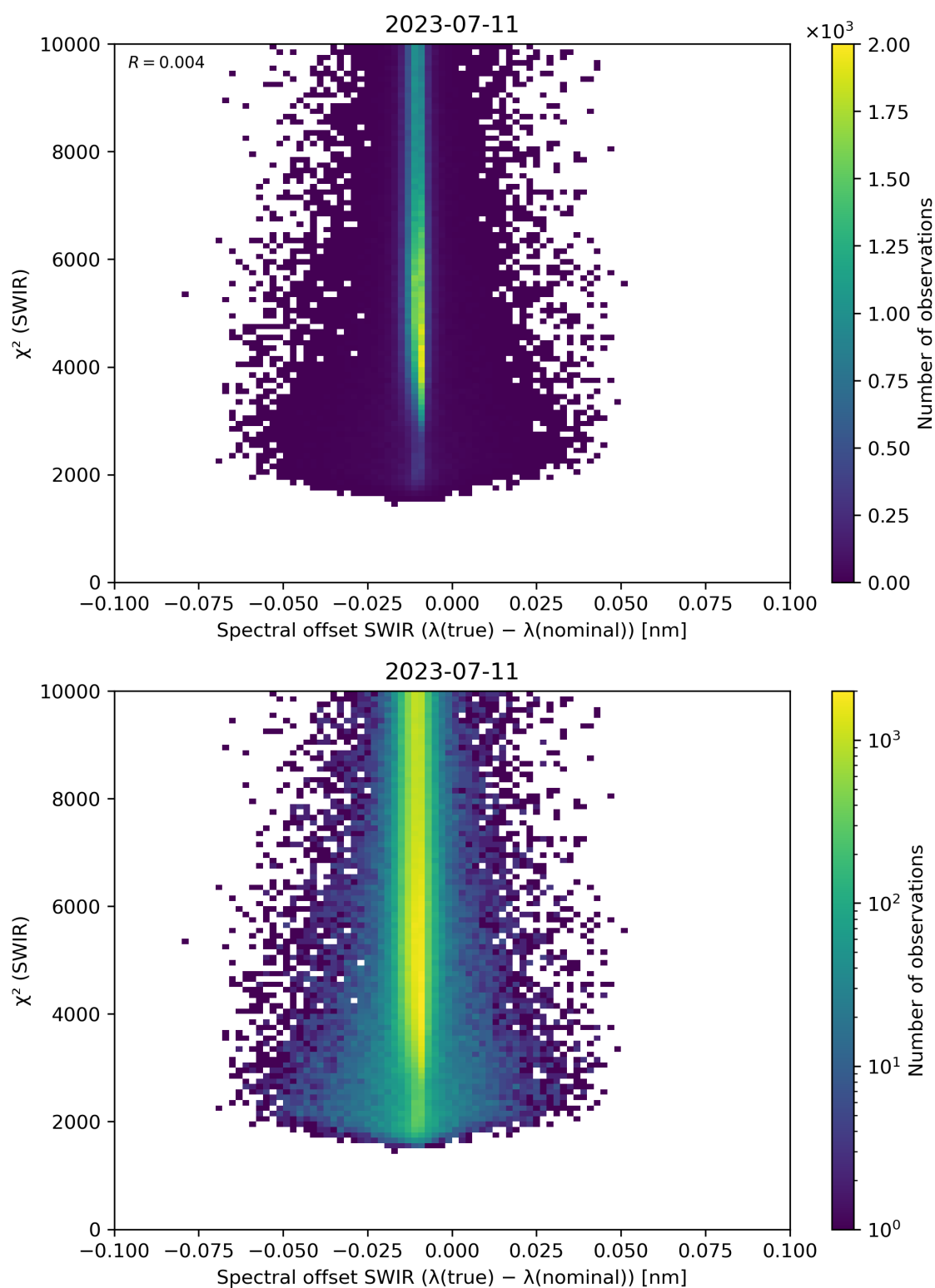
Figure 118: Scatter density plot of “Spectral offset SWIR ( \lambda(\text{true}) - \lambda(\text{nominal}) )” against “ \chi^2 (SWIR)” for 2023-07-10 to 2023-07-12.
