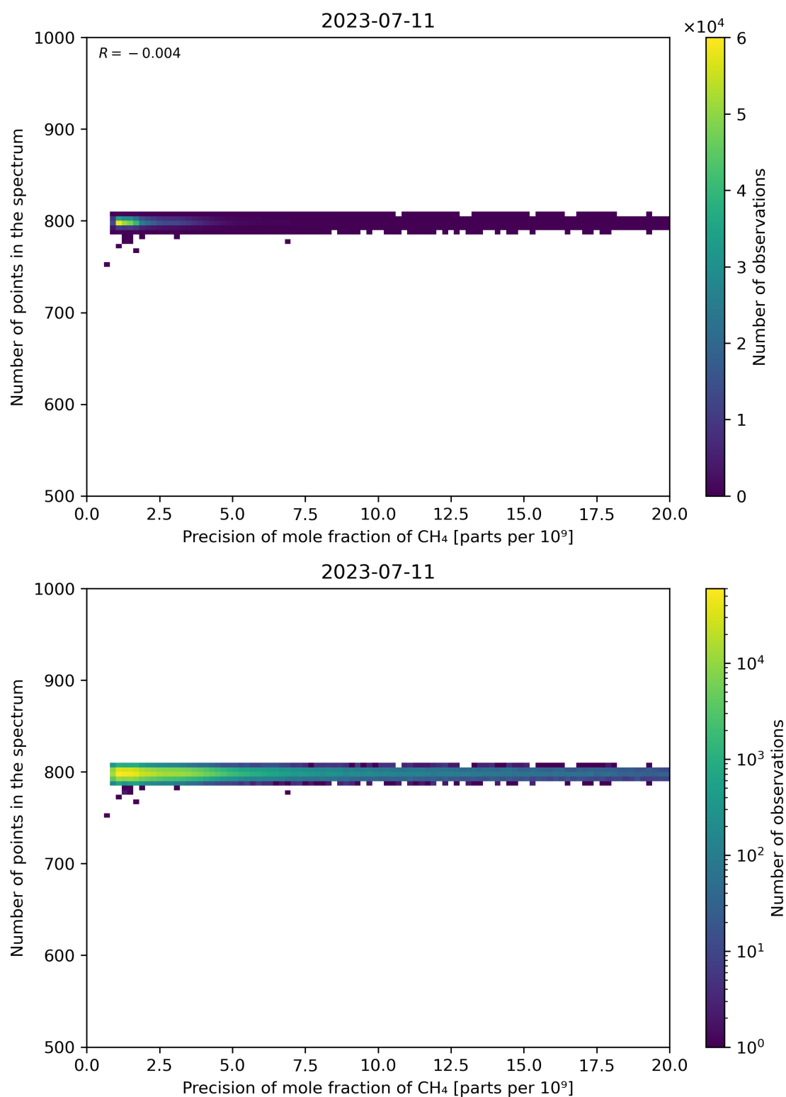
Figure 84: Scatter density plot of “Precision of mole fraction of CH 4 ” against “Number of points in the spectrum” for 2023-07-10 to 2023-07-12.
