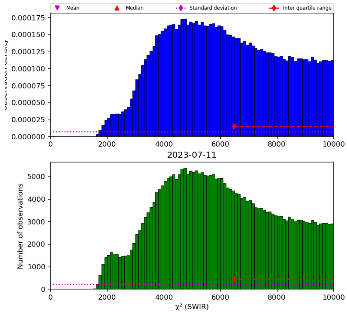
Figure 28: Histogram of “ \chi^2 (SWIR)” for 2023-07-10 to 2023-07-12
