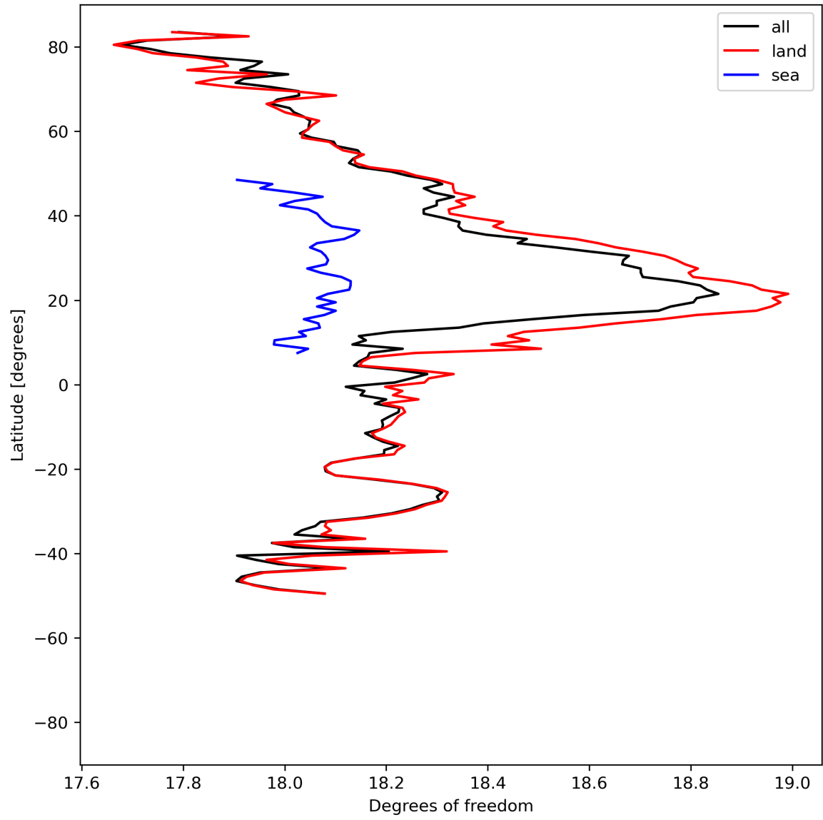
Figure 19: Zonal average of “Degrees of freedom” for 2023-07-10 to 2023-07-12.
