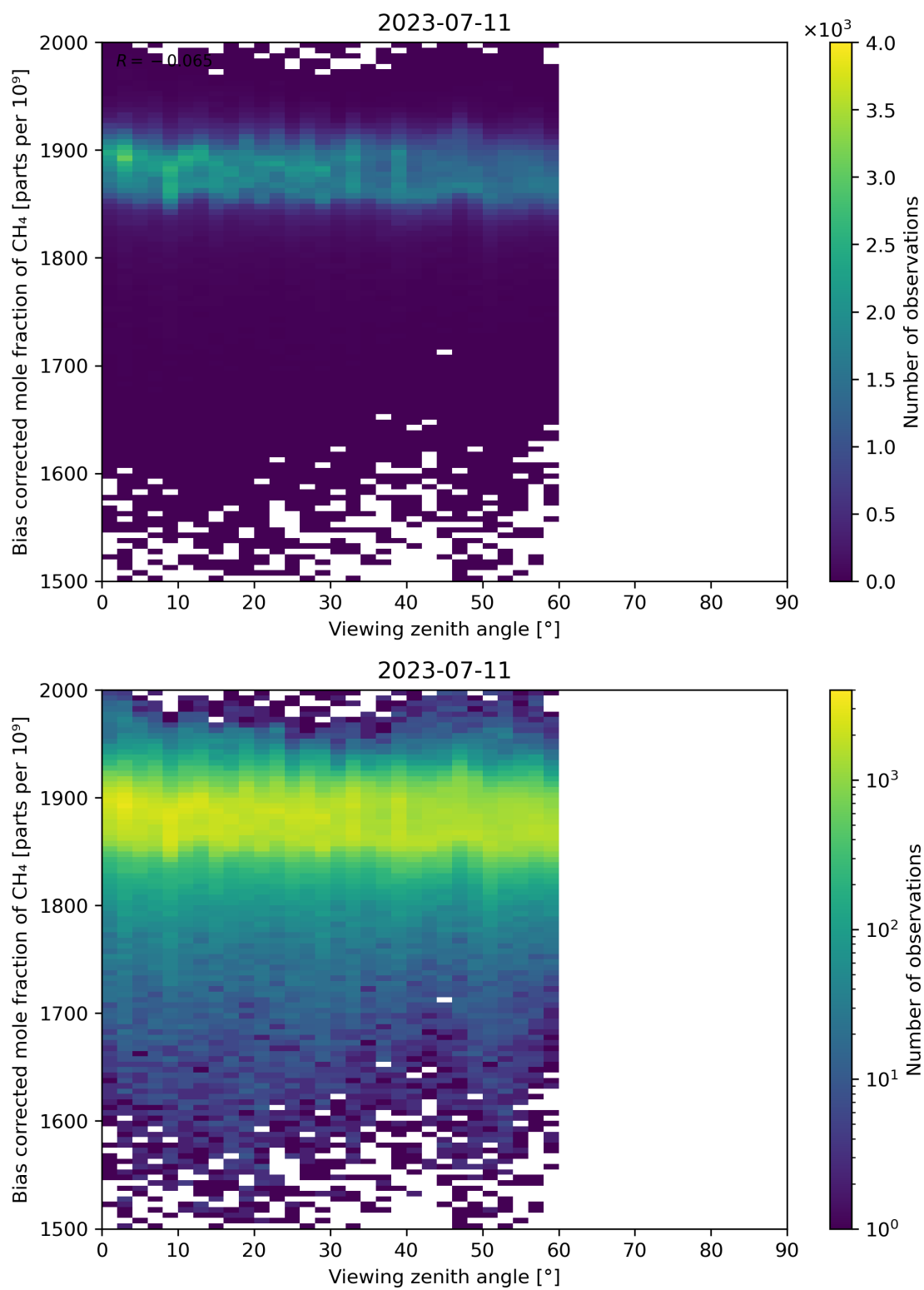
Figure 111: Scatter density plot of “Viewing zenith angle” against “Bias corrected mole fraction of CH 4 ” for 2023-07-10 to 2023-07-12.
