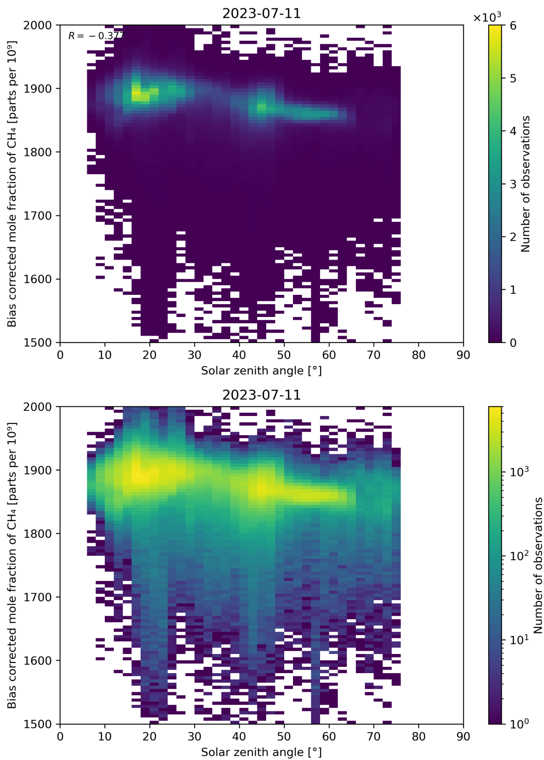
Figure 100: Scatter density plot of “Solar zenith angle” against “Bias corrected mole fraction of \text{CH}_4 ” for 2023-07-10 to 2023-07-12.
