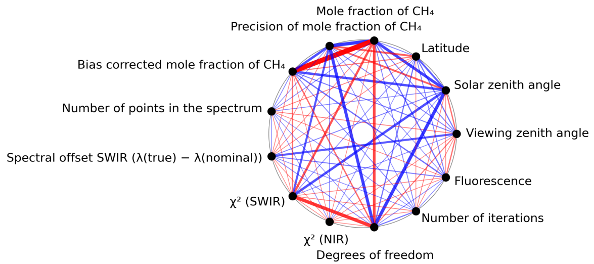
Figure 1: Map of correlation graph for 2023-07-10 to 2023-07-12.
