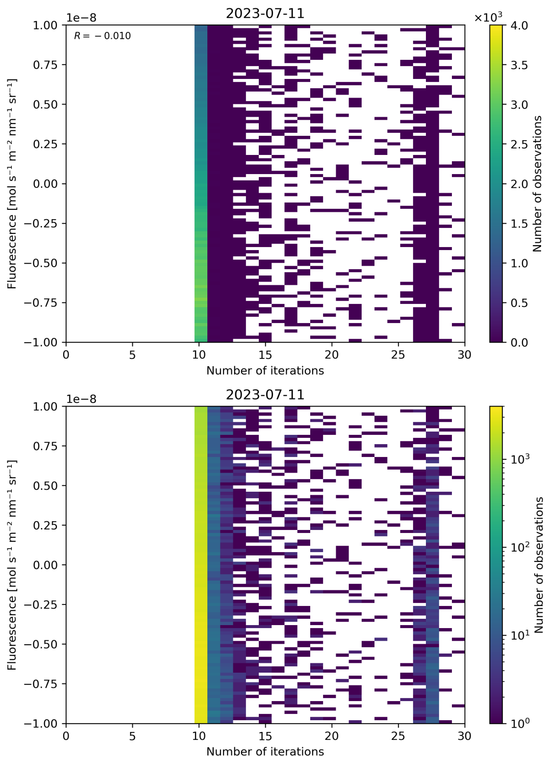
Figure 87: Scatter density plot of “Number of iterations” against “Fluorescence” for 2023-07-10 to 2023-07-12.
