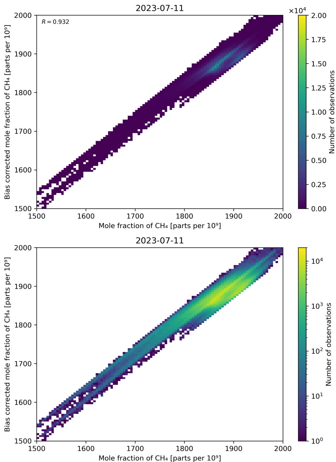
Figure 74: Scatter density plot of “Mole fraction of CH 4 ” against “Bias corrected mole fraction of CH 4 ” for 2023-07-10 to 2023-07-12.
