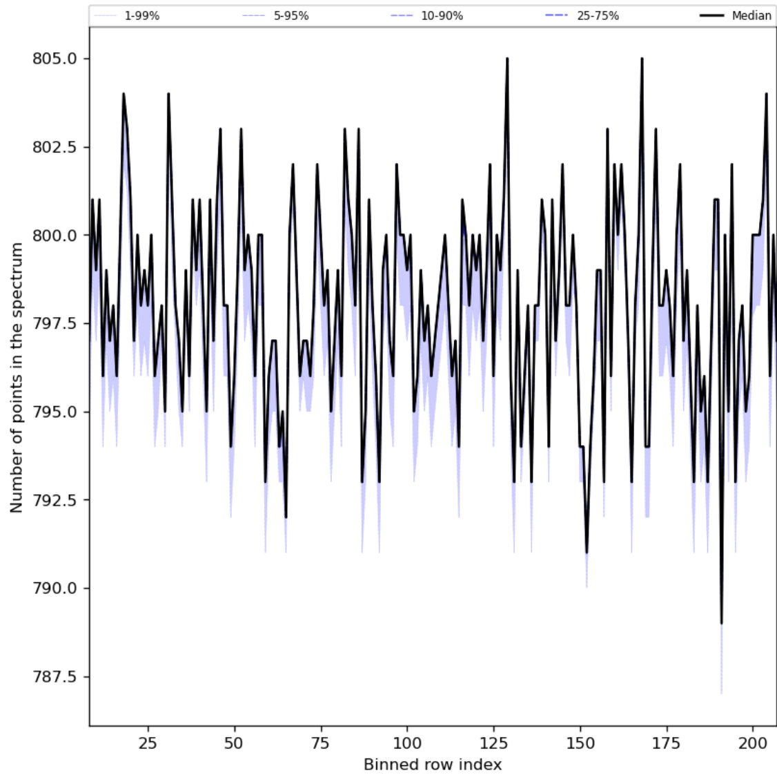
Figure 37: Along track statistics of “Number of points in the spectrum” for 2023-07-10 to 2023-07-12
