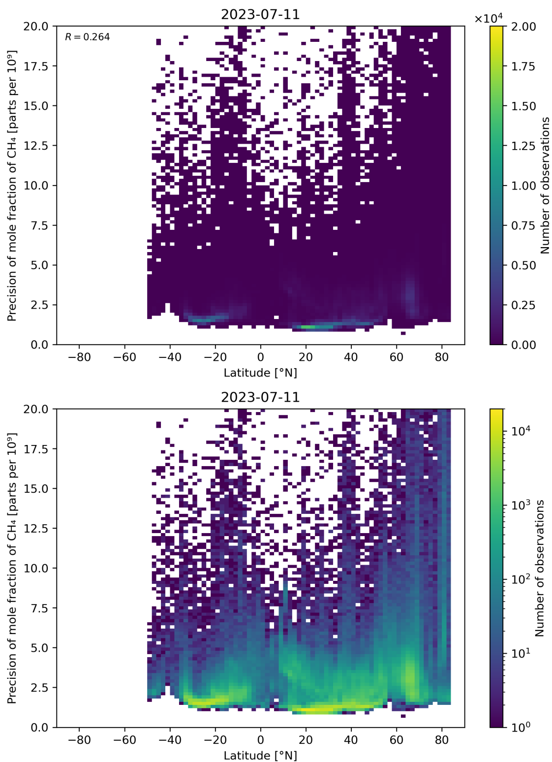
Figure 59: Scatter density plot of “Latitude” against “Precision of mole fraction of \text{CH}_4 ” for 2023-07-10 to 2023-07-12.
