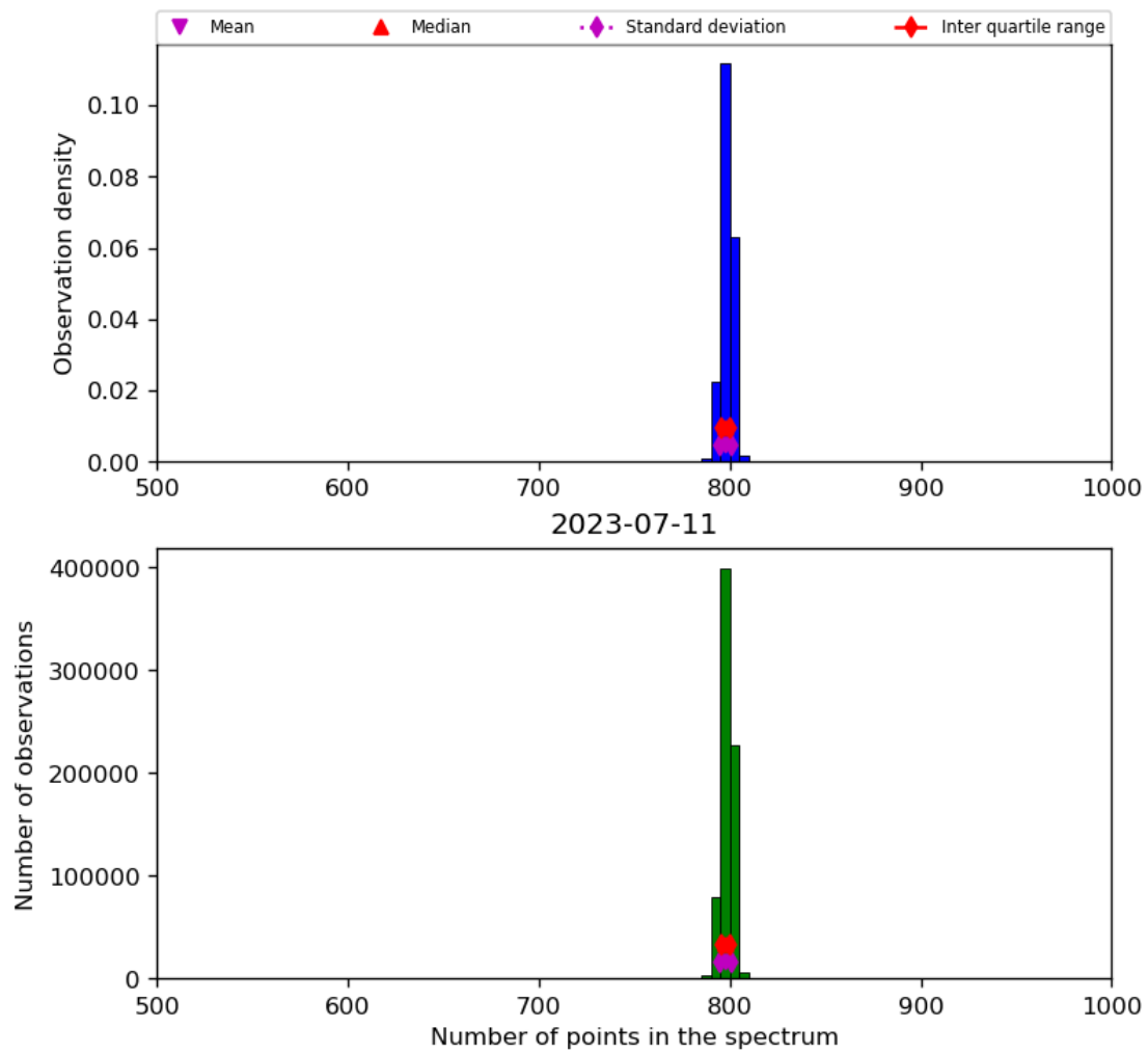
Figure 26: Histogram of “Number of points in the spectrum” for 2023-07-10 to 2023-07-12
