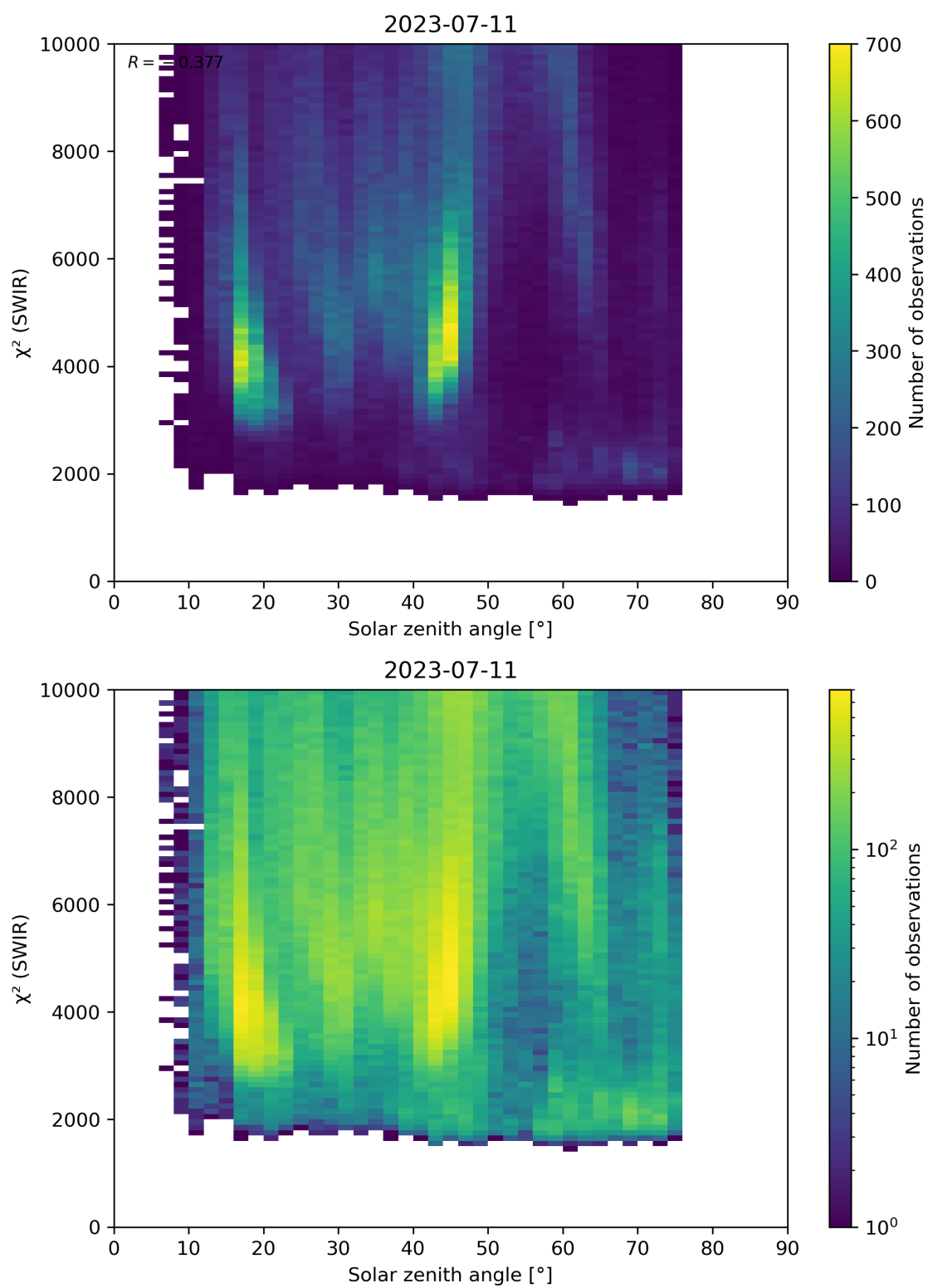
Figure 95: Scatter density plot of “Solar zenith angle” against “ \chi^2 (SWIR)” for 2023-07-10 to 2023-07-12.
