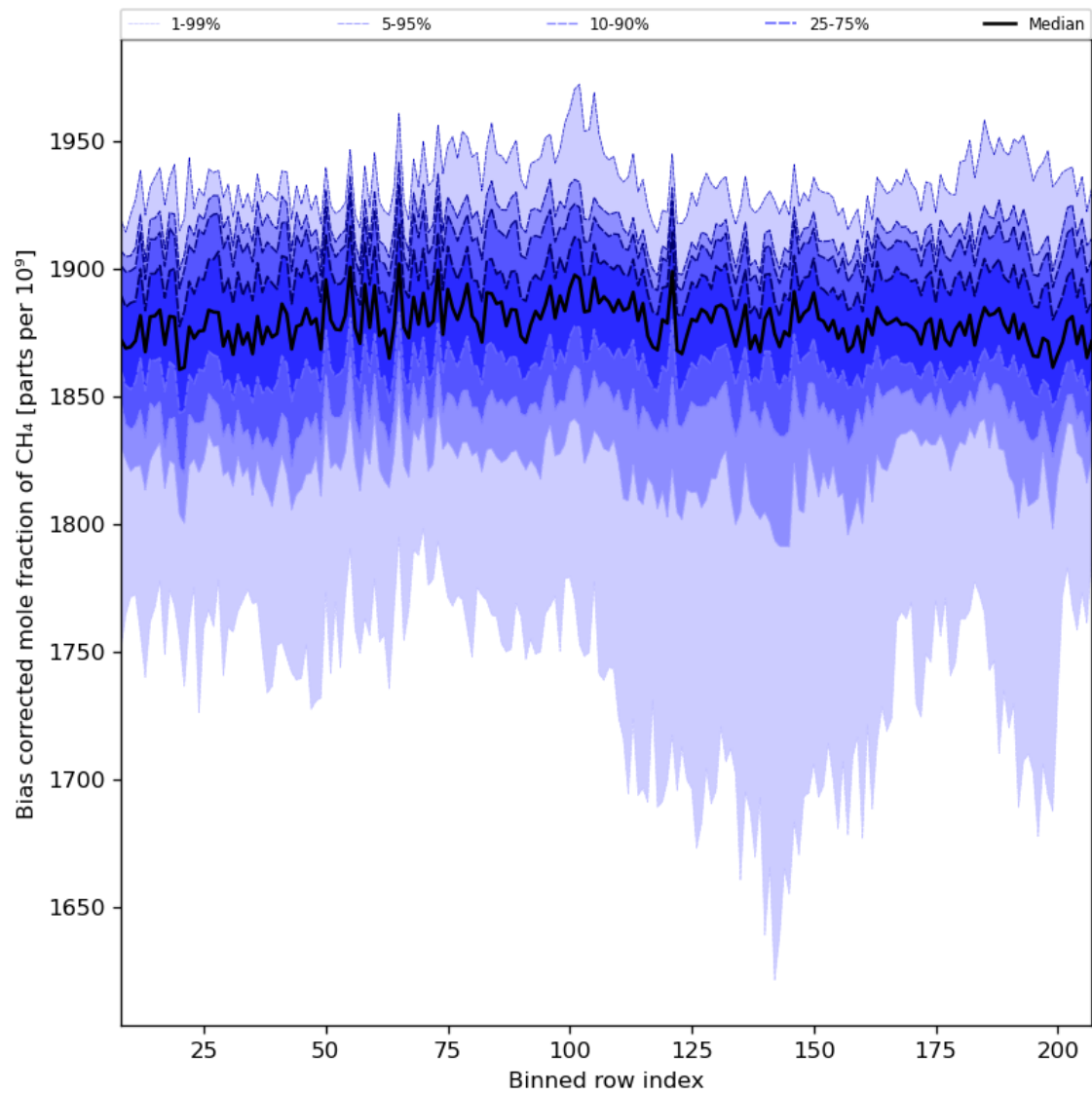
Figure 36: Along track statistics of “Bias corrected mole fraction of CH 4 ” for 2023-07-10 to 2023-07-12
