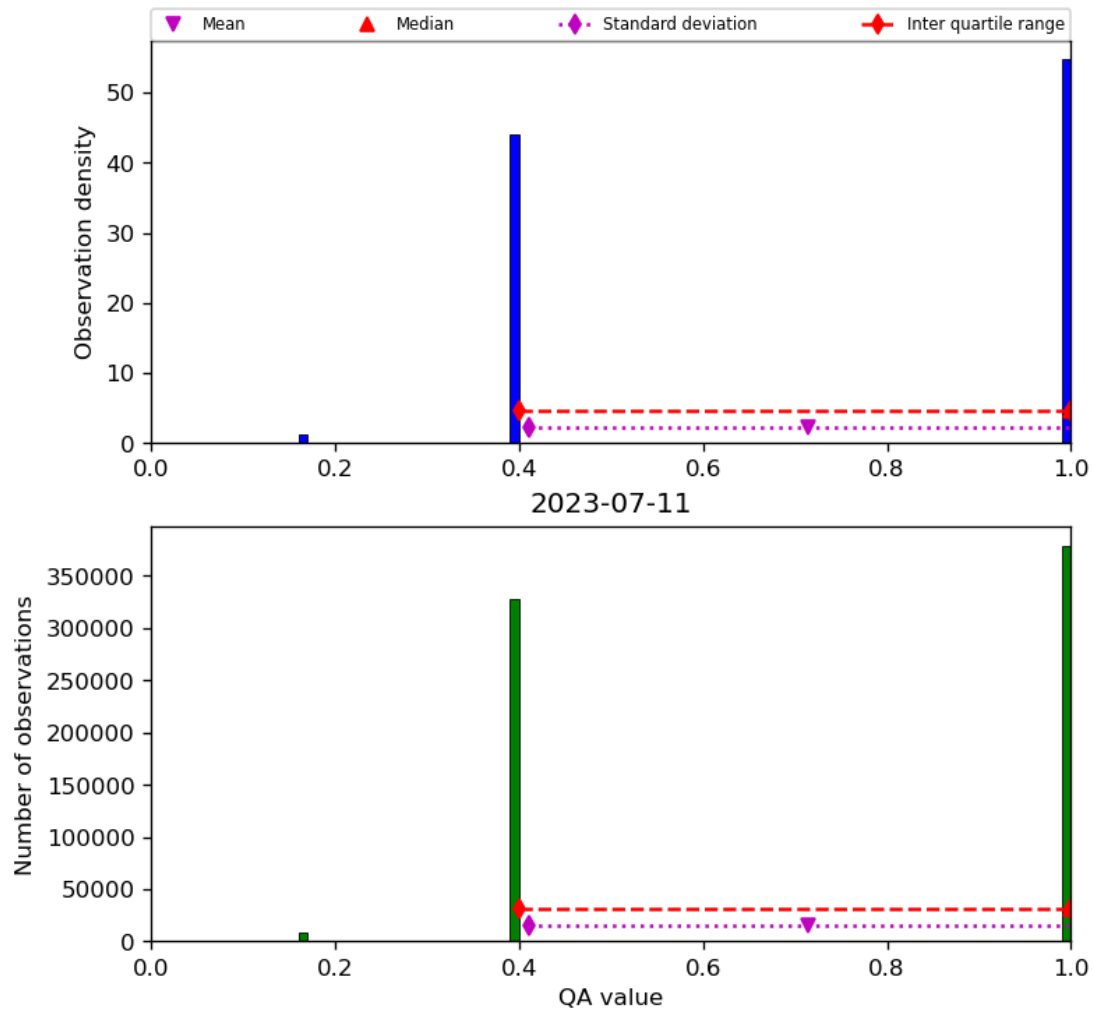
Figure 22: Histogram of “QA value” for 2023-07-10 to 2023-07-12
