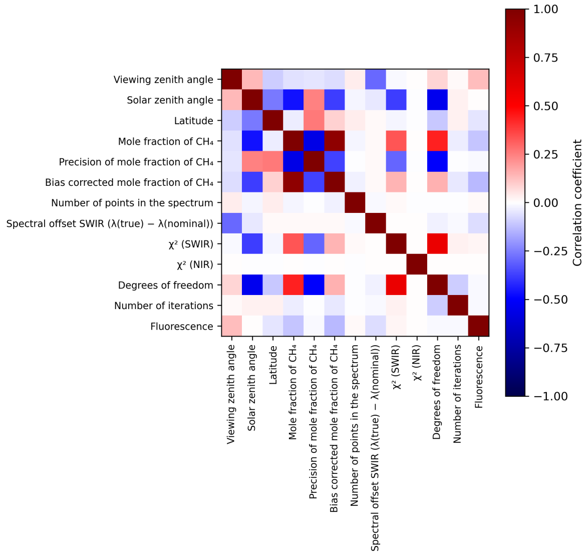
Figure 2: Map of correlation matrix for 2023-07-10 to 2023-07-12.
