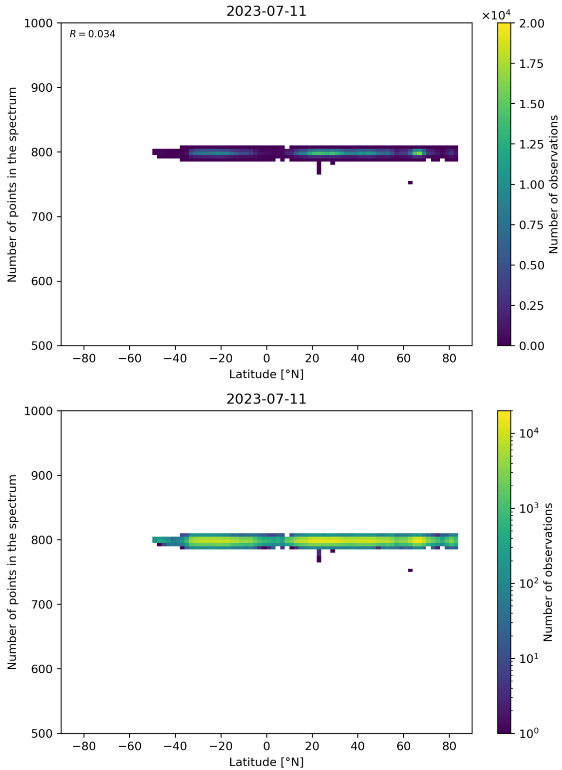
Figure 61: Scatter density plot of “Latitude” against “Number of points in the spectrum” for 2023-07-10 to 2023-07-12.
