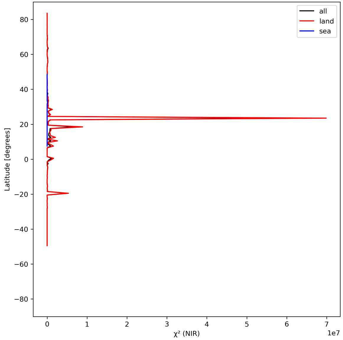
Figure 18: Zonal average of “ \chi^2 (NIR)” for 2023-07-10 to 2023-07-12.
