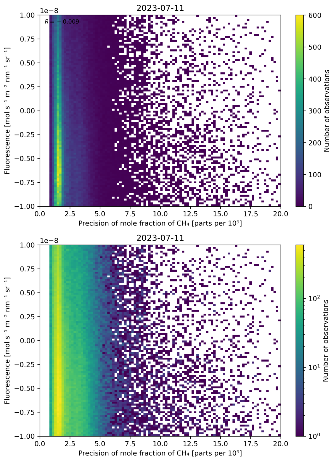
Figure 81: Scatter density plot of “Precision of mole fraction of CH 4 ” against “Fluorescence” for 2023-07-10 to 2023-07-12.
