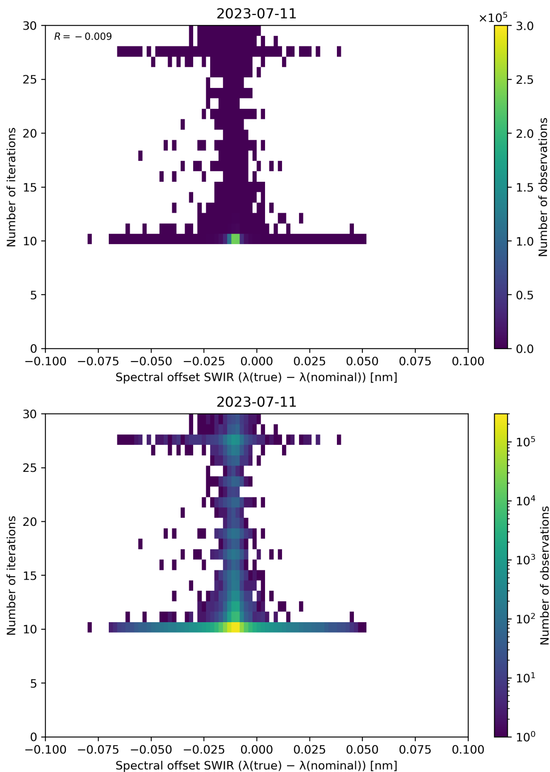
Figure 121: Scatter density plot of “Spectral offset SWIR ( \lambda(\text{true}) - \lambda(\text{nominal}) )” against “Number of iterations” for 2023-07-10 to 2023-07-12.
