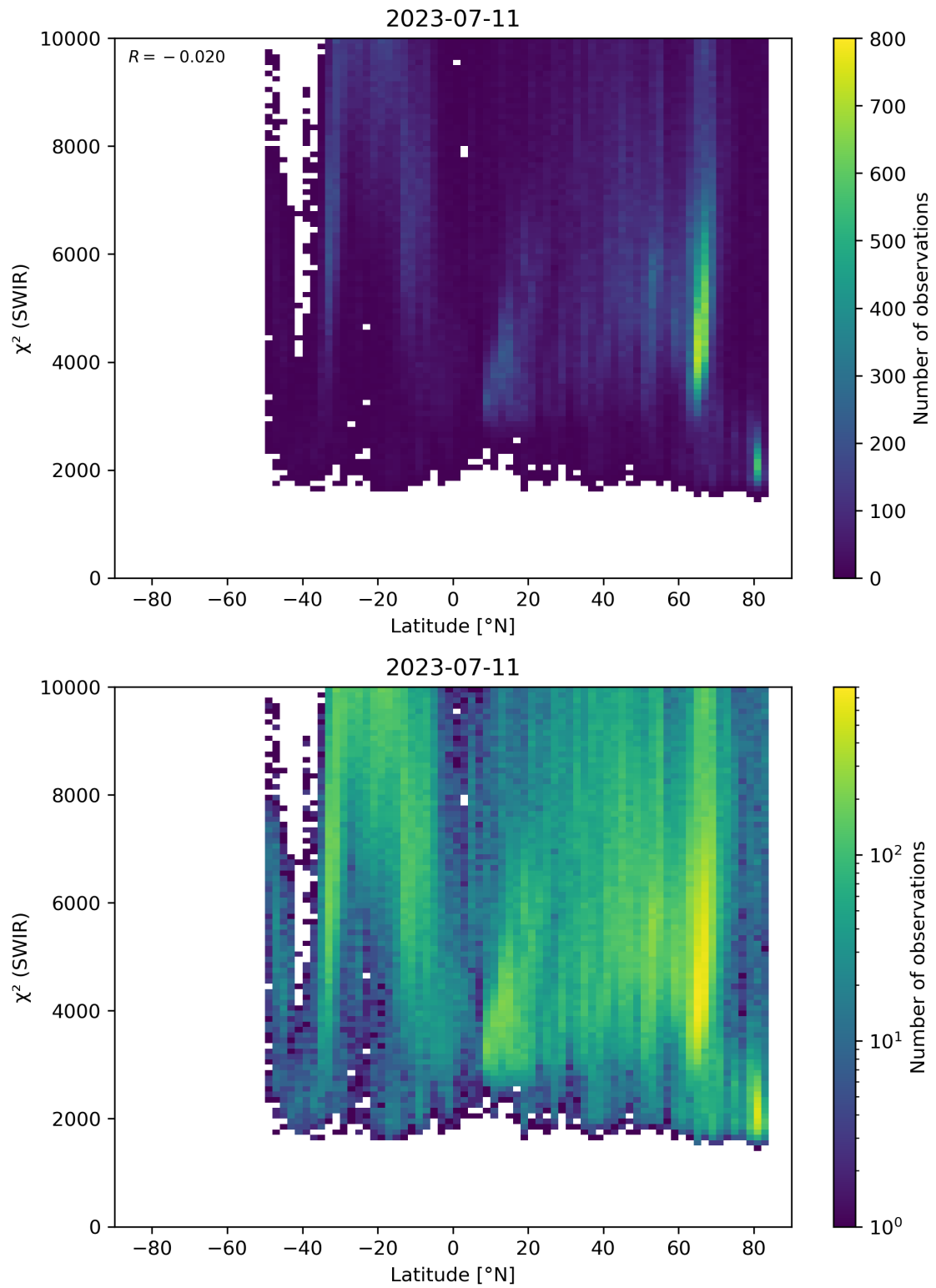
Figure 54: Scatter density plot of “Latitude” against “ \chi^2 (SWIR)” for 2023-07-10 to 2023-07-12.
