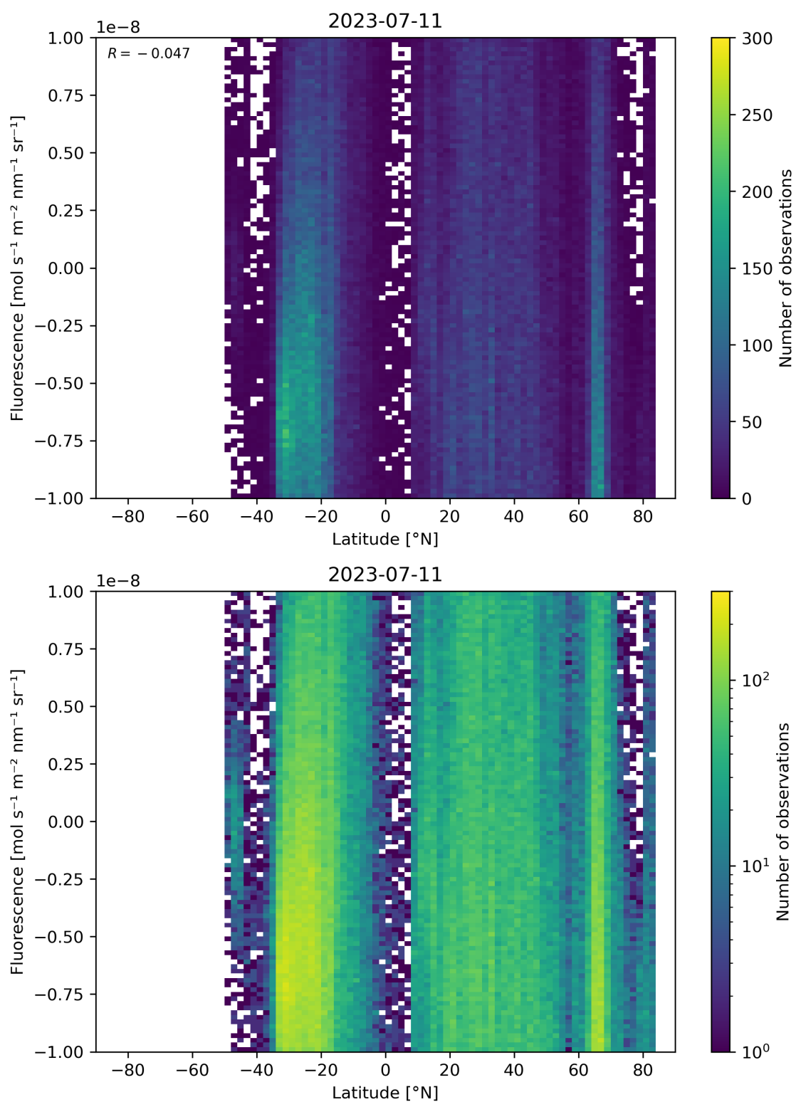
Figure 56: Scatter density plot of “Latitude” against “Fluorescence” for 2023-07-10 to 2023-07-12.
