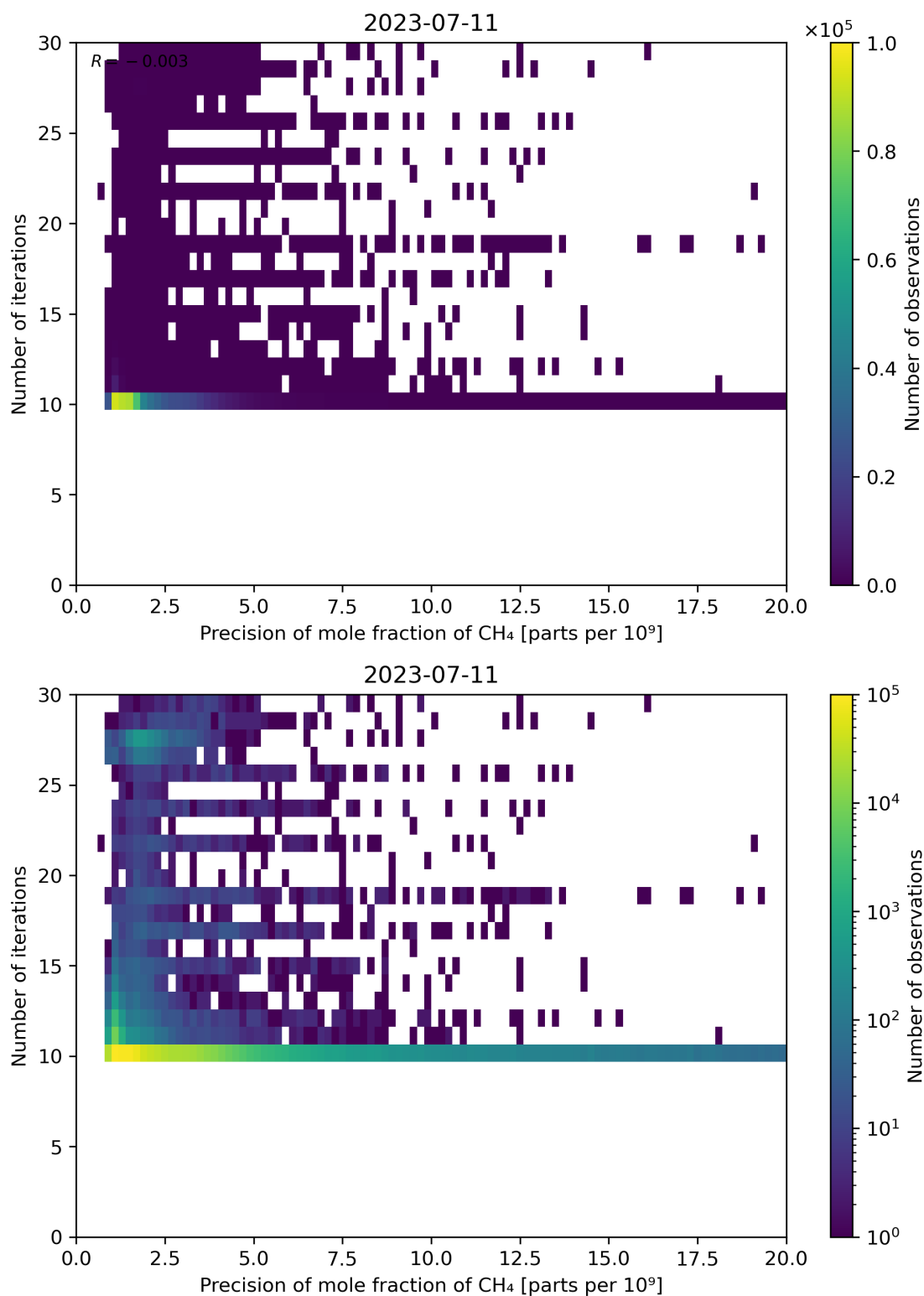
Figure 83: Scatter density plot of “Precision of mole fraction of CH 4 ” against “Number of iterations” for 2023-07-10 to 2023-07-12.
