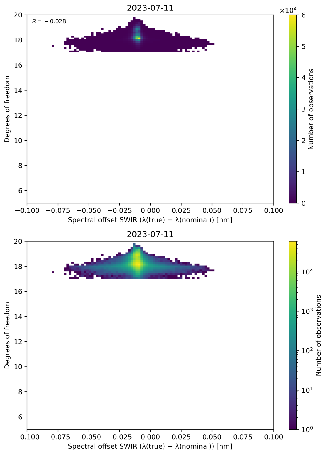
Figure 119: Scatter density plot of “Spectral offset SWIR ( \lambda(\text{true}) - \lambda(\text{nominal}) )” against “Degrees of freedom” for 2023-07-10 to 2023-07-12.
