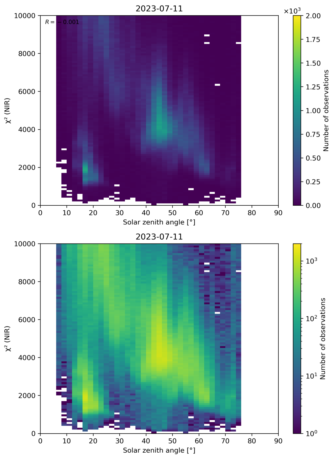
Figure 94: Scatter density plot of “Solar zenith angle” against “ \chi^2 (NIR)” for 2023-07-10 to 2023-07-12.
