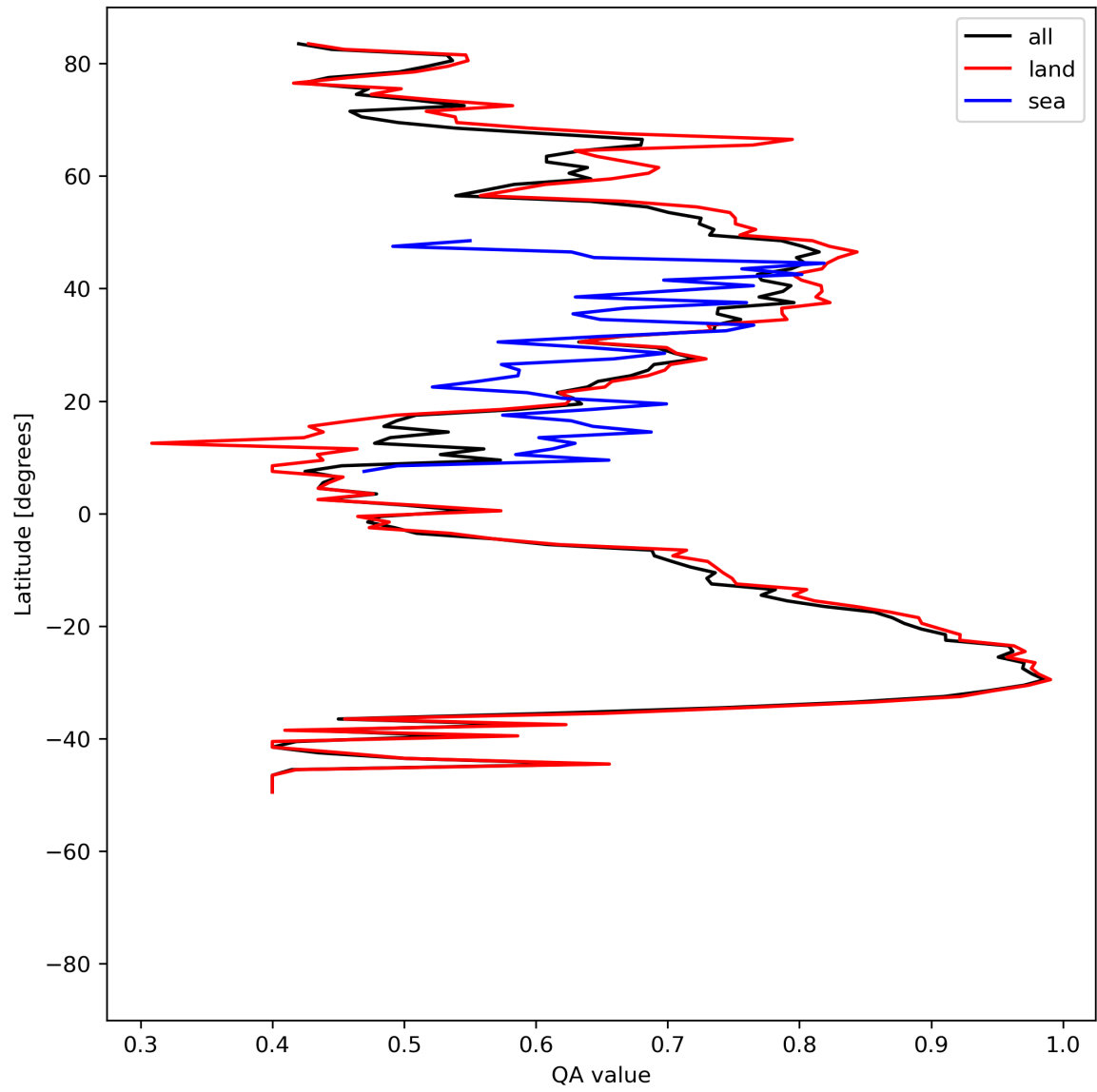
Figure 11: Zonal average of “QA value” for 2023-07-10 to 2023-07-12.
