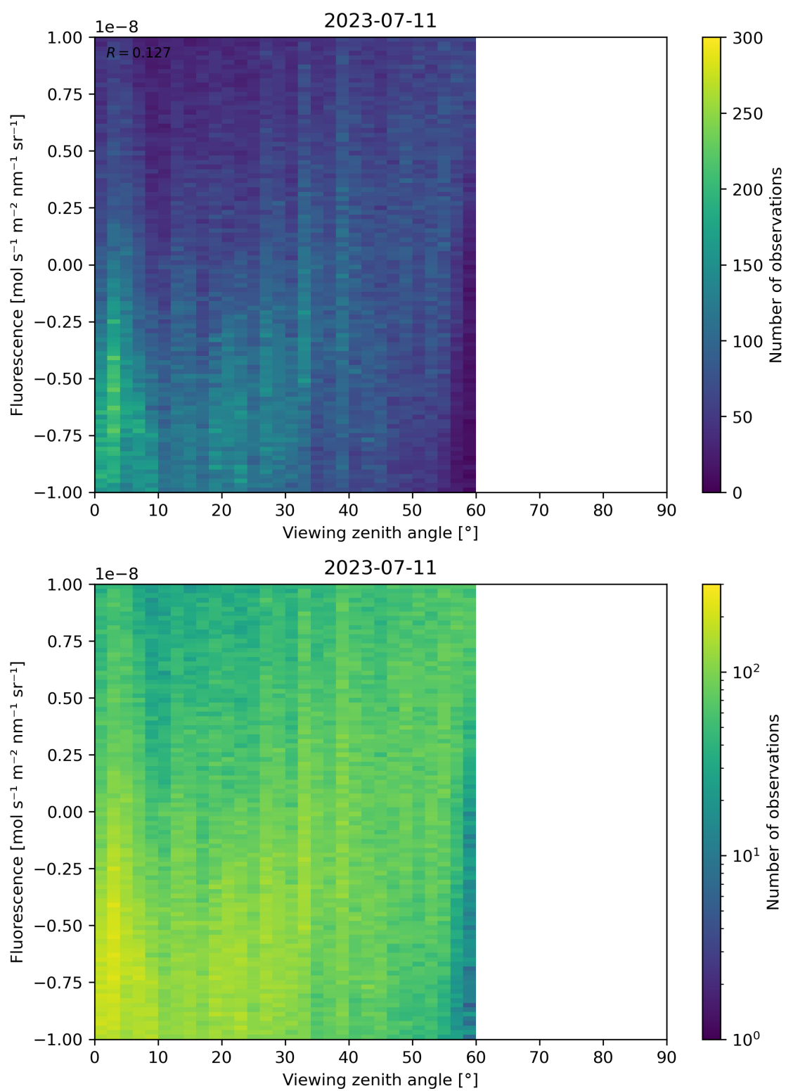
Figure 108: Scatter density plot of “Viewing zenith angle” against “Fluorescence” for 2023-07-10 to 2023-07-12.
