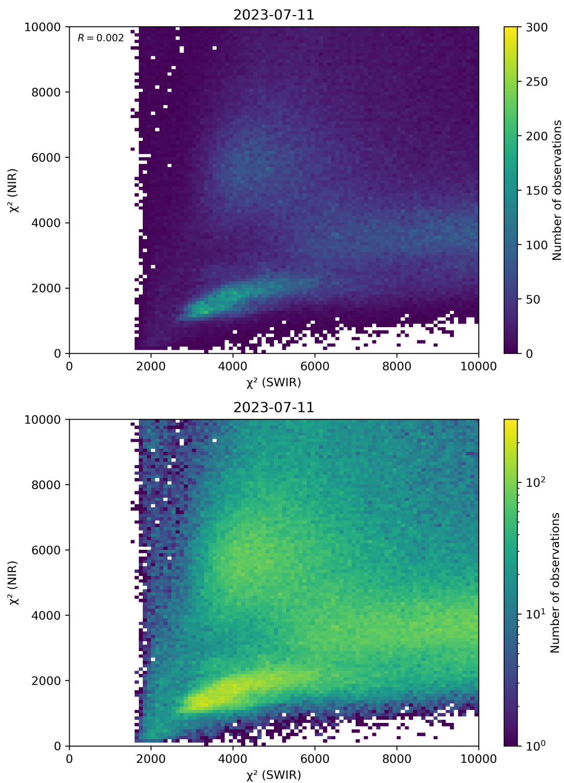
Figure 47: Scatter density plot of “ \chi^2 (SWIR)” against “ \chi^2 (NIR)” for 2023-07-10 to 2023-07-12.
