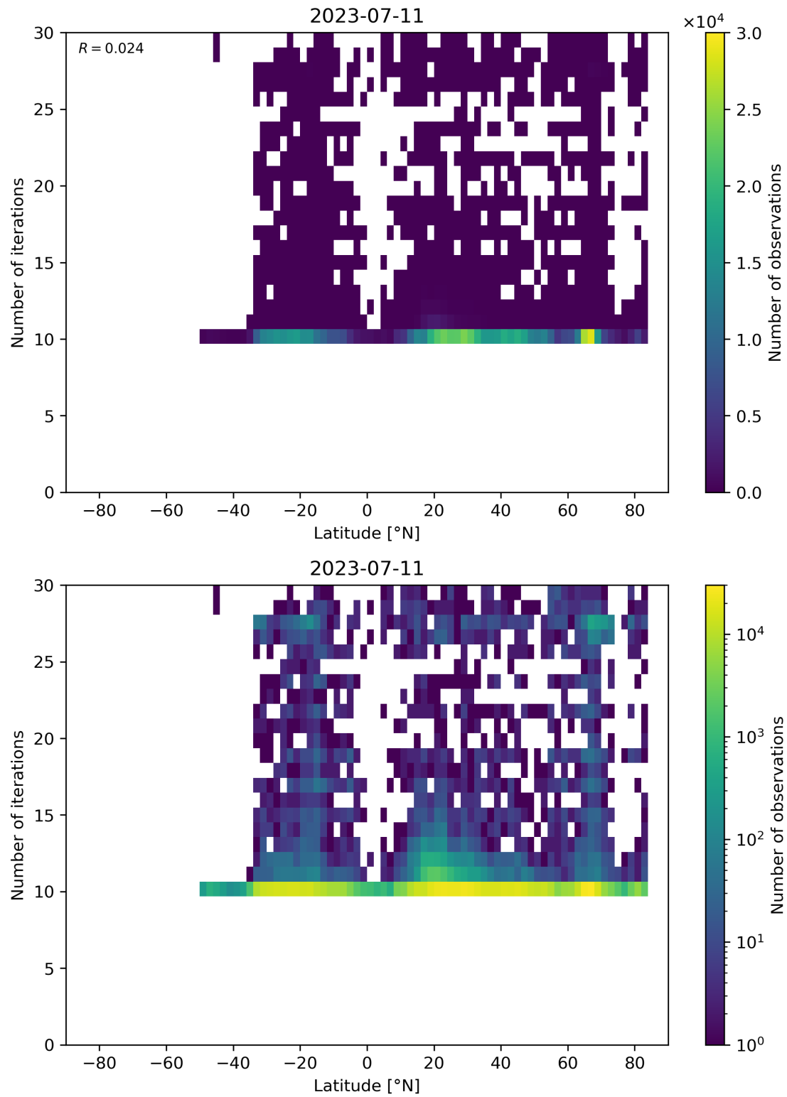
Figure 60: Scatter density plot of “Latitude” against “Number of iterations” for 2023-07-10 to 2023-07-12.
