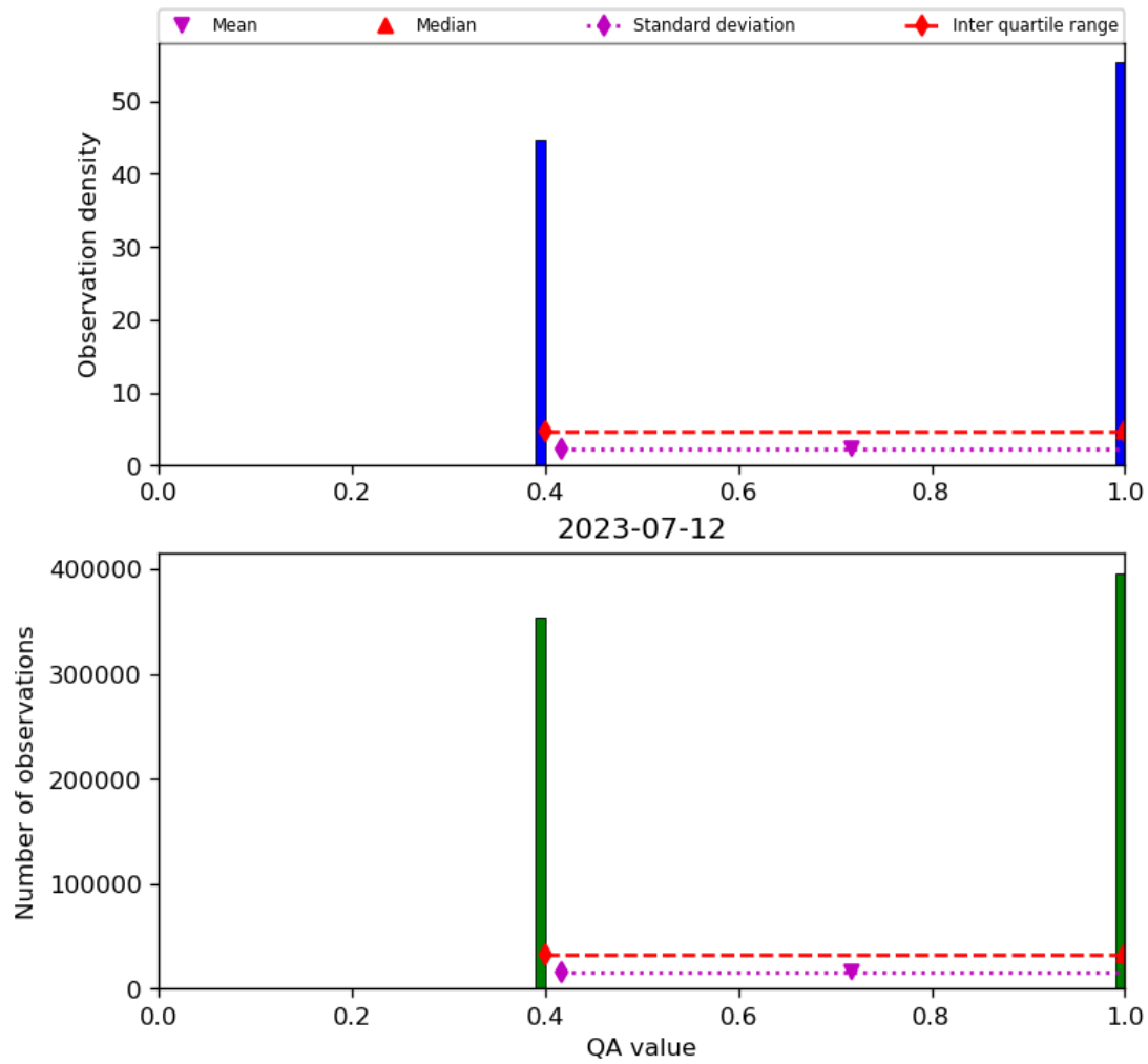
Figure 22: Histogram of “QA value” for 2023-07-11 to 2023-07-13
