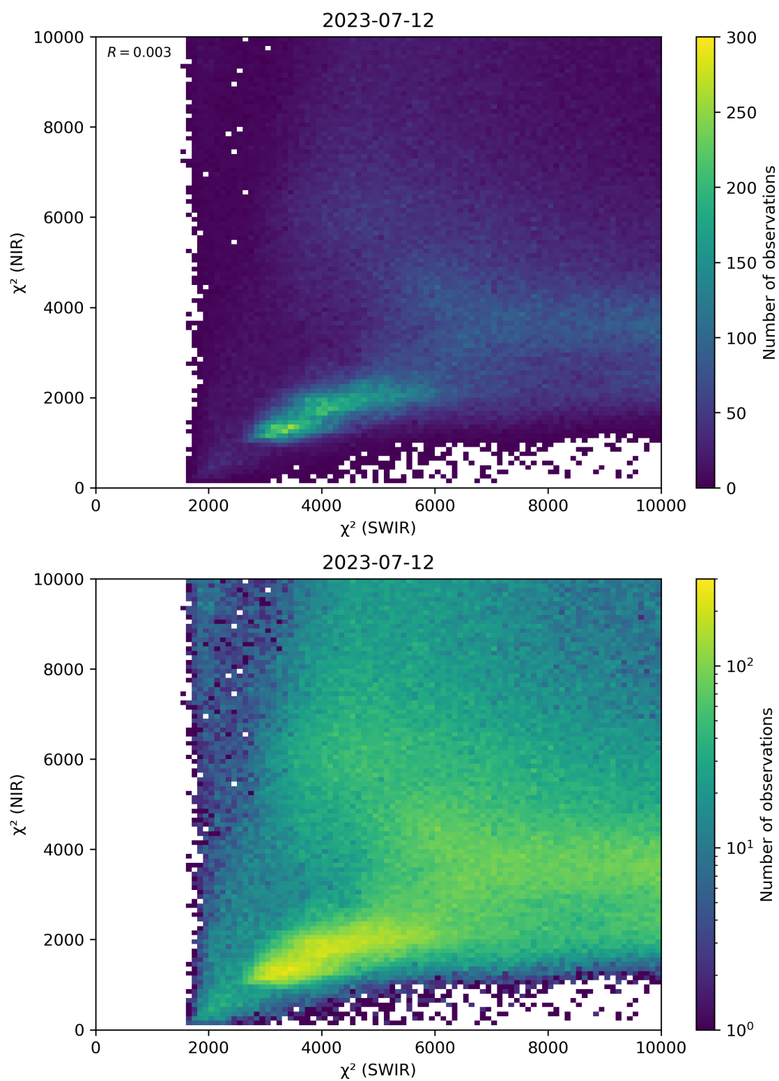
Figure 47: Scatter density plot of “ \chi^2 (SWIR)” against “ \chi^2 (NIR)” for 2023-07-11 to 2023-07-13.
