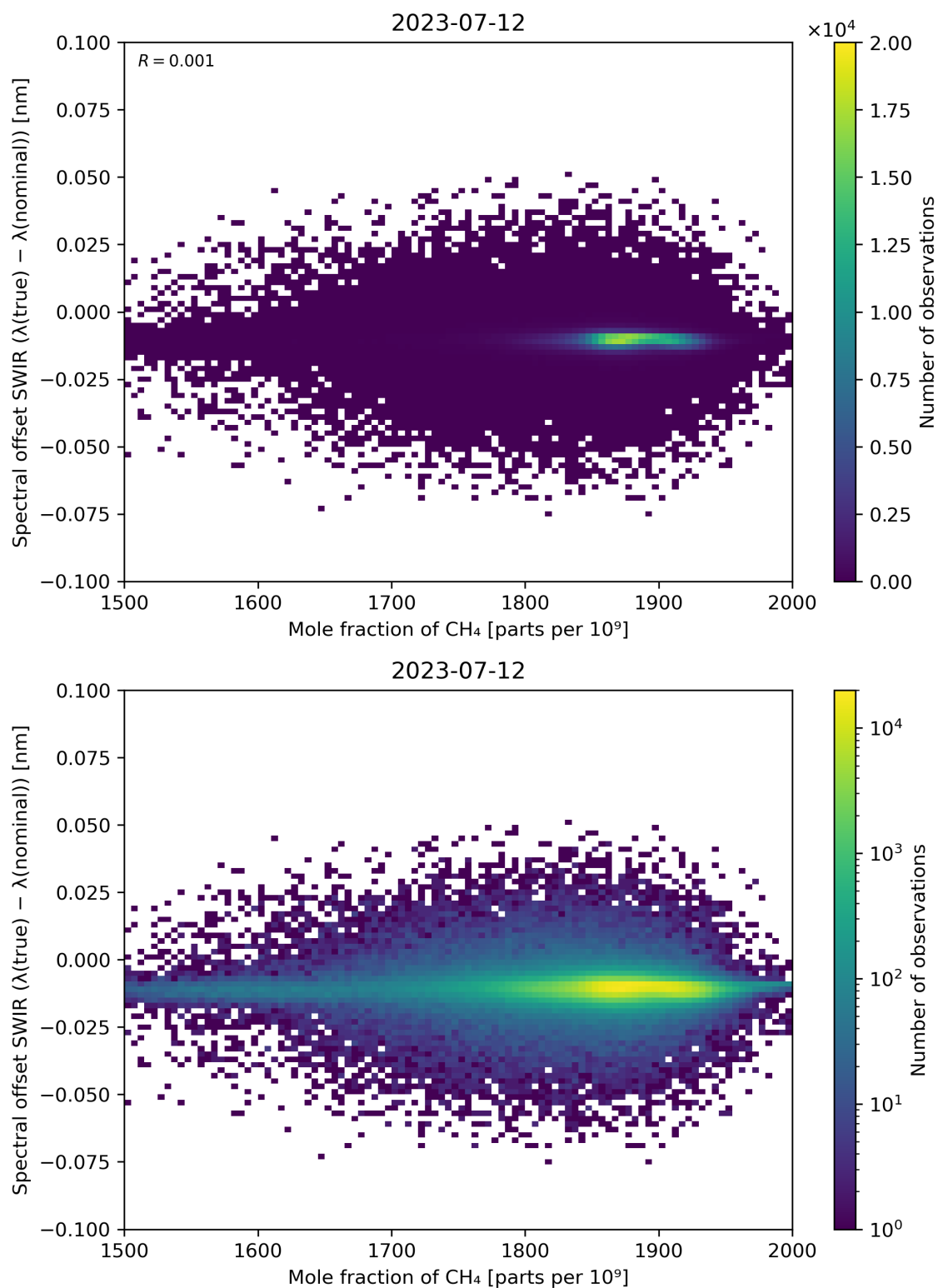
Figure 86: Scatter density plot of “Mole fraction of CH 4 ” against “Spectral offset SWIR ( \lambda(\text{true}) - \lambda(\text{nominal}) )” for 2023-07-11 to 2023-07-13.
