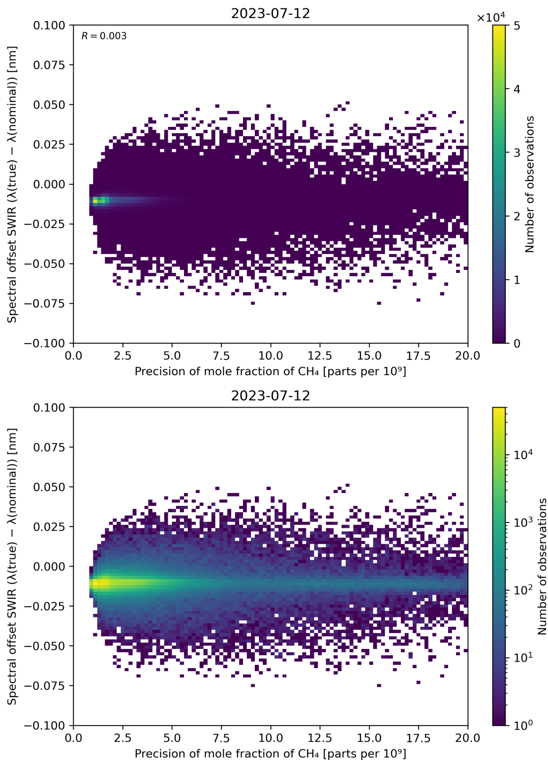
Figure 85: Scatter density plot of “Precision of mole fraction of CH 4 ” against “Spectral offset SWIR ( \lambda(\text{true}) - \lambda(\text{nominal}) )” for 2023-07-11 to 2023-07-13.
