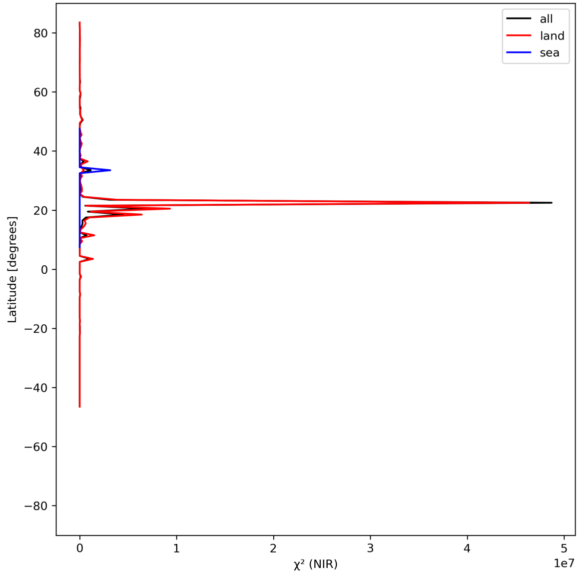
Figure 18: Zonal average of “ \chi^2 (NIR)” for 2023-07-11 to 2023-07-13.
