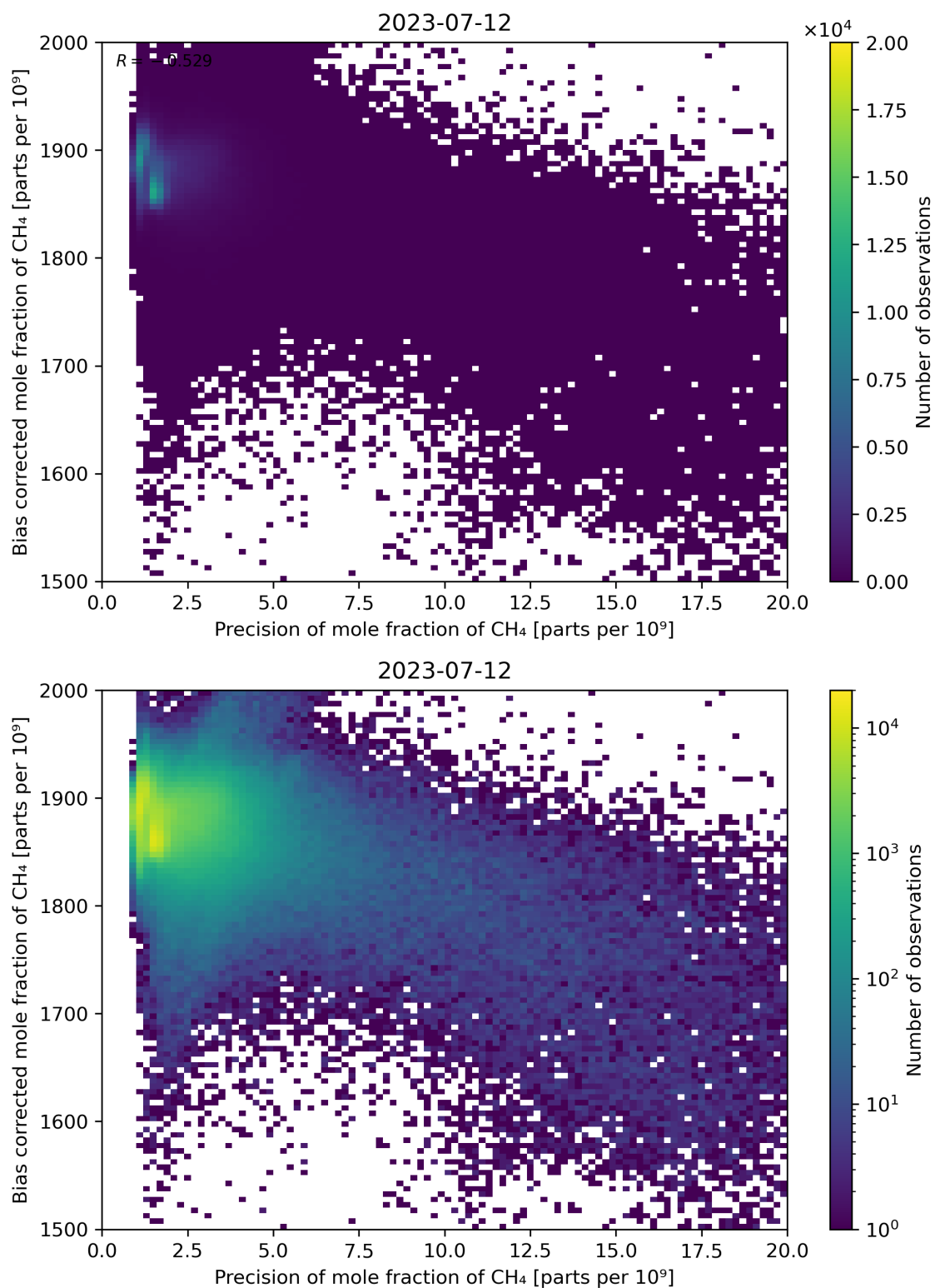
Figure 82: Scatter density plot of “Precision of mole fraction of CH 4 ” against “Bias corrected mole fraction of CH 4 ” for 2023-07-11 to 2023-07-13.
