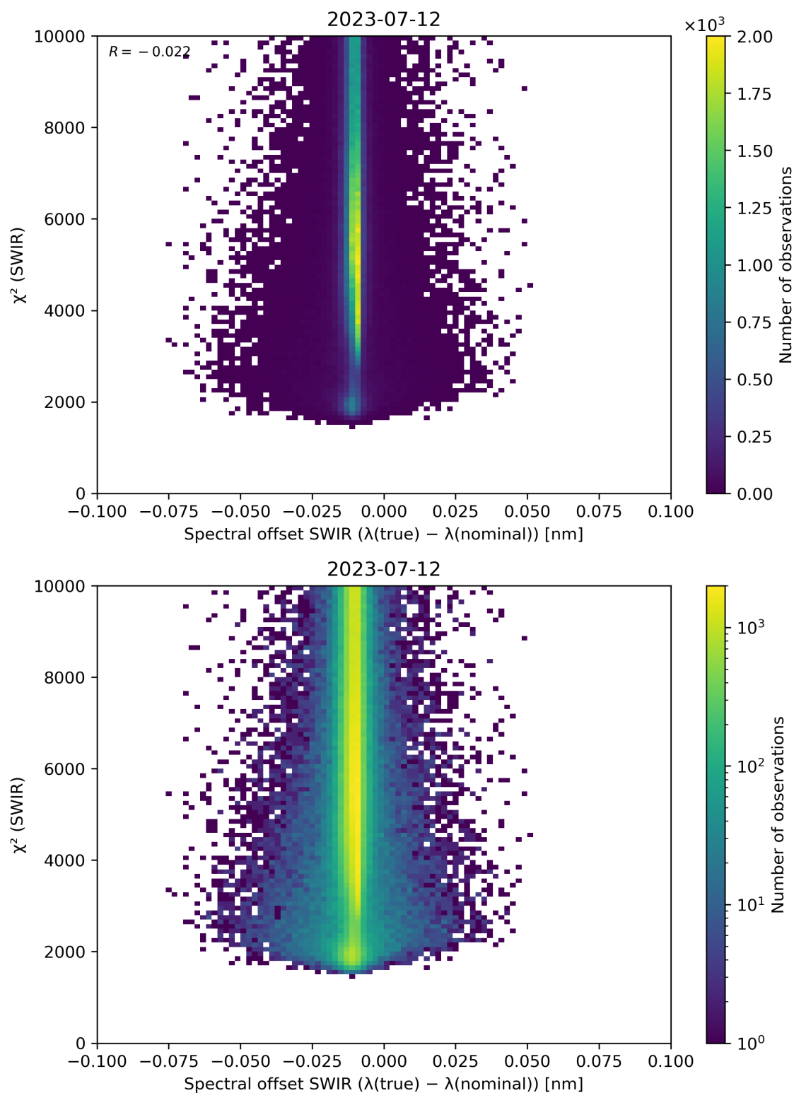
Figure 118: Scatter density plot of “Spectral offset SWIR ( \lambda(\text{true}) - \lambda(\text{nominal}) )” against “ \chi^2 (SWIR)” for 2023-07-11 to 2023-07-13.
