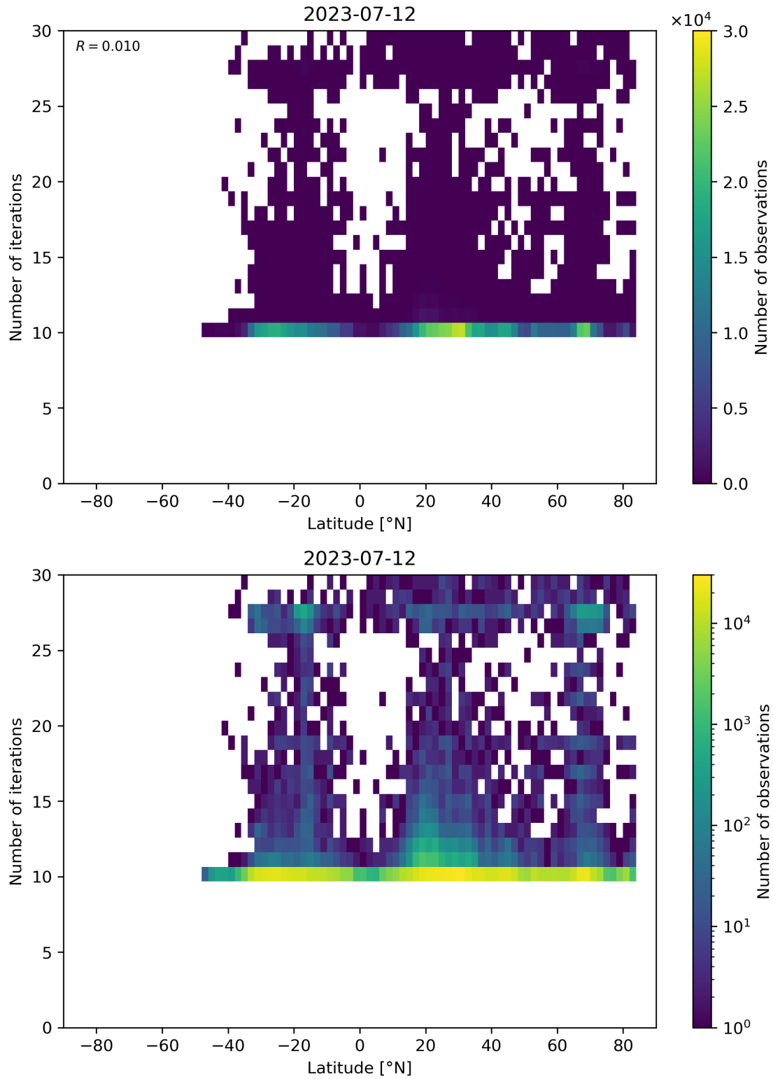
Figure 60: Scatter density plot of “Latitude” against “Number of iterations” for 2023-07-11 to 2023-07-13.
