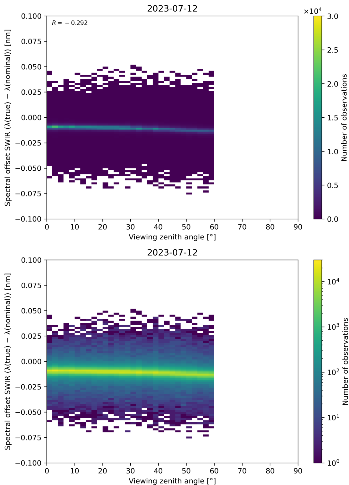
Figure 116: Scatter density plot of “Viewing zenith angle” against “Spectral offset SWIR ( \lambda(\text{true}) - \lambda(\text{nominal}) )” for 2023-07-11 to 2023-07-13.
