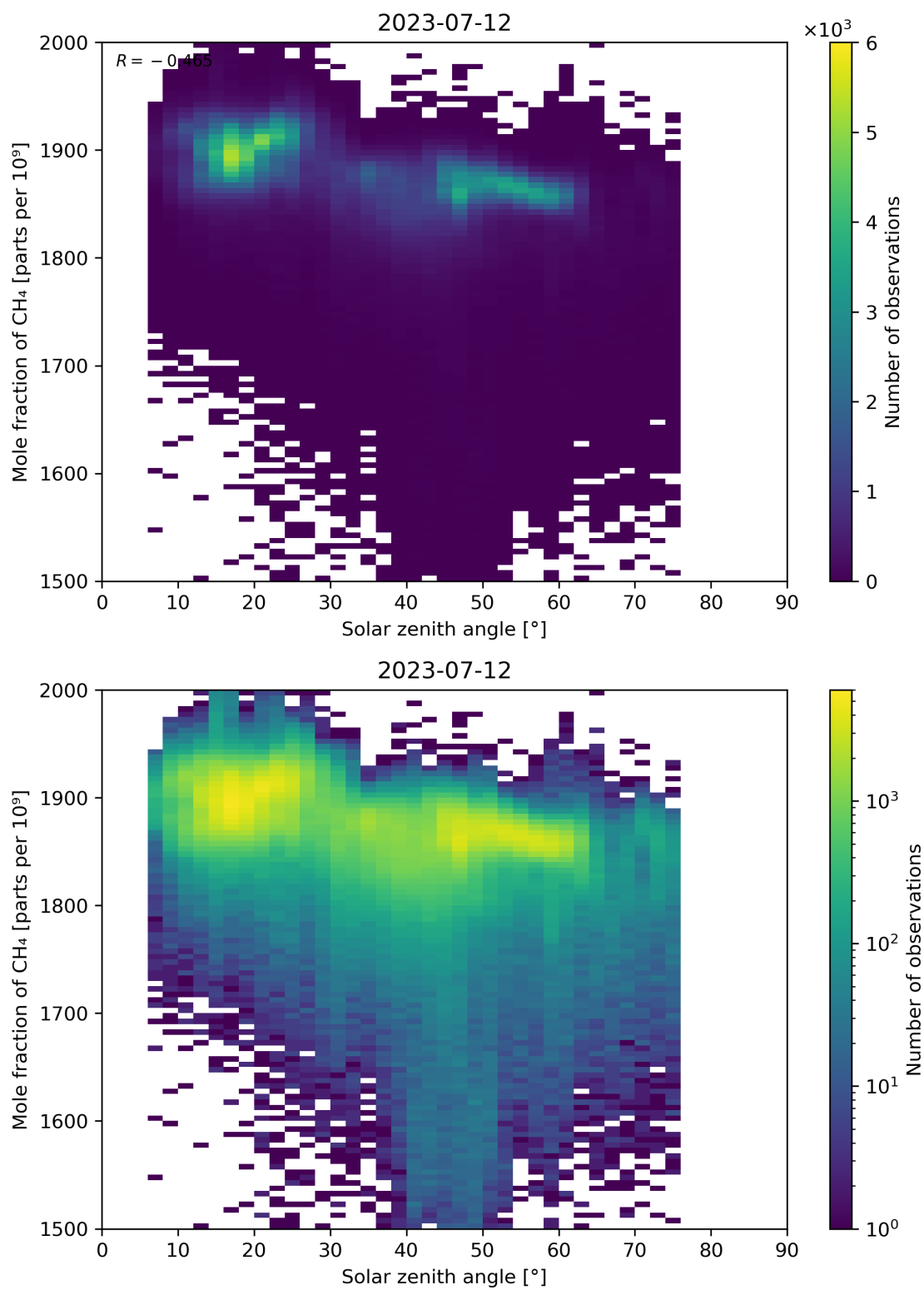
Figure 99: Scatter density plot of “Solar zenith angle” against “Mole fraction of \text{CH}_4 ” for 2023-07-11 to 2023-07-13.
