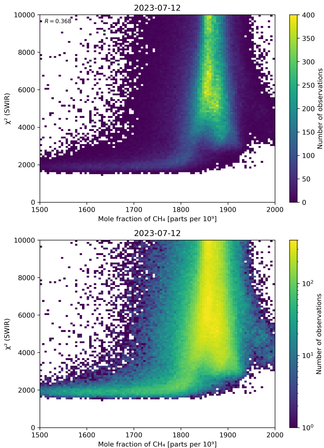
Figure 71: Scatter density plot of “Mole fraction of \text{CH}_4 ” against “ \chi^2 (SWIR)” for 2023-07-11 to 2023-07-13.
