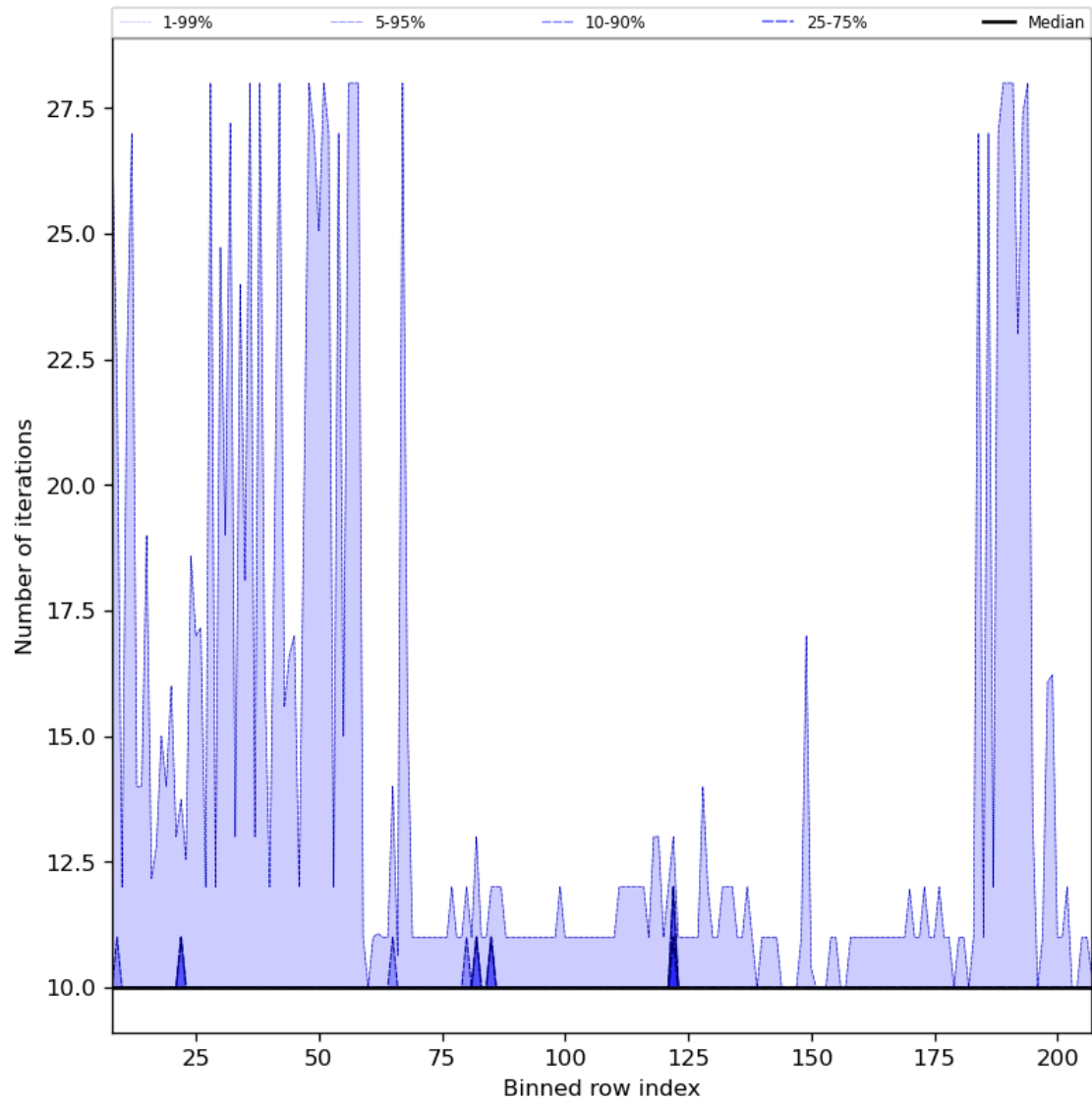
Figure 42: Along track statistics of “Number of iterations” for 2023-07-11 to 2023-07-13
