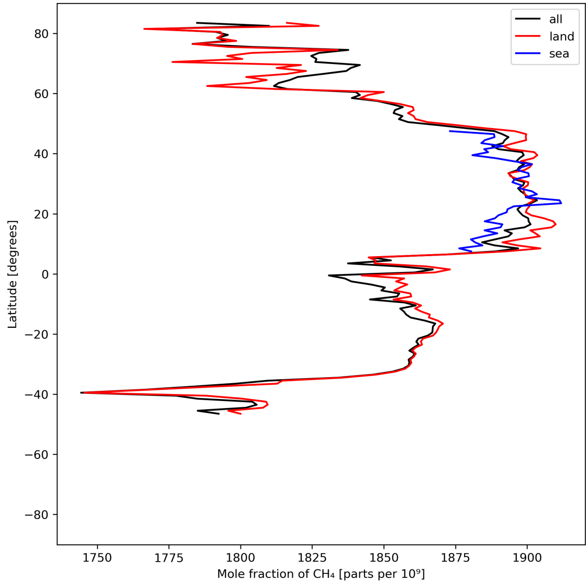
Figure 12: Zonal average of “Mole fraction of \text{CH}_4 ” for 2023-07-11 to 2023-07-13.
