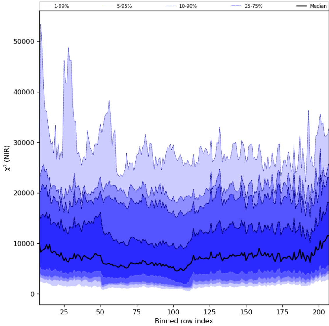
Figure 40: Along track statistics of “ \chi^2 (NIR)” for 2023-07-11 to 2023-07-13
