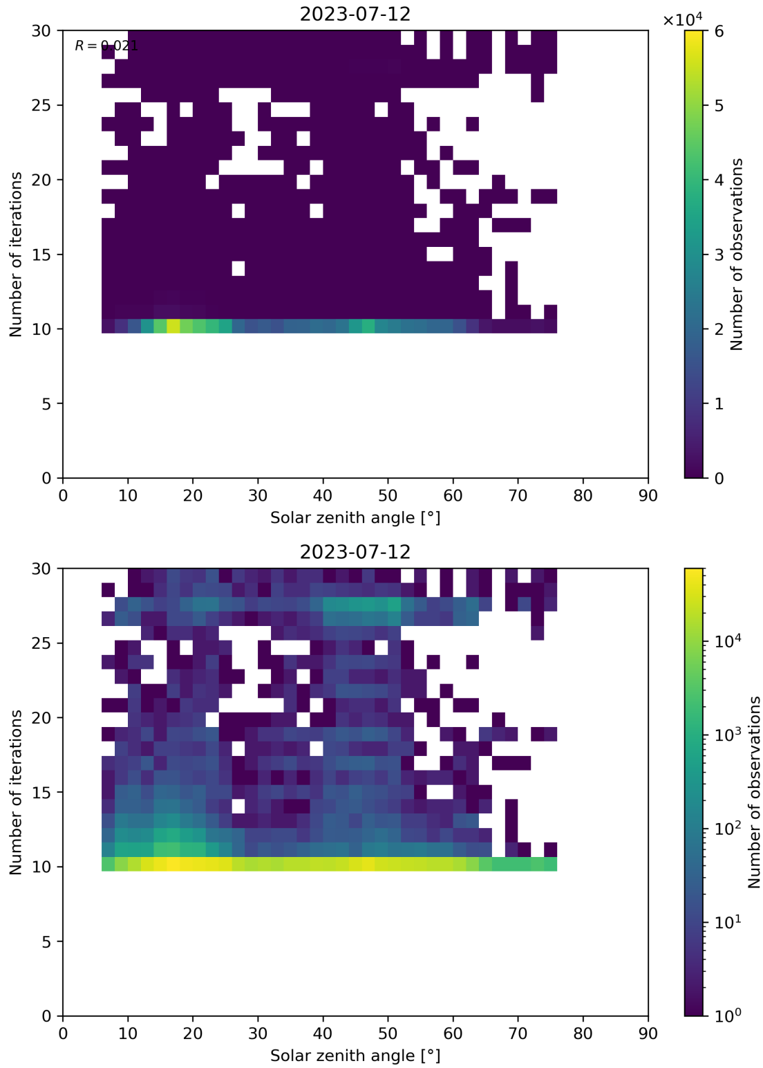
Figure 102: Scatter density plot of “Solar zenith angle” against “Number of iterations” for 2023-07-11 to 2023-07-13.
