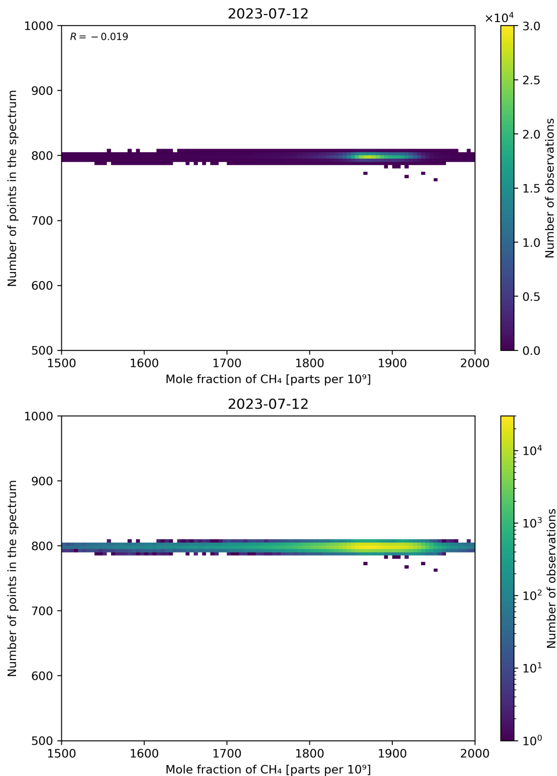
Figure 77: Scatter density plot of “Mole fraction of CH 4 ” against “Number of points in the spectrum” for 2023-07-11 to 2023-07-13.
