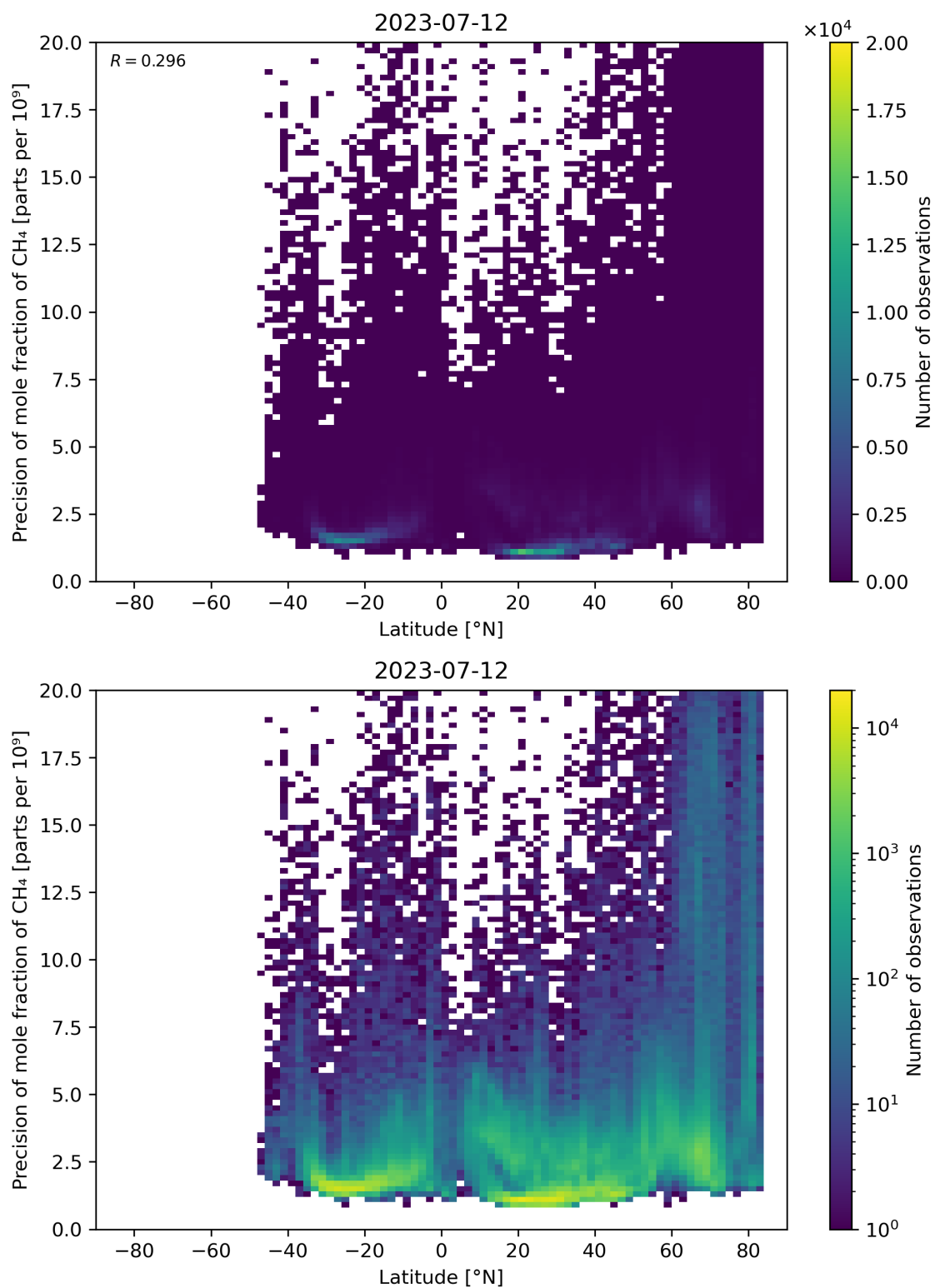
Figure 59: Scatter density plot of “Latitude” against “Precision of mole fraction of \text{CH}_4 ” for 2023-07-11 to 2023-07-13.
