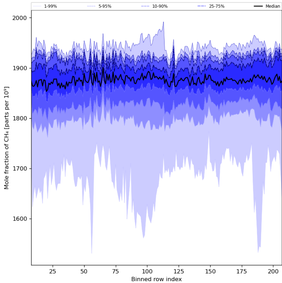
Figure 34: Along track statistics of “Mole fraction of CH 4 ” for 2023-07-11 to 2023-07-13
