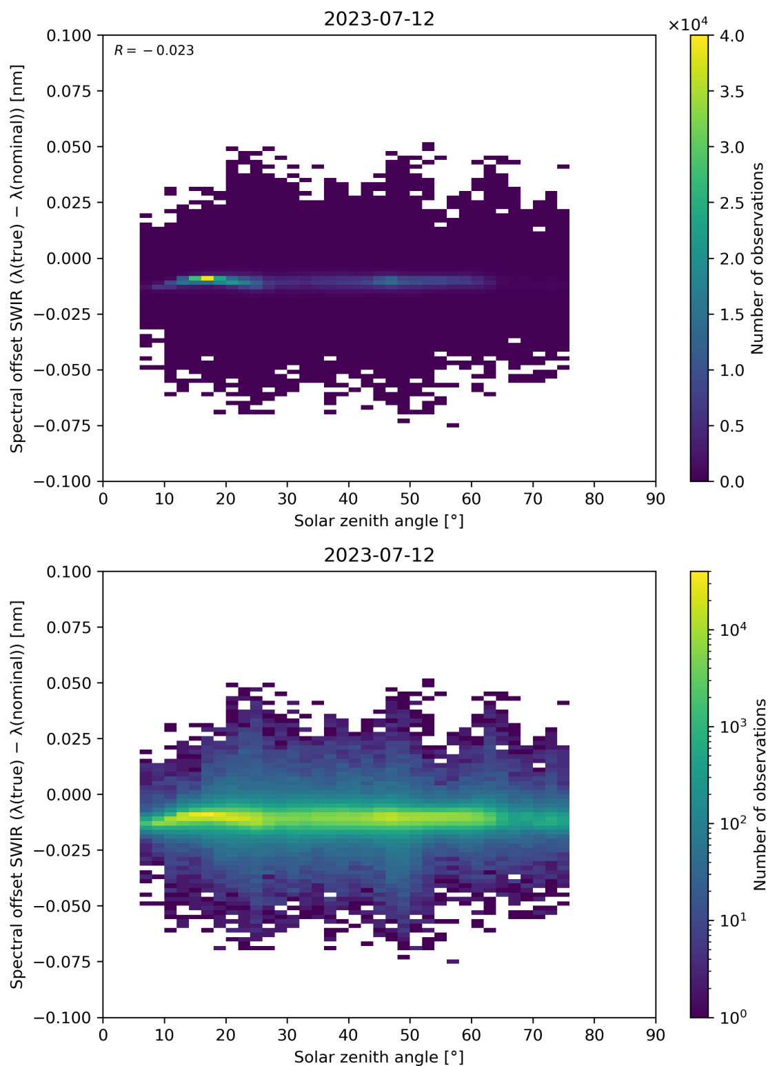
Figure 104: Scatter density plot of “Solar zenith angle” against “Spectral offset SWIR ( \lambda(\text{true}) - \lambda(\text{nominal}) )” for 2023-07-11 to 2023-07-13.
