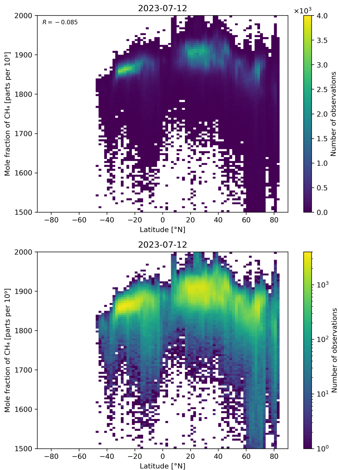
Figure 57: Scatter density plot of “Latitude” against “Mole fraction of \text{CH}_4 ” for 2023-07-11 to 2023-07-13.
