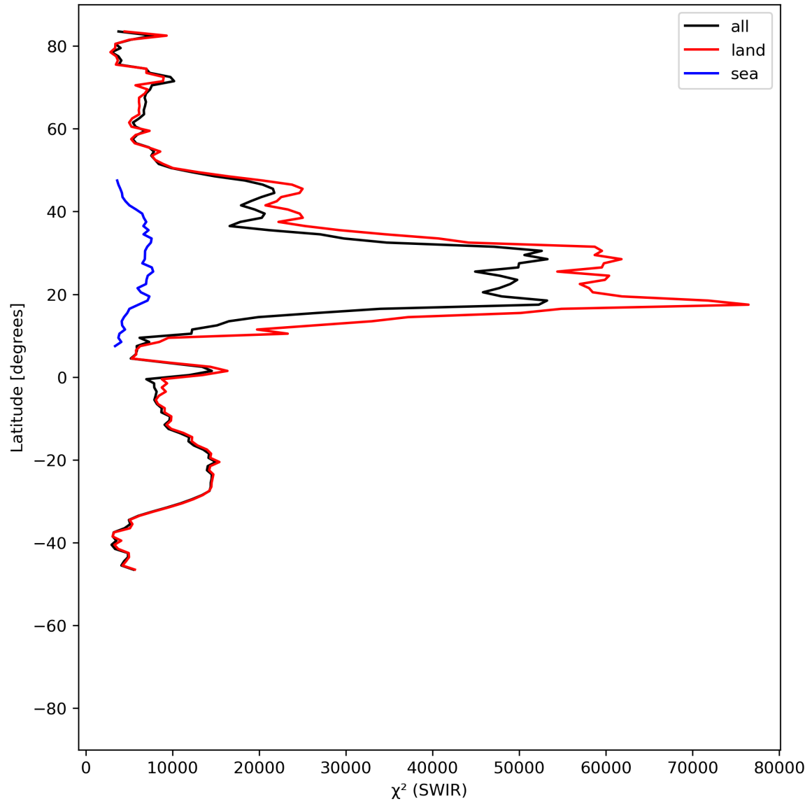
Figure 17: Zonal average of “ \chi^2 (SWIR)” for 2023-07-11 to 2023-07-13.
