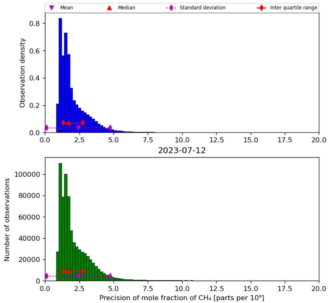
Figure 24: Histogram of “Precision of mole fraction of CH 4 ” for 2023-07-11 to 2023-07-13
