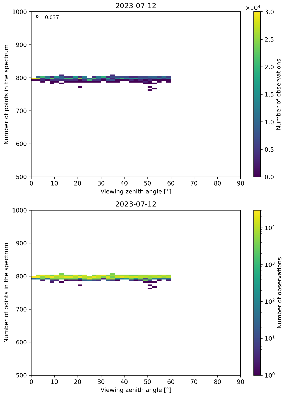
Figure 114: Scatter density plot of “Viewing zenith angle” against “Number of points in the spectrum” for 2023-07-11 to 2023-07-13.
