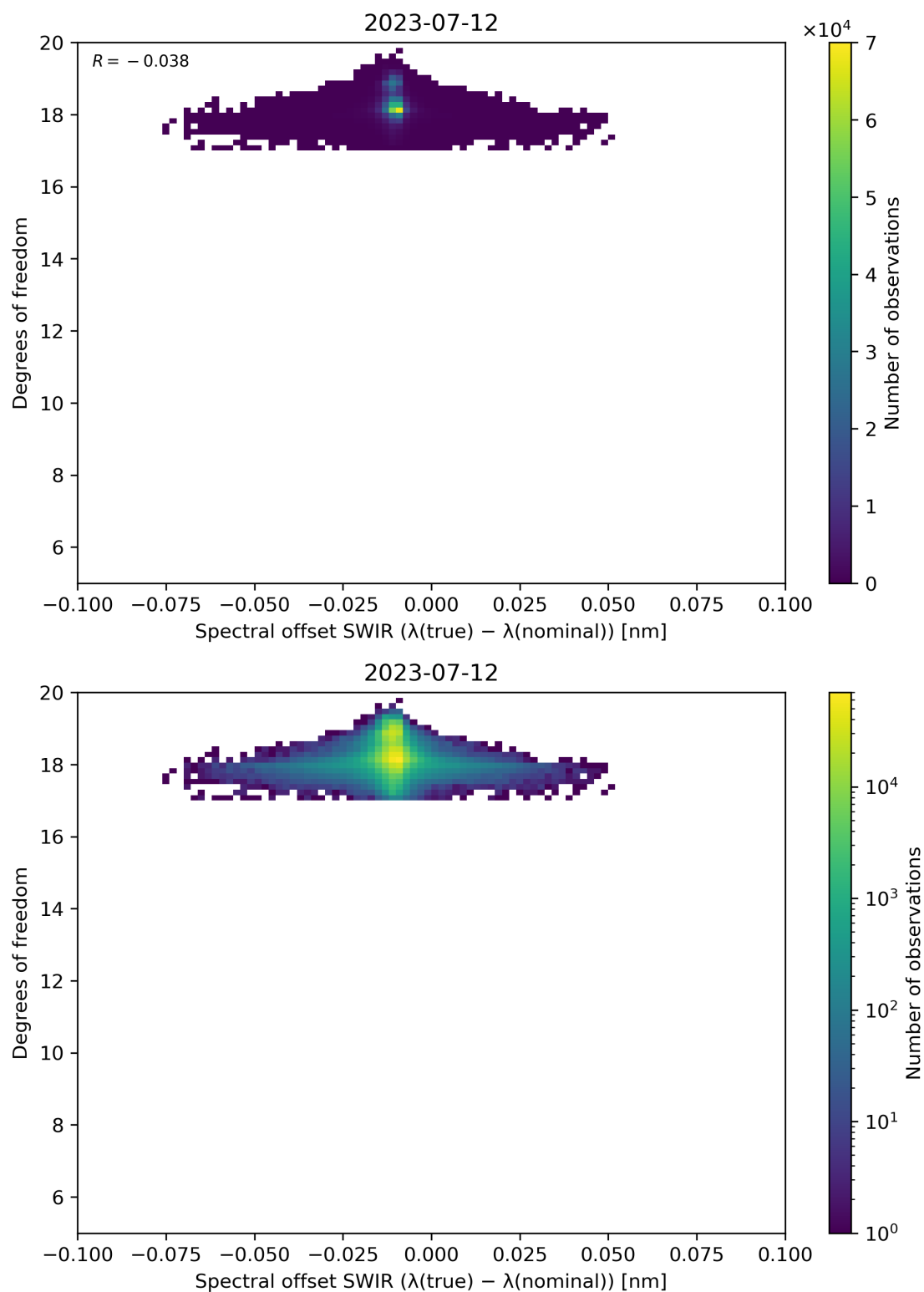
Figure 119: Scatter density plot of “Spectral offset SWIR ( \lambda(\text{true}) - \lambda(\text{nominal}) )” against “Degrees of freedom” for 2023-07-11 to 2023-07-13.
