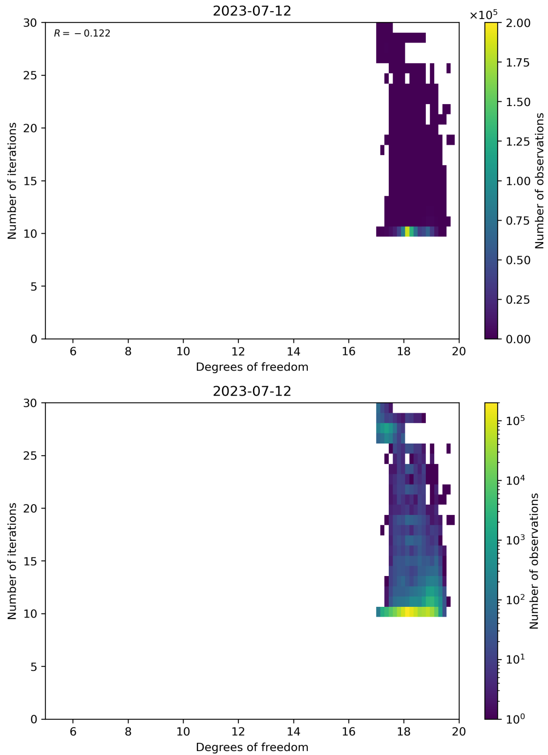
Figure 52: Scatter density plot of “Degrees of freedom” against “Number of iterations” for 2023-07-11 to 2023-07-13.
