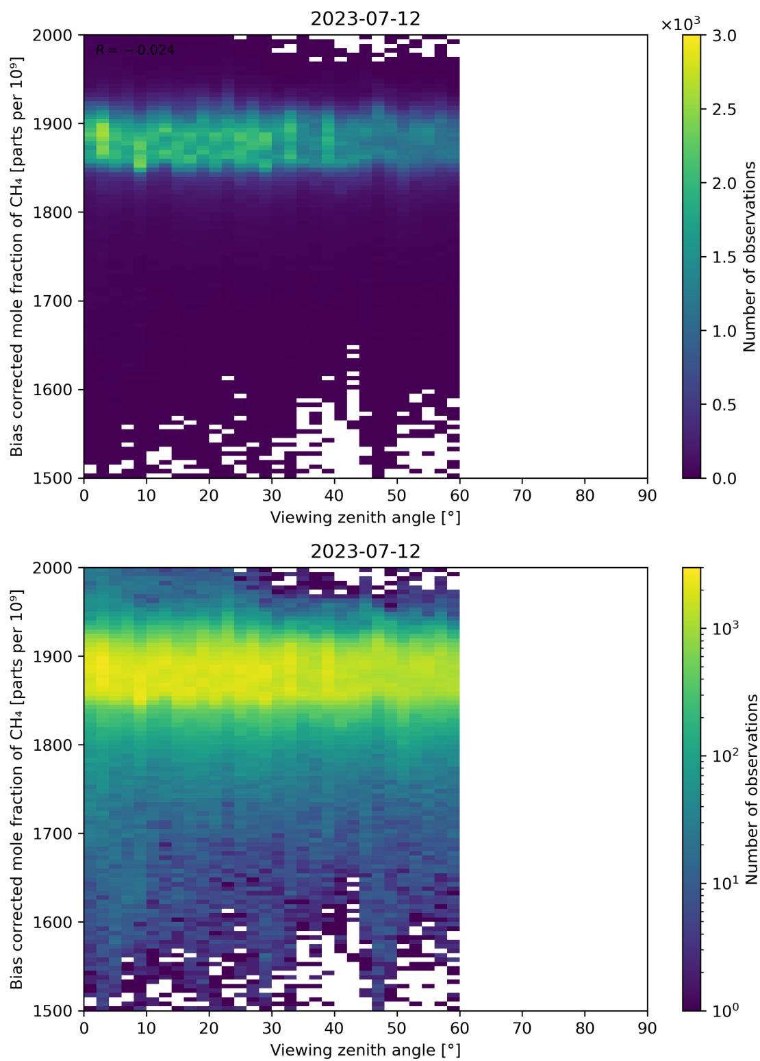
Figure 111: Scatter density plot of “Viewing zenith angle” against “Bias corrected mole fraction of CH 4 ” for 2023-07-11 to 2023-07-13.
