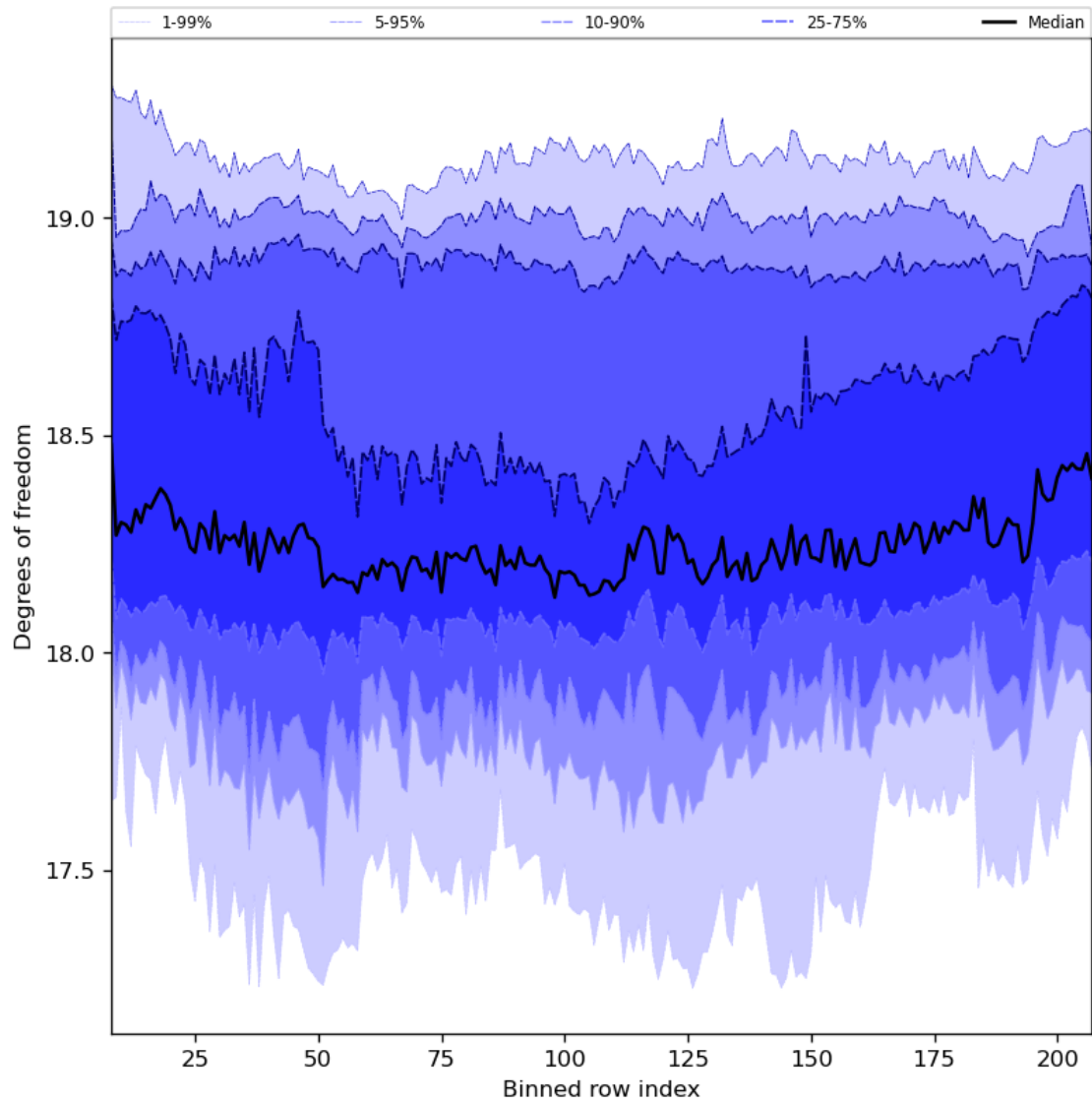
Figure 41: Along track statistics of “Degrees of freedom” for 2023-07-11 to 2023-07-13
