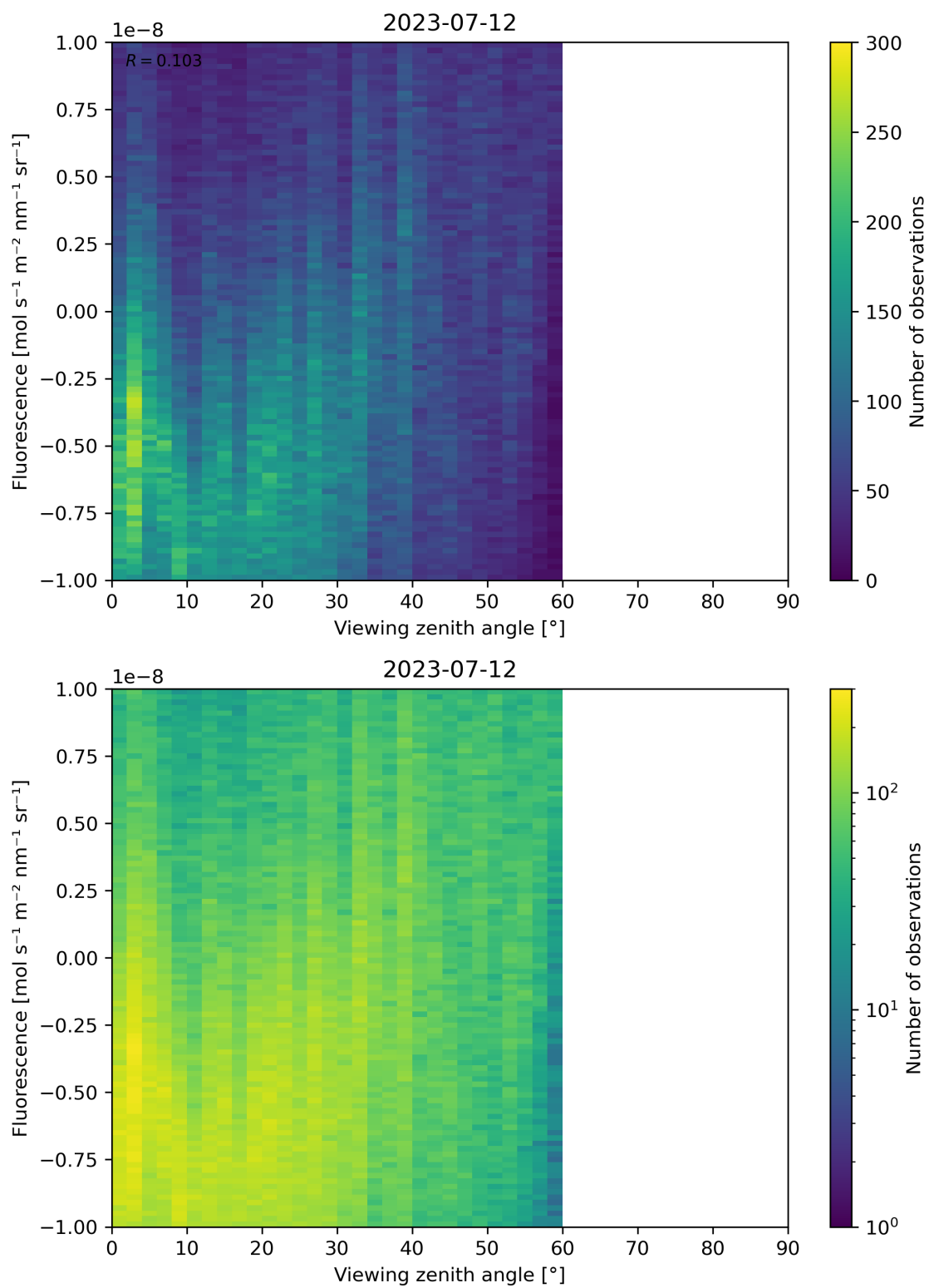
Figure 108: Scatter density plot of “Viewing zenith angle” against “Fluorescence” for 2023-07-11 to 2023-07-13.
