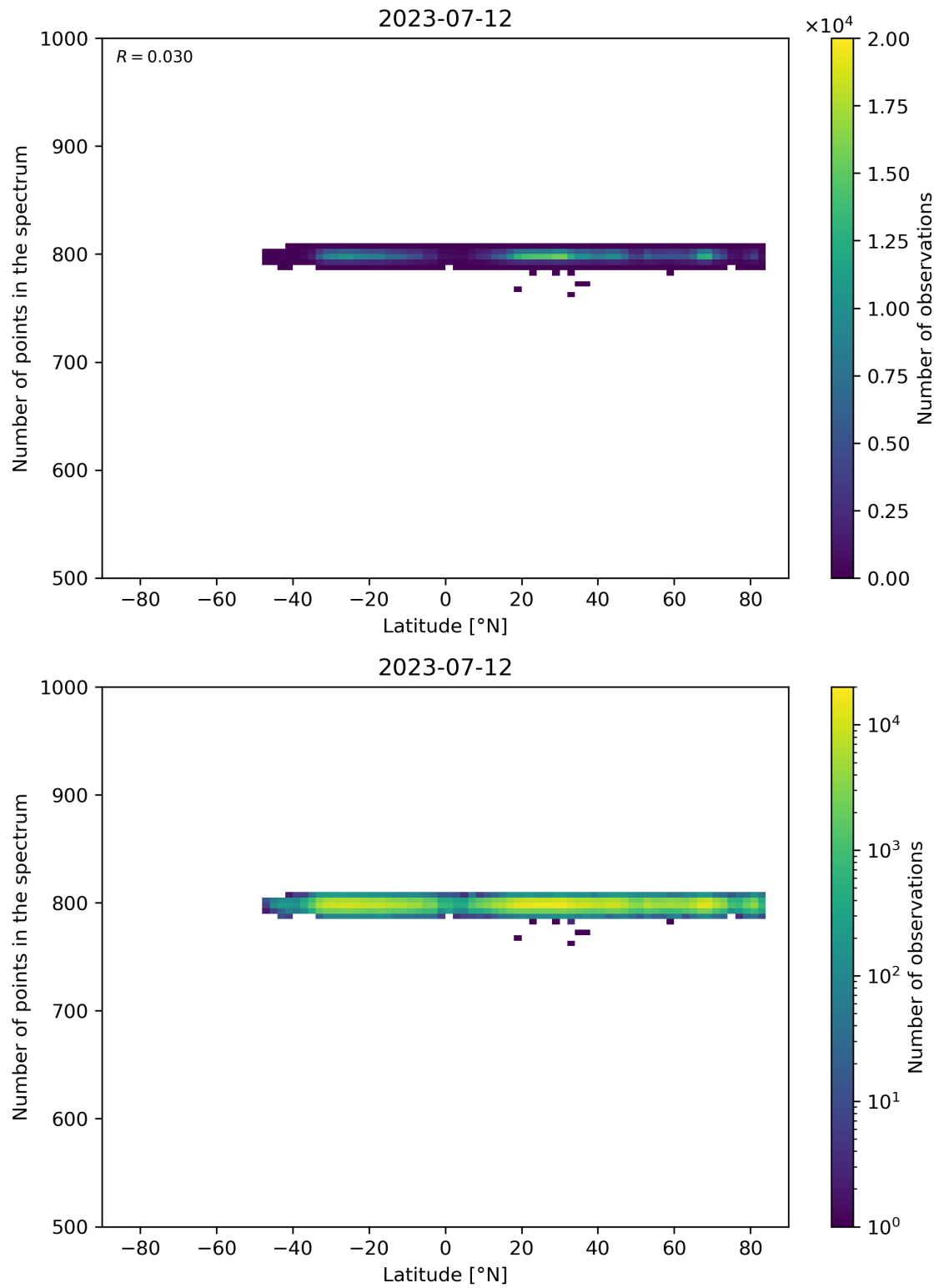
Figure 61: Scatter density plot of “Latitude” against “Number of points in the spectrum” for 2023-07-11 to 2023-07-13.
