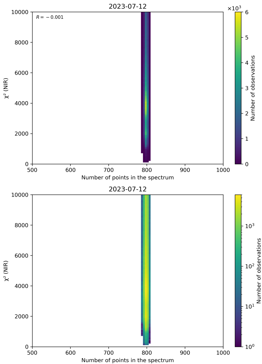
Figure 88: Scatter density plot of “Number of points in the spectrum” against “ \chi^2 (NIR)” for 2023-07-11 to 2023-07-13.
