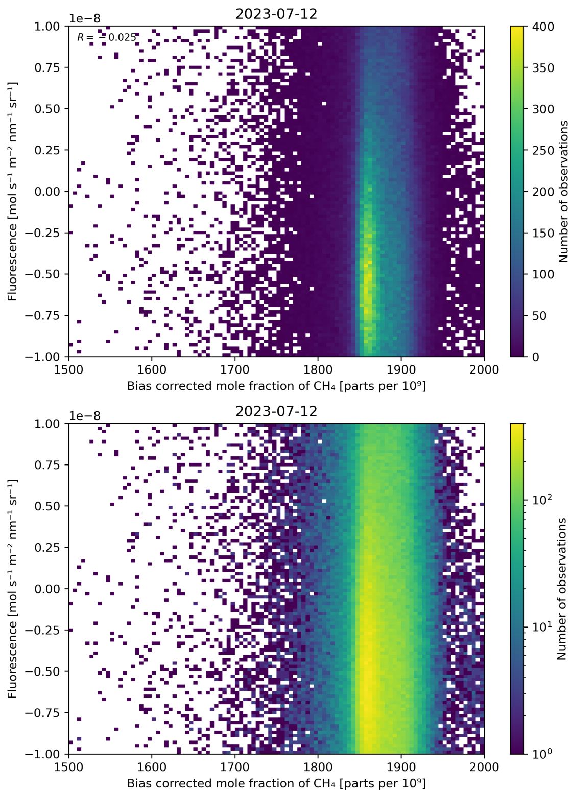
Figure 66: Scatter density plot of “Bias corrected mole fraction of \text{CH}_4 ” against “Fluorescence” for 2023-07-11 to 2023-07-13.
