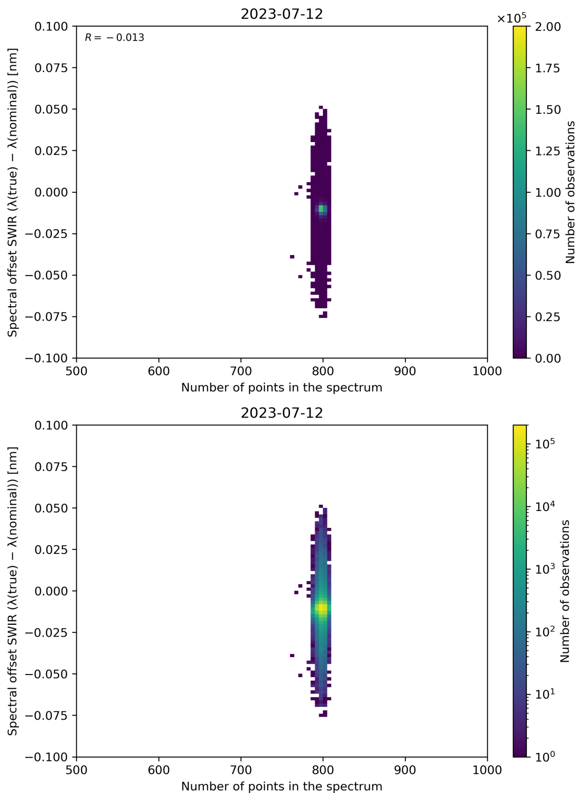
Figure 93: Scatter density plot of “Number of points in the spectrum” against “Spectral offset SWIR ( \lambda(\text{true}) - \lambda(\text{nominal}) )” for 2023-07-11 to 2023-07-13.
