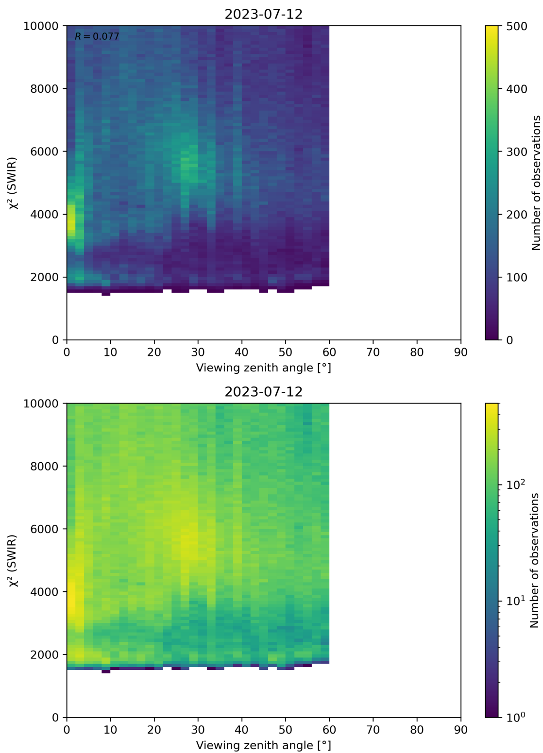
Figure 106: Scatter density plot of “Viewing zenith angle” against “ \chi^2 (SWIR)” for 2023-07-11 to 2023-07-13.
