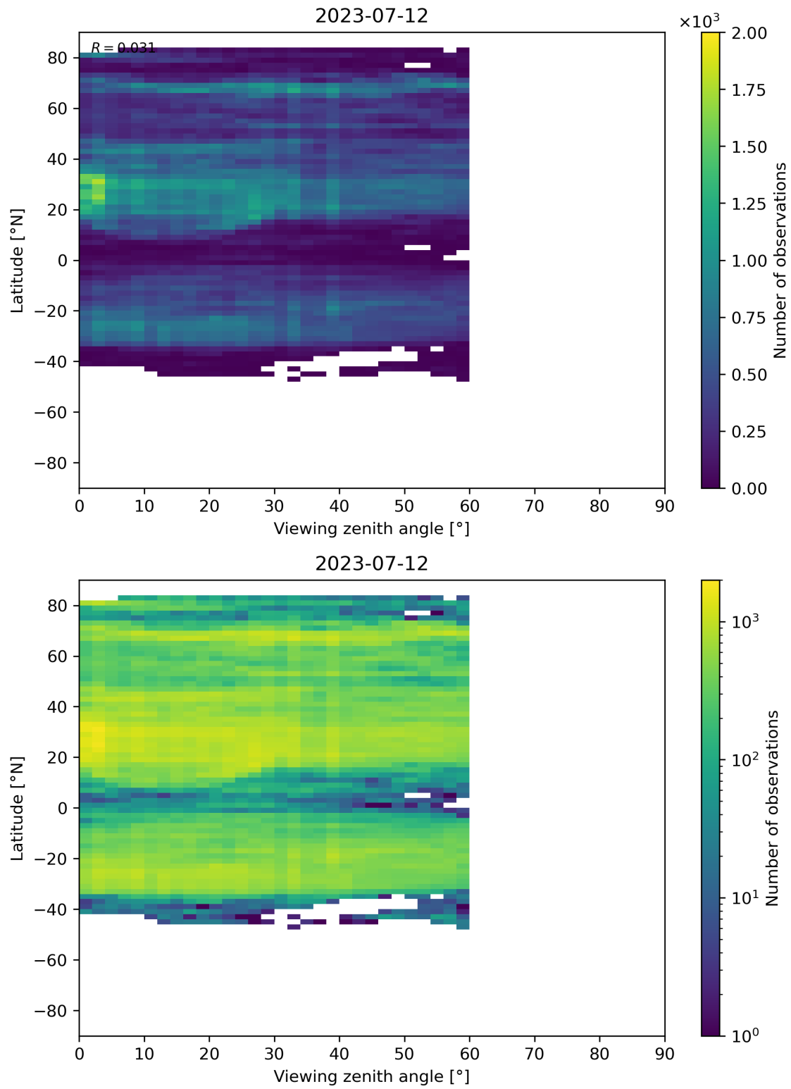
Figure 109: Scatter density plot of “Viewing zenith angle” against “Latitude” for 2023-07-11 to 2023-07-13.
