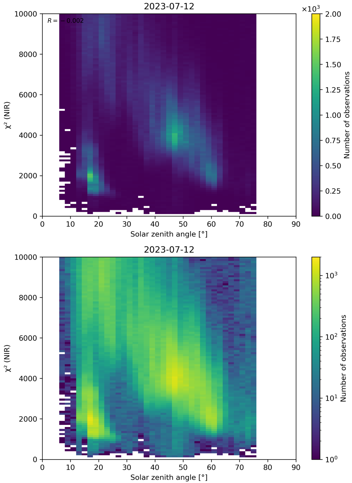
Figure 94: Scatter density plot of “Solar zenith angle” against “ \chi^2 (NIR)” for 2023-07-11 to 2023-07-13.
