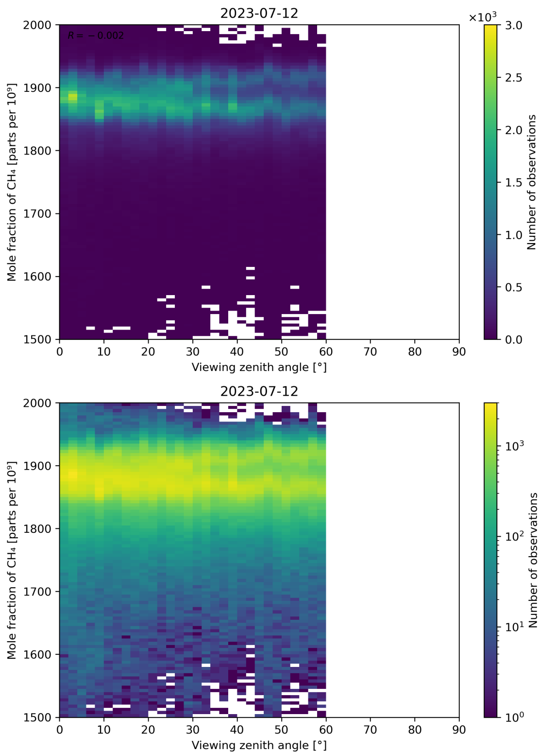
Figure 110: Scatter density plot of “Viewing zenith angle” against “Mole fraction of CH 4 ” for 2023-07-11 to 2023-07-13.
