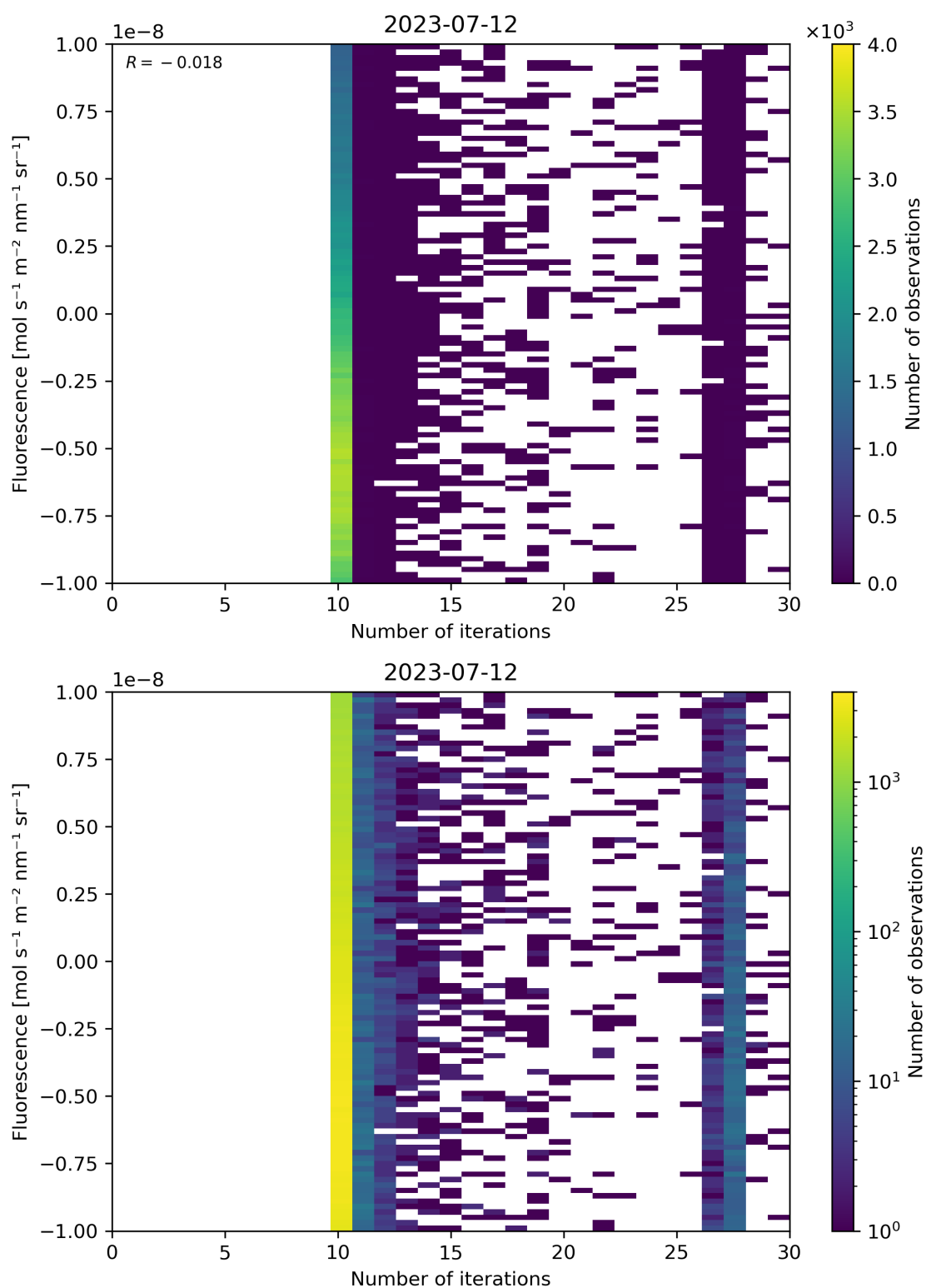
Figure 87: Scatter density plot of “Number of iterations” against “Fluorescence” for 2023-07-11 to 2023-07-13.
