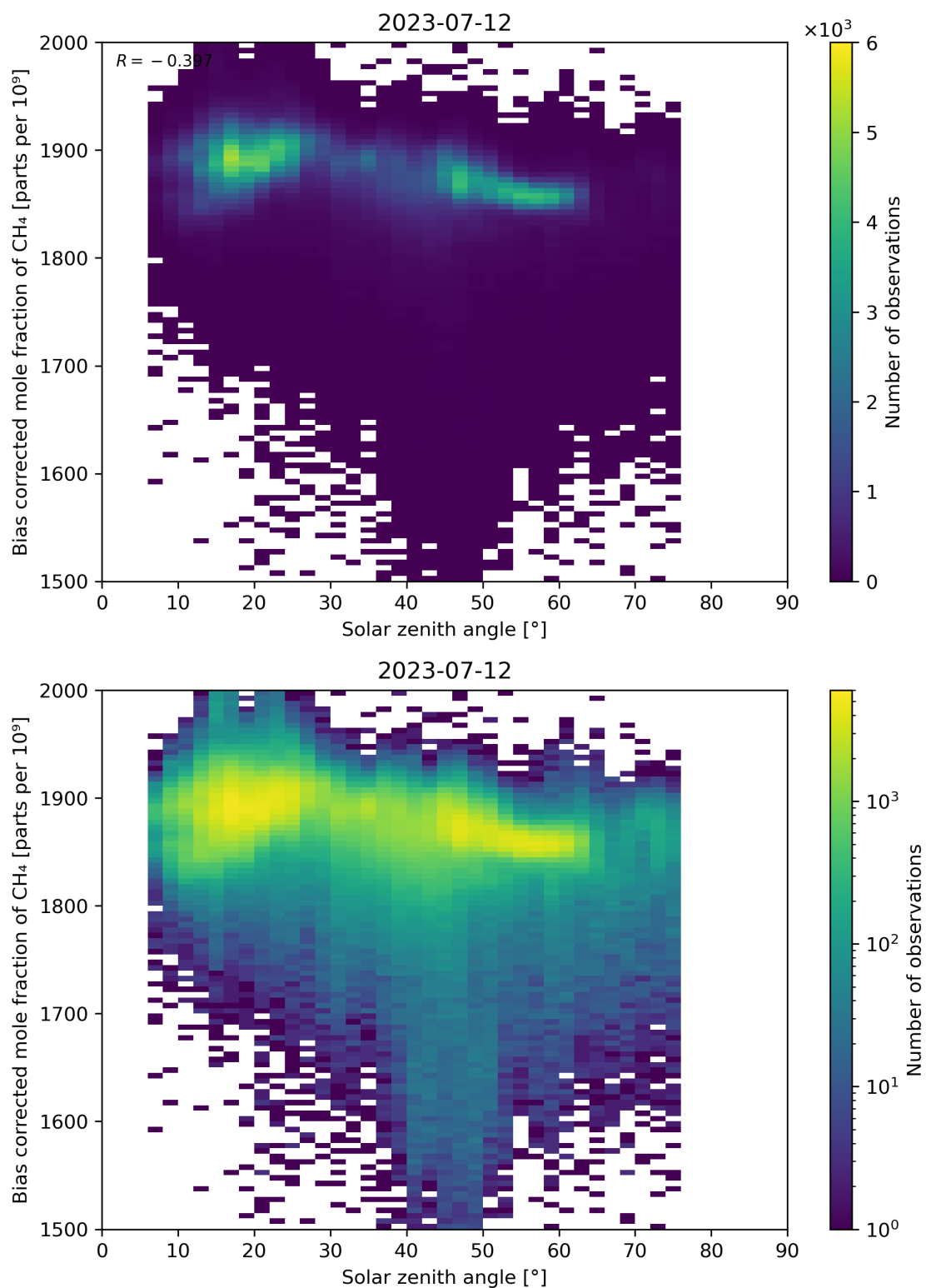
Figure 100: Scatter density plot of “Solar zenith angle” against “Bias corrected mole fraction of CH 4 ” for 2023-07-11 to 2023-07-13.
