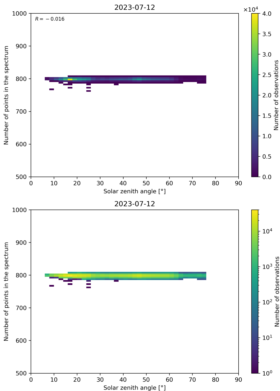
Figure 103: Scatter density plot of “Solar zenith angle” against “Number of points in the spectrum” for 2023-07-11 to 2023-07-13.
