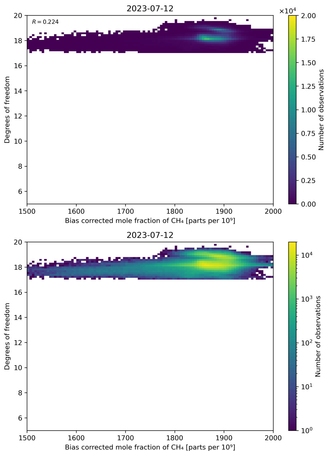
Figure 65: Scatter density plot of “Bias corrected mole fraction of CH 4 ” against “Degrees of freedom” for 2023-07-11 to 2023-07-13.
