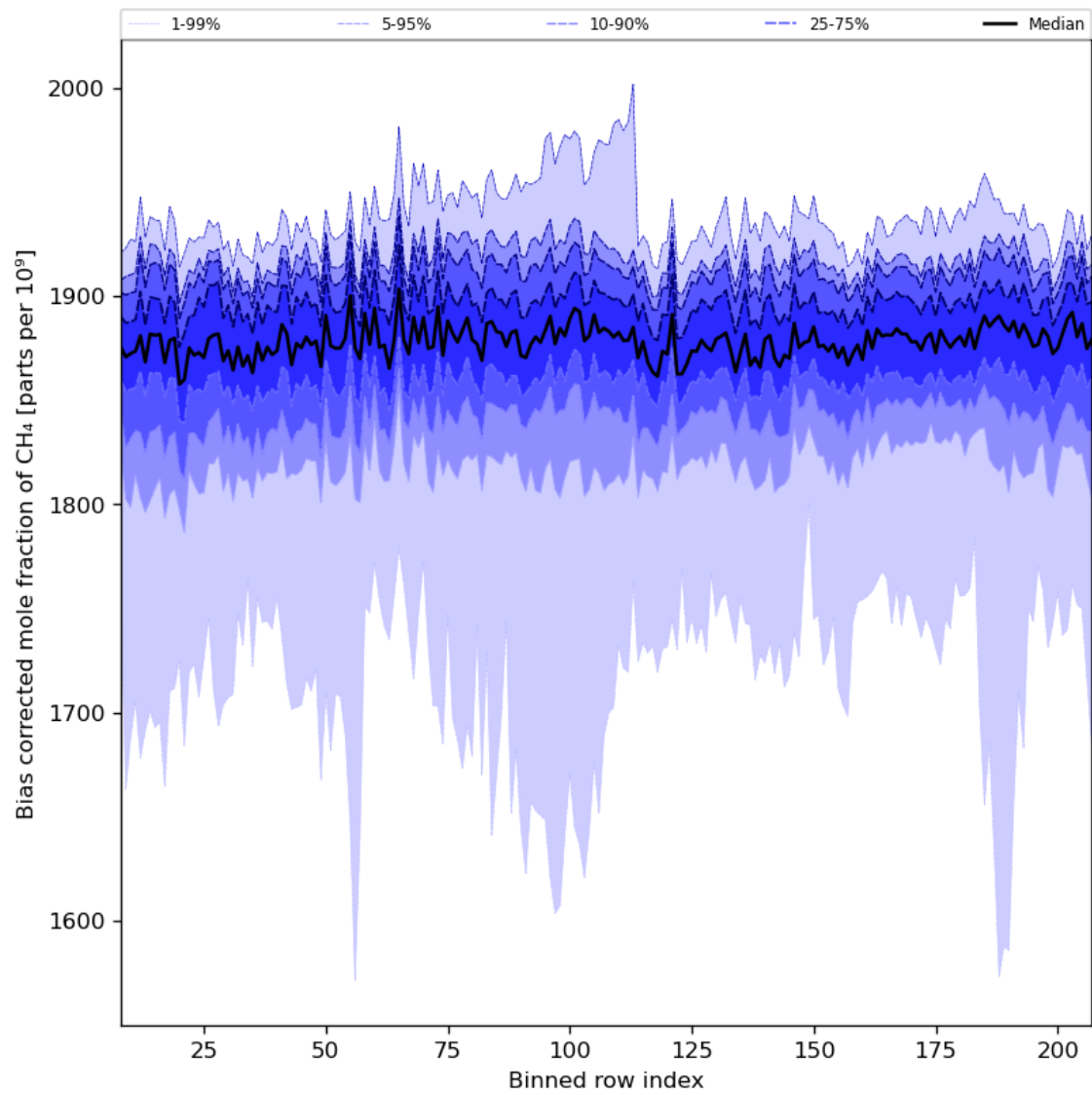
Figure 36: Along track statistics of “Bias corrected mole fraction of CH 4 ” for 2023-07-11 to 2023-07-13
