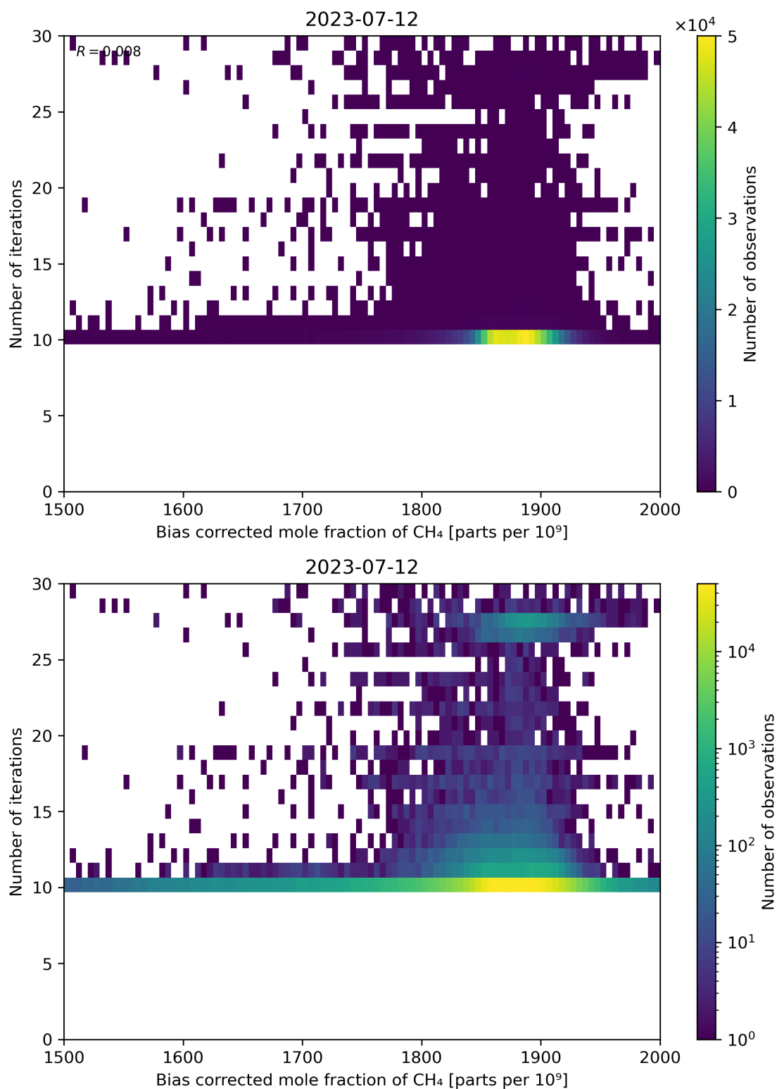
Figure 67: Scatter density plot of “Bias corrected mole fraction of CH 4 ” against “Number of iterations” for 2023-07-11 to 2023-07-13.
