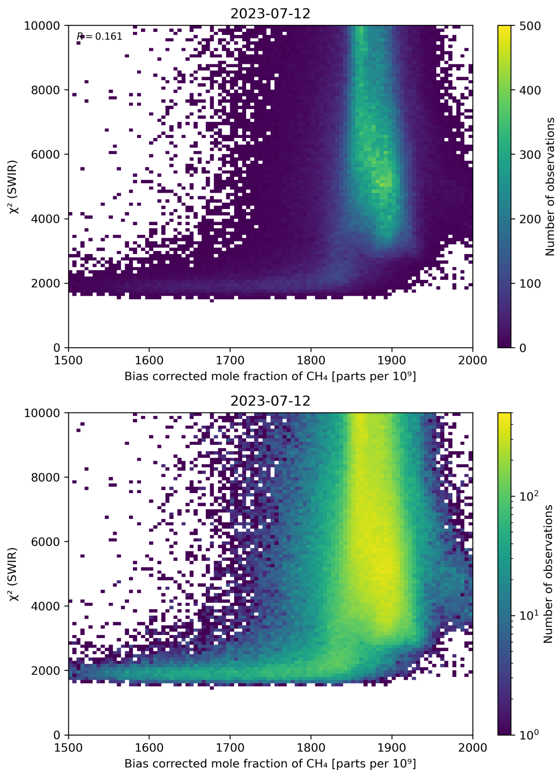
Figure 64: Scatter density plot of “Bias corrected mole fraction of \text{CH}_4 ” against “ \chi^2 (SWIR)” for 2023-07-11 to 2023-07-13.
