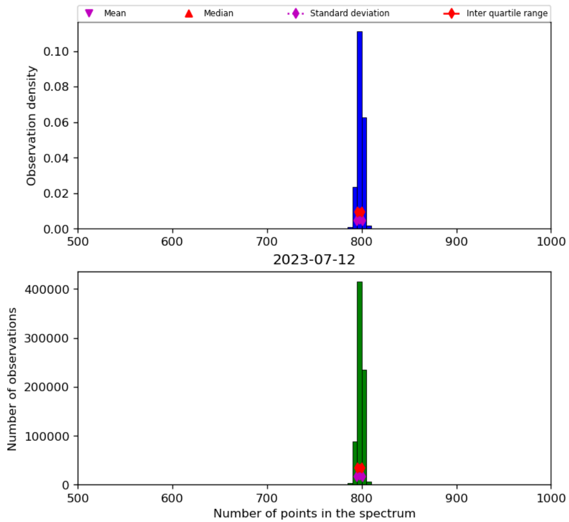
Figure 26: Histogram of “Number of points in the spectrum” for 2023-07-11 to 2023-07-13
