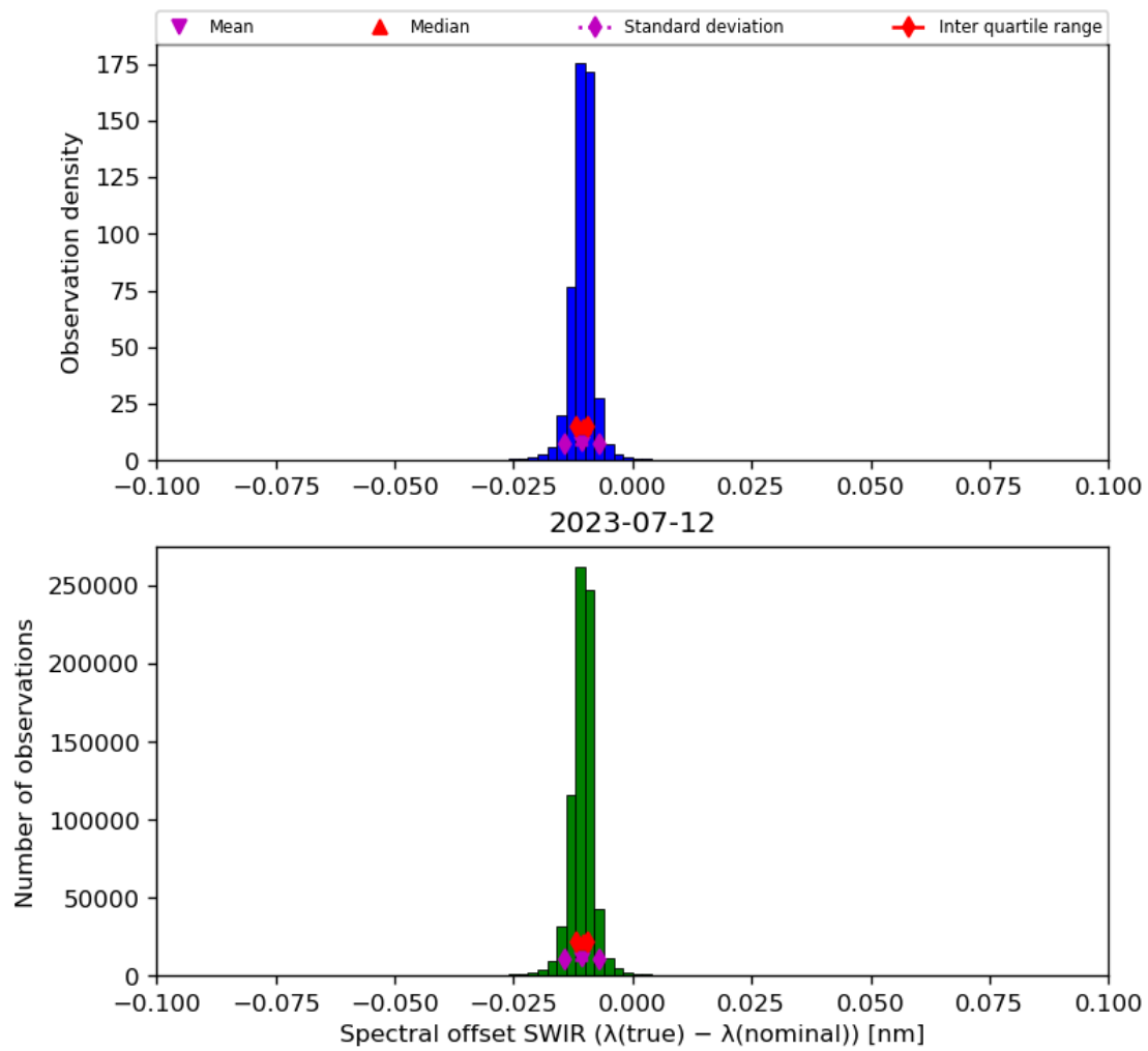
Figure 27: Histogram of “Spectral offset SWIR ( \lambda(\text{true}) - \lambda(\text{nominal}) )” for 2023-07-11 to 2023-07-13
