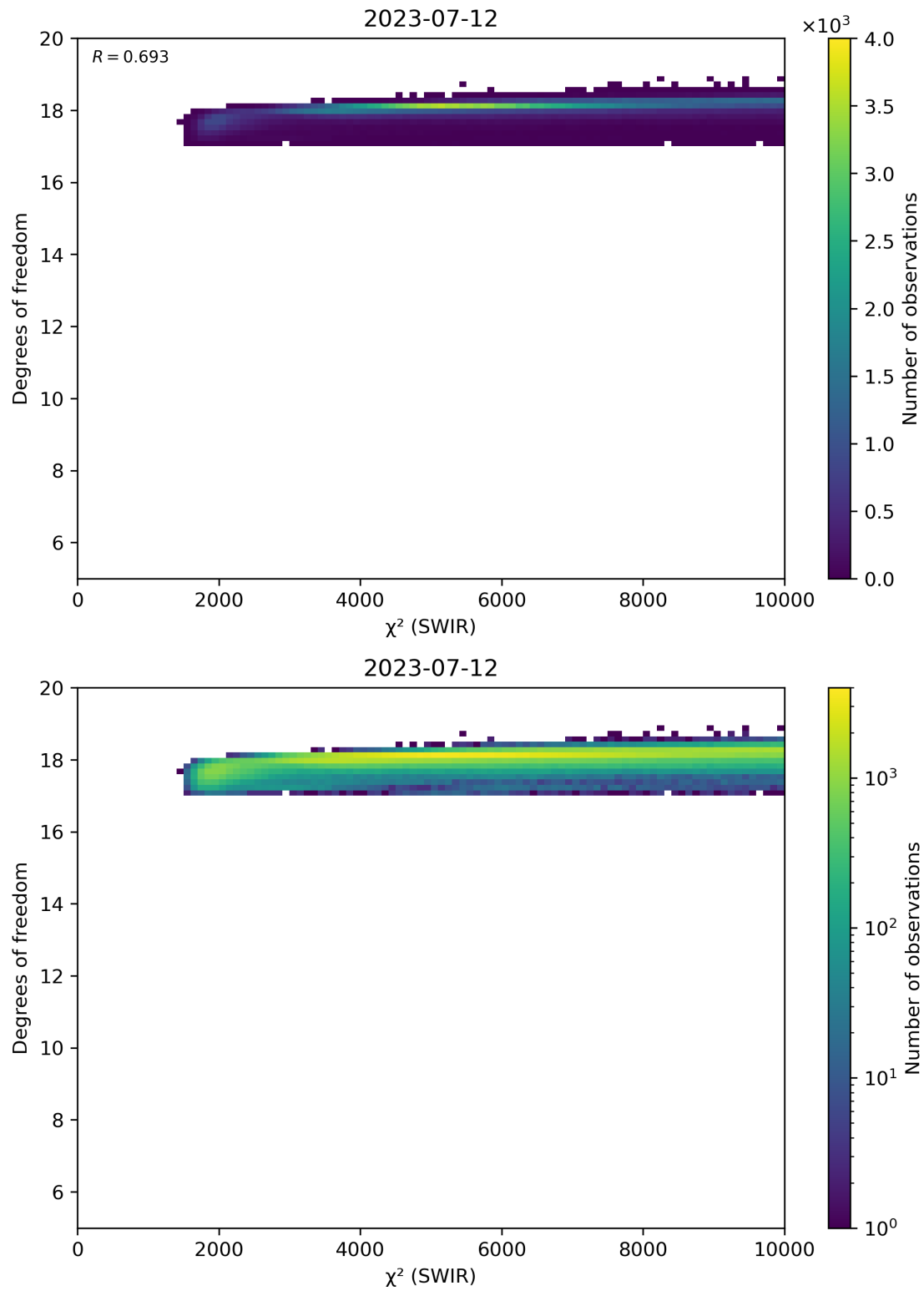
Figure 48: Scatter density plot of “ \chi^2 (SWIR)” against “Degrees of freedom” for 2023-07-11 to 2023-07-13.
