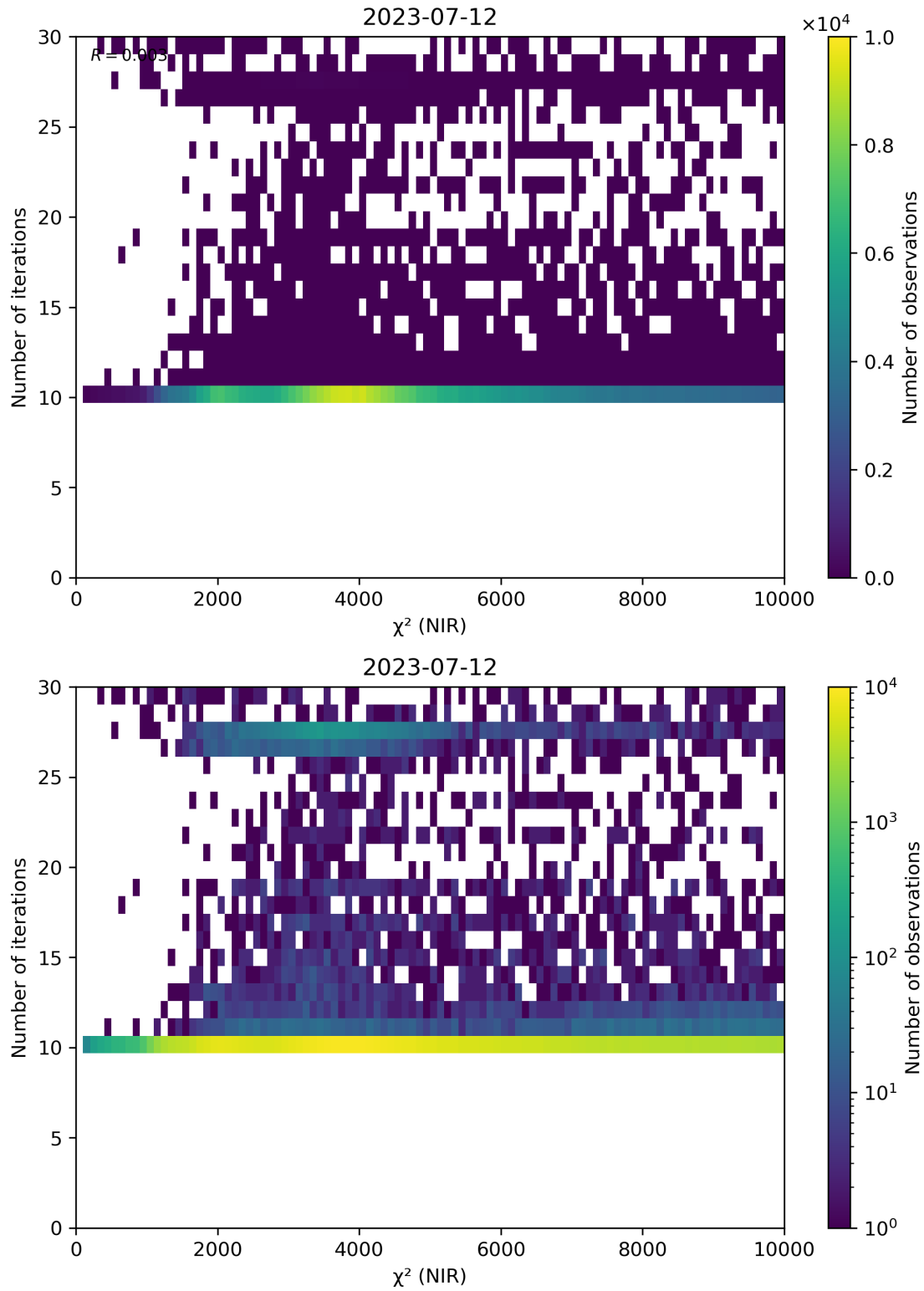
Figure 46: Scatter density plot of “ \chi^2 (NIR)” against “Number of iterations” for 2023-07-11 to 2023-07-13.
