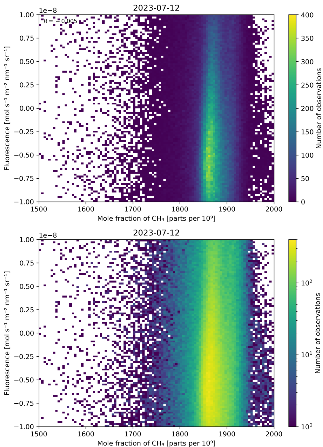
Figure 73: Scatter density plot of “Mole fraction of \text{CH}_4 ” against “Fluorescence” for 2023-07-11 to 2023-07-13.
