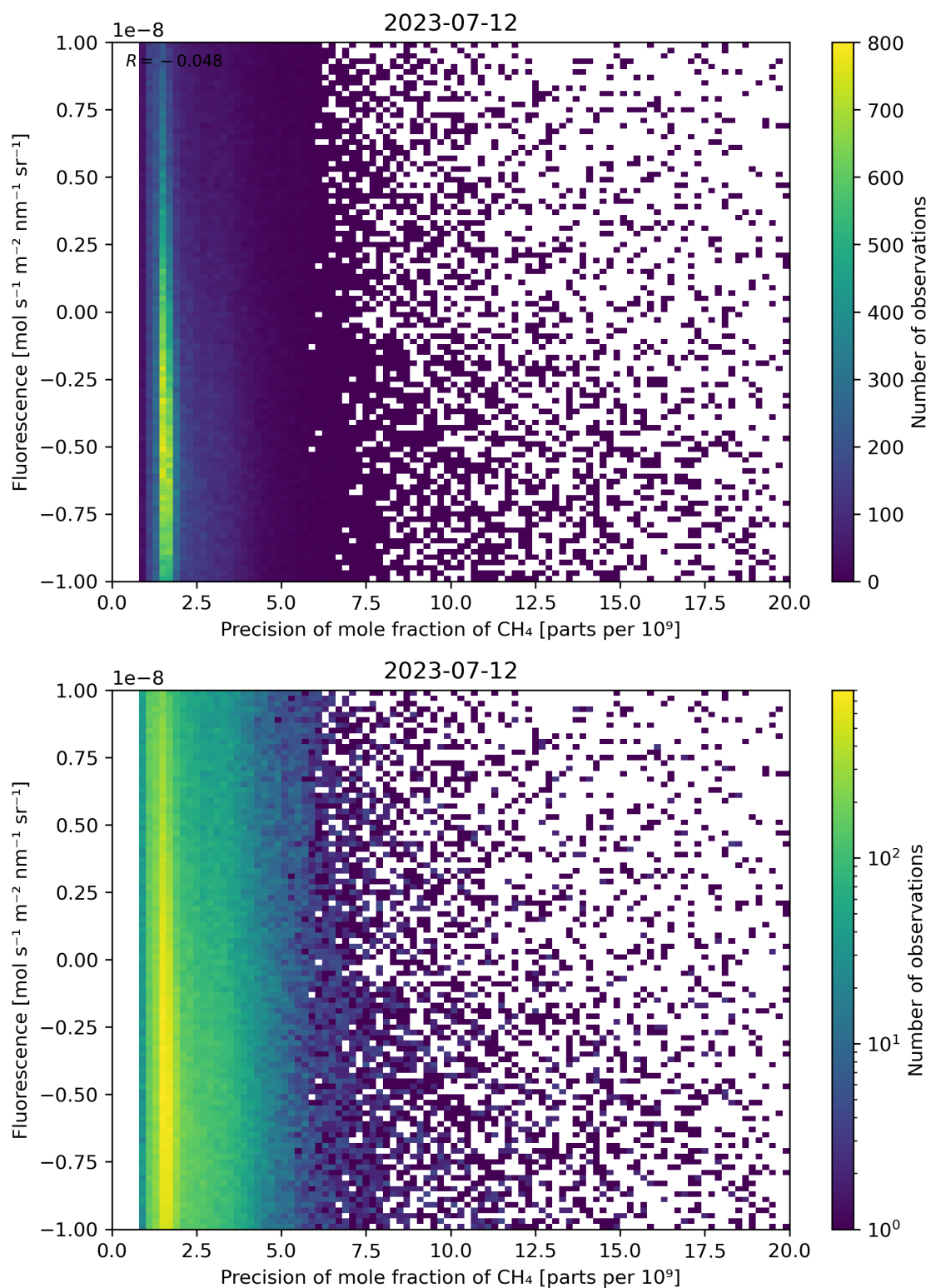
Figure 81: Scatter density plot of “Precision of mole fraction of CH 4 ” against “Fluorescence” for 2023-07-11 to 2023-07-13.
