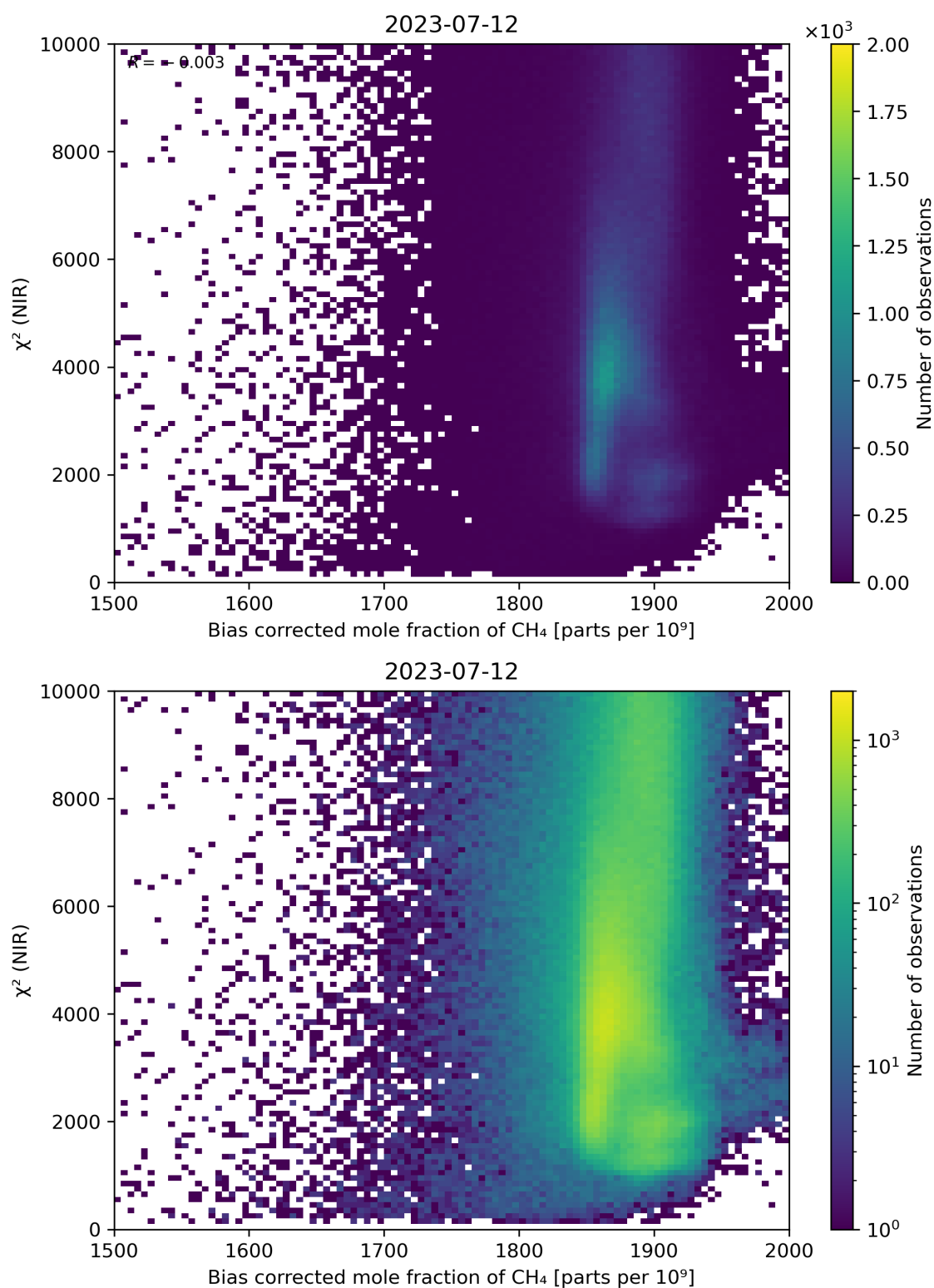
Figure 63: Scatter density plot of “Bias corrected mole fraction of CH 4 ” against “ \chi^2 (NIR)” for 2023-07-11 to 2023-07-13.
