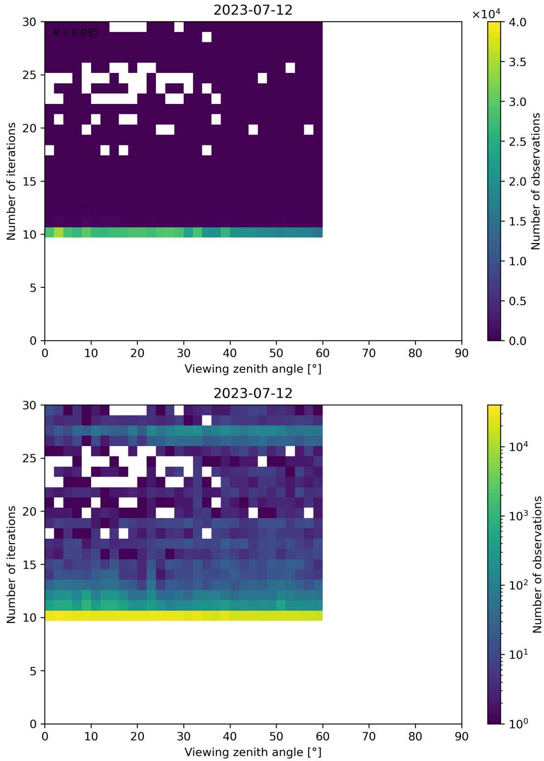
Figure 113: Scatter density plot of “Viewing zenith angle” against “Number of iterations” for 2023-07-11 to 2023-07-13.
