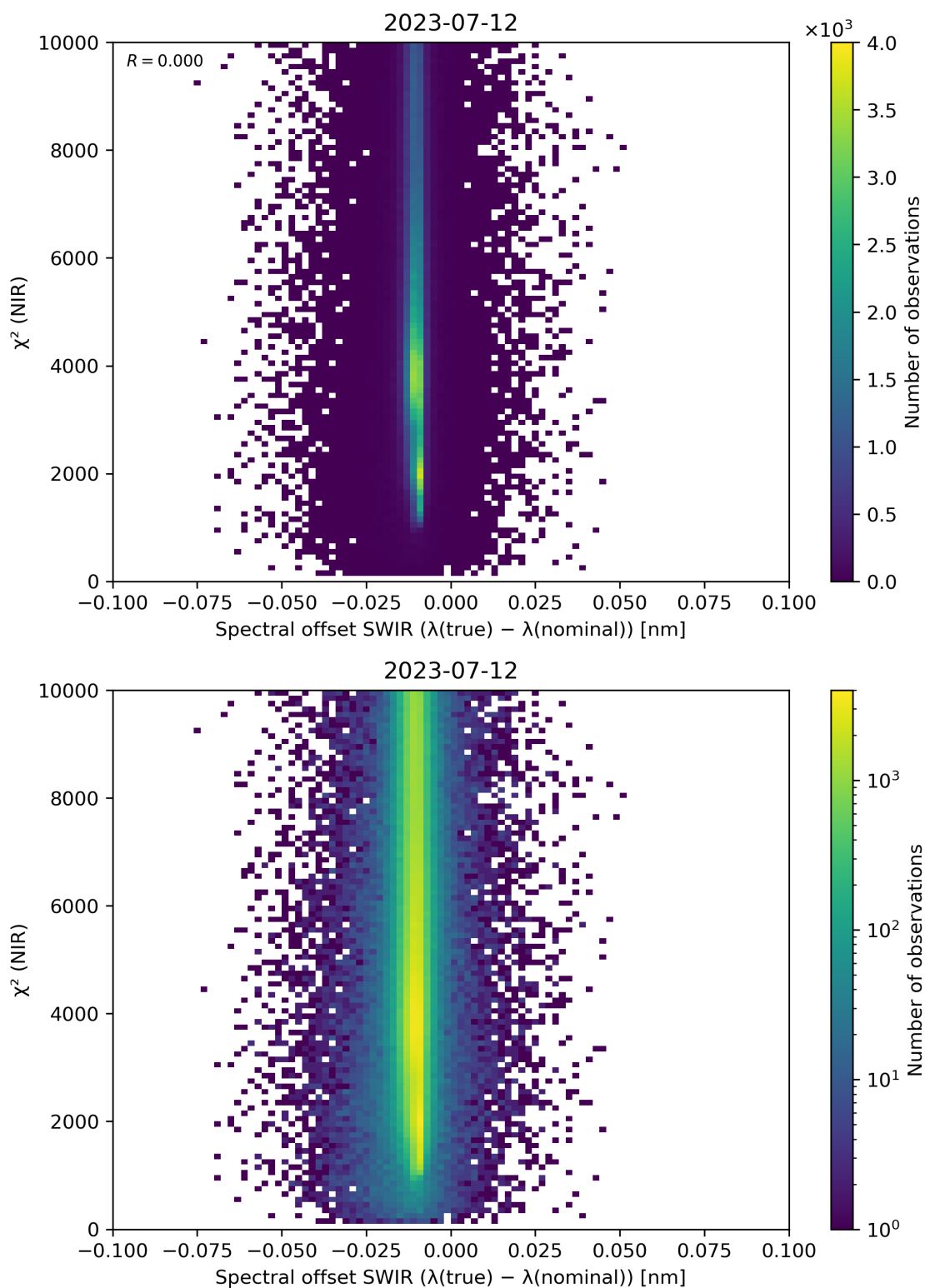
Figure 117: Scatter density plot of “Spectral offset SWIR ( \lambda(\text{true}) - \lambda(\text{nominal}) )” against “ \chi^2 (NIR)” for 2023-07-11 to 2023-07-13.
