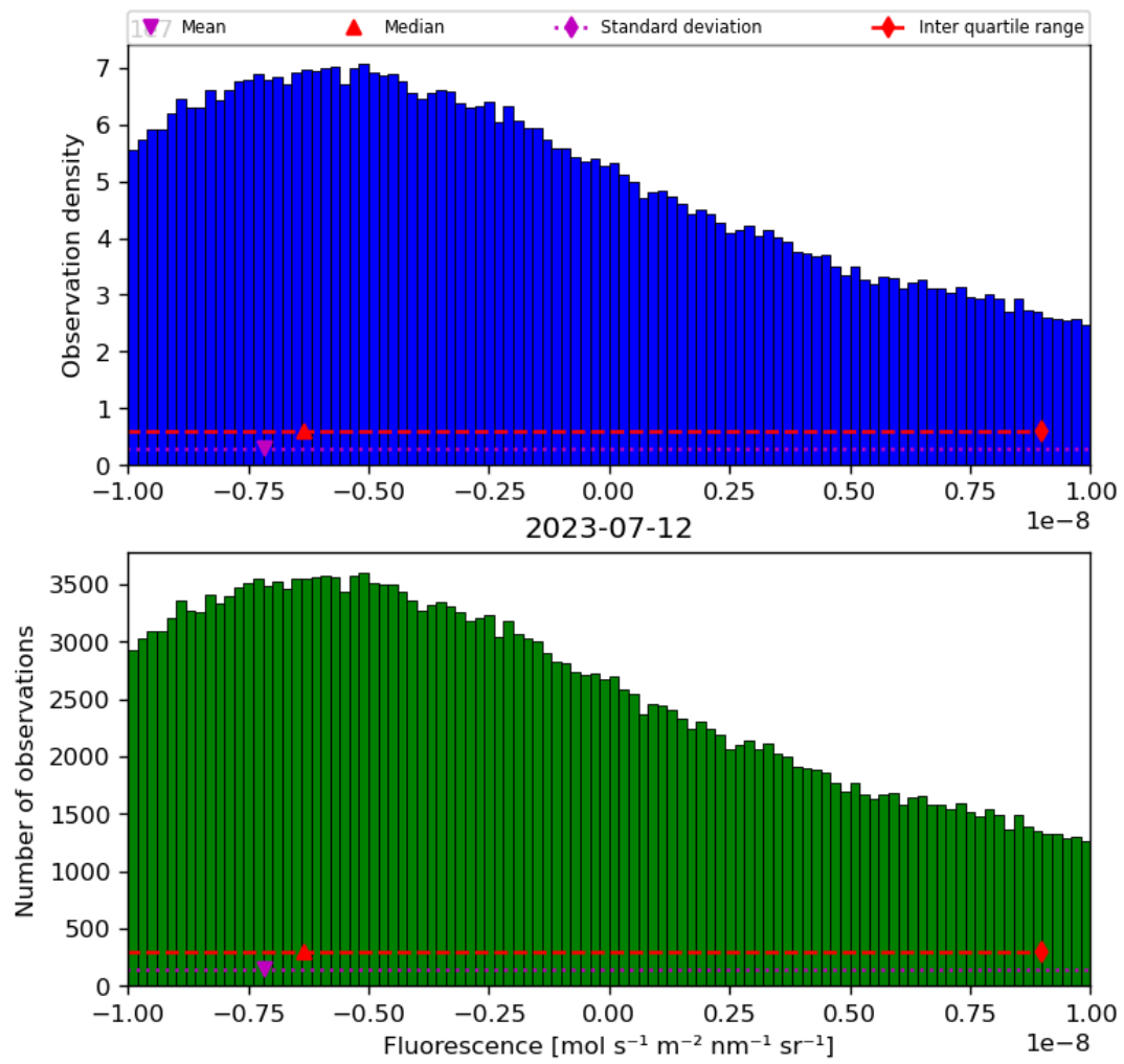
Figure 32: Histogram of “Fluorescence” for 2023-07-11 to 2023-07-13
