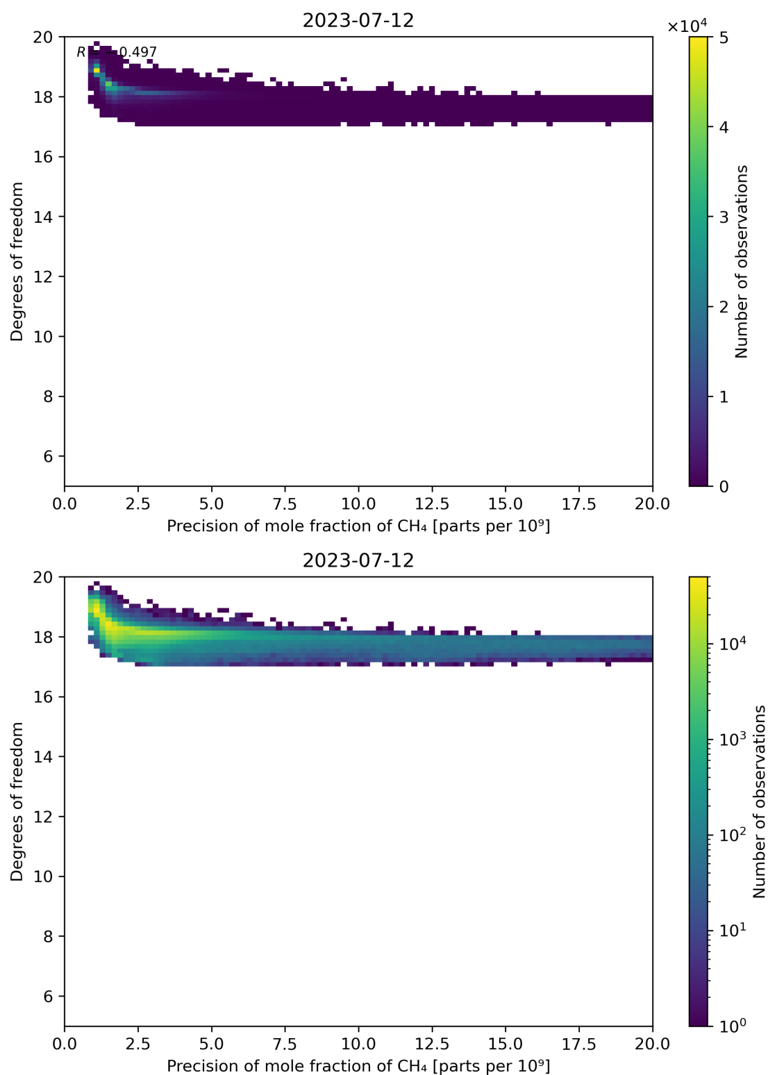
Figure 80: Scatter density plot of “Precision of mole fraction of CH 4 ” against “Degrees of freedom” for 2023-07-11 to 2023-07-13.
