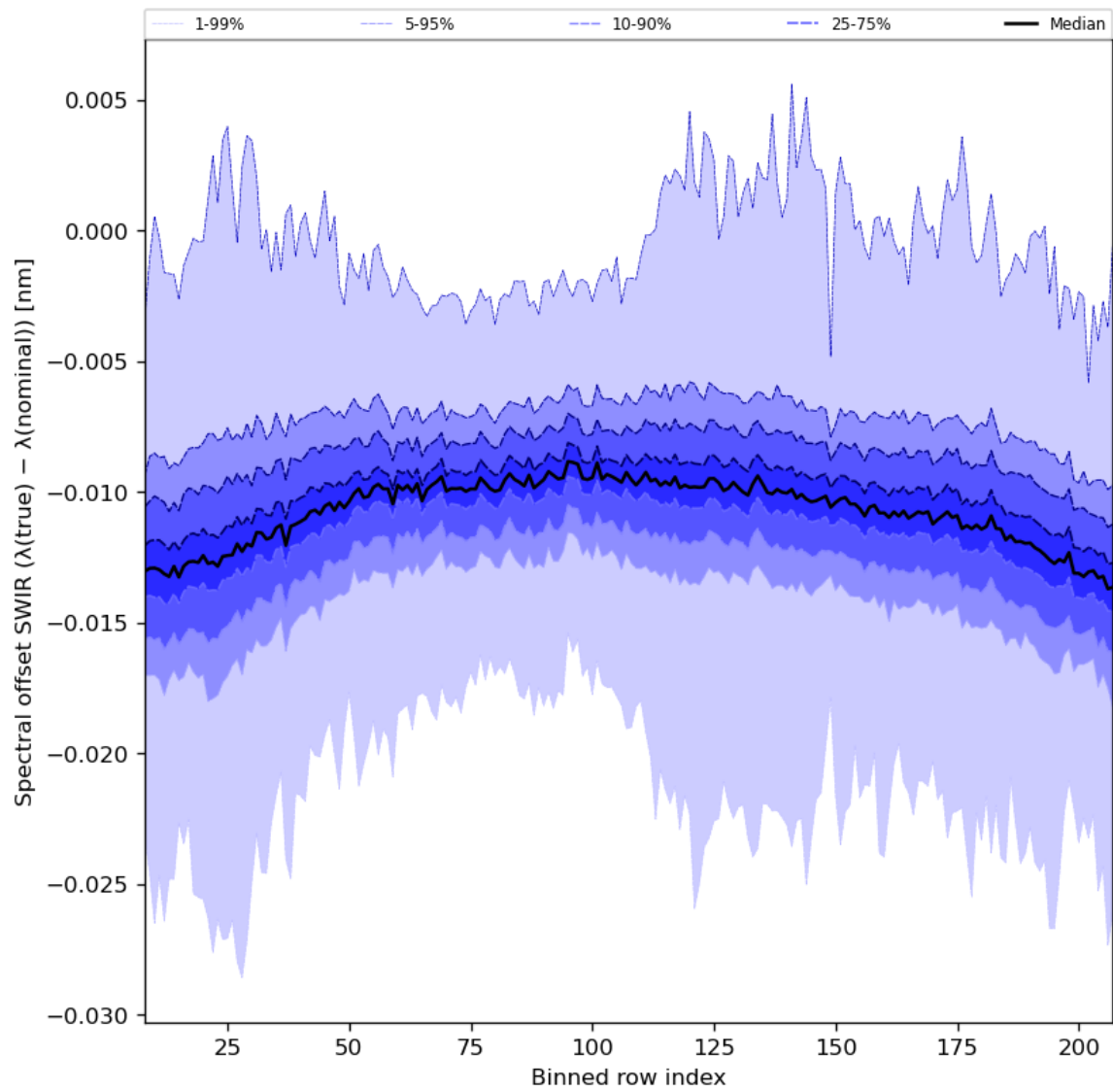
Figure 38: Along track statistics of “Spectral offset SWIR ( \lambda(\text{true}) - \lambda(\text{nominal}) )” for 2023-07-11 to 2023-07-13
