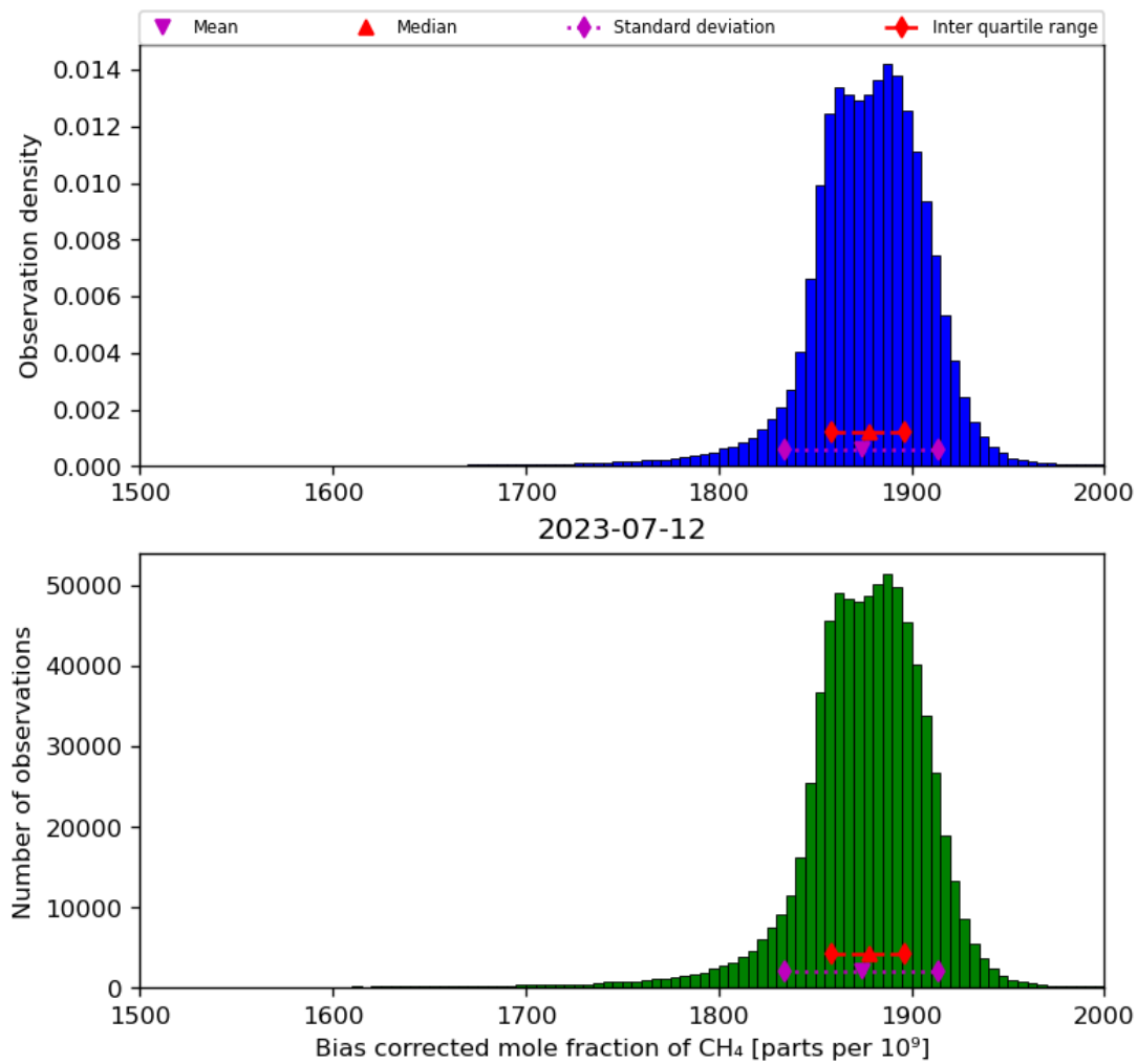
Figure 25: Histogram of “Bias corrected mole fraction of CH 4 ” for 2023-07-11 to 2023-07-13
