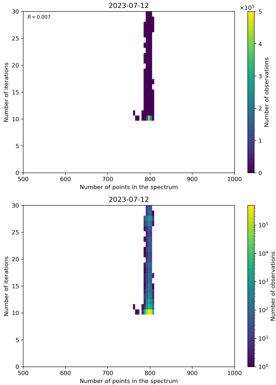
Figure 92: Scatter density plot of “Number of points in the spectrum” against “Number of iterations” for 2023-07-11 to 2023-07-13.
