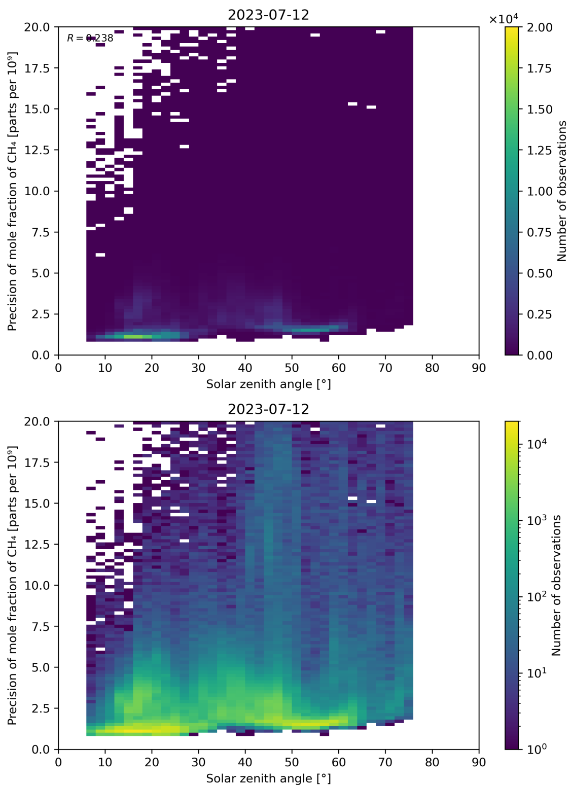
Figure 101: Scatter density plot of “Solar zenith angle” against “Precision of mole fraction of CH 4 ” for 2023-07-11 to 2023-07-13.
