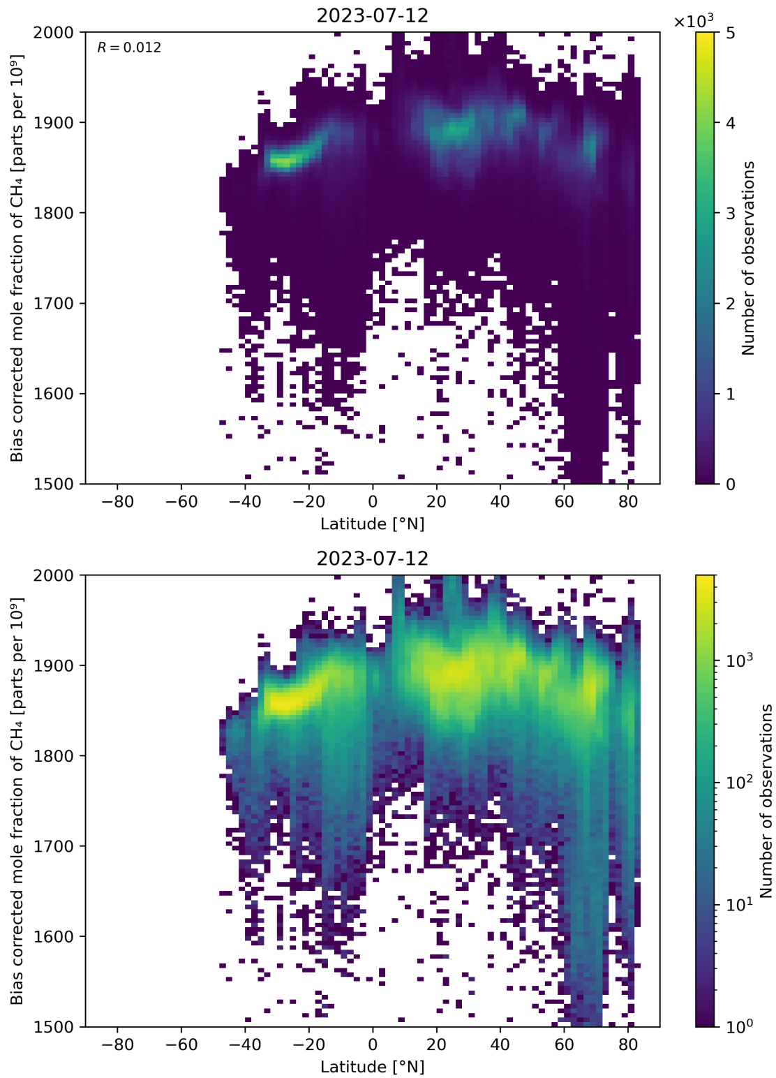
Figure 58: Scatter density plot of “Latitude” against “Bias corrected mole fraction of \text{CH}_4 ” for 2023-07-11 to 2023-07-13.
