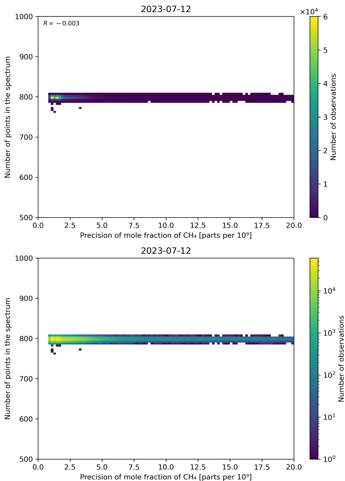
Figure 84: Scatter density plot of “Precision of mole fraction of CH 4 ” against “Number of points in the spectrum” for 2023-07-11 to 2023-07-13.
