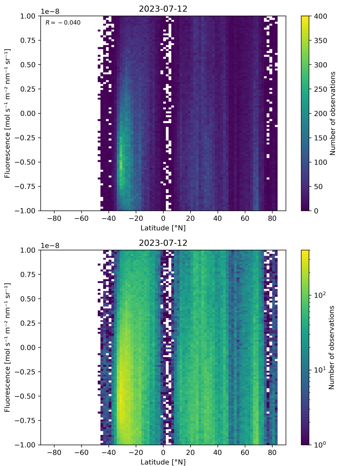
Figure 56: Scatter density plot of “Latitude” against “Fluorescence” for 2023-07-11 to 2023-07-13.
