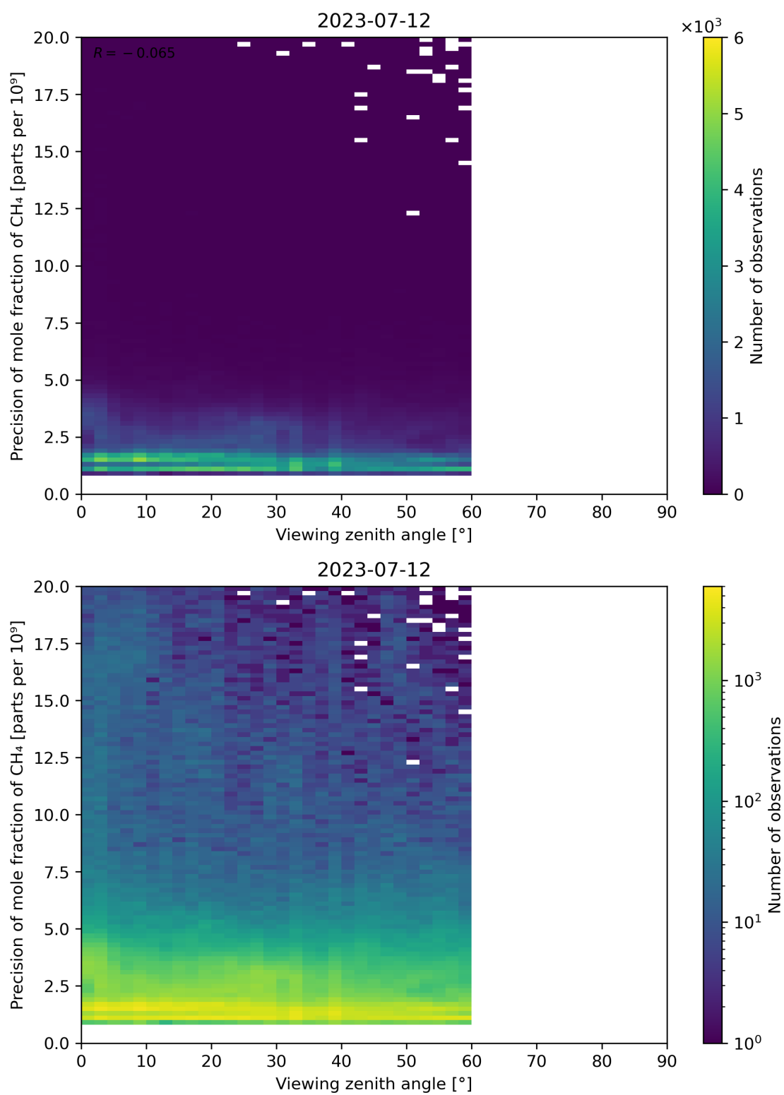
Figure 112: Scatter density plot of “Viewing zenith angle” against “Precision of mole fraction of CH 4 ” for 2023-07-11 to 2023-07-13.
