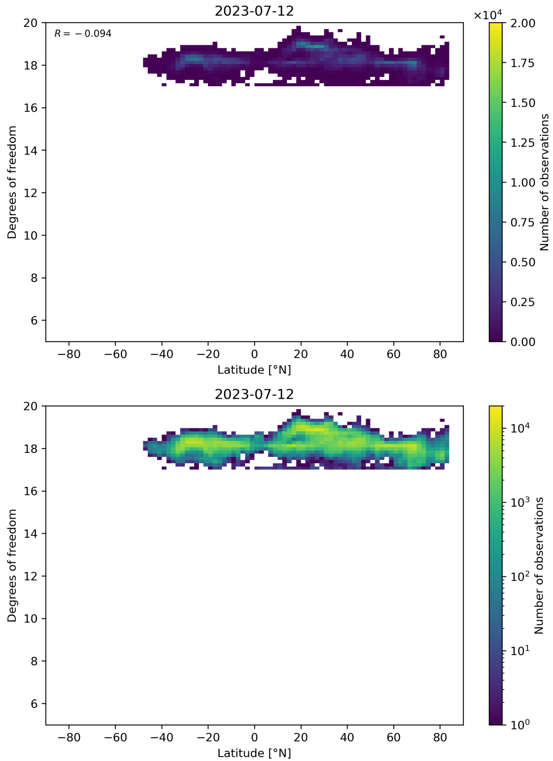
Figure 55: Scatter density plot of “Latitude” against “Degrees of freedom” for 2023-07-11 to 2023-07-13.
