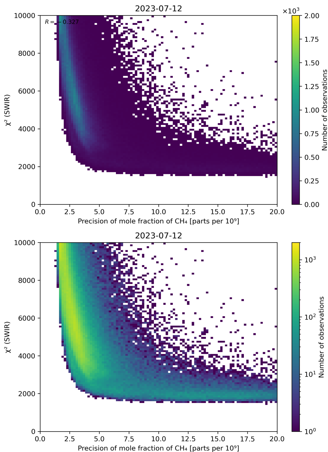
Figure 79: Scatter density plot of “Precision of mole fraction of \text{CH}_4 ” against “ \chi^2 (SWIR)” for 2023-07-11 to 2023-07-13.
