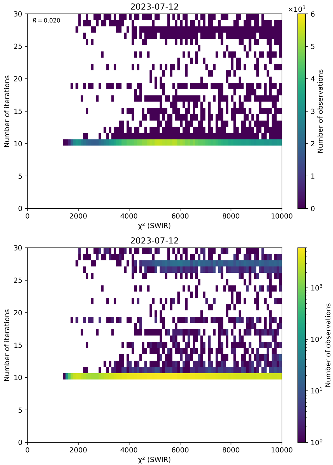
Figure 50: Scatter density plot of “ \chi^2 (SWIR)” against “Number of iterations” for 2023-07-11 to 2023-07-13.
