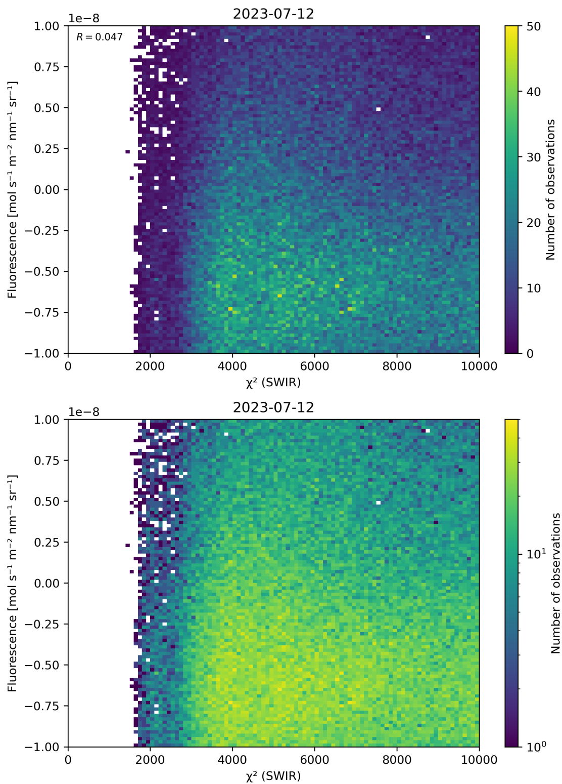
Figure 49: Scatter density plot of “ \chi^2 (SWIR)” against “Fluorescence” for 2023-07-11 to 2023-07-13.
