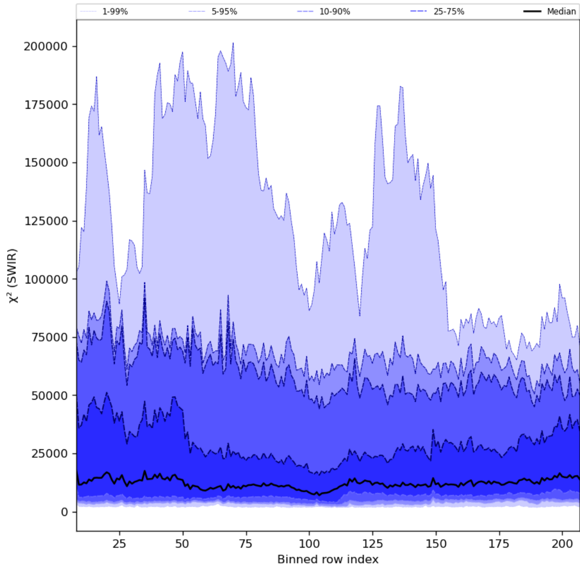
Figure 39: Along track statistics of “ \chi^2 (SWIR)” for 2023-07-11 to 2023-07-13
