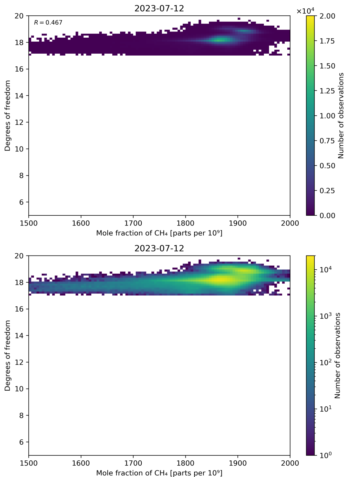
Figure 72: Scatter density plot of “Mole fraction of CH 4 ” against “Degrees of freedom” for 2023-07-11 to 2023-07-13.
