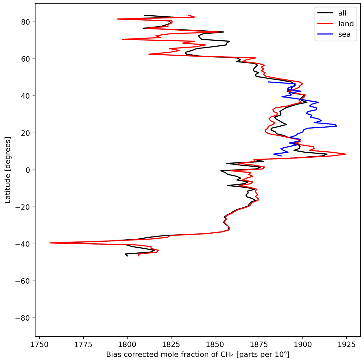
Figure 14: Zonal average of “Bias corrected mole fraction of CH 4 ” for 2023-07-11 to 2023-07-13.
