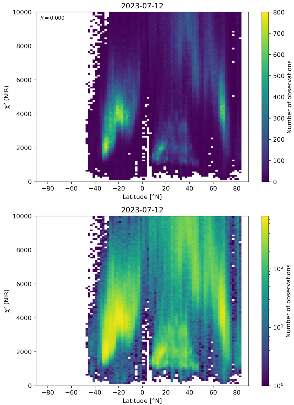
Figure 53: Scatter density plot of “Latitude” against “ \chi^2 (NIR)” for 2023-07-11 to 2023-07-13.
