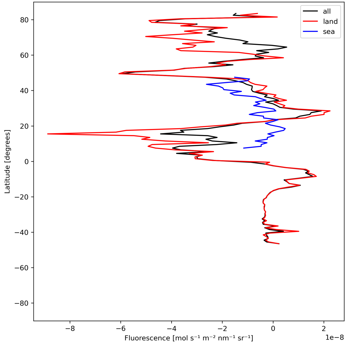
Figure 21: Zonal average of “Fluorescence” for 2023-07-11 to 2023-07-13.
