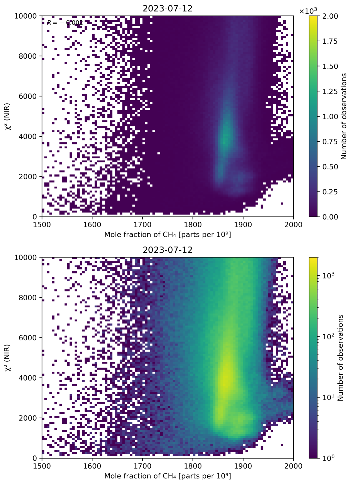
Figure 70: Scatter density plot of “Mole fraction of \text{CH}_4 ” against “ \chi^2 (NIR)” for 2023-07-11 to 2023-07-13.
