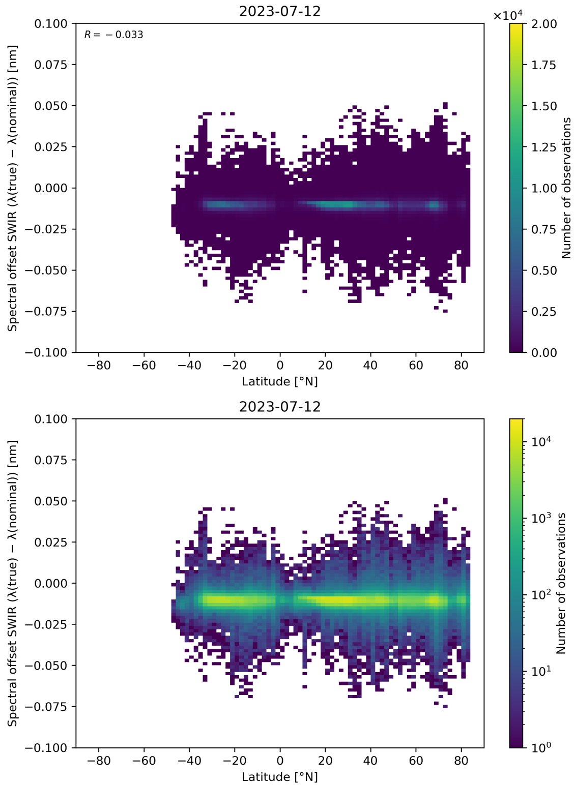
Figure 62: Scatter density plot of “Latitude” against “Spectral offset SWIR ( \lambda(\text{true}) - \lambda(\text{nominal}) )” for 2023-07-11 to 2023-07-13.
