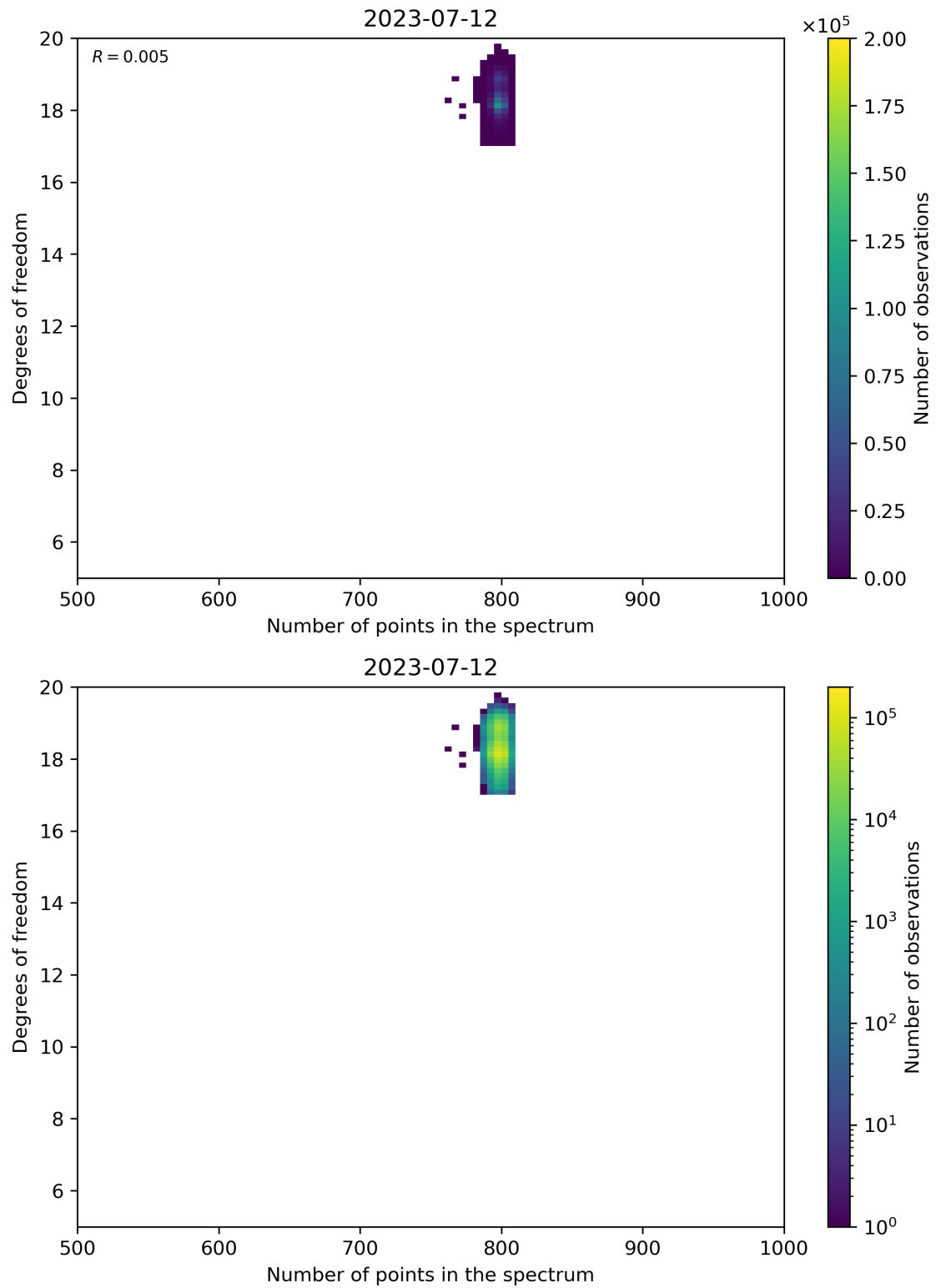
Figure 90: Scatter density plot of “Number of points in the spectrum” against “Degrees of freedom” for 2023-07-11 to 2023-07-13.
