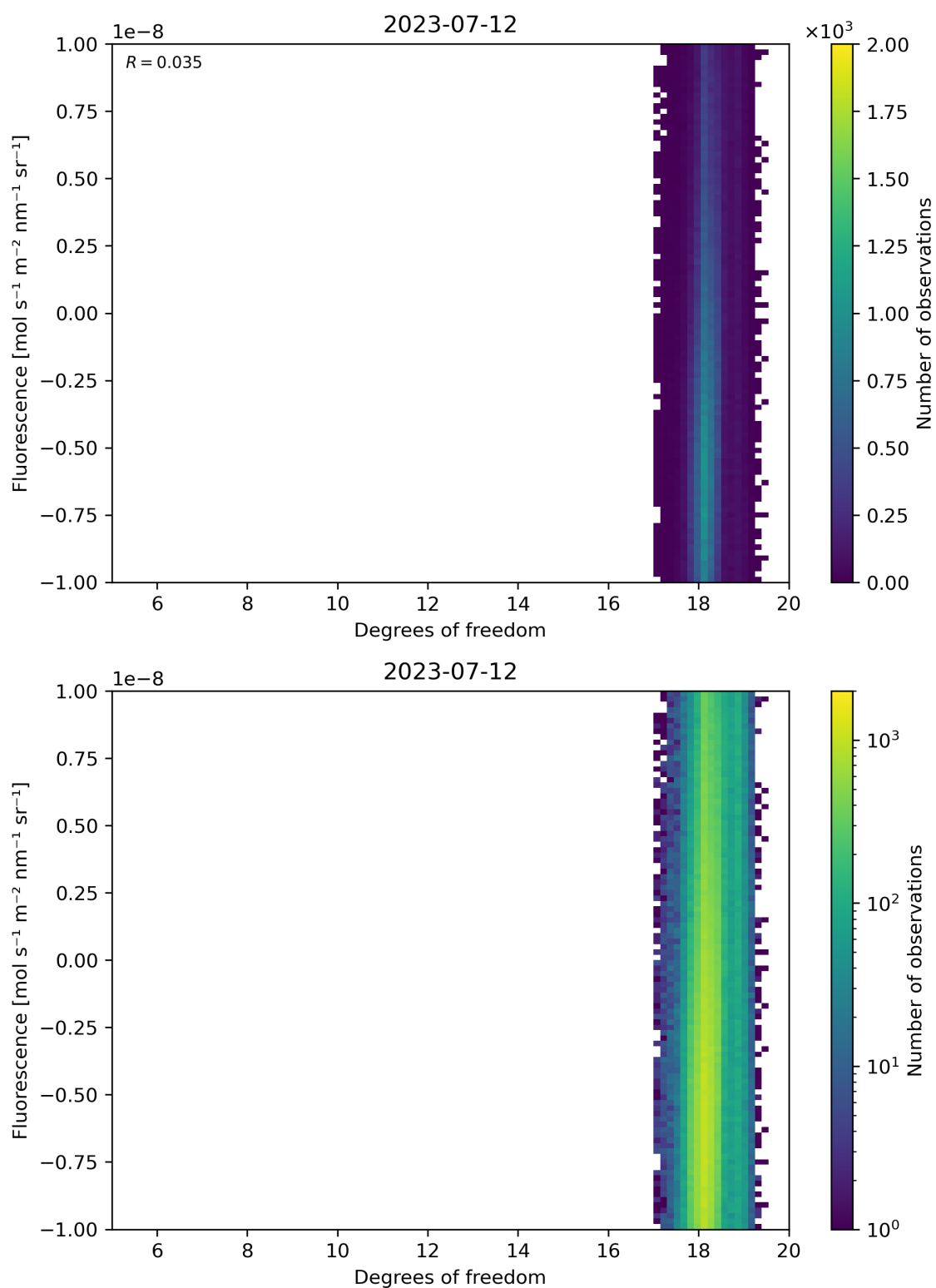
Figure 51: Scatter density plot of “Degrees of freedom” against “Fluorescence” for 2023-07-11 to 2023-07-13.
