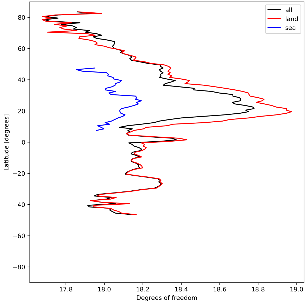
Figure 19: Zonal average of “Degrees of freedom” for 2023-07-11 to 2023-07-13.
