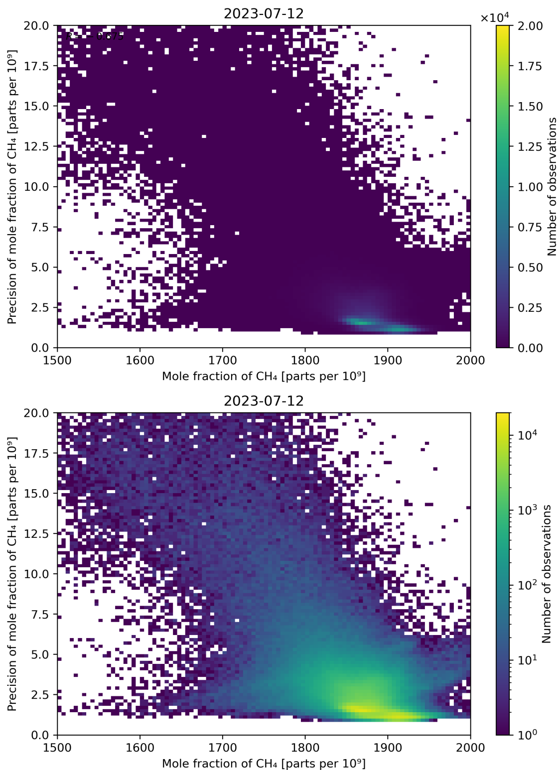
Figure 75: Scatter density plot of “Mole fraction of CH 4 ” against “Precision of mole fraction of CH 4 ” for 2023-07-11 to 2023-07-13.
