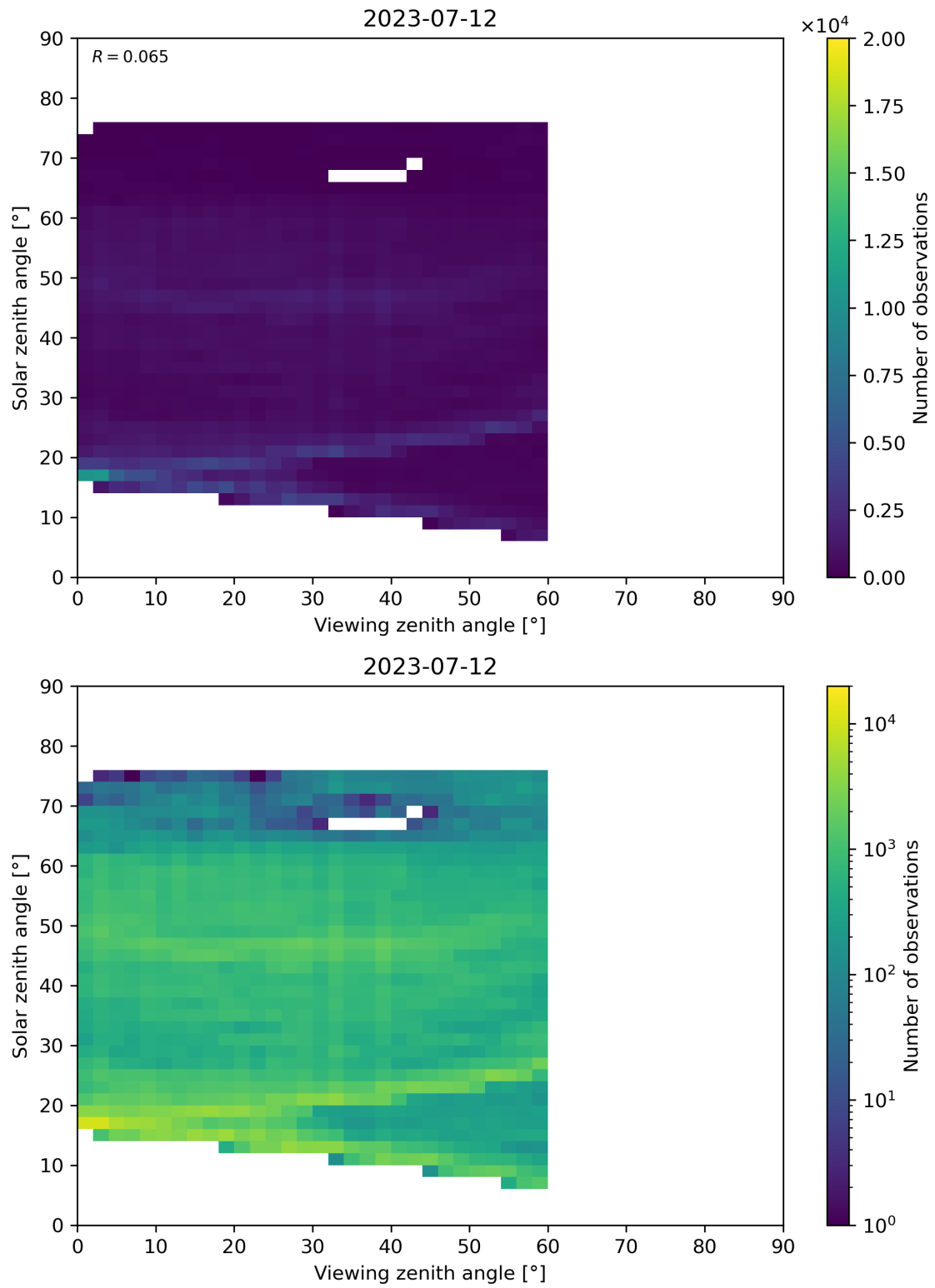
Figure 115: Scatter density plot of “Viewing zenith angle” against “Solar zenith angle” for 2023-07-11 to 2023-07-13.
