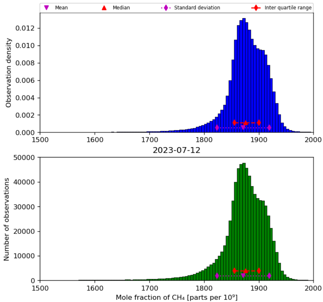
Figure 23: Histogram of “Mole fraction of CH 4 ” for 2023-07-11 to 2023-07-13
