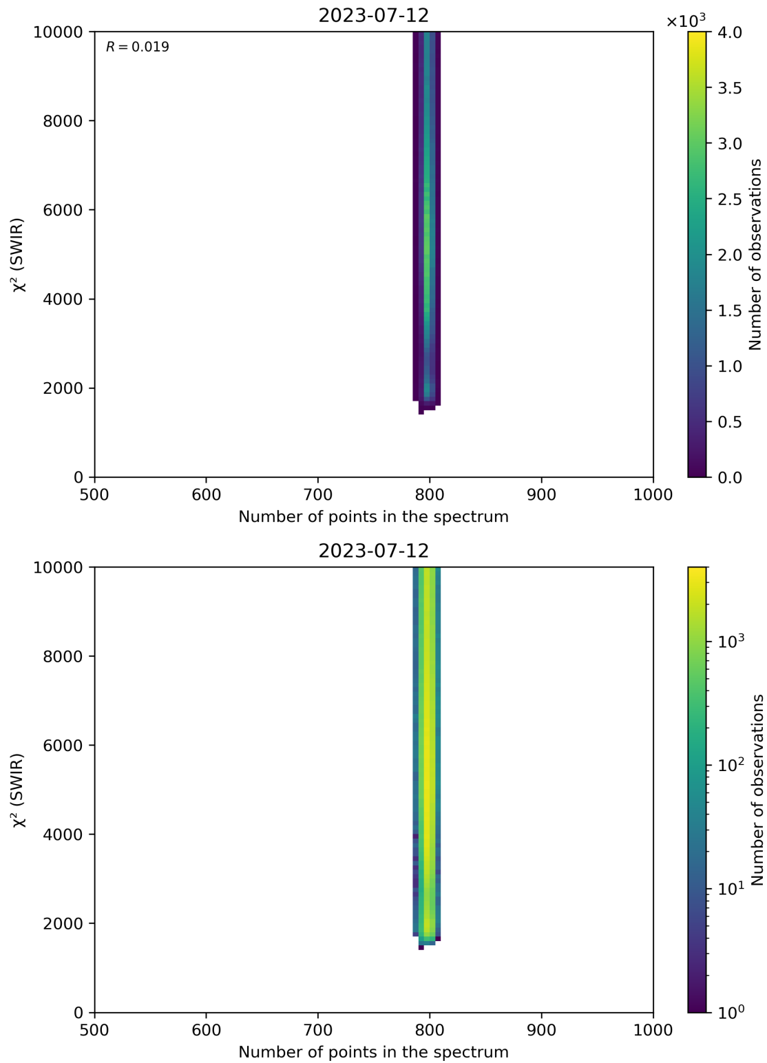
Figure 89: Scatter density plot of “Number of points in the spectrum” against “ \chi^2 (SWIR)” for 2023-07-11 to 2023-07-13.
