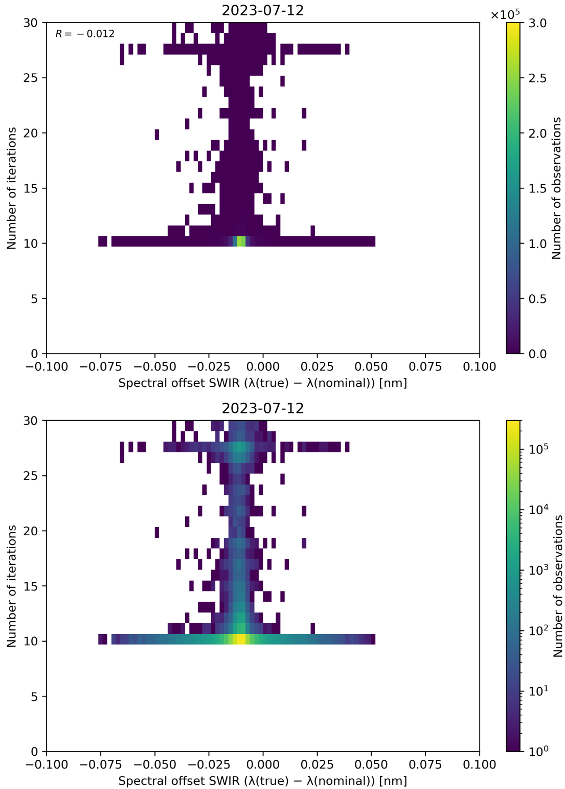
Figure 121: Scatter density plot of “Spectral offset SWIR ( \lambda(\text{true}) - \lambda(\text{nominal}) )” against “Number of iterations” for 2023-07-11 to 2023-07-13.
