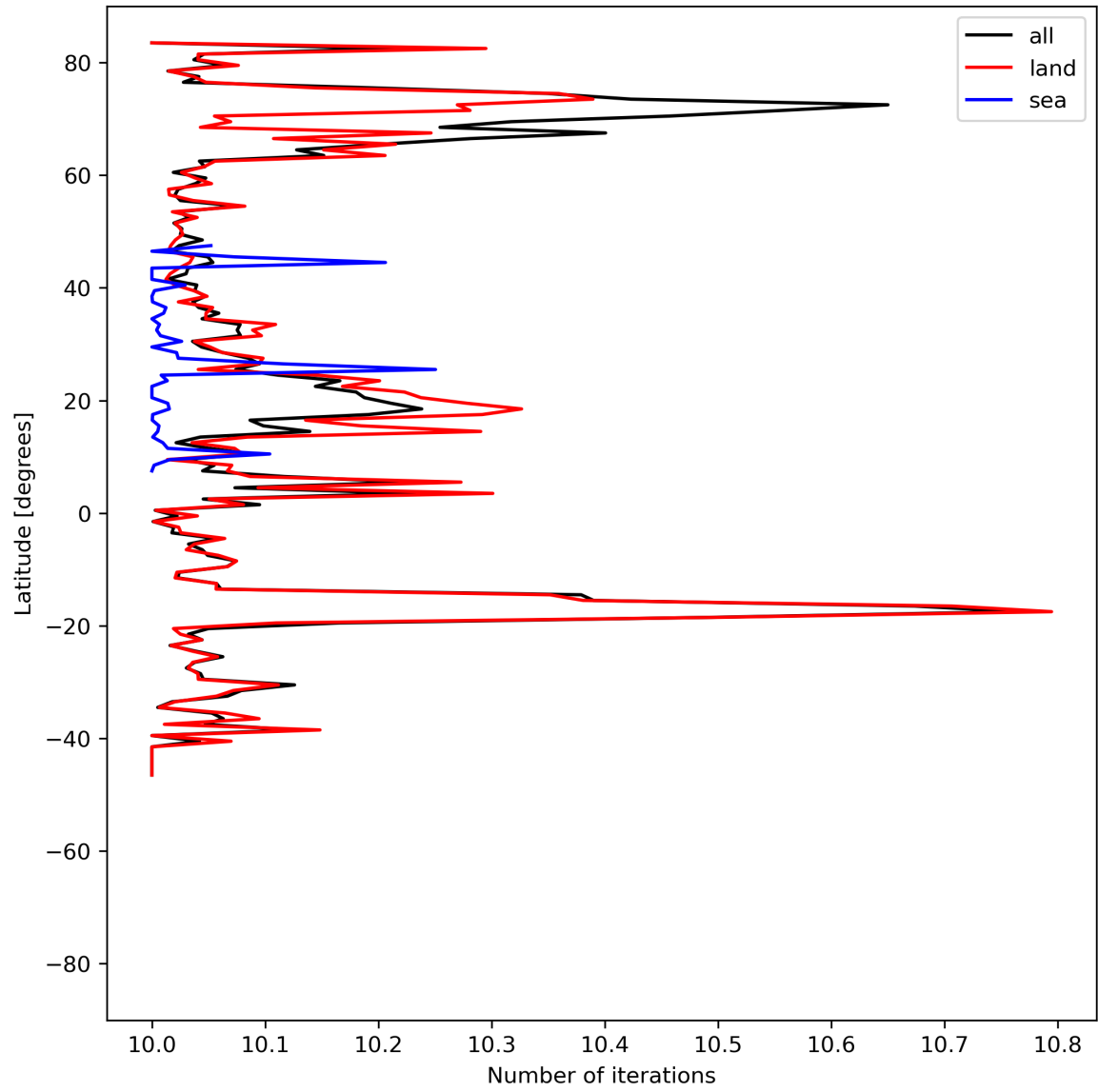
Figure 20: Zonal average of “Number of iterations” for 2023-07-11 to 2023-07-13.
