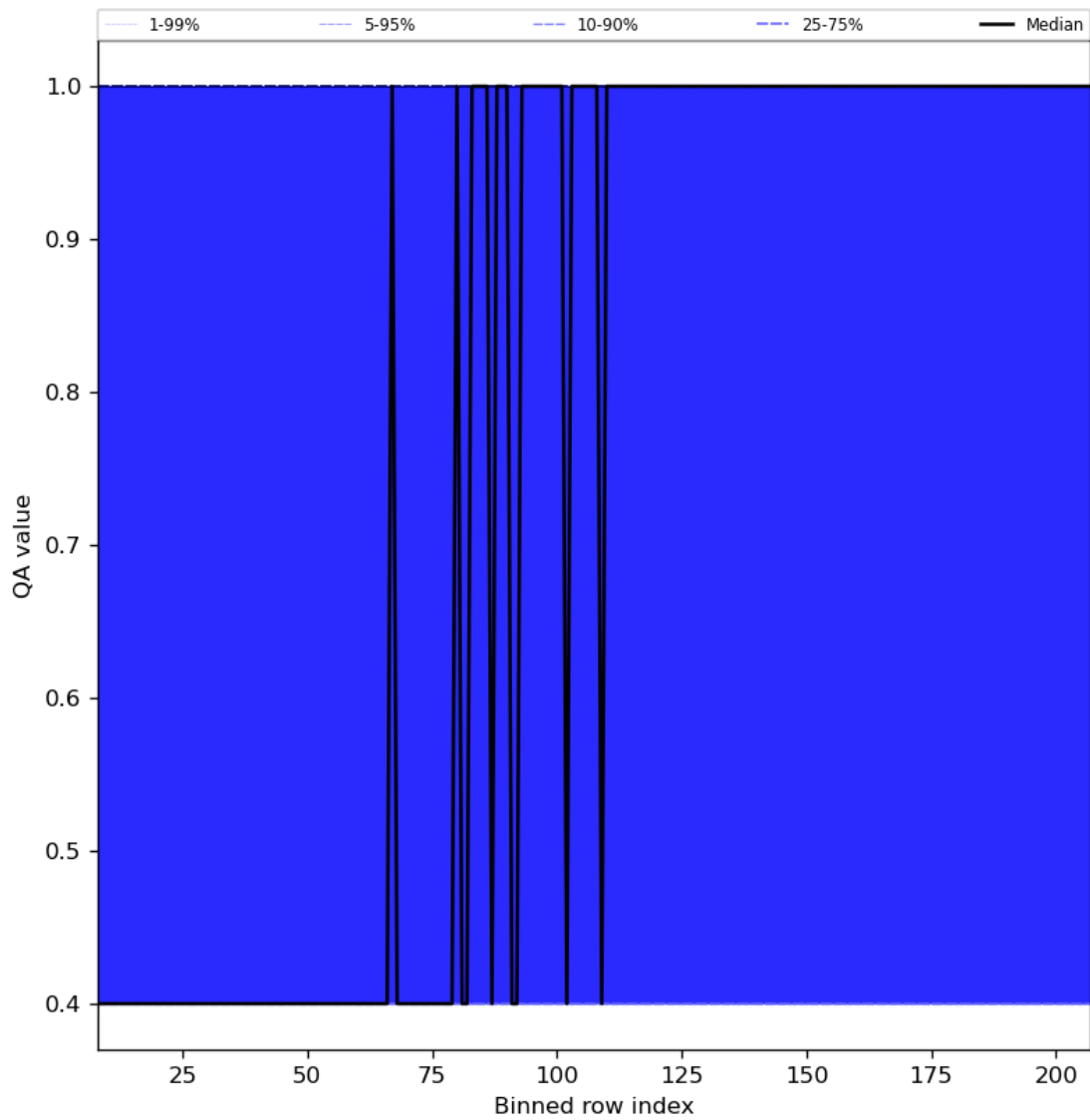
Figure 33: Along track statistics of “QA value” for 2023-07-11 to 2023-07-13
