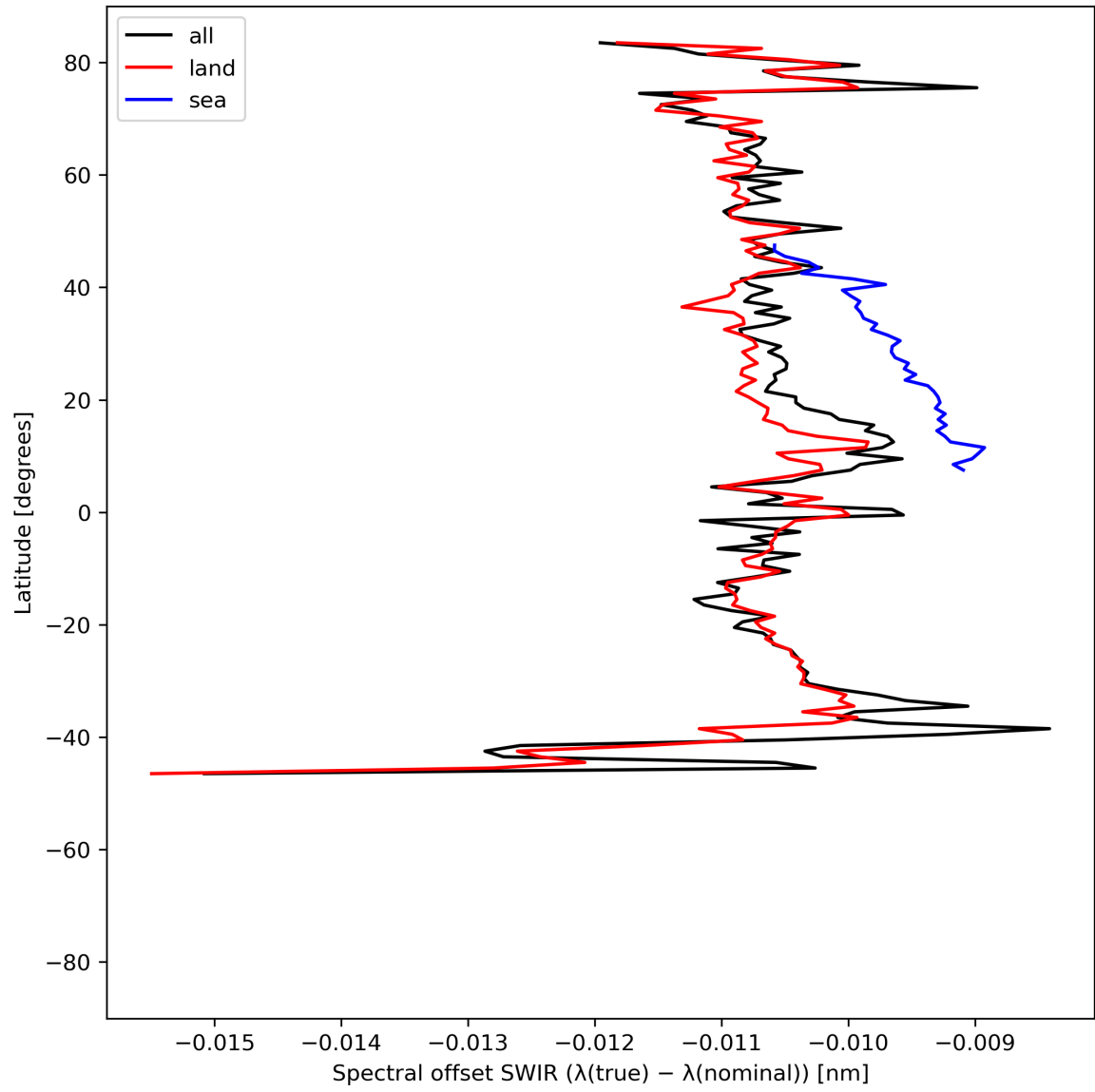
Figure 16: Zonal average of “Spectral offset SWIR ( \lambda(\text{true}) - \lambda(\text{nominal}) )” for 2023-07-11 to 2023-07-13.
