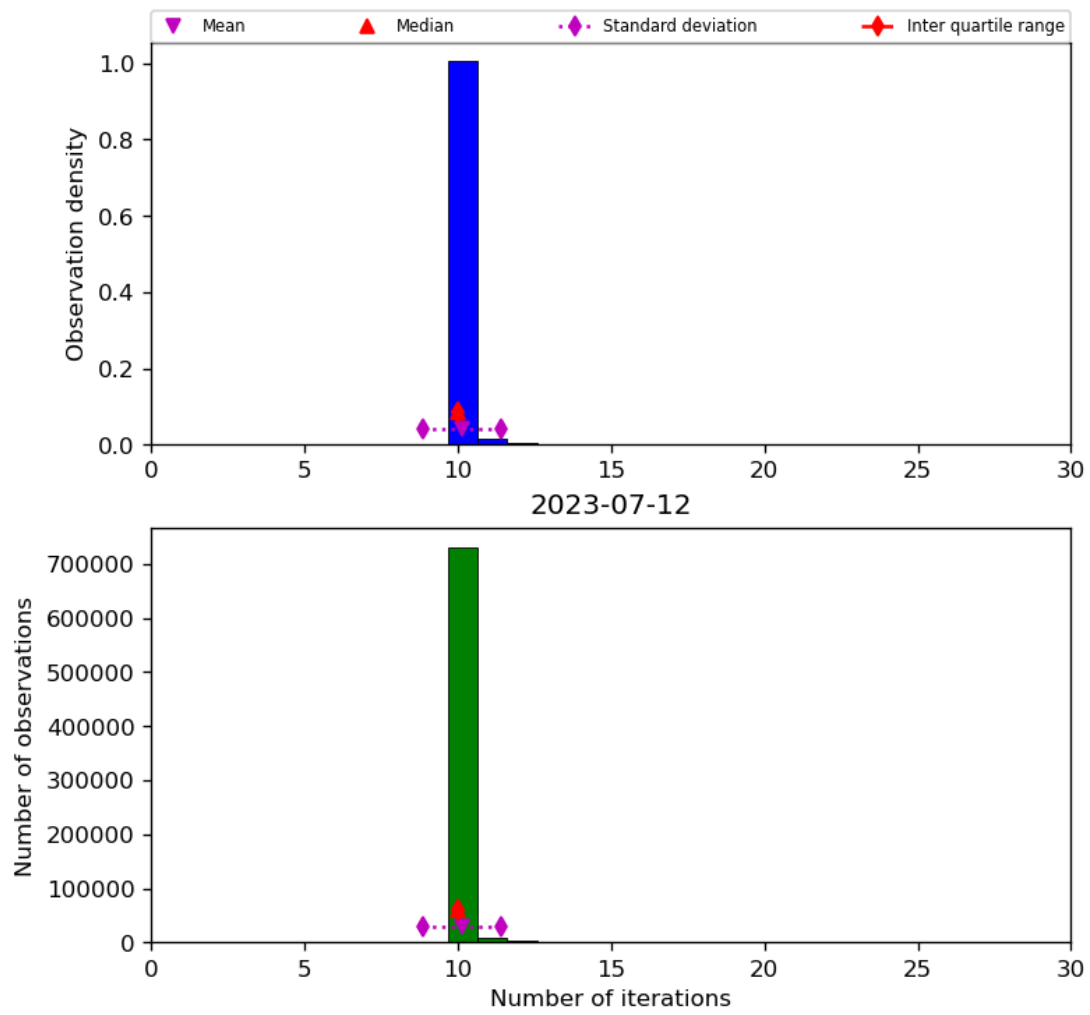
Figure 31: Histogram of “Number of iterations” for 2023-07-11 to 2023-07-13
