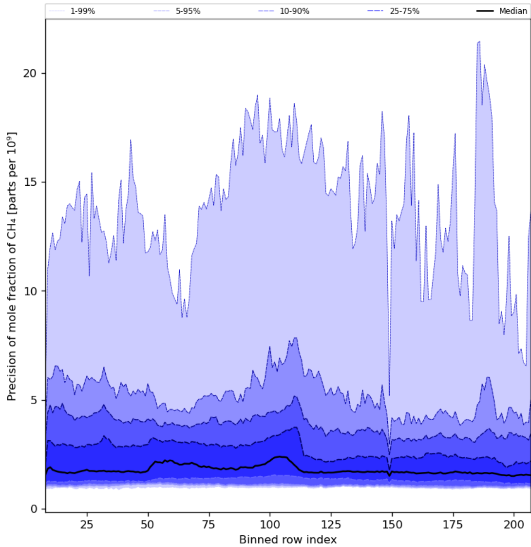
Figure 35: Along track statistics of “Precision of mole fraction of CH 4 ” for 2023-07-11 to 2023-07-13
