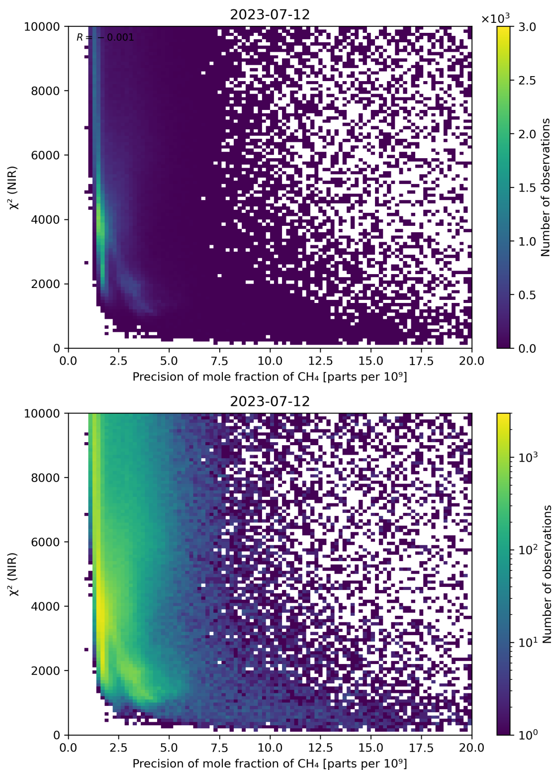
Figure 78: Scatter density plot of “Precision of mole fraction of \text{CH}_4 ” against “ \chi^2 (NIR)” for 2023-07-11 to 2023-07-13.
