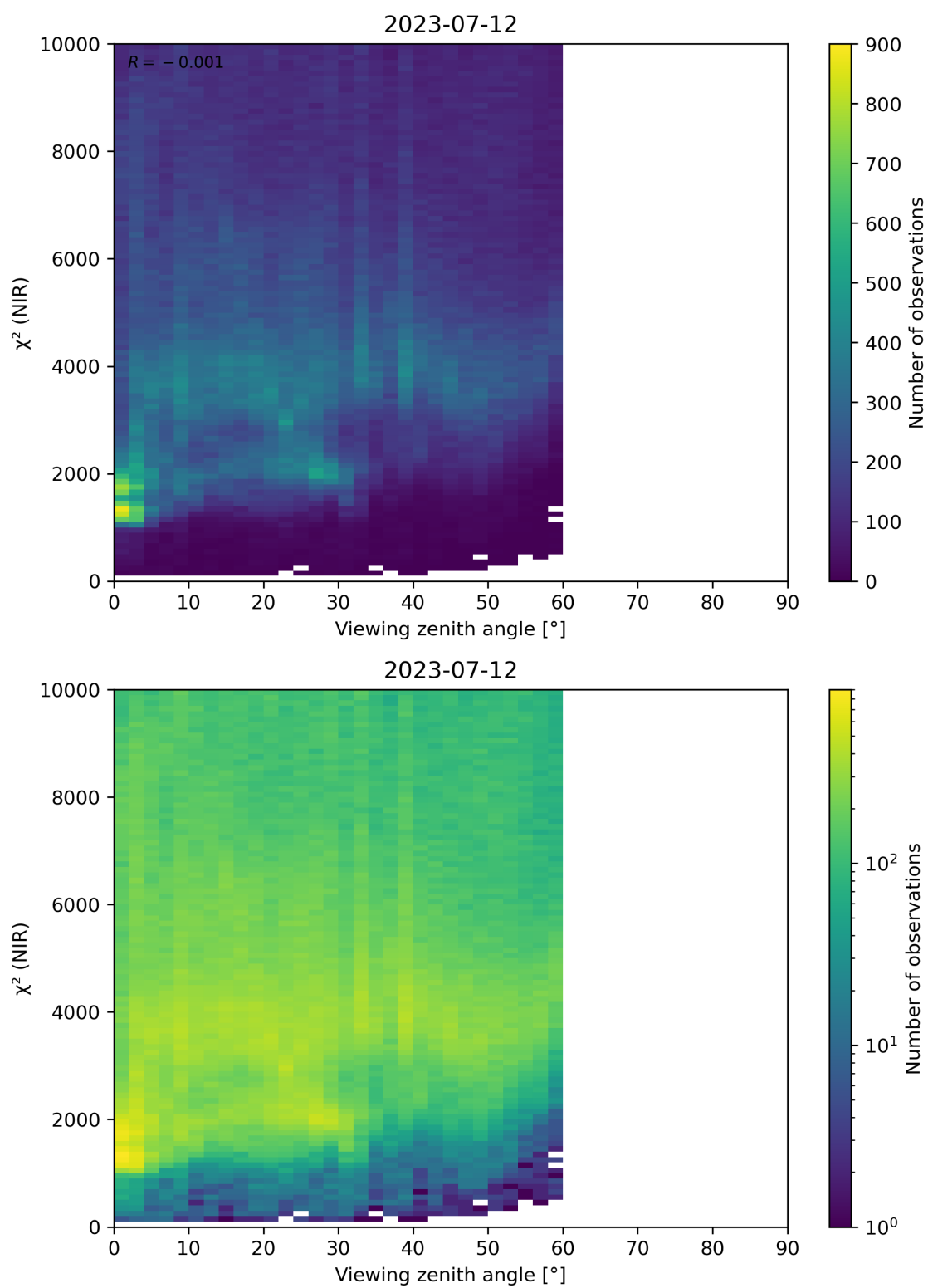
Figure 105: Scatter density plot of “Viewing zenith angle” against “ \chi^2 (NIR)” for 2023-07-11 to 2023-07-13.
