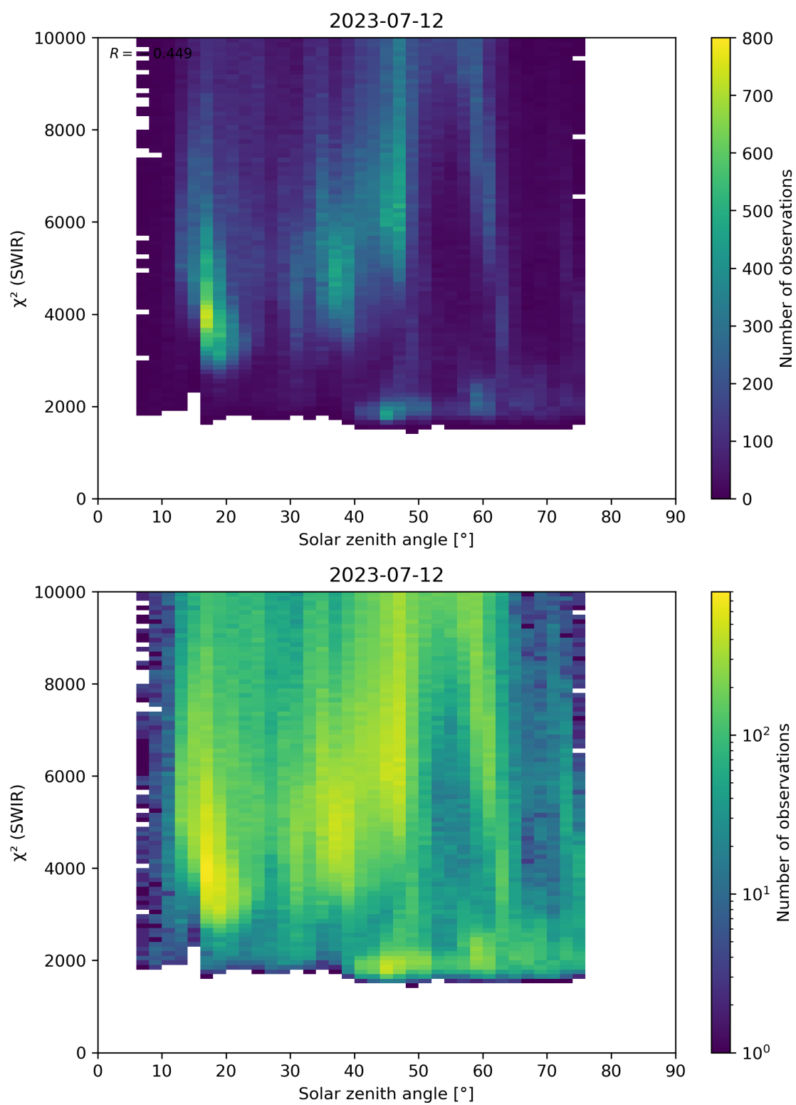
Figure 95: Scatter density plot of “Solar zenith angle” against “ \chi^2 (SWIR)” for 2023-07-11 to 2023-07-13.
