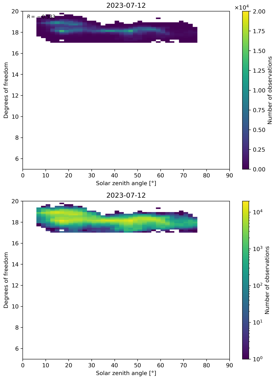
Figure 96: Scatter density plot of “Solar zenith angle” against “Degrees of freedom” for 2023-07-11 to 2023-07-13.
