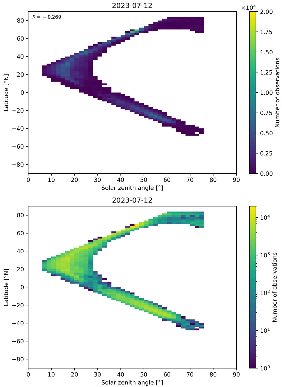
Figure 98: Scatter density plot of “Solar zenith angle” against “Latitude” for 2023-07-11 to 2023-07-13.
