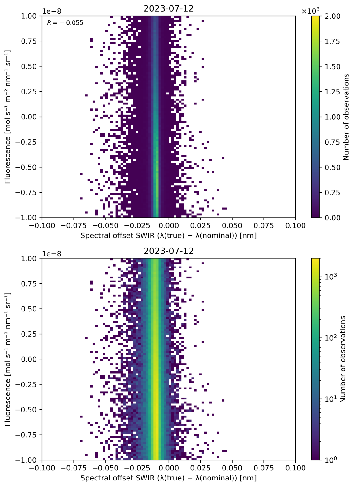
Figure 120: Scatter density plot of “Spectral offset SWIR ( \lambda(\text{true}) - \lambda(\text{nominal}) )” against “Fluorescence” for 2023-07-11 to 2023-07-13.
