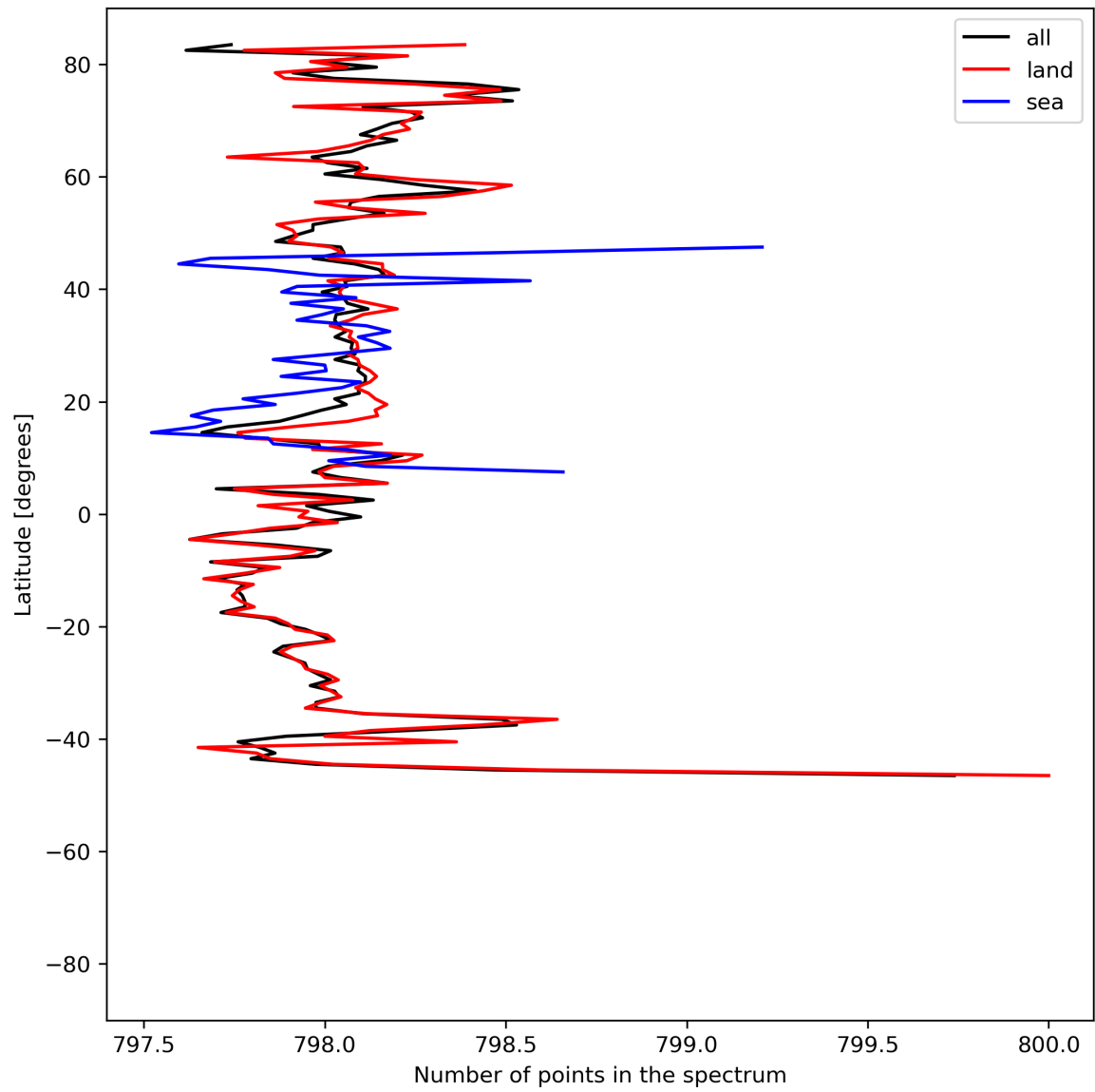
Figure 15: Zonal average of “Number of points in the spectrum” for 2023-07-11 to 2023-07-13.
