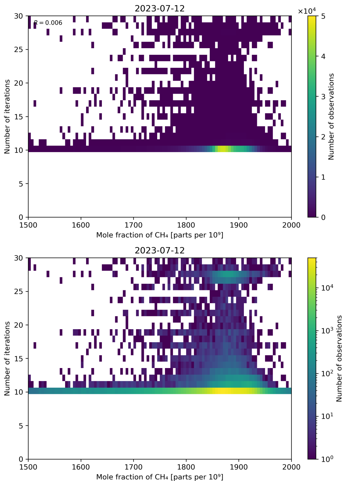
Figure 76: Scatter density plot of “Mole fraction of CH 4 ” against “Number of iterations” for 2023-07-11 to 2023-07-13.
