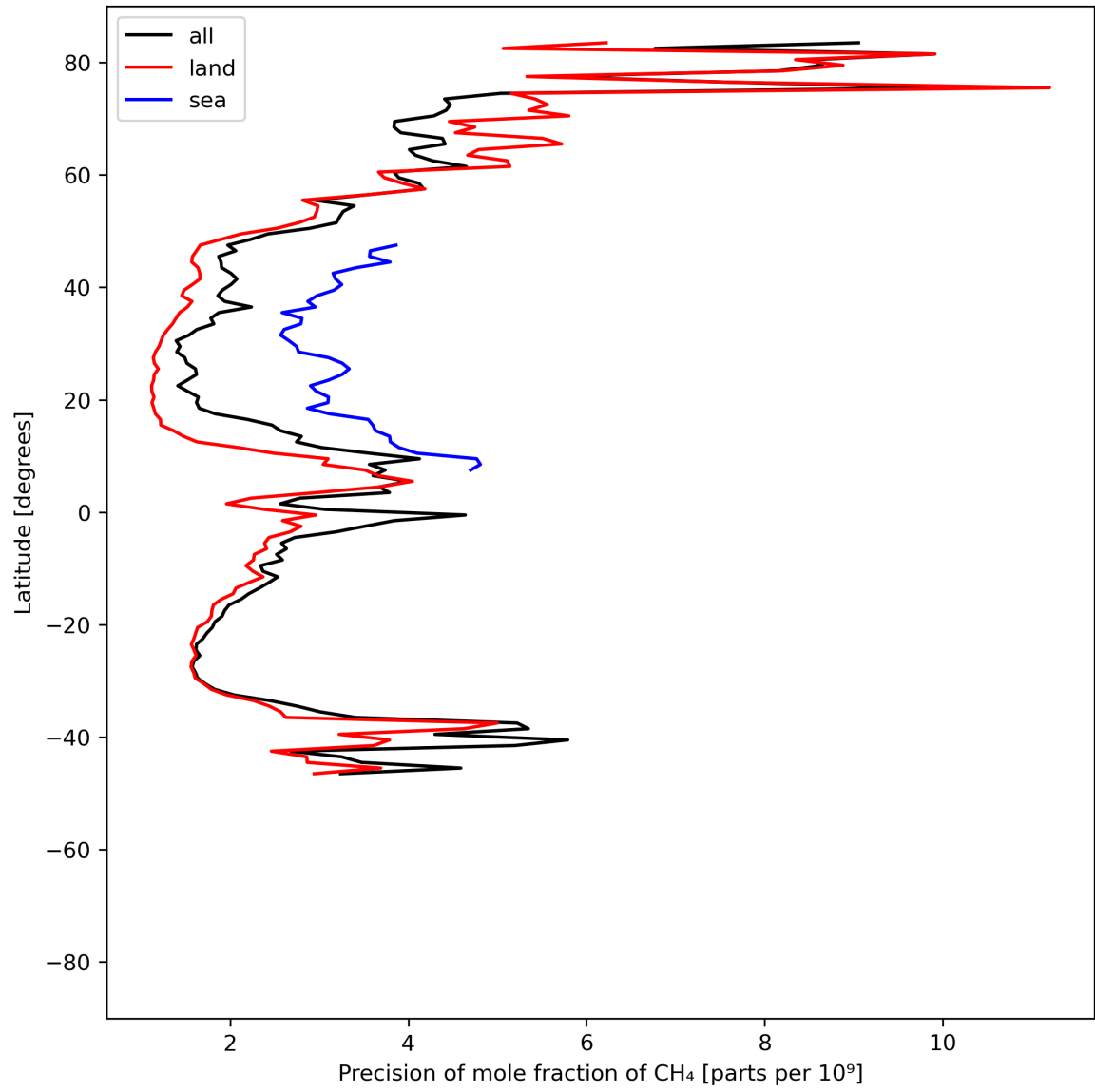
Figure 13: Zonal average of “Precision of mole fraction of CH 4 ” for 2023-07-11 to 2023-07-13.
