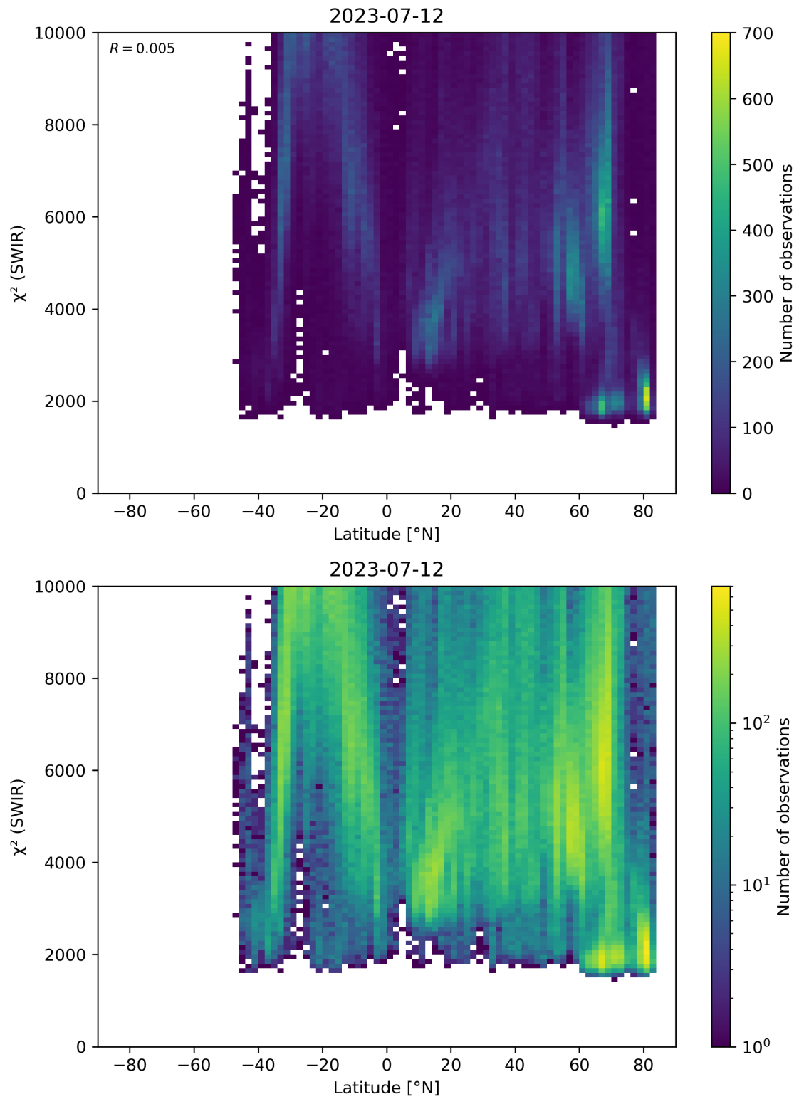
Figure 54: Scatter density plot of “Latitude” against “ \chi^2 (SWIR)” for 2023-07-11 to 2023-07-13.
