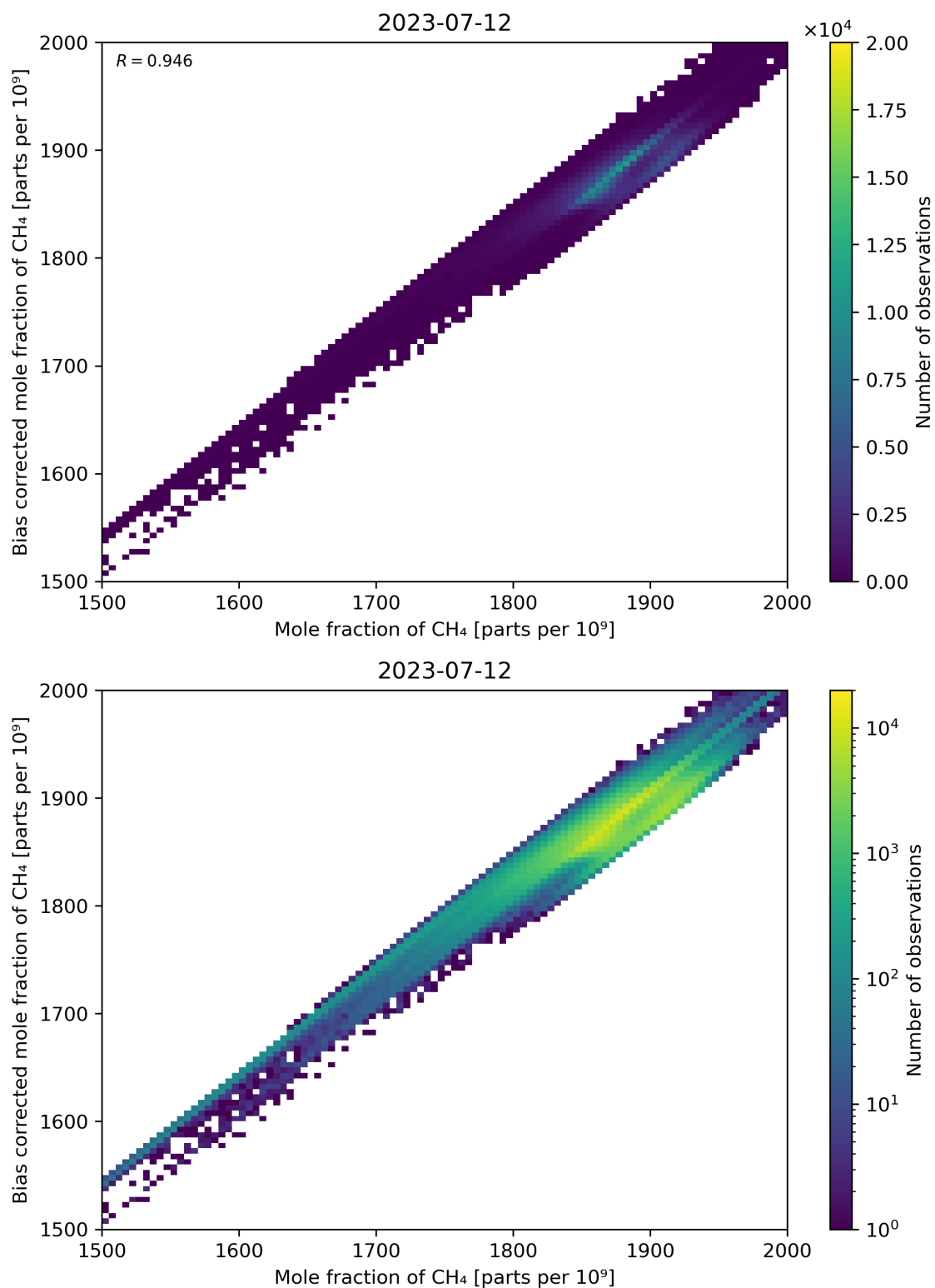
Figure 74: Scatter density plot of “Mole fraction of CH 4 ” against “Bias corrected mole fraction of CH 4 ” for 2023-07-11 to 2023-07-13.
