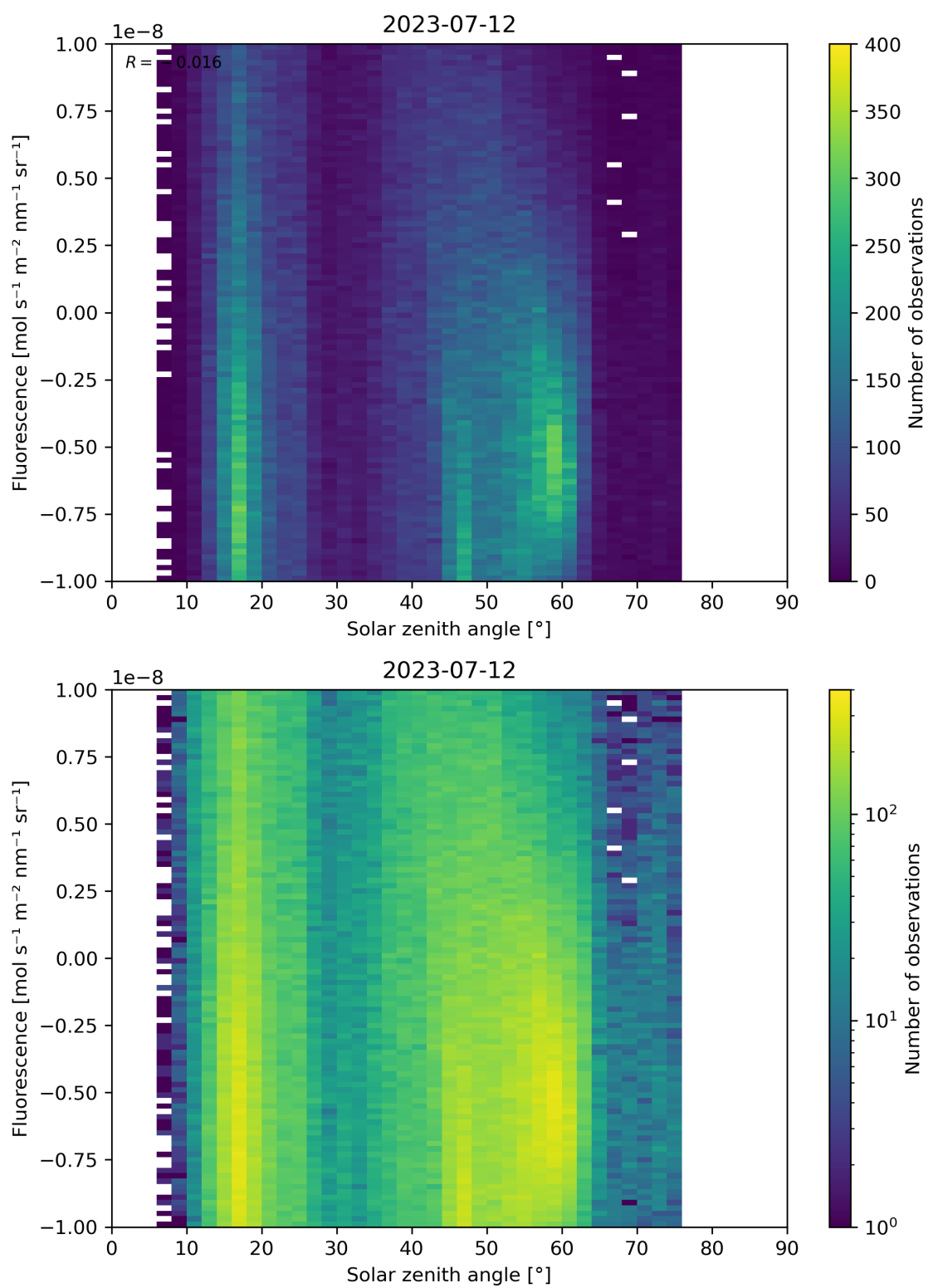
Figure 97: Scatter density plot of “Solar zenith angle” against “Fluorescence” for 2023-07-11 to 2023-07-13.
