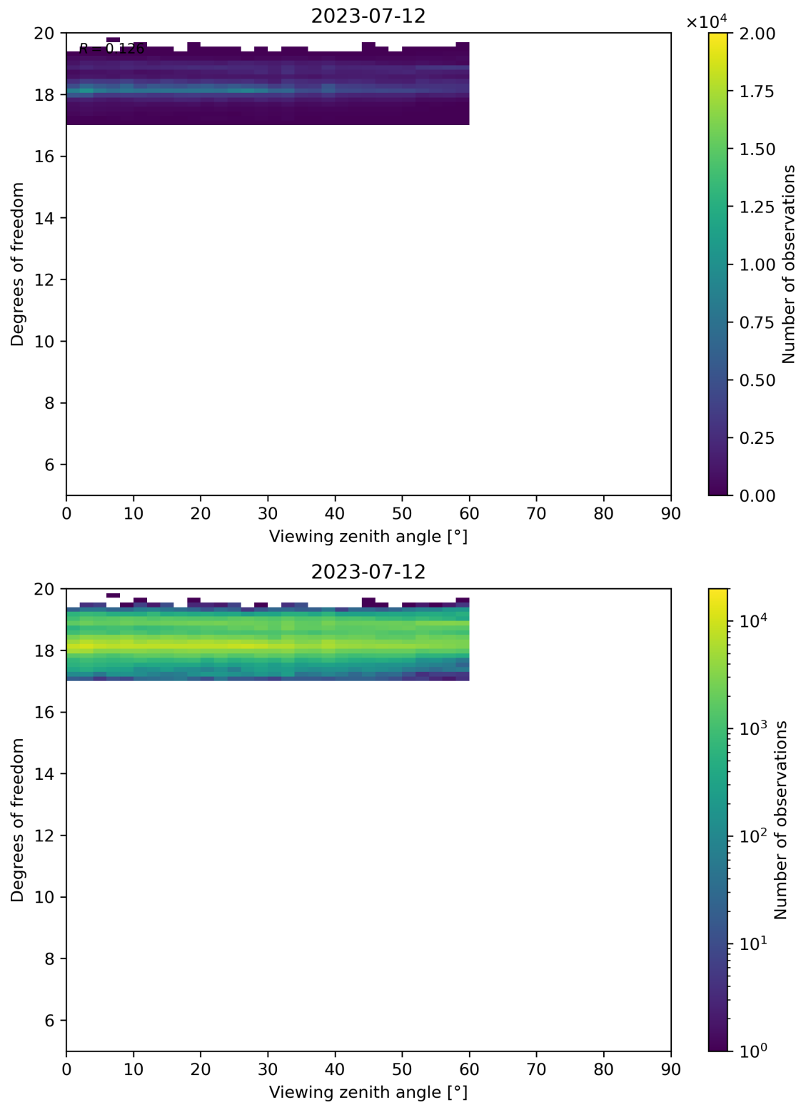
Figure 107: Scatter density plot of “Viewing zenith angle” against “Degrees of freedom” for 2023-07-11 to 2023-07-13.
