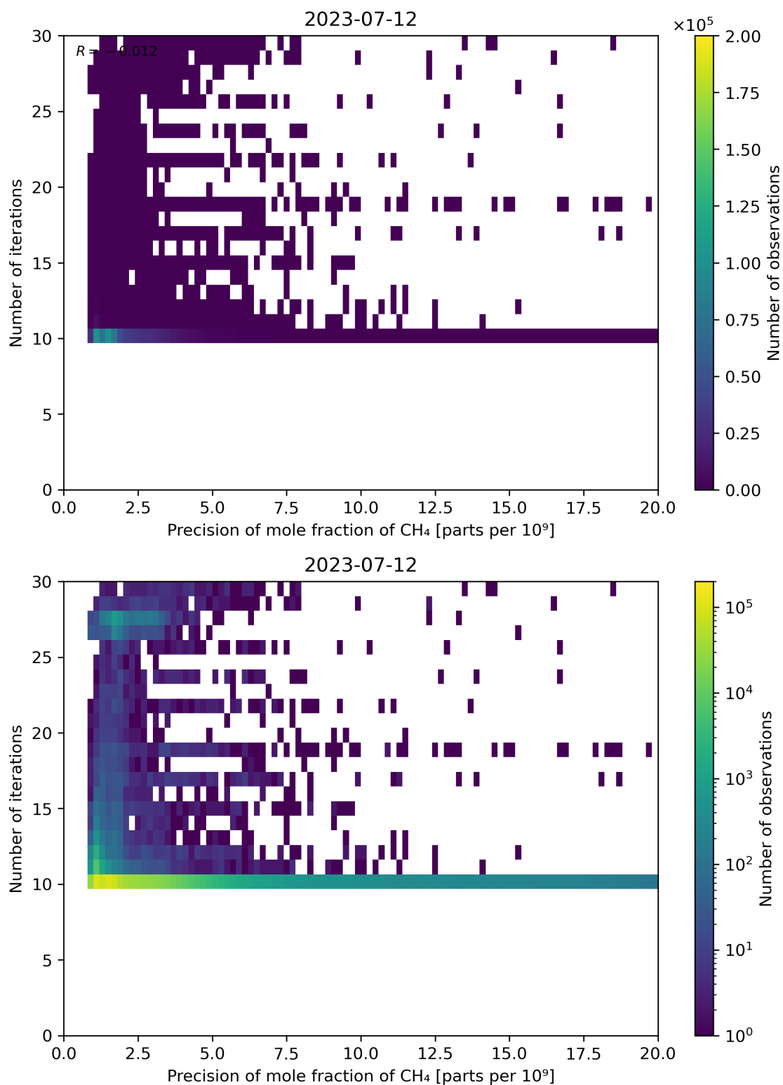
Figure 83: Scatter density plot of “Precision of mole fraction of CH 4 ” against “Number of iterations” for 2023-07-11 to 2023-07-13.
