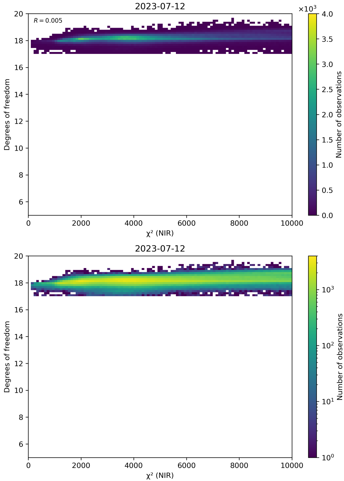
Figure 44: Scatter density plot of “ \chi^2 (NIR)” against “Degrees of freedom” for 2023-07-11 to 2023-07-13.
