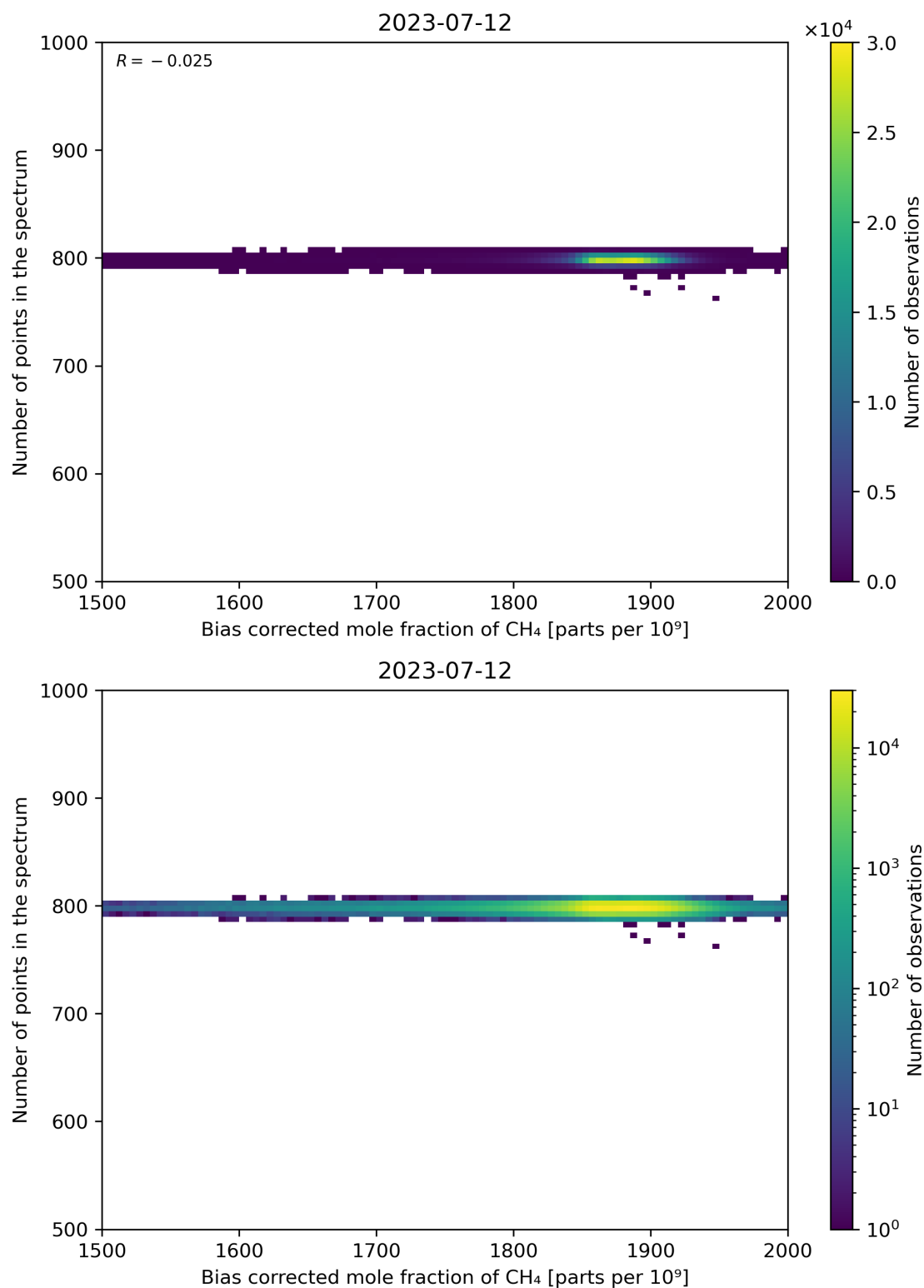
Figure 68: Scatter density plot of “Bias corrected mole fraction of CH 4 ” against “Number of points in the spectrum” for 2023-07-11 to 2023-07-13.
