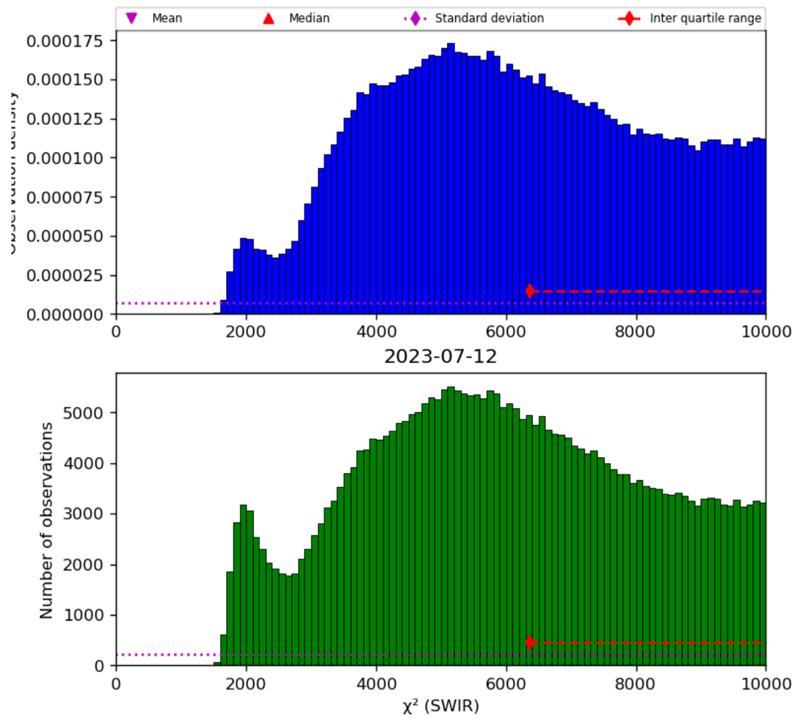
Figure 28: Histogram of “ \chi^2 (SWIR)” for 2023-07-11 to 2023-07-13
