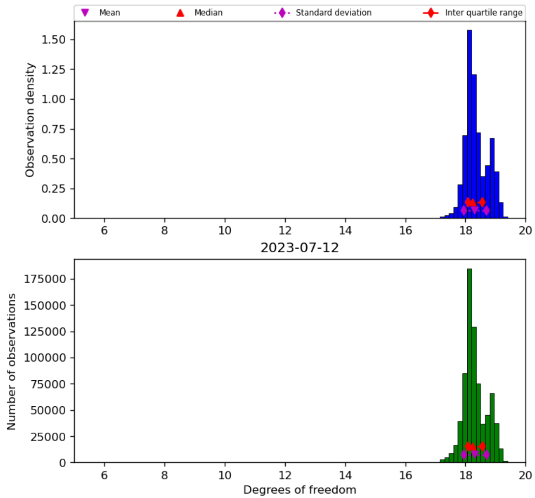
Figure 30: Histogram of “Degrees of freedom” for 2023-07-11 to 2023-07-13
