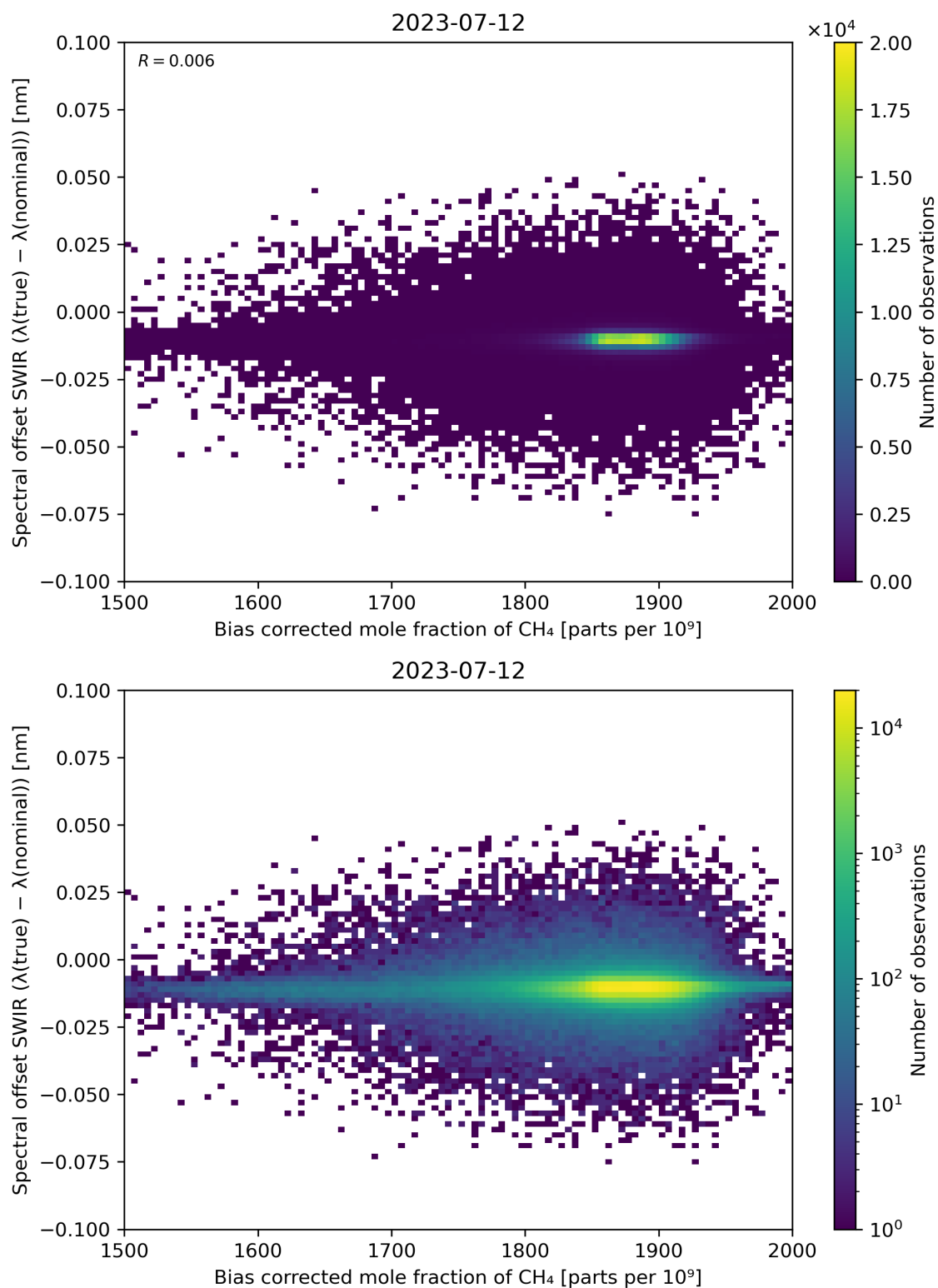
Figure 69: Scatter density plot of “Bias corrected mole fraction of \text{CH}_4 ” against “Spectral offset SWIR ( \lambda(\text{true}) - \lambda(\text{nominal}) )” for 2023-07-11 to 2023-07-13.
