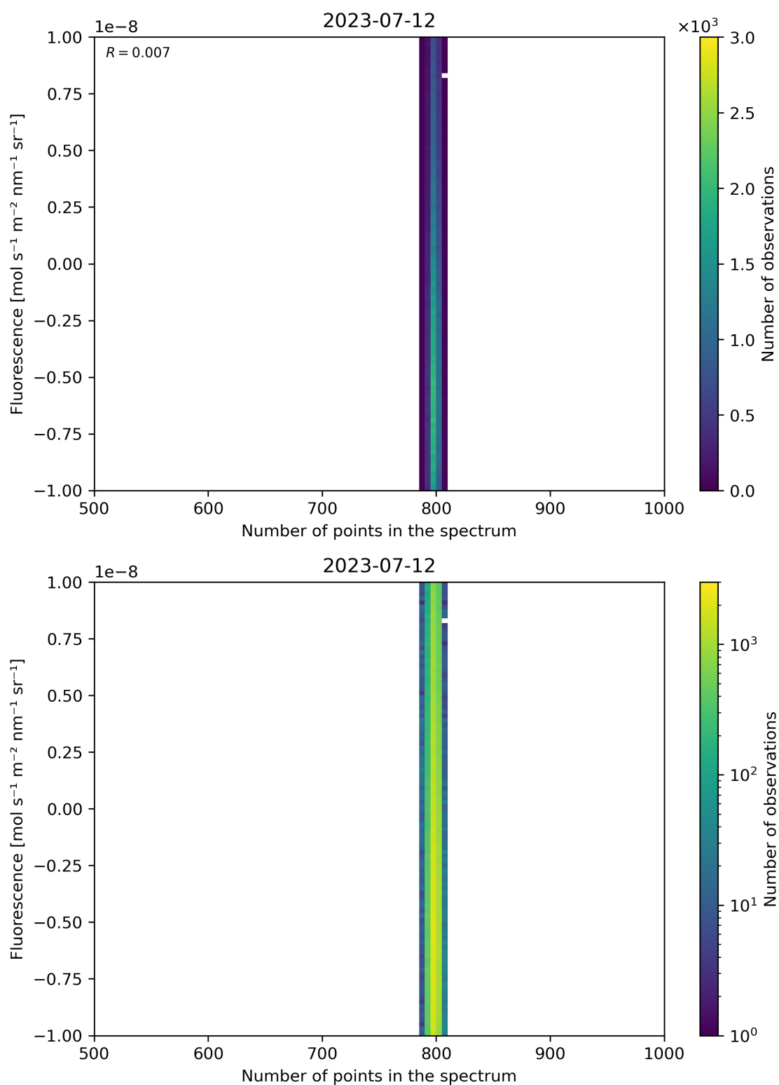
Figure 91: Scatter density plot of “Number of points in the spectrum” against “Fluorescence” for 2023-07-11 to 2023-07-13.
