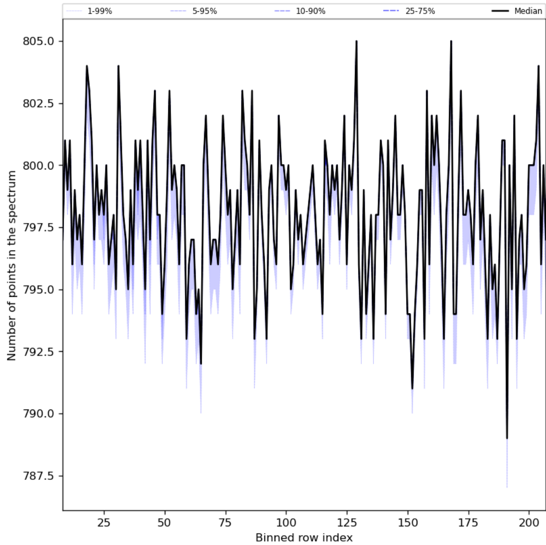
Figure 37: Along track statistics of “Number of points in the spectrum” for 2023-07-11 to 2023-07-13
