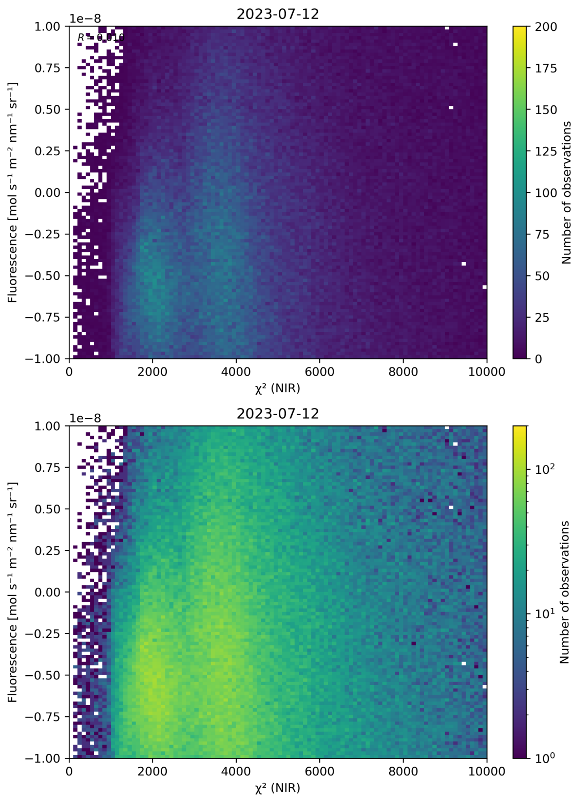
Figure 45: Scatter density plot of “ \chi^2 (NIR)” against “Fluorescence” for 2023-07-11 to 2023-07-13.
