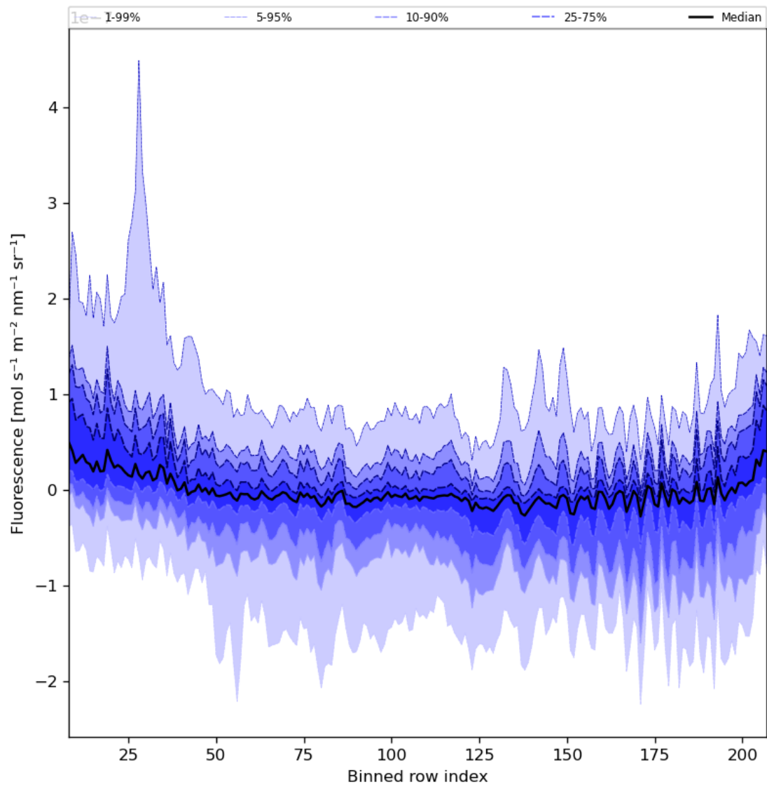
Figure 43: Along track statistics of “Fluorescence” for 2023-07-11 to 2023-07-13
