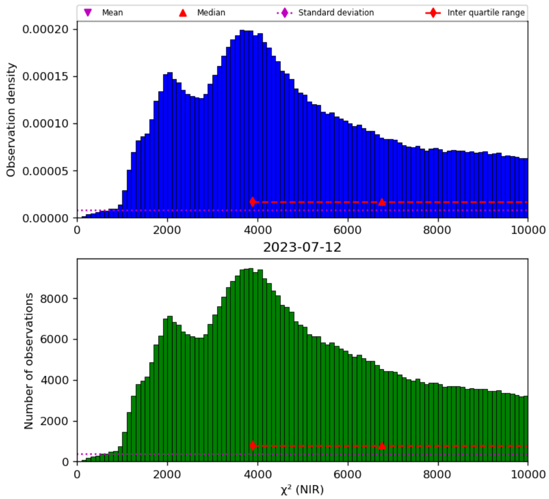
Figure 29: Histogram of “ \chi^2 (NIR)” for 2023-07-11 to 2023-07-13
