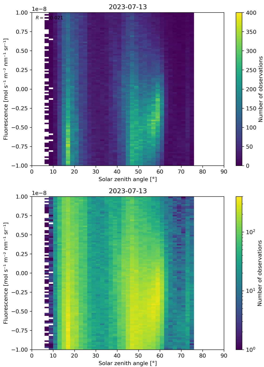
Figure 97: Scatter density plot of “Solar zenith angle” against “Fluorescence” for 2023-07-13 to 2023-07-14.
