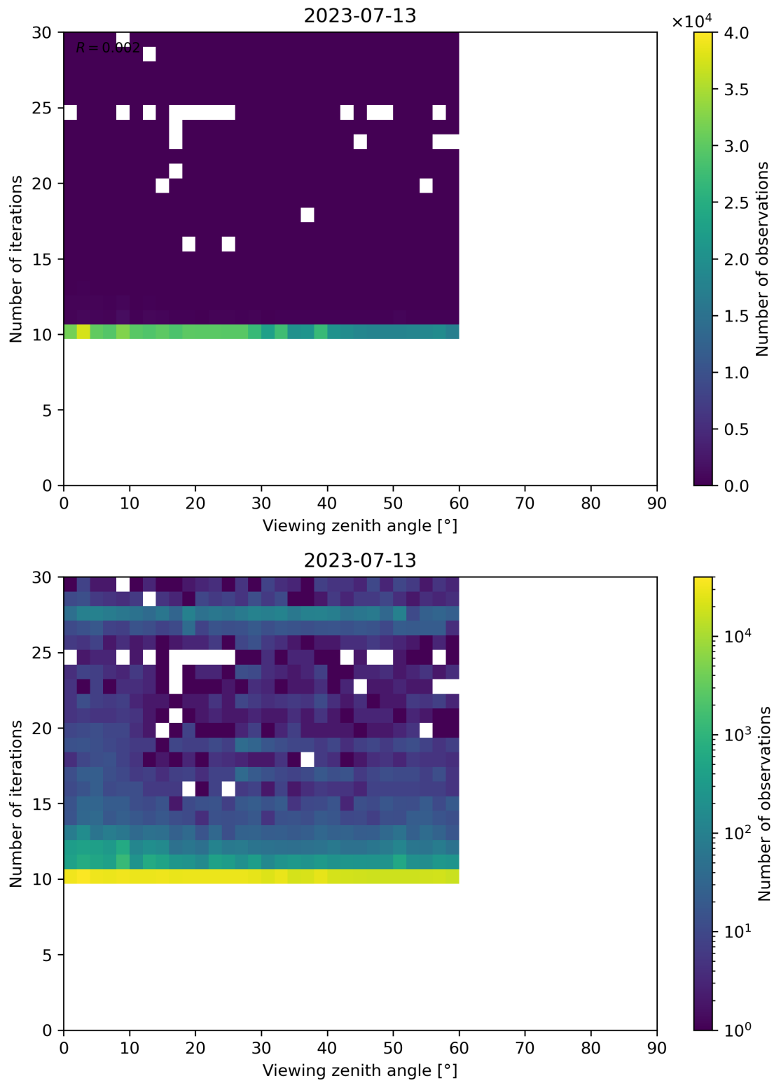
Figure 113: Scatter density plot of “Viewing zenith angle” against “Number of iterations” for 2023-07-13 to 2023-07-14.
