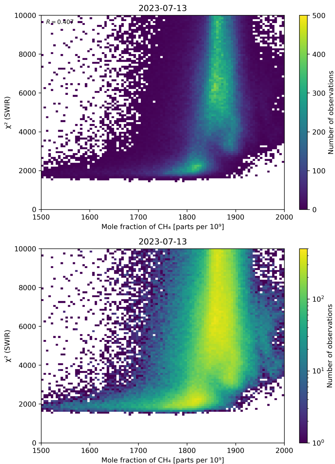
Figure 71: Scatter density plot of “Mole fraction of CH 4 ” against “ \chi^2 (SWIR)” for 2023-07-13 to 2023-07-14.
