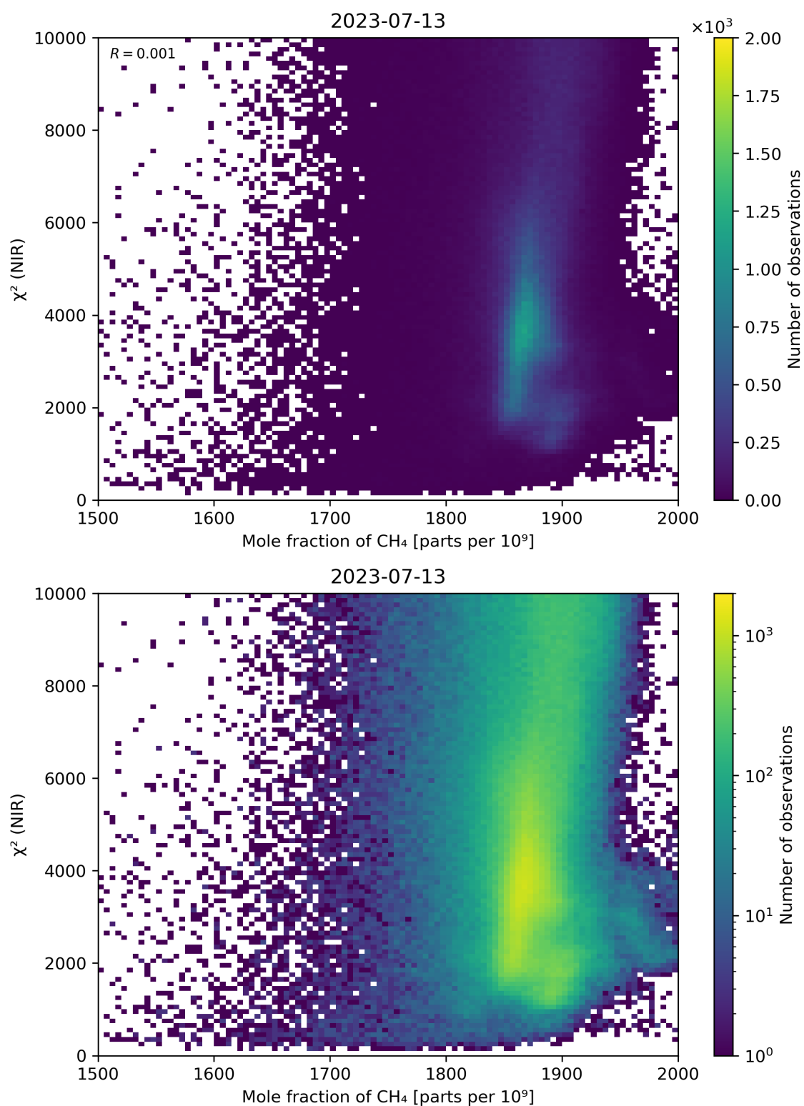
Figure 70: Scatter density plot of “Mole fraction of \text{CH}_4 ” against “ \chi^2 (NIR)” for 2023-07-13 to 2023-07-14.
