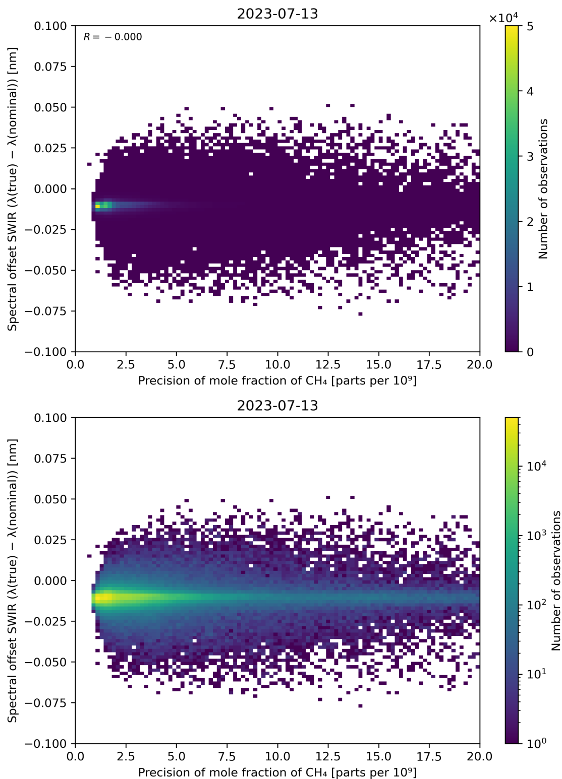
Figure 85: Scatter density plot of “Precision of mole fraction of CH 4 ” against “Spectral offset SWIR ( \lambda(\text{true}) - \lambda(\text{nominal}) )” for 2023-07-13 to 2023-07-14.
