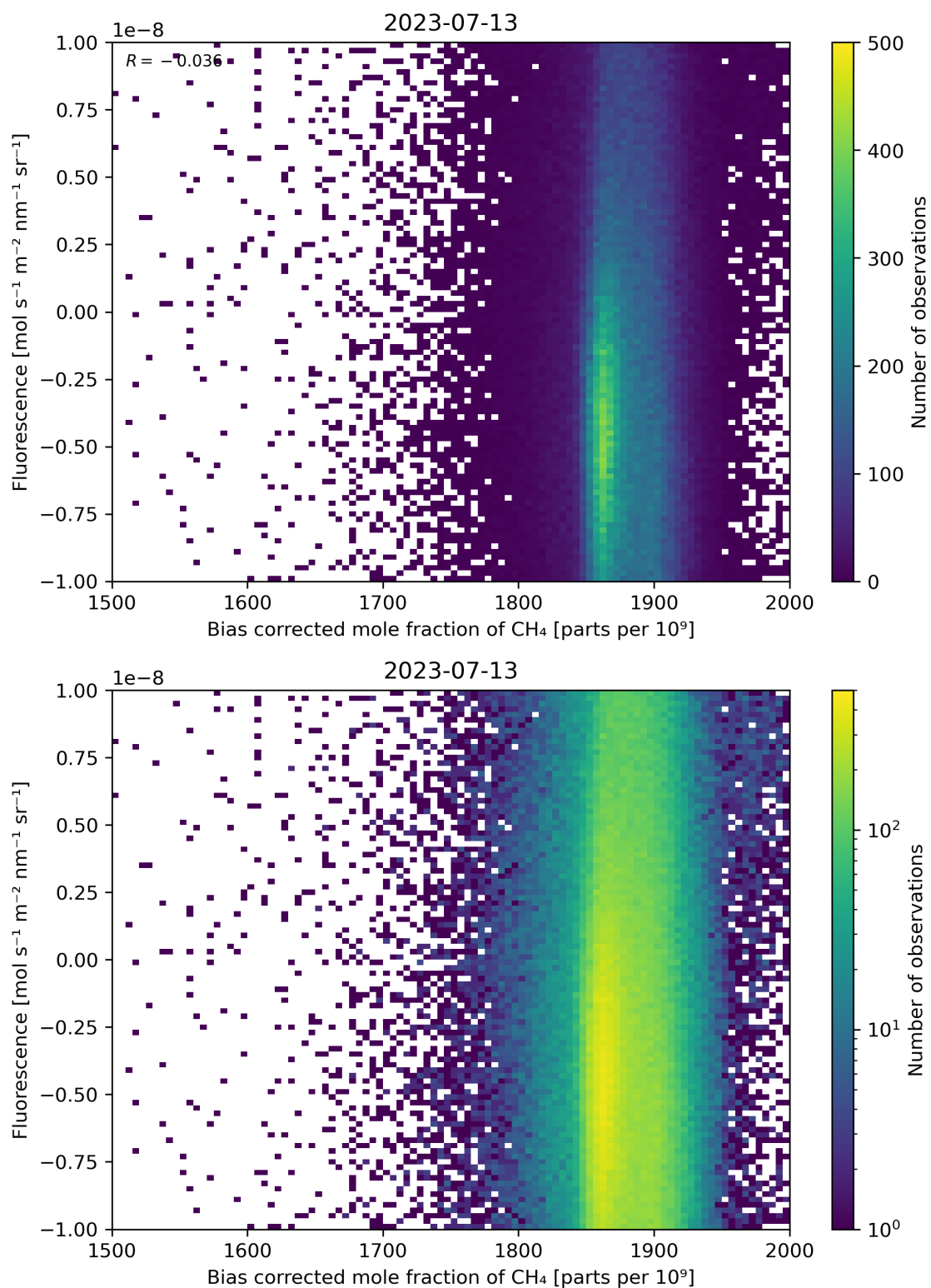
Figure 66: Scatter density plot of “Bias corrected mole fraction of \text{CH}_4 ” against “Fluorescence” for 2023-07-13 to 2023-07-14.
