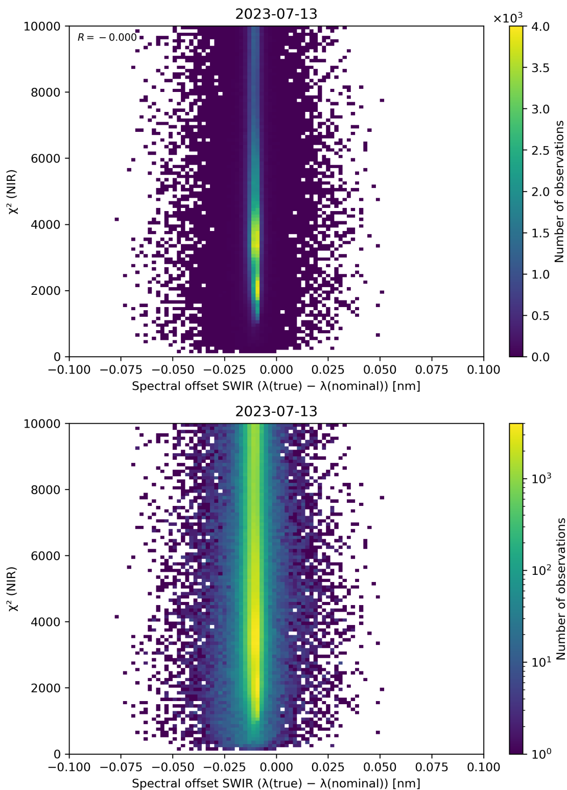
Figure 117: Scatter density plot of “Spectral offset SWIR ( \lambda(\text{true}) - \lambda(\text{nominal}) )” against “ \chi^2 (NIR)” for 2023-07-13 to 2023-07-14.
