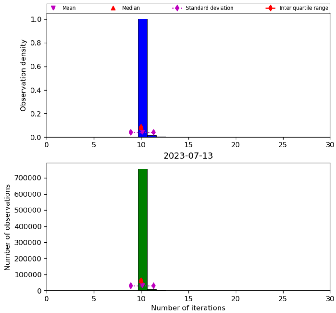
Figure 31: Histogram of “Number of iterations” for 2023-07-13 to 2023-07-14
