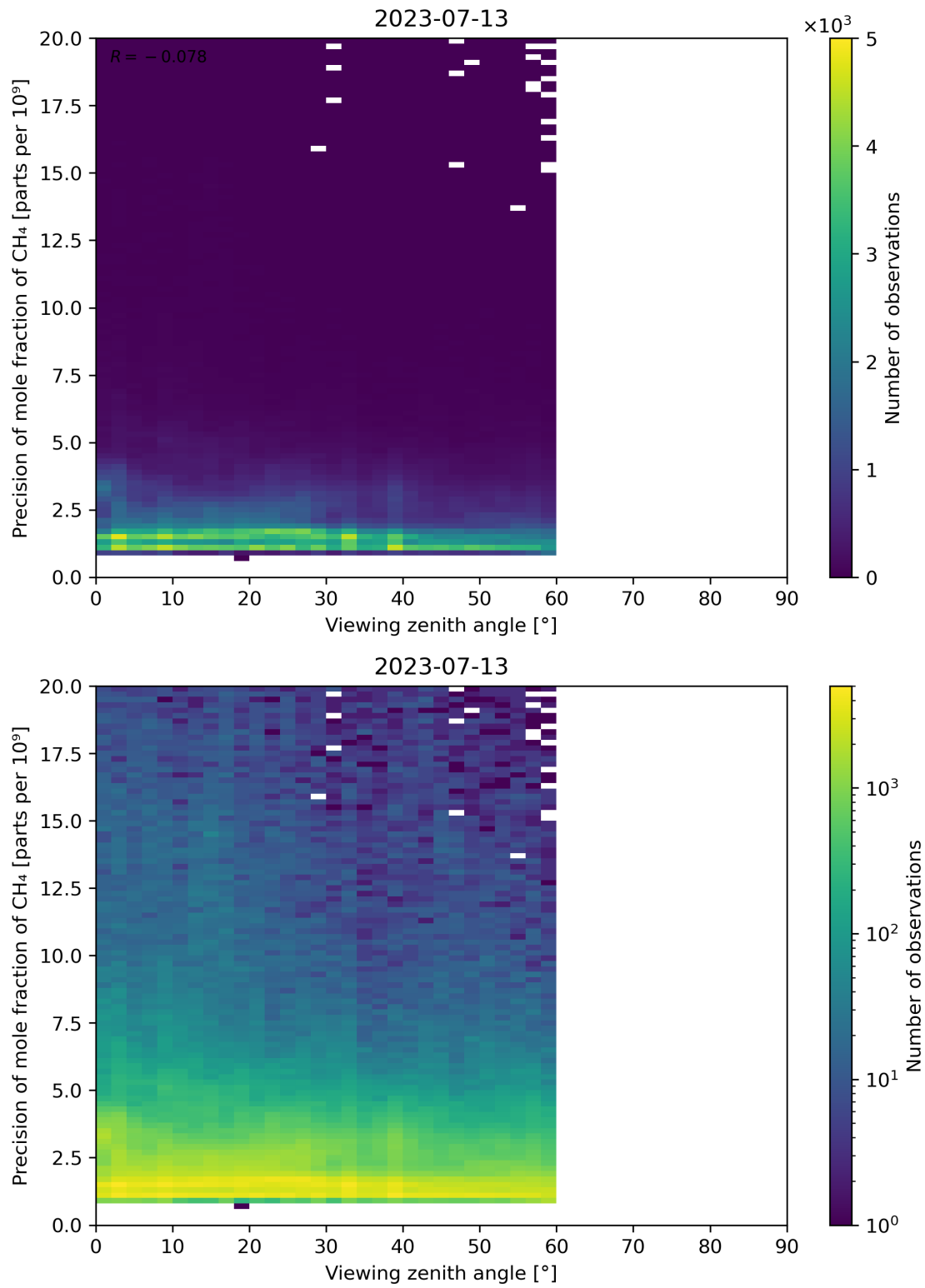
Figure 112: Scatter density plot of “Viewing zenith angle” against “Precision of mole fraction of CH 4 ” for 2023-07-13 to 2023-07-14.
