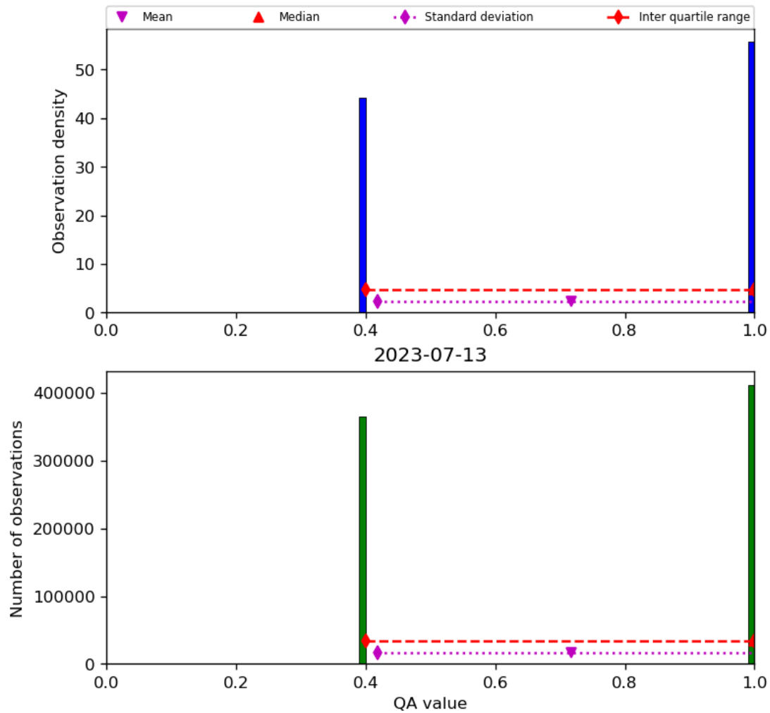
Figure 22: Histogram of “QA value” for 2023-07-13 to 2023-07-14
