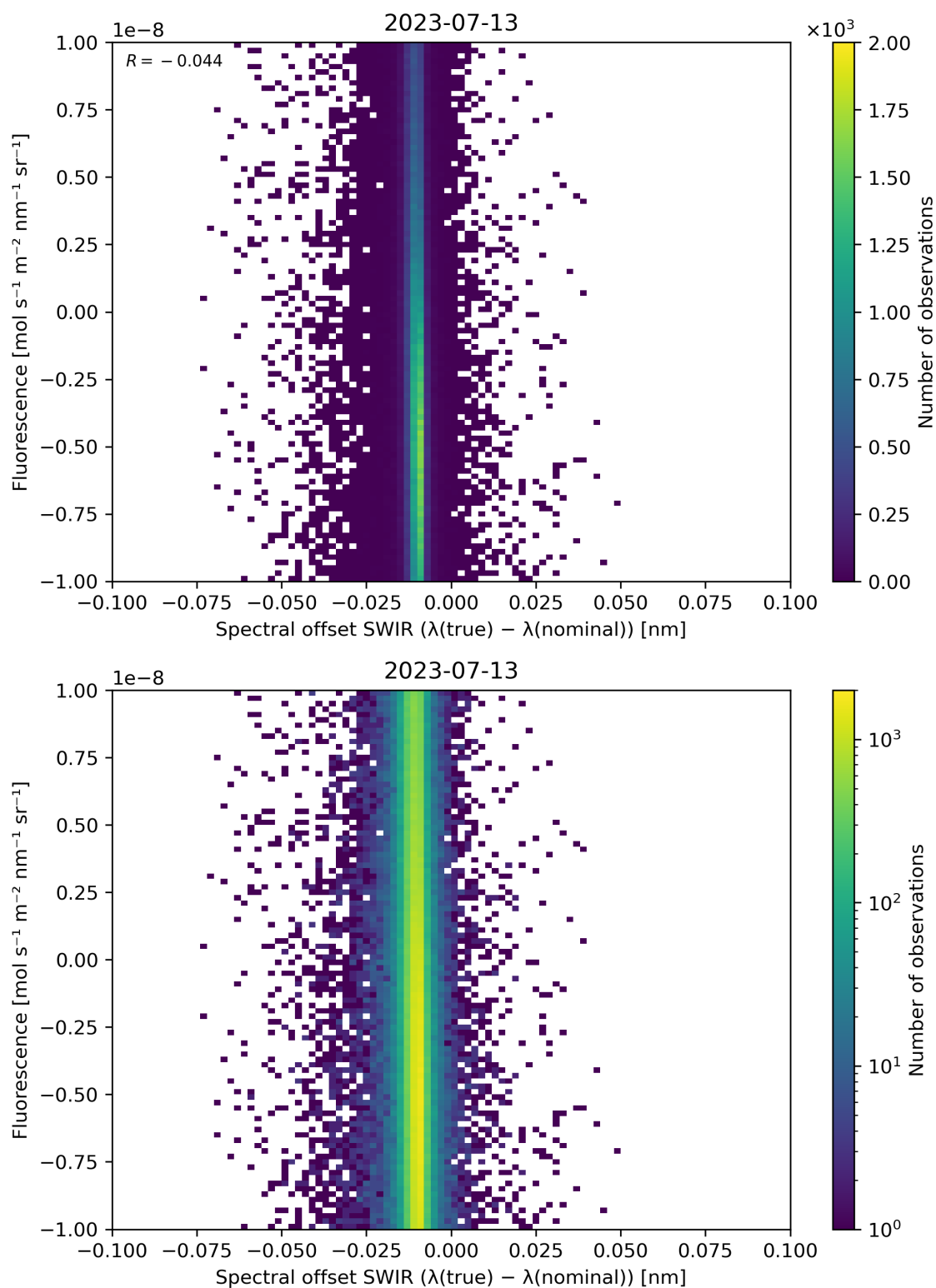
Figure 120: Scatter density plot of “Spectral offset SWIR ( \lambda(\text{true}) - \lambda(\text{nominal}) )” against “Fluorescence” for 2023-07-13 to 2023-07-14.
