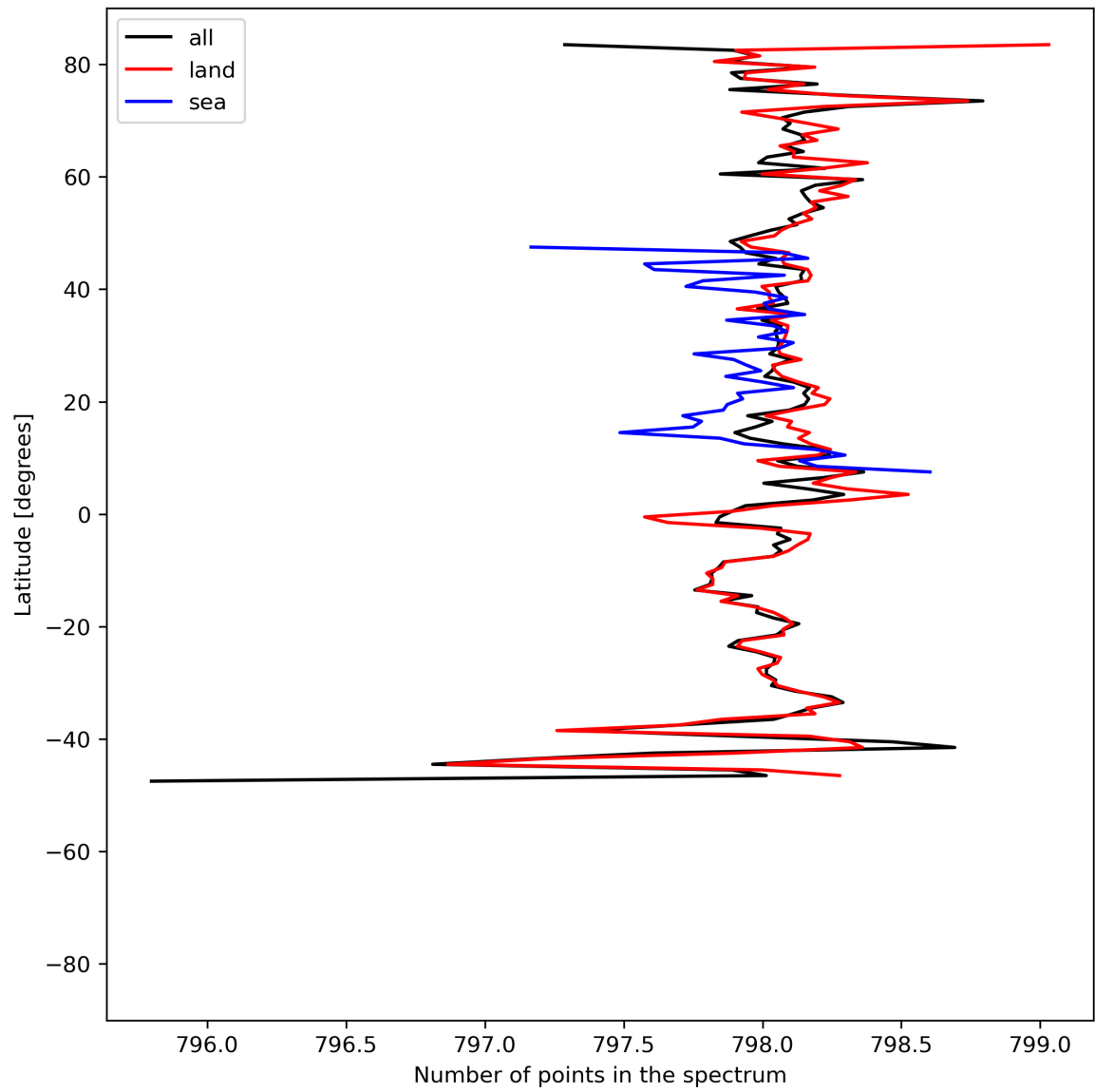
Figure 15: Zonal average of “Number of points in the spectrum” for 2023-07-13 to 2023-07-14.
