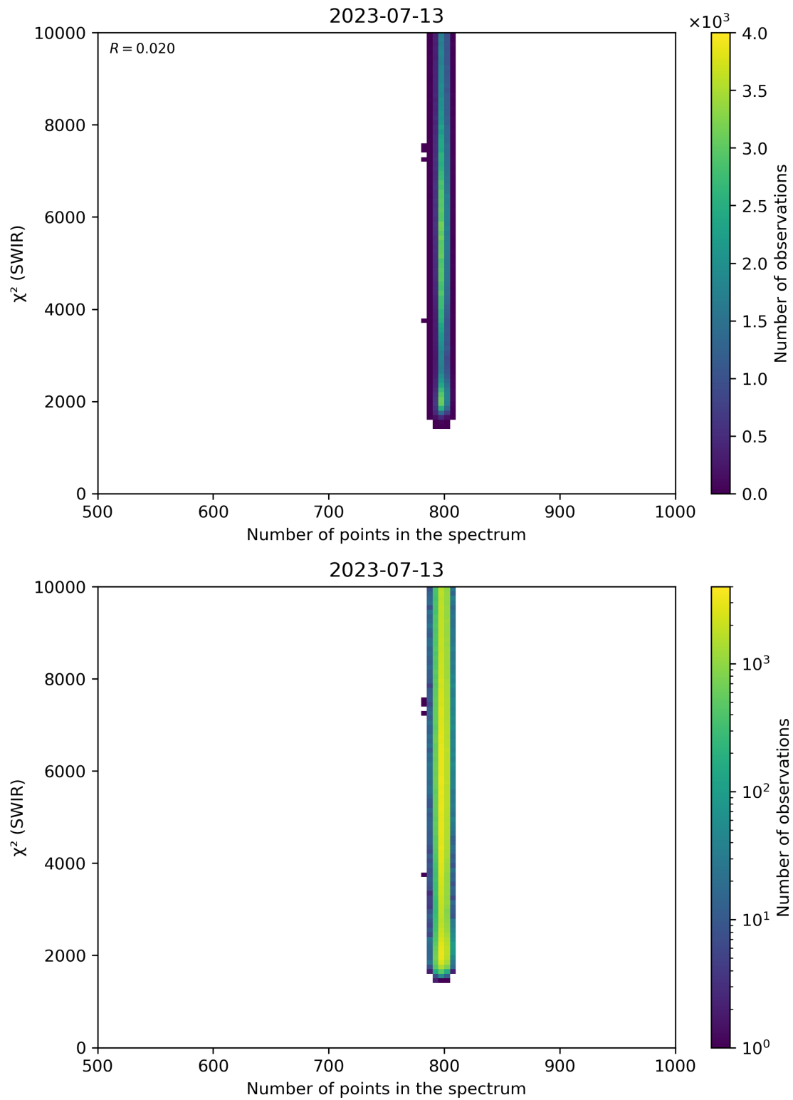
Figure 89: Scatter density plot of “Number of points in the spectrum” against “ \chi^2 (SWIR)” for 2023-07-13 to 2023-07-14.
