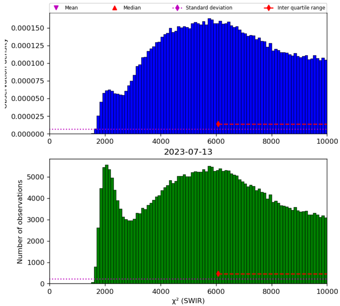
Figure 28: Histogram of “ \chi^2 (SWIR)” for 2023-07-13 to 2023-07-14
