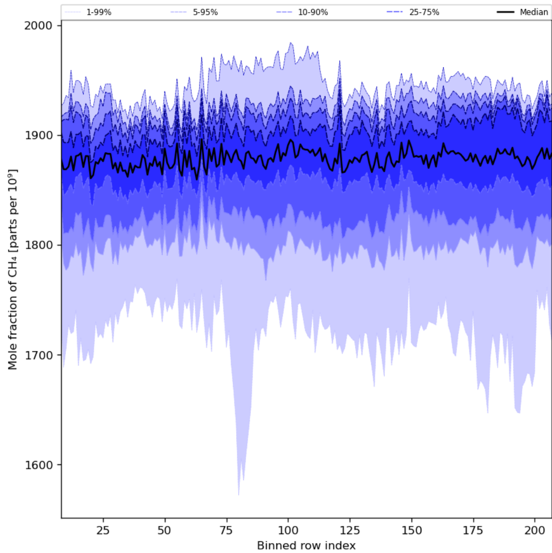
Figure 34: Along track statistics of “Mole fraction of CH 4 ” for 2023-07-13 to 2023-07-14
