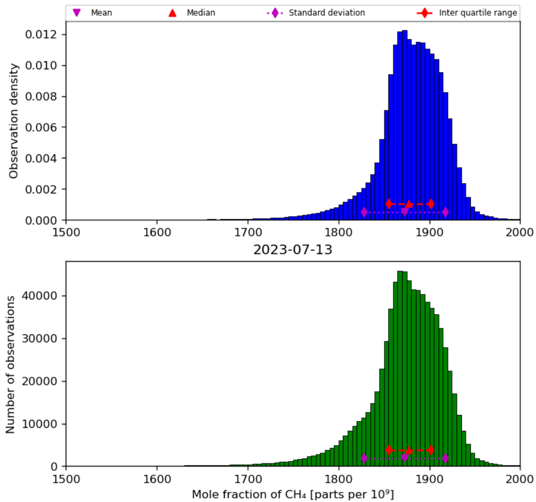
Figure 23: Histogram of “Mole fraction of CH 4 ” for 2023-07-13 to 2023-07-14
