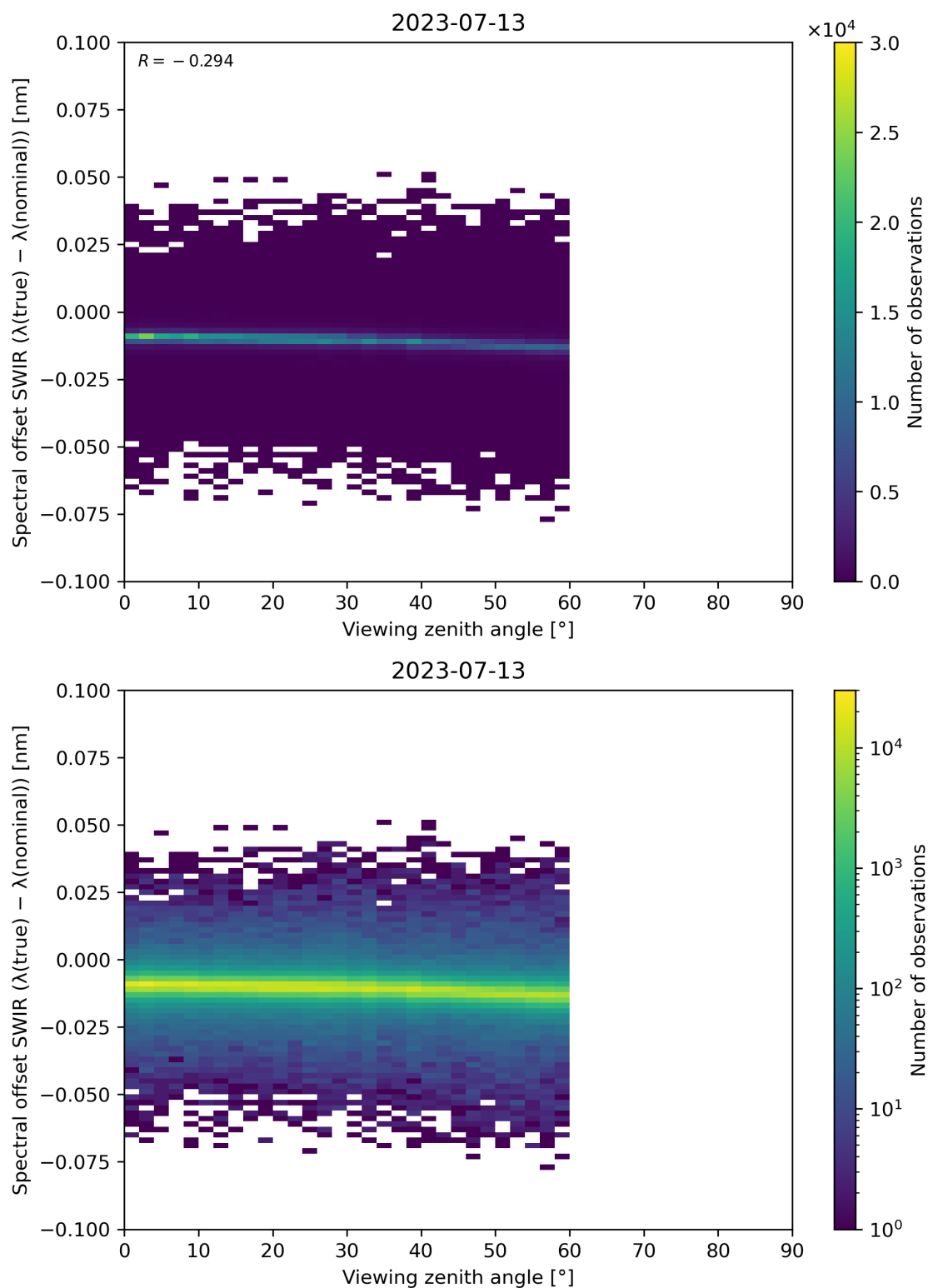
Figure 116: Scatter density plot of “Viewing zenith angle” against “Spectral offset SWIR ( \lambda(\text{true}) - \lambda(\text{nominal}) )” for 2023-07-13 to 2023-07-14.
