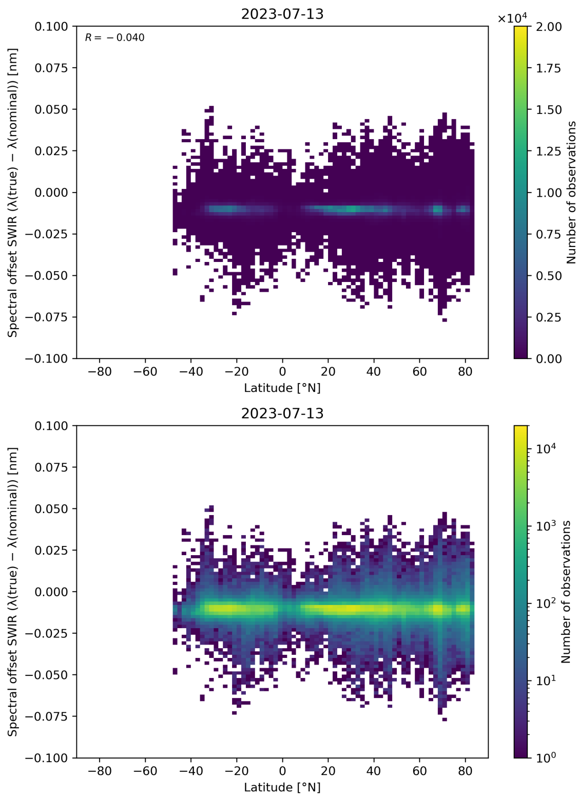
Figure 62: Scatter density plot of “Latitude” against “Spectral offset SWIR ( \lambda(\text{true}) - \lambda(\text{nominal}) )” for 2023-07-13 to 2023-07-14.
