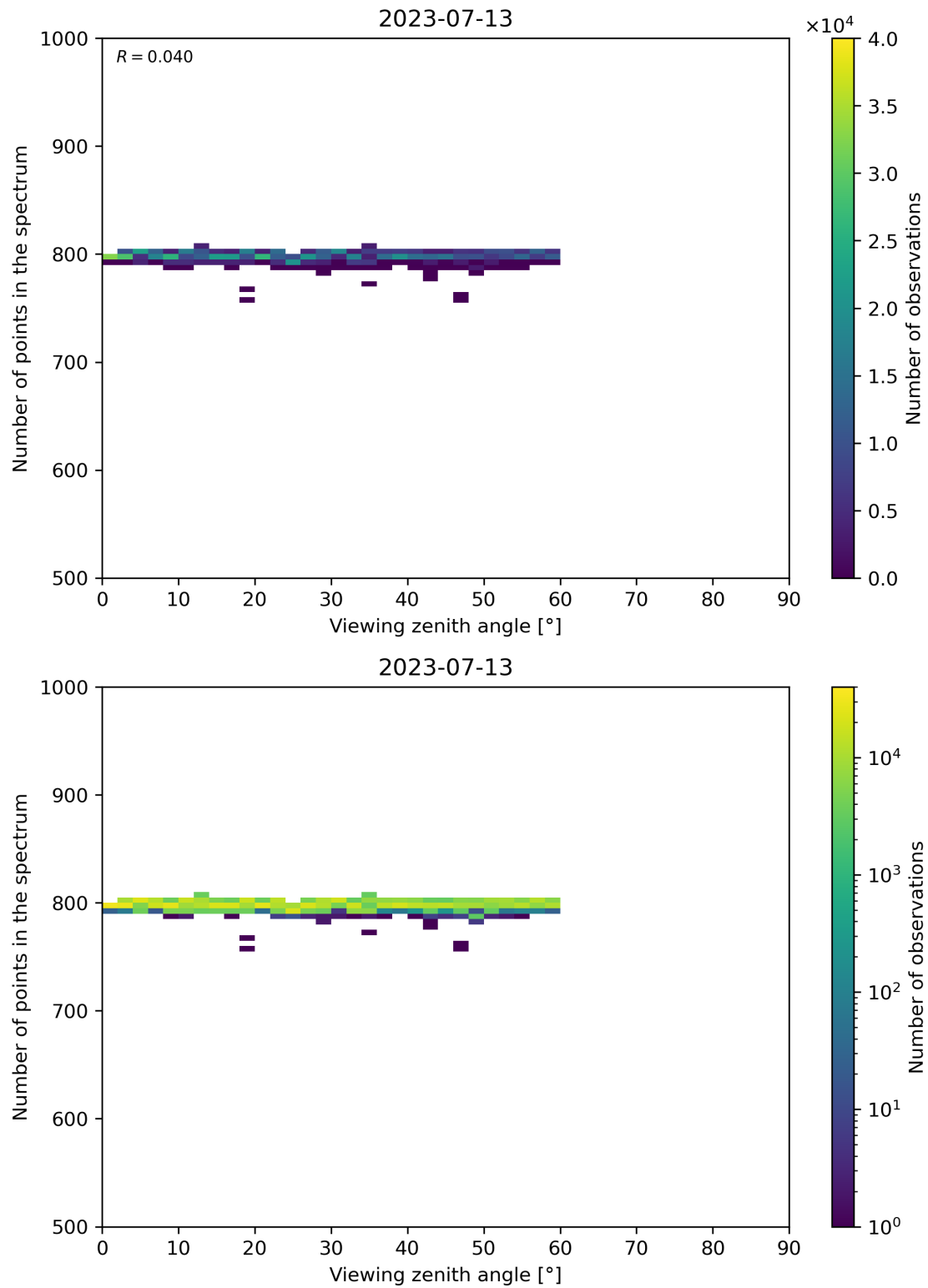
Figure 114: Scatter density plot of “Viewing zenith angle” against “Number of points in the spectrum” for 2023-07-13 to 2023-07-14.
