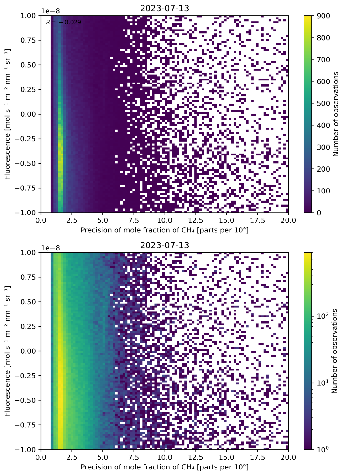
Figure 81: Scatter density plot of “Precision of mole fraction of \text{CH}_4 ” against “Fluorescence” for 2023-07-13 to 2023-07-14.
