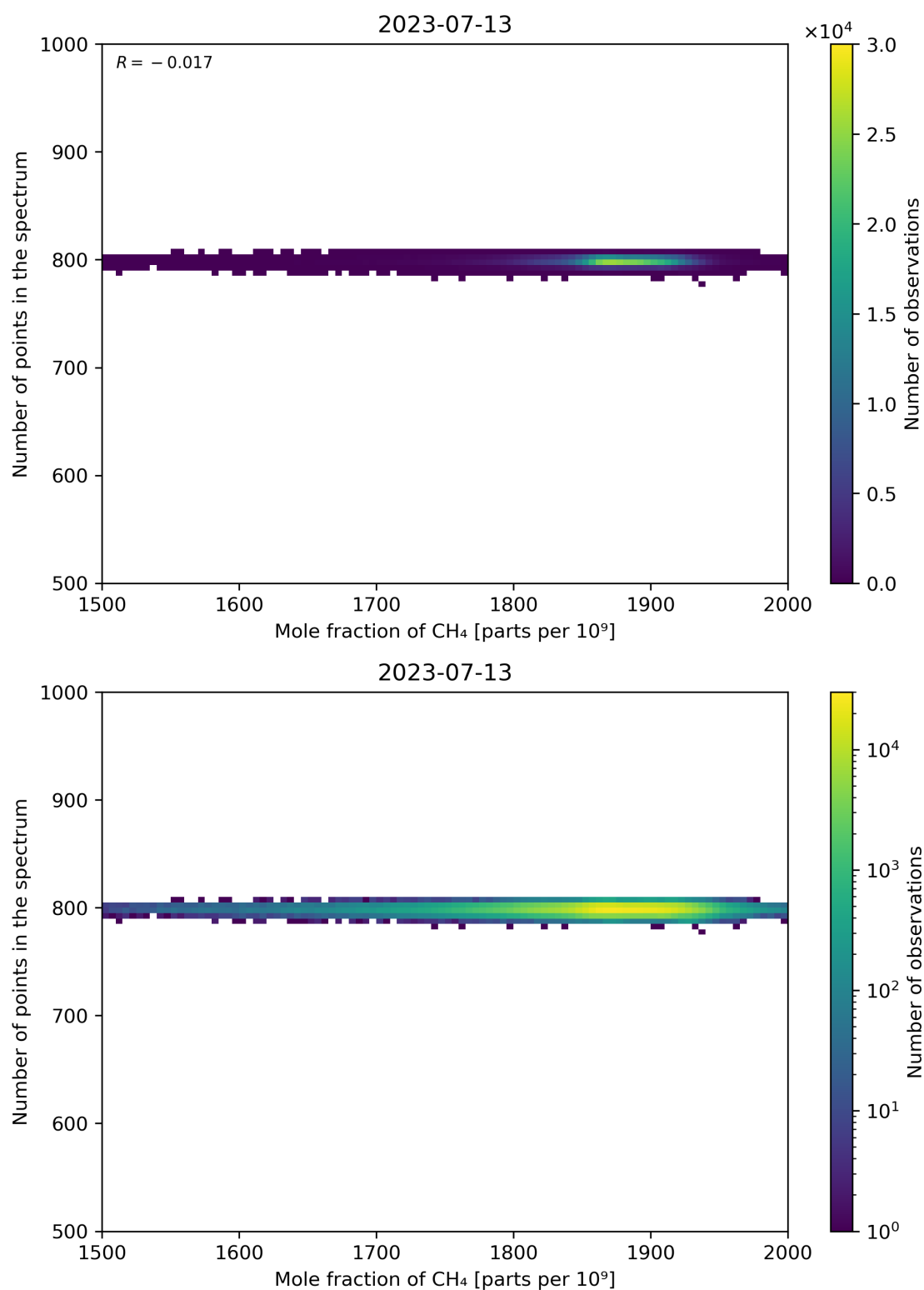
Figure 77: Scatter density plot of “Mole fraction of CH 4 ” against “Number of points in the spectrum” for 2023-07-13 to 2023-07-14.
