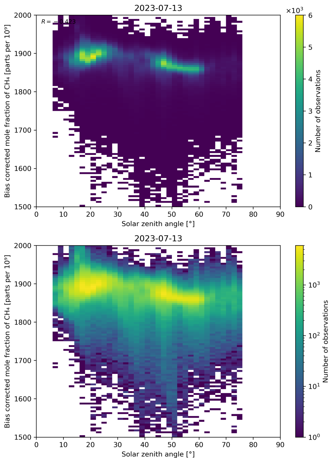
Figure 100: Scatter density plot of “Solar zenith angle” against “Bias corrected mole fraction of CH 4 ” for 2023-07-13 to 2023-07-14.
