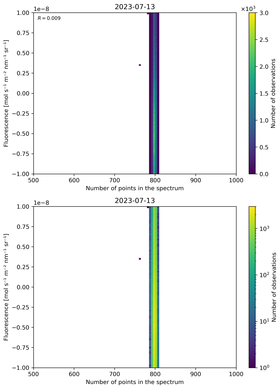
Figure 91: Scatter density plot of “Number of points in the spectrum” against “Fluorescence” for 2023-07-13 to 2023-07-14.
