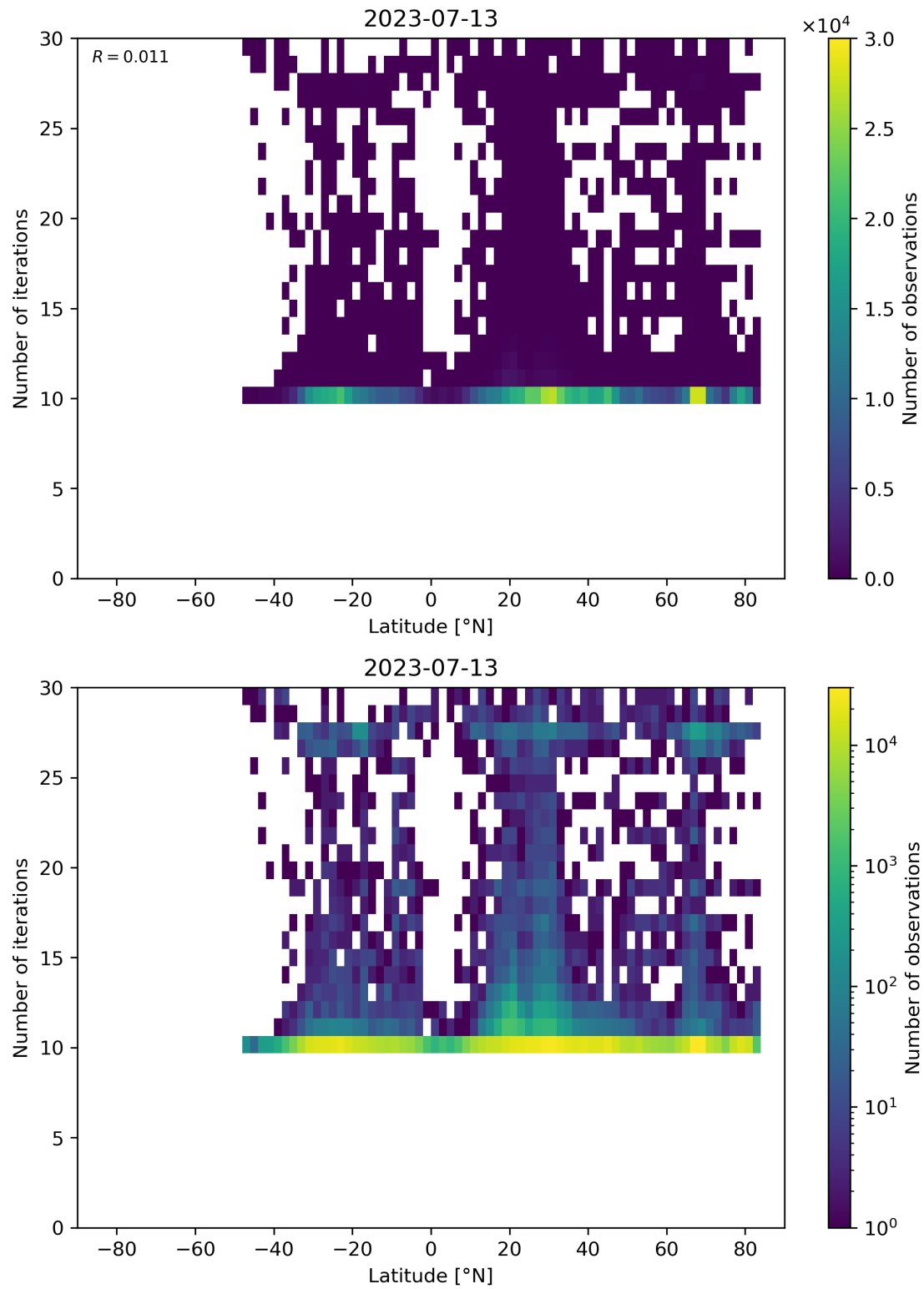
Figure 60: Scatter density plot of “Latitude” against “Number of iterations” for 2023-07-13 to 2023-07-14.
