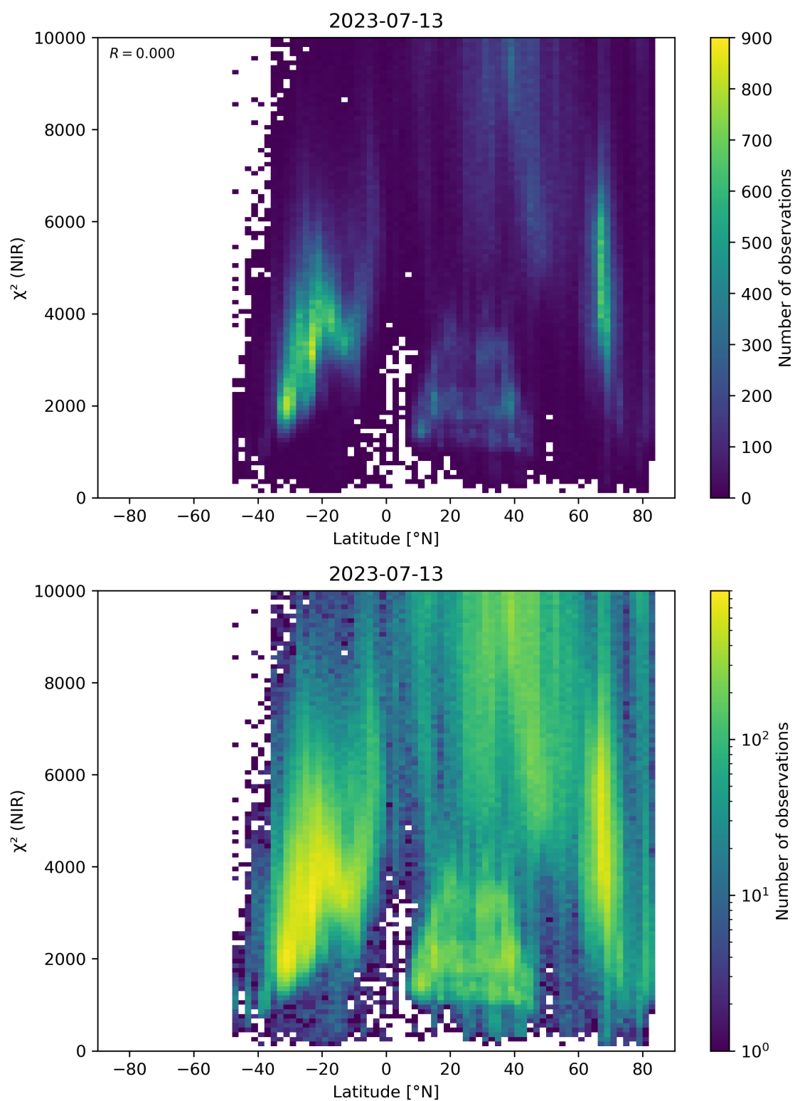
Figure 53: Scatter density plot of “Latitude” against “ \chi^2 (NIR)” for 2023-07-13 to 2023-07-14.
