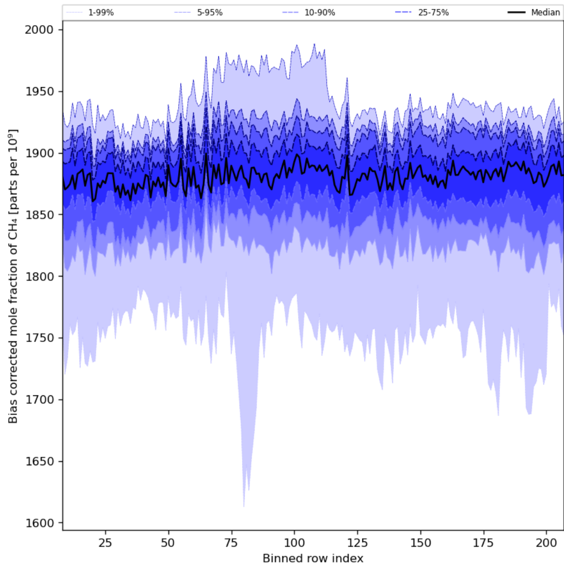
Figure 36: Along track statistics of “Bias corrected mole fraction of CH 4 ” for 2023-07-13 to 2023-07-14
