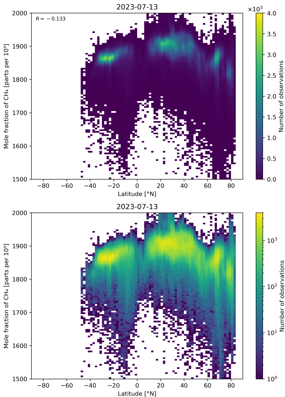
Figure 57: Scatter density plot of “Latitude” against “Mole fraction of CH 4 ” for 2023-07-13 to 2023-07-14.
