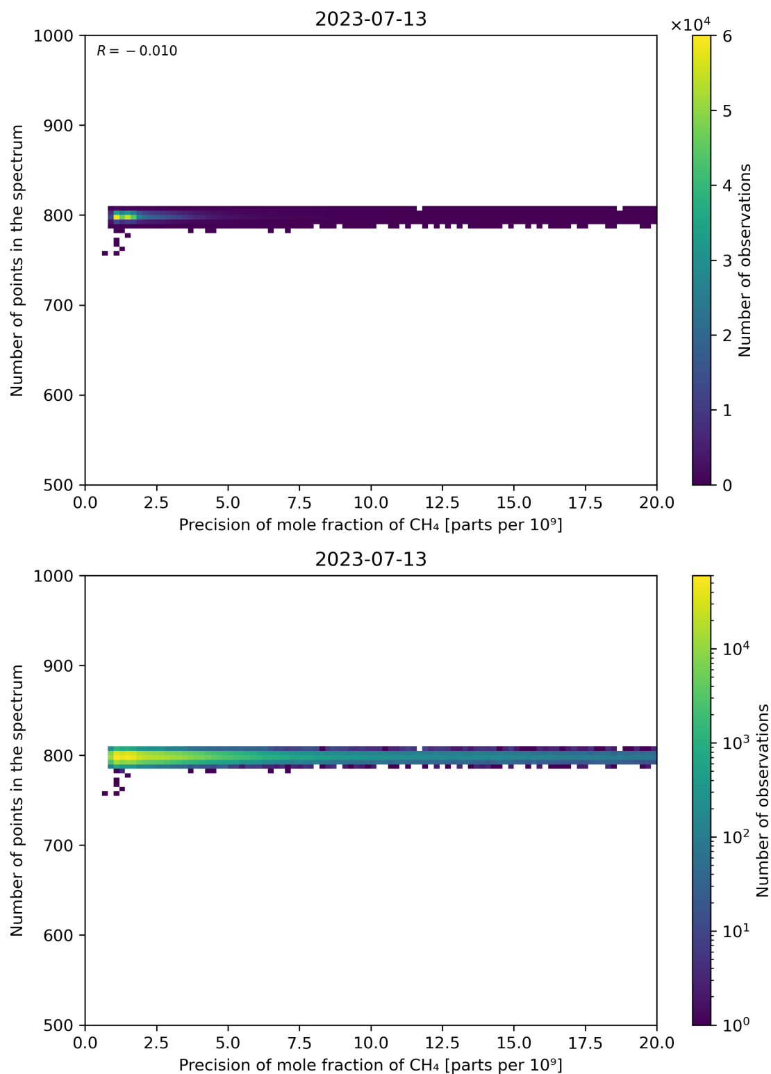
Figure 84: Scatter density plot of “Precision of mole fraction of CH 4 ” against “Number of points in the spectrum” for 2023-07-13 to 2023-07-14.
