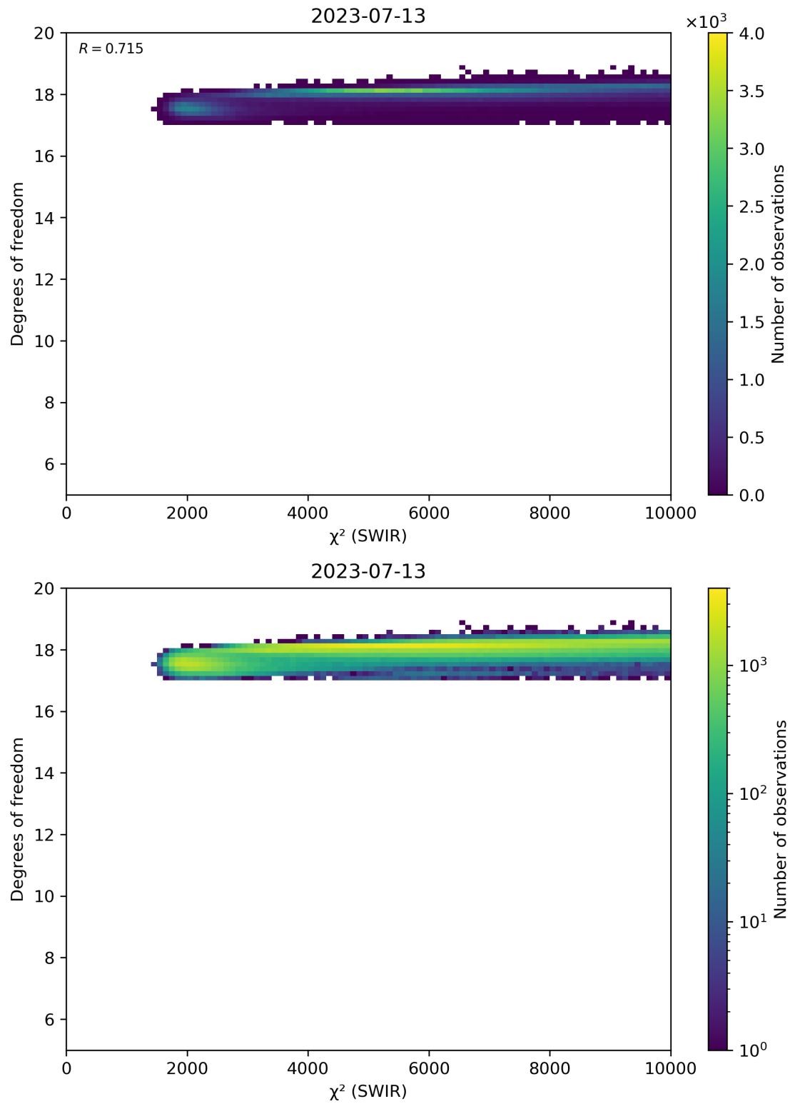
Figure 48: Scatter density plot of “ \chi^2 (SWIR)” against “Degrees of freedom” for 2023-07-13 to 2023-07-14.
