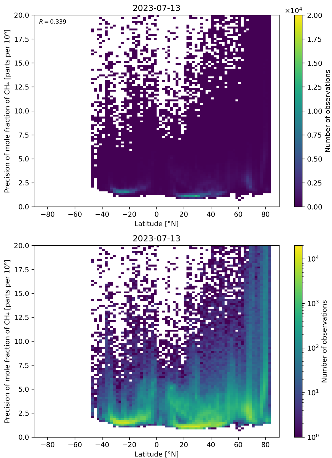
Figure 59: Scatter density plot of “Latitude” against “Precision of mole fraction of \text{CH}_4 ” for 2023-07-13 to 2023-07-14.
