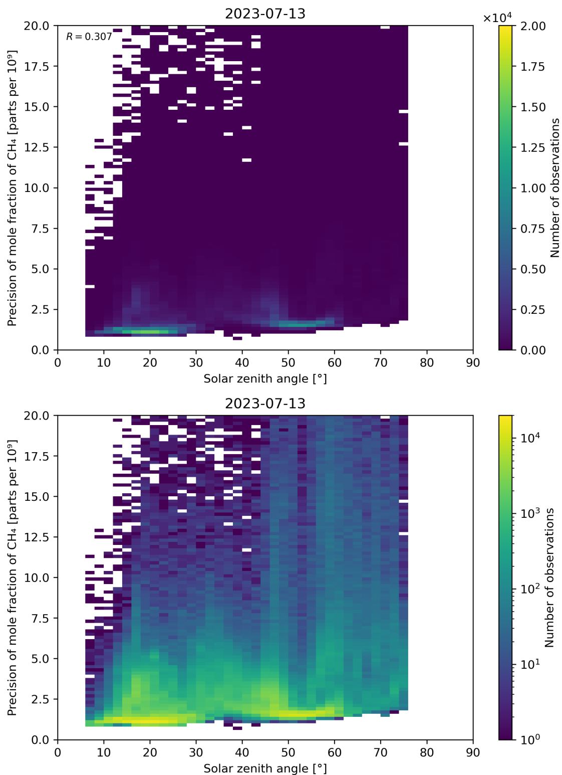
Figure 101: Scatter density plot of “Solar zenith angle” against “Precision of mole fraction of \text{CH}_4 ” for 2023-07-13 to 2023-07-14.
