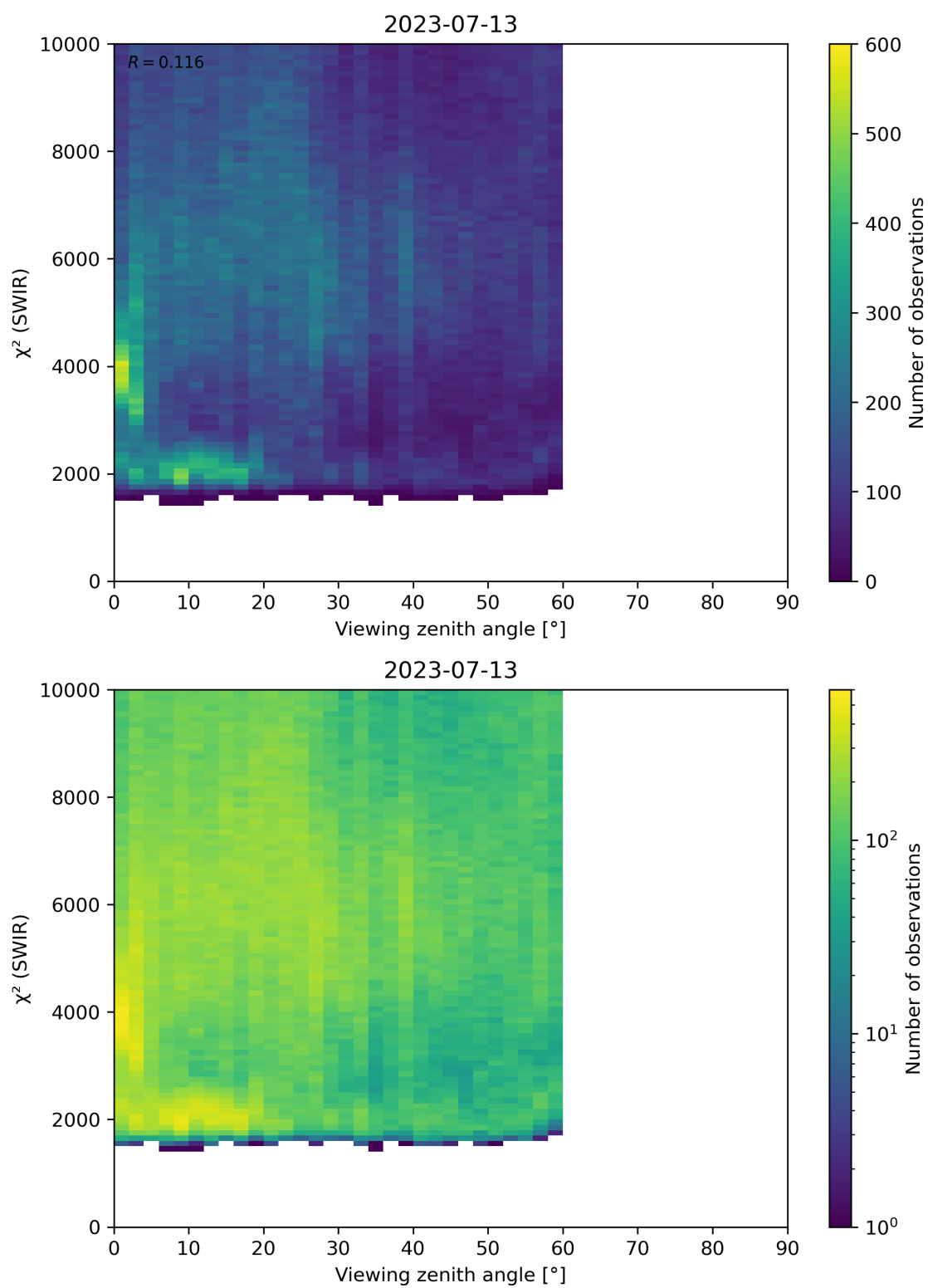
Figure 106: Scatter density plot of “Viewing zenith angle” against “ \chi^2 (SWIR)” for 2023-07-13 to 2023-07-14.
