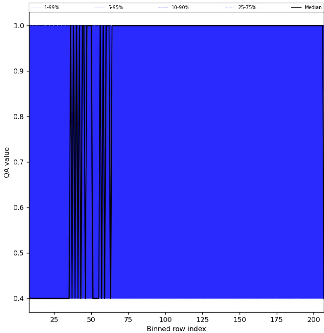
Figure 33: Along track statistics of “QA value” for 2023-07-13 to 2023-07-14
