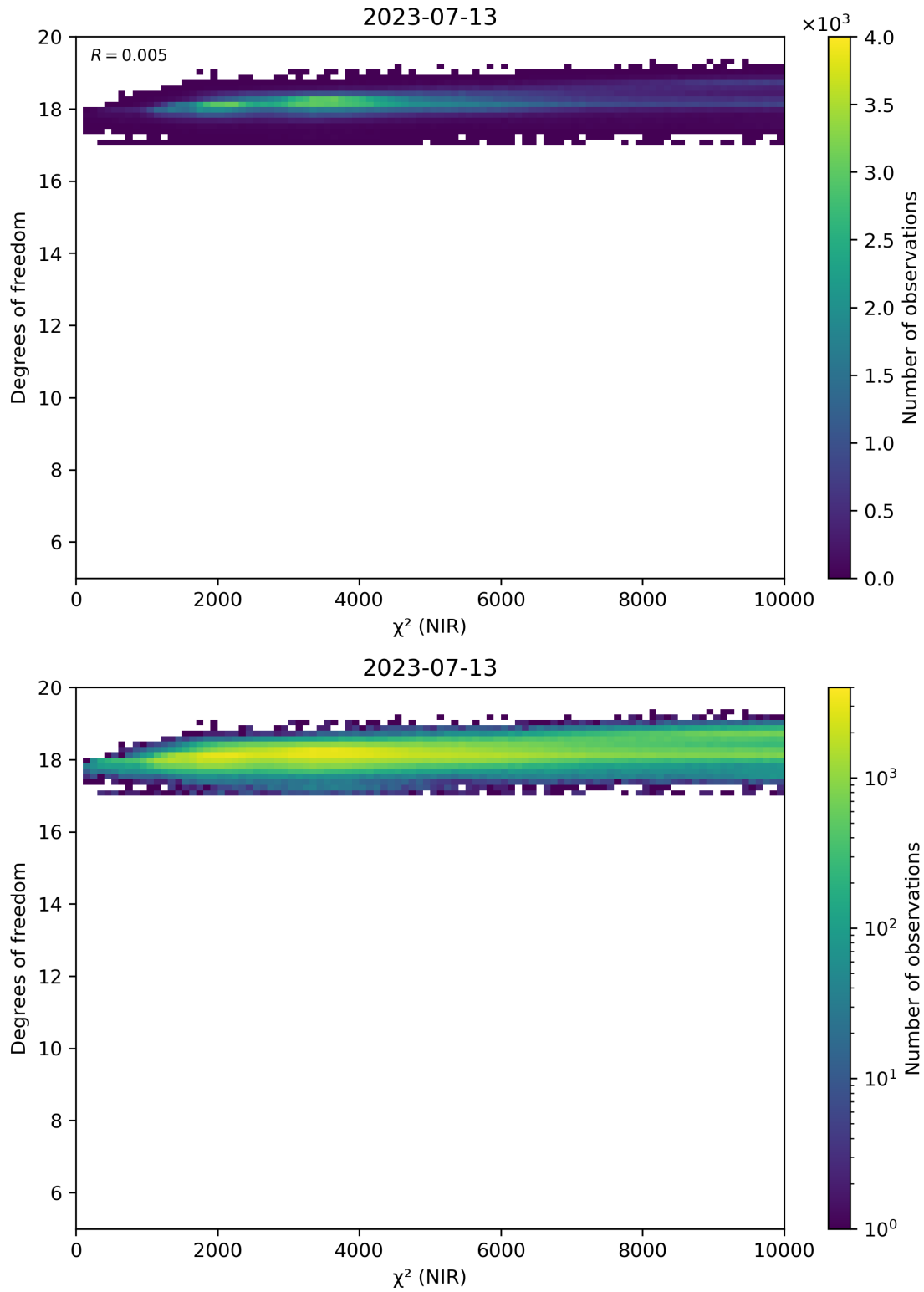
Figure 44: Scatter density plot of “ \chi^2 (NIR)” against “Degrees of freedom” for 2023-07-13 to 2023-07-14.
