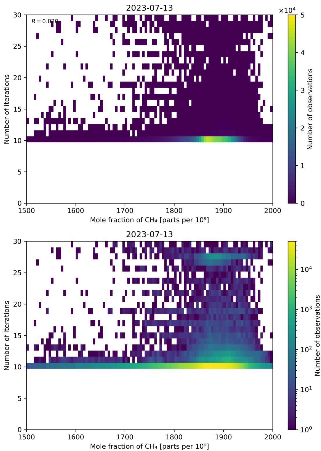
Figure 76: Scatter density plot of “Mole fraction of CH 4 ” against “Number of iterations” for 2023-07-13 to 2023-07-14.
