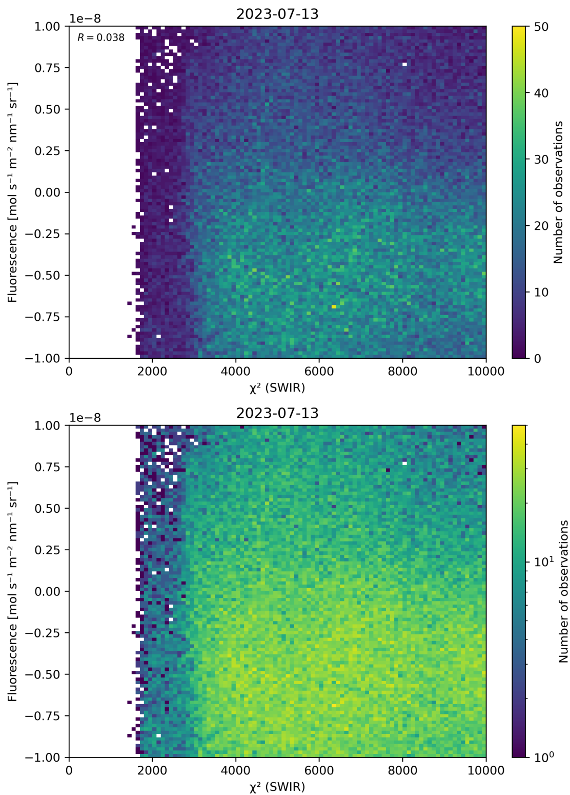
Figure 49: Scatter density plot of “ \chi^2 (SWIR)” against “Fluorescence” for 2023-07-13 to 2023-07-14.
