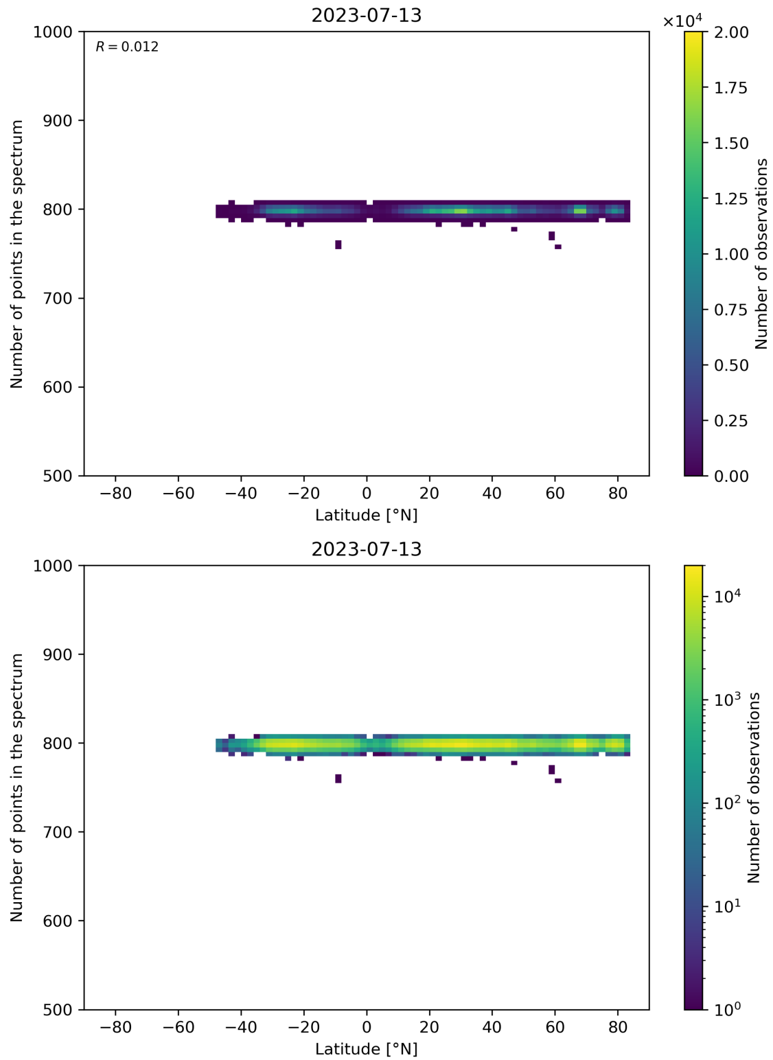
Figure 61: Scatter density plot of “Latitude” against “Number of points in the spectrum” for 2023-07-13 to 2023-07-14.
