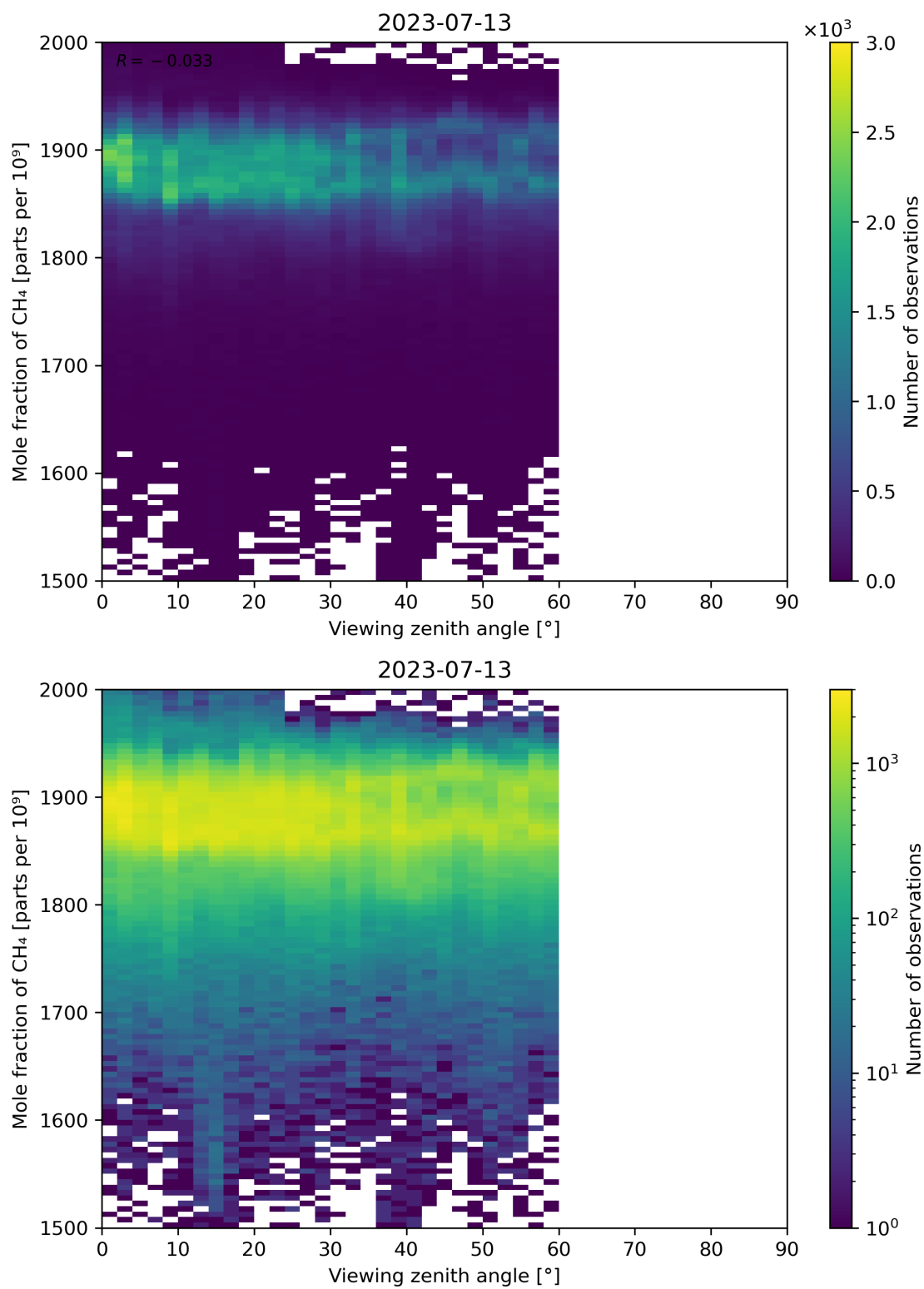
Figure 110: Scatter density plot of “Viewing zenith angle” against “Mole fraction of CH 4 ” for 2023-07-13 to 2023-07-14.
