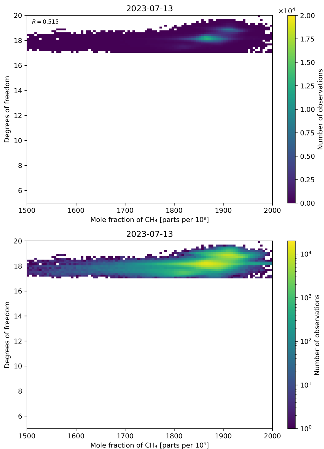
Figure 72: Scatter density plot of “Mole fraction of CH 4 ” against “Degrees of freedom” for 2023-07-13 to 2023-07-14.
