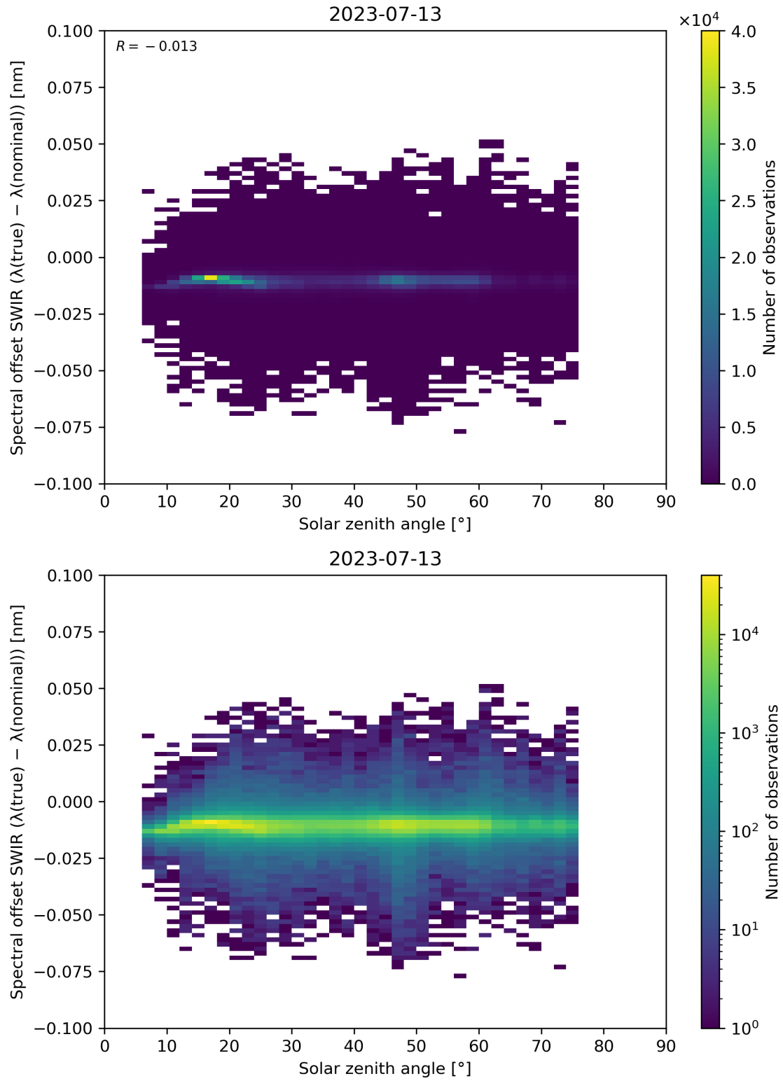
Figure 104: Scatter density plot of “Solar zenith angle” against “Spectral offset SWIR ( \lambda(\text{true}) - \lambda(\text{nominal}) )” for 2023-07-13 to 2023-07-14.
