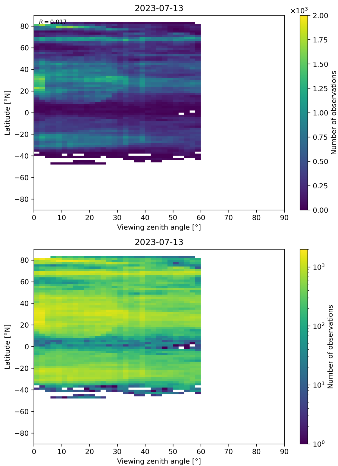
Figure 109: Scatter density plot of “Viewing zenith angle” against “Latitude” for 2023-07-13 to 2023-07-14.
