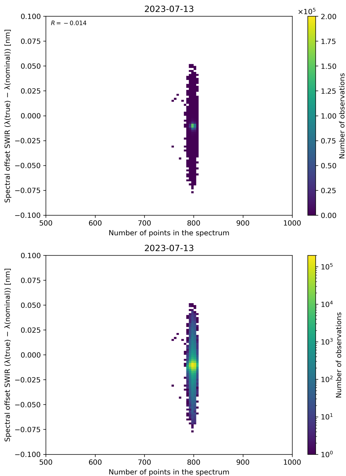
Figure 93: Scatter density plot of “Number of points in the spectrum” against “Spectral offset SWIR ( \lambda(\text{true}) - \lambda(\text{nominal}) )” for 2023-07-13 to 2023-07-14.
