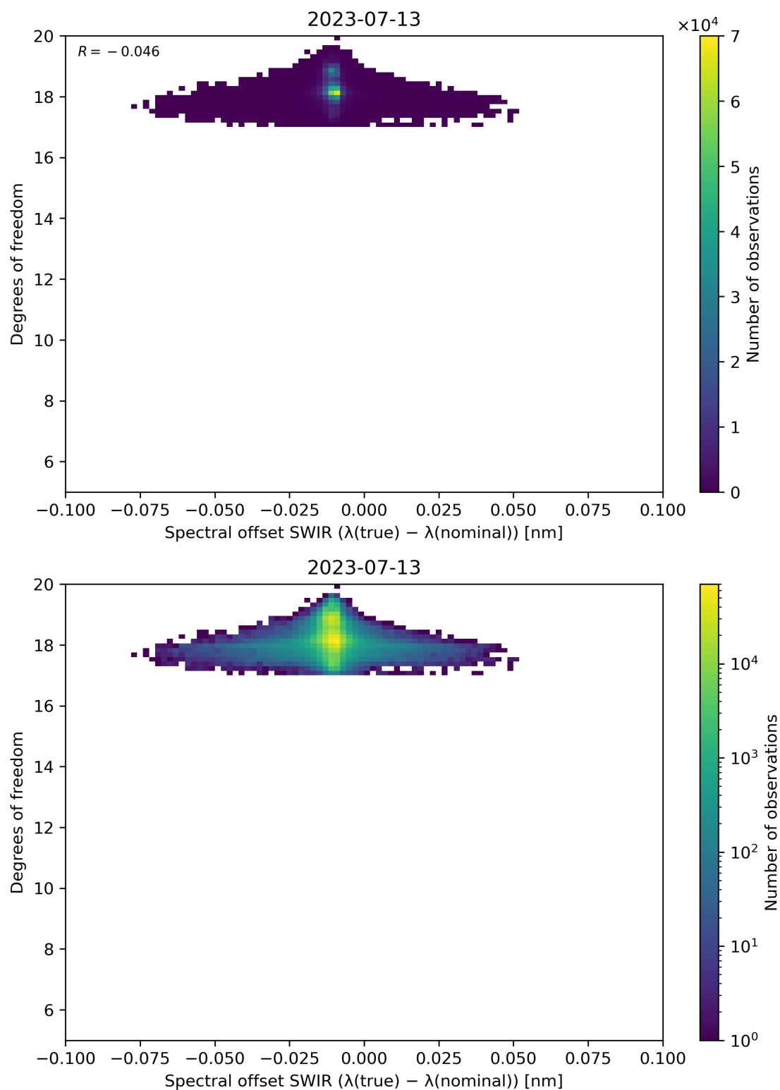
Figure 119: Scatter density plot of “Spectral offset SWIR ( \lambda(\text{true}) - \lambda(\text{nominal}) )” against “Degrees of freedom” for 2023-07-13 to 2023-07-14.
