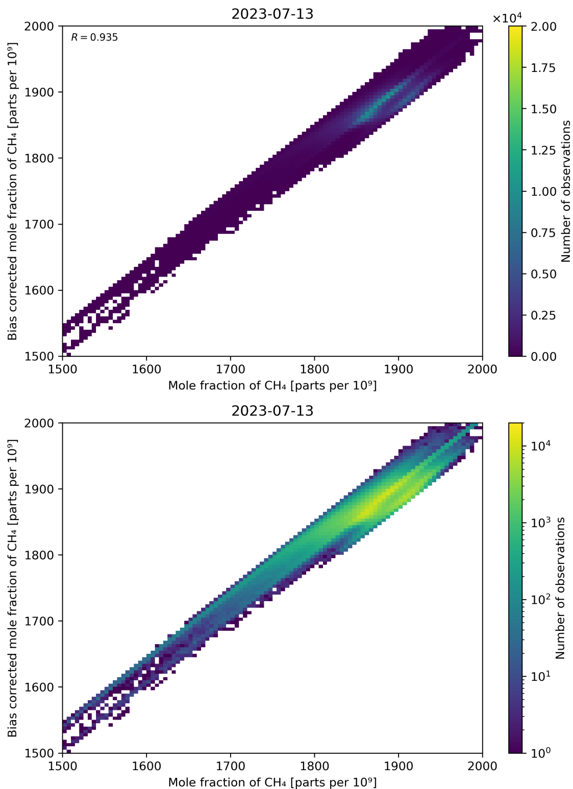
Figure 74: Scatter density plot of “Mole fraction of CH 4 ” against “Bias corrected mole fraction of CH 4 ” for 2023-07-13 to 2023-07-14.
