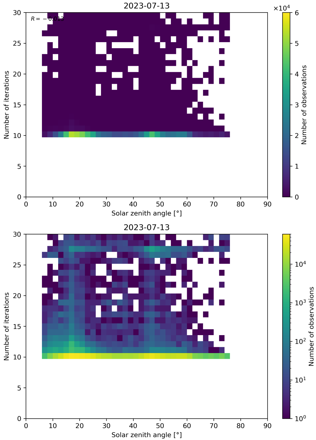
Figure 102: Scatter density plot of “Solar zenith angle” against “Number of iterations” for 2023-07-13 to 2023-07-14.
