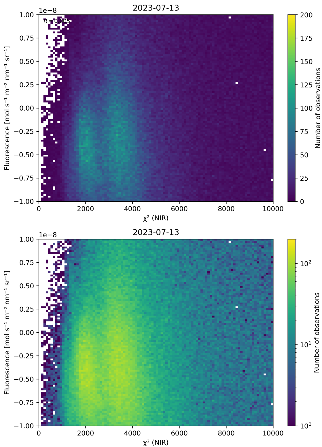
Figure 45: Scatter density plot of “ \chi^2 (NIR)” against “Fluorescence” for 2023-07-13 to 2023-07-14.
