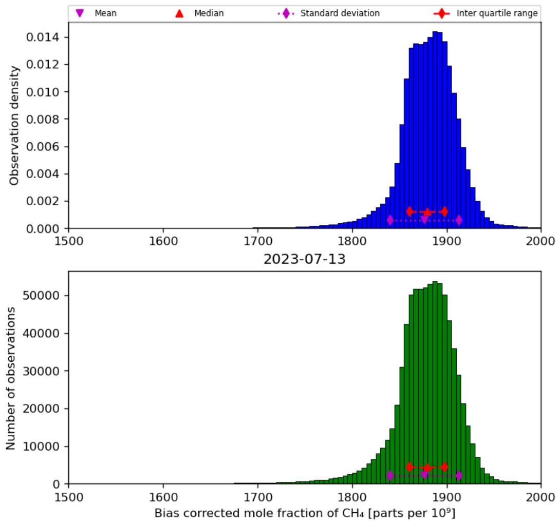
Figure 25: Histogram of “Bias corrected mole fraction of CH 4 ” for 2023-07-13 to 2023-07-14
