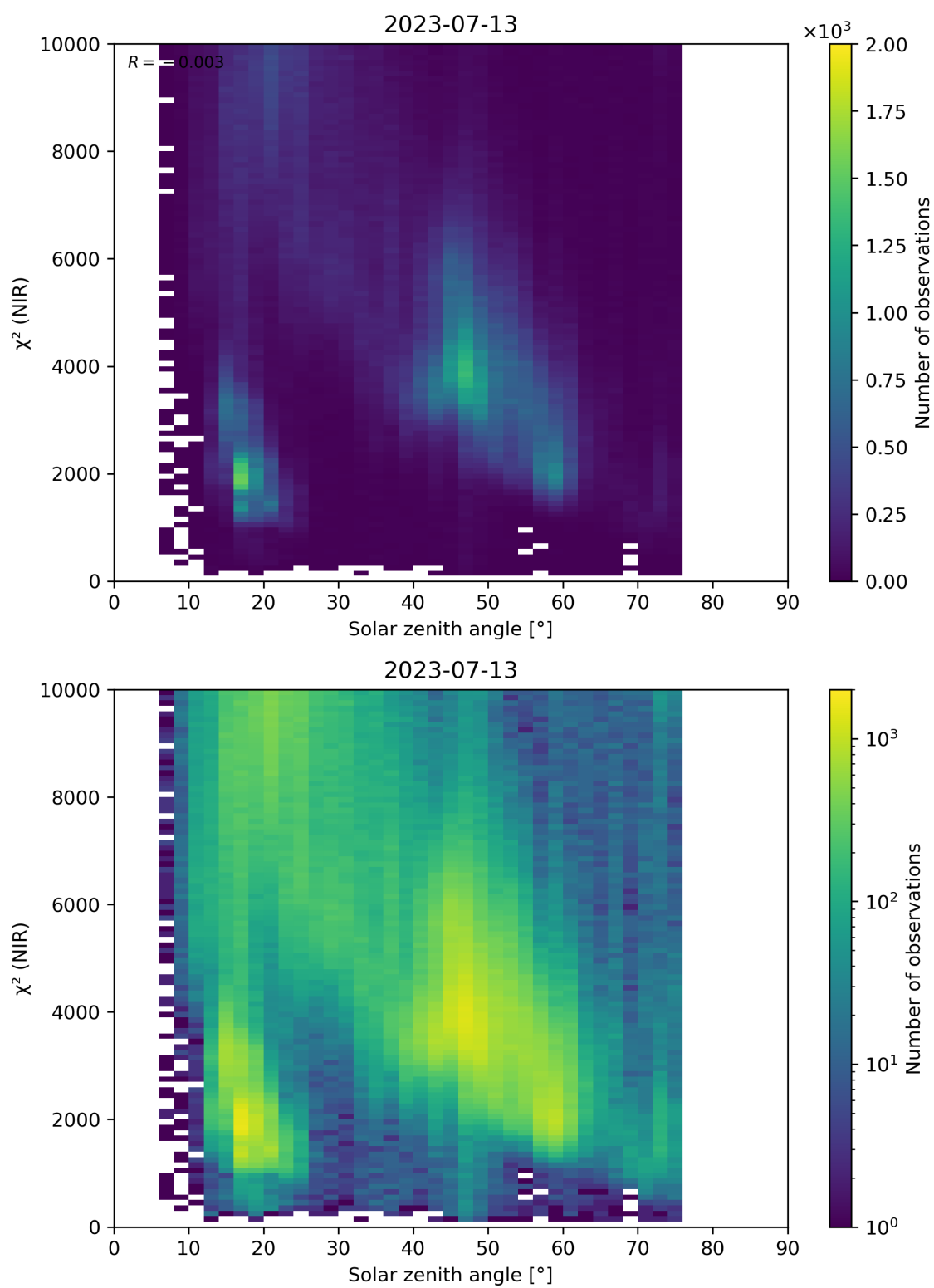
Figure 94: Scatter density plot of “Solar zenith angle” against “ \chi^2 (NIR)” for 2023-07-13 to 2023-07-14.
