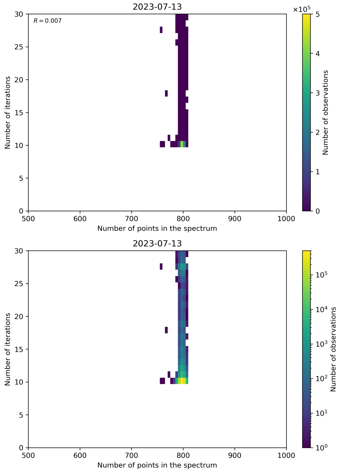
Figure 92: Scatter density plot of “Number of points in the spectrum” against “Number of iterations” for 2023-07-13 to 2023-07-14.
