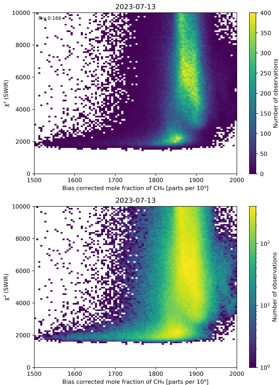
Figure 64: Scatter density plot of “Bias corrected mole fraction of CH 4 ” against “ \chi^2 (SWIR)” for 2023-07-13 to 2023-07-14.
