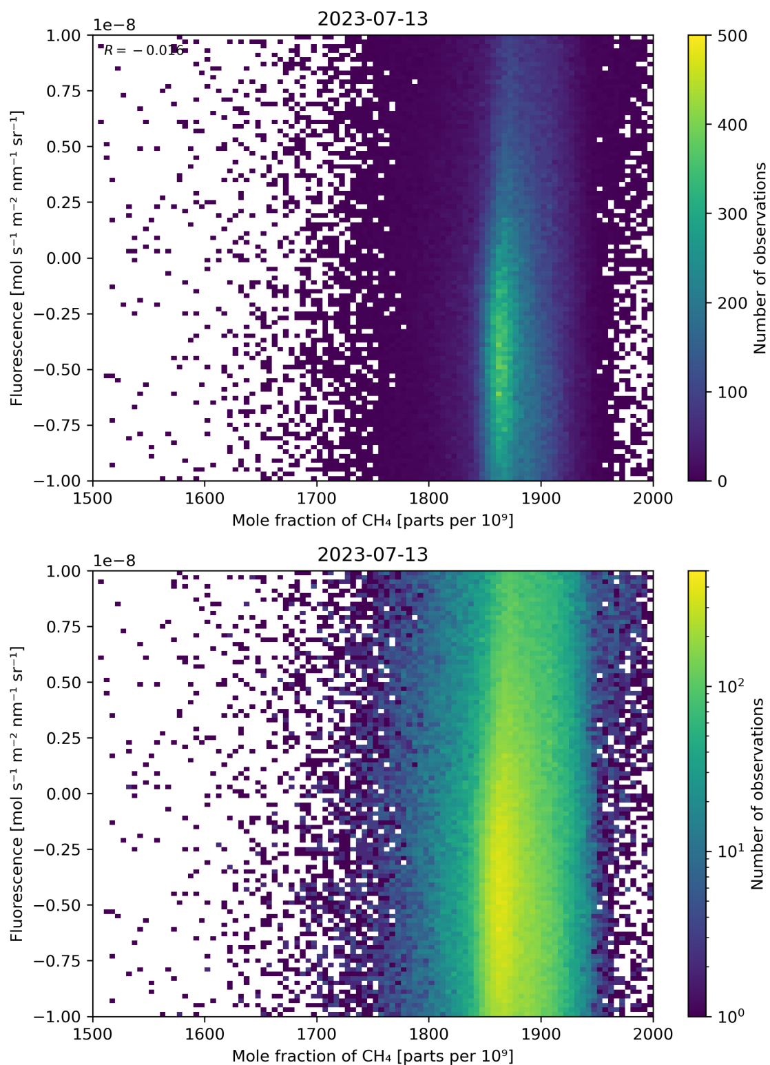
Figure 73: Scatter density plot of “Mole fraction of \text{CH}_4 ” against “Fluorescence” for 2023-07-13 to 2023-07-14.
