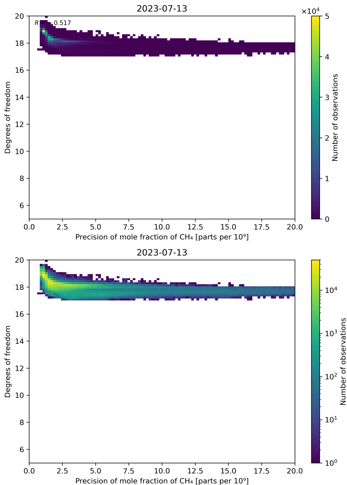
Figure 80: Scatter density plot of “Precision of mole fraction of CH 4 ” against “Degrees of freedom” for 2023-07-13 to 2023-07-14.
