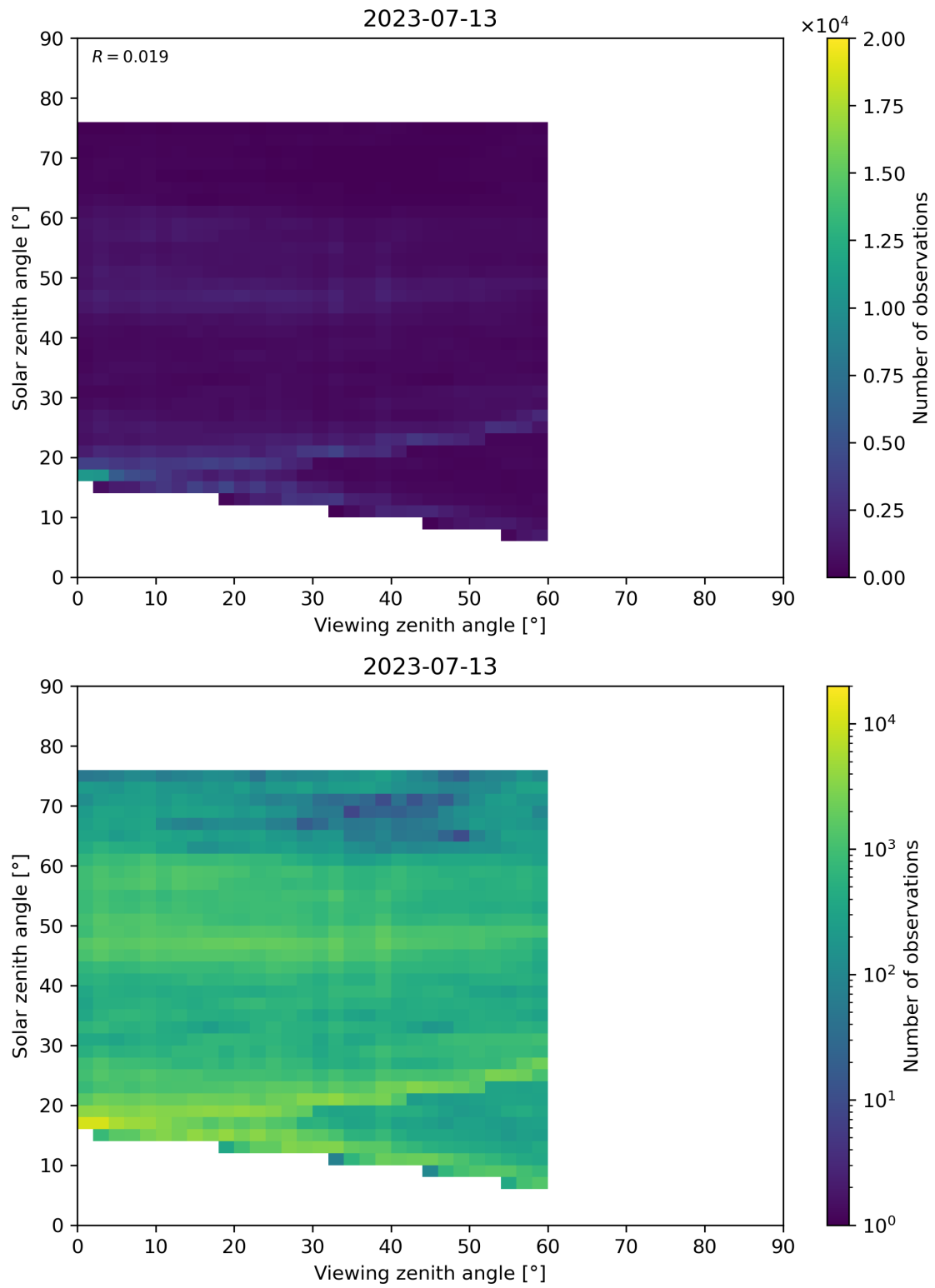
Figure 115: Scatter density plot of “Viewing zenith angle” against “Solar zenith angle” for 2023-07-13 to 2023-07-14.
