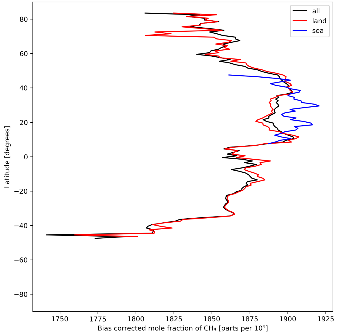
Figure 14: Zonal average of “Bias corrected mole fraction of CH 4 ” for 2023-07-13 to 2023-07-14.
