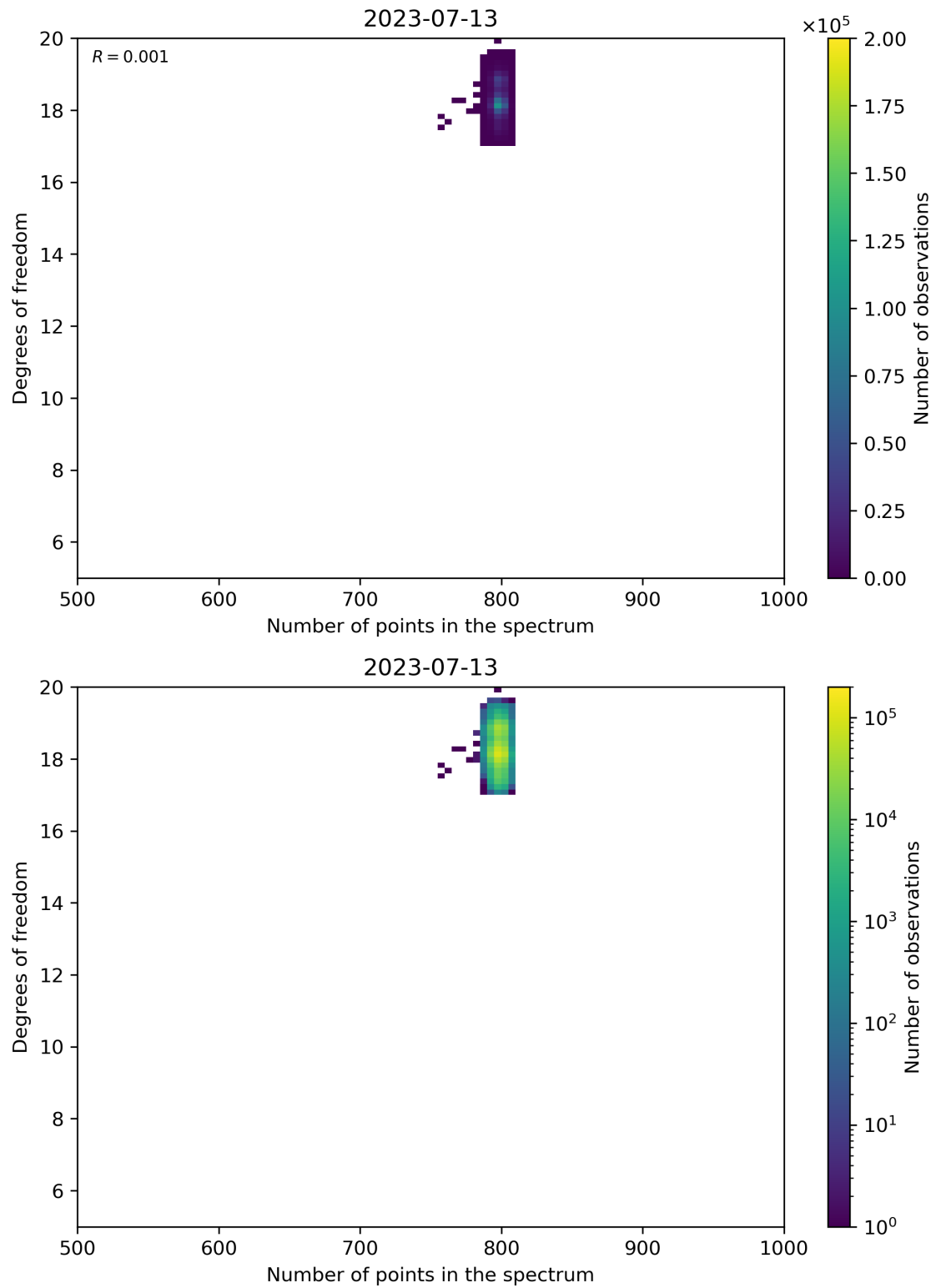
Figure 90: Scatter density plot of “Number of points in the spectrum” against “Degrees of freedom” for 2023-07-13 to 2023-07-14.
