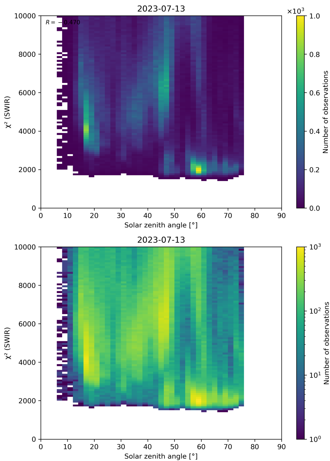
Figure 95: Scatter density plot of “Solar zenith angle” against “ \chi^2 (SWIR)” for 2023-07-13 to 2023-07-14.
