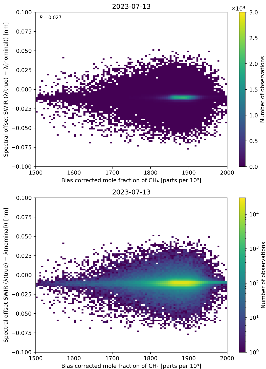
Figure 69: Scatter density plot of “Bias corrected mole fraction of \text{CH}_4 ” against “Spectral offset SWIR ( \lambda(\text{true}) - \lambda(\text{nominal}) )” for 2023-07-13 to 2023-07-14.
