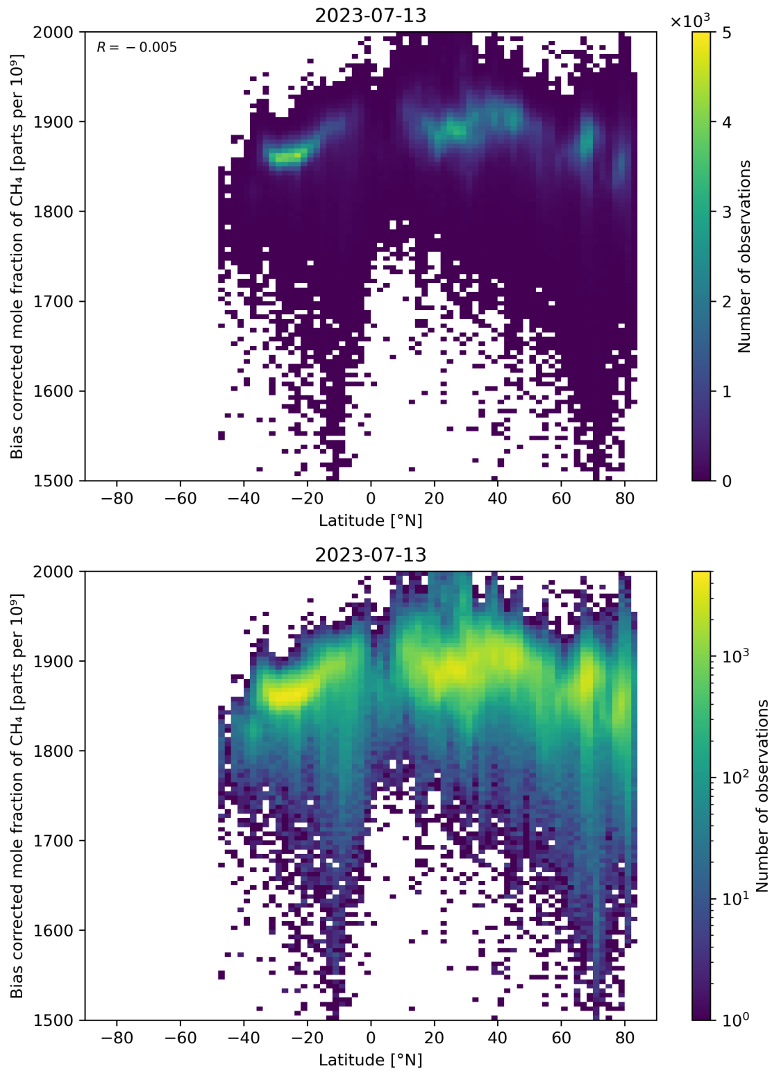
Figure 58: Scatter density plot of “Latitude” against “Bias corrected mole fraction of CH 4 ” for 2023-07-13 to 2023-07-14.
