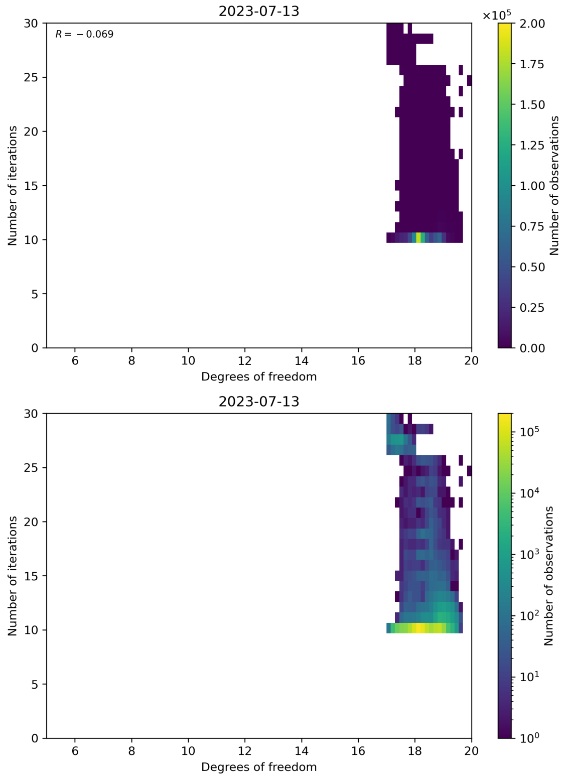
Figure 52: Scatter density plot of “Degrees of freedom” against “Number of iterations” for 2023-07-13 to 2023-07-14.
