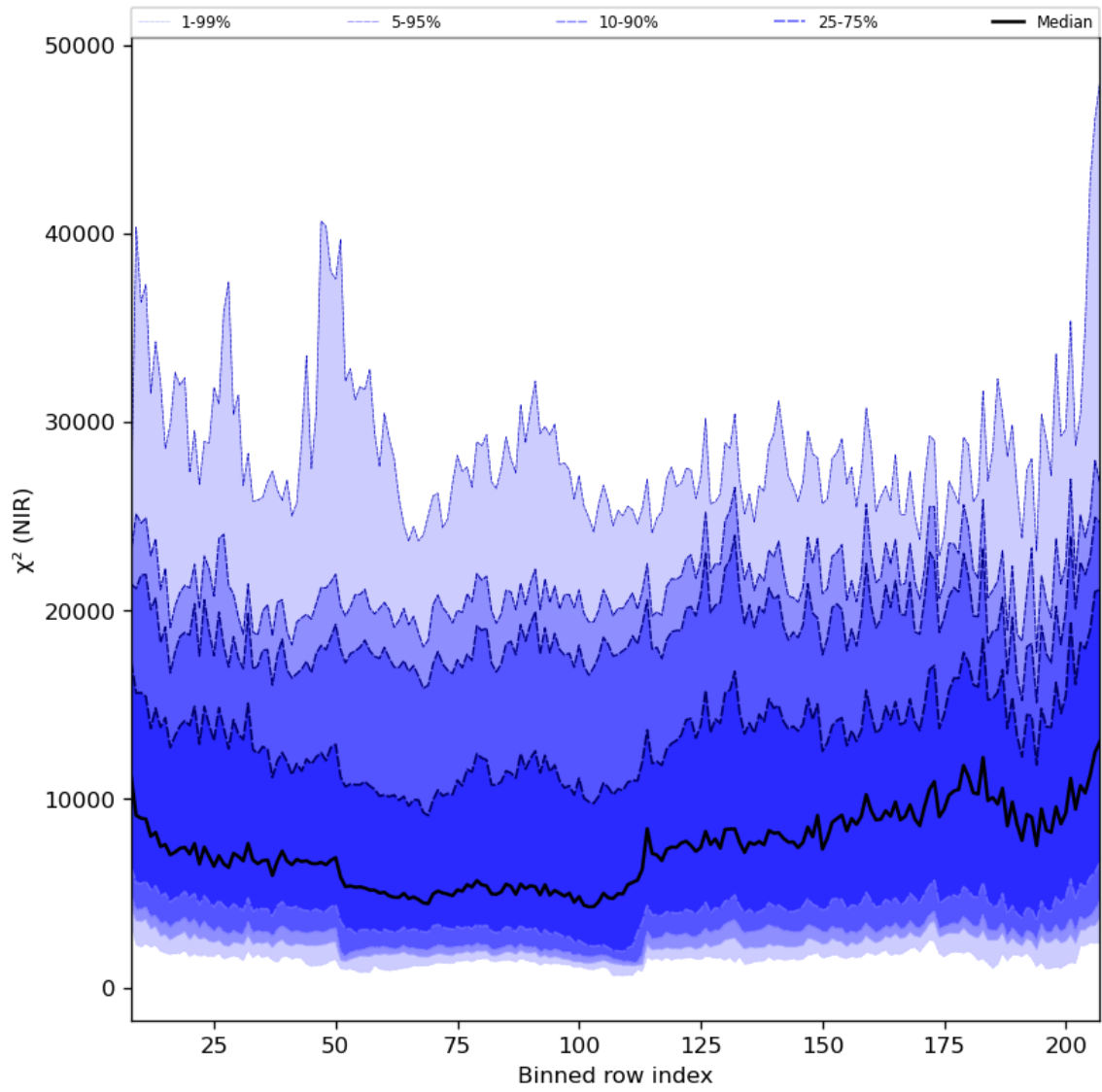
Figure 40: Along track statistics of “ \chi^2 (NIR)” for 2023-07-13 to 2023-07-14
