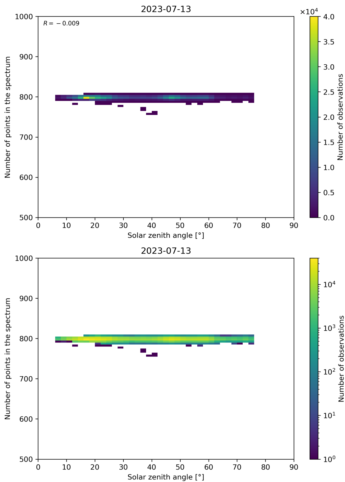
Figure 103: Scatter density plot of “Solar zenith angle” against “Number of points in the spectrum” for 2023-07-13 to 2023-07-14.
