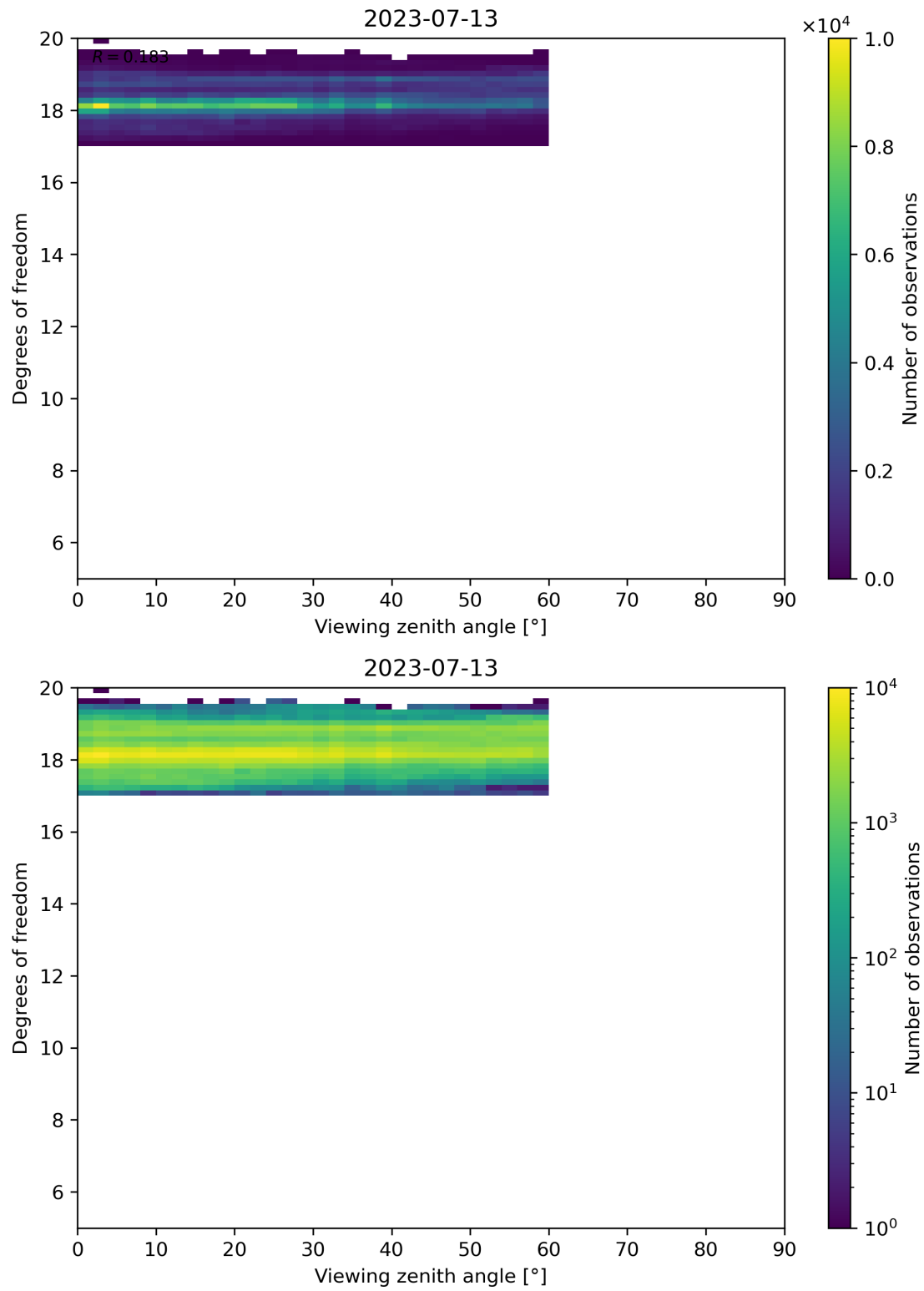
Figure 107: Scatter density plot of “Viewing zenith angle” against “Degrees of freedom” for 2023-07-13 to 2023-07-14.
