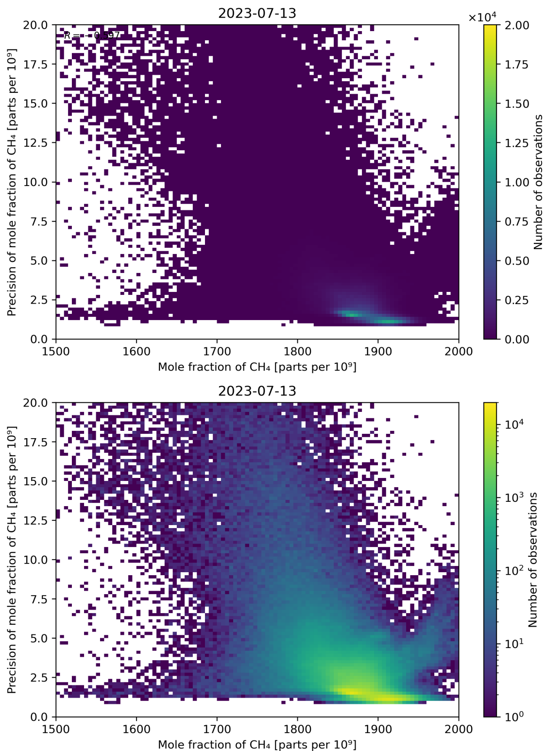
Figure 75: Scatter density plot of “Mole fraction of CH 4 ” against “Precision of mole fraction of CH 4 ” for 2023-07-13 to 2023-07-14.
