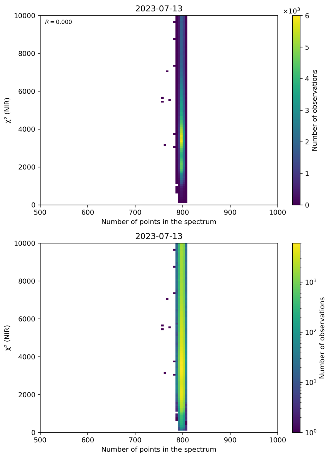
Figure 88: Scatter density plot of “Number of points in the spectrum” against “ \chi^2 (NIR)” for 2023-07-13 to 2023-07-14.
