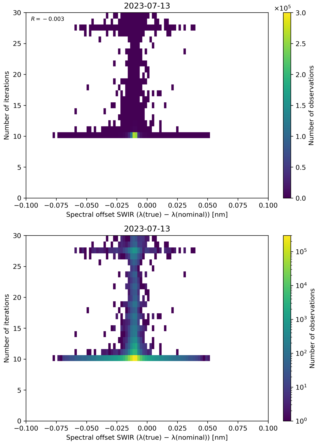
Figure 121: Scatter density plot of “Spectral offset SWIR ( \lambda(\text{true}) - \lambda(\text{nominal}) )” against “Number of iterations” for 2023-07-13 to 2023-07-14.
