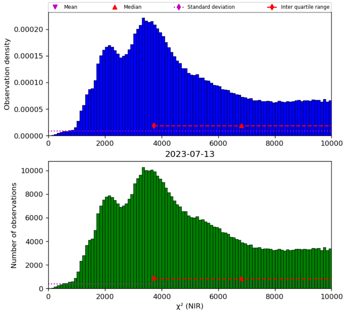
Figure 29: Histogram of “ \chi^2 (NIR)” for 2023-07-13 to 2023-07-14
