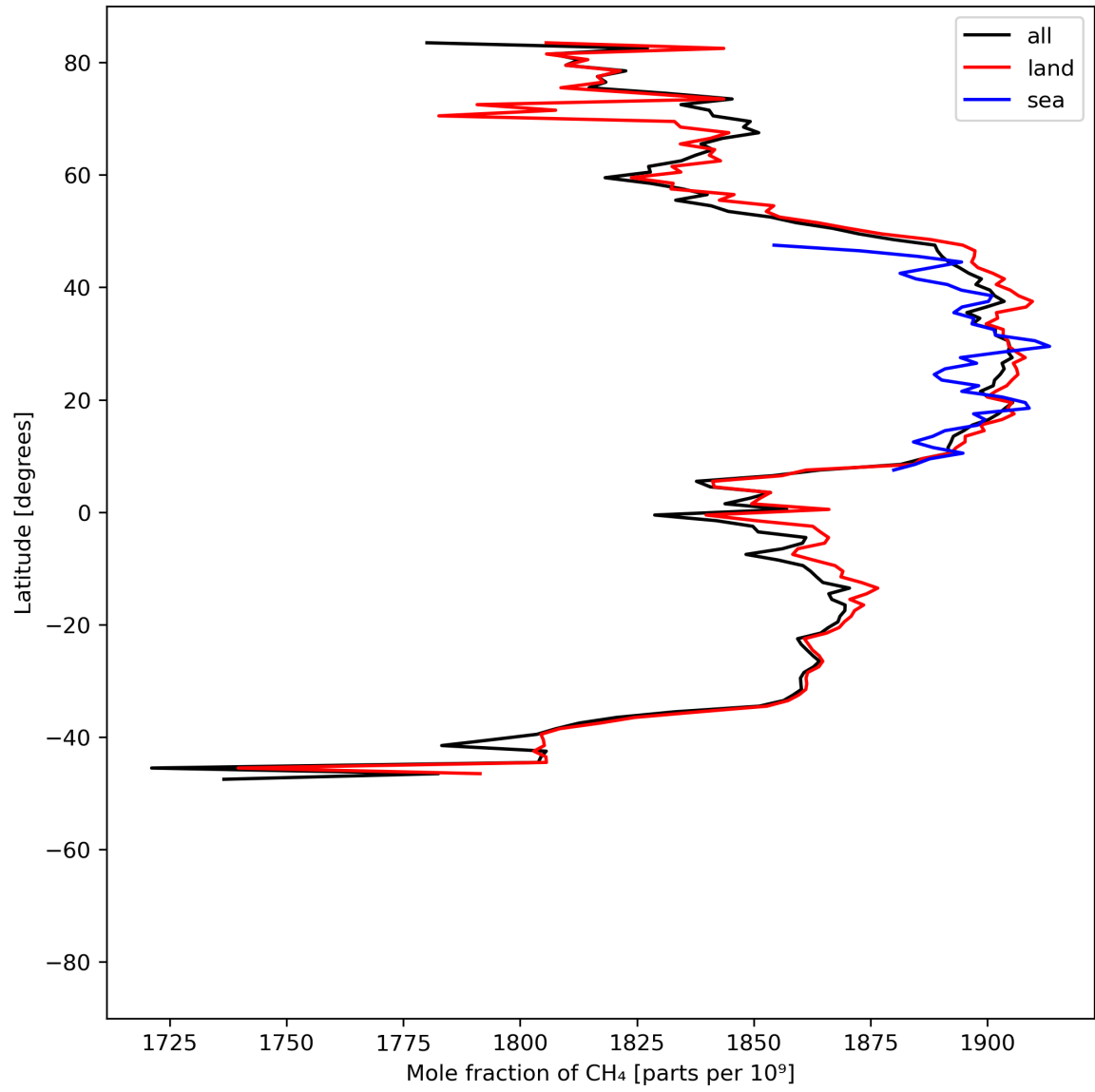
Figure 12: Zonal average of “Mole fraction of CH 4 ” for 2023-07-13 to 2023-07-14.
