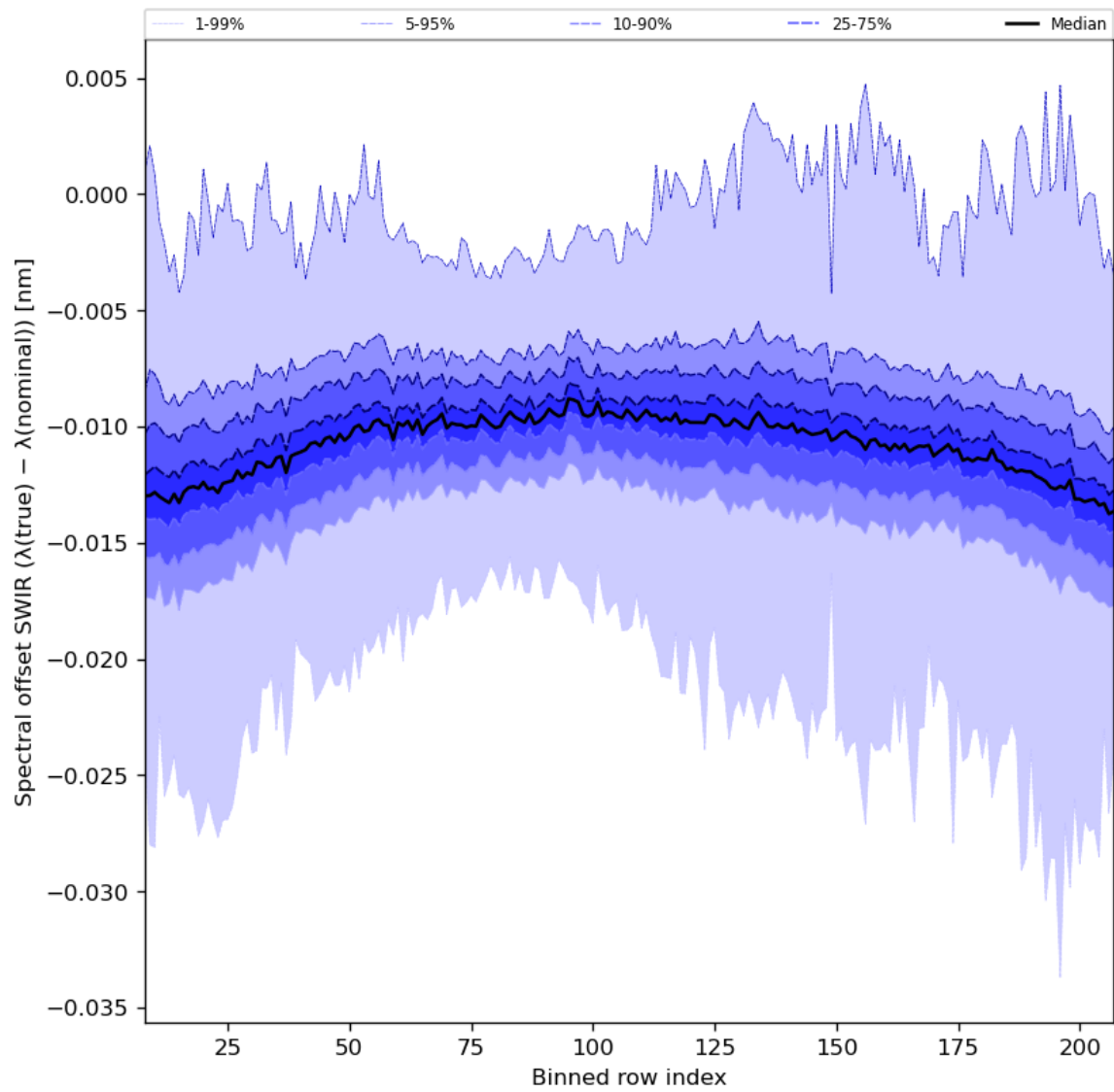
Figure 38: Along track statistics of “Spectral offset SWIR ( \lambda(\text{true}) - \lambda(\text{nominal}) )” for 2023-07-13 to 2023-07-14
