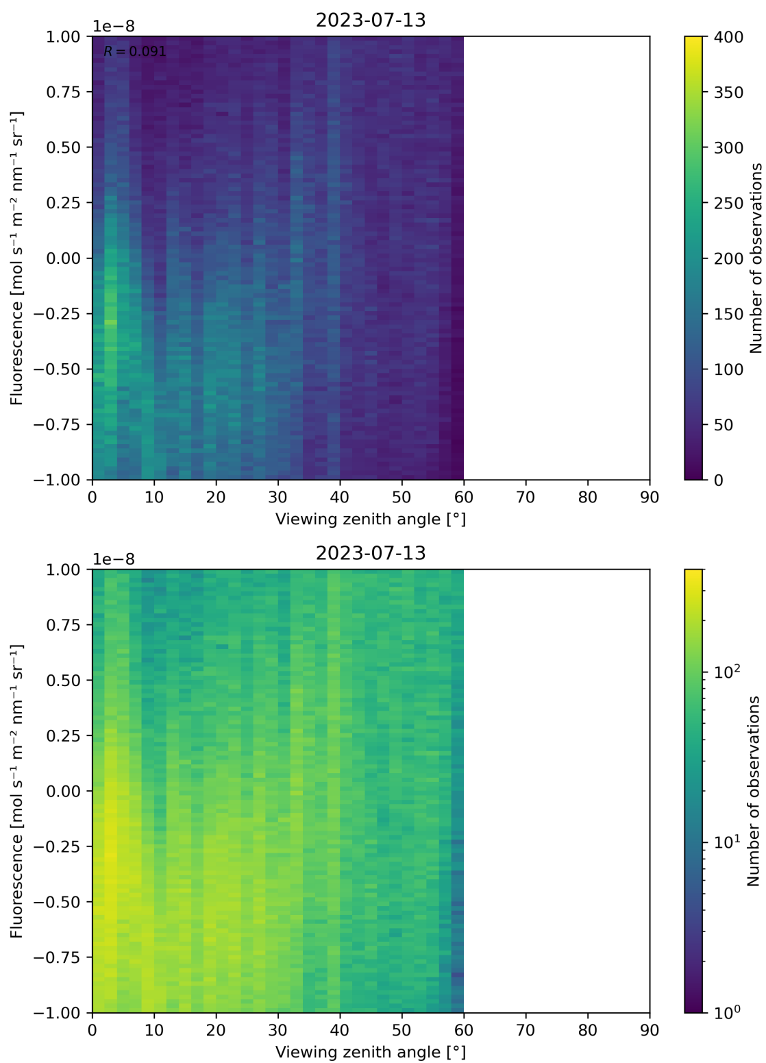
Figure 108: Scatter density plot of “Viewing zenith angle” against “Fluorescence” for 2023-07-13 to 2023-07-14.
