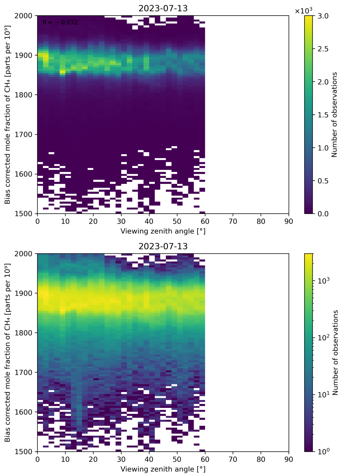
Figure 111: Scatter density plot of “Viewing zenith angle” against “Bias corrected mole fraction of CH 4 ” for 2023-07-13 to 2023-07-14.
