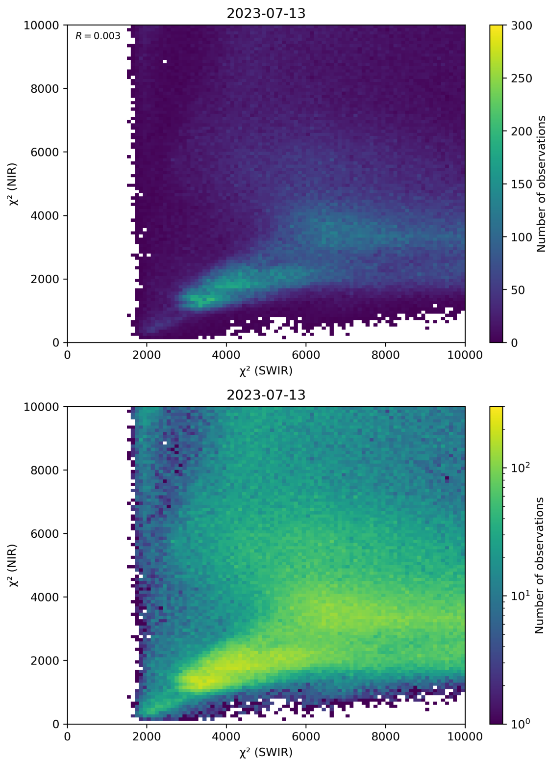
Figure 47: Scatter density plot of “ \chi^2 (SWIR)” against “ \chi^2 (NIR)” for 2023-07-13 to 2023-07-14.
