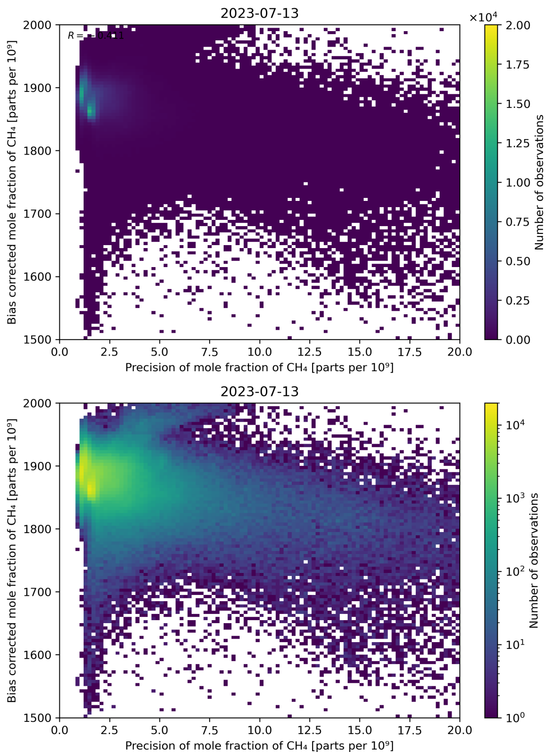
Figure 82: Scatter density plot of “Precision of mole fraction of \text{CH}_4 ” against “Bias corrected mole fraction of \text{CH}_4 ” for 2023-07-13 to 2023-07-14.
