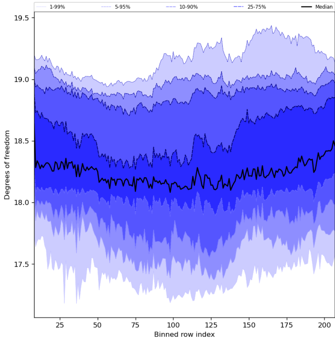
Figure 41: Along track statistics of “Degrees of freedom” for 2023-07-13 to 2023-07-14
