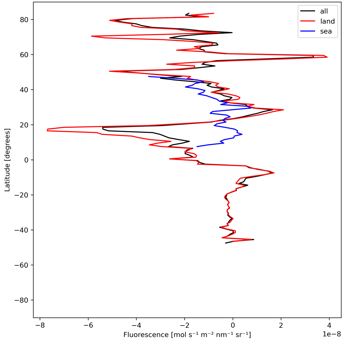
Figure 21: Zonal average of “Fluorescence” for 2023-07-13 to 2023-07-14.
