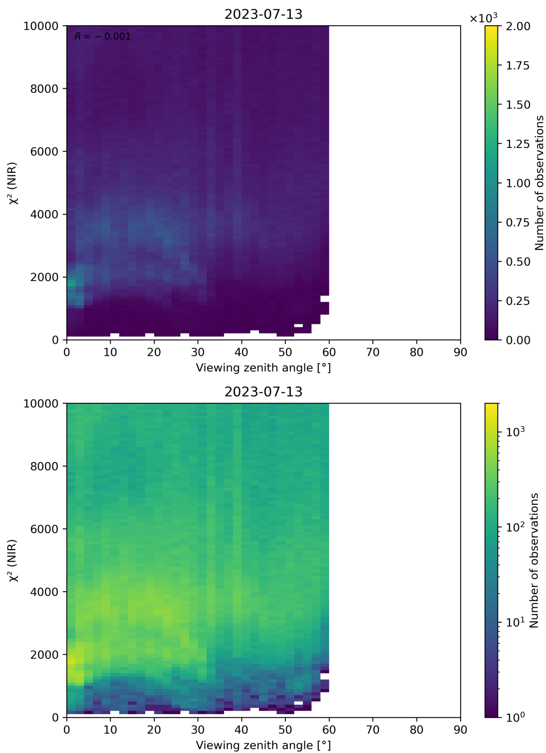
Figure 105: Scatter density plot of “Viewing zenith angle” against “ \chi^2 (NIR)” for 2023-07-13 to 2023-07-14.
