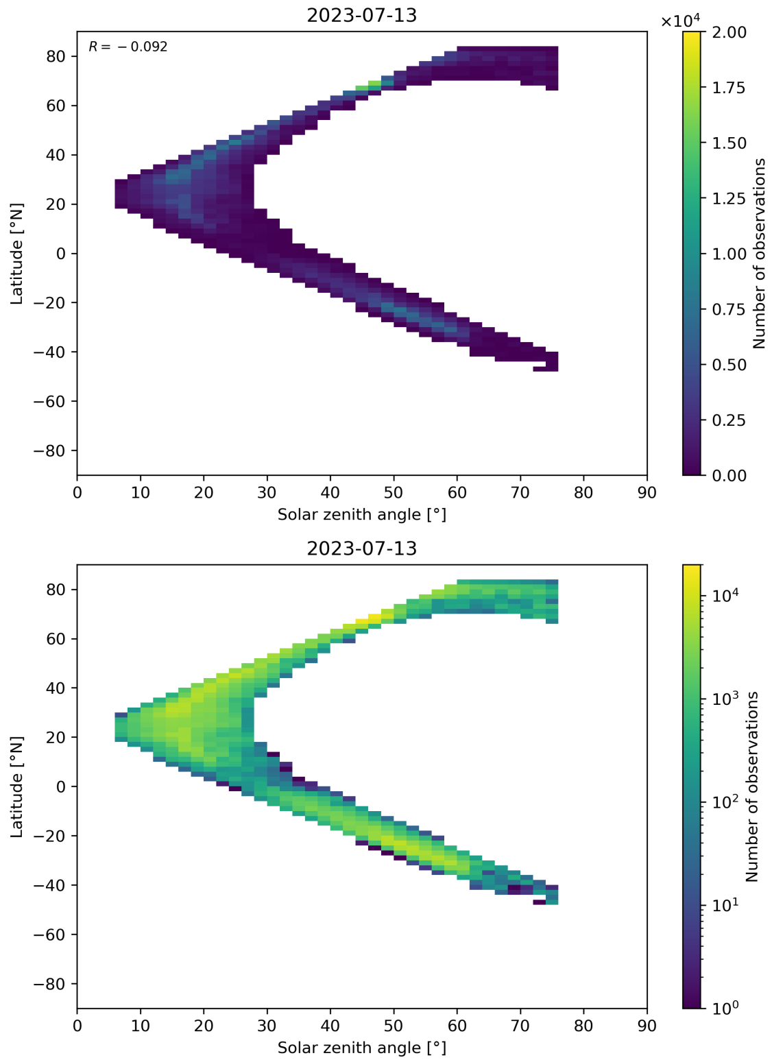
Figure 98: Scatter density plot of “Solar zenith angle” against “Latitude” for 2023-07-13 to 2023-07-14.
