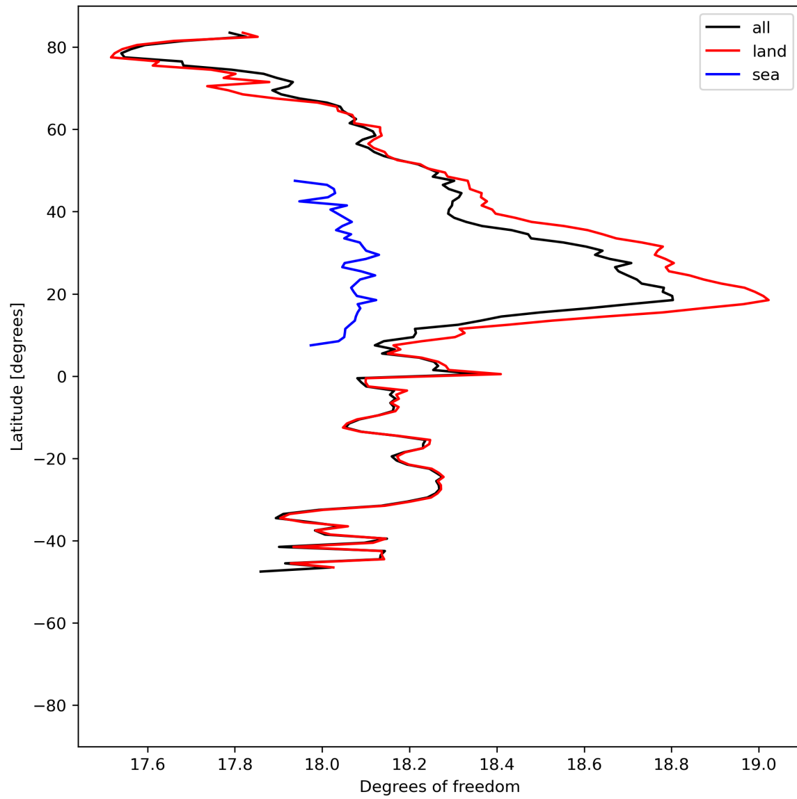
Figure 19: Zonal average of “Degrees of freedom” for 2023-07-13 to 2023-07-14.
