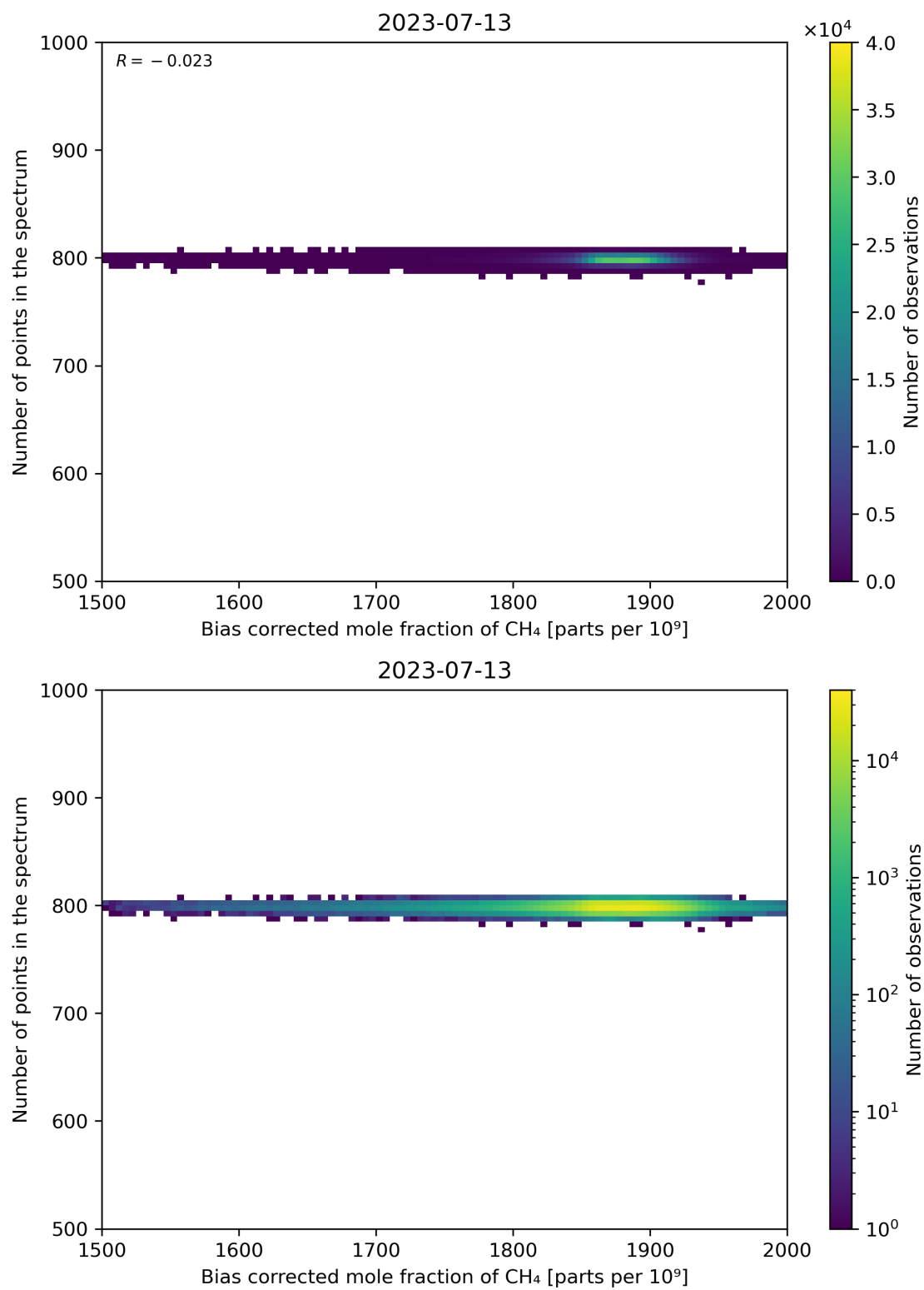
Figure 68: Scatter density plot of “Bias corrected mole fraction of CH 4 ” against “Number of points in the spectrum” for 2023-07-13 to 2023-07-14.
