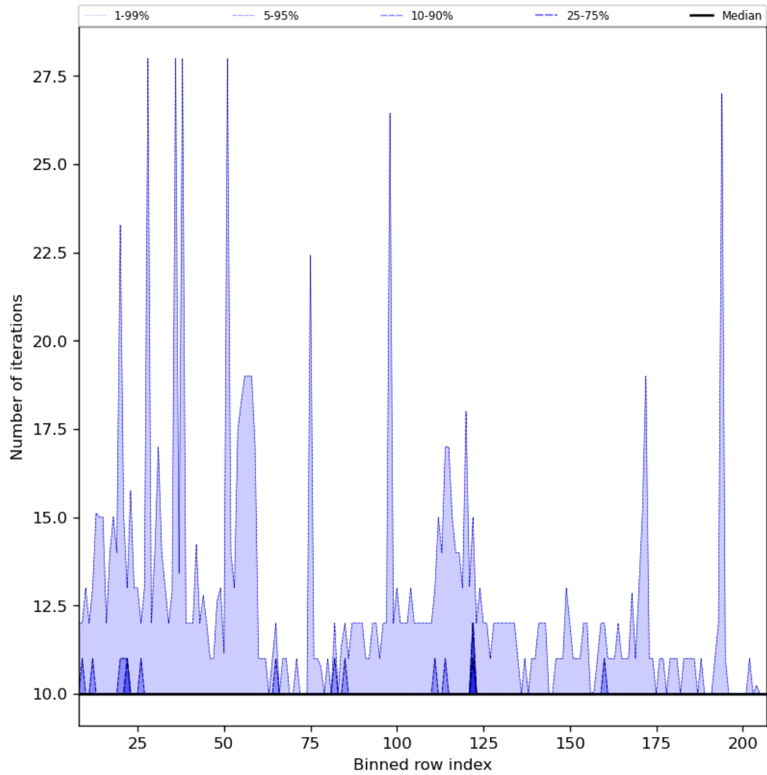
Figure 42: Along track statistics of “Number of iterations” for 2023-07-13 to 2023-07-14
