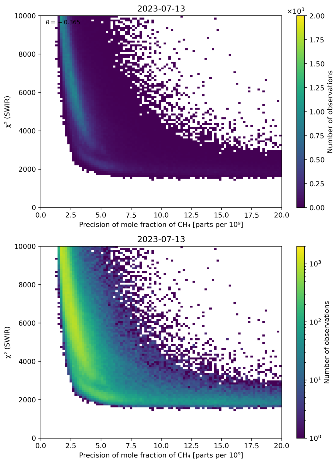
Figure 79: Scatter density plot of “Precision of mole fraction of CH 4 ” against “ \chi^2 (SWIR)” for 2023-07-13 to 2023-07-14.
