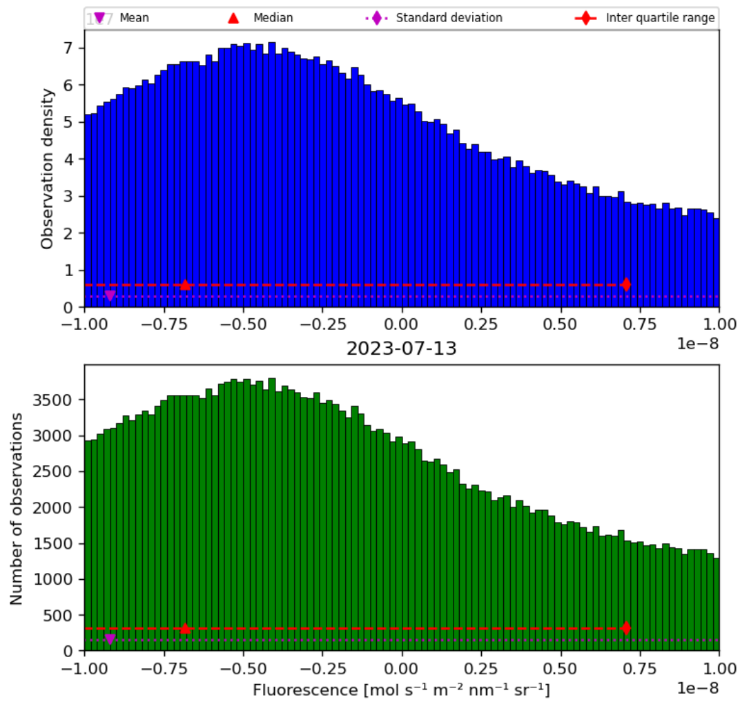
Figure 32: Histogram of “Fluorescence” for 2023-07-13 to 2023-07-14
