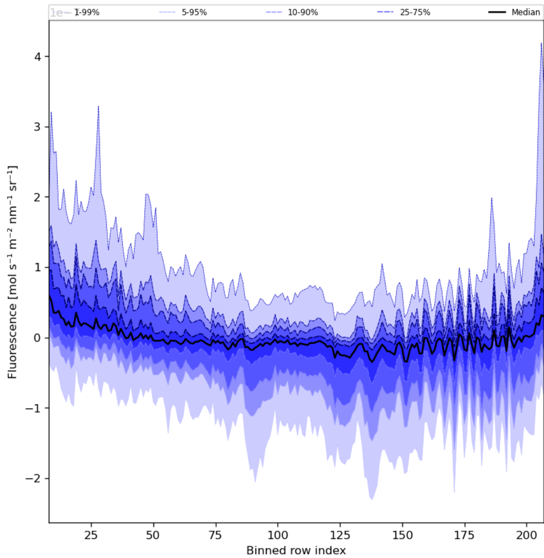
Figure 43: Along track statistics of “Fluorescence” for 2023-07-13 to 2023-07-14
