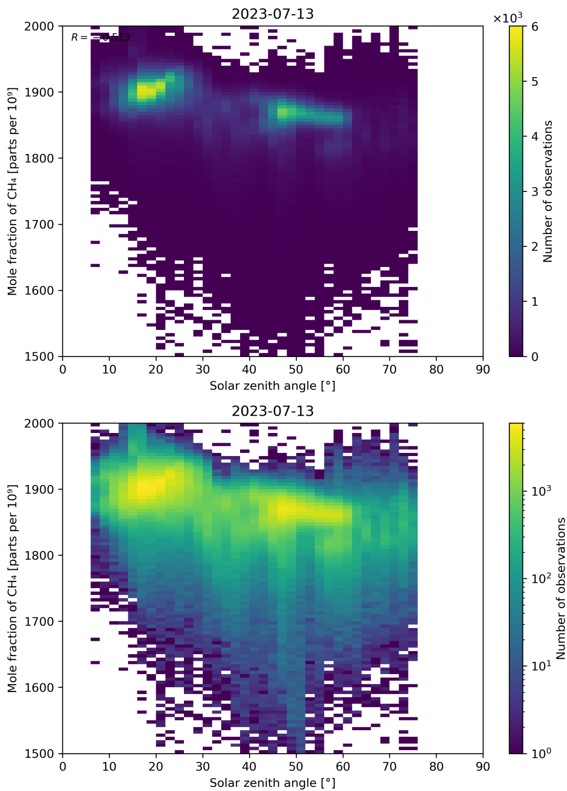
Figure 99: Scatter density plot of “Solar zenith angle” against “Mole fraction of CH 4 ” for 2023-07-13 to 2023-07-14.
