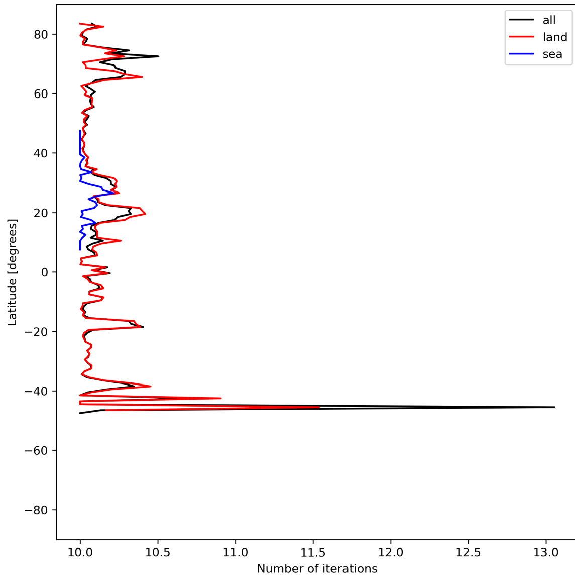
Figure 20: Zonal average of “Number of iterations” for 2023-07-13 to 2023-07-14.
