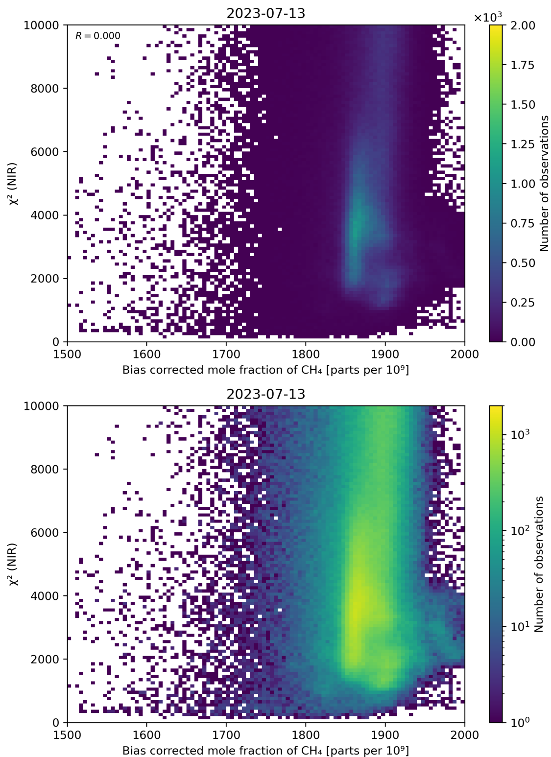
Figure 63: Scatter density plot of “Bias corrected mole fraction of CH 4 ” against “ \chi^2 (NIR)” for 2023-07-13 to 2023-07-14.
