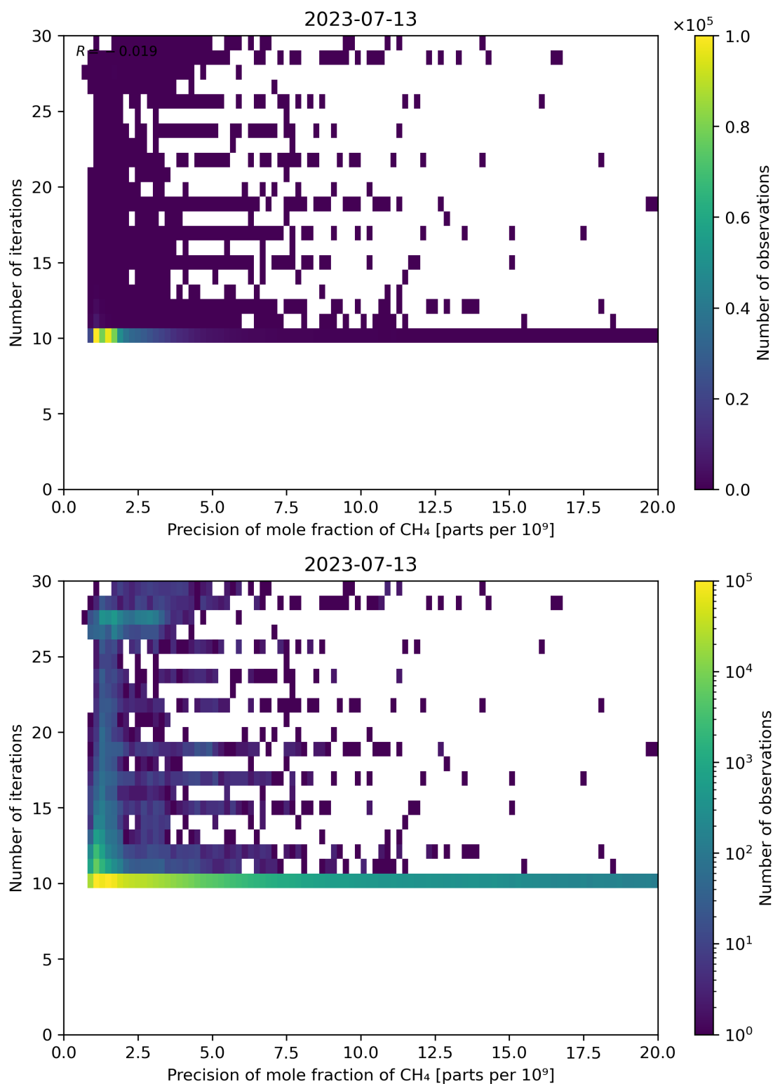
Figure 83: Scatter density plot of “Precision of mole fraction of CH 4 ” against “Number of iterations” for 2023-07-13 to 2023-07-14.
