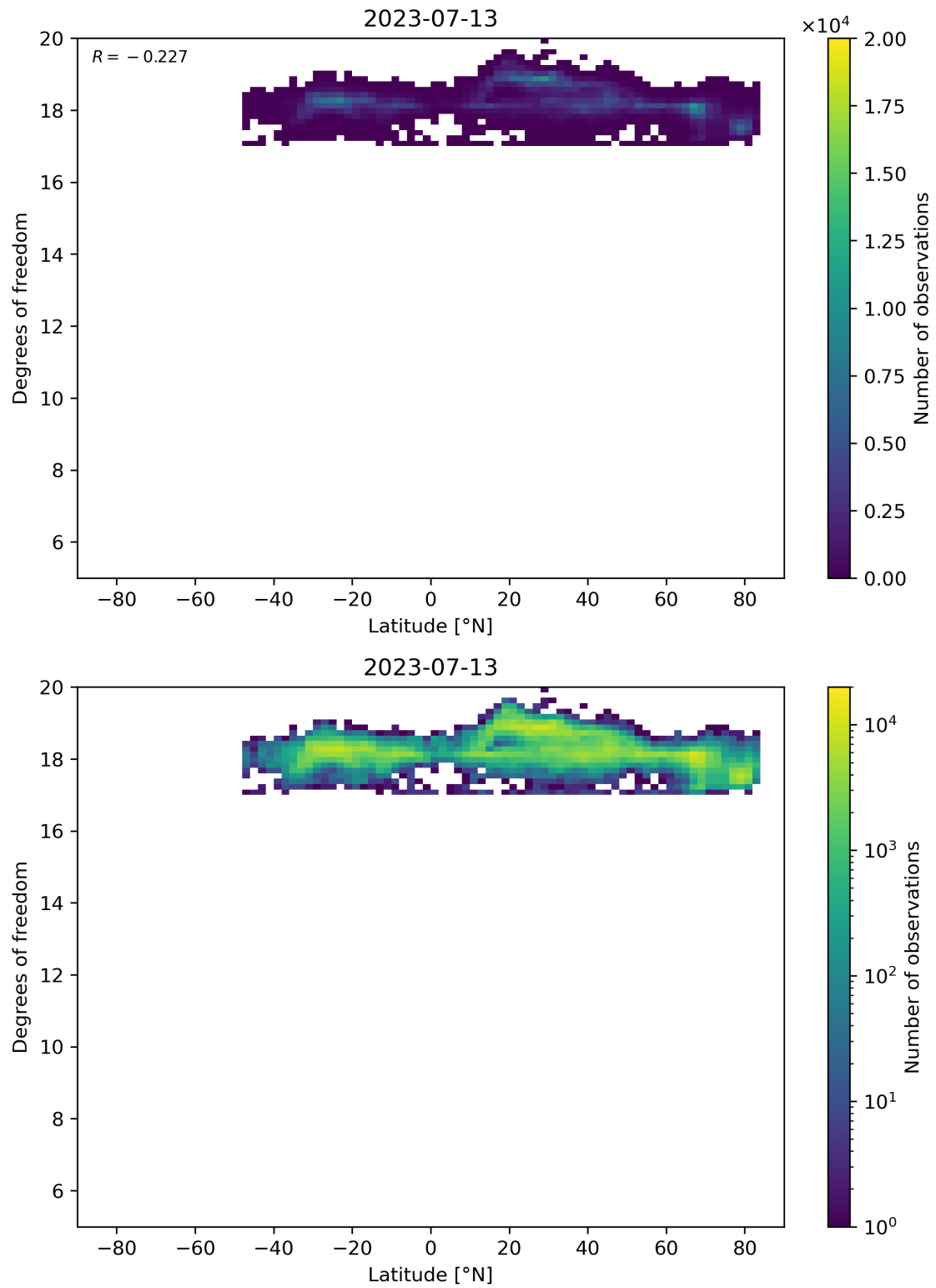
Figure 55: Scatter density plot of “Latitude” against “Degrees of freedom” for 2023-07-13 to 2023-07-14.
