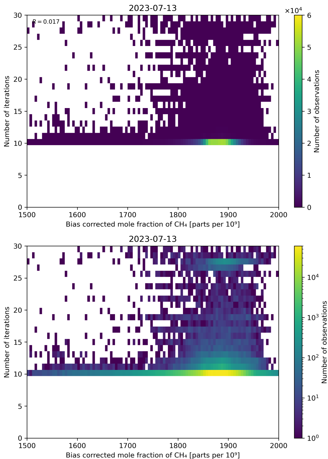
Figure 67: Scatter density plot of “Bias corrected mole fraction of CH 4 ” against “Number of iterations” for 2023-07-13 to 2023-07-14.
