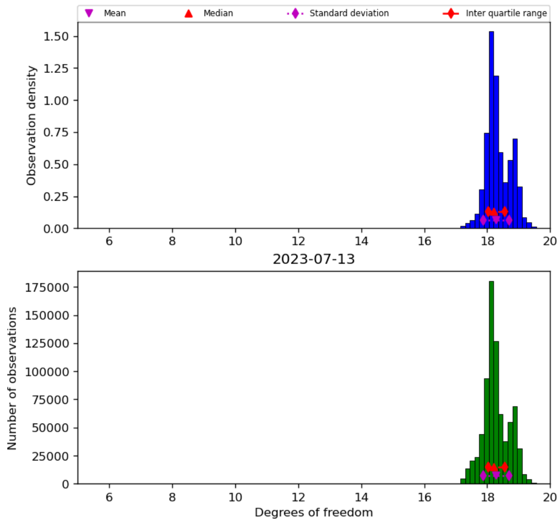
Figure 30: Histogram of “Degrees of freedom” for 2023-07-13 to 2023-07-14
