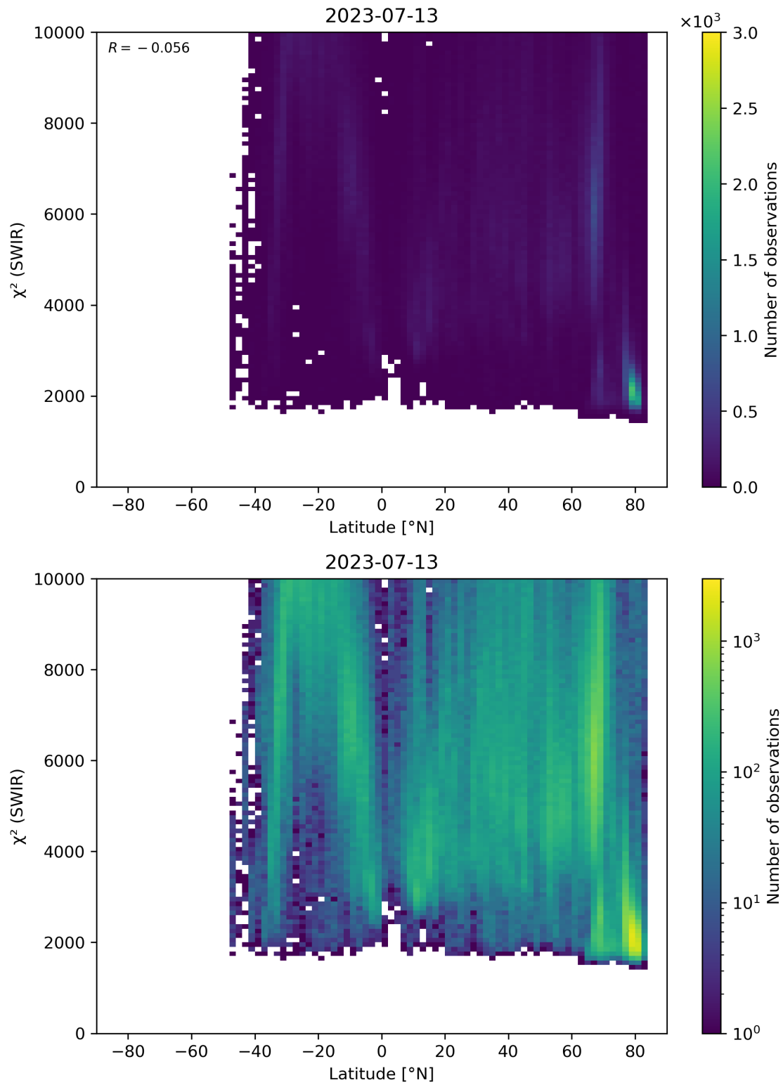
Figure 54: Scatter density plot of “Latitude” against “ \chi^2 (SWIR)” for 2023-07-13 to 2023-07-14.
