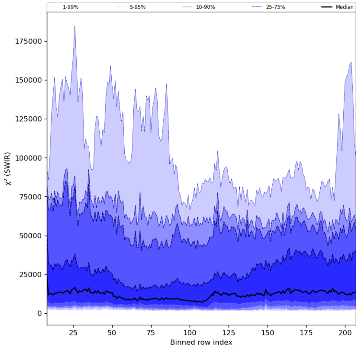
Figure 39: Along track statistics of “ \chi^2 (SWIR)” for 2023-07-13 to 2023-07-14
