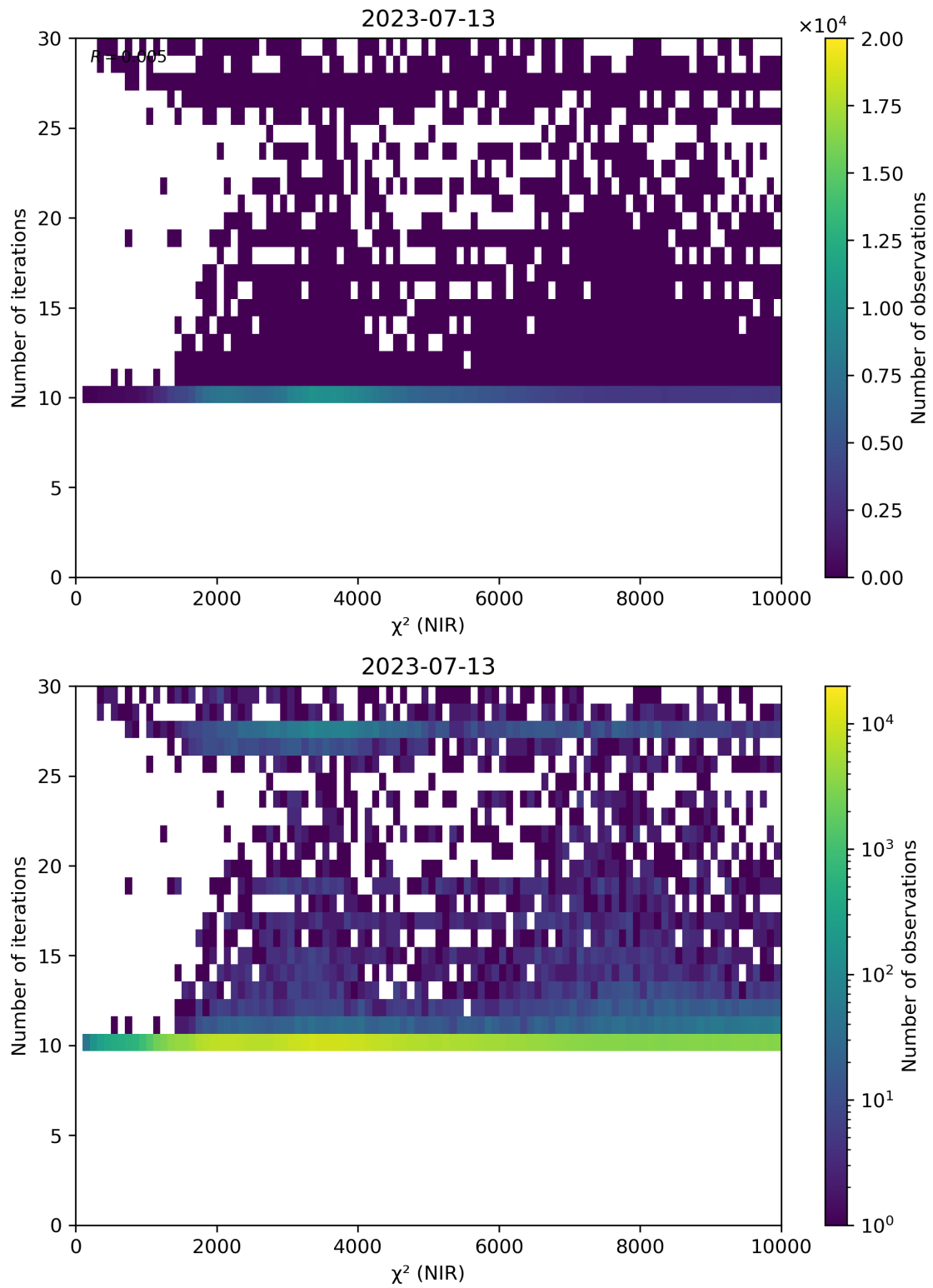
Figure 46: Scatter density plot of “ \chi^2 (NIR)” against “Number of iterations” for 2023-07-13 to 2023-07-14.
