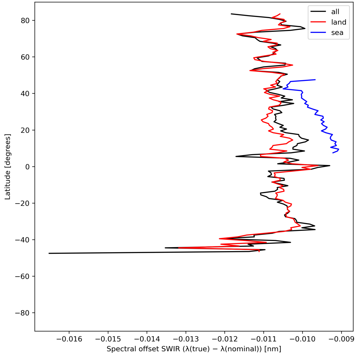
Figure 16: Zonal average of “Spectral offset SWIR ( \lambda(\text{true}) - \lambda(\text{nominal}) )” for 2023-07-13 to 2023-07-14.
