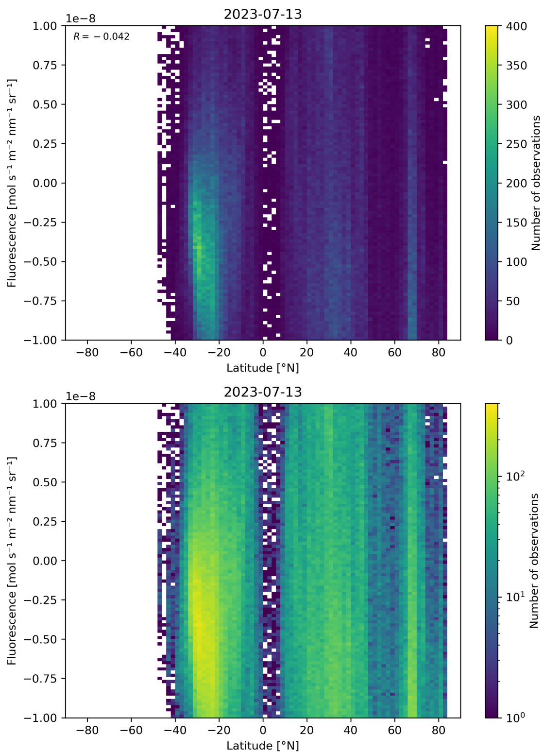
Figure 56: Scatter density plot of “Latitude” against “Fluorescence” for 2023-07-13 to 2023-07-14.
