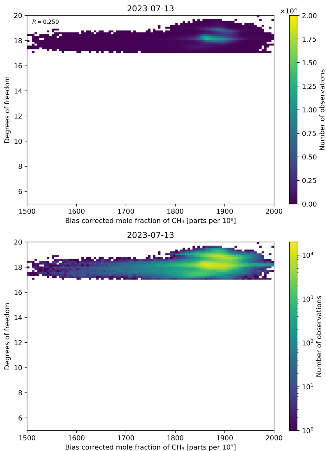
Figure 65: Scatter density plot of “Bias corrected mole fraction of CH 4 ” against “Degrees of freedom” for 2023-07-13 to 2023-07-14.
