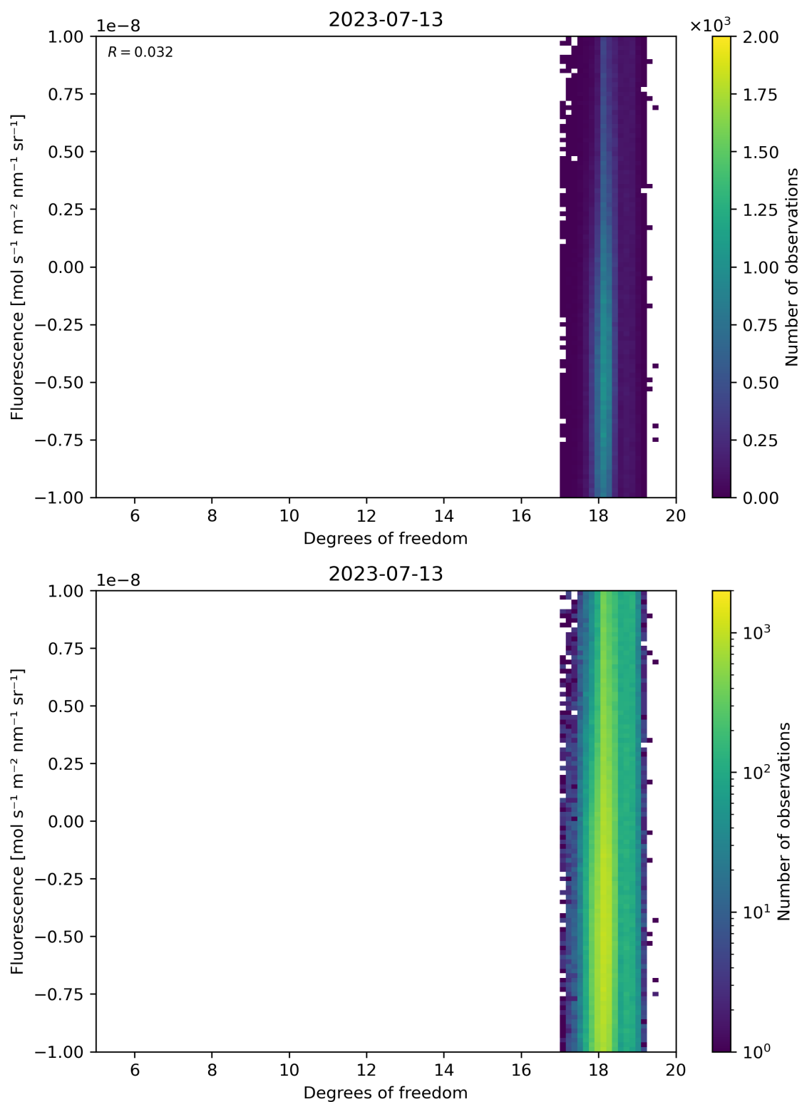
Figure 51: Scatter density plot of “Degrees of freedom” against “Fluorescence” for 2023-07-13 to 2023-07-14.
