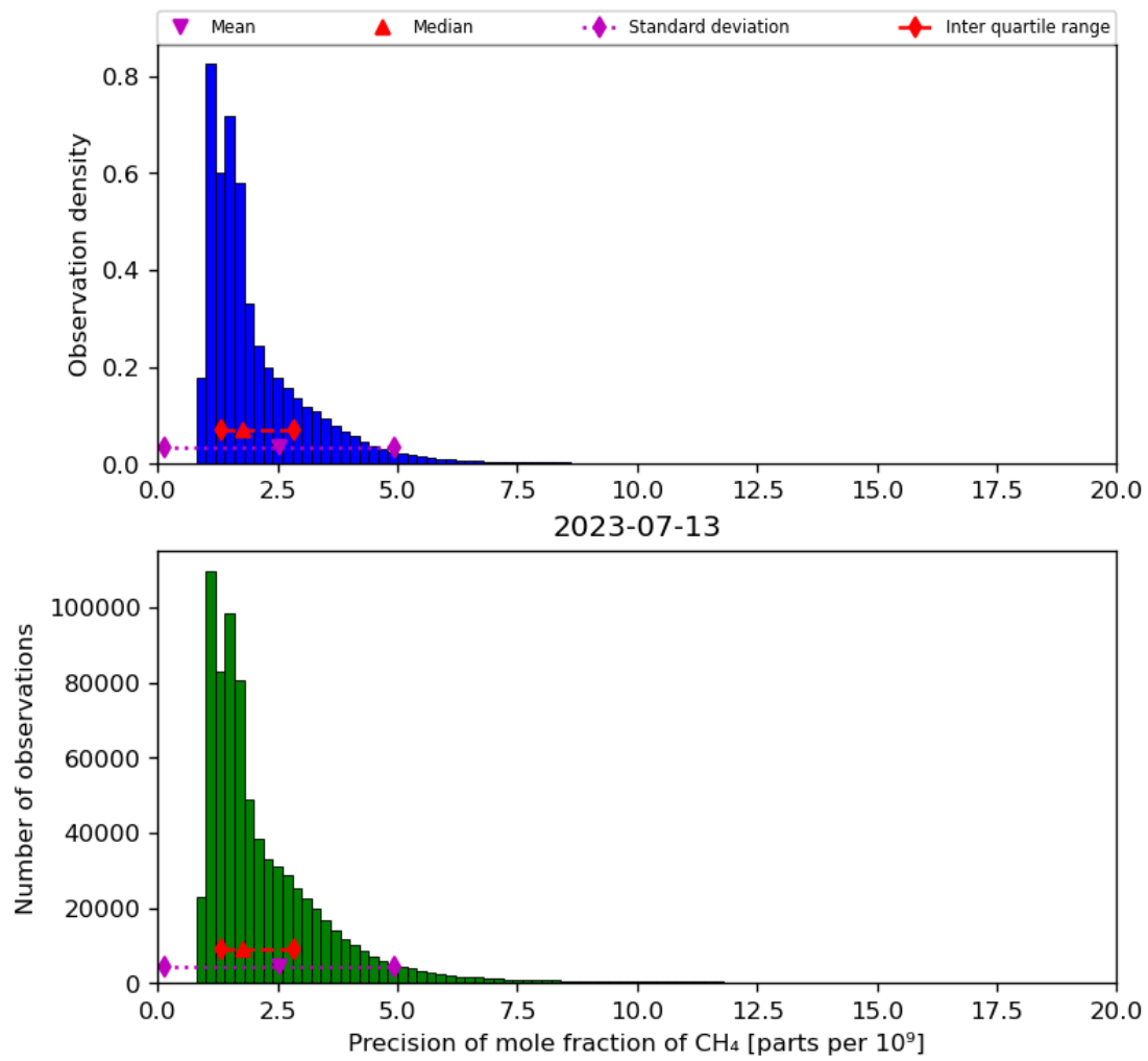
Figure 24: Histogram of “Precision of mole fraction of CH 4 ” for 2023-07-13 to 2023-07-14
