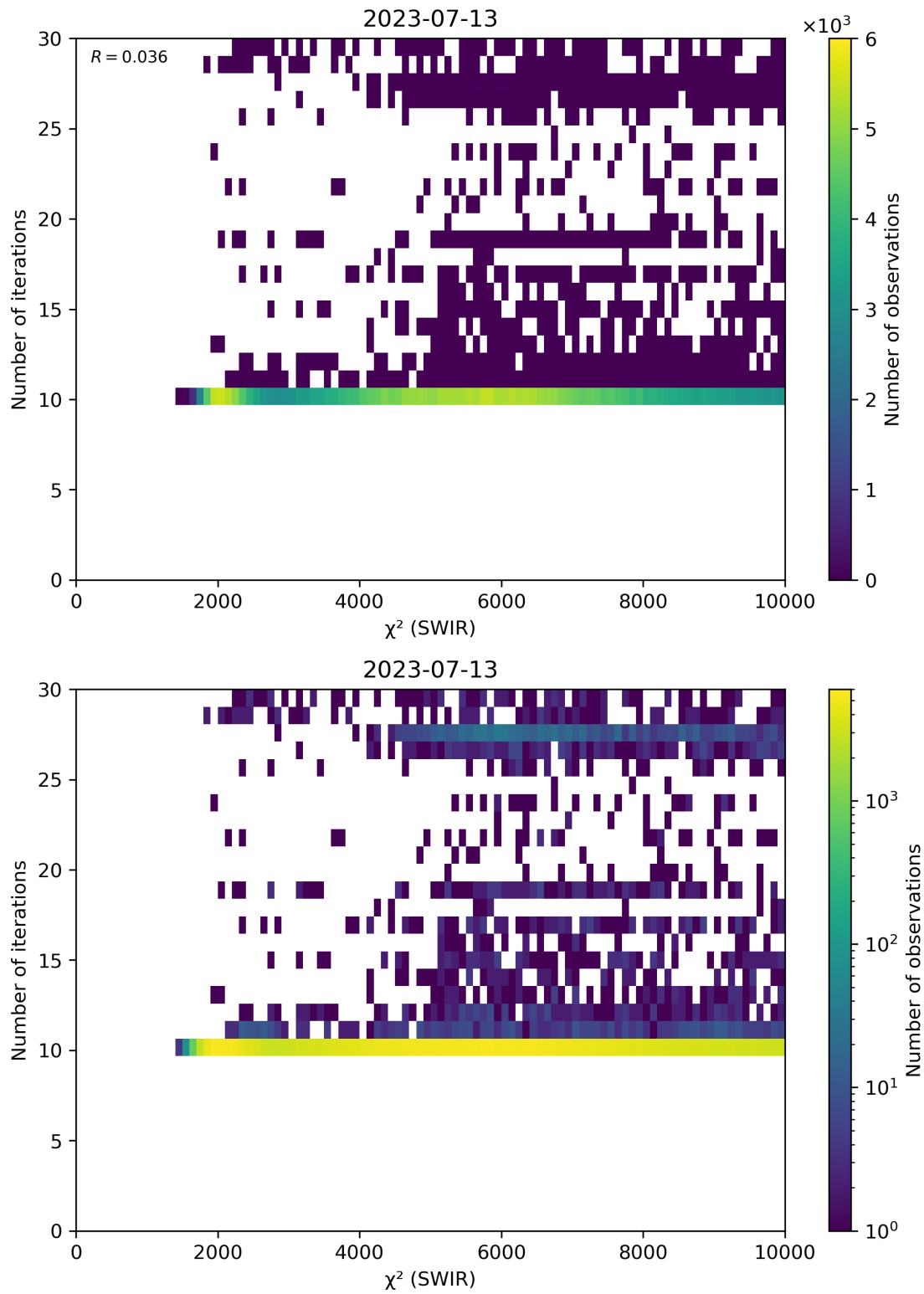
Figure 50: Scatter density plot of “ \chi^2 (SWIR)” against “Number of iterations” for 2023-07-13 to 2023-07-14.
