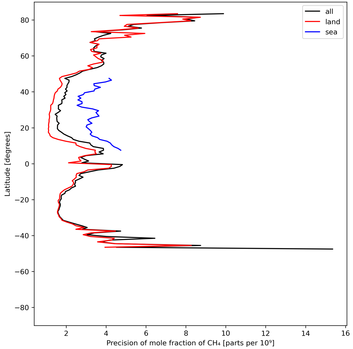
Figure 13: Zonal average of “Precision of mole fraction of CH 4 ” for 2023-07-13 to 2023-07-14.
