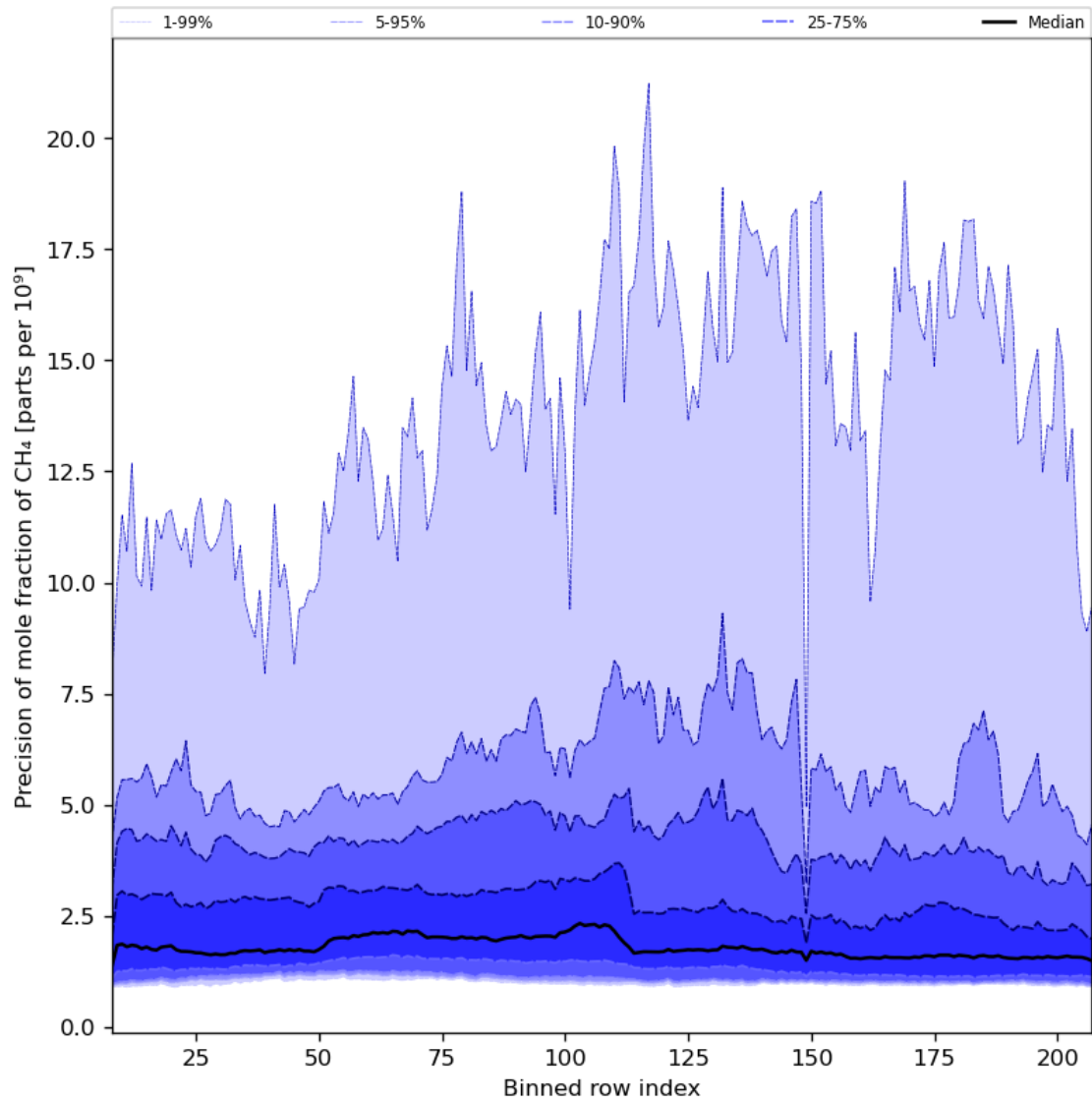
Figure 35: Along track statistics of “Precision of mole fraction of CH 4 ” for 2023-07-13 to 2023-07-14
