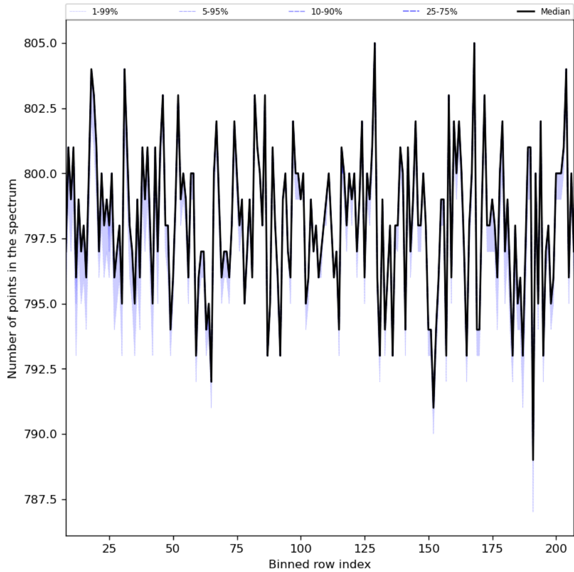
Figure 37: Along track statistics of “Number of points in the spectrum” for 2023-07-13 to 2023-07-14
