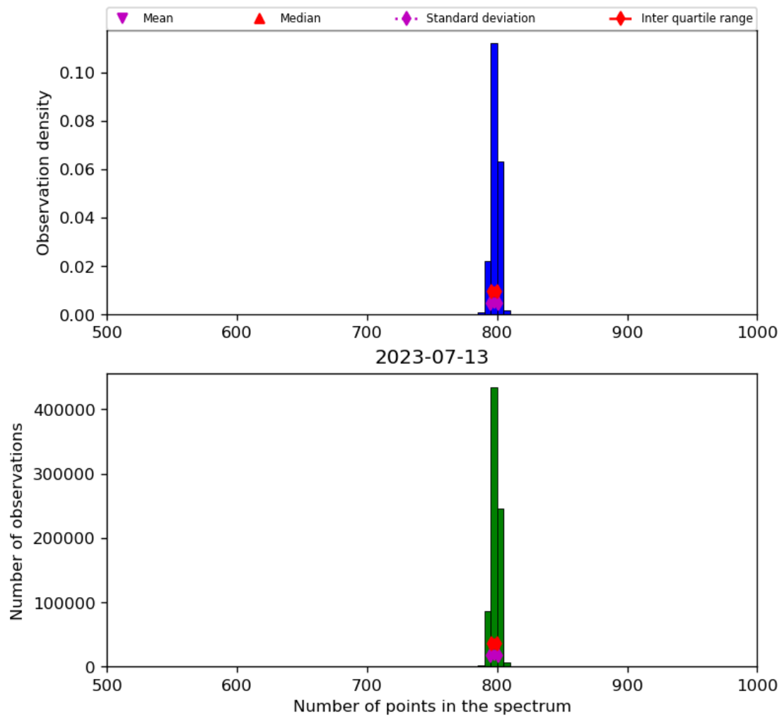
Figure 26: Histogram of “Number of points in the spectrum” for 2023-07-13 to 2023-07-14
