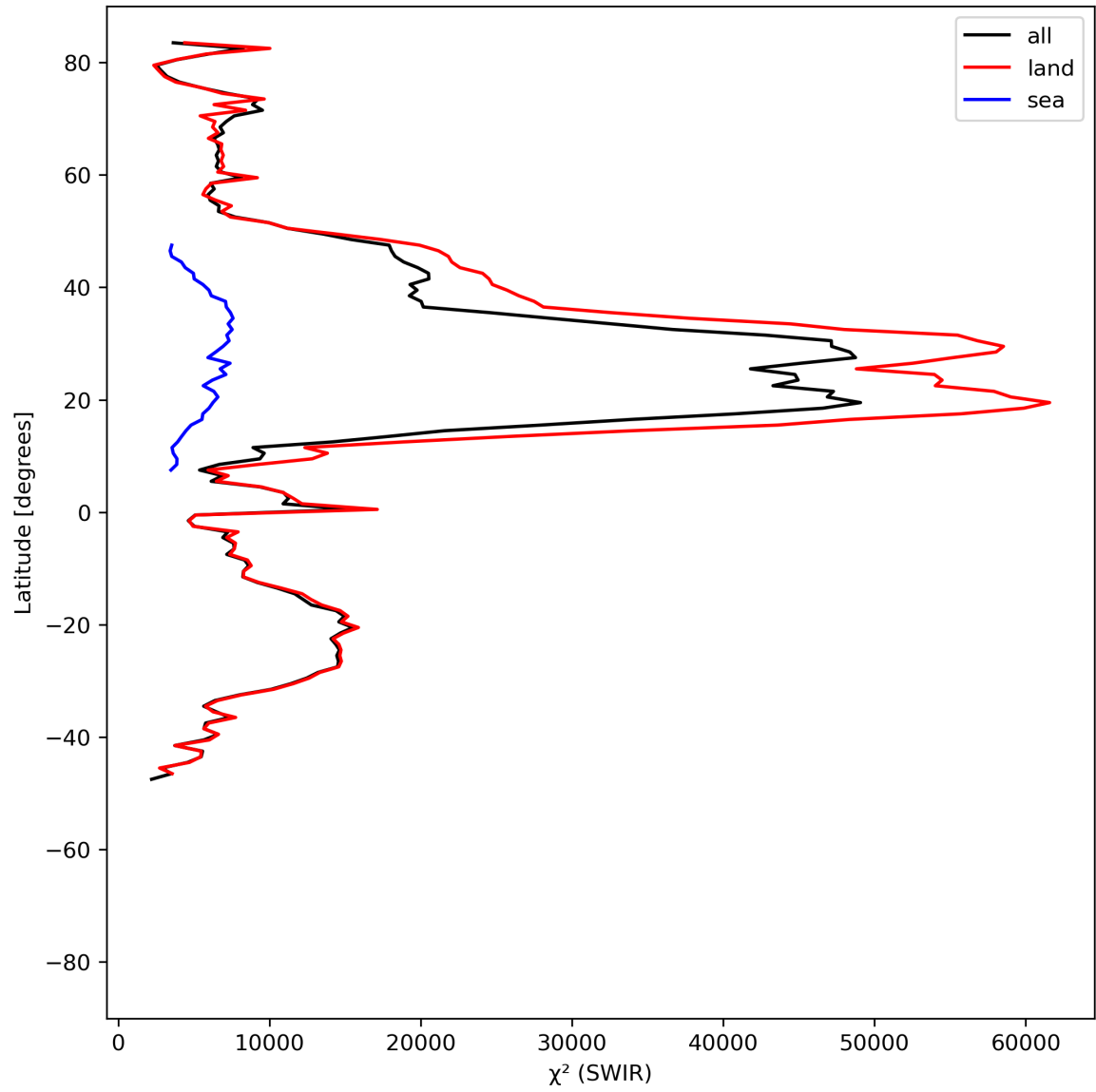
Figure 17: Zonal average of “ \chi^2 (SWIR)” for 2023-07-13 to 2023-07-14.
