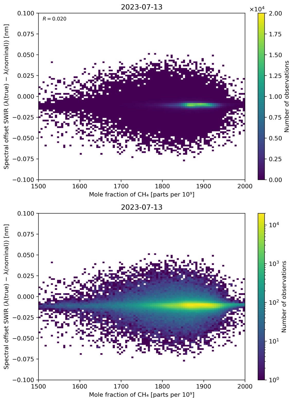
Figure 86: Scatter density plot of “Mole fraction of CH 4 ” against “Spectral offset SWIR ( \lambda(\text{true}) - \lambda(\text{nominal}) )” for 2023-07-13 to 2023-07-14.
