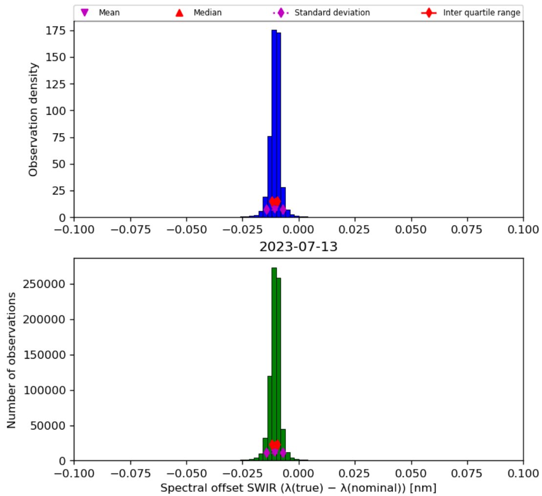
Figure 27: Histogram of “Spectral offset SWIR ( \lambda(\text{true}) - \lambda(\text{nominal}) )” for 2023-07-13 to 2023-07-14
