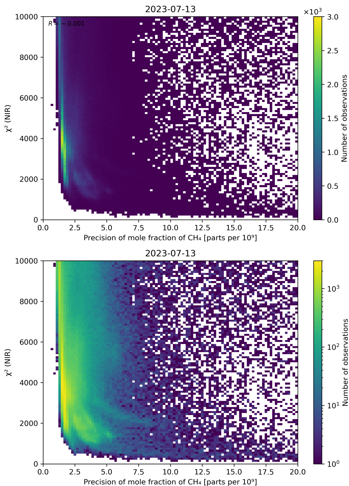
Figure 78: Scatter density plot of “Precision of mole fraction of CH 4 ” against “ \chi^2 (NIR)” for 2023-07-13 to 2023-07-14.
