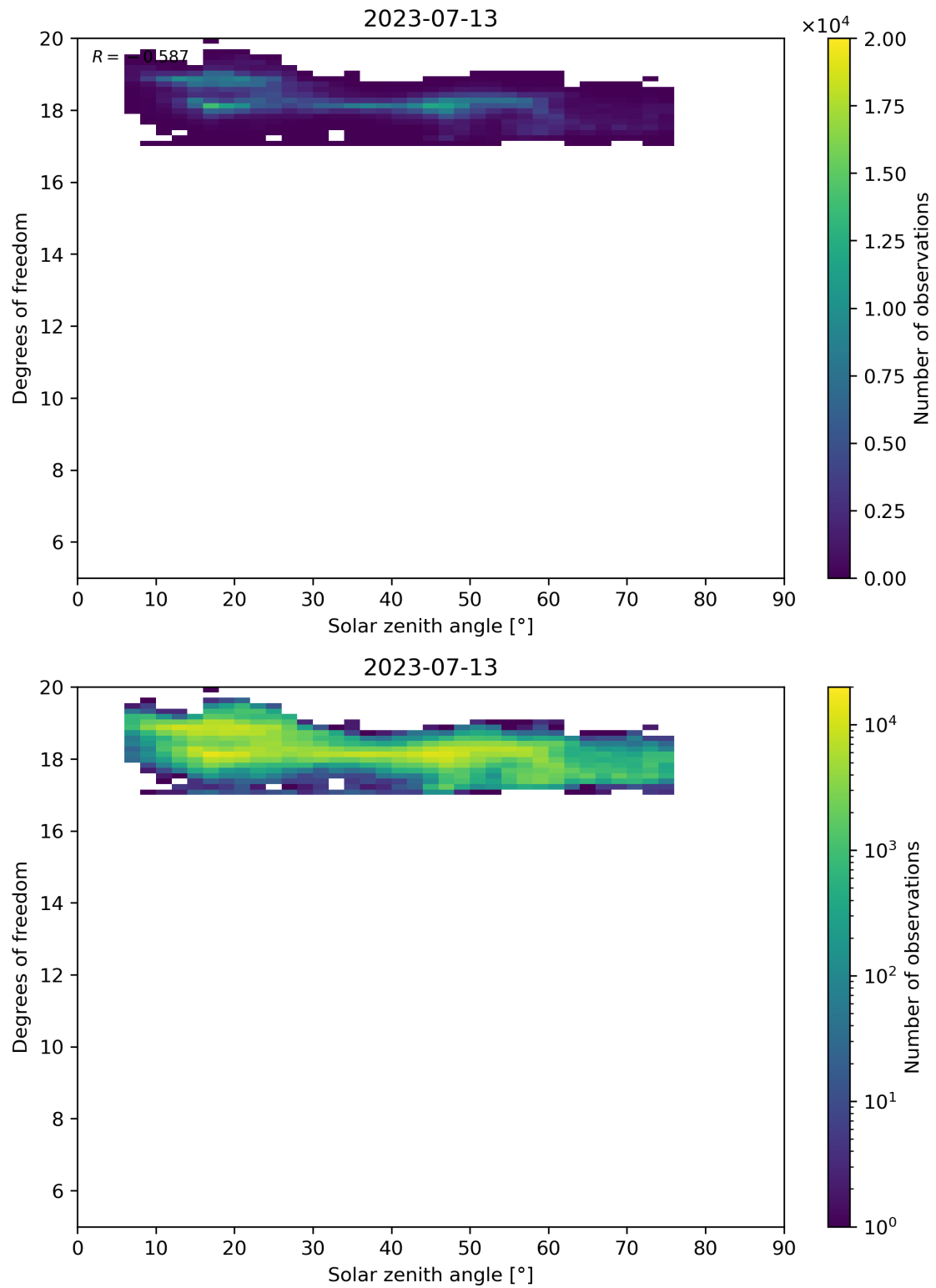
Figure 96: Scatter density plot of “Solar zenith angle” against “Degrees of freedom” for 2023-07-13 to 2023-07-14.
