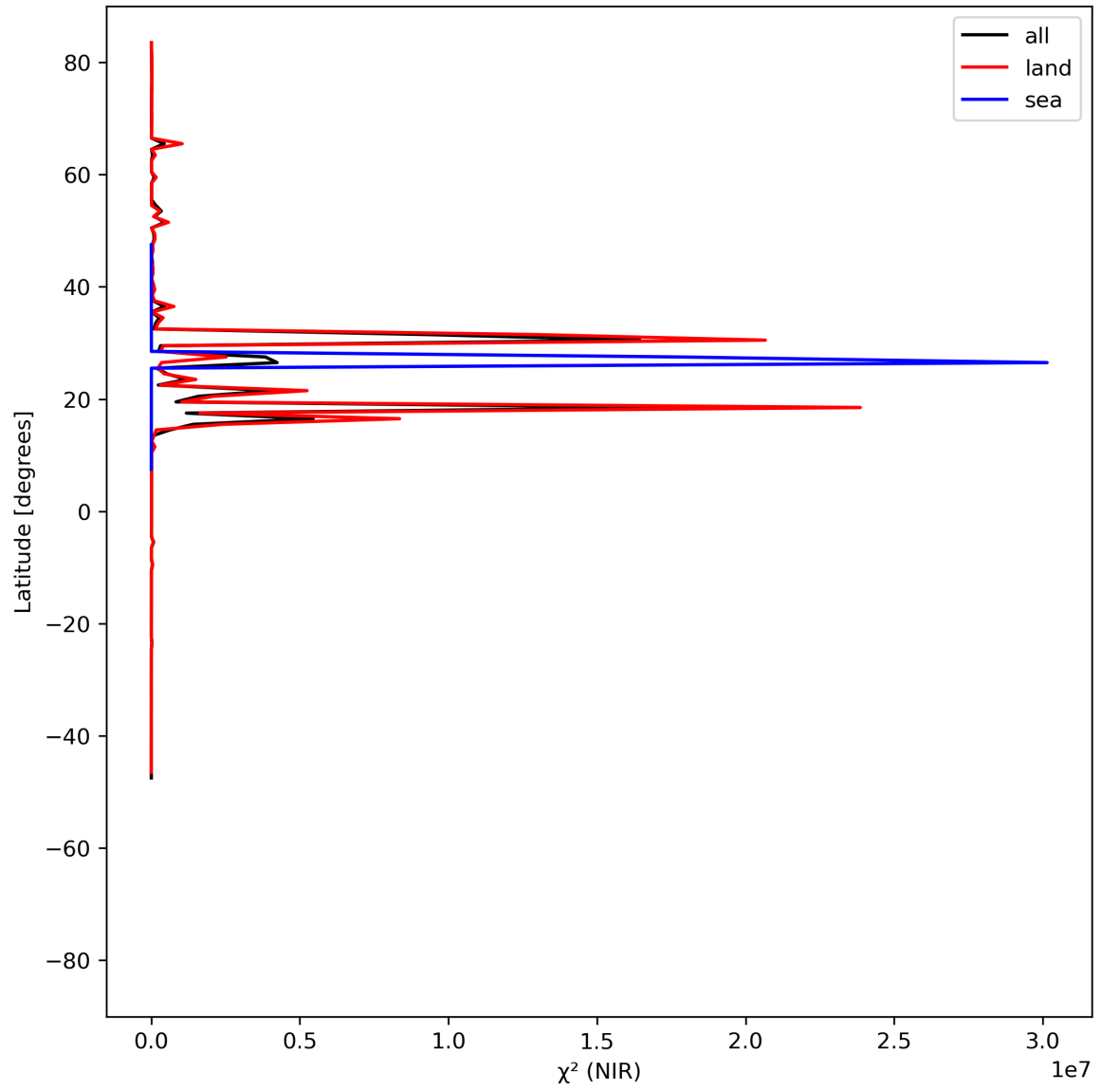
Figure 18: Zonal average of “ \chi^2 (NIR)” for 2023-07-13 to 2023-07-14.
