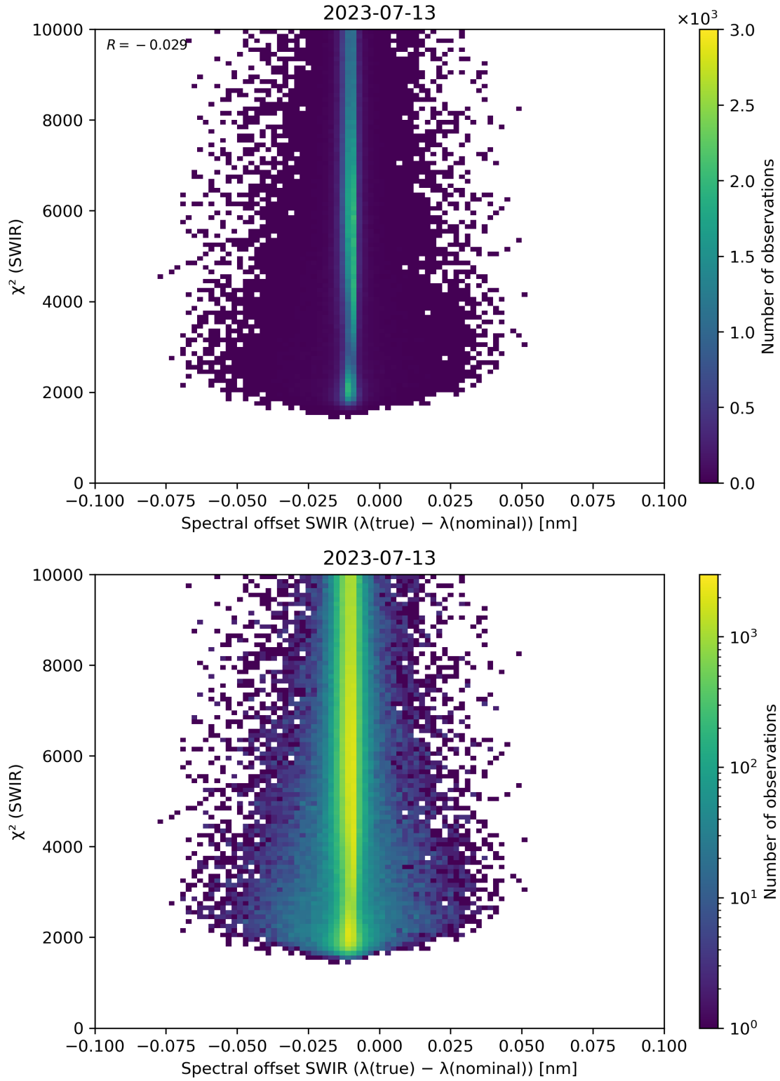
Figure 118: Scatter density plot of “Spectral offset SWIR ( \lambda(\text{true}) - \lambda(\text{nominal}) )” against “ \chi^2 (SWIR)” for 2023-07-13 to 2023-07-14.
