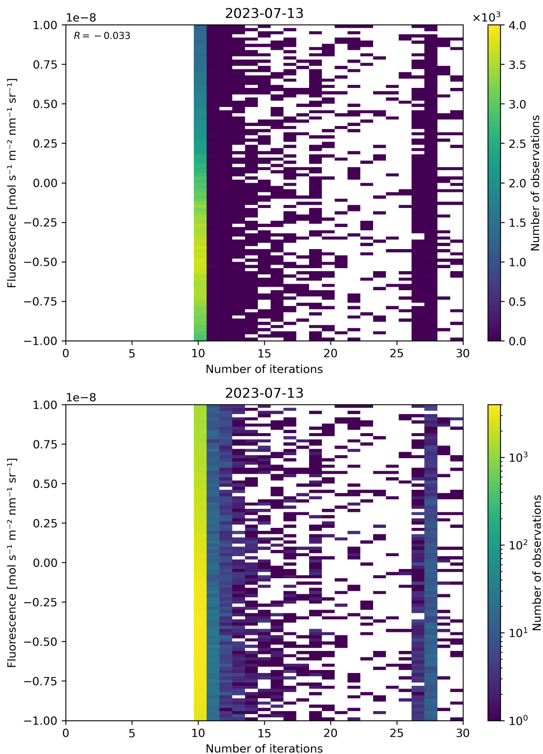
Figure 87: Scatter density plot of “Number of iterations” against “Fluorescence” for 2023-07-13 to 2023-07-14.
