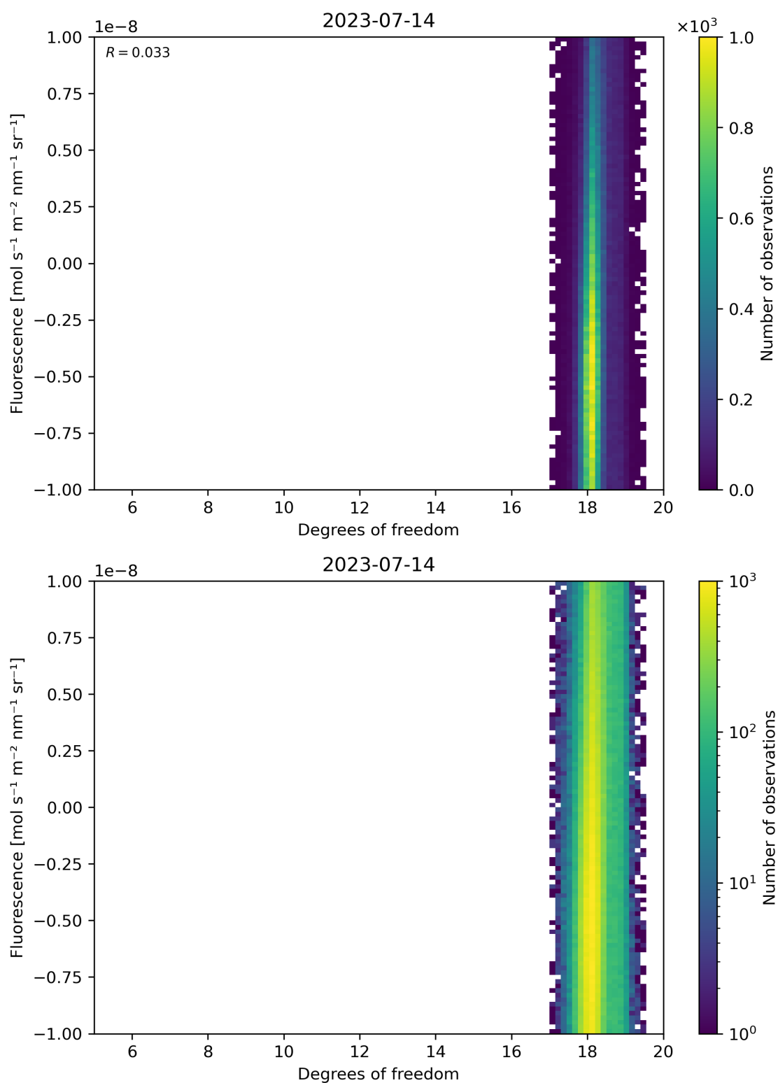
Figure 51: Scatter density plot of “Degrees of freedom” against “Fluorescence” for 2023-07-14 to 2023-07-15.
