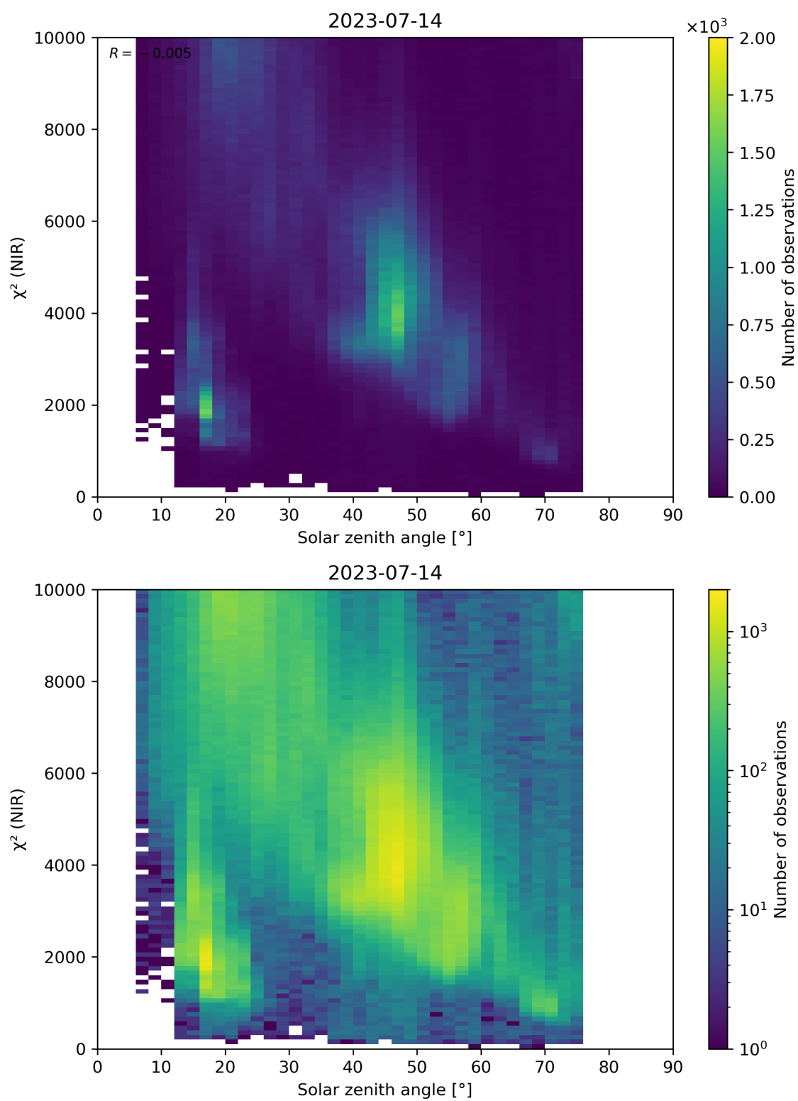
Figure 94: Scatter density plot of “Solar zenith angle” against “ \chi^2 (NIR)” for 2023-07-14 to 2023-07-15.
