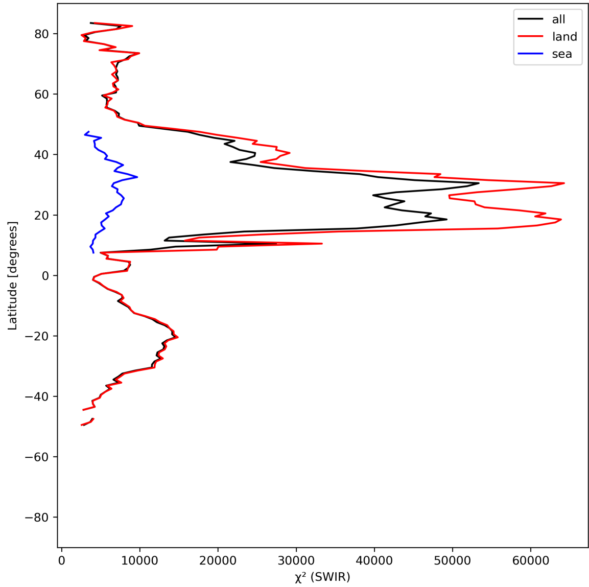
Figure 17: Zonal average of “ \chi^2 (SWIR)” for 2023-07-14 to 2023-07-15.
