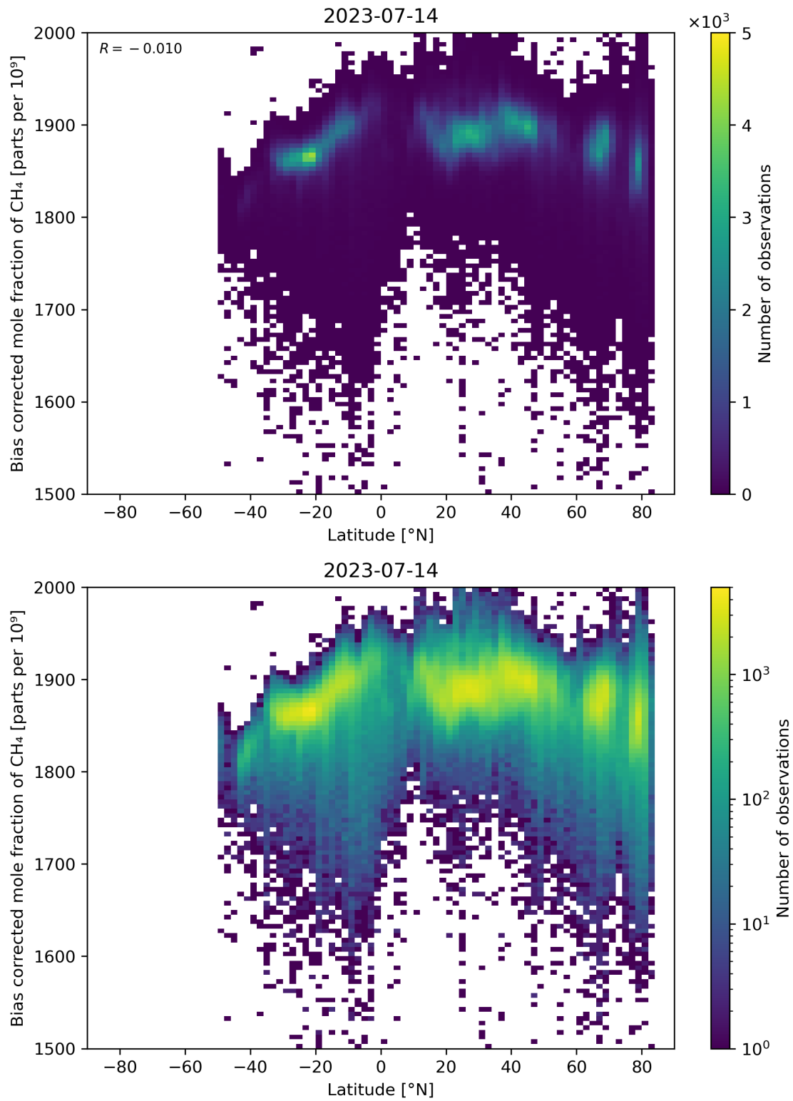
Figure 58: Scatter density plot of “Latitude” against “Bias corrected mole fraction of CH 4 ” for 2023-07-14 to 2023-07-15.
