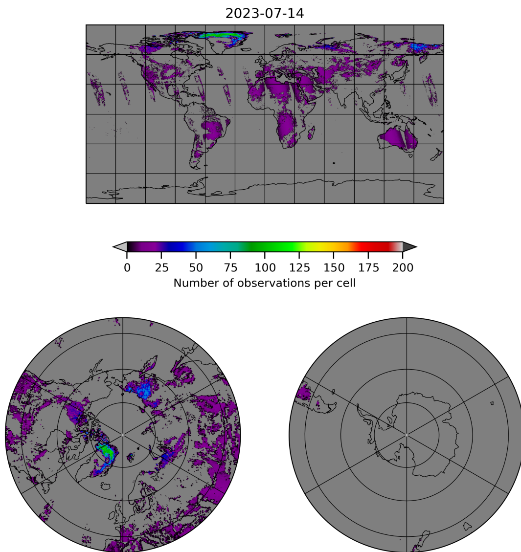
Figure 10: Map of the number of observations for 2023-07-14 to 2023-07-15
