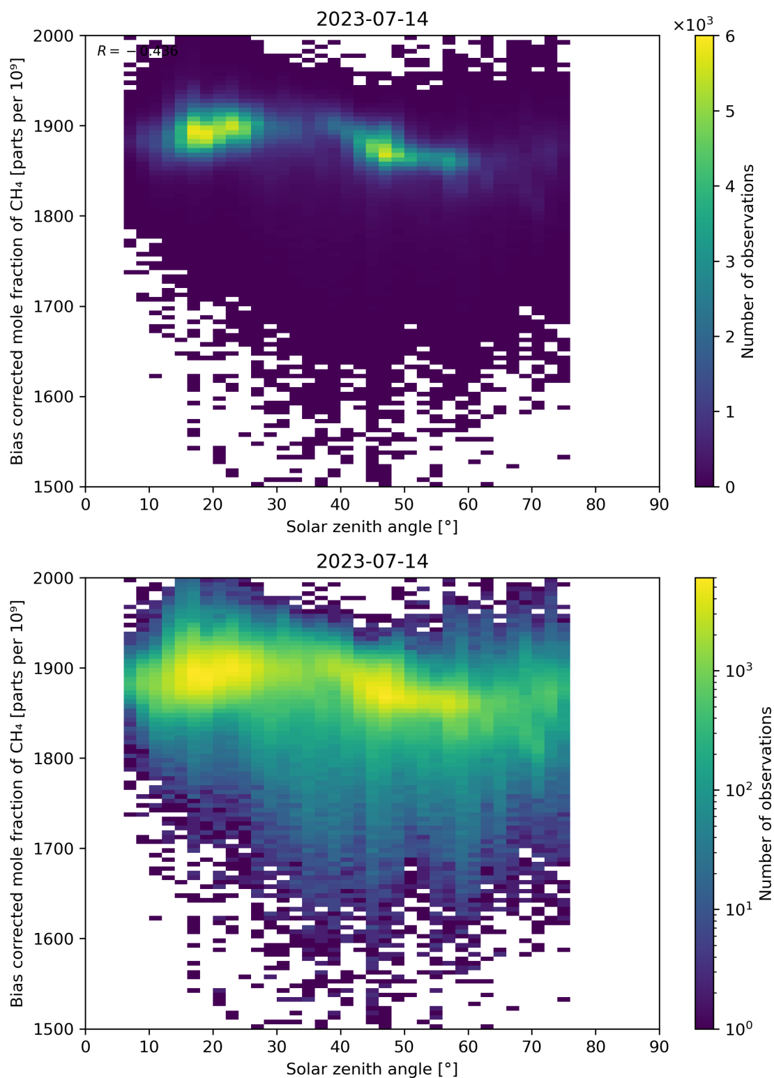
Figure 100: Scatter density plot of “Solar zenith angle” against “Bias corrected mole fraction of CH 4 ” for 2023-07-14 to 2023-07-15.
