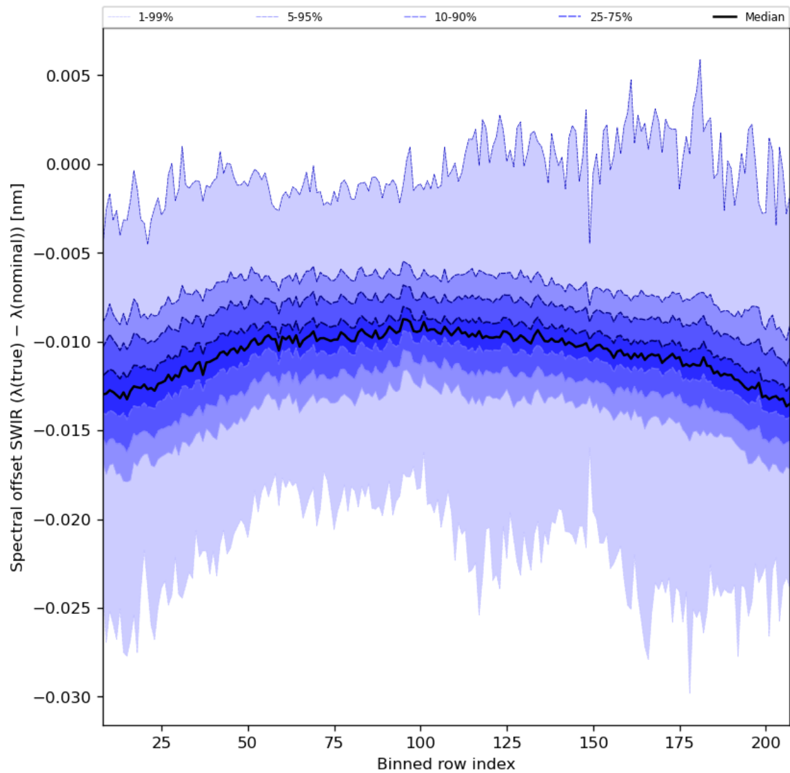
Figure 38: Along track statistics of “Spectral offset SWIR ( \lambda(\text{true}) - \lambda(\text{nominal}) )” for 2023-07-14 to 2023-07-15
