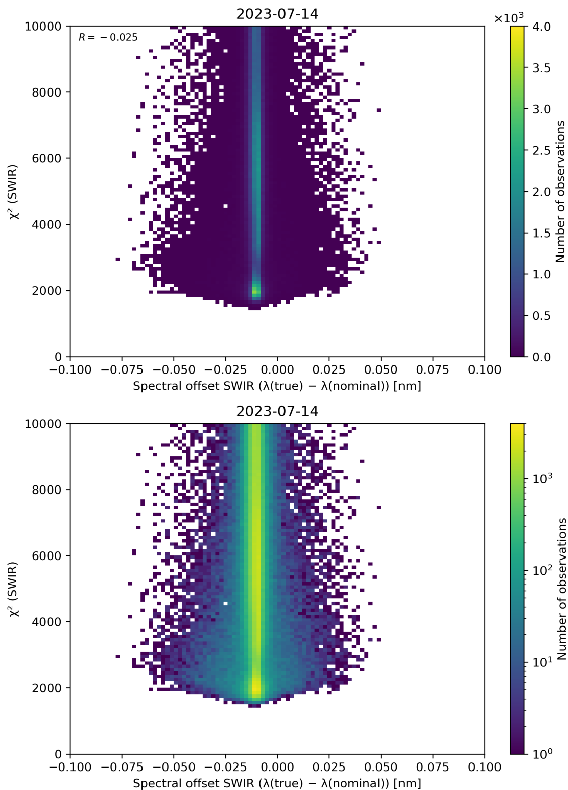
Figure 118: Scatter density plot of “Spectral offset SWIR ( \lambda(\text{true}) - \lambda(\text{nominal}) )” against “ \chi^2 (SWIR)” for 2023-07-14 to 2023-07-15.
