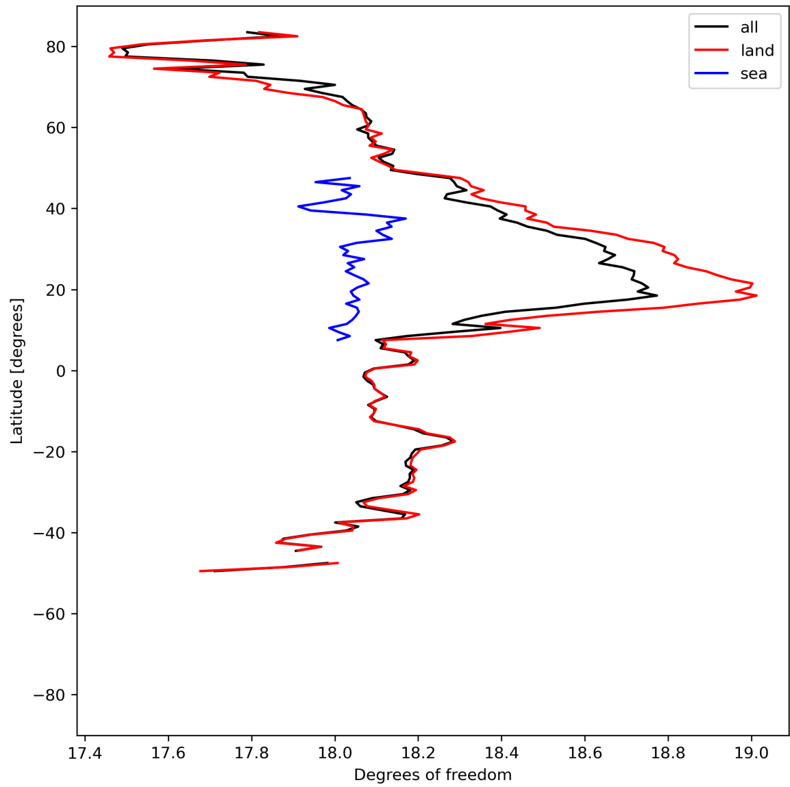
Figure 19: Zonal average of “Degrees of freedom” for 2023-07-14 to 2023-07-15.
