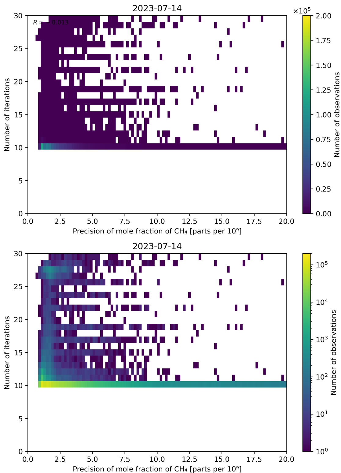
Figure 83: Scatter density plot of “Precision of mole fraction of CH 4 ” against “Number of iterations” for 2023-07-14 to 2023-07-15.
