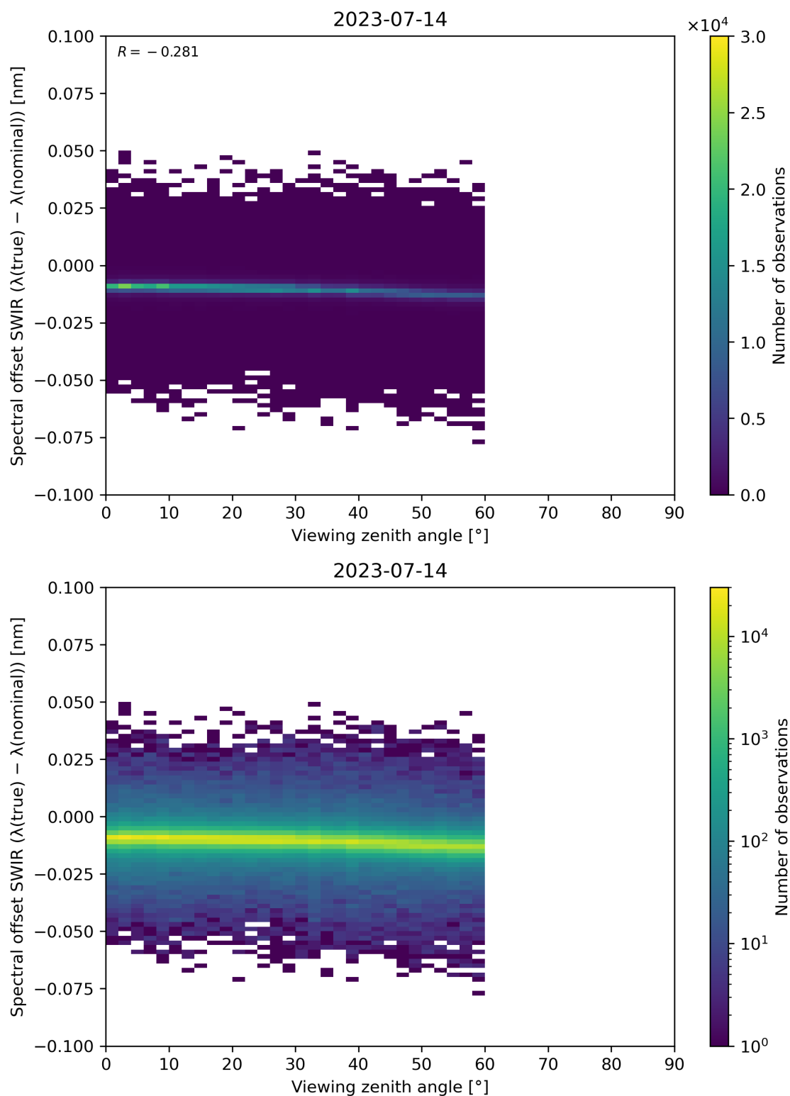
Figure 116: Scatter density plot of “Viewing zenith angle” against “Spectral offset SWIR ( \lambda(\text{true}) - \lambda(\text{nominal}) )” for 2023-07-14 to 2023-07-15.
