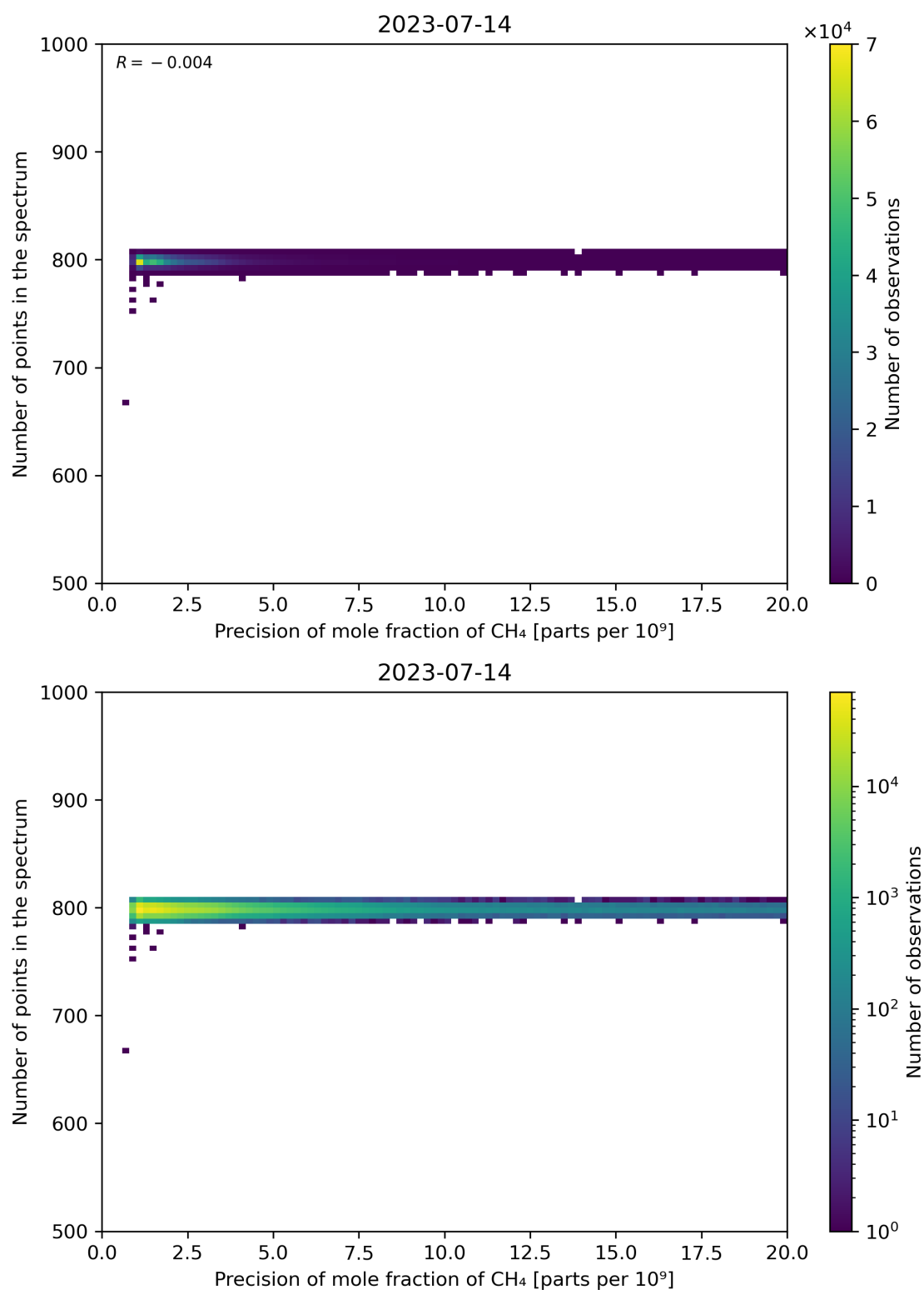
Figure 84: Scatter density plot of “Precision of mole fraction of CH 4 ” against “Number of points in the spectrum” for 2023-07-14 to 2023-07-15.
