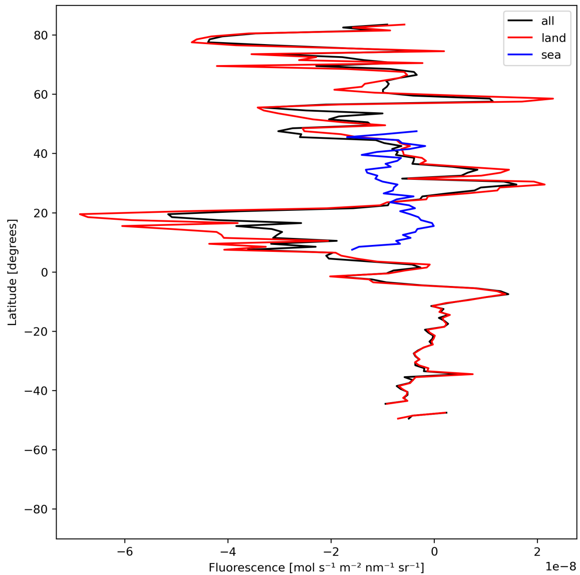
Figure 21: Zonal average of “Fluorescence” for 2023-07-14 to 2023-07-15.
