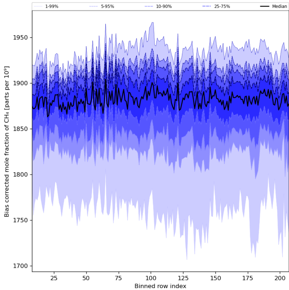
Figure 36: Along track statistics of “Bias corrected mole fraction of CH 4 ” for 2023-07-14 to 2023-07-15
