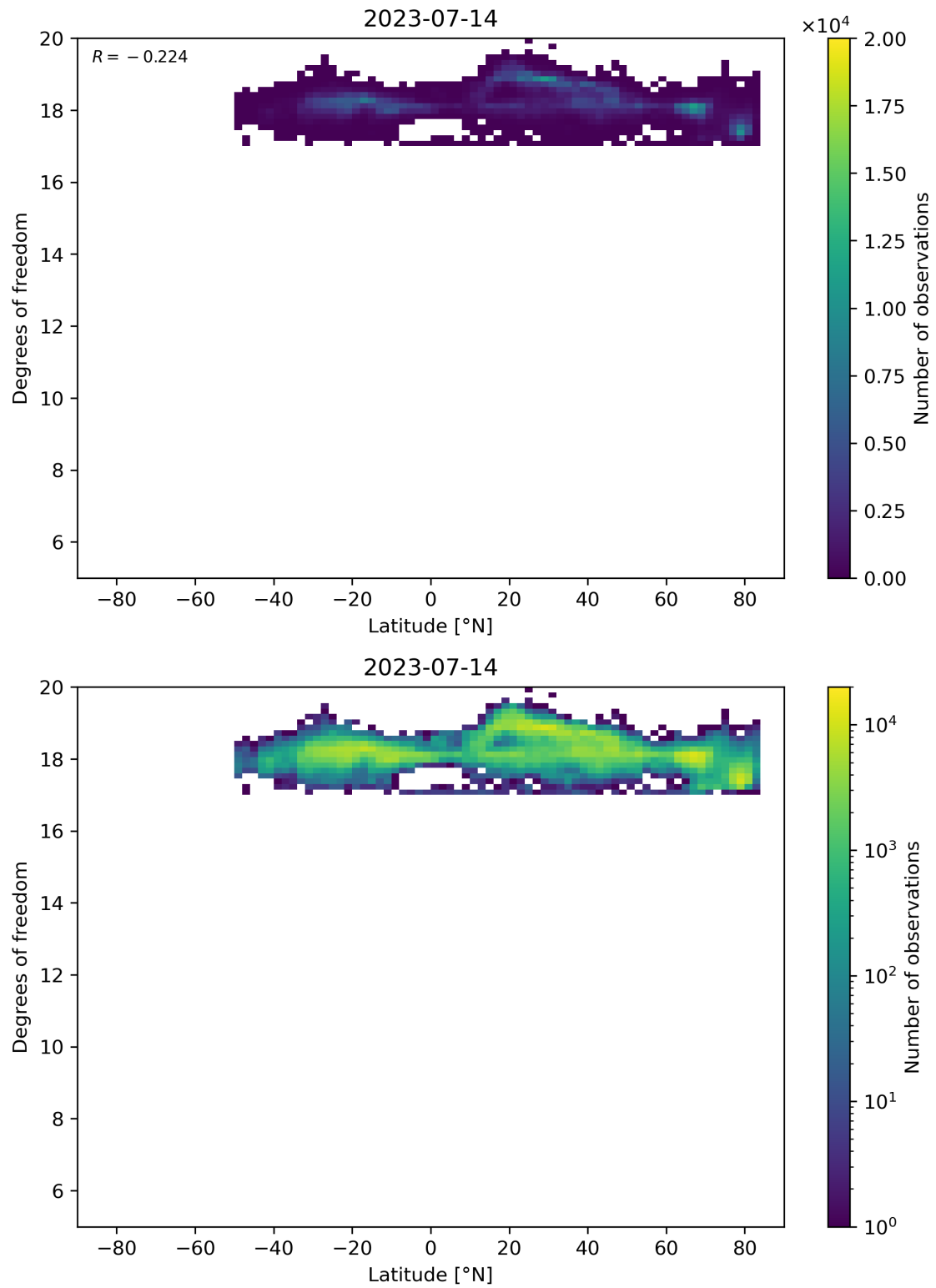
Figure 55: Scatter density plot of “Latitude” against “Degrees of freedom” for 2023-07-14 to 2023-07-15.
