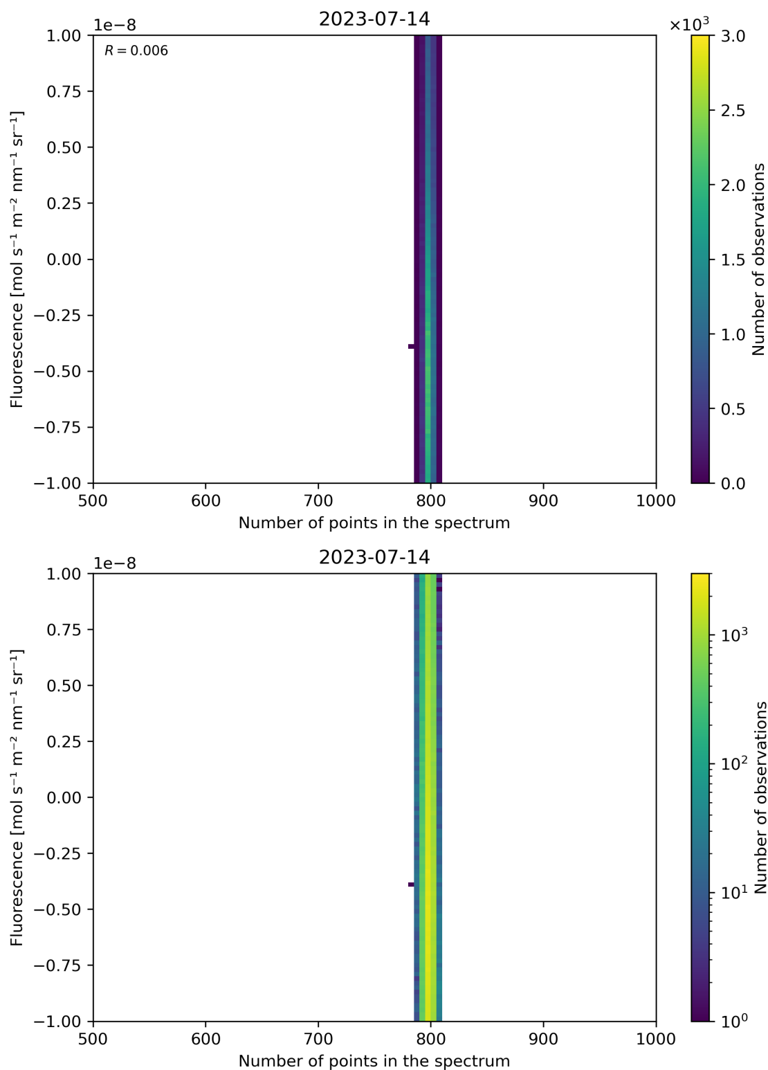
Figure 91: Scatter density plot of “Number of points in the spectrum” against “Fluorescence” for 2023-07-14 to 2023-07-15.
