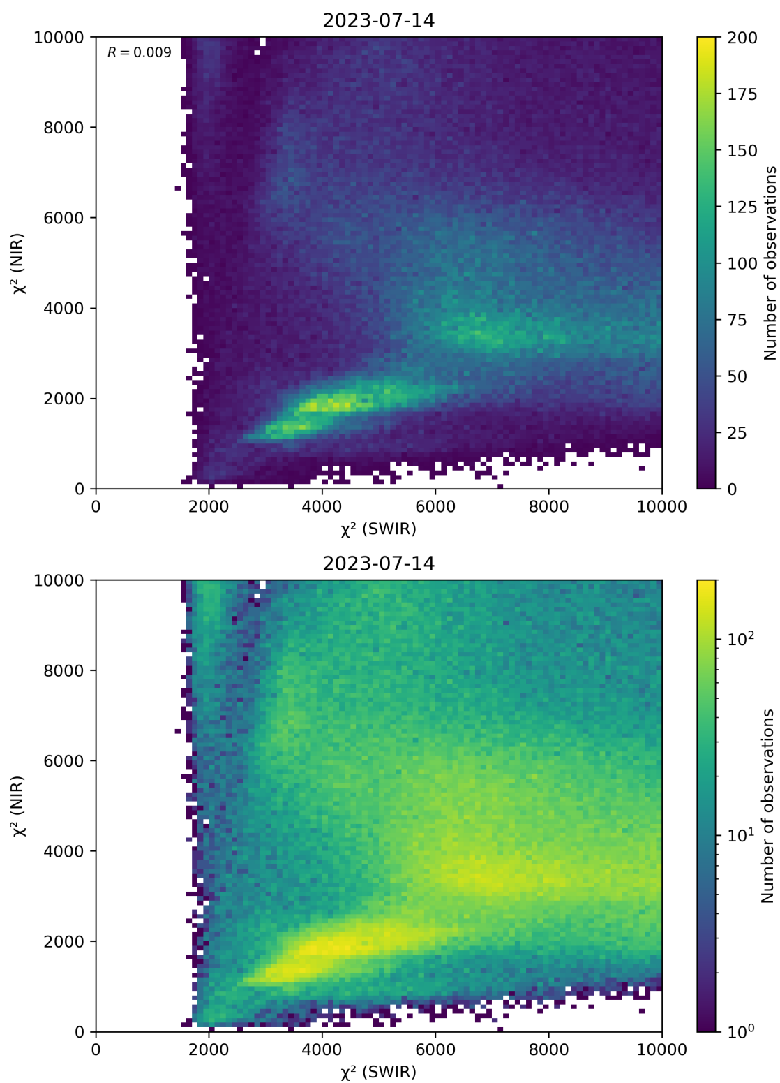
Figure 47: Scatter density plot of “ \chi^2 (SWIR)” against “ \chi^2 (NIR)” for 2023-07-14 to 2023-07-15.
