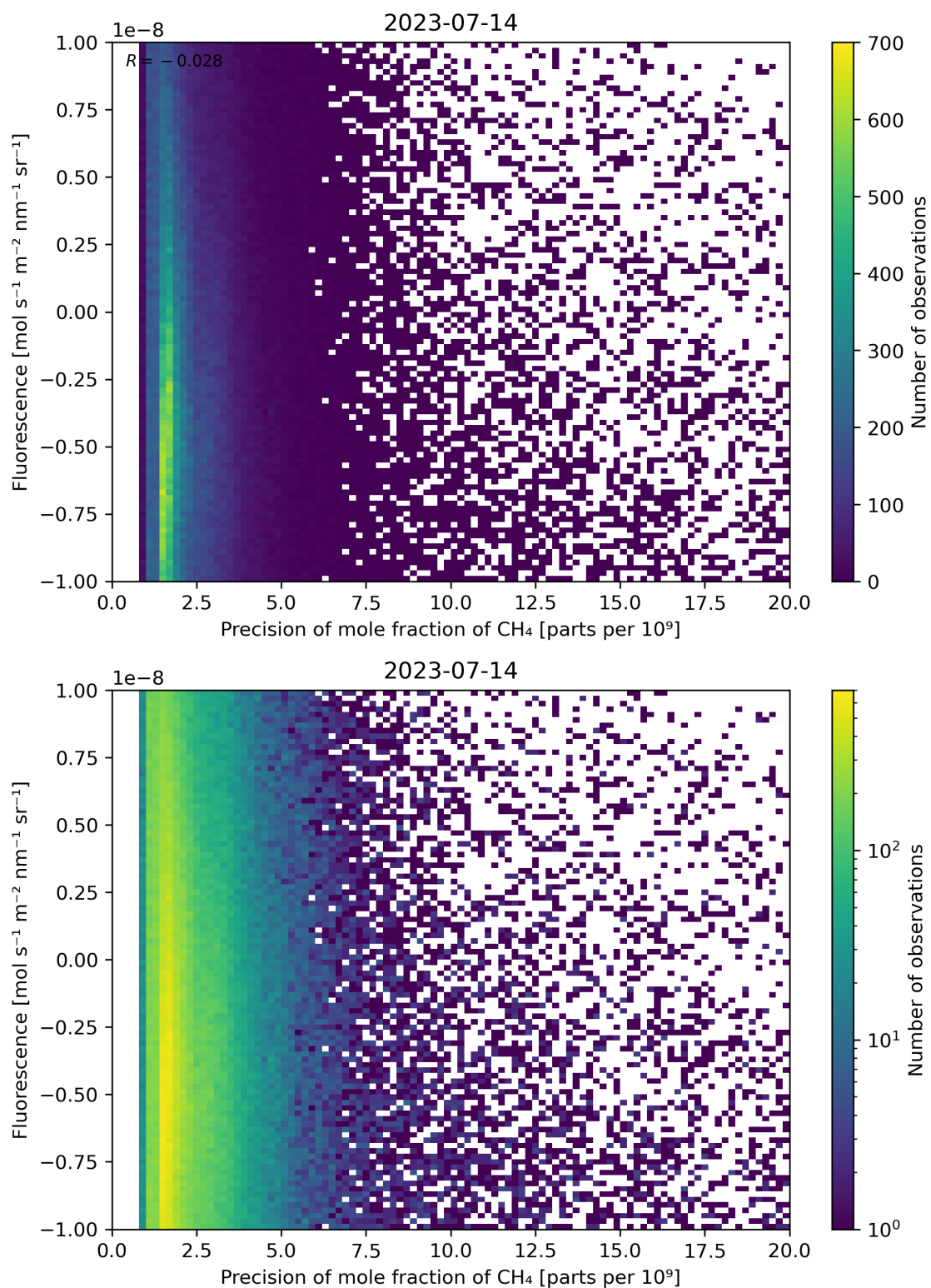
Figure 81: Scatter density plot of “Precision of mole fraction of CH 4 ” against “Fluorescence” for 2023-07-14 to 2023-07-15.
