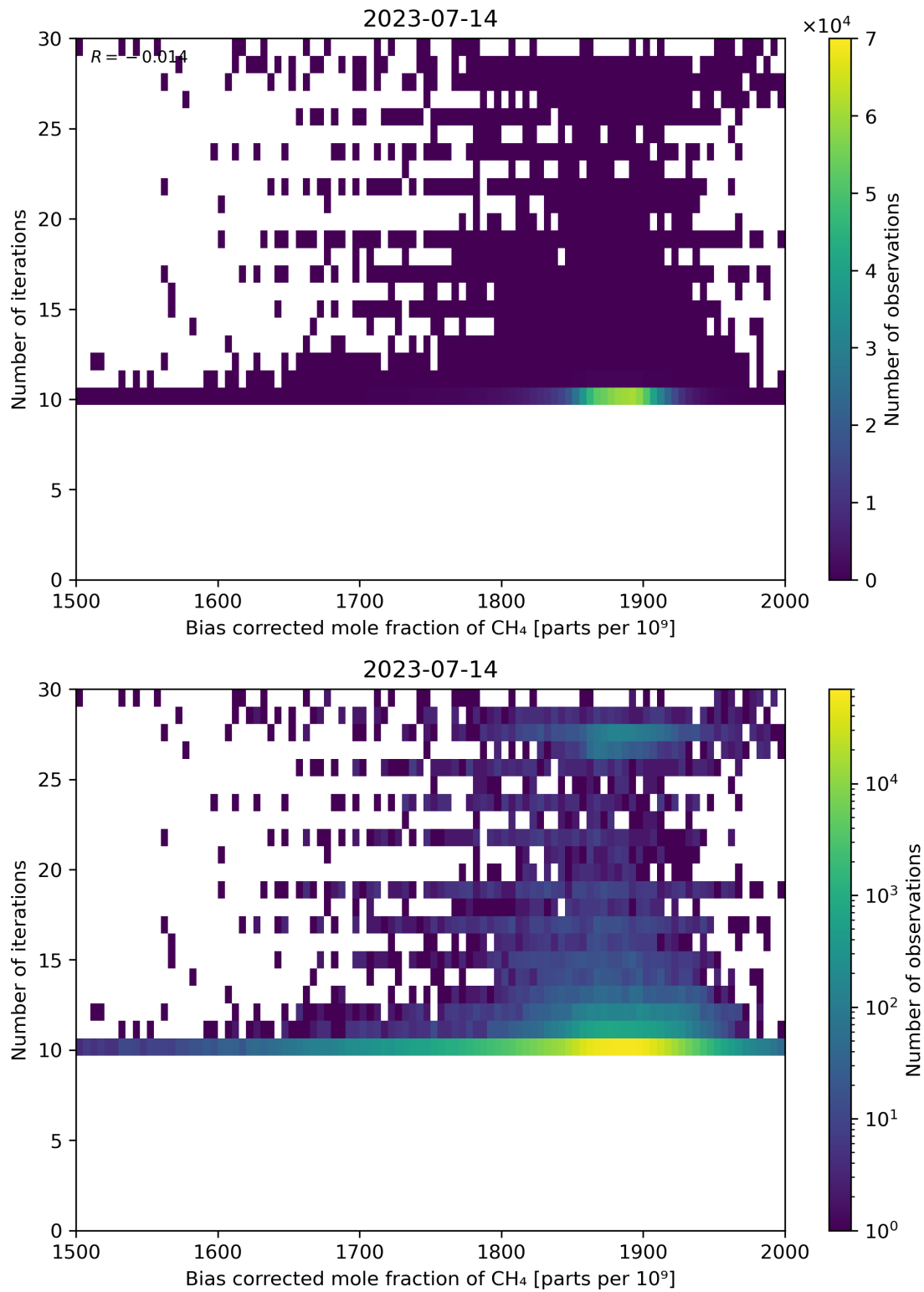
Figure 67: Scatter density plot of “Bias corrected mole fraction of CH 4 ” against “Number of iterations” for 2023-07-14 to 2023-07-15.
