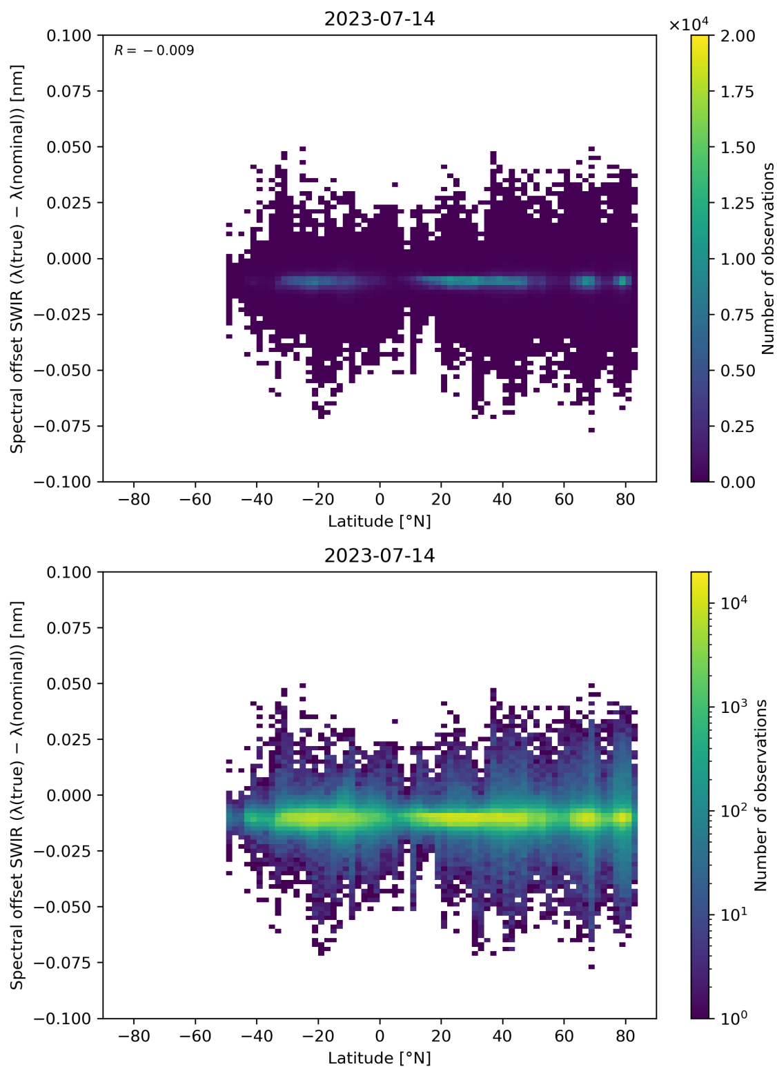
Figure 62: Scatter density plot of “Latitude” against “Spectral offset SWIR ( \lambda(\text{true}) - \lambda(\text{nominal}) )” for 2023-07-14 to 2023-07-15.
