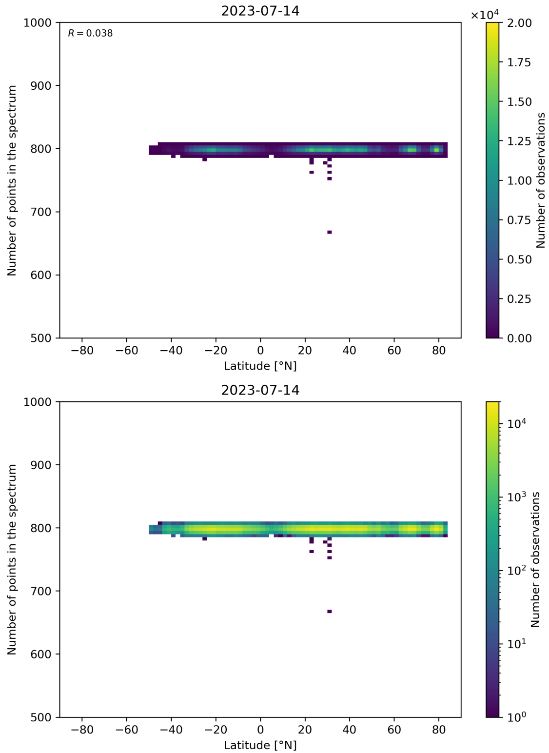
Figure 61: Scatter density plot of “Latitude” against “Number of points in the spectrum” for 2023-07-14 to 2023-07-15.
