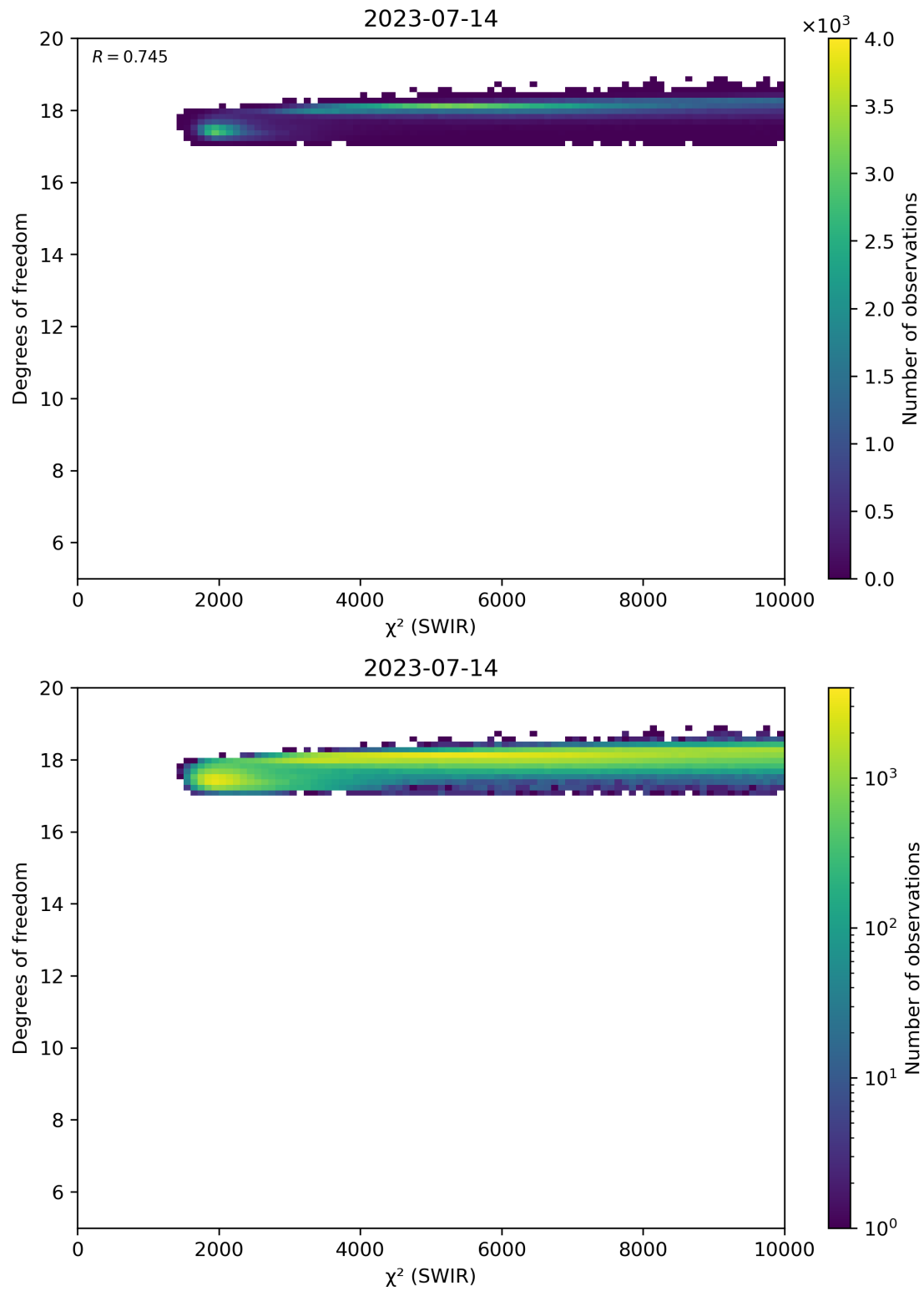
Figure 48: Scatter density plot of “ \chi^2 (SWIR)” against “Degrees of freedom” for 2023-07-14 to 2023-07-15.
