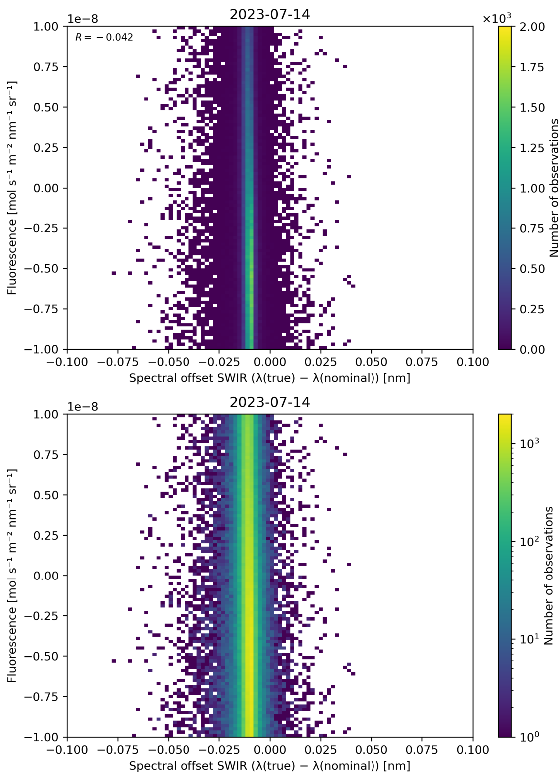
Figure 120: Scatter density plot of “Spectral offset SWIR ( \lambda(\text{true}) - \lambda(\text{nominal}) )” against “Fluorescence” for 2023-07-14 to 2023-07-15.
