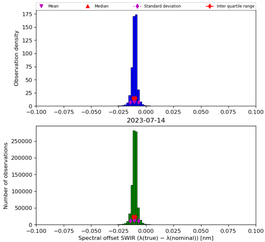
Figure 27: Histogram of “Spectral offset SWIR ( \lambda(\text{true}) - \lambda(\text{nominal}) )” for 2023-07-14 to 2023-07-15
