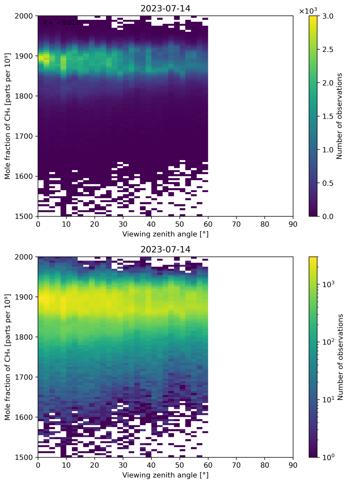
Figure 110: Scatter density plot of “Viewing zenith angle” against “Mole fraction of CH 4 ” for 2023-07-14 to 2023-07-15.
