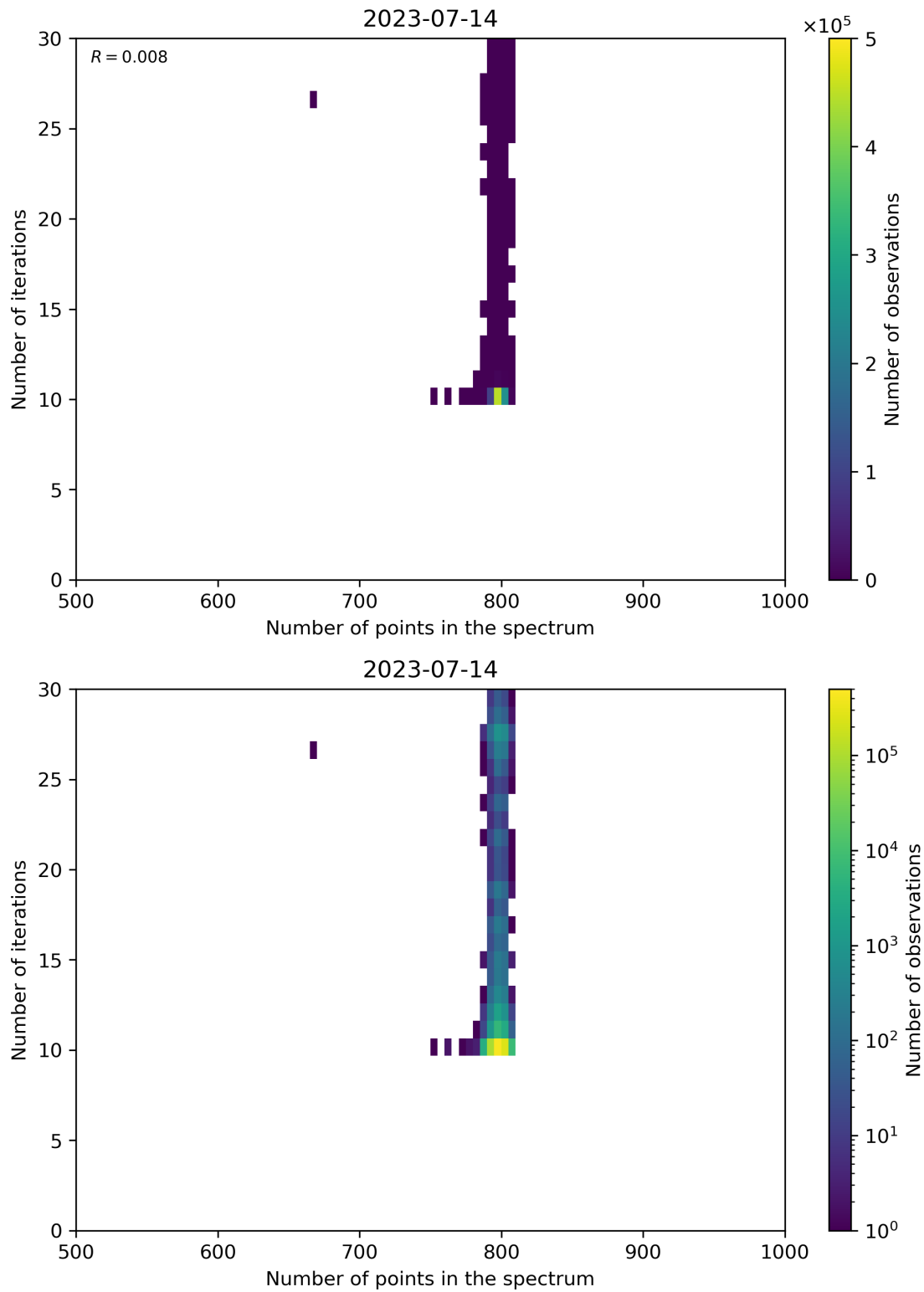
Figure 92: Scatter density plot of “Number of points in the spectrum” against “Number of iterations” for 2023-07-14 to 2023-07-15.
