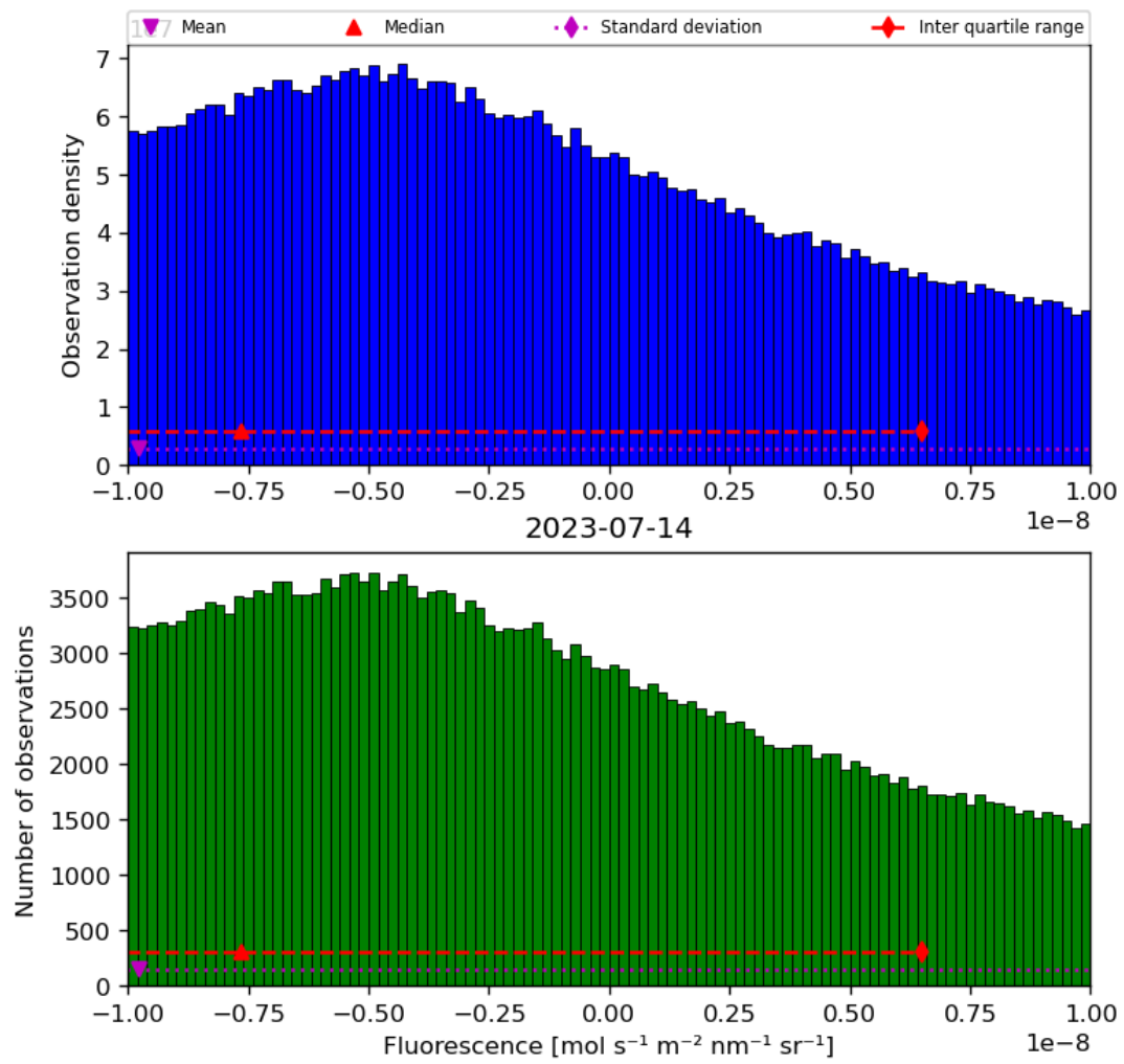
Figure 32: Histogram of “Fluorescence” for 2023-07-14 to 2023-07-15
