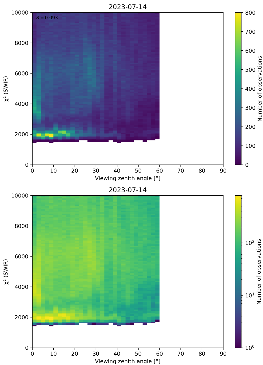
Figure 106: Scatter density plot of “Viewing zenith angle” against “ \chi^2 (SWIR)” for 2023-07-14 to 2023-07-15.
