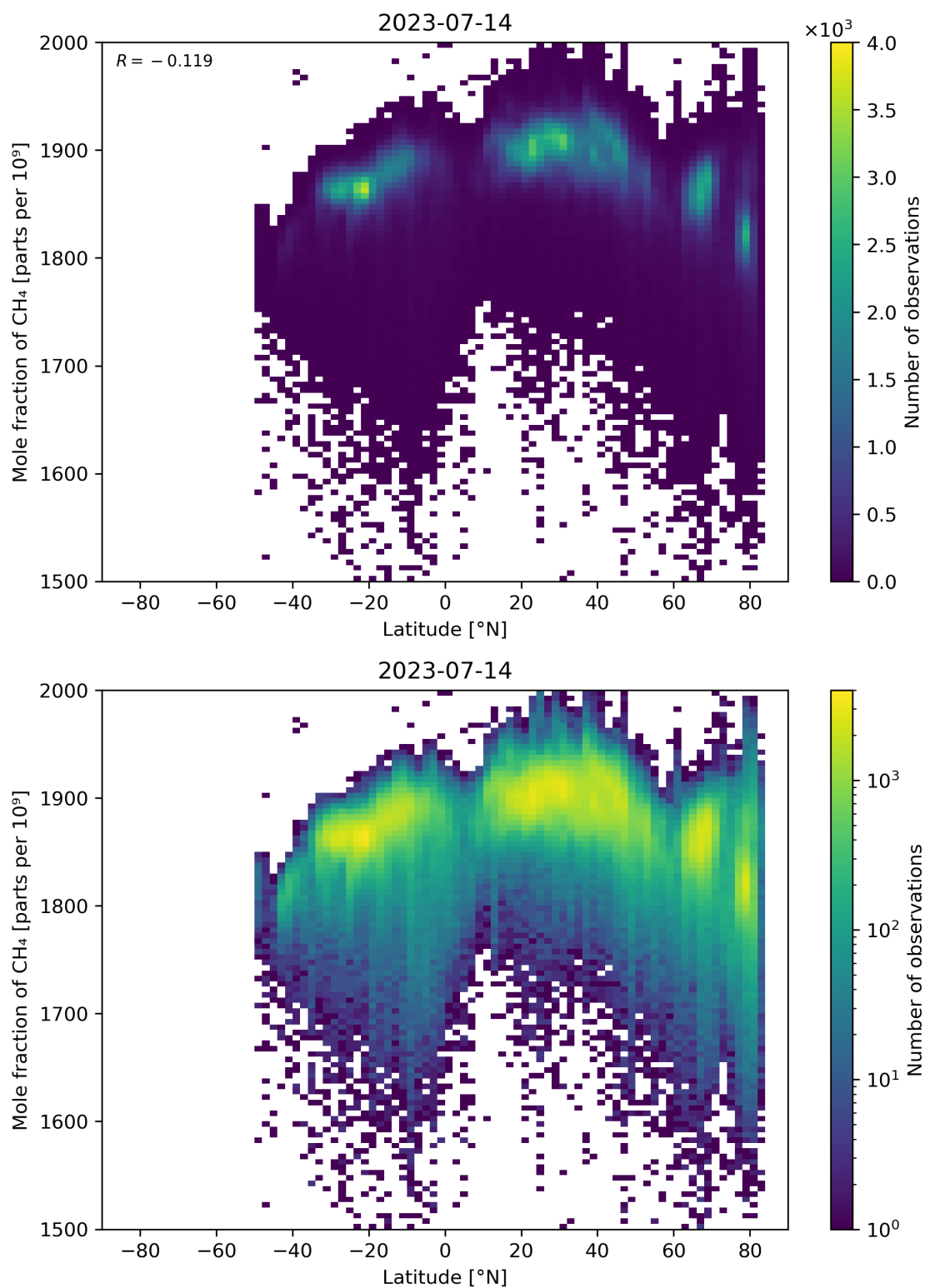
Figure 57: Scatter density plot of “Latitude” against “Mole fraction of CH 4 ” for 2023-07-14 to 2023-07-15.
