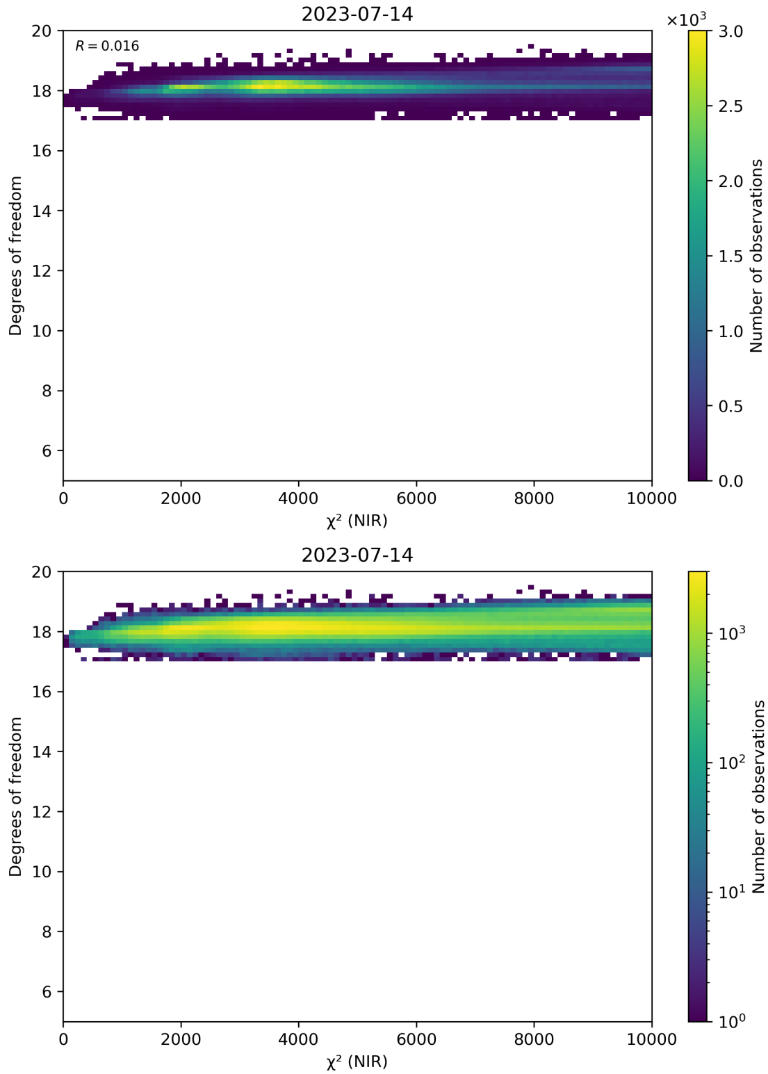
Figure 44: Scatter density plot of “ \chi^2 (NIR)” against “Degrees of freedom” for 2023-07-14 to 2023-07-15.
