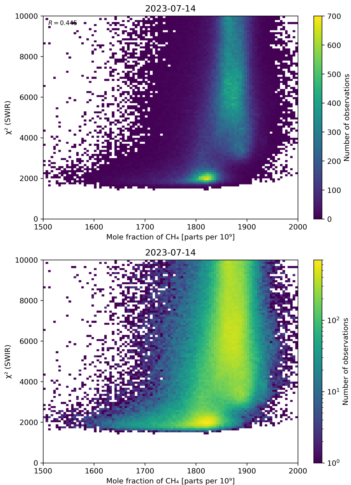
Figure 71: Scatter density plot of “Mole fraction of \text{CH}_4 ” against “ \chi^2 (SWIR)” for 2023-07-14 to 2023-07-15.
