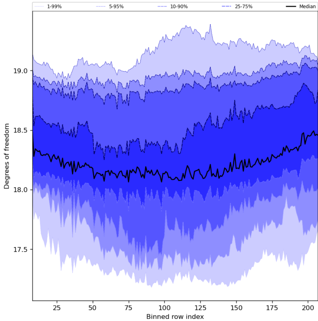
Figure 41: Along track statistics of “Degrees of freedom” for 2023-07-14 to 2023-07-15
