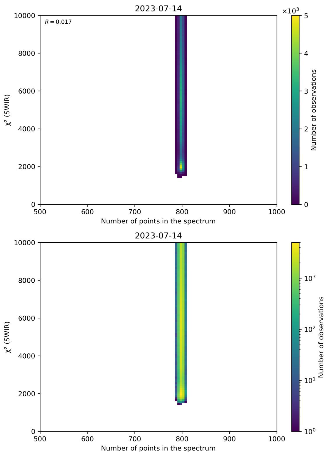
Figure 89: Scatter density plot of “Number of points in the spectrum” against “ \chi^2 (SWIR)” for 2023-07-14 to 2023-07-15.
