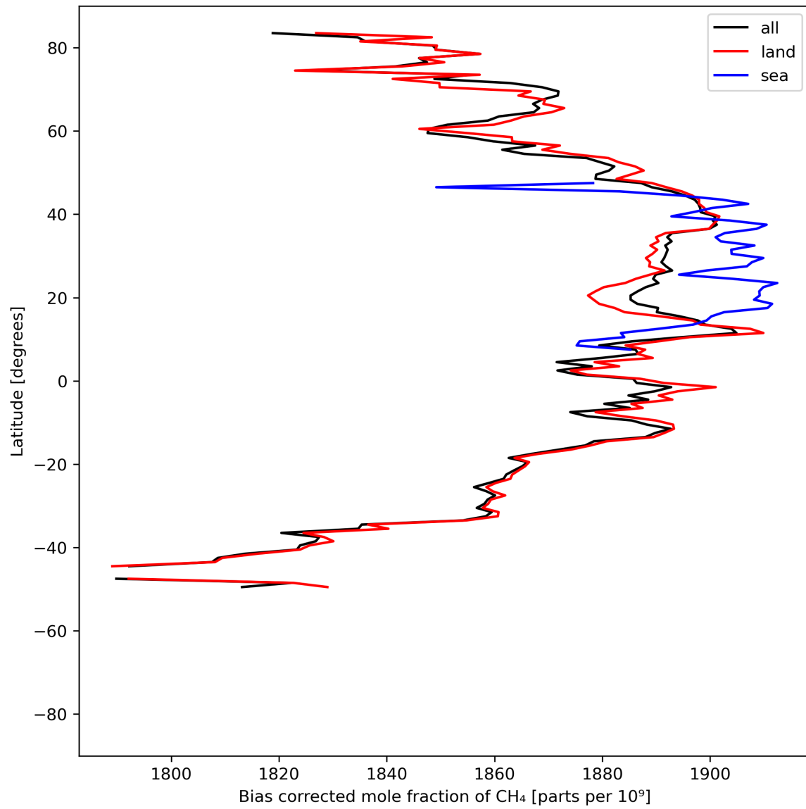
Figure 14: Zonal average of “Bias corrected mole fraction of CH 4 ” for 2023-07-14 to 2023-07-15.
