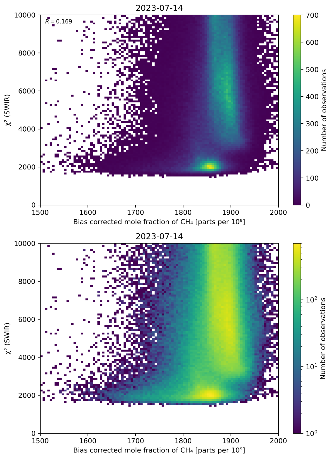
Figure 64: Scatter density plot of “Bias corrected mole fraction of CH 4 ” against “ \chi^2 (SWIR)” for 2023-07-14 to 2023-07-15.
