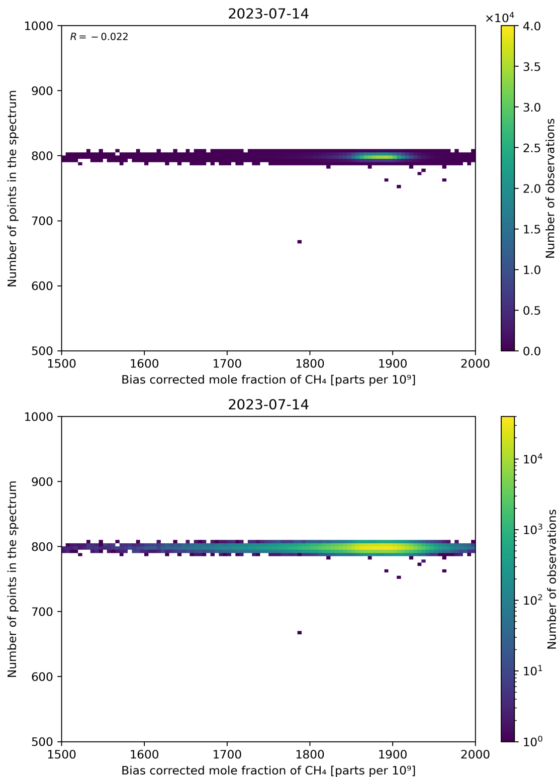
Figure 68: Scatter density plot of “Bias corrected mole fraction of CH 4 ” against “Number of points in the spectrum” for 2023-07-14 to 2023-07-15.
