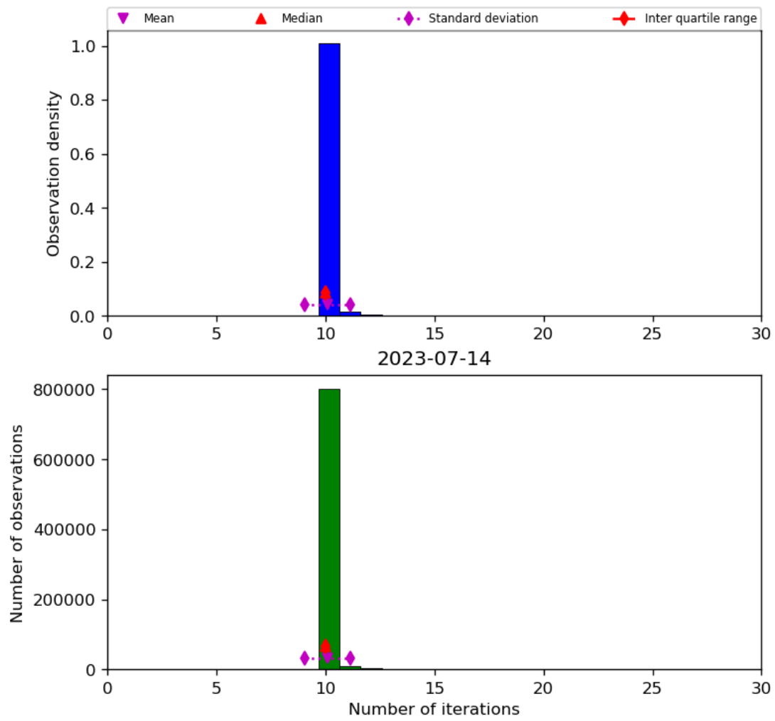
Figure 31: Histogram of “Number of iterations” for 2023-07-14 to 2023-07-15
