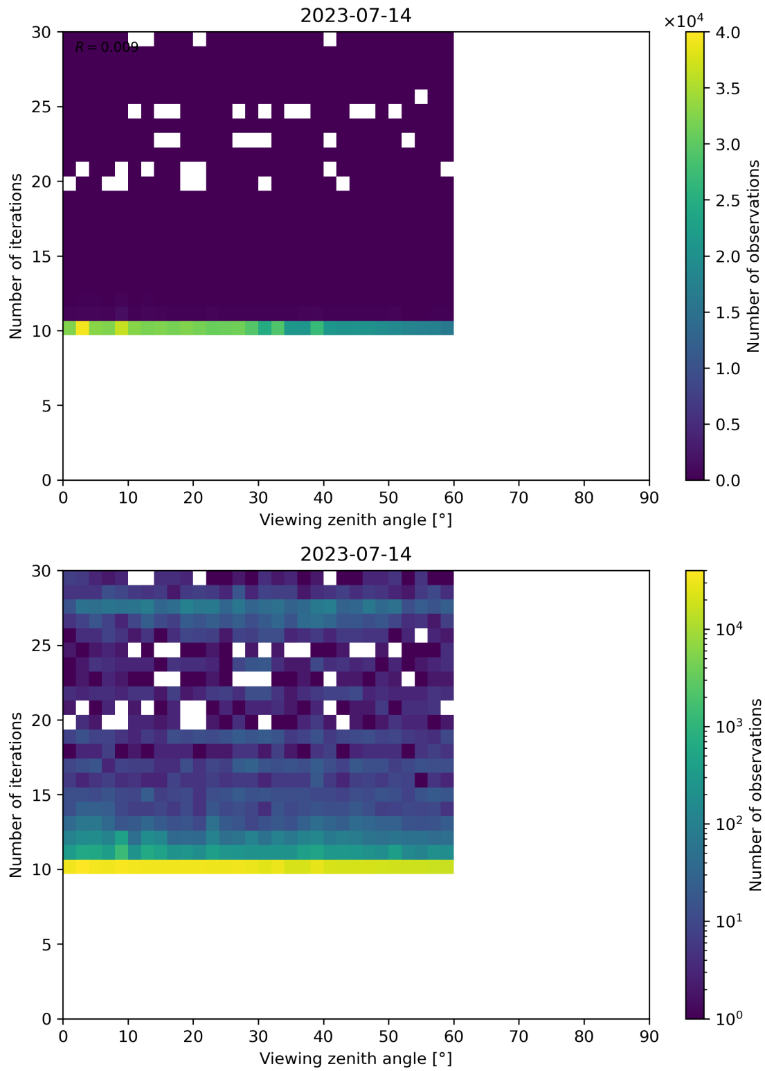
Figure 113: Scatter density plot of “Viewing zenith angle” against “Number of iterations” for 2023-07-14 to 2023-07-15.
