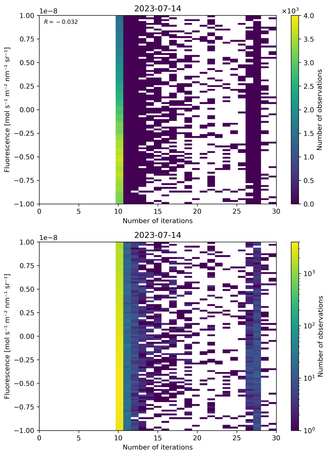
Figure 87: Scatter density plot of “Number of iterations” against “Fluorescence” for 2023-07-14 to 2023-07-15.
