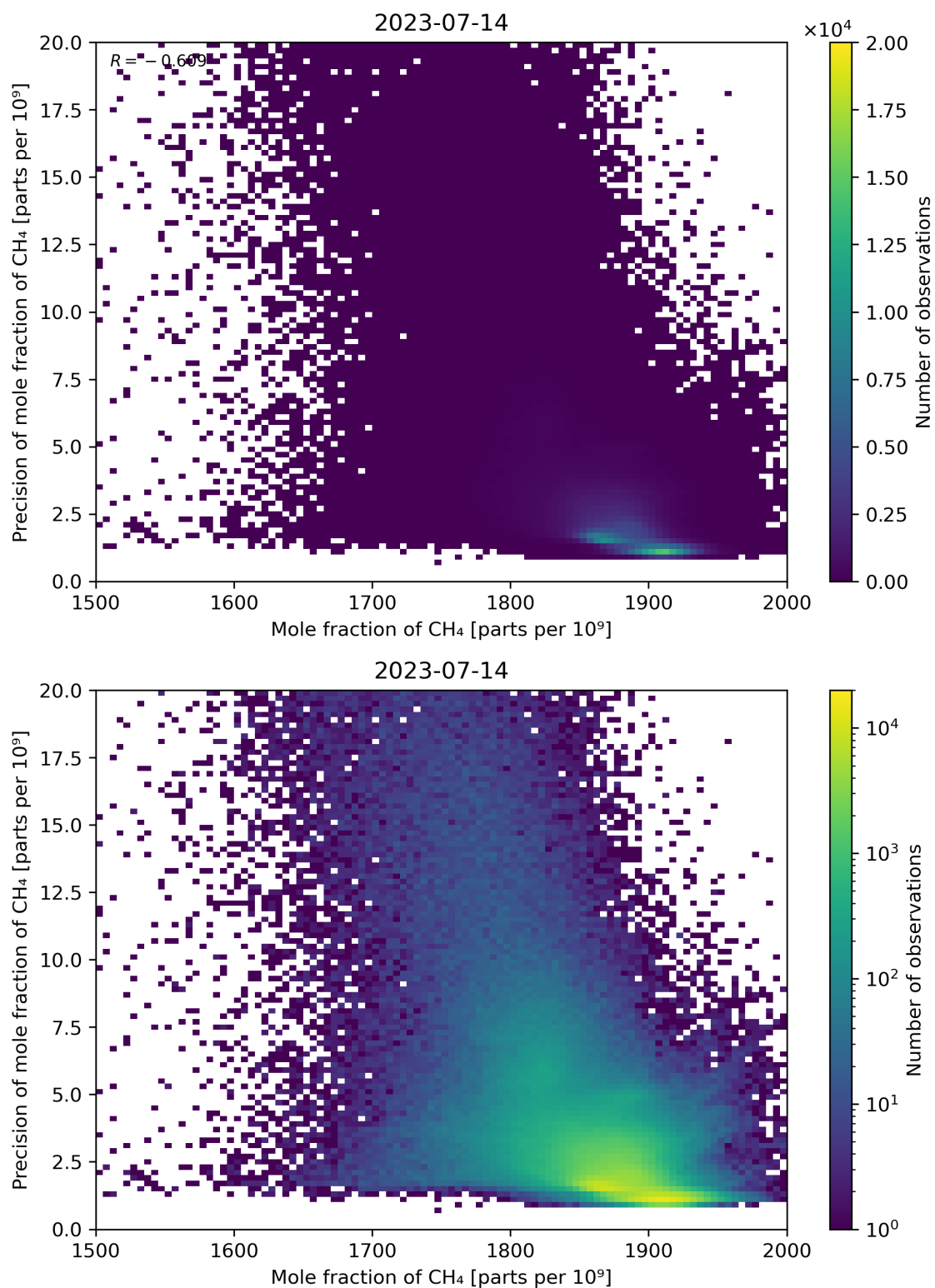
Figure 75: Scatter density plot of “Mole fraction of CH 4 ” against “Precision of mole fraction of CH 4 ” for 2023-07-14 to 2023-07-15.
