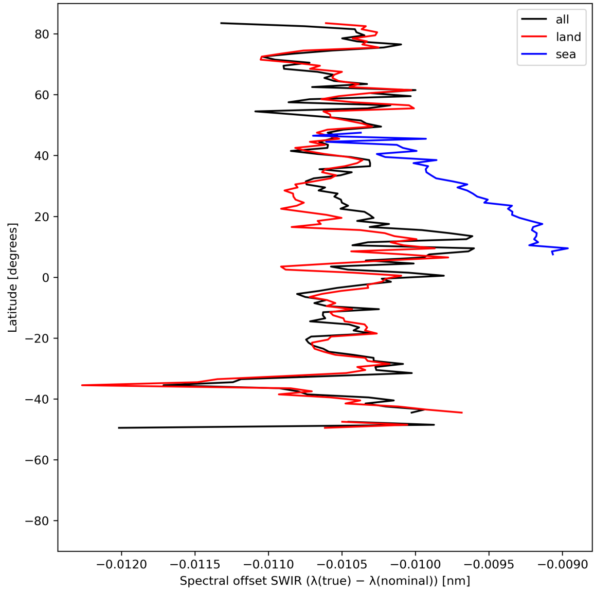
Figure 16: Zonal average of “Spectral offset SWIR ( \lambda(\text{true}) - \lambda(\text{nominal}) )” for 2023-07-14 to 2023-07-15.
