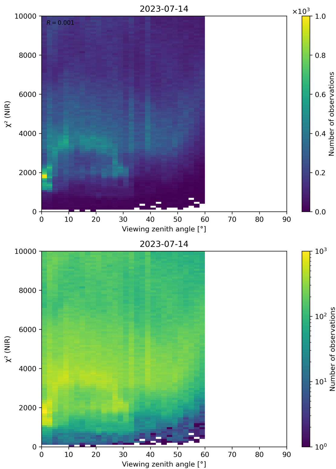
Figure 105: Scatter density plot of “Viewing zenith angle” against “ \chi^2 (NIR)” for 2023-07-14 to 2023-07-15.
