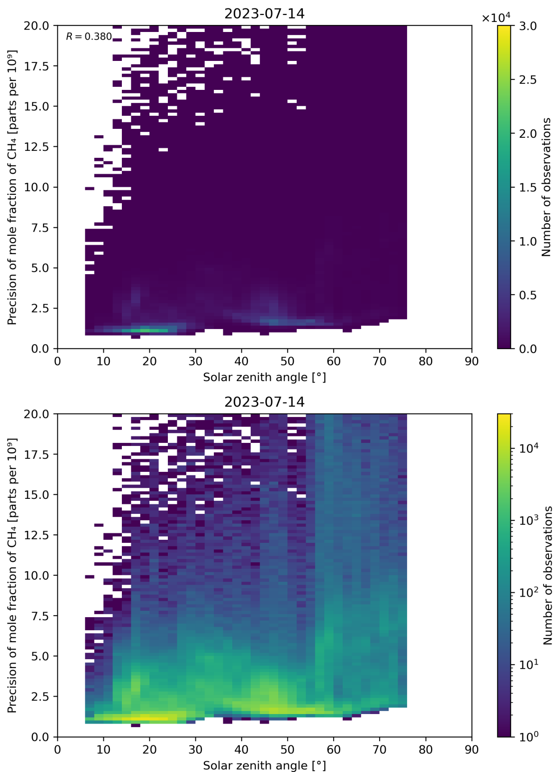
Figure 101: Scatter density plot of “Solar zenith angle” against “Precision of mole fraction of CH 4 ” for 2023-07-14 to 2023-07-15.
