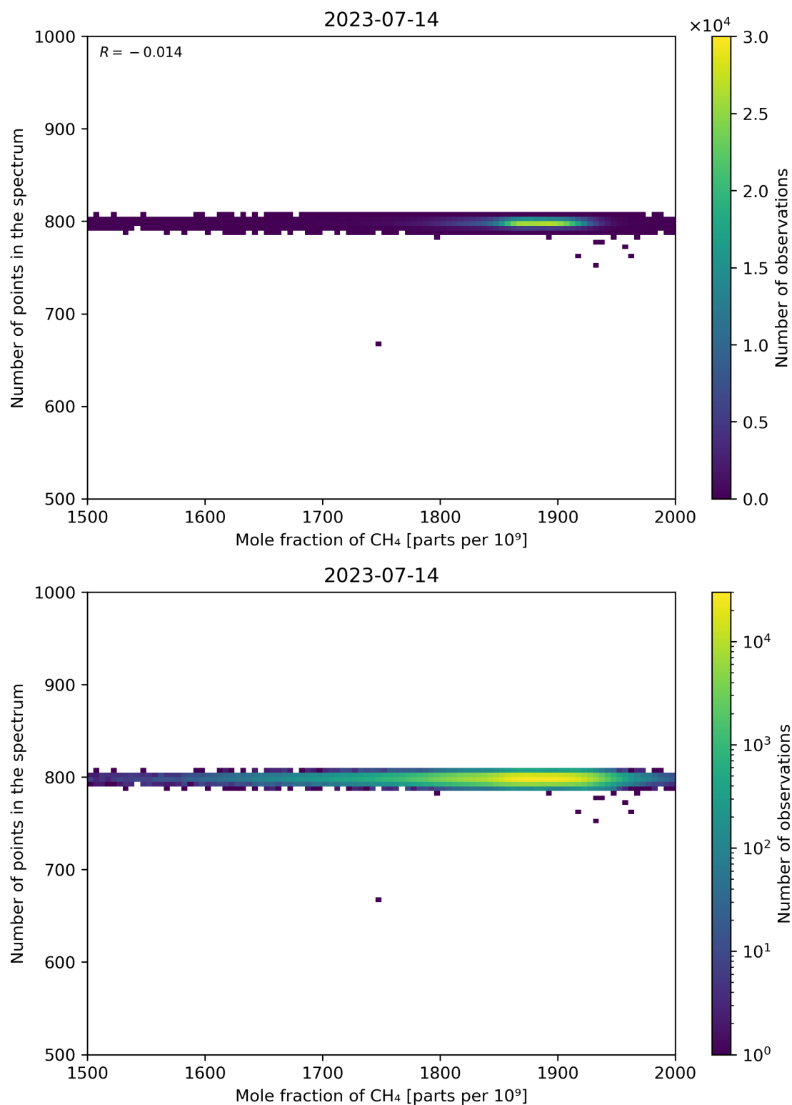
Figure 77: Scatter density plot of “Mole fraction of CH 4 ” against “Number of points in the spectrum” for 2023-07-14 to 2023-07-15.
