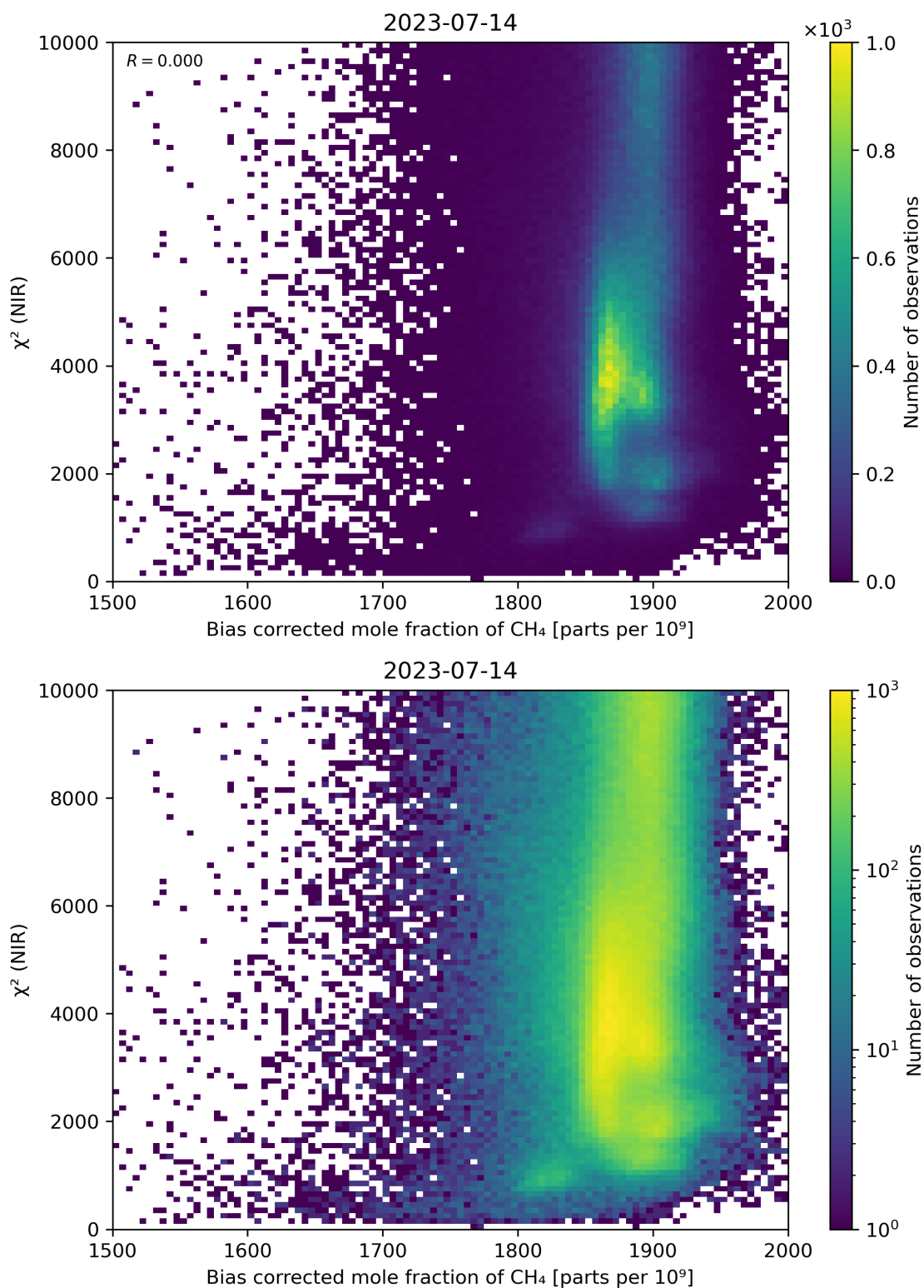
Figure 63: Scatter density plot of “Bias corrected mole fraction of CH 4 ” against “ \chi^2 (NIR)” for 2023-07-14 to 2023-07-15.
