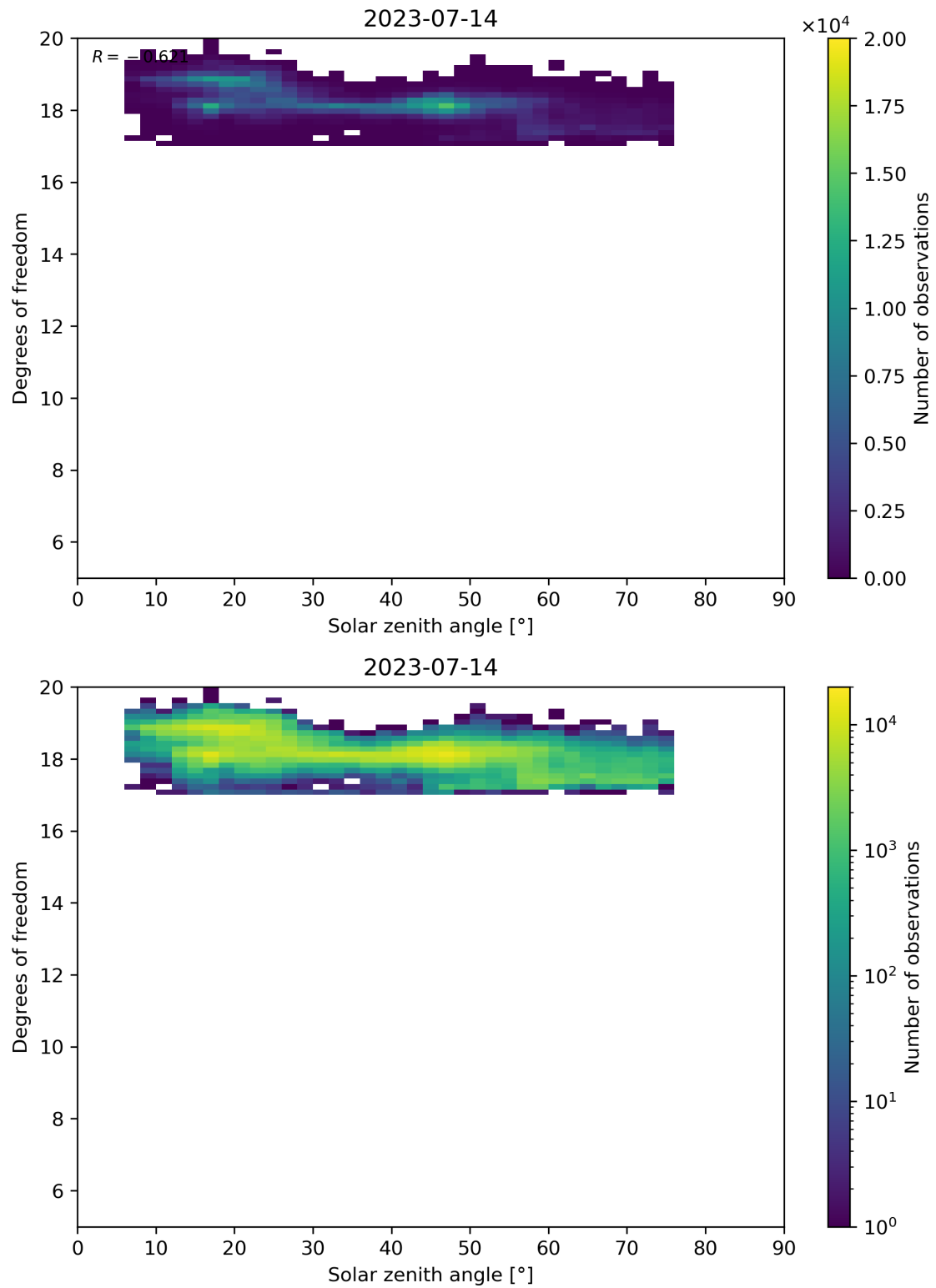
Figure 96: Scatter density plot of “Solar zenith angle” against “Degrees of freedom” for 2023-07-14 to 2023-07-15.
