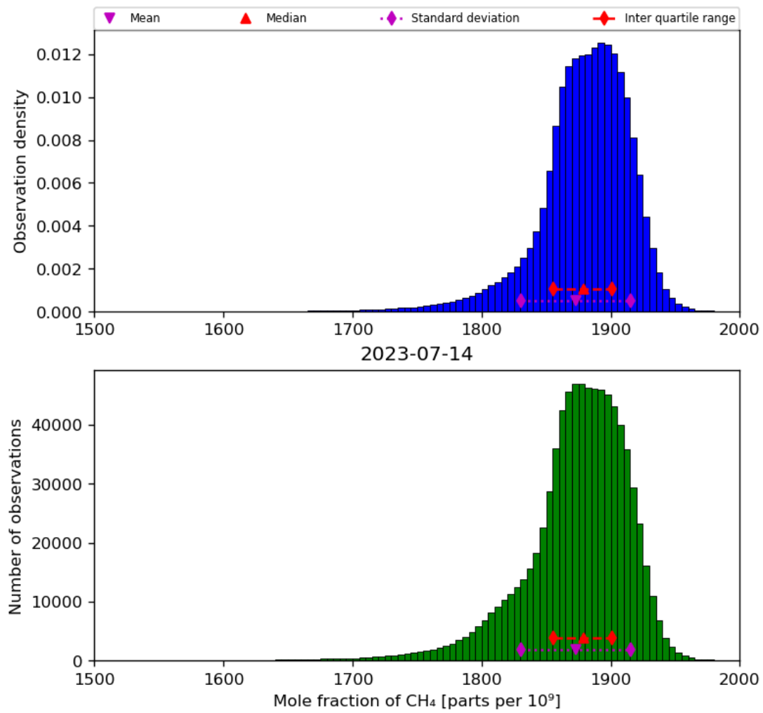
Figure 23: Histogram of “Mole fraction of CH 4 ” for 2023-07-14 to 2023-07-15
