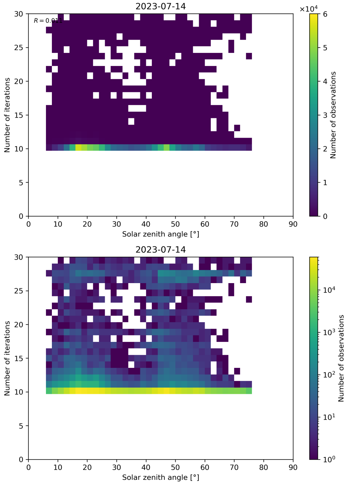
Figure 102: Scatter density plot of “Solar zenith angle” against “Number of iterations” for 2023-07-14 to 2023-07-15.
