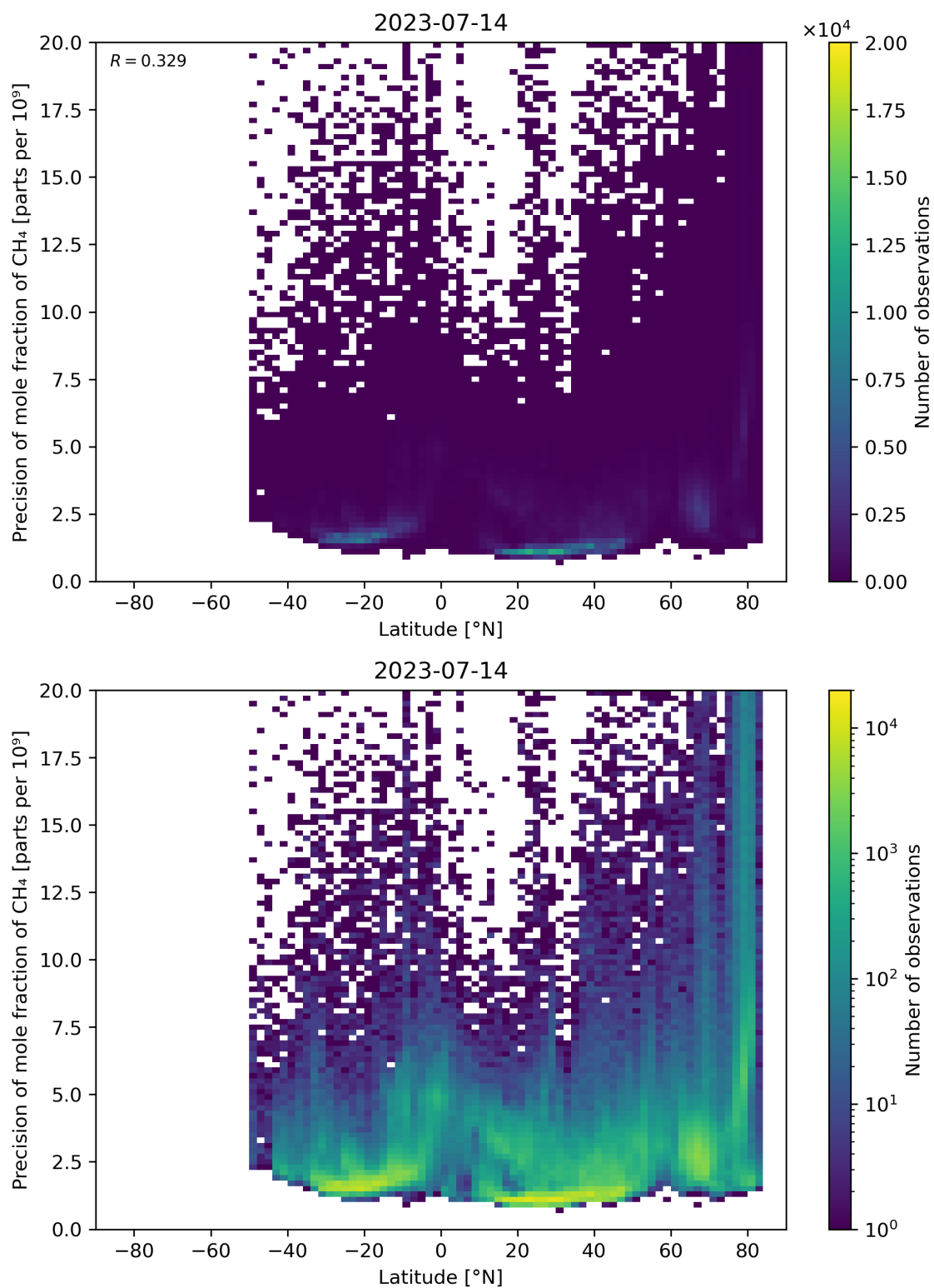
Figure 59: Scatter density plot of “Latitude” against “Precision of mole fraction of CH 4 ” for 2023-07-14 to 2023-07-15.
