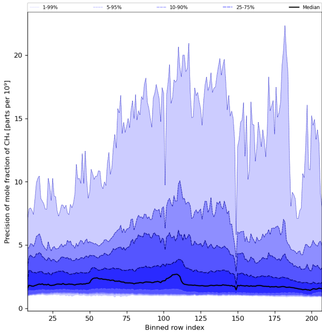
Figure 35: Along track statistics of “Precision of mole fraction of CH 4 ” for 2023-07-14 to 2023-07-15
