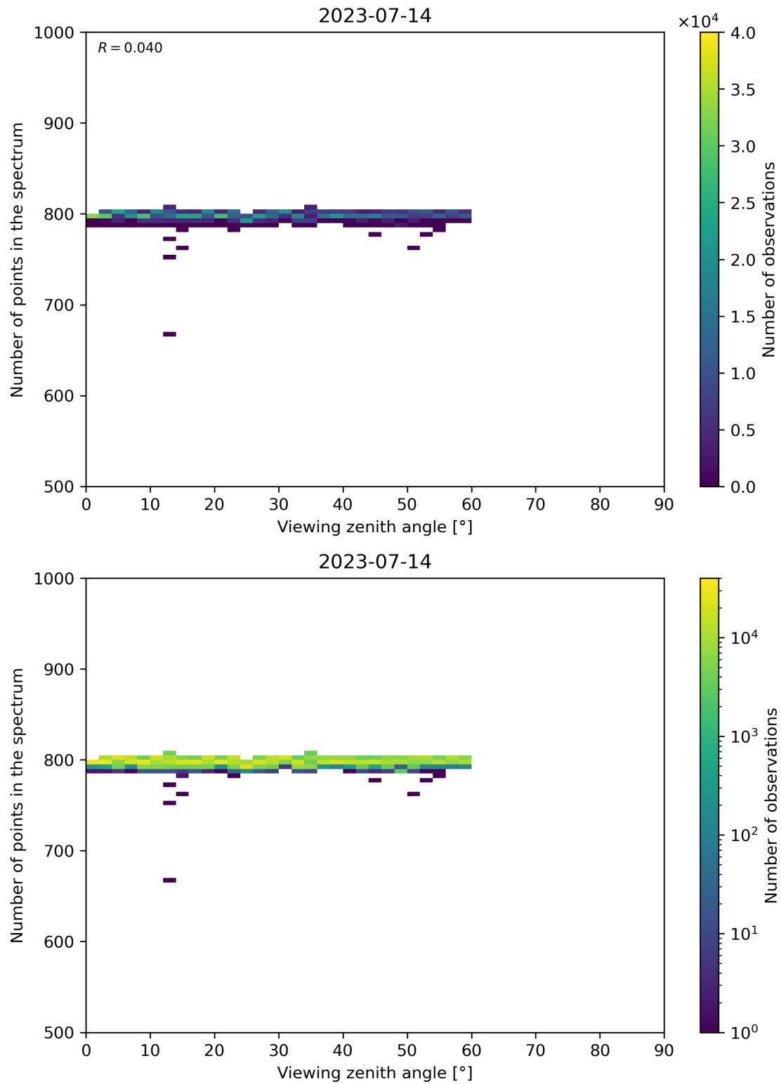
Figure 114: Scatter density plot of “Viewing zenith angle” against “Number of points in the spectrum” for 2023-07-14 to 2023-07-15.
