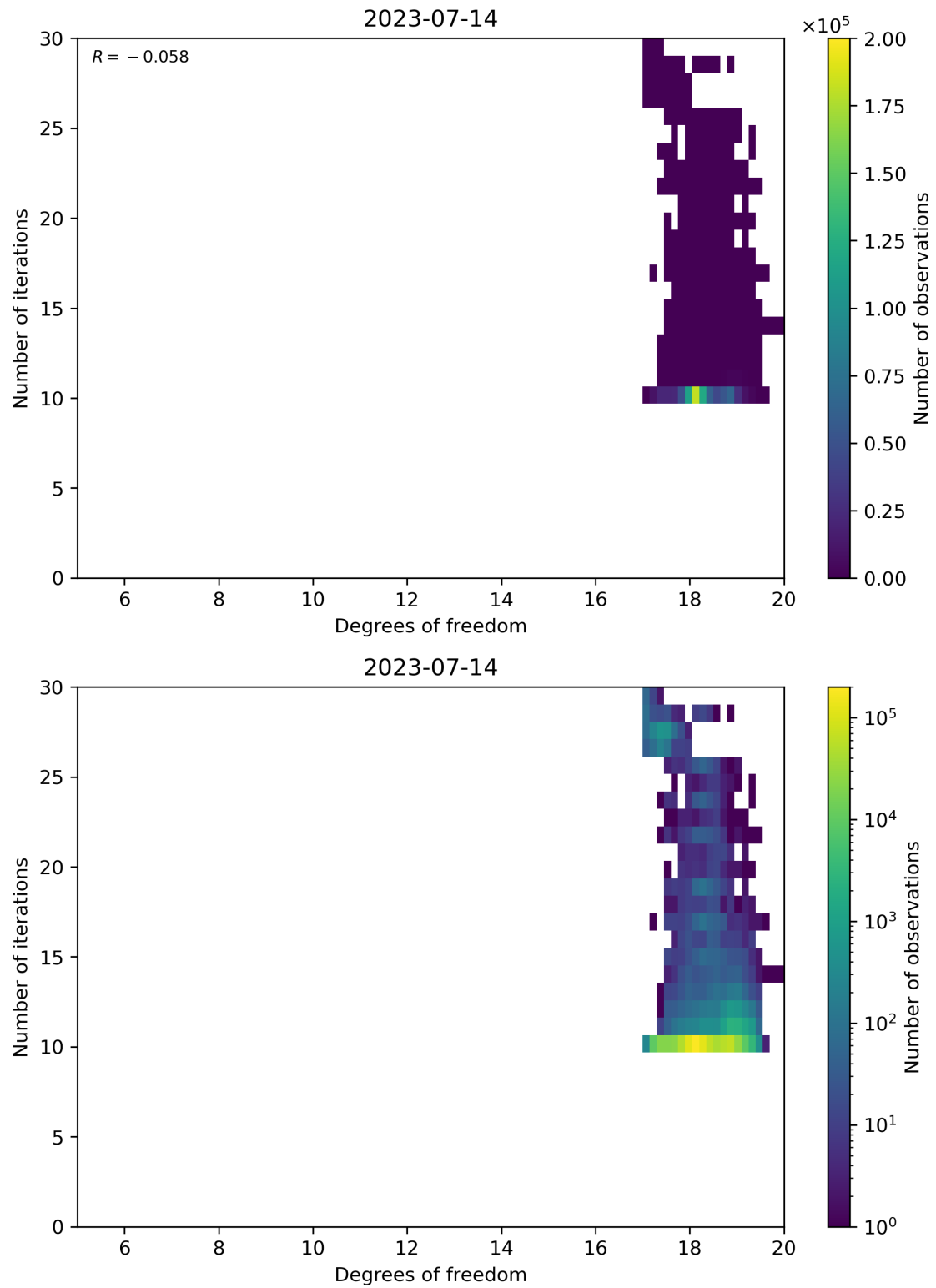
Figure 52: Scatter density plot of “Degrees of freedom” against “Number of iterations” for 2023-07-14 to 2023-07-15.
