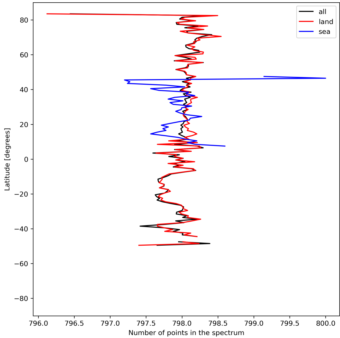
Figure 15: Zonal average of “Number of points in the spectrum” for 2023-07-14 to 2023-07-15.
