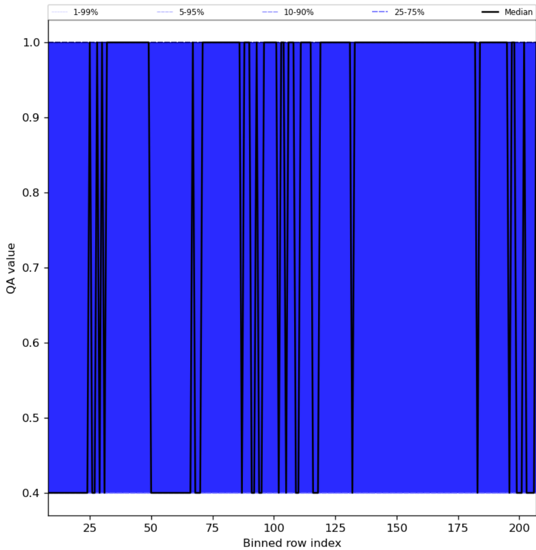
Figure 33: Along track statistics of “QA value” for 2023-07-14 to 2023-07-15
