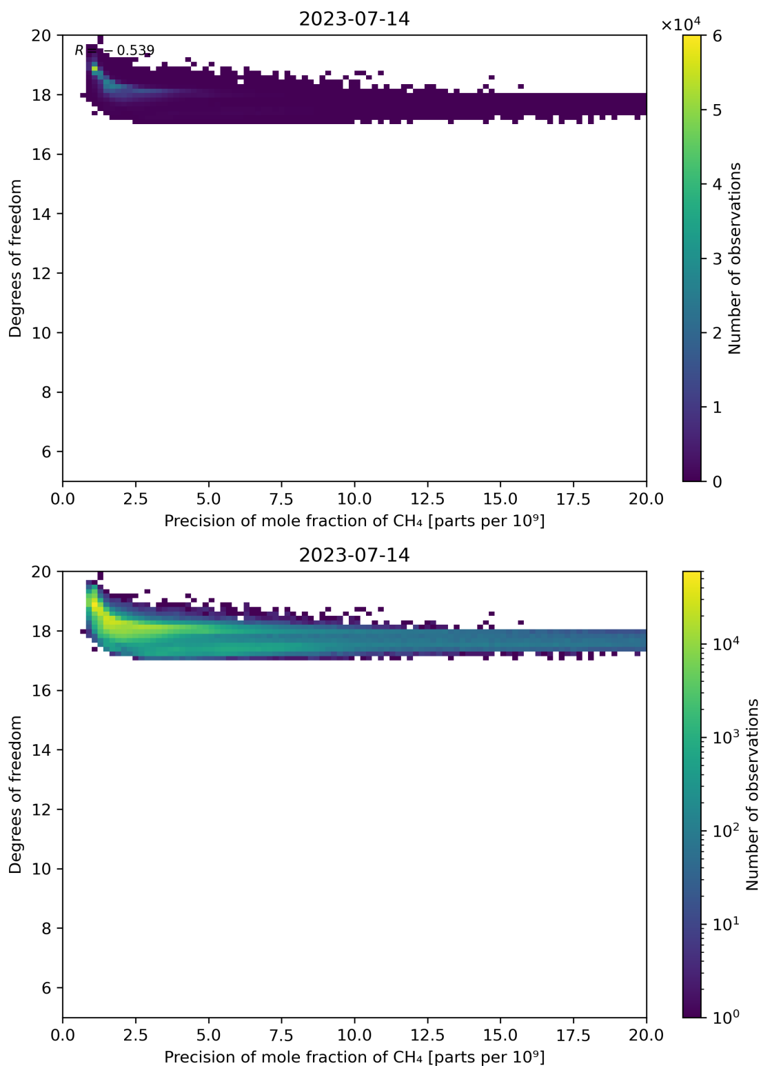
Figure 80: Scatter density plot of “Precision of mole fraction of CH 4 ” against “Degrees of freedom” for 2023-07-14 to 2023-07-15.
