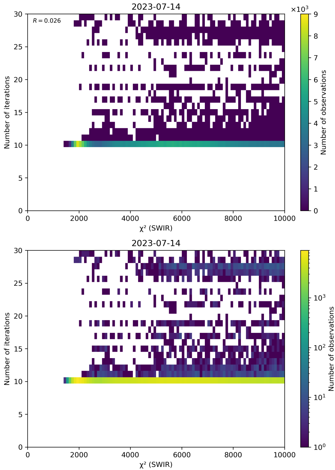
Figure 50: Scatter density plot of “ \chi^2 (SWIR)” against “Number of iterations” for 2023-07-14 to 2023-07-15.
