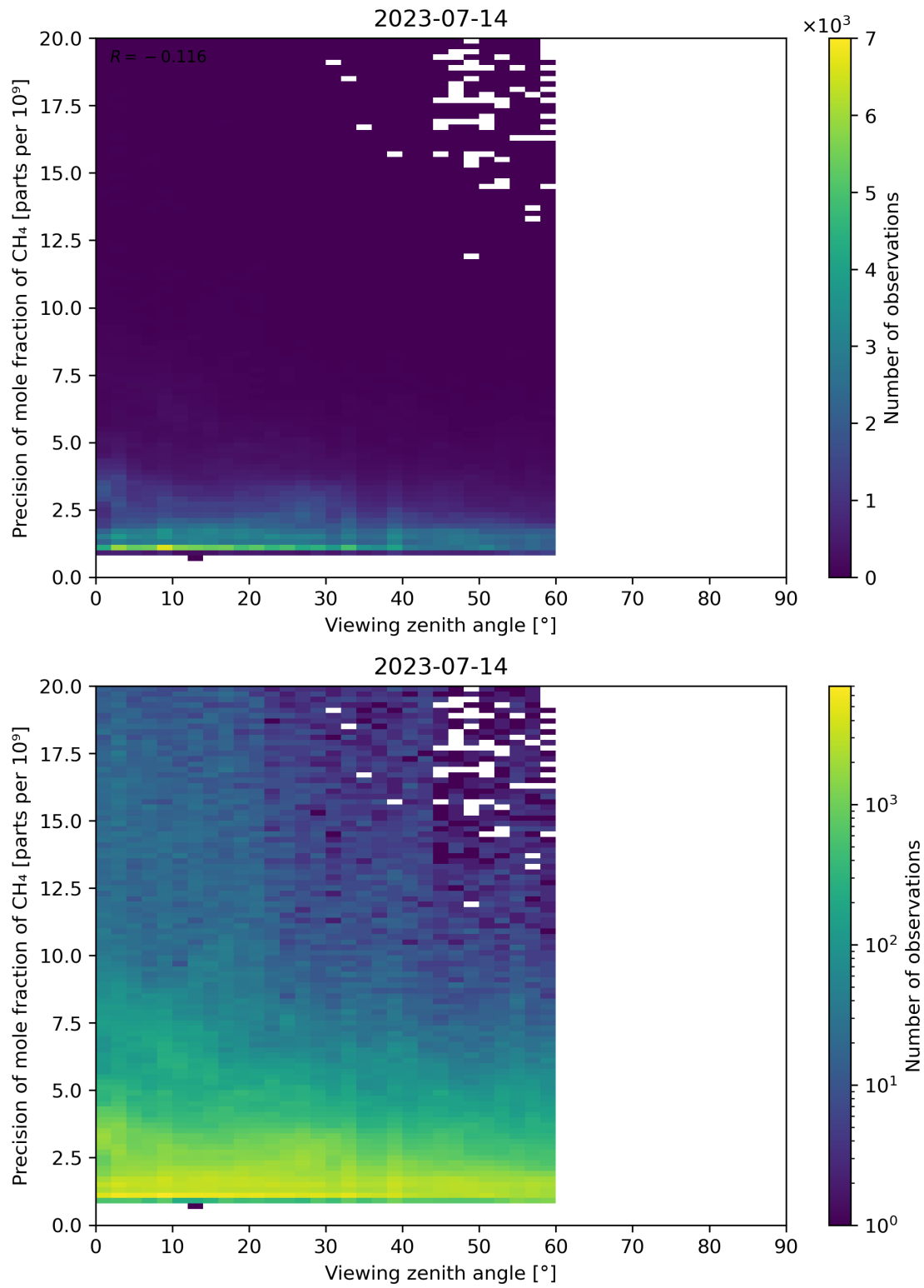
Figure 112: Scatter density plot of “Viewing zenith angle” against “Precision of mole fraction of CH 4 ” for 2023-07-14 to 2023-07-15.
