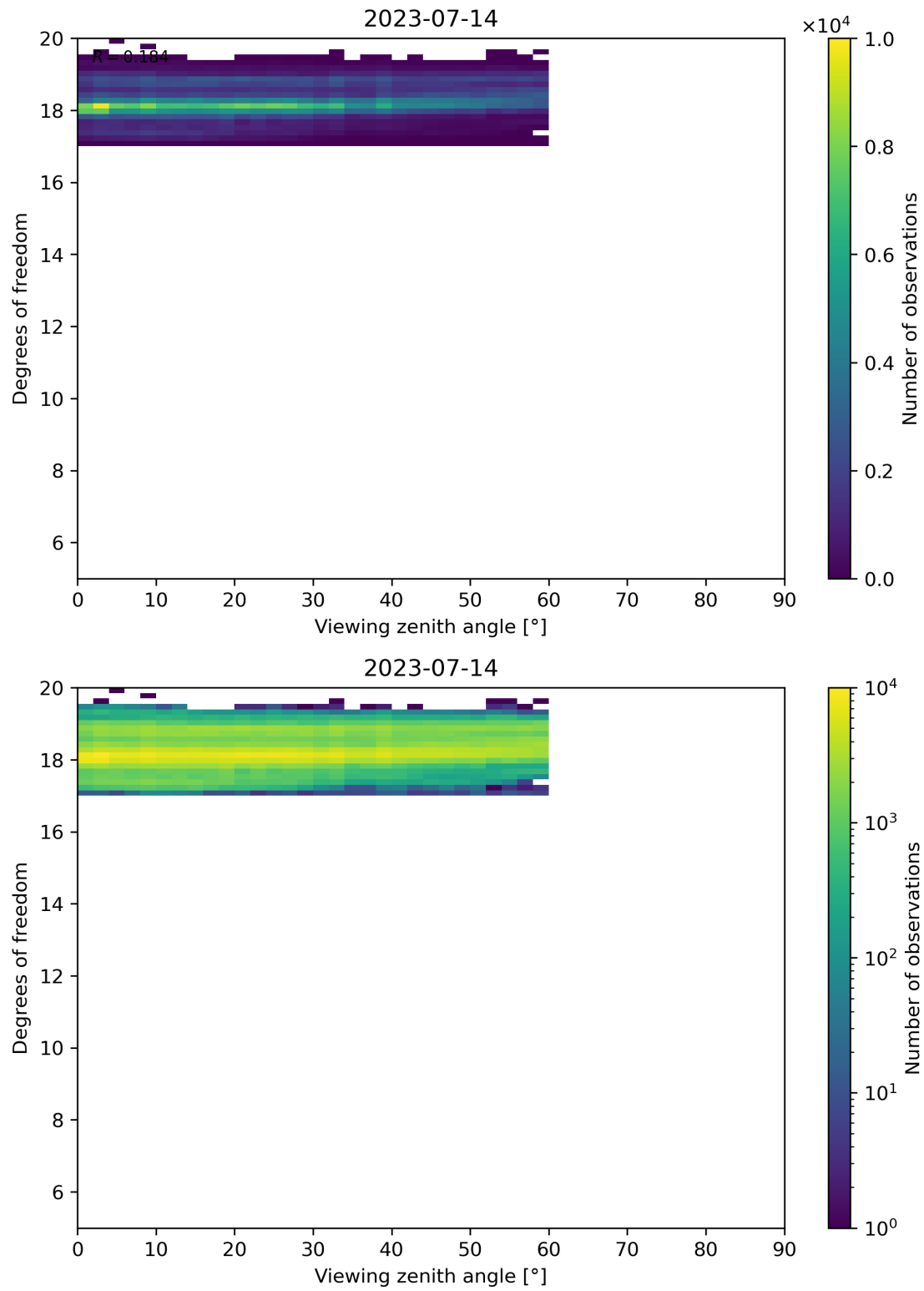
Figure 107: Scatter density plot of “Viewing zenith angle” against “Degrees of freedom” for 2023-07-14 to 2023-07-15.
