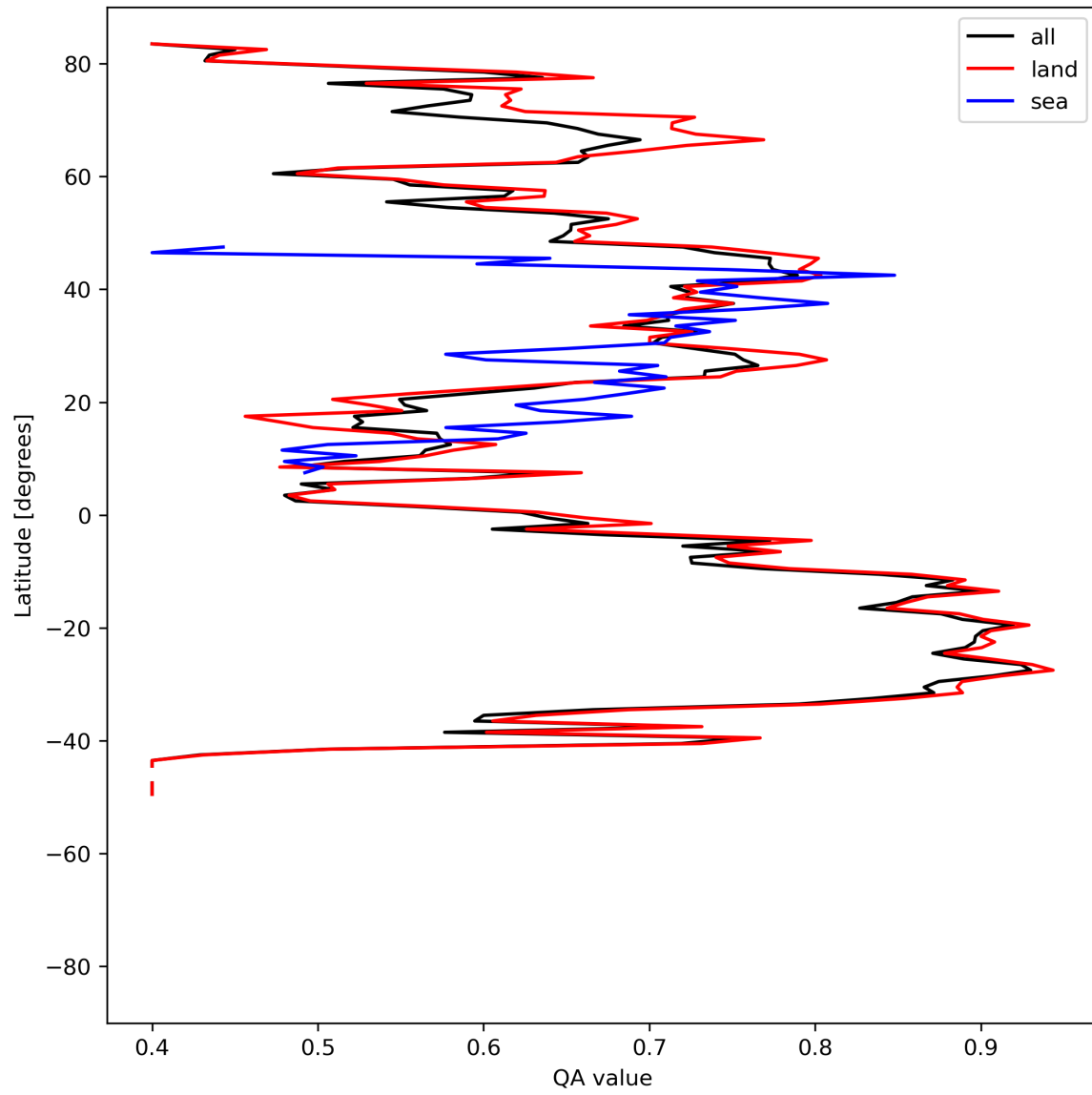
Figure 11: Zonal average of “QA value” for 2023-07-14 to 2023-07-15.
