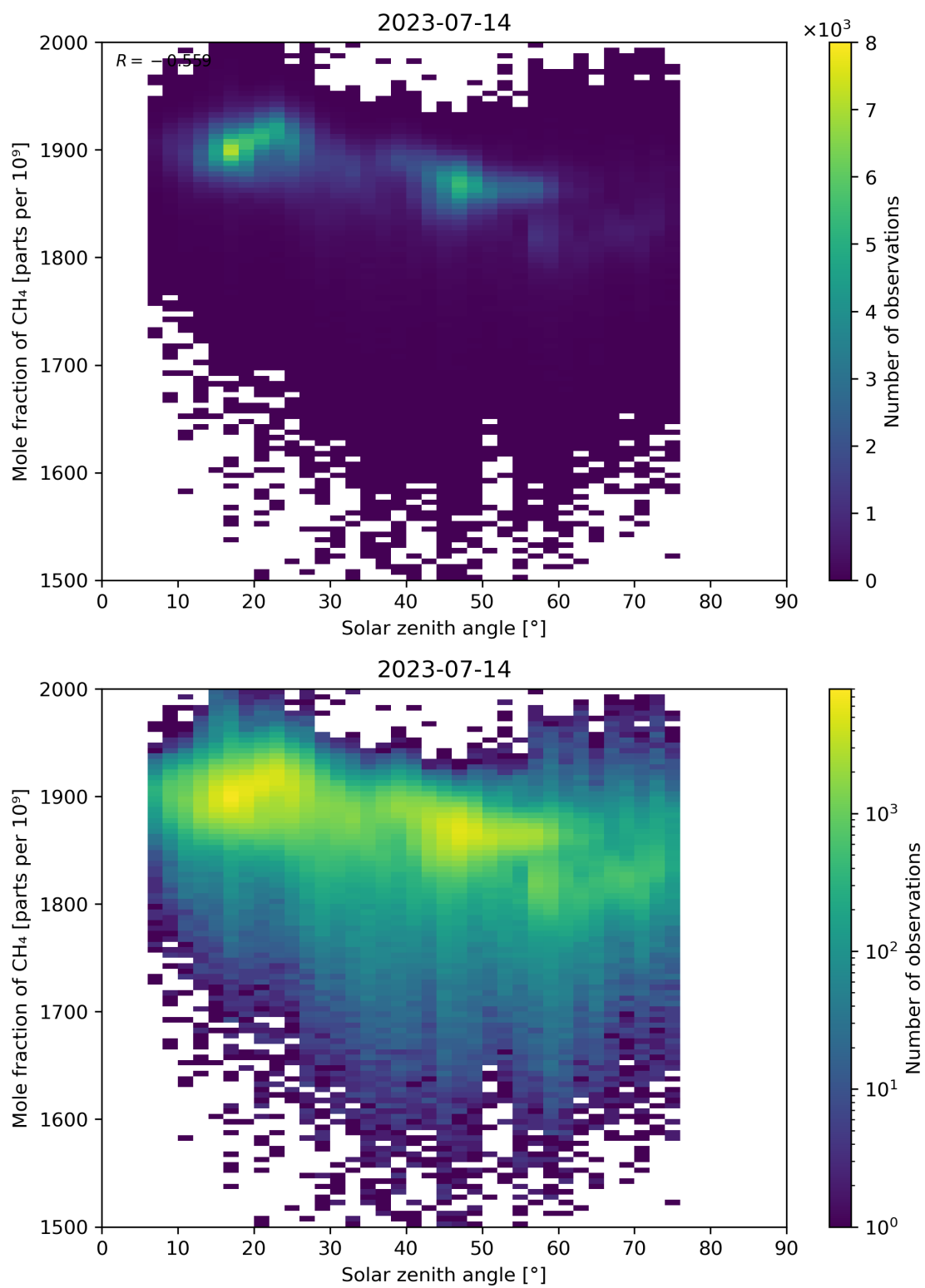
Figure 99: Scatter density plot of “Solar zenith angle” against “Mole fraction of CH 4 ” for 2023-07-14 to 2023-07-15.
