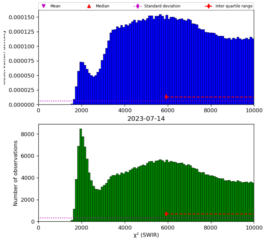
Figure 28: Histogram of “ \chi^2 (SWIR)” for 2023-07-14 to 2023-07-15
