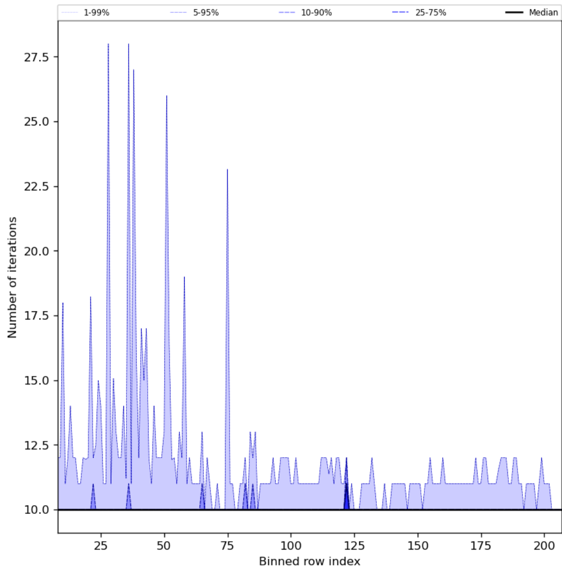
Figure 42: Along track statistics of “Number of iterations” for 2023-07-14 to 2023-07-15
