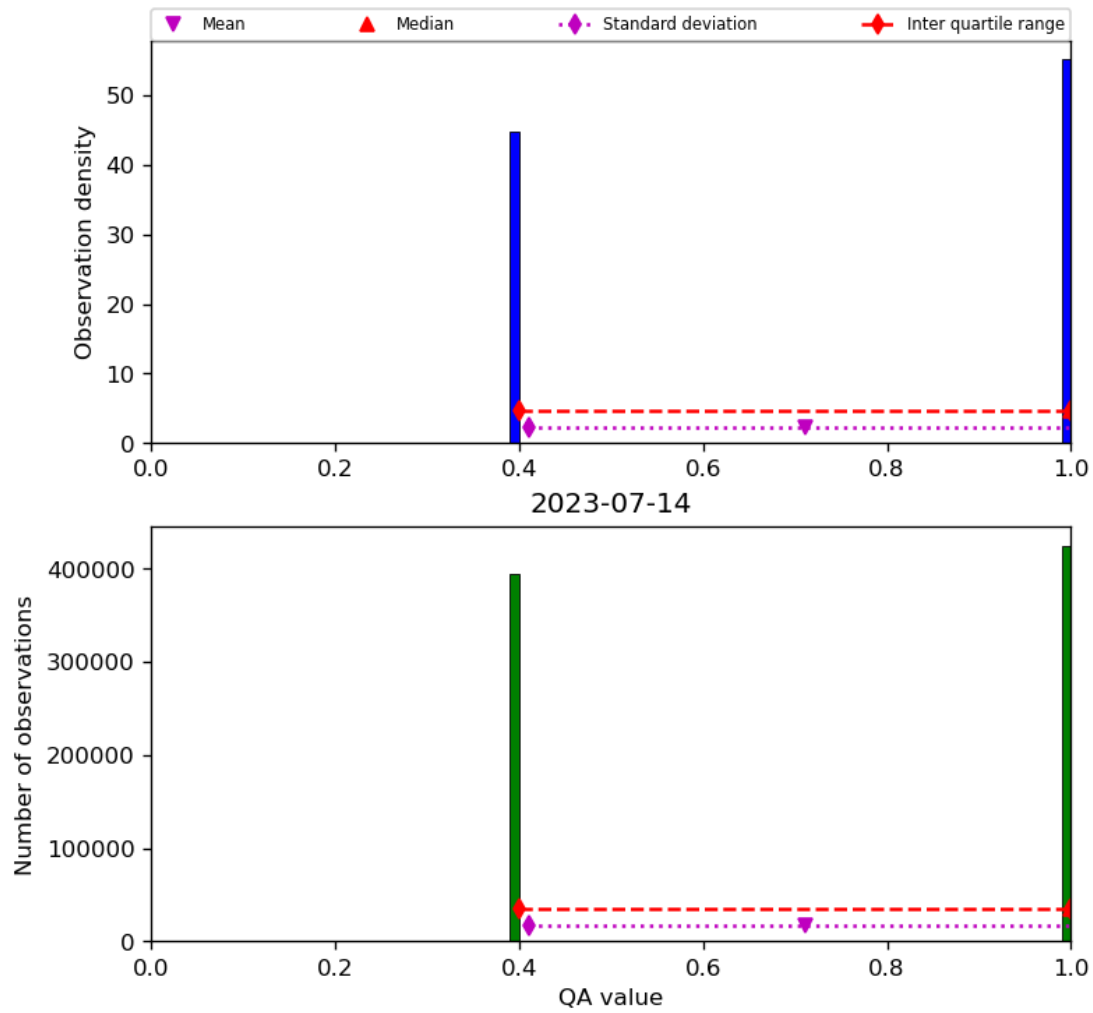
Figure 22: Histogram of “QA value” for 2023-07-14 to 2023-07-15
