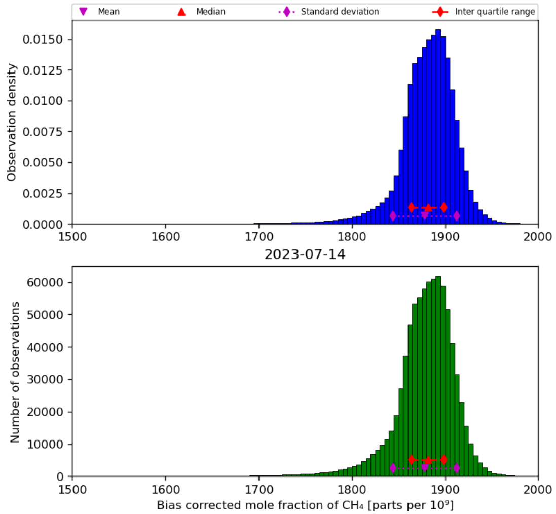
Figure 25: Histogram of “Bias corrected mole fraction of CH 4 ” for 2023-07-14 to 2023-07-15
