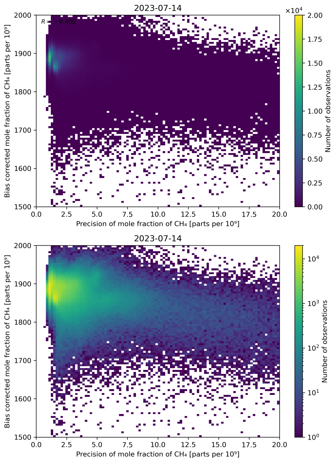
Figure 82: Scatter density plot of “Precision of mole fraction of CH 4 ” against “Bias corrected mole fraction of CH 4 ” for 2023-07-14 to 2023-07-15.
