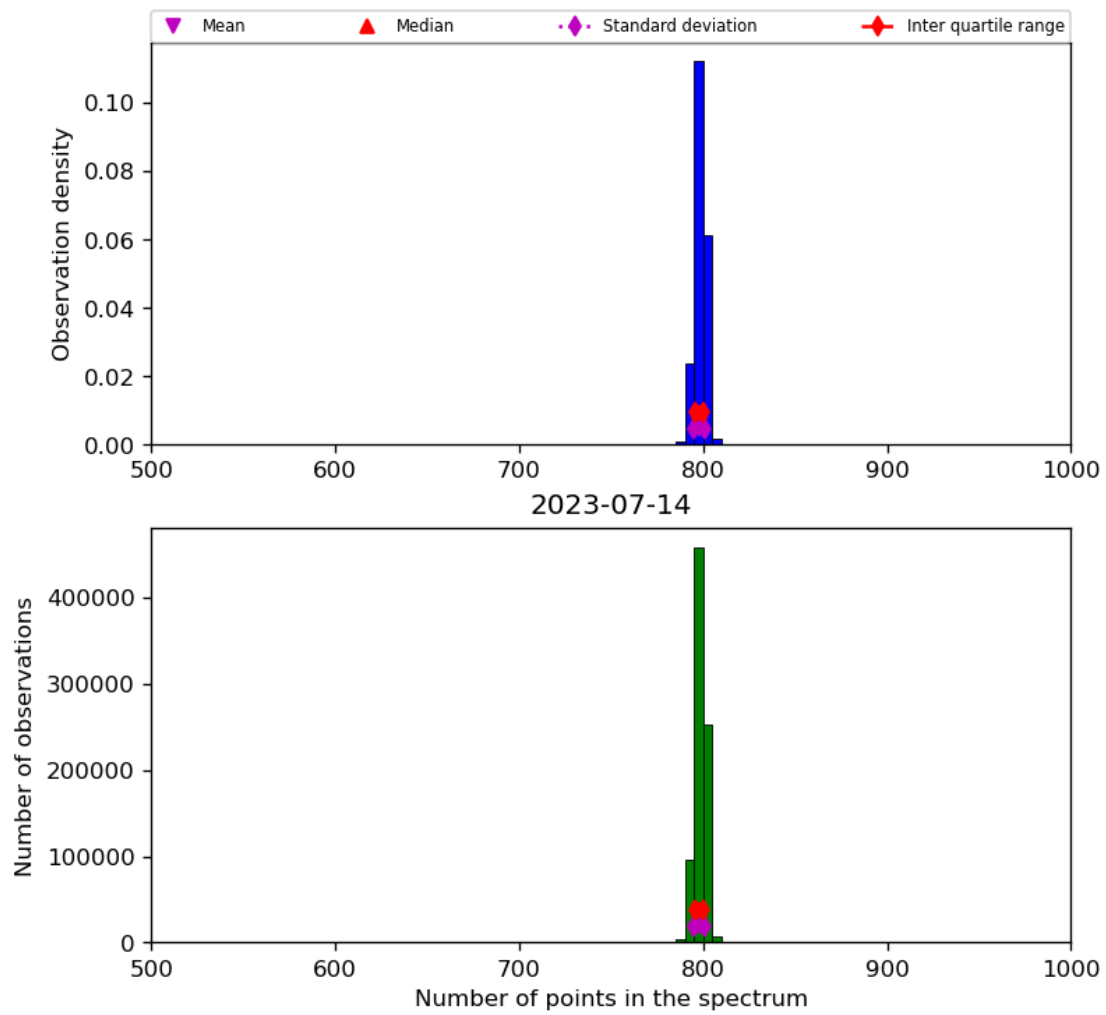
Figure 26: Histogram of “Number of points in the spectrum” for 2023-07-14 to 2023-07-15
