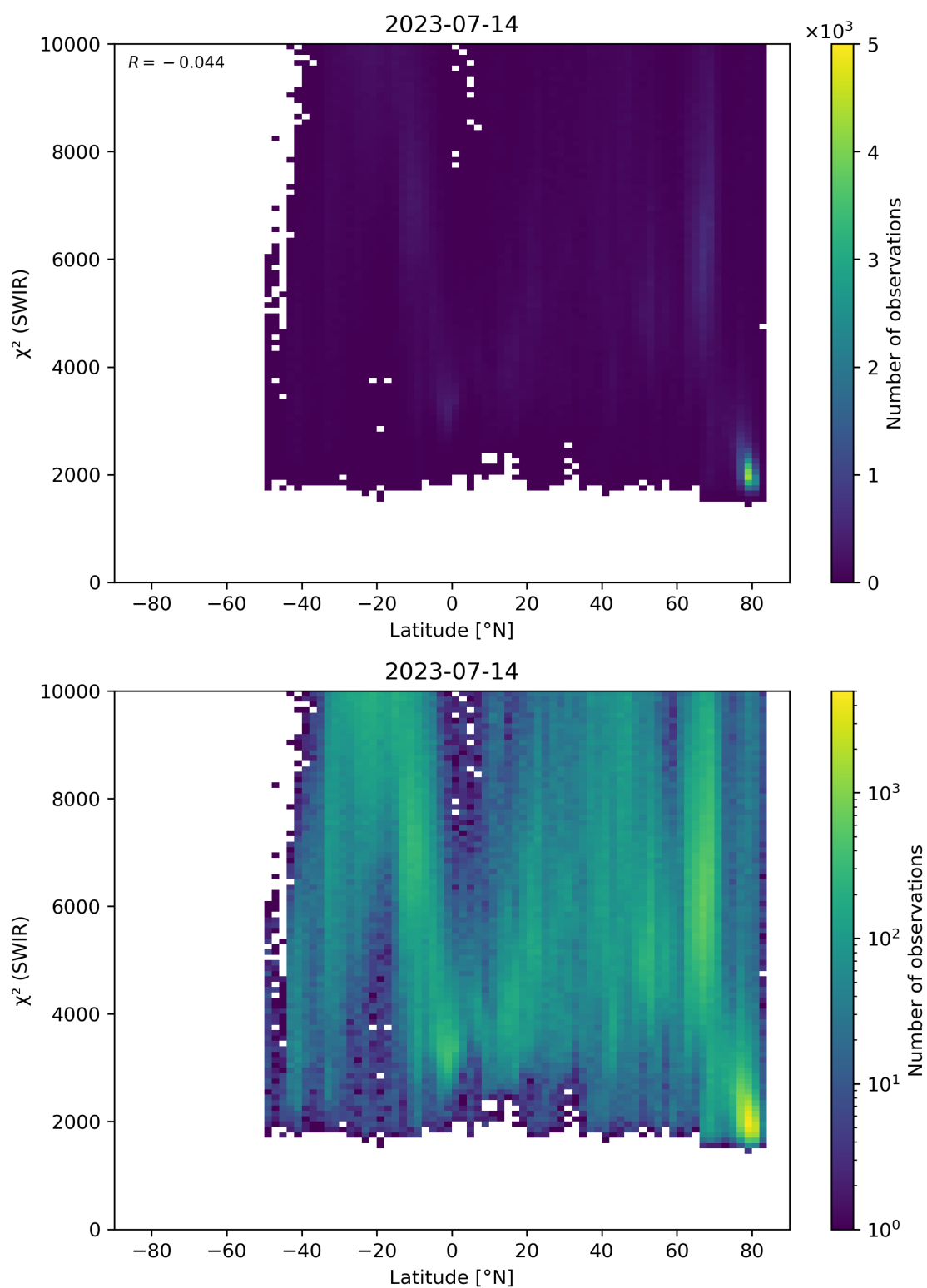
Figure 54: Scatter density plot of “Latitude” against “ \chi^2 (SWIR)” for 2023-07-14 to 2023-07-15.
