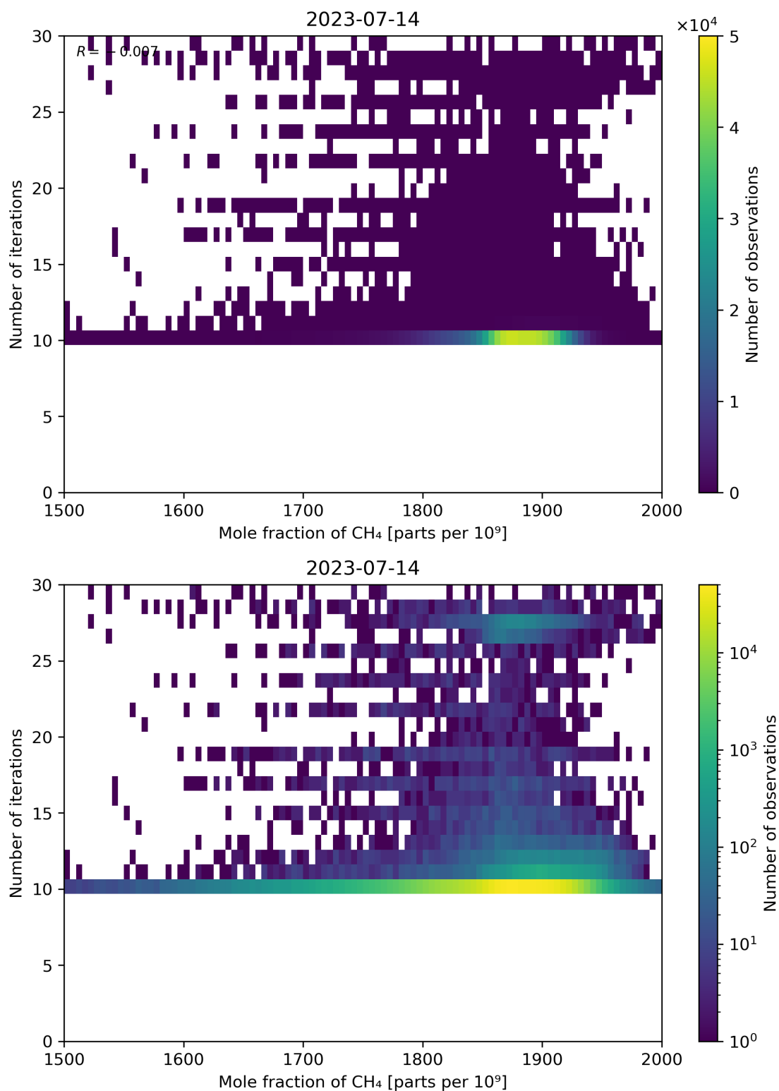
Figure 76: Scatter density plot of “Mole fraction of CH 4 ” against “Number of iterations” for 2023-07-14 to 2023-07-15.
