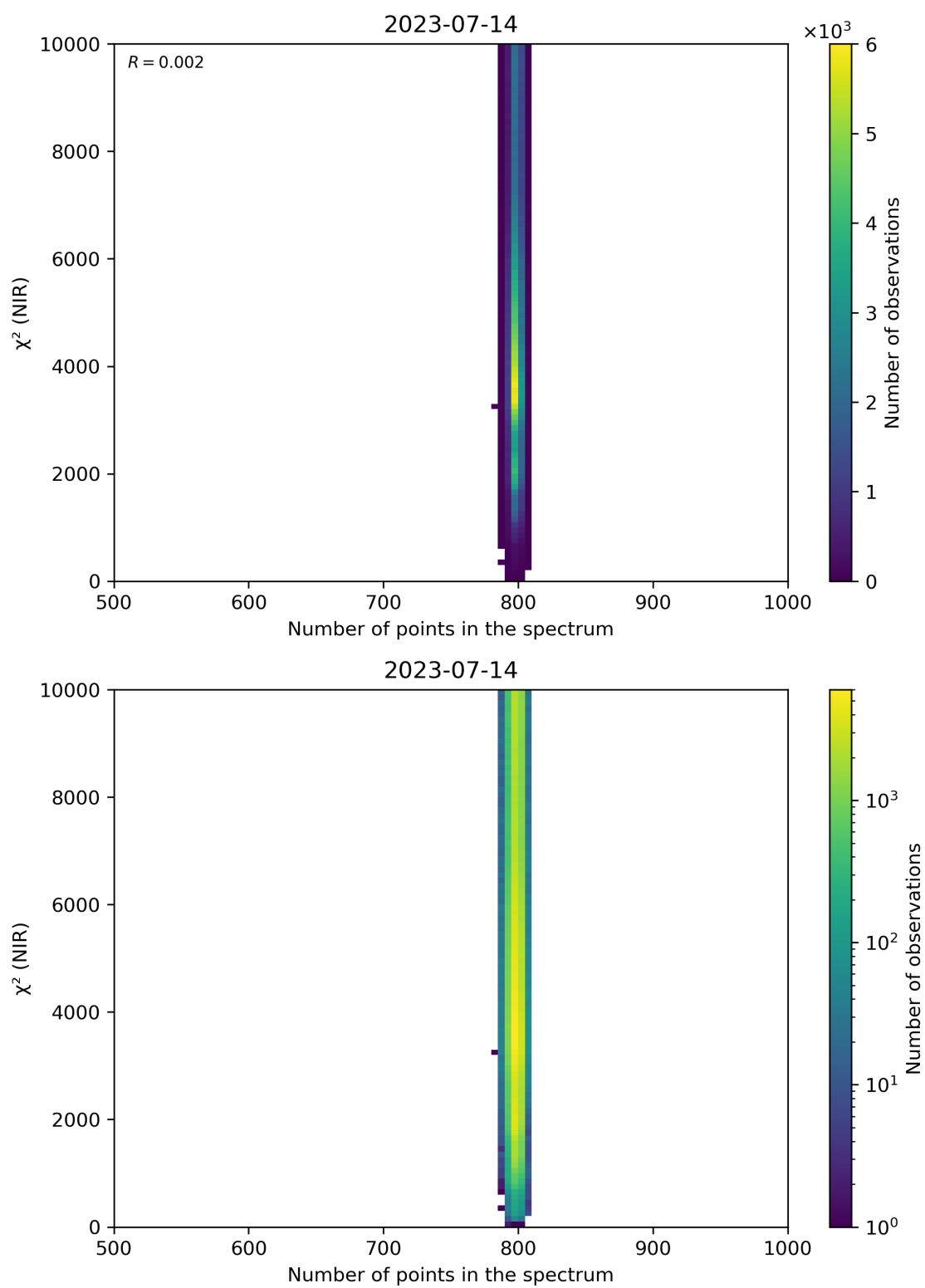
Figure 88: Scatter density plot of “Number of points in the spectrum” against “ \chi^2 (NIR)” for 2023-07-14 to 2023-07-15.
