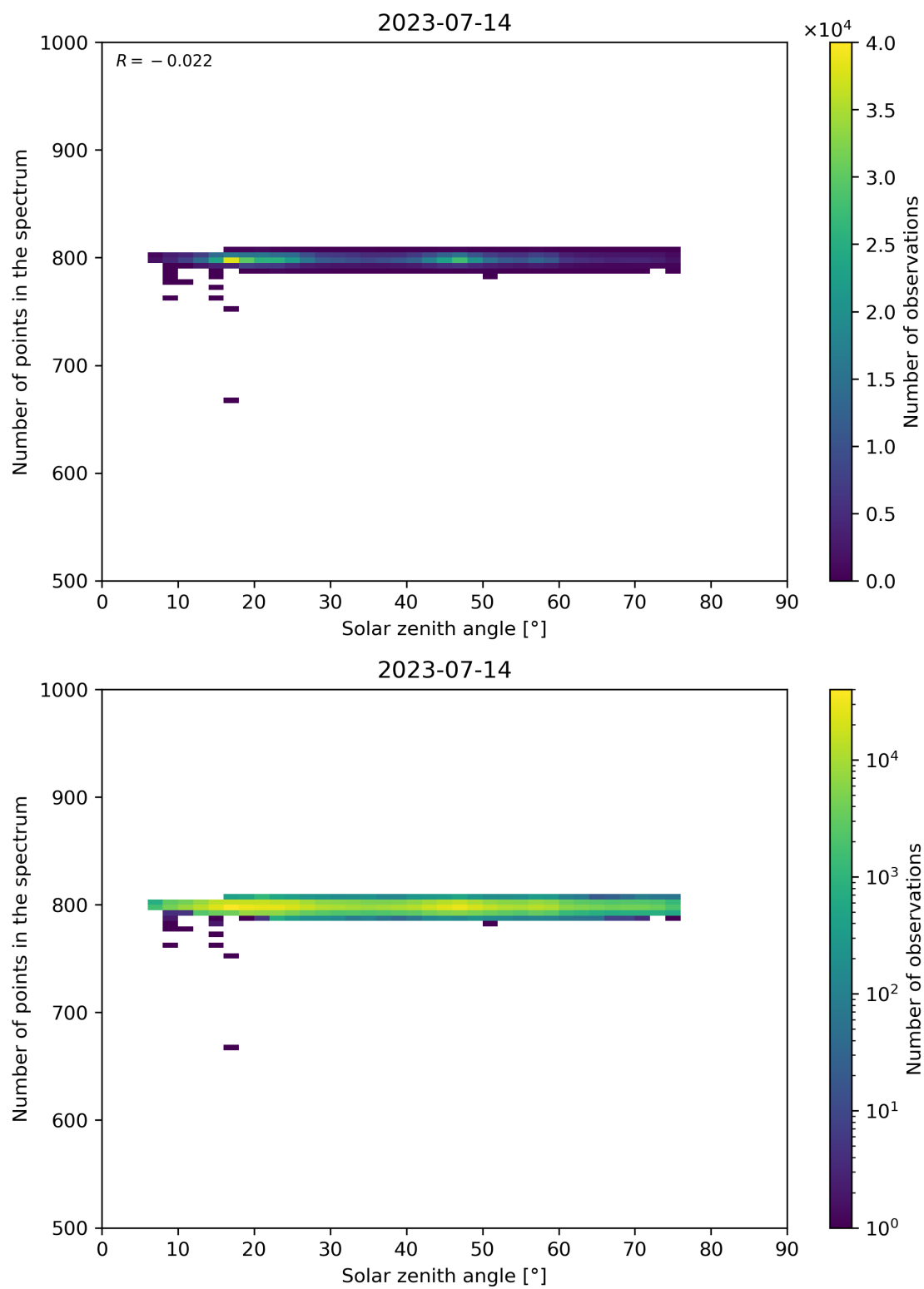
Figure 103: Scatter density plot of “Solar zenith angle” against “Number of points in the spectrum” for 2023-07-14 to 2023-07-15.
