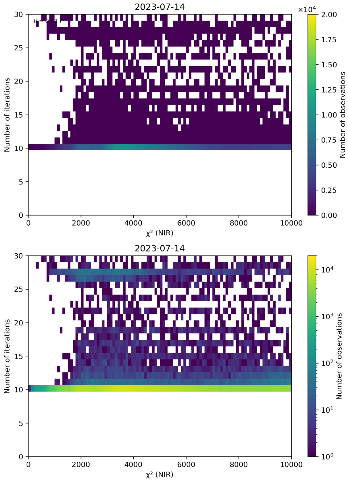
Figure 46: Scatter density plot of “ \chi^2 (NIR)” against “Number of iterations” for 2023-07-14 to 2023-07-15.
