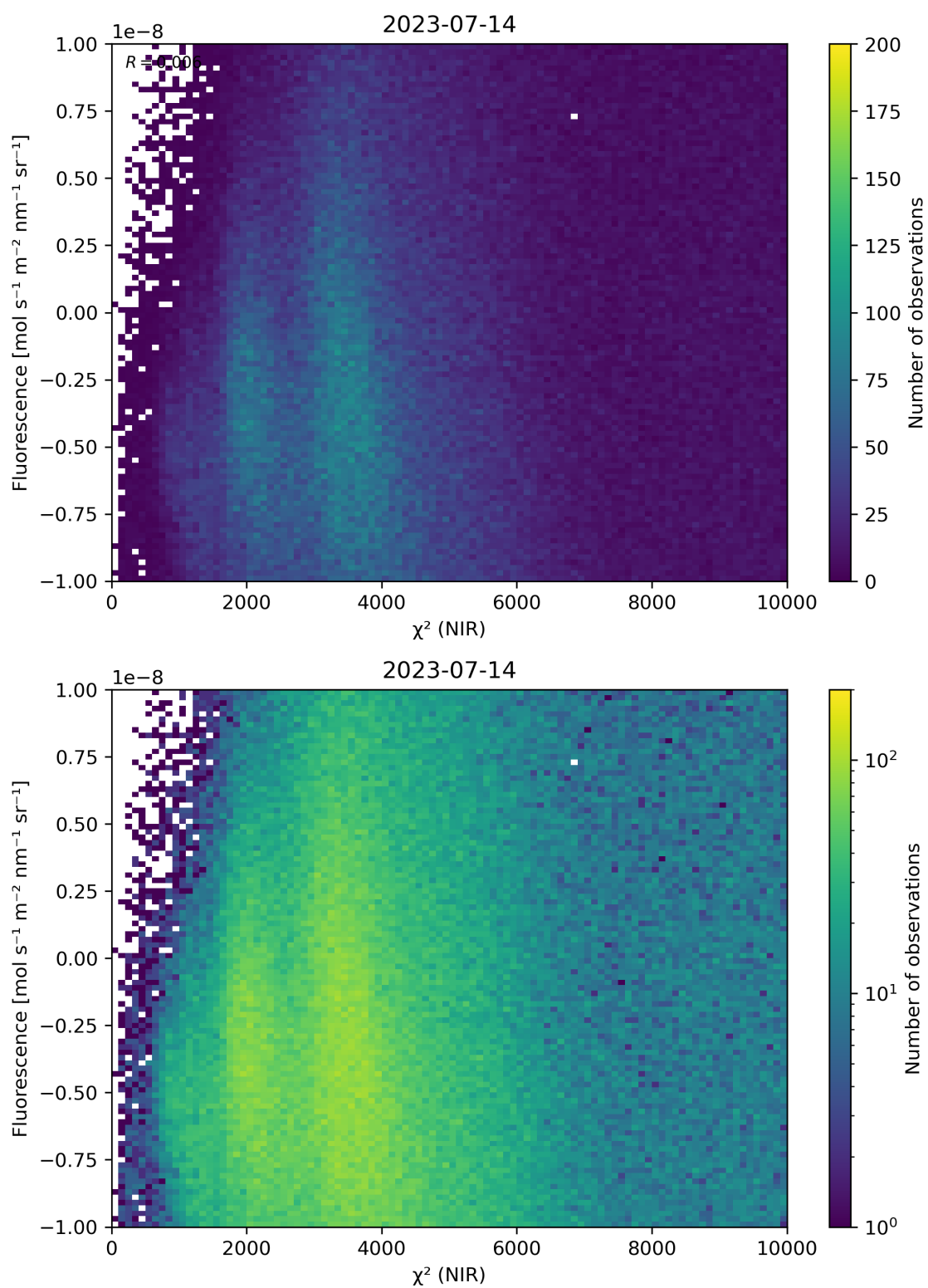
Figure 45: Scatter density plot of “ \chi^2 (NIR)” against “Fluorescence” for 2023-07-14 to 2023-07-15.
