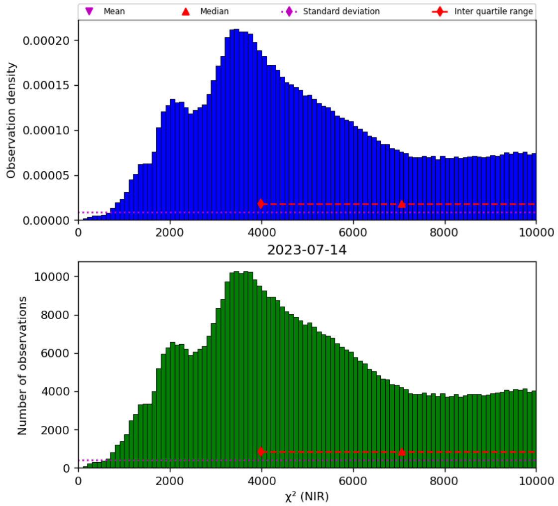
Figure 29: Histogram of " \chi^2 (NIR)" for 2023-07-14 to 2023-07-15
