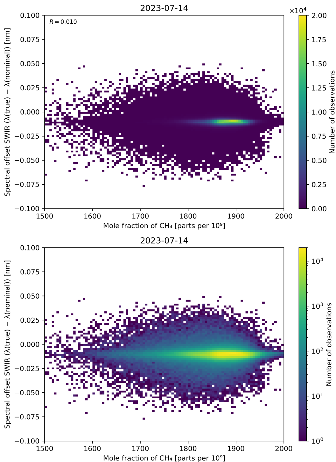
Figure 86: Scatter density plot of “Mole fraction of CH 4 ” against “Spectral offset SWIR ( \lambda(\text{true}) - \lambda(\text{nominal}) )” for 2023-07-14 to 2023-07-15.
