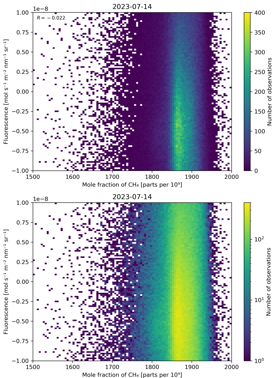
Figure 73: Scatter density plot of “Mole fraction of \text{CH}_4 ” against “Fluorescence” for 2023-07-14 to 2023-07-15.
