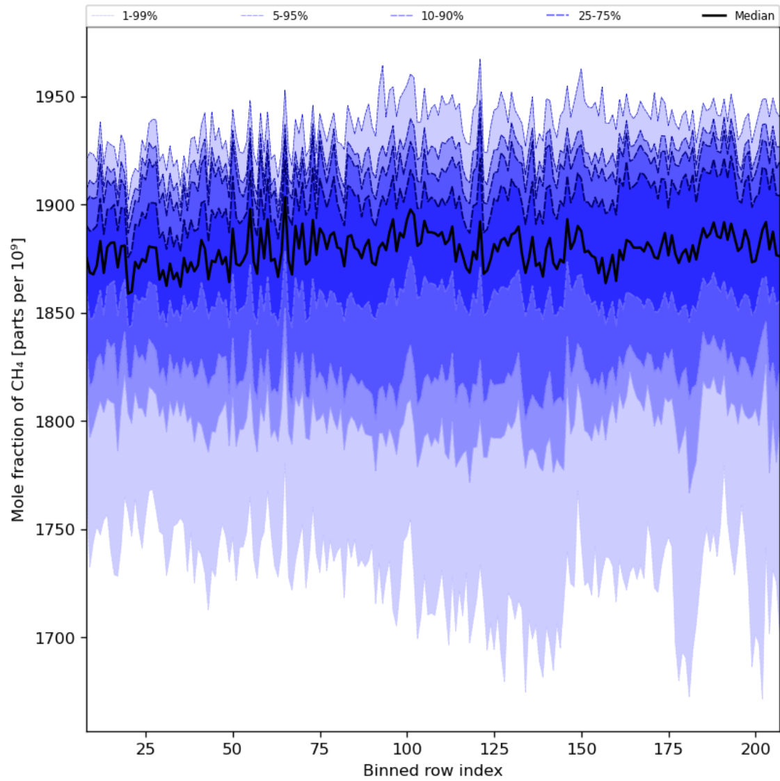
Figure 34: Along track statistics of “Mole fraction of CH 4 ” for 2023-07-14 to 2023-07-15
