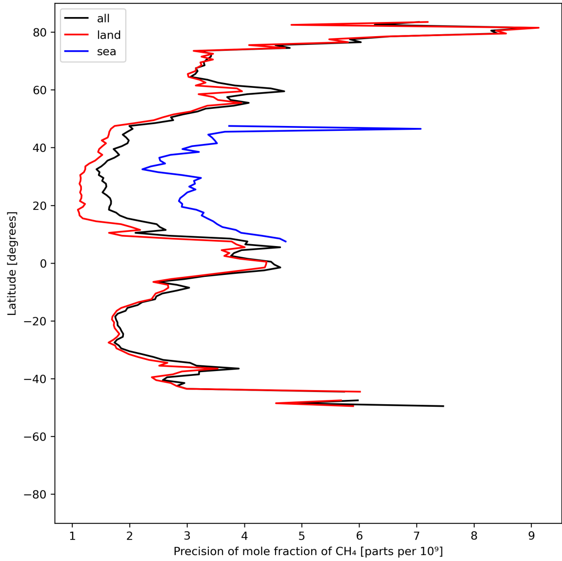
Figure 13: Zonal average of “Precision of mole fraction of CH 4 ” for 2023-07-14 to 2023-07-15.
