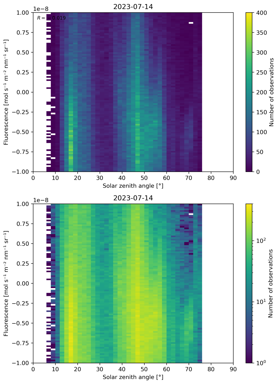
Figure 97: Scatter density plot of “Solar zenith angle” against “Fluorescence” for 2023-07-14 to 2023-07-15.
