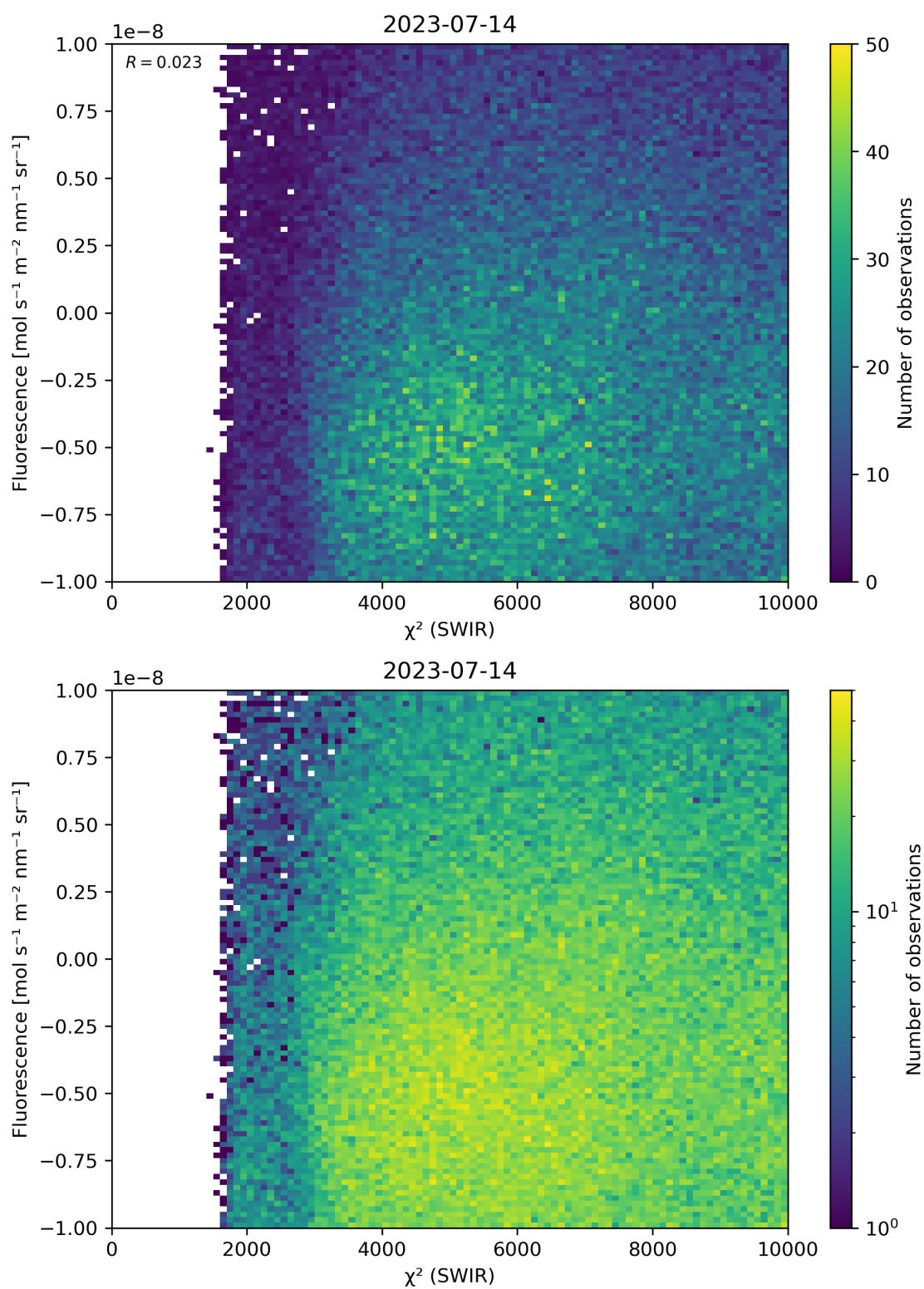
Figure 49: Scatter density plot of “ \chi^2 (SWIR)” against “Fluorescence” for 2023-07-14 to 2023-07-15.
