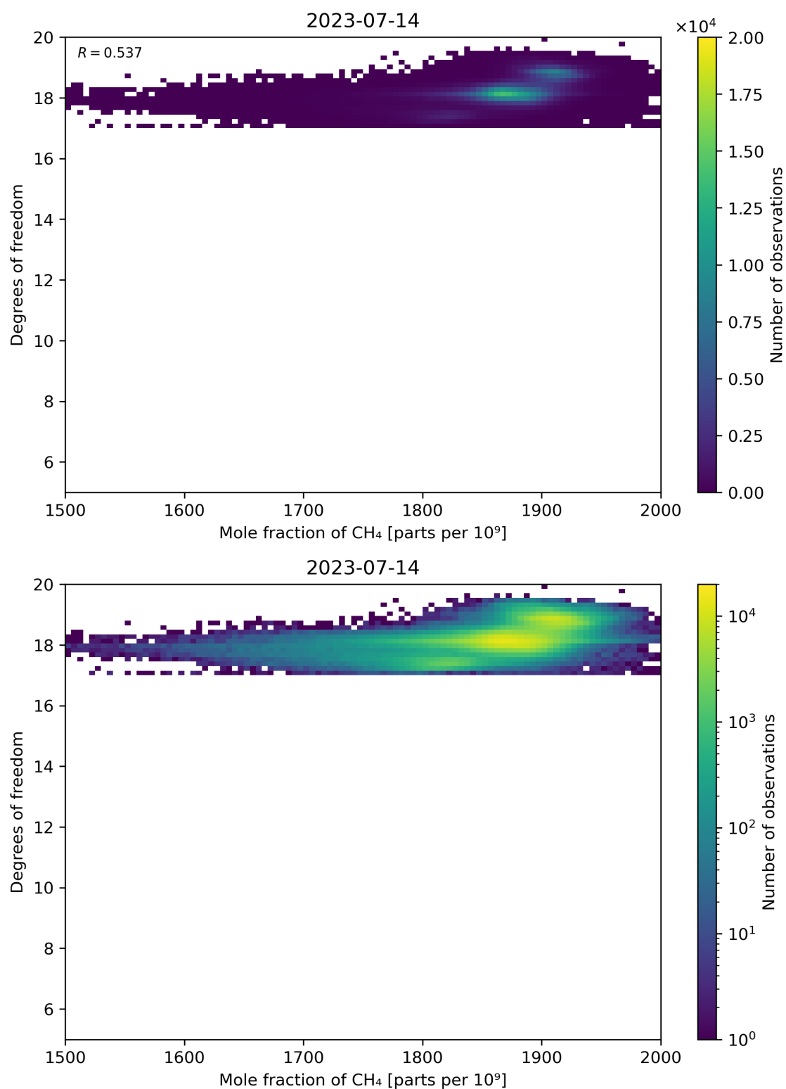
Figure 72: Scatter density plot of “Mole fraction of CH 4 ” against “Degrees of freedom” for 2023-07-14 to 2023-07-15.
