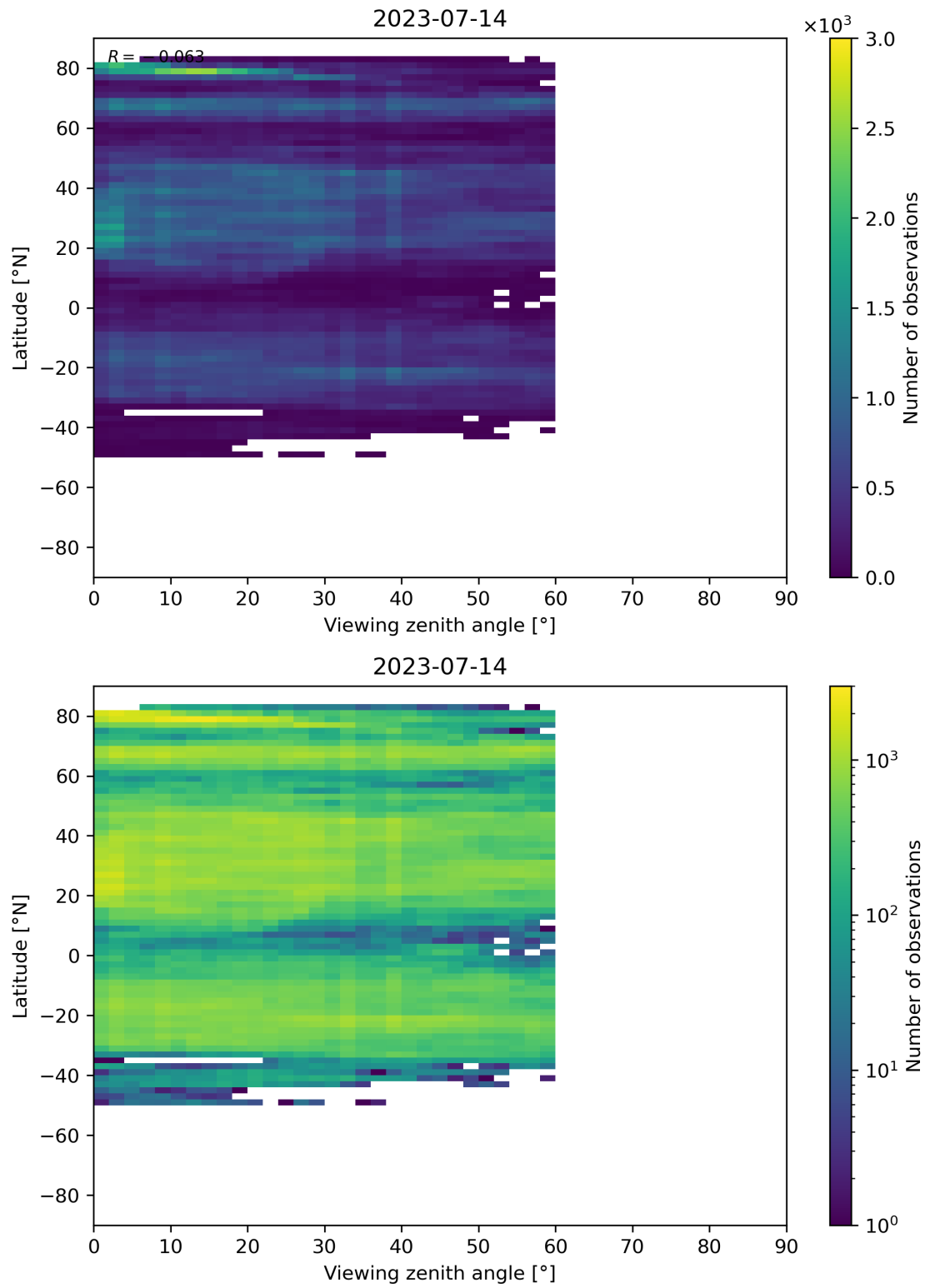
Figure 109: Scatter density plot of “Viewing zenith angle” against “Latitude” for 2023-07-14 to 2023-07-15.
