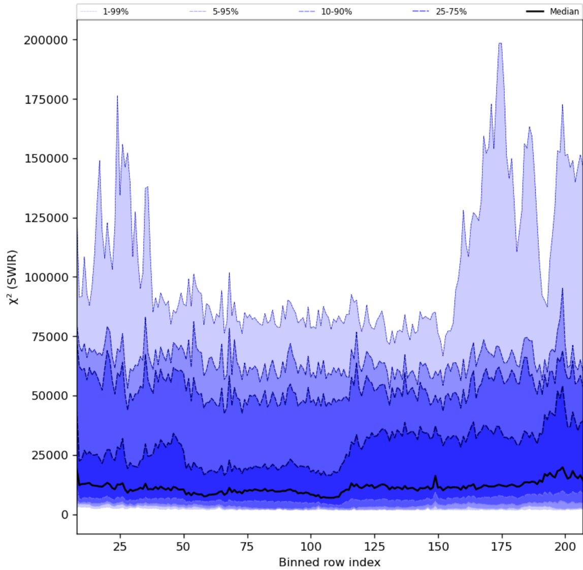
Figure 39: Along track statistics of " \chi^2 (SWIR)" for 2023-07-14 to 2023-07-15
