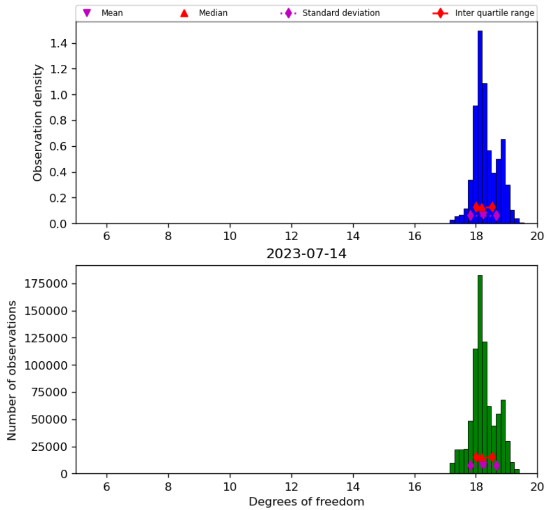
Figure 30: Histogram of “Degrees of freedom” for 2023-07-14 to 2023-07-15
