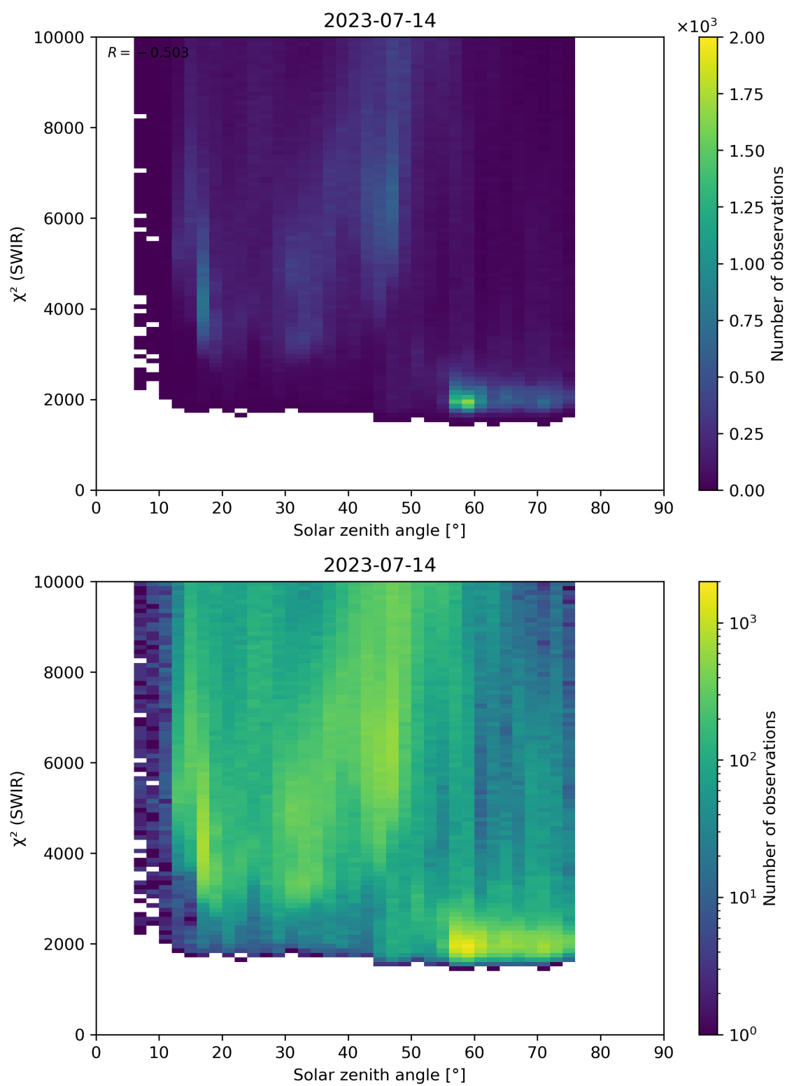
Figure 95: Scatter density plot of “Solar zenith angle” against “ \chi^2 (SWIR)” for 2023-07-14 to 2023-07-15.
