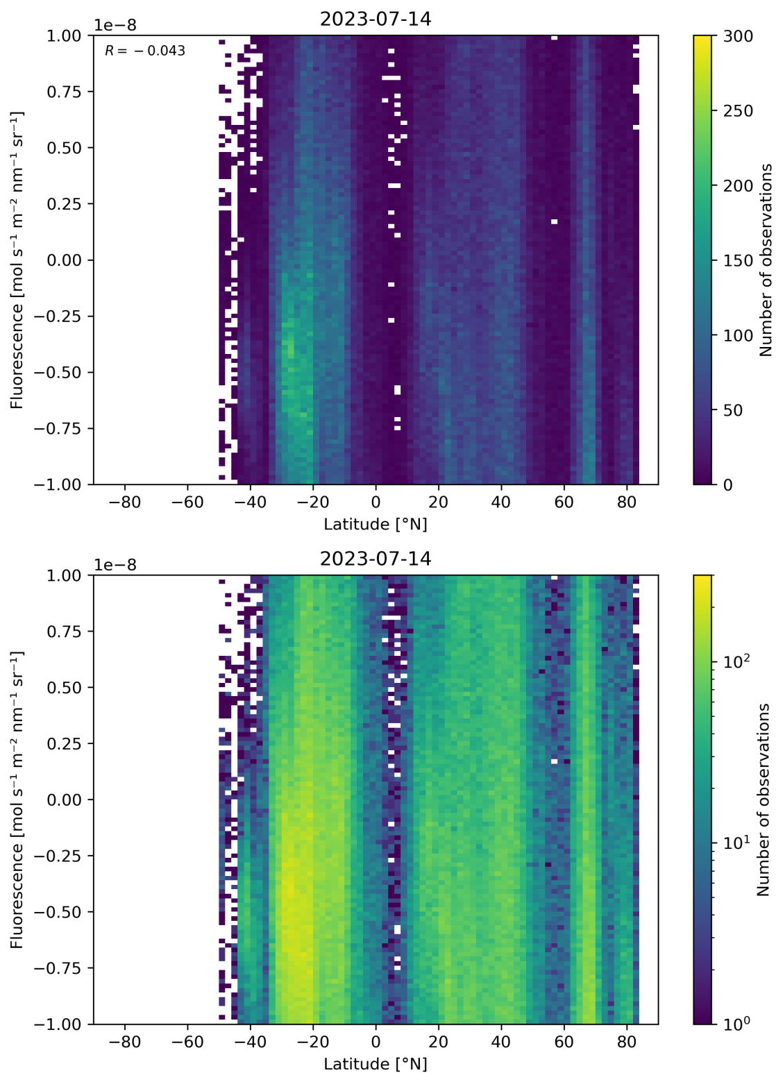
Figure 56: Scatter density plot of “Latitude” against “Fluorescence” for 2023-07-14 to 2023-07-15.
