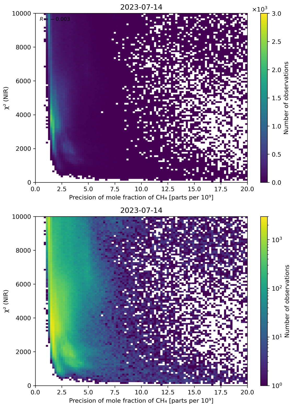
Figure 78: Scatter density plot of “Precision of mole fraction of CH 4 ” against “ \chi^2 (NIR)” for 2023-07-14 to 2023-07-15.
