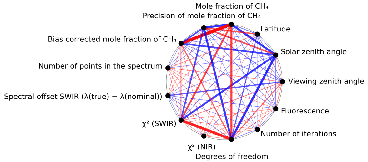
Figure 1: Map of correlation graph for 2023-07-14 to 2023-07-15.
