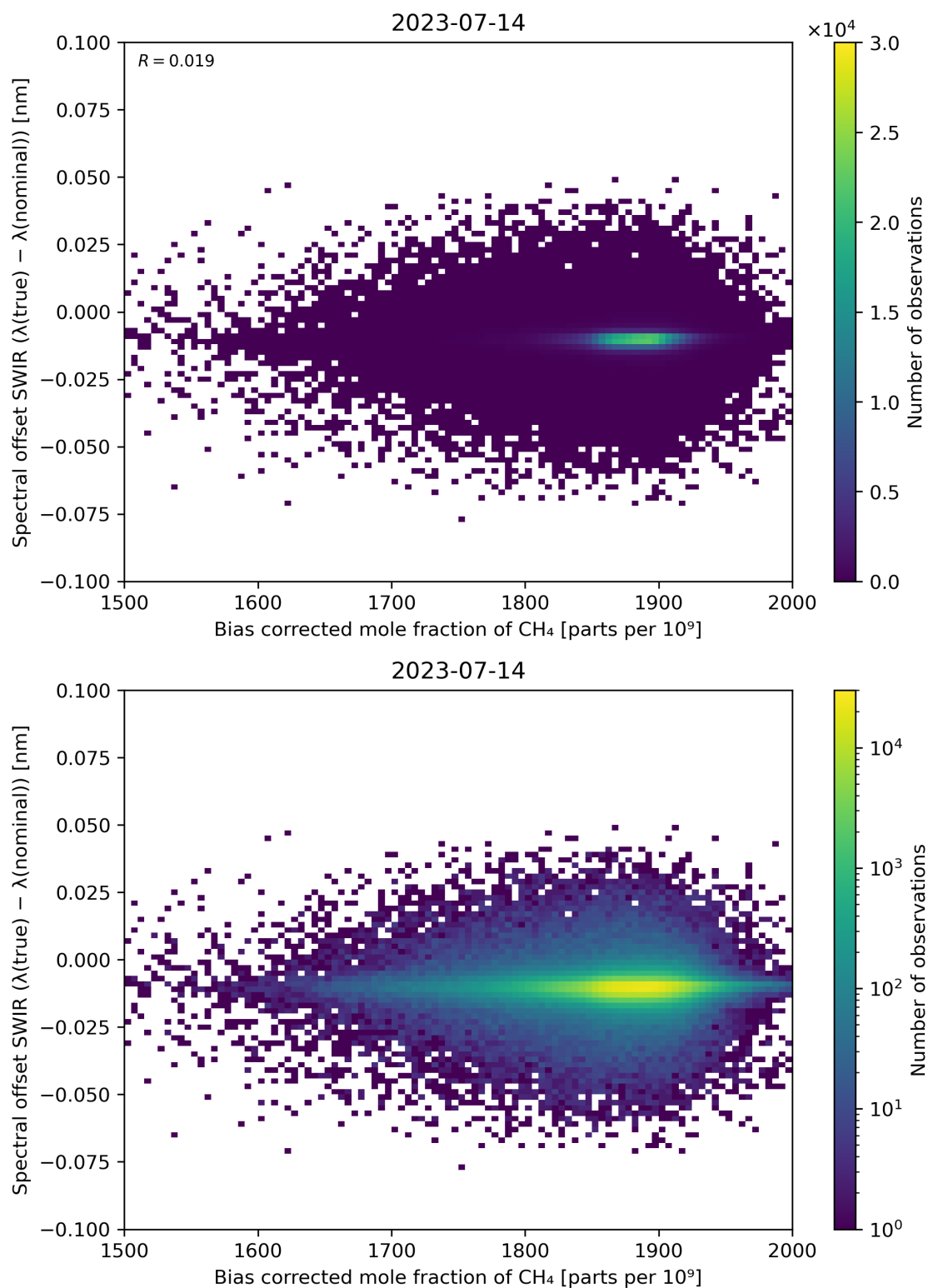
Figure 69: Scatter density plot of “Bias corrected mole fraction of \text{CH}_4 ” against “Spectral offset SWIR ( \lambda(\text{true}) - \lambda(\text{nominal}) )” for 2023-07-14 to 2023-07-15.
