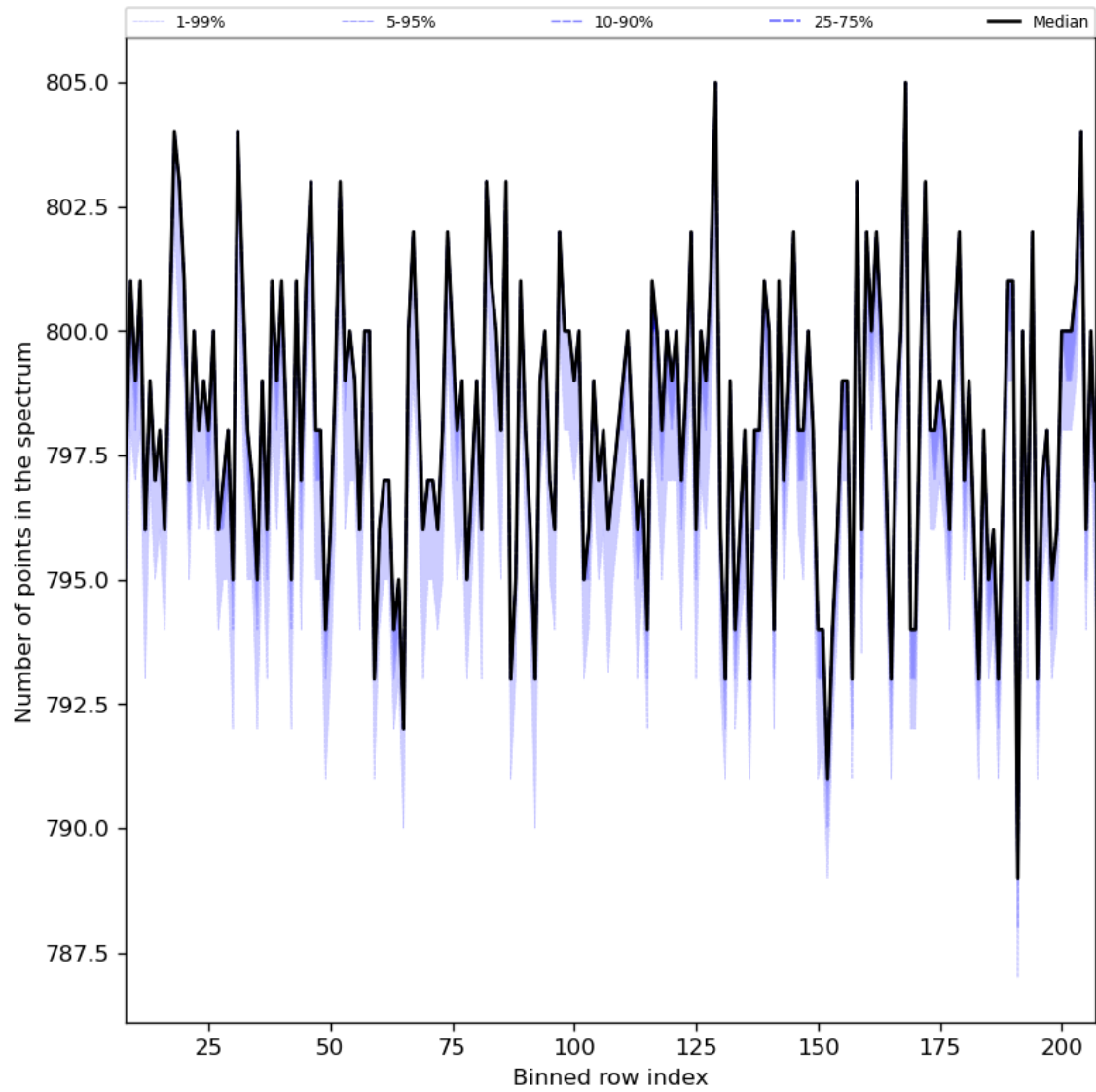
Figure 37: Along track statistics of “Number of points in the spectrum” for 2023-07-14 to 2023-07-15
