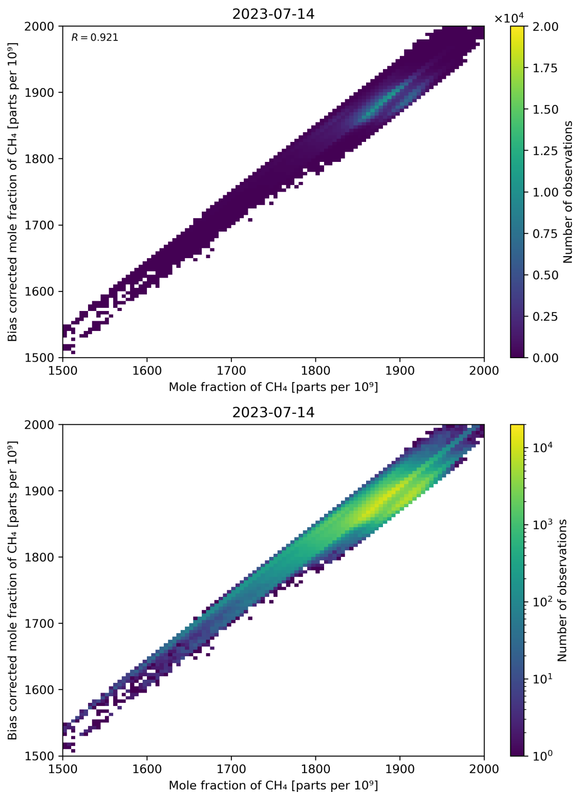
Figure 74: Scatter density plot of “Mole fraction of CH 4 ” against “Bias corrected mole fraction of CH 4 ” for 2023-07-14 to 2023-07-15.
