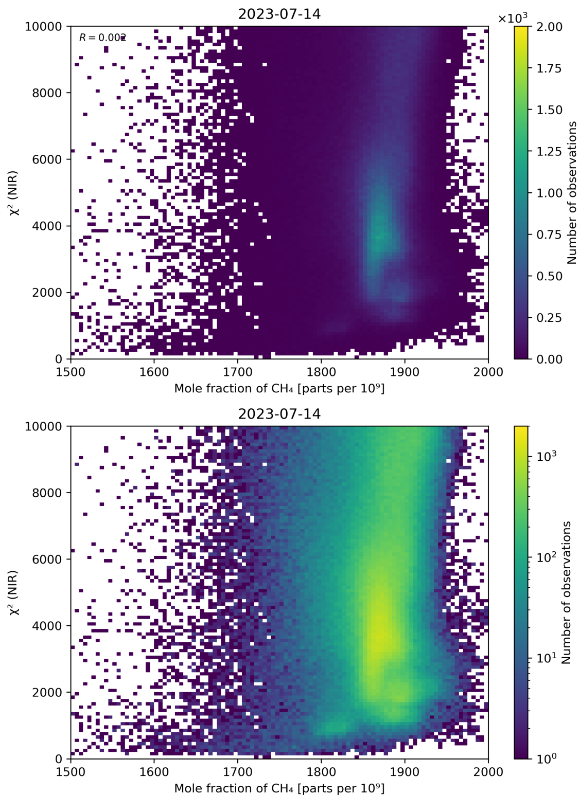
Figure 70: Scatter density plot of “Mole fraction of \text{CH}_4 ” against “ \chi^2 (NIR)” for 2023-07-14 to 2023-07-15.
