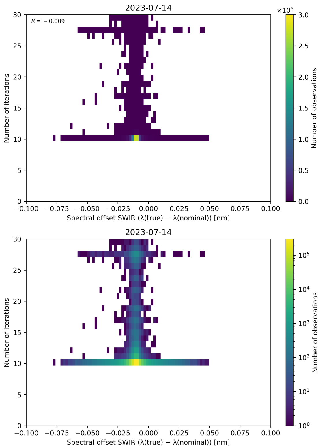
Figure 121: Scatter density plot of “Spectral offset SWIR ( \lambda(\text{true}) - \lambda(\text{nominal}) )” against “Number of iterations” for 2023-07-14 to 2023-07-15.
