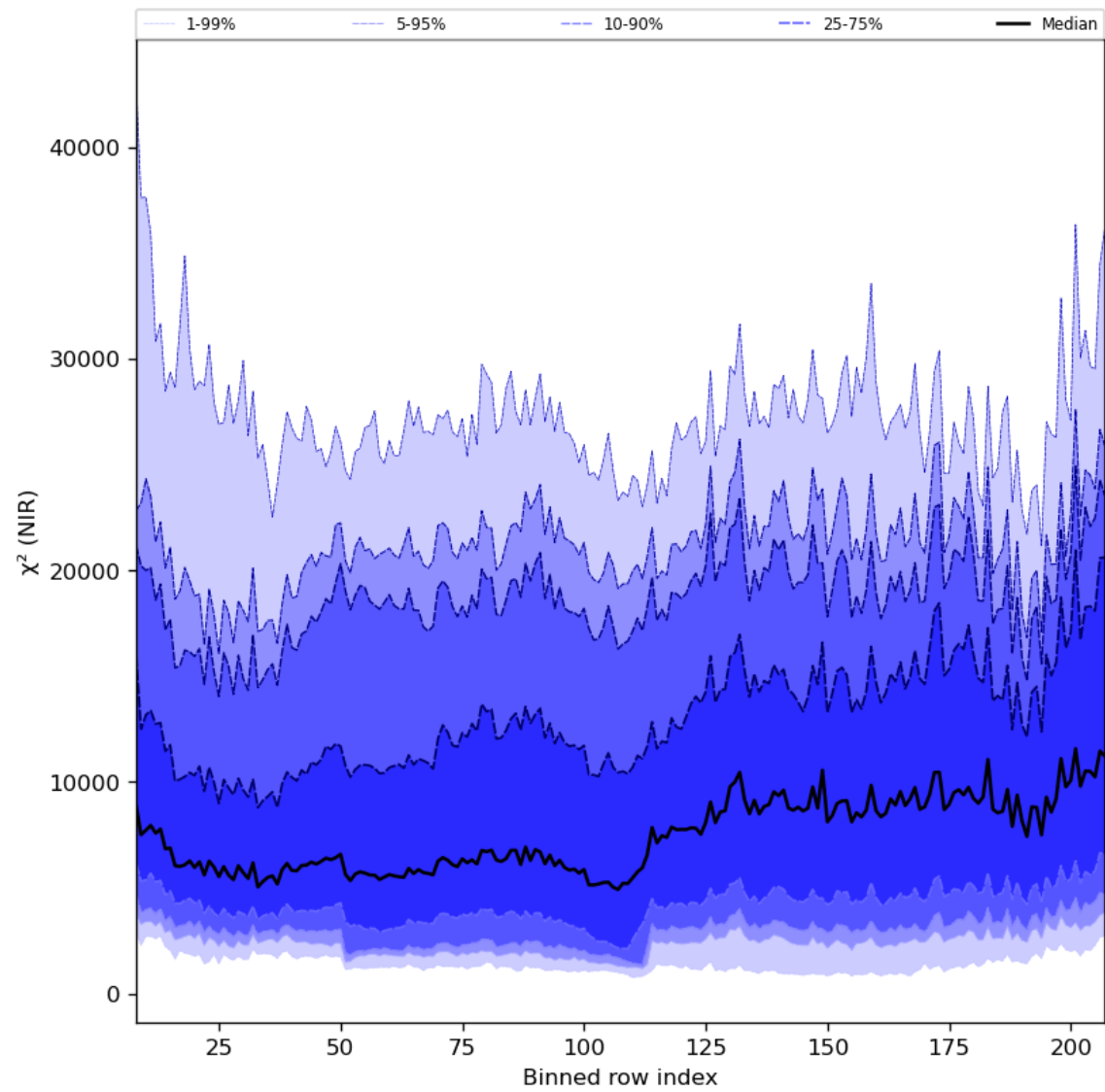
Figure 40: Along track statistics of “ \chi^2 (NIR)” for 2023-07-14 to 2023-07-15
