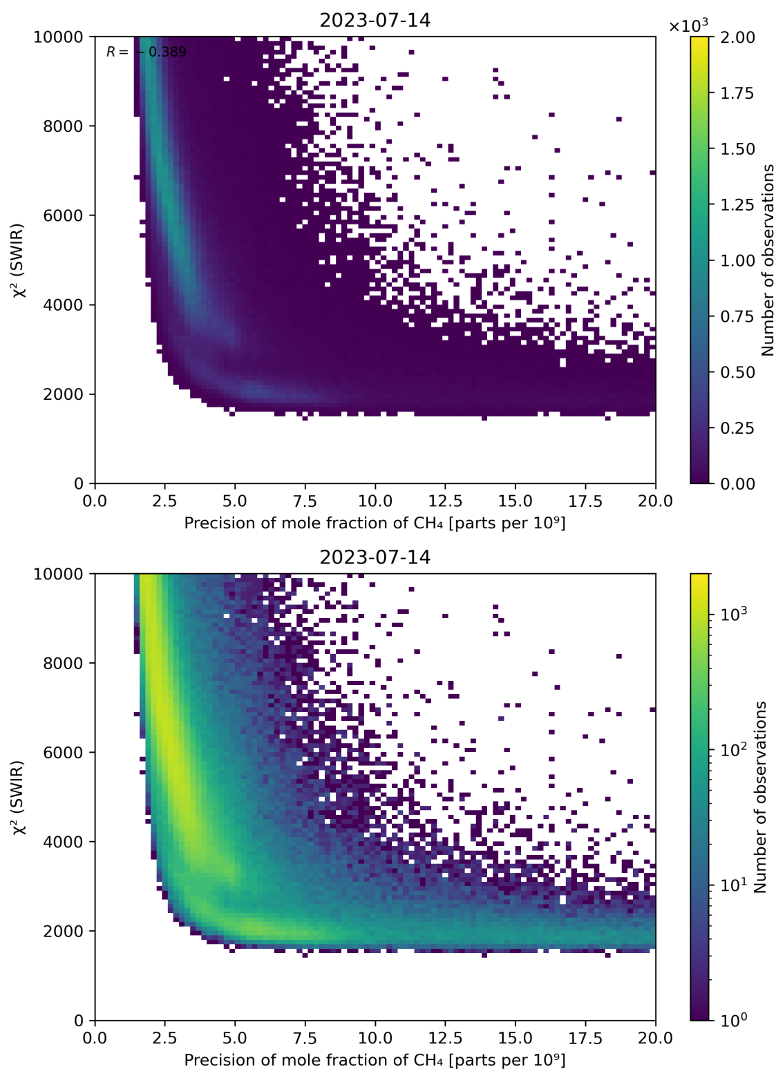
Figure 79: Scatter density plot of “Precision of mole fraction of \text{CH}_4 ” against “ \chi^2 (SWIR)” for 2023-07-14 to 2023-07-15.
