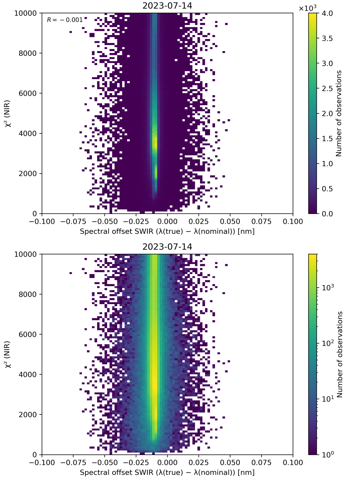
Figure 117: Scatter density plot of “Spectral offset SWIR ( \lambda(\text{true}) - \lambda(\text{nominal}) )” against “ \chi^2 (NIR)” for 2023-07-14 to 2023-07-15.
