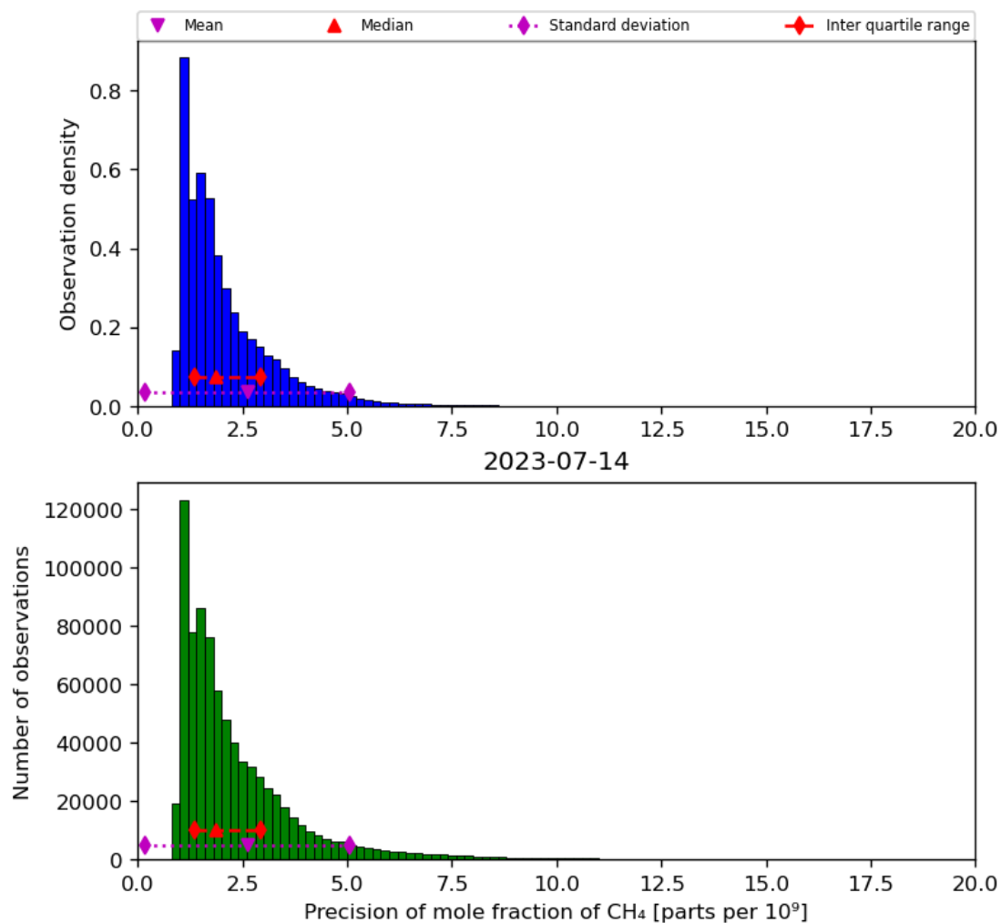
Figure 24: Histogram of “Precision of mole fraction of CH 4 ” for 2023-07-14 to 2023-07-15
