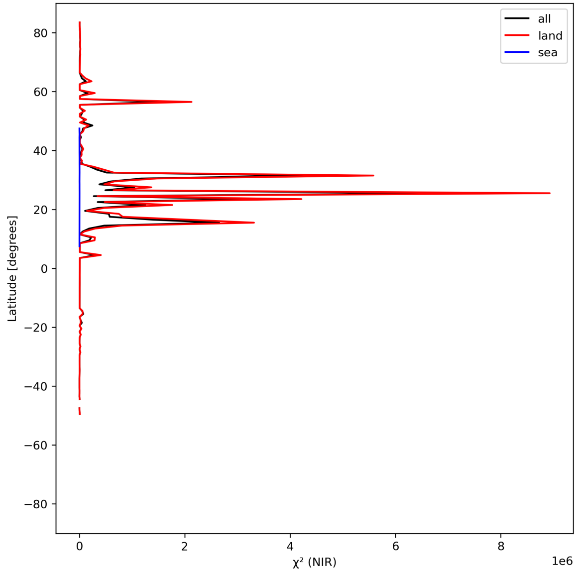
Figure 18: Zonal average of “ \chi^2 (NIR)” for 2023-07-14 to 2023-07-15.
