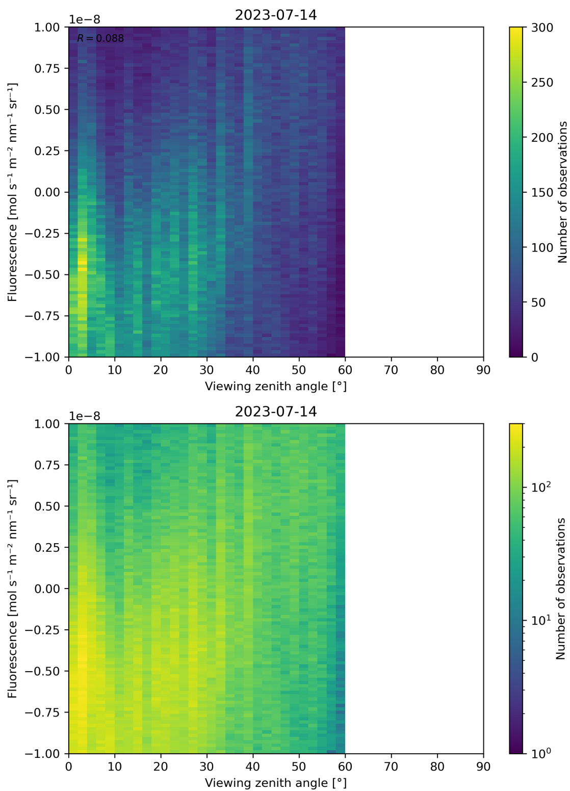
Figure 108: Scatter density plot of “Viewing zenith angle” against “Fluorescence” for 2023-07-14 to 2023-07-15.
