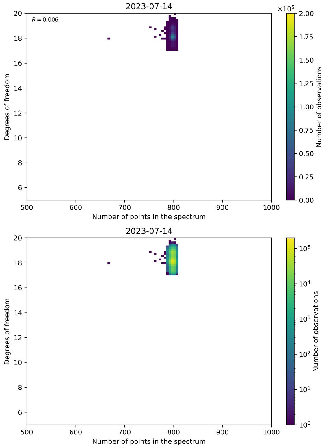
Figure 90: Scatter density plot of “Number of points in the spectrum” against “Degrees of freedom” for 2023-07-14 to 2023-07-15.
