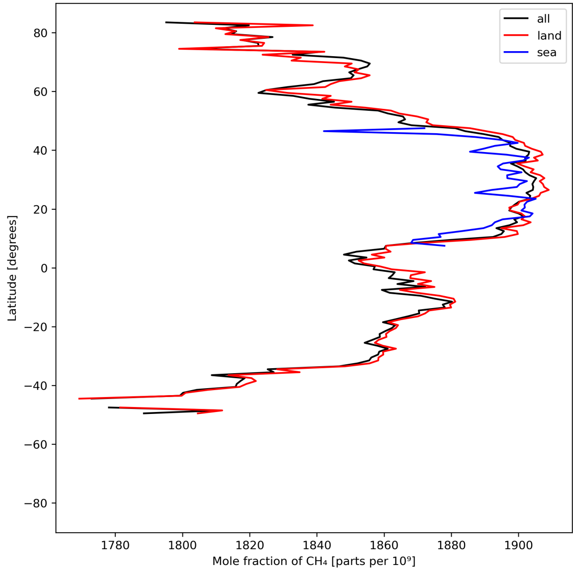
Figure 12: Zonal average of “Mole fraction of \text{CH}_4 ” for 2023-07-14 to 2023-07-15.
