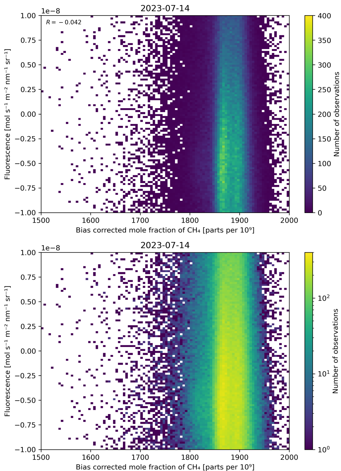
Figure 66: Scatter density plot of “Bias corrected mole fraction of \text{CH}_4 ” against “Fluorescence” for 2023-07-14 to 2023-07-15.
