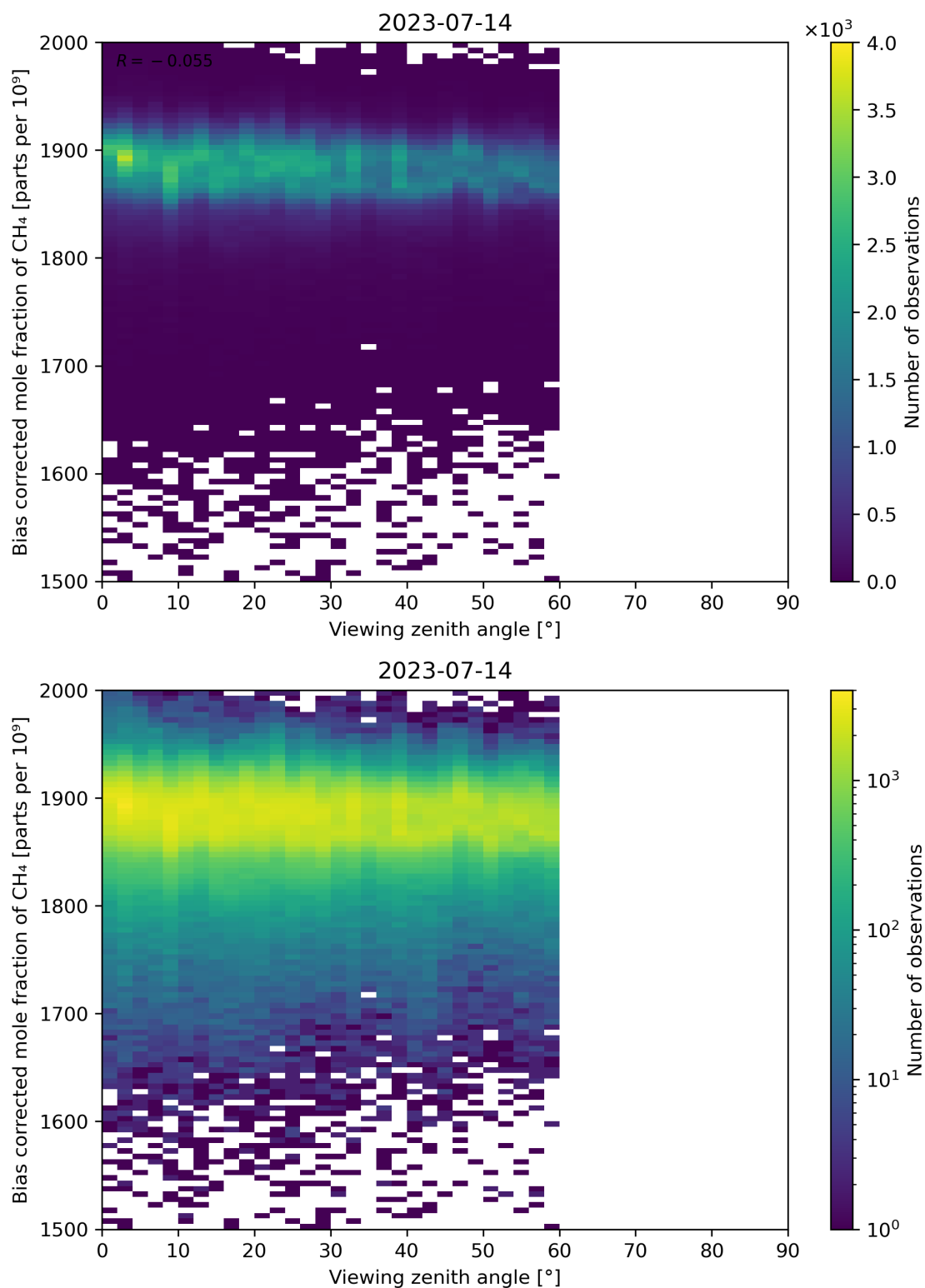
Figure 111: Scatter density plot of “Viewing zenith angle” against “Bias corrected mole fraction of CH 4 ” for 2023-07-14 to 2023-07-15.
