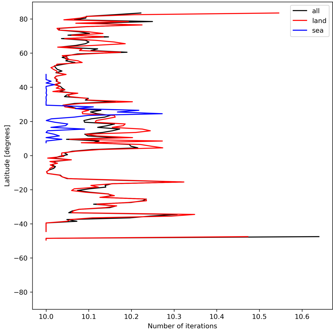
Figure 20: Zonal average of “Number of iterations” for 2023-07-14 to 2023-07-15.
