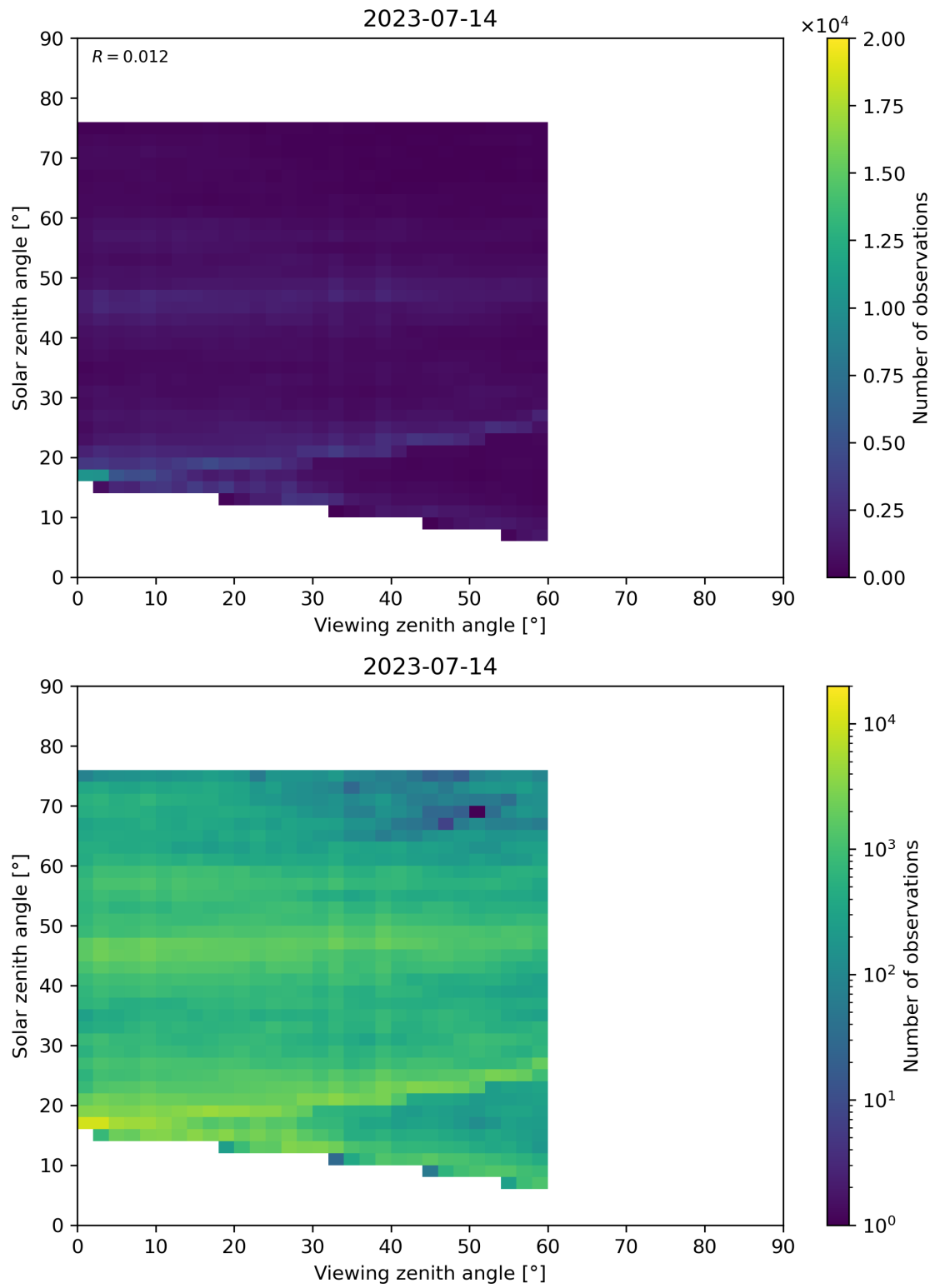
Figure 115: Scatter density plot of “Viewing zenith angle” against “Solar zenith angle” for 2023-07-14 to 2023-07-15.
