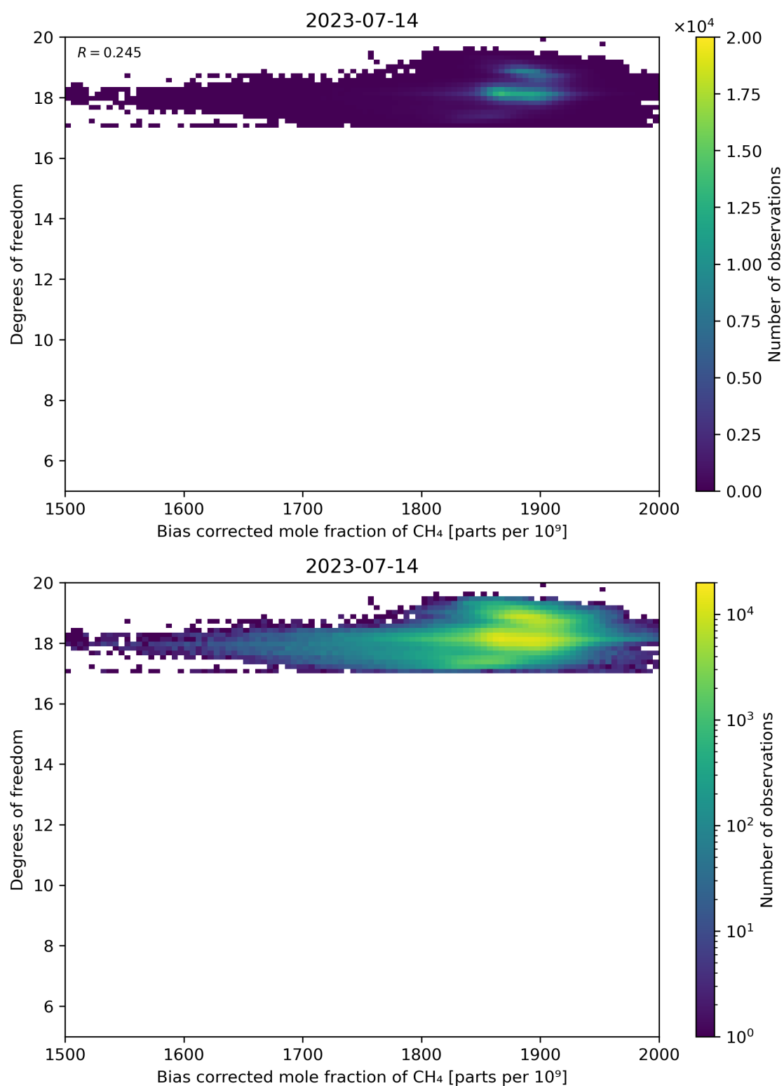
Figure 65: Scatter density plot of “Bias corrected mole fraction of CH 4 ” against “Degrees of freedom” for 2023-07-14 to 2023-07-15.
