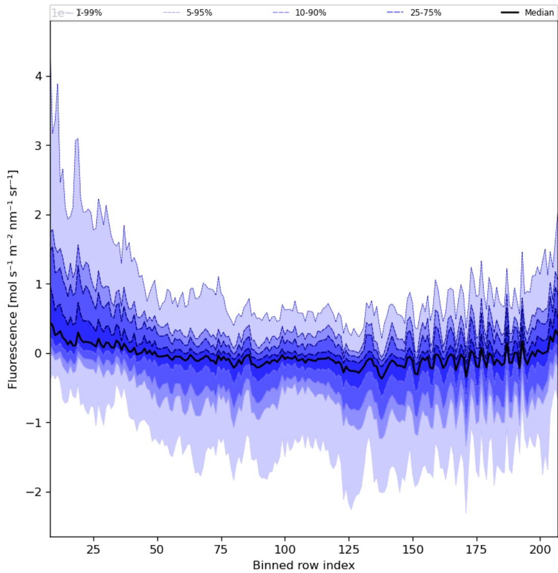
Figure 43: Along track statistics of “Fluorescence” for 2023-07-14 to 2023-07-15
