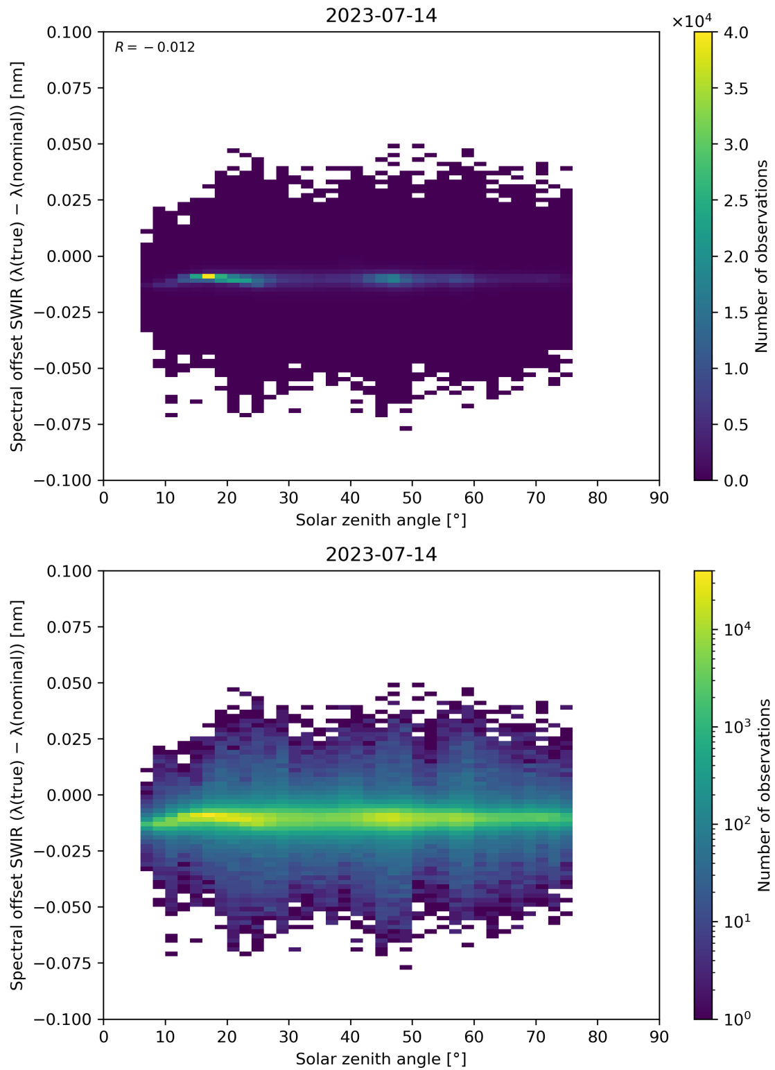
Figure 104: Scatter density plot of “Solar zenith angle” against “Spectral offset SWIR ( \lambda(\text{true}) - \lambda(\text{nominal}) )” for 2023-07-14 to 2023-07-15.
