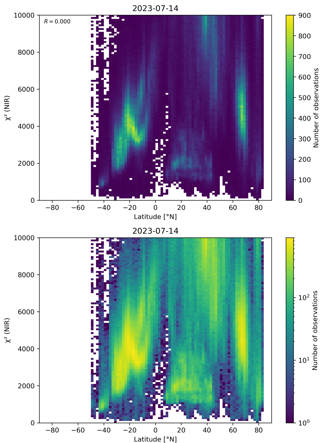
Figure 53: Scatter density plot of “Latitude” against “ \chi^2 (NIR)” for 2023-07-14 to 2023-07-15.
