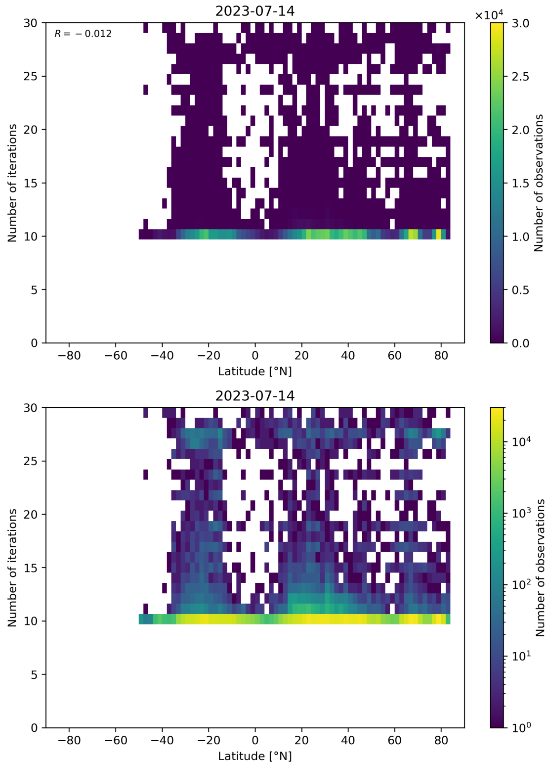
Figure 60: Scatter density plot of “Latitude” against “Number of iterations” for 2023-07-14 to 2023-07-15.
