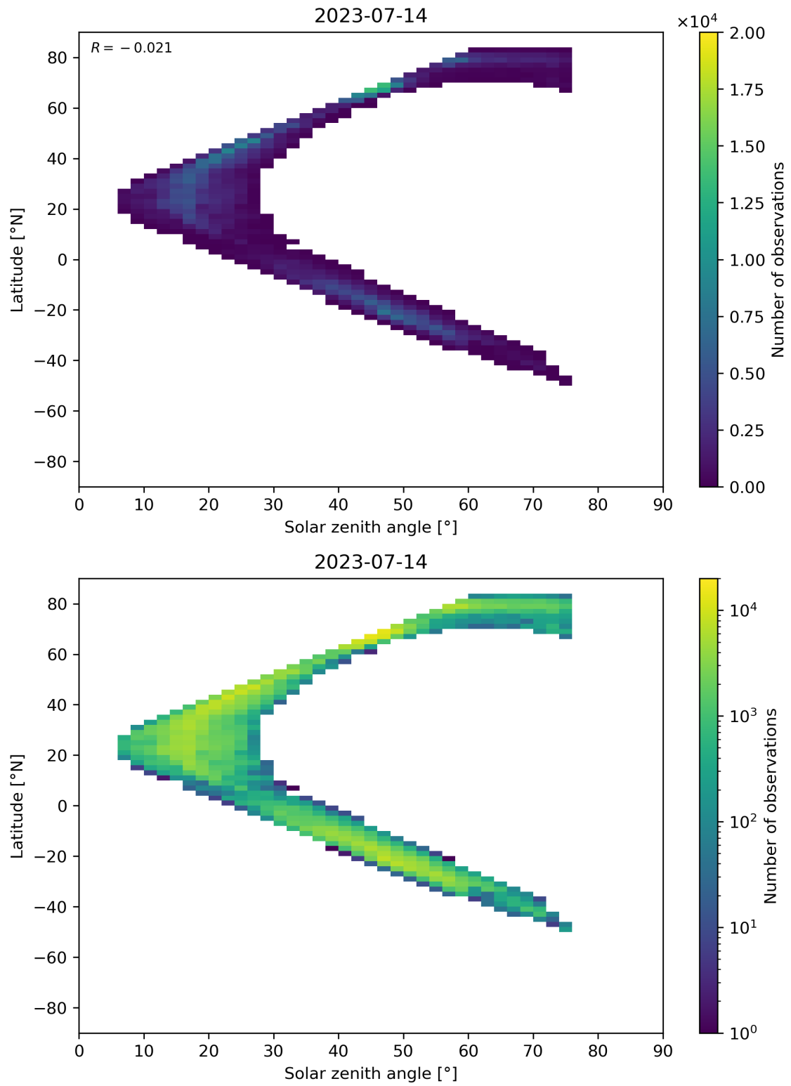
Figure 98: Scatter density plot of “Solar zenith angle” against “Latitude” for 2023-07-14 to 2023-07-15.
