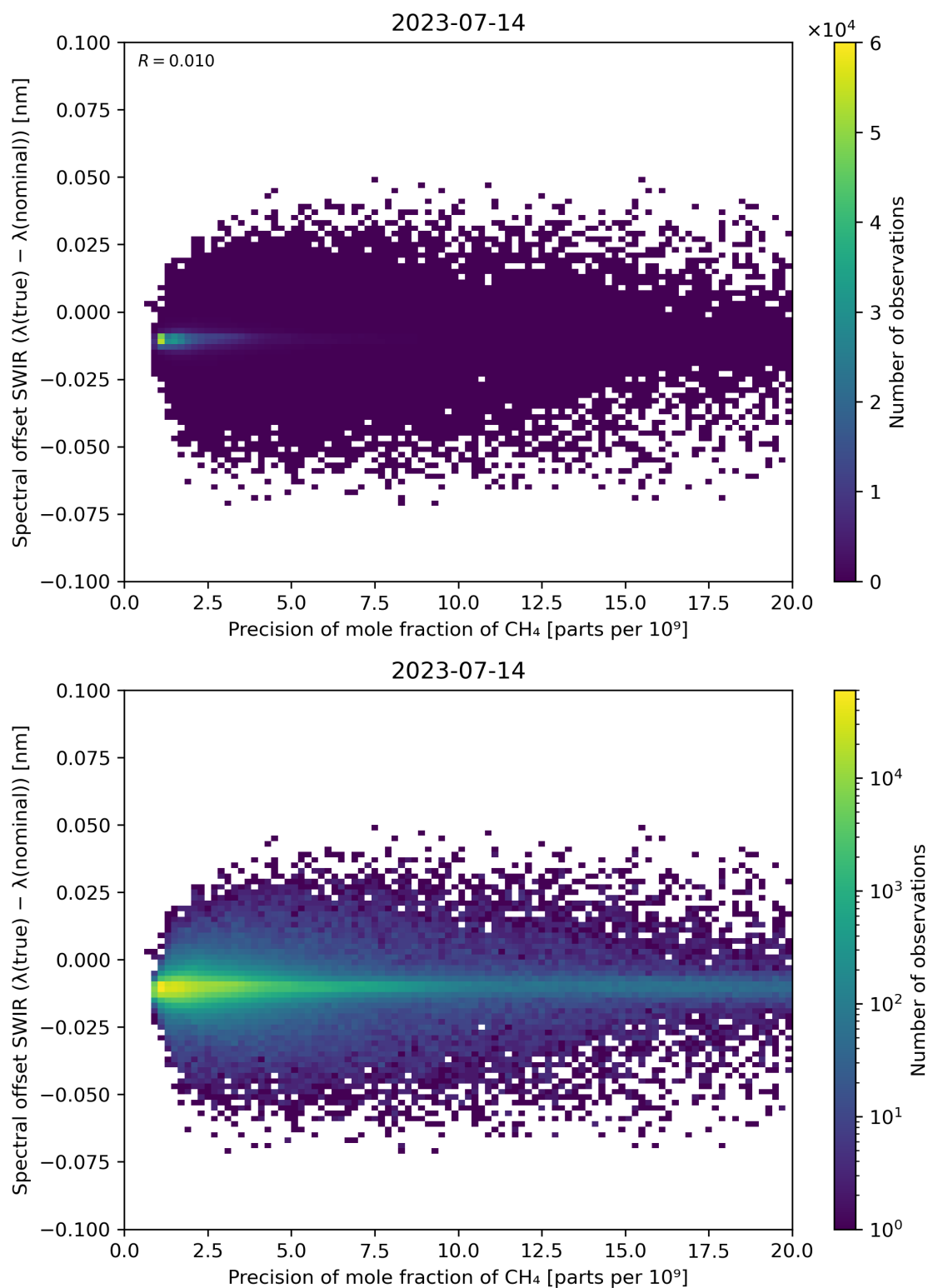
Figure 85: Scatter density plot of “Precision of mole fraction of CH 4 ” against “Spectral offset SWIR ( \lambda(\text{true}) - \lambda(\text{nominal}) )” for 2023-07-14 to 2023-07-15.
