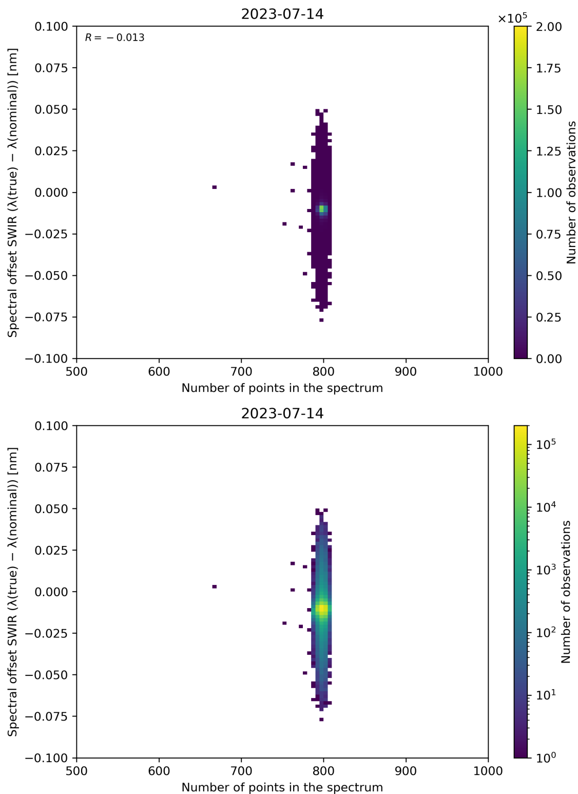
Figure 93: Scatter density plot of “Number of points in the spectrum” against “Spectral offset SWIR ( \lambda(\text{true}) - \lambda(\text{nominal}) )” for 2023-07-14 to 2023-07-15.
