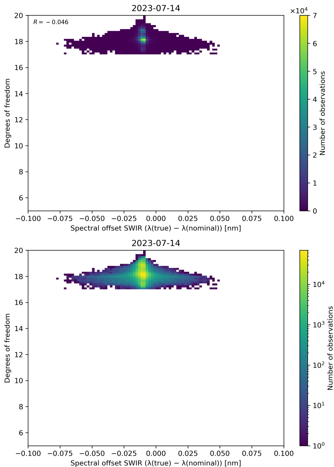
Figure 119: Scatter density plot of “Spectral offset SWIR ( \lambda(\text{true}) - \lambda(\text{nominal}) )” against “Degrees of freedom” for 2023-07-14 to 2023-07-15.
