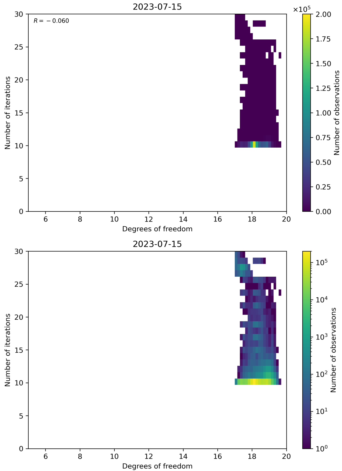
Figure 52: Scatter density plot of “Degrees of freedom” against “Number of iterations” for 2023-07-14 to 2023-07-16.
