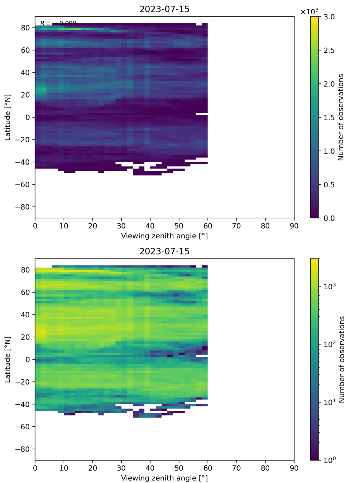
Figure 109: Scatter density plot of “Viewing zenith angle” against “Latitude” for 2023-07-14 to 2023-07-16.
