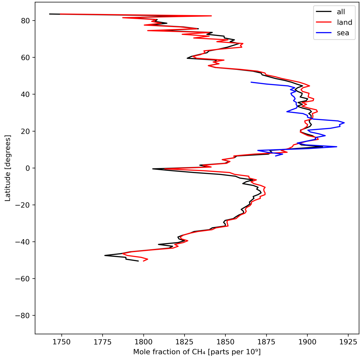
Figure 12: Zonal average of “Mole fraction of \text{CH}_4 ” for 2023-07-14 to 2023-07-16.
