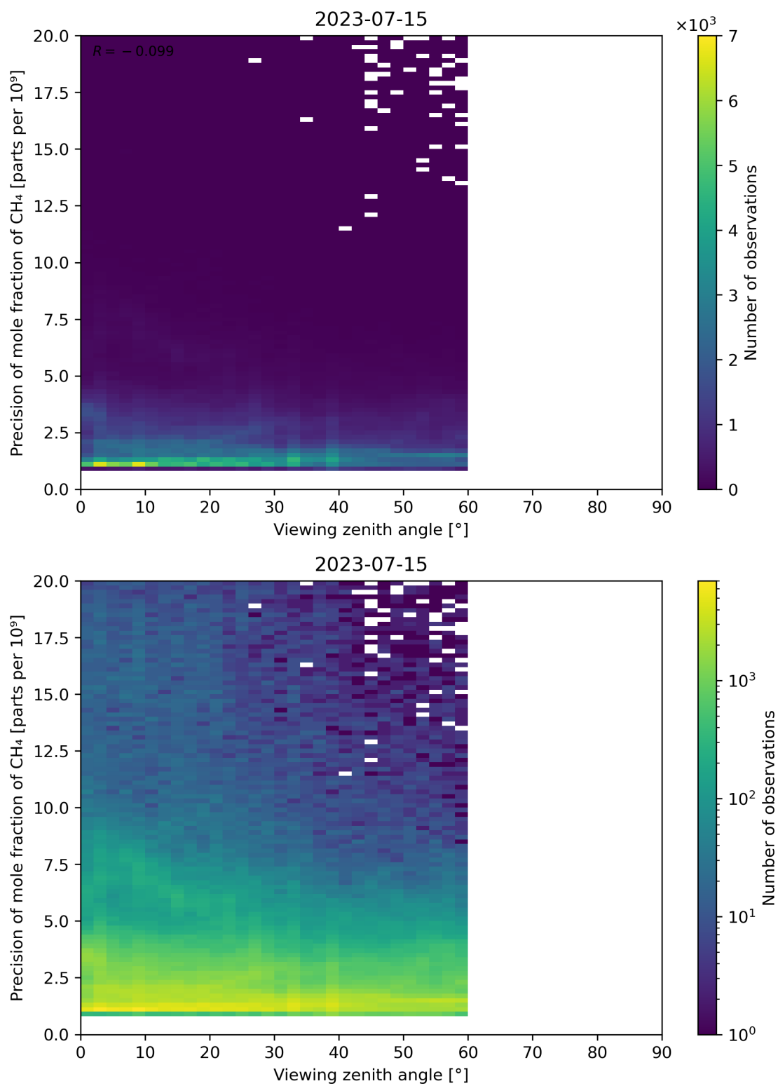
Figure 112: Scatter density plot of “Viewing zenith angle” against “Precision of mole fraction of CH 4 ” for 2023-07-14 to 2023-07-16.
