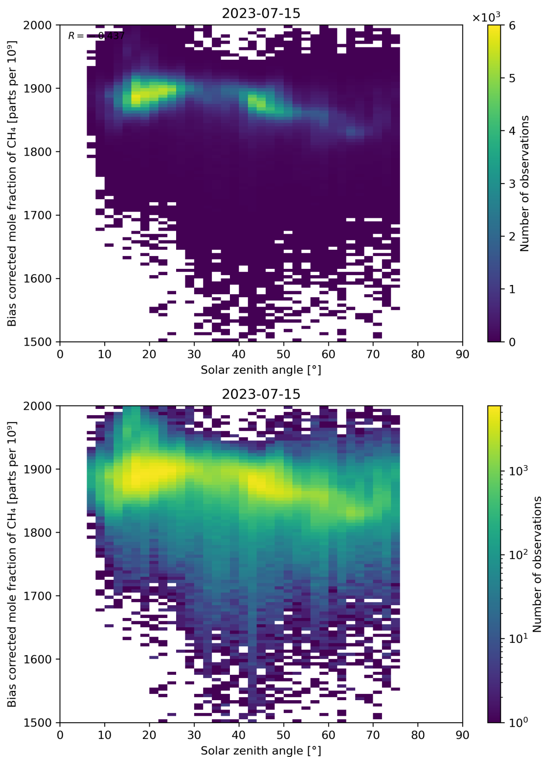
Figure 100: Scatter density plot of “Solar zenith angle” against “Bias corrected mole fraction of CH 4 ” for 2023-07-14 to 2023-07-16.
