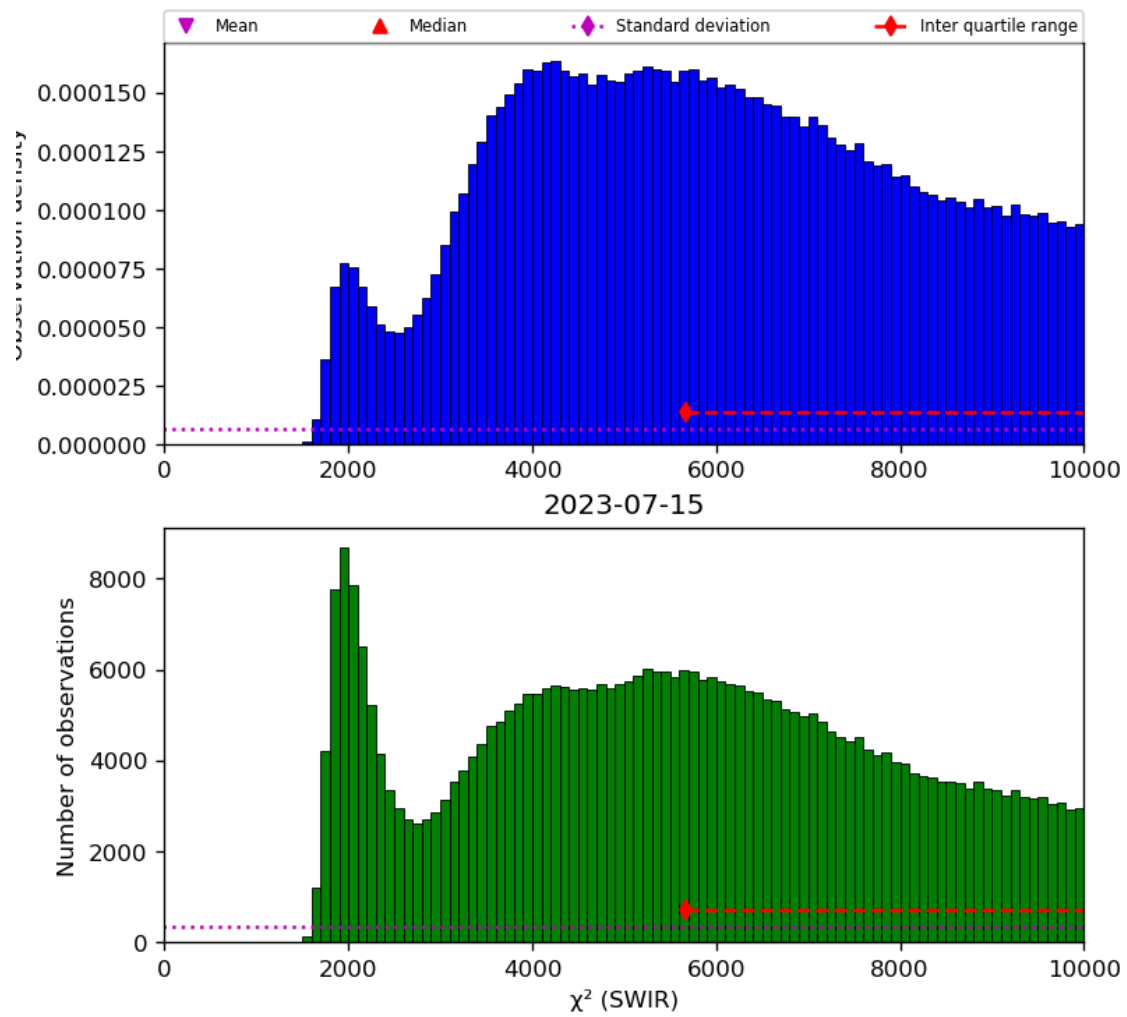
Figure 28: Histogram of “ \chi^2 (SWIR)” for 2023-07-14 to 2023-07-16
