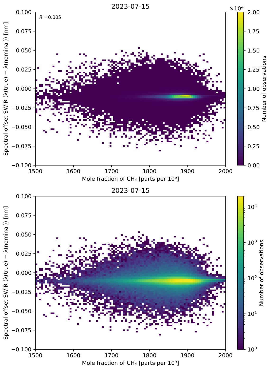
Figure 86: Scatter density plot of “Mole fraction of CH 4 ” against “Spectral offset SWIR ( \lambda(\text{true}) - \lambda(\text{nominal}) )” for 2023-07-14 to 2023-07-16.
