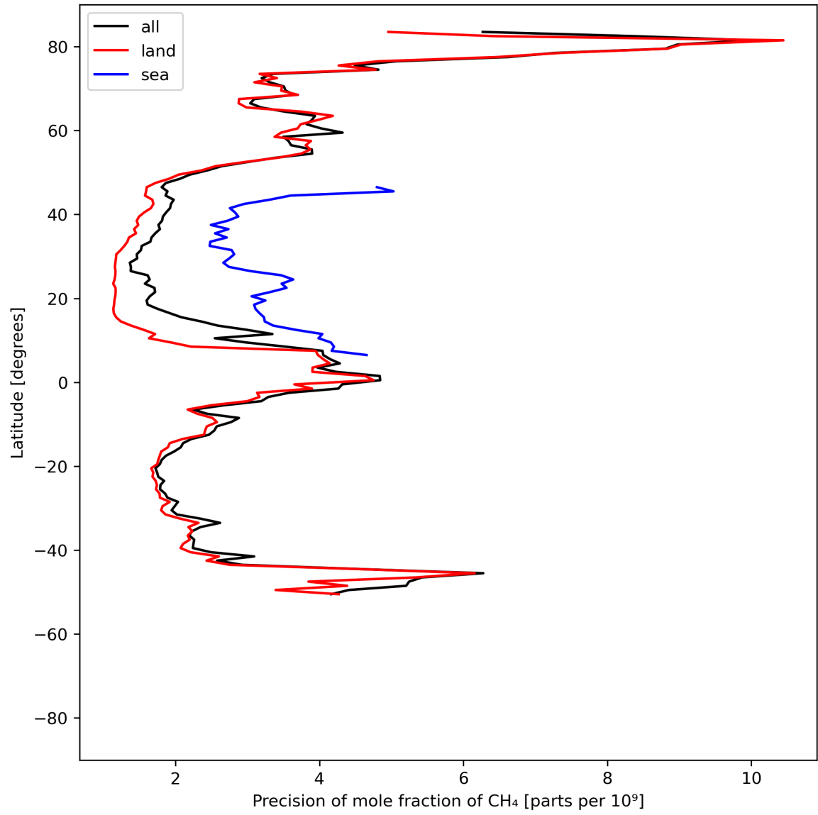
Figure 13: Zonal average of “Precision of mole fraction of CH 4 ” for 2023-07-14 to 2023-07-16.
