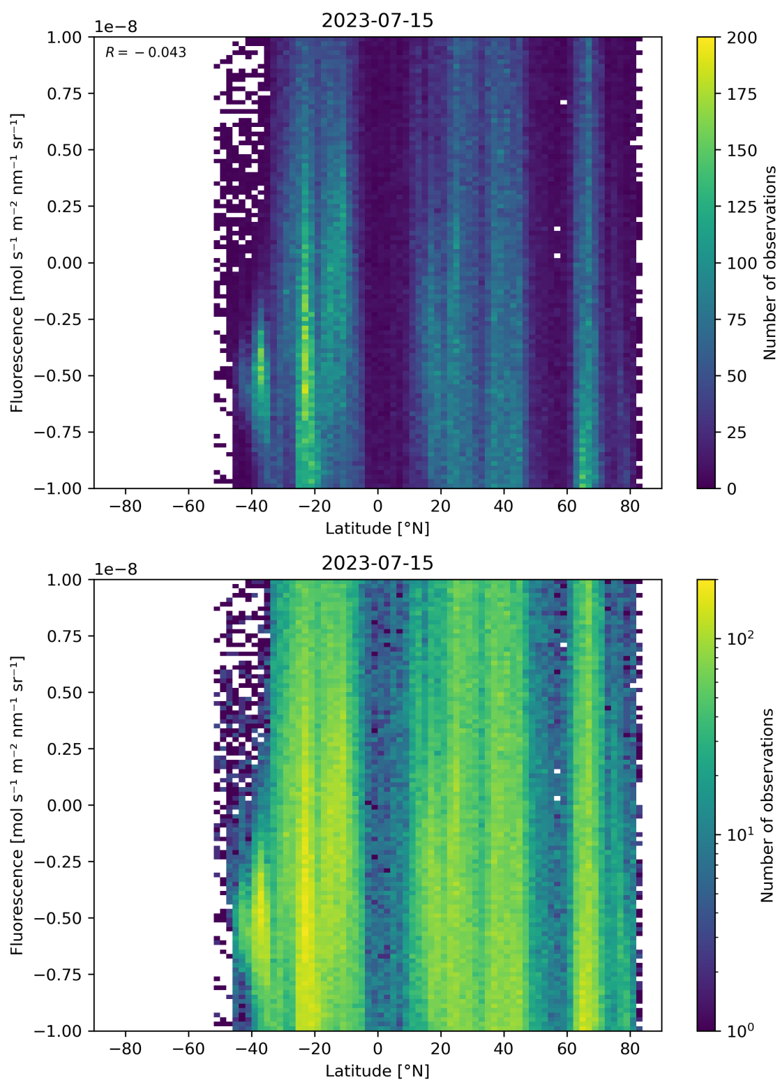
Figure 56: Scatter density plot of “Latitude” against “Fluorescence” for 2023-07-14 to 2023-07-16.
