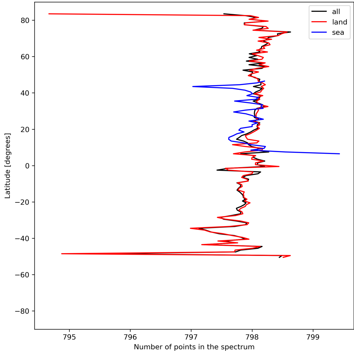
Figure 15: Zonal average of “Number of points in the spectrum” for 2023-07-14 to 2023-07-16.
