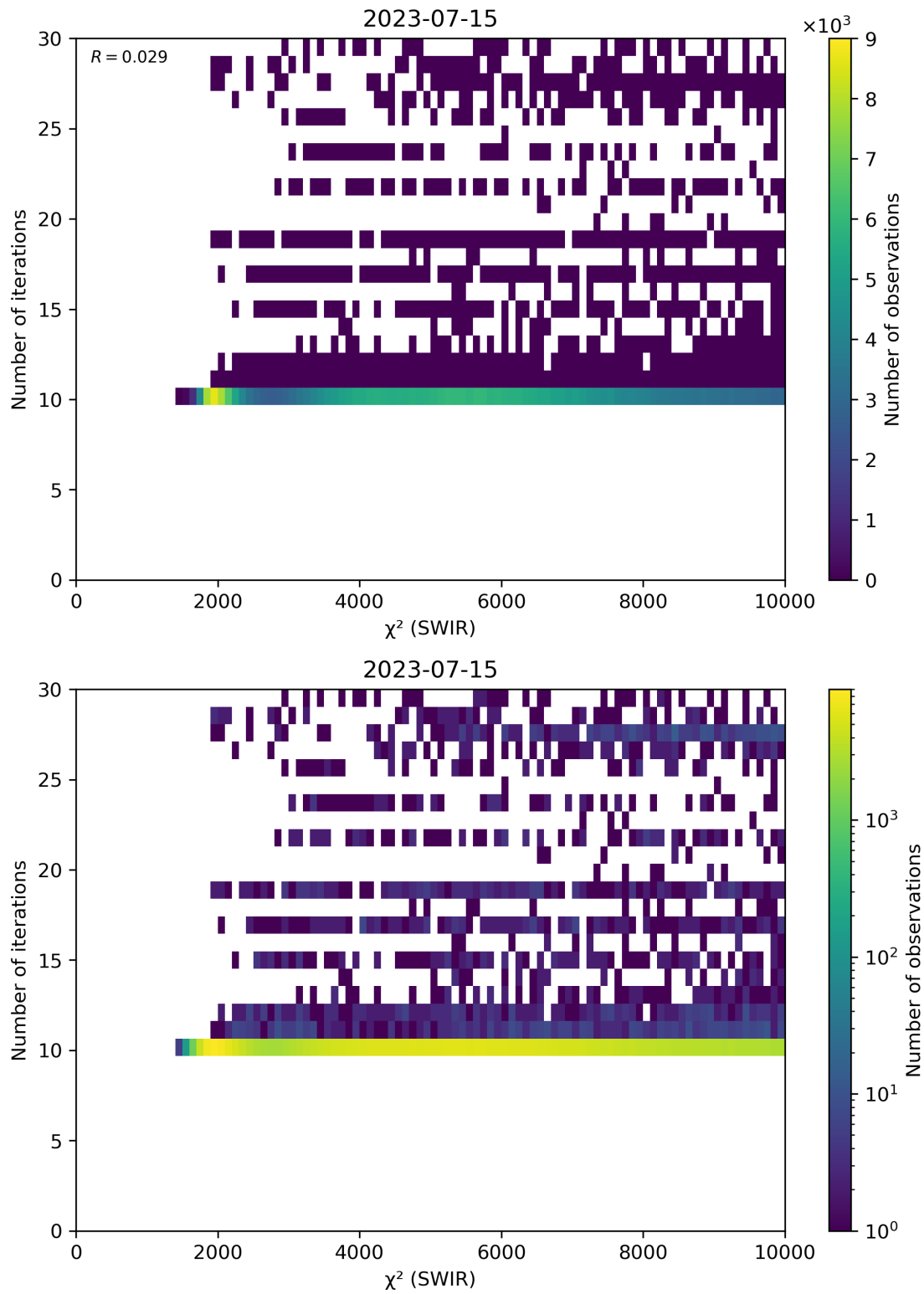
Figure 50: Scatter density plot of “ \chi^2 (SWIR)” against “Number of iterations” for 2023-07-14 to 2023-07-16.
