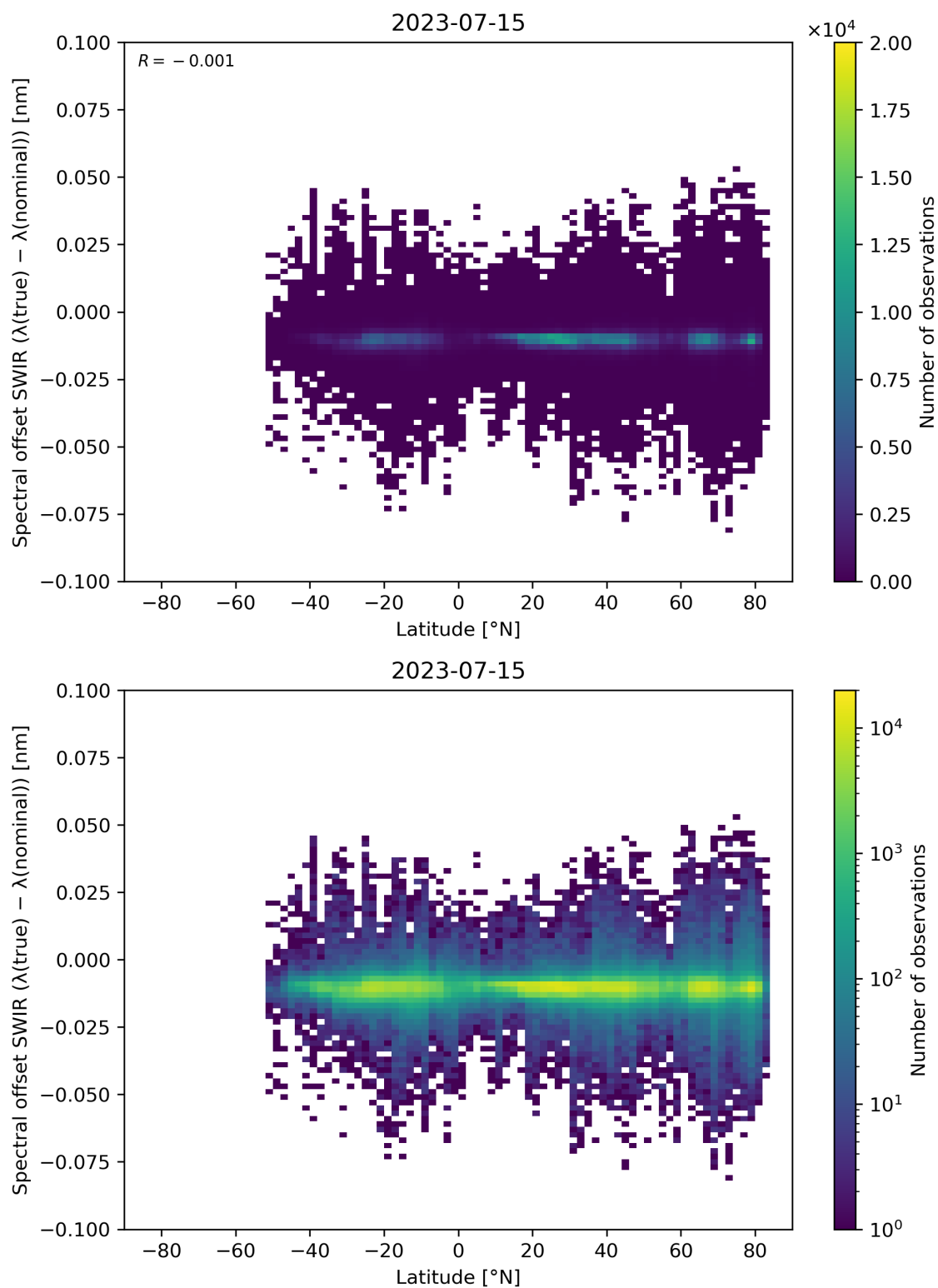
Figure 62: Scatter density plot of “Latitude” against “Spectral offset SWIR ( \lambda(\text{true}) - \lambda(\text{nominal}) )” for 2023-07-14 to 2023-07-16.
