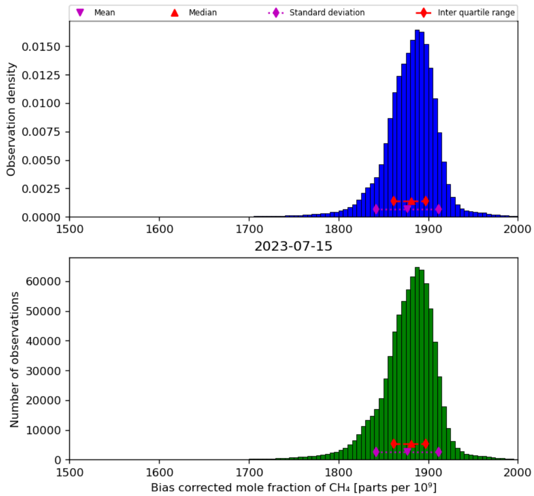
Figure 25: Histogram of “Bias corrected mole fraction of CH 4 ” for 2023-07-14 to 2023-07-16
