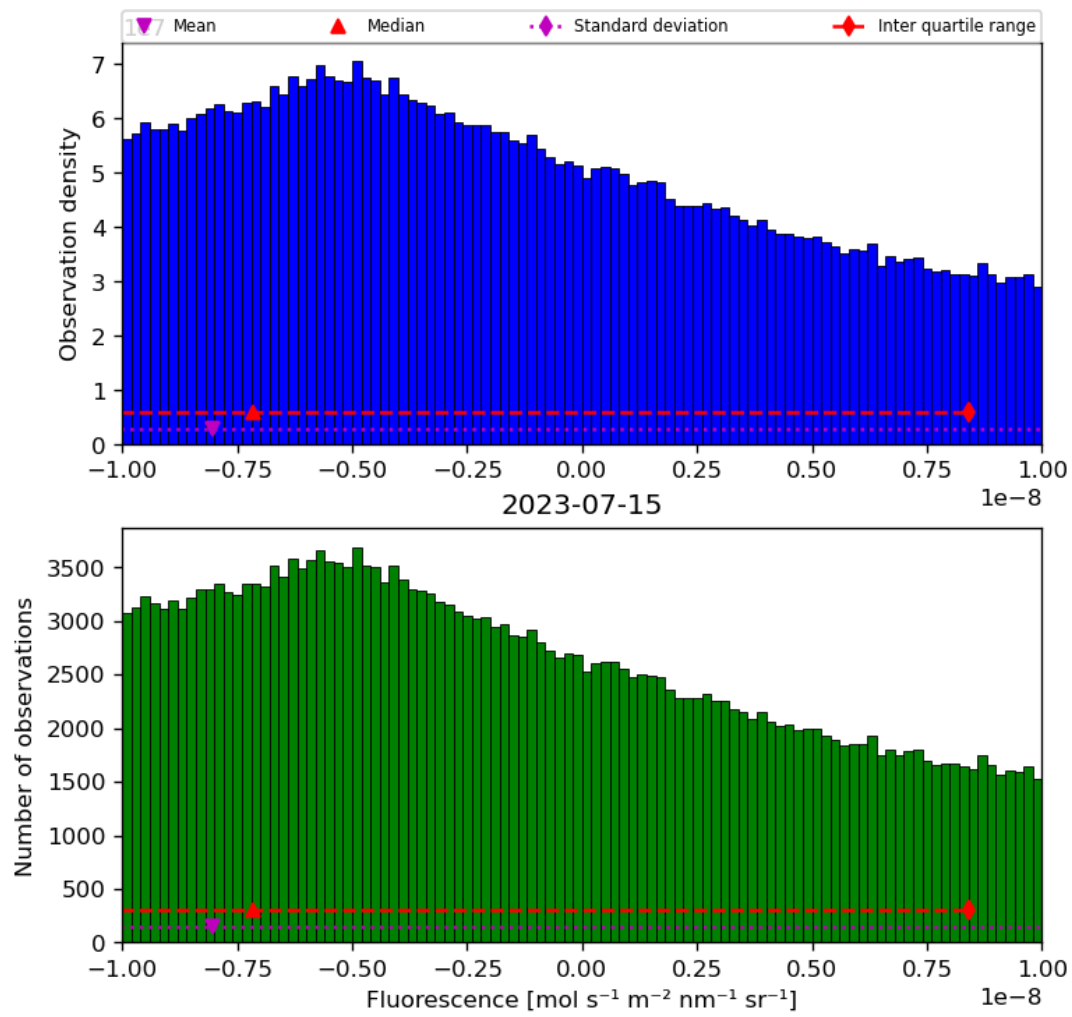
Figure 32: Histogram of “Fluorescence” for 2023-07-14 to 2023-07-16
