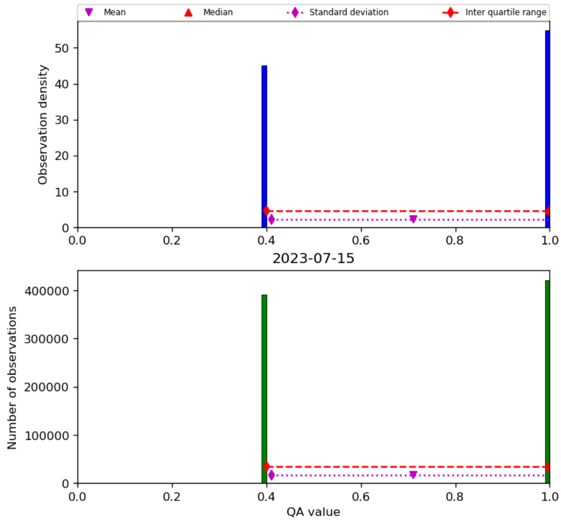
Figure 22: Histogram of “QA value” for 2023-07-14 to 2023-07-16
