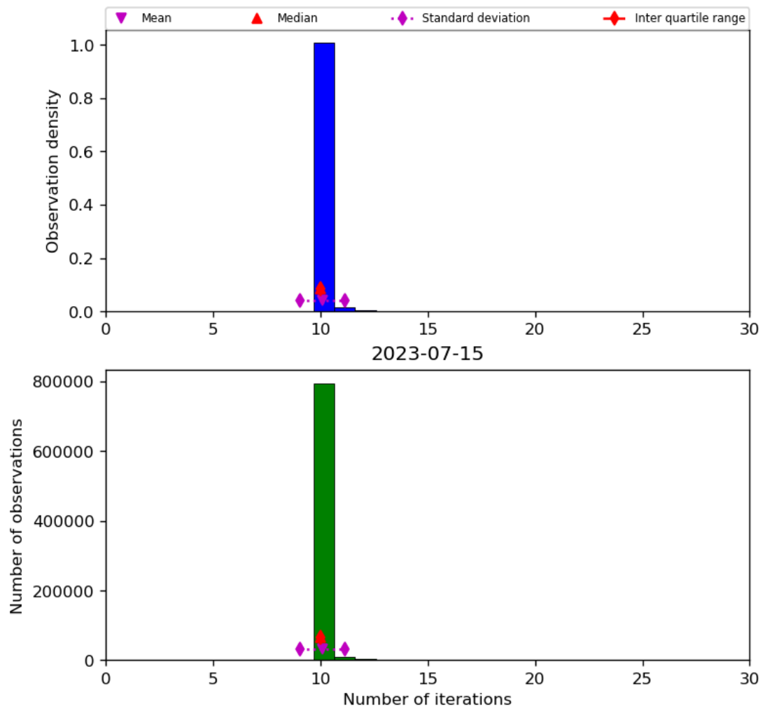
Figure 31: Histogram of “Number of iterations” for 2023-07-14 to 2023-07-16
