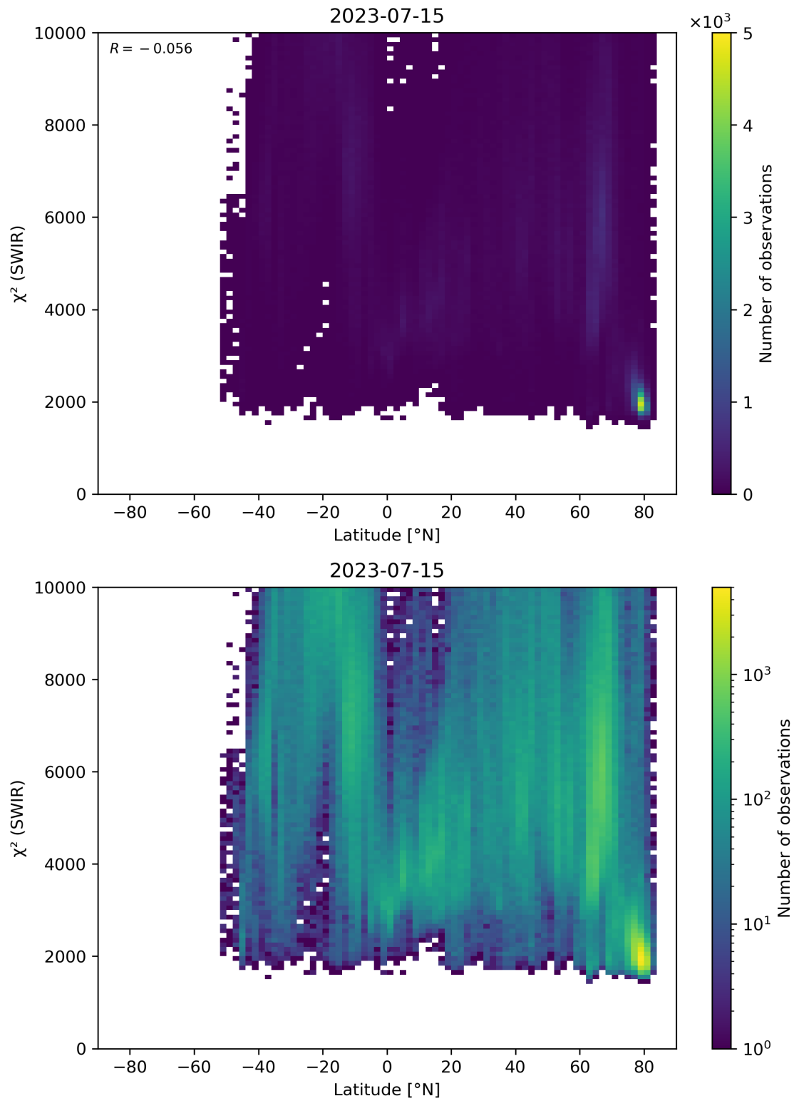
Figure 54: Scatter density plot of “Latitude” against “ \chi^2 (SWIR)” for 2023-07-14 to 2023-07-16.
