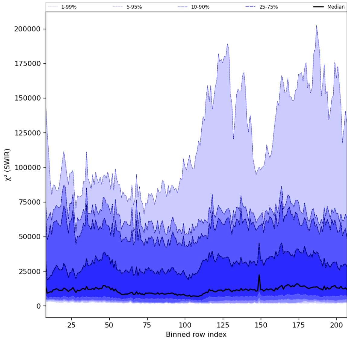
Figure 39: Along track statistics of “ \chi^2 (SWIR)” for 2023-07-14 to 2023-07-16
