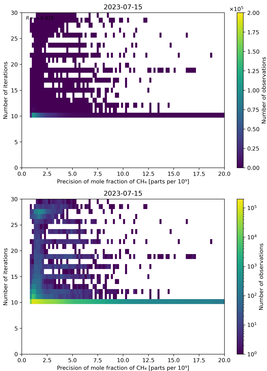
Figure 83: Scatter density plot of “Precision of mole fraction of CH 4 ” against “Number of iterations” for 2023-07-14 to 2023-07-16.
