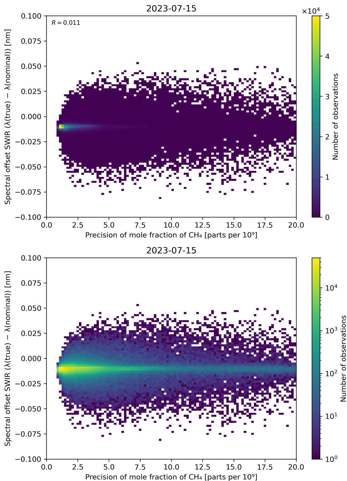
Figure 85: Scatter density plot of “Precision of mole fraction of CH 4 ” against “Spectral offset SWIR ( \lambda(\text{true}) - \lambda(\text{nominal}) )” for 2023-07-14 to 2023-07-16.
