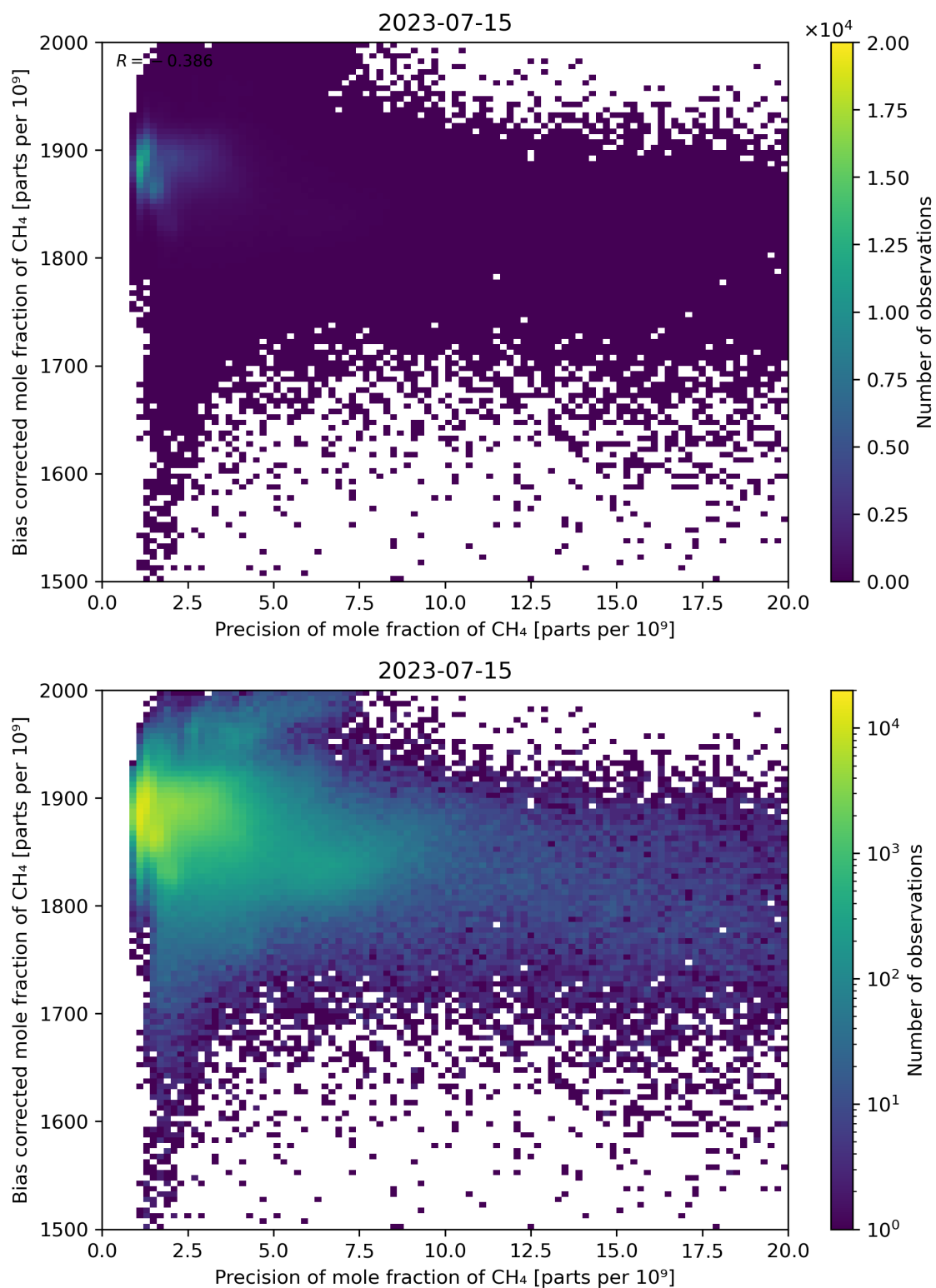
Figure 82: Scatter density plot of “Precision of mole fraction of CH 4 ” against “Bias corrected mole fraction of CH 4 ” for 2023-07-14 to 2023-07-16.
