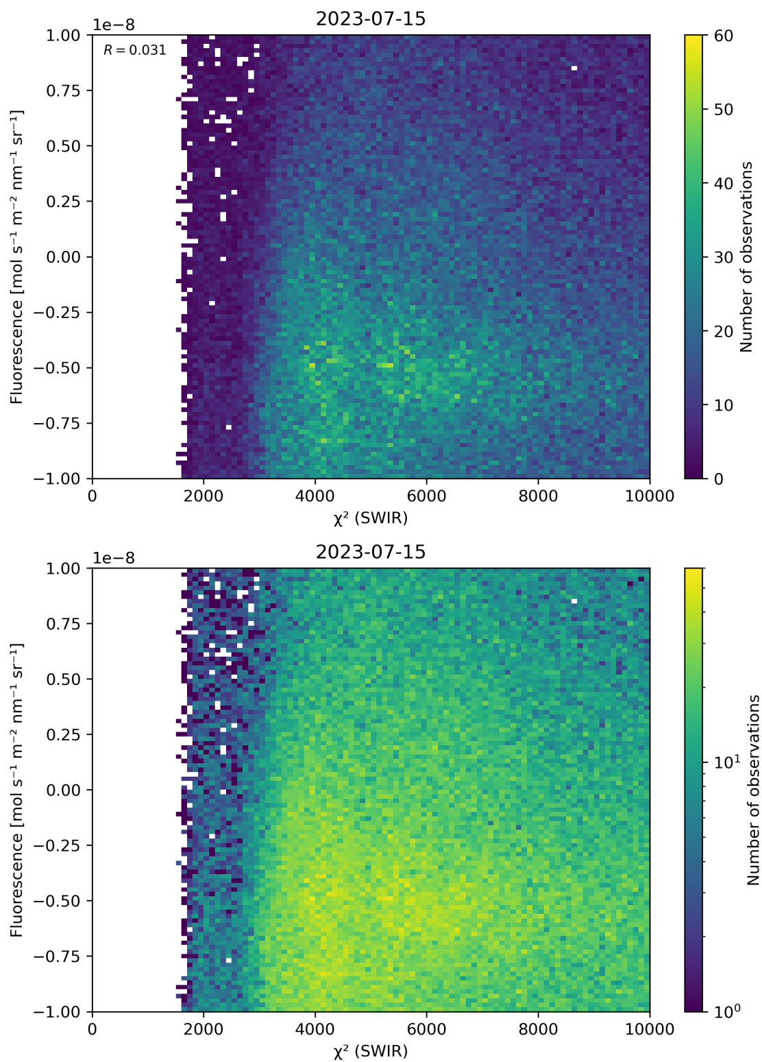
Figure 49: Scatter density plot of “ \chi^2 (SWIR)” against “Fluorescence” for 2023-07-14 to 2023-07-16.
