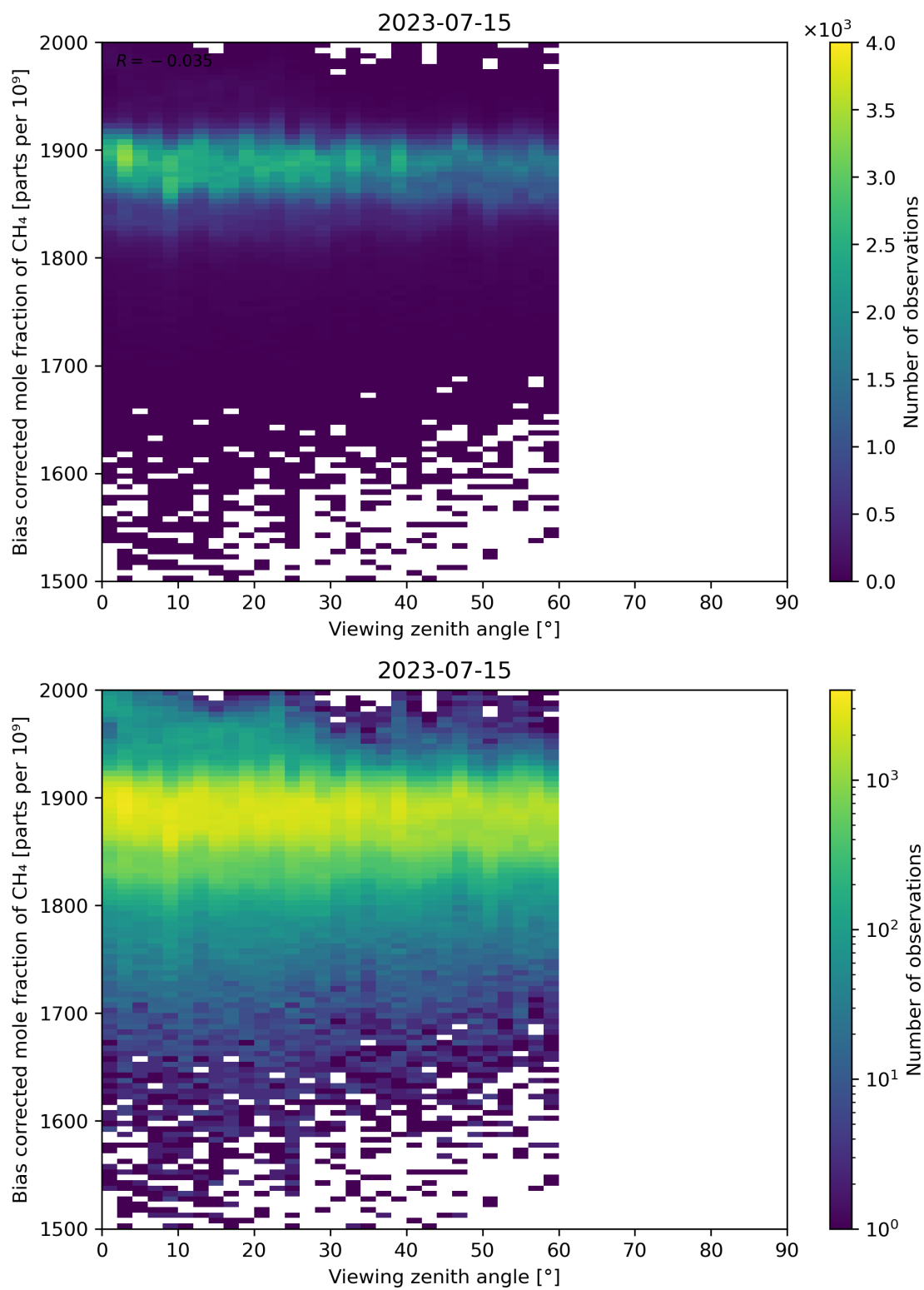
Figure 111: Scatter density plot of “Viewing zenith angle” against “Bias corrected mole fraction of CH 4 ” for 2023-07-14 to 2023-07-16.
