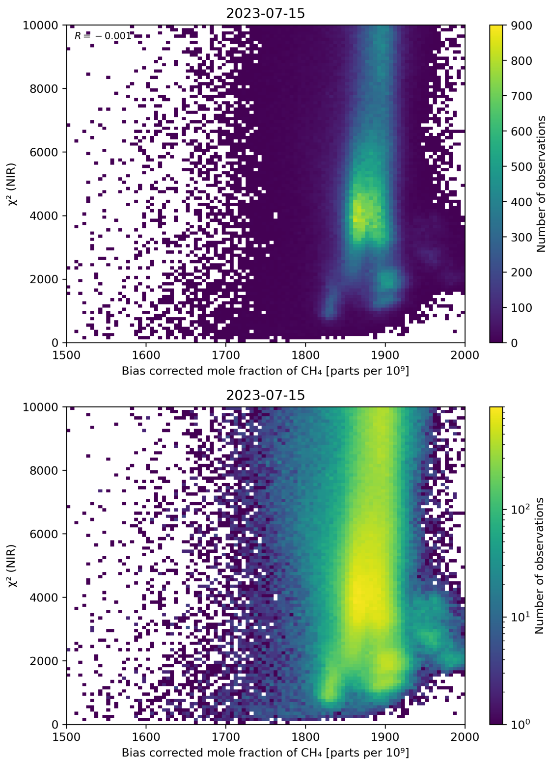
Figure 63: Scatter density plot of “Bias corrected mole fraction of CH 4 ” against “ \chi^2 (NIR)” for 2023-07-14 to 2023-07-16.
