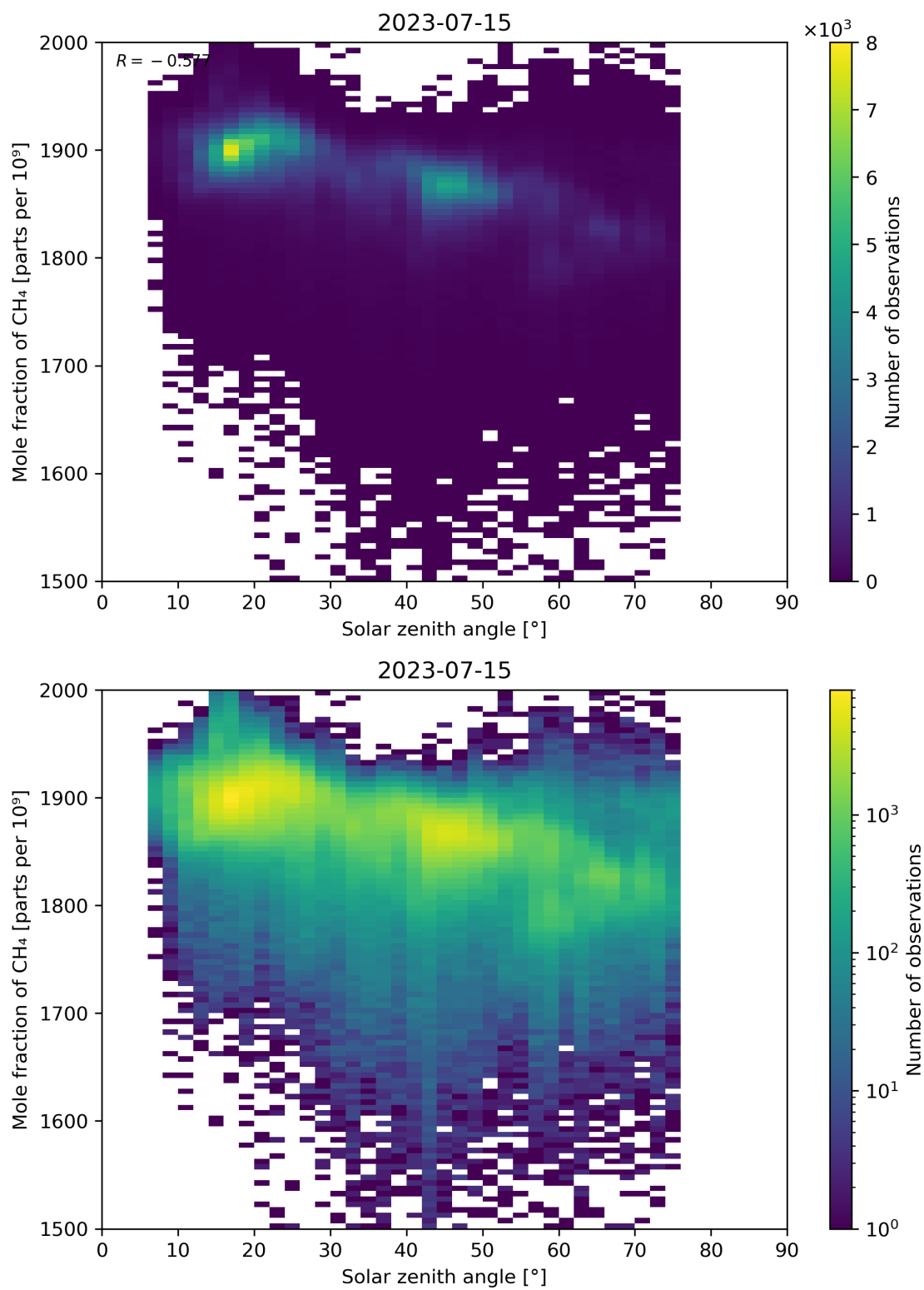
Figure 99: Scatter density plot of “Solar zenith angle” against “Mole fraction of CH 4 ” for 2023-07-14 to 2023-07-16.
