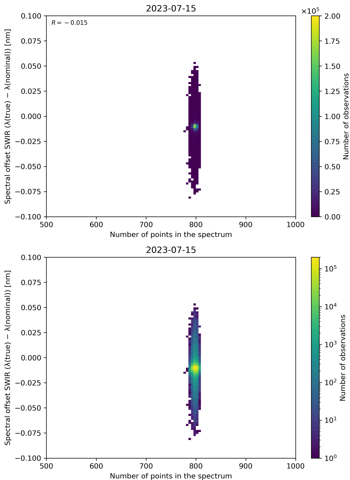
Figure 93: Scatter density plot of “Number of points in the spectrum” against “Spectral offset SWIR ( \lambda(\text{true}) - \lambda(\text{nominal}) )” for 2023-07-14 to 2023-07-16.
