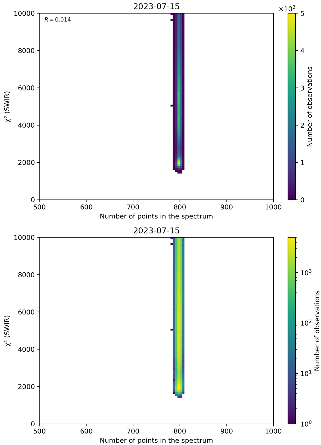
Figure 89: Scatter density plot of “Number of points in the spectrum” against “ \chi^2 (SWIR)” for 2023-07-14 to 2023-07-16.
