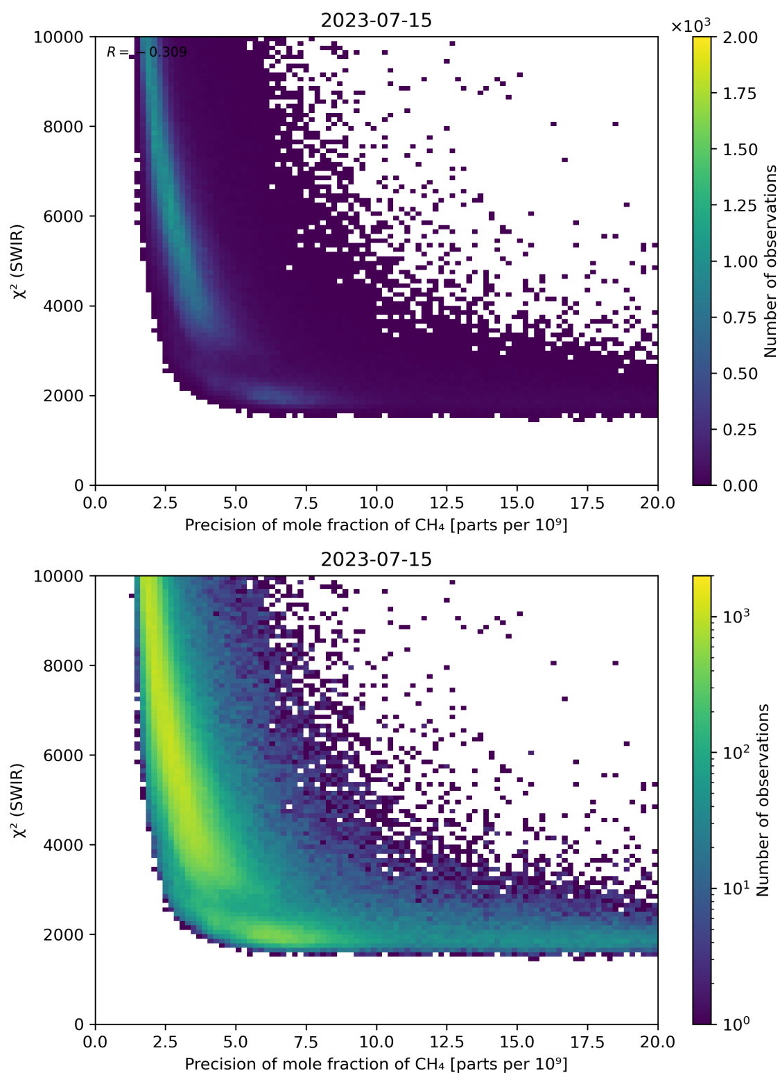
Figure 79: Scatter density plot of “Precision of mole fraction of CH 4 ” against “ \chi^2 (SWIR)” for 2023-07-14 to 2023-07-16.
