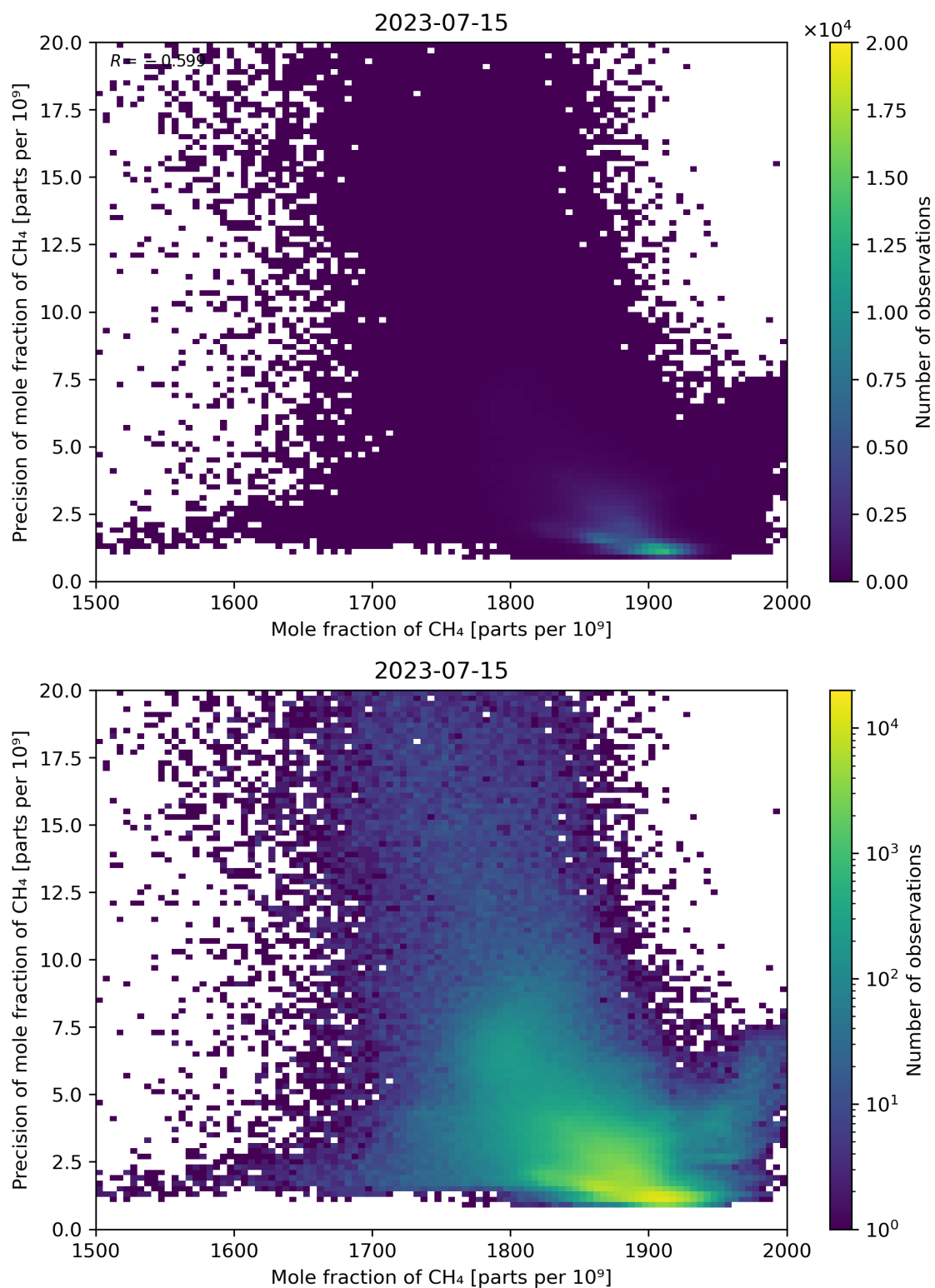
Figure 75: Scatter density plot of “Mole fraction of CH 4 ” against “Precision of mole fraction of CH 4 ” for 2023-07-14 to 2023-07-16.
