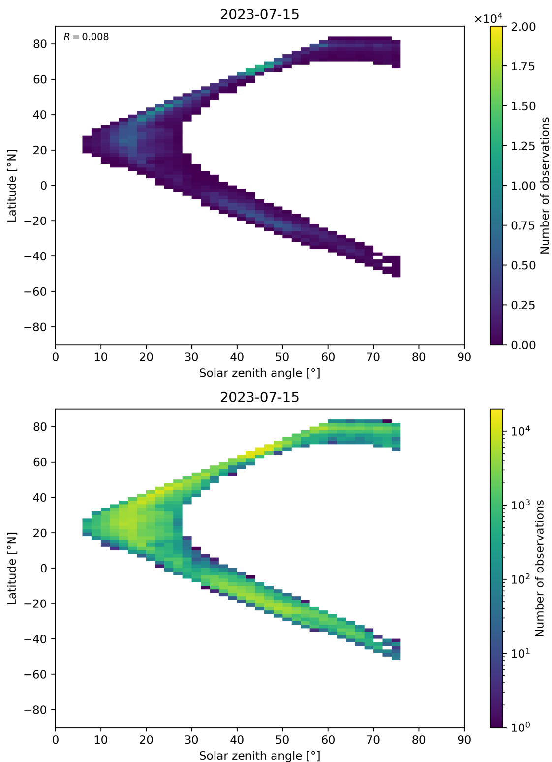
Figure 98: Scatter density plot of “Solar zenith angle” against “Latitude” for 2023-07-14 to 2023-07-16.
