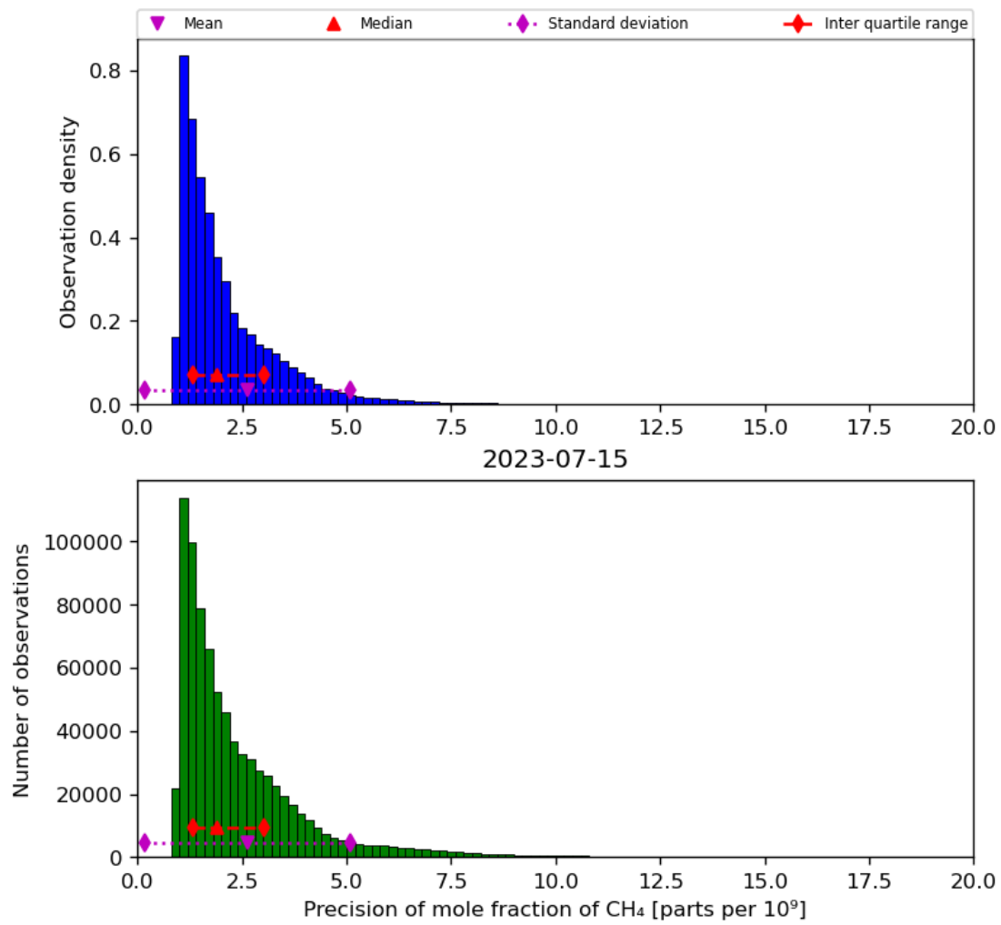
Figure 24: Histogram of “Precision of mole fraction of CH 4 ” for 2023-07-14 to 2023-07-16
