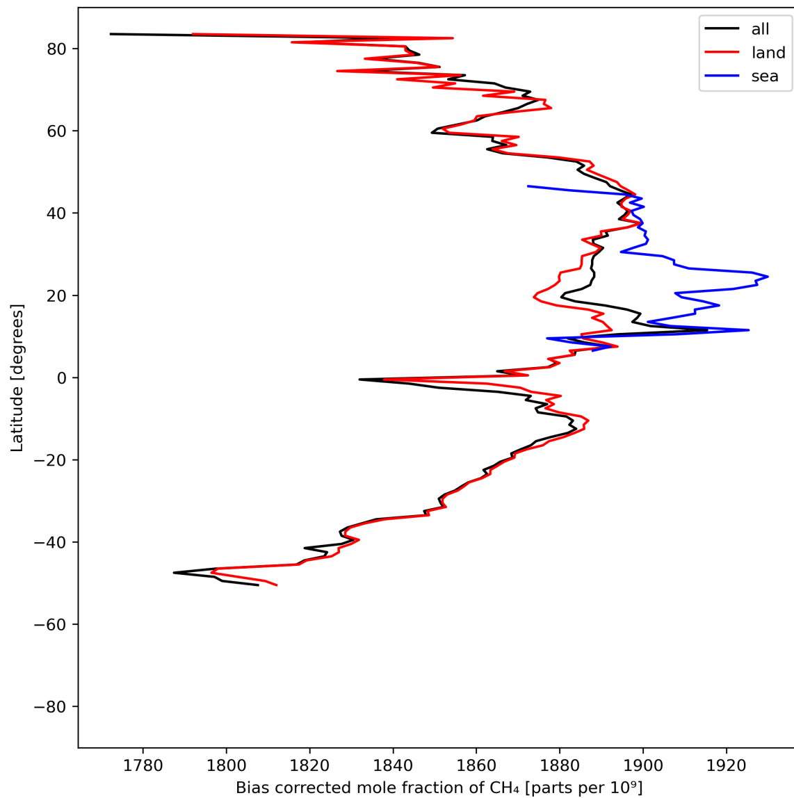
Figure 14: Zonal average of “Bias corrected mole fraction of CH 4 ” for 2023-07-14 to 2023-07-16.
