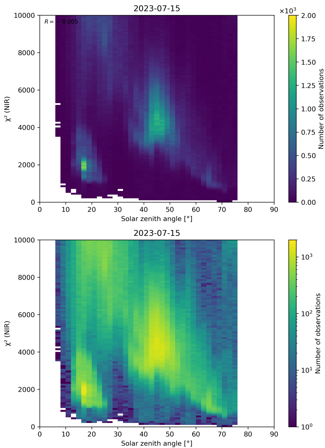
Figure 94: Scatter density plot of “Solar zenith angle” against “ \chi^2 (NIR)” for 2023-07-14 to 2023-07-16.
