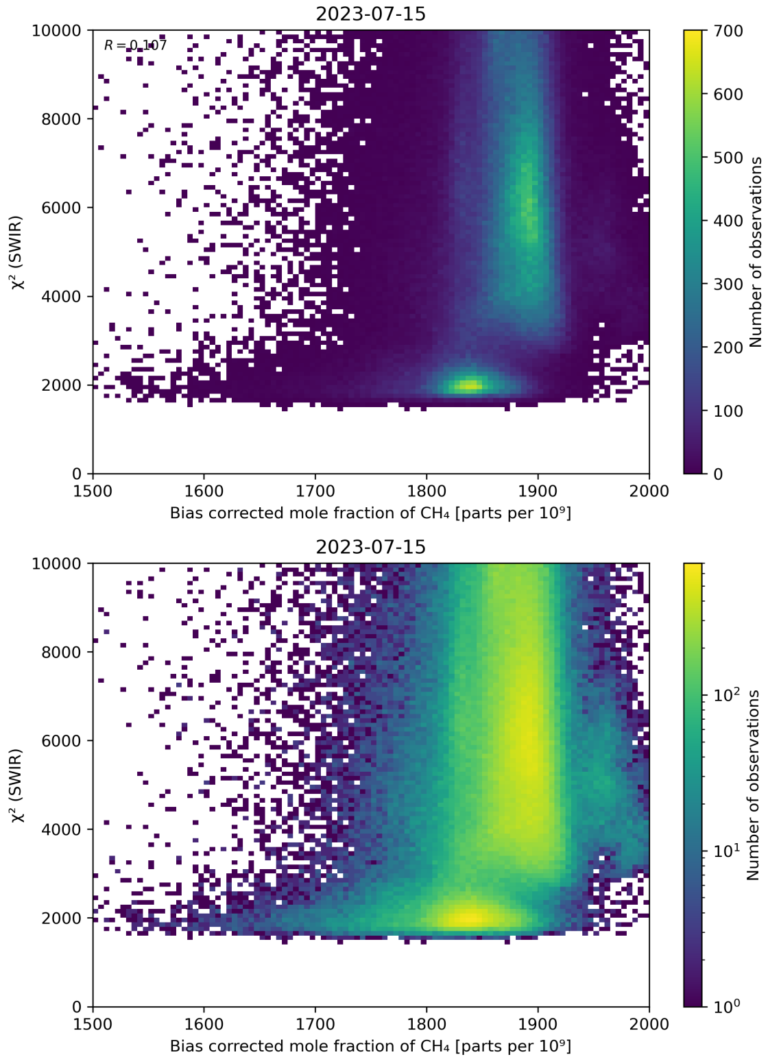
Figure 64: Scatter density plot of “Bias corrected mole fraction of CH 4 ” against “ \chi^2 (SWIR)” for 2023-07-14 to 2023-07-16.
