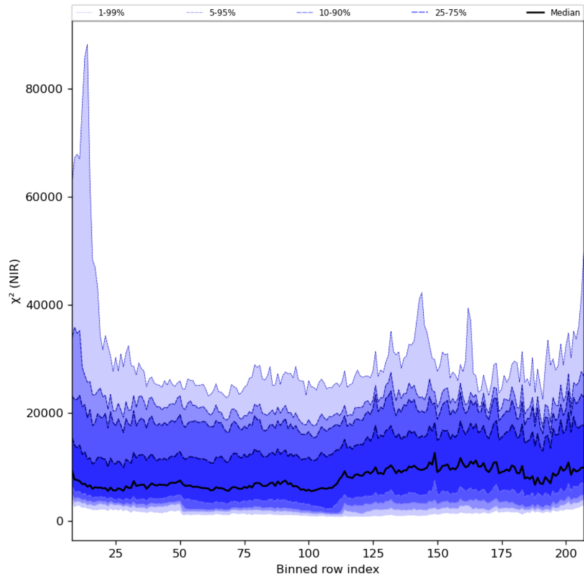
Figure 40: Along track statistics of “ \chi^2 (NIR)” for 2023-07-14 to 2023-07-16
