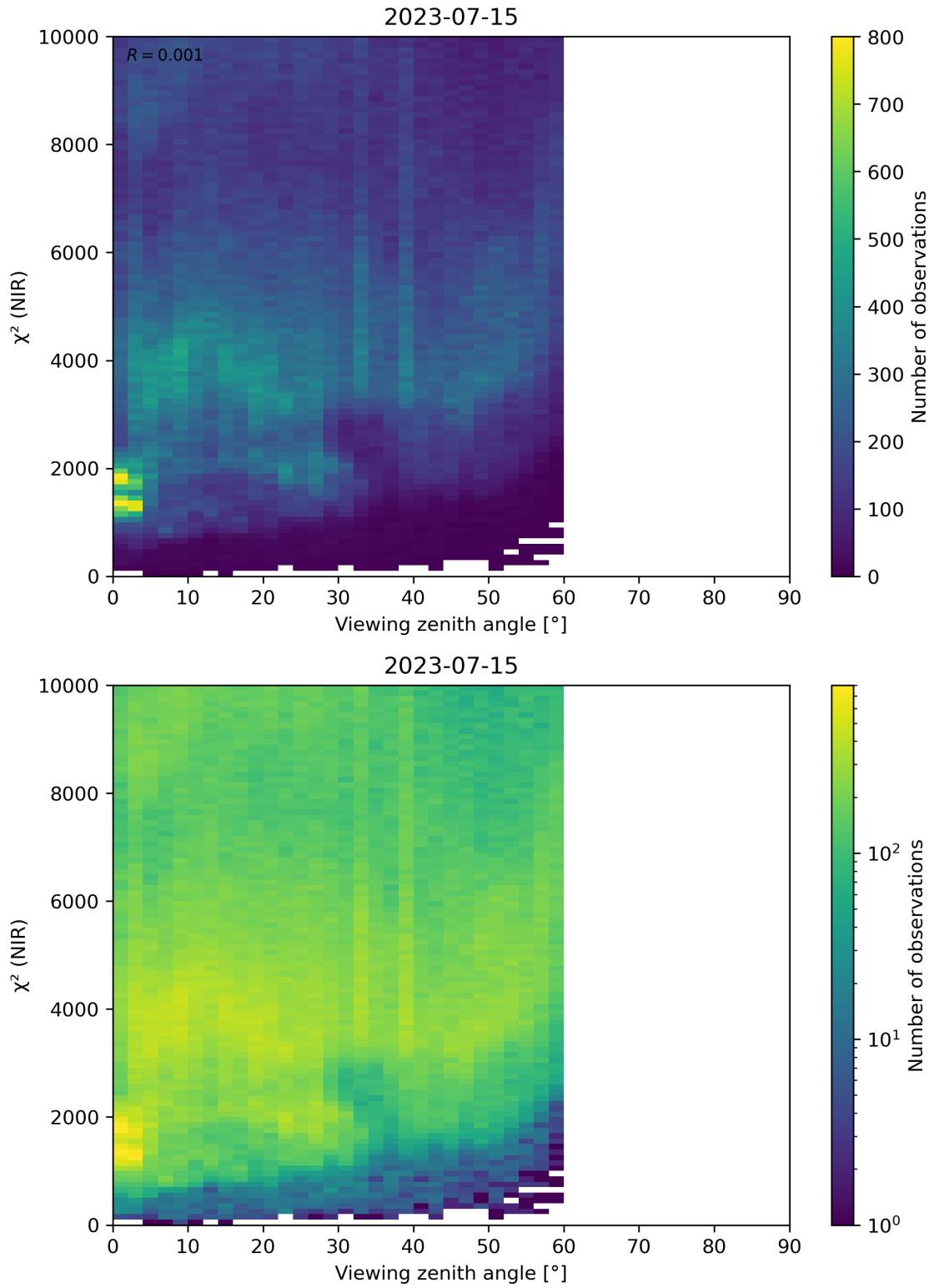
Figure 105: Scatter density plot of “Viewing zenith angle” against “ \chi^2 (NIR)” for 2023-07-14 to 2023-07-16.
