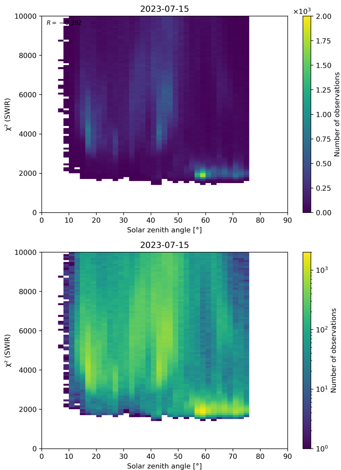
Figure 95: Scatter density plot of “Solar zenith angle” against “ \chi^2 (SWIR)” for 2023-07-14 to 2023-07-16.
