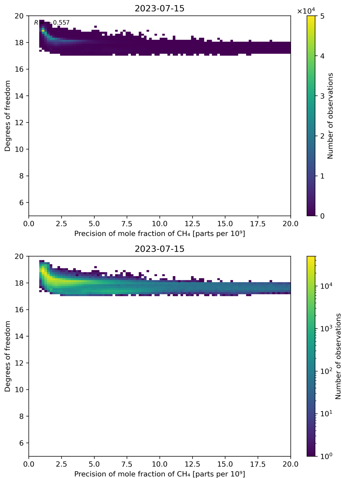
Figure 80: Scatter density plot of “Precision of mole fraction of CH 4 ” against “Degrees of freedom” for 2023-07-14 to 2023-07-16.
