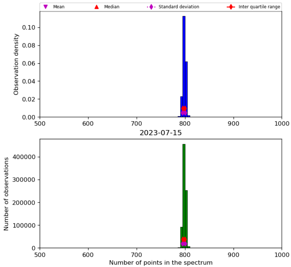
Figure 26: Histogram of “Number of points in the spectrum” for 2023-07-14 to 2023-07-16
