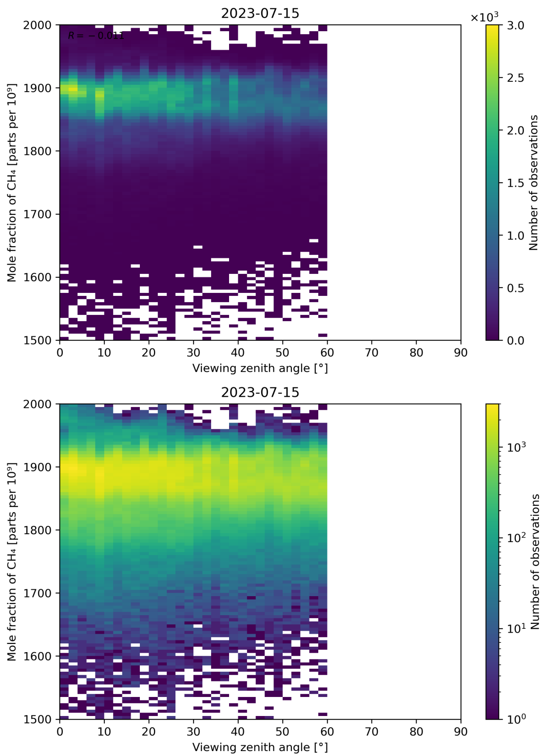
Figure 110: Scatter density plot of “Viewing zenith angle” against “Mole fraction of CH 4 ” for 2023-07-14 to 2023-07-16.
