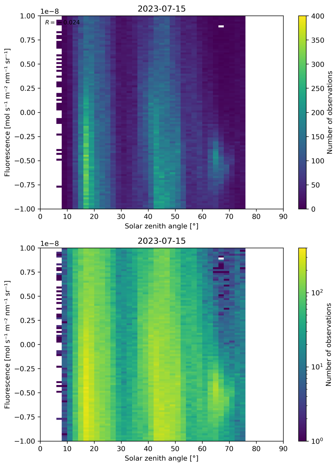
Figure 97: Scatter density plot of “Solar zenith angle” against “Fluorescence” for 2023-07-14 to 2023-07-16.
