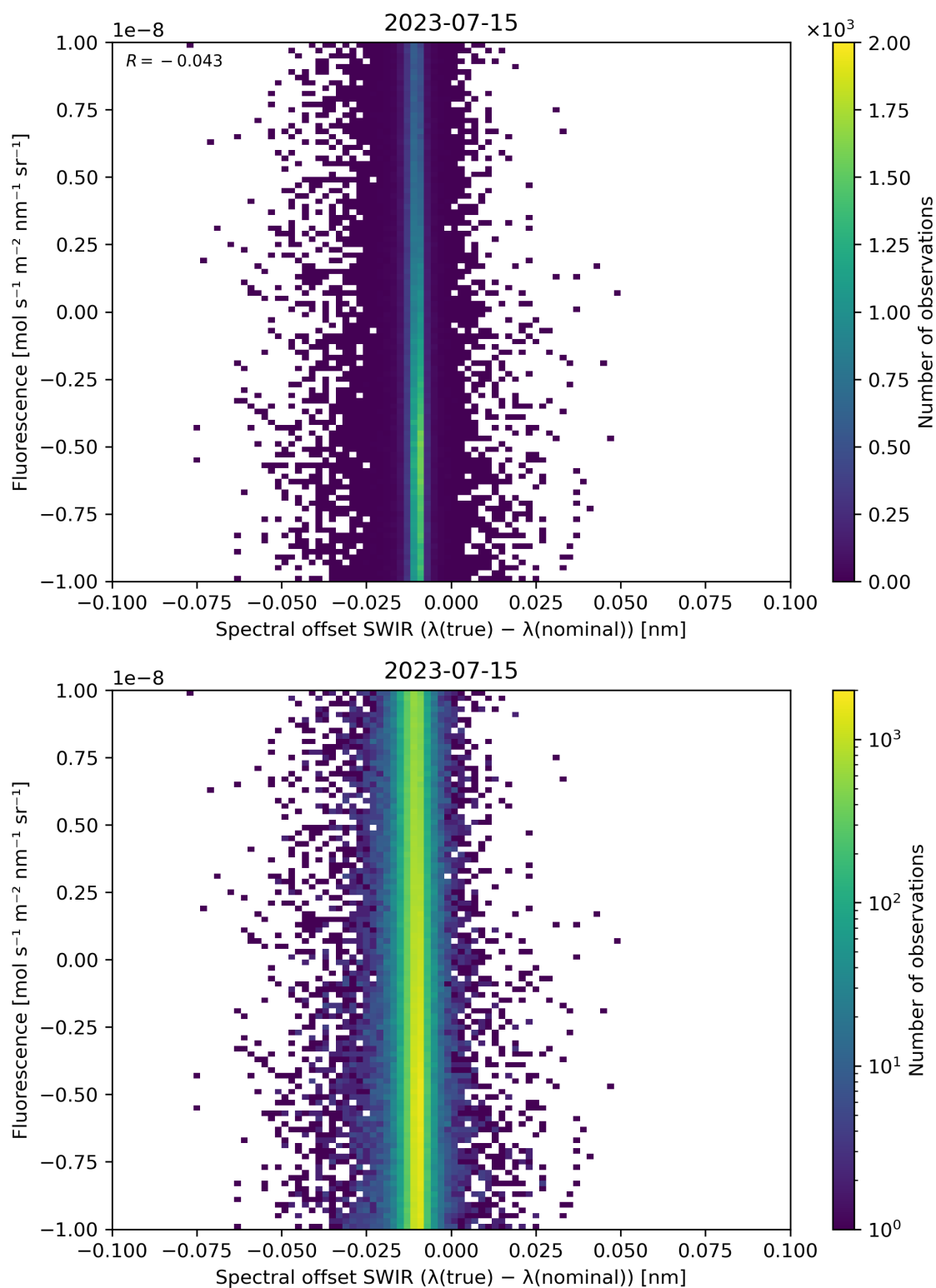
Figure 120: Scatter density plot of “Spectral offset SWIR ( \lambda(\text{true}) - \lambda(\text{nominal}) )” against “Fluorescence” for 2023-07-14 to 2023-07-16.
