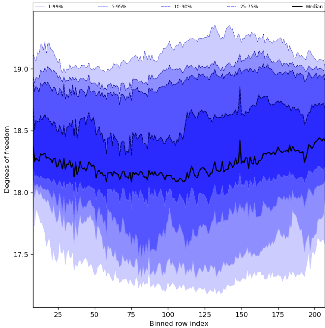
Figure 41: Along track statistics of “Degrees of freedom” for 2023-07-14 to 2023-07-16
