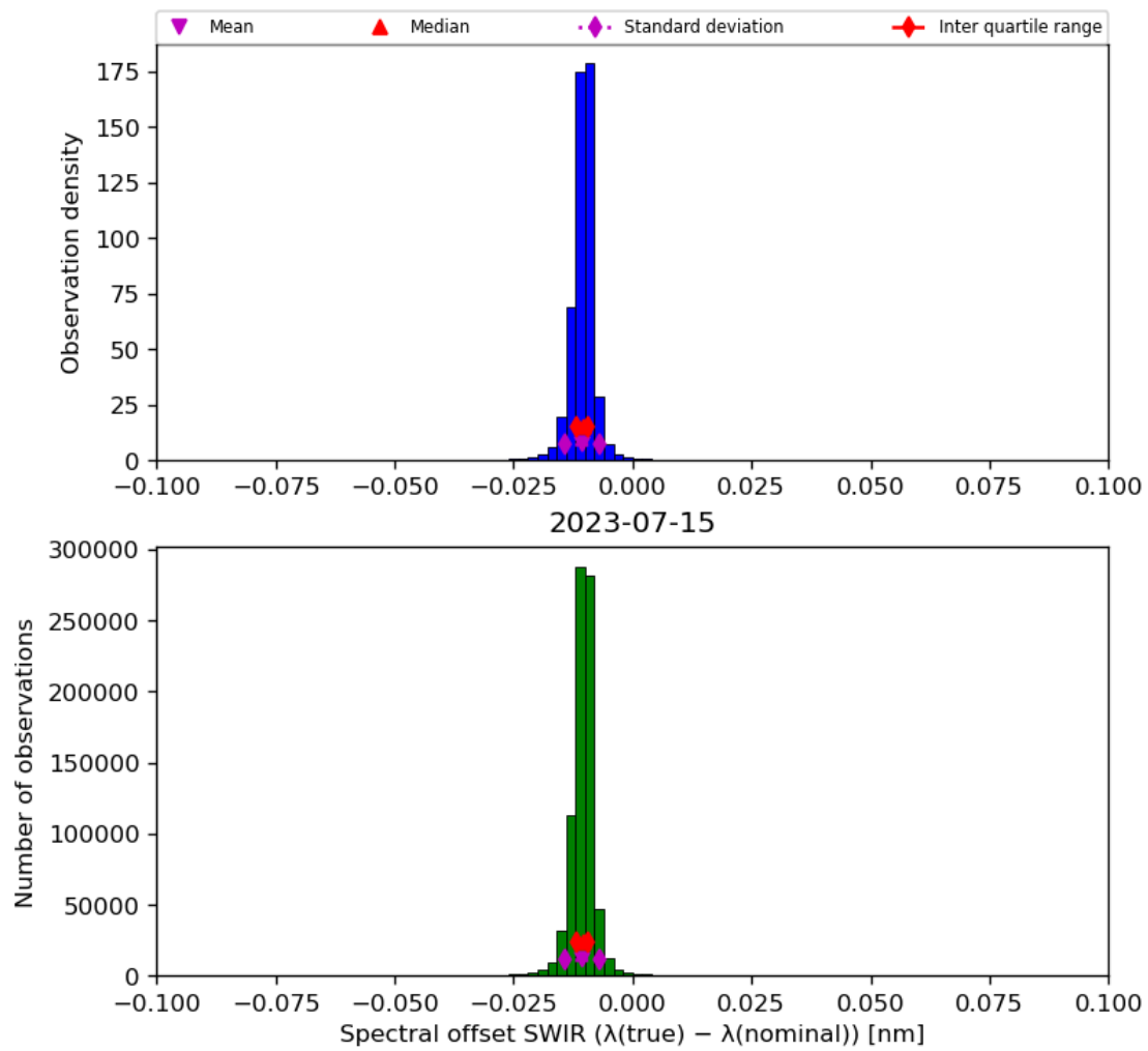
Figure 27: Histogram of “Spectral offset SWIR ( \lambda(\text{true}) - \lambda(\text{nominal}) )” for 2023-07-14 to 2023-07-16
