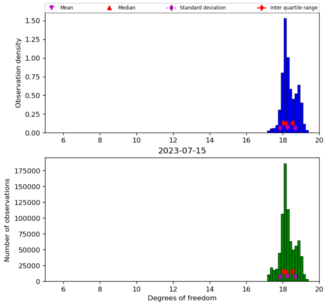
Figure 30: Histogram of “Degrees of freedom” for 2023-07-14 to 2023-07-16
