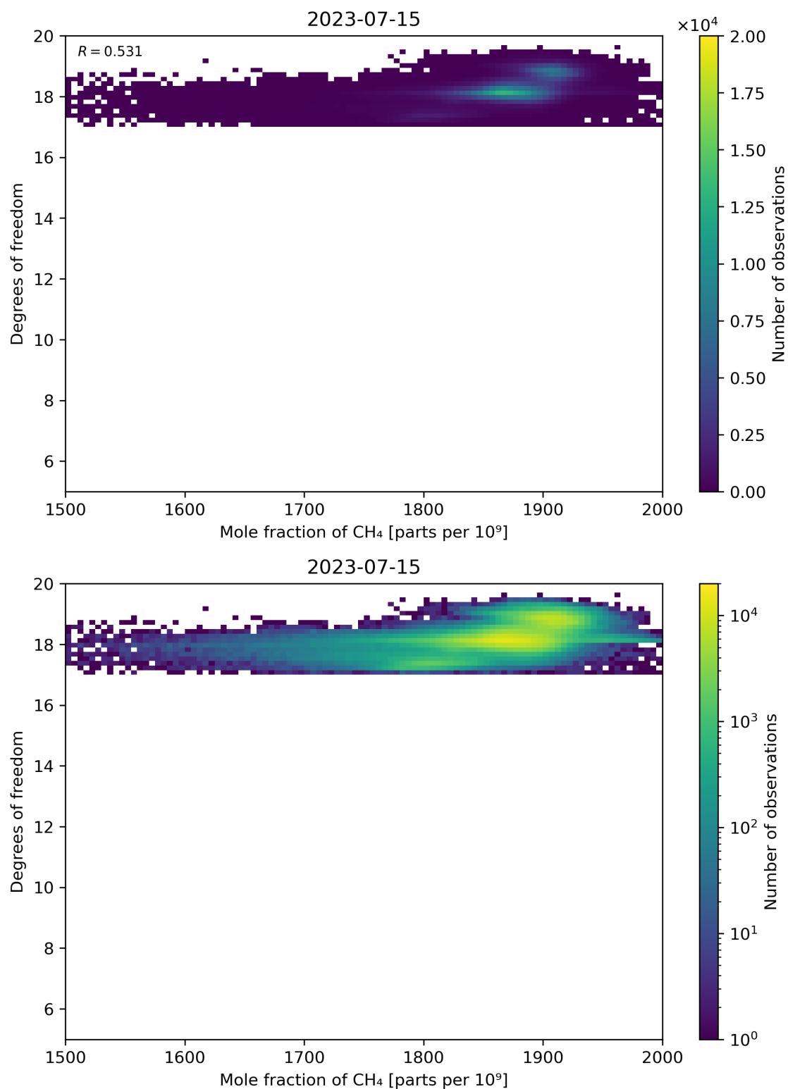
Figure 72: Scatter density plot of “Mole fraction of CH 4 ” against “Degrees of freedom” for 2023-07-14 to 2023-07-16.
