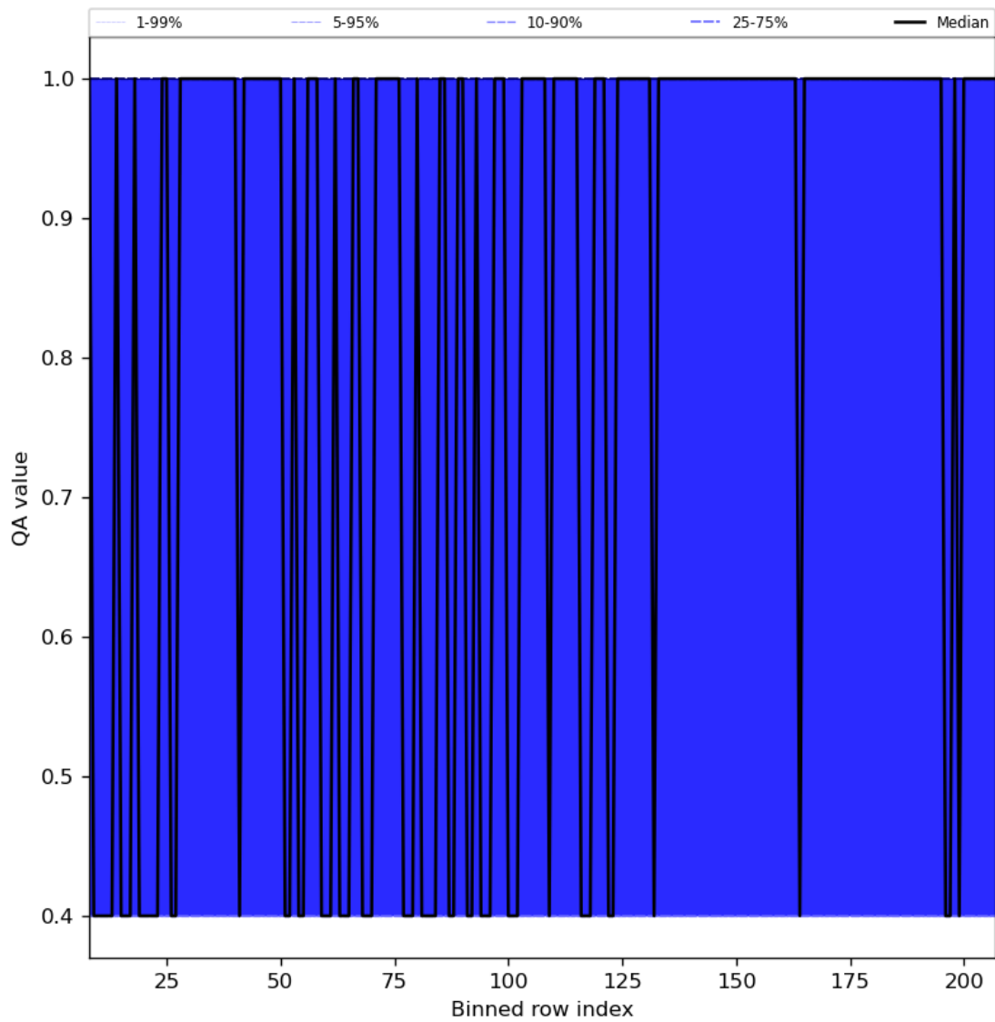
Figure 33: Along track statistics of “QA value” for 2023-07-14 to 2023-07-16
