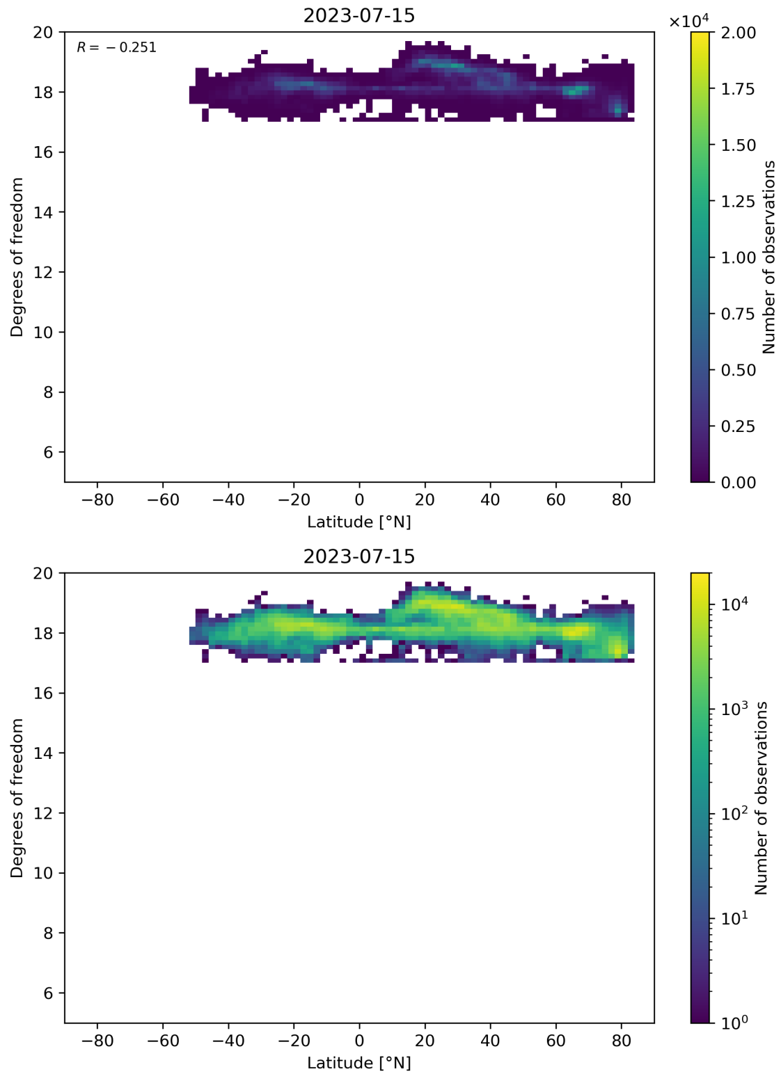
Figure 55: Scatter density plot of “Latitude” against “Degrees of freedom” for 2023-07-14 to 2023-07-16.
