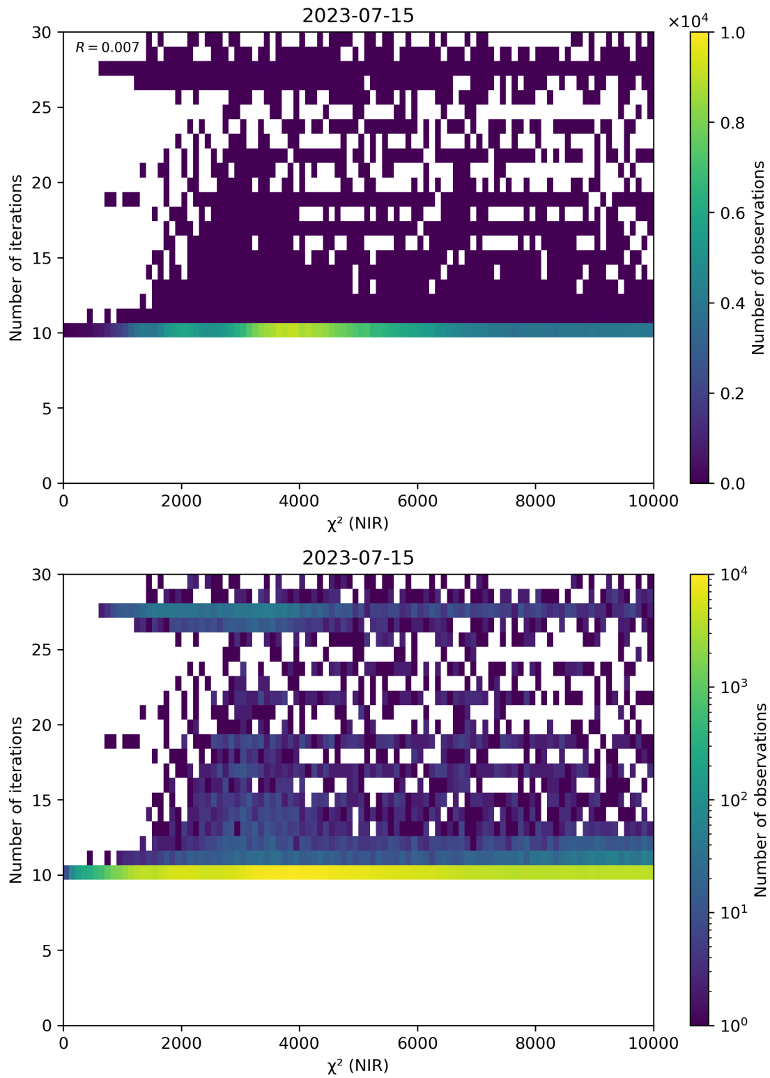
Figure 46: Scatter density plot of “ \chi^2 (NIR)” against “Number of iterations” for 2023-07-14 to 2023-07-16.
