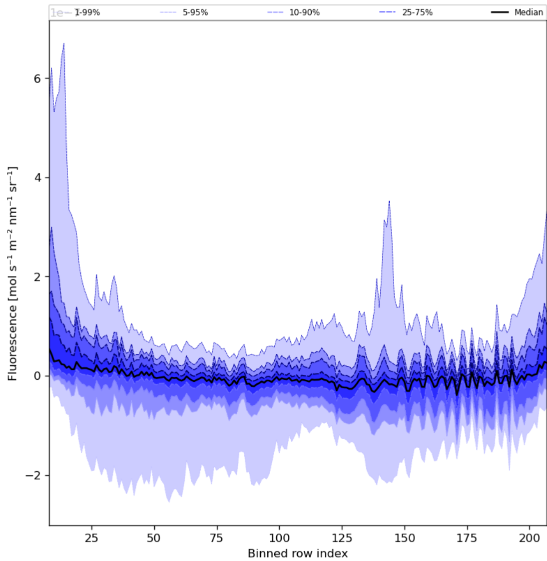
Figure 43: Along track statistics of “Fluorescence” for 2023-07-14 to 2023-07-16
