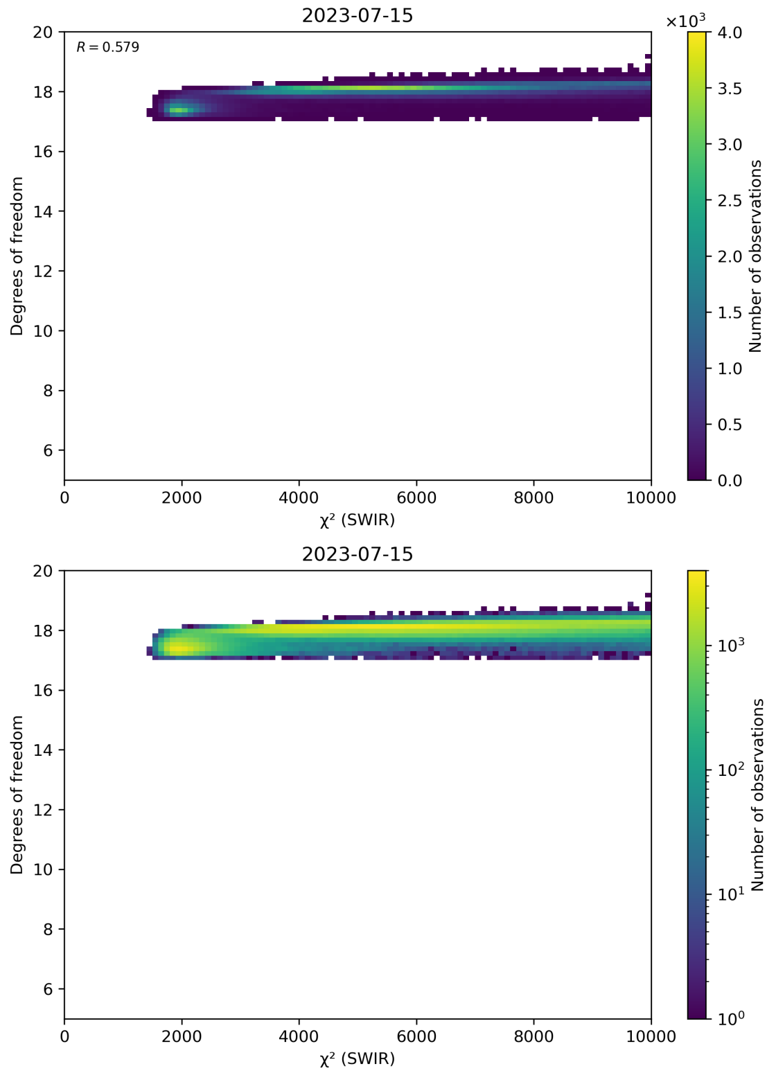
Figure 48: Scatter density plot of “ \chi^2 (SWIR)” against “Degrees of freedom” for 2023-07-14 to 2023-07-16.
