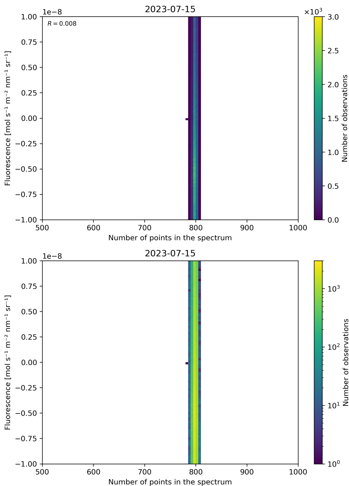
Figure 91: Scatter density plot of “Number of points in the spectrum” against “Fluorescence” for 2023-07-14 to 2023-07-16.
