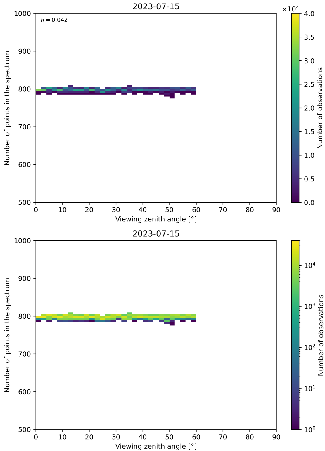
Figure 114: Scatter density plot of “Viewing zenith angle” against “Number of points in the spectrum” for 2023-07-14 to 2023-07-16.
