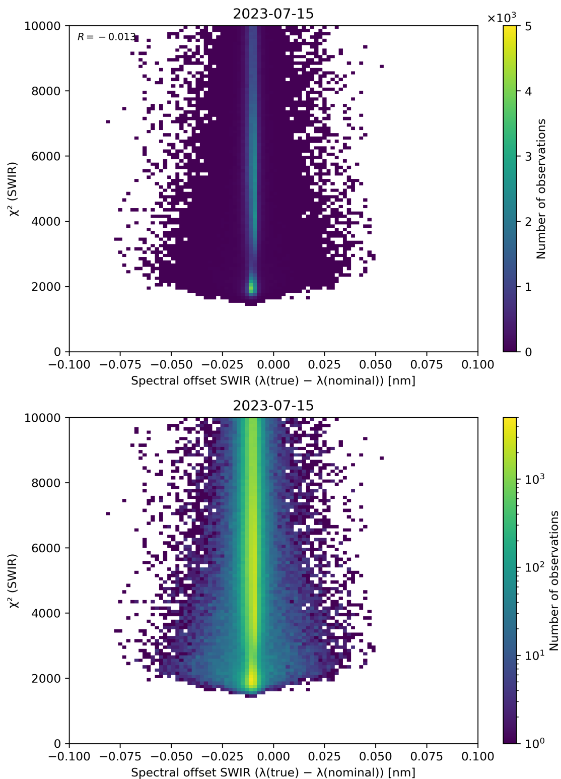
Figure 118: Scatter density plot of “Spectral offset SWIR ( \lambda(\text{true}) - \lambda(\text{nominal}) )” against “ \chi^2 (SWIR)” for 2023-07-14 to 2023-07-16.
