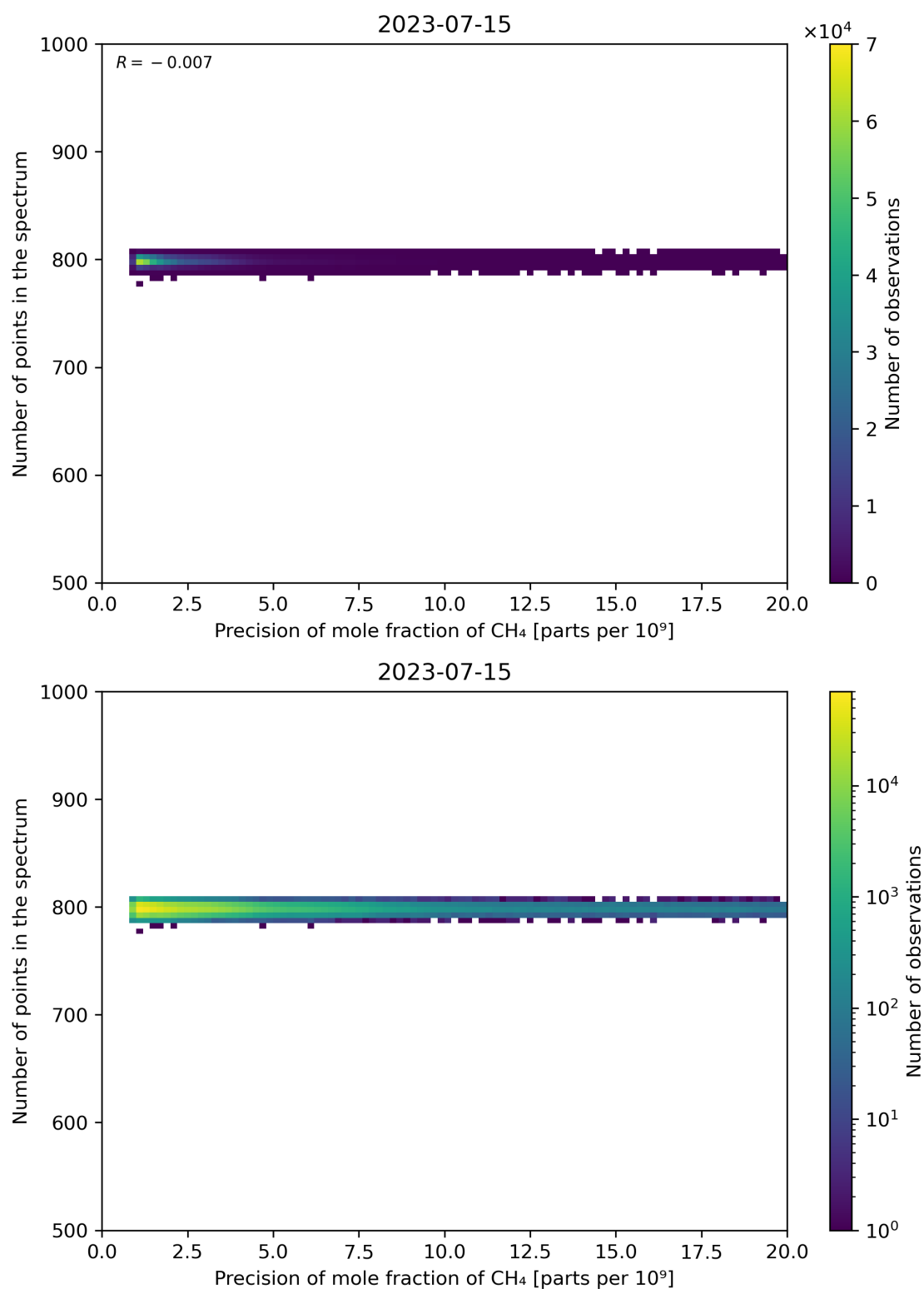
Figure 84: Scatter density plot of “Precision of mole fraction of CH 4 ” against “Number of points in the spectrum” for 2023-07-14 to 2023-07-16.
