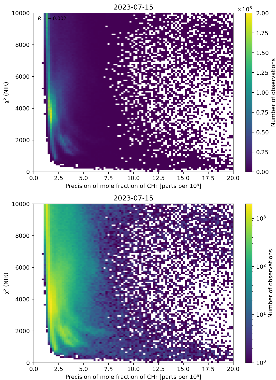
Figure 78: Scatter density plot of “Precision of mole fraction of CH 4 ” against “ \chi^2 (NIR)” for 2023-07-14 to 2023-07-16.
