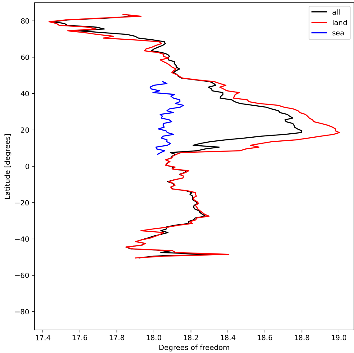
Figure 19: Zonal average of “Degrees of freedom” for 2023-07-14 to 2023-07-16.
