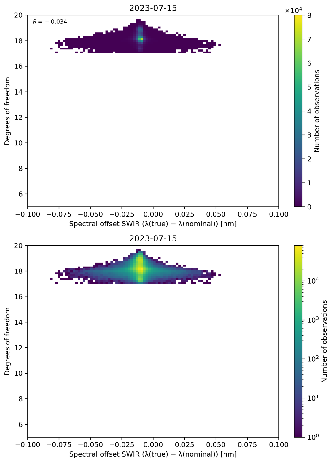
Figure 119: Scatter density plot of “Spectral offset SWIR ( \lambda(\text{true}) - \lambda(\text{nominal}) )” against “Degrees of freedom” for 2023-07-14 to 2023-07-16.
