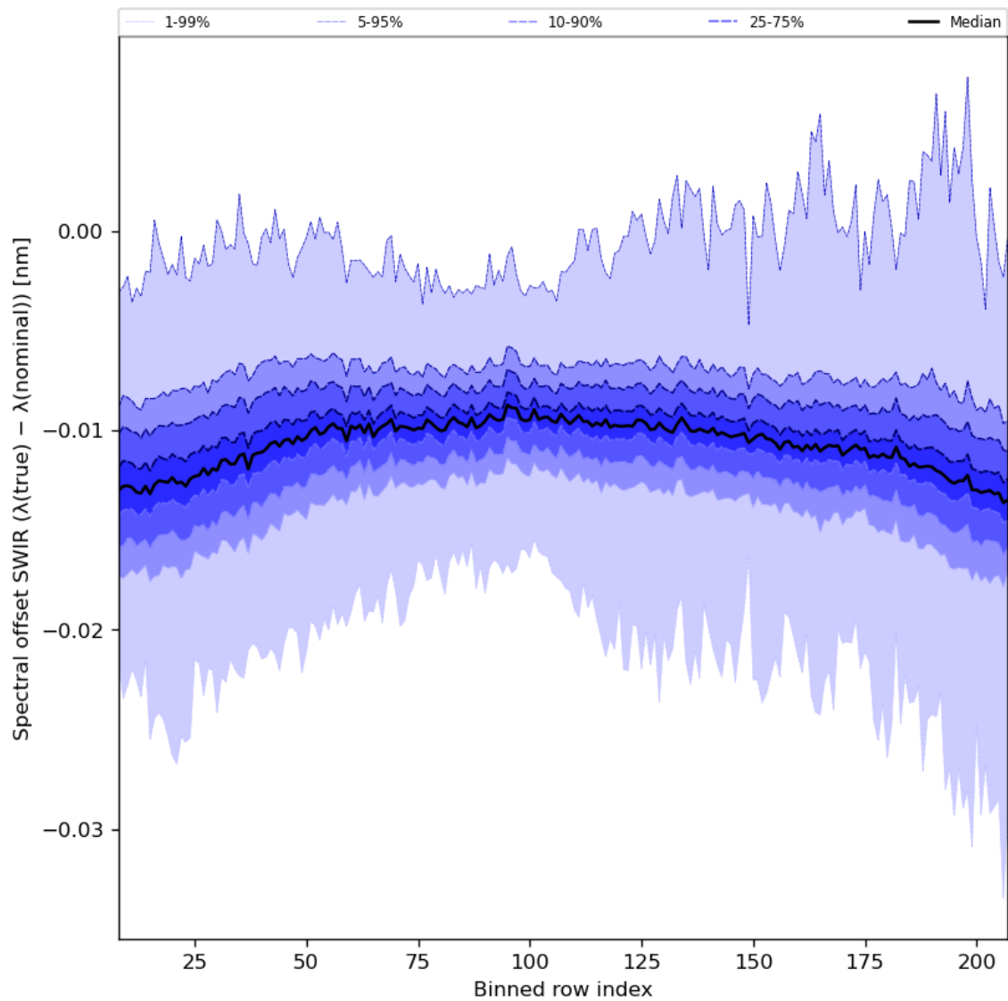
Figure 38: Along track statistics of “Spectral offset SWIR ( \lambda(\text{true}) - \lambda(\text{nominal}) )” for 2023-07-14 to 2023-07-16
