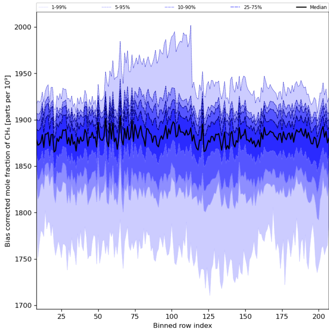
Figure 36: Along track statistics of “Bias corrected mole fraction of CH 4 ” for 2023-07-14 to 2023-07-16
