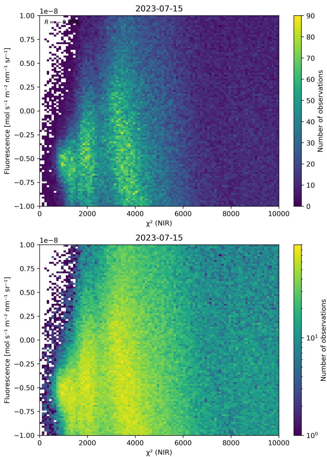
Figure 45: Scatter density plot of “ \chi^2 (NIR)” against “Fluorescence” for 2023-07-14 to 2023-07-16.
