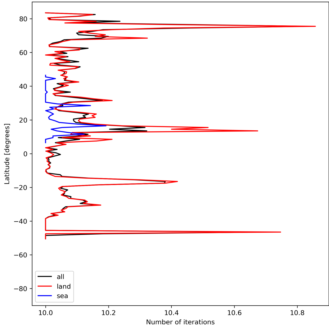
Figure 20: Zonal average of “Number of iterations” for 2023-07-14 to 2023-07-16.
