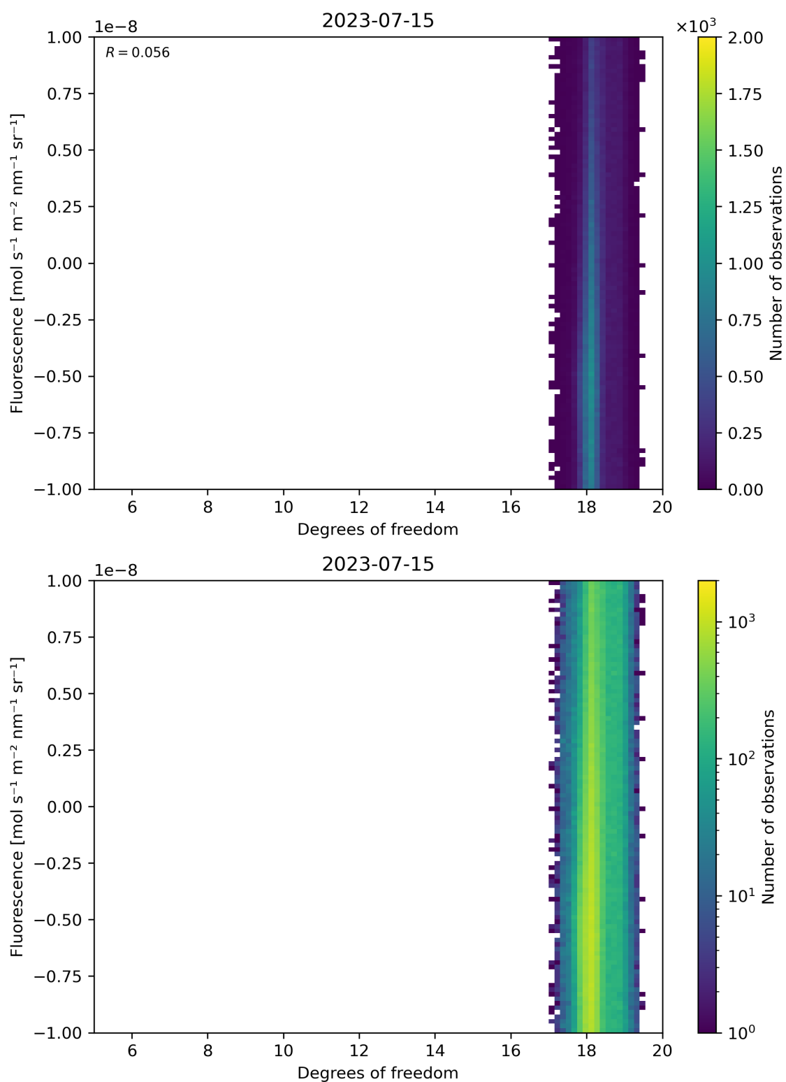
Figure 51: Scatter density plot of “Degrees of freedom” against “Fluorescence” for 2023-07-14 to 2023-07-16.
