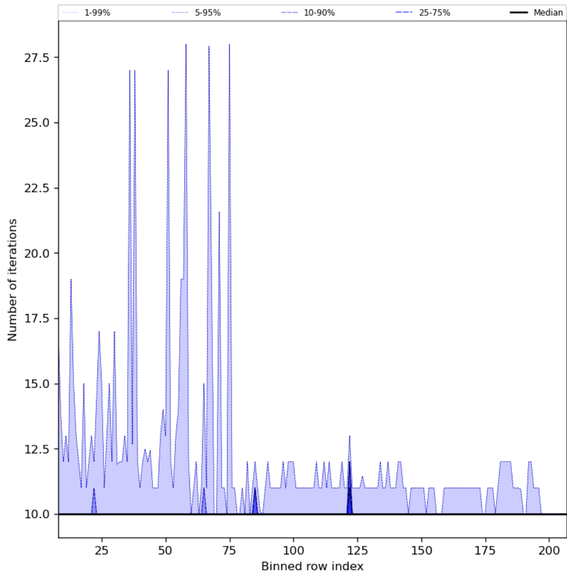
Figure 42: Along track statistics of “Number of iterations” for 2023-07-14 to 2023-07-16
