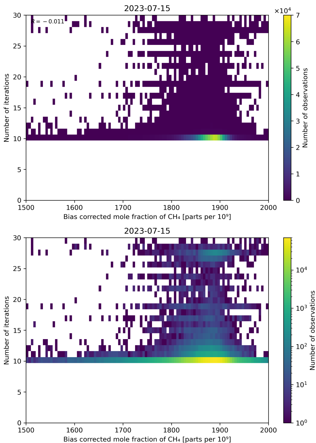
Figure 67: Scatter density plot of “Bias corrected mole fraction of CH 4 ” against “Number of iterations” for 2023-07-14 to 2023-07-16.
