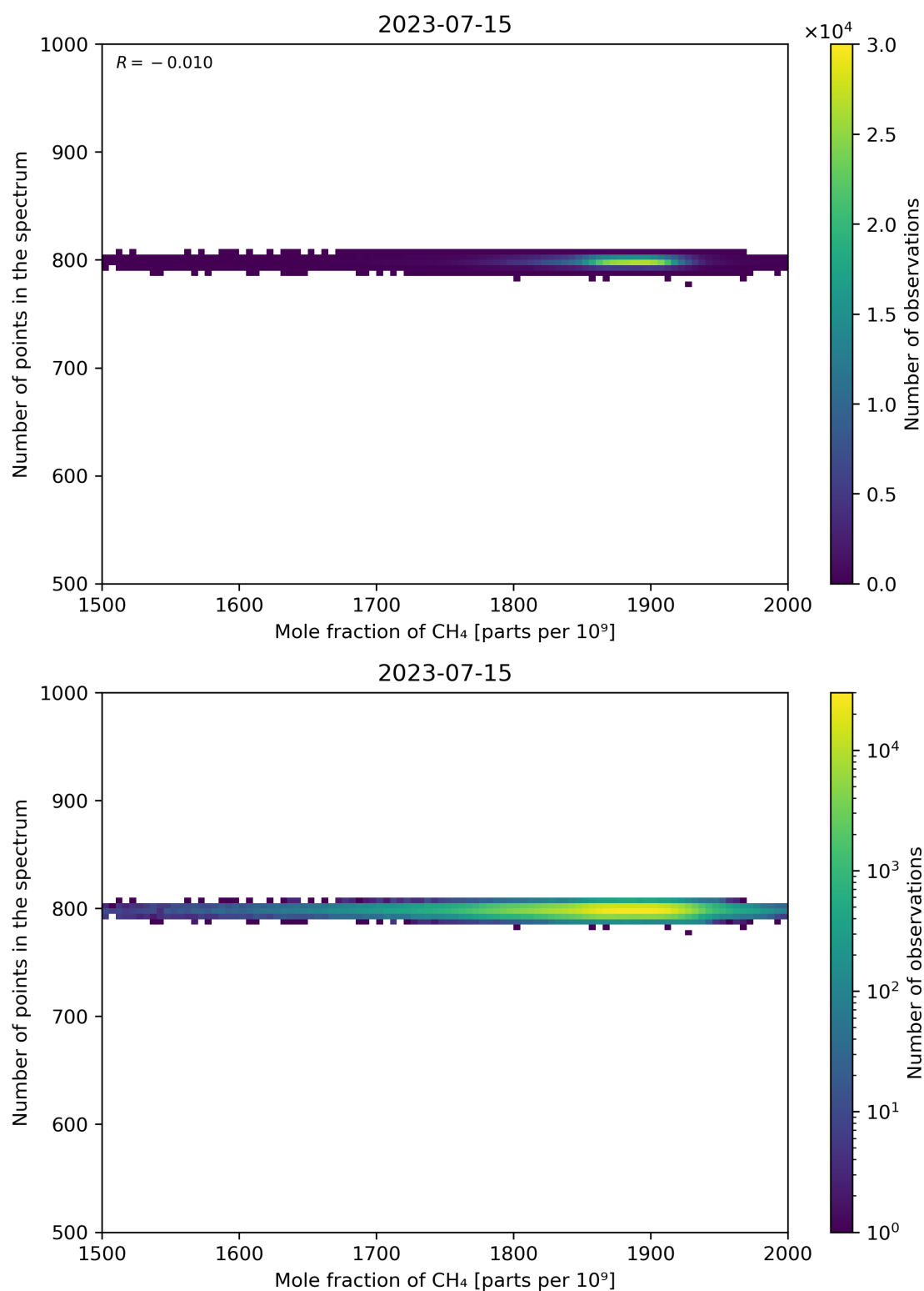
Figure 77: Scatter density plot of “Mole fraction of CH 4 ” against “Number of points in the spectrum” for 2023-07-14 to 2023-07-16.
