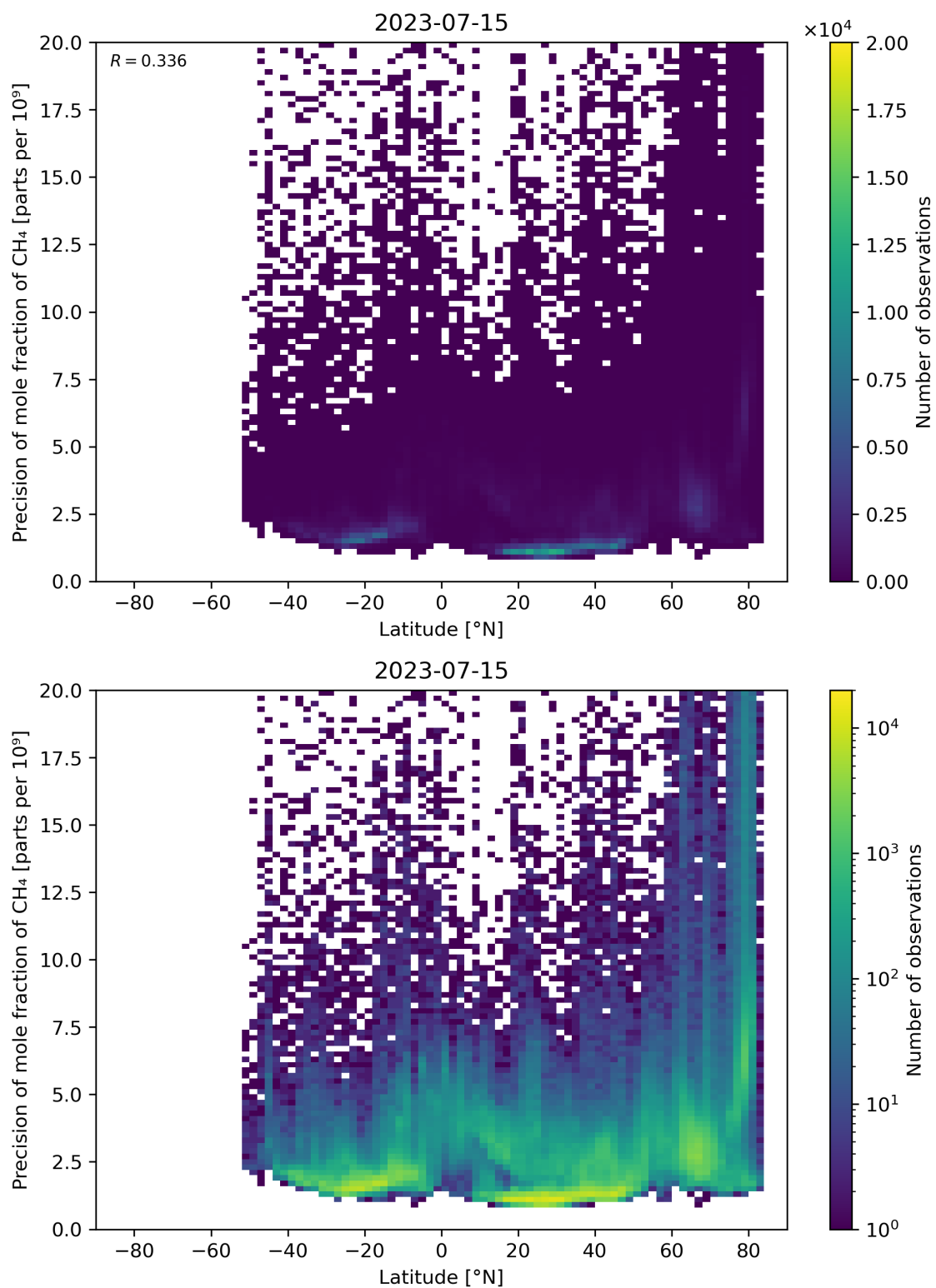
Figure 59: Scatter density plot of “Latitude” against “Precision of mole fraction of \text{CH}_4 ” for 2023-07-14 to 2023-07-16.
