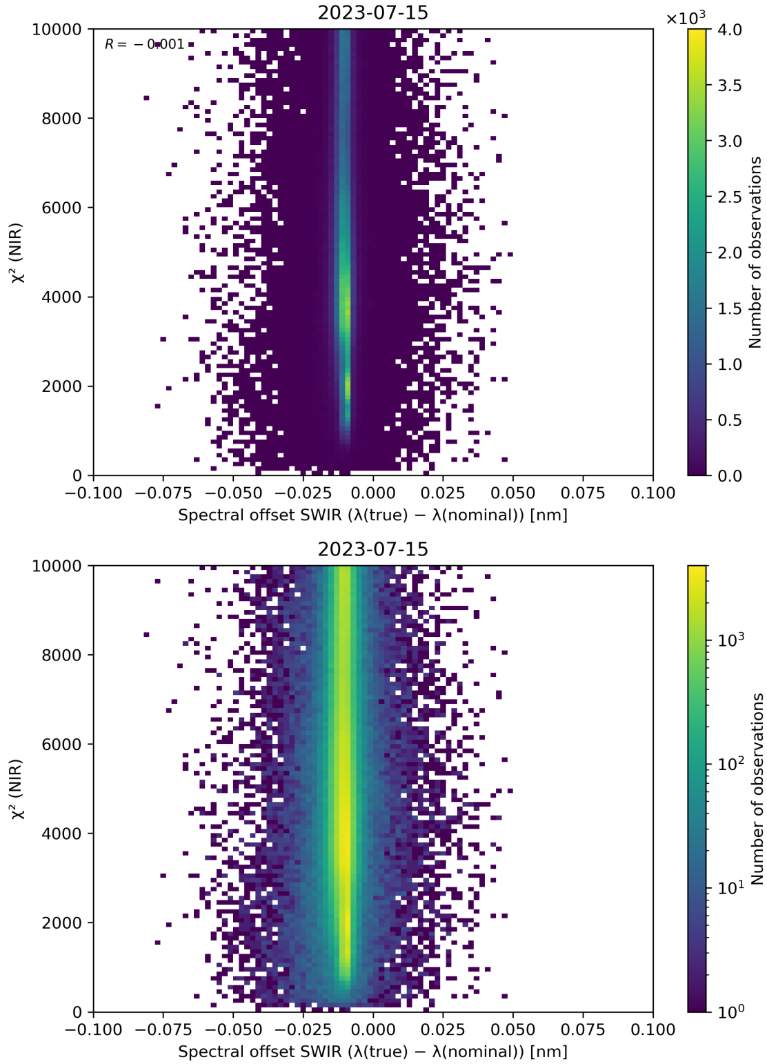
Figure 117: Scatter density plot of “Spectral offset SWIR ( \lambda(\text{true}) - \lambda(\text{nominal}) )” against “ \chi^2 (NIR)” for 2023-07-14 to 2023-07-16.
