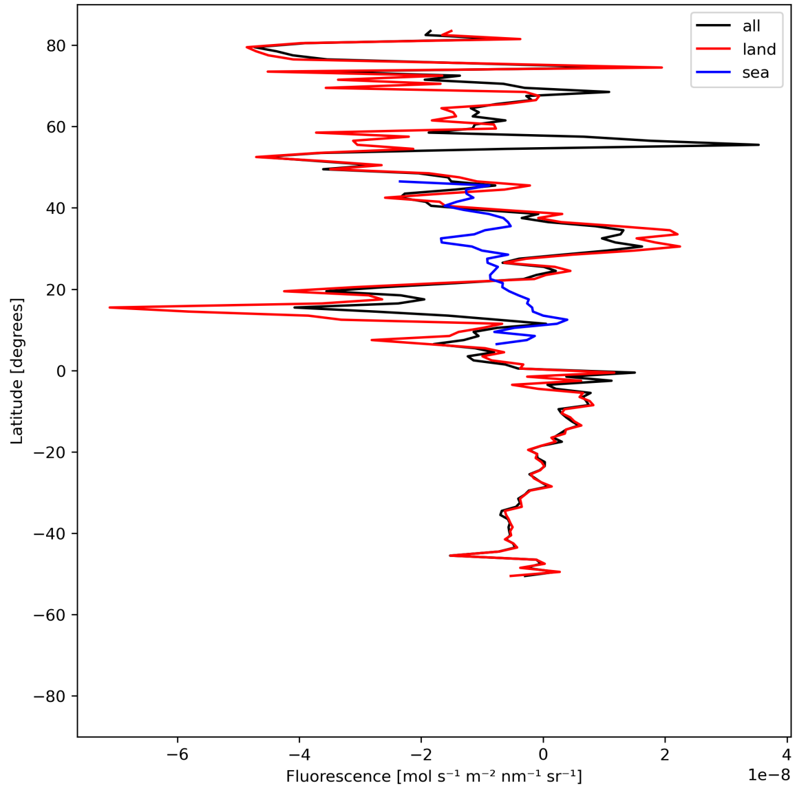
Figure 21: Zonal average of “Fluorescence” for 2023-07-14 to 2023-07-16.
