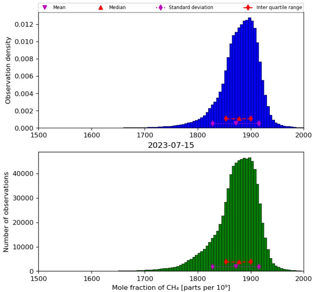
Figure 23: Histogram of “Mole fraction of CH 4 ” for 2023-07-14 to 2023-07-16
