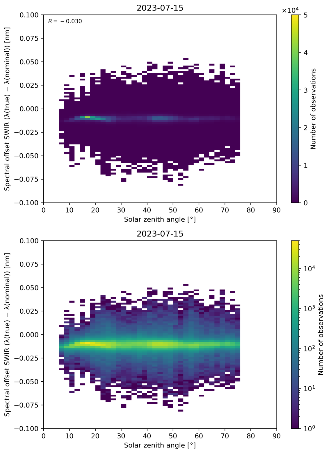
Figure 104: Scatter density plot of “Solar zenith angle” against “Spectral offset SWIR ( \lambda(\text{true}) - \lambda(\text{nominal}) )” for 2023-07-14 to 2023-07-16.
