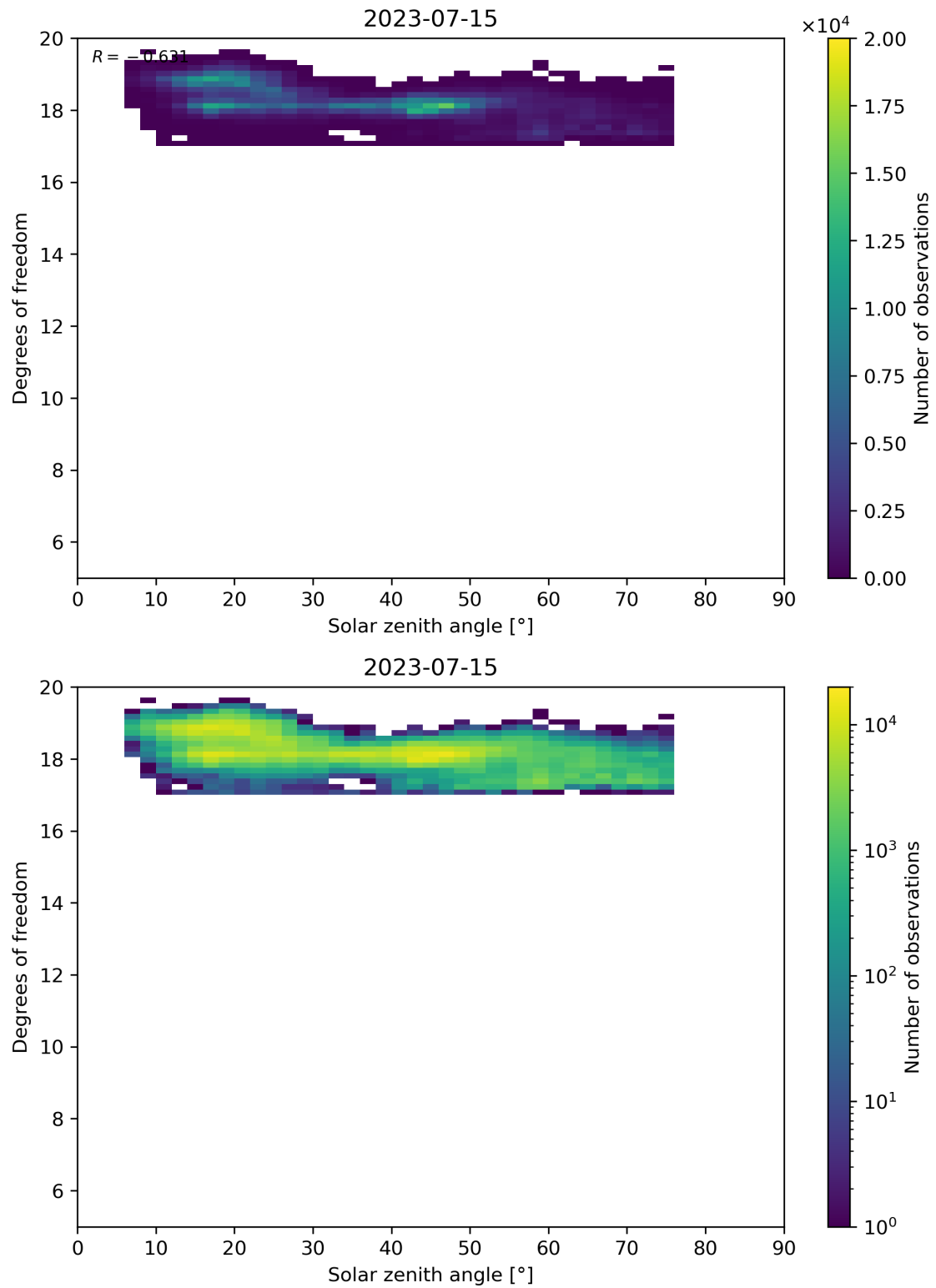
Figure 96: Scatter density plot of “Solar zenith angle” against “Degrees of freedom” for 2023-07-14 to 2023-07-16.
