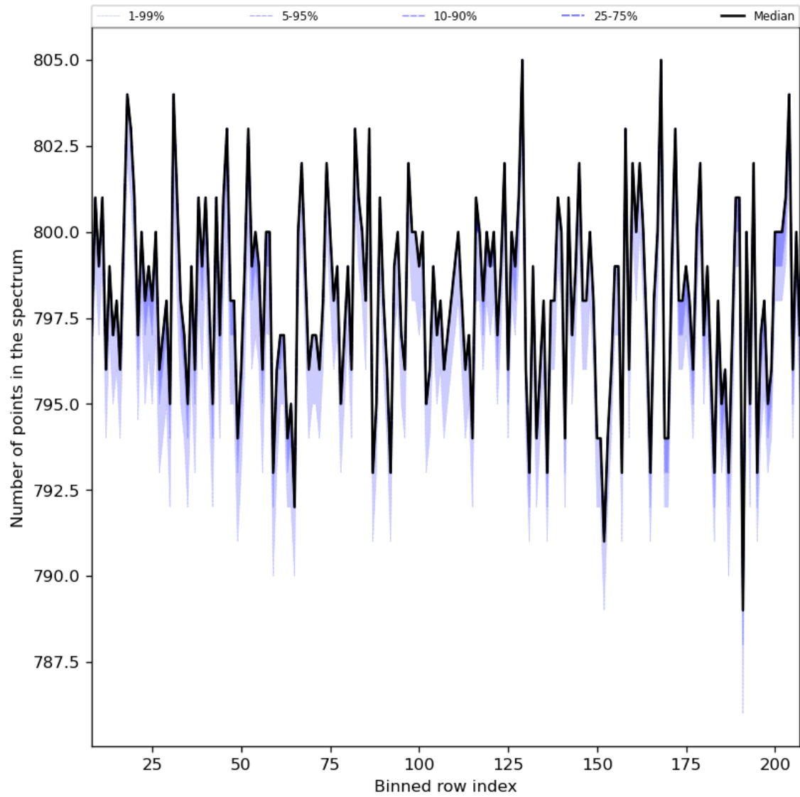
Figure 37: Along track statistics of “Number of points in the spectrum” for 2023-07-14 to 2023-07-16
