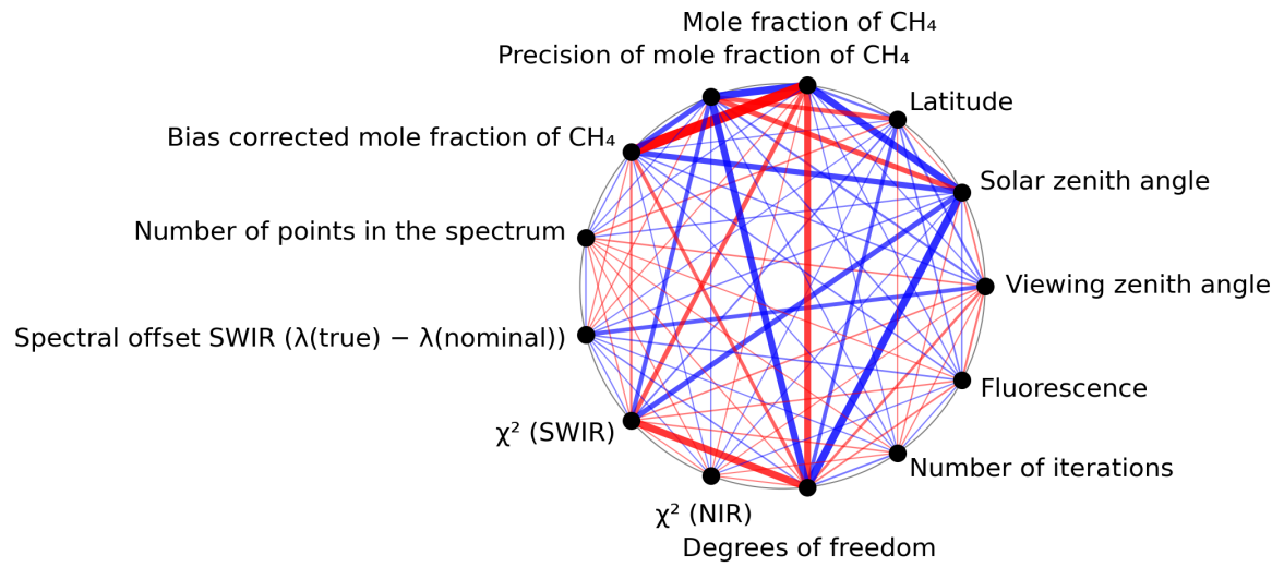
Figure 1: Map of correlation graph for 2023-07-14 to 2023-07-16.
