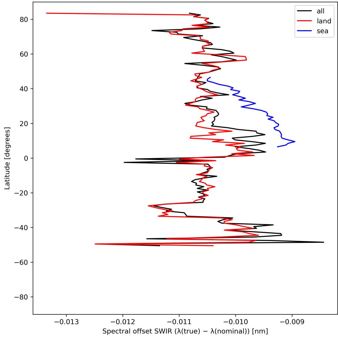
Figure 16: Zonal average of “Spectral offset SWIR ( \lambda(\text{true}) - \lambda(\text{nominal}) )” for 2023-07-14 to 2023-07-16.
