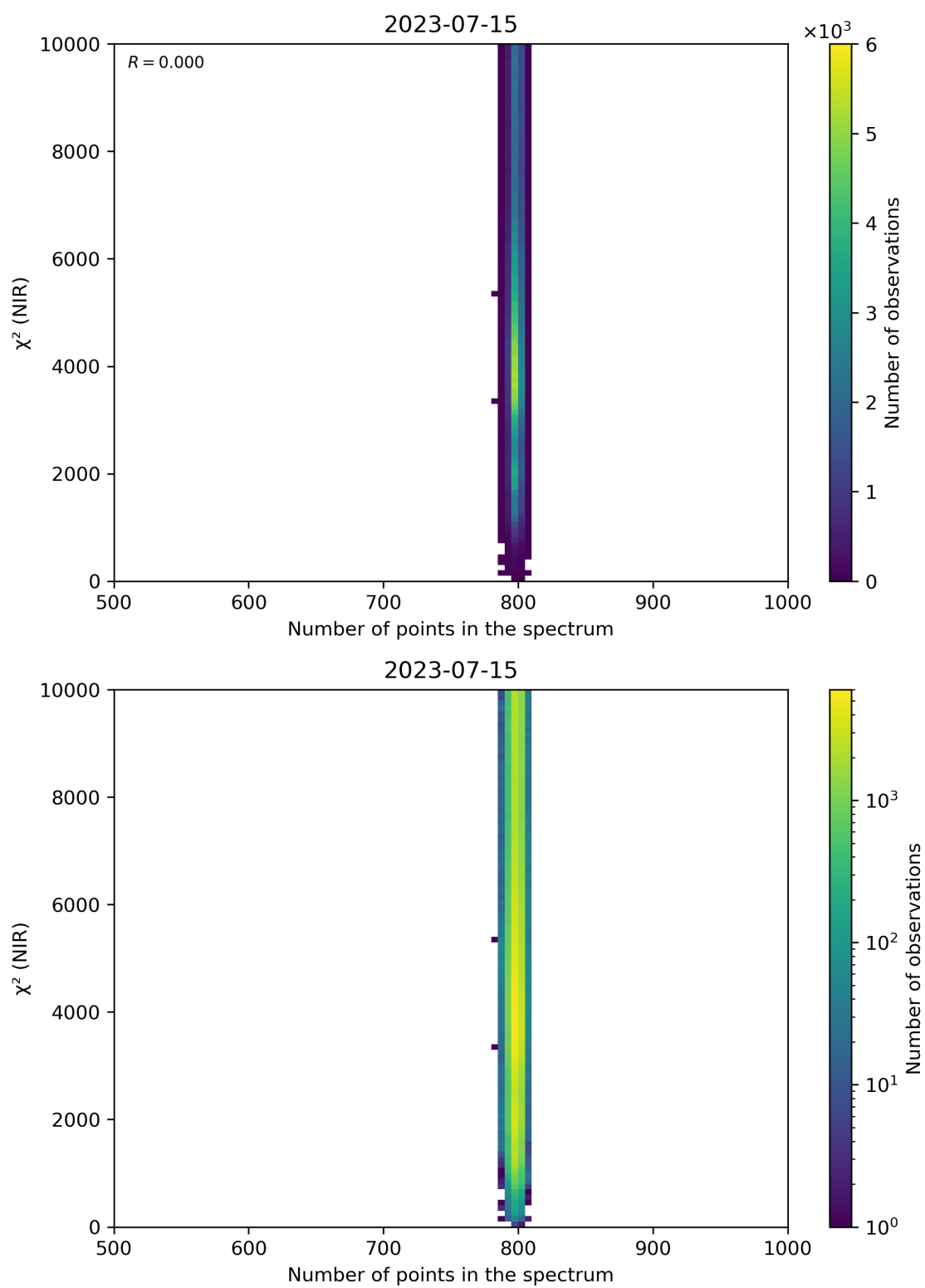
Figure 88: Scatter density plot of “Number of points in the spectrum” against “ \chi^2 (NIR)” for 2023-07-14 to 2023-07-16.
