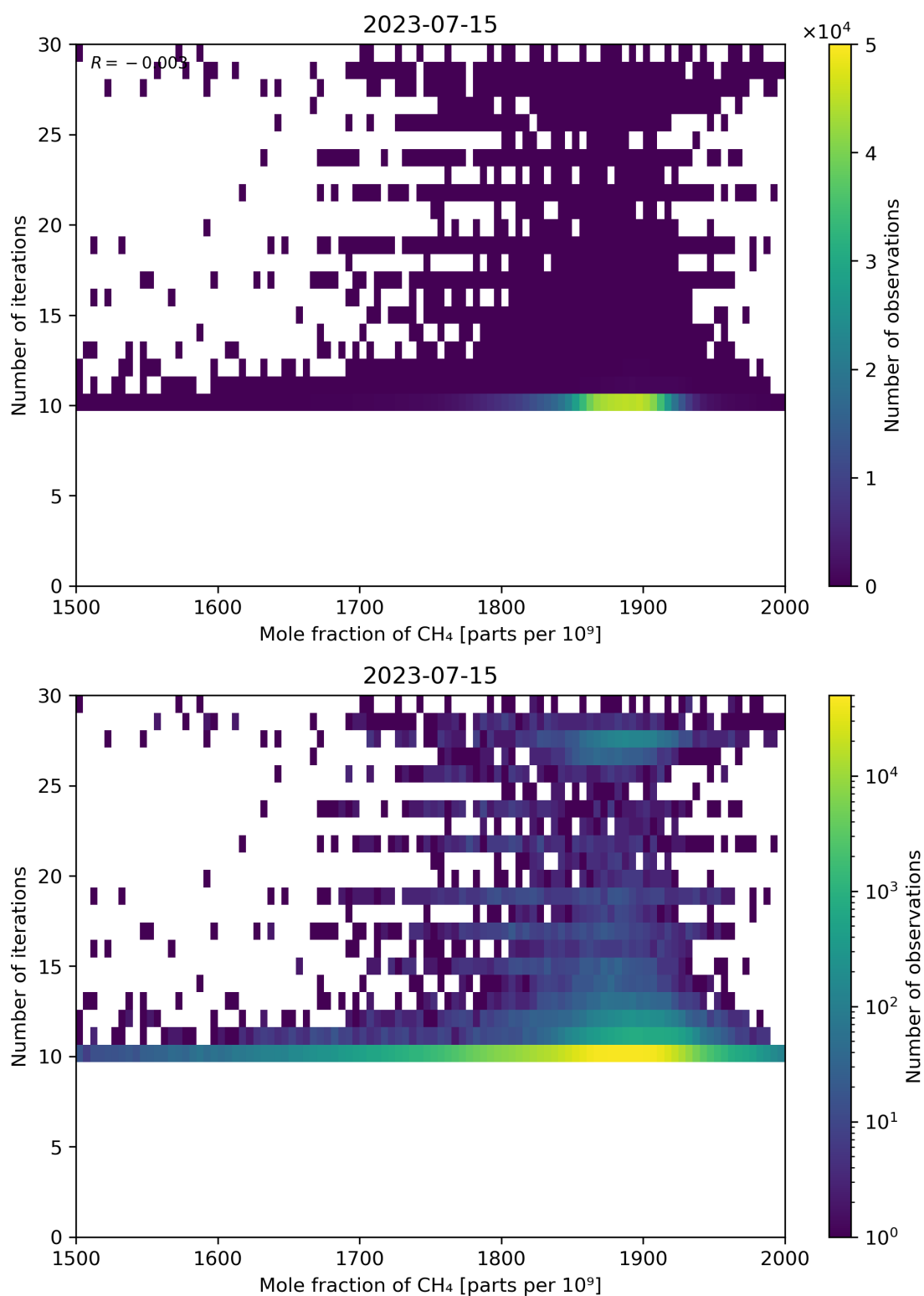
Figure 76: Scatter density plot of “Mole fraction of CH 4 ” against “Number of iterations” for 2023-07-14 to 2023-07-16.
