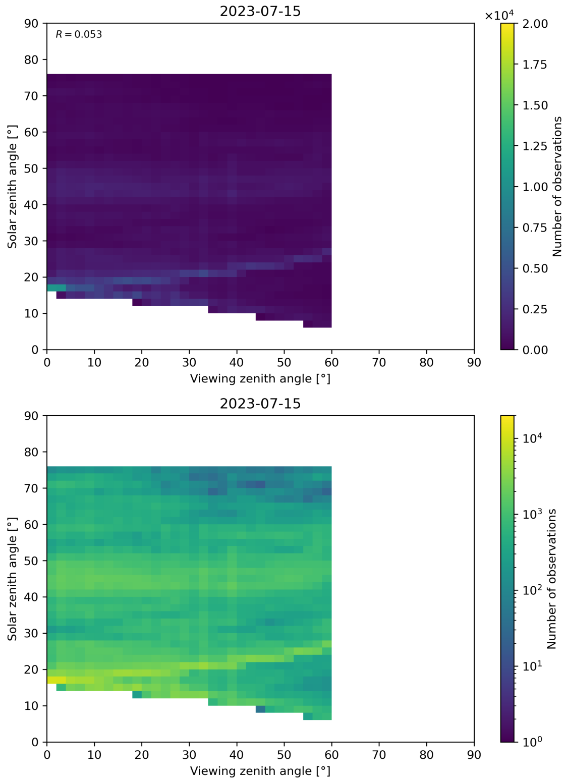
Figure 115: Scatter density plot of “Viewing zenith angle” against “Solar zenith angle” for 2023-07-14 to 2023-07-16.
