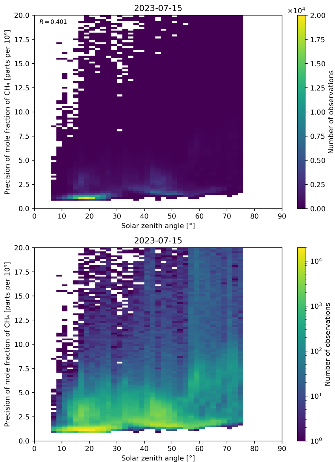
Figure 101: Scatter density plot of “Solar zenith angle” against “Precision of mole fraction of CH 4 ” for 2023-07-14 to 2023-07-16.
