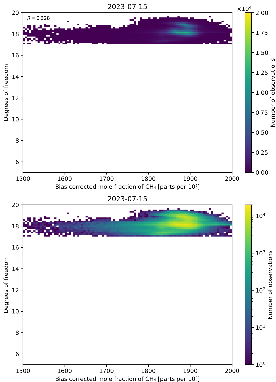
Figure 65: Scatter density plot of “Bias corrected mole fraction of CH 4 ” against “Degrees of freedom” for 2023-07-14 to 2023-07-16.
