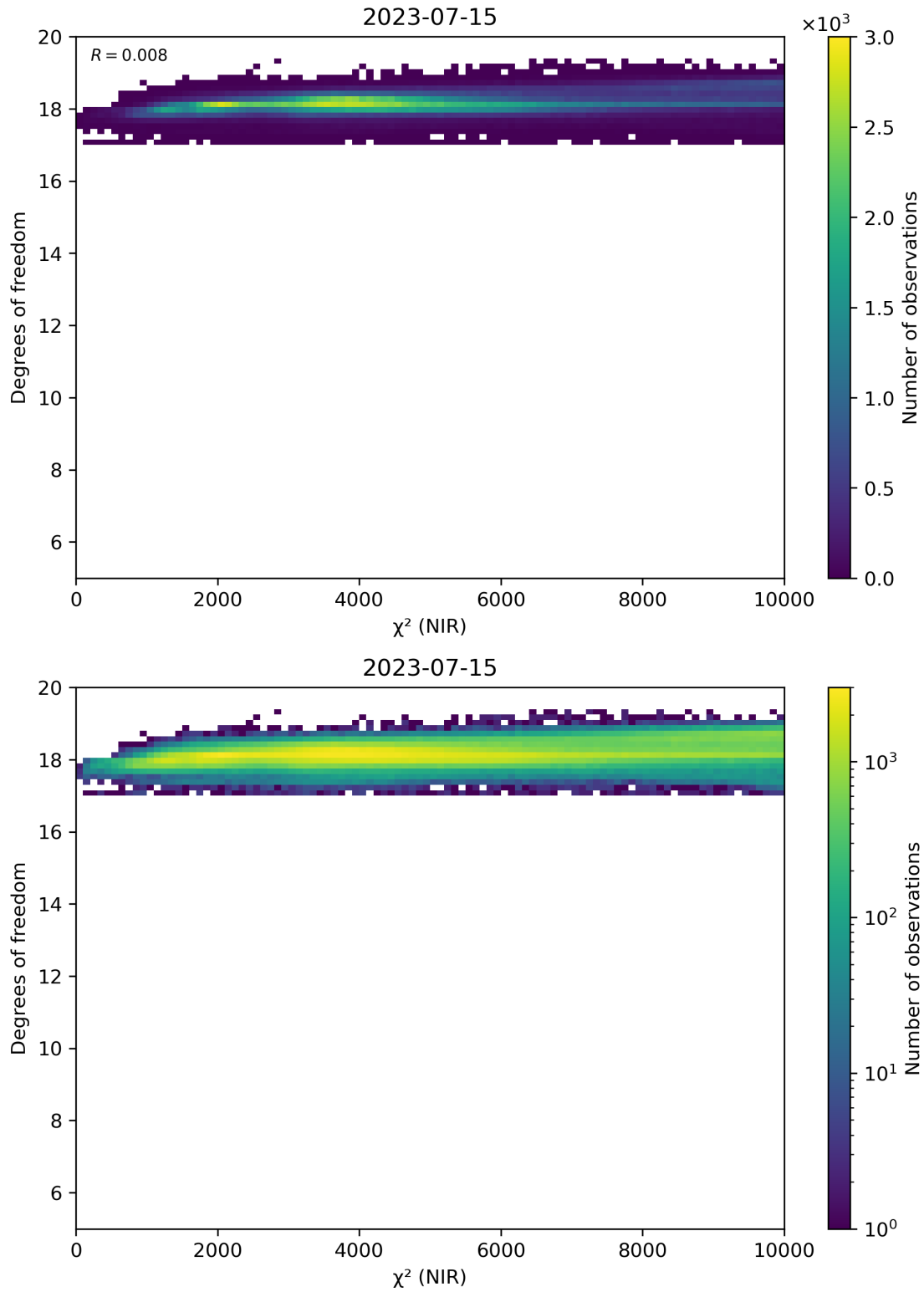
Figure 44: Scatter density plot of “ \chi^2 (NIR)” against “Degrees of freedom” for 2023-07-14 to 2023-07-16.
