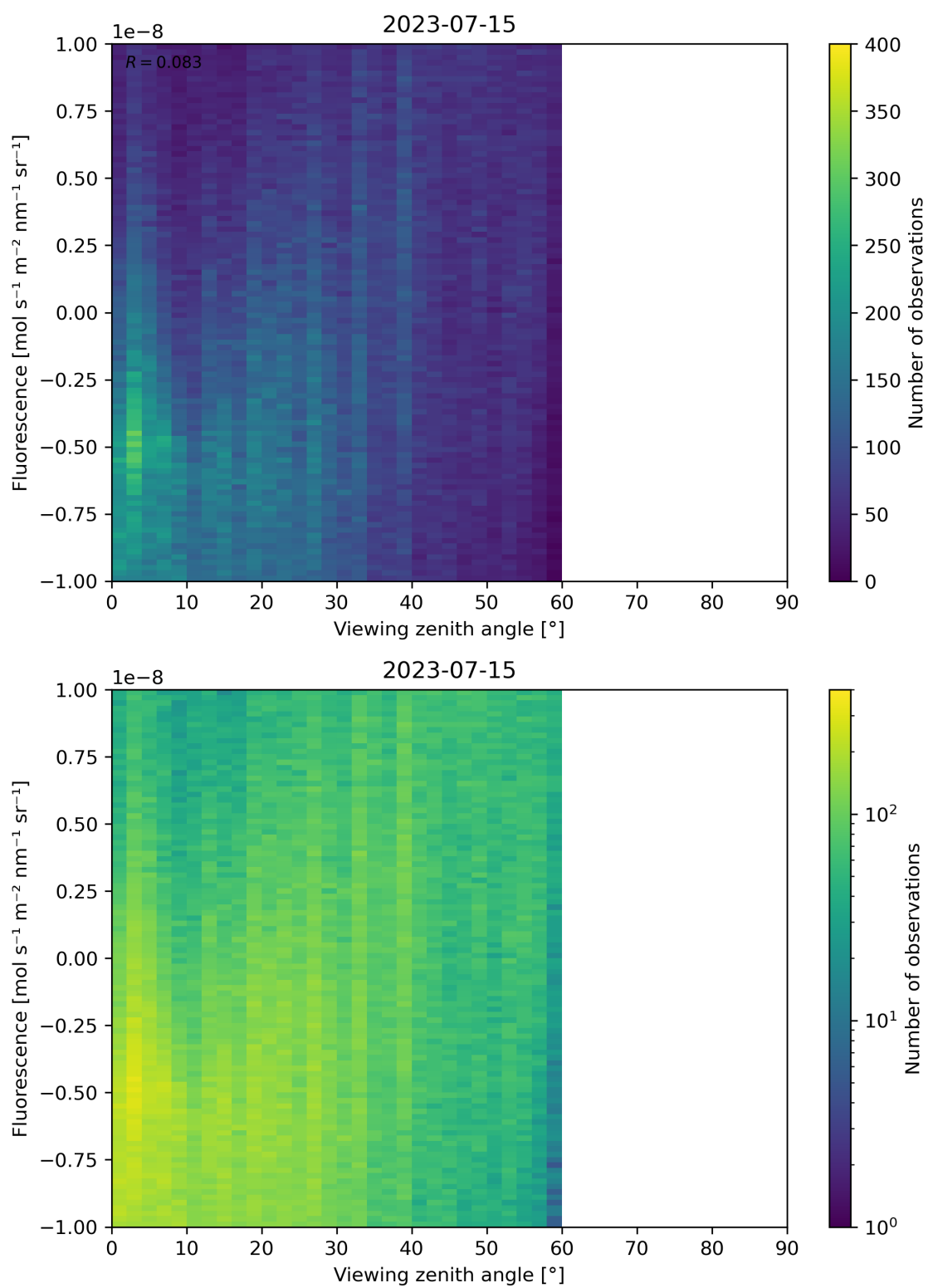
Figure 108: Scatter density plot of “Viewing zenith angle” against “Fluorescence” for 2023-07-14 to 2023-07-16.
