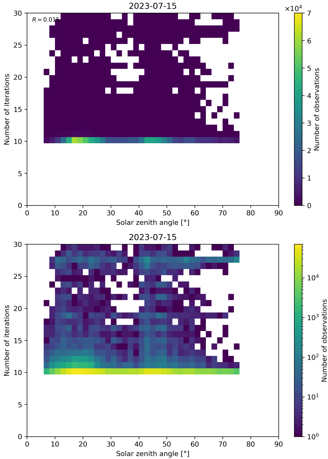
Figure 102: Scatter density plot of “Solar zenith angle” against “Number of iterations” for 2023-07-14 to 2023-07-16.
