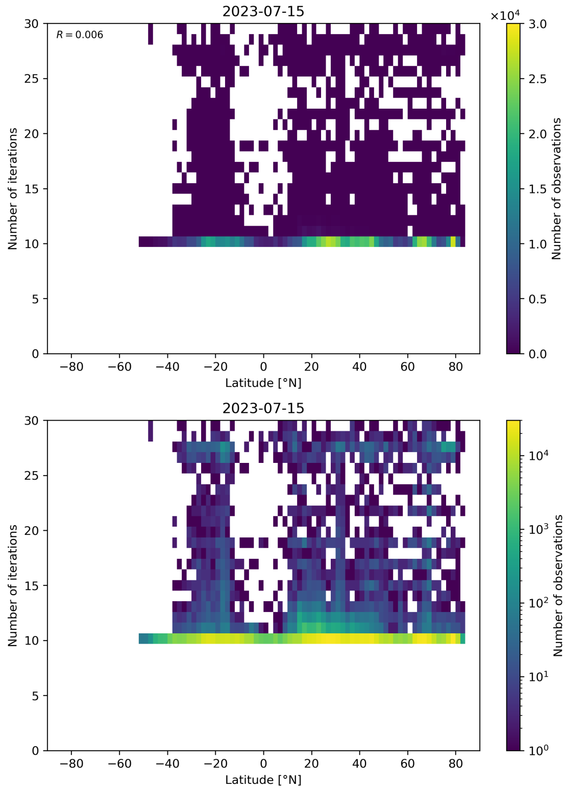
Figure 60: Scatter density plot of “Latitude” against “Number of iterations” for 2023-07-14 to 2023-07-16.
