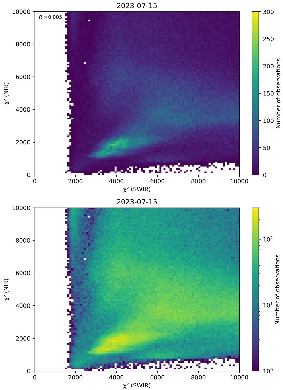
Figure 47: Scatter density plot of “ \chi^2 (SWIR)” against “ \chi^2 (NIR)” for 2023-07-14 to 2023-07-16.
