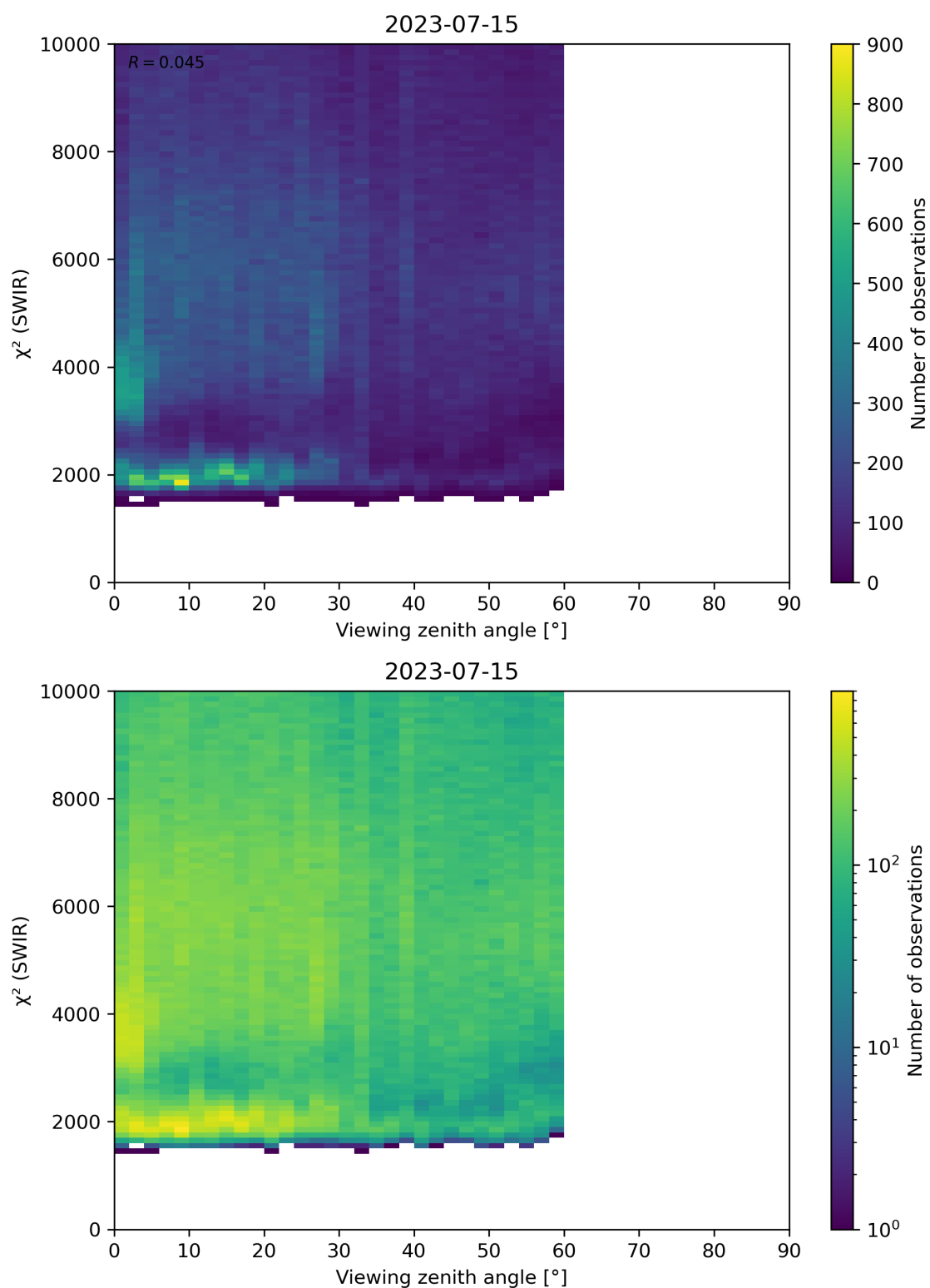
Figure 106: Scatter density plot of “Viewing zenith angle” against “ \chi^2 (SWIR)” for 2023-07-14 to 2023-07-16.
