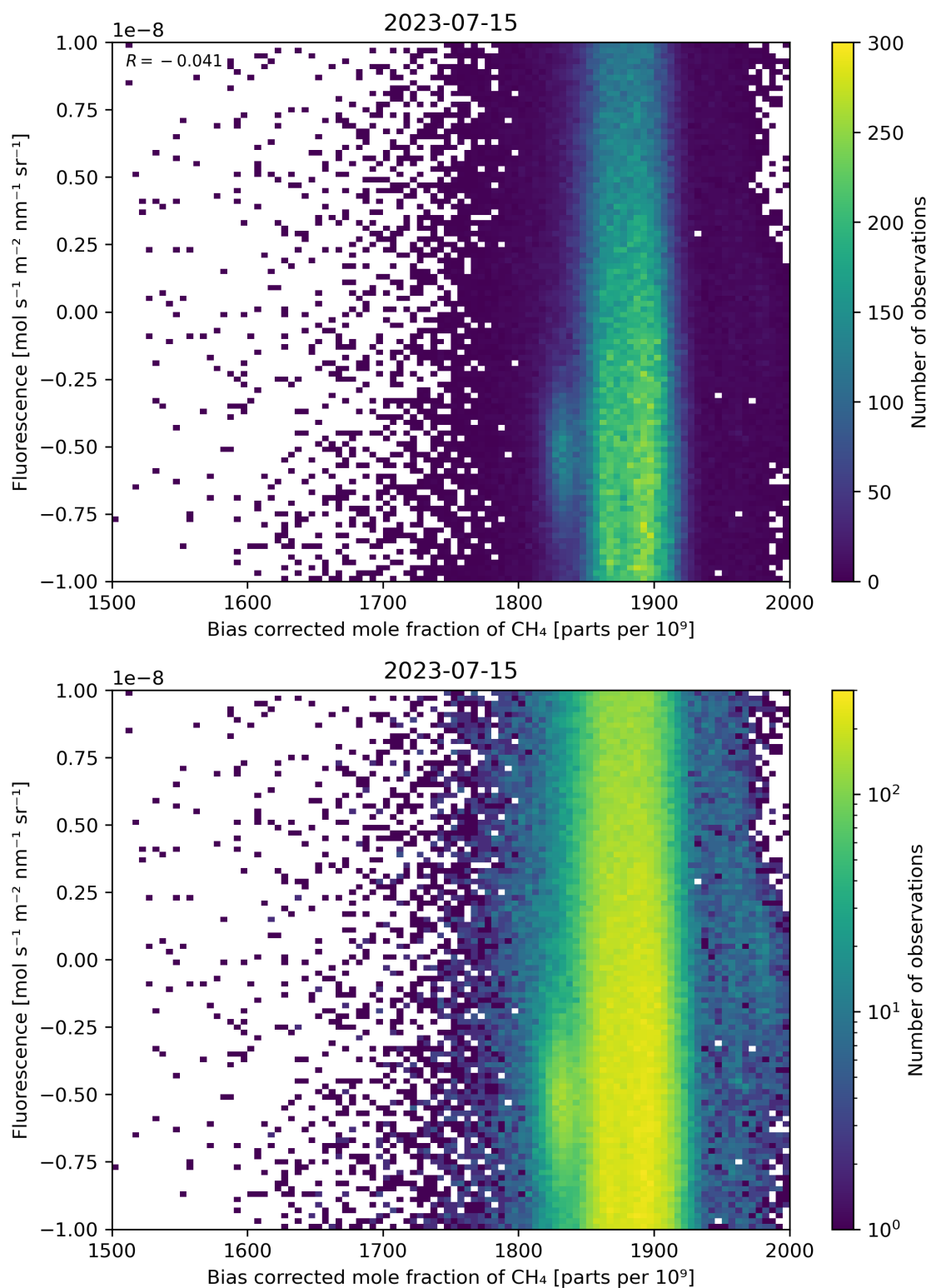
Figure 66: Scatter density plot of “Bias corrected mole fraction of \text{CH}_4 ” against “Fluorescence” for 2023-07-14 to 2023-07-16.
