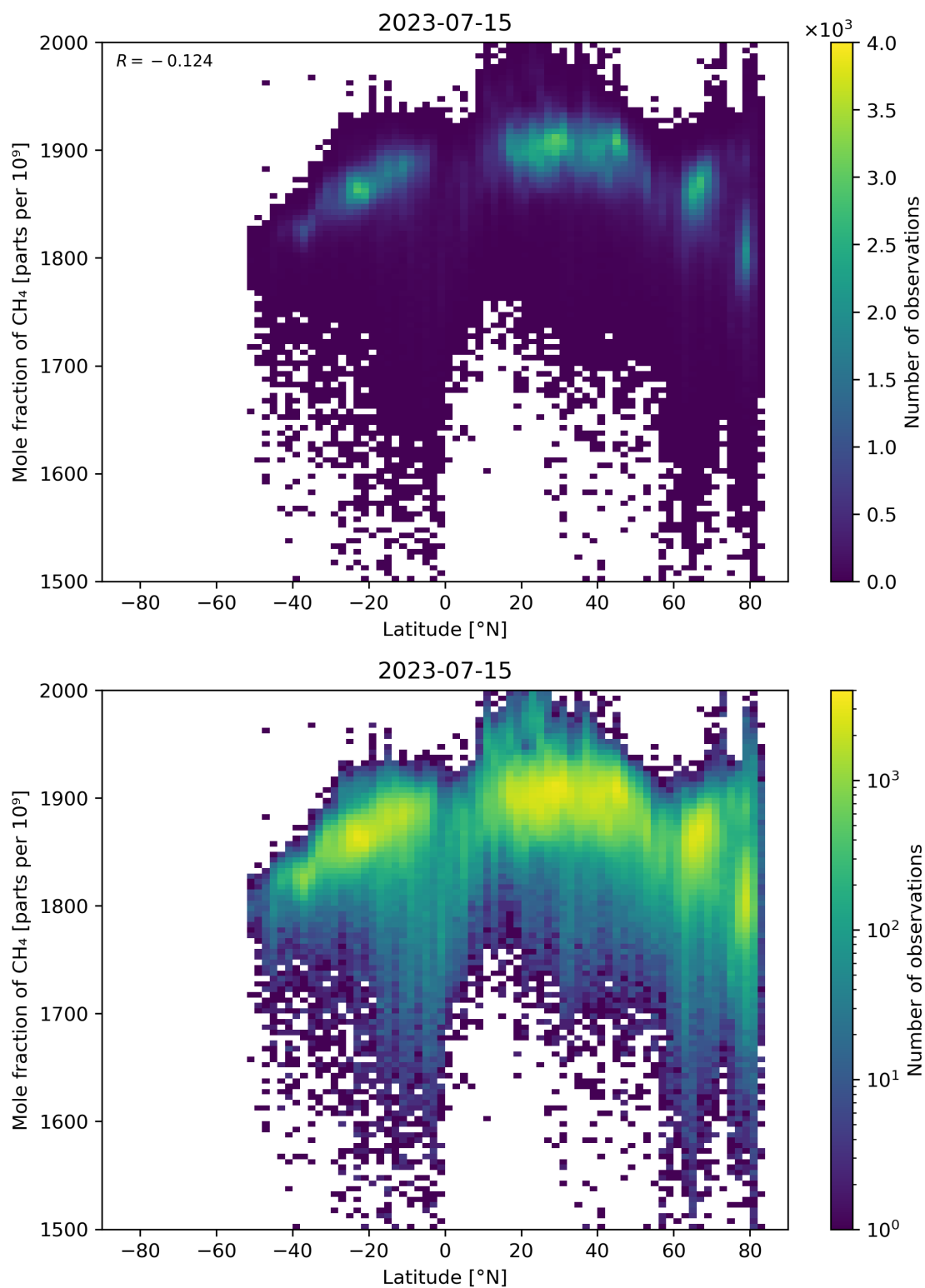
Figure 57: Scatter density plot of “Latitude” against “Mole fraction of CH 4 ” for 2023-07-14 to 2023-07-16.
