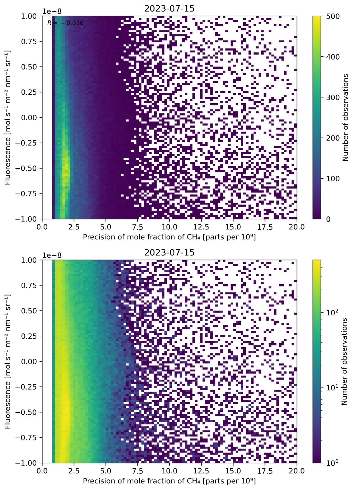
Figure 81: Scatter density plot of “Precision of mole fraction of \text{CH}_4 ” against “Fluorescence” for 2023-07-14 to 2023-07-16.
