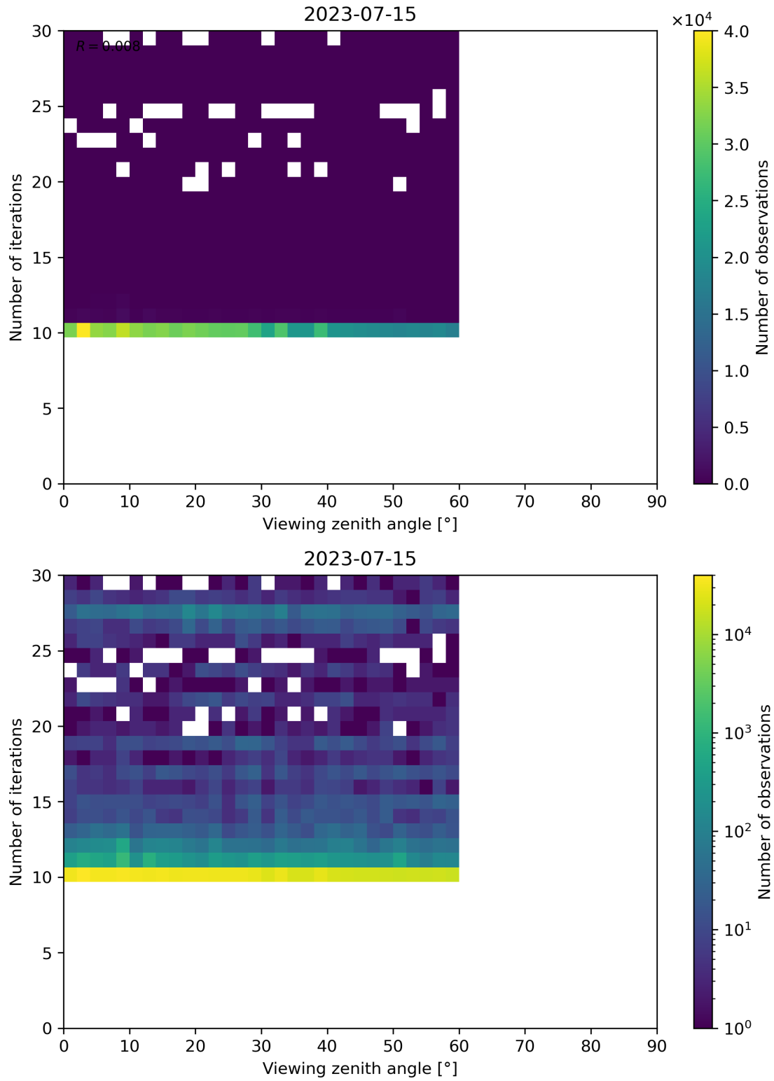
Figure 113: Scatter density plot of “Viewing zenith angle” against “Number of iterations” for 2023-07-14 to 2023-07-16.
