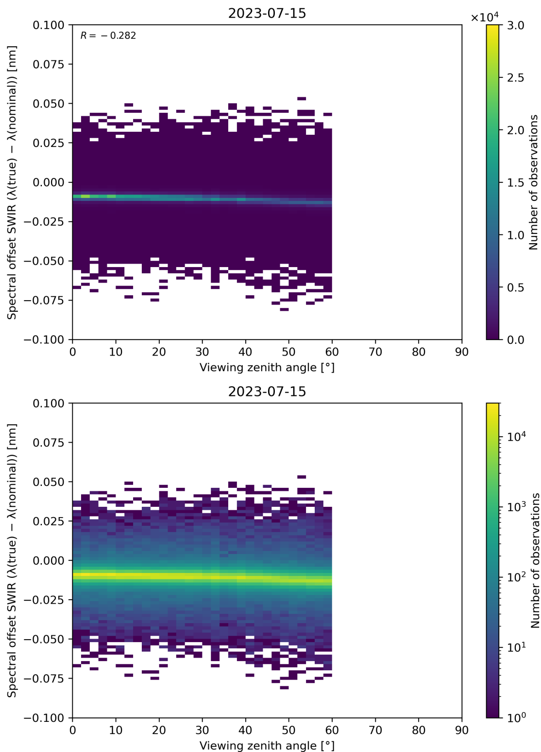
Figure 116: Scatter density plot of “Viewing zenith angle” against “Spectral offset SWIR ( \lambda(\text{true}) - \lambda(\text{nominal}) )” for 2023-07-14 to 2023-07-16.
