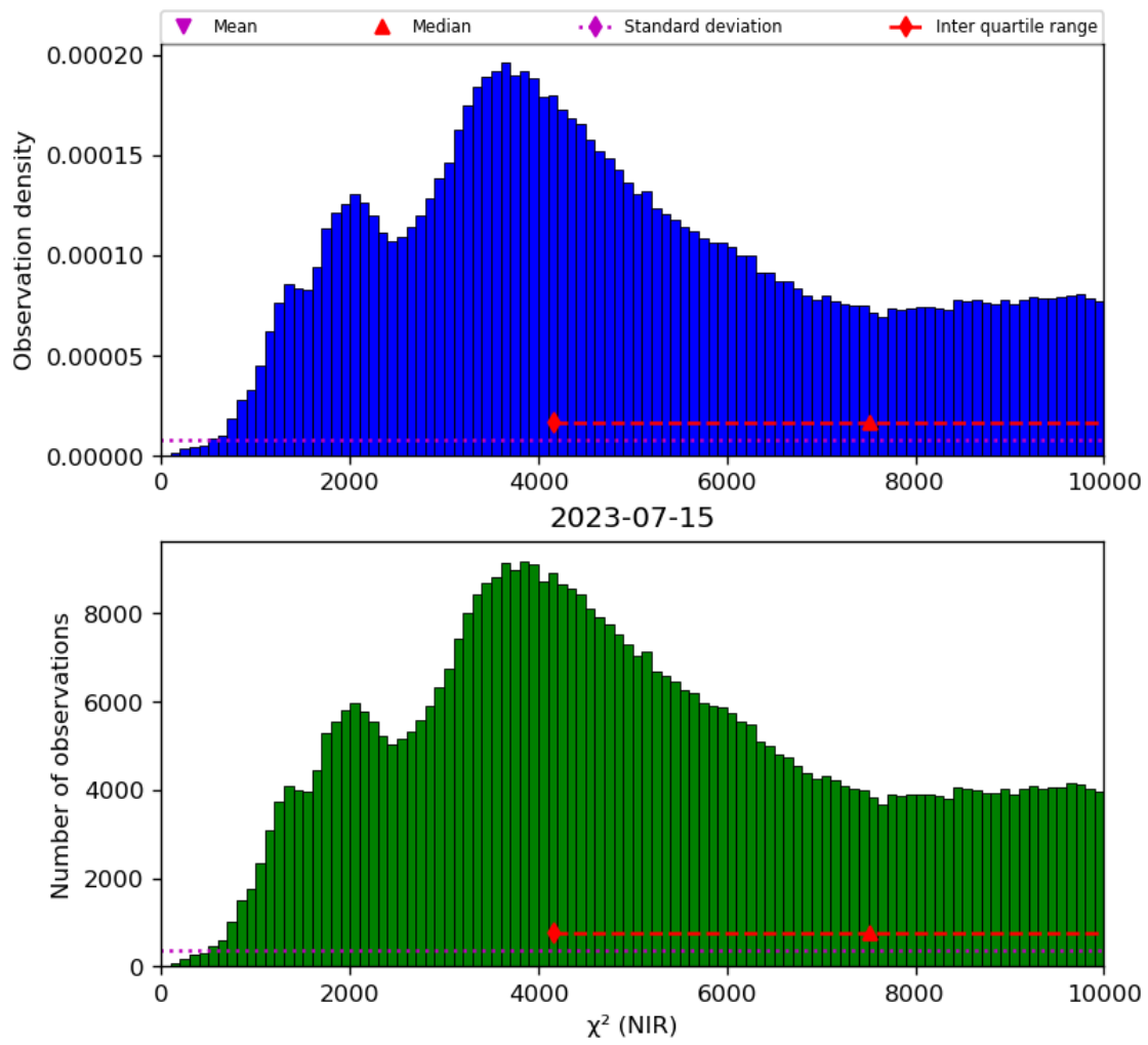
Figure 29: Histogram of “ \chi^2 (NIR)” for 2023-07-14 to 2023-07-16
