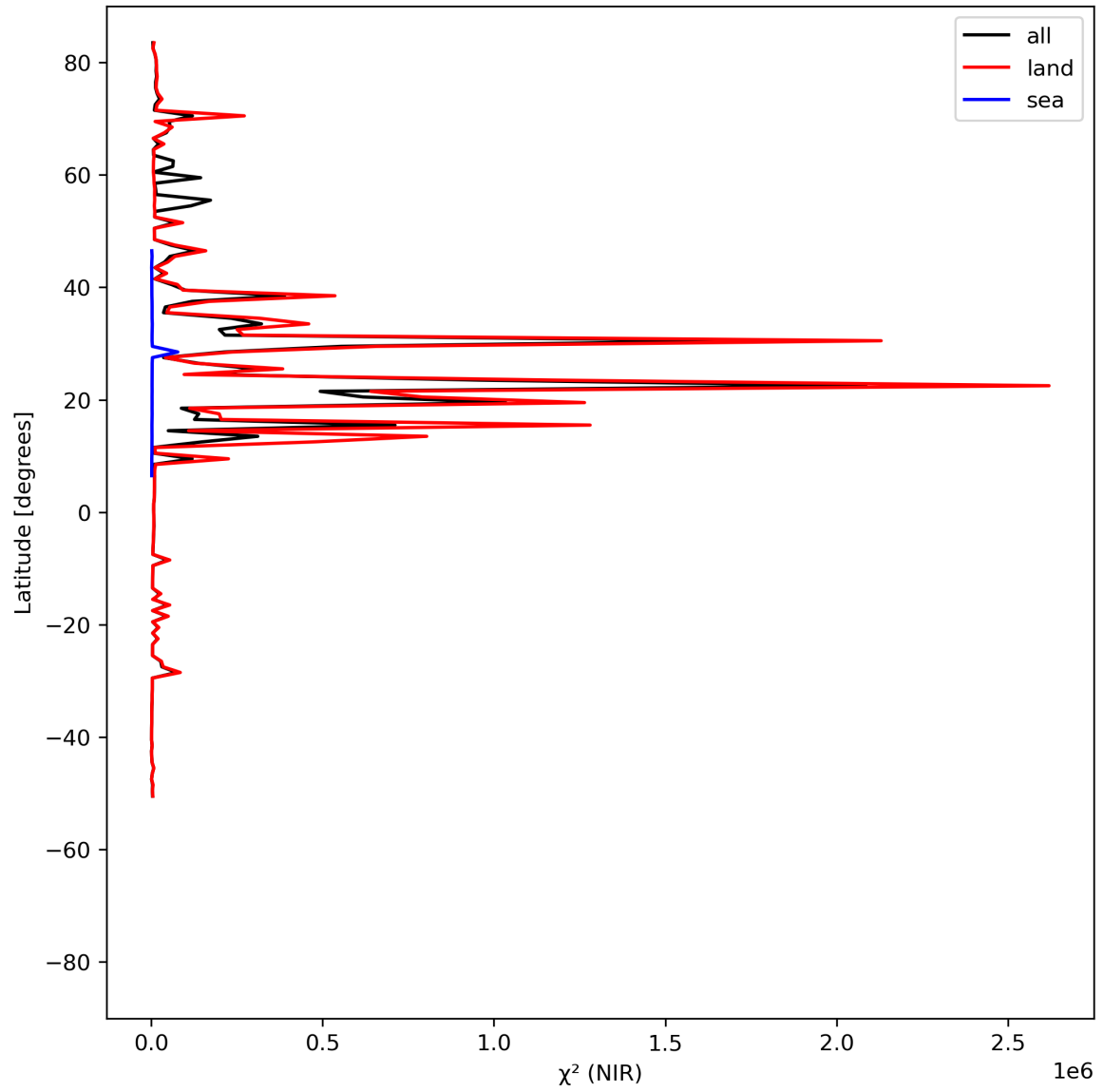
Figure 18: Zonal average of “ \chi^2 (NIR)” for 2023-07-14 to 2023-07-16.
