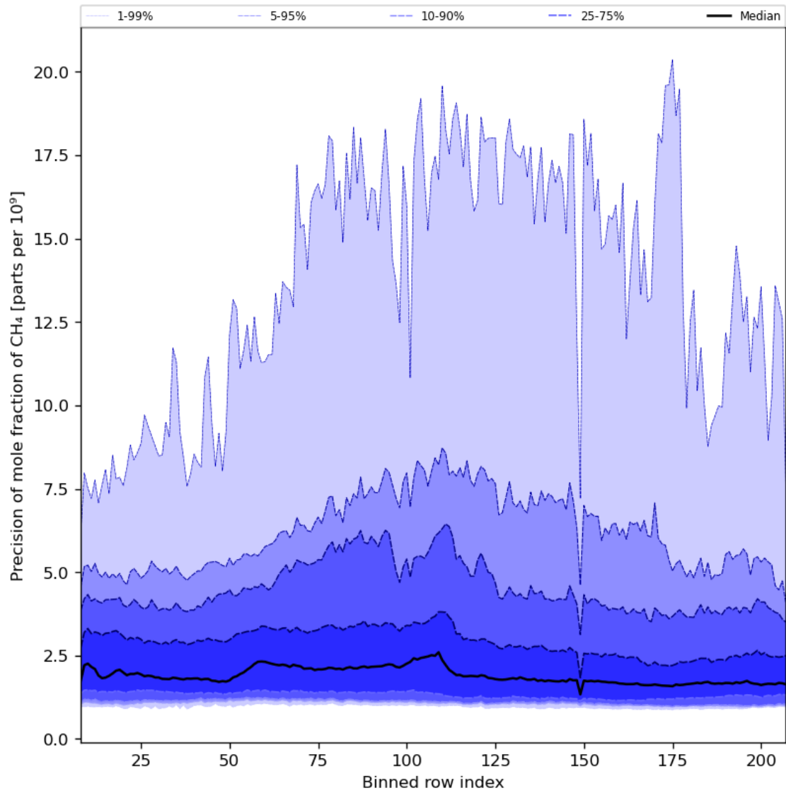
Figure 35: Along track statistics of “Precision of mole fraction of CH 4 ” for 2023-07-14 to 2023-07-16
