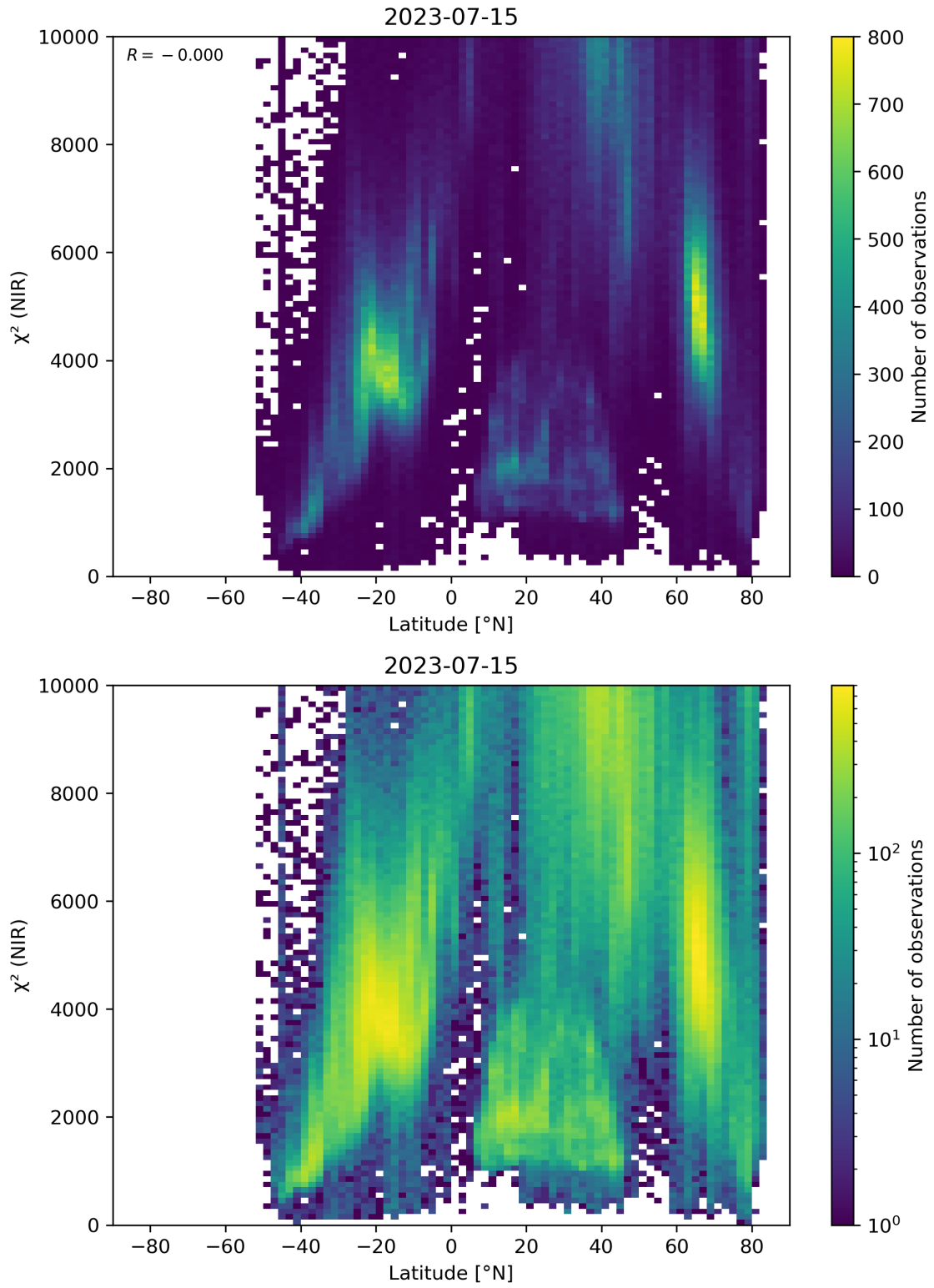
Figure 53: Scatter density plot of “Latitude” against “ \chi^2 (NIR)” for 2023-07-14 to 2023-07-16.
