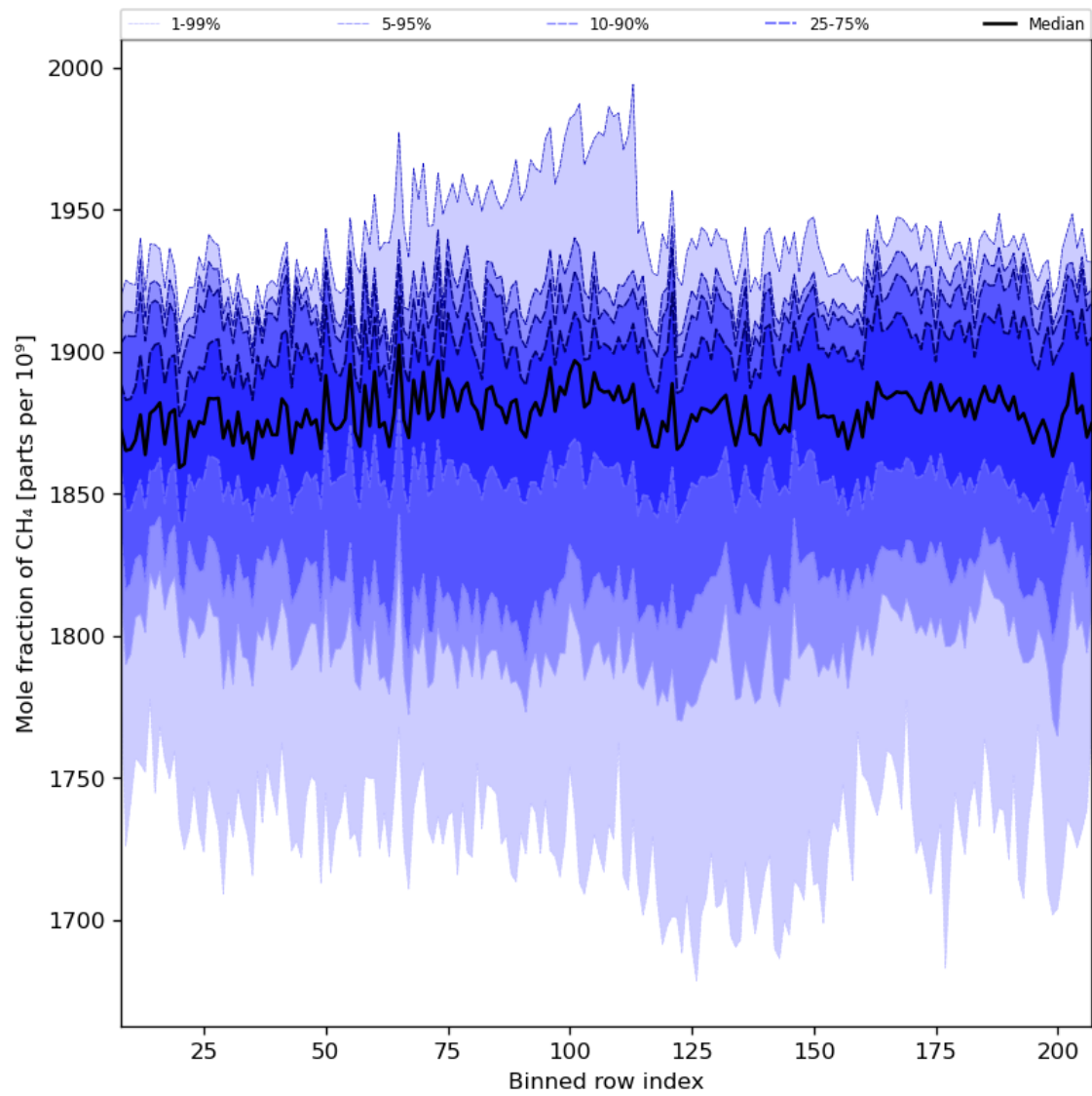
Figure 34: Along track statistics of “Mole fraction of CH 4 ” for 2023-07-14 to 2023-07-16
