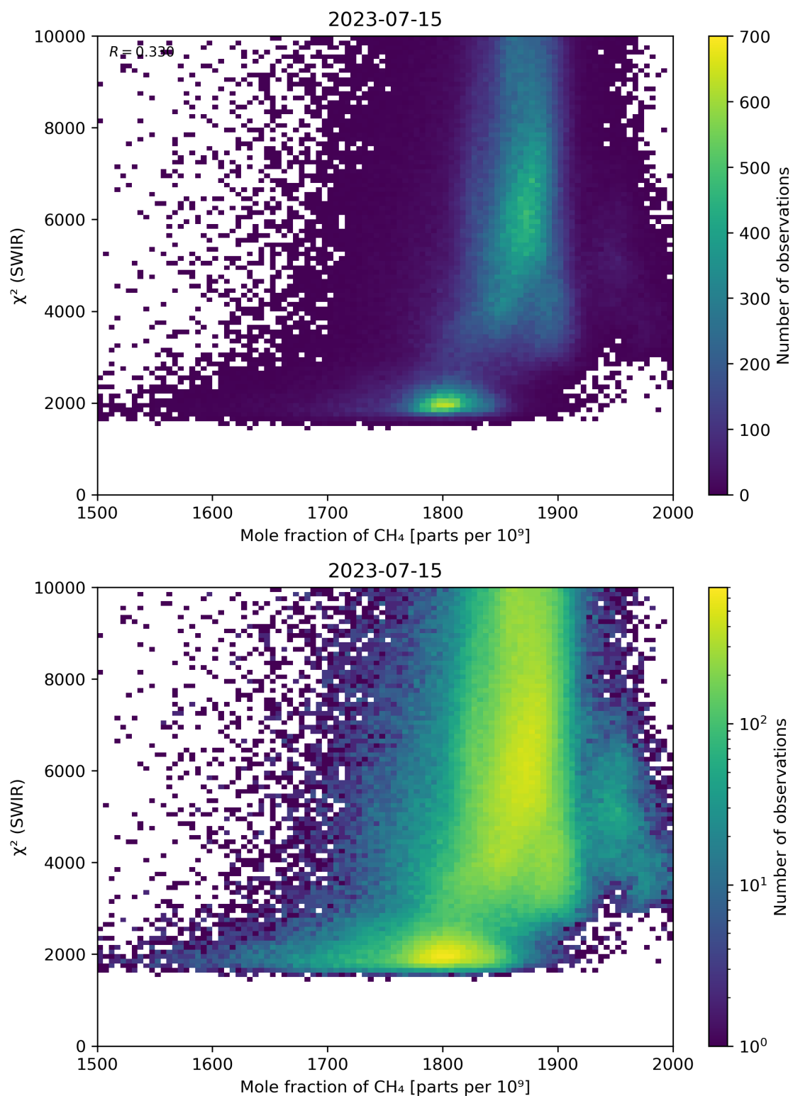
Figure 71: Scatter density plot of “Mole fraction of \text{CH}_4 ” against “ \chi^2 (SWIR)” for 2023-07-14 to 2023-07-16.
