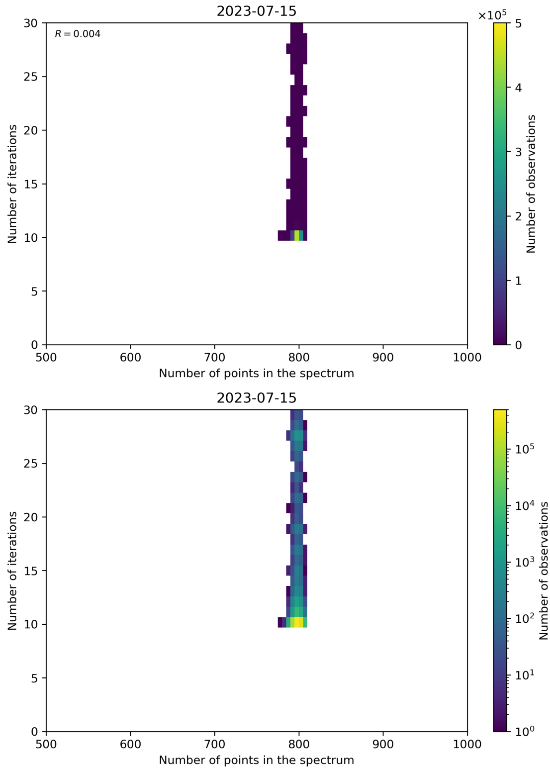
Figure 92: Scatter density plot of “Number of points in the spectrum” against “Number of iterations” for 2023-07-14 to 2023-07-16.
