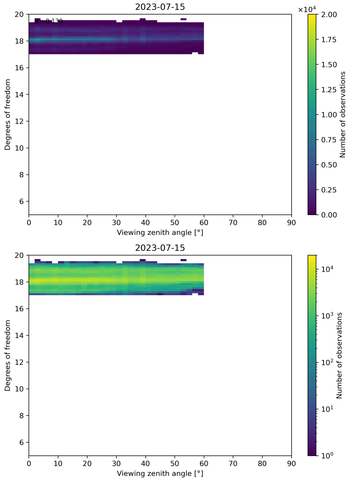
Figure 107: Scatter density plot of “Viewing zenith angle” against “Degrees of freedom” for 2023-07-14 to 2023-07-16.
