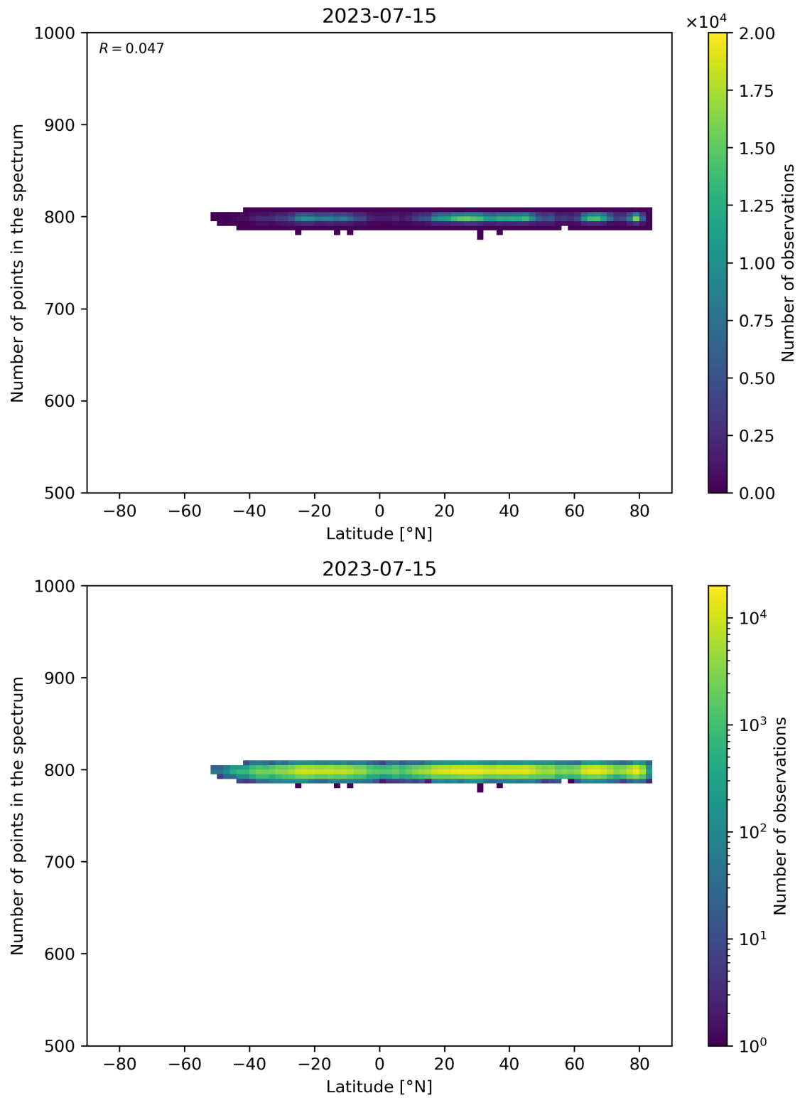
Figure 61: Scatter density plot of “Latitude” against “Number of points in the spectrum” for 2023-07-14 to 2023-07-16.
