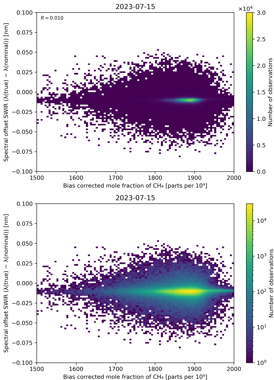
Figure 69: Scatter density plot of “Bias corrected mole fraction of \text{CH}_4 ” against “Spectral offset SWIR ( \lambda(\text{true}) - \lambda(\text{nominal}) )” for 2023-07-14 to 2023-07-16.
