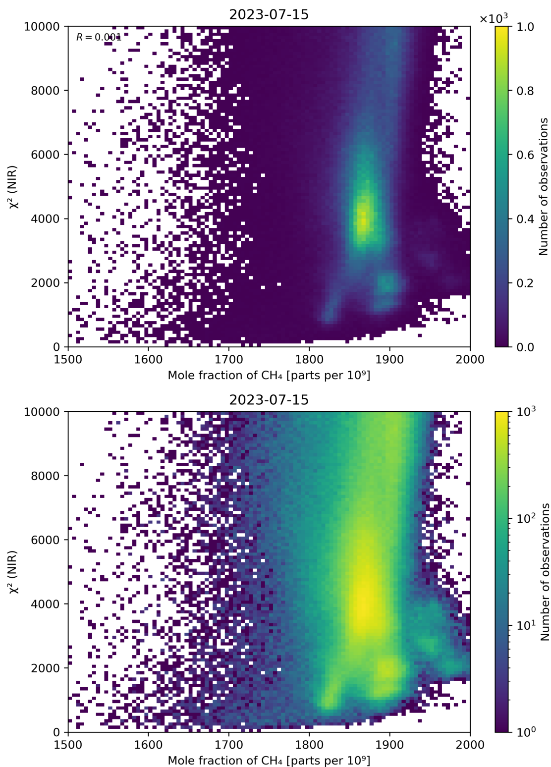
Figure 70: Scatter density plot of “Mole fraction of CH 4 ” against “ \chi^2 (NIR)” for 2023-07-14 to 2023-07-16.
