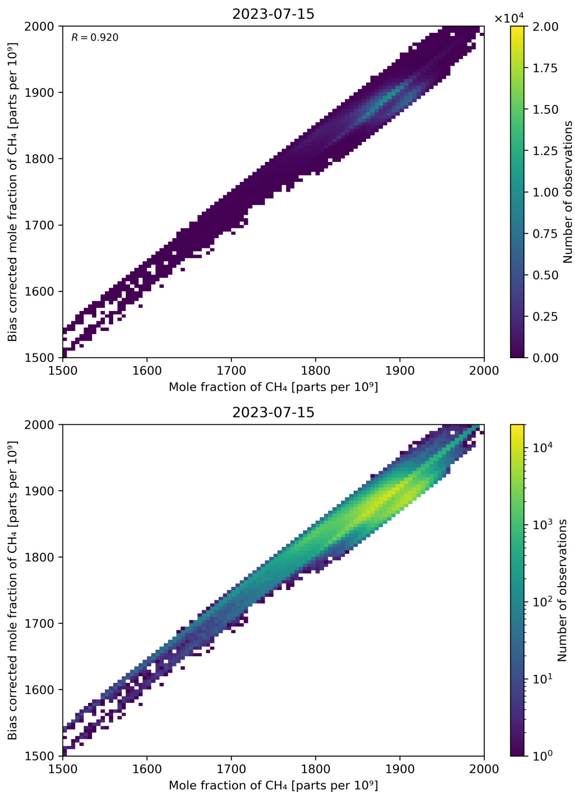
Figure 74: Scatter density plot of “Mole fraction of CH 4 ” against “Bias corrected mole fraction of CH 4 ” for 2023-07-14 to 2023-07-16.
