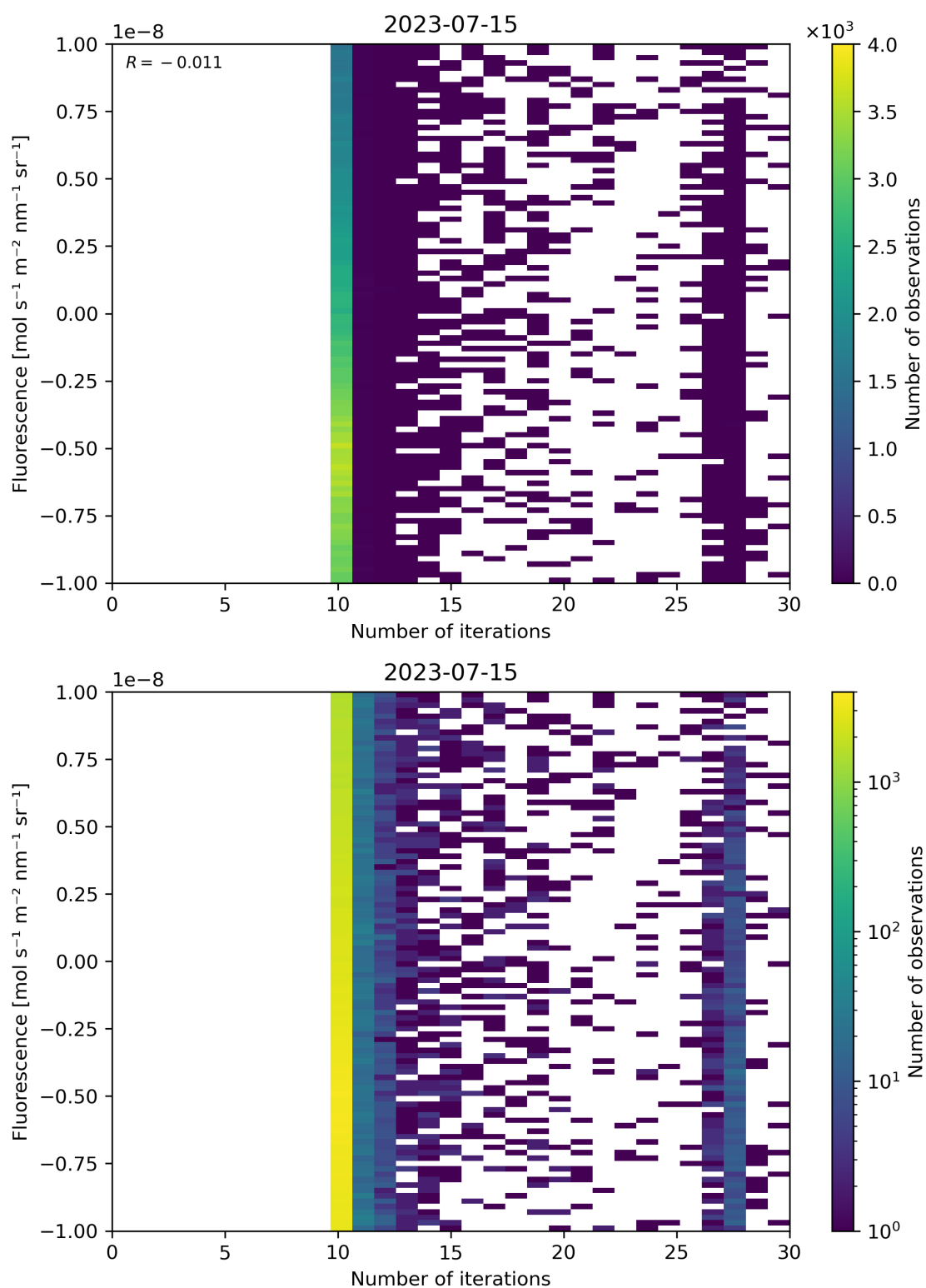
Figure 87: Scatter density plot of “Number of iterations” against “Fluorescence” for 2023-07-14 to 2023-07-16.
