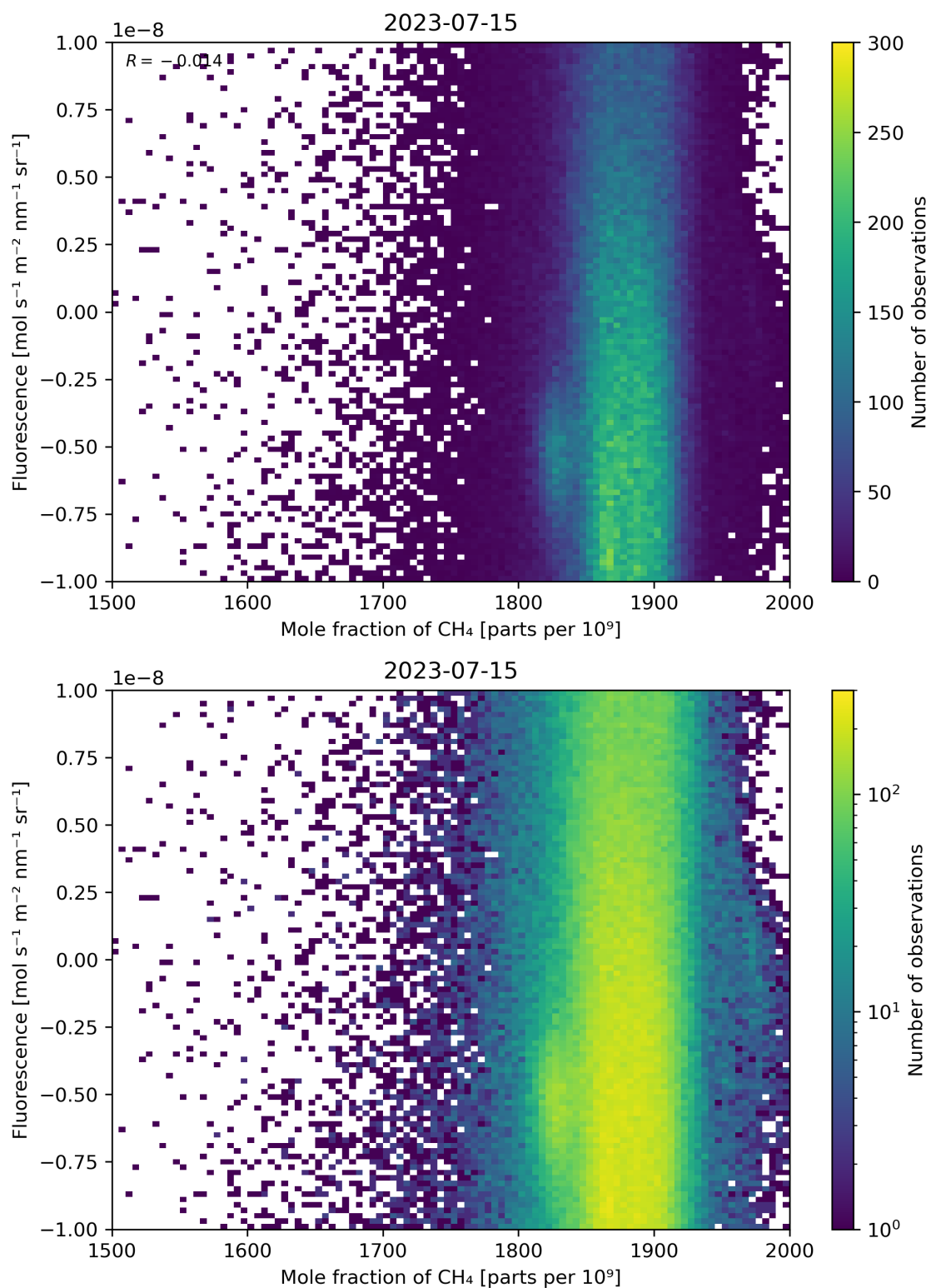
Figure 73: Scatter density plot of “Mole fraction of \text{CH}_4 ” against “Fluorescence” for 2023-07-14 to 2023-07-16.
