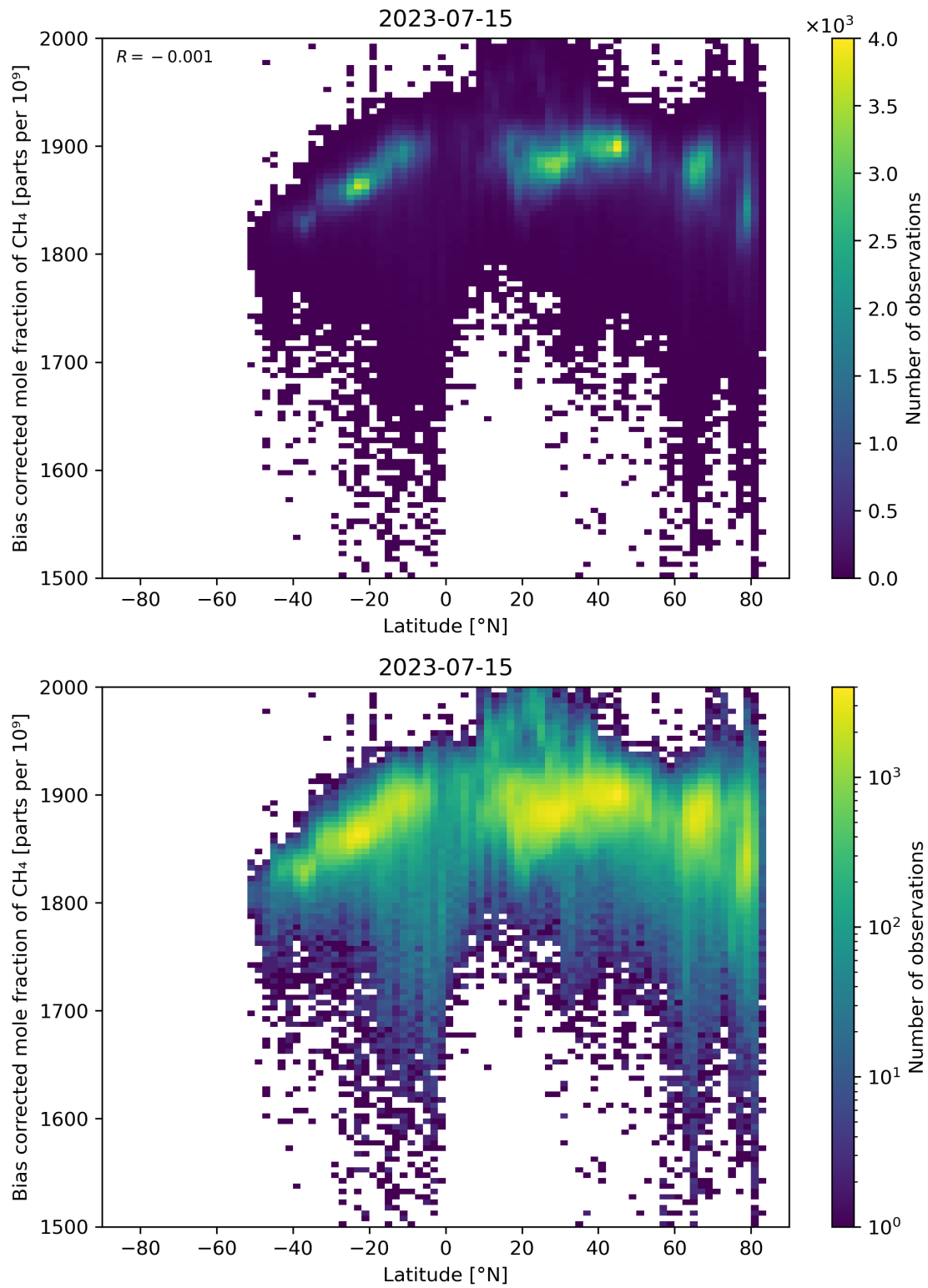
Figure 58: Scatter density plot of “Latitude” against “Bias corrected mole fraction of \text{CH}_4 ” for 2023-07-14 to 2023-07-16.
