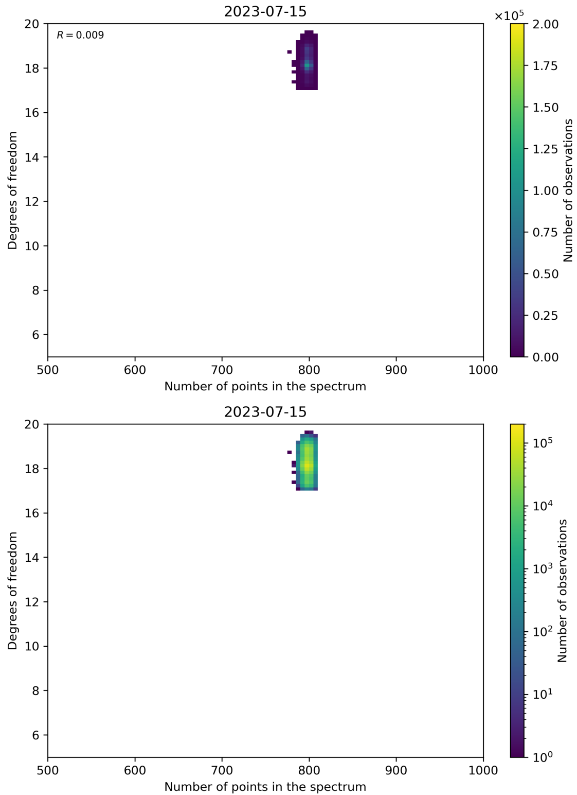
Figure 90: Scatter density plot of “Number of points in the spectrum” against “Degrees of freedom” for 2023-07-14 to 2023-07-16.
