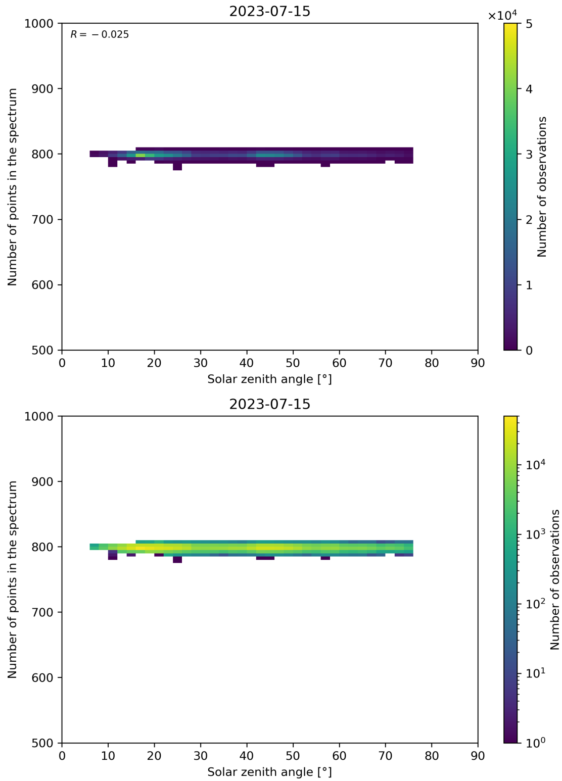
Figure 103: Scatter density plot of “Solar zenith angle” against “Number of points in the spectrum” for 2023-07-14 to 2023-07-16.
