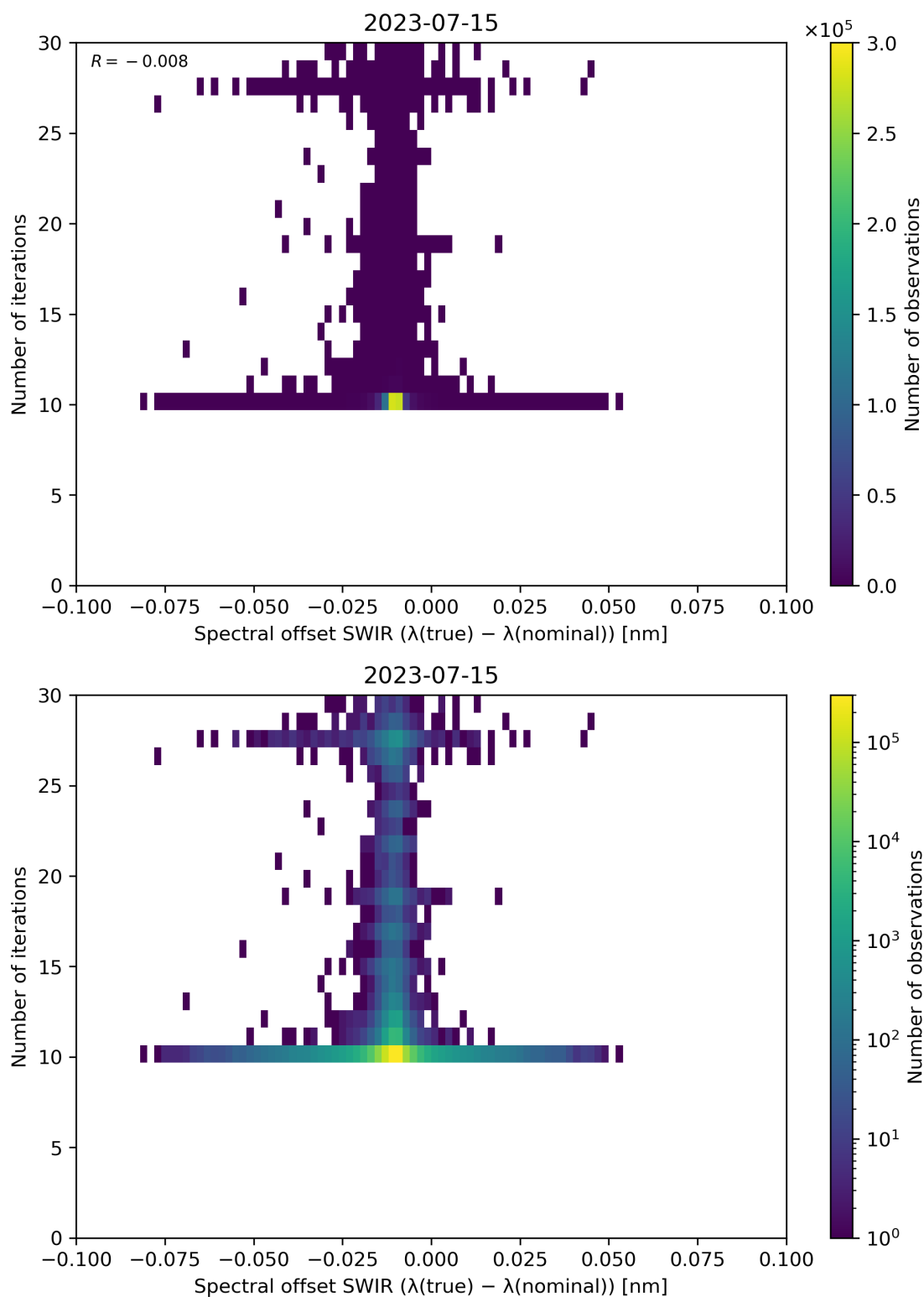
Figure 121: Scatter density plot of “Spectral offset SWIR ( \lambda(\text{true}) - \lambda(\text{nominal}) )” against “Number of iterations” for 2023-07-14 to 2023-07-16.
