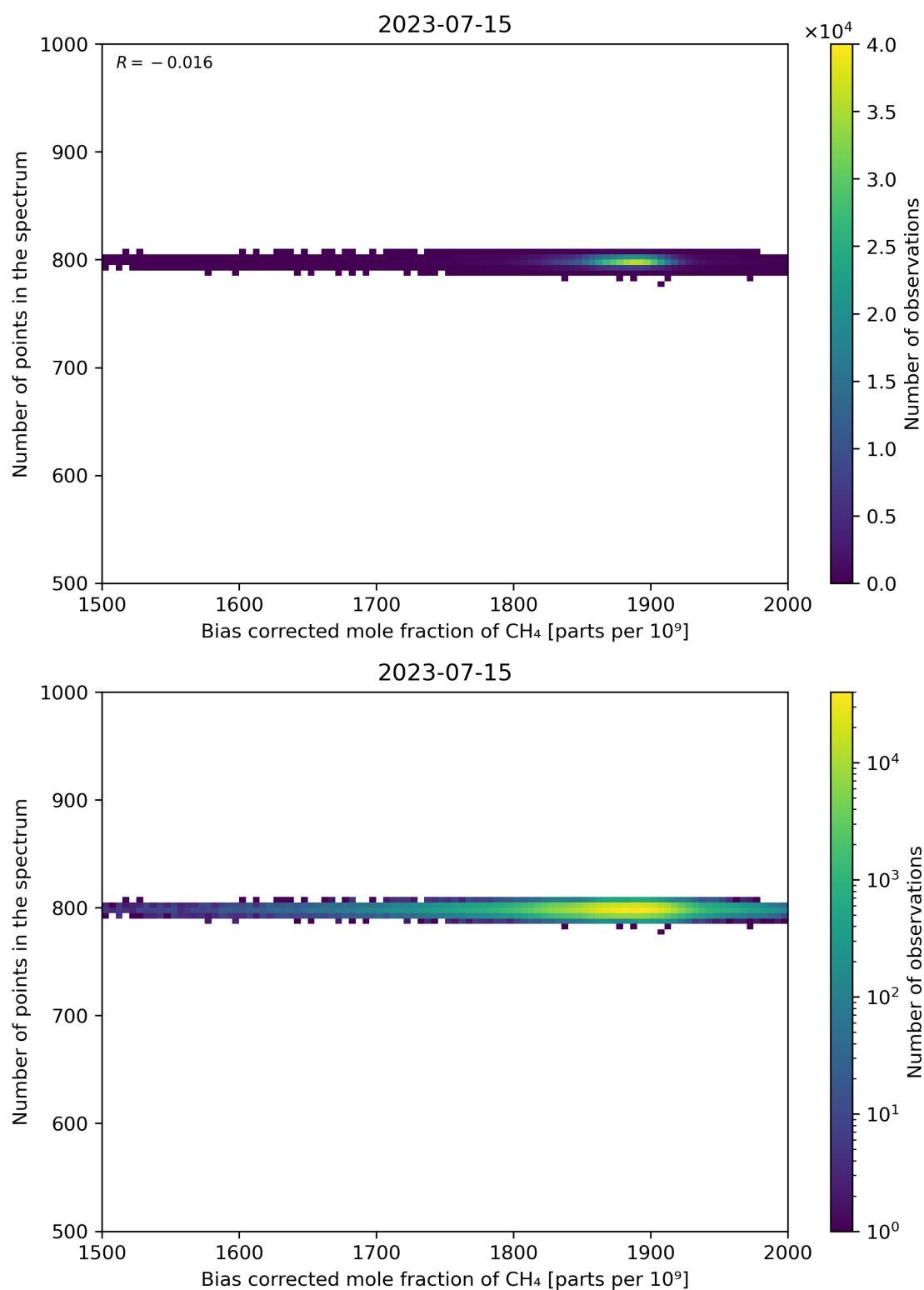
Figure 68: Scatter density plot of “Bias corrected mole fraction of CH 4 ” against “Number of points in the spectrum” for 2023-07-14 to 2023-07-16.
