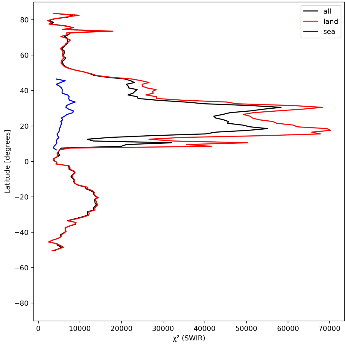
Figure 17: Zonal average of “ \chi^2 (SWIR)” for 2023-07-14 to 2023-07-16.
