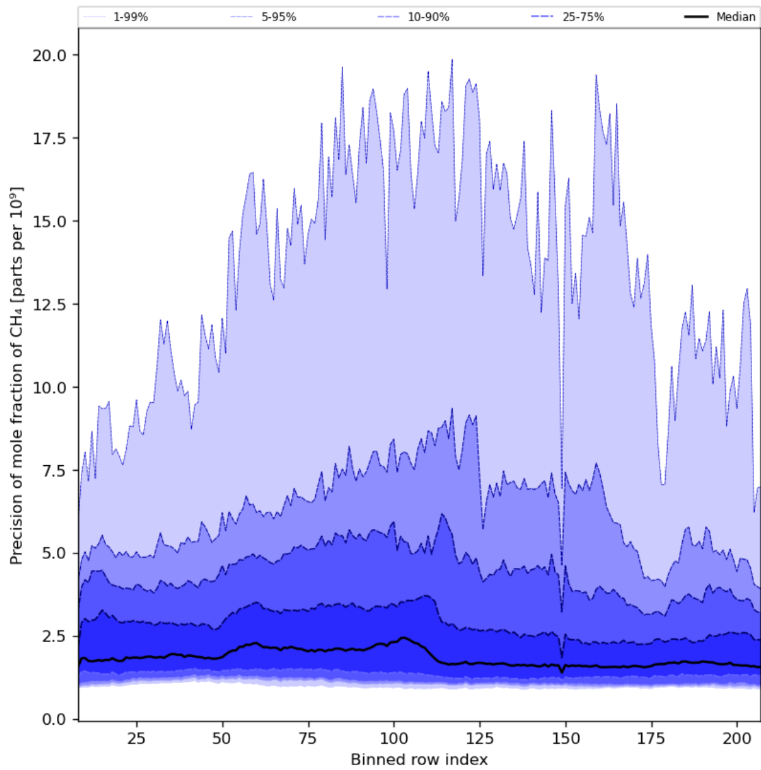
Figure 35: Along track statistics of “Precision of mole fraction of \text{CH}_4 ” for 2023-07-15 to 2023-07-17
