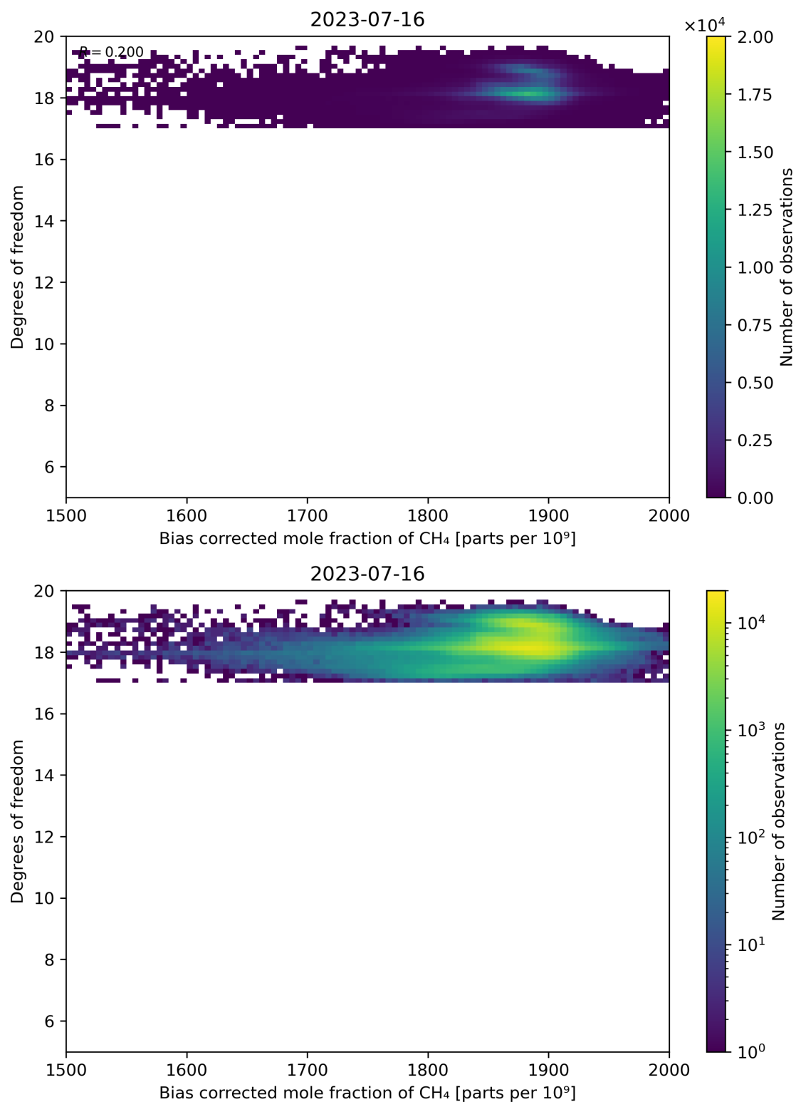
Figure 65: Scatter density plot of “Bias corrected mole fraction of CH 4 ” against “Degrees of freedom” for 2023-07-15 to 2023-07-17.
