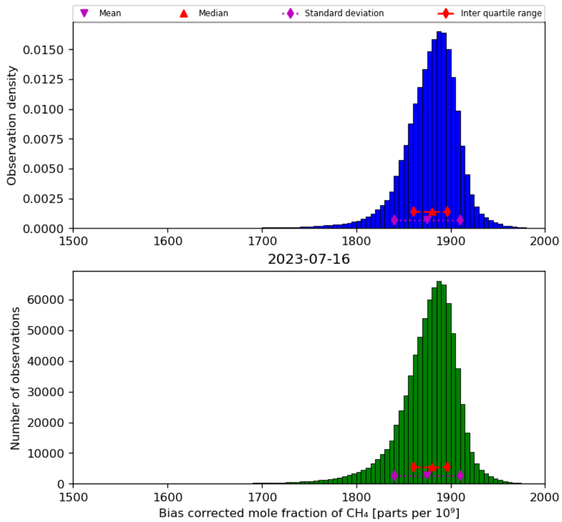
Figure 25: Histogram of “Bias corrected mole fraction of \text{CH}_4 ” for 2023-07-15 to 2023-07-17
