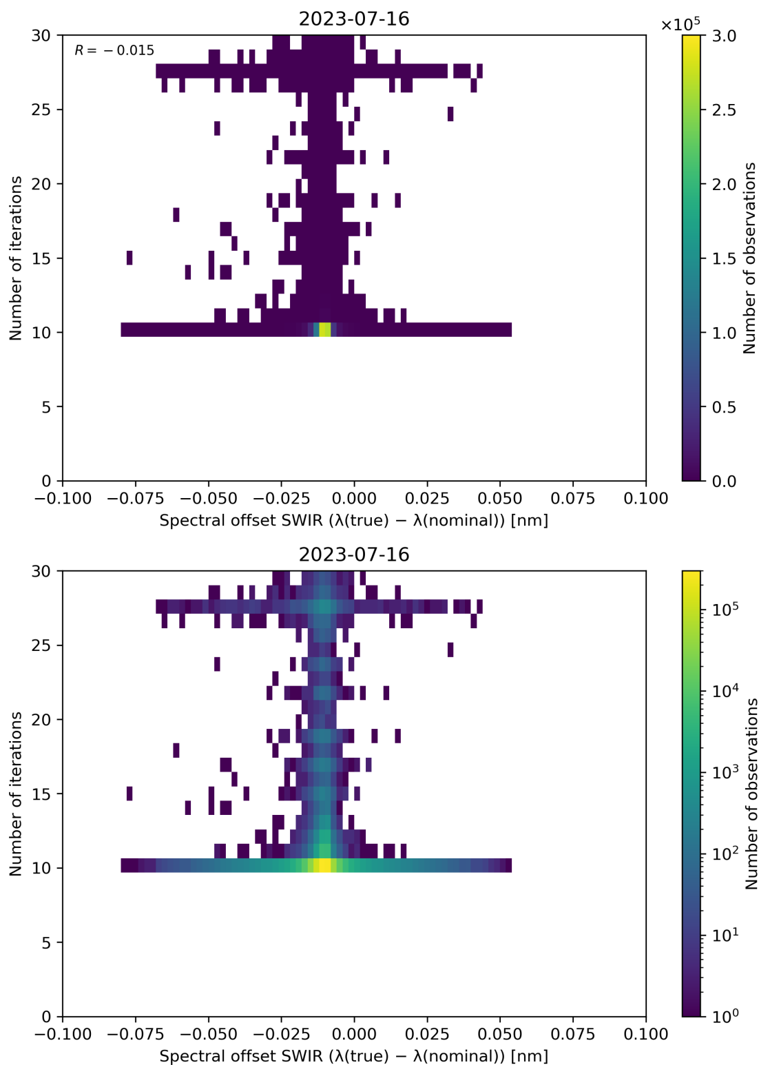
Figure 121: Scatter density plot of “Spectral offset SWIR ( \lambda(\text{true}) - \lambda(\text{nominal}) )” against “Number of iterations” for 2023-07-15 to 2023-07-17.
