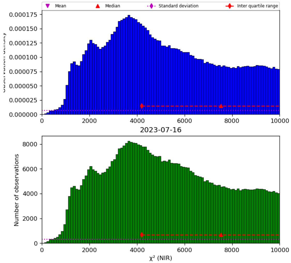
Figure 29: Histogram of “ \chi^2 (NIR)” for 2023-07-15 to 2023-07-17
