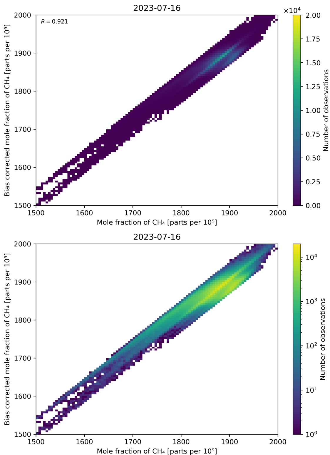
Figure 74: Scatter density plot of “Mole fraction of CH 4 ” against “Bias corrected mole fraction of CH 4 ” for 2023-07-15 to 2023-07-17.
