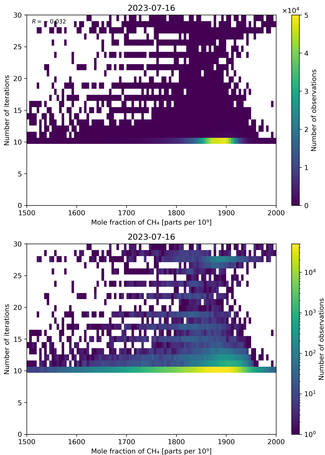
Figure 76: Scatter density plot of “Mole fraction of CH 4 ” against “Number of iterations” for 2023-07-15 to 2023-07-17.
