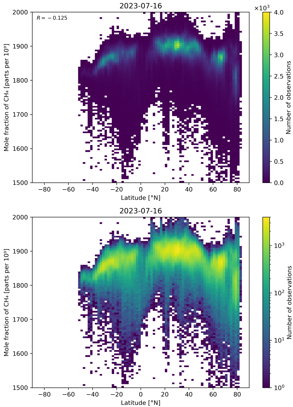
Figure 57: Scatter density plot of “Latitude” against “Mole fraction of CH 4 ” for 2023-07-15 to 2023-07-17.
