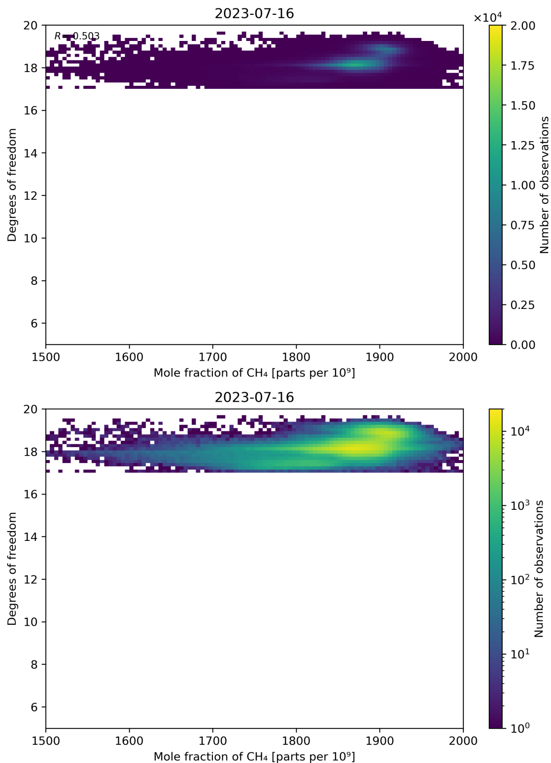
Figure 72: Scatter density plot of “Mole fraction of CH 4 ” against “Degrees of freedom” for 2023-07-15 to 2023-07-17.
