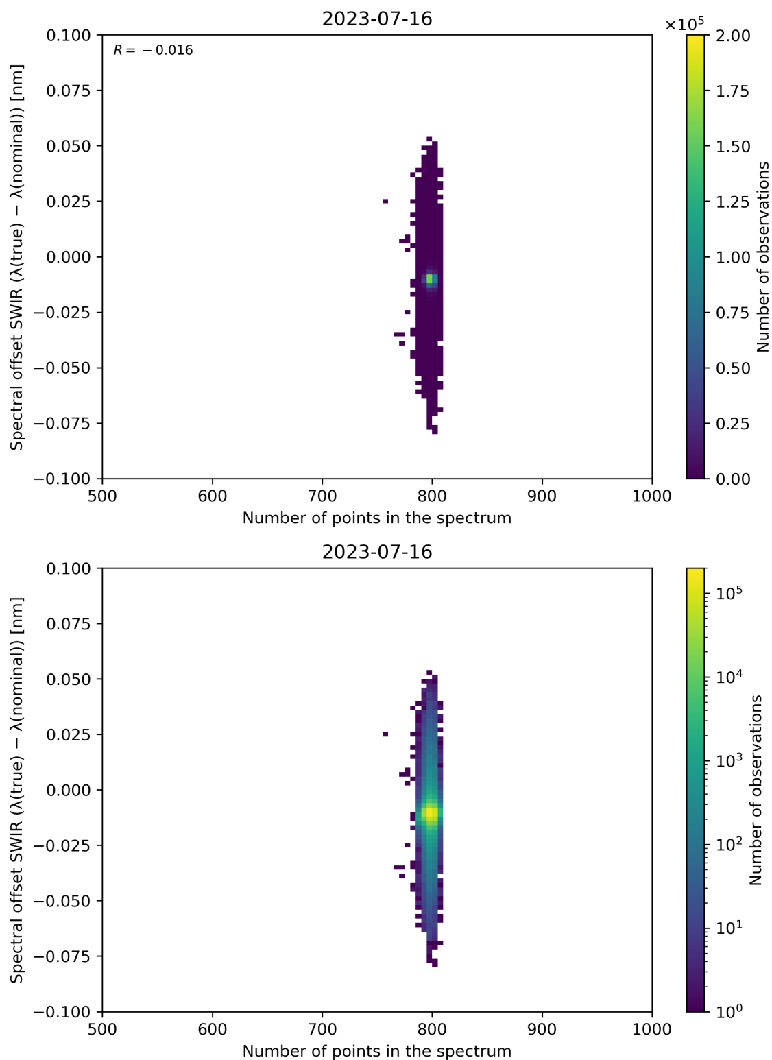
Figure 93: Scatter density plot of “Number of points in the spectrum” against “Spectral offset SWIR ( \lambda(\text{true}) - \lambda(\text{nominal}) )” for 2023-07-15 to 2023-07-17.
