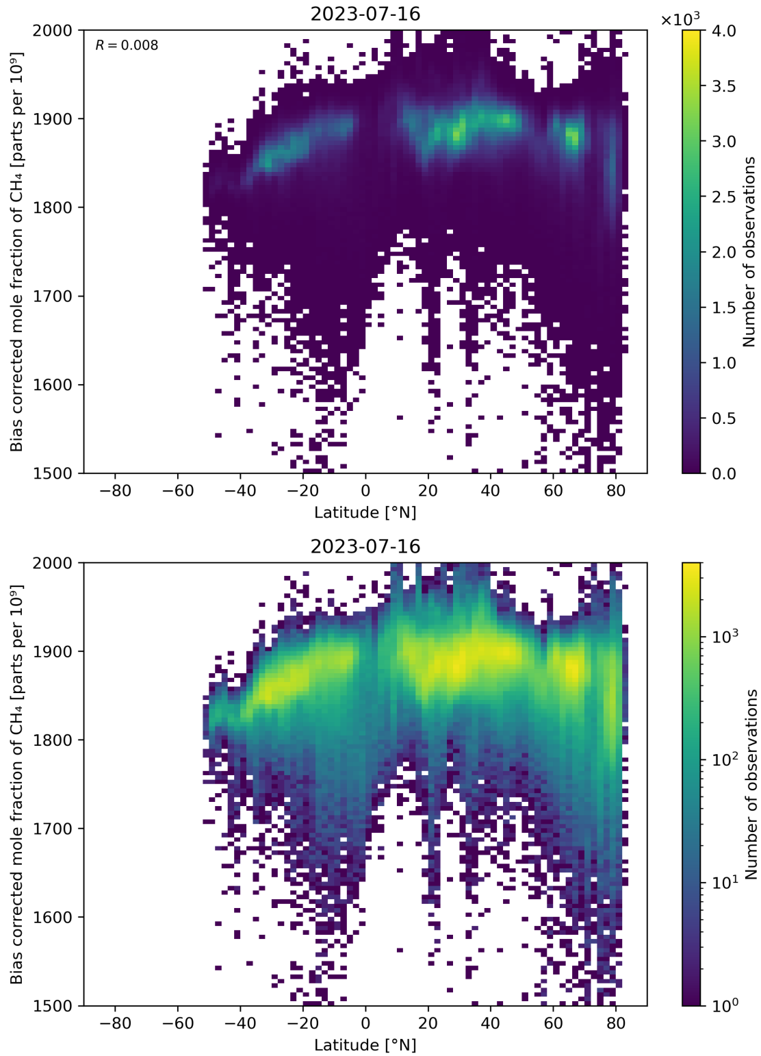
Figure 58: Scatter density plot of “Latitude” against “Bias corrected mole fraction of \text{CH}_4 ” for 2023-07-15 to 2023-07-17.
