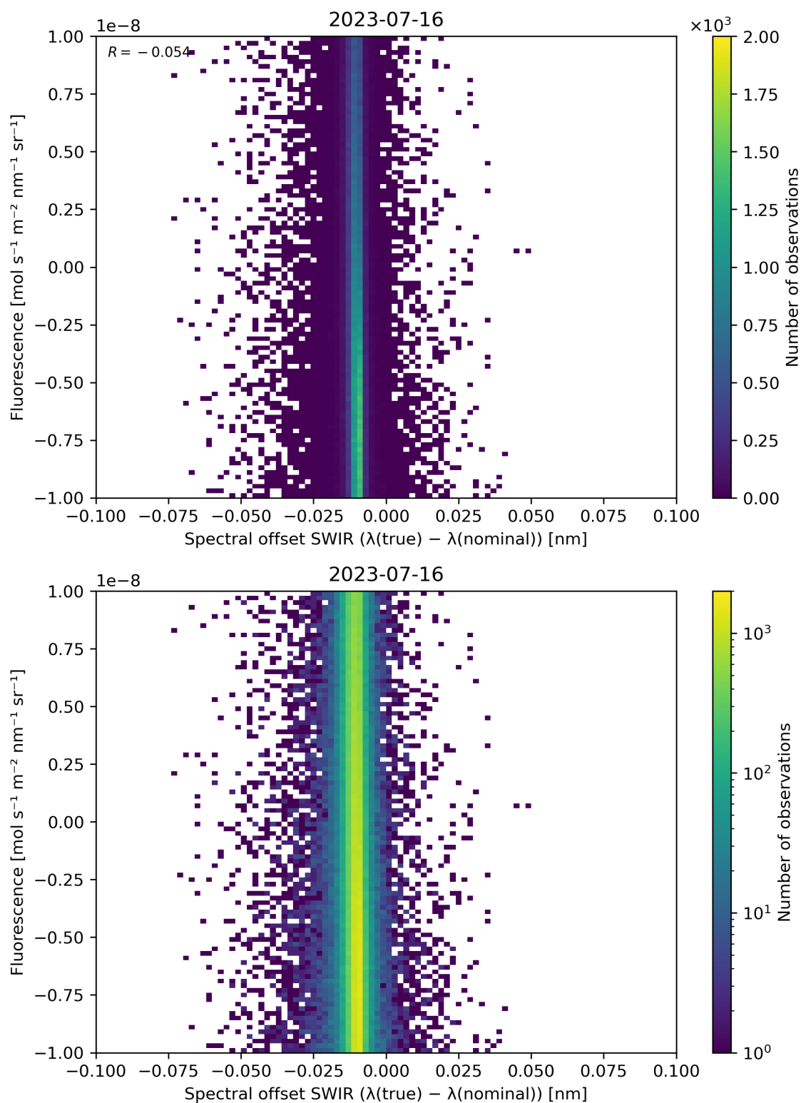
Figure 120: Scatter density plot of “Spectral offset SWIR ( \lambda(\text{true}) - \lambda(\text{nominal}) )” against “Fluorescence” for 2023-07-15 to 2023-07-17.
