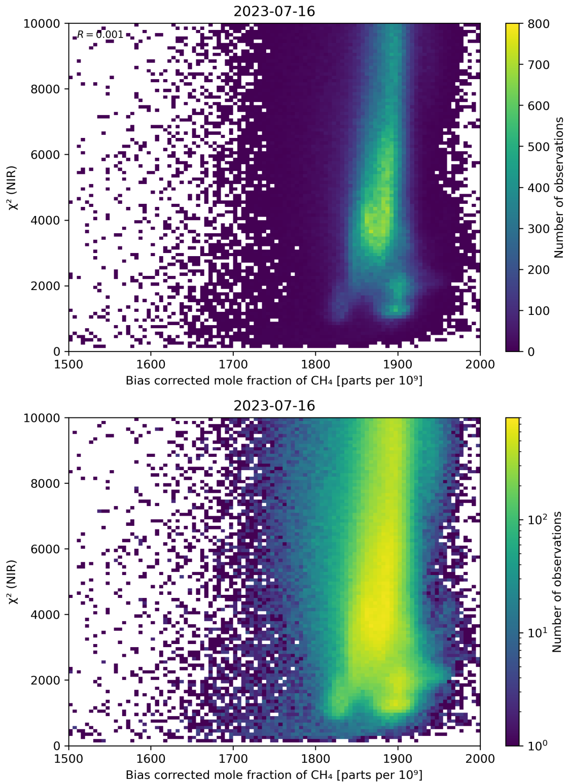
Figure 63: Scatter density plot of “Bias corrected mole fraction of CH 4 ” against “ \chi^2 (NIR)” for 2023-07-15 to 2023-07-17.
