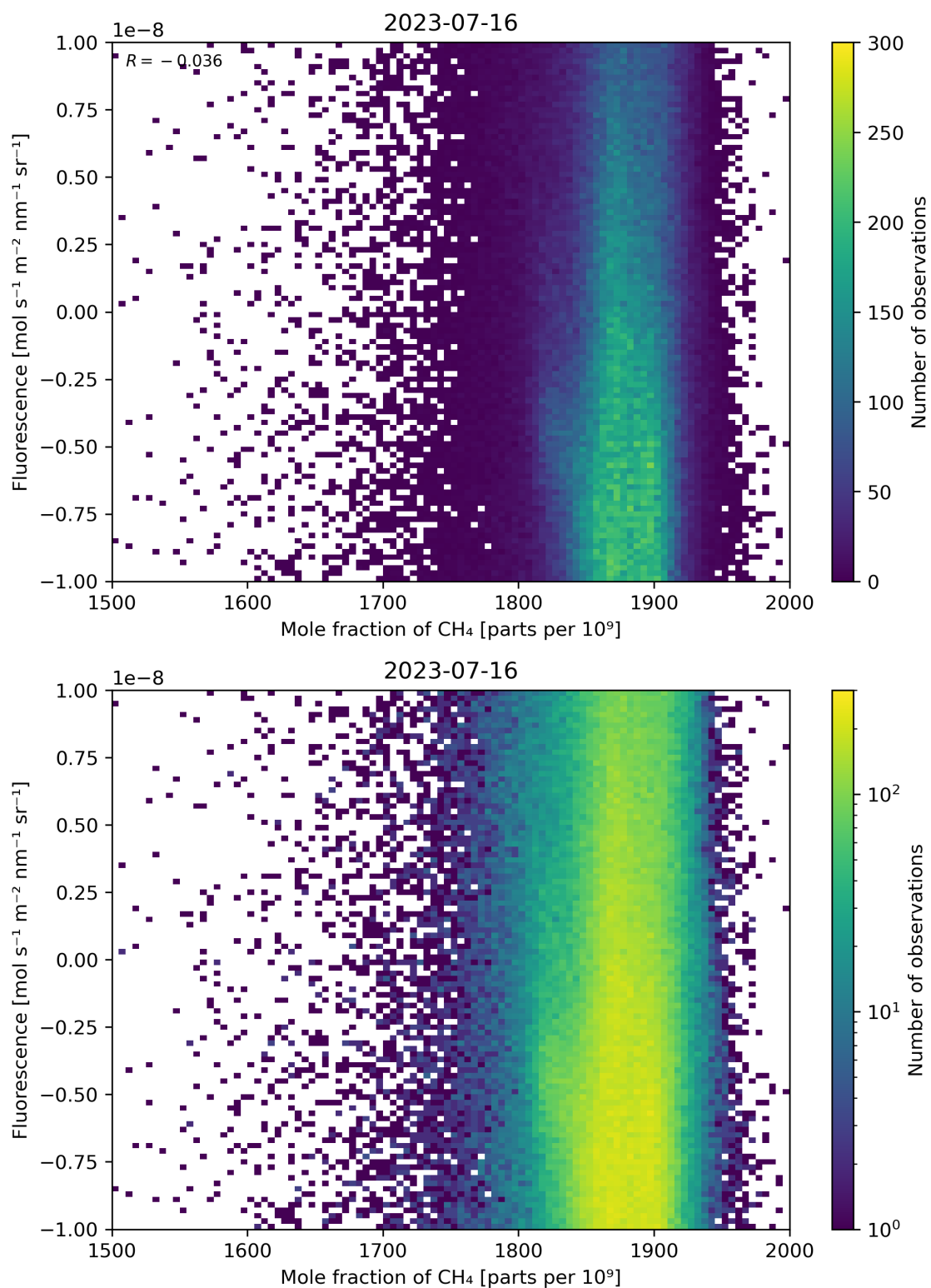
Figure 73: Scatter density plot of “Mole fraction of \text{CH}_4 ” against “Fluorescence” for 2023-07-15 to 2023-07-17.
