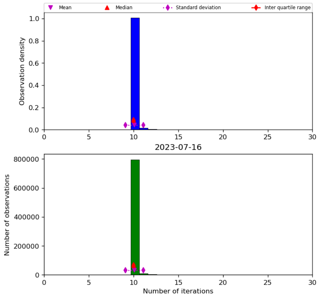
Figure 31: Histogram of “Number of iterations” for 2023-07-15 to 2023-07-17
