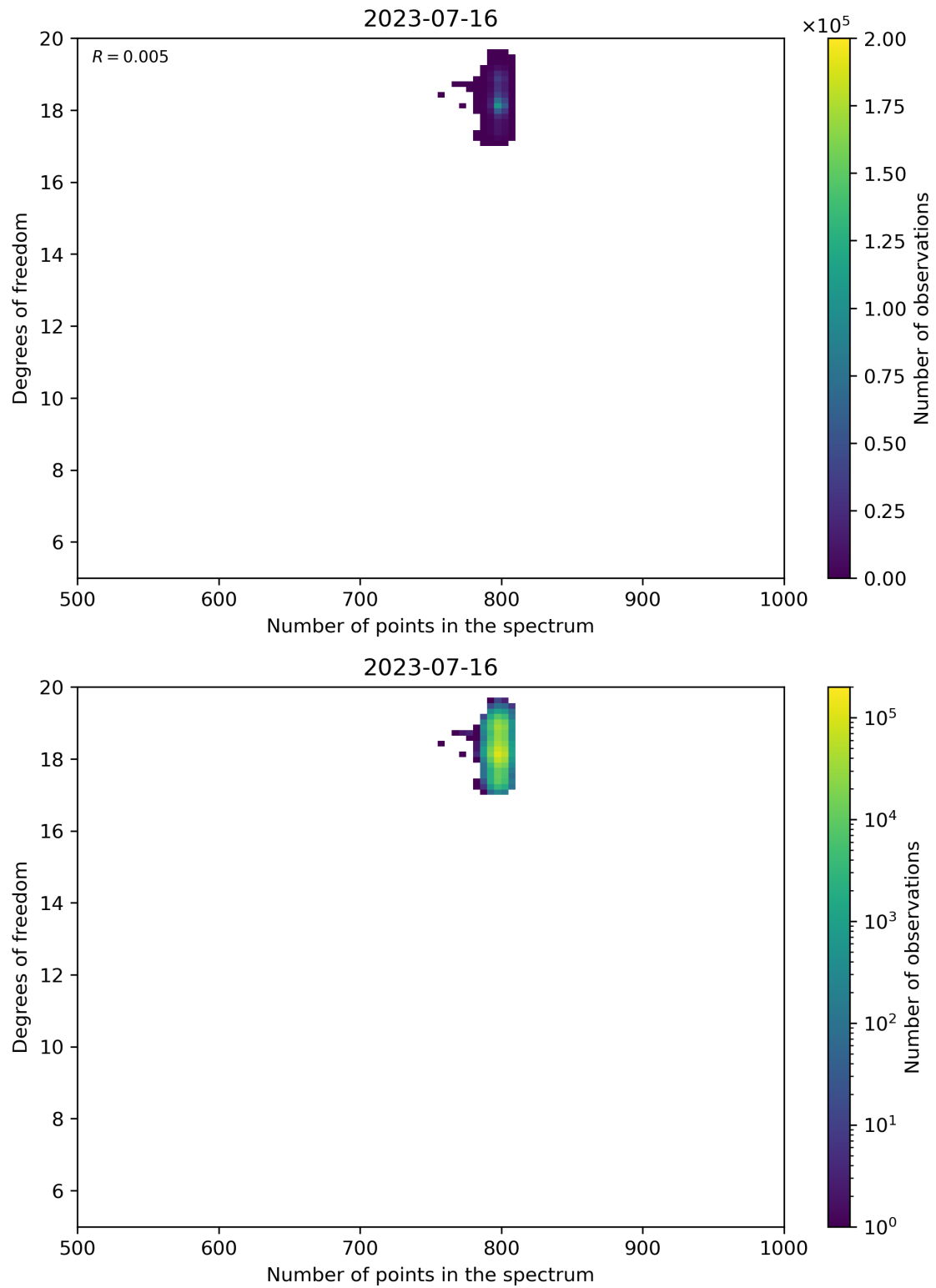
Figure 90: Scatter density plot of “Number of points in the spectrum” against “Degrees of freedom” for 2023-07-15 to 2023-07-17.
