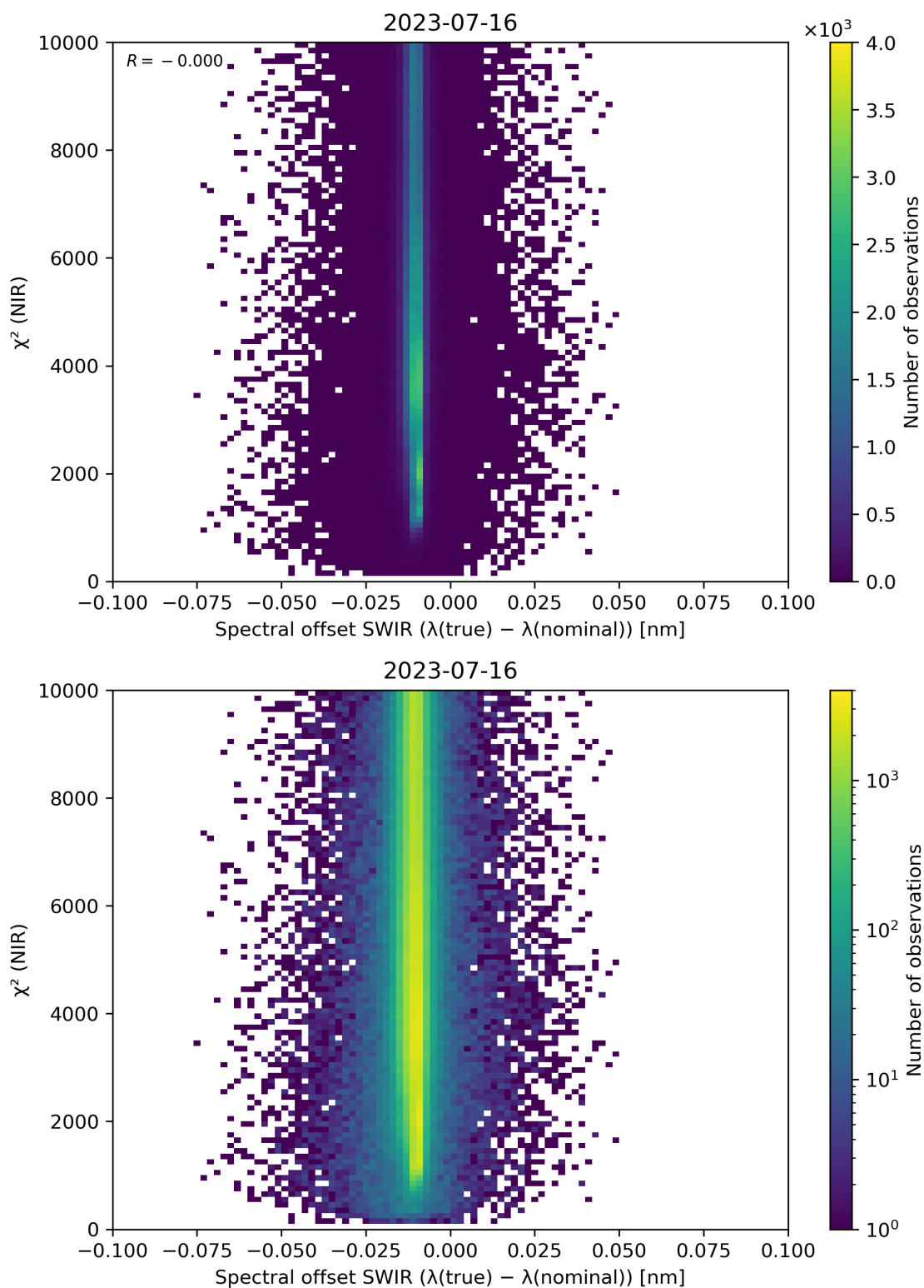
Figure 117: Scatter density plot of “Spectral offset SWIR ( \lambda(\text{true}) - \lambda(\text{nominal}) )” against “ \chi^2 (NIR)” for 2023-07-15 to 2023-07-17.
