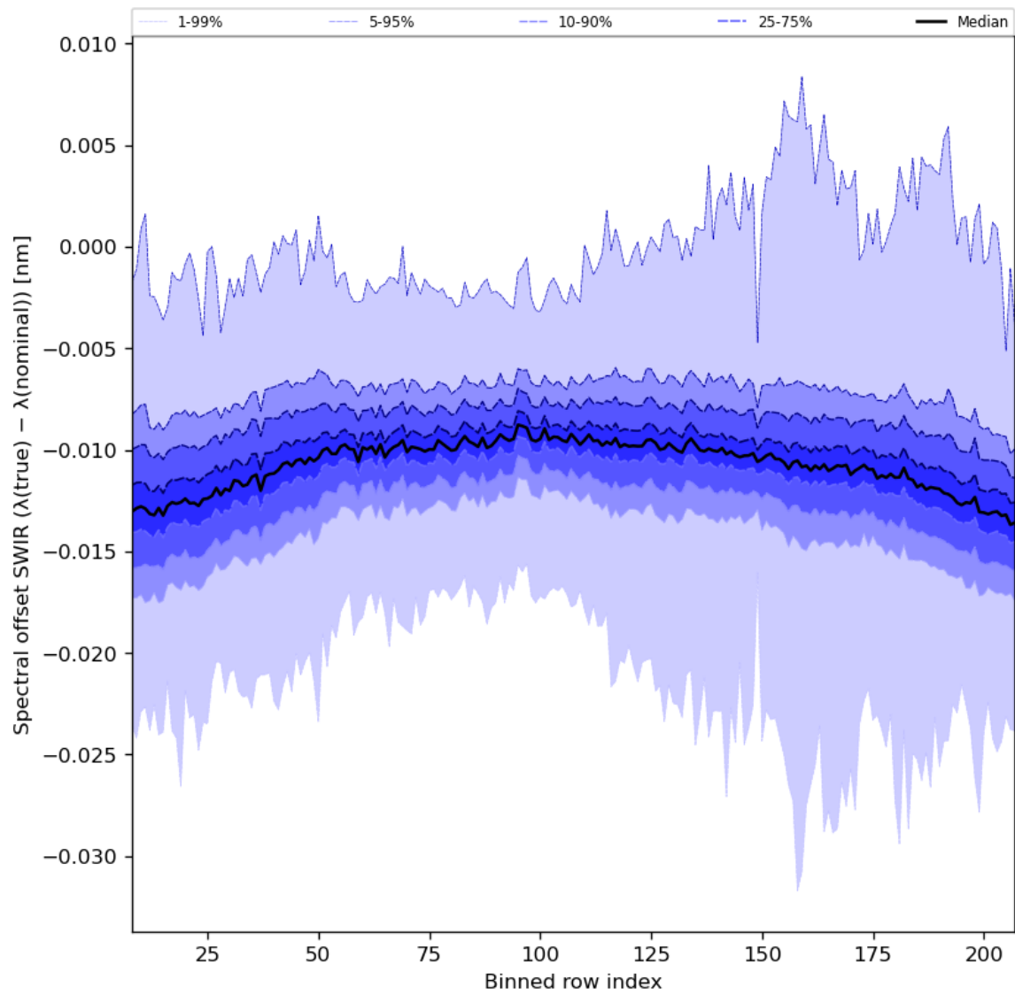
Figure 38: Along track statistics of “Spectral offset SWIR ( \lambda(\text{true}) - \lambda(\text{nominal}) )” for 2023-07-15 to 2023-07-17
