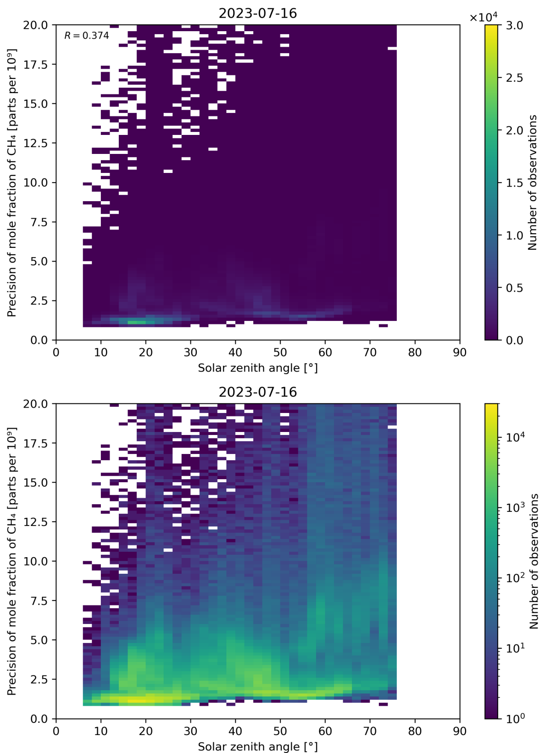
Figure 101: Scatter density plot of “Solar zenith angle” against “Precision of mole fraction of CH 4 ” for 2023-07-15 to 2023-07-17.
