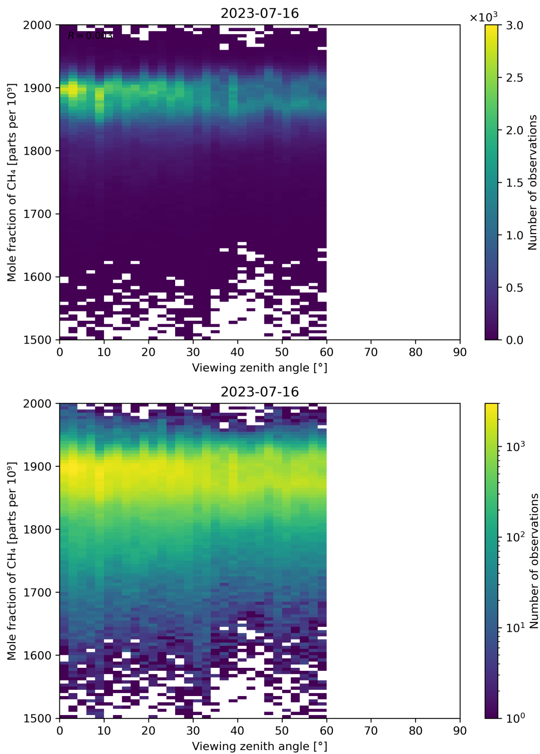
Figure 110: Scatter density plot of “Viewing zenith angle” against “Mole fraction of CH 4 ” for 2023-07-15 to 2023-07-17.
