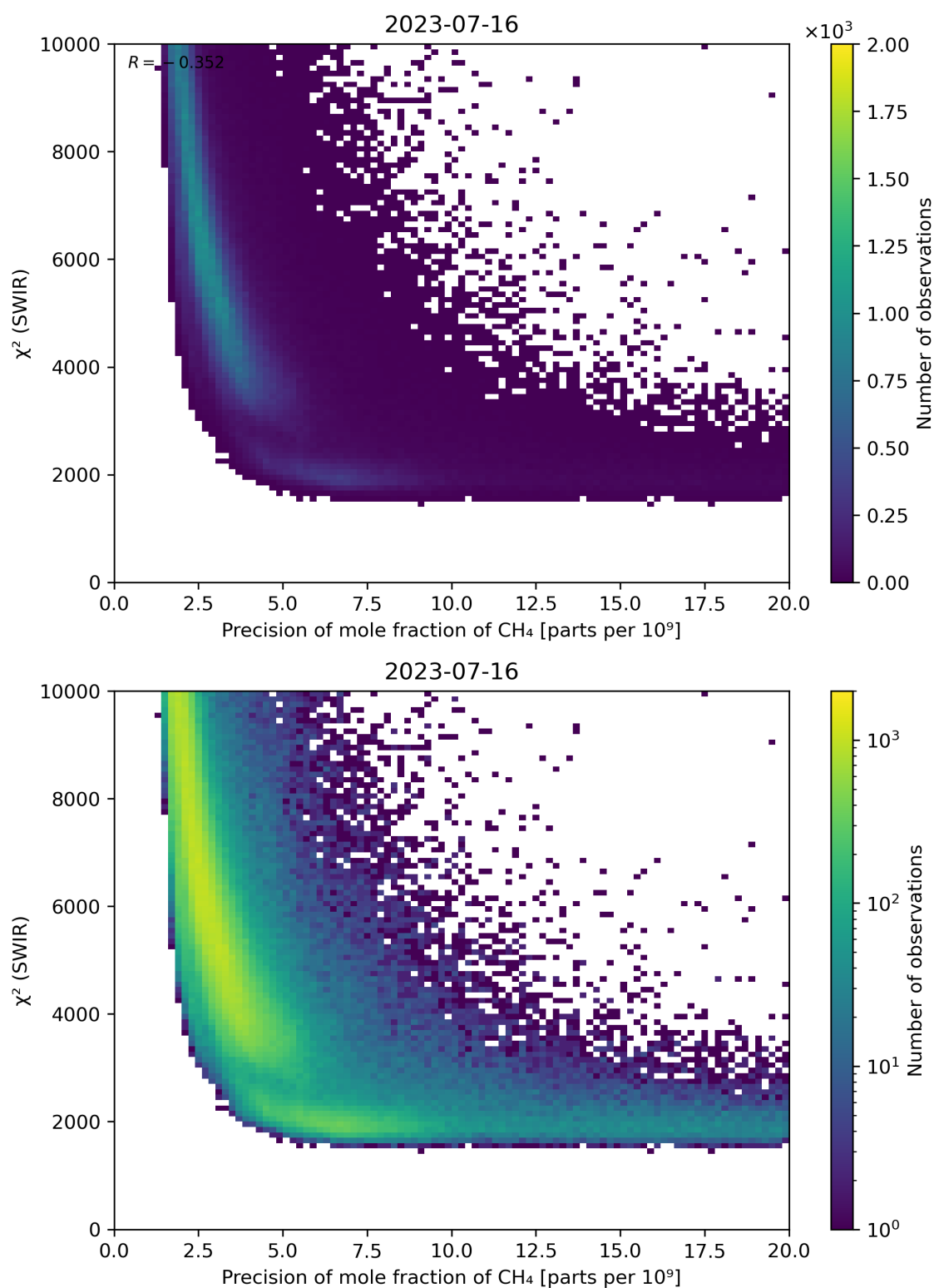
Figure 79: Scatter density plot of “Precision of mole fraction of CH 4 ” against “ \chi^2 (SWIR)” for 2023-07-15 to 2023-07-17.
