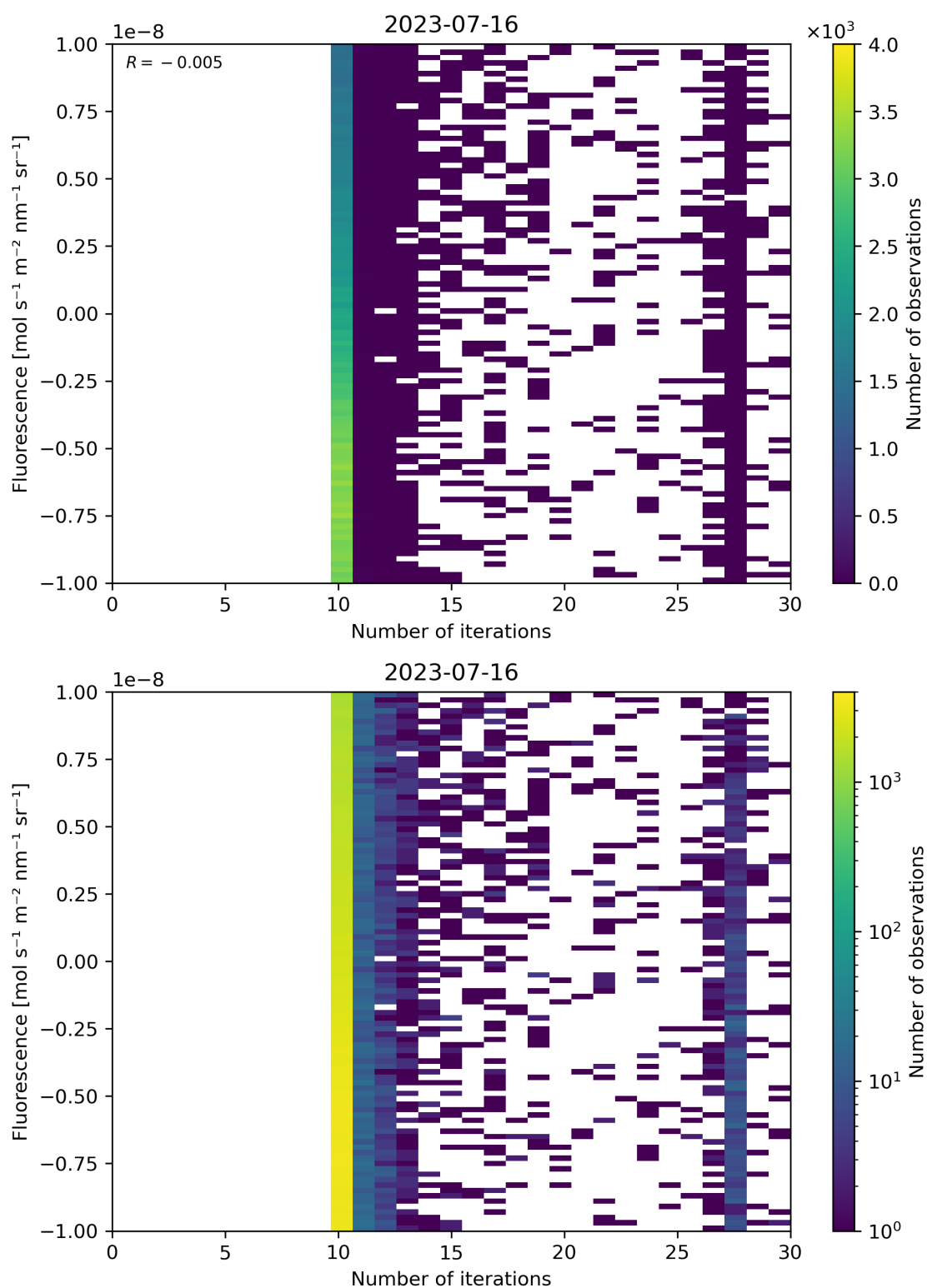
Figure 87: Scatter density plot of “Number of iterations” against “Fluorescence” for 2023-07-15 to 2023-07-17.
