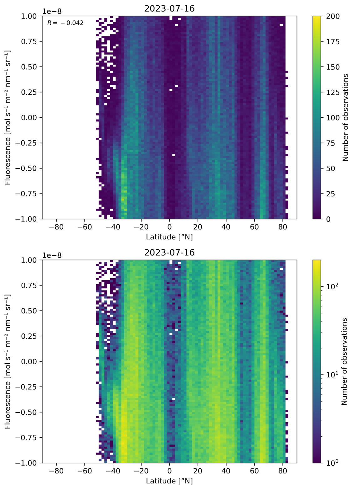
Figure 56: Scatter density plot of “Latitude” against “Fluorescence” for 2023-07-15 to 2023-07-17.
