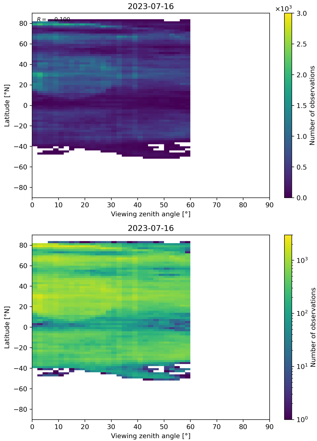
Figure 109: Scatter density plot of “Viewing zenith angle” against “Latitude” for 2023-07-15 to 2023-07-17.
