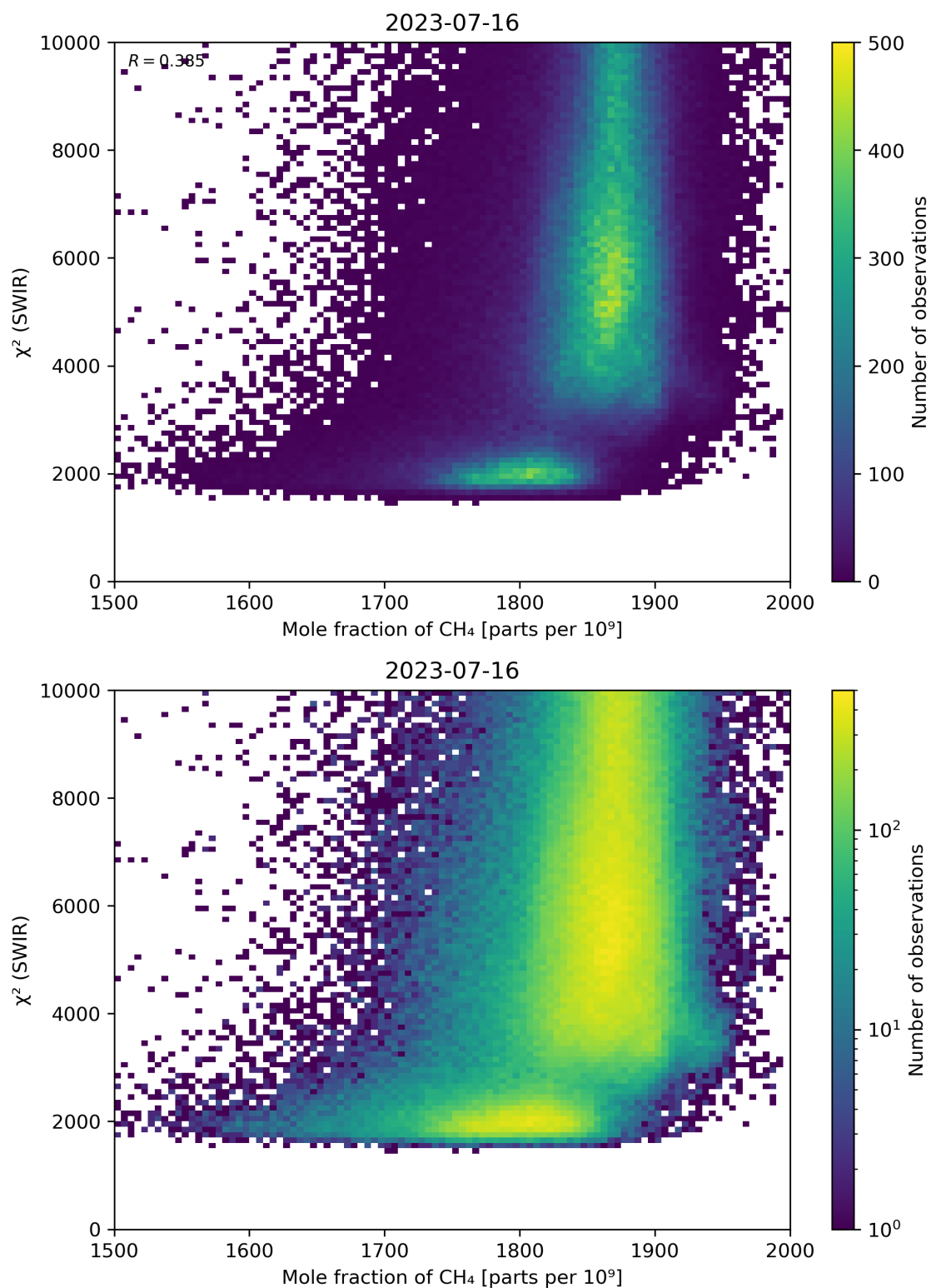
Figure 71: Scatter density plot of “Mole fraction of \text{CH}_4 ” against “ \chi^2 (SWIR)” for 2023-07-15 to 2023-07-17.
