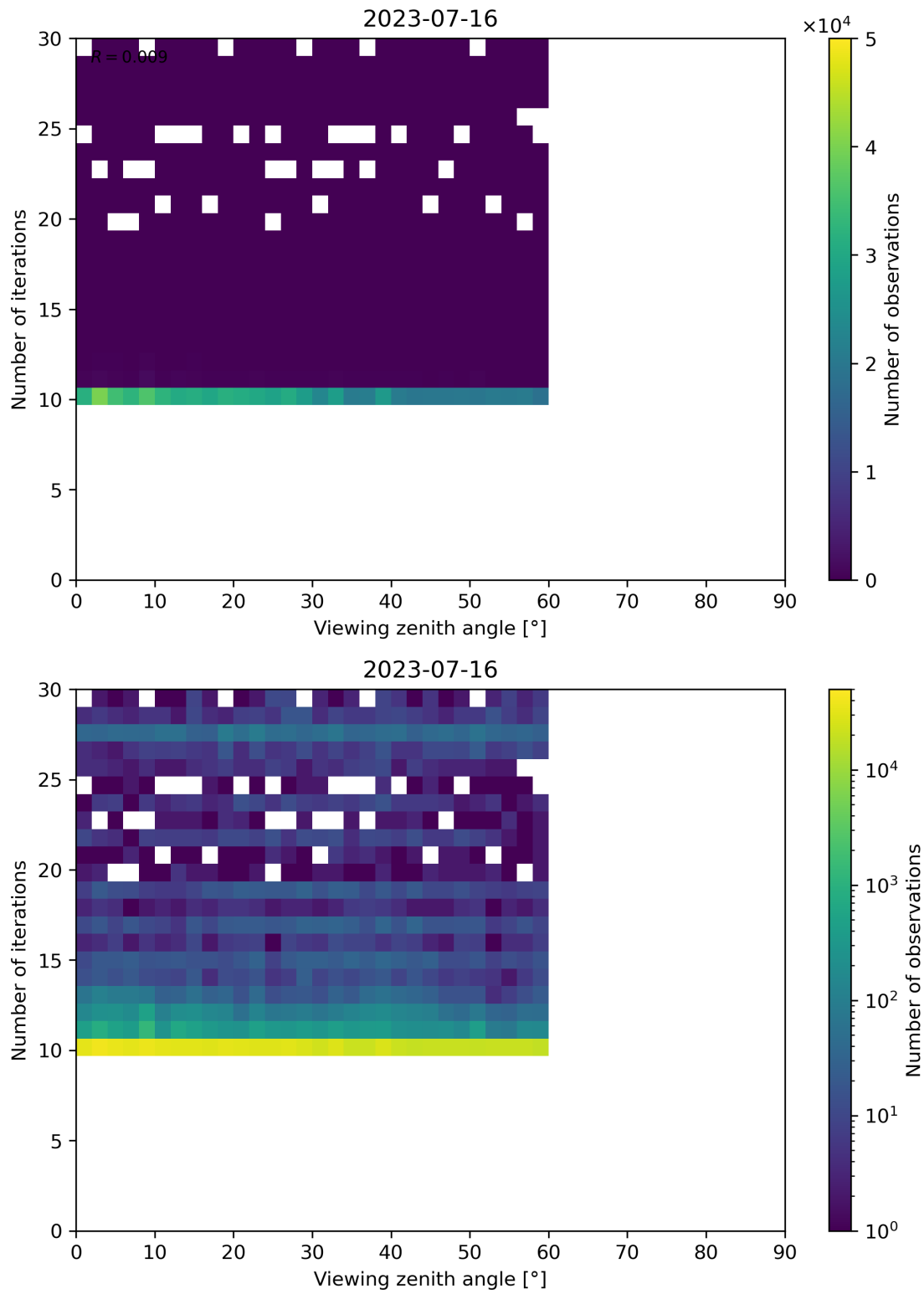
Figure 113: Scatter density plot of “Viewing zenith angle” against “Number of iterations” for 2023-07-15 to 2023-07-17.
