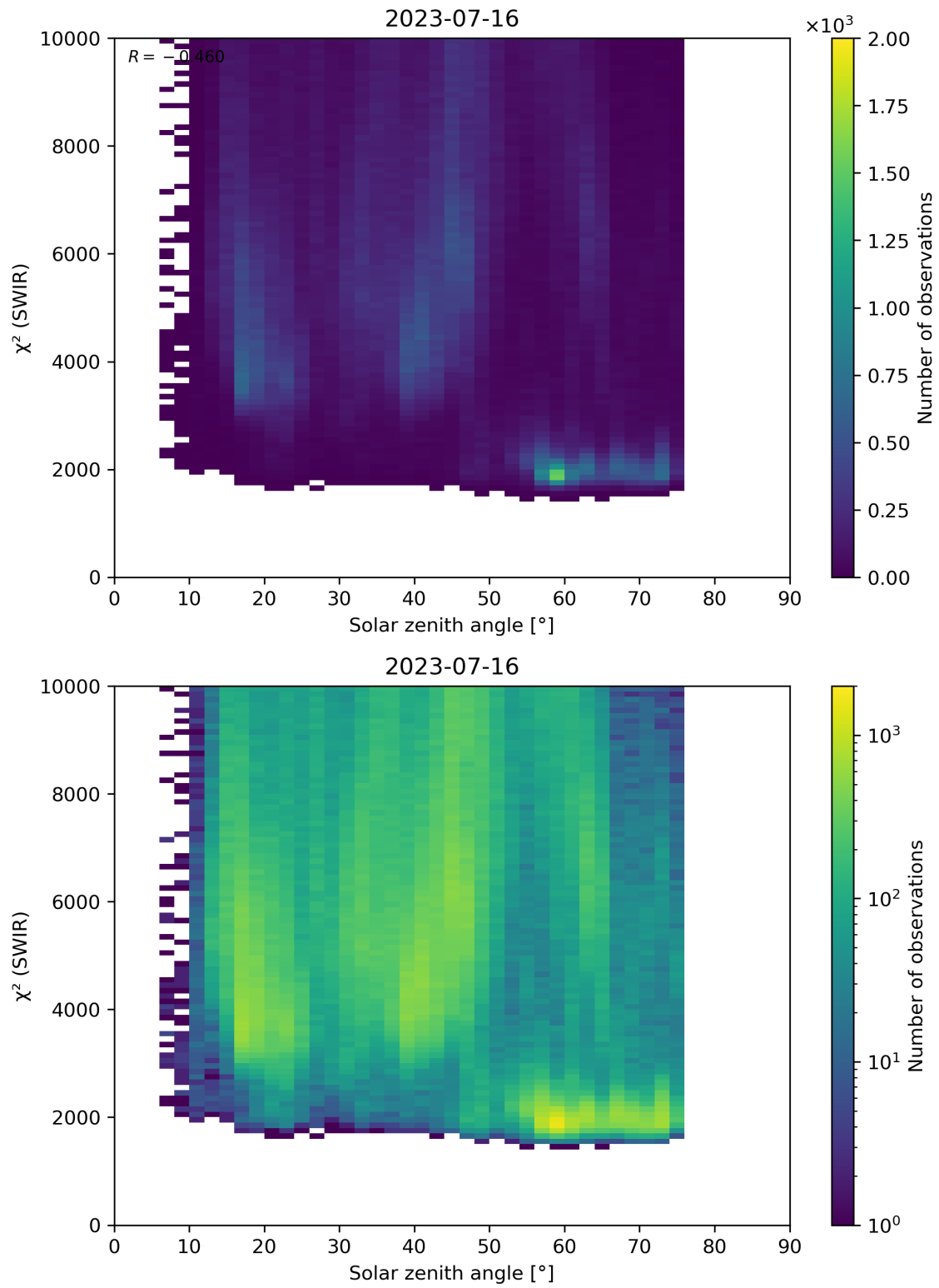
Figure 95: Scatter density plot of “Solar zenith angle” against “ \chi^2 (SWIR)” for 2023-07-15 to 2023-07-17.
