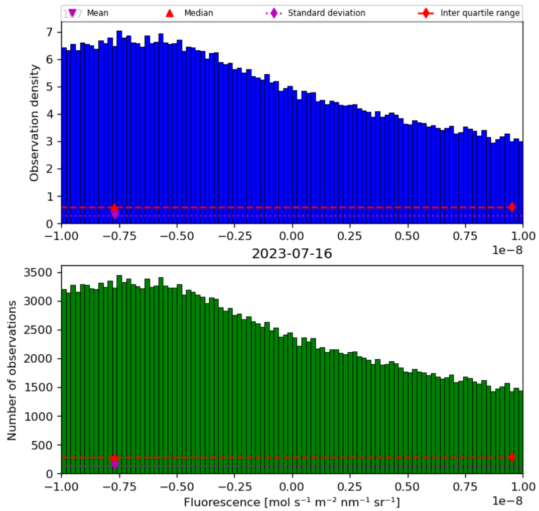
Figure 32: Histogram of “Fluorescence” for 2023-07-15 to 2023-07-17
