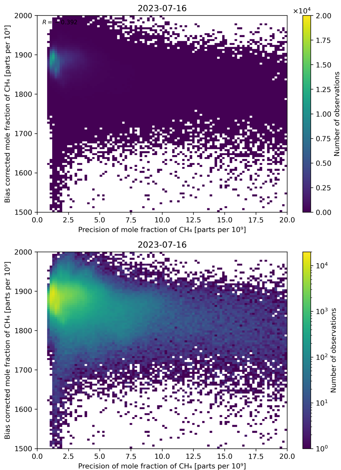
Figure 82: Scatter density plot of “Precision of mole fraction of \text{CH}_4 ” against “Bias corrected mole fraction of \text{CH}_4 ” for 2023-07-15 to 2023-07-17.
