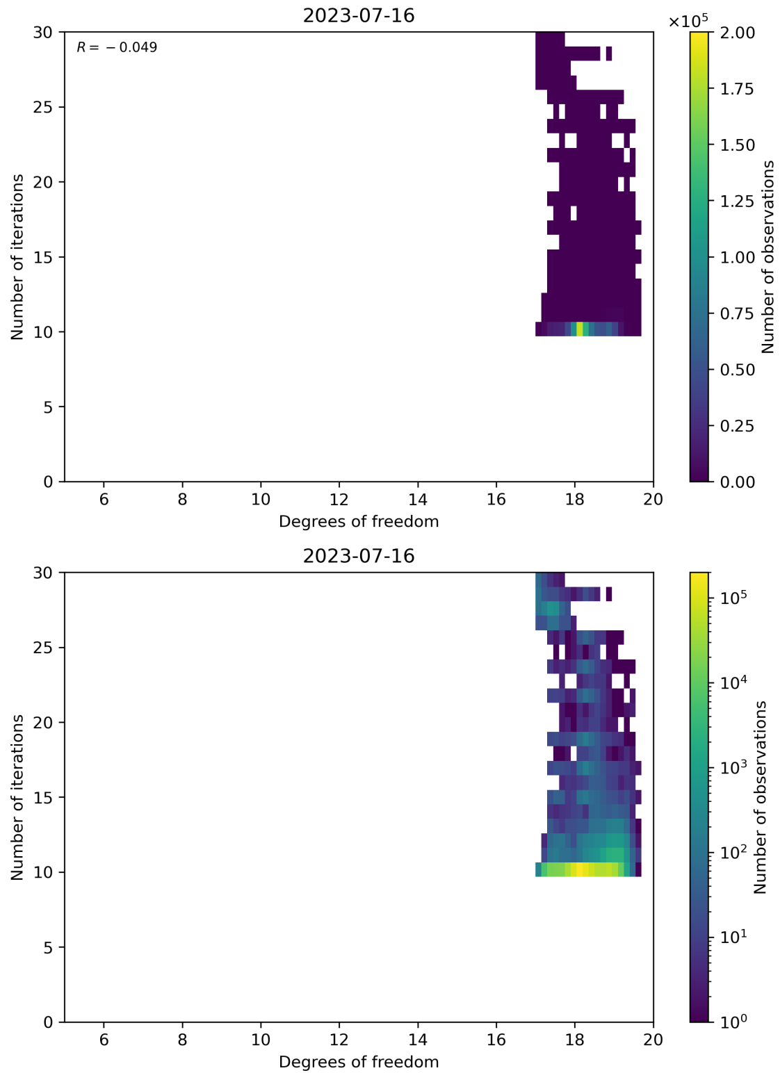
Figure 52: Scatter density plot of “Degrees of freedom” against “Number of iterations” for 2023-07-15 to 2023-07-17.
