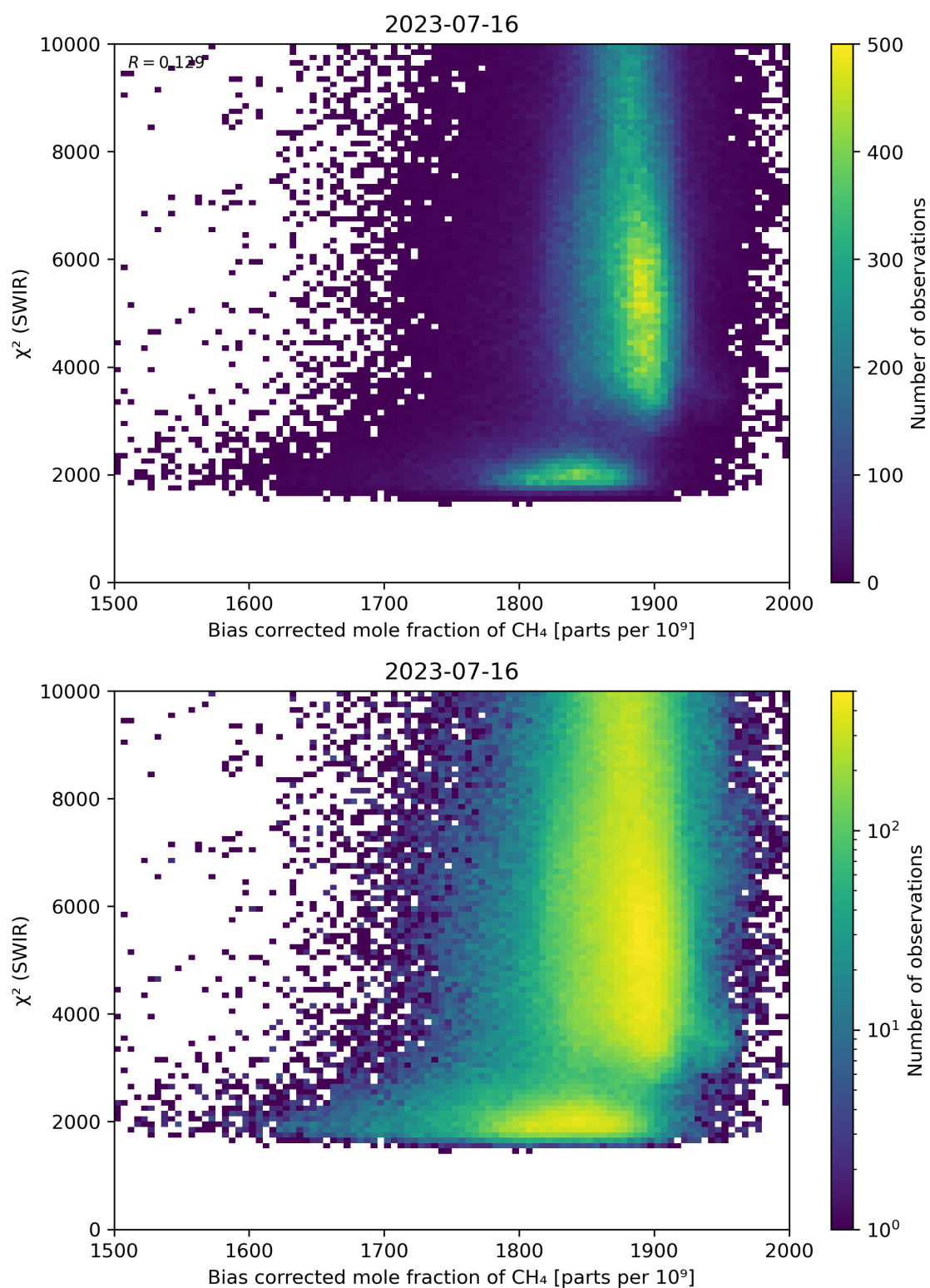
Figure 64: Scatter density plot of “Bias corrected mole fraction of CH 4 ” against “ \chi^2 (SWIR)” for 2023-07-15 to 2023-07-17.
