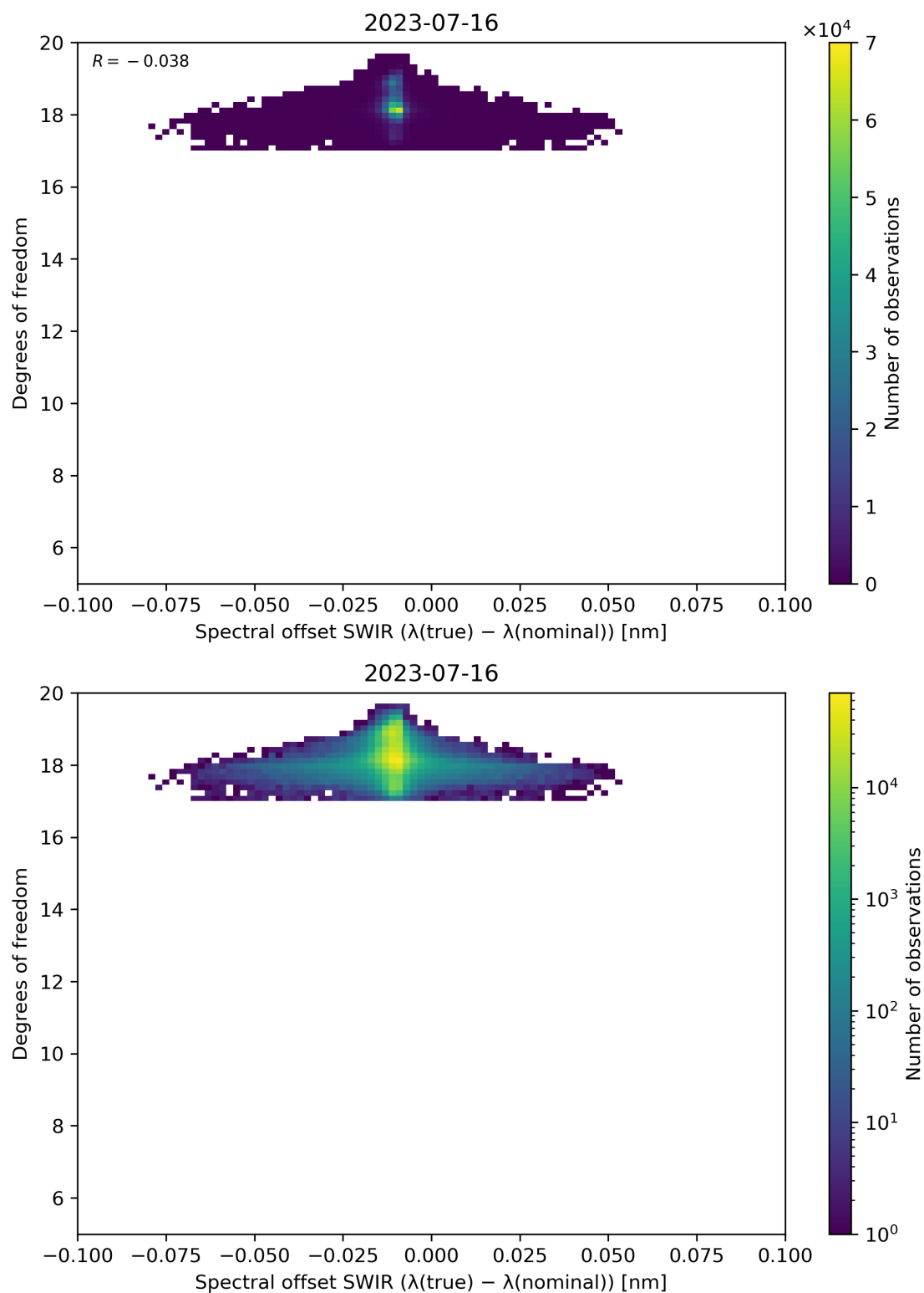
Figure 119: Scatter density plot of “Spectral offset SWIR ( \lambda(\text{true}) - \lambda(\text{nominal}) )” against “Degrees of freedom” for 2023-07-15 to 2023-07-17.
