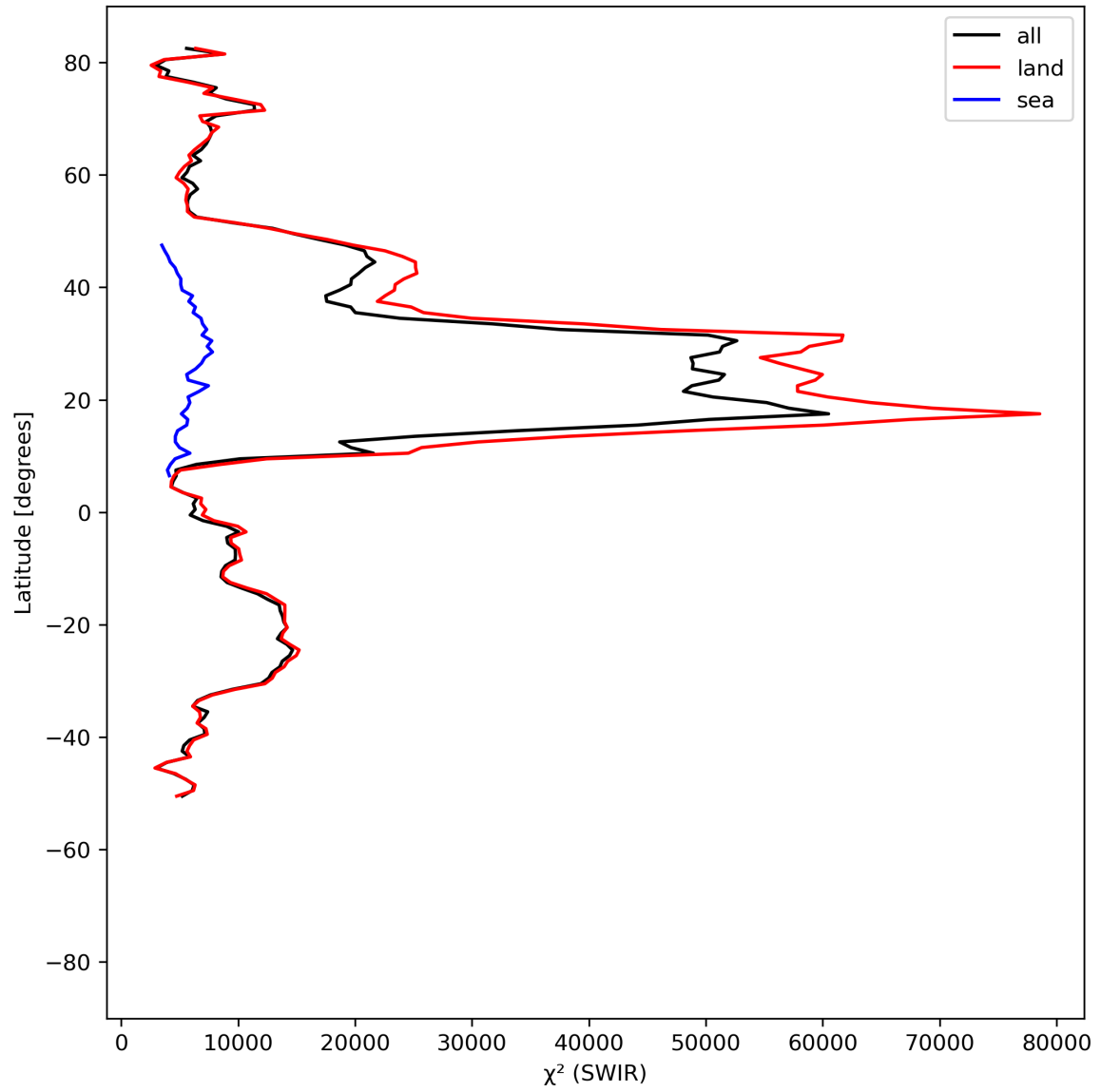
Figure 17: Zonal average of “ \chi^2 (SWIR)” for 2023-07-15 to 2023-07-17.
