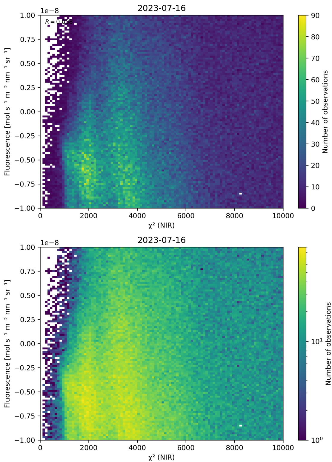
Figure 45: Scatter density plot of “ \chi^2 (NIR)” against “Fluorescence” for 2023-07-15 to 2023-07-17.
