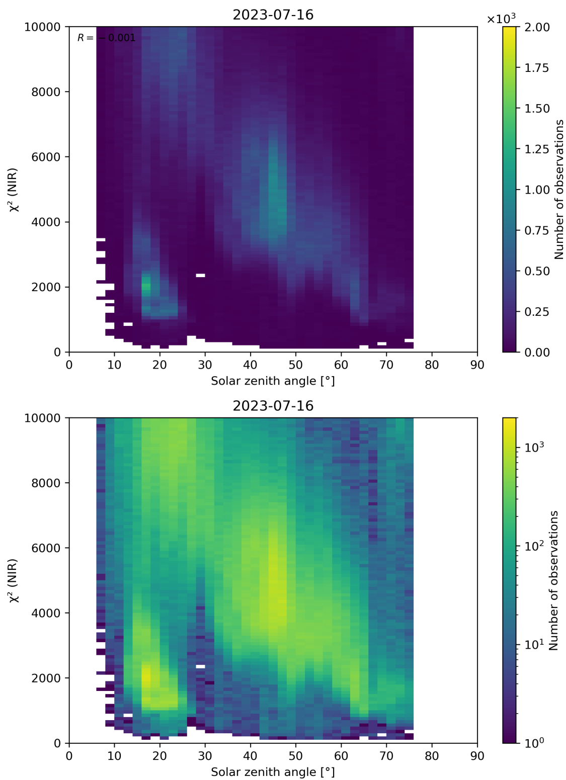
Figure 94: Scatter density plot of “Solar zenith angle” against “ \chi^2 (NIR)” for 2023-07-15 to 2023-07-17.
