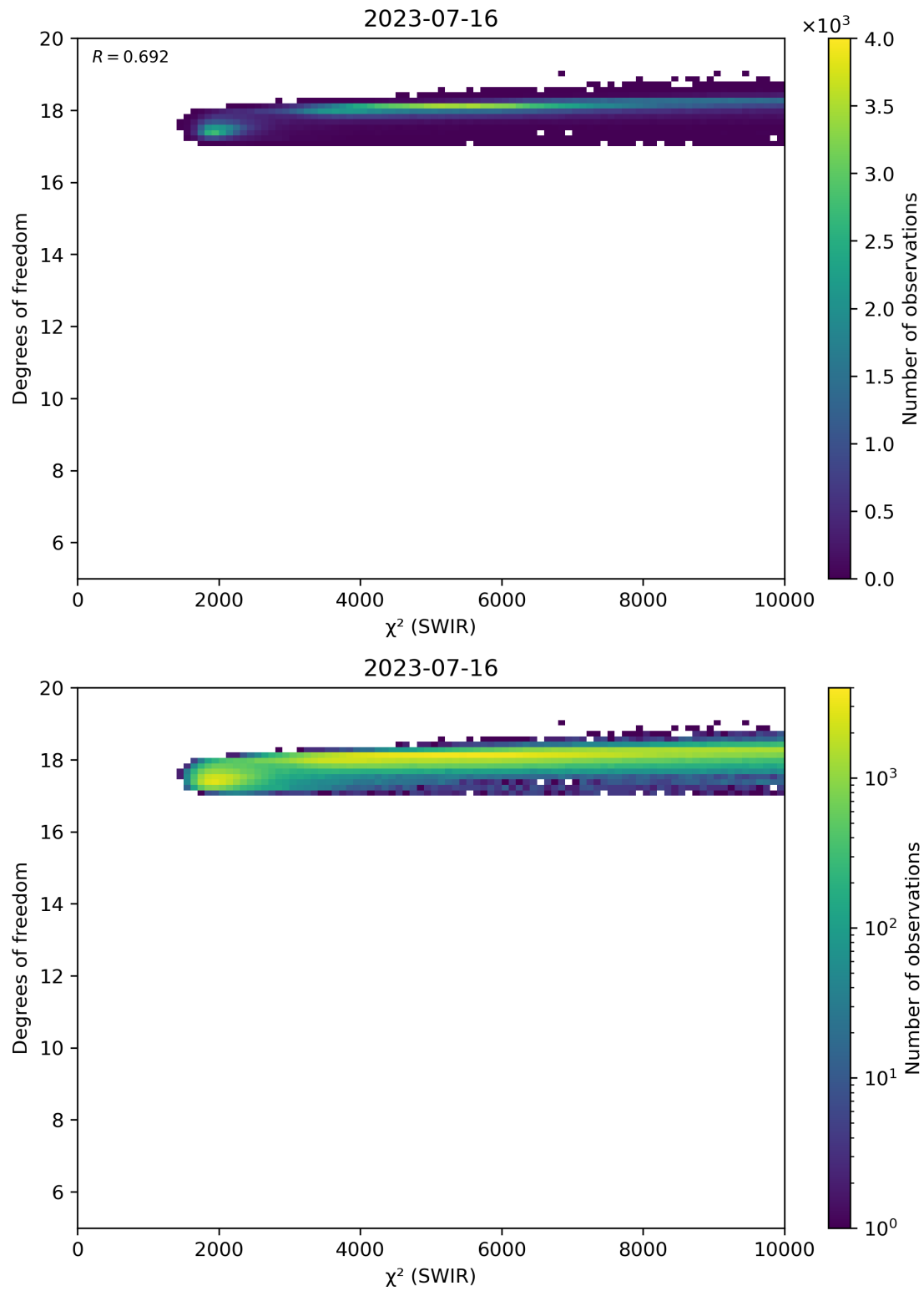
Figure 48: Scatter density plot of “ \chi^2 (SWIR)” against “Degrees of freedom” for 2023-07-15 to 2023-07-17.
