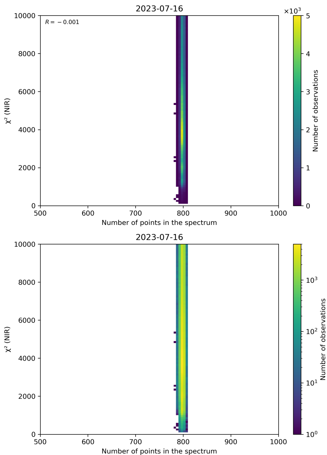
Figure 88: Scatter density plot of “Number of points in the spectrum” against “ \chi^2 (NIR)” for 2023-07-15 to 2023-07-17.
