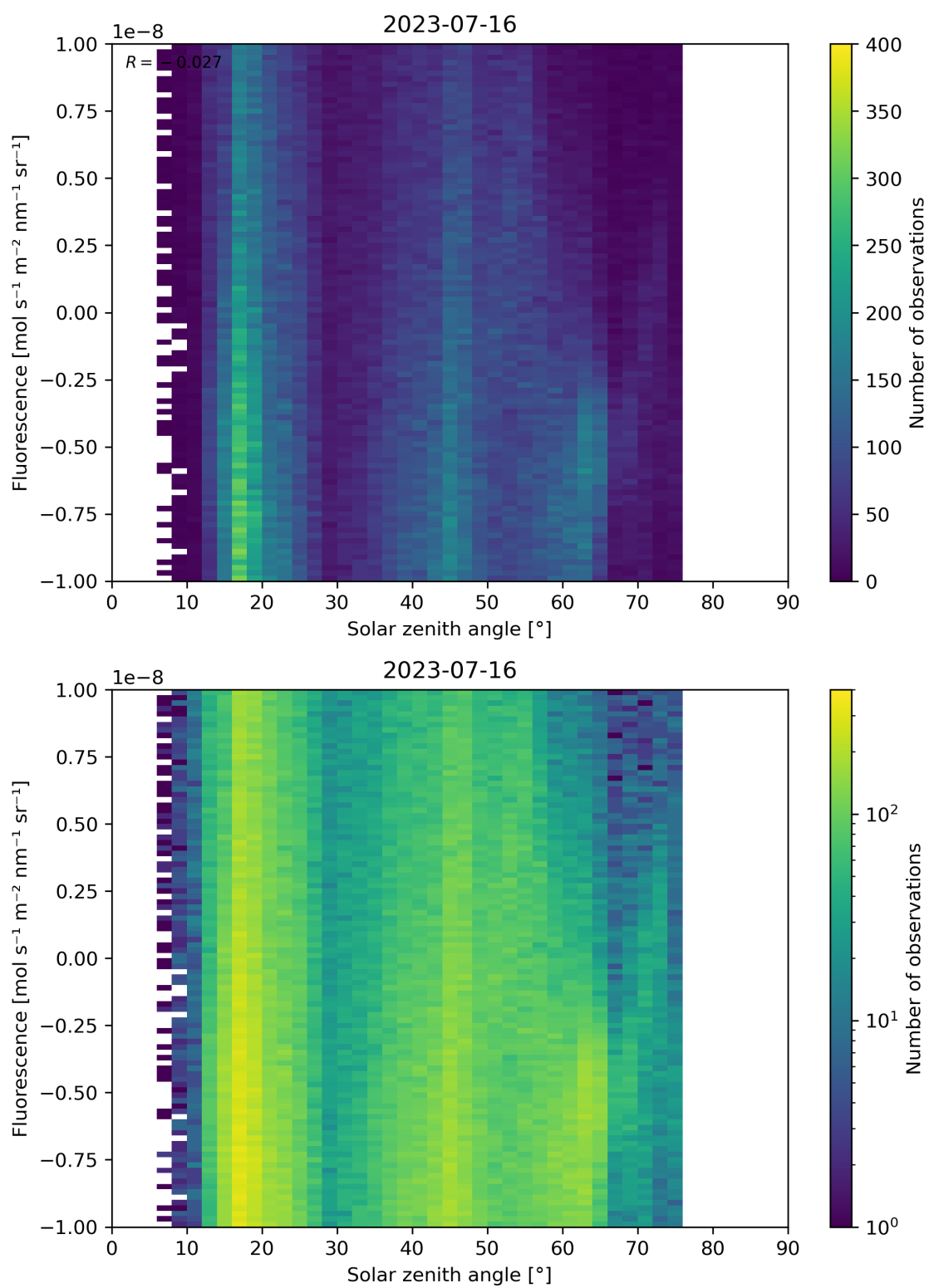
Figure 97: Scatter density plot of “Solar zenith angle” against “Fluorescence” for 2023-07-15 to 2023-07-17.
