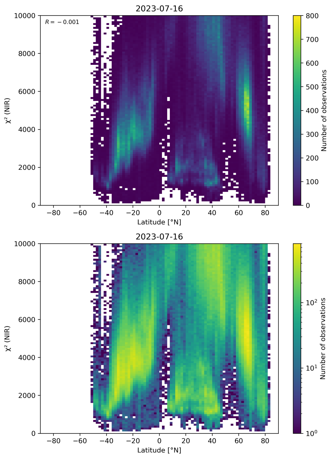
Figure 53: Scatter density plot of “Latitude” against “ \chi^2 (NIR)” for 2023-07-15 to 2023-07-17.
