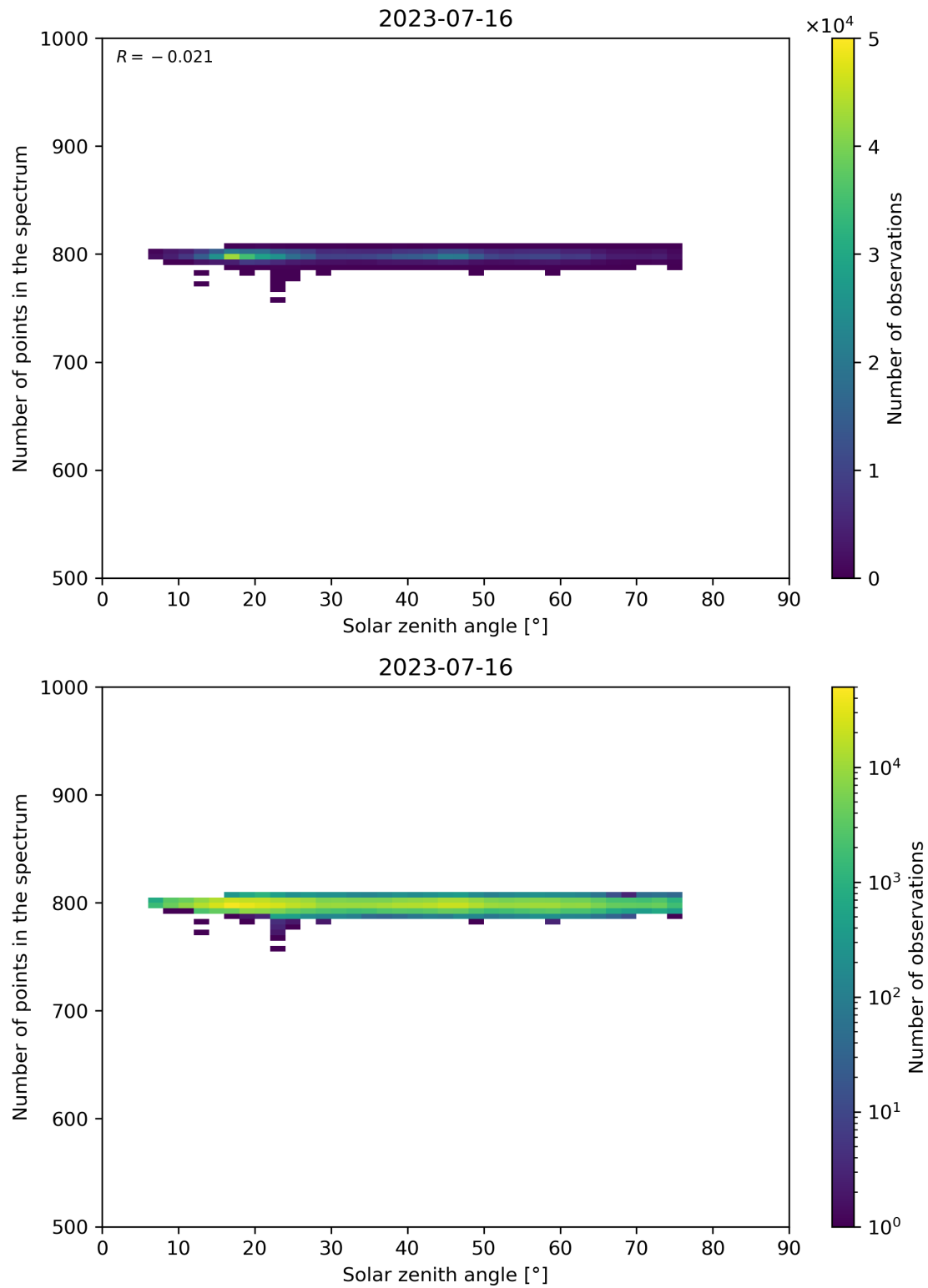
Figure 103: Scatter density plot of “Solar zenith angle” against “Number of points in the spectrum” for 2023-07-15 to 2023-07-17.
