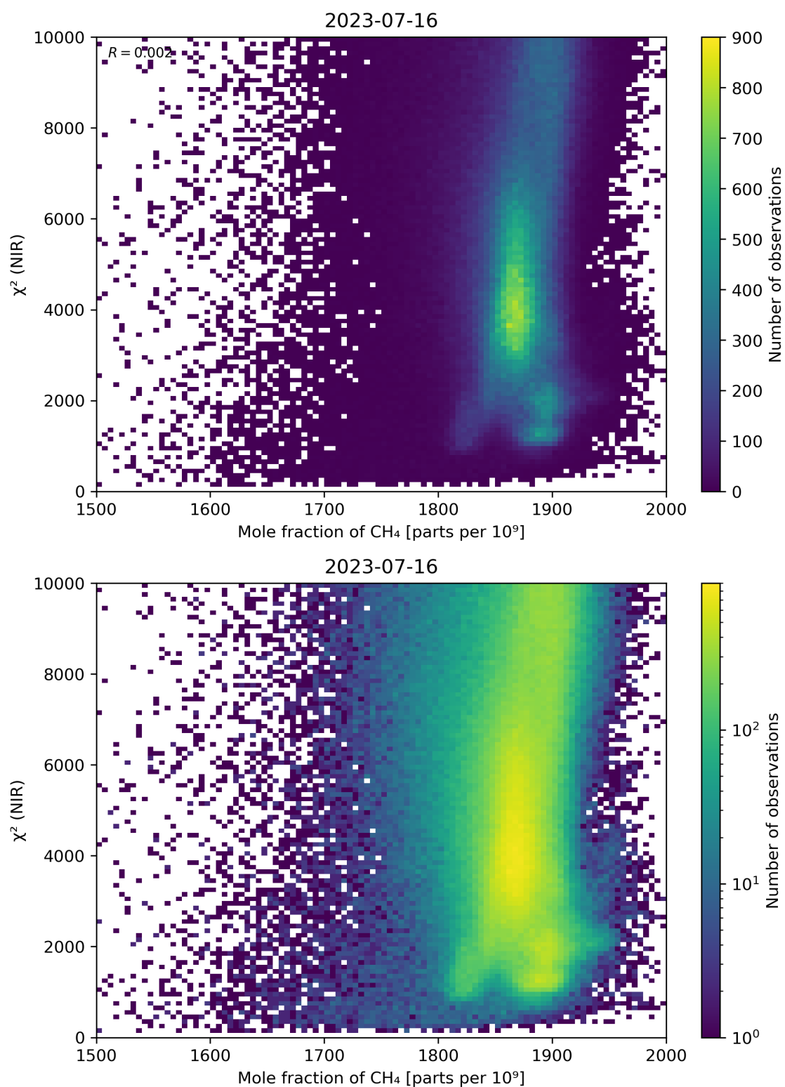
Figure 70: Scatter density plot of “Mole fraction of CH 4 ” against “ \chi^2 (NIR)” for 2023-07-15 to 2023-07-17.
