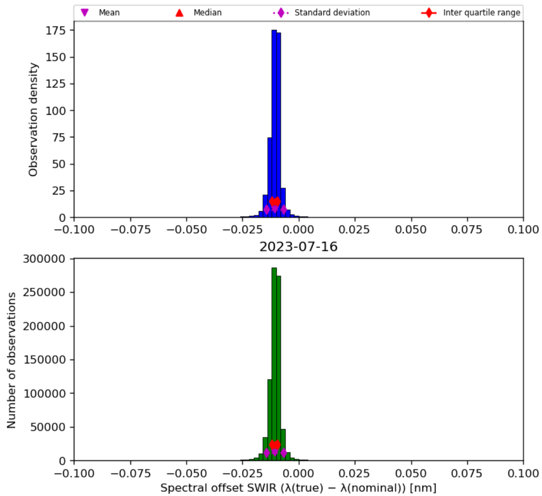
Figure 27: Histogram of “Spectral offset SWIR ( \lambda(\text{true}) - \lambda(\text{nominal}) )” for 2023-07-15 to 2023-07-17
