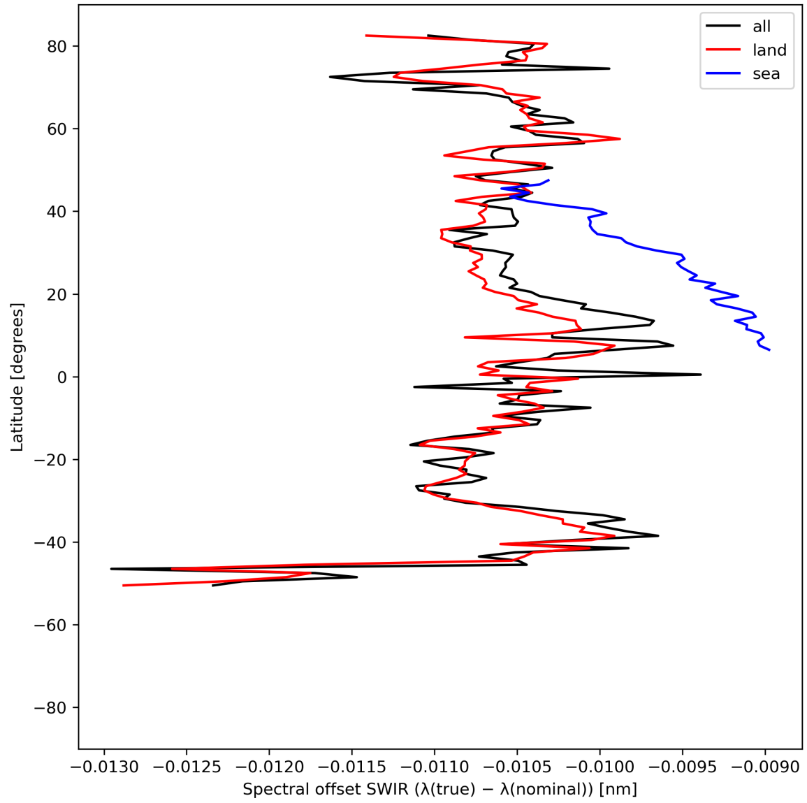
Figure 16: Zonal average of “Spectral offset SWIR ( \lambda(\text{true}) - \lambda(\text{nominal}) )” for 2023-07-15 to 2023-07-17.
