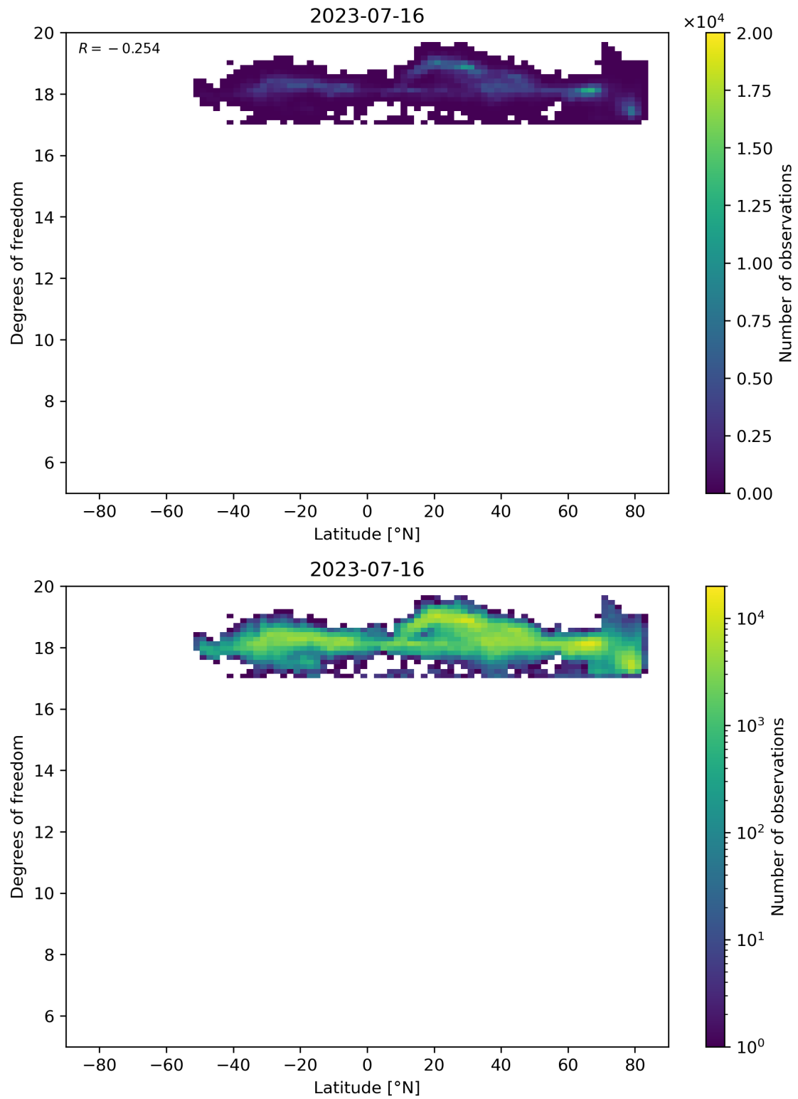
Figure 55: Scatter density plot of “Latitude” against “Degrees of freedom” for 2023-07-15 to 2023-07-17.
