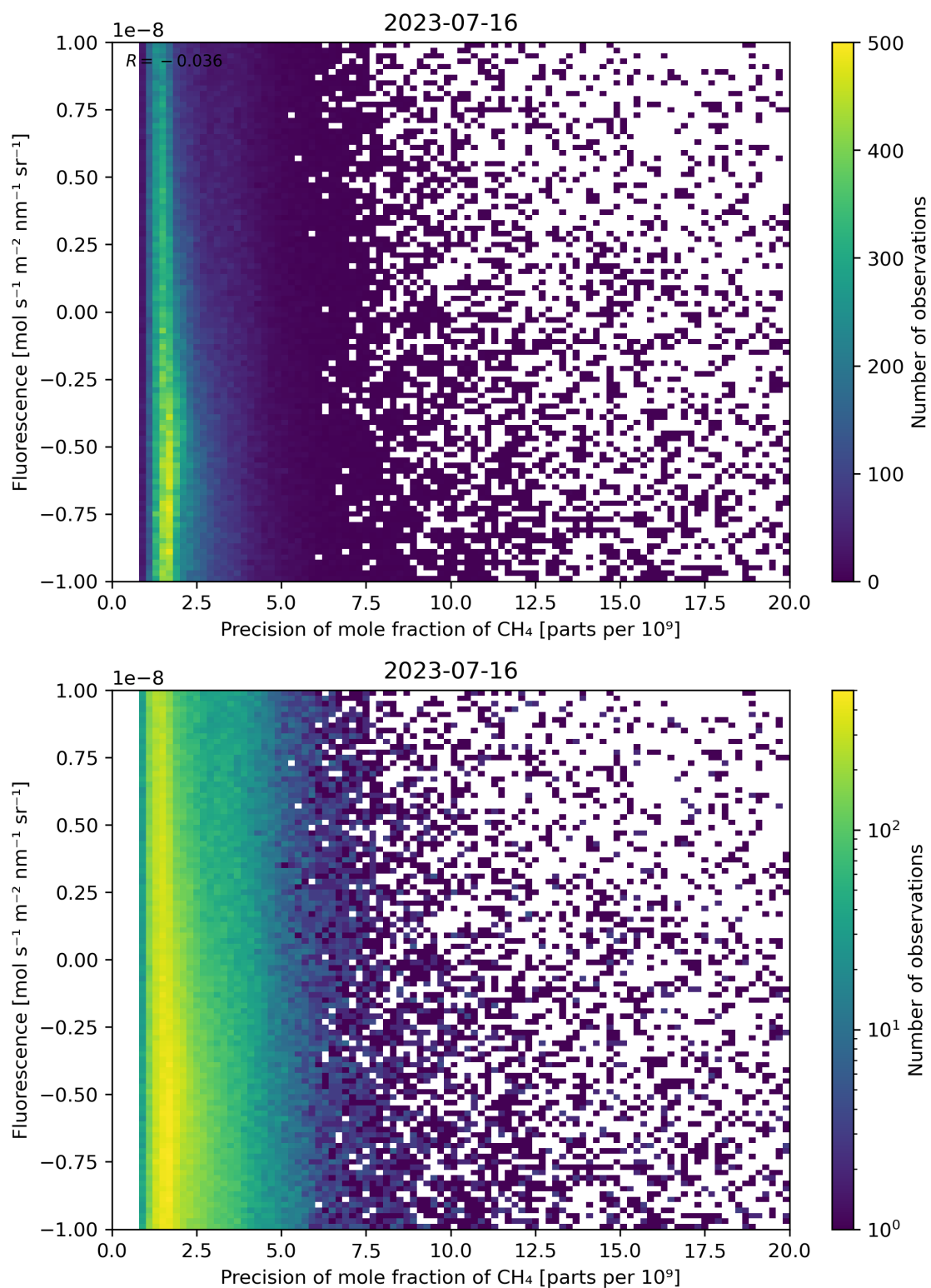
Figure 81: Scatter density plot of “Precision of mole fraction of \text{CH}_4 ” against “Fluorescence” for 2023-07-15 to 2023-07-17.
