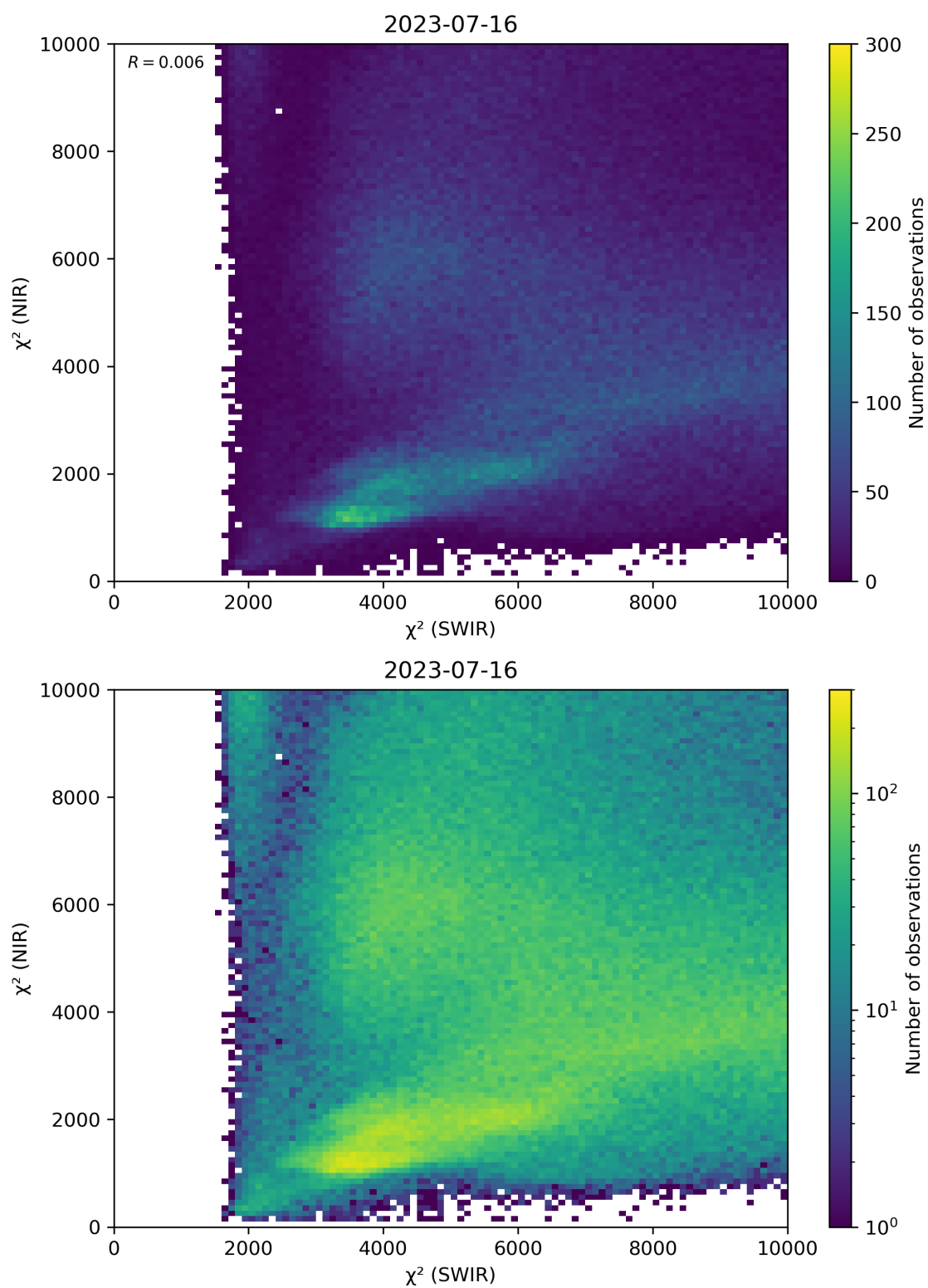
Figure 47: Scatter density plot of “ \chi^2 (SWIR)” against “ \chi^2 (NIR)” for 2023-07-15 to 2023-07-17.
