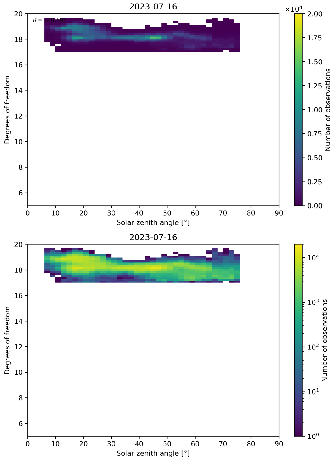
Figure 96: Scatter density plot of “Solar zenith angle” against “Degrees of freedom” for 2023-07-15 to 2023-07-17.
