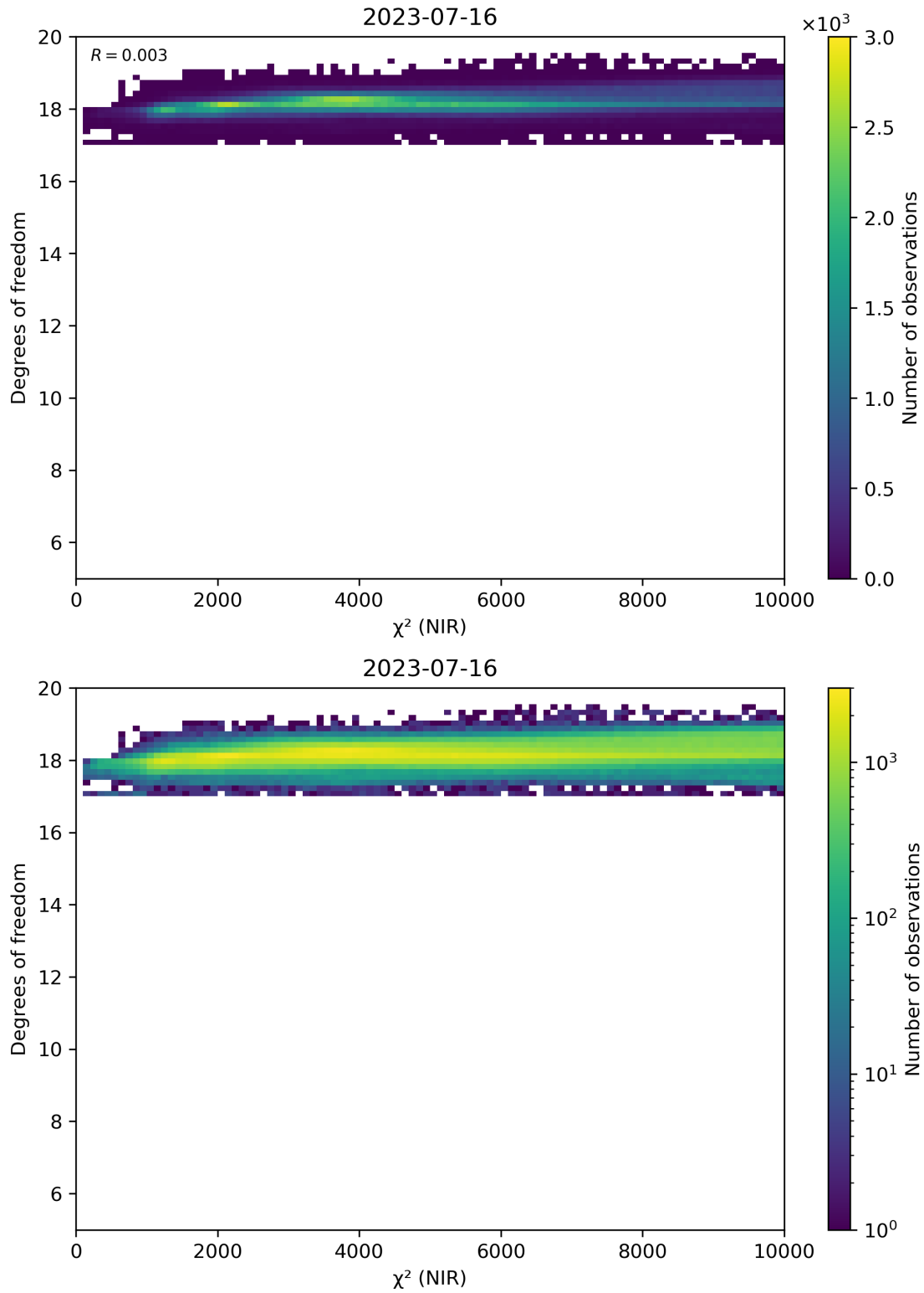
Figure 44: Scatter density plot of “ \chi^2 (NIR)” against “Degrees of freedom” for 2023-07-15 to 2023-07-17.
