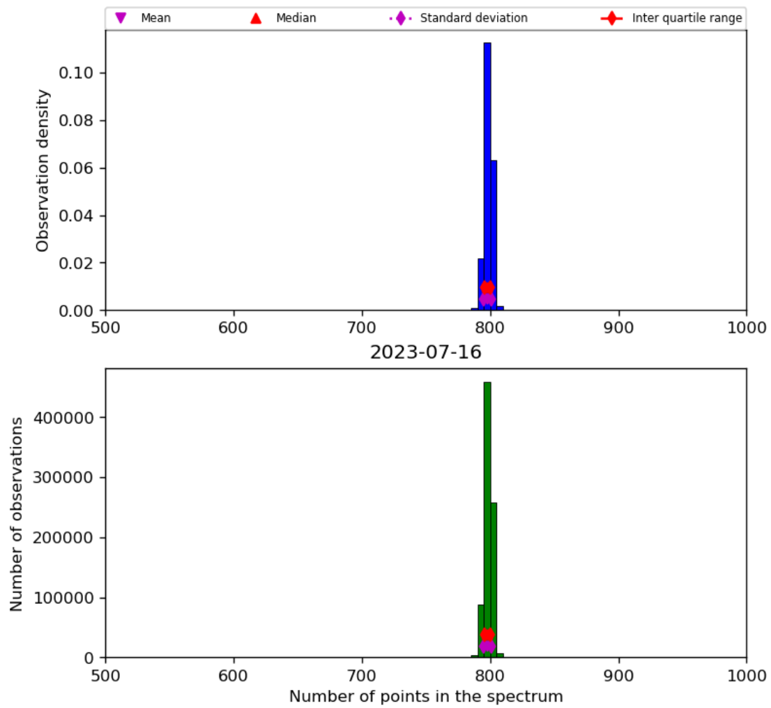
Figure 26: Histogram of “Number of points in the spectrum” for 2023-07-15 to 2023-07-17
