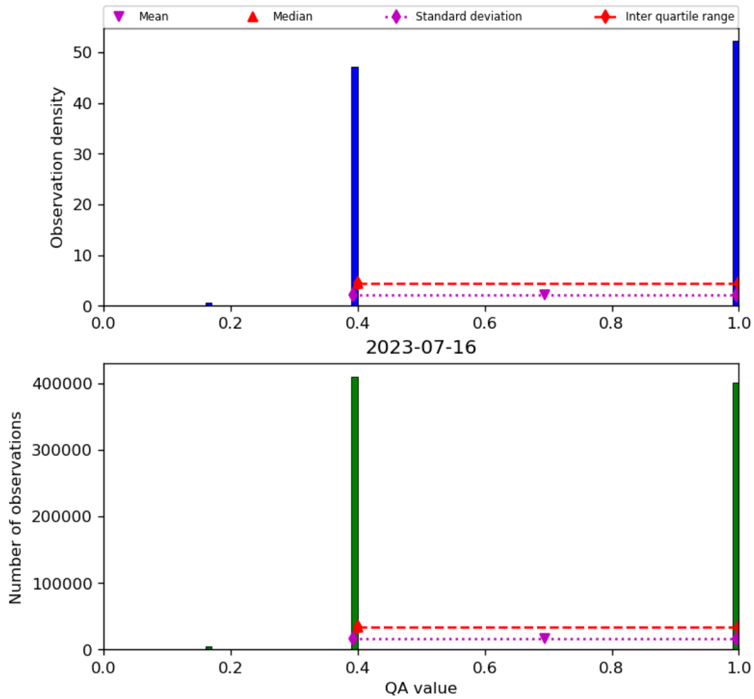
Figure 22: Histogram of “QA value” for 2023-07-15 to 2023-07-17
