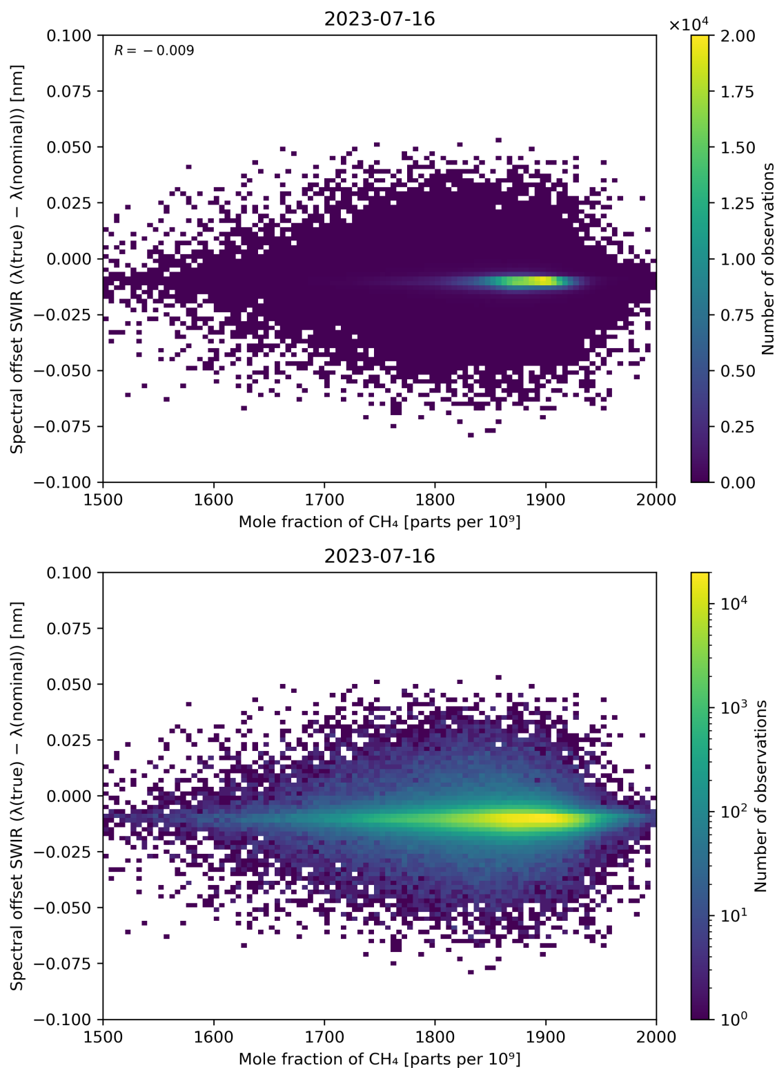
Figure 86: Scatter density plot of “Mole fraction of CH 4 ” against “Spectral offset SWIR ( \lambda(\text{true}) - \lambda(\text{nominal}) )” for 2023-07-15 to 2023-07-17.
