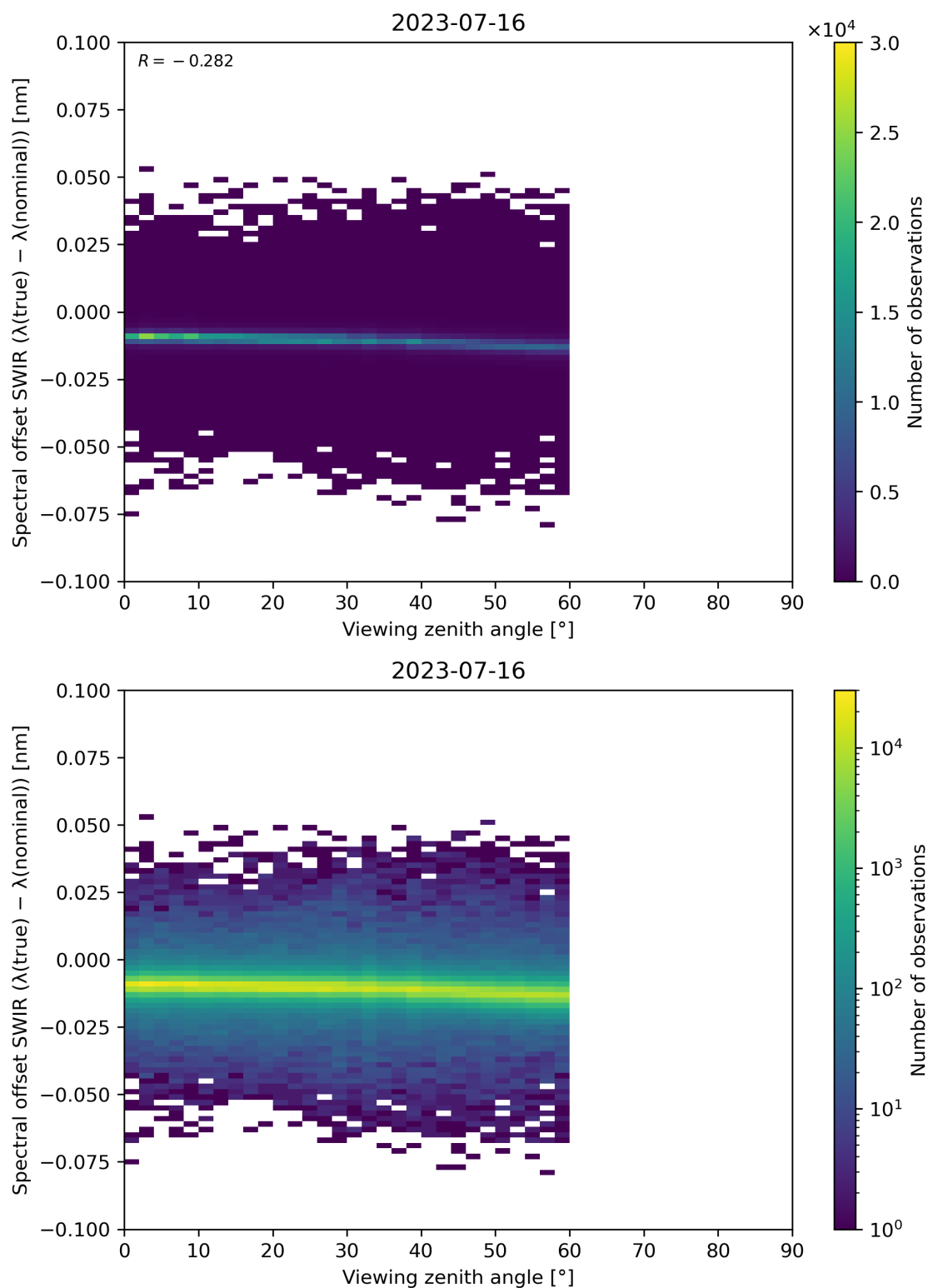
Figure 116: Scatter density plot of “Viewing zenith angle” against “Spectral offset SWIR ( \lambda(\text{true}) - \lambda(\text{nominal}) )” for 2023-07-15 to 2023-07-17.
