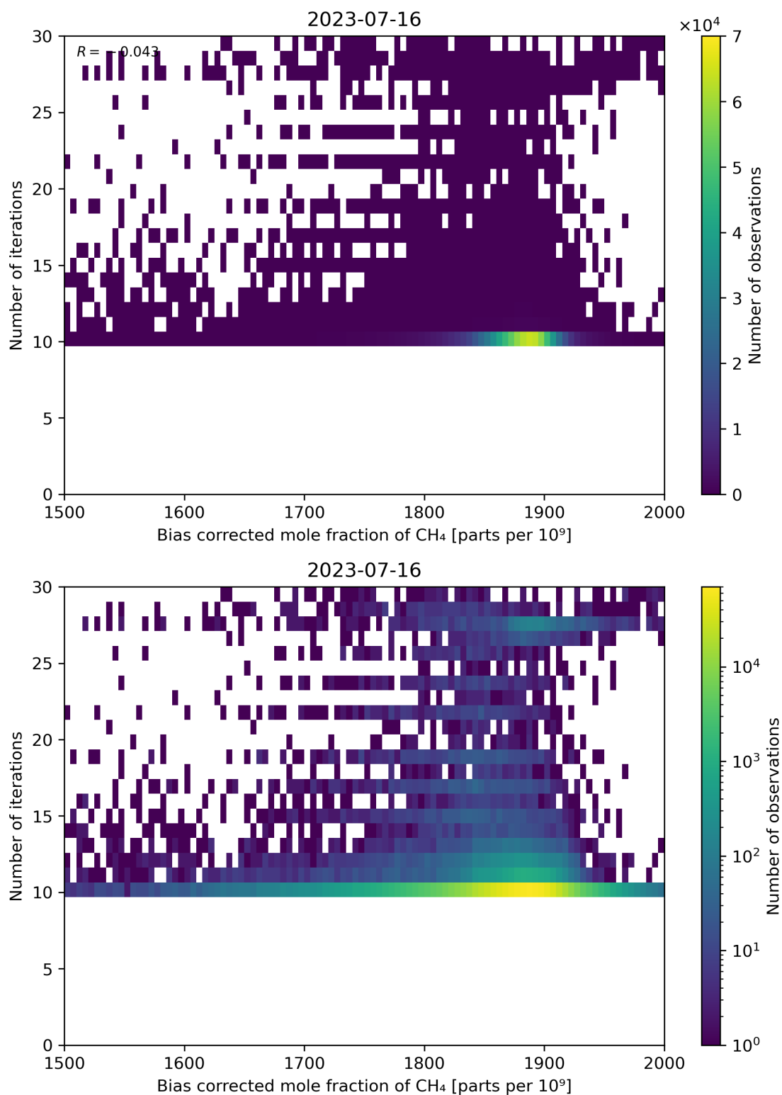
Figure 67: Scatter density plot of “Bias corrected mole fraction of CH 4 ” against “Number of iterations” for 2023-07-15 to 2023-07-17.
