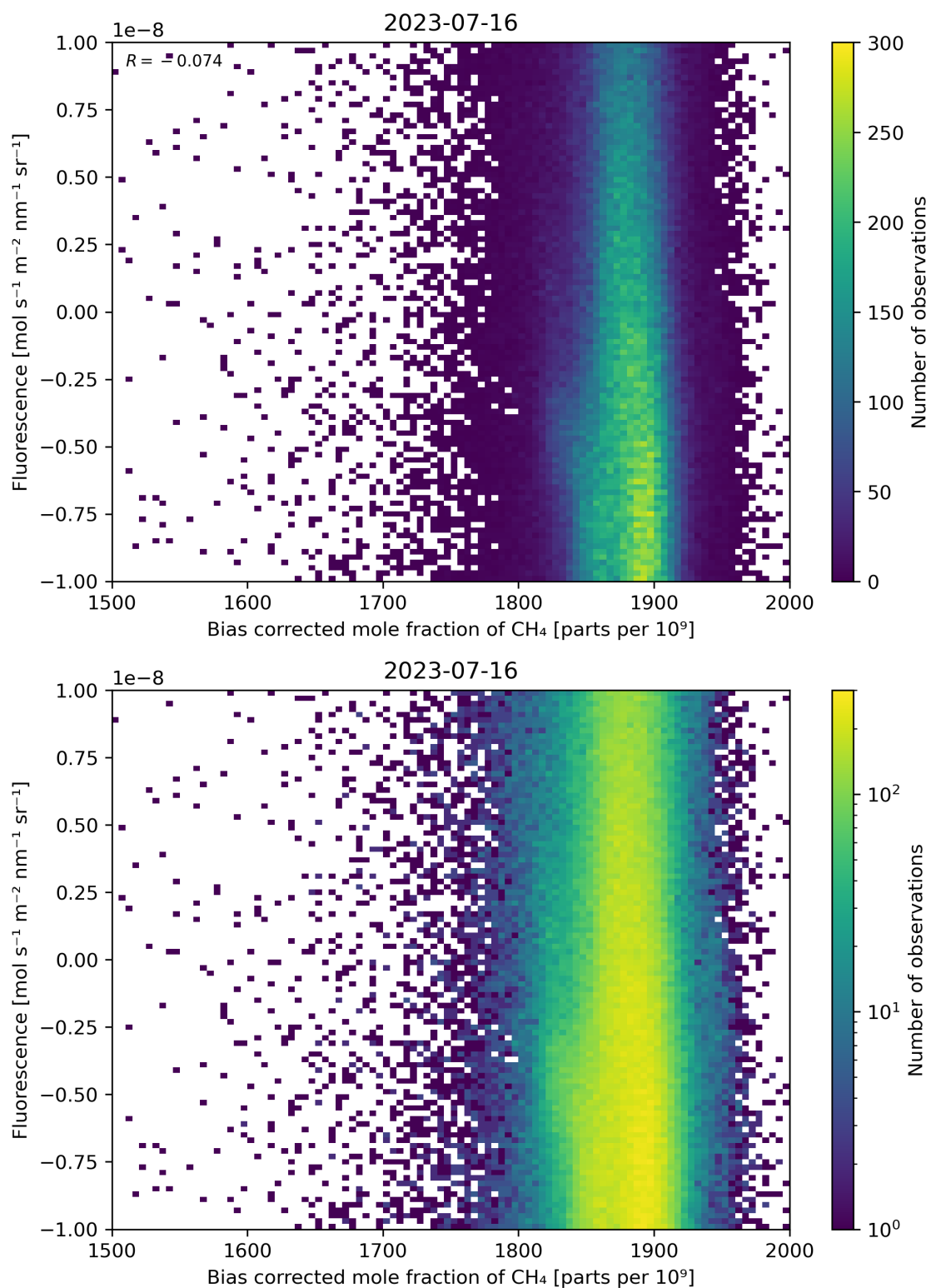
Figure 66: Scatter density plot of “Bias corrected mole fraction of \text{CH}_4 ” against “Fluorescence” for 2023-07-15 to 2023-07-17.
