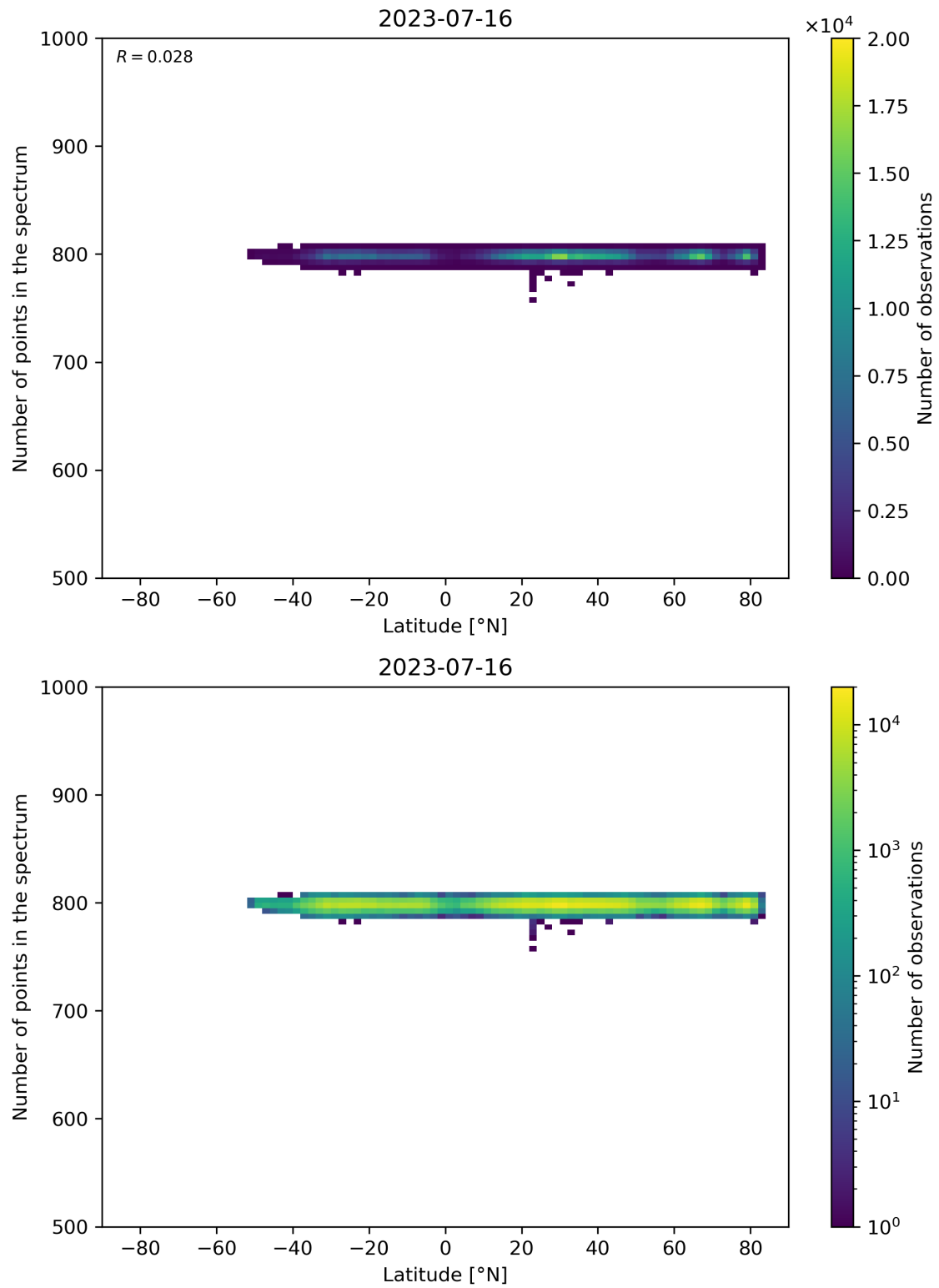
Figure 61: Scatter density plot of “Latitude” against “Number of points in the spectrum” for 2023-07-15 to 2023-07-17.
