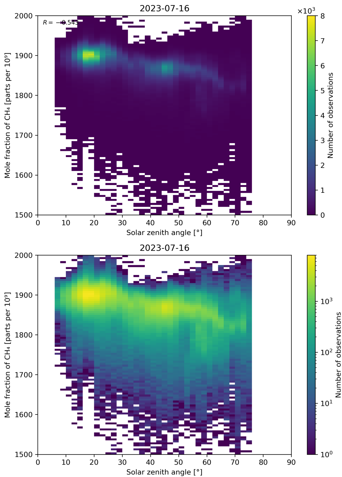
Figure 99: Scatter density plot of “Solar zenith angle” against “Mole fraction of CH 4 ” for 2023-07-15 to 2023-07-17.
