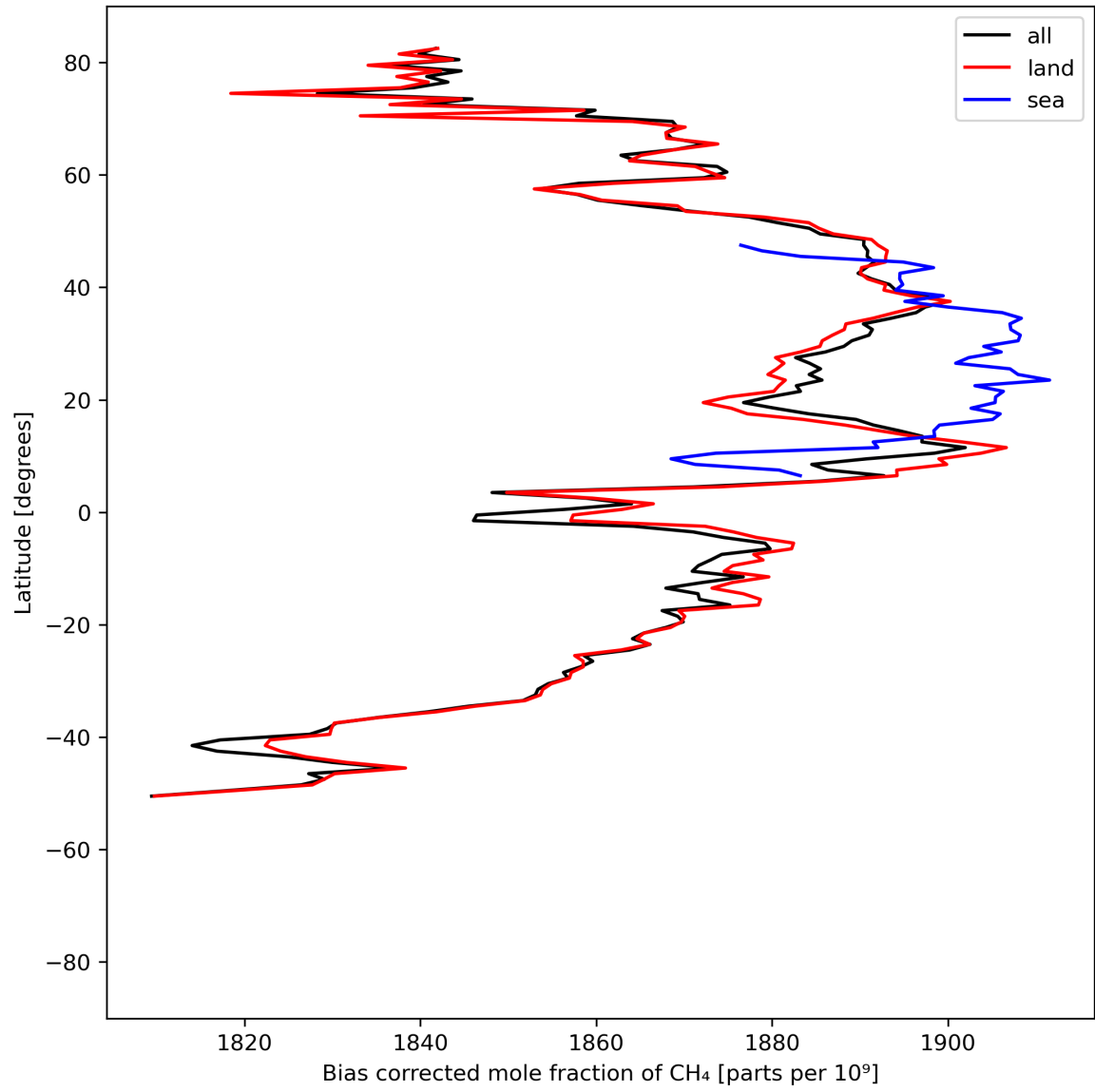
Figure 14: Zonal average of “Bias corrected mole fraction of CH 4 ” for 2023-07-15 to 2023-07-17.
