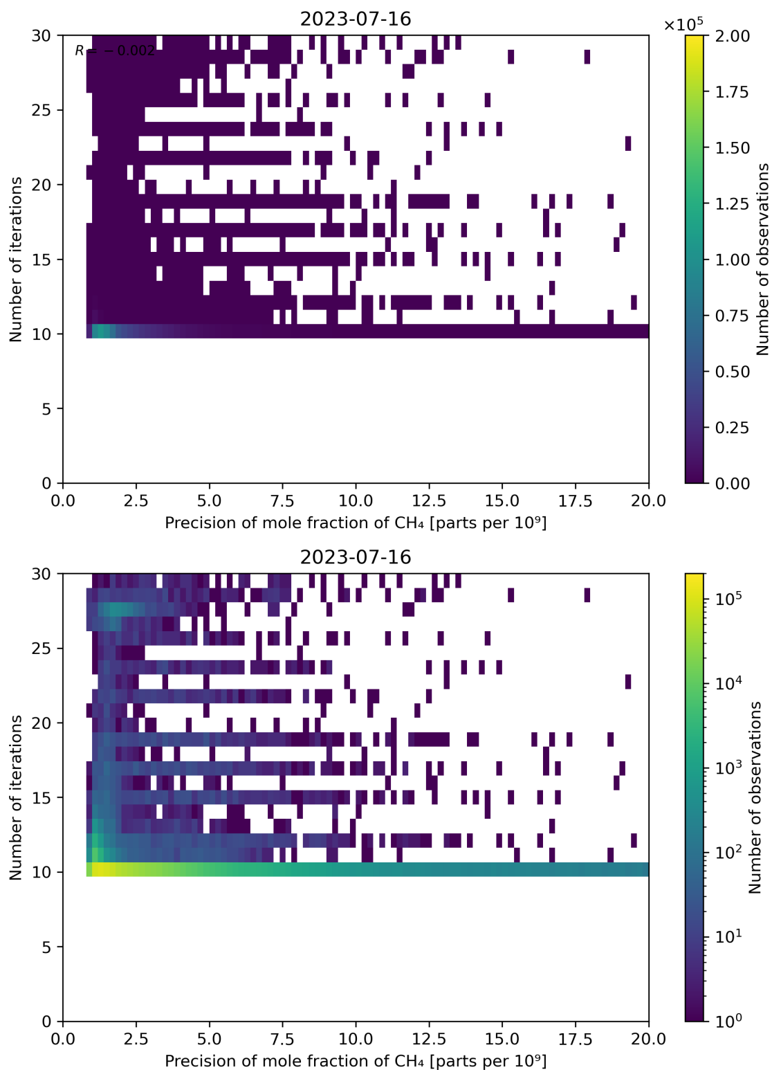
Figure 83: Scatter density plot of “Precision of mole fraction of CH 4 ” against “Number of iterations” for 2023-07-15 to 2023-07-17.
