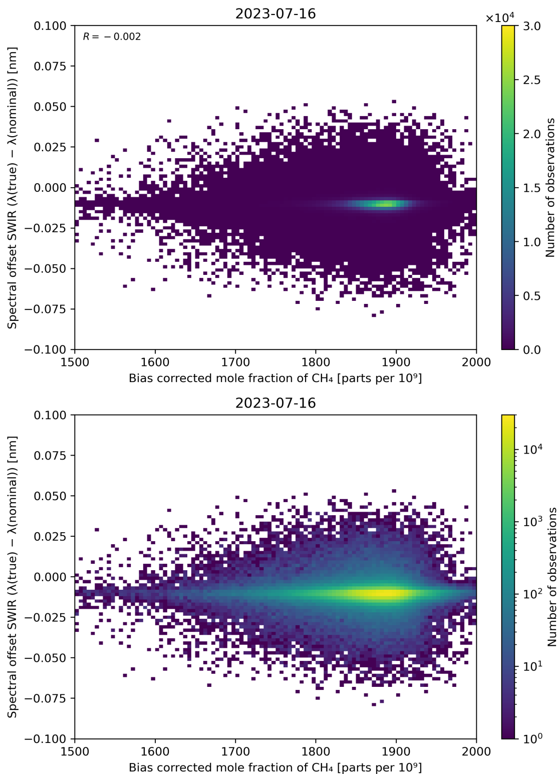
Figure 69: Scatter density plot of “Bias corrected mole fraction of \text{CH}_4 ” against “Spectral offset SWIR ( \lambda(\text{true}) - \lambda(\text{nominal}) )” for 2023-07-15 to 2023-07-17.
