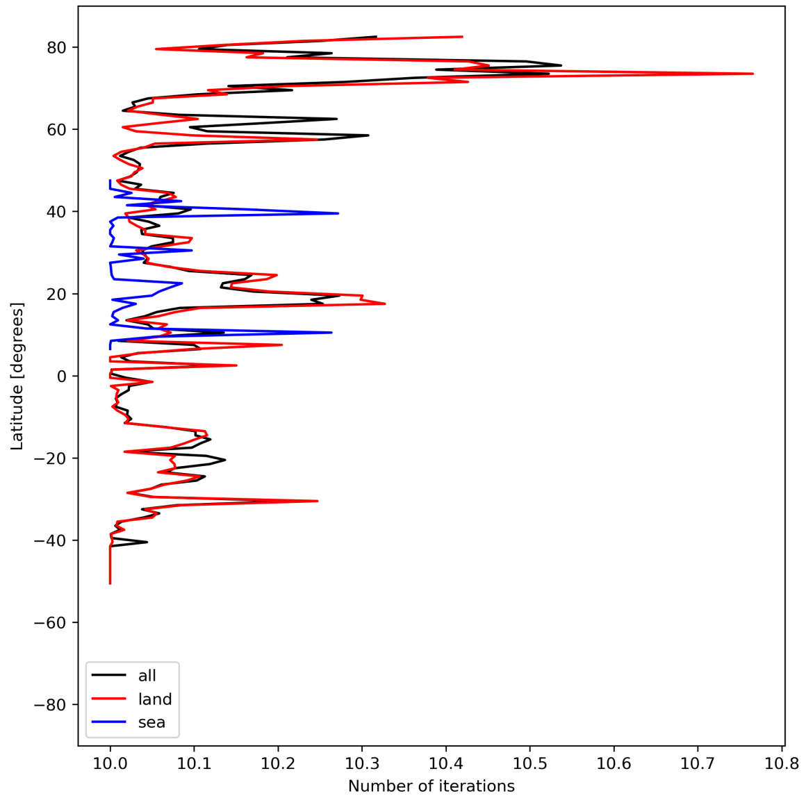
Figure 20: Zonal average of “Number of iterations” for 2023-07-15 to 2023-07-17.
