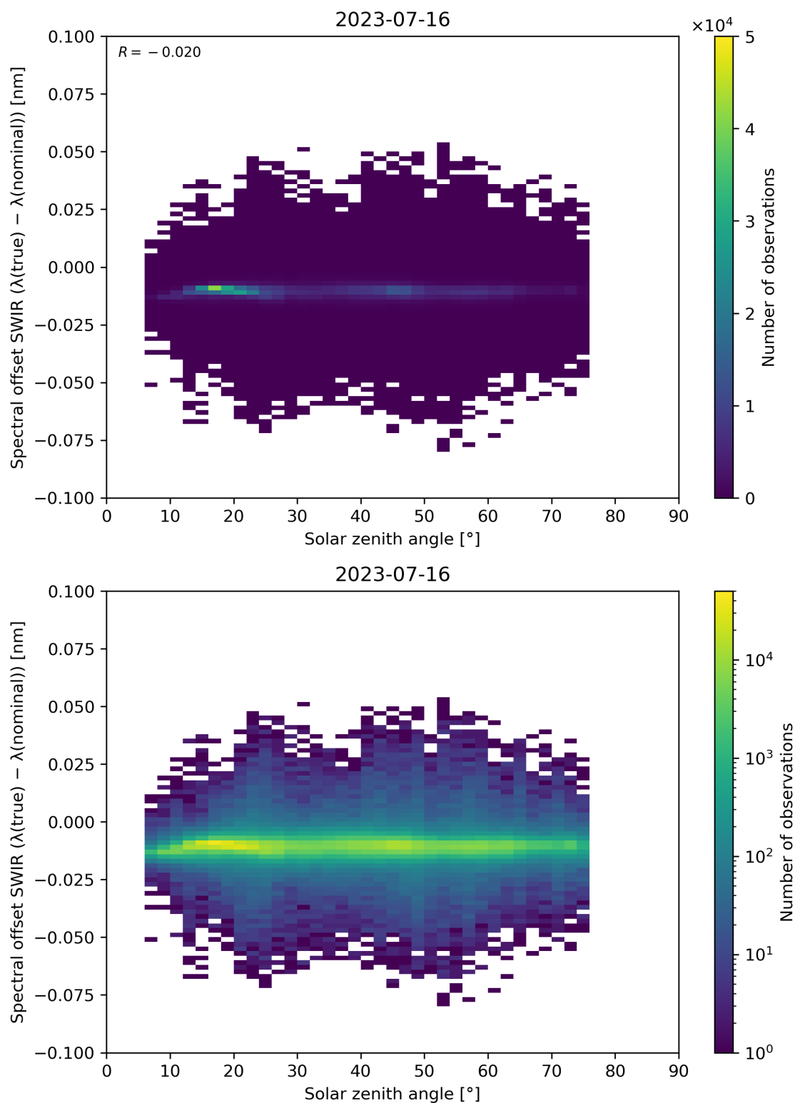
Figure 104: Scatter density plot of “Solar zenith angle” against “Spectral offset SWIR ( \lambda(\text{true}) - \lambda(\text{nominal}) )” for 2023-07-15 to 2023-07-17.
