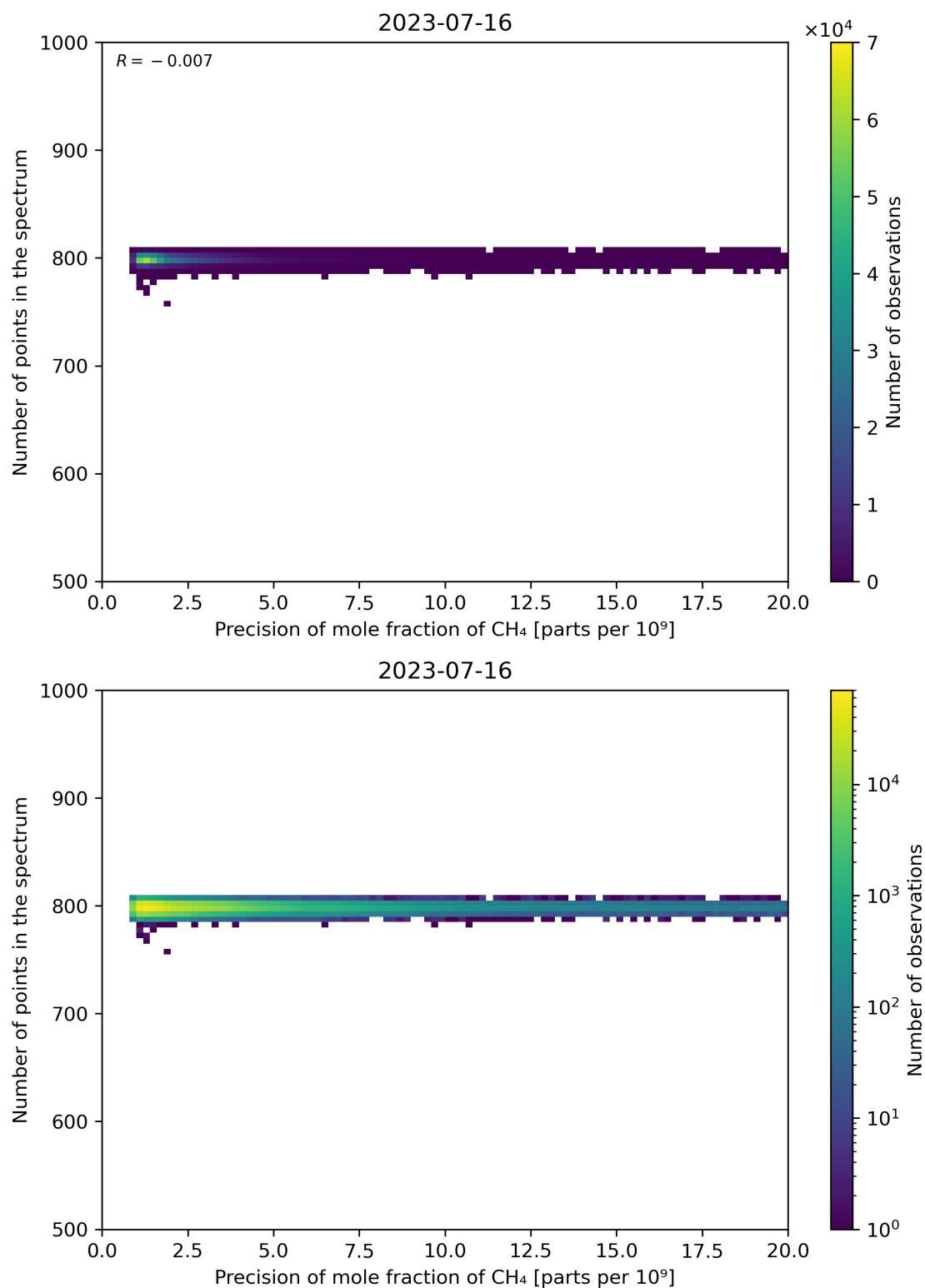
Figure 84: Scatter density plot of “Precision of mole fraction of CH 4 ” against “Number of points in the spectrum” for 2023-07-15 to 2023-07-17.
