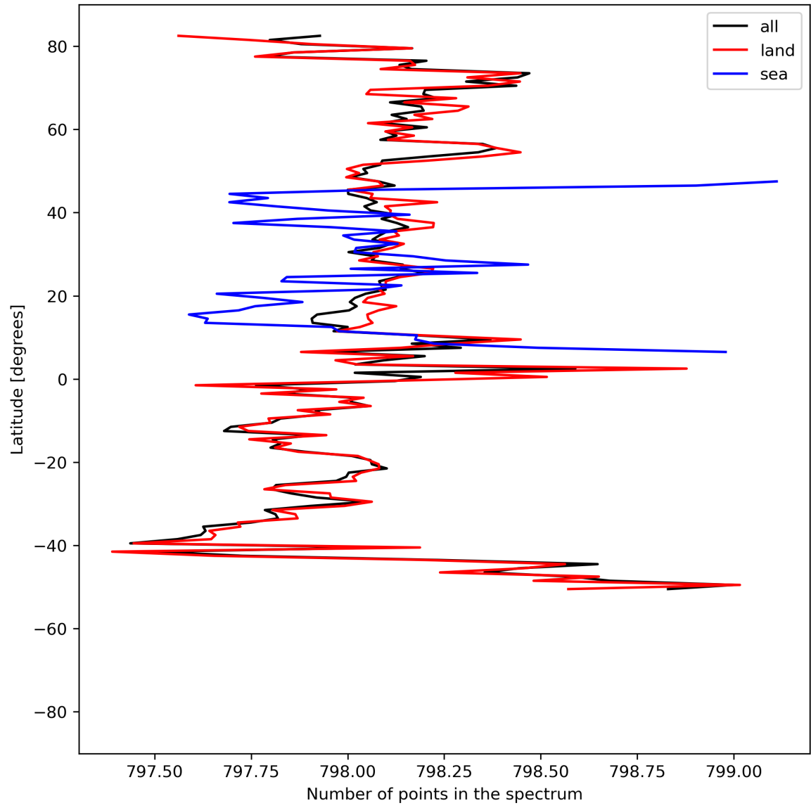
Figure 15: Zonal average of “Number of points in the spectrum” for 2023-07-15 to 2023-07-17.
