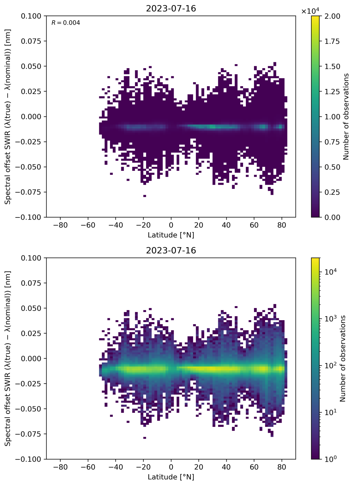
Figure 62: Scatter density plot of “Latitude” against “Spectral offset SWIR ( \lambda(\text{true}) - \lambda(\text{nominal}) )” for 2023-07-15 to 2023-07-17.
