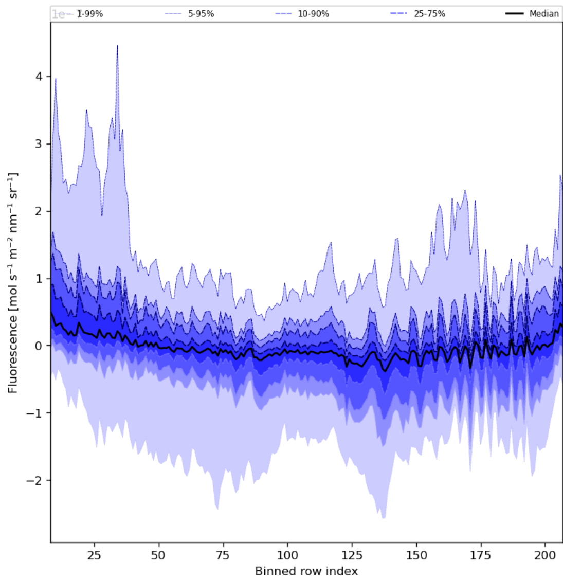
Figure 43: Along track statistics of “Fluorescence” for 2023-07-15 to 2023-07-17
