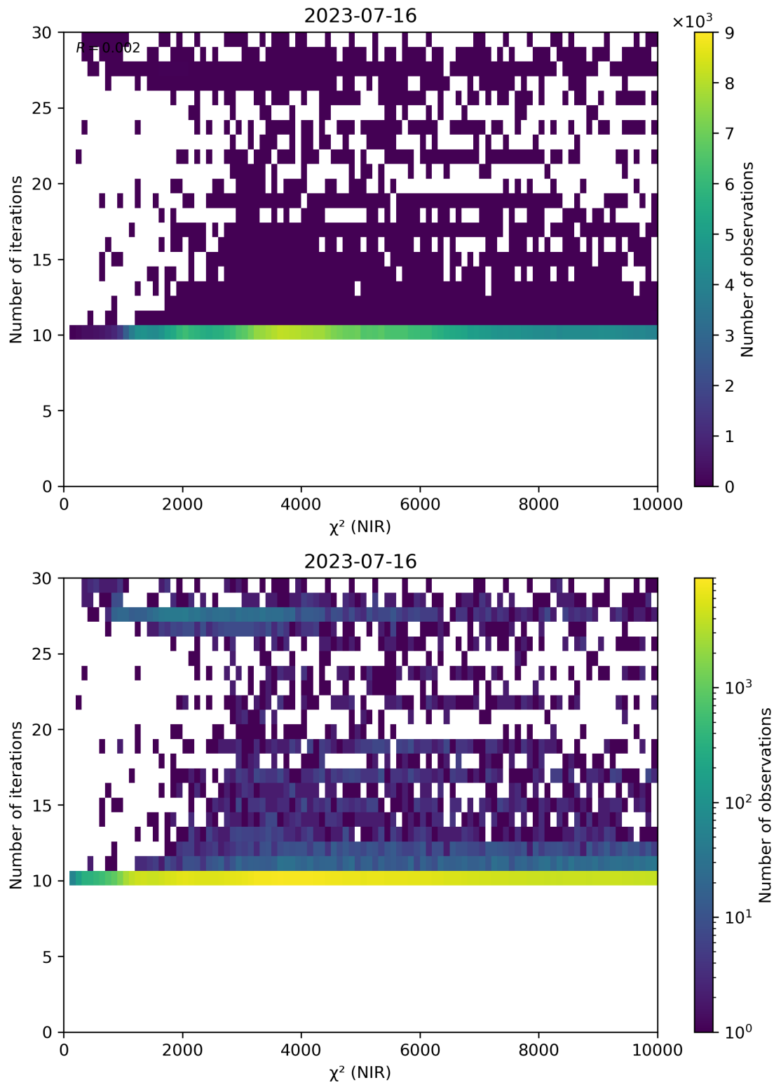
Figure 46: Scatter density plot of “ \chi^2 (NIR)” against “Number of iterations” for 2023-07-15 to 2023-07-17.
