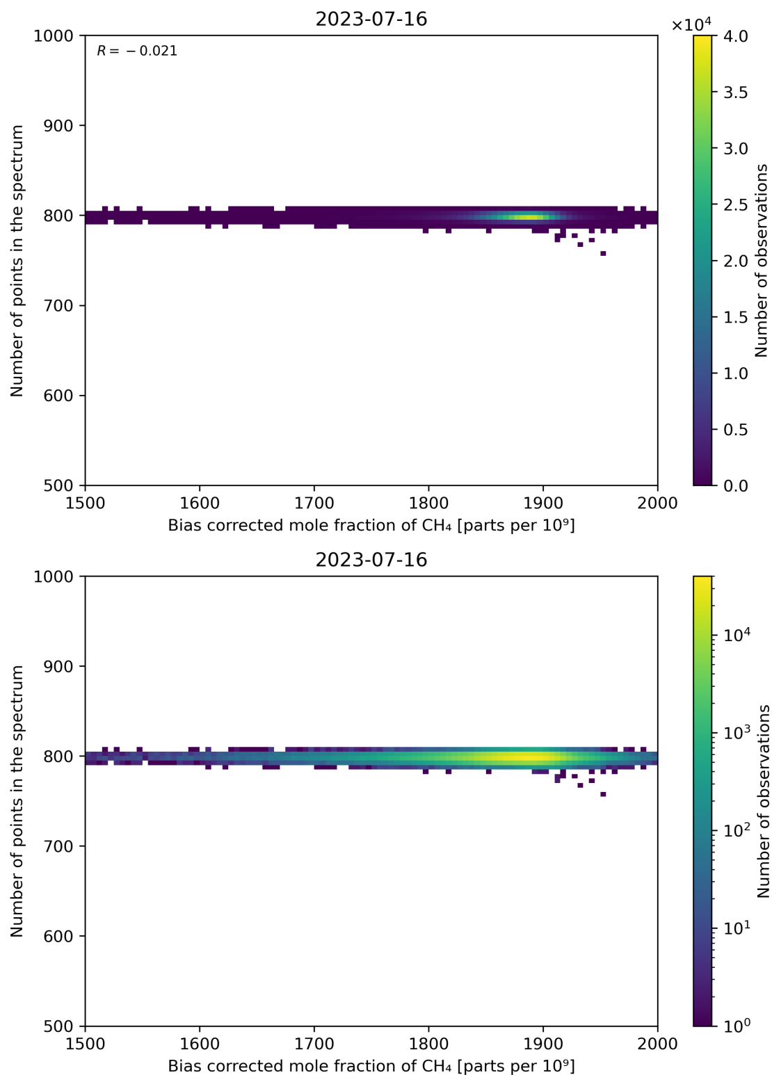
Figure 68: Scatter density plot of “Bias corrected mole fraction of CH 4 ” against “Number of points in the spectrum” for 2023-07-15 to 2023-07-17.
