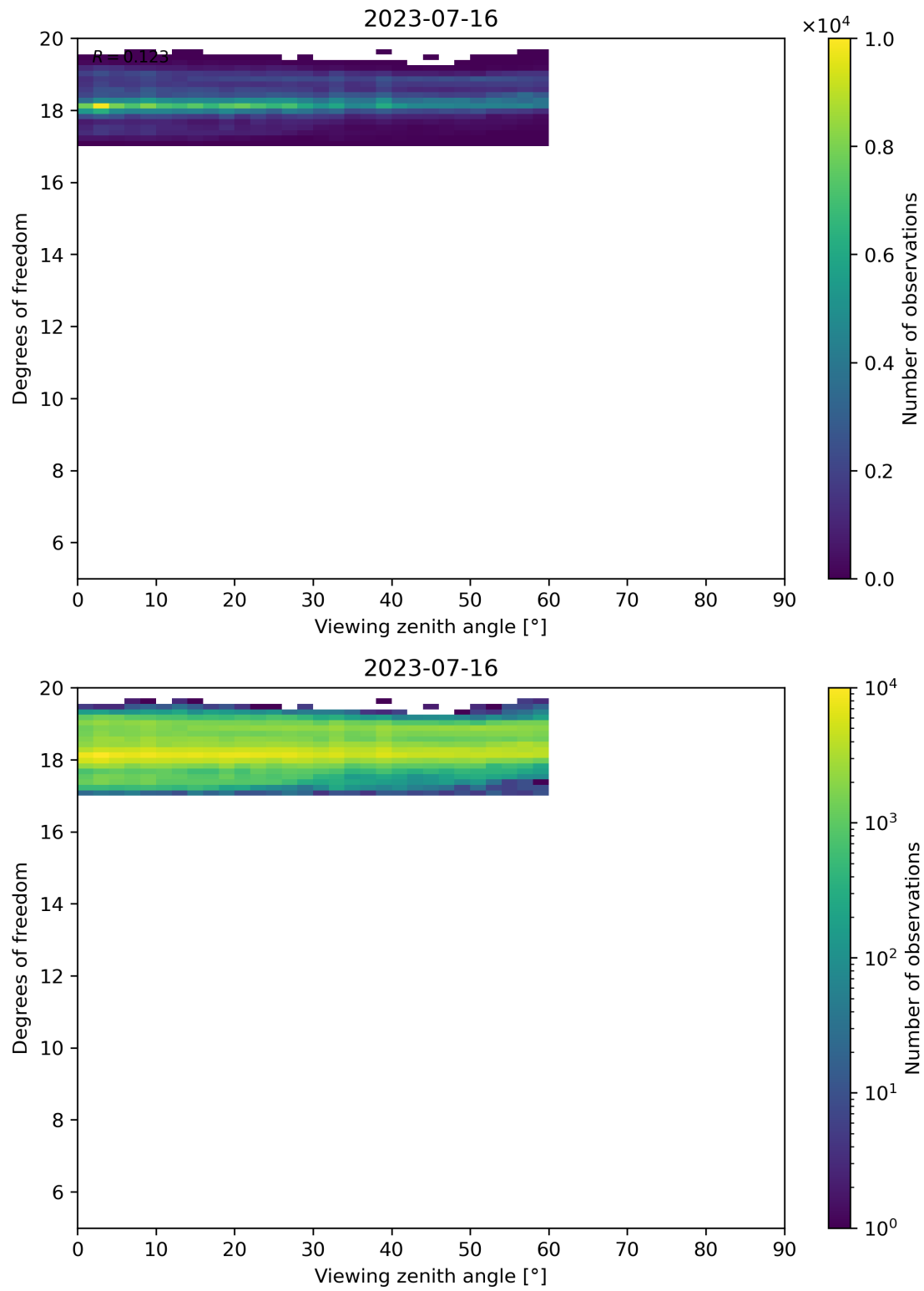
Figure 107: Scatter density plot of “Viewing zenith angle” against “Degrees of freedom” for 2023-07-15 to 2023-07-17.
