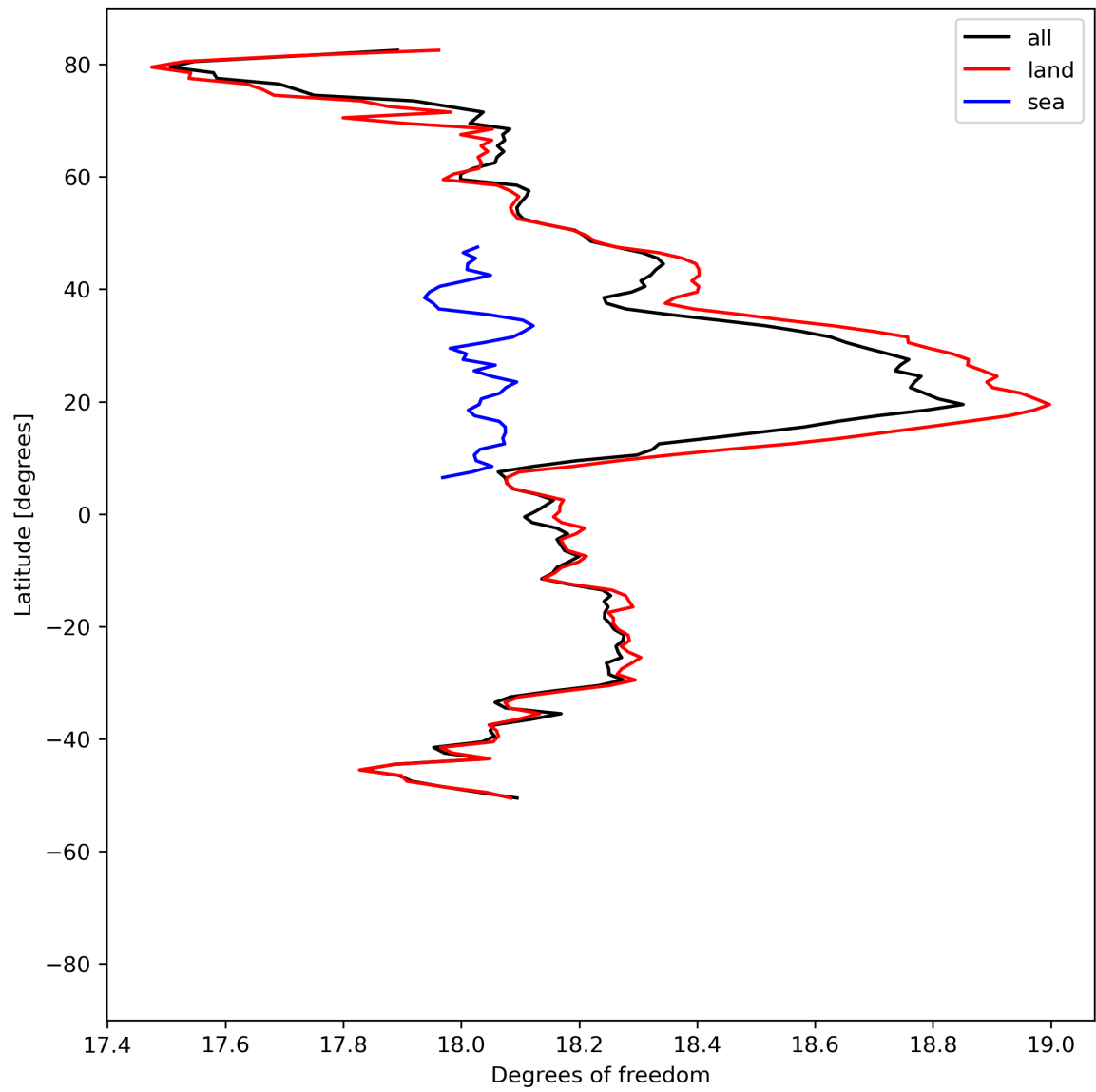
Figure 19: Zonal average of “Degrees of freedom” for 2023-07-15 to 2023-07-17.
