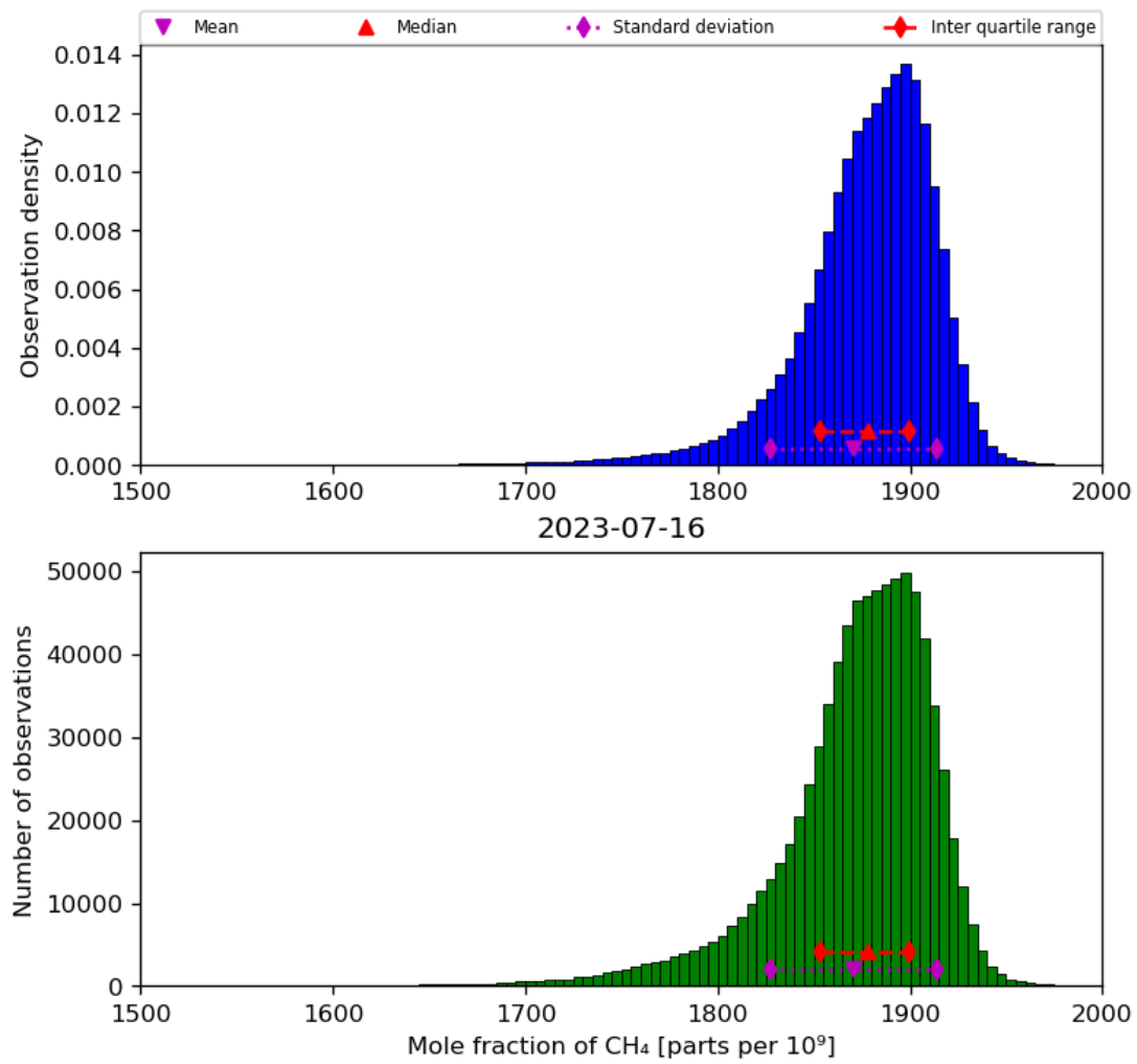
Figure 23: Histogram of "Mole fraction of CH 4 " for 2023-07-15 to 2023-07-17
