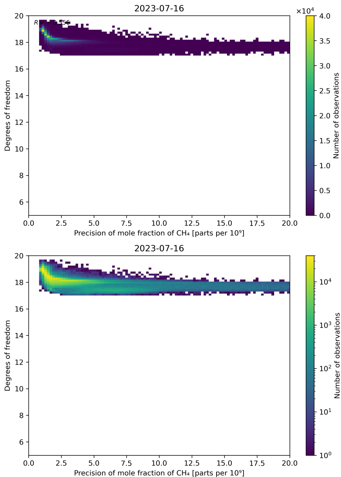
Figure 80: Scatter density plot of “Precision of mole fraction of CH 4 ” against “Degrees of freedom” for 2023-07-15 to 2023-07-17.
