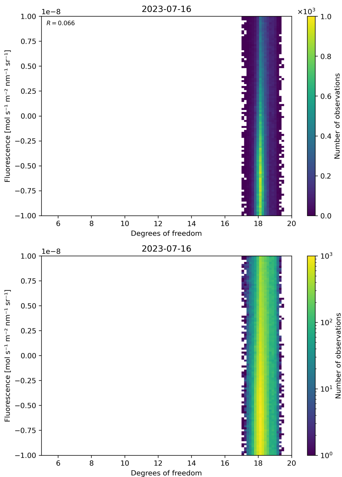
Figure 51: Scatter density plot of “Degrees of freedom” against “Fluorescence” for 2023-07-15 to 2023-07-17.
