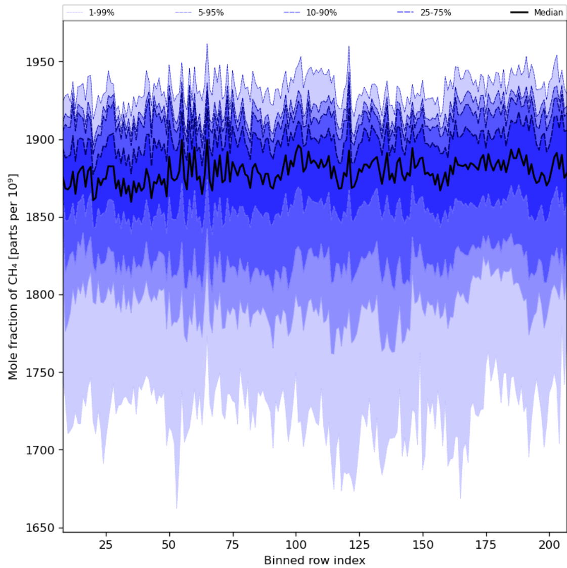
Figure 34: Along track statistics of “Mole fraction of CH 4 ” for 2023-07-15 to 2023-07-17
