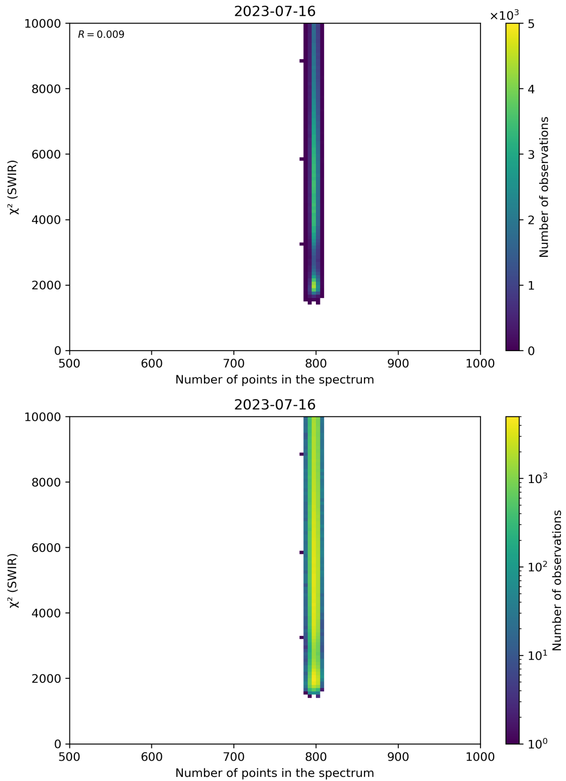
Figure 89: Scatter density plot of “Number of points in the spectrum” against “ \chi^2 (SWIR)” for 2023-07-15 to 2023-07-17.
