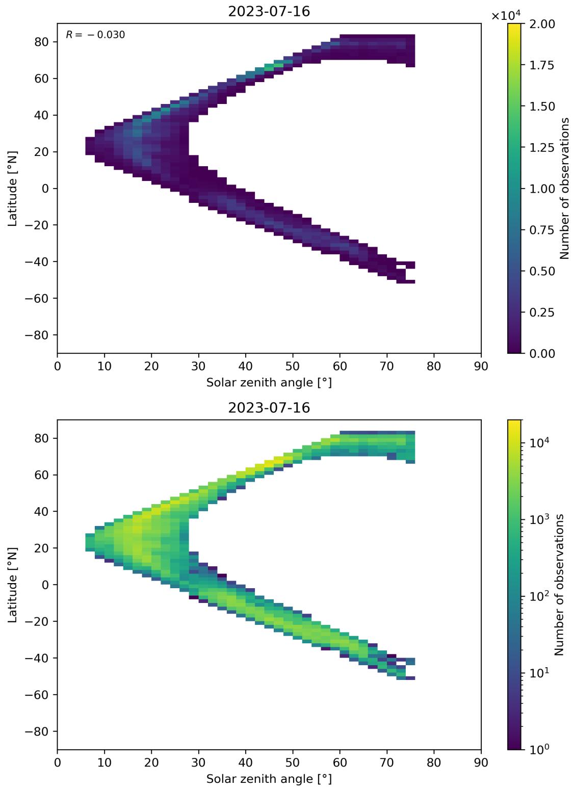
Figure 98: Scatter density plot of “Solar zenith angle” against “Latitude” for 2023-07-15 to 2023-07-17.
