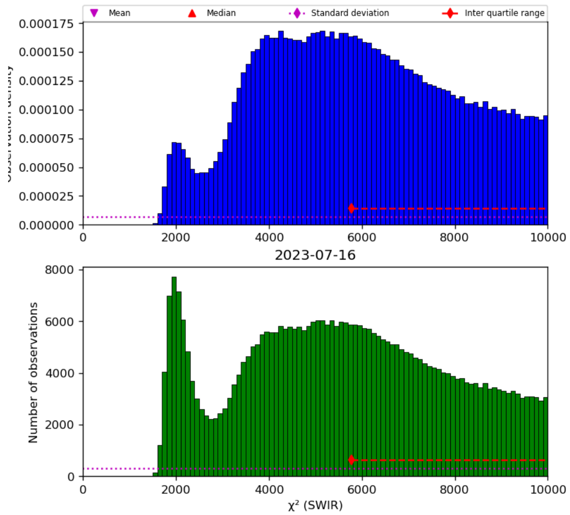
Figure 28: Histogram of “ \chi^2 (SWIR)” for 2023-07-15 to 2023-07-17
