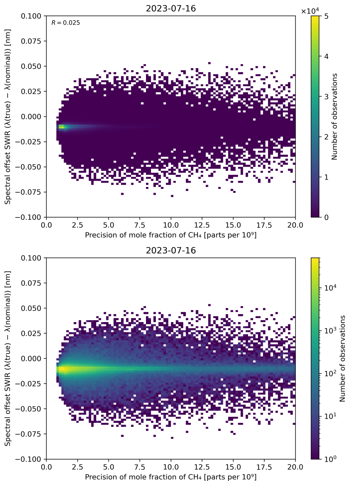
Figure 85: Scatter density plot of “Precision of mole fraction of CH 4 ” against “Spectral offset SWIR ( \lambda(\text{true}) - \lambda(\text{nominal}) )” for 2023-07-15 to 2023-07-17.
