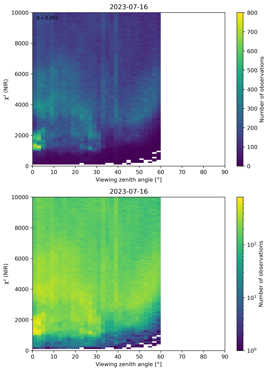
Figure 105: Scatter density plot of “Viewing zenith angle” against “ \chi^2 (NIR)” for 2023-07-15 to 2023-07-17.
