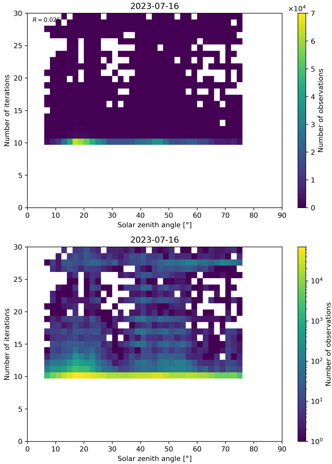
Figure 102: Scatter density plot of “Solar zenith angle” against “Number of iterations” for 2023-07-15 to 2023-07-17.
