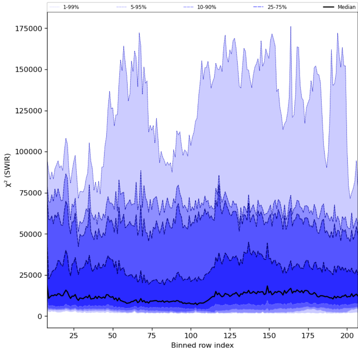
Figure 39: Along track statistics of " \chi^2 (SWIR)" for 2023-07-15 to 2023-07-17
