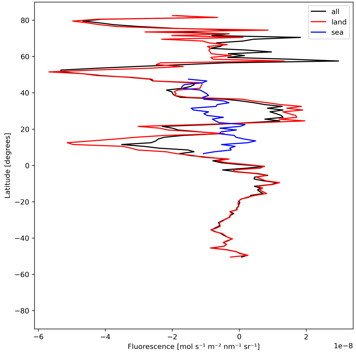
Figure 21: Zonal average of “Fluorescence” for 2023-07-15 to 2023-07-17.
