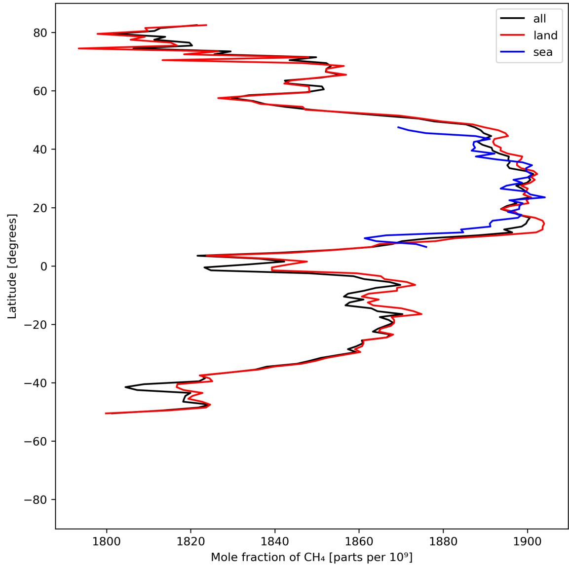
Figure 12: Zonal average of “Mole fraction of CH 4 ” for 2023-07-15 to 2023-07-17.
