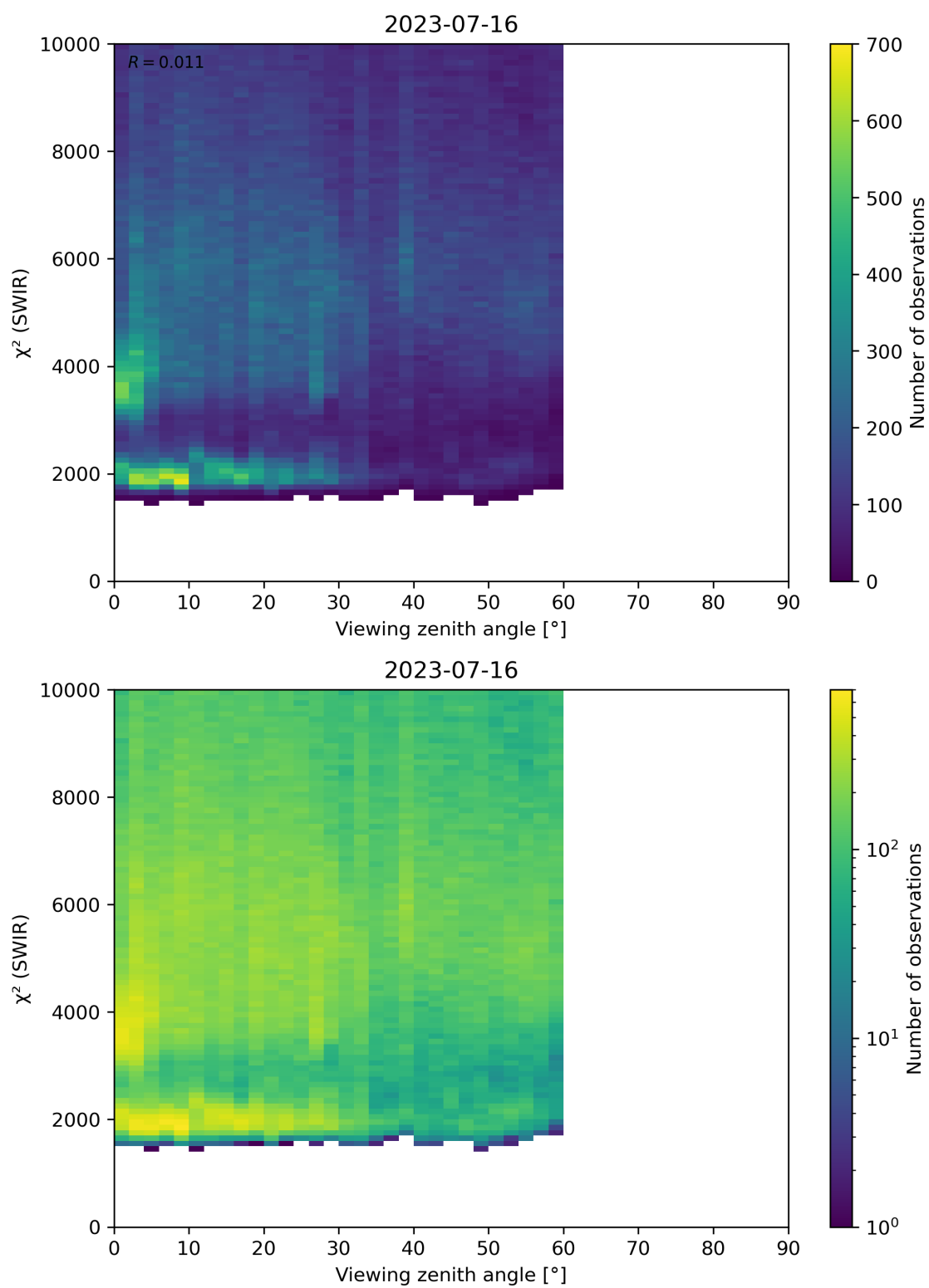
Figure 106: Scatter density plot of “Viewing zenith angle” against “ \chi^2 (SWIR)” for 2023-07-15 to 2023-07-17.
