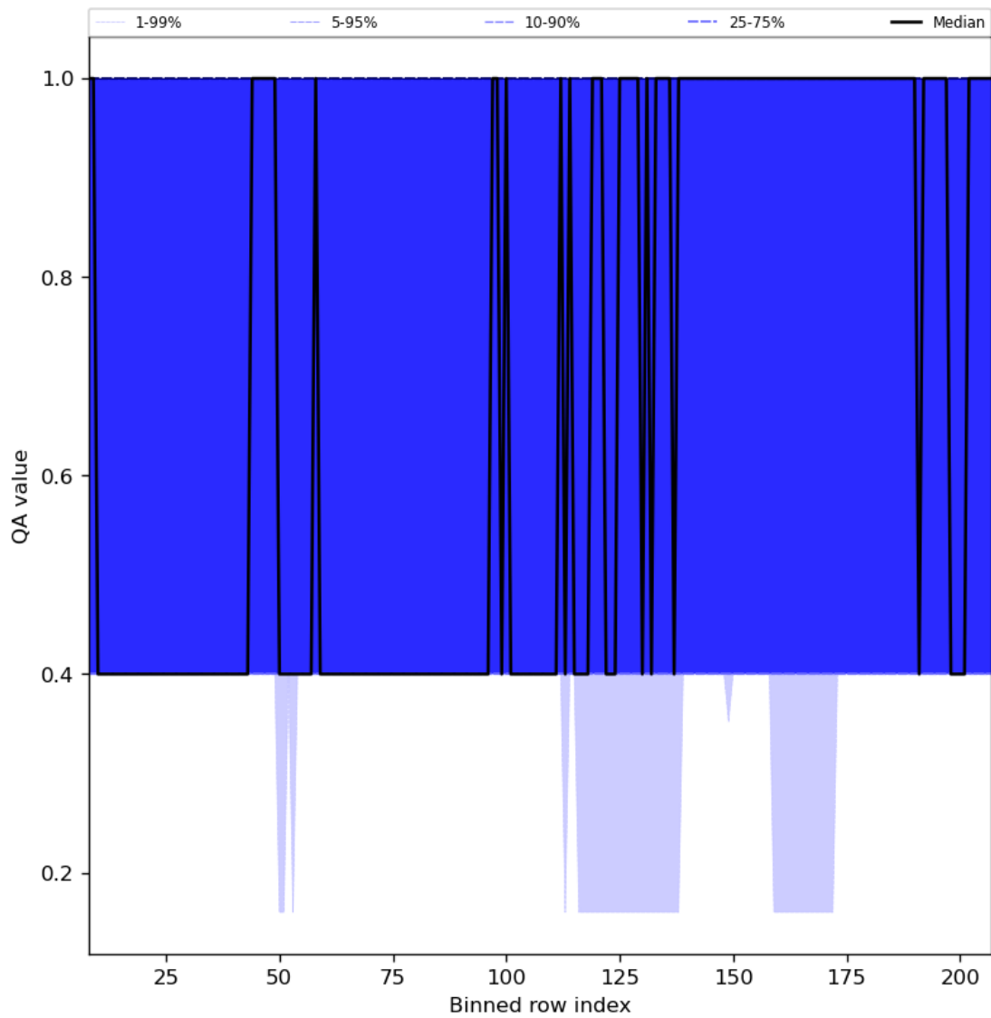
Figure 33: Along track statistics of “QA value” for 2023-07-15 to 2023-07-17
