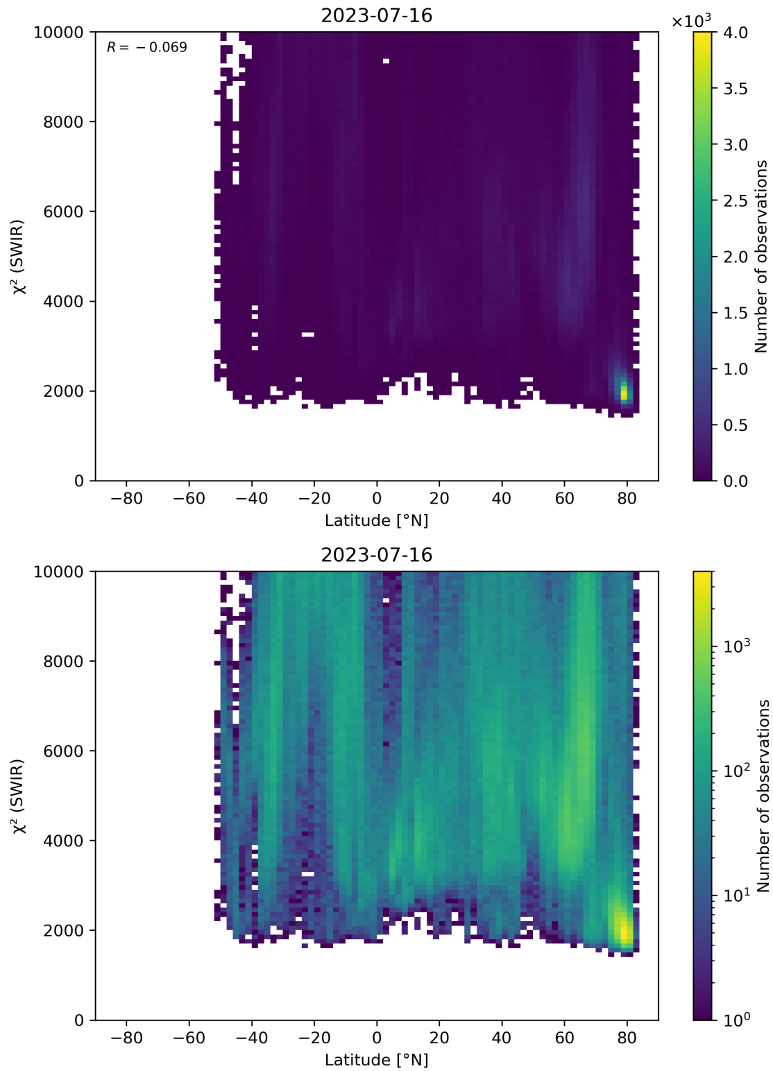
Figure 54: Scatter density plot of “Latitude” against “ \chi^2 (SWIR)” for 2023-07-15 to 2023-07-17.
