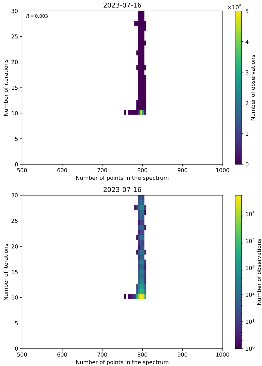
Figure 92: Scatter density plot of “Number of points in the spectrum” against “Number of iterations” for 2023-07-15 to 2023-07-17.
