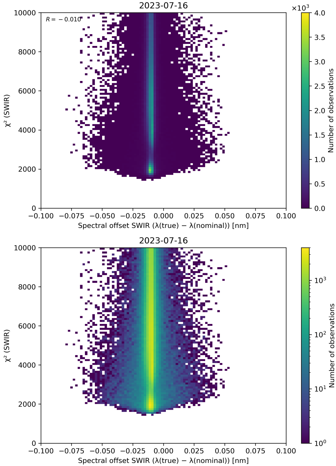
Figure 118: Scatter density plot of “Spectral offset SWIR ( \lambda(\text{true}) - \lambda(\text{nominal}) )” against “ \chi^2 (SWIR)” for 2023-07-15 to 2023-07-17.
