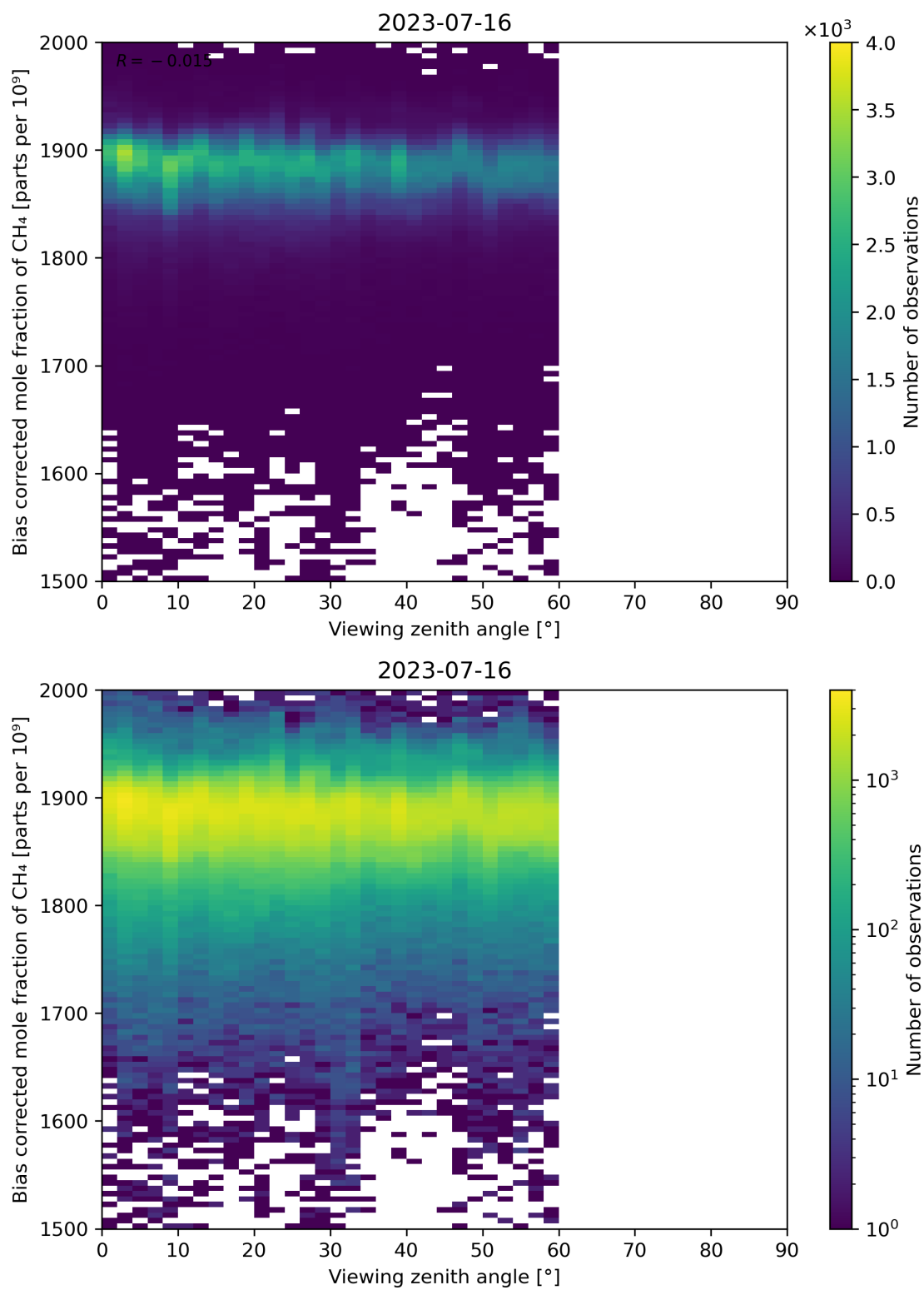
Figure 111: Scatter density plot of “Viewing zenith angle” against “Bias corrected mole fraction of CH 4 ” for 2023-07-15 to 2023-07-17.
