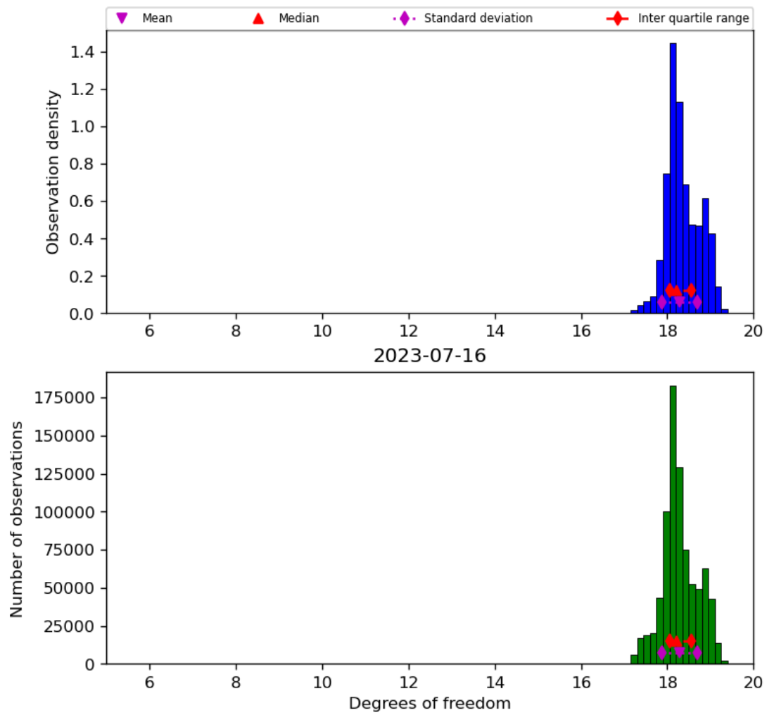
Figure 30: Histogram of “Degrees of freedom” for 2023-07-15 to 2023-07-17
