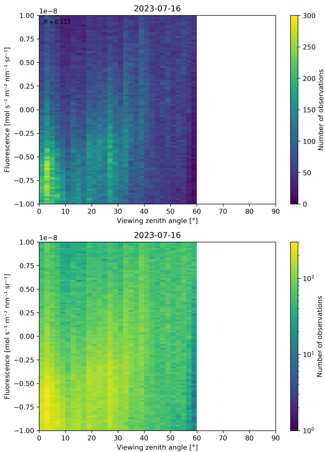
Figure 108: Scatter density plot of “Viewing zenith angle” against “Fluorescence” for 2023-07-15 to 2023-07-17.
