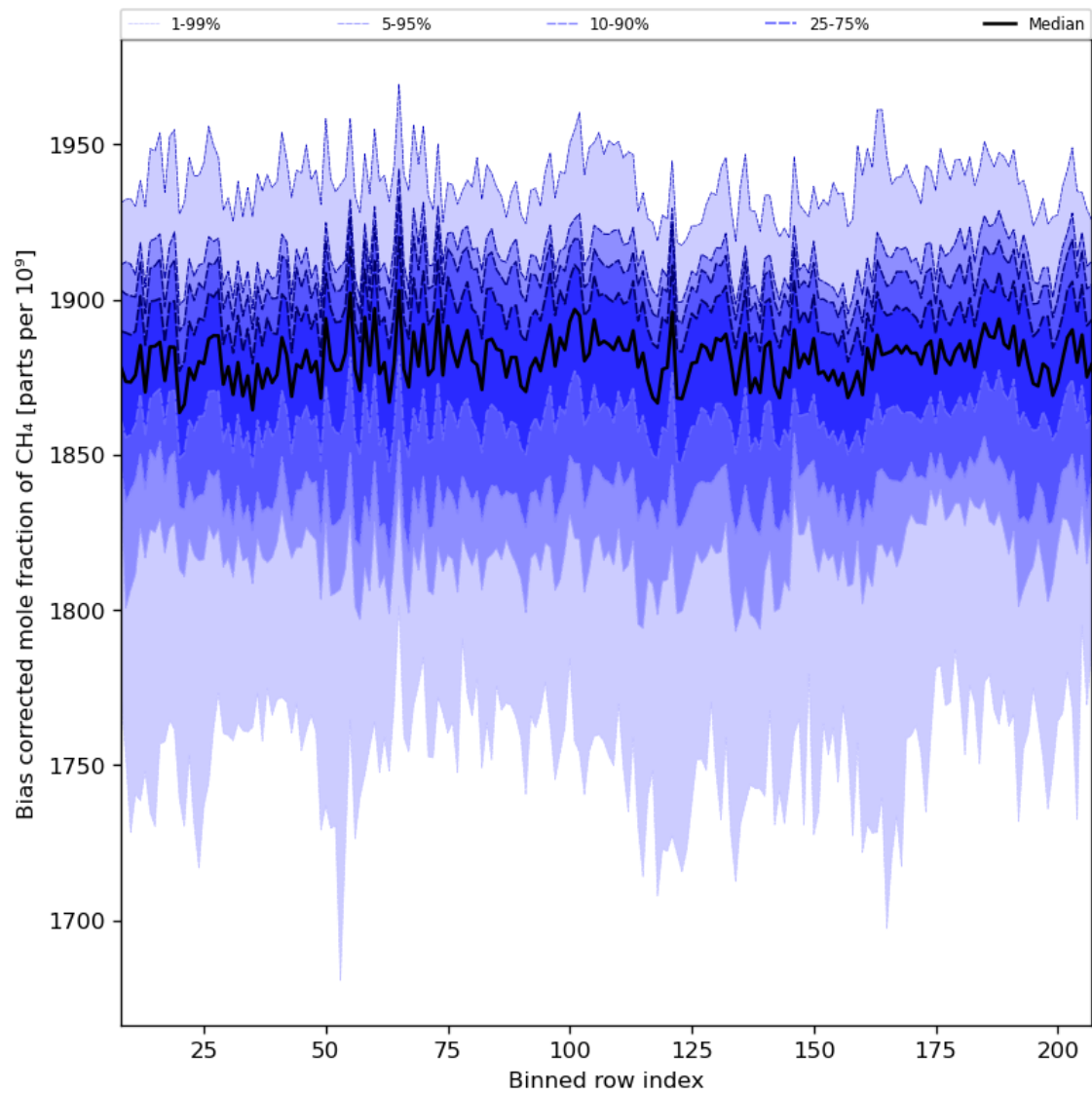
Figure 36: Along track statistics of “Bias corrected mole fraction of CH 4 ” for 2023-07-15 to 2023-07-17
