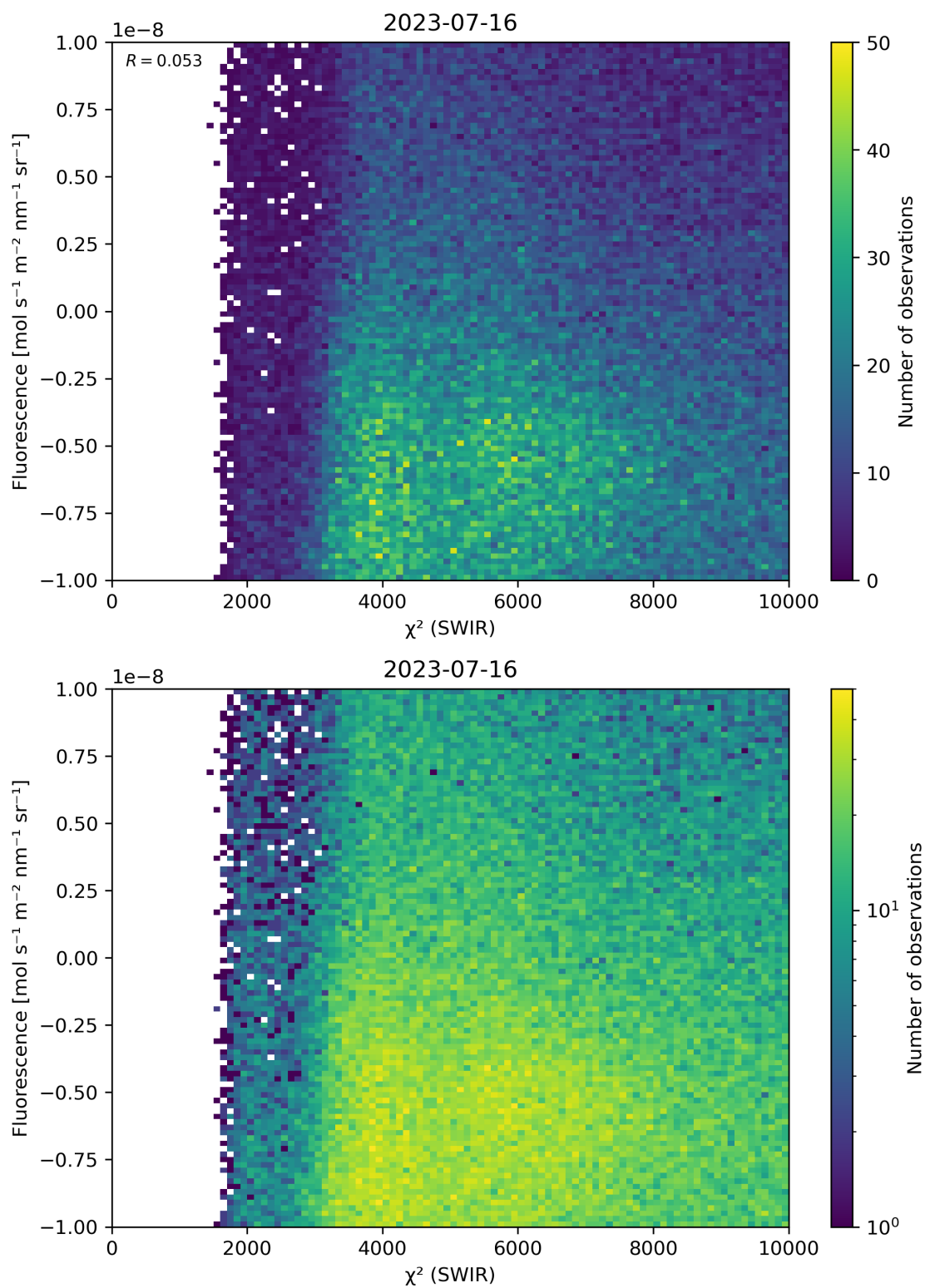
Figure 49: Scatter density plot of “ \chi^2 (SWIR)” against “Fluorescence” for 2023-07-15 to 2023-07-17.
