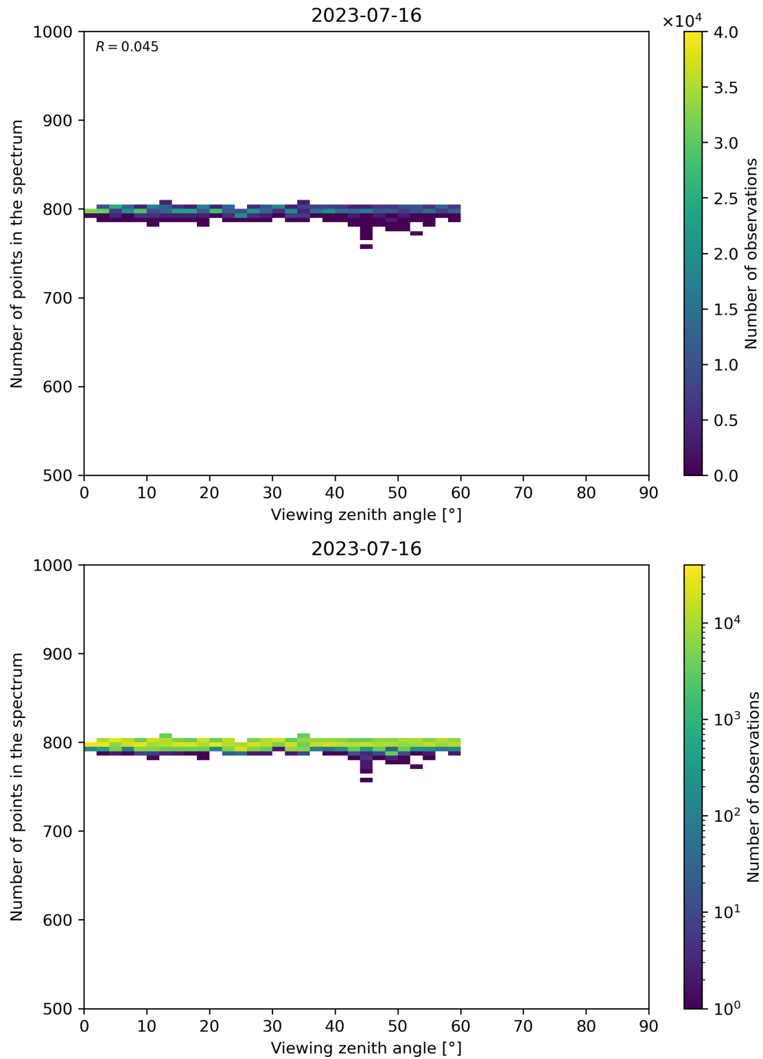
Figure 114: Scatter density plot of “Viewing zenith angle” against “Number of points in the spectrum” for 2023-07-15 to 2023-07-17.
