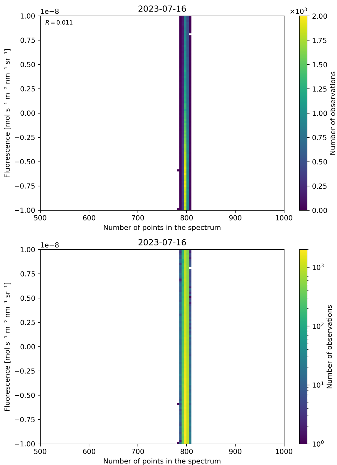
Figure 91: Scatter density plot of “Number of points in the spectrum” against “Fluorescence” for 2023-07-15 to 2023-07-17.
