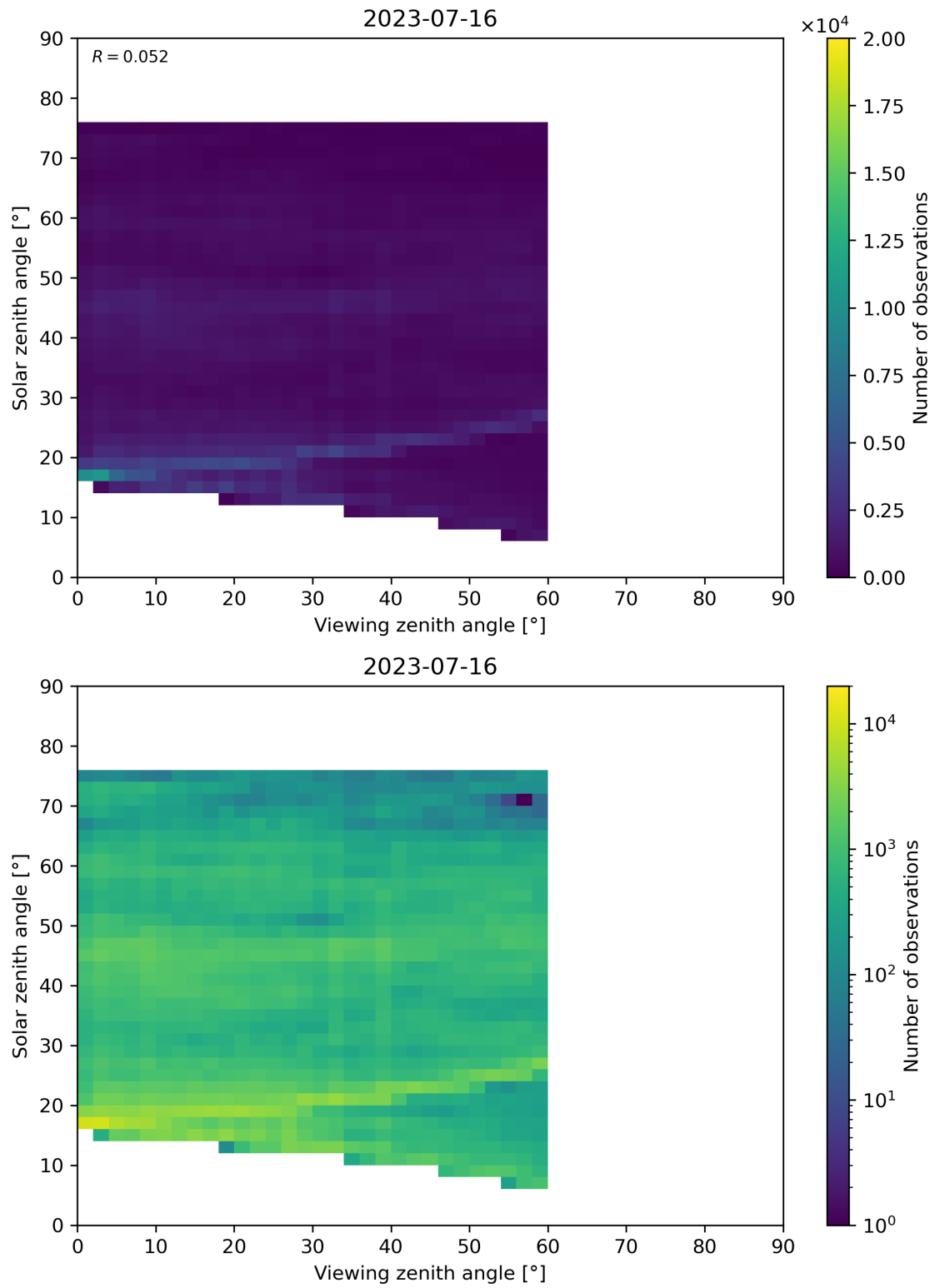
Figure 115: Scatter density plot of “Viewing zenith angle” against “Solar zenith angle” for 2023-07-15 to 2023-07-17.
