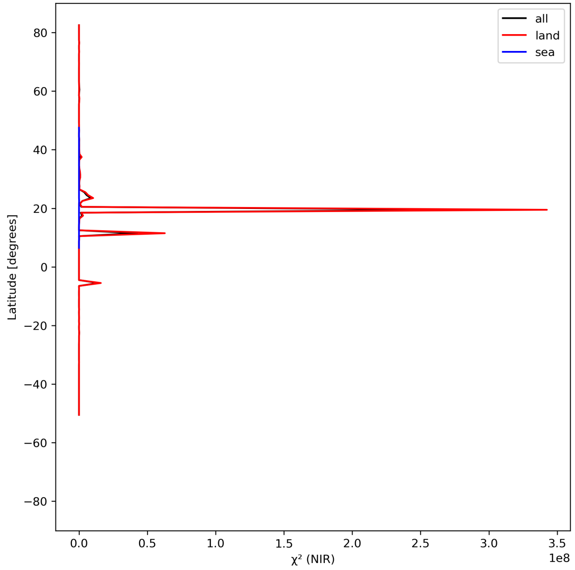
Figure 18: Zonal average of “ \chi^2 (NIR)” for 2023-07-15 to 2023-07-17.
