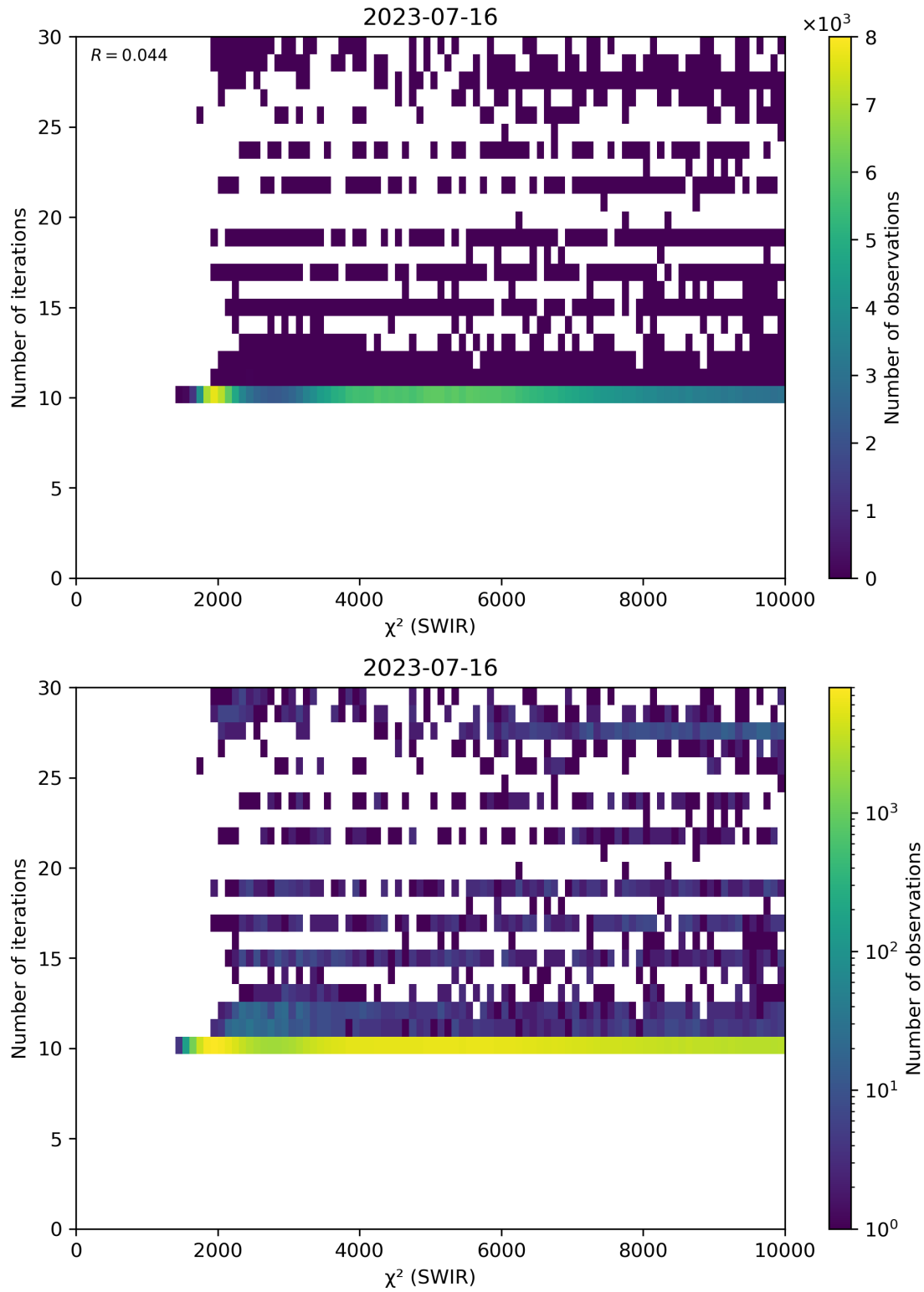
Figure 50: Scatter density plot of “ \chi^2 (SWIR)” against “Number of iterations” for 2023-07-15 to 2023-07-17.
