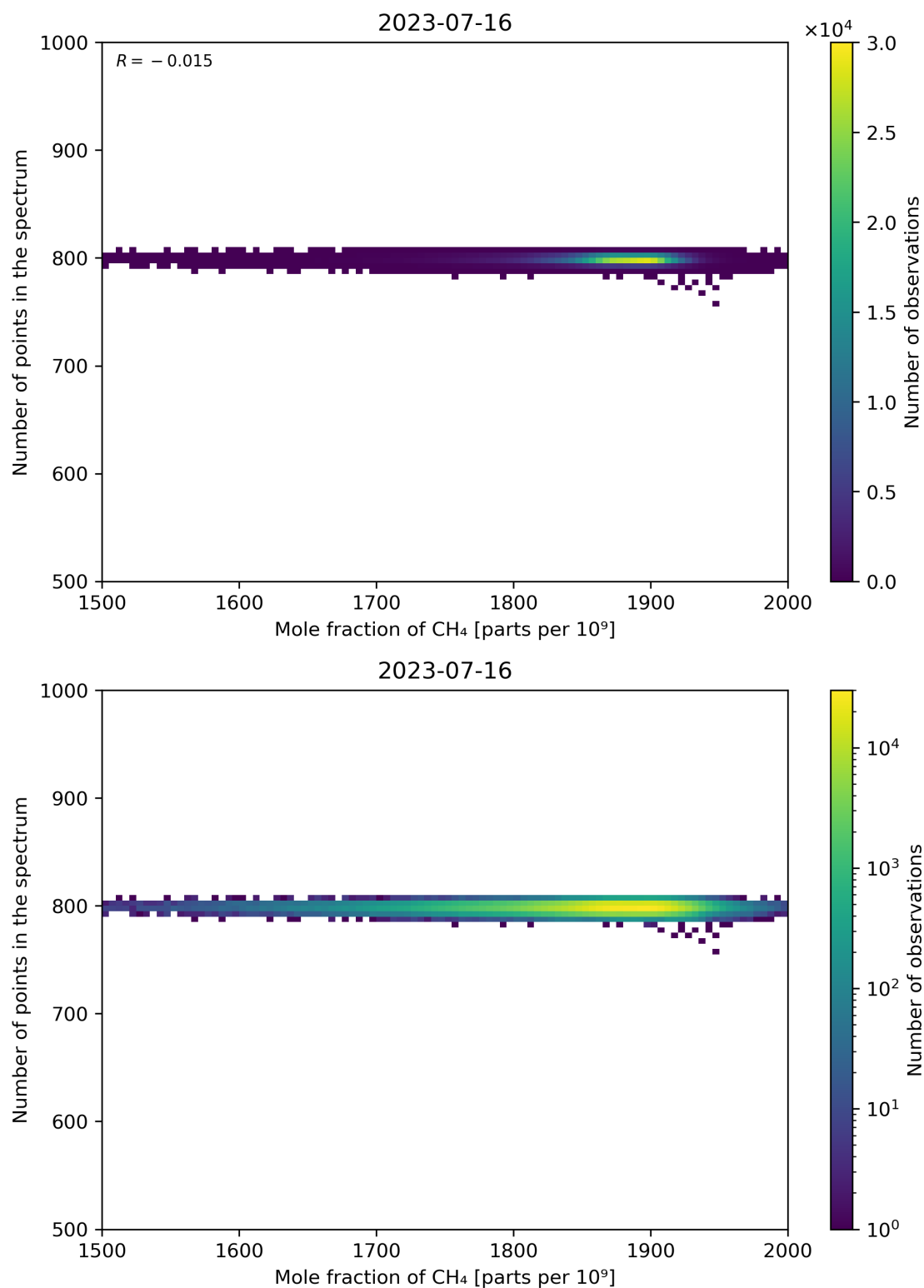
Figure 77: Scatter density plot of “Mole fraction of CH 4 ” against “Number of points in the spectrum” for 2023-07-15 to 2023-07-17.
