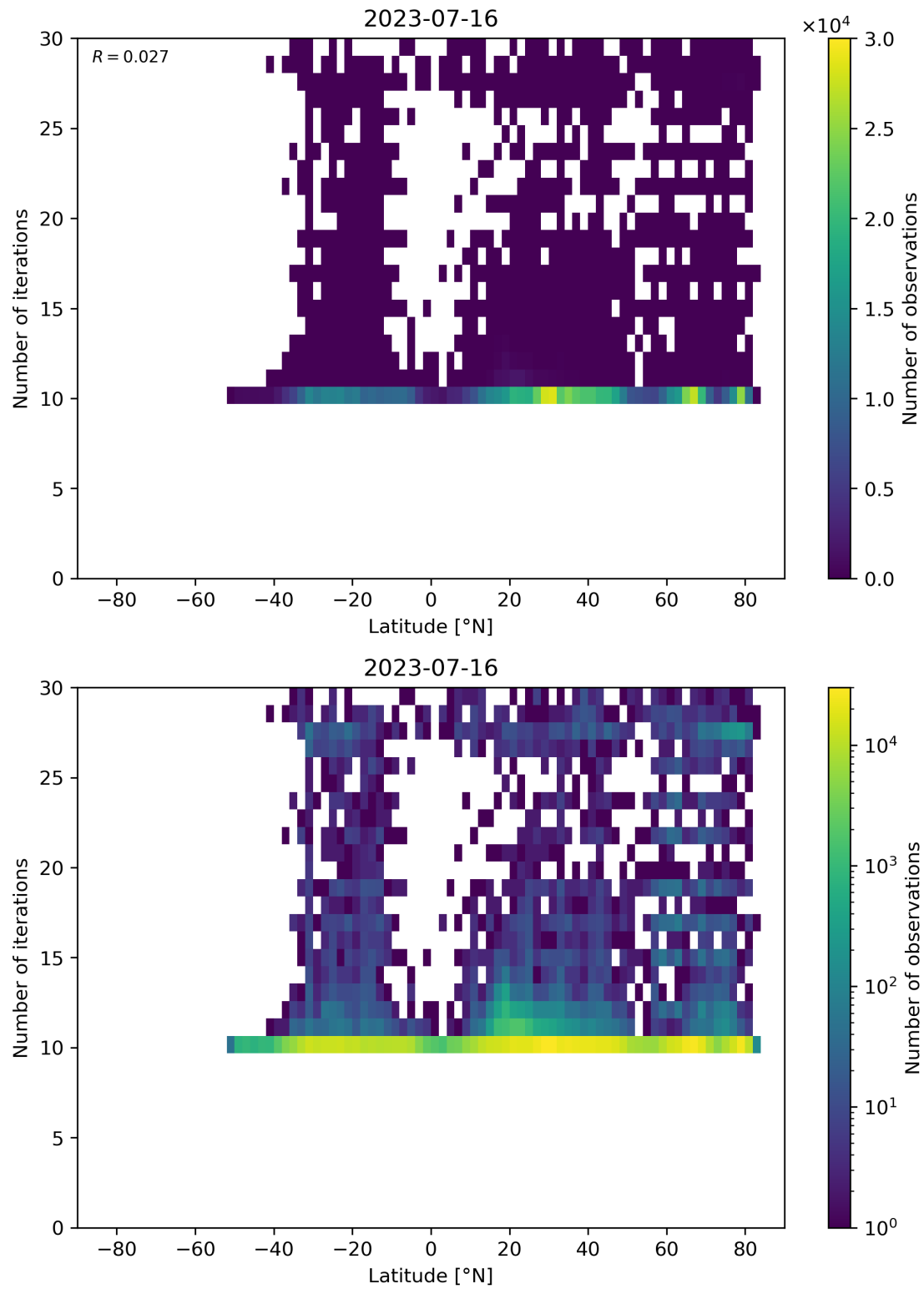
Figure 60: Scatter density plot of “Latitude” against “Number of iterations” for 2023-07-15 to 2023-07-17.
