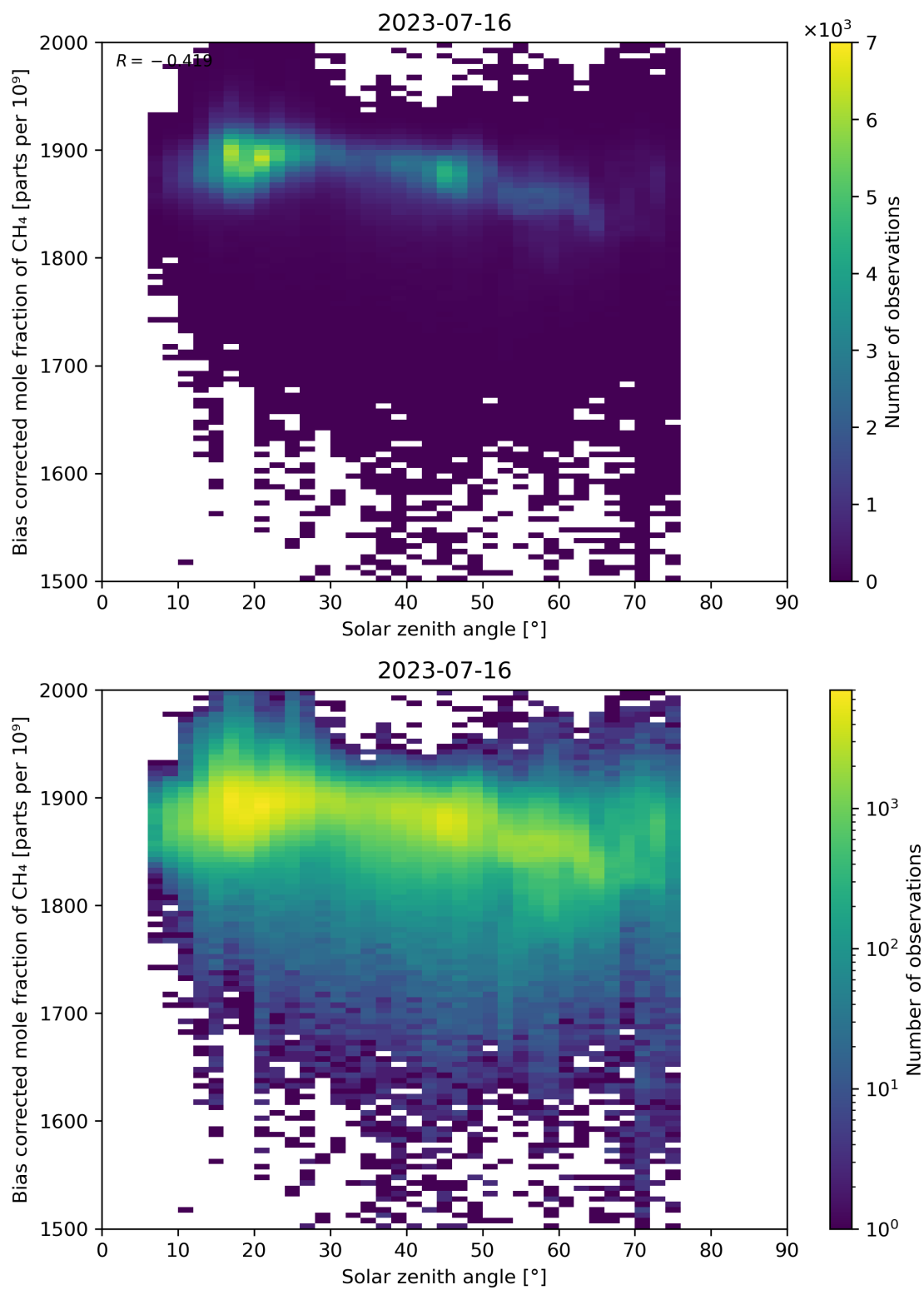
Figure 100: Scatter density plot of “Solar zenith angle” against “Bias corrected mole fraction of CH 4 ” for 2023-07-15 to 2023-07-17.
