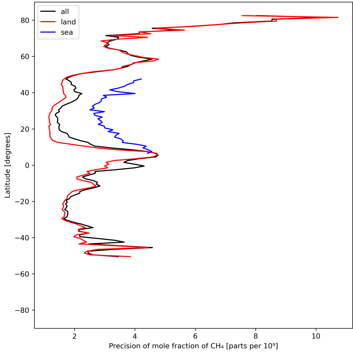
Figure 13: Zonal average of “Precision of mole fraction of CH 4 ” for 2023-07-15 to 2023-07-17.
