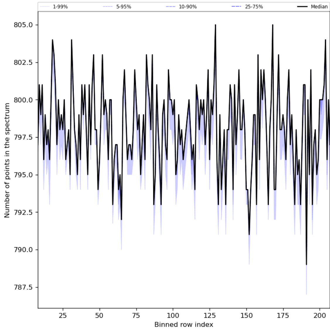
Figure 37: Along track statistics of “Number of points in the spectrum” for 2023-07-15 to 2023-07-17
