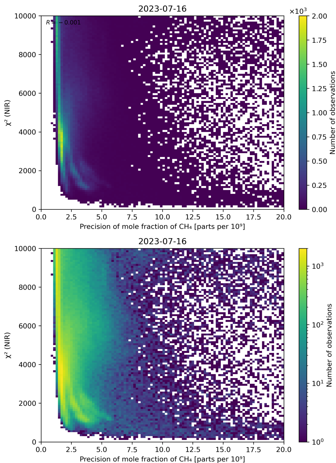
Figure 78: Scatter density plot of “Precision of mole fraction of \text{CH}_4 ” against “ \chi^2 (NIR)” for 2023-07-15 to 2023-07-17.
