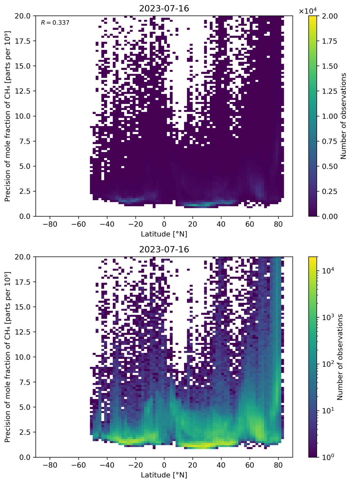
Figure 59: Scatter density plot of “Latitude” against “Precision of mole fraction of \text{CH}_4 ” for 2023-07-15 to 2023-07-17.
