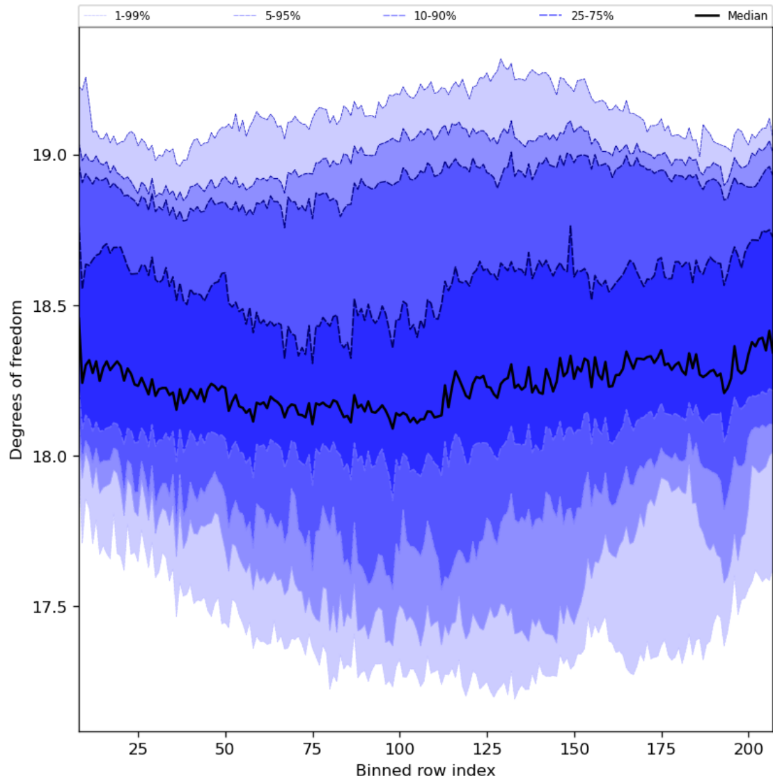
Figure 41: Along track statistics of “Degrees of freedom” for 2023-07-15 to 2023-07-17
