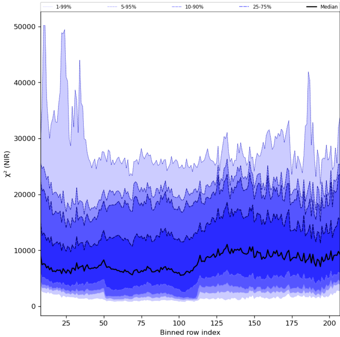
Figure 40: Along track statistics of “ \chi^2 (NIR)” for 2023-07-15 to 2023-07-17
