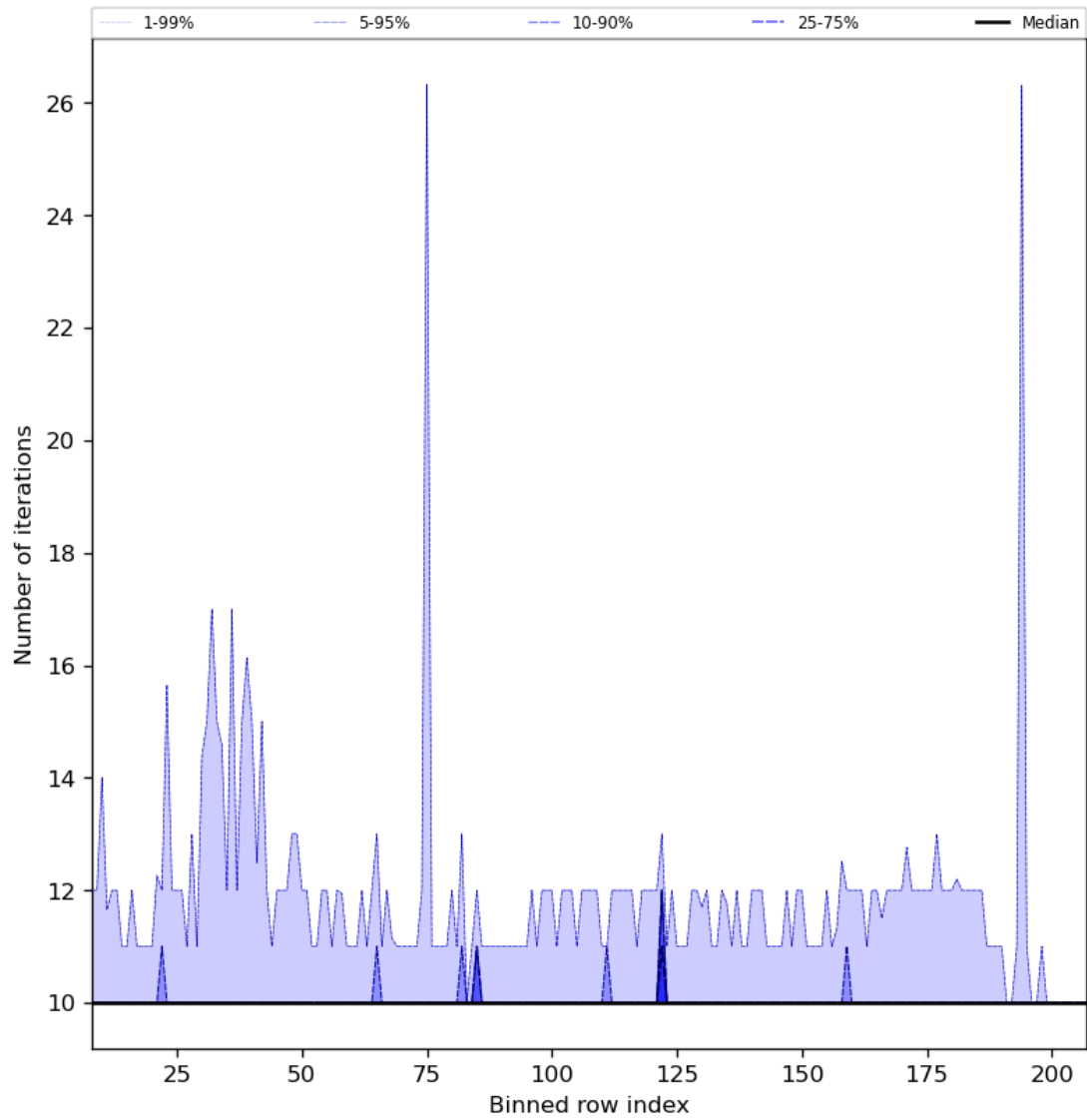
Figure 42: Along track statistics of “Number of iterations” for 2023-07-15 to 2023-07-17
