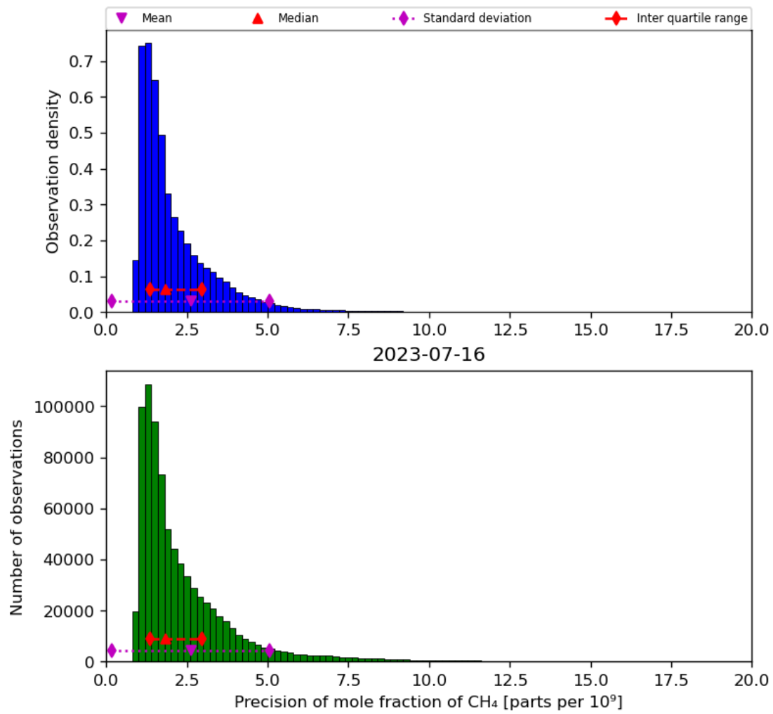
Figure 24: Histogram of “Precision of mole fraction of CH 4 ” for 2023-07-15 to 2023-07-17
