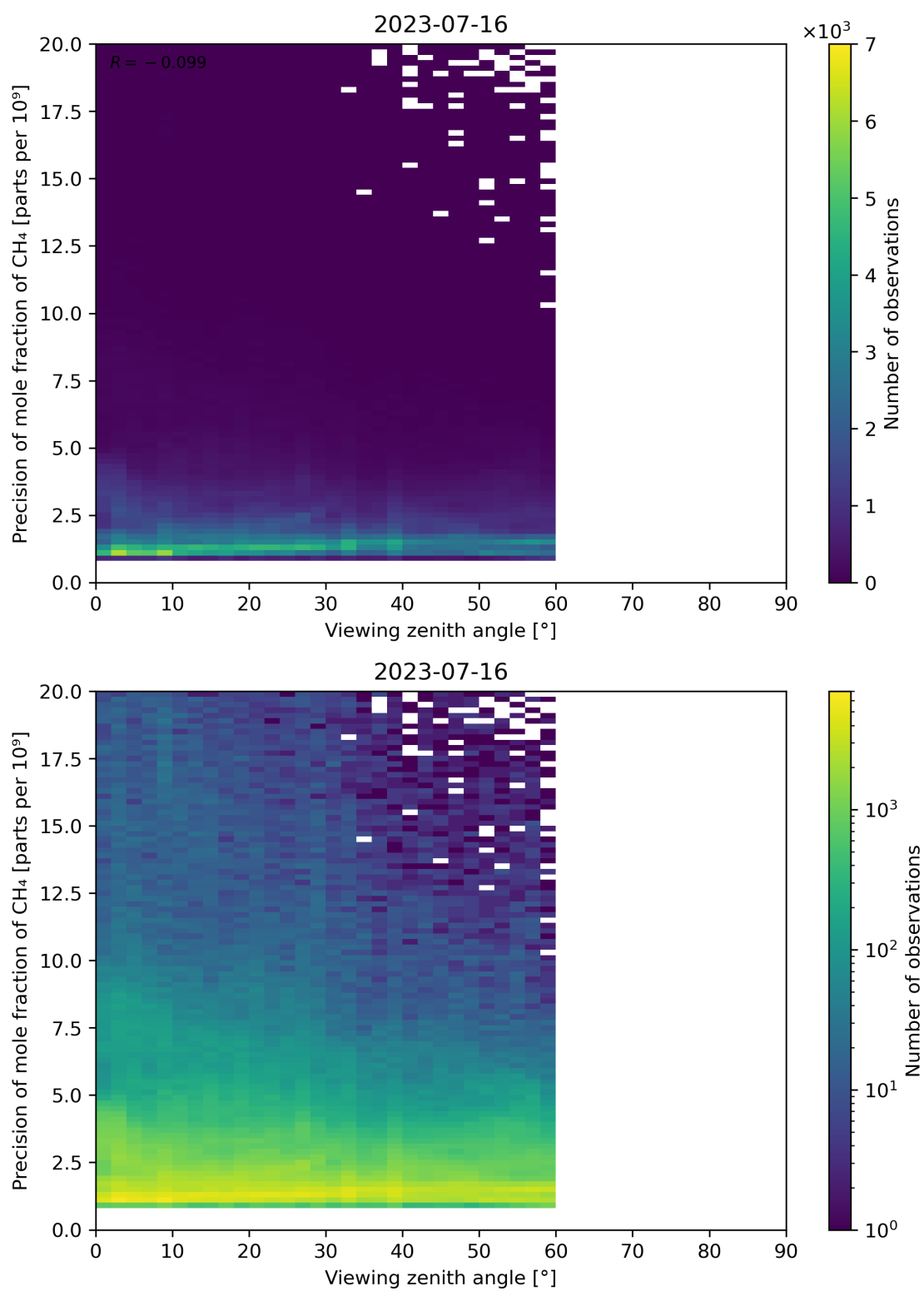
Figure 112: Scatter density plot of “Viewing zenith angle” against “Precision of mole fraction of \text{CH}_4 ” for 2023-07-15 to 2023-07-17.
