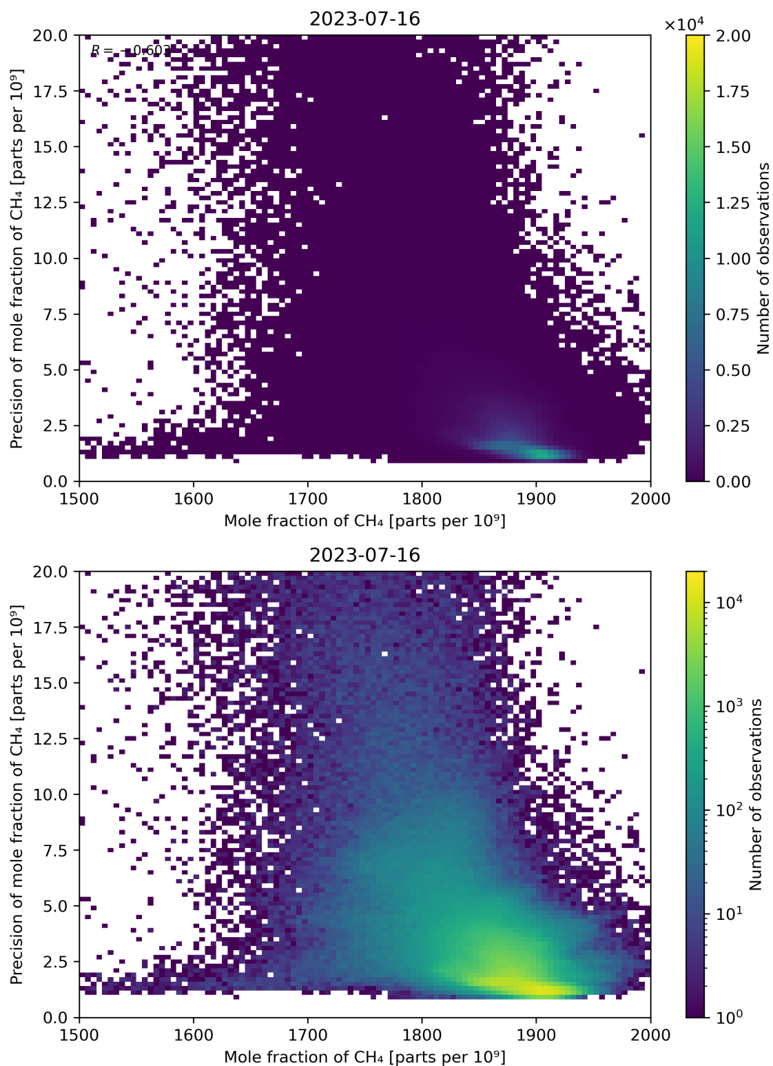
Figure 75: Scatter density plot of “Mole fraction of CH 4 ” against “Precision of mole fraction of CH 4 ” for 2023-07-15 to 2023-07-17.
