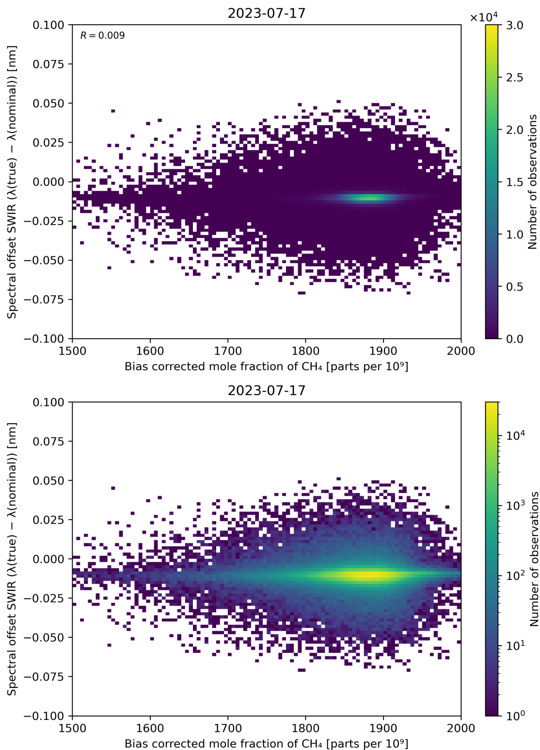
Figure 69: Scatter density plot of “Bias corrected mole fraction of \text{CH}_4 ” against “Spectral offset SWIR ( \lambda(\text{true}) - \lambda(\text{nominal}) )” for 2023-07-16 to 2023-07-18.
