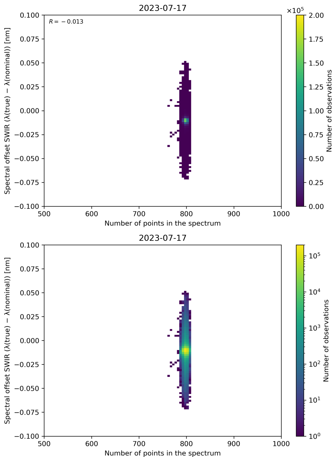
Figure 93: Scatter density plot of “Number of points in the spectrum” against “Spectral offset SWIR ( \lambda(\text{true}) - \lambda(\text{nominal}) )” for 2023-07-16 to 2023-07-18.
