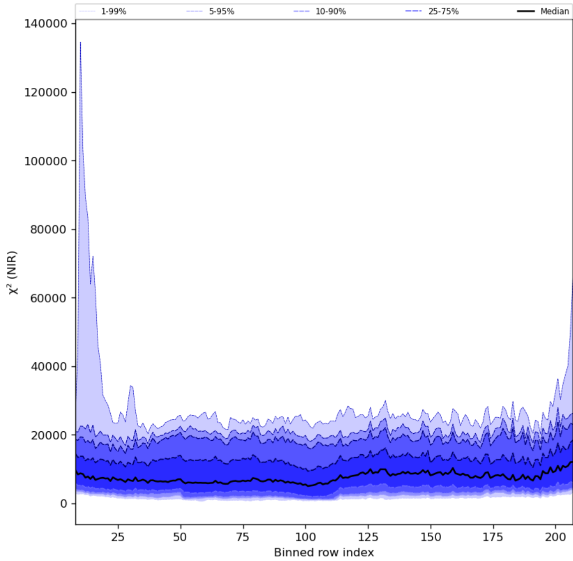
Figure 40: Along track statistics of “ \chi^2 (NIR)” for 2023-07-16 to 2023-07-18
