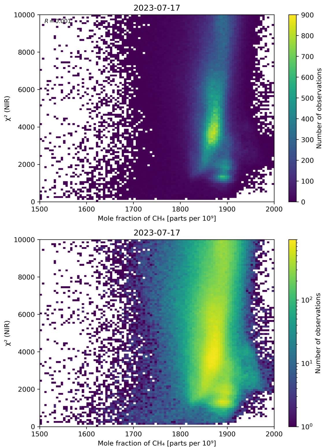
Figure 70: Scatter density plot of “Mole fraction of CH 4 ” against “ \chi^2 (NIR)” for 2023-07-16 to 2023-07-18.
