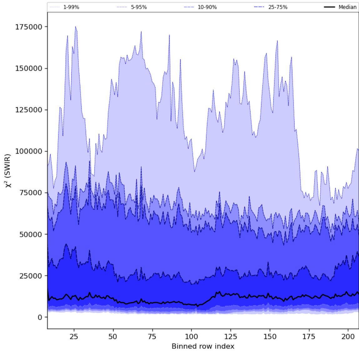
Figure 39: Along track statistics of “ \chi^2 (SWIR)” for 2023-07-16 to 2023-07-18
