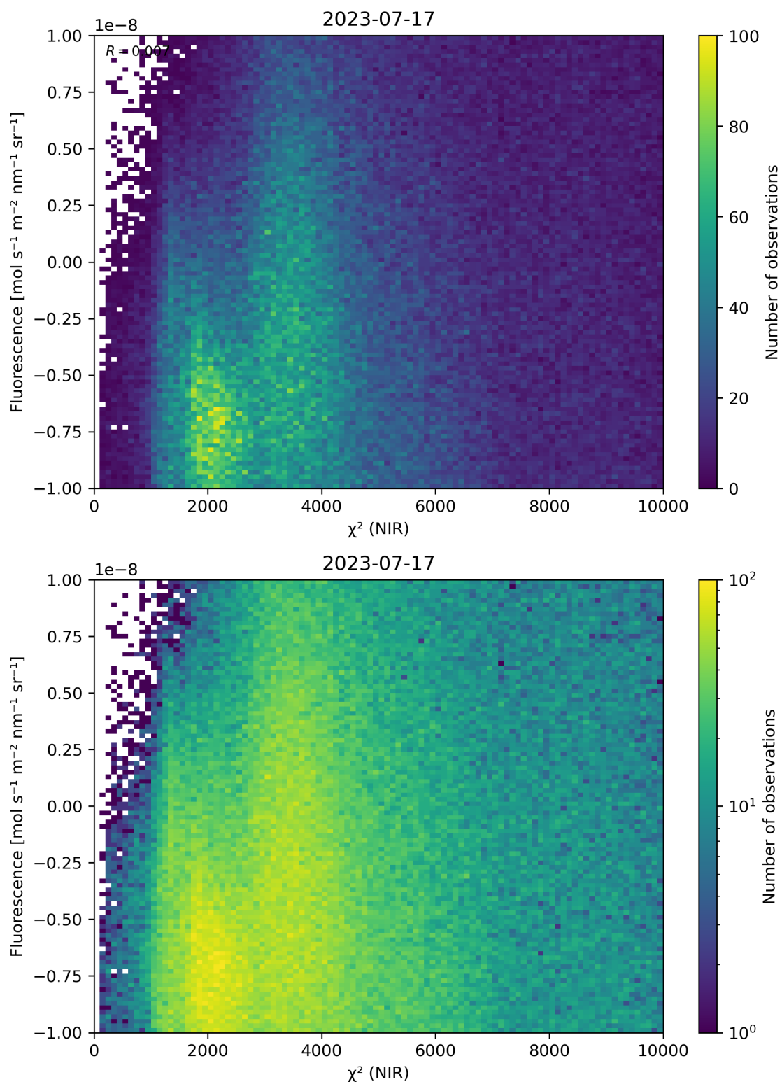
Figure 45: Scatter density plot of “ \chi^2 (NIR)” against “Fluorescence” for 2023-07-16 to 2023-07-18.
