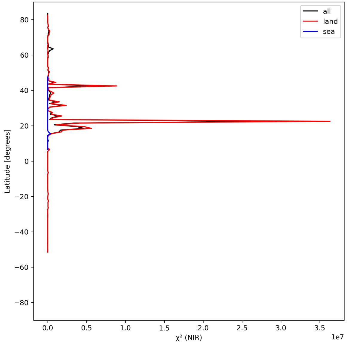
Figure 18: Zonal average of “ \chi^2 (NIR)” for 2023-07-16 to 2023-07-18.
