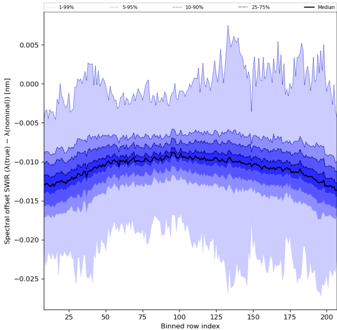
Figure 38: Along track statistics of “Spectral offset SWIR ( \lambda(\text{true}) - \lambda(\text{nominal}) )” for 2023-07-16 to 2023-07-18
