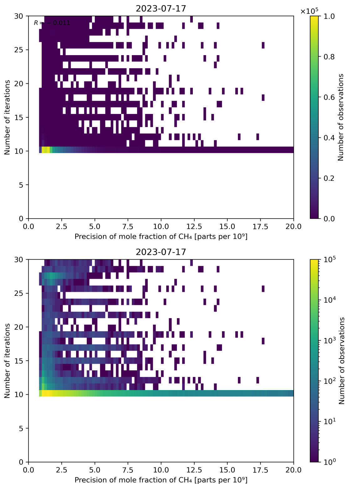
Figure 83: Scatter density plot of “Precision of mole fraction of CH 4 ” against “Number of iterations” for 2023-07-16 to 2023-07-18.
