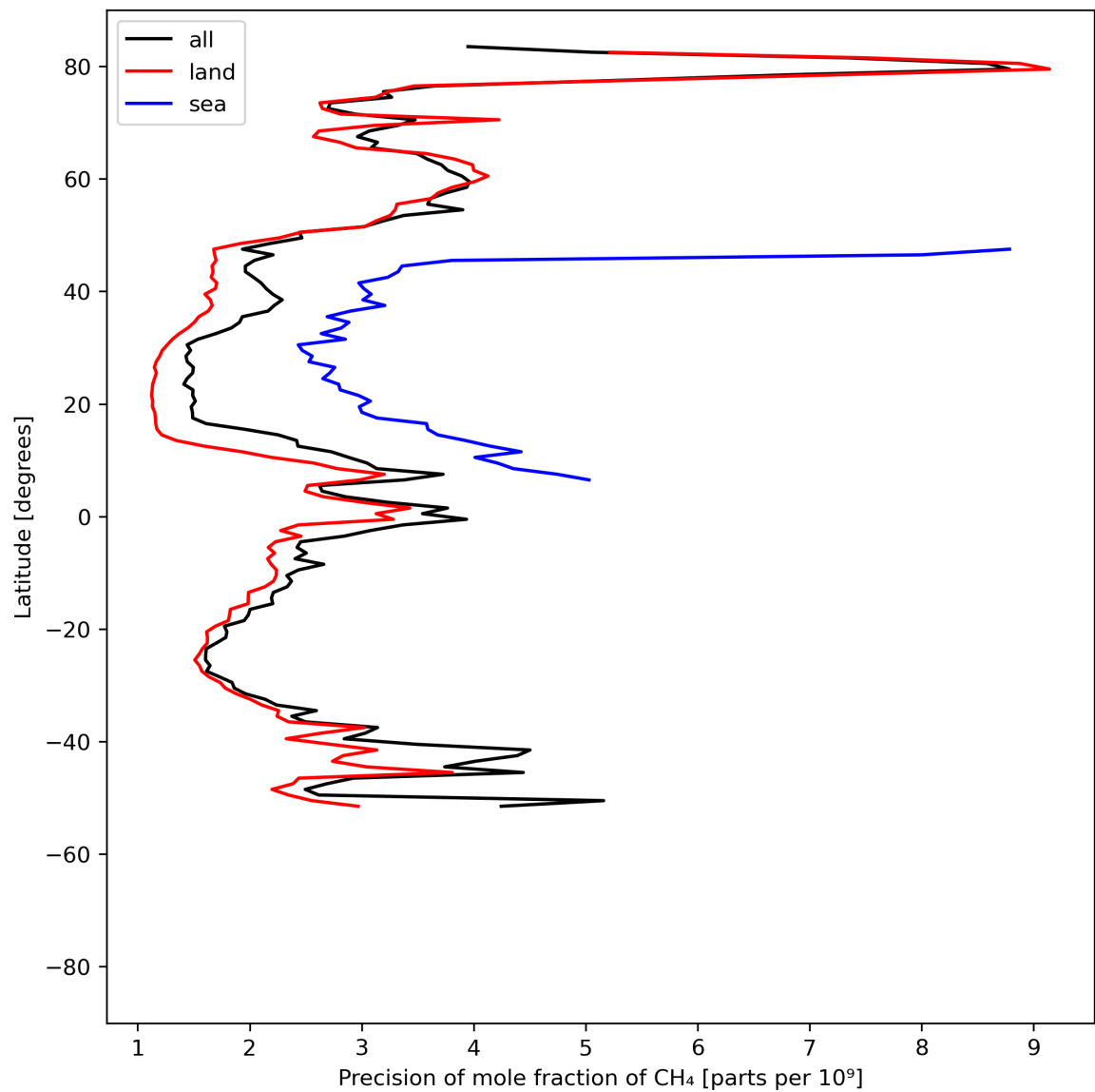
Figure 13: Zonal average of “Precision of mole fraction of CH 4 ” for 2023-07-16 to 2023-07-18.
