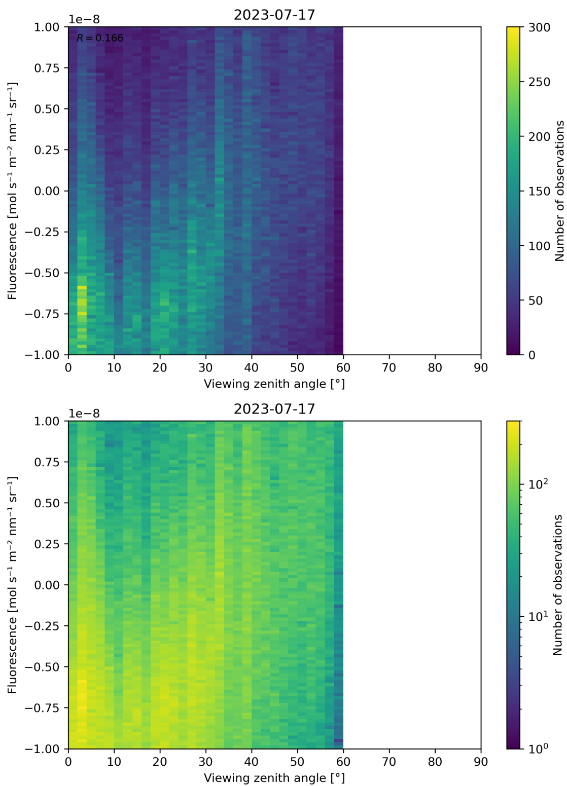
Figure 108: Scatter density plot of “Viewing zenith angle” against “Fluorescence” for 2023-07-16 to 2023-07-18.
