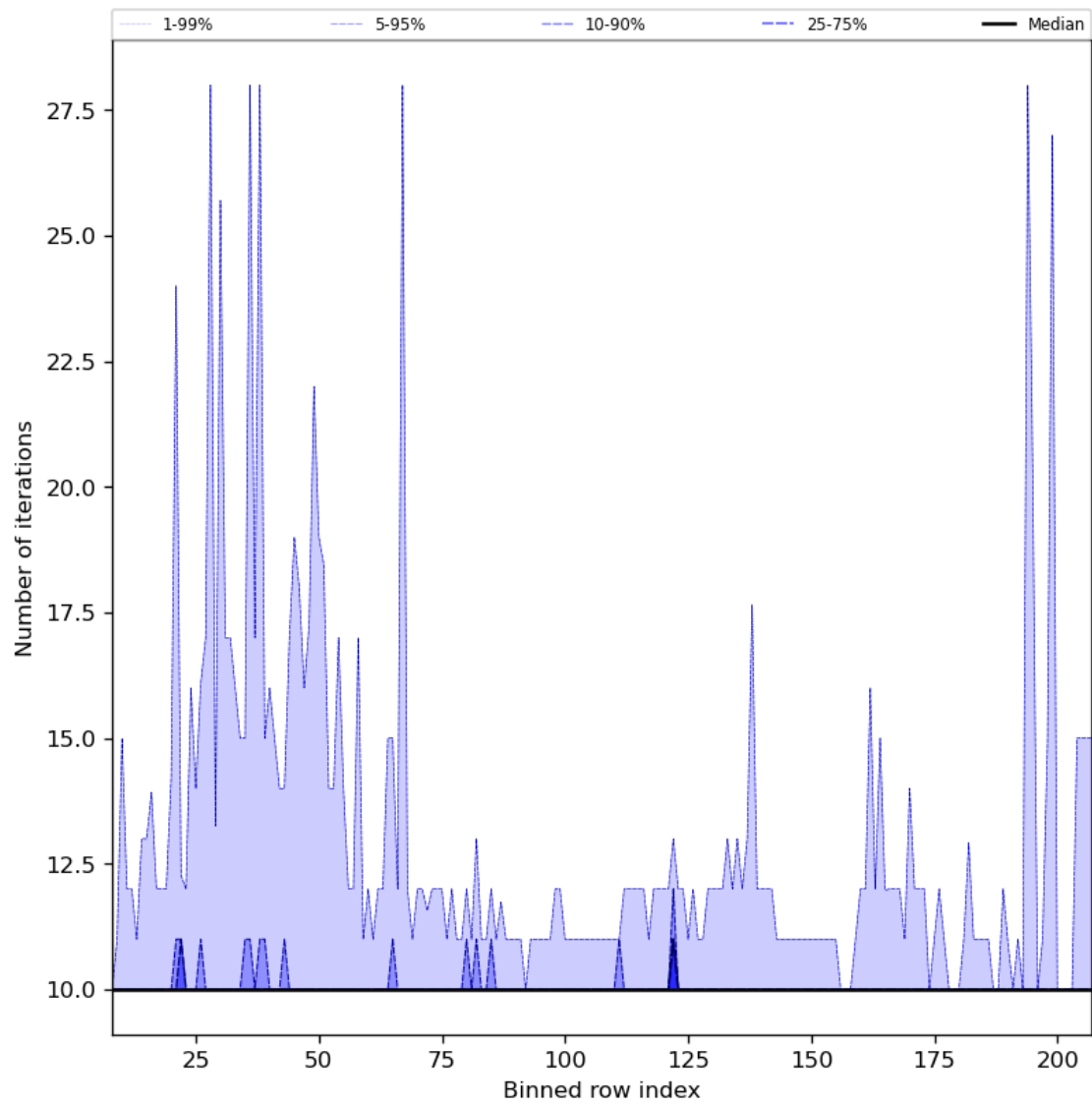
Figure 42: Along track statistics of “Number of iterations” for 2023-07-16 to 2023-07-18
