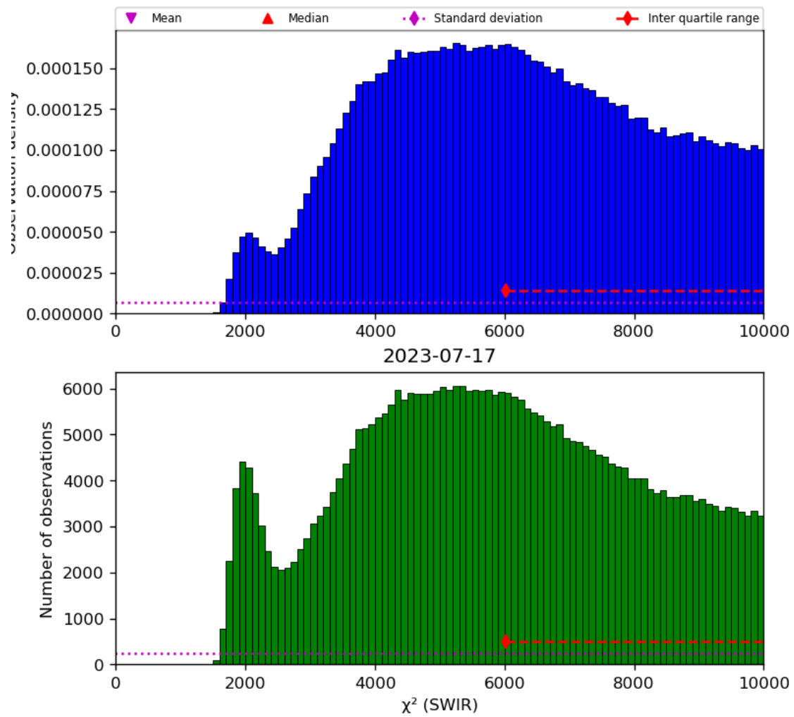
Figure 28: Histogram of “ \chi^2 (SWIR)” for 2023-07-16 to 2023-07-18
