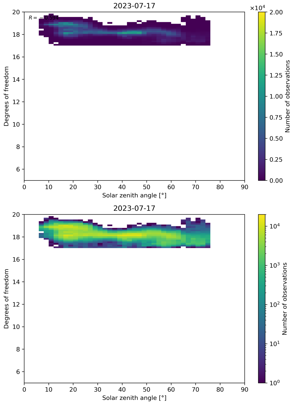
Figure 96: Scatter density plot of “Solar zenith angle” against “Degrees of freedom” for 2023-07-16 to 2023-07-18.
