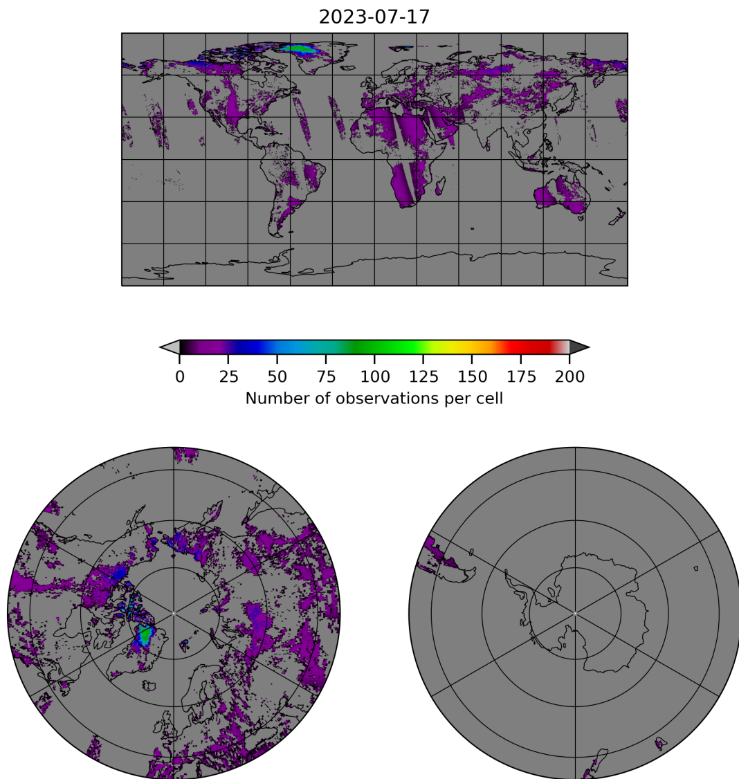
Figure 10: Map of the number of observations for 2023-07-16 to 2023-07-18
