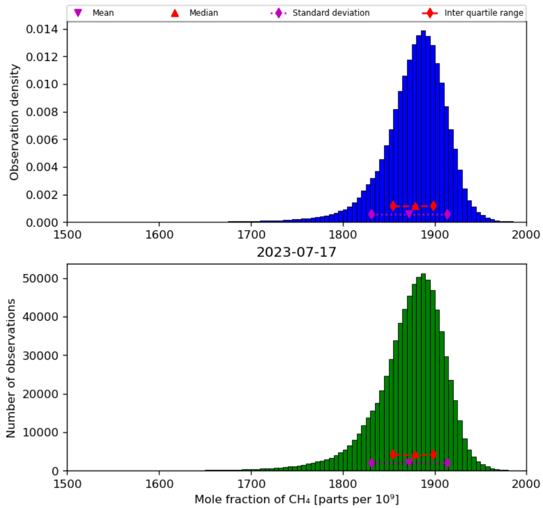
Figure 23: Histogram of “Mole fraction of CH 4 ” for 2023-07-16 to 2023-07-18
