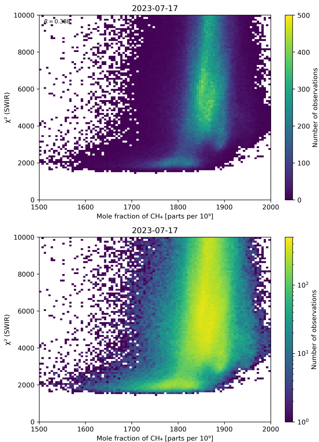
Figure 71: Scatter density plot of “Mole fraction of \text{CH}_4 ” against “ \chi^2 (SWIR)” for 2023-07-16 to 2023-07-18.
