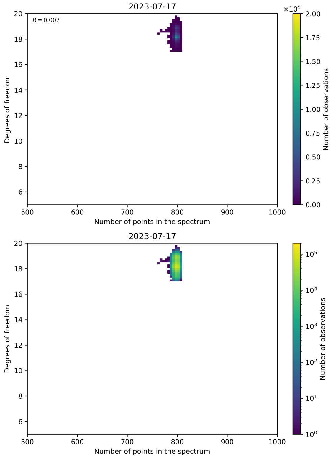
Figure 90: Scatter density plot of “Number of points in the spectrum” against “Degrees of freedom” for 2023-07-16 to 2023-07-18.
