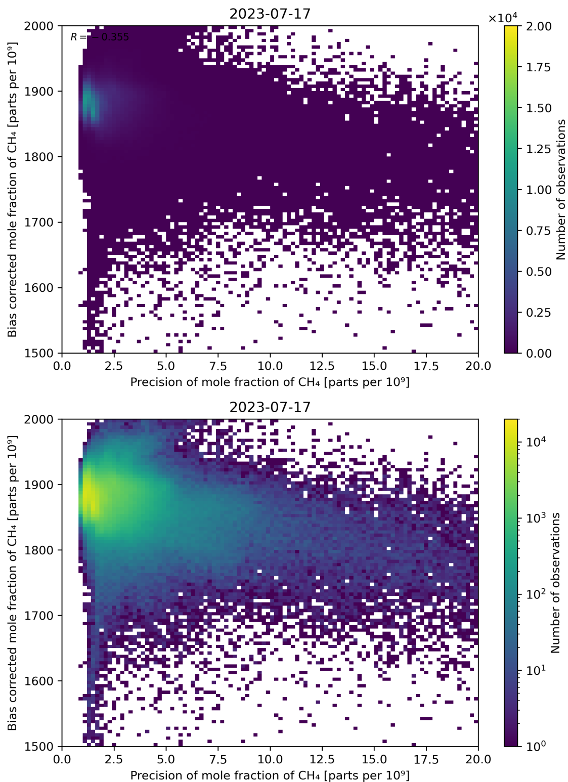
Figure 82: Scatter density plot of “Precision of mole fraction of CH 4 ” against “Bias corrected mole fraction of CH 4 ” for 2023-07-16 to 2023-07-18.
