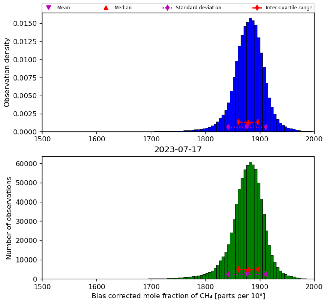
Figure 25: Histogram of “Bias corrected mole fraction of CH 4 ” for 2023-07-16 to 2023-07-18
