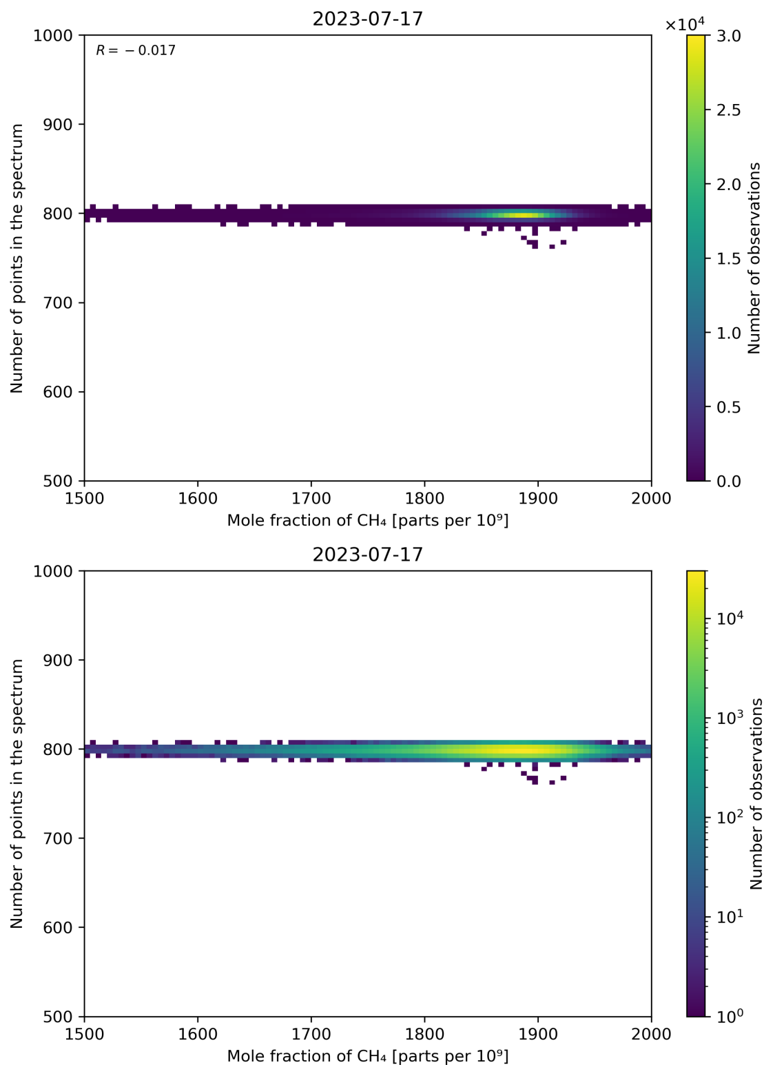
Figure 77: Scatter density plot of “Mole fraction of CH 4 ” against “Number of points in the spectrum” for 2023-07-16 to 2023-07-18.
