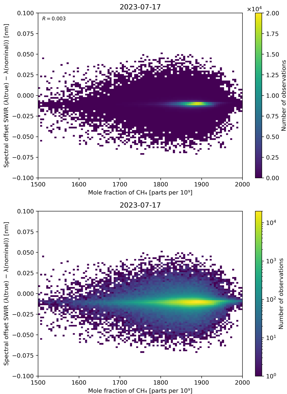
Figure 86: Scatter density plot of “Mole fraction of CH 4 ” against “Spectral offset SWIR ( \lambda(\text{true}) - \lambda(\text{nominal}) )” for 2023-07-16 to 2023-07-18.
