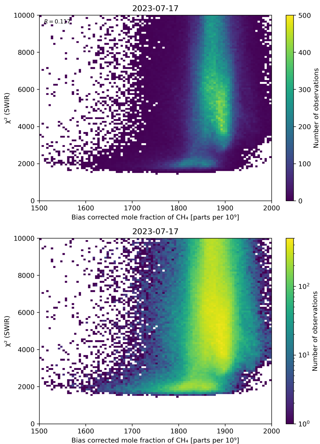
Figure 64: Scatter density plot of “Bias corrected mole fraction of CH 4 ” against “ \chi^2 (SWIR)” for 2023-07-16 to 2023-07-18.
