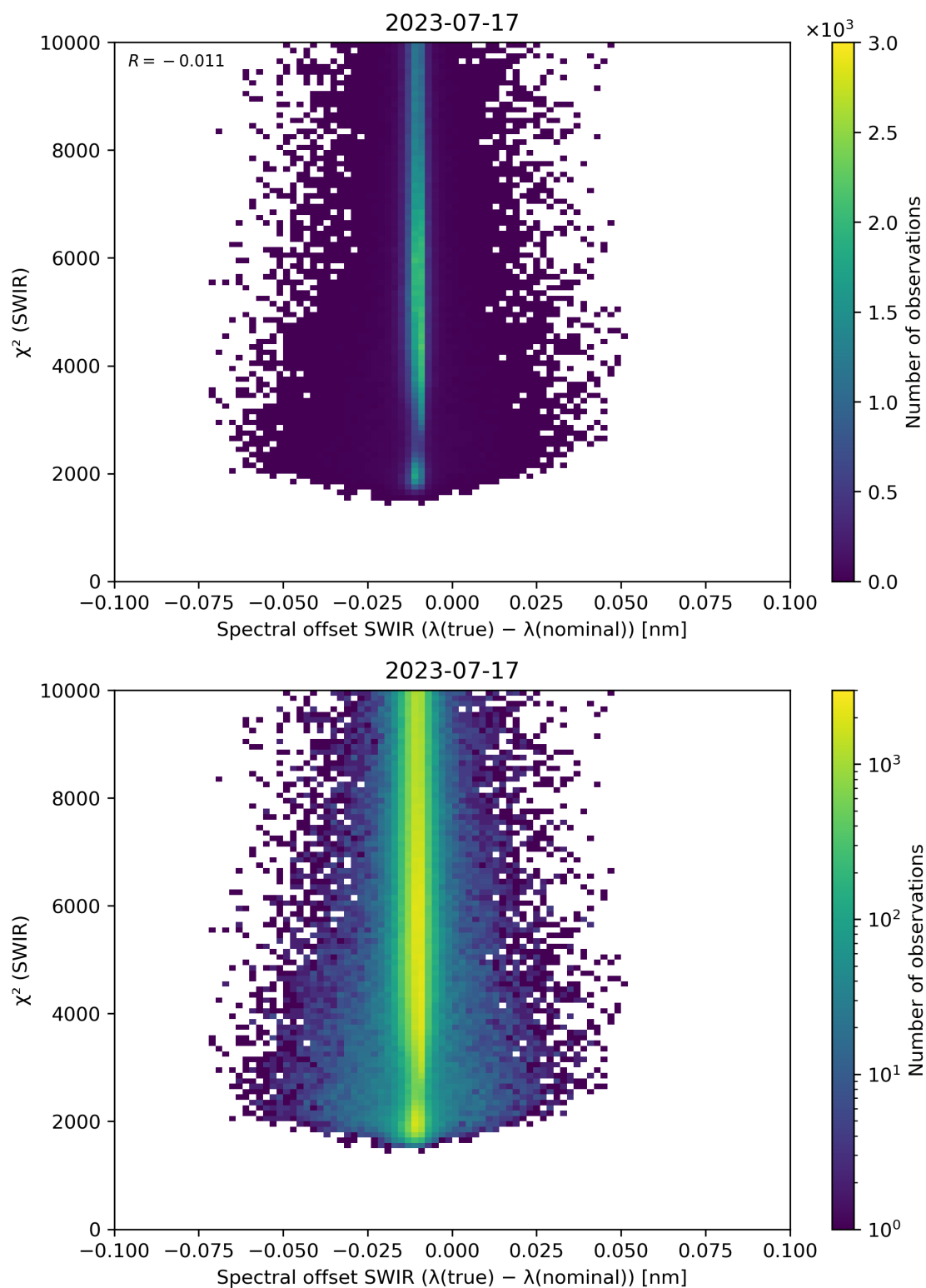
Figure 118: Scatter density plot of “Spectral offset SWIR ( \lambda(\text{true}) - \lambda(\text{nominal}) )” against “ \chi^2 (SWIR)” for 2023-07-16 to 2023-07-18.
