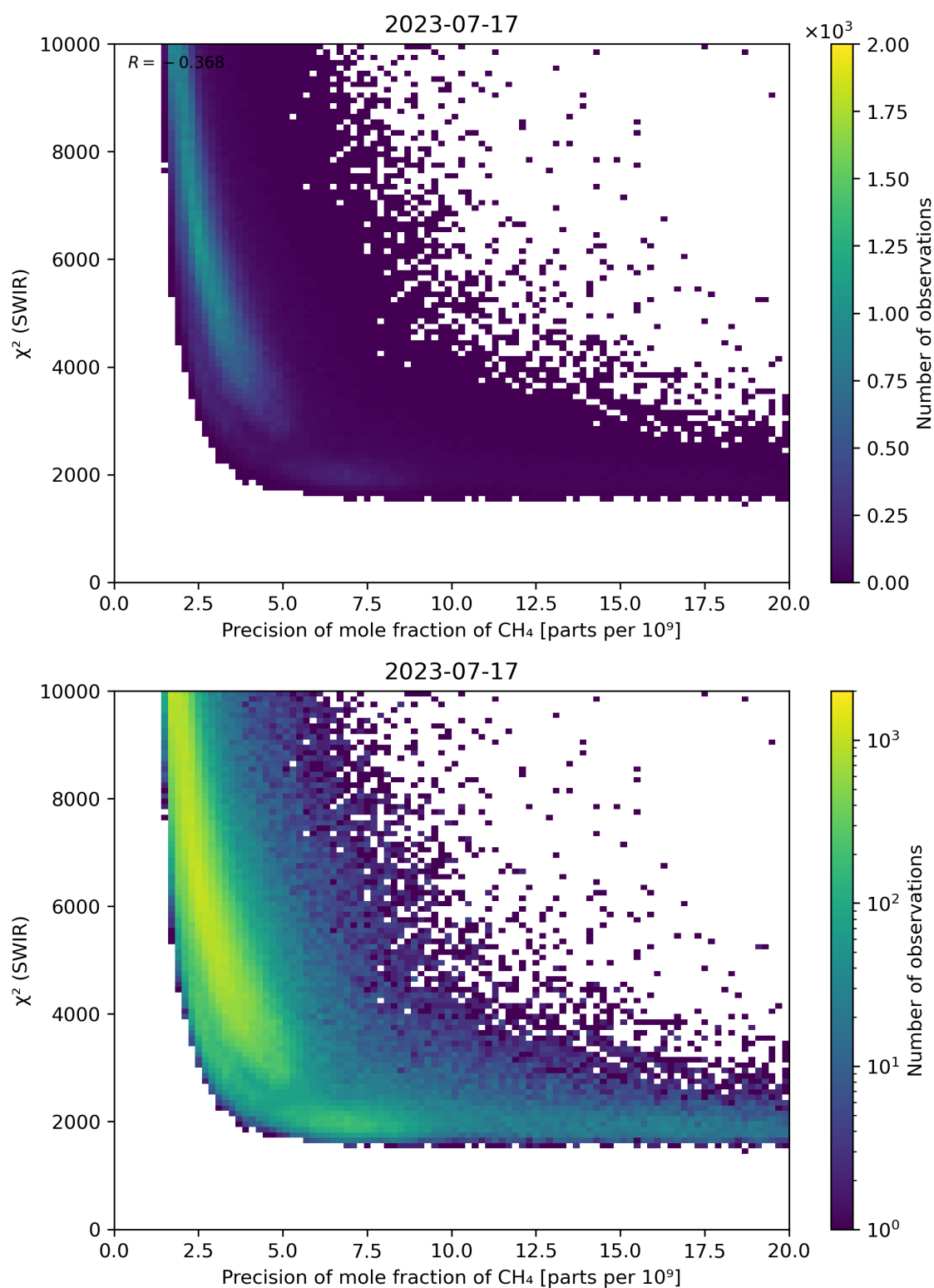
Figure 79: Scatter density plot of “Precision of mole fraction of \text{CH}_4 ” against “ \chi^2 (SWIR)” for 2023-07-16 to 2023-07-18.
