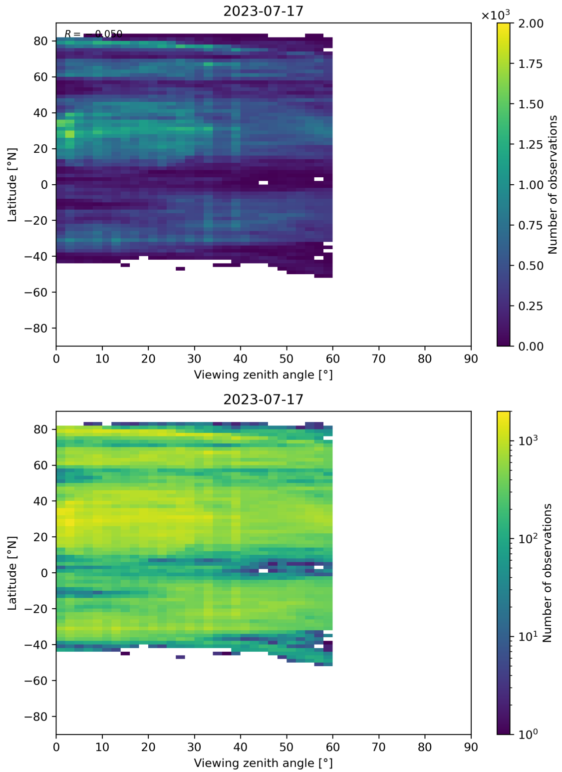
Figure 109: Scatter density plot of “Viewing zenith angle” against “Latitude” for 2023-07-16 to 2023-07-18.
