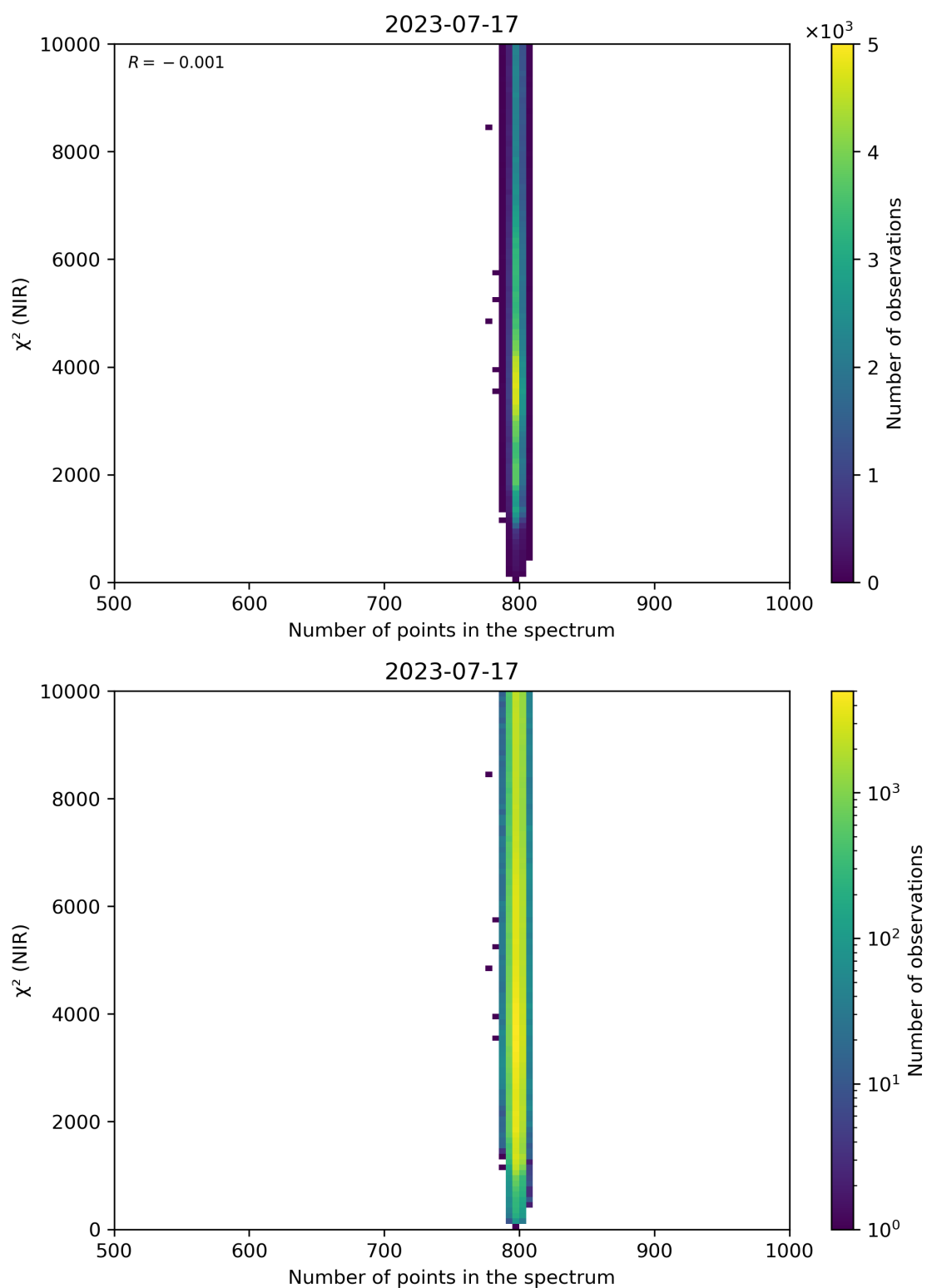
Figure 88: Scatter density plot of “Number of points in the spectrum” against “ \chi^2 (NIR)” for 2023-07-16 to 2023-07-18.
