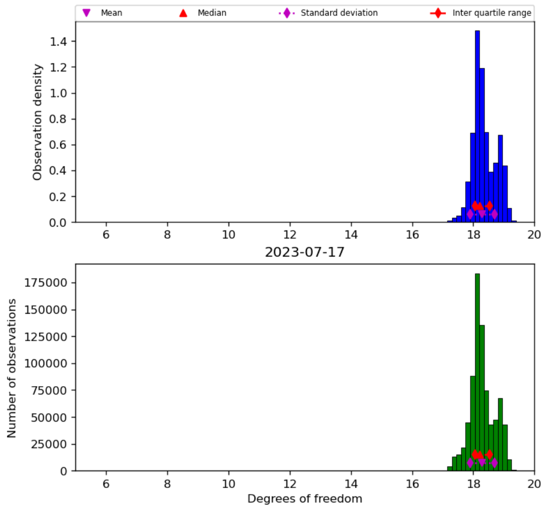
Figure 30: Histogram of “Degrees of freedom” for 2023-07-16 to 2023-07-18
