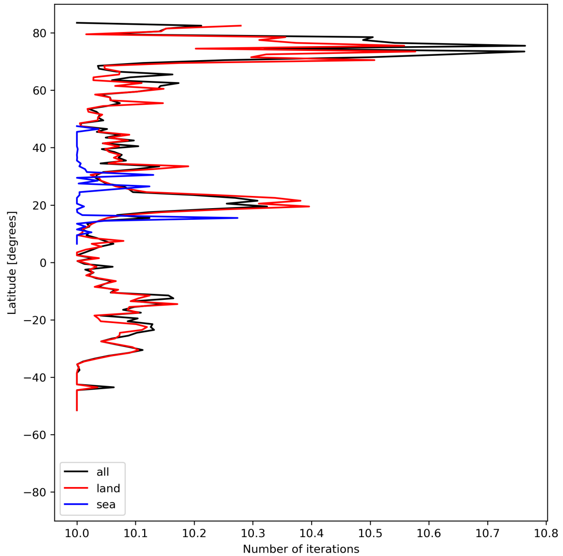
Figure 20: Zonal average of “Number of iterations” for 2023-07-16 to 2023-07-18.
