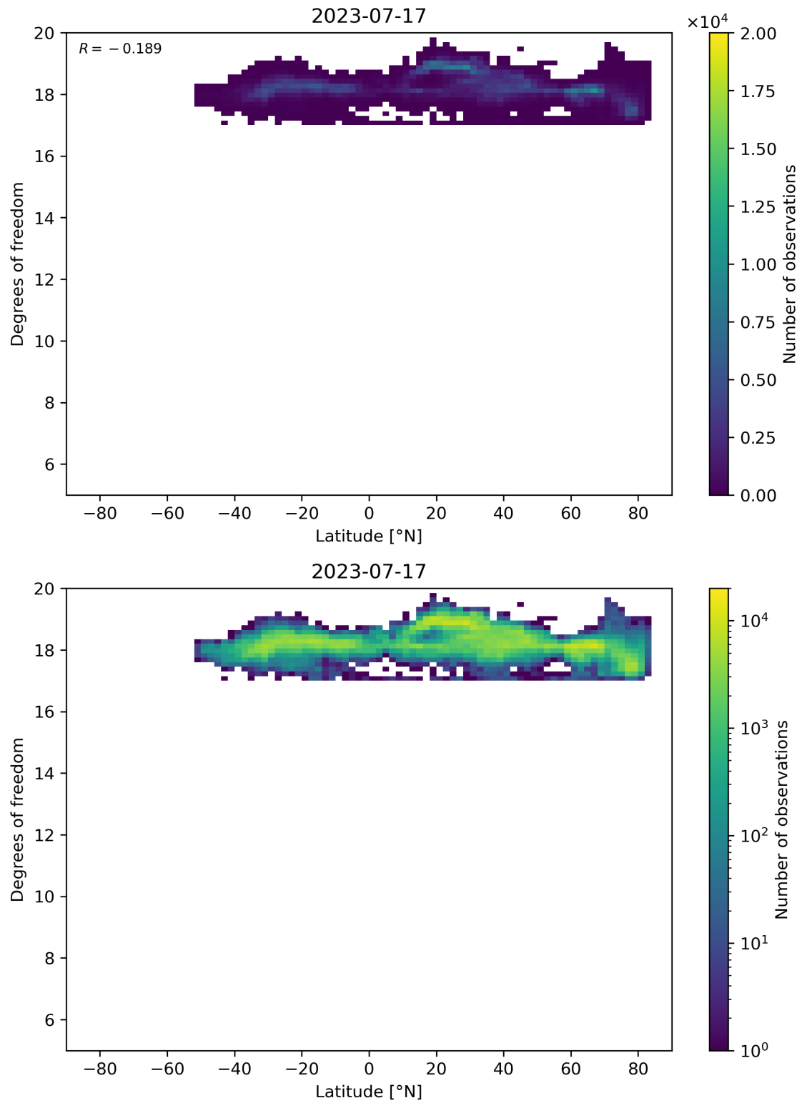
Figure 55: Scatter density plot of “Latitude” against “Degrees of freedom” for 2023-07-16 to 2023-07-18.
