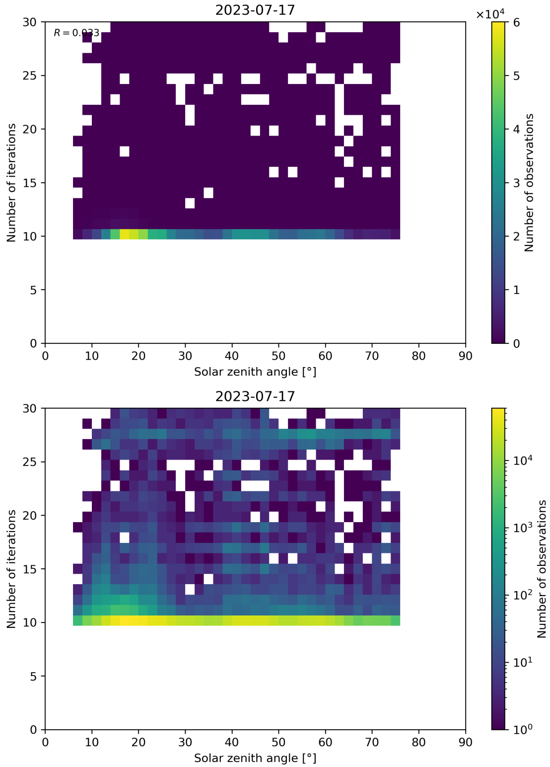
Figure 102: Scatter density plot of “Solar zenith angle” against “Number of iterations” for 2023-07-16 to 2023-07-18.
