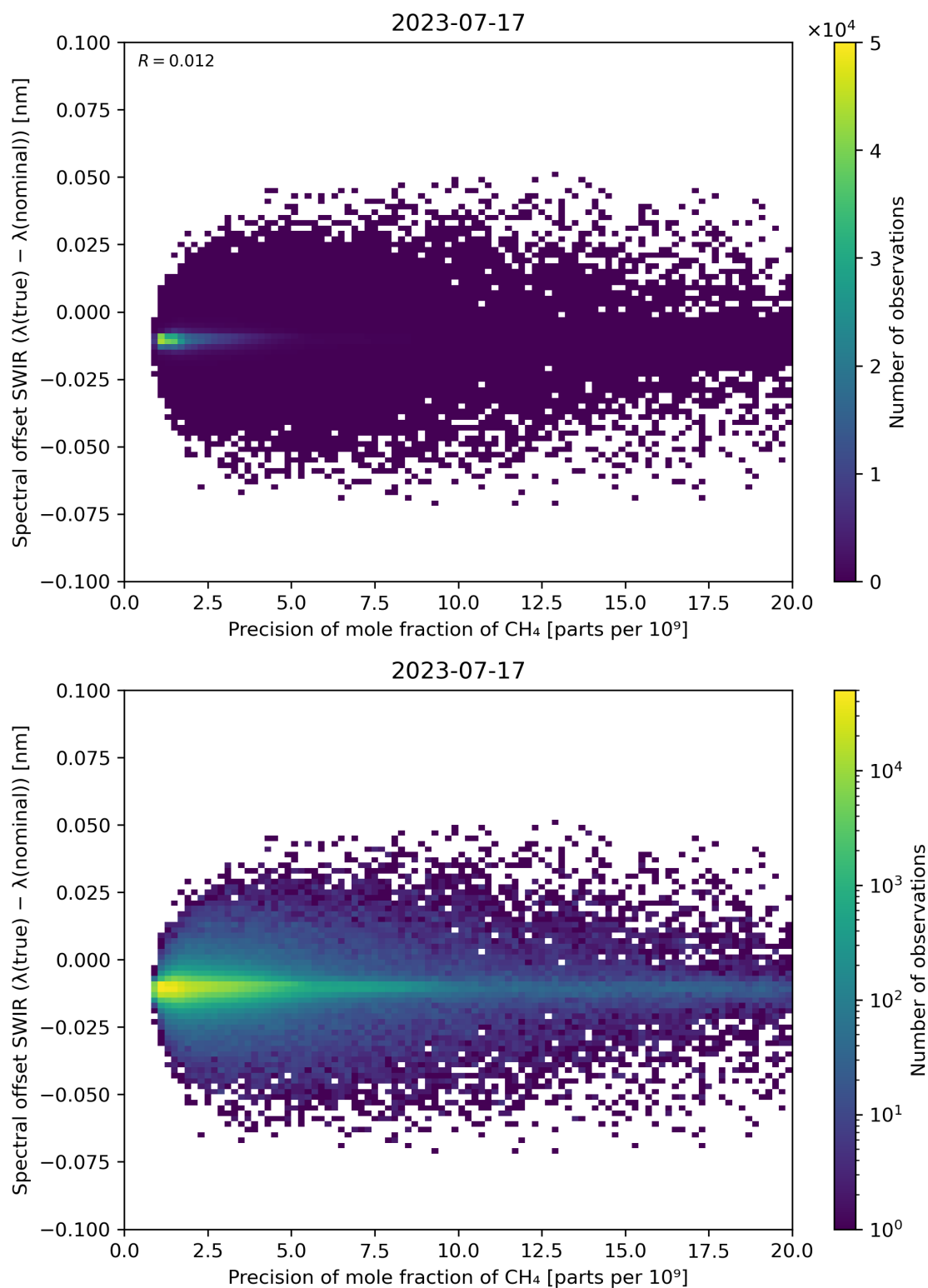
Figure 85: Scatter density plot of “Precision of mole fraction of CH 4 ” against “Spectral offset SWIR ( \lambda(\text{true}) - \lambda(\text{nominal}) )” for 2023-07-16 to 2023-07-18.
