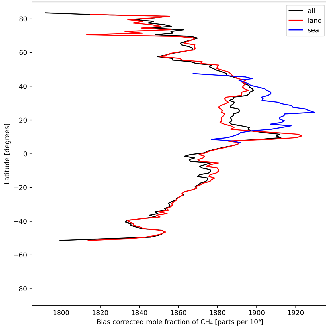
Figure 14: Zonal average of “Bias corrected mole fraction of CH 4 ” for 2023-07-16 to 2023-07-18.
