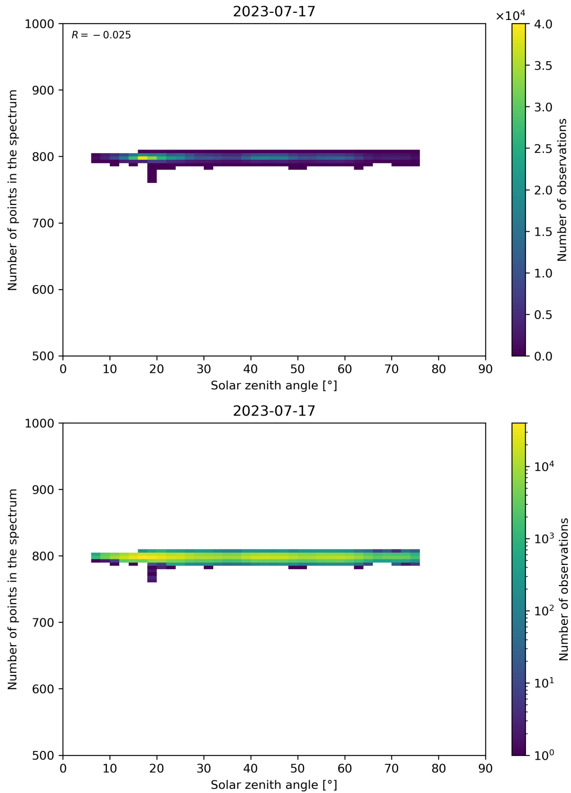
Figure 103: Scatter density plot of “Solar zenith angle” against “Number of points in the spectrum” for 2023-07-16 to 2023-07-18.
