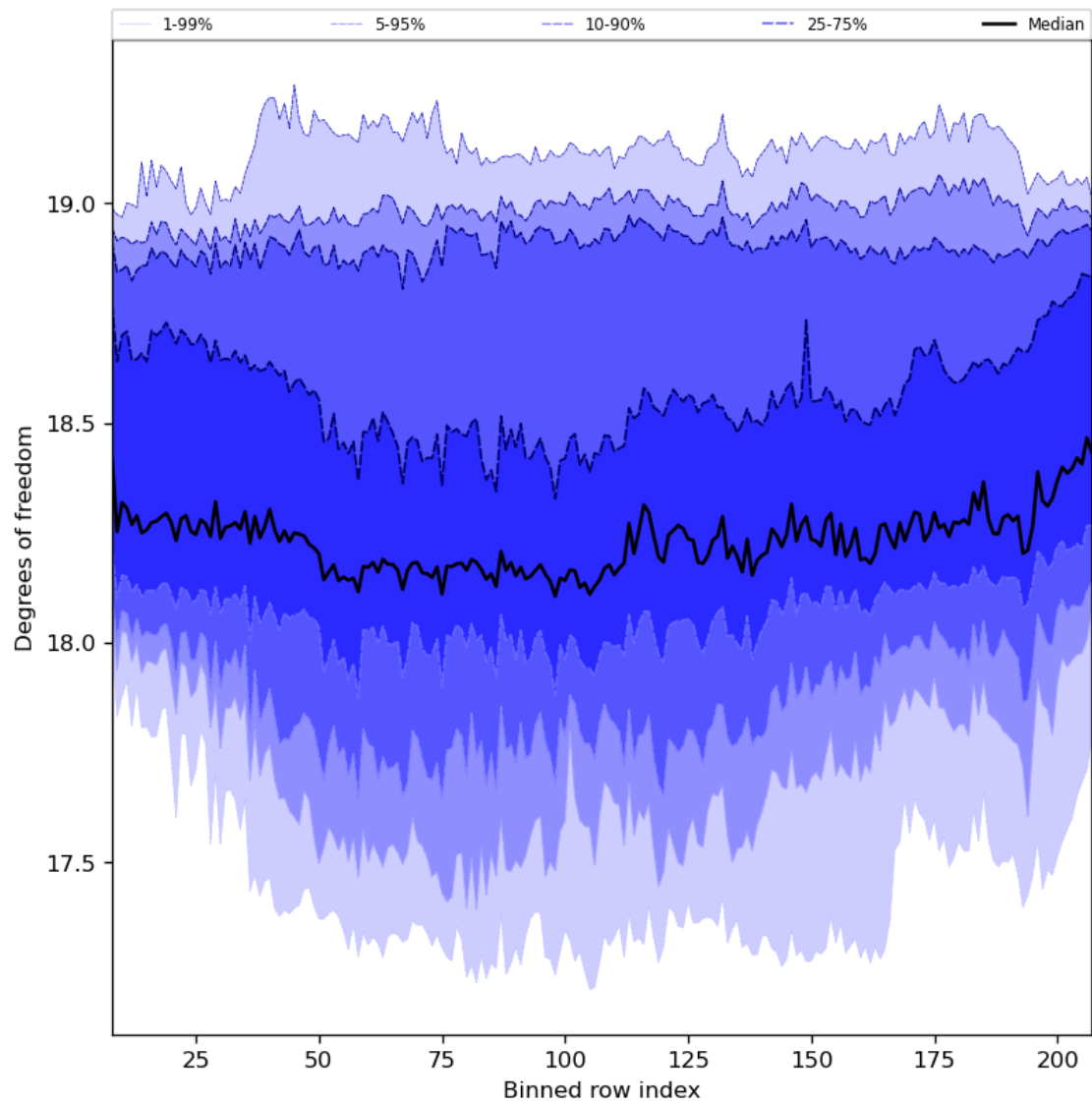
Figure 41: Along track statistics of “Degrees of freedom” for 2023-07-16 to 2023-07-18
