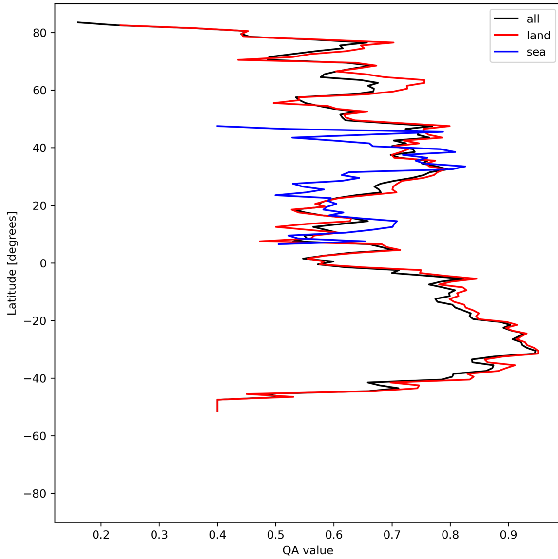
Figure 11: Zonal average of “QA value” for 2023-07-16 to 2023-07-18.
