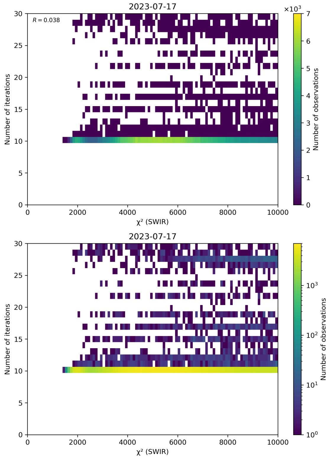
Figure 50: Scatter density plot of “ \chi^2 (SWIR)” against “Number of iterations” for 2023-07-16 to 2023-07-18.
