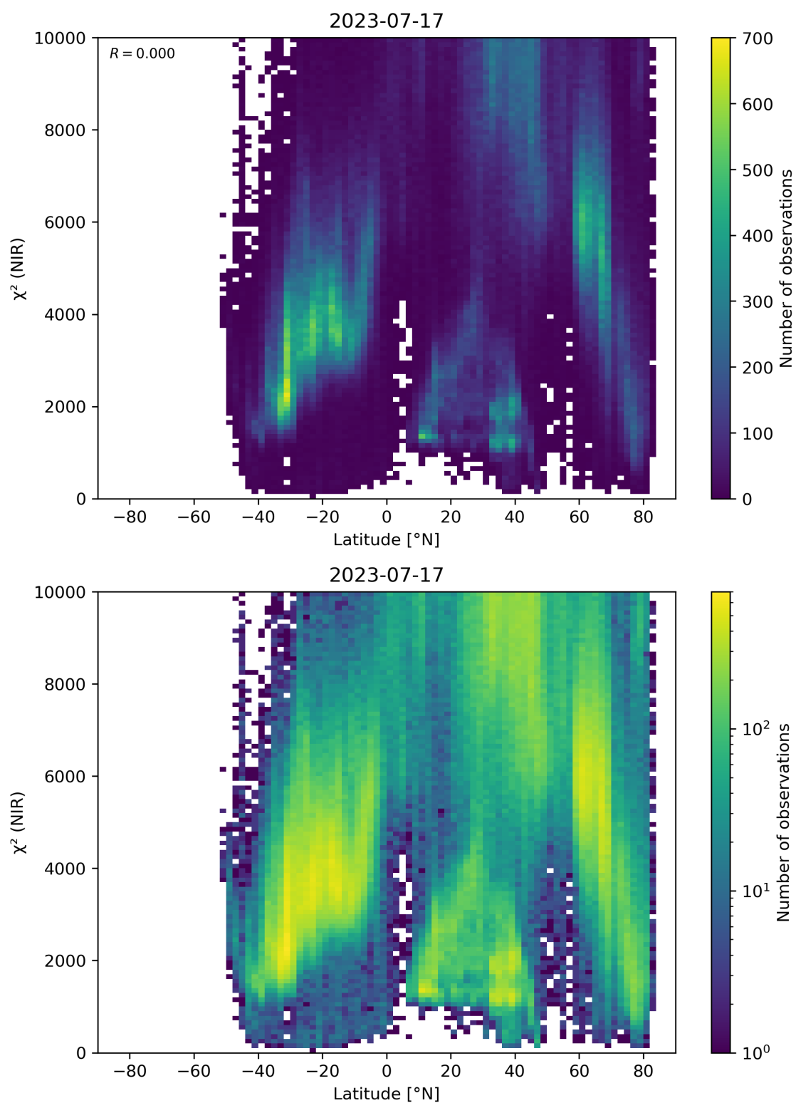
Figure 53: Scatter density plot of “Latitude” against “ \chi^2 (NIR)” for 2023-07-16 to 2023-07-18.
