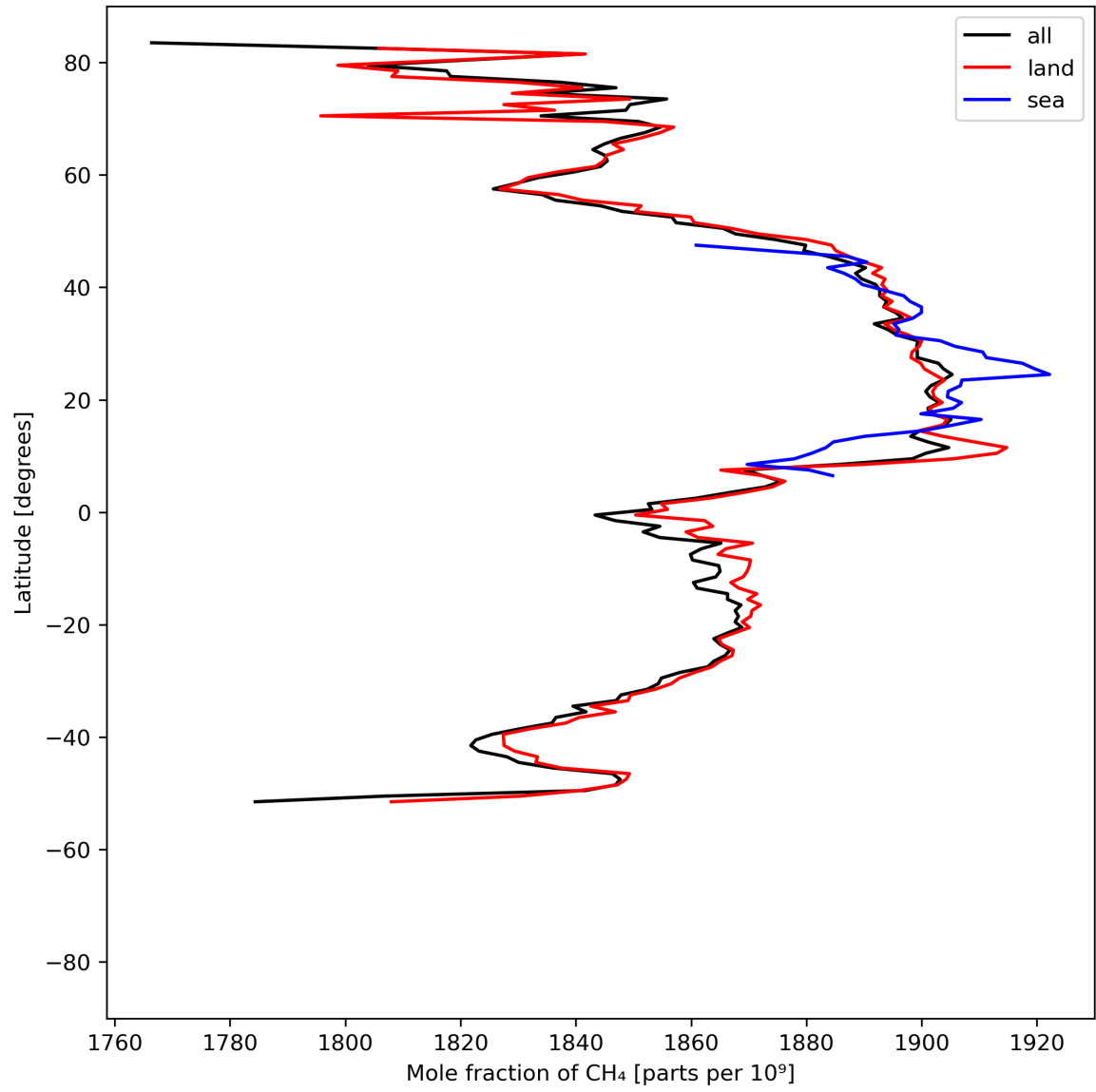
Figure 12: Zonal average of “Mole fraction of \text{CH}_4 ” for 2023-07-16 to 2023-07-18.
