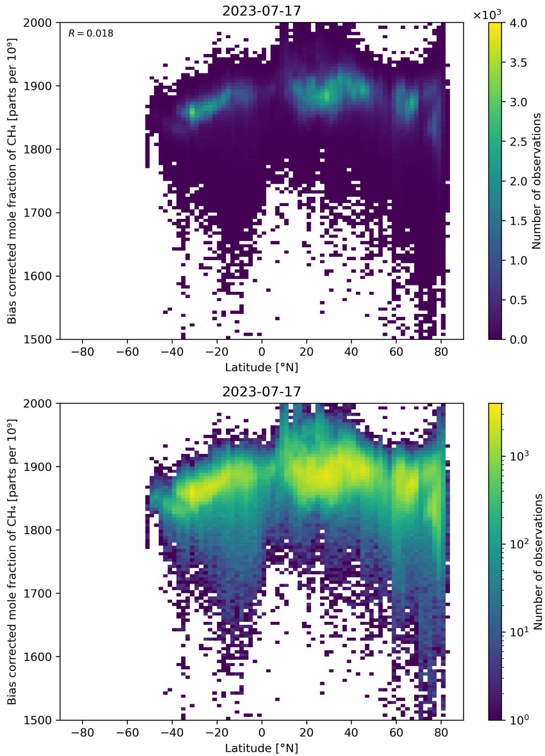
Figure 58: Scatter density plot of “Latitude” against “Bias corrected mole fraction of \text{CH}_4 ” for 2023-07-16 to 2023-07-18.
