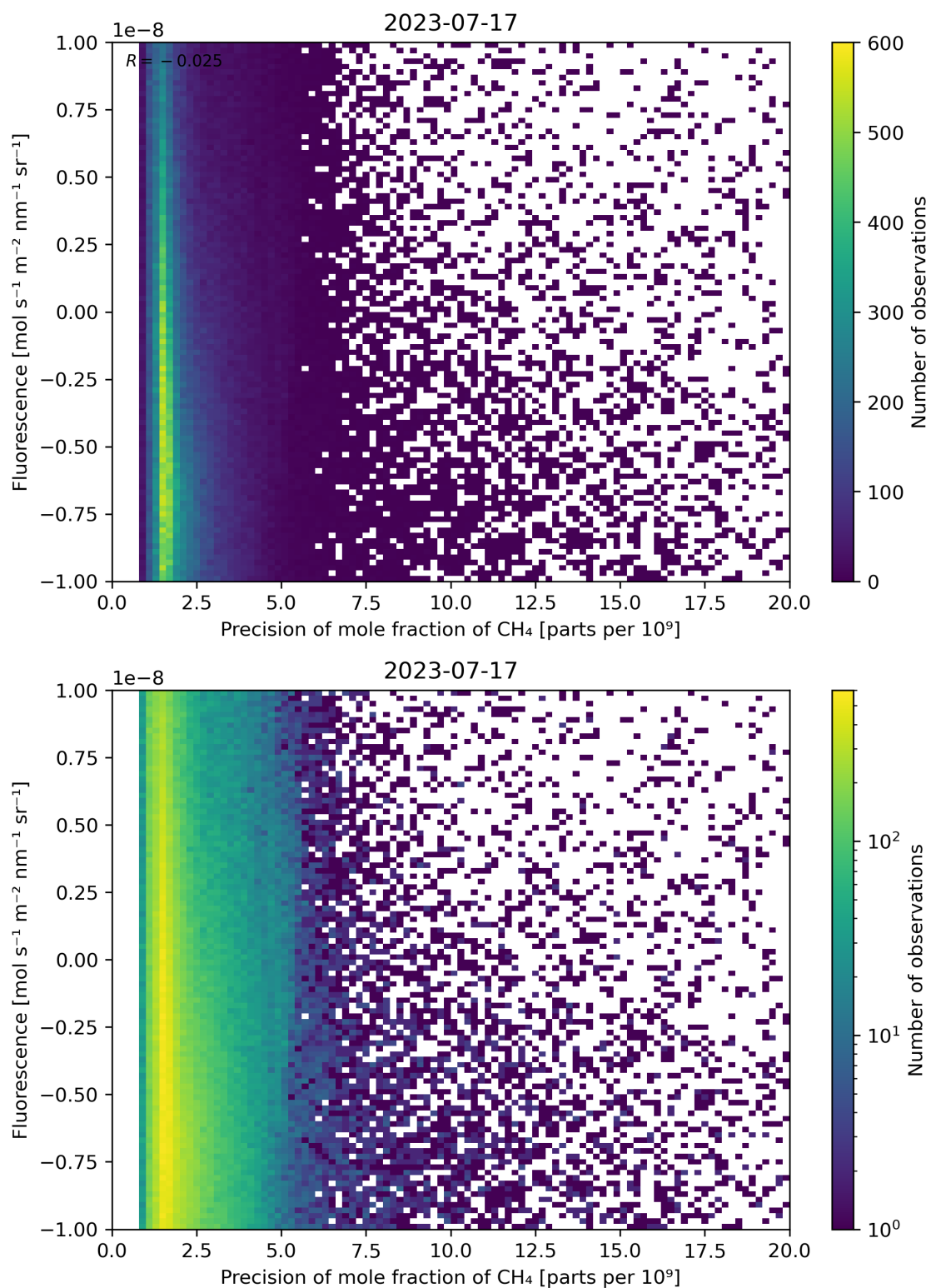
Figure 81: Scatter density plot of “Precision of mole fraction of CH 4 ” against “Fluorescence” for 2023-07-16 to 2023-07-18.
