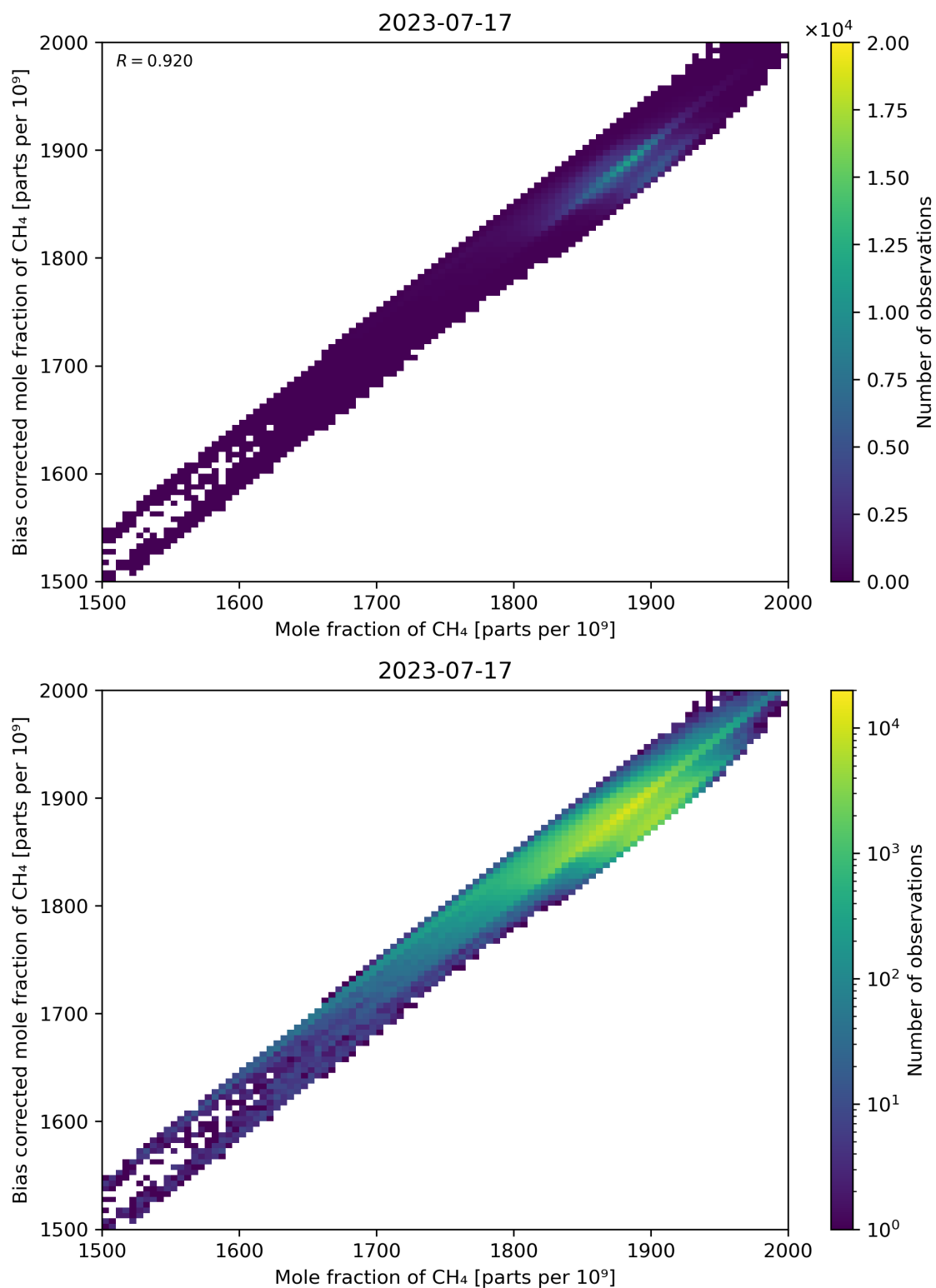
Figure 74: Scatter density plot of “Mole fraction of CH 4 ” against “Bias corrected mole fraction of CH 4 ” for 2023-07-16 to 2023-07-18.
