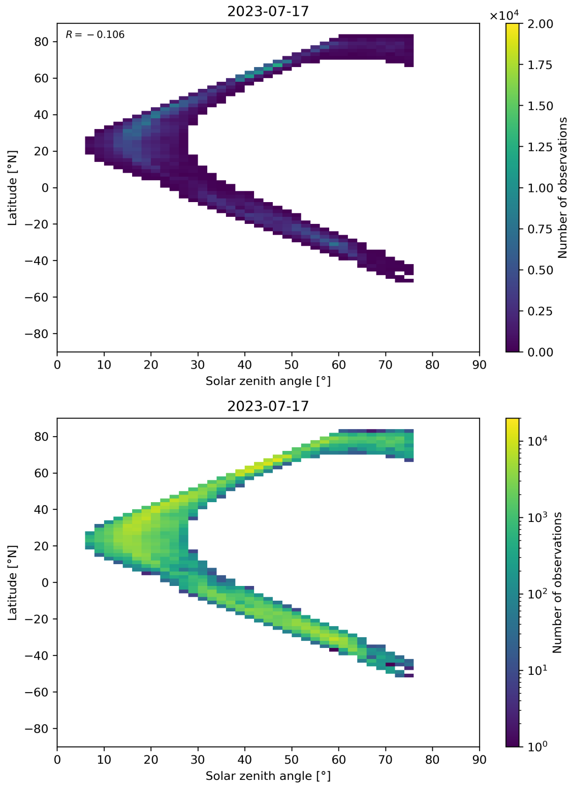
Figure 98: Scatter density plot of “Solar zenith angle” against “Latitude” for 2023-07-16 to 2023-07-18.
