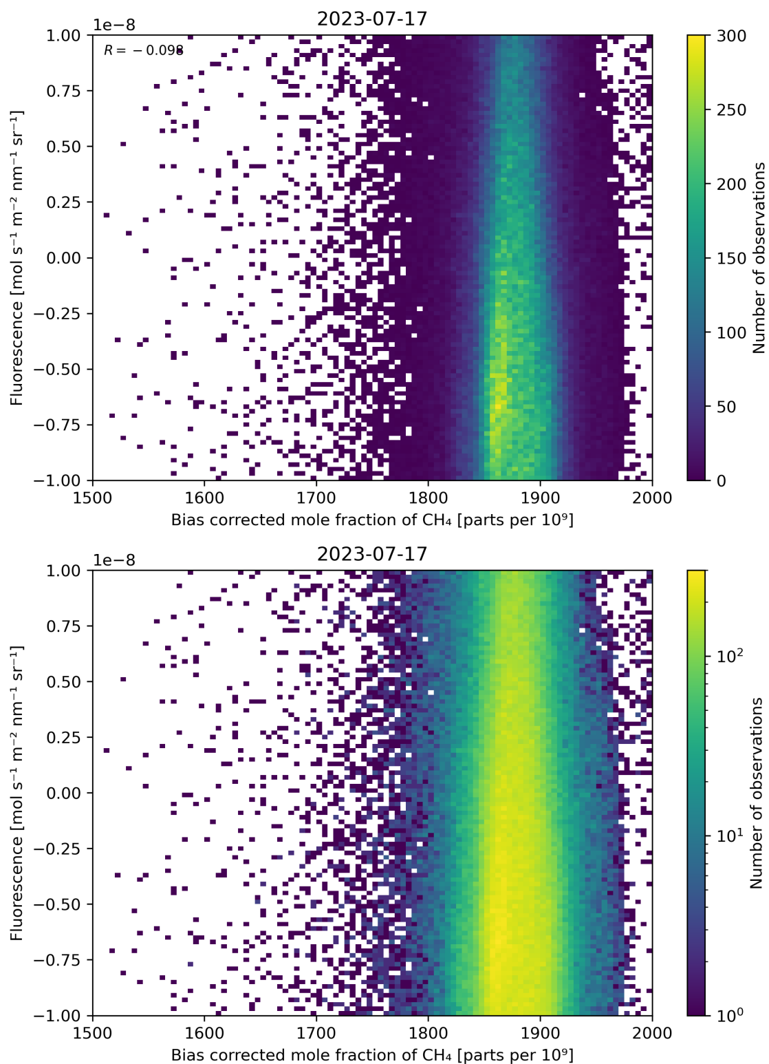
Figure 66: Scatter density plot of “Bias corrected mole fraction of \text{CH}_4 ” against “Fluorescence” for 2023-07-16 to 2023-07-18.
