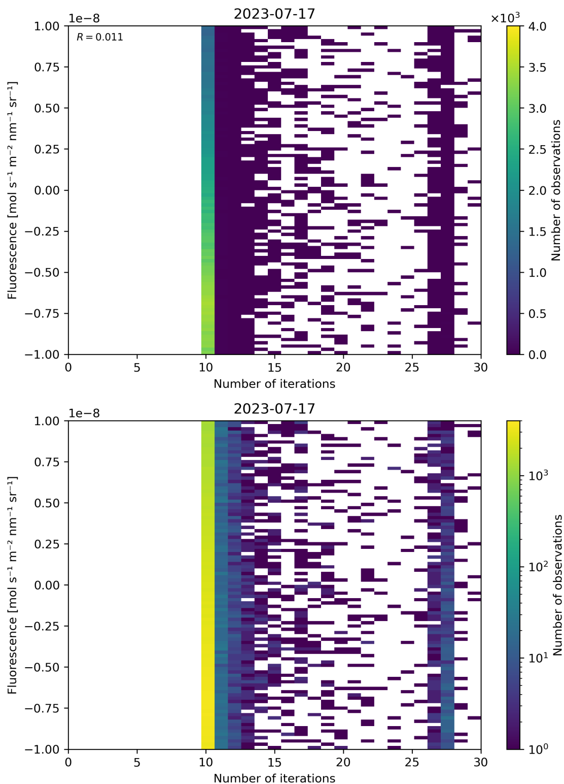
Figure 87: Scatter density plot of “Number of iterations” against “Fluorescence” for 2023-07-16 to 2023-07-18.
