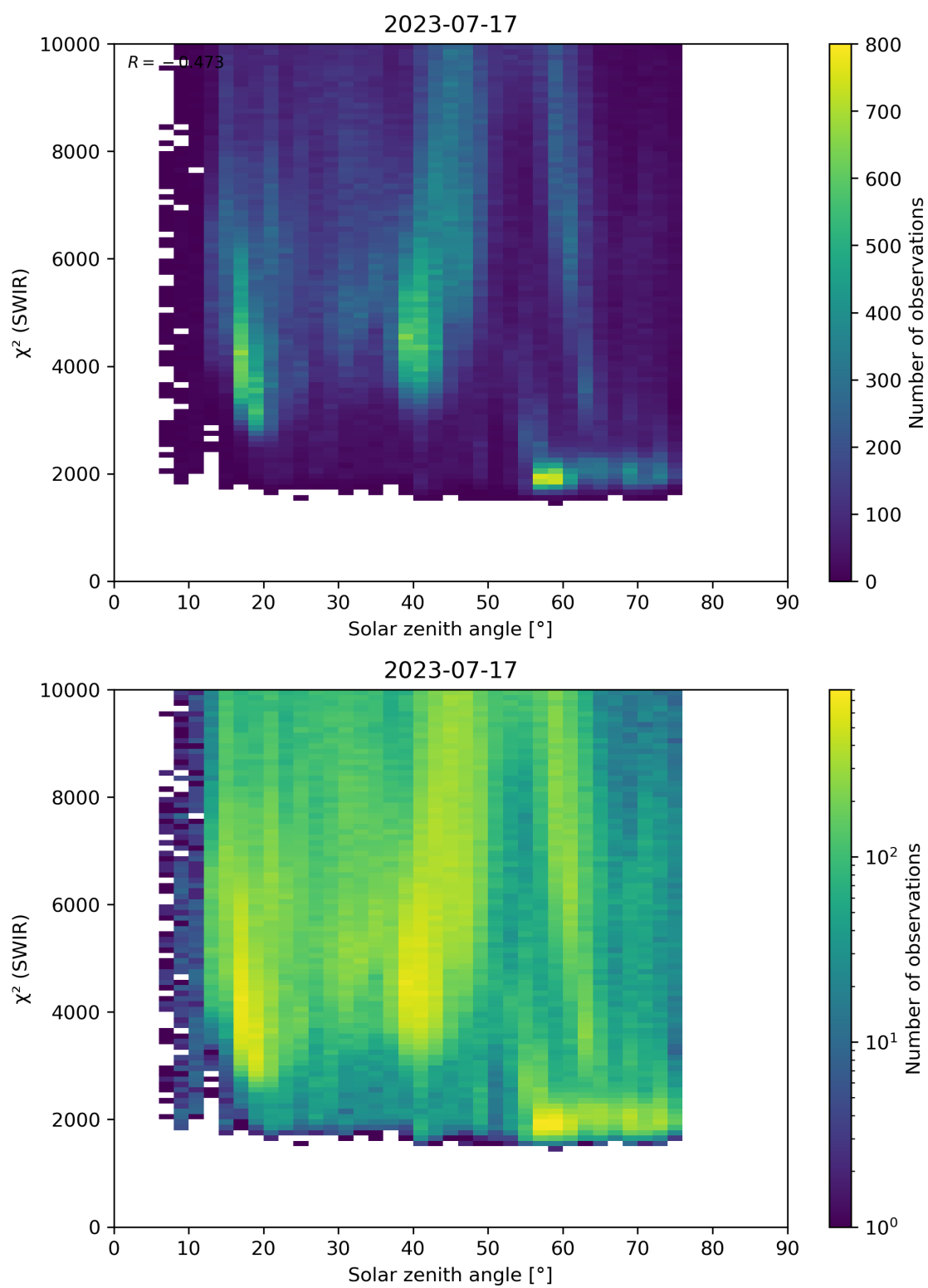
Figure 95: Scatter density plot of “Solar zenith angle” against “ \chi^2 (SWIR)” for 2023-07-16 to 2023-07-18.
