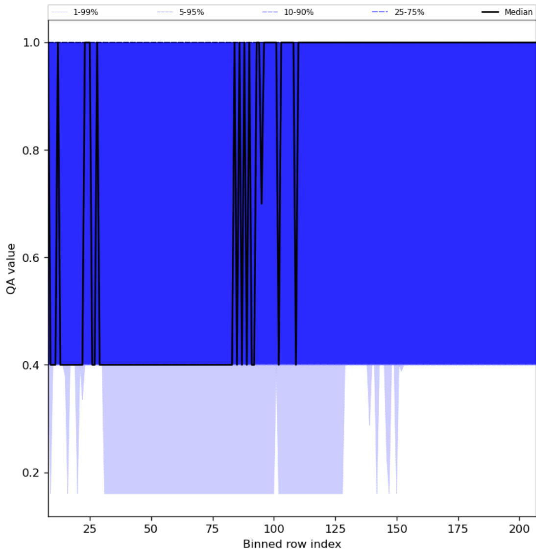
Figure 33: Along track statistics of “QA value” for 2023-07-16 to 2023-07-18
