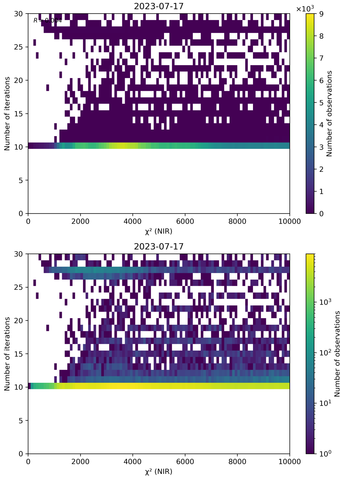
Figure 46: Scatter density plot of “ \chi^2 (NIR)” against “Number of iterations” for 2023-07-16 to 2023-07-18.
