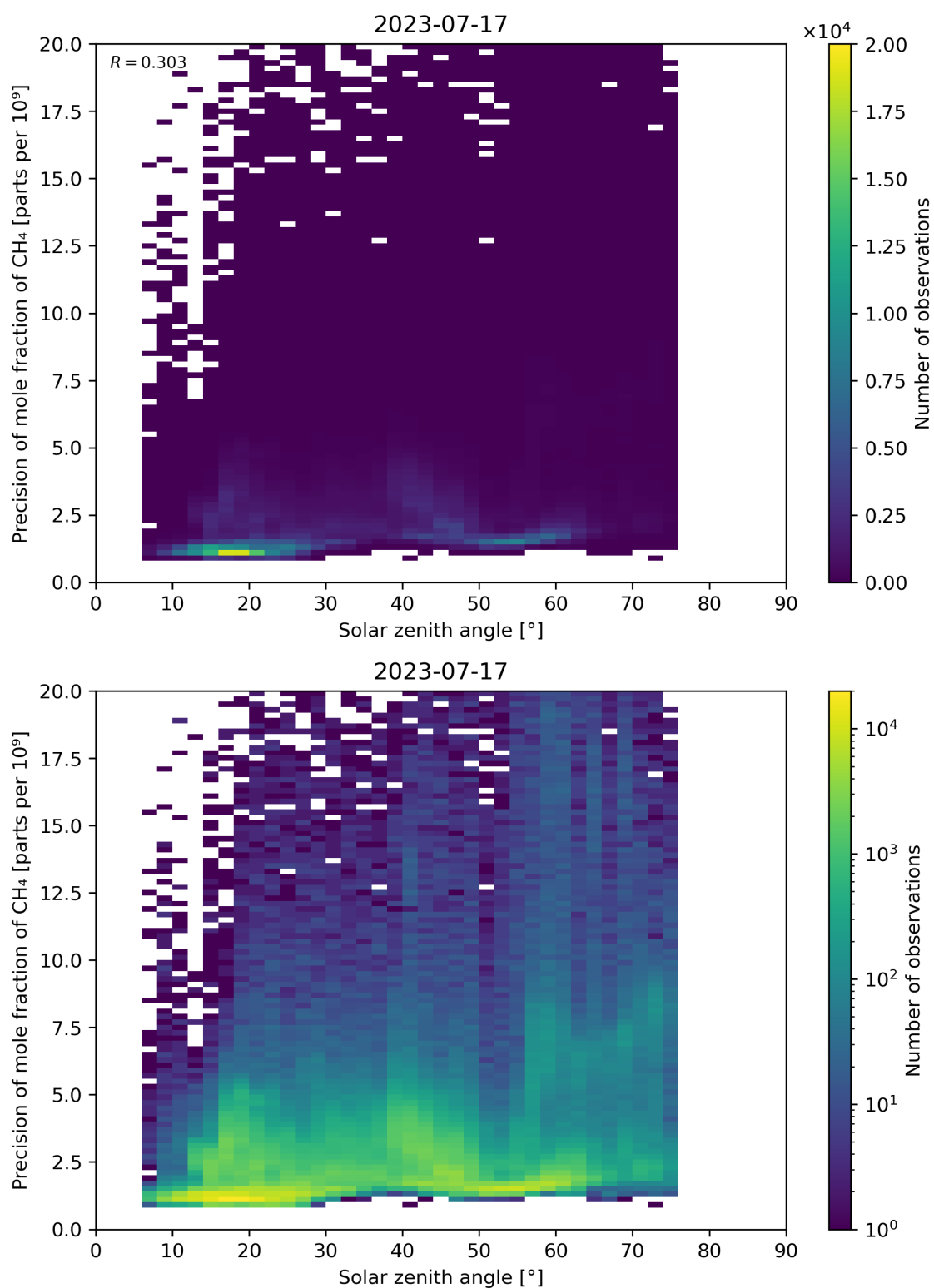
Figure 101: Scatter density plot of “Solar zenith angle” against “Precision of mole fraction of CH 4 ” for 2023-07-16 to 2023-07-18.
