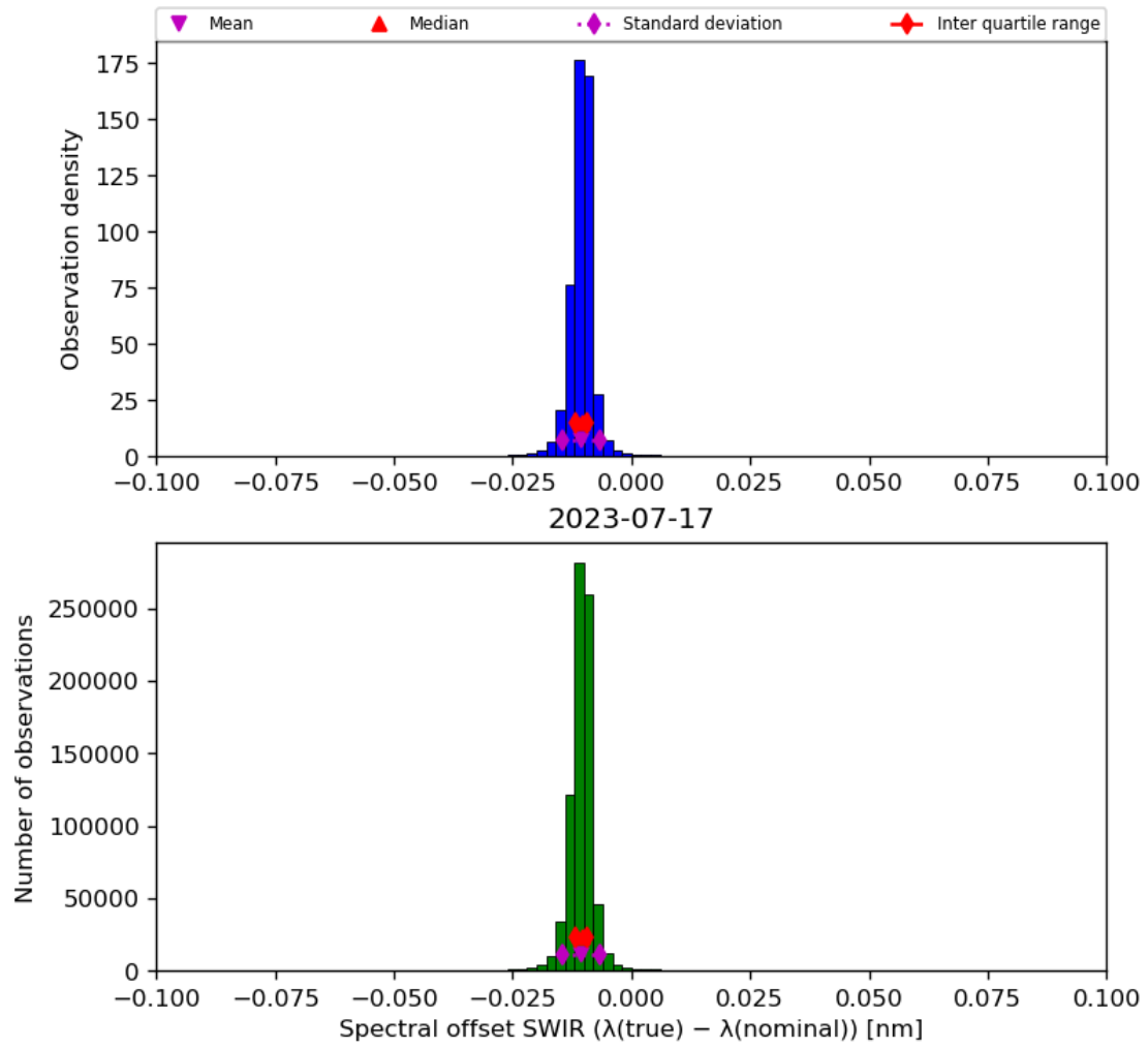
Figure 27: Histogram of “Spectral offset SWIR ( \lambda(\text{true}) - \lambda(\text{nominal}) )” for 2023-07-16 to 2023-07-18
