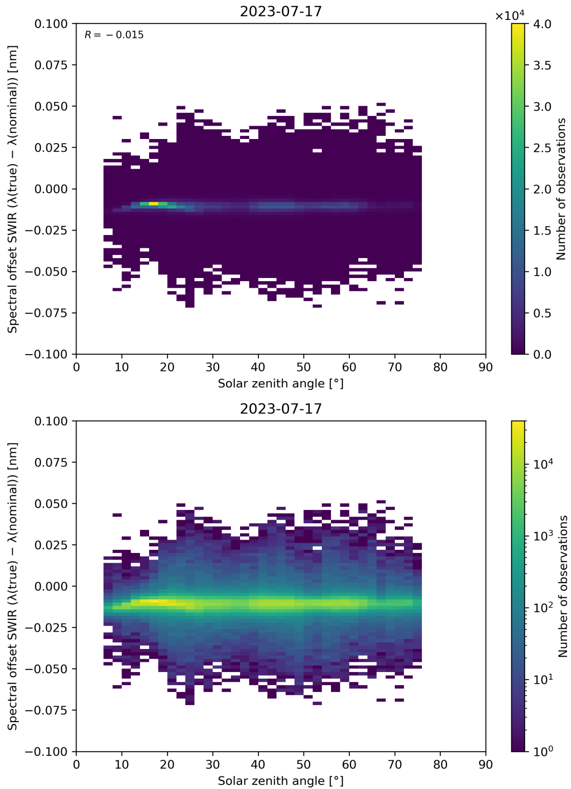
Figure 104: Scatter density plot of “Solar zenith angle” against “Spectral offset SWIR ( \lambda(\text{true}) - \lambda(\text{nominal}) )” for 2023-07-16 to 2023-07-18.
