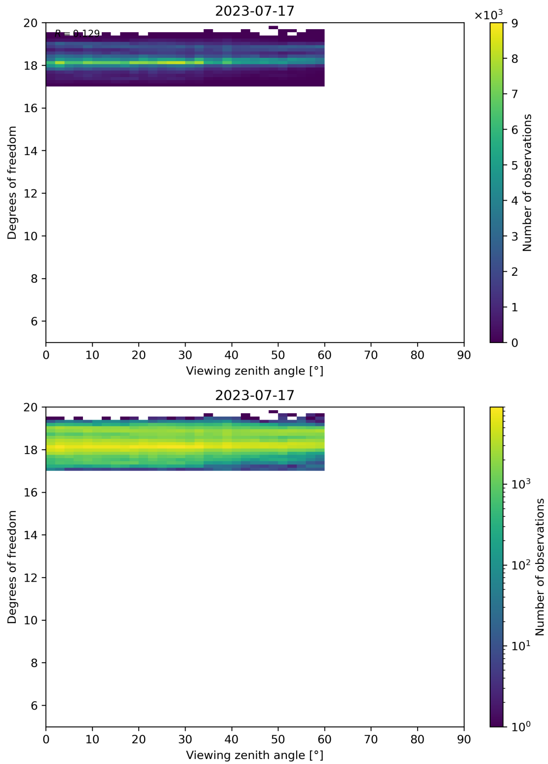
Figure 107: Scatter density plot of “Viewing zenith angle” against “Degrees of freedom” for 2023-07-16 to 2023-07-18.
