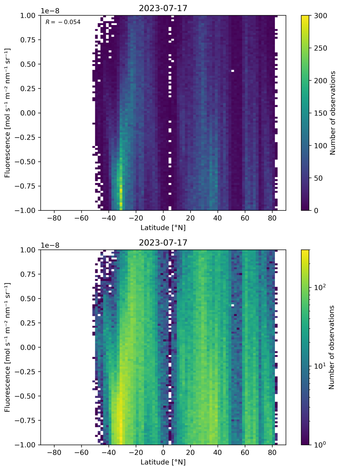
Figure 56: Scatter density plot of “Latitude” against “Fluorescence” for 2023-07-16 to 2023-07-18.
