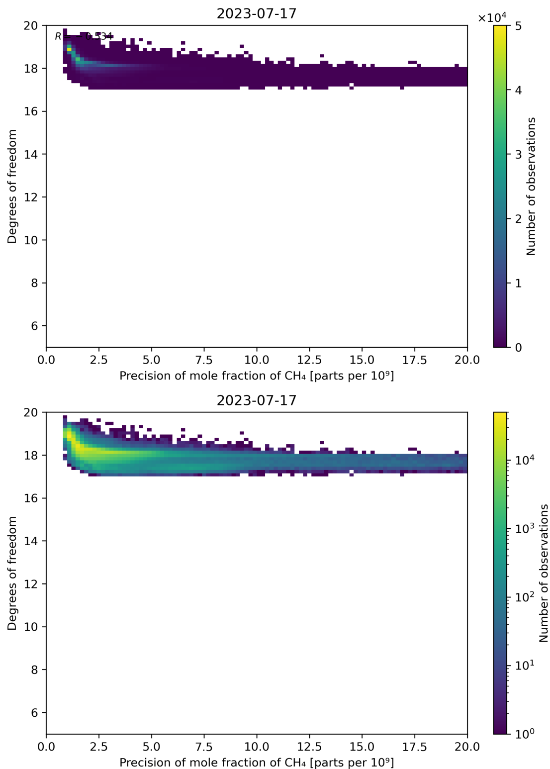
Figure 80: Scatter density plot of “Precision of mole fraction of CH 4 ” against “Degrees of freedom” for 2023-07-16 to 2023-07-18.
