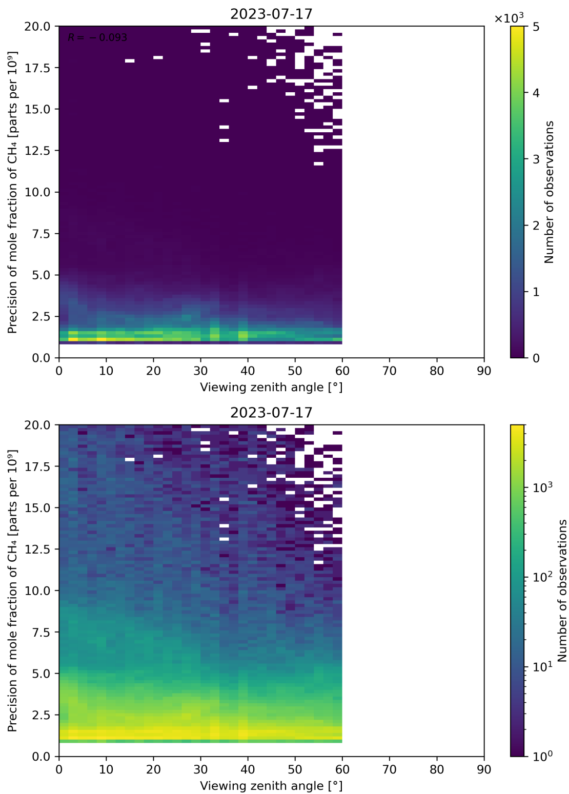
Figure 112: Scatter density plot of “Viewing zenith angle” against “Precision of mole fraction of CH 4 ” for 2023-07-16 to 2023-07-18.
