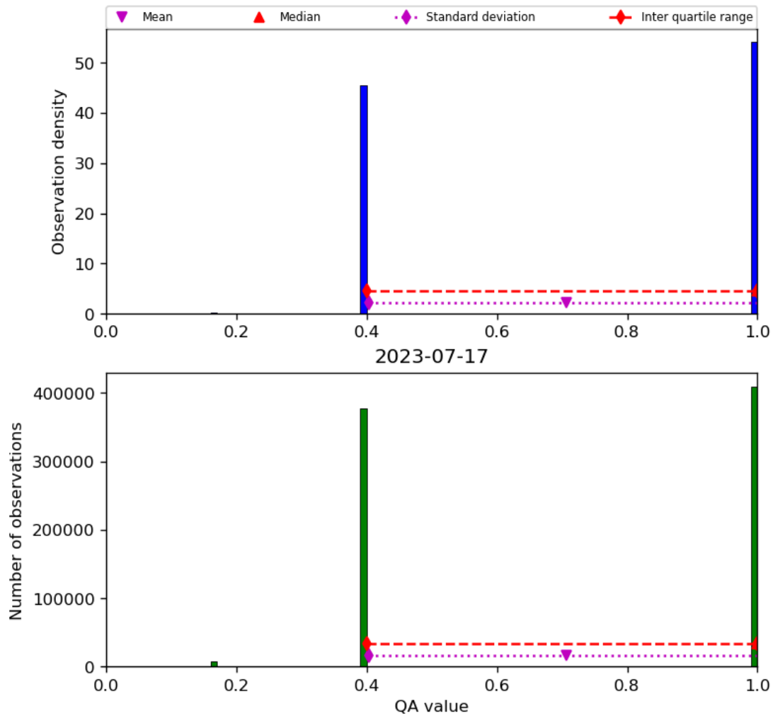
Figure 22: Histogram of “QA value” for 2023-07-16 to 2023-07-18
