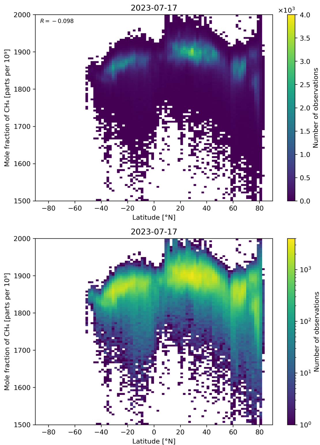
Figure 57: Scatter density plot of “Latitude” against “Mole fraction of CH 4 ” for 2023-07-16 to 2023-07-18.
