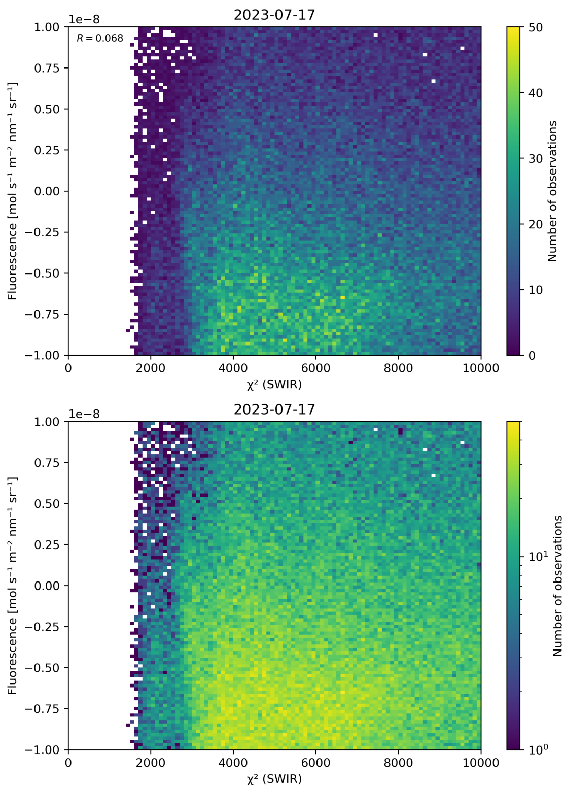
Figure 49: Scatter density plot of “ \chi^2 (SWIR)” against “Fluorescence” for 2023-07-16 to 2023-07-18.
