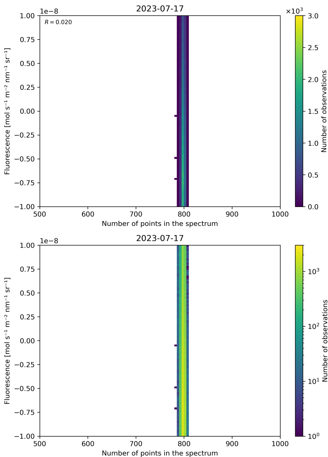
Figure 91: Scatter density plot of “Number of points in the spectrum” against “Fluorescence” for 2023-07-16 to 2023-07-18.
