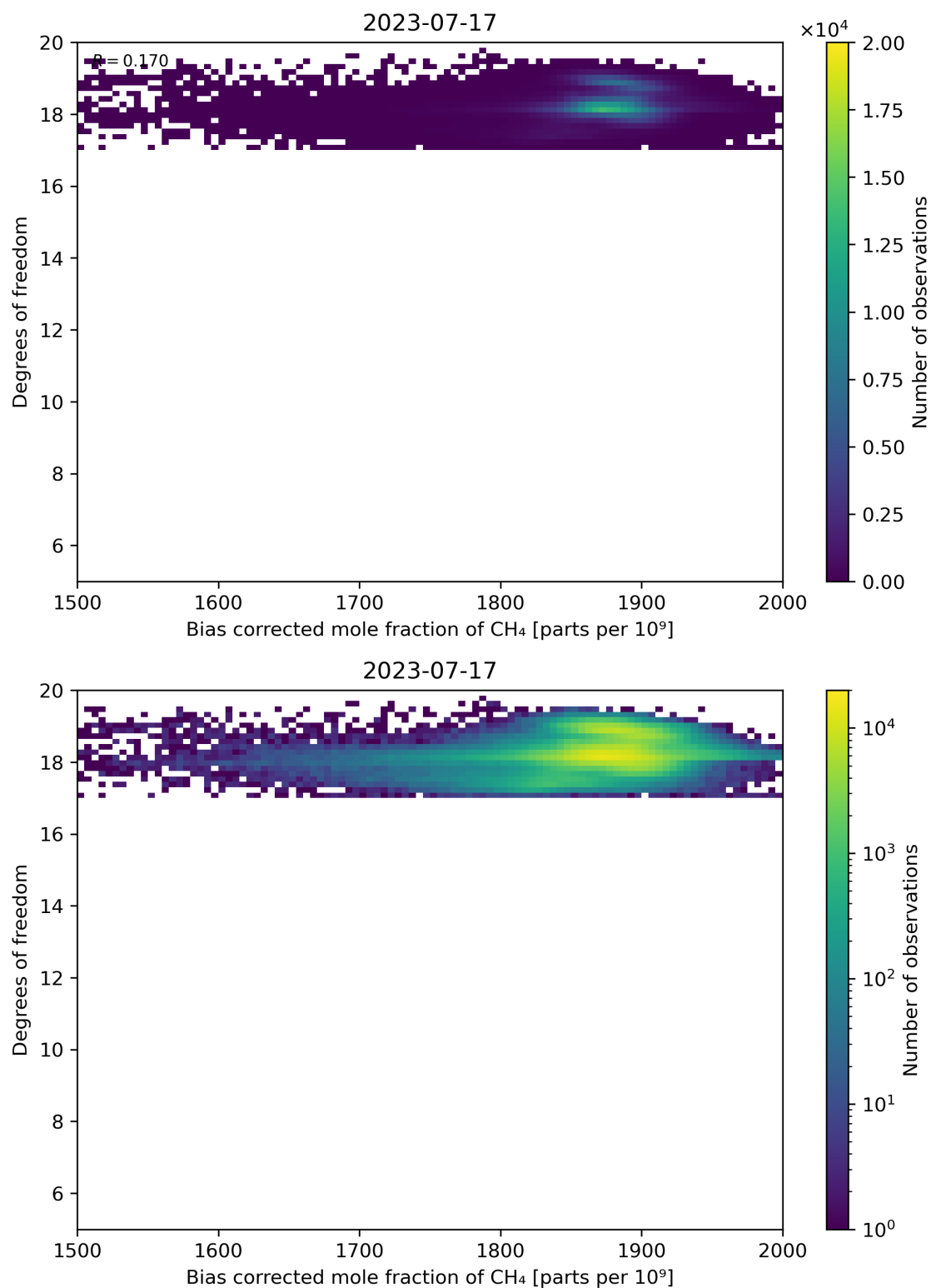
Figure 65: Scatter density plot of “Bias corrected mole fraction of CH 4 ” against “Degrees of freedom” for 2023-07-16 to 2023-07-18.
