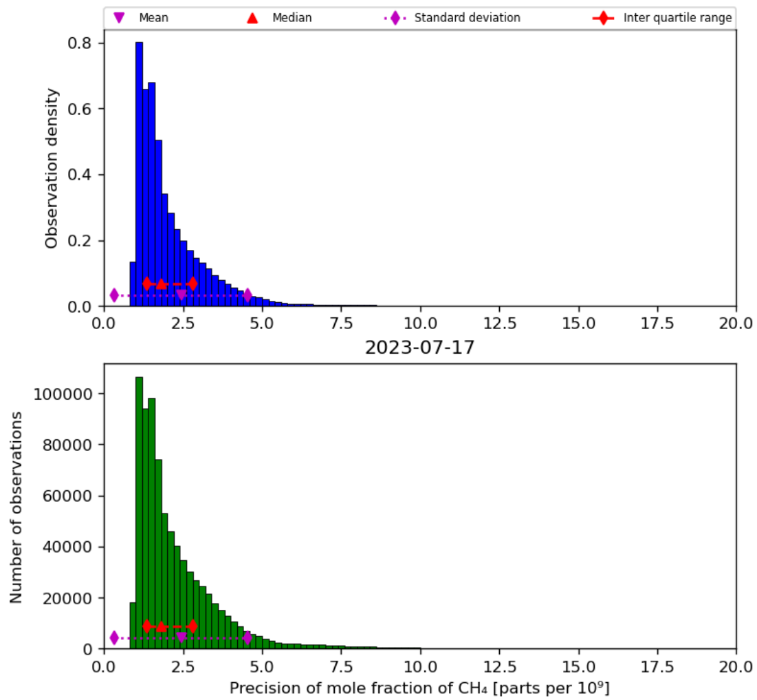
Figure 24: Histogram of “Precision of mole fraction of CH 4 ” for 2023-07-16 to 2023-07-18
