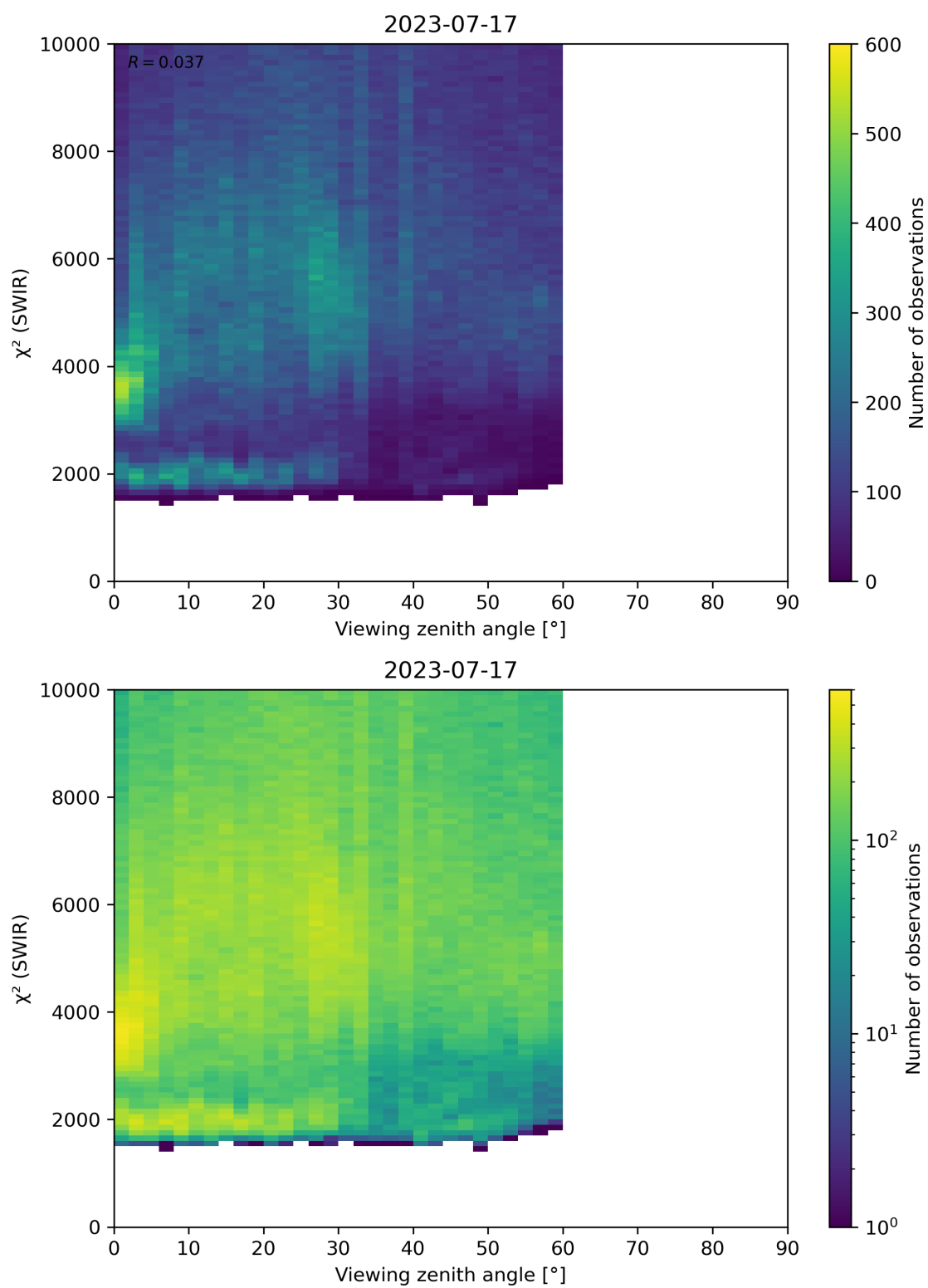
Figure 106: Scatter density plot of “Viewing zenith angle” against “ \chi^2 (SWIR)” for 2023-07-16 to 2023-07-18.
