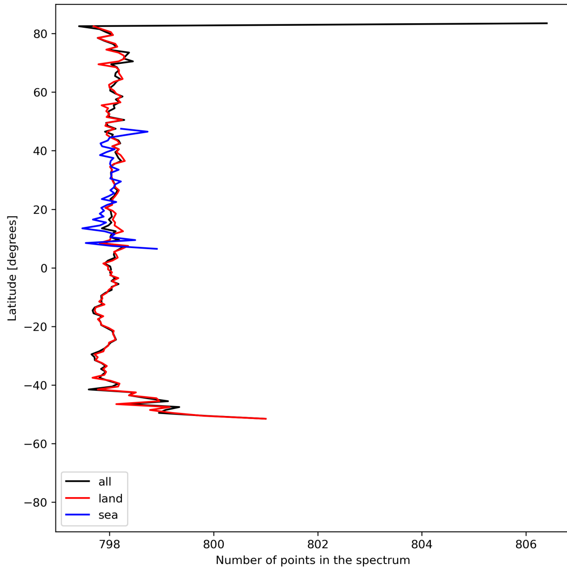
Figure 15: Zonal average of “Number of points in the spectrum” for 2023-07-16 to 2023-07-18.
