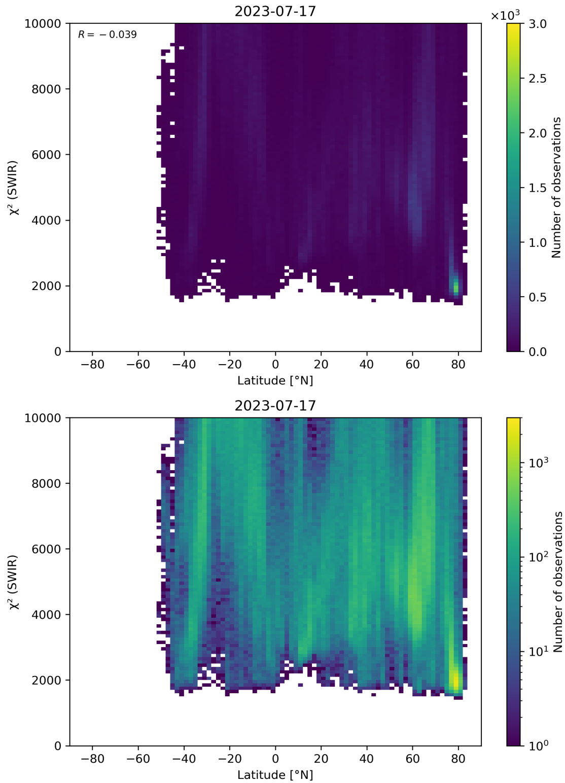
Figure 54: Scatter density plot of “Latitude” against “ \chi^2 (SWIR)” for 2023-07-16 to 2023-07-18.
