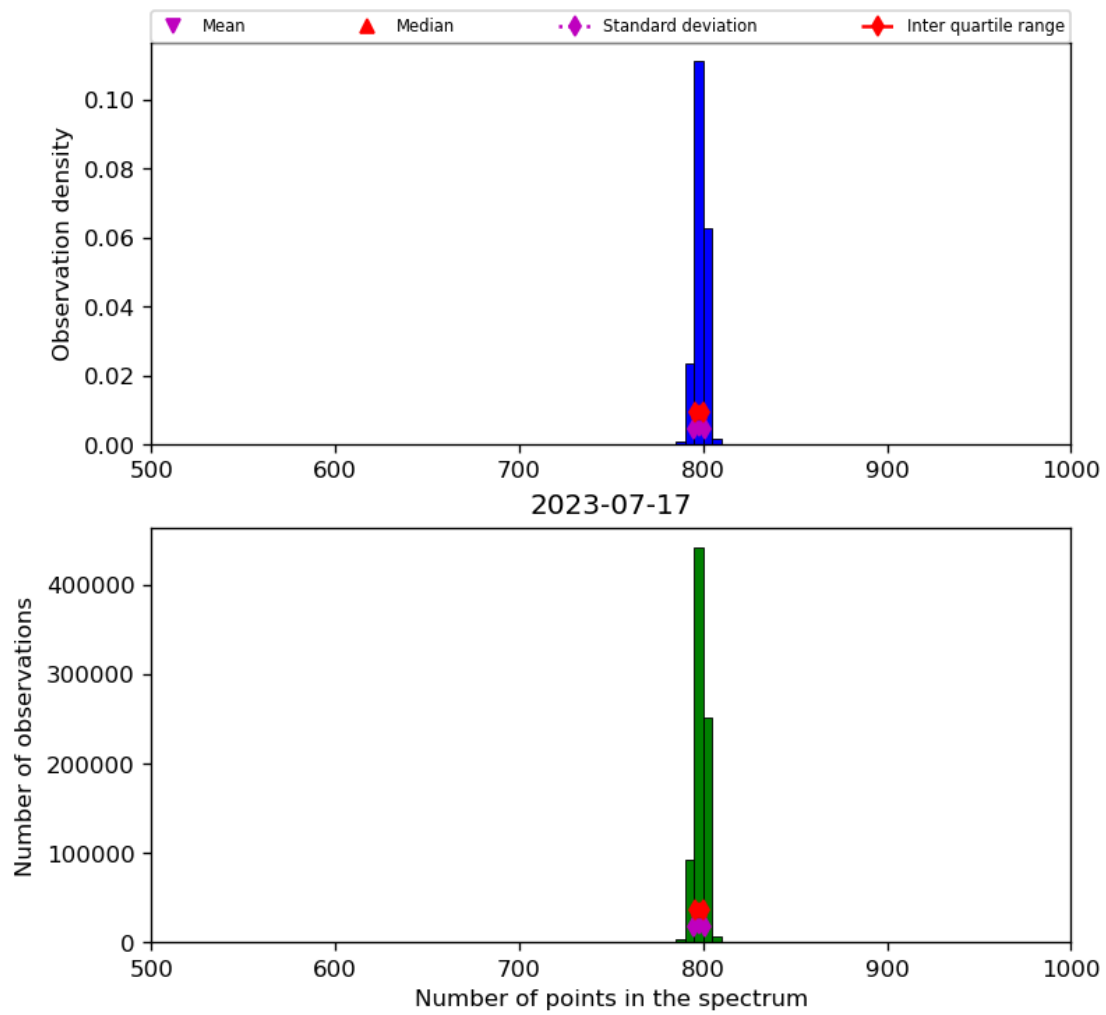
Figure 26: Histogram of “Number of points in the spectrum” for 2023-07-16 to 2023-07-18
