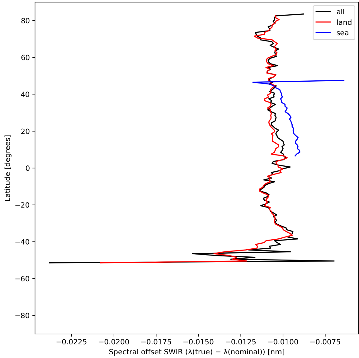
Figure 16: Zonal average of “Spectral offset SWIR ( \lambda(\text{true}) - \lambda(\text{nominal}) )” for 2023-07-16 to 2023-07-18.
