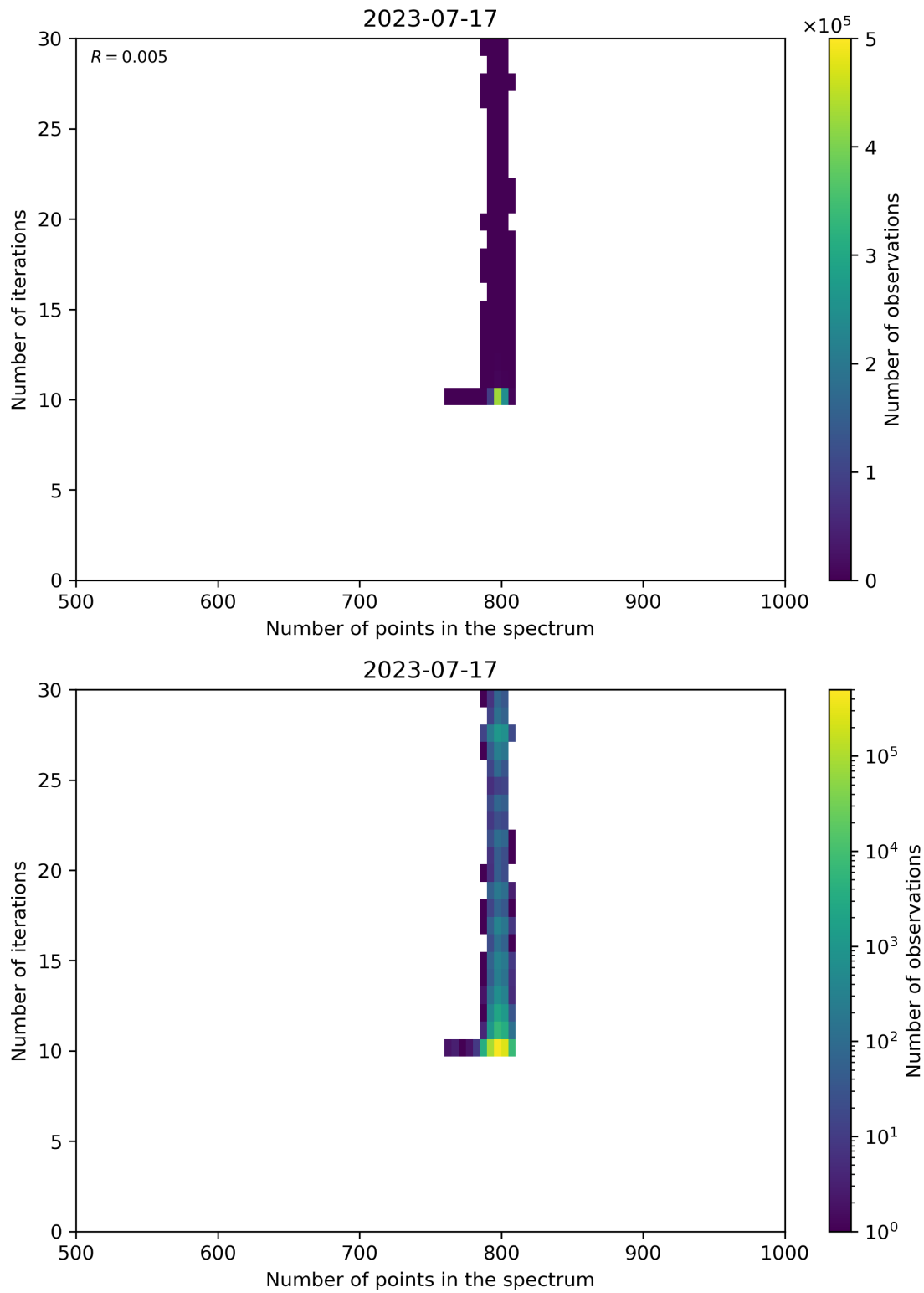
Figure 92: Scatter density plot of “Number of points in the spectrum” against “Number of iterations” for 2023-07-16 to 2023-07-18.
