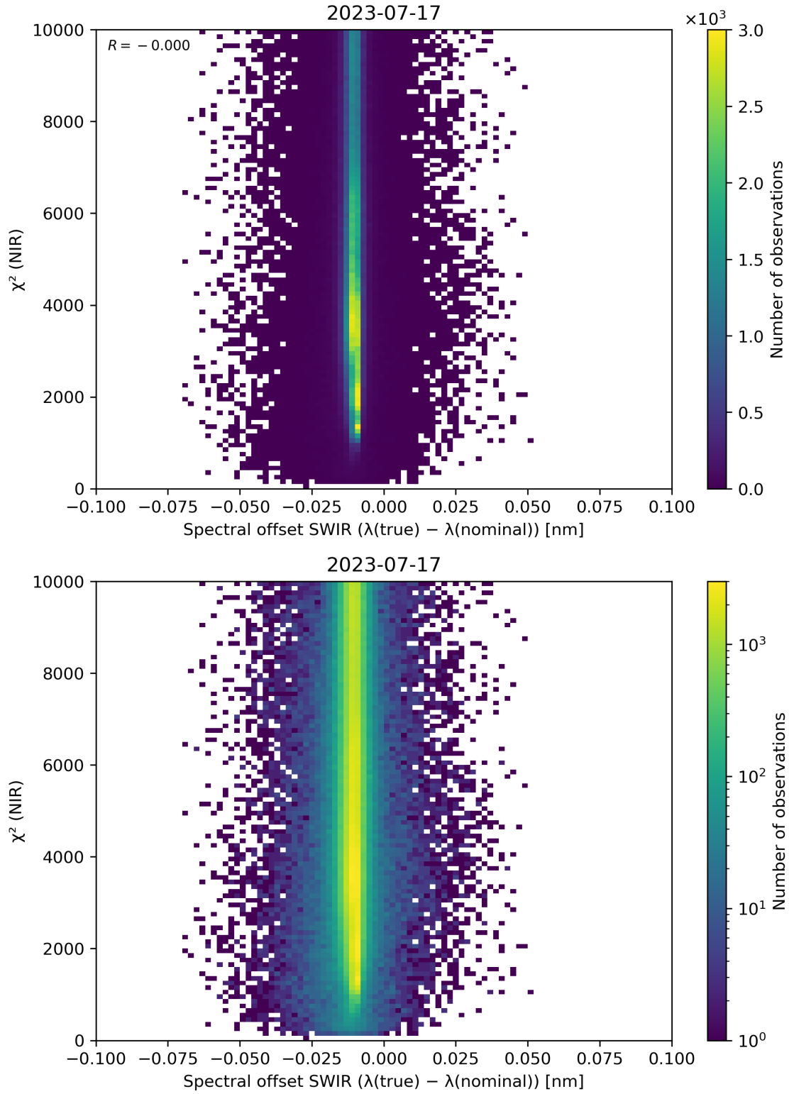
Figure 117: Scatter density plot of “Spectral offset SWIR ( \lambda(\text{true}) - \lambda(\text{nominal}) )” against “ \chi^2 (NIR)” for 2023-07-16 to 2023-07-18.
