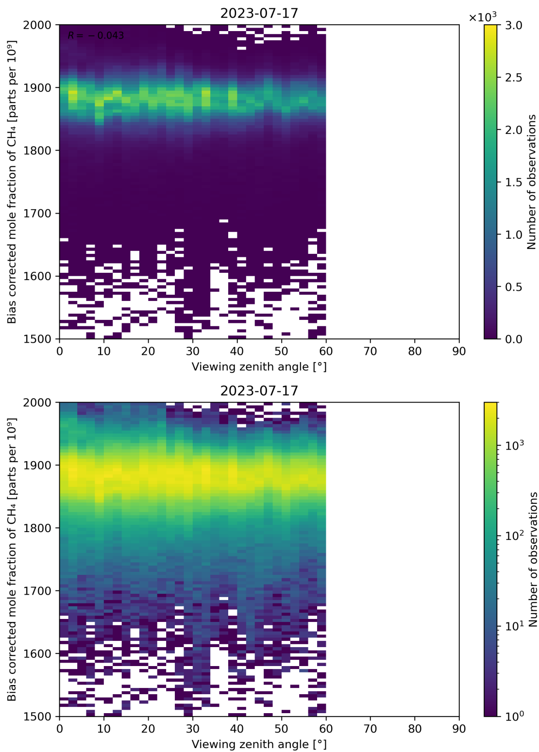
Figure 111: Scatter density plot of “Viewing zenith angle” against “Bias corrected mole fraction of CH 4 ” for 2023-07-16 to 2023-07-18.
