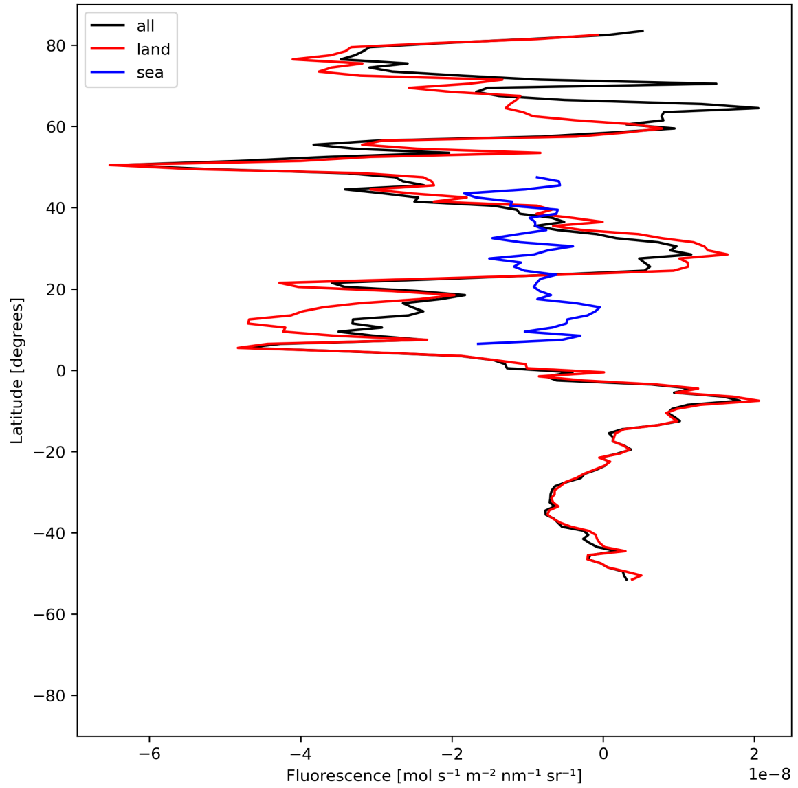
Figure 21: Zonal average of “Fluorescence” for 2023-07-16 to 2023-07-18.
