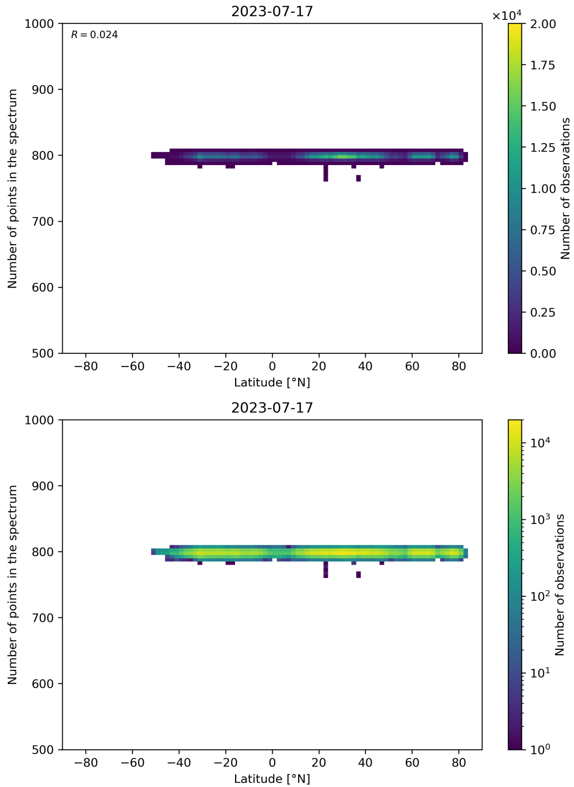
Figure 61: Scatter density plot of “Latitude” against “Number of points in the spectrum” for 2023-07-16 to 2023-07-18.
