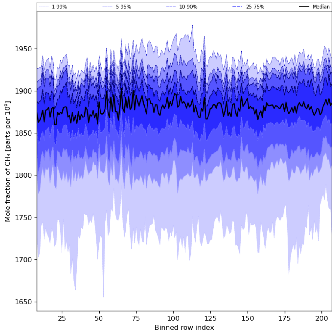
Figure 34: Along track statistics of “Mole fraction of CH 4 ” for 2023-07-16 to 2023-07-18
