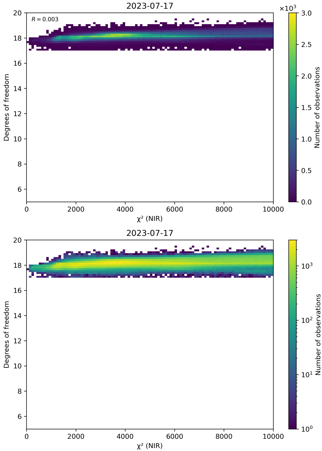
Figure 44: Scatter density plot of “ \chi^2 (NIR)” against “Degrees of freedom” for 2023-07-16 to 2023-07-18.
