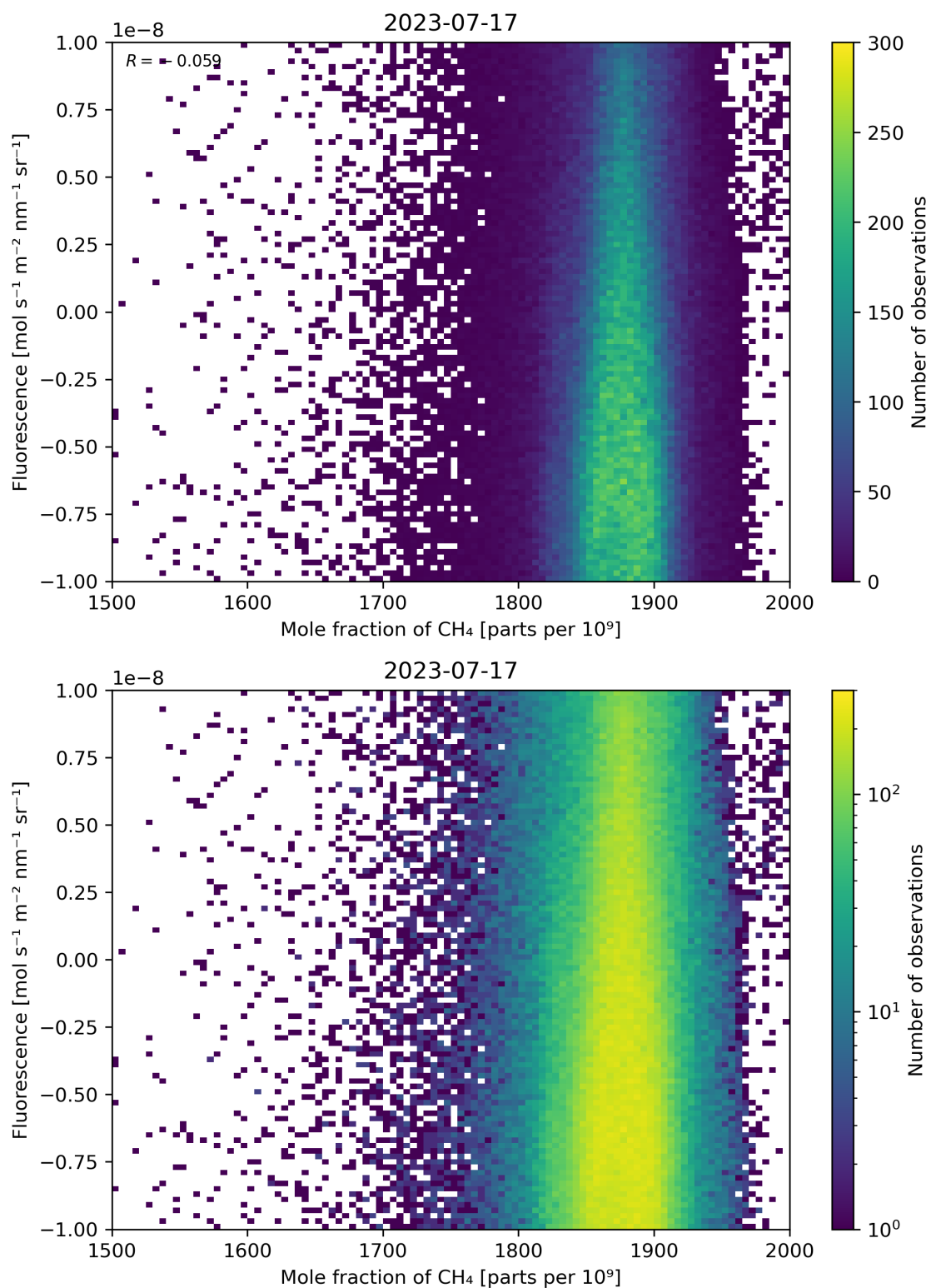
Figure 73: Scatter density plot of “Mole fraction of \text{CH}_4 ” against “Fluorescence” for 2023-07-16 to 2023-07-18.
