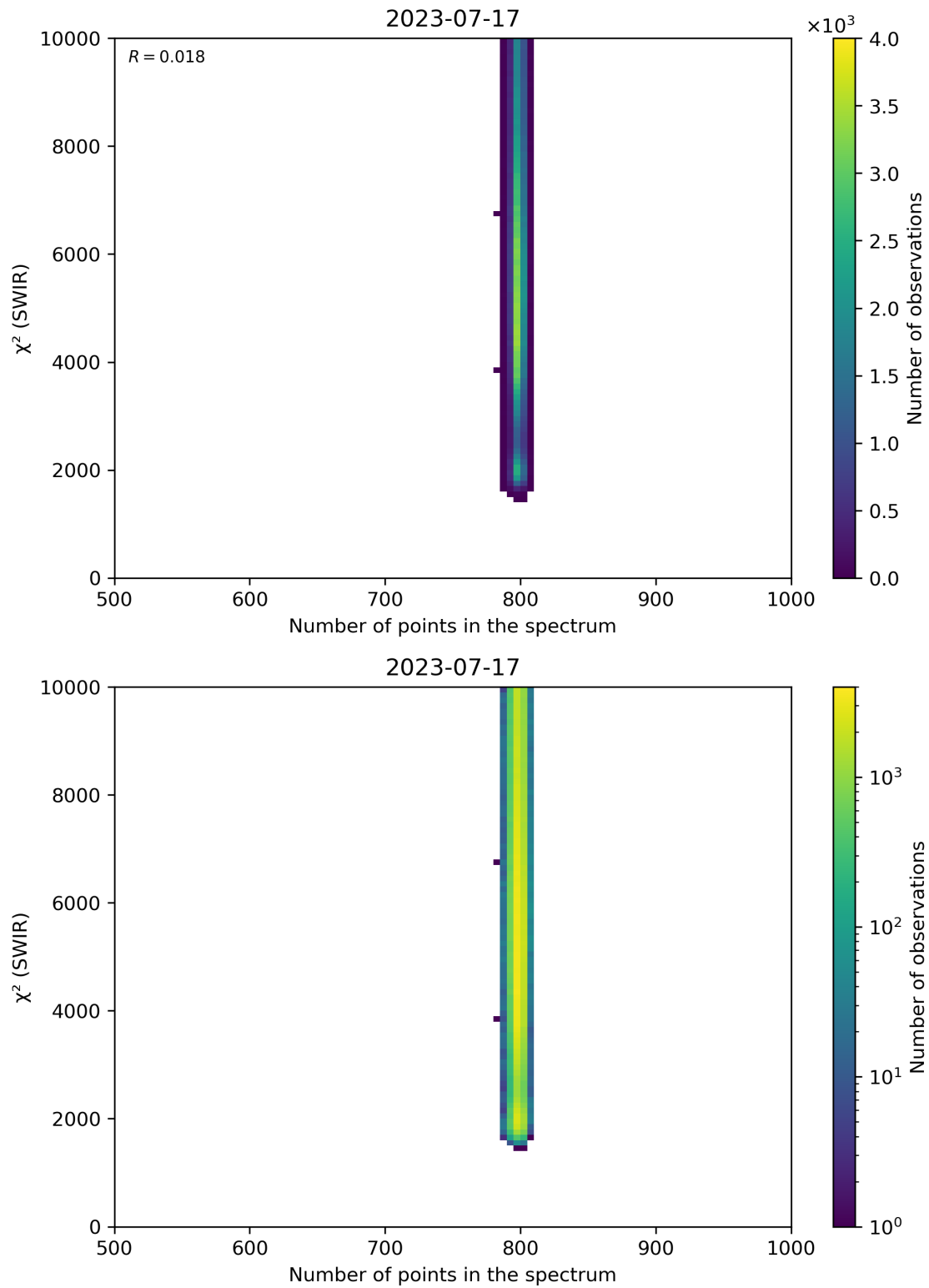
Figure 89: Scatter density plot of “Number of points in the spectrum” against “ \chi^2 (SWIR)” for 2023-07-16 to 2023-07-18.
