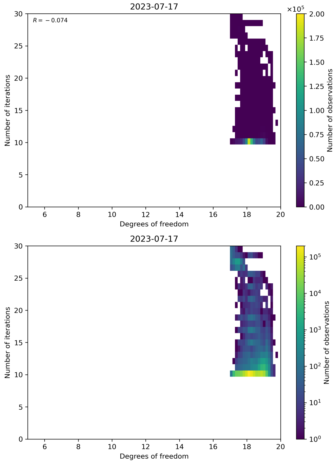
Figure 52: Scatter density plot of “Degrees of freedom” against “Number of iterations” for 2023-07-16 to 2023-07-18.
