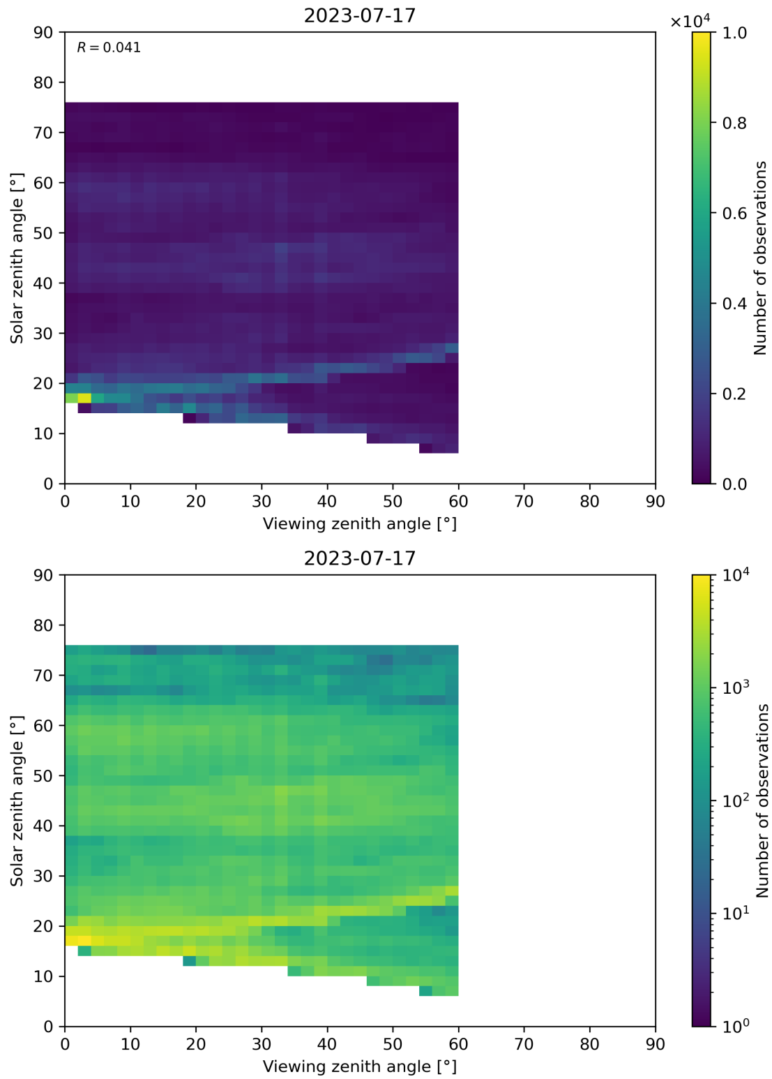
Figure 115: Scatter density plot of “Viewing zenith angle” against “Solar zenith angle” for 2023-07-16 to 2023-07-18.
