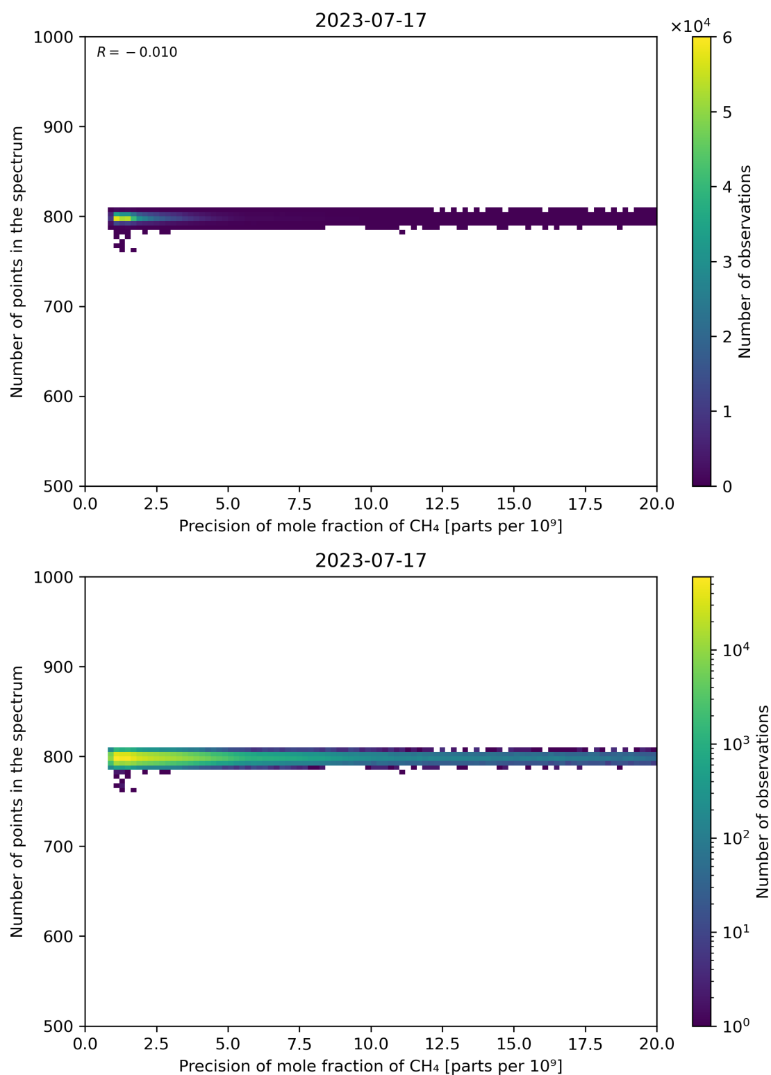
Figure 84: Scatter density plot of “Precision of mole fraction of CH 4 ” against “Number of points in the spectrum” for 2023-07-16 to 2023-07-18.
