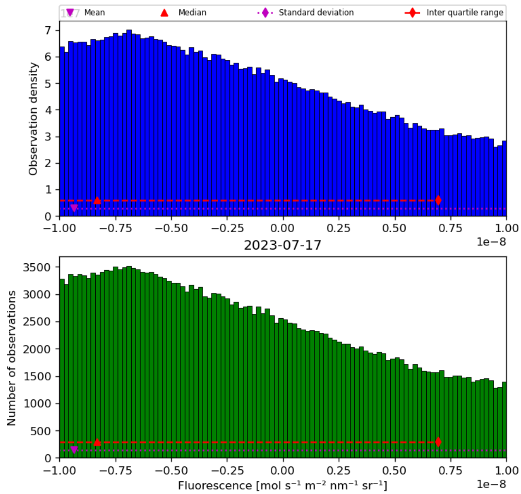
Figure 32: Histogram of “Fluorescence” for 2023-07-16 to 2023-07-18
