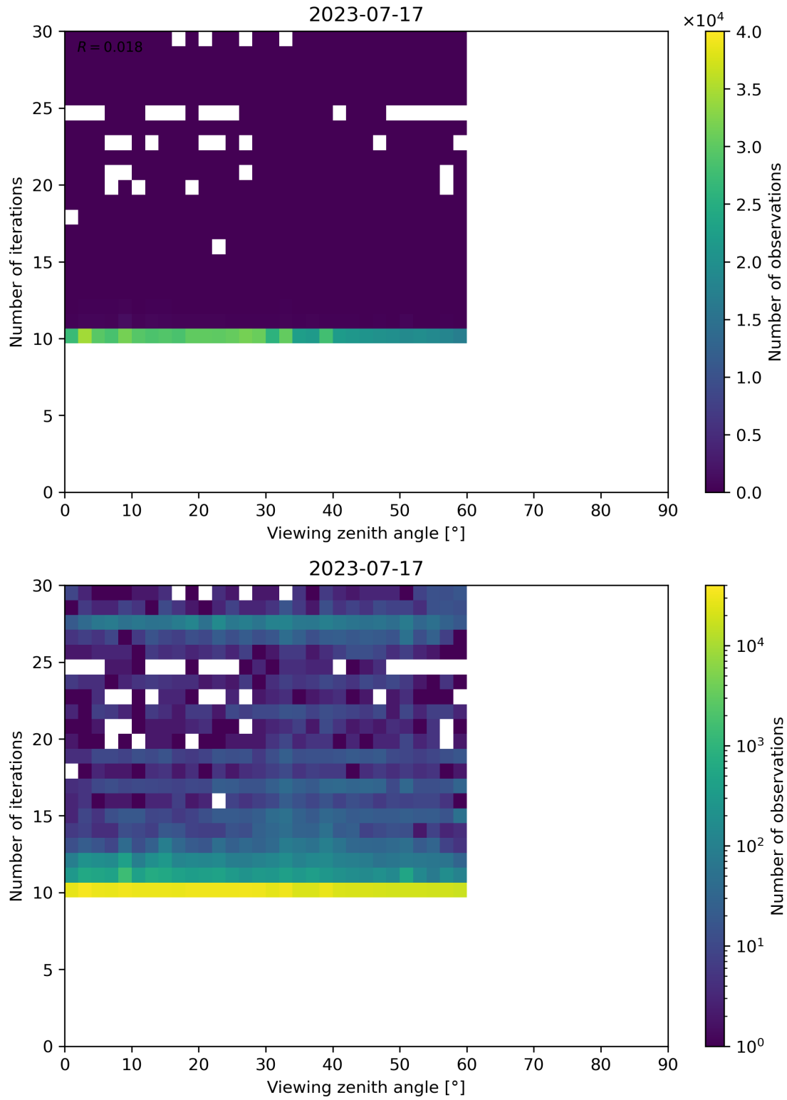
Figure 113: Scatter density plot of “Viewing zenith angle” against “Number of iterations” for 2023-07-16 to 2023-07-18.
