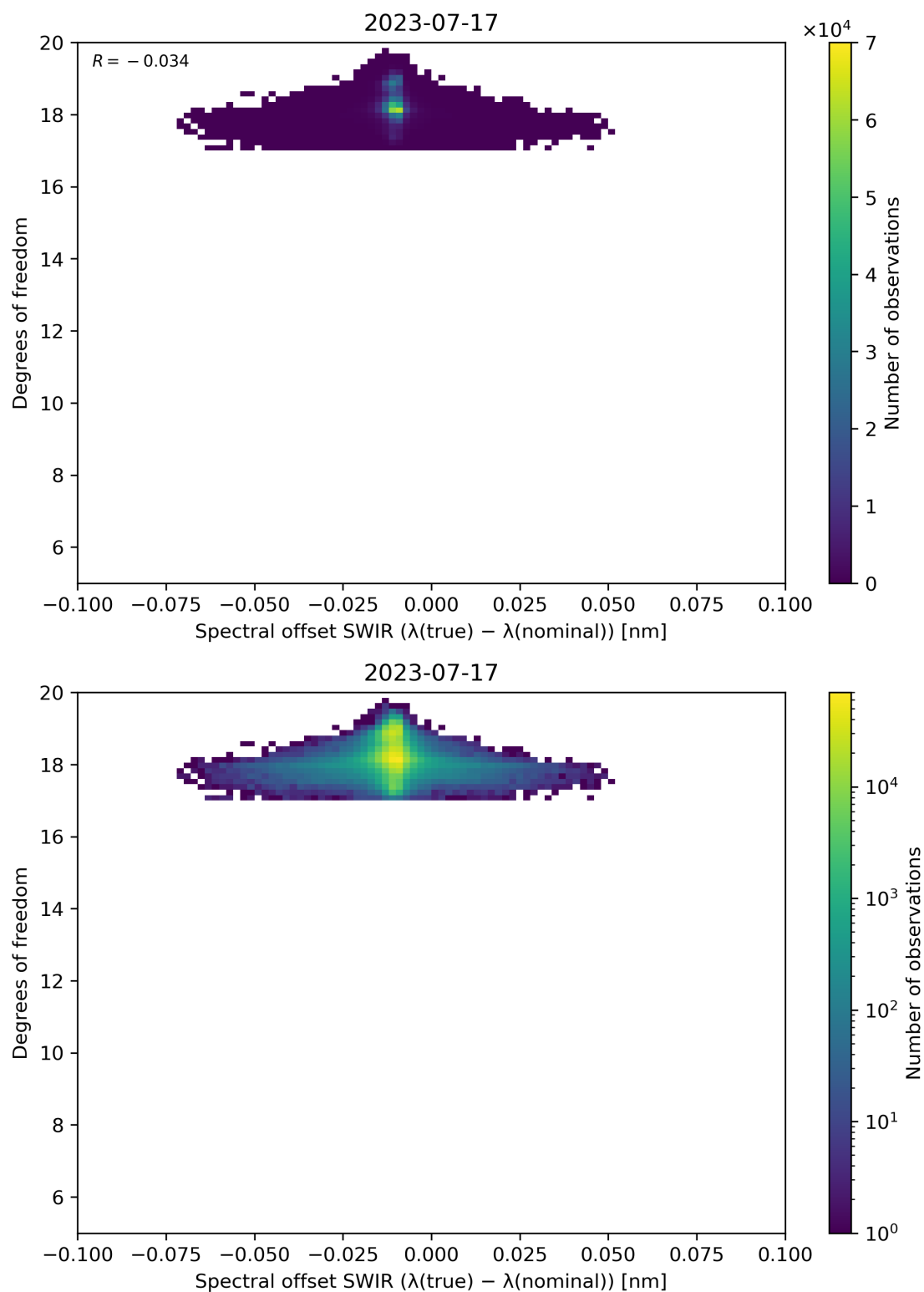
Figure 119: Scatter density plot of “Spectral offset SWIR ( \lambda(\text{true}) - \lambda(\text{nominal}) )” against “Degrees of freedom” for 2023-07-16 to 2023-07-18.
