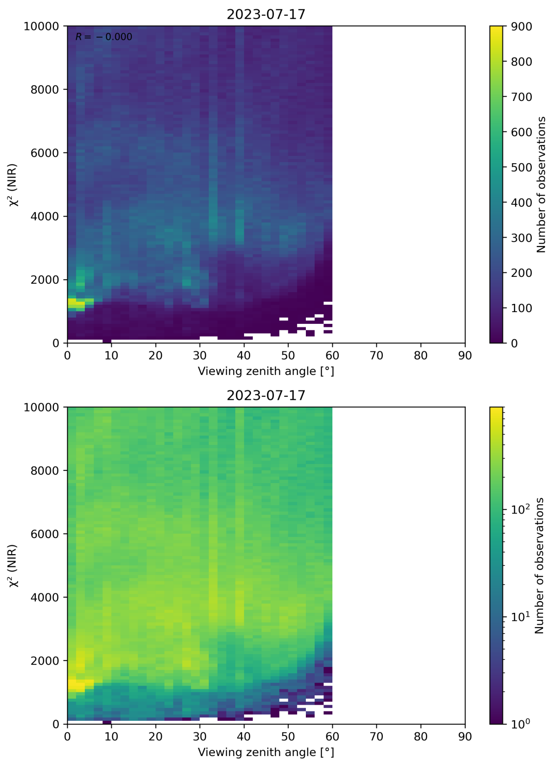
Figure 105: Scatter density plot of “Viewing zenith angle” against “ \chi^2 (NIR)” for 2023-07-16 to 2023-07-18.
