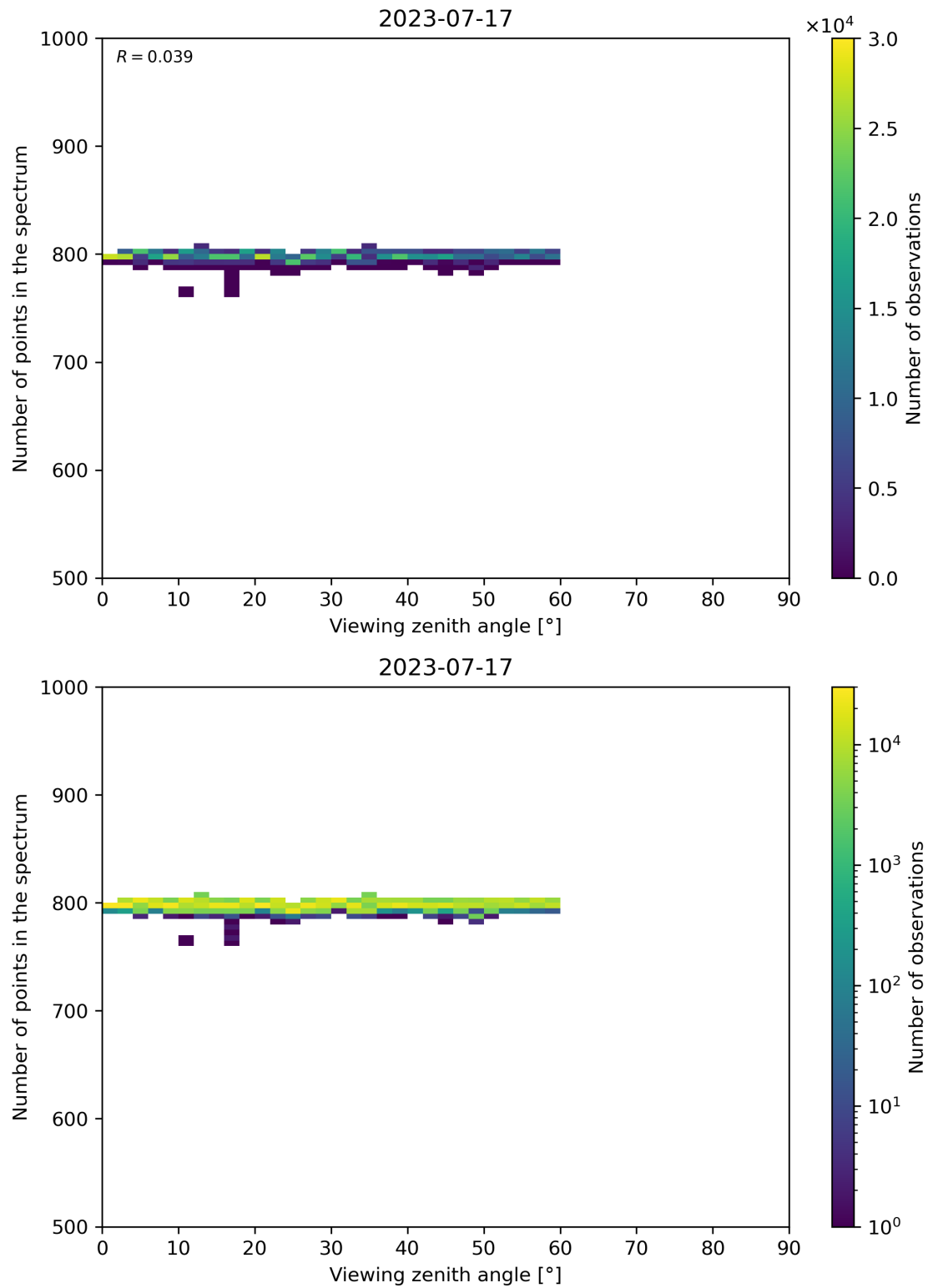
Figure 114: Scatter density plot of “Viewing zenith angle” against “Number of points in the spectrum” for 2023-07-16 to 2023-07-18.
