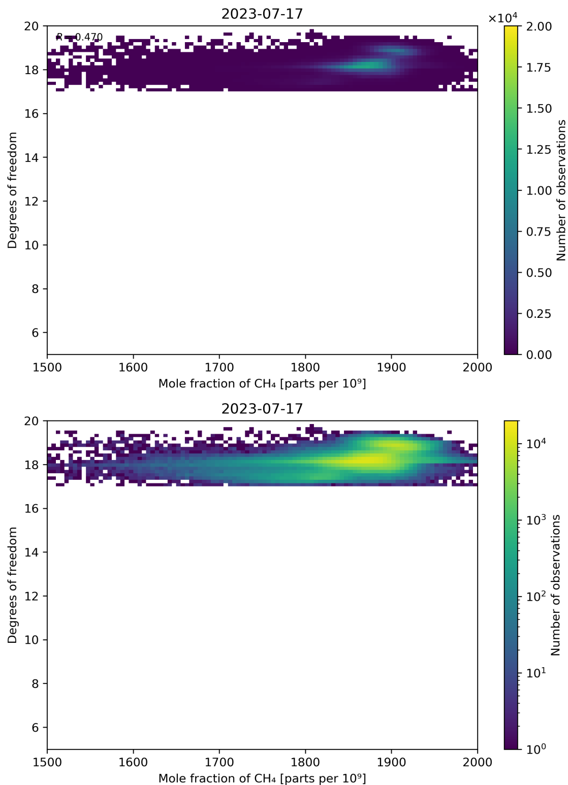
Figure 72: Scatter density plot of “Mole fraction of CH 4 ” against “Degrees of freedom” for 2023-07-16 to 2023-07-18.
