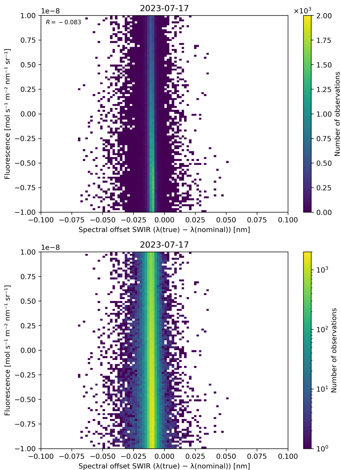
Figure 120: Scatter density plot of “Spectral offset SWIR ( \lambda(\text{true}) - \lambda(\text{nominal}) )” against “Fluorescence” for 2023-07-16 to 2023-07-18.
