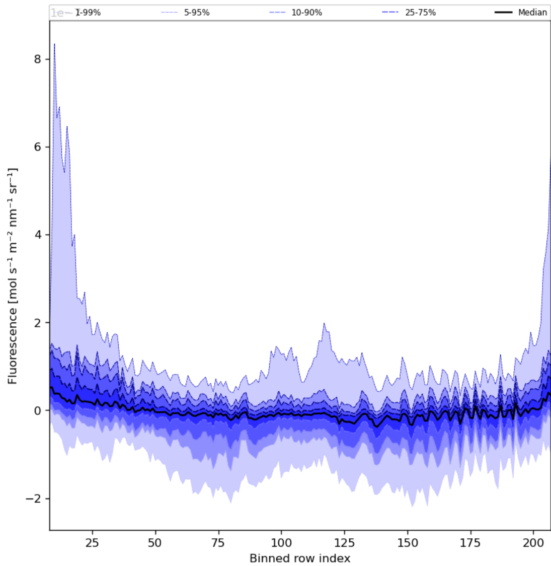
Figure 43: Along track statistics of “Fluorescence” for 2023-07-16 to 2023-07-18
