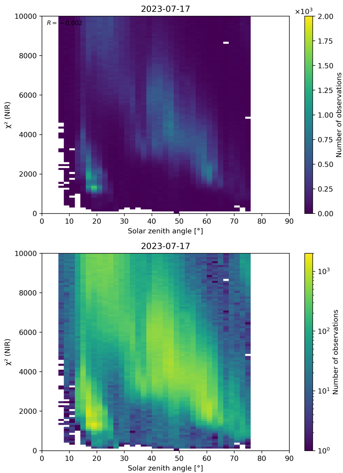
Figure 94: Scatter density plot of “Solar zenith angle” against “ \chi^2 (NIR)” for 2023-07-16 to 2023-07-18.
