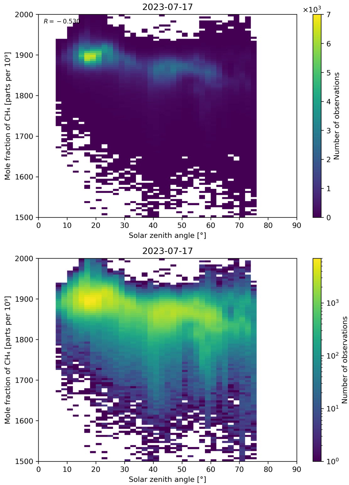
Figure 99: Scatter density plot of “Solar zenith angle” against “Mole fraction of CH 4 ” for 2023-07-16 to 2023-07-18.
