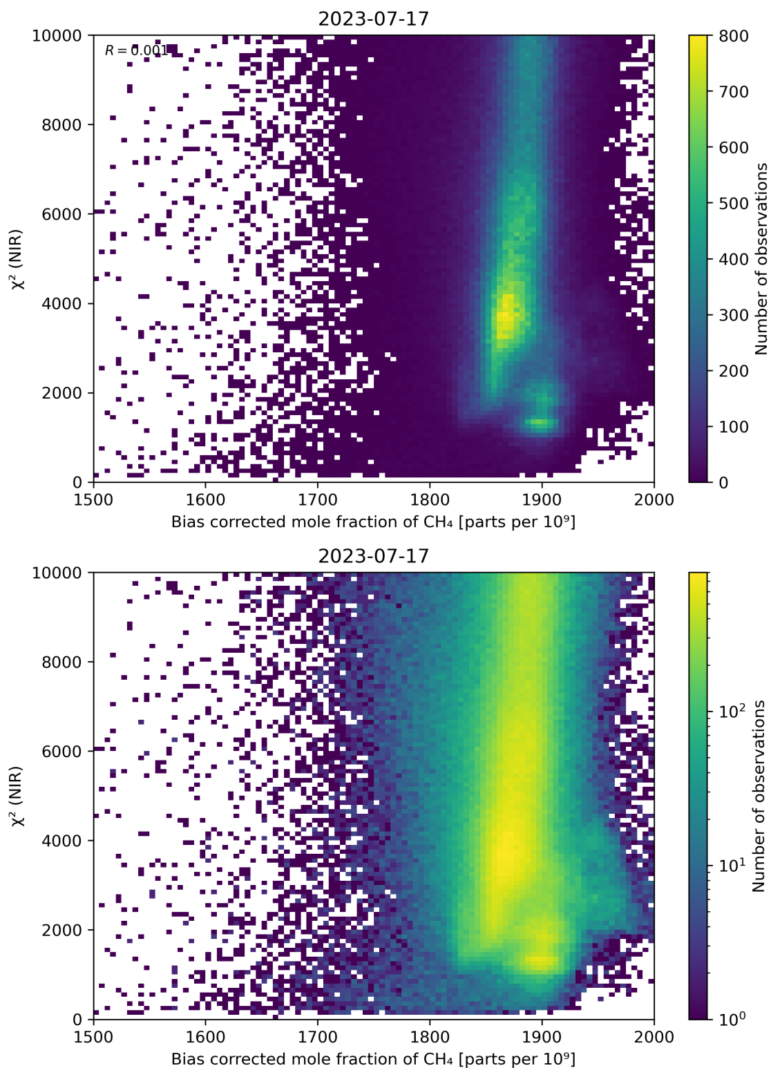
Figure 63: Scatter density plot of “Bias corrected mole fraction of CH 4 ” against “ \chi^2 (NIR)” for 2023-07-16 to 2023-07-18.
