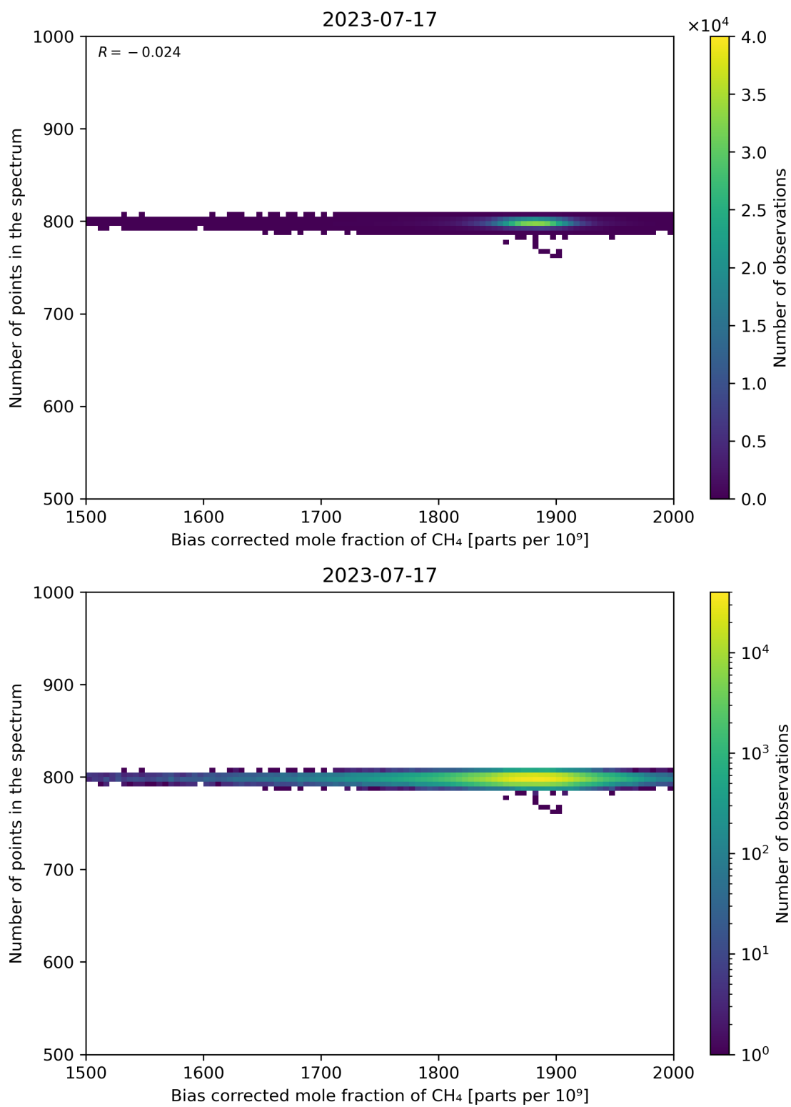
Figure 68: Scatter density plot of “Bias corrected mole fraction of CH 4 ” against “Number of points in the spectrum” for 2023-07-16 to 2023-07-18.
