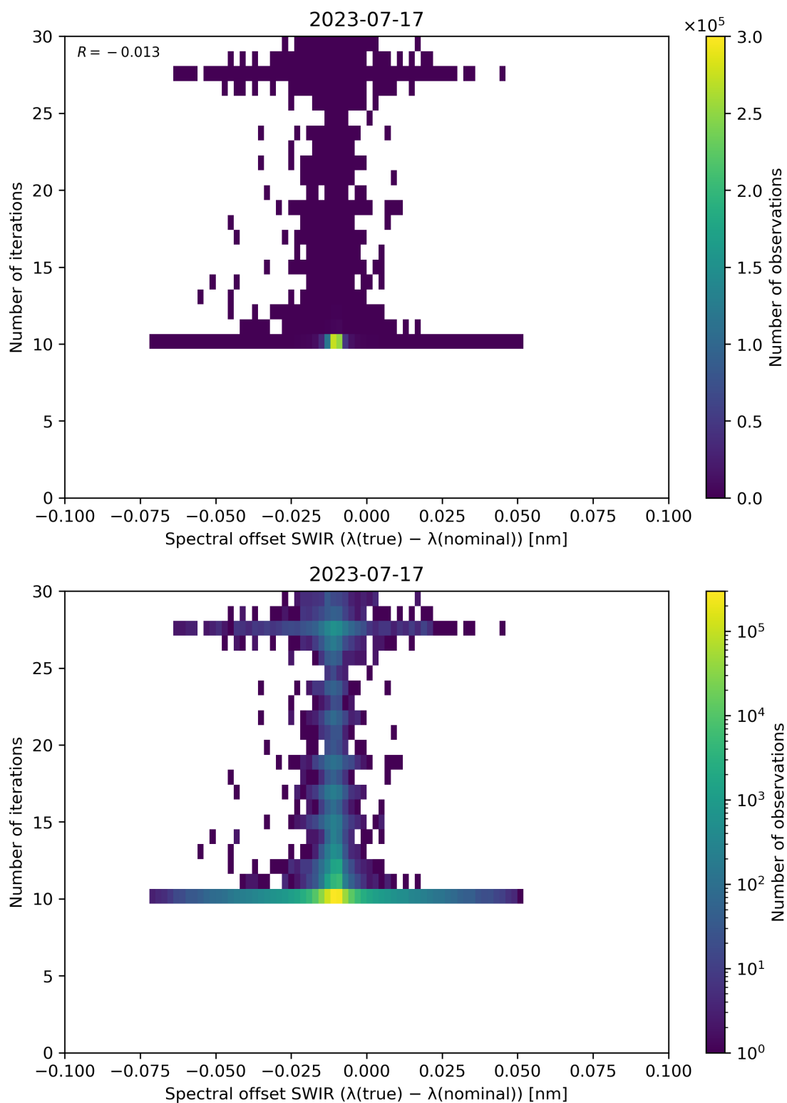
Figure 121: Scatter density plot of “Spectral offset SWIR ( \lambda(\text{true}) - \lambda(\text{nominal}) )” against “Number of iterations” for 2023-07-16 to 2023-07-18.
