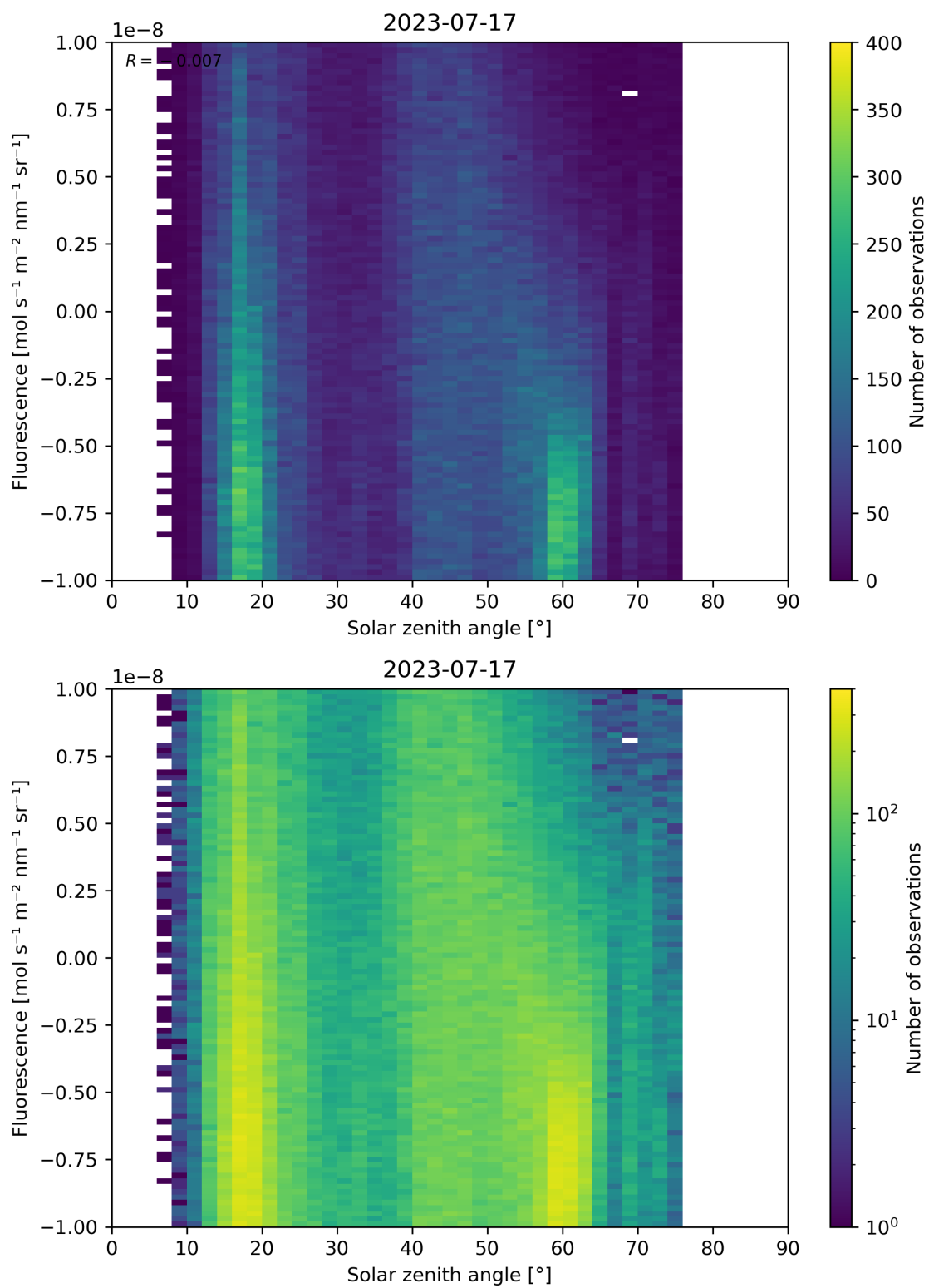
Figure 97: Scatter density plot of “Solar zenith angle” against “Fluorescence” for 2023-07-16 to 2023-07-18.
