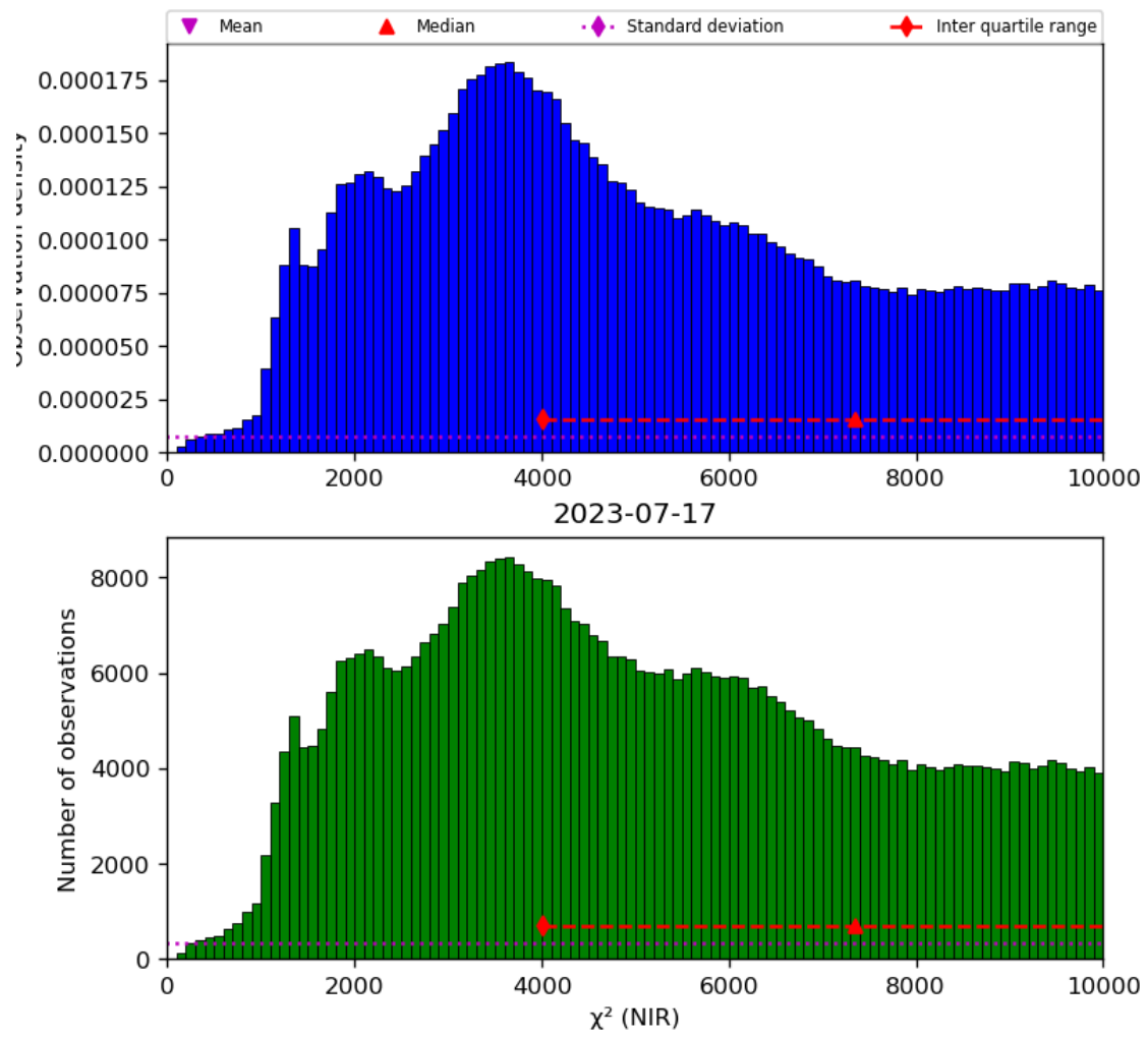
Figure 29: Histogram of “ \chi^2 (NIR)” for 2023-07-16 to 2023-07-18
