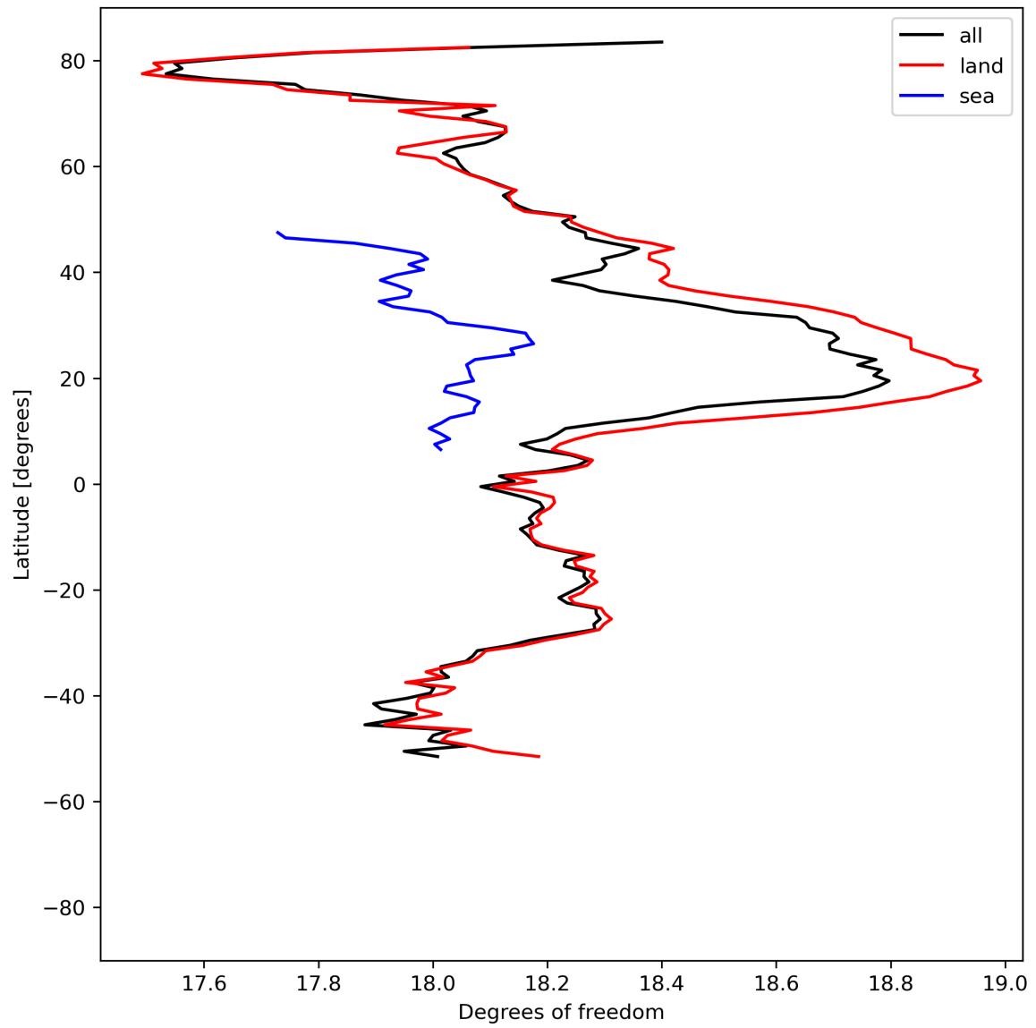
Figure 19: Zonal average of “Degrees of freedom” for 2023-07-16 to 2023-07-18.
