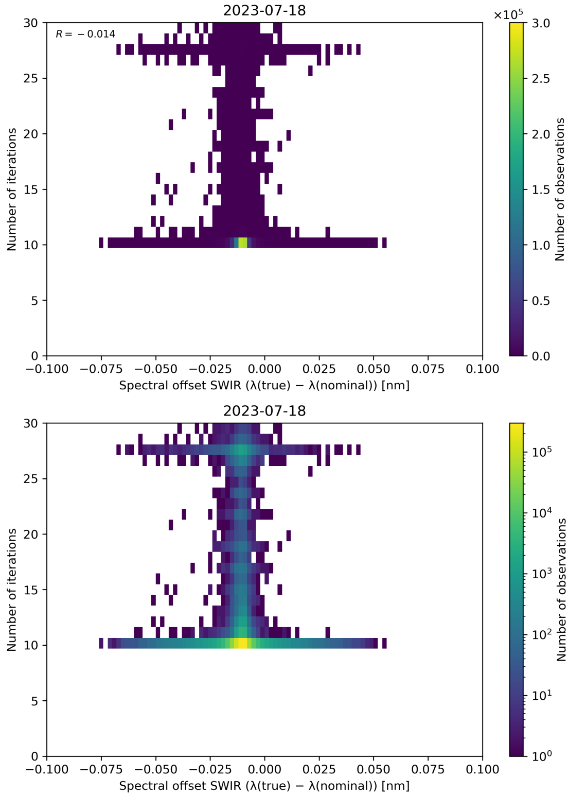
Figure 121: Scatter density plot of “Spectral offset SWIR ( \lambda(\text{true}) - \lambda(\text{nominal}) )” against “Number of iterations” for 2023-07-17 to 2023-07-19.
