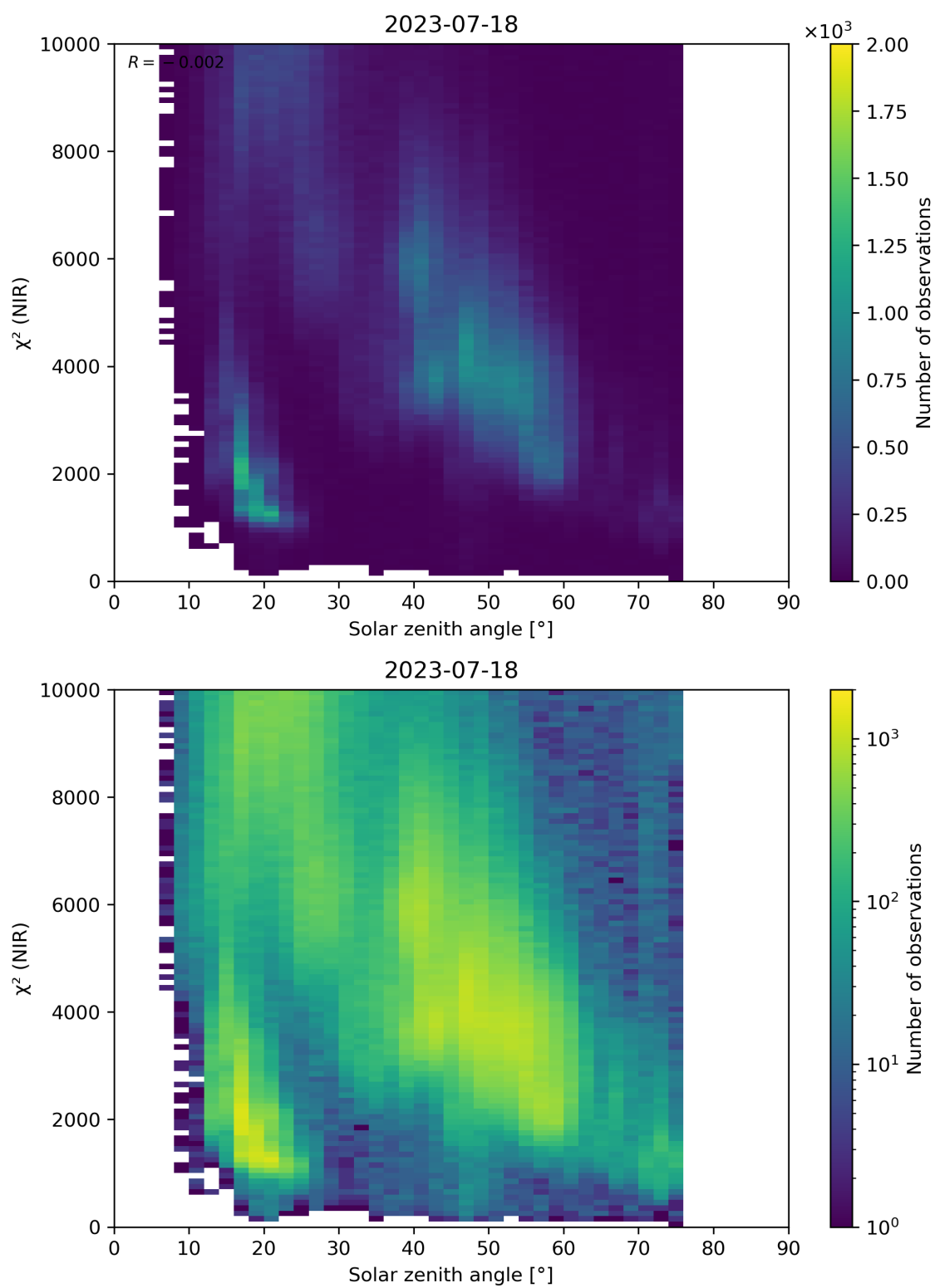
Figure 94: Scatter density plot of “Solar zenith angle” against “ \chi^2 (NIR)” for 2023-07-17 to 2023-07-19.
