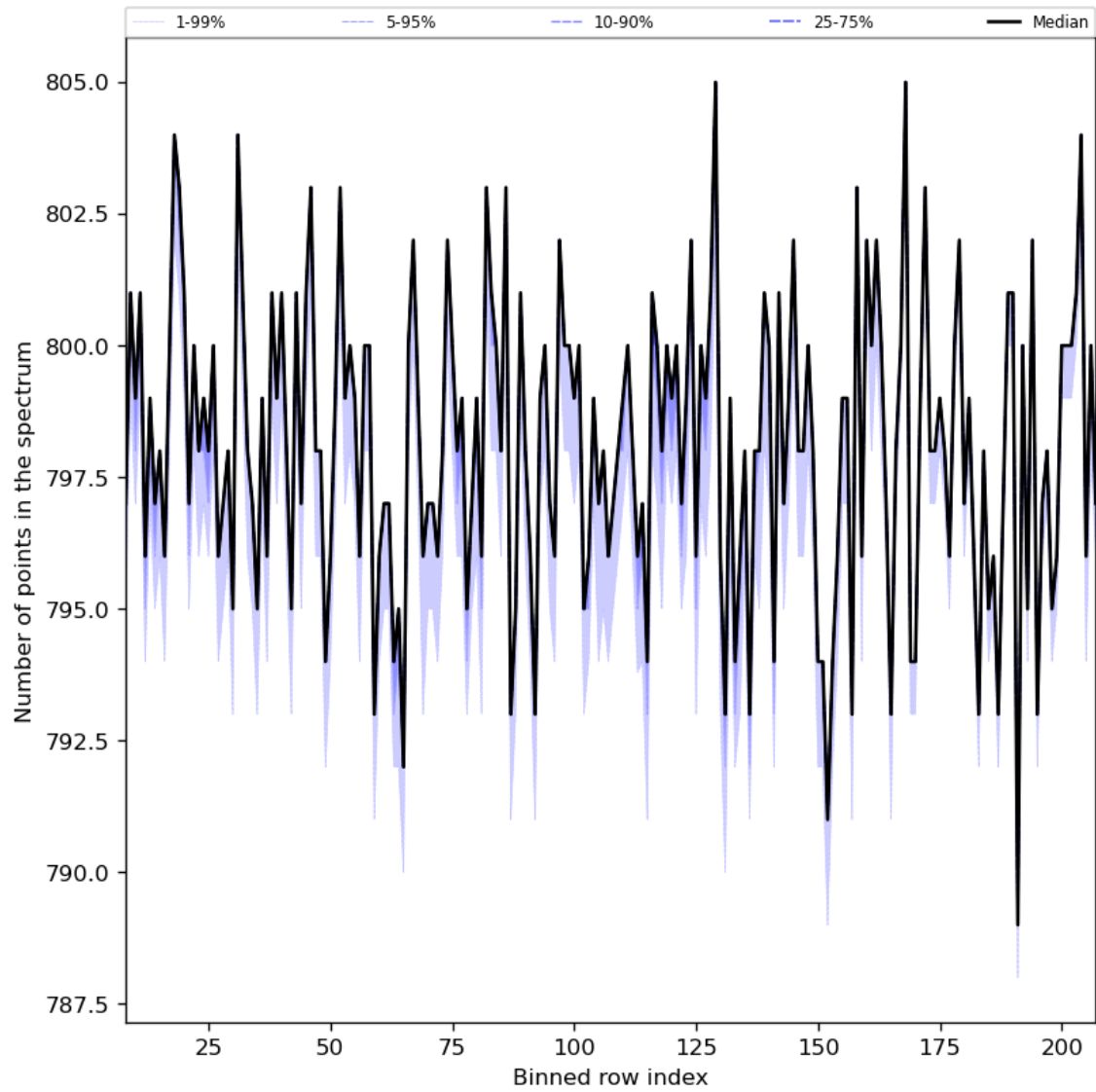
Figure 37: Along track statistics of “Number of points in the spectrum” for 2023-07-17 to 2023-07-19
