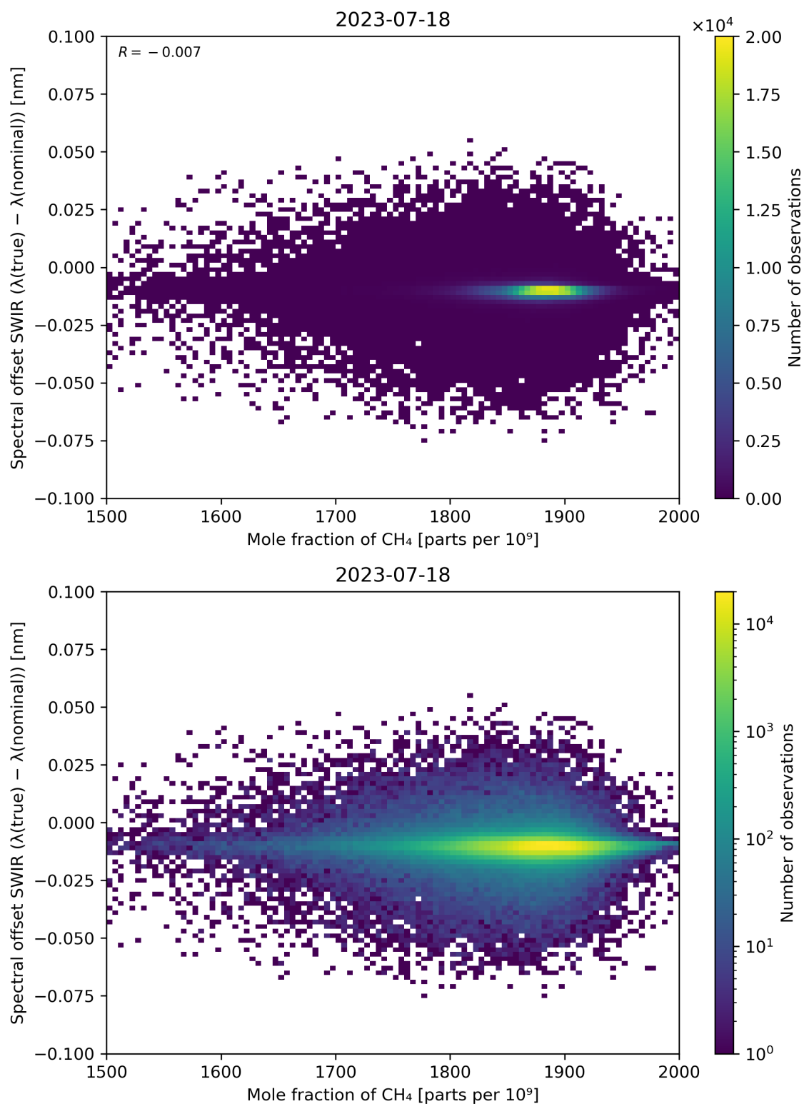
Figure 86: Scatter density plot of “Mole fraction of CH 4 ” against “Spectral offset SWIR ( \lambda(\text{true}) - \lambda(\text{nominal}) )” for 2023-07-17 to 2023-07-19.
