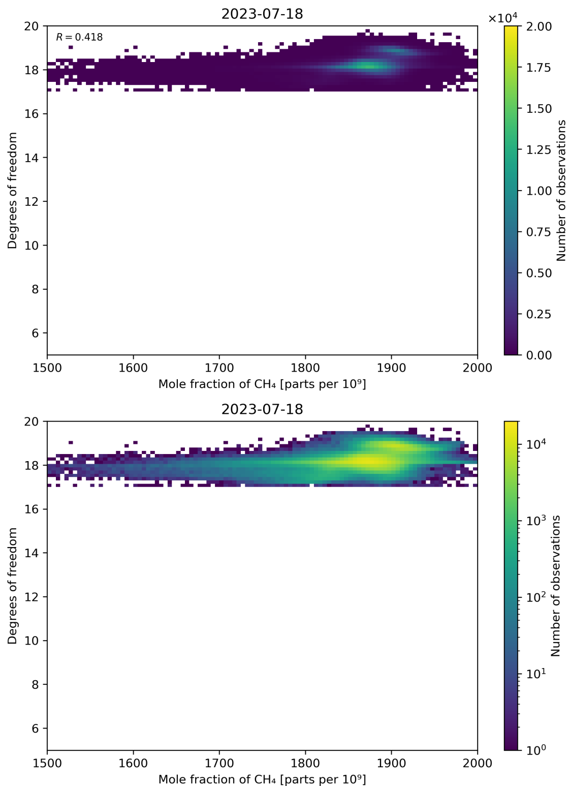
Figure 72: Scatter density plot of “Mole fraction of CH 4 ” against “Degrees of freedom” for 2023-07-17 to 2023-07-19.
