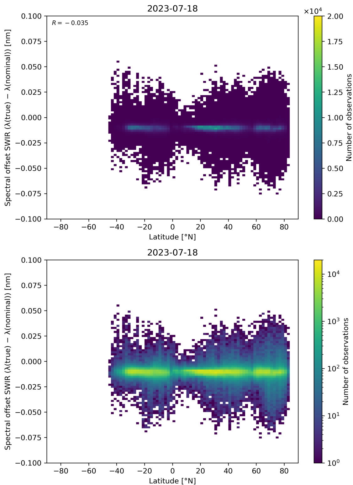
Figure 62: Scatter density plot of “Latitude” against “Spectral offset SWIR ( \lambda(\text{true}) - \lambda(\text{nominal}) )” for 2023-07-17 to 2023-07-19.
