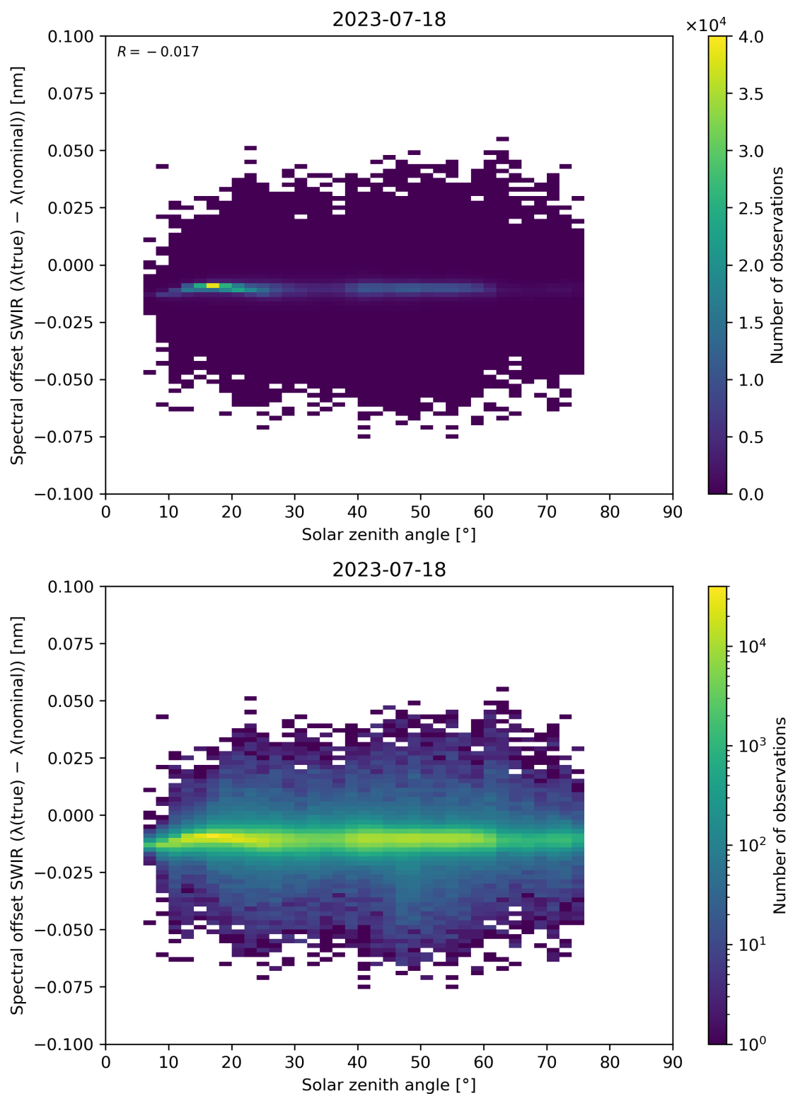
Figure 104: Scatter density plot of “Solar zenith angle” against “Spectral offset SWIR ( \lambda(\text{true}) - \lambda(\text{nominal}) )” for 2023-07-17 to 2023-07-19.
