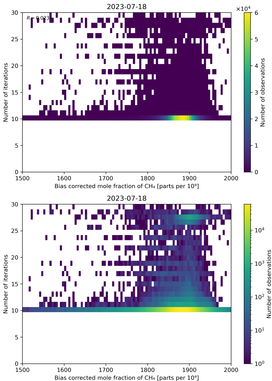
Figure 67: Scatter density plot of “Bias corrected mole fraction of CH 4 ” against “Number of iterations” for 2023-07-17 to 2023-07-19.
