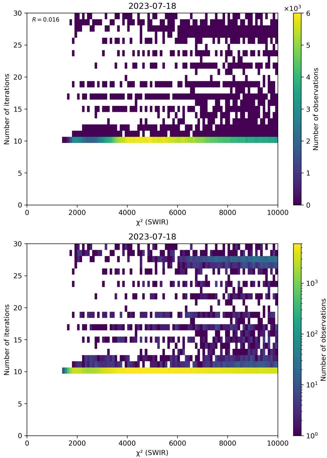
Figure 50: Scatter density plot of “ \chi^2 (SWIR)” against “Number of iterations” for 2023-07-17 to 2023-07-19.
