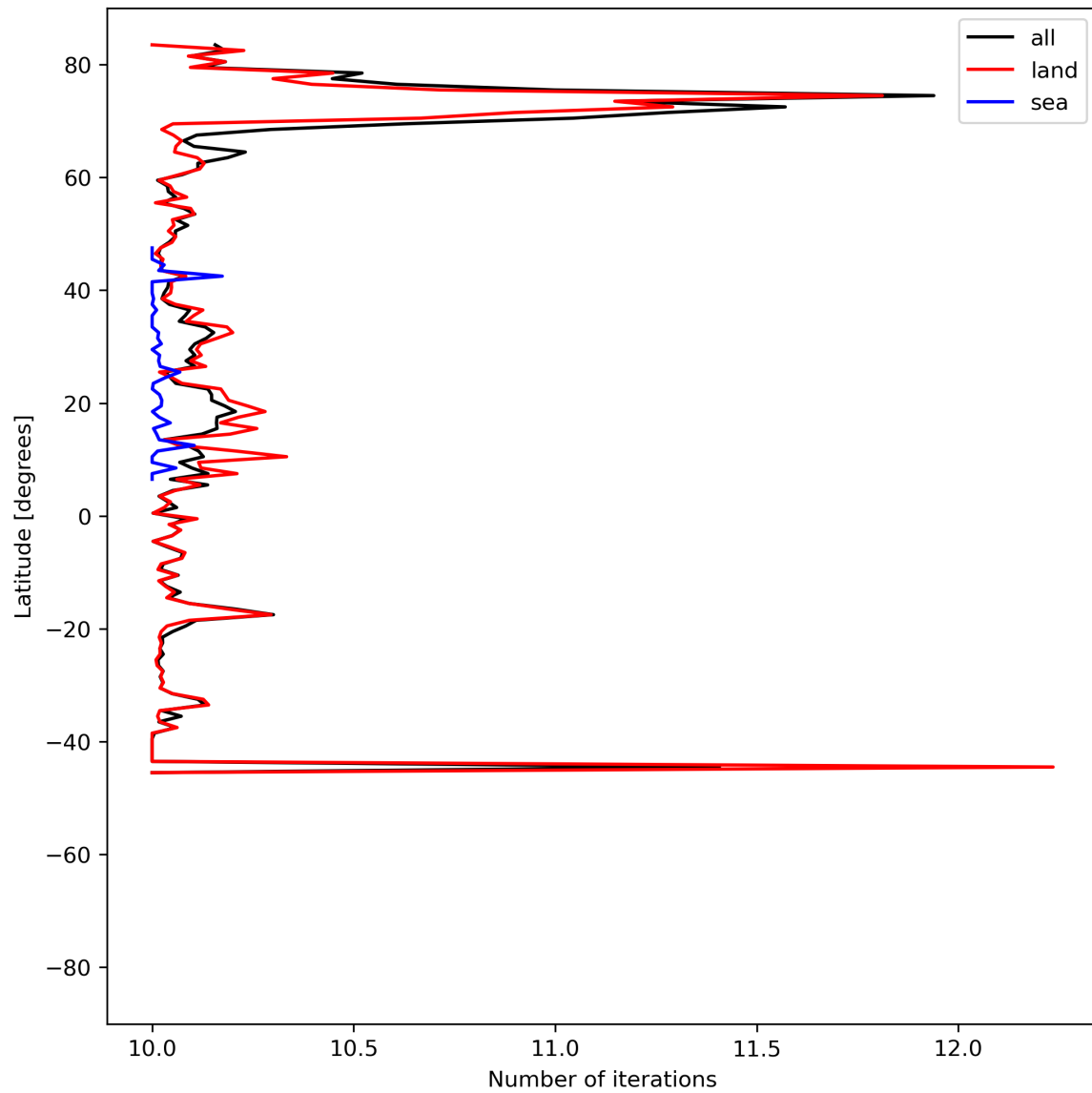
Figure 20: Zonal average of “Number of iterations” for 2023-07-17 to 2023-07-19.
