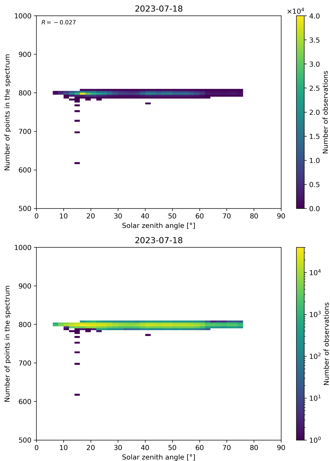
Figure 103: Scatter density plot of “Solar zenith angle” against “Number of points in the spectrum” for 2023-07-17 to 2023-07-19.
