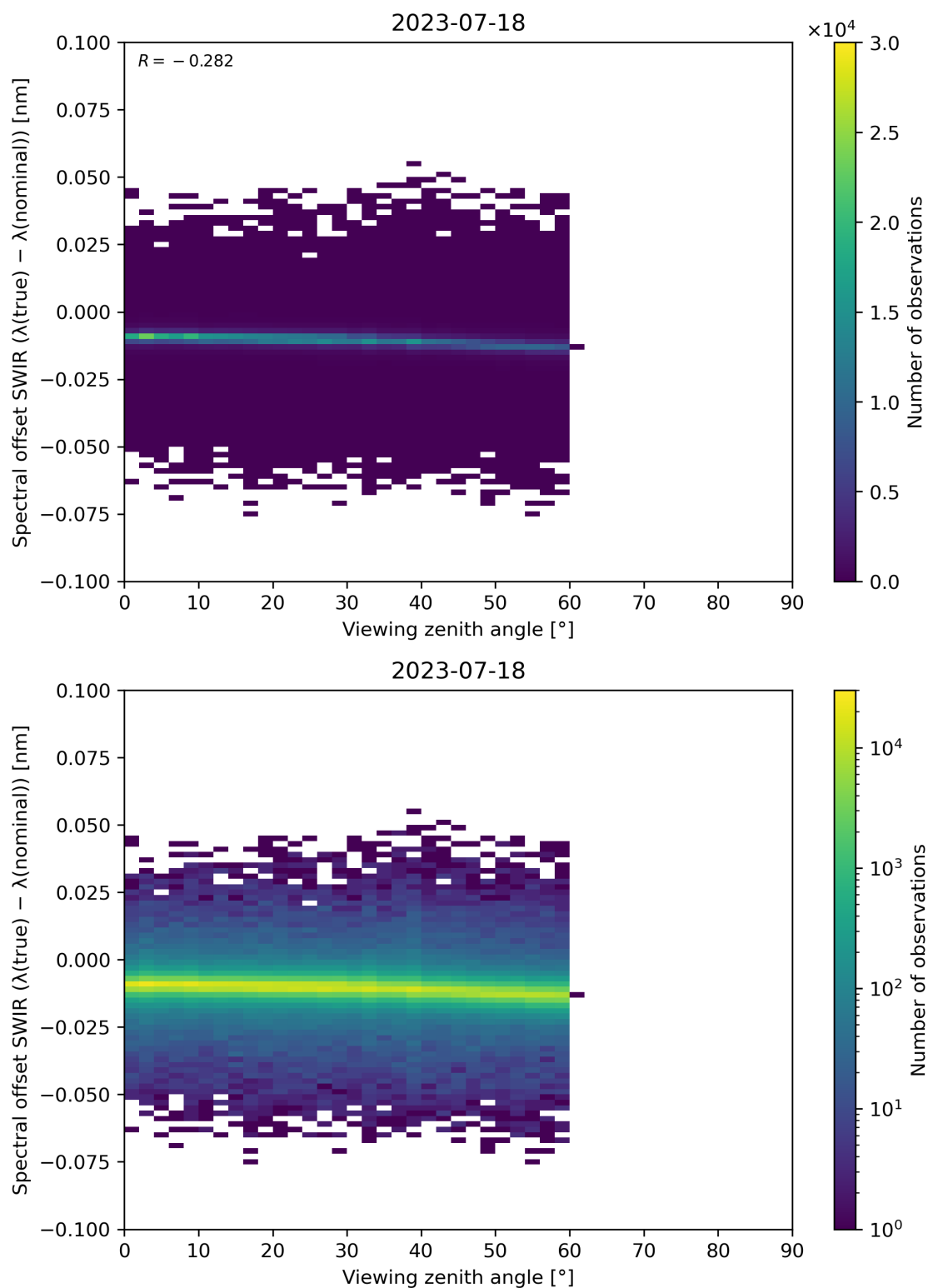
Figure 116: Scatter density plot of “Viewing zenith angle” against “Spectral offset SWIR ( \lambda(\text{true}) - \lambda(\text{nominal}) )” for 2023-07-17 to 2023-07-19.
