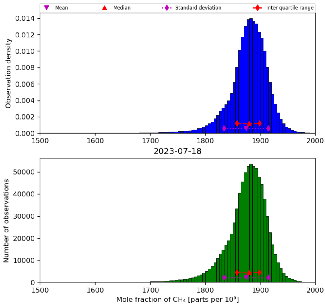
Figure 23: Histogram of “Mole fraction of CH 4 ” for 2023-07-17 to 2023-07-19
