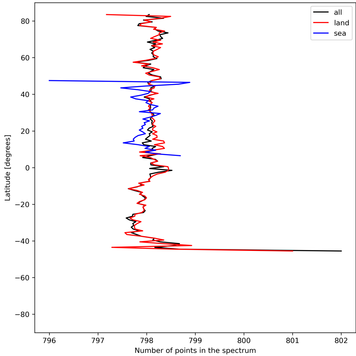
Figure 15: Zonal average of “Number of points in the spectrum” for 2023-07-17 to 2023-07-19.
