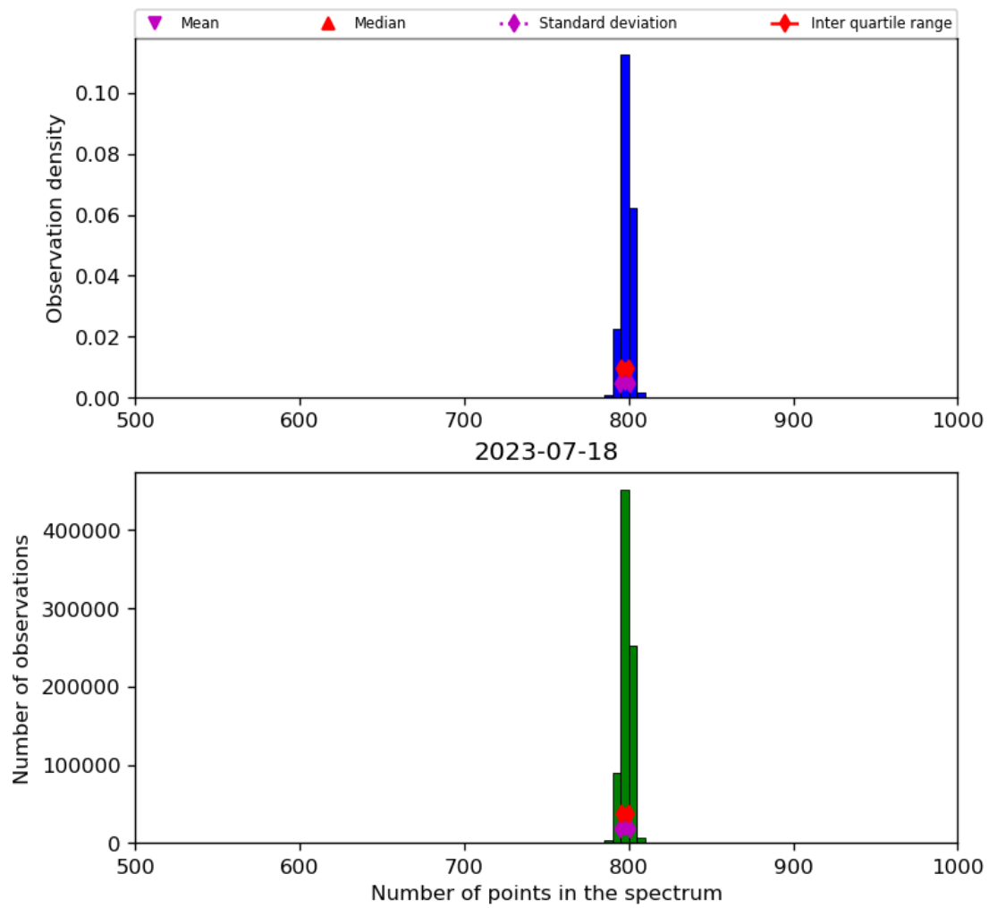
Figure 26: Histogram of “Number of points in the spectrum” for 2023-07-17 to 2023-07-19
