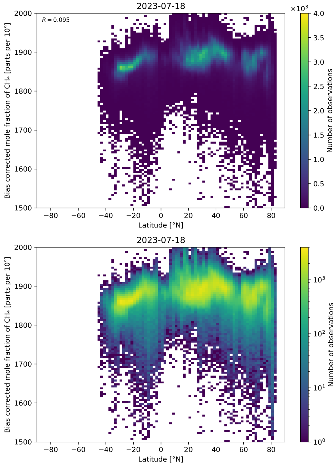
Figure 58: Scatter density plot of “Latitude” against “Bias corrected mole fraction of \text{CH}_4 ” for 2023-07-17 to 2023-07-19.
