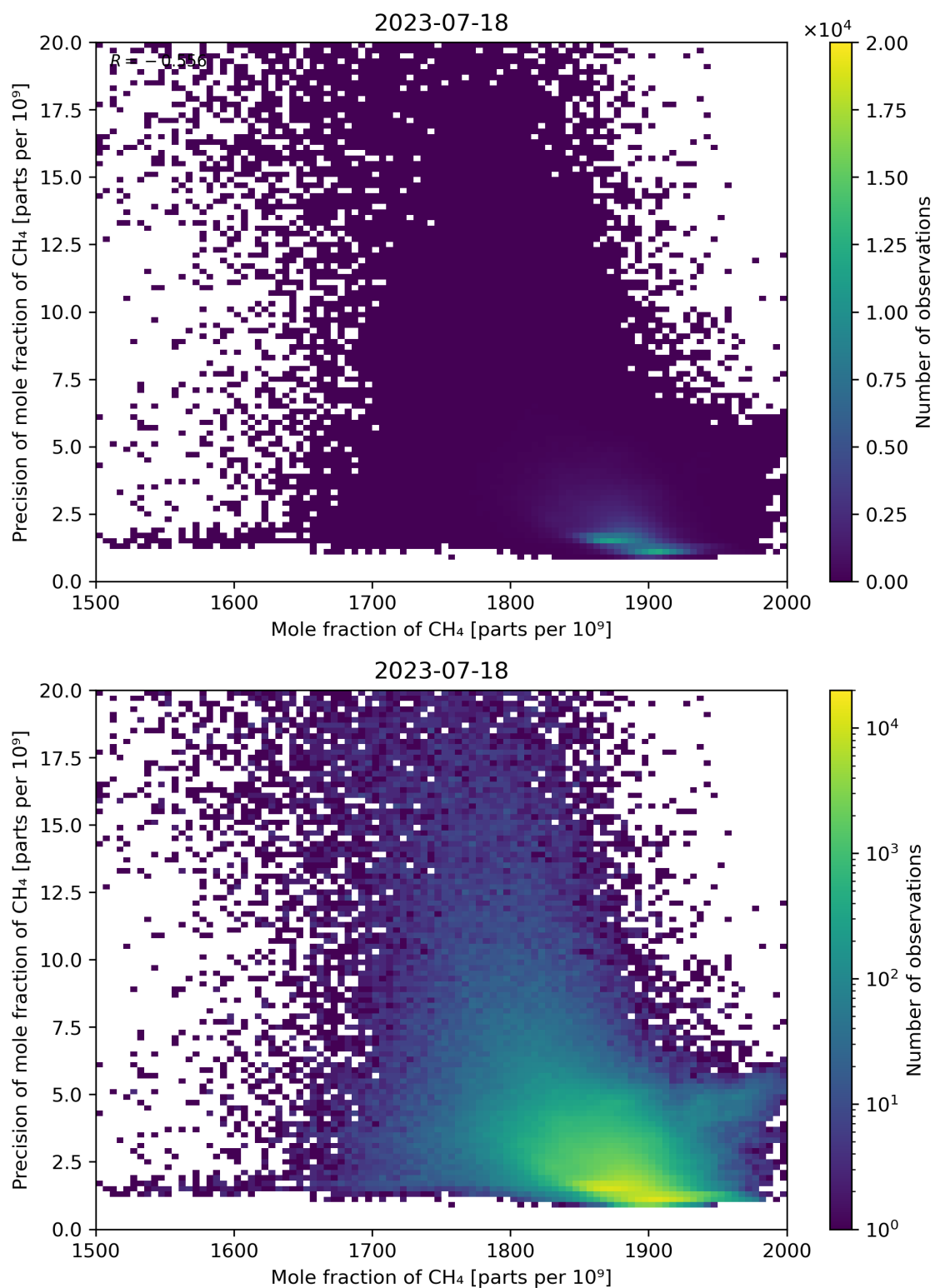
Figure 75: Scatter density plot of “Mole fraction of CH 4 ” against “Precision of mole fraction of CH 4 ” for 2023-07-17 to 2023-07-19.
