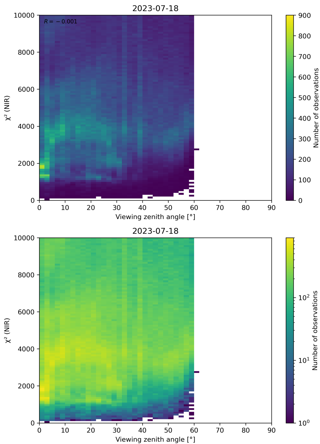
Figure 105: Scatter density plot of “Viewing zenith angle” against “ \chi^2 (NIR)” for 2023-07-17 to 2023-07-19.
