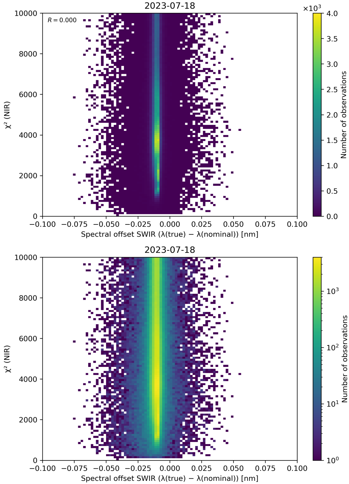
Figure 117: Scatter density plot of “Spectral offset SWIR ( \lambda(\text{true}) - \lambda(\text{nominal}) )” against “ \chi^2 (NIR)” for 2023-07-17 to 2023-07-19.
