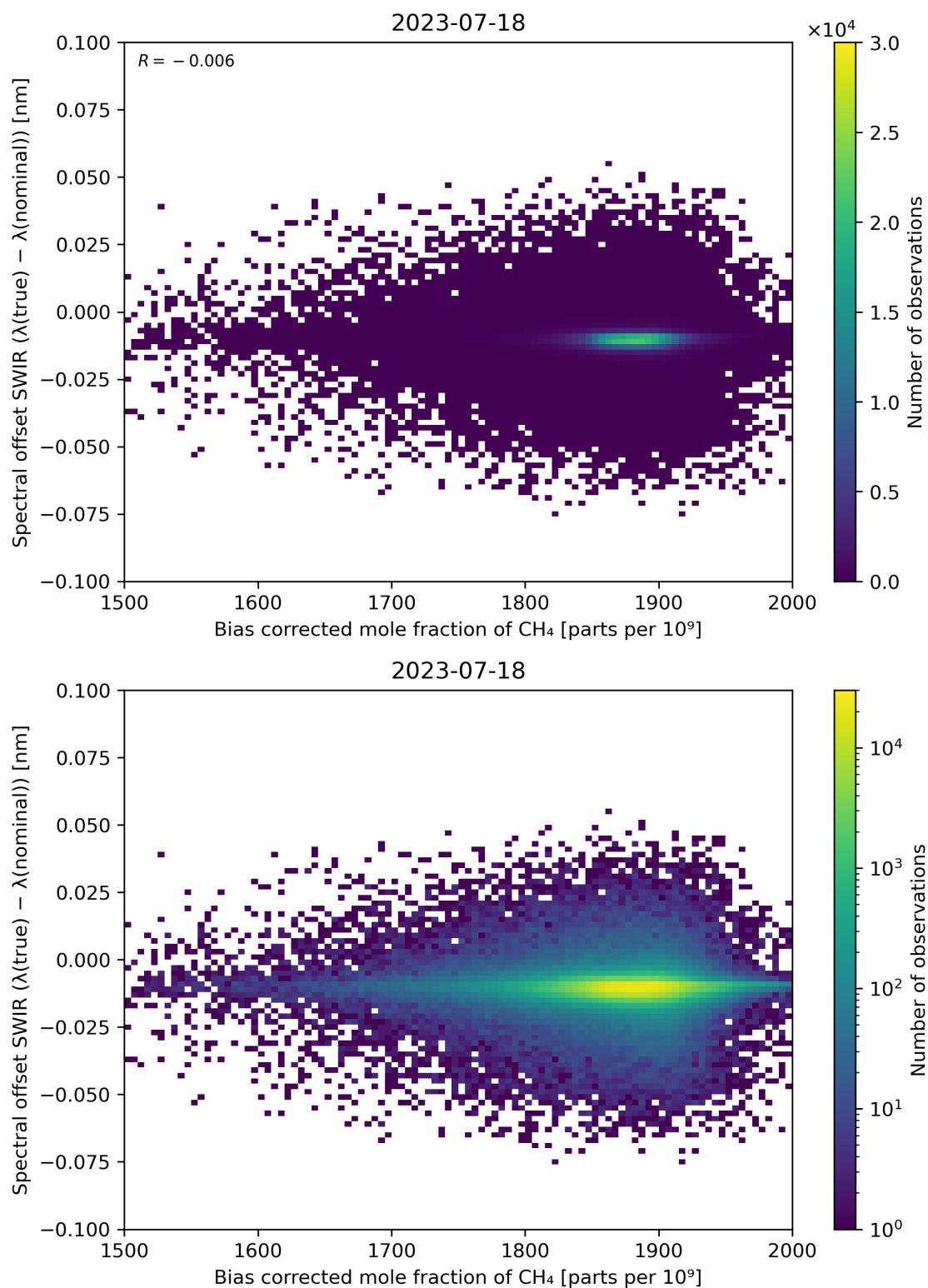
Figure 69: Scatter density plot of “Bias corrected mole fraction of \text{CH}_4 ” against “Spectral offset SWIR ( \lambda(\text{true}) - \lambda(\text{nominal}) )” for 2023-07-17 to 2023-07-19.
