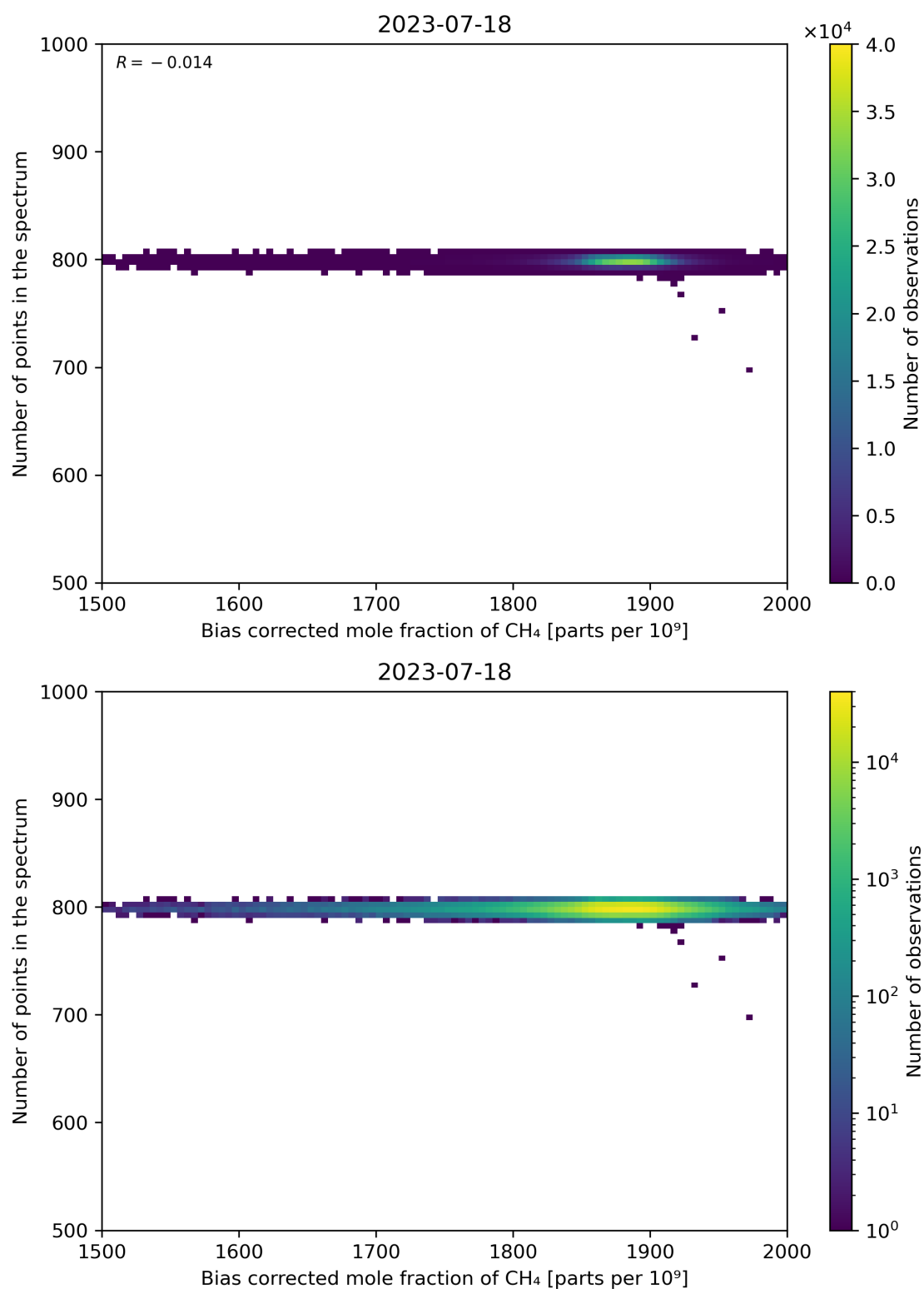
Figure 68: Scatter density plot of “Bias corrected mole fraction of CH 4 ” against “Number of points in the spectrum” for 2023-07-17 to 2023-07-19.
