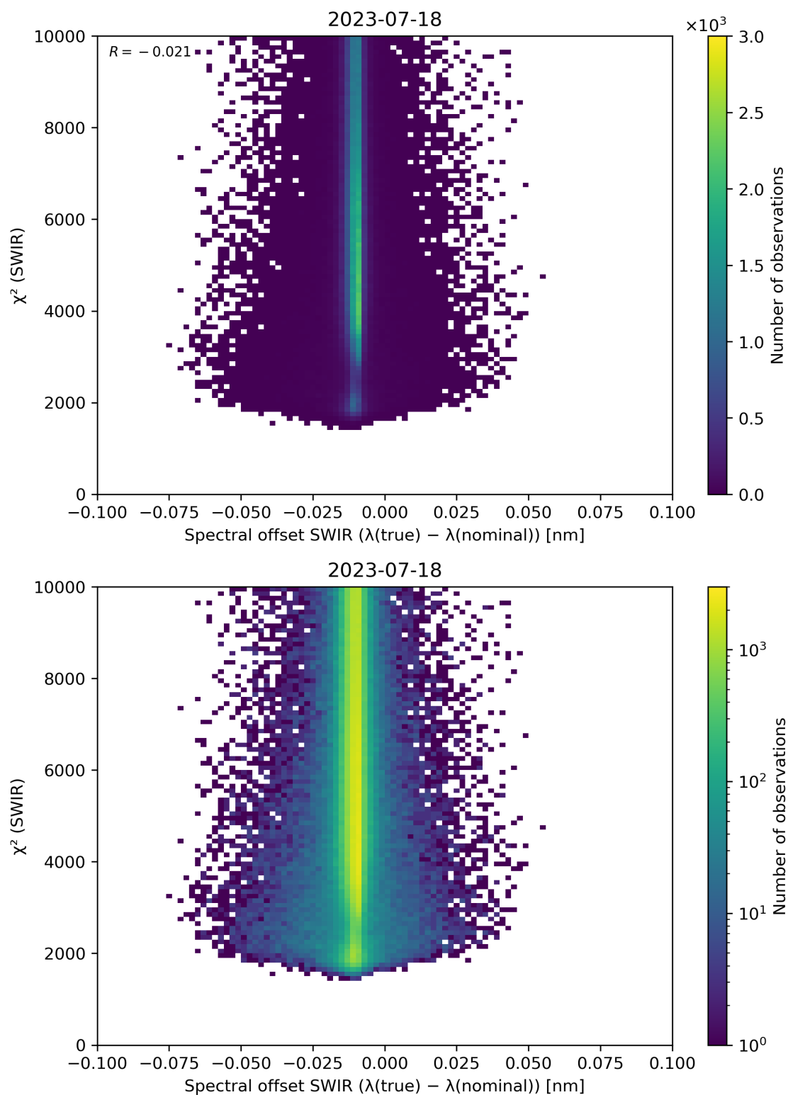
Figure 118: Scatter density plot of “Spectral offset SWIR ( \lambda(\text{true}) - \lambda(\text{nominal}) )” against “ \chi^2 (SWIR)” for 2023-07-17 to 2023-07-19.
