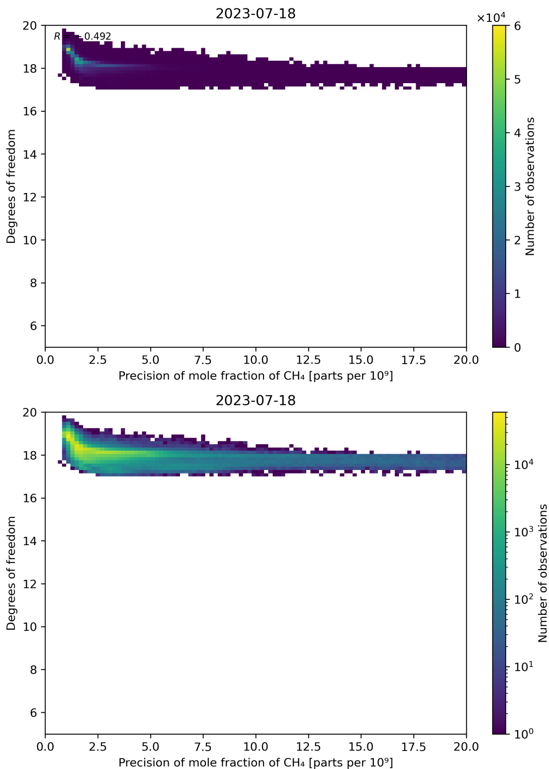
Figure 80: Scatter density plot of “Precision of mole fraction of CH 4 ” against “Degrees of freedom” for 2023-07-17 to 2023-07-19.
