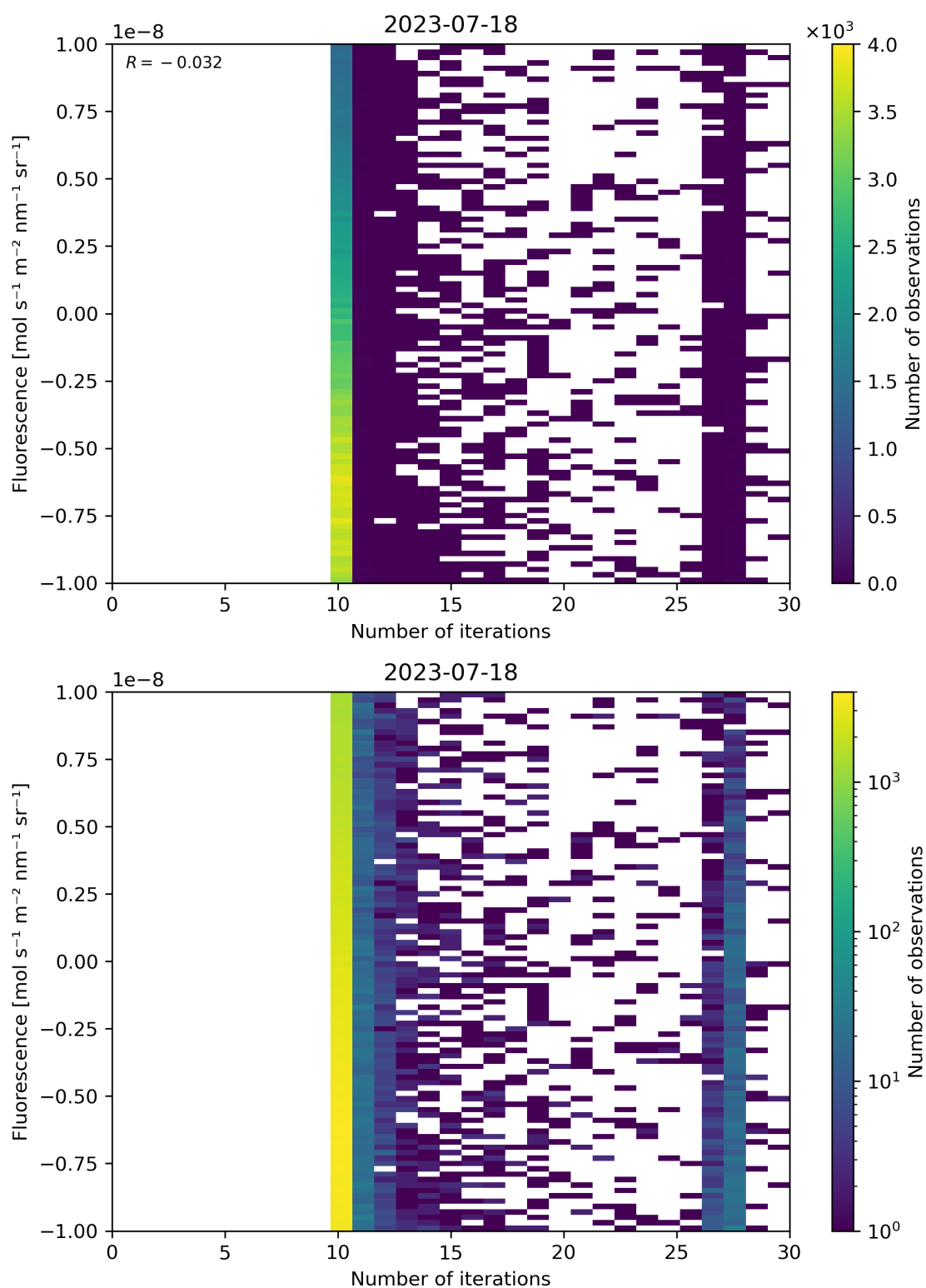
Figure 87: Scatter density plot of “Number of iterations” against “Fluorescence” for 2023-07-17 to 2023-07-19.
