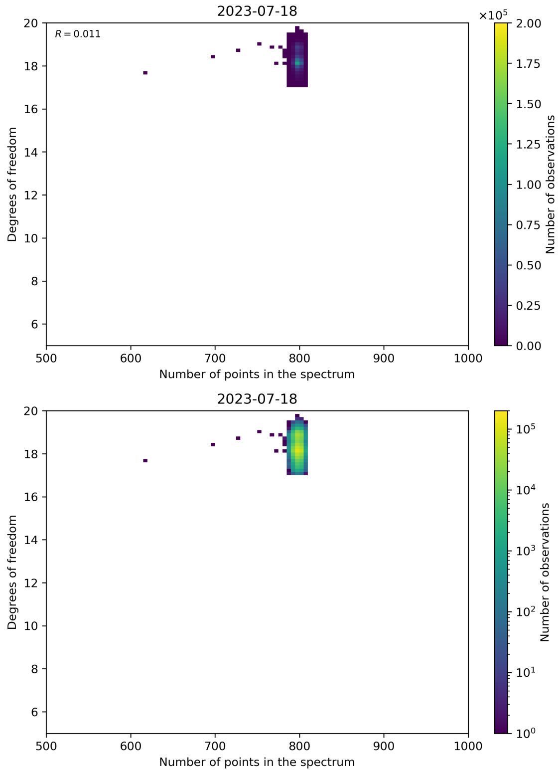
Figure 90: Scatter density plot of “Number of points in the spectrum” against “Degrees of freedom” for 2023-07-17 to 2023-07-19.
