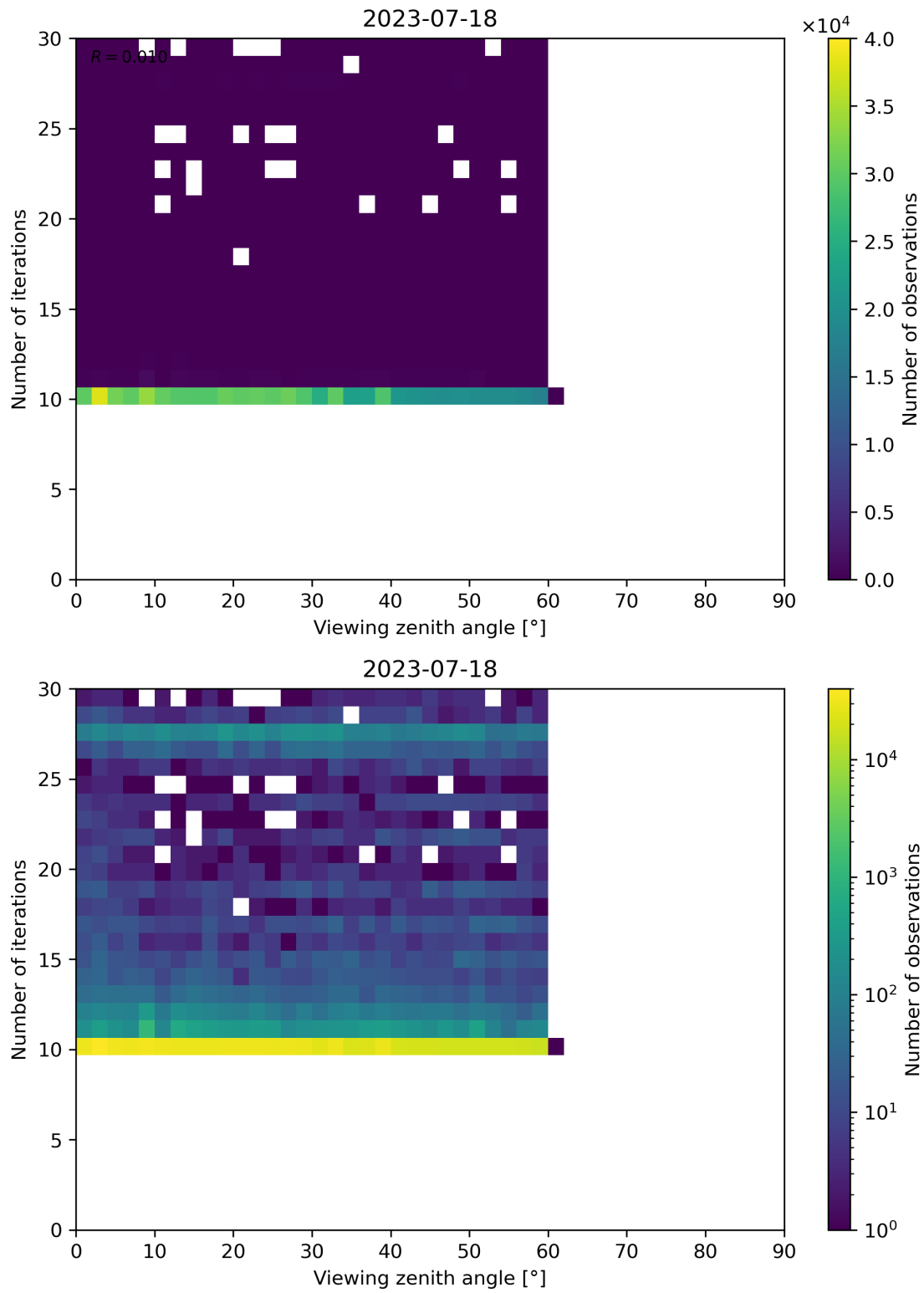
Figure 113: Scatter density plot of “Viewing zenith angle” against “Number of iterations” for 2023-07-17 to 2023-07-19.
