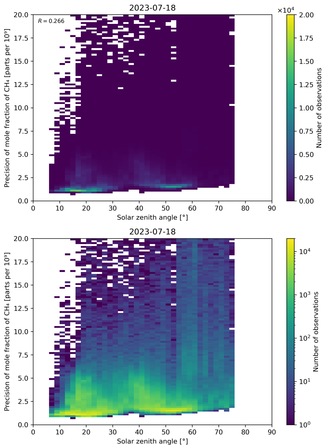
Figure 101: Scatter density plot of “Solar zenith angle” against “Precision of mole fraction of CH 4 ” for 2023-07-17 to 2023-07-19.
