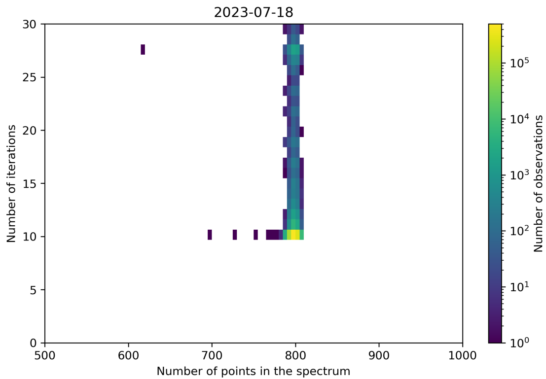
Figure 92: Scatter density plot of “Number of points in the spectrum” against “Number of iterations” for 2023-07-17 to 2023-07-19.
