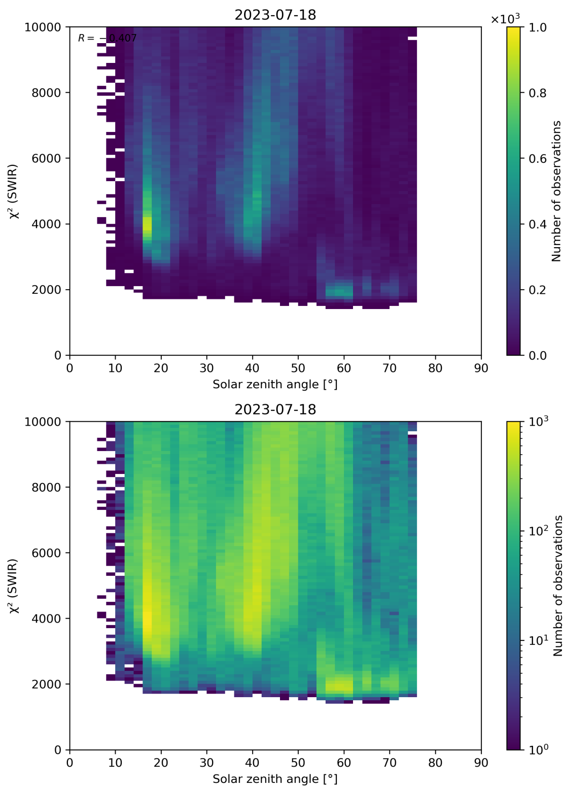
Figure 95: Scatter density plot of “Solar zenith angle” against “ \chi^2 (SWIR)” for 2023-07-17 to 2023-07-19.
