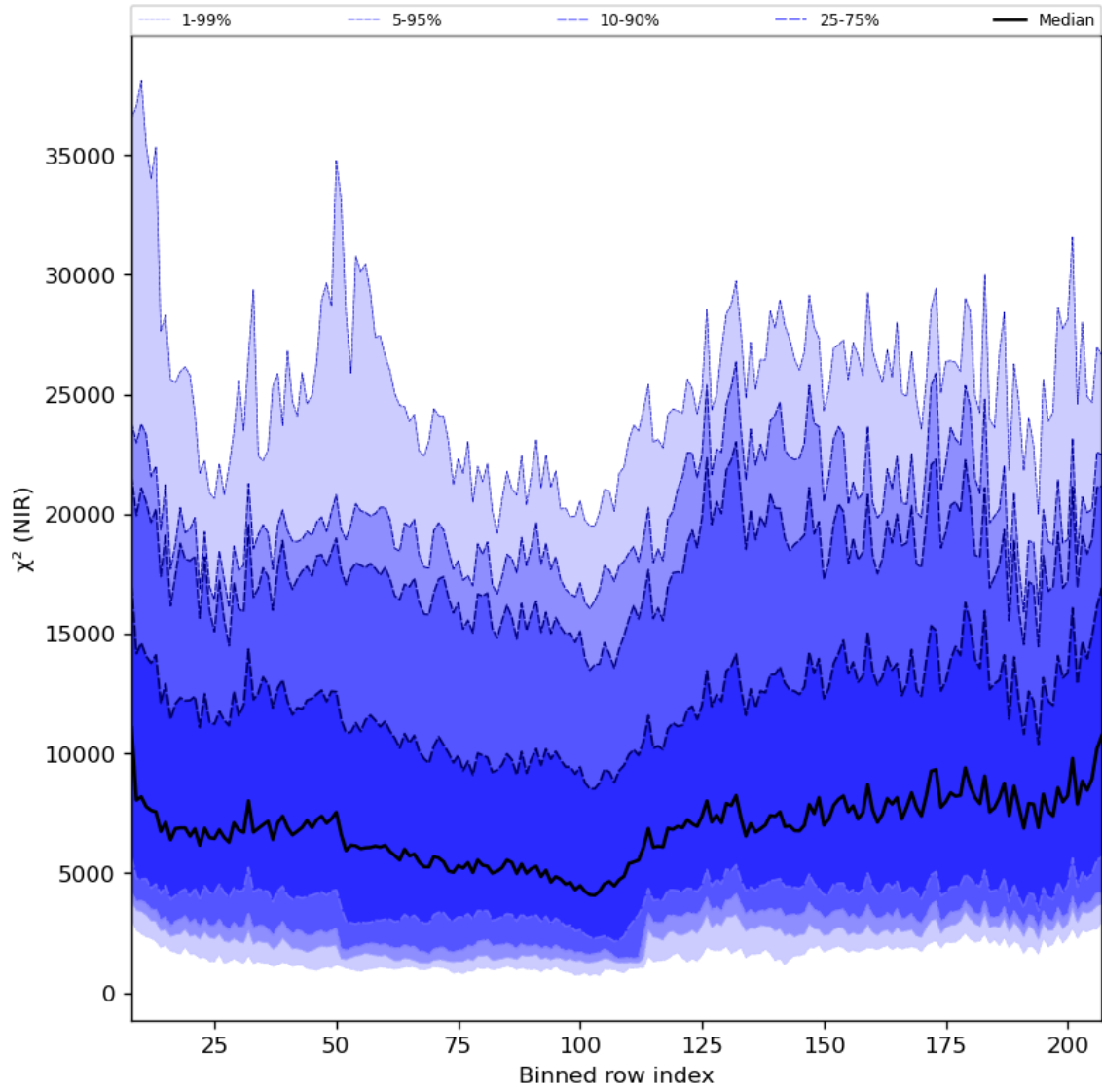
Figure 40: Along track statistics of “ \chi^2 (NIR)” for 2023-07-17 to 2023-07-19
