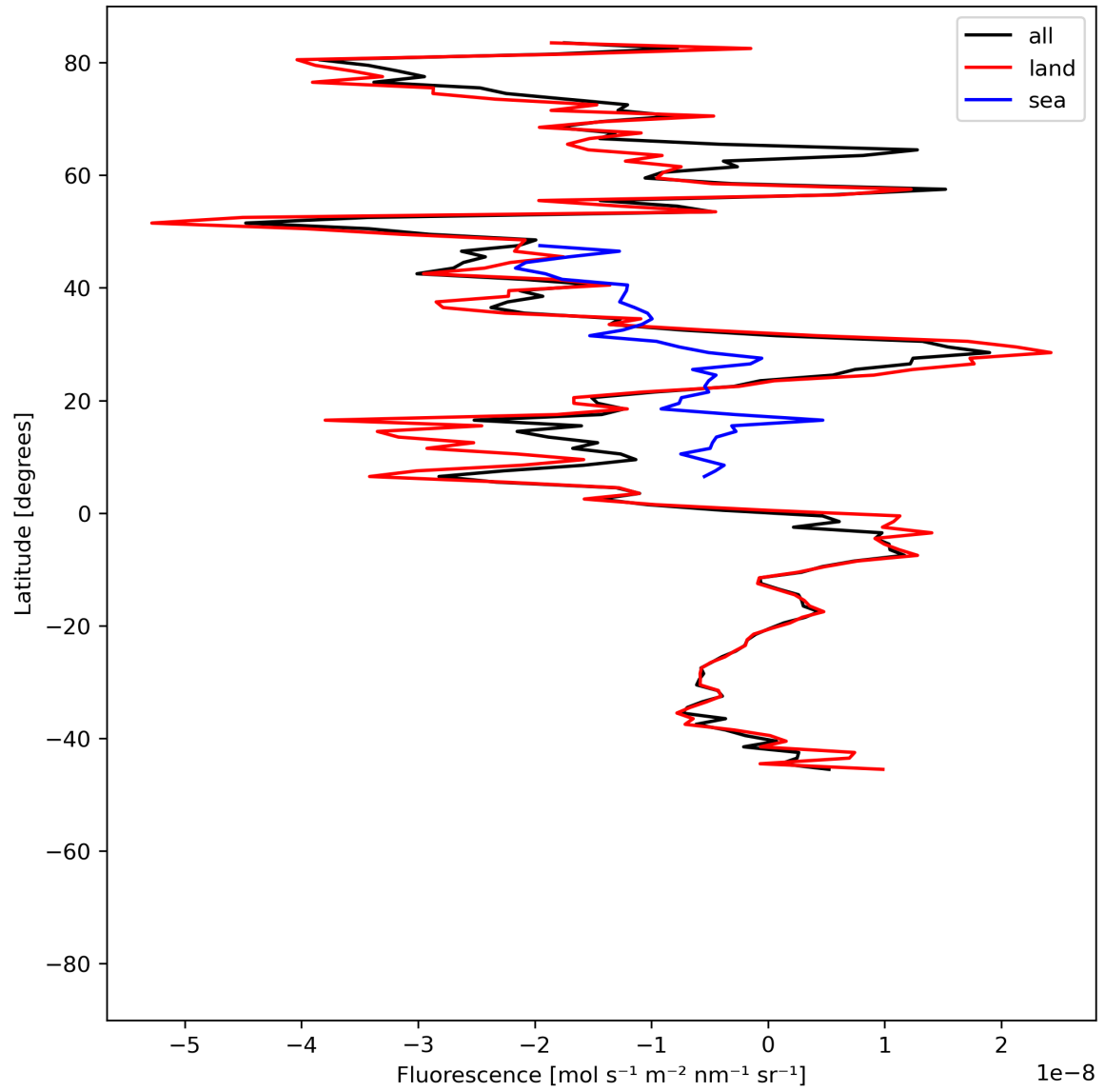
Figure 21: Zonal average of “Fluorescence” for 2023-07-17 to 2023-07-19.
