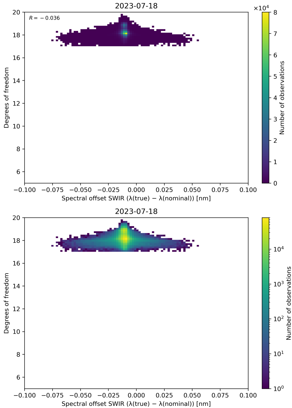
Figure 119: Scatter density plot of “Spectral offset SWIR ( \lambda(\text{true}) - \lambda(\text{nominal}) )” against “Degrees of freedom” for 2023-07-17 to 2023-07-19.
