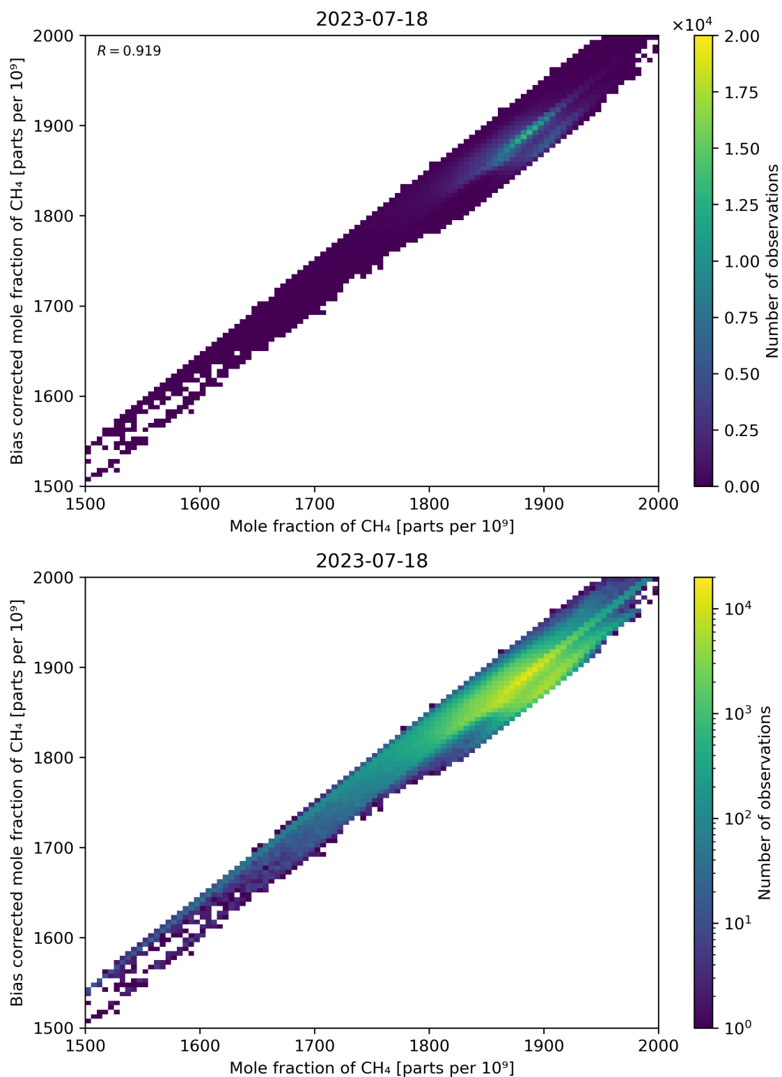
Figure 74: Scatter density plot of “Mole fraction of CH 4 ” against “Bias corrected mole fraction of CH 4 ” for 2023-07-17 to 2023-07-19.
