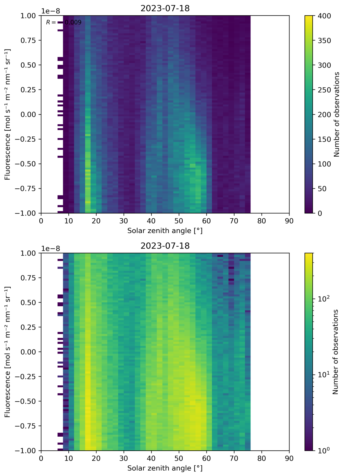
Figure 97: Scatter density plot of “Solar zenith angle” against “Fluorescence” for 2023-07-17 to 2023-07-19.
