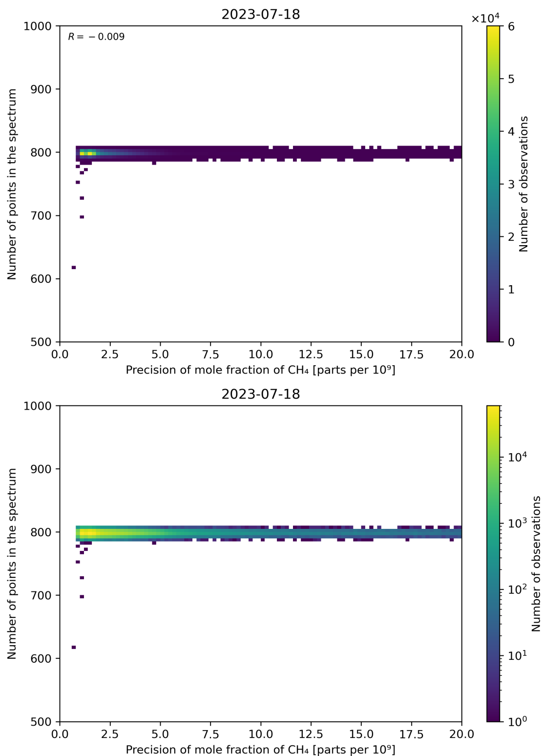
Figure 84: Scatter density plot of “Precision of mole fraction of CH 4 ” against “Number of points in the spectrum” for 2023-07-17 to 2023-07-19.
