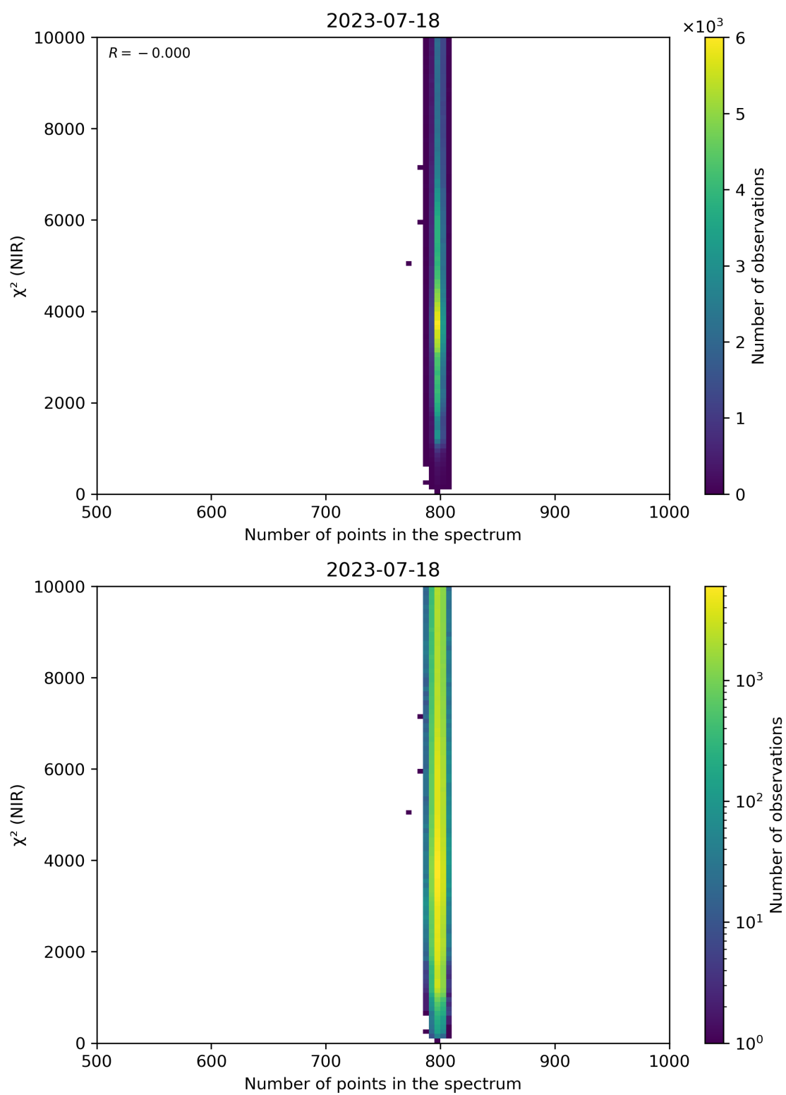
Figure 88: Scatter density plot of “Number of points in the spectrum” against “ \chi^2 (NIR)” for 2023-07-17 to 2023-07-19.
