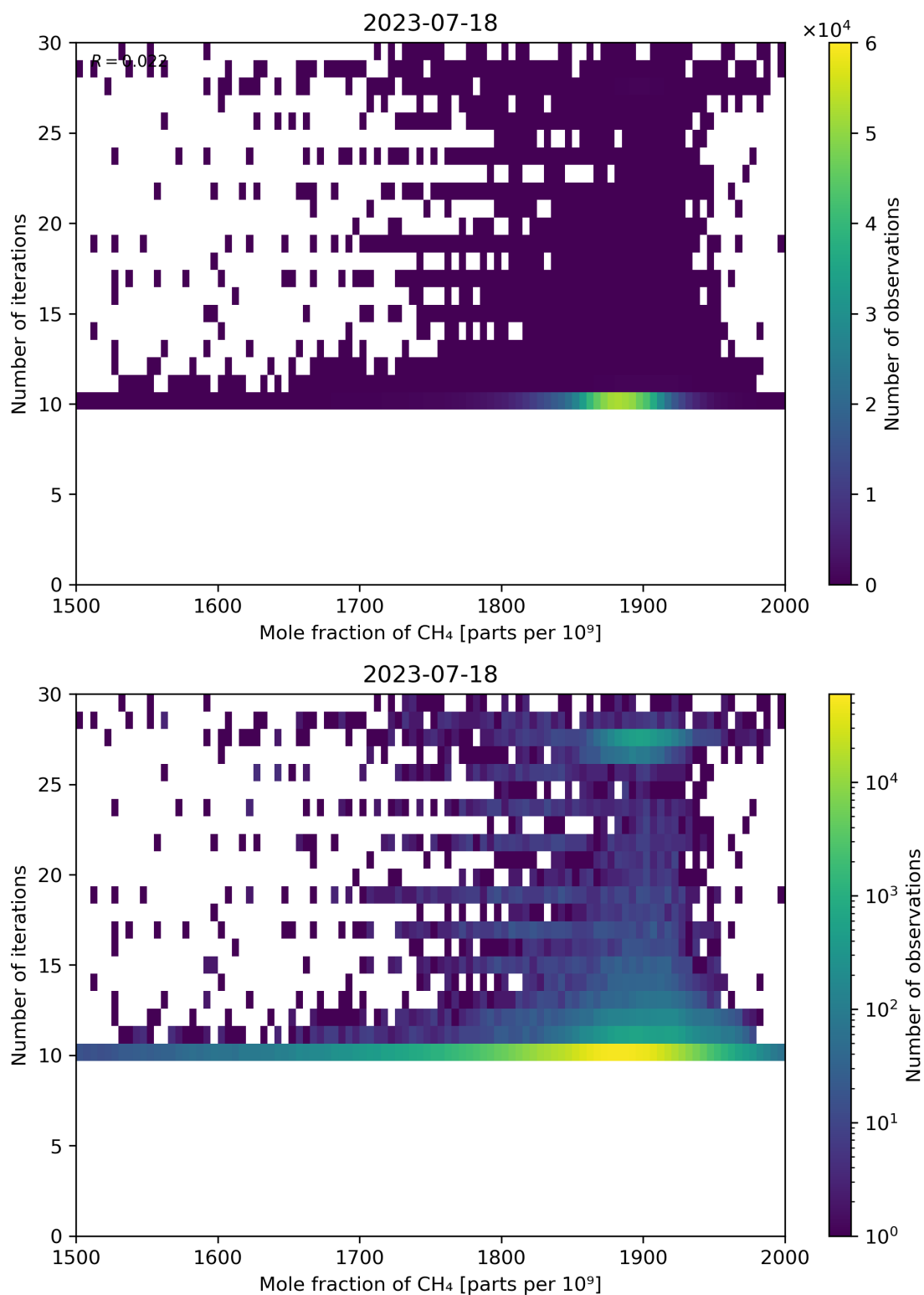
Figure 76: Scatter density plot of “Mole fraction of CH 4 ” against “Number of iterations” for 2023-07-17 to 2023-07-19.
