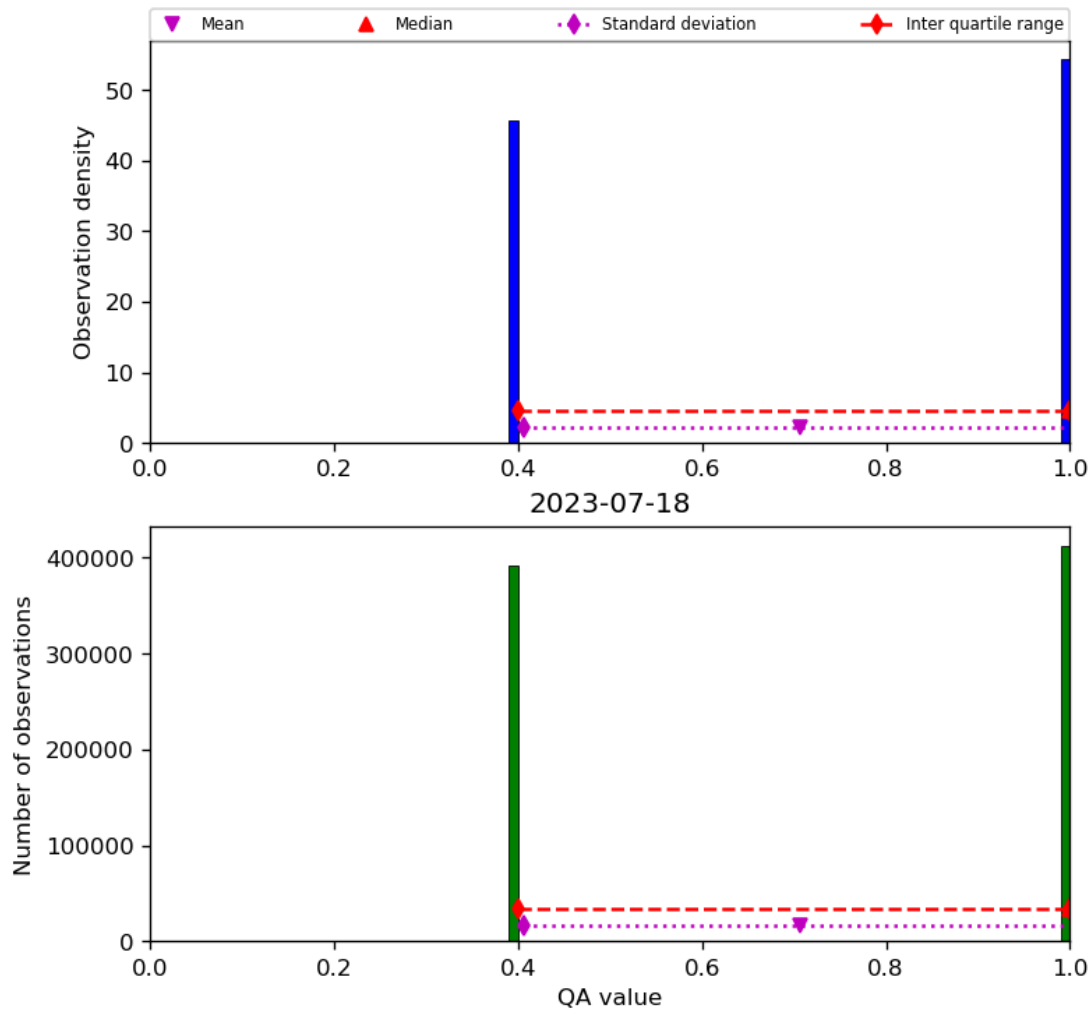
Figure 22: Histogram of “QA value” for 2023-07-17 to 2023-07-19
