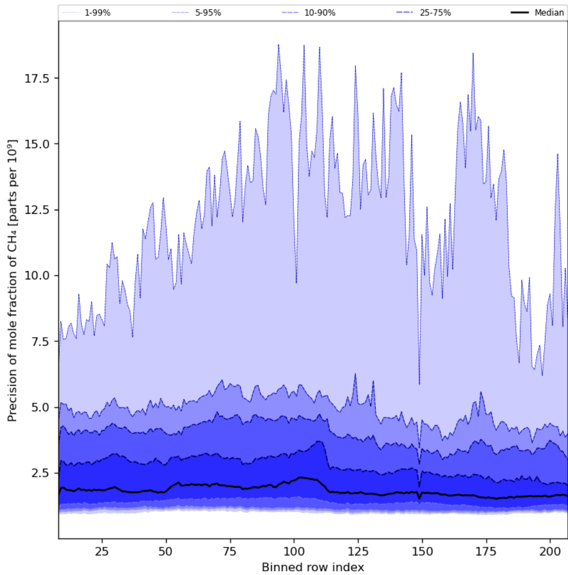
Figure 35: Along track statistics of “Precision of mole fraction of CH 4 ” for 2023-07-17 to 2023-07-19
