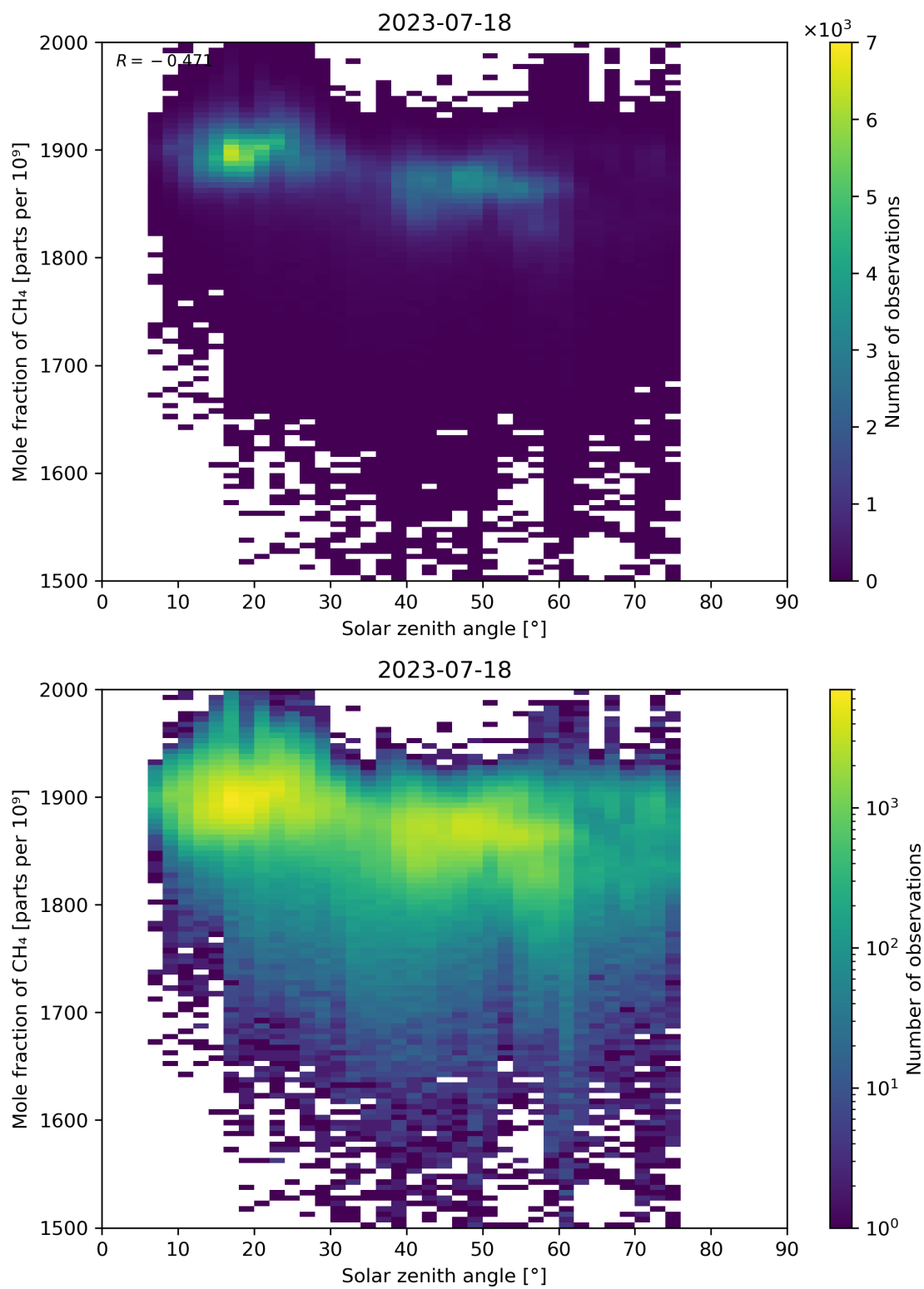
Figure 99: Scatter density plot of “Solar zenith angle” against “Mole fraction of \text{CH}_4 ” for 2023-07-17 to 2023-07-19.
