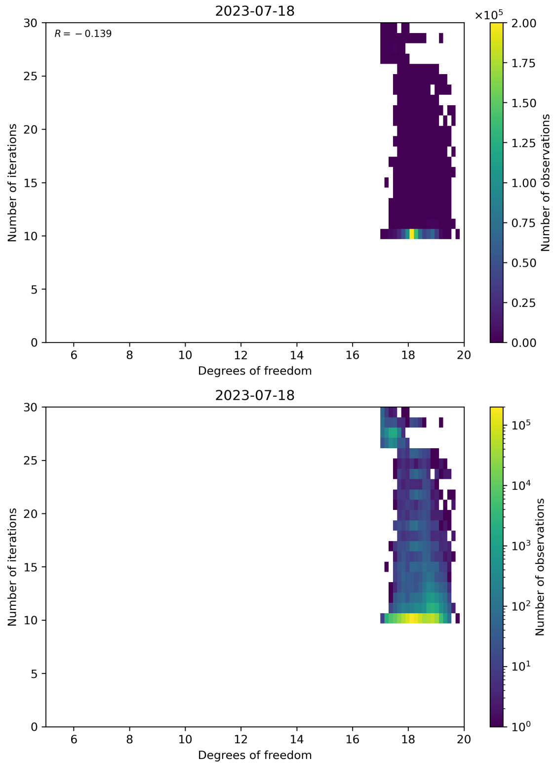
Figure 52: Scatter density plot of “Degrees of freedom” against “Number of iterations” for 2023-07-17 to 2023-07-19.
