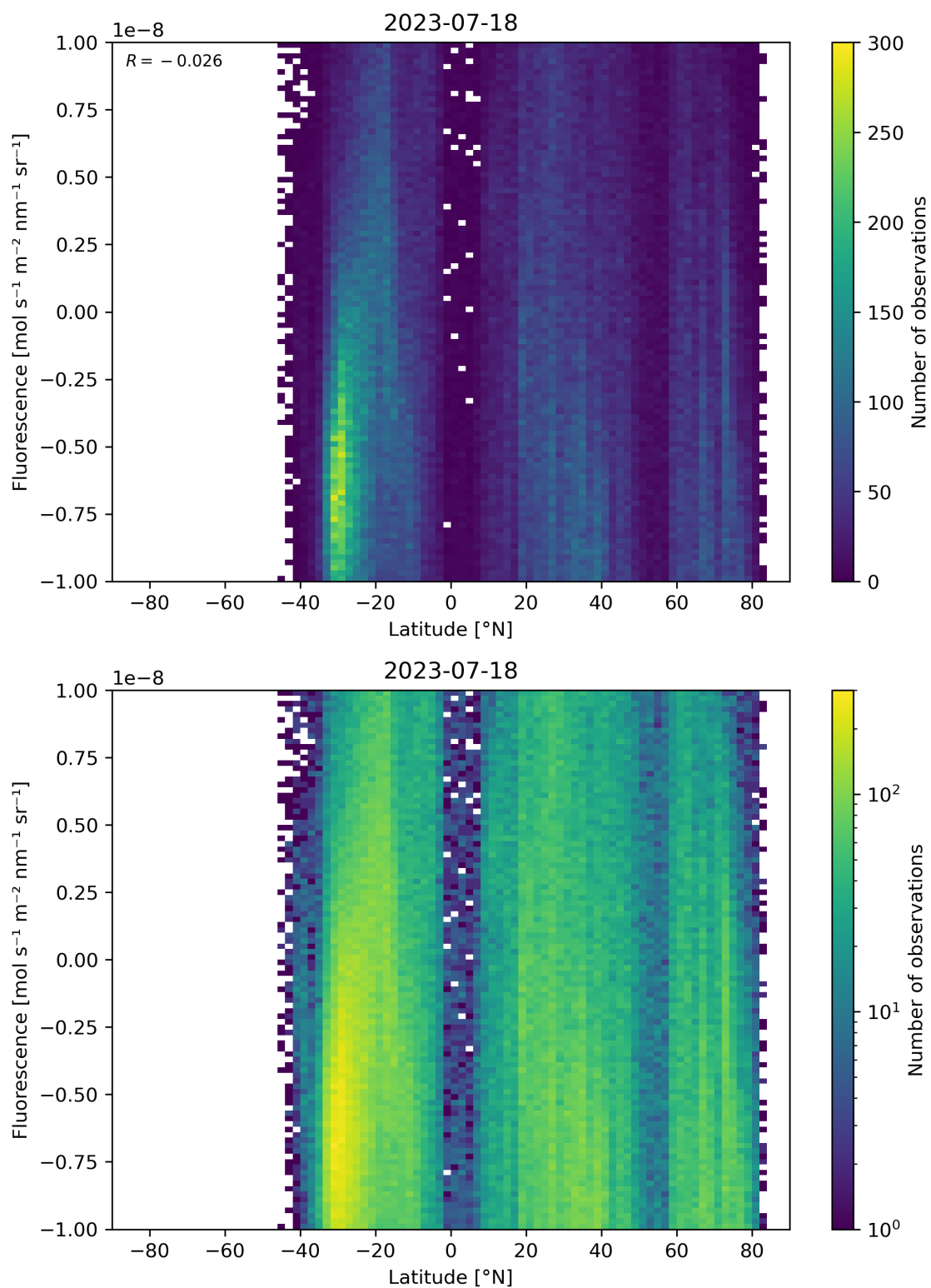
Figure 56: Scatter density plot of “Latitude” against “Fluorescence” for 2023-07-17 to 2023-07-19.
