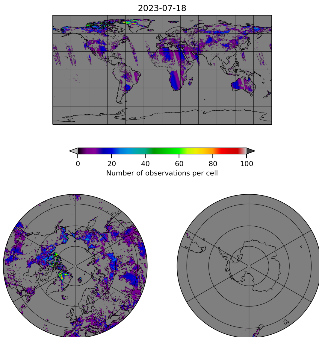
Figure 10: Map of the number of observations for 2023-07-17 to 2023-07-19
