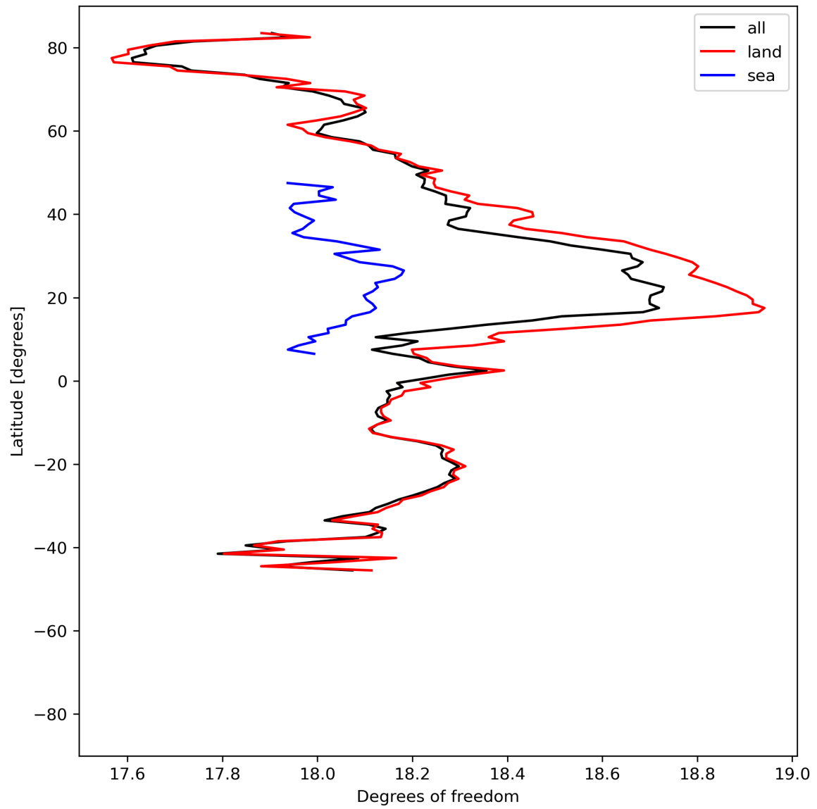
Figure 19: Zonal average of “Degrees of freedom” for 2023-07-17 to 2023-07-19.
