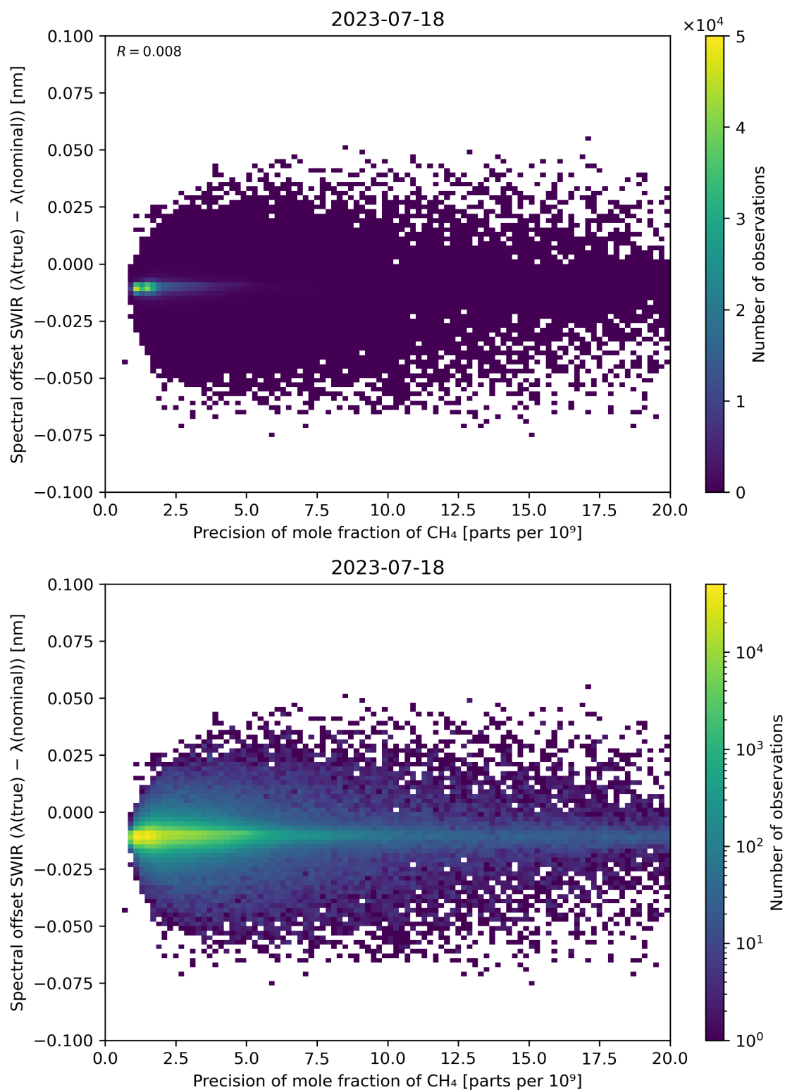
Figure 85: Scatter density plot of “Precision of mole fraction of CH 4 ” against “Spectral offset SWIR ( \lambda(\text{true}) - \lambda(\text{nominal}) )” for 2023-07-17 to 2023-07-19.
