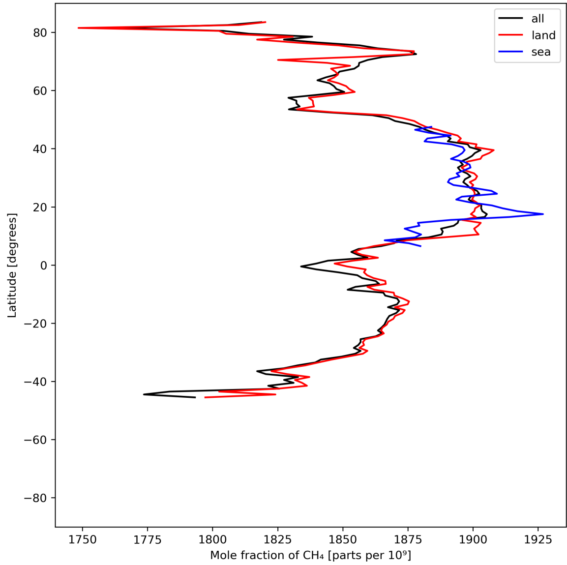
Figure 12: Zonal average of “Mole fraction of \text{CH}_4 ” for 2023-07-17 to 2023-07-19.
