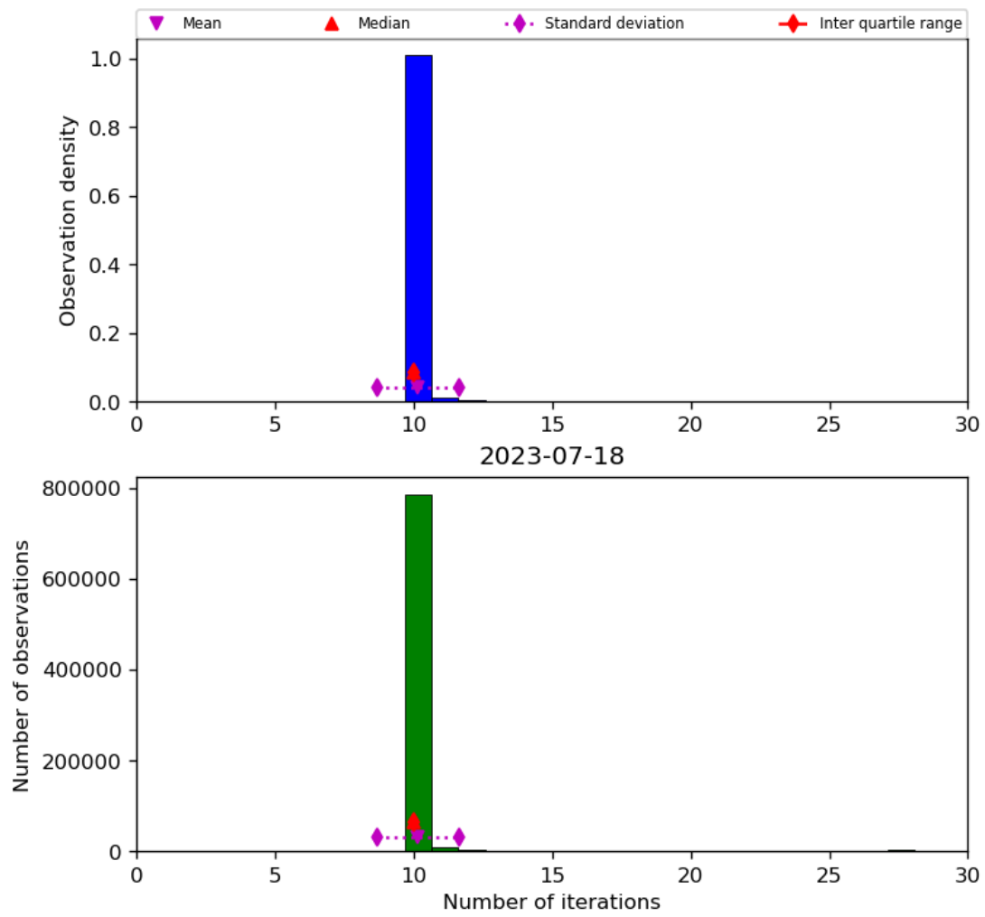
Figure 31: Histogram of “Number of iterations” for 2023-07-17 to 2023-07-19
