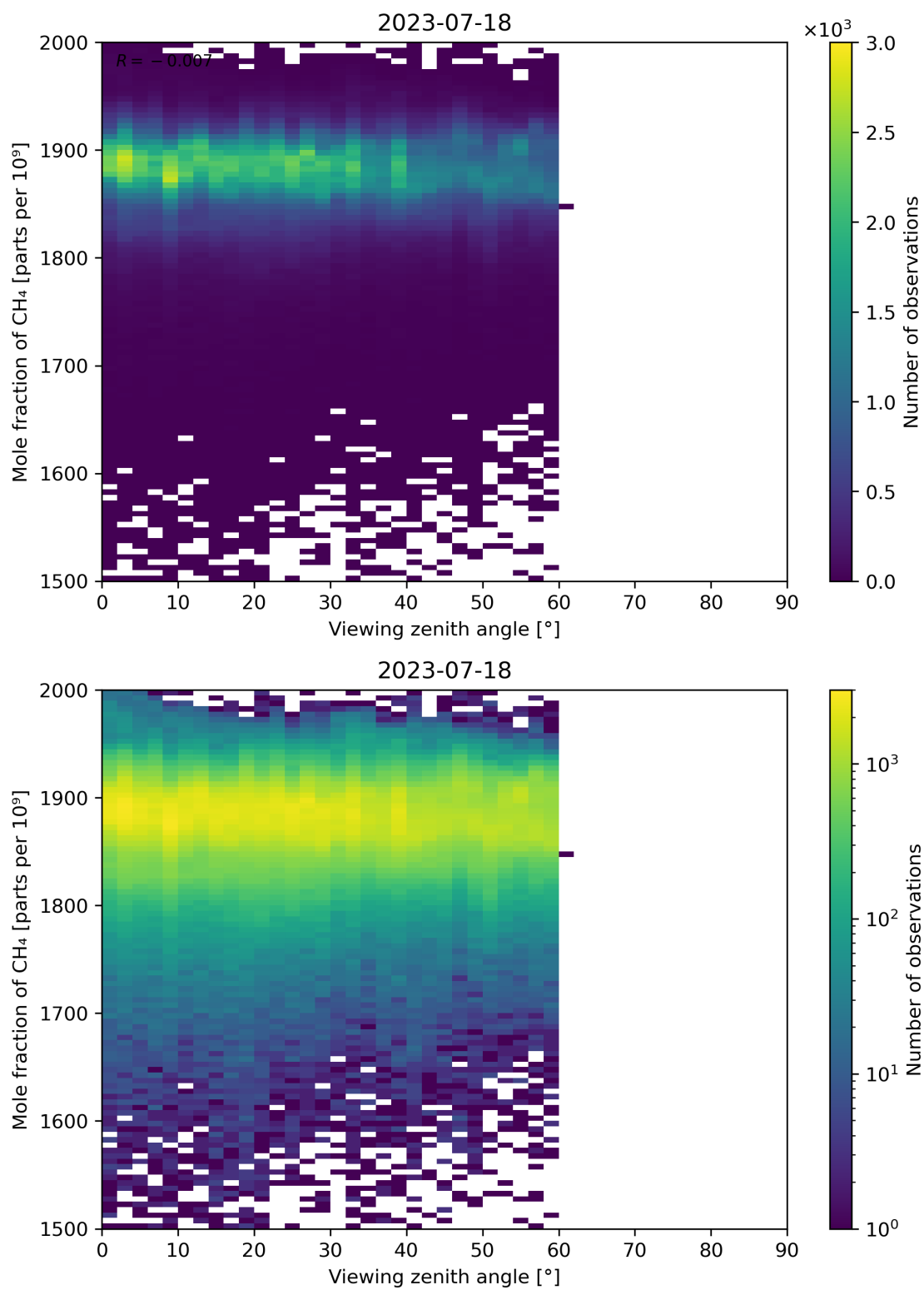
Figure 110: Scatter density plot of “Viewing zenith angle” against “Mole fraction of CH 4 ” for 2023-07-17 to 2023-07-19.
