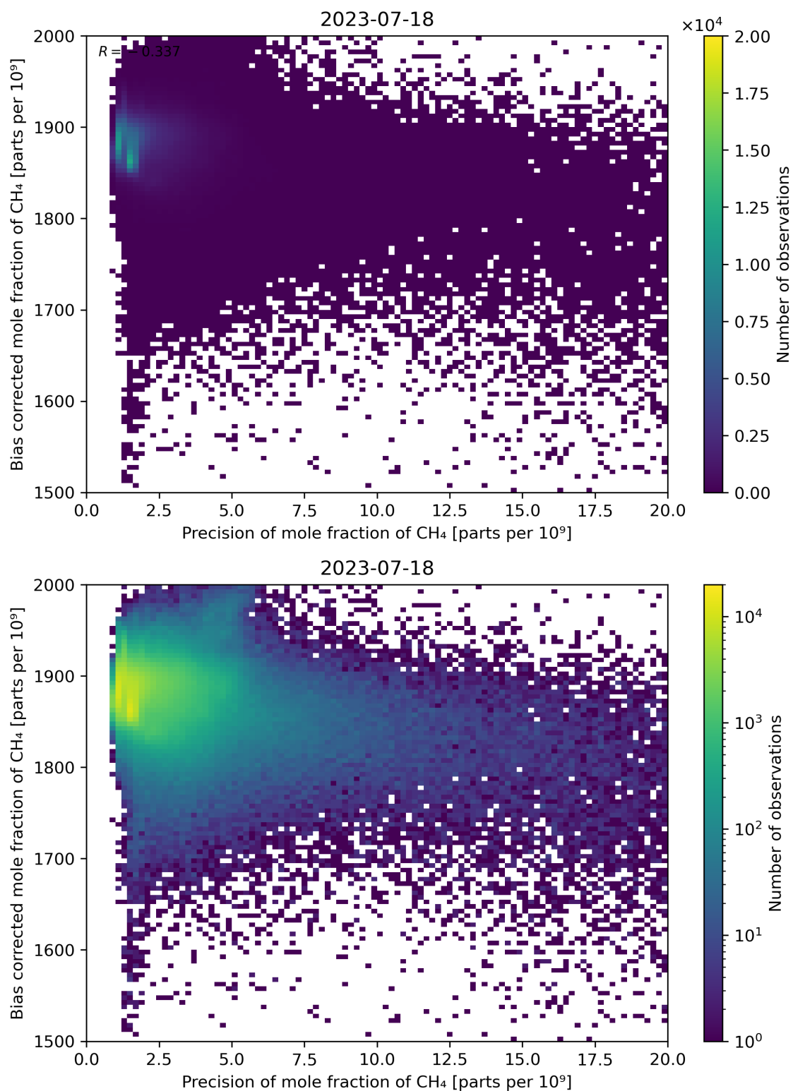
Figure 82: Scatter density plot of “Precision of mole fraction of CH 4 ” against “Bias corrected mole fraction of CH 4 ” for 2023-07-17 to 2023-07-19.
