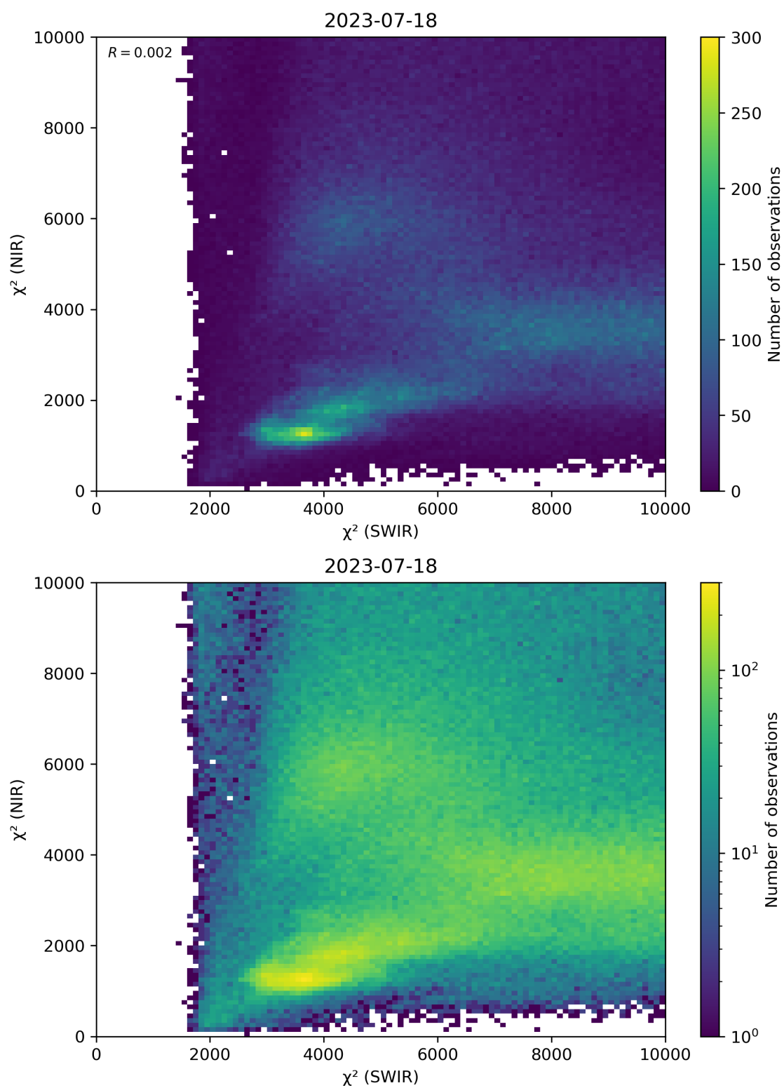
Figure 47: Scatter density plot of “ \chi^2 (SWIR)” against “ \chi^2 (NIR)” for 2023-07-17 to 2023-07-19.
