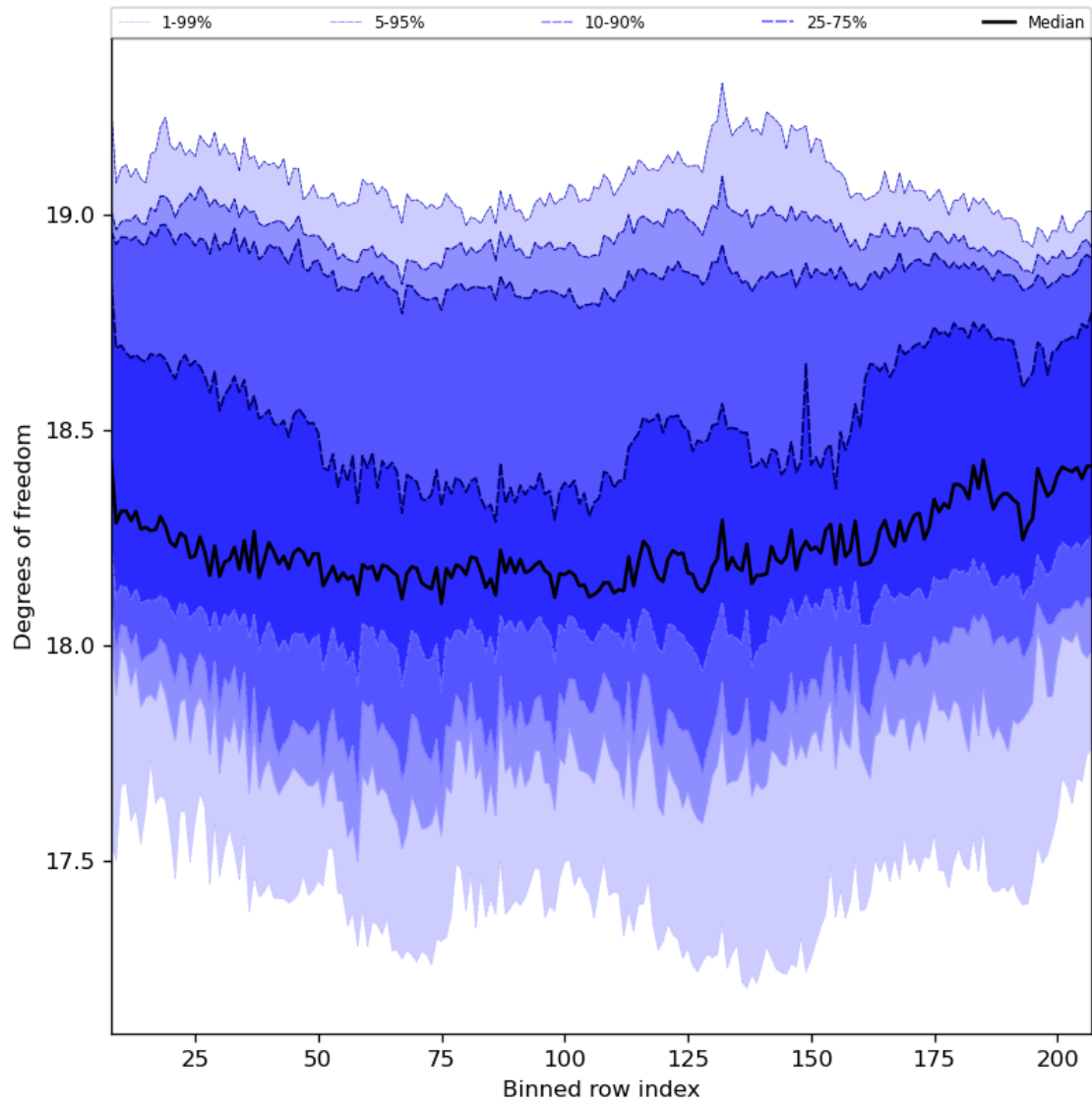
Figure 41: Along track statistics of “Degrees of freedom” for 2023-07-17 to 2023-07-19
