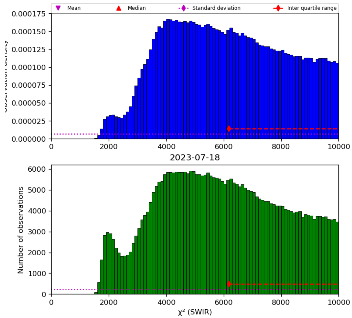
Figure 28: Histogram of “ \chi^2 (SWIR)” for 2023-07-17 to 2023-07-19
