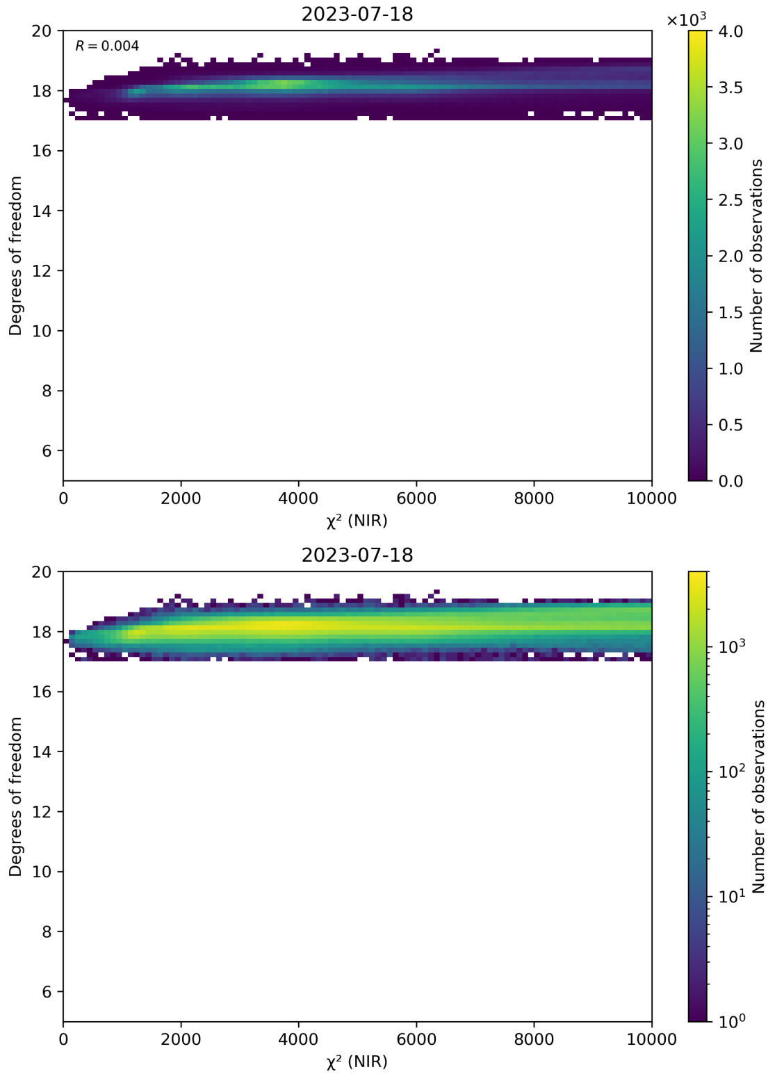
Figure 44: Scatter density plot of “ \chi^2 (NIR)” against “Degrees of freedom” for 2023-07-17 to 2023-07-19.
