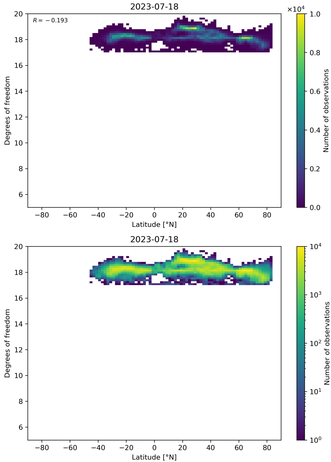
Figure 55: Scatter density plot of “Latitude” against “Degrees of freedom” for 2023-07-17 to 2023-07-19.
