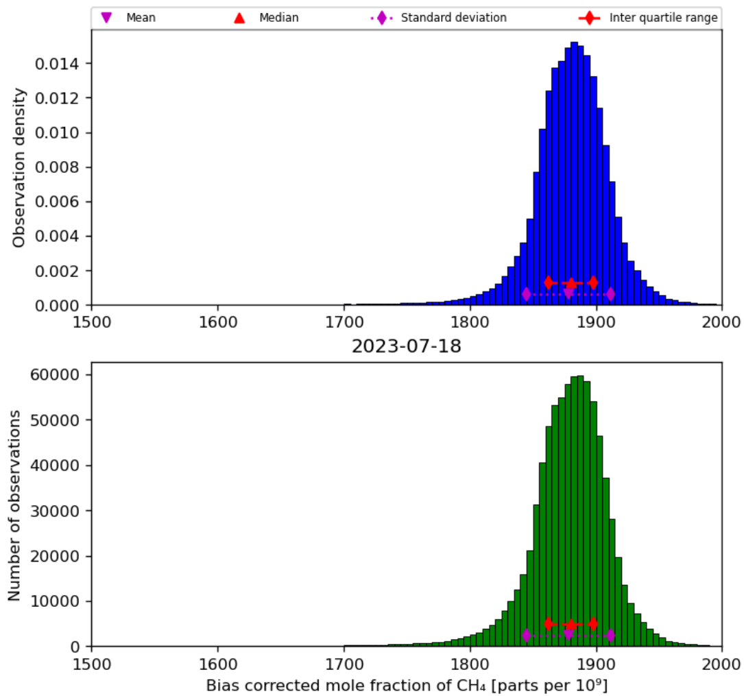
Figure 25: Histogram of “Bias corrected mole fraction of CH 4 ” for 2023-07-17 to 2023-07-19
