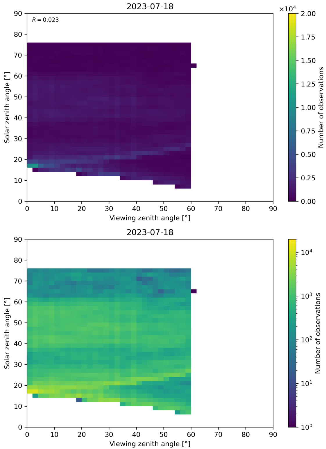
Figure 115: Scatter density plot of “Viewing zenith angle” against “Solar zenith angle” for 2023-07-17 to 2023-07-19.
