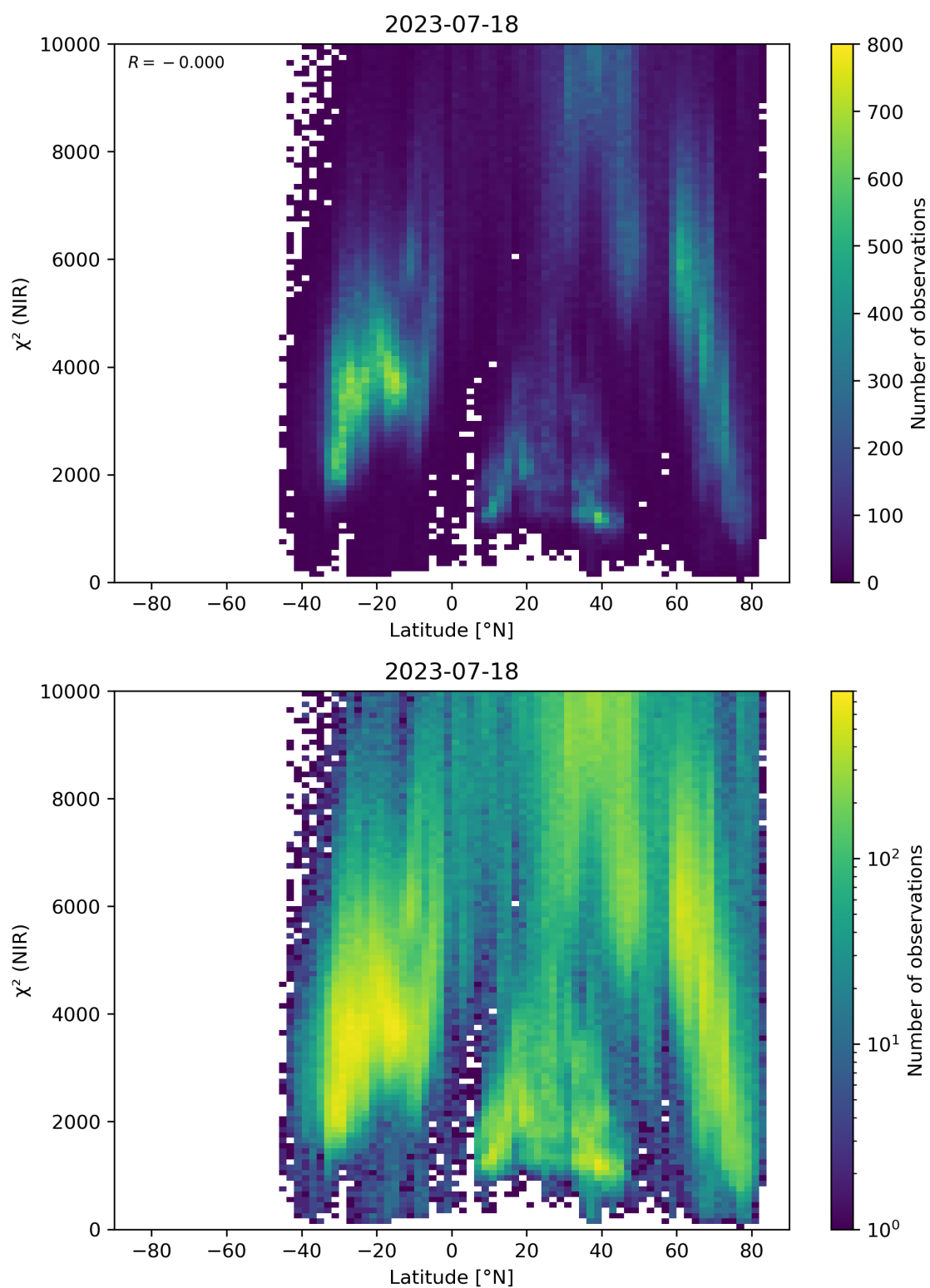
Figure 53: Scatter density plot of “Latitude” against “ \chi^2 (NIR)” for 2023-07-17 to 2023-07-19.
