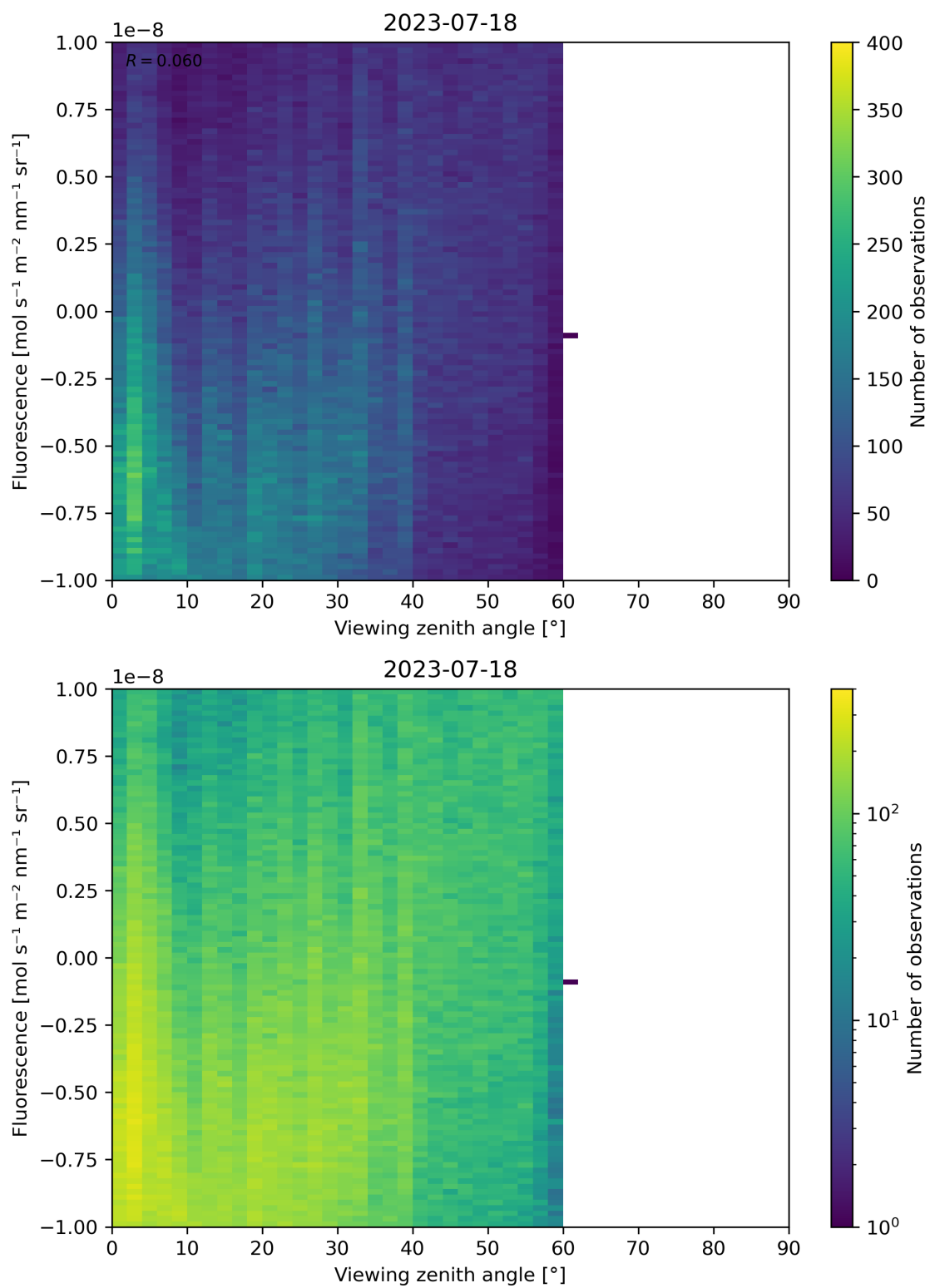
Figure 108: Scatter density plot of “Viewing zenith angle” against “Fluorescence” for 2023-07-17 to 2023-07-19.
