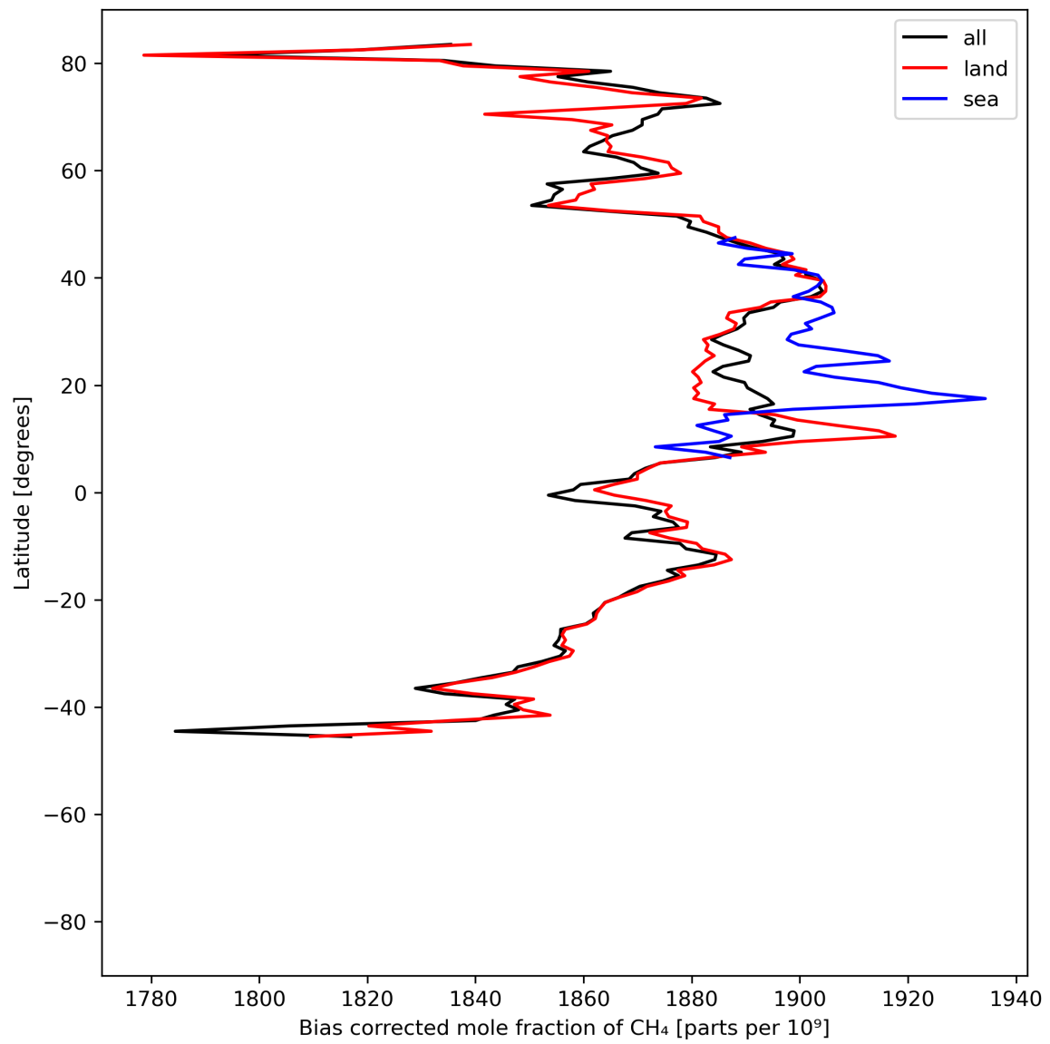
Figure 14: Zonal average of “Bias corrected mole fraction of CH 4 ” for 2023-07-17 to 2023-07-19.
