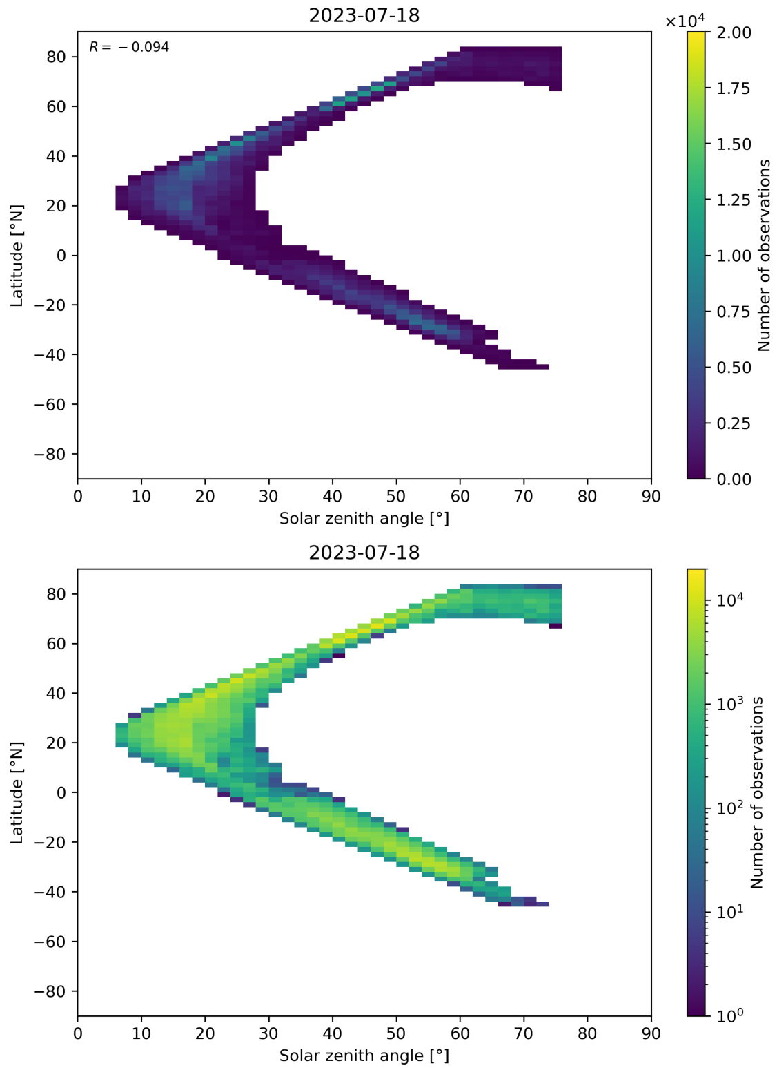
Figure 98: Scatter density plot of “Solar zenith angle” against “Latitude” for 2023-07-17 to 2023-07-19.
