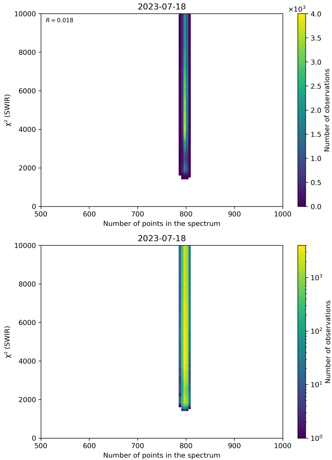
Figure 89: Scatter density plot of “Number of points in the spectrum” against “ \chi^2 (SWIR)” for 2023-07-17 to 2023-07-19.
