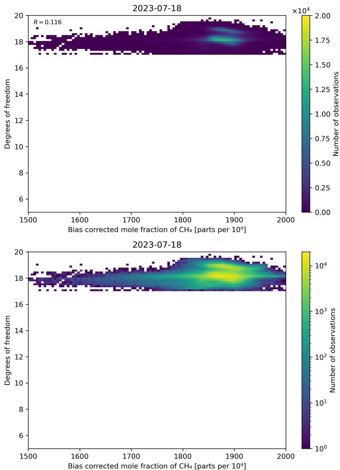
Figure 65: Scatter density plot of “Bias corrected mole fraction of CH 4 ” against “Degrees of freedom” for 2023-07-17 to 2023-07-19.
