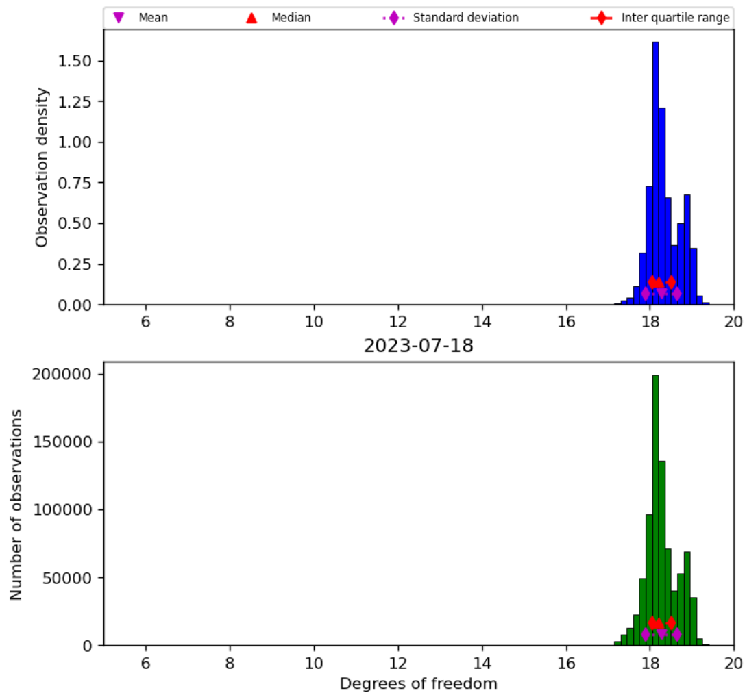
Figure 30: Histogram of “Degrees of freedom” for 2023-07-17 to 2023-07-19
