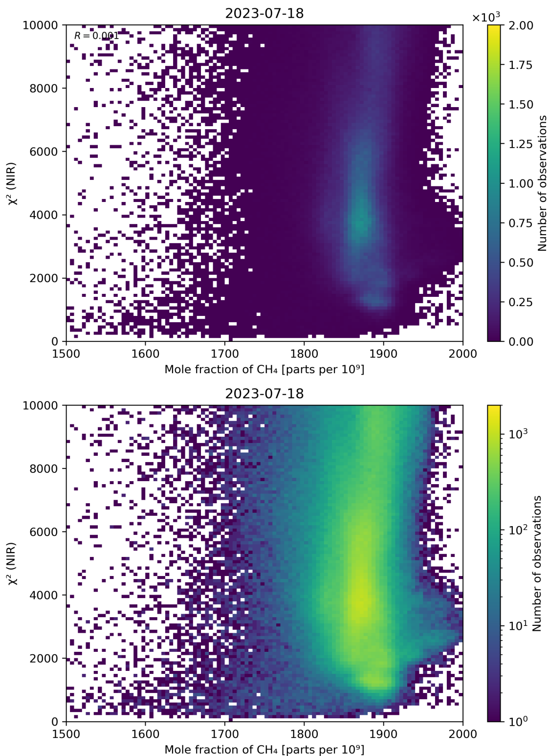
Figure 70: Scatter density plot of “Mole fraction of \text{CH}_4 ” against “ \chi^2 (NIR)” for 2023-07-17 to 2023-07-19.
