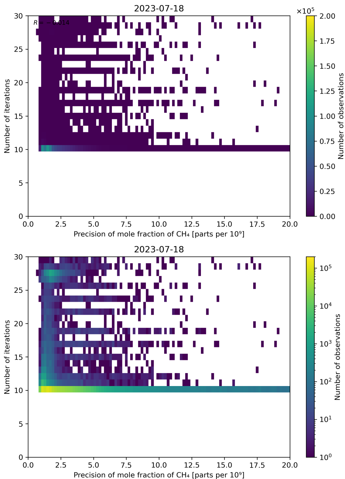
Figure 83: Scatter density plot of “Precision of mole fraction of CH 4 ” against “Number of iterations” for 2023-07-17 to 2023-07-19.
