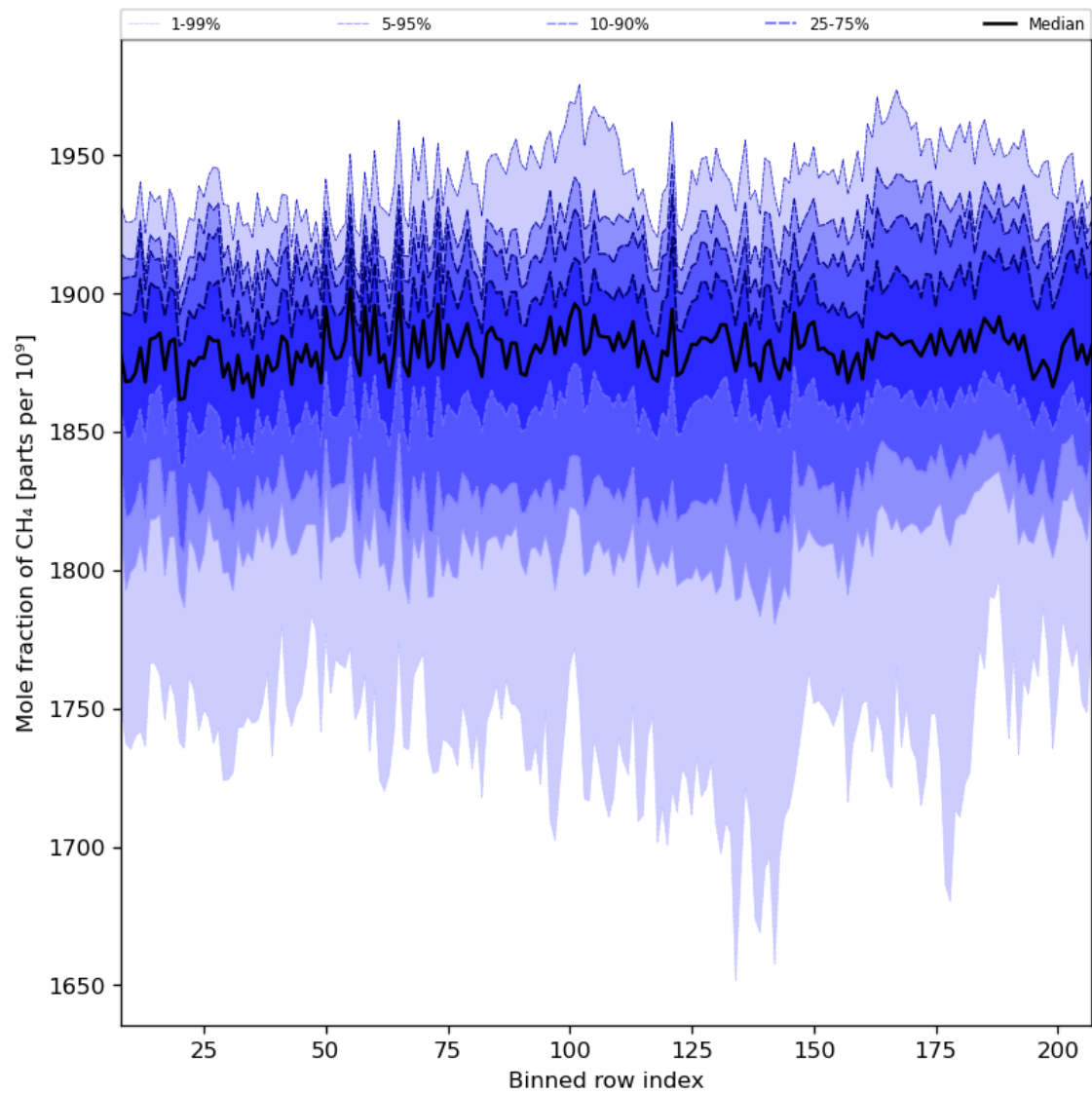
Figure 34: Along track statistics of “Mole fraction of CH 4 ” for 2023-07-17 to 2023-07-19
