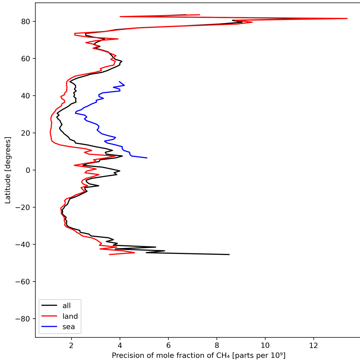
Figure 13: Zonal average of “Precision of mole fraction of CH 4 ” for 2023-07-17 to 2023-07-19.
