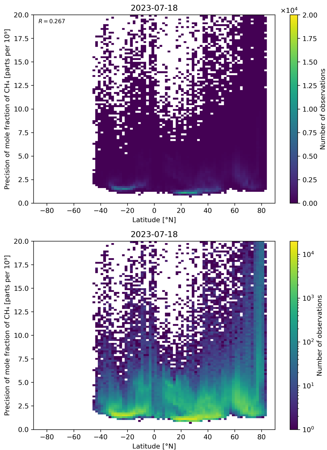
Figure 59: Scatter density plot of “Latitude” against “Precision of mole fraction of CH 4 ” for 2023-07-17 to 2023-07-19.
