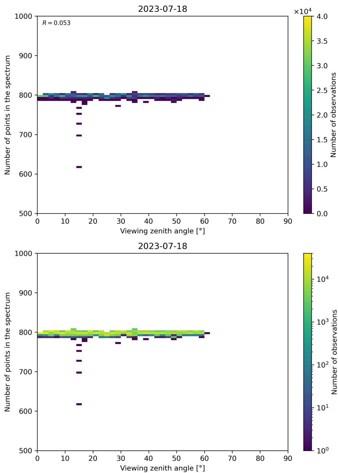
Figure 114: Scatter density plot of “Viewing zenith angle” against “Number of points in the spectrum” for 2023-07-17 to 2023-07-19.
