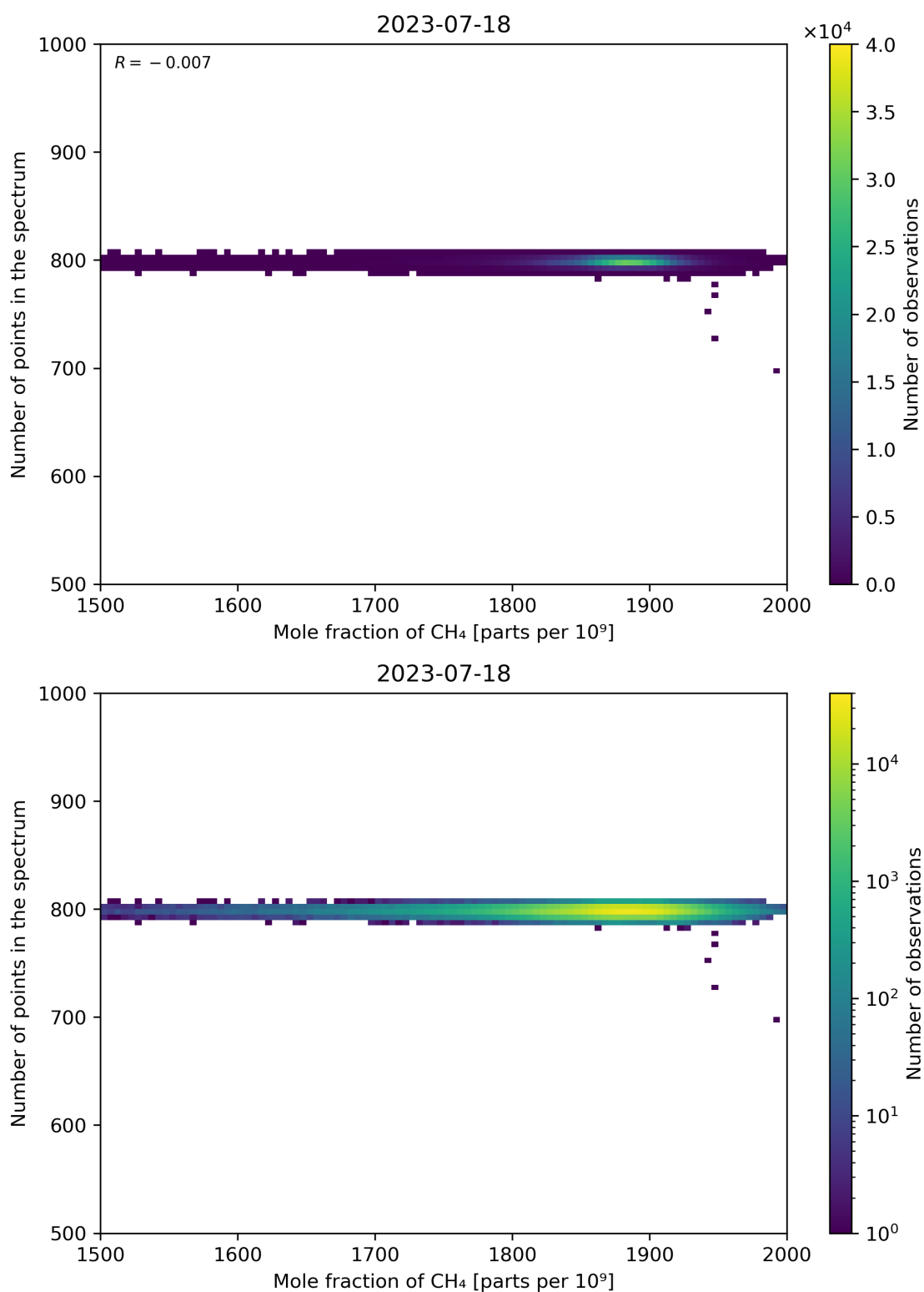
Figure 77: Scatter density plot of “Mole fraction of CH 4 ” against “Number of points in the spectrum” for 2023-07-17 to 2023-07-19.
