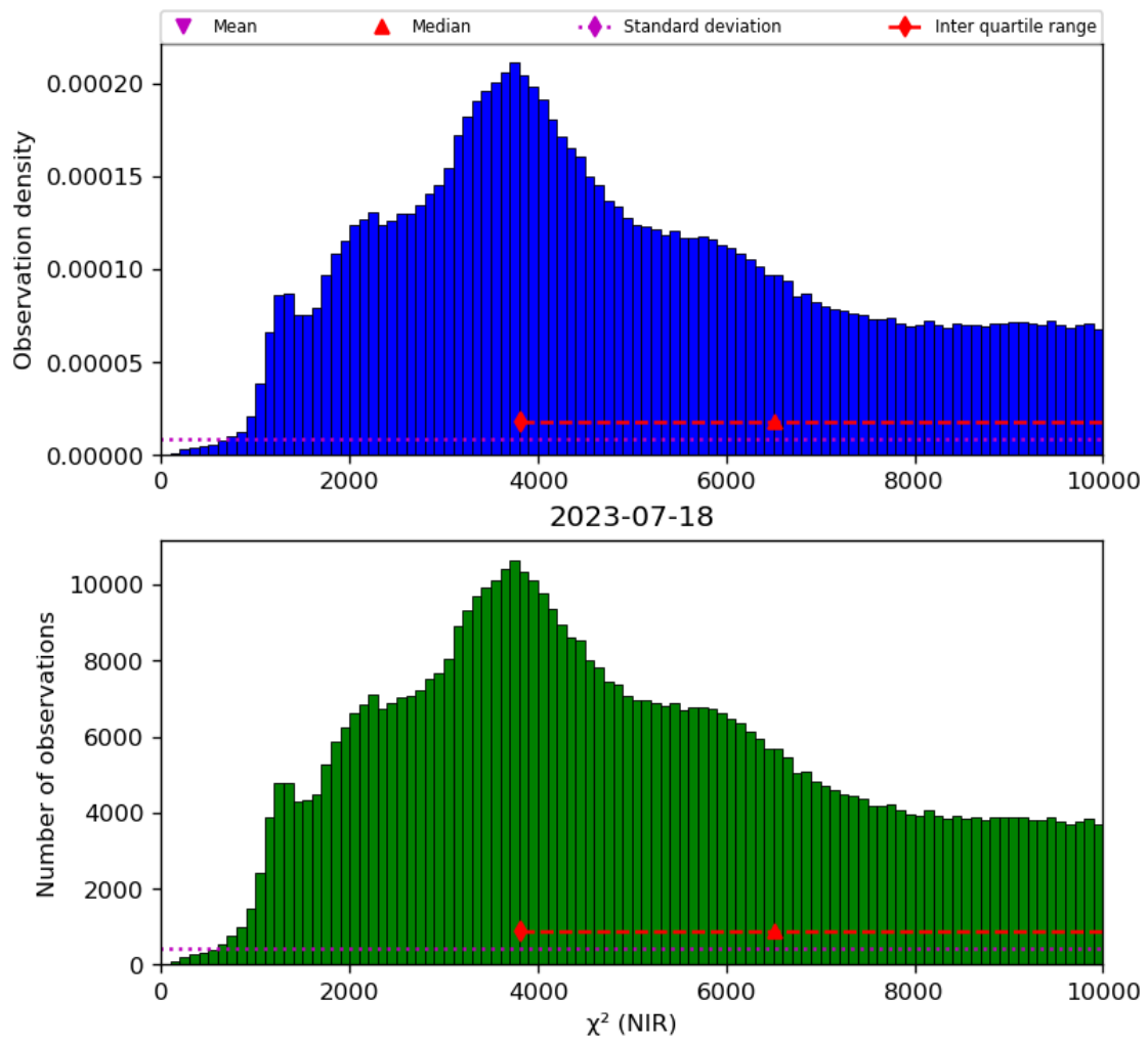
Figure 29: Histogram of “ \chi^2 (NIR)” for 2023-07-17 to 2023-07-19
