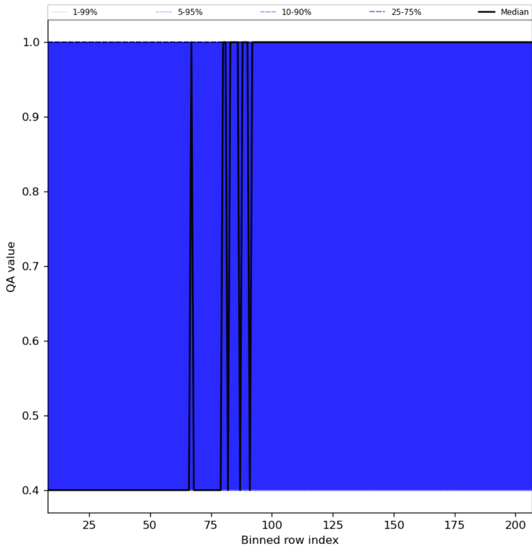
Figure 33: Along track statistics of “QA value” for 2023-07-17 to 2023-07-19
