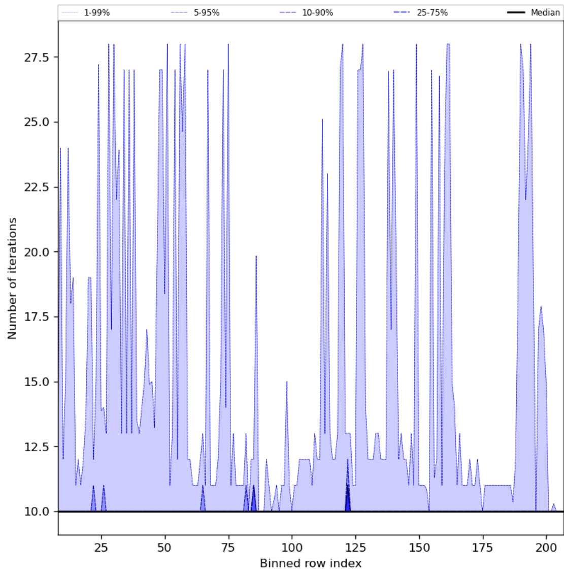
Figure 42: Along track statistics of “Number of iterations” for 2023-07-17 to 2023-07-19
