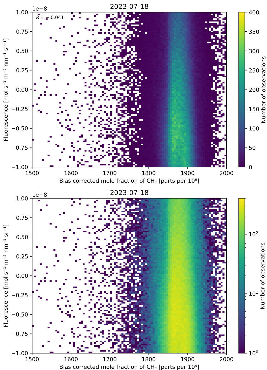
Figure 66: Scatter density plot of “Bias corrected mole fraction of \text{CH}_4 ” against “Fluorescence” for 2023-07-17 to 2023-07-19.
