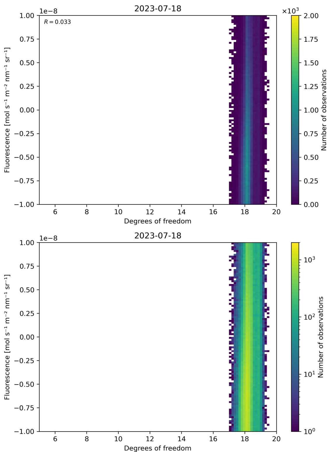
Figure 51: Scatter density plot of “Degrees of freedom” against “Fluorescence” for 2023-07-17 to 2023-07-19.
