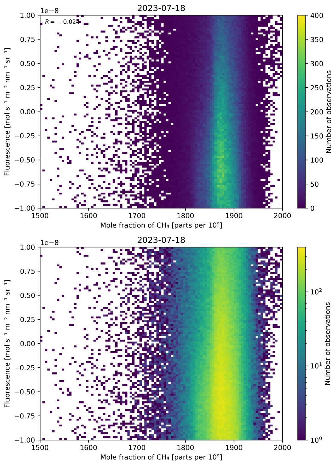
Figure 73: Scatter density plot of “Mole fraction of \text{CH}_4 ” against “Fluorescence” for 2023-07-17 to 2023-07-19.
