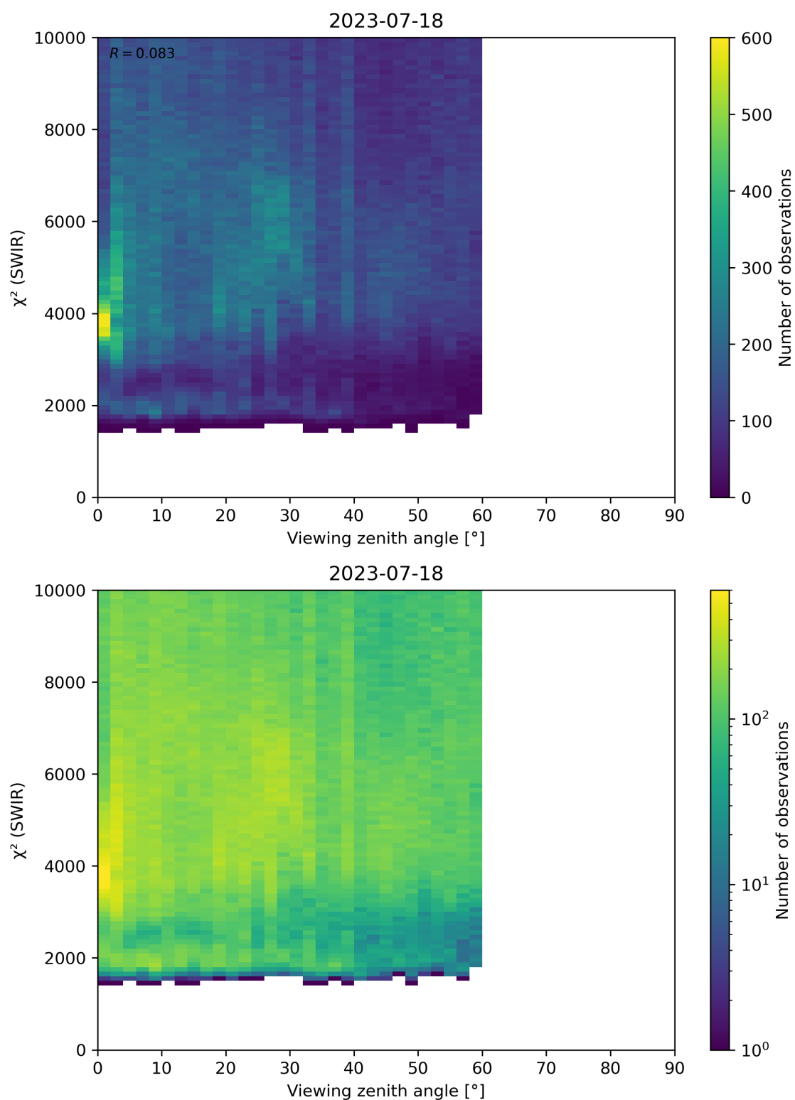
Figure 106: Scatter density plot of “Viewing zenith angle” against “ \chi^2 (SWIR)” for 2023-07-17 to 2023-07-19.
