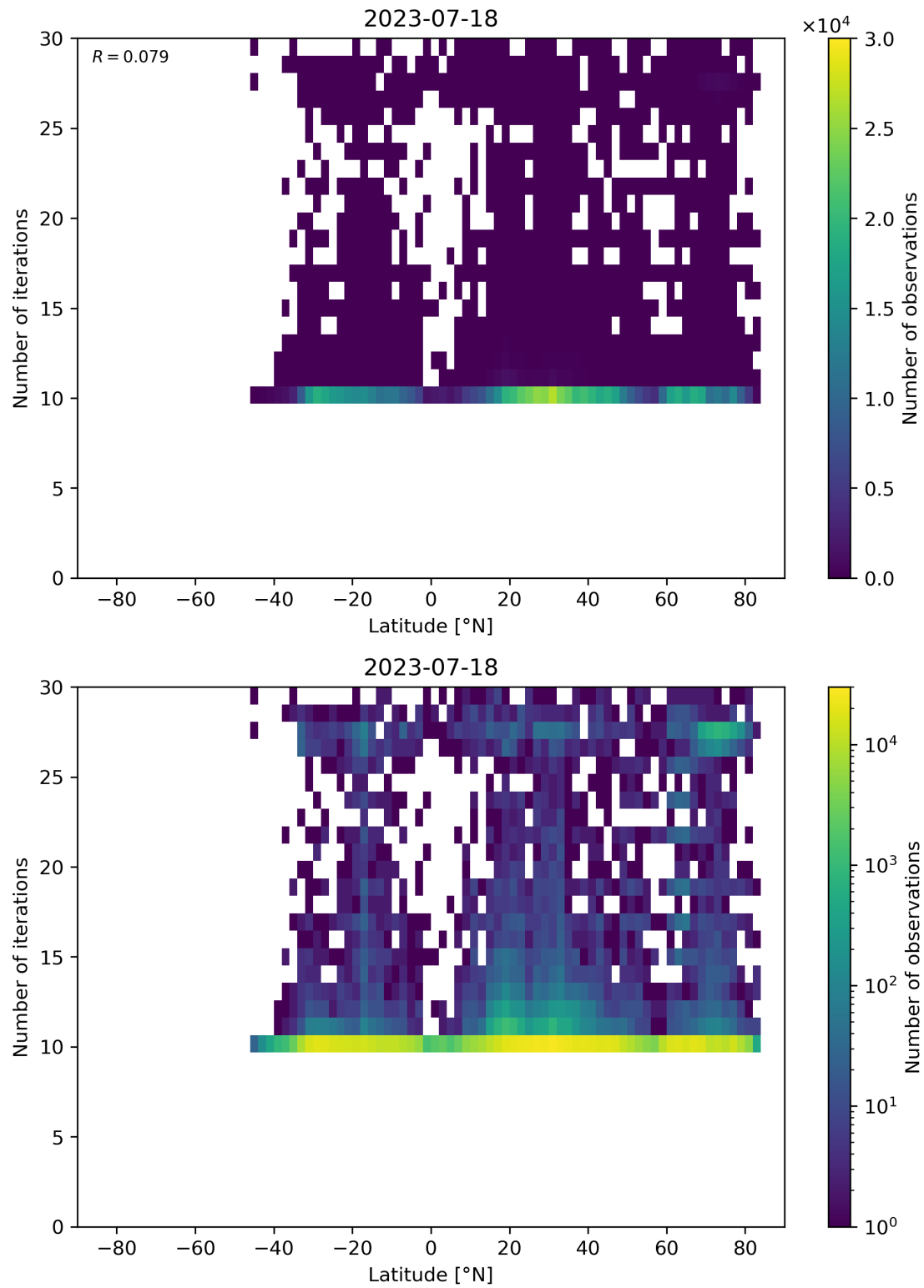
Figure 60: Scatter density plot of “Latitude” against “Number of iterations” for 2023-07-17 to 2023-07-19.
