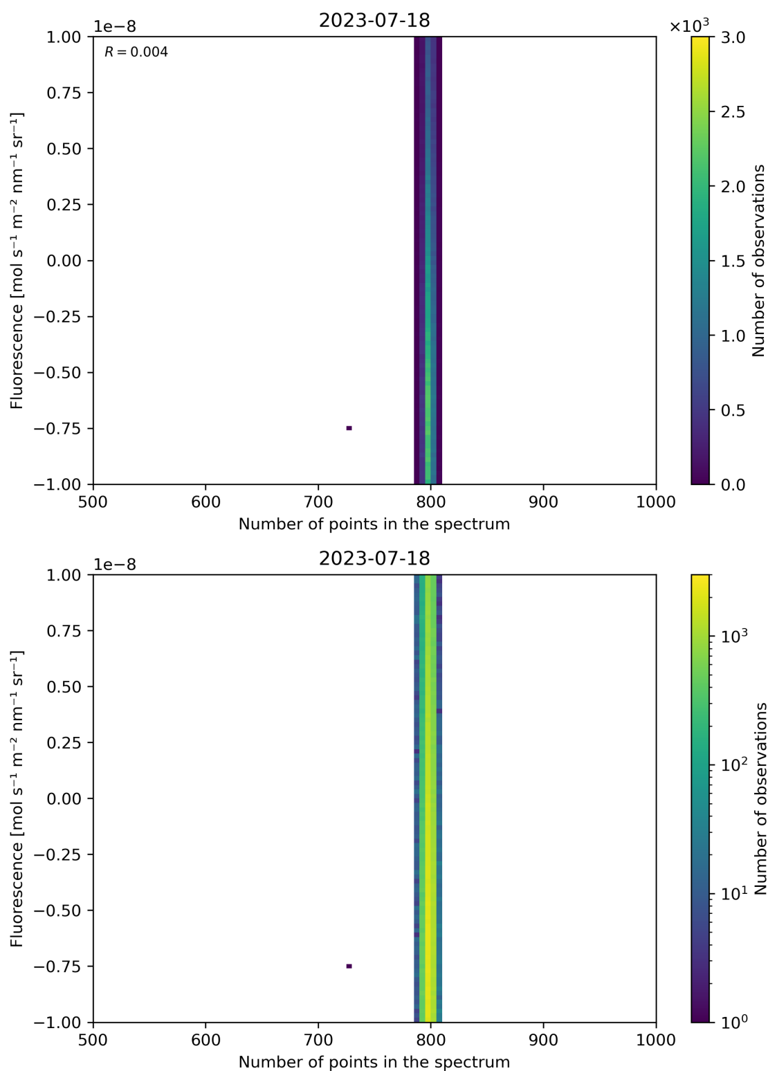
Figure 91: Scatter density plot of “Number of points in the spectrum” against “Fluorescence” for 2023-07-17 to 2023-07-19.
