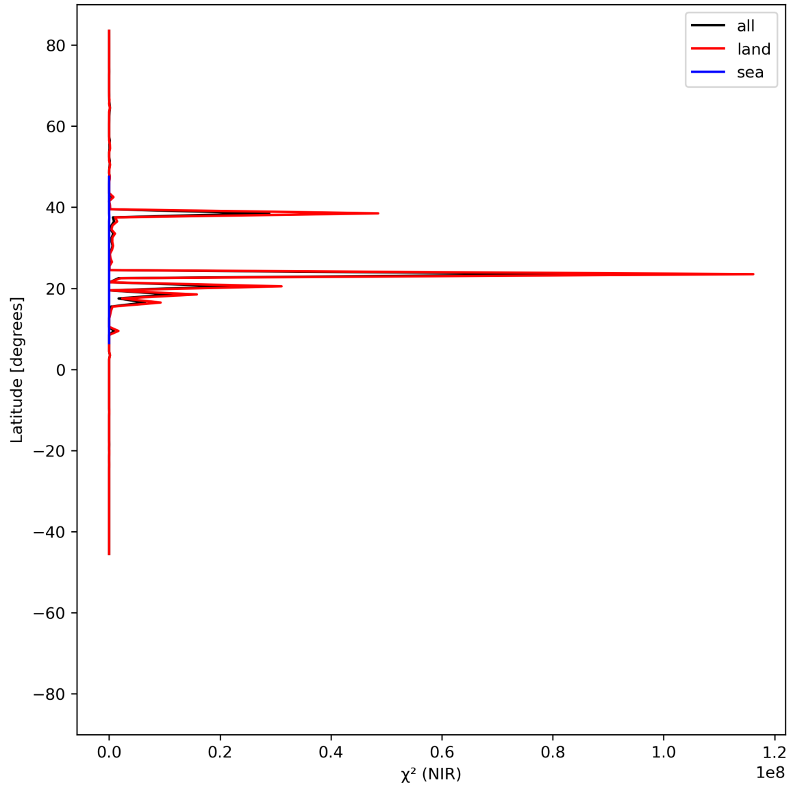
Figure 18: Zonal average of “ \chi^2 (NIR)” for 2023-07-17 to 2023-07-19.
