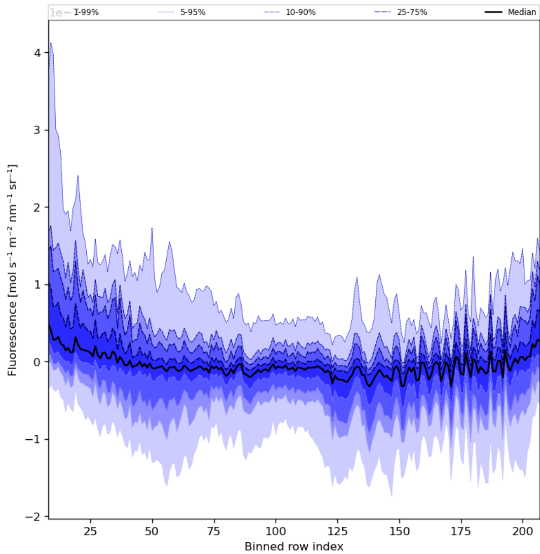
Figure 43: Along track statistics of “Fluorescence” for 2023-07-17 to 2023-07-19
