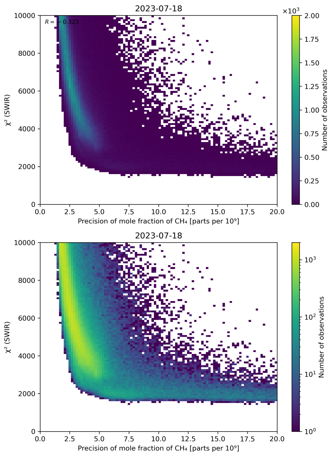
Figure 79: Scatter density plot of “Precision of mole fraction of CH 4 ” against “ \chi^2 (SWIR)” for 2023-07-17 to 2023-07-19.
