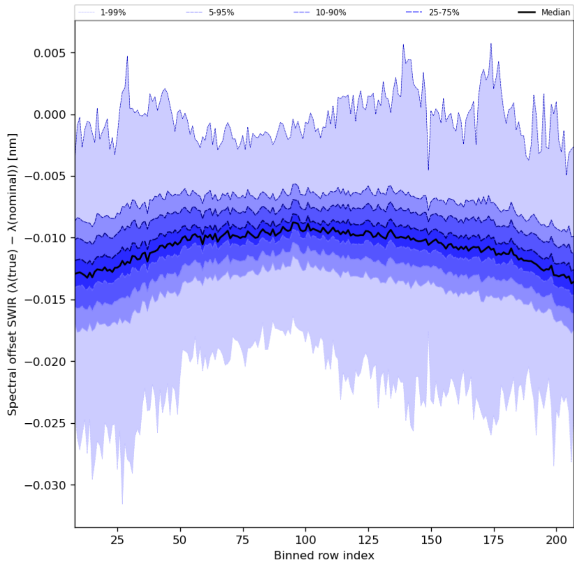
Figure 38: Along track statistics of “Spectral offset SWIR ( \lambda(\text{true}) - \lambda(\text{nominal}) )” for 2023-07-17 to 2023-07-19
