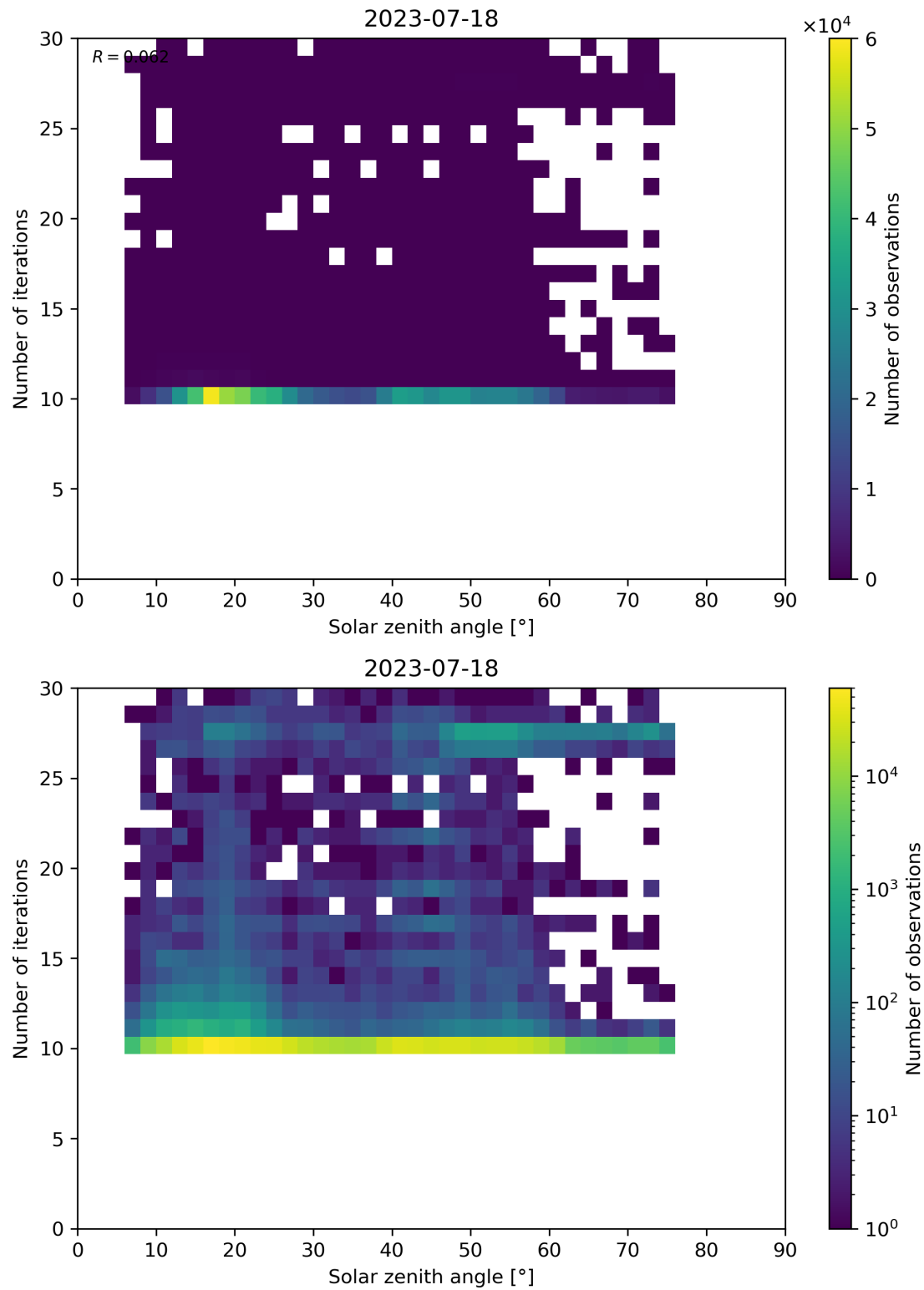
Figure 102: Scatter density plot of “Solar zenith angle” against “Number of iterations” for 2023-07-17 to 2023-07-19.
