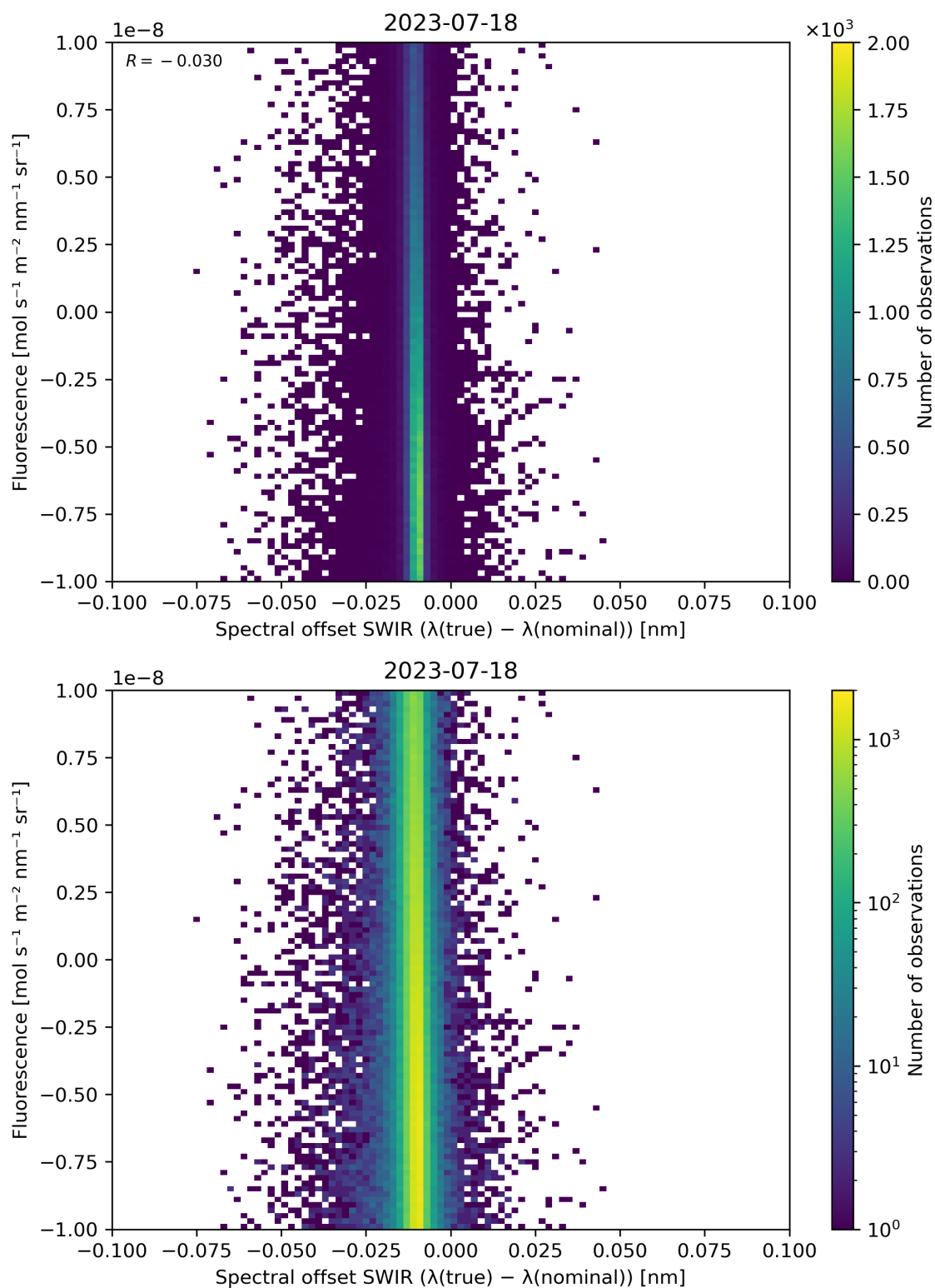
Figure 120: Scatter density plot of “Spectral offset SWIR ( \lambda(\text{true}) - \lambda(\text{nominal}) )” against “Fluorescence” for 2023-07-17 to 2023-07-19.
