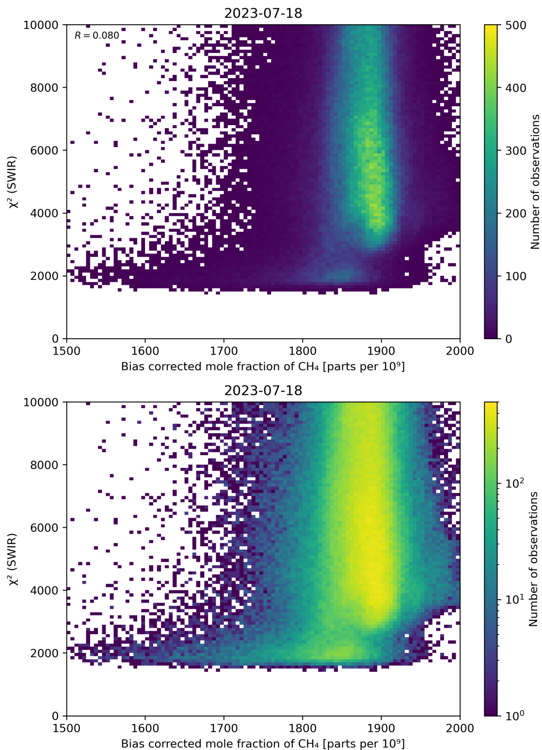
Figure 64: Scatter density plot of “Bias corrected mole fraction of CH 4 ” against “ \chi^2 (SWIR)” for 2023-07-17 to 2023-07-19.
