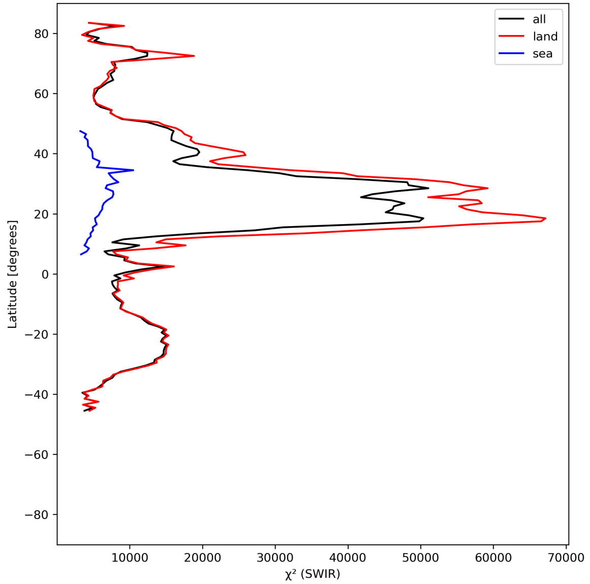
Figure 17: Zonal average of “ \chi^2 (SWIR)” for 2023-07-17 to 2023-07-19.
