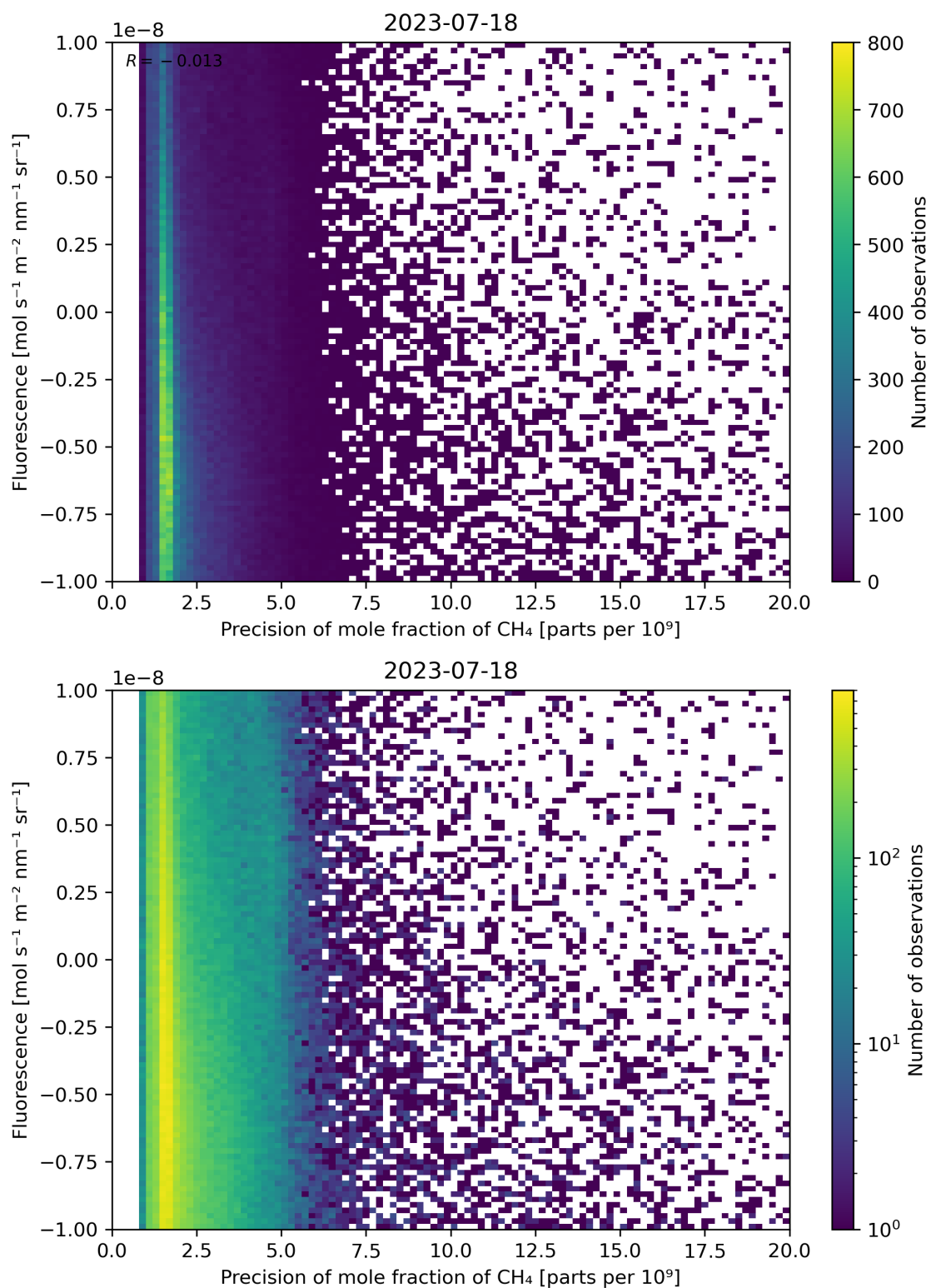
Figure 81: Scatter density plot of “Precision of mole fraction of CH 4 ” against “Fluorescence” for 2023-07-17 to 2023-07-19.
