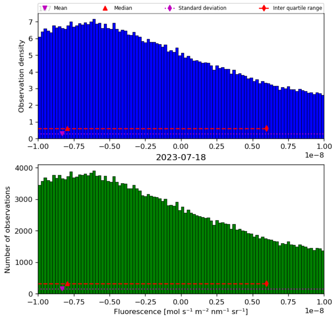
Figure 32: Histogram of “Fluorescence” for 2023-07-17 to 2023-07-19
