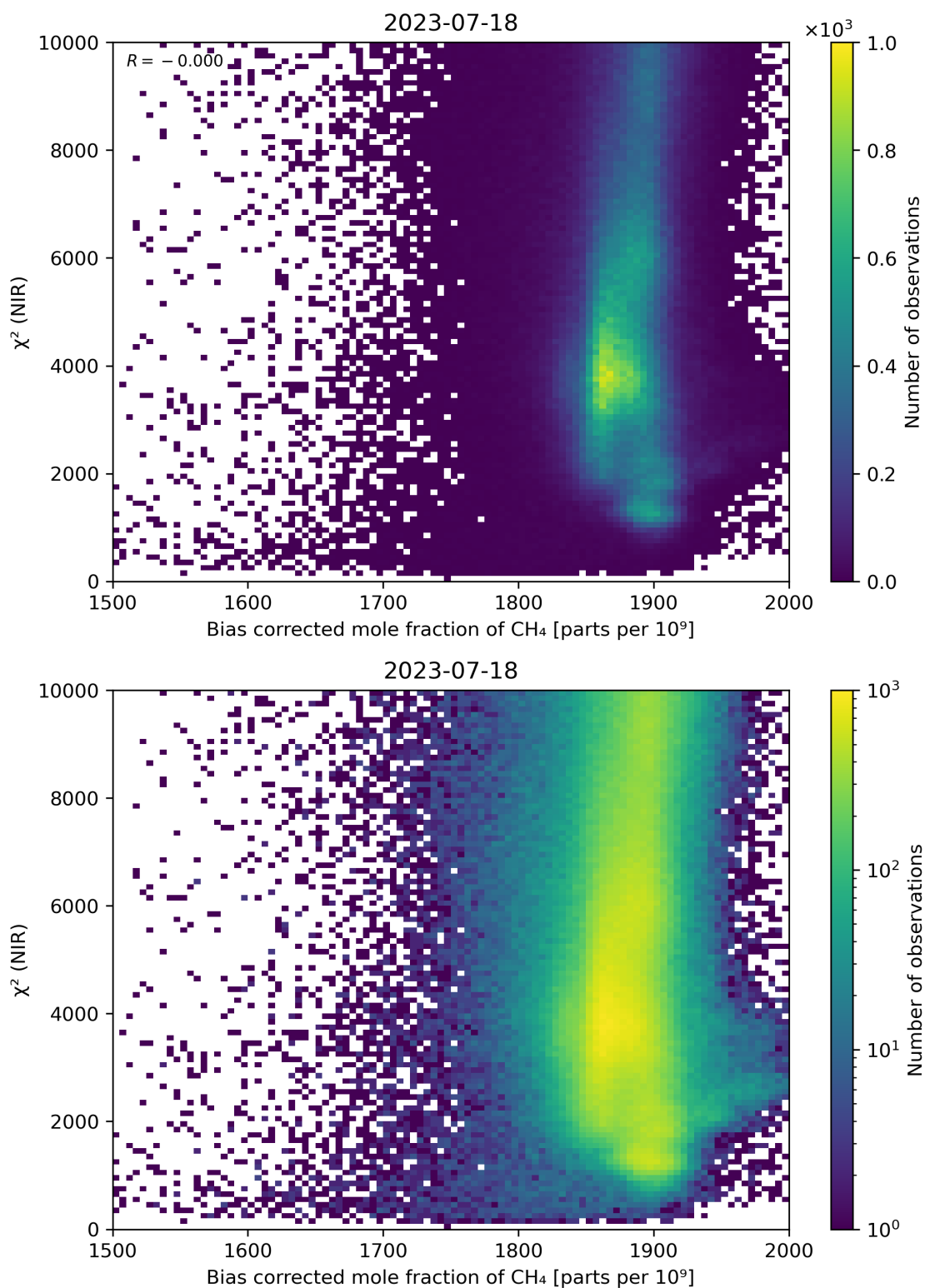
Figure 63: Scatter density plot of “Bias corrected mole fraction of CH 4 ” against “ \chi^2 (NIR)” for 2023-07-17 to 2023-07-19.
