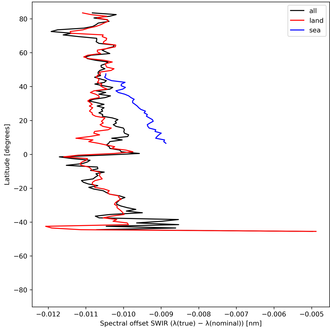
Figure 16: Zonal average of “Spectral offset SWIR ( \lambda(\text{true}) - \lambda(\text{nominal}) )” for 2023-07-17 to 2023-07-19.
