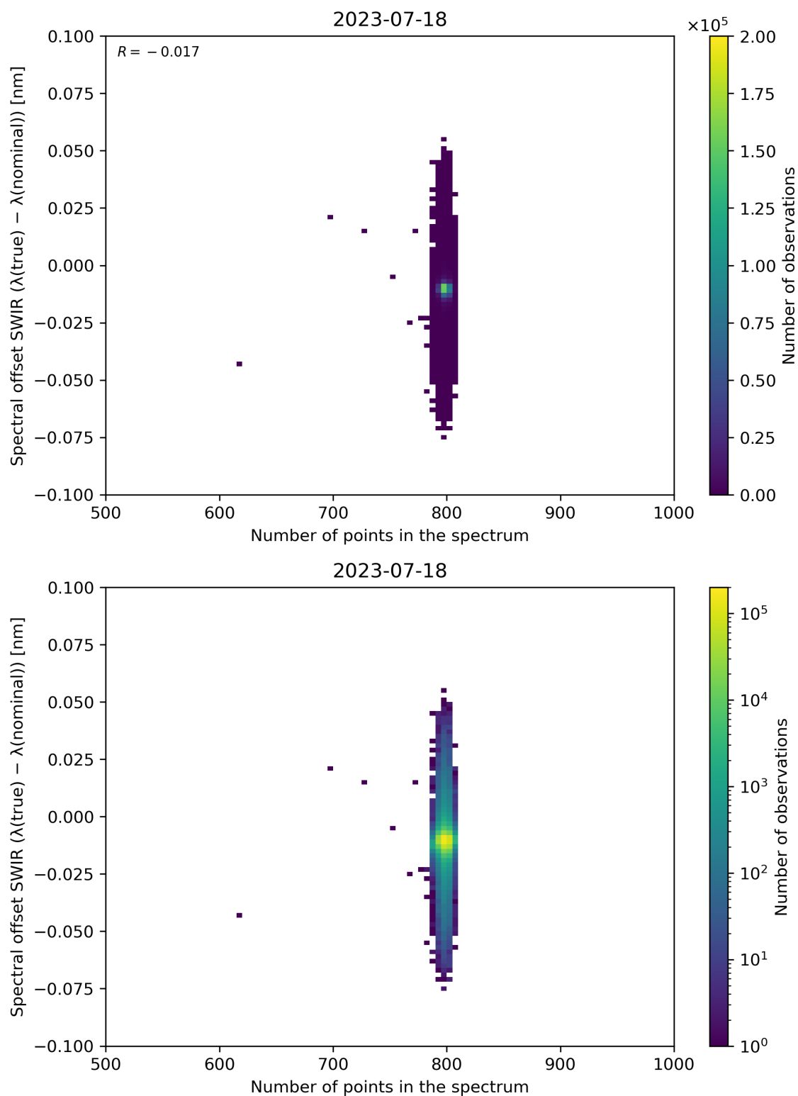
Figure 93: Scatter density plot of “Number of points in the spectrum” against “Spectral offset SWIR ( \lambda(\text{true}) - \lambda(\text{nominal}) )” for 2023-07-17 to 2023-07-19.
