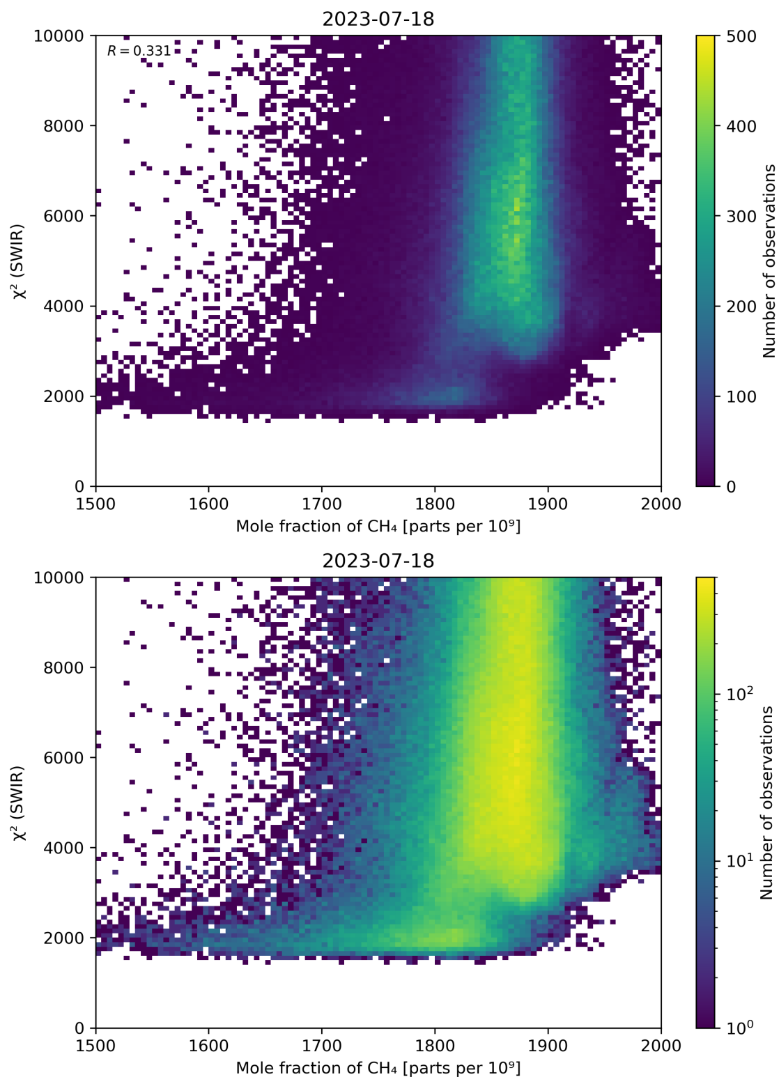
Figure 71: Scatter density plot of “Mole fraction of \text{CH}_4 ” against “ \chi^2 (SWIR)” for 2023-07-17 to 2023-07-19.
