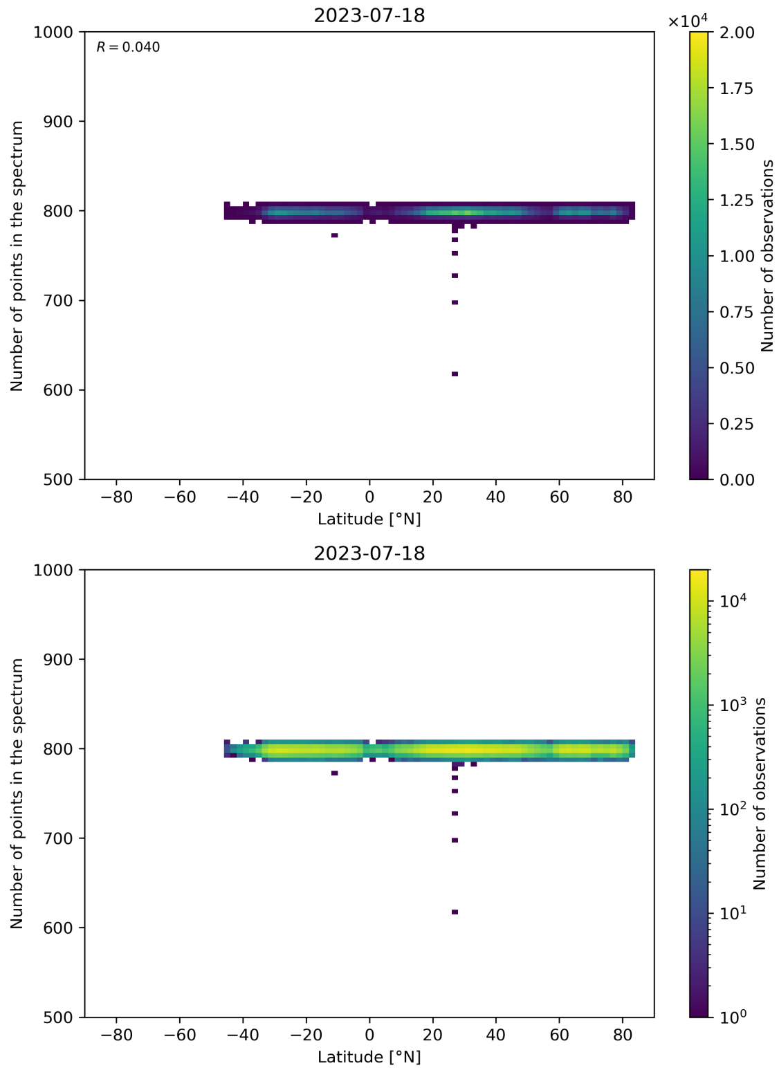
Figure 61: Scatter density plot of “Latitude” against “Number of points in the spectrum” for 2023-07-17 to 2023-07-19.
