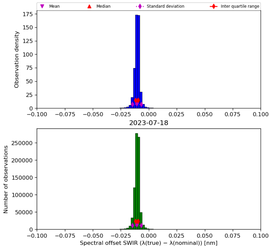
Figure 27: Histogram of “Spectral offset SWIR ( \lambda(\text{true}) - \lambda(\text{nominal}) )” for 2023-07-17 to 2023-07-19
