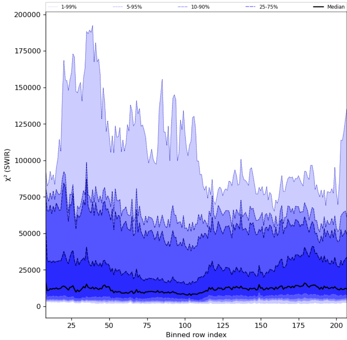
Figure 39: Along track statistics of “ \chi^2 (SWIR)” for 2023-07-17 to 2023-07-19
