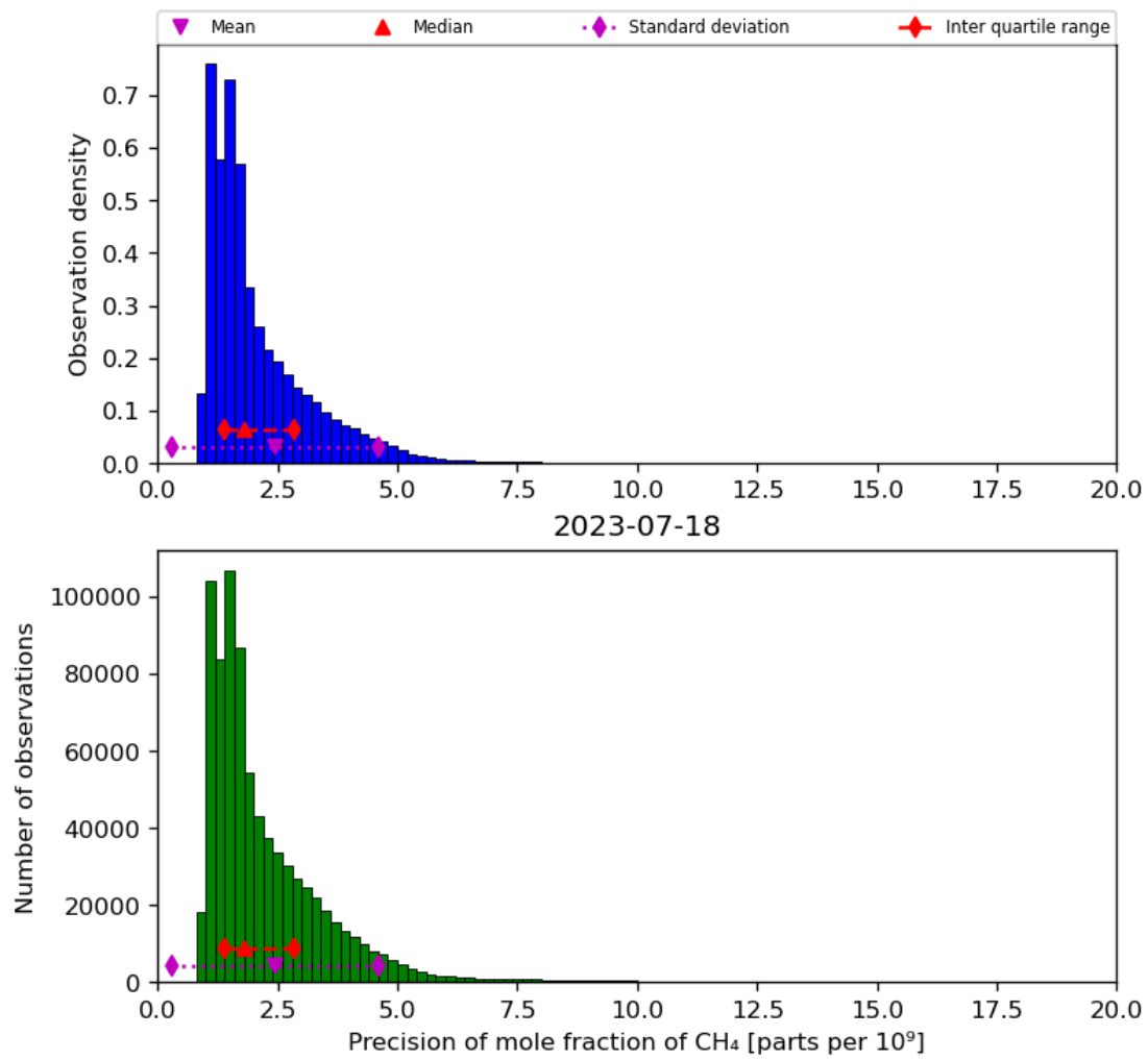
Figure 24: Histogram of “Precision of mole fraction of CH 4 ” for 2023-07-17 to 2023-07-19
