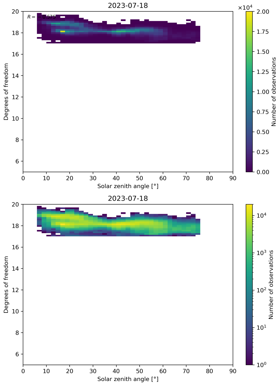
Figure 96: Scatter density plot of “Solar zenith angle” against “Degrees of freedom” for 2023-07-17 to 2023-07-19.
