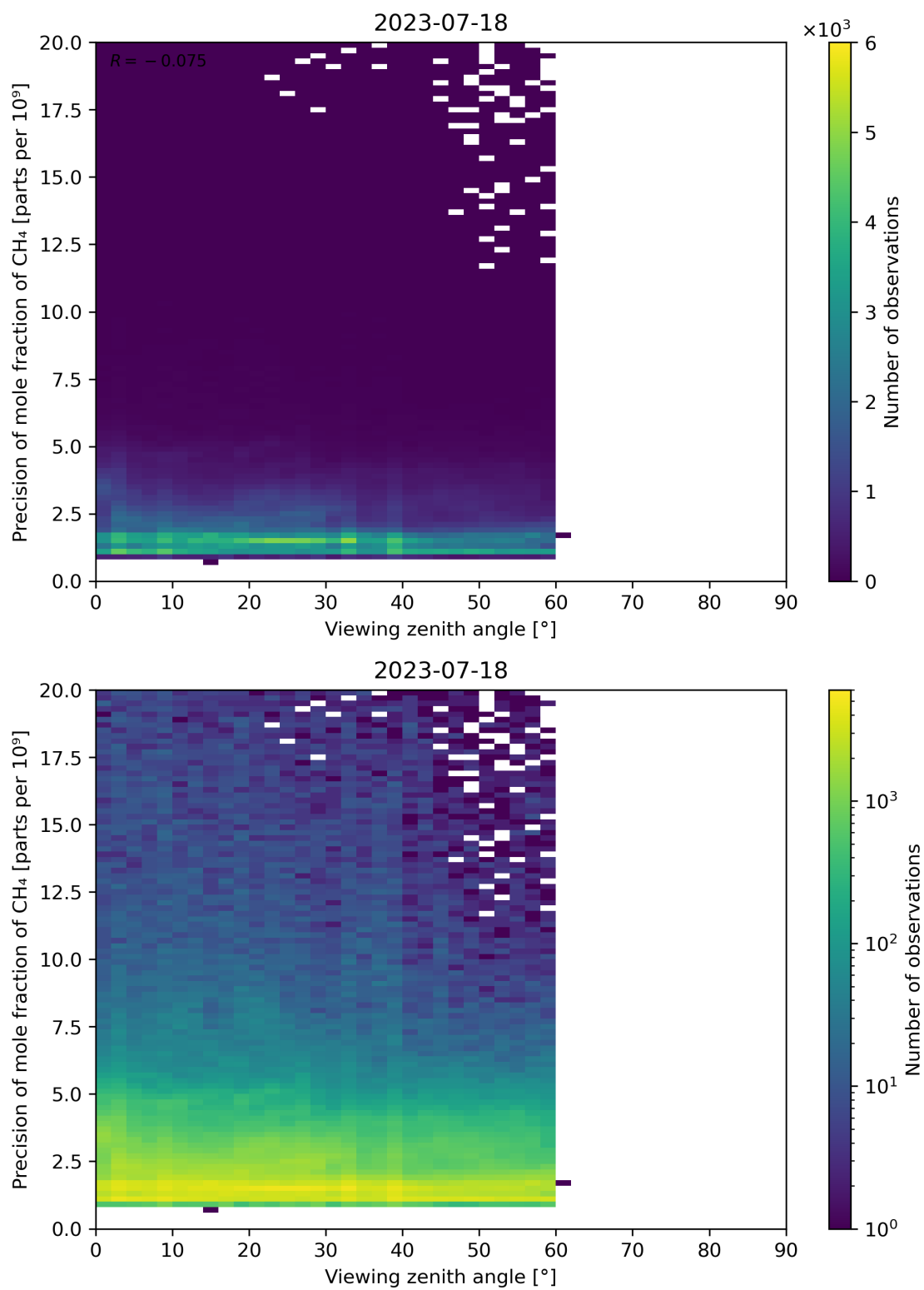
Figure 112: Scatter density plot of “Viewing zenith angle” against “Precision of mole fraction of CH 4 ” for 2023-07-17 to 2023-07-19.
