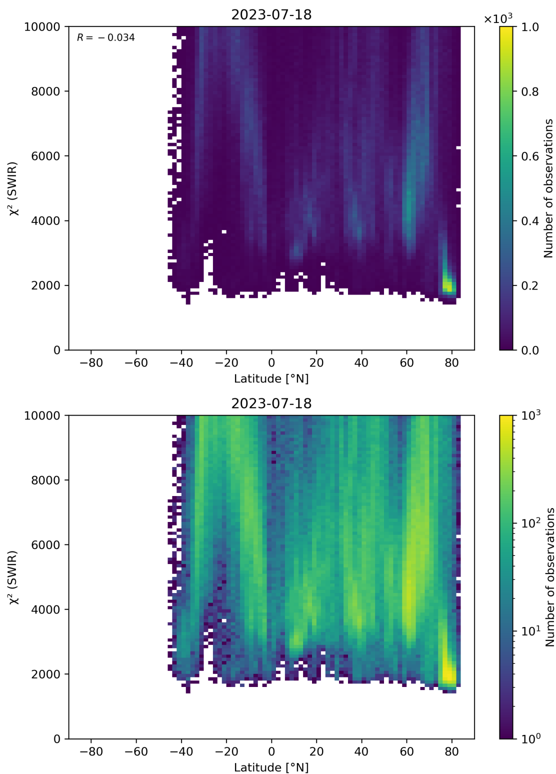
Figure 54: Scatter density plot of “Latitude” against “ \chi^2 (SWIR)” for 2023-07-17 to 2023-07-19.
