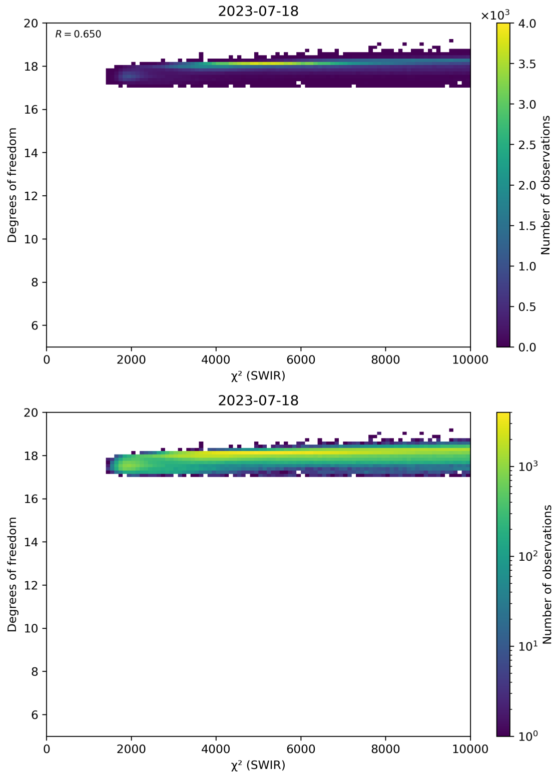
Figure 48: Scatter density plot of “ \chi^2 (SWIR)” against “Degrees of freedom” for 2023-07-17 to 2023-07-19.
