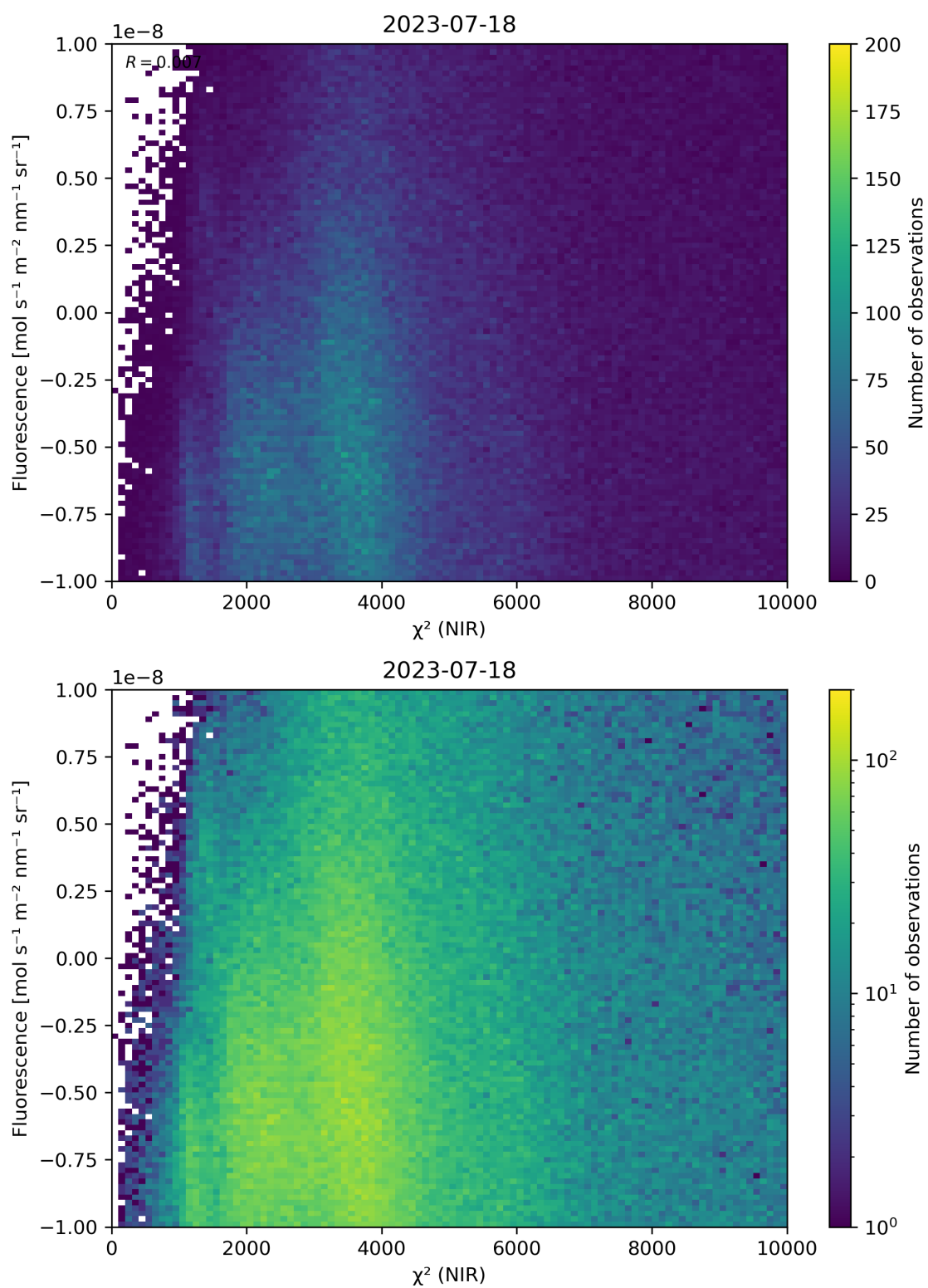
Figure 45: Scatter density plot of “ \chi^2 (NIR)” against “Fluorescence” for 2023-07-17 to 2023-07-19.
