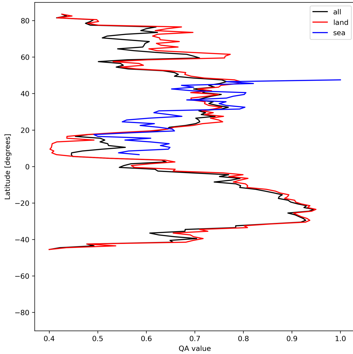
Figure 11: Zonal average of “QA value” for 2023-07-17 to 2023-07-19.
