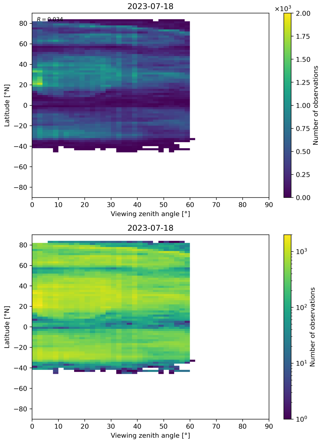
Figure 109: Scatter density plot of “Viewing zenith angle” against “Latitude” for 2023-07-17 to 2023-07-19.
