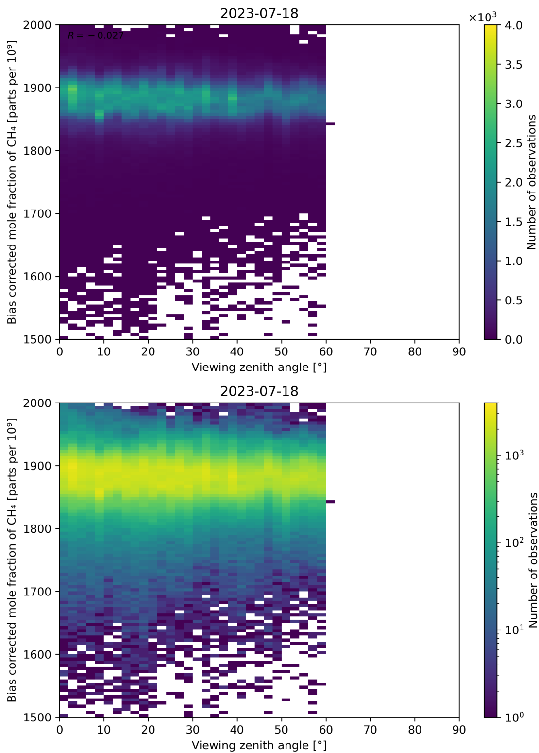
Figure 111: Scatter density plot of “Viewing zenith angle” against “Bias corrected mole fraction of CH 4 ” for 2023-07-17 to 2023-07-19.
