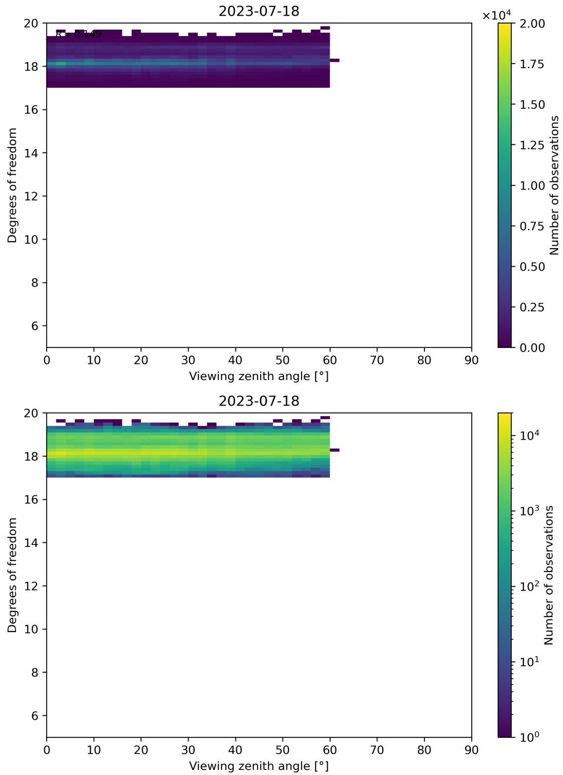
Figure 107: Scatter density plot of “Viewing zenith angle” against “Degrees of freedom” for 2023-07-17 to 2023-07-19.
