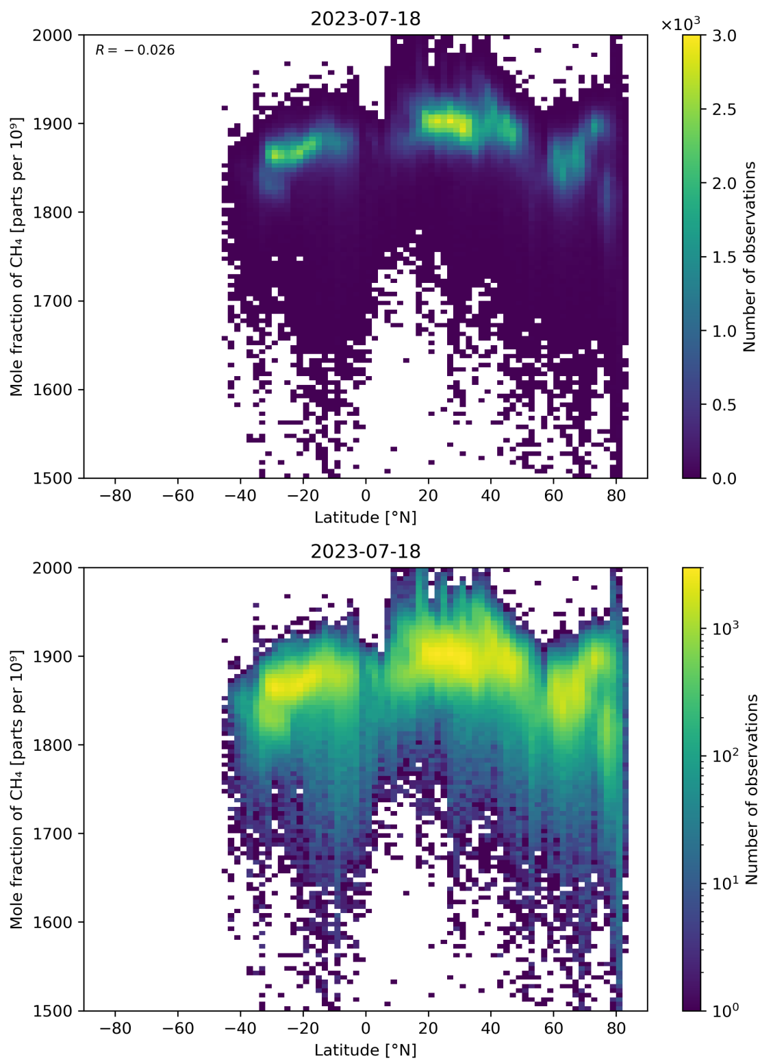
Figure 57: Scatter density plot of “Latitude” against “Mole fraction of \text{CH}_4 ” for 2023-07-17 to 2023-07-19.
