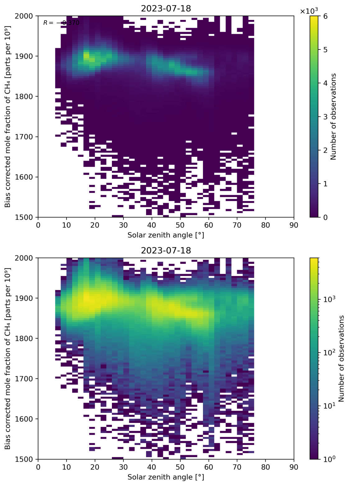
Figure 100: Scatter density plot of “Solar zenith angle” against “Bias corrected mole fraction of \text{CH}_4 ” for 2023-07-17 to 2023-07-19.
