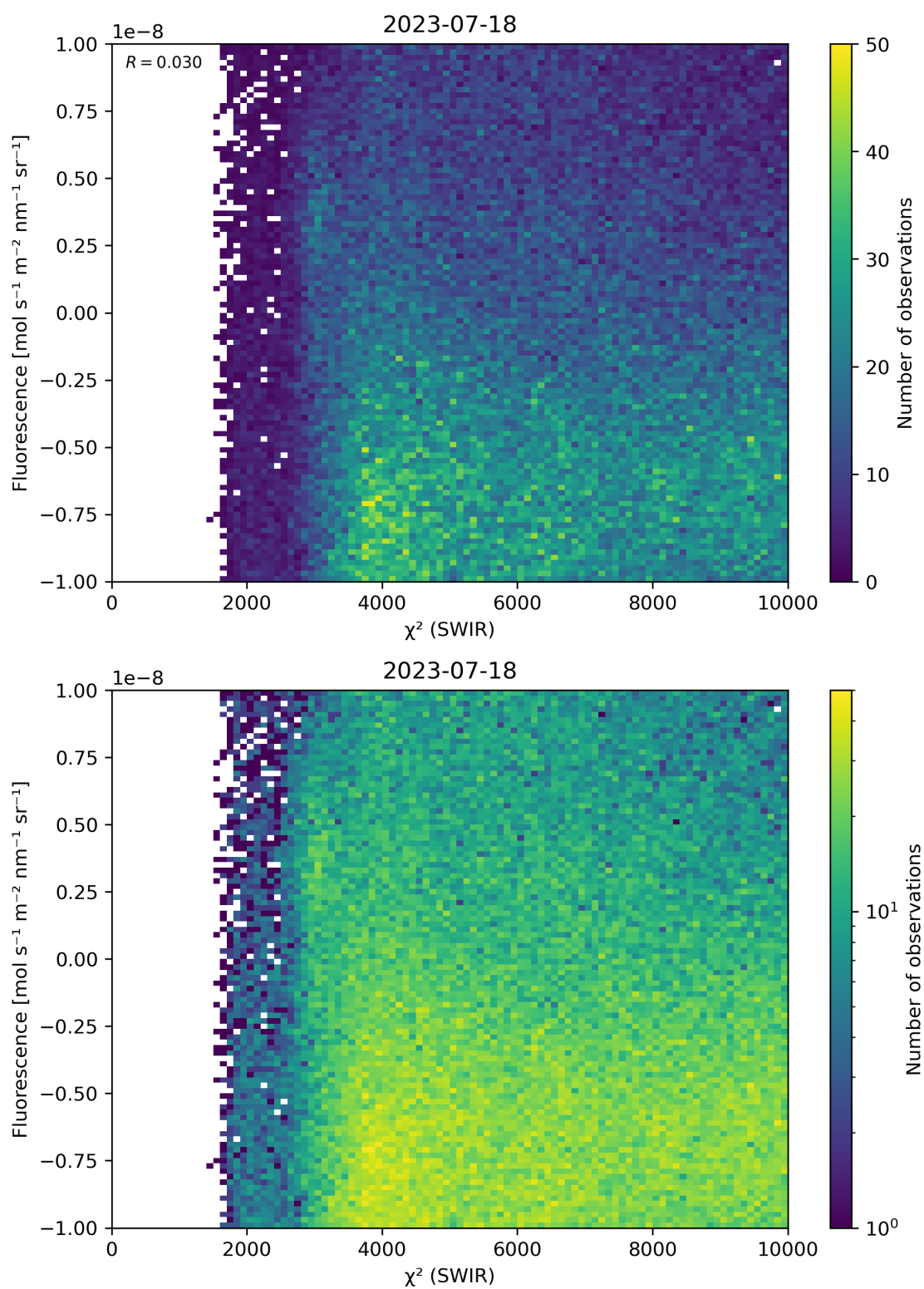
Figure 49: Scatter density plot of “ \chi^2 (SWIR)” against “Fluorescence” for 2023-07-17 to 2023-07-19.
