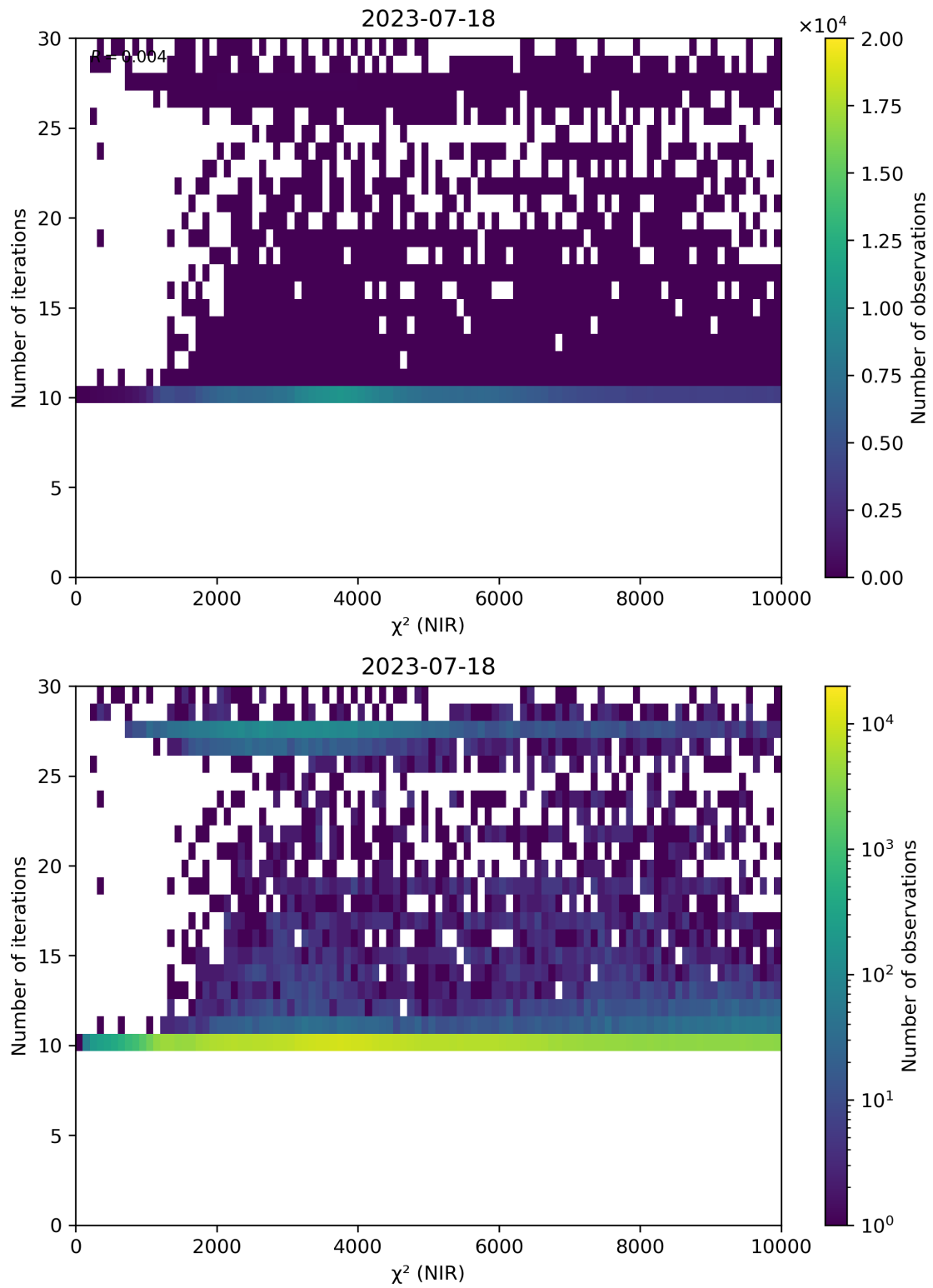
Figure 46: Scatter density plot of “ \chi^2 (NIR)” against “Number of iterations” for 2023-07-17 to 2023-07-19.
