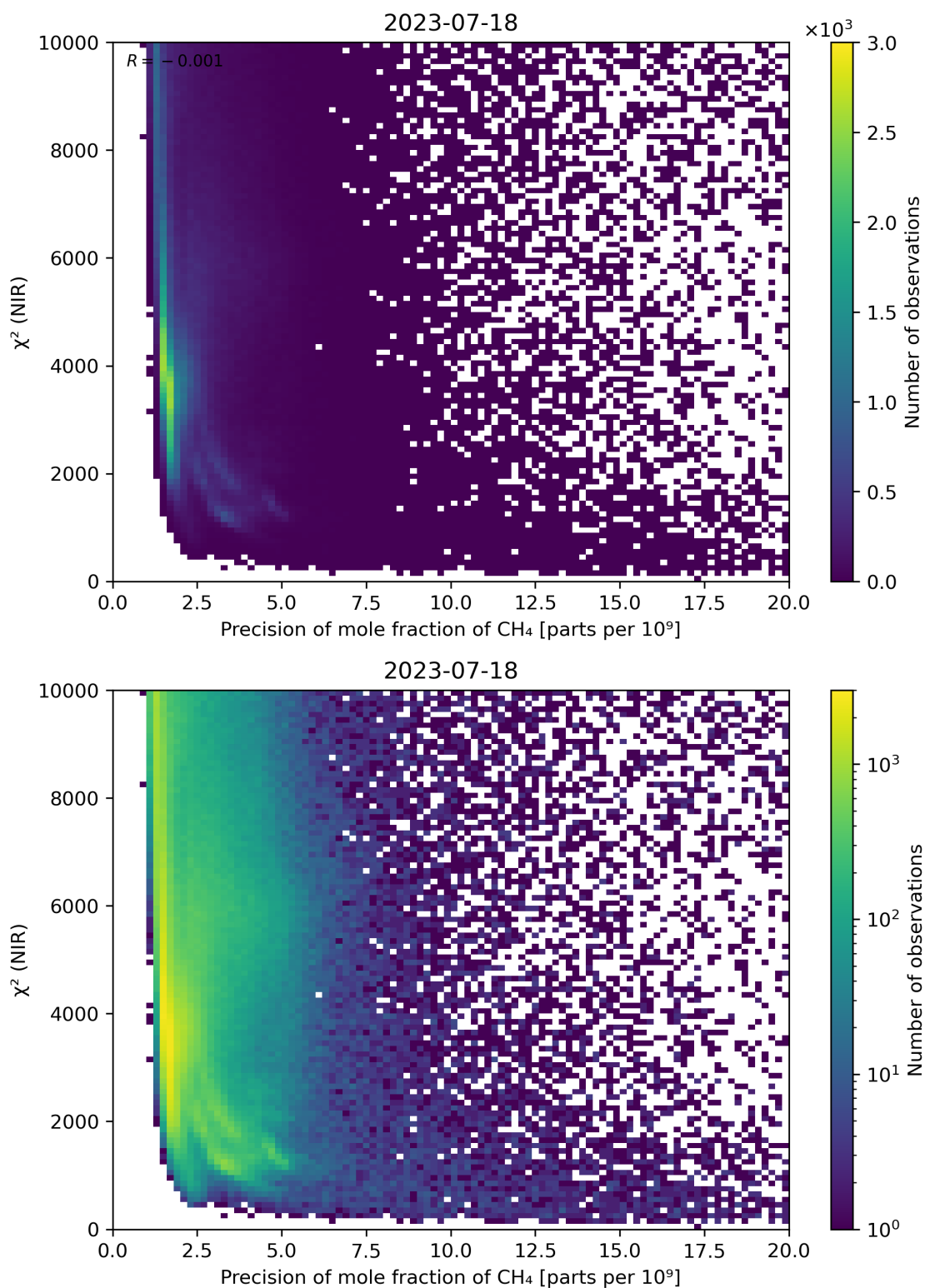
Figure 78: Scatter density plot of “Precision of mole fraction of CH 4 ” against “ \chi^2 (NIR)” for 2023-07-17 to 2023-07-19.
