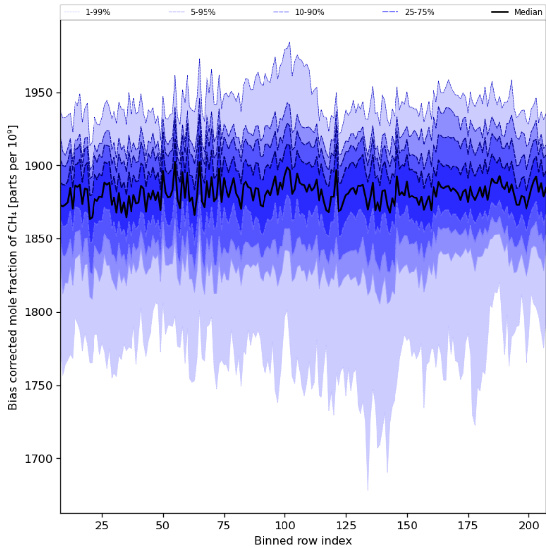
Figure 36: Along track statistics of “Bias corrected mole fraction of CH 4 ” for 2023-07-17 to 2023-07-19
