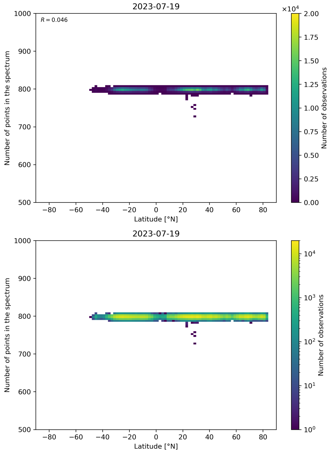
Figure 61: Scatter density plot of “Latitude” against “Number of points in the spectrum” for 2023-07-19 to 2023-07-20.
