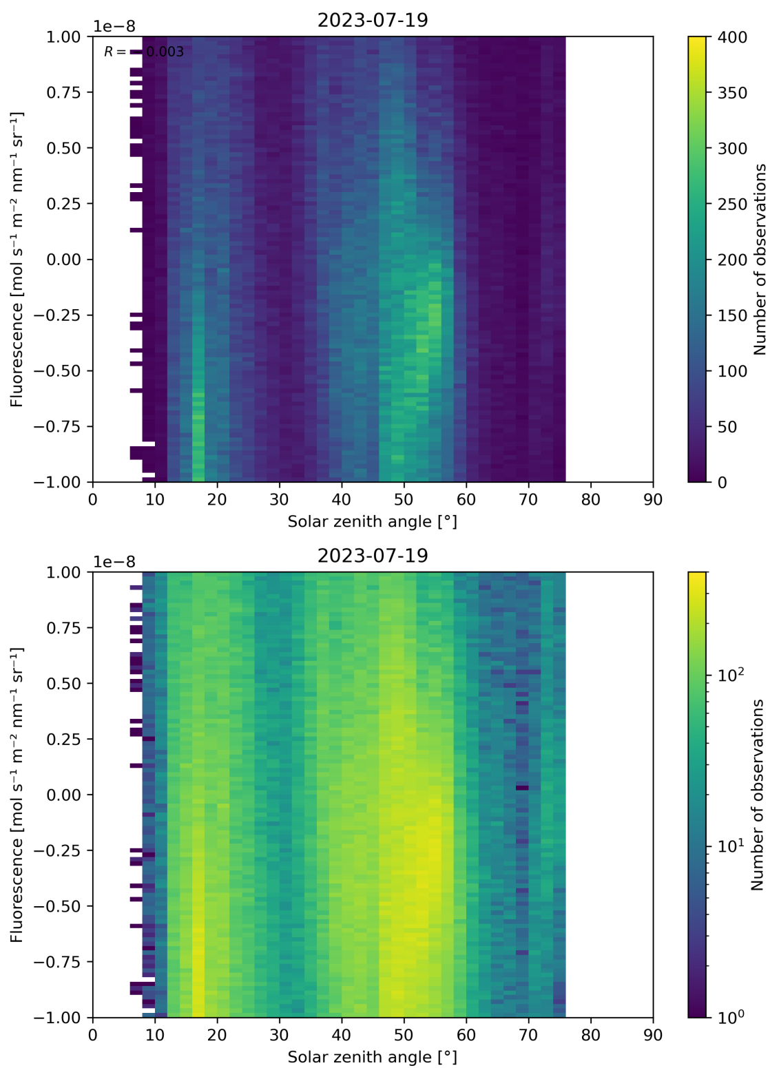
Figure 97: Scatter density plot of “Solar zenith angle” against “Fluorescence” for 2023-07-19 to 2023-07-20.
