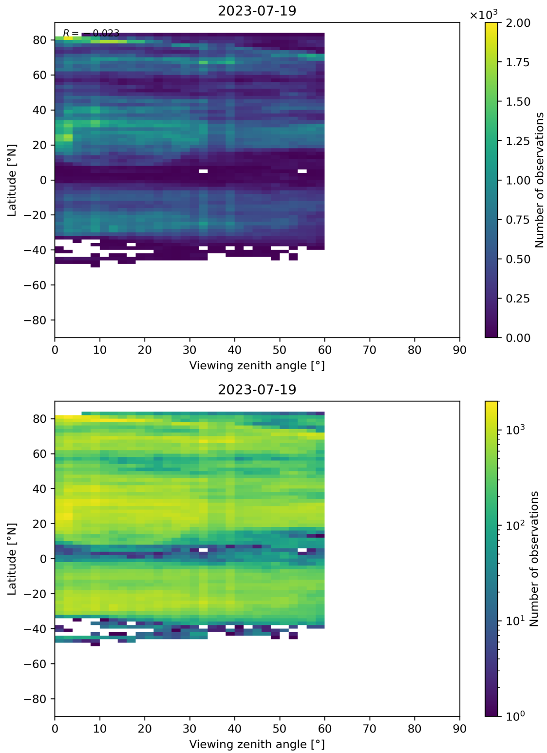
Figure 109: Scatter density plot of “Viewing zenith angle” against “Latitude” for 2023-07-19 to 2023-07-20.
