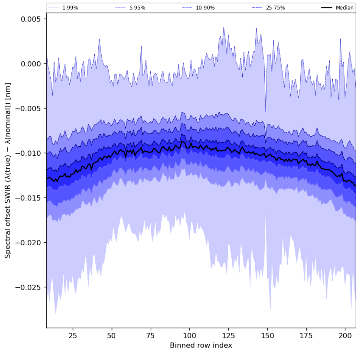
Figure 38: Along track statistics of “Spectral offset SWIR ( \lambda(\text{true}) - \lambda(\text{nominal}) )” for 2023-07-19 to 2023-07-20
