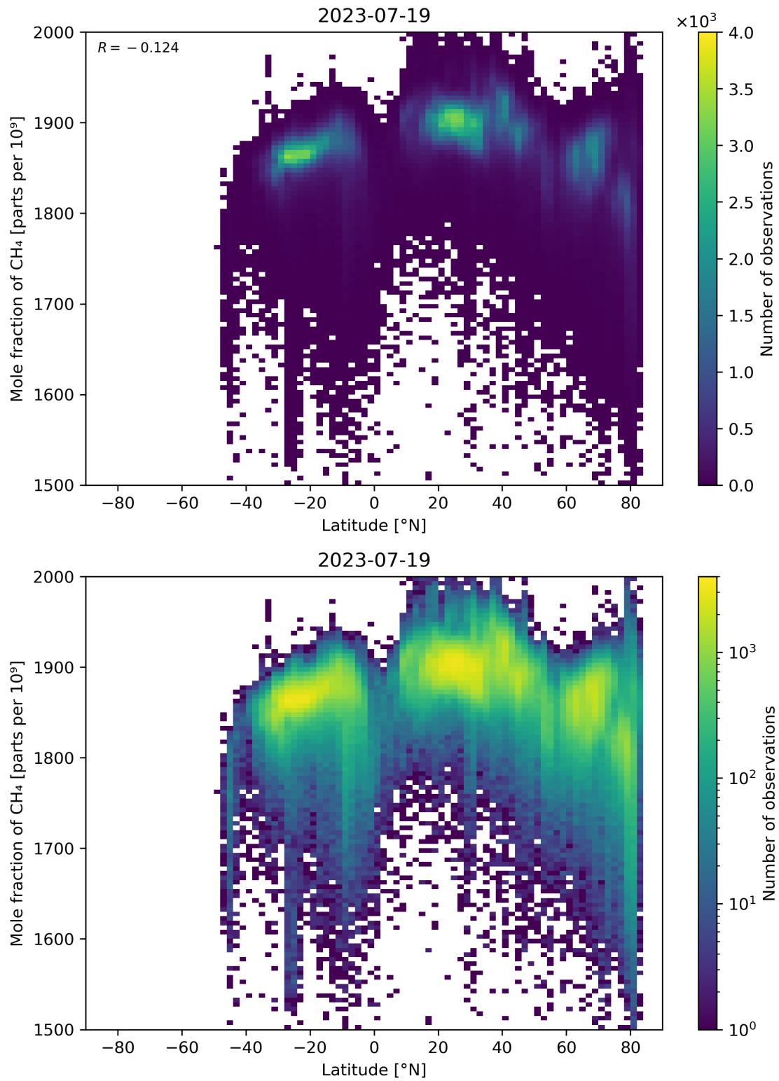
Figure 57: Scatter density plot of “Latitude” against “Mole fraction of \text{CH}_4 ” for 2023-07-19 to 2023-07-20.
