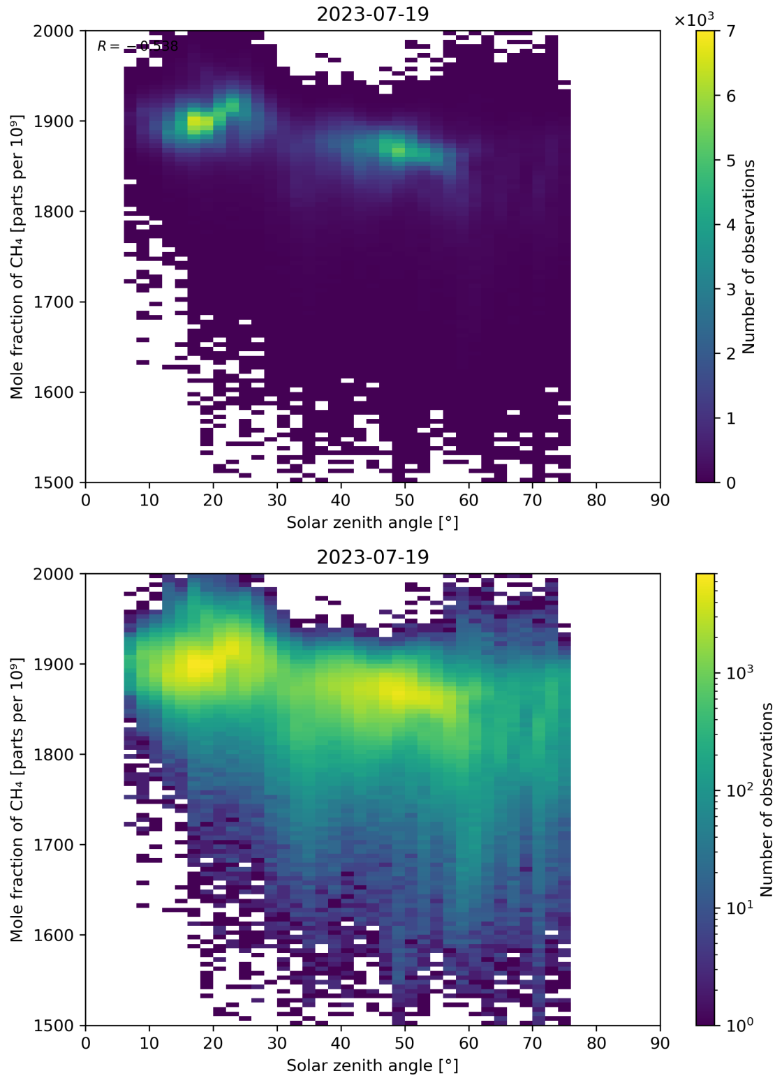
Figure 99: Scatter density plot of “Solar zenith angle” against “Mole fraction of CH 4 ” for 2023-07-19 to 2023-07-20.
