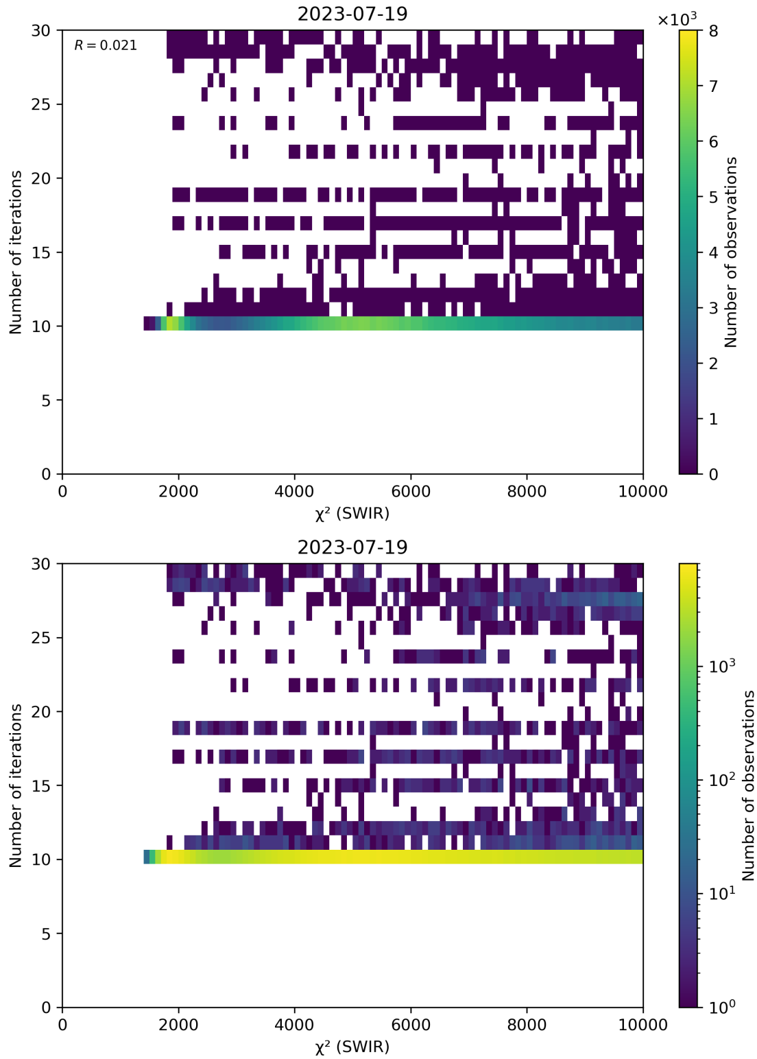
Figure 50: Scatter density plot of “ \chi^2 (SWIR)” against “Number of iterations” for 2023-07-19 to 2023-07-20.
