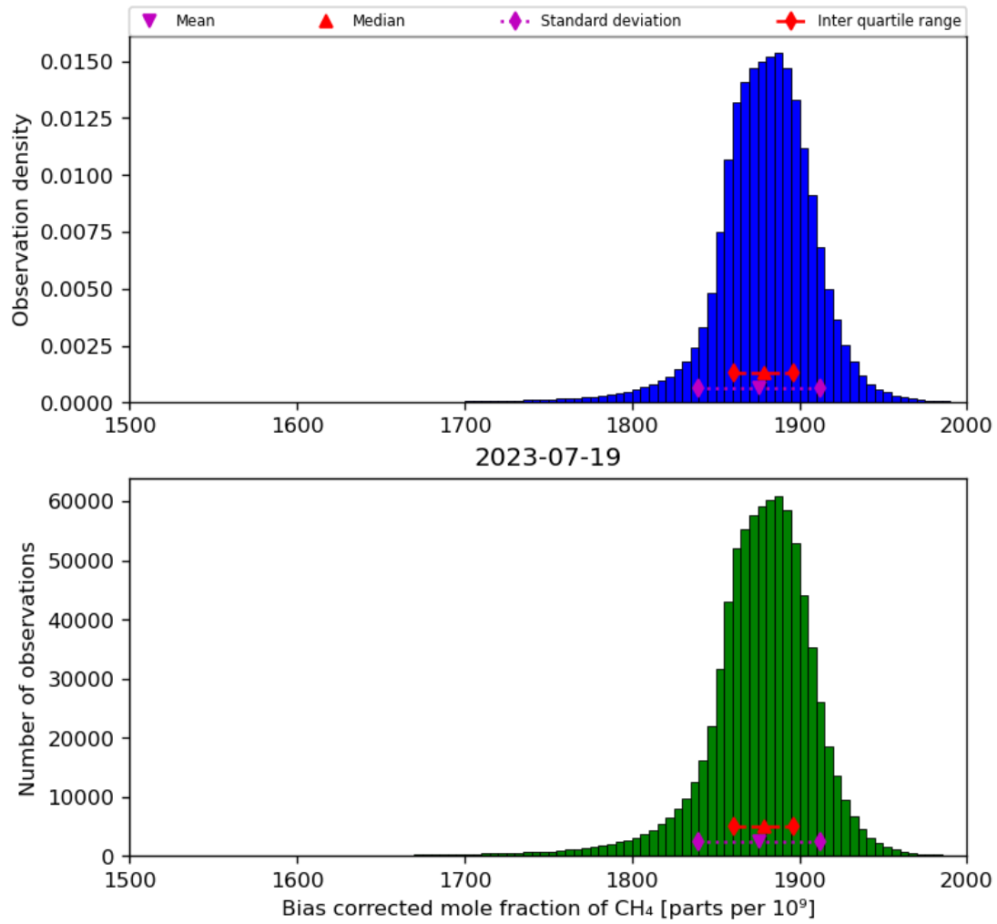
Figure 25: Histogram of “Bias corrected mole fraction of CH 4 ” for 2023-07-19 to 2023-07-20
