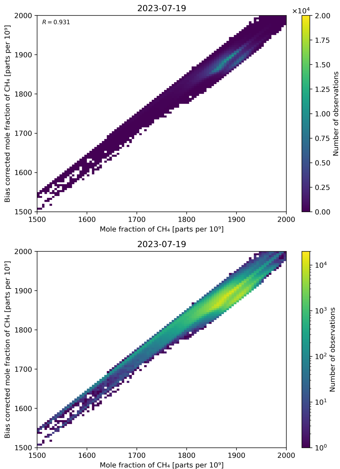
Figure 74: Scatter density plot of “Mole fraction of CH 4 ” against “Bias corrected mole fraction of CH 4 ” for 2023-07-19 to 2023-07-20.
