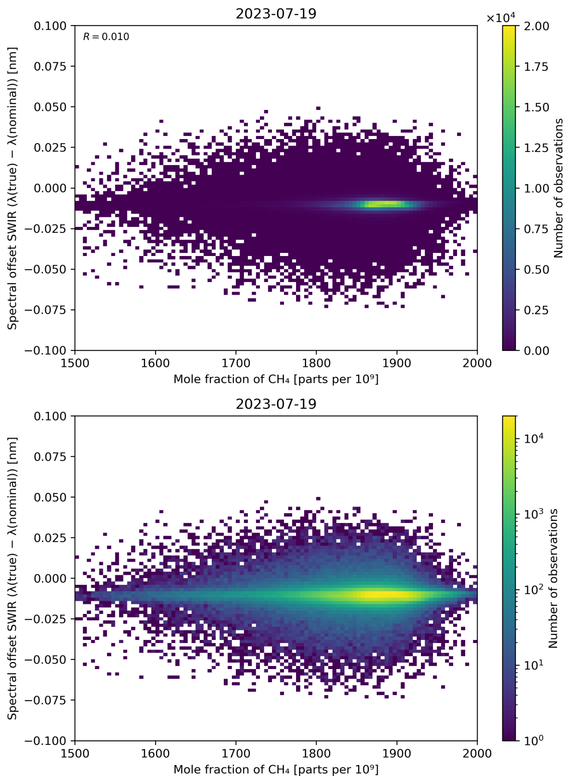
Figure 86: Scatter density plot of “Mole fraction of CH 4 ” against “Spectral offset SWIR ( \lambda(\text{true}) - \lambda(\text{nominal}) )” for 2023-07-19 to 2023-07-20.
