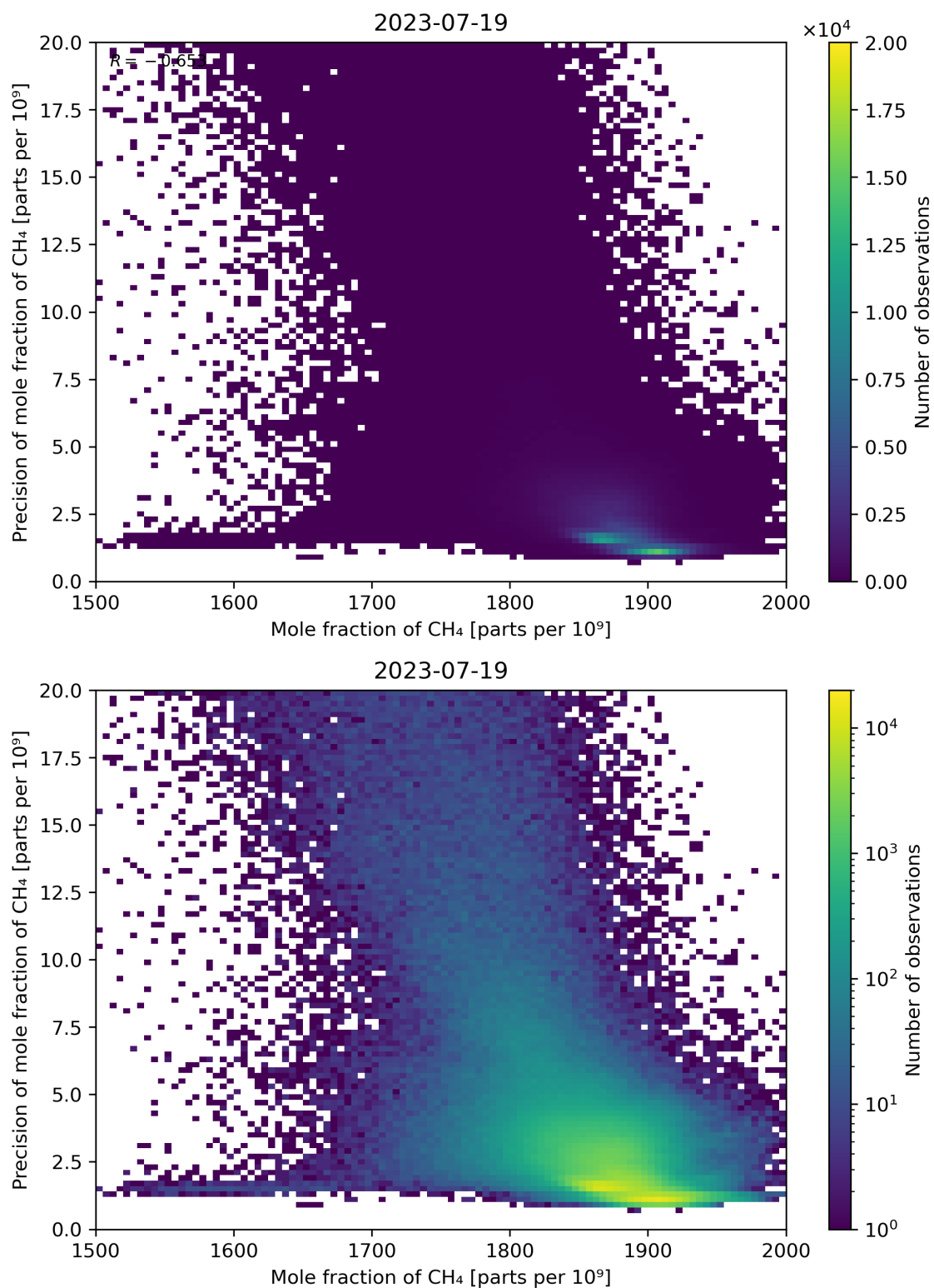
Figure 75: Scatter density plot of “Mole fraction of CH 4 ” against “Precision of mole fraction of CH 4 ” for 2023-07-19 to 2023-07-20.
