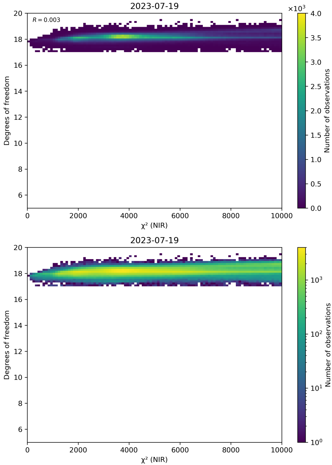
Figure 44: Scatter density plot of “ \chi^2 (NIR)” against “Degrees of freedom” for 2023-07-19 to 2023-07-20.
