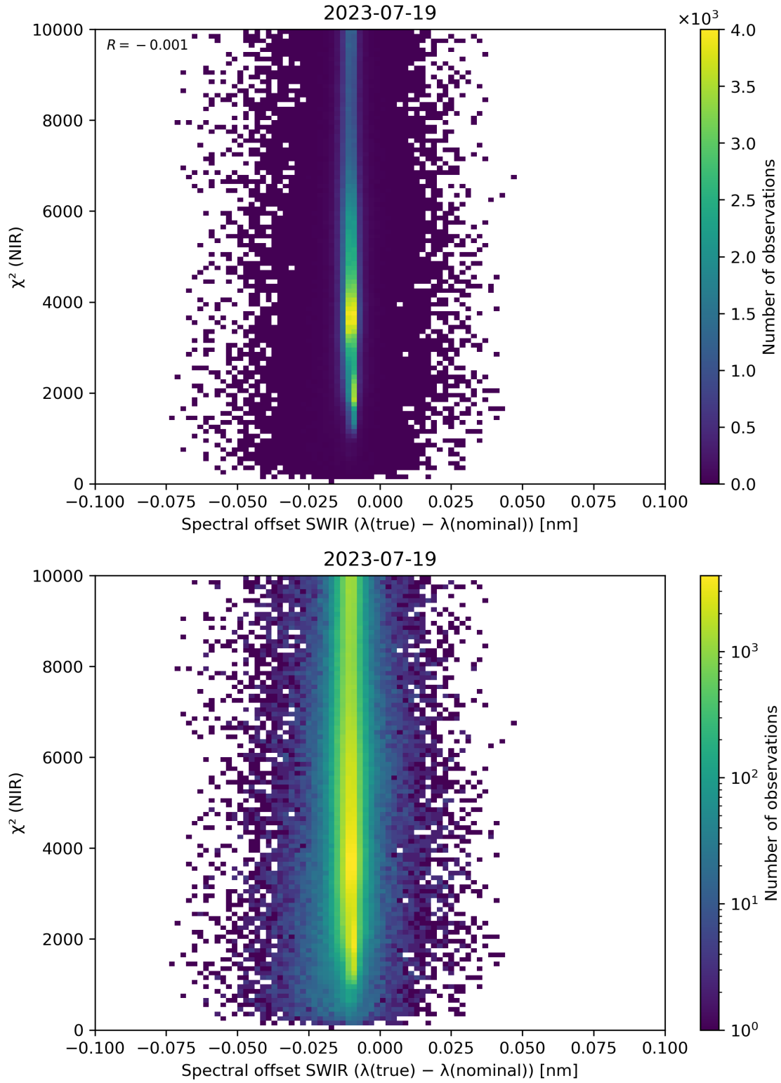
Figure 117: Scatter density plot of “Spectral offset SWIR ( \lambda(\text{true}) - \lambda(\text{nominal}) )” against “ \chi^2 (NIR)” for 2023-07-19 to 2023-07-20.
