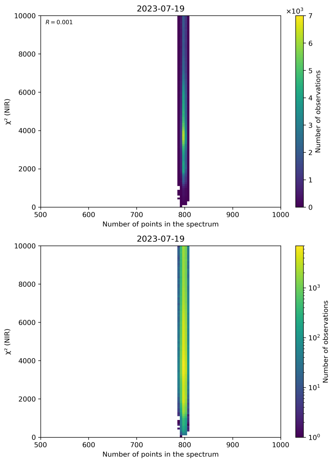
Figure 88: Scatter density plot of “Number of points in the spectrum” against “ \chi^2 (NIR)” for 2023-07-19 to 2023-07-20.
