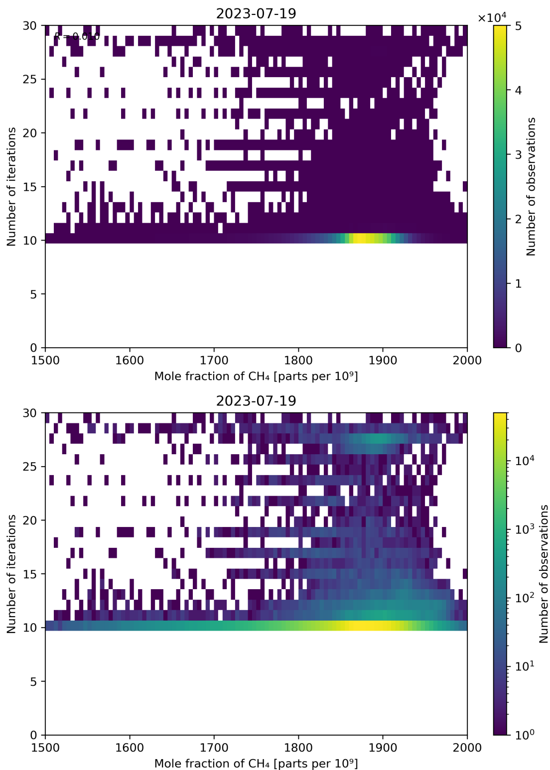
Figure 76: Scatter density plot of “Mole fraction of CH 4 ” against “Number of iterations” for 2023-07-19 to 2023-07-20.
