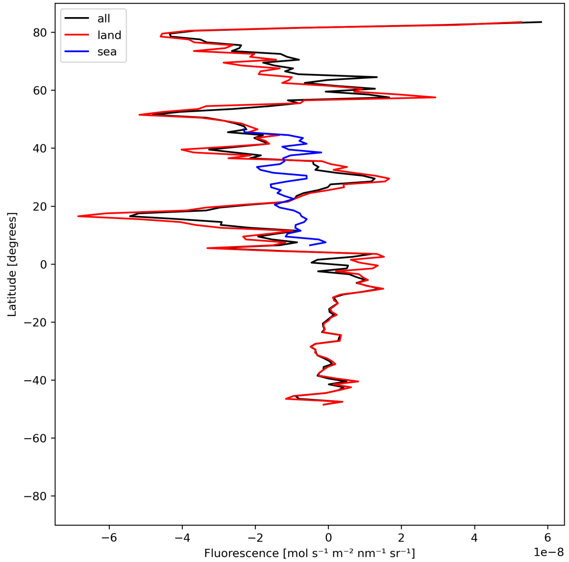
Figure 21: Zonal average of “Fluorescence” for 2023-07-19 to 2023-07-20.
