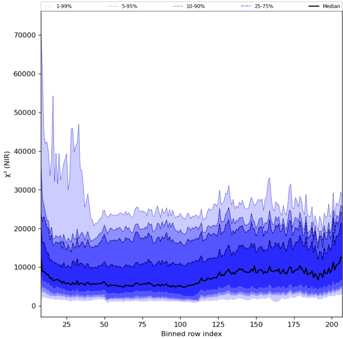
Figure 40: Along track statistics of " \chi^2 (NIR)" for 2023-07-19 to 2023-07-20
