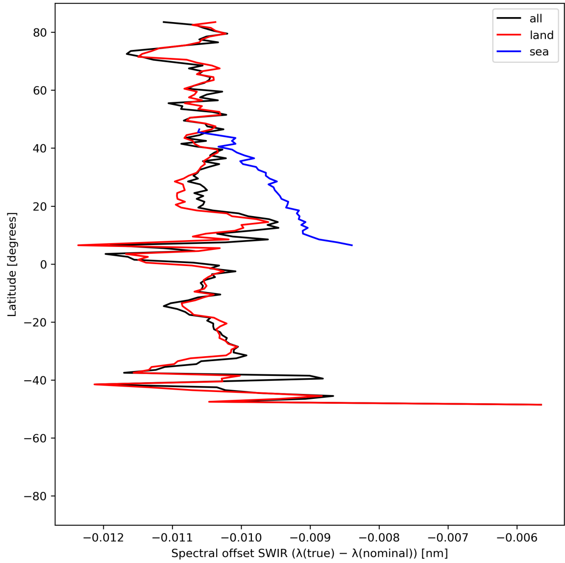
Figure 16: Zonal average of “Spectral offset SWIR ( \lambda(\text{true}) - \lambda(\text{nominal}) )” for 2023-07-19 to 2023-07-20.
