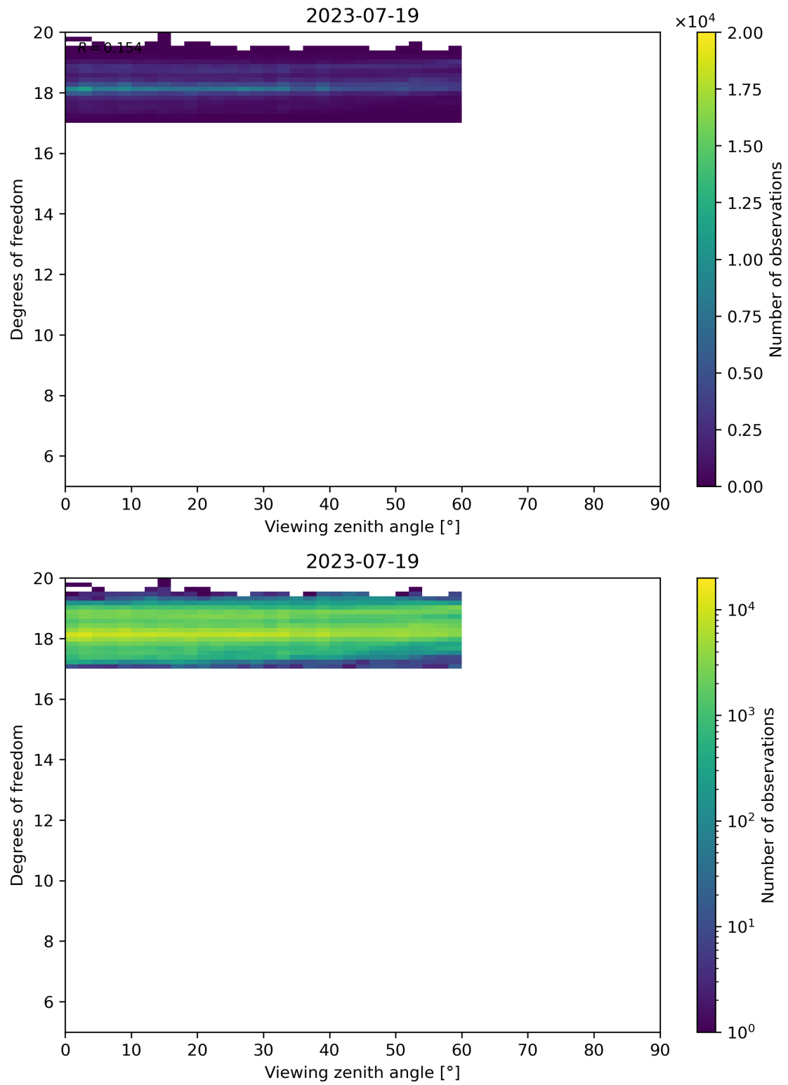
Figure 107: Scatter density plot of “Viewing zenith angle” against “Degrees of freedom” for 2023-07-19 to 2023-07-20.
