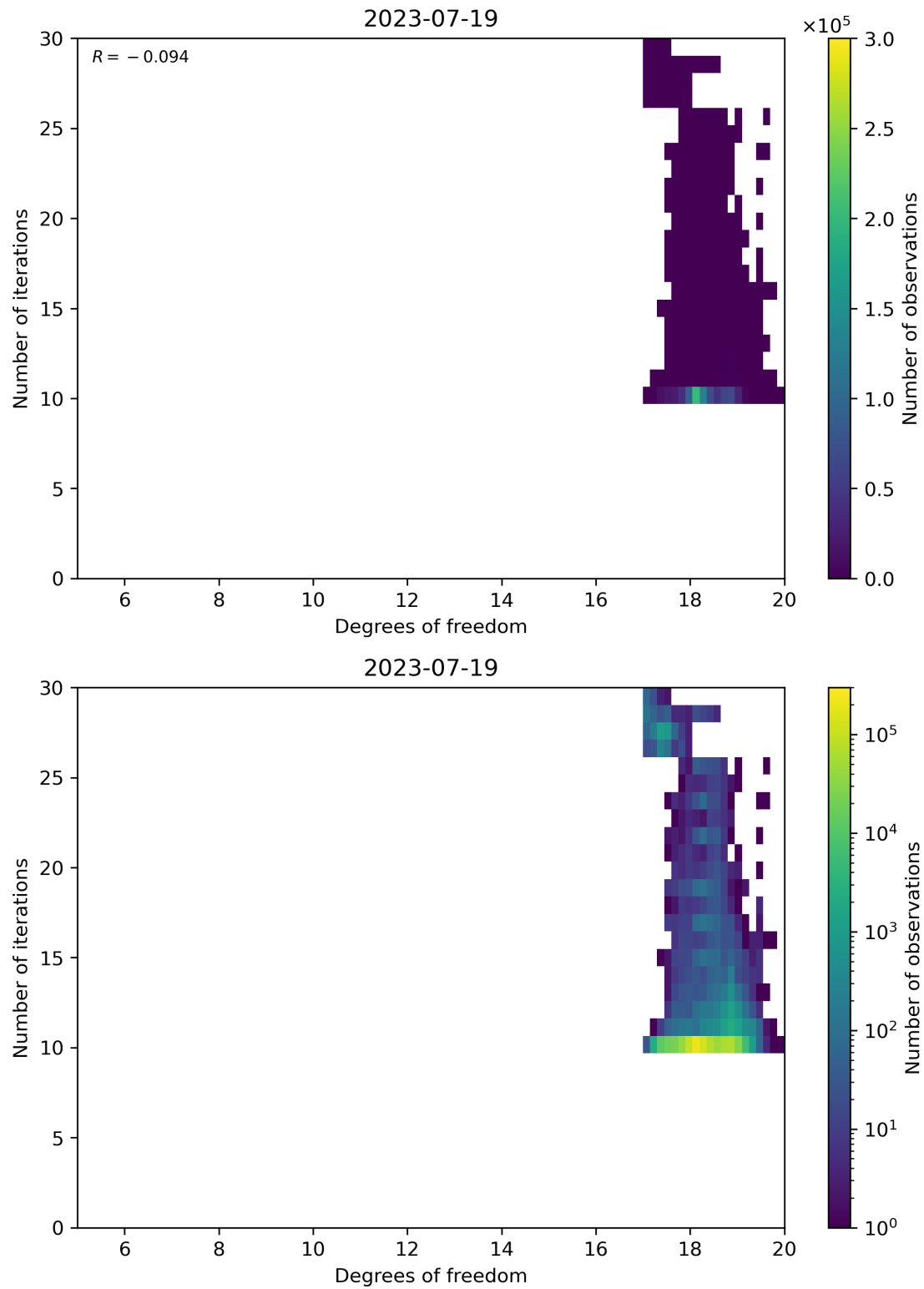
Figure 52: Scatter density plot of “Degrees of freedom” against “Number of iterations” for 2023-07-19 to 2023-07-20.
