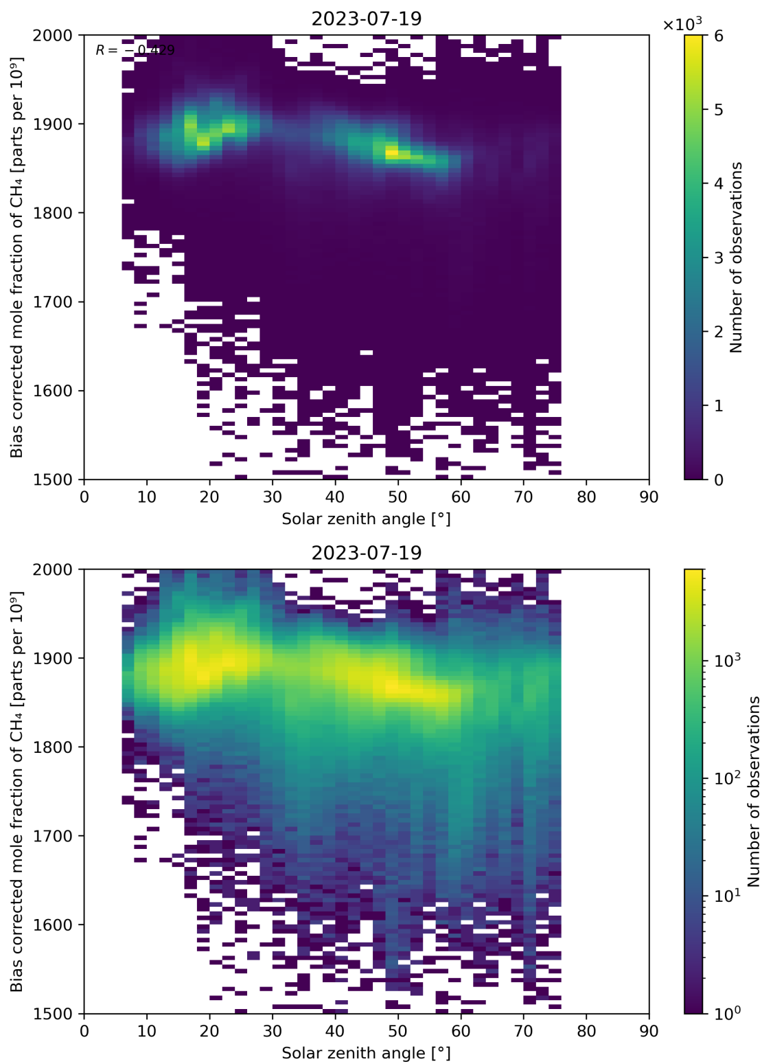
Figure 100: Scatter density plot of “Solar zenith angle” against “Bias corrected mole fraction of CH 4 ” for 2023-07-19 to 2023-07-20.
