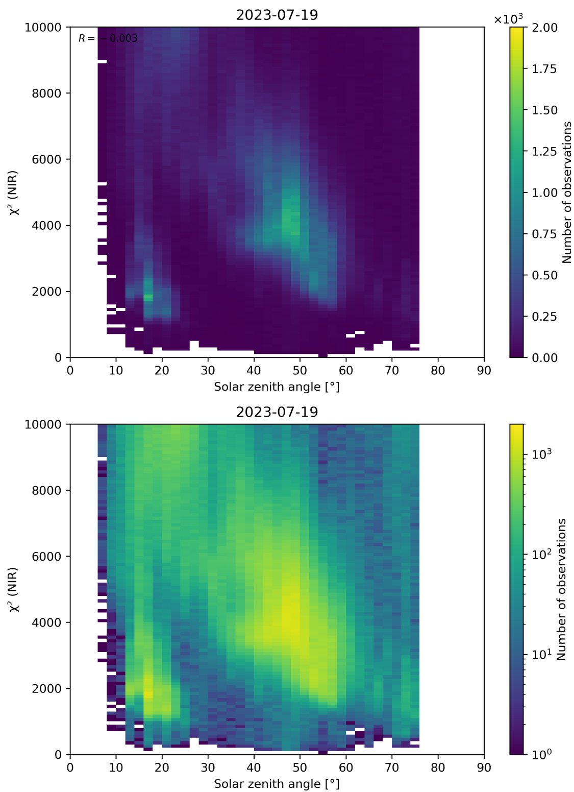
Figure 94: Scatter density plot of “Solar zenith angle” against “ \chi^2 (NIR)” for 2023-07-19 to 2023-07-20.
