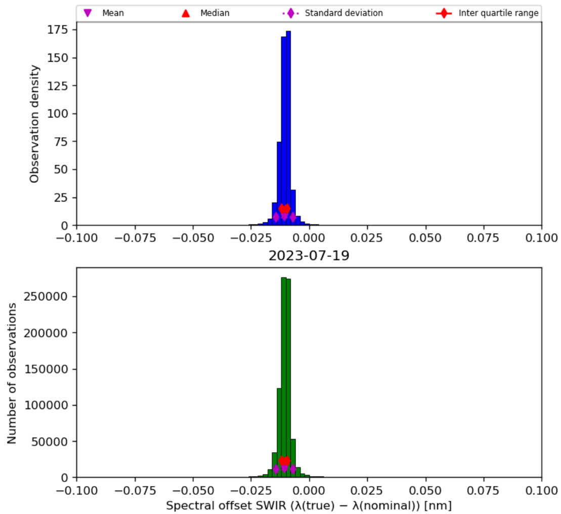
Figure 27: Histogram of “Spectral offset SWIR ( \lambda(\text{true}) - \lambda(\text{nominal}) )” for 2023-07-19 to 2023-07-20
