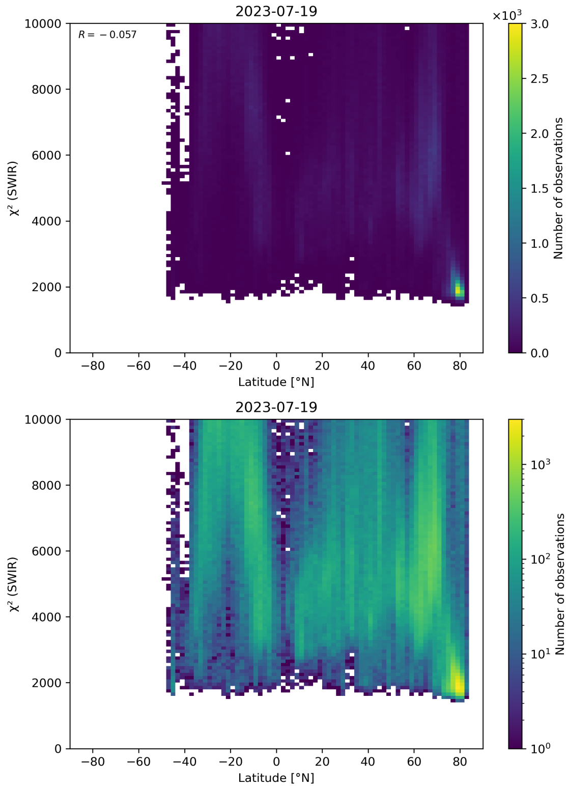
Figure 54: Scatter density plot of “Latitude” against “ \chi^2 (SWIR)” for 2023-07-19 to 2023-07-20.
