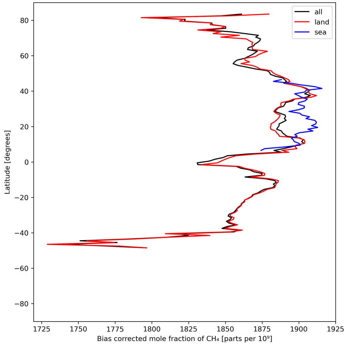
Figure 14: Zonal average of “Bias corrected mole fraction of \text{CH}_4 ” for 2023-07-19 to 2023-07-20.
