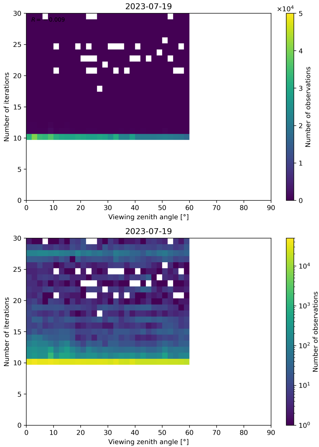
Figure 113: Scatter density plot of “Viewing zenith angle” against “Number of iterations” for 2023-07-19 to 2023-07-20.
