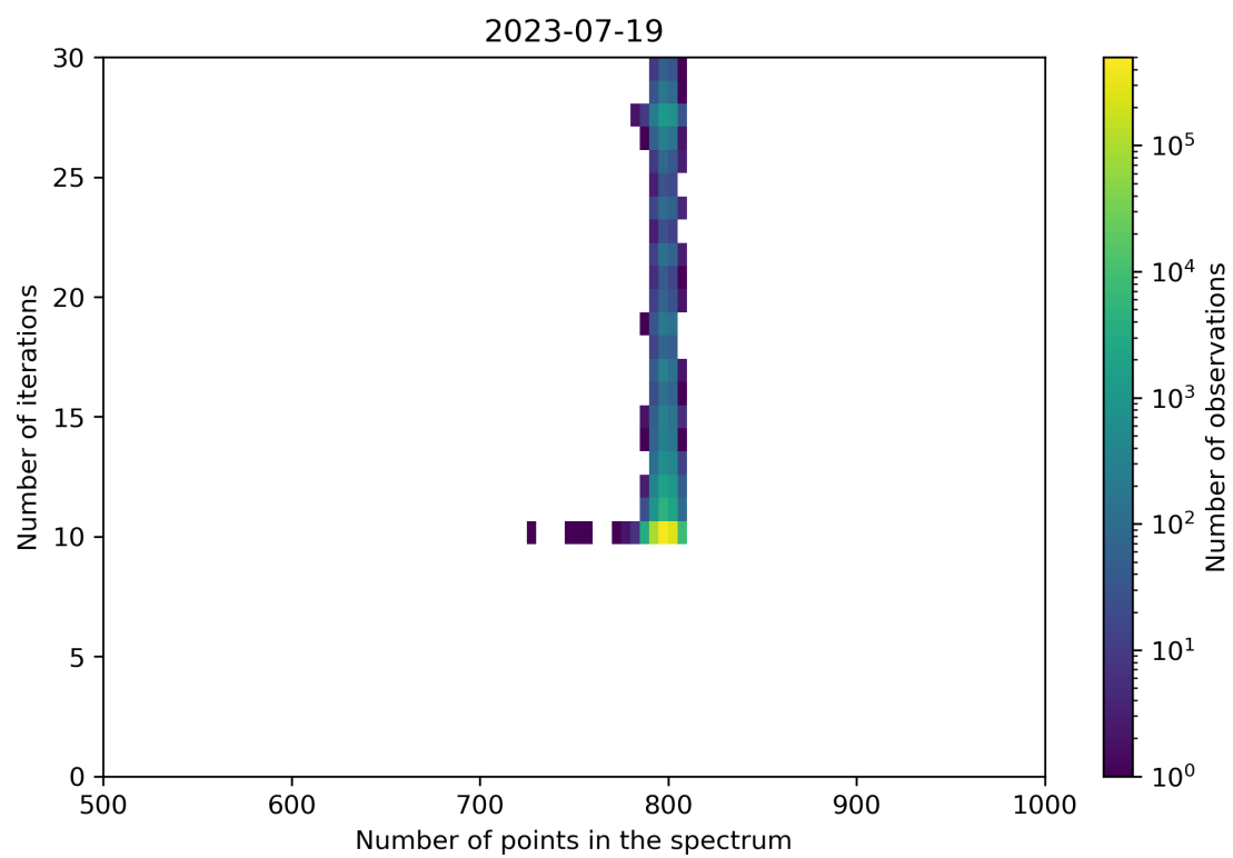
Figure 92: Scatter density plot of “Number of points in the spectrum” against “Number of iterations” for 2023-07-19 to 2023-07-20.
