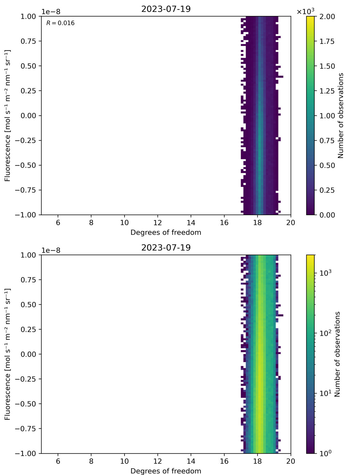
Figure 51: Scatter density plot of “Degrees of freedom” against “Fluorescence” for 2023-07-19 to 2023-07-20.
