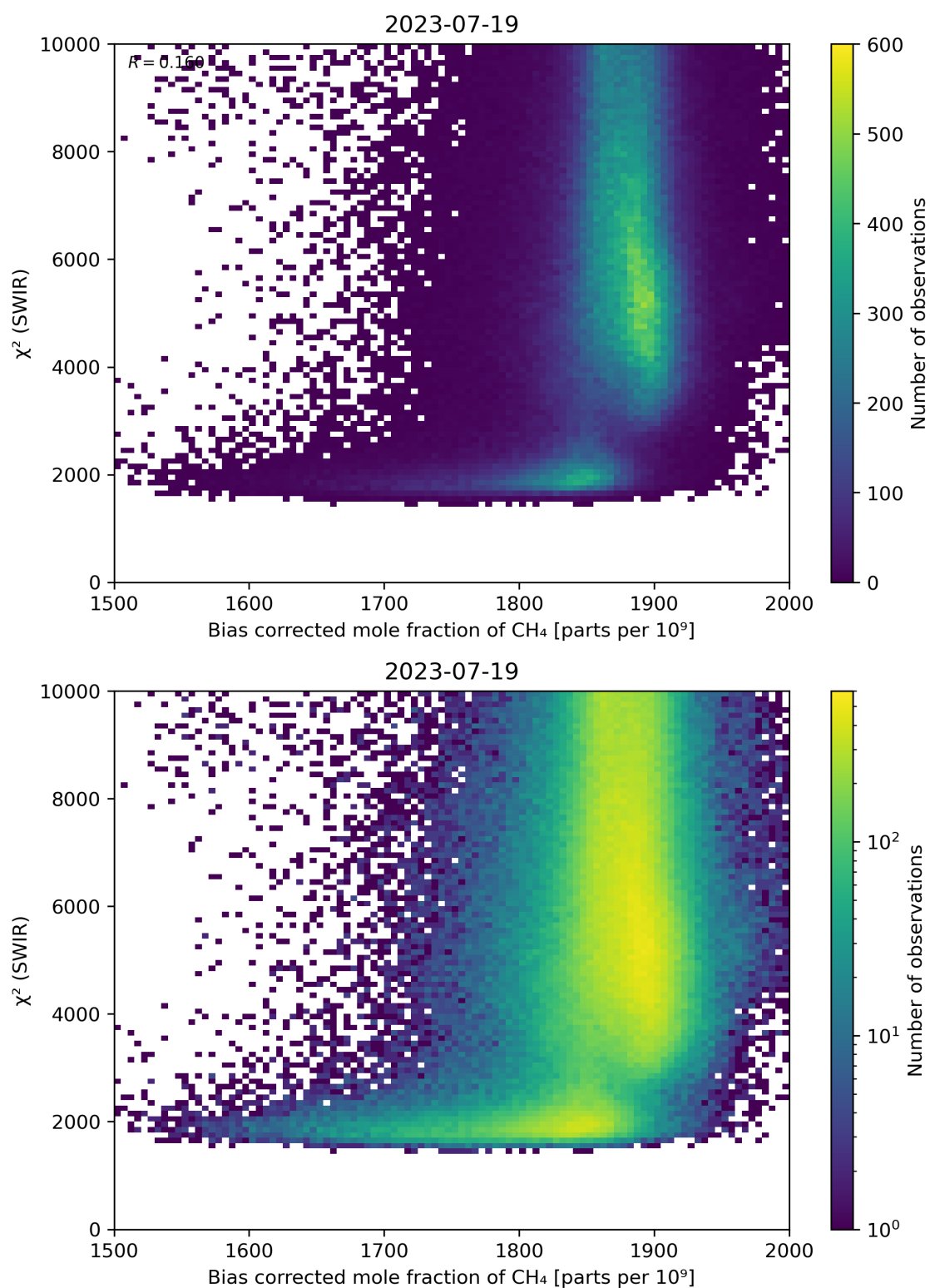
Figure 64: Scatter density plot of “Bias corrected mole fraction of CH 4 ” against “ \chi^2 (SWIR)” for 2023-07-19 to 2023-07-20.
