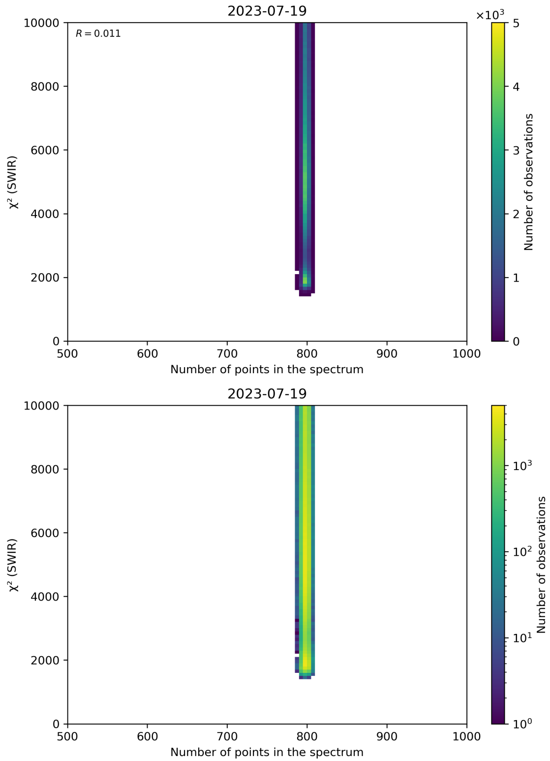
Figure 89: Scatter density plot of “Number of points in the spectrum” against “ \chi^2 (SWIR)” for 2023-07-19 to 2023-07-20.
