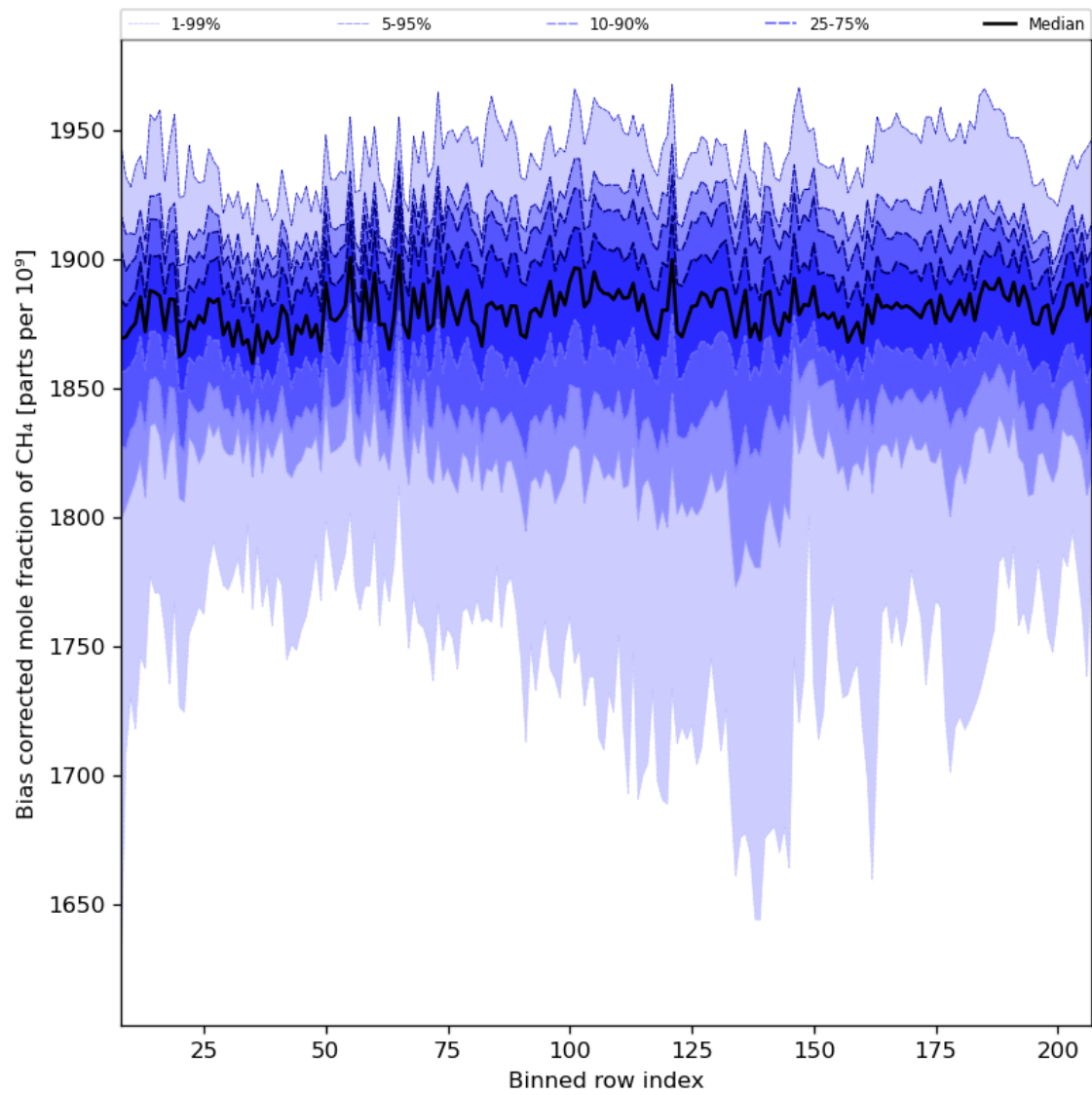
Figure 36: Along track statistics of “Bias corrected mole fraction of CH 4 ” for 2023-07-19 to 2023-07-20
