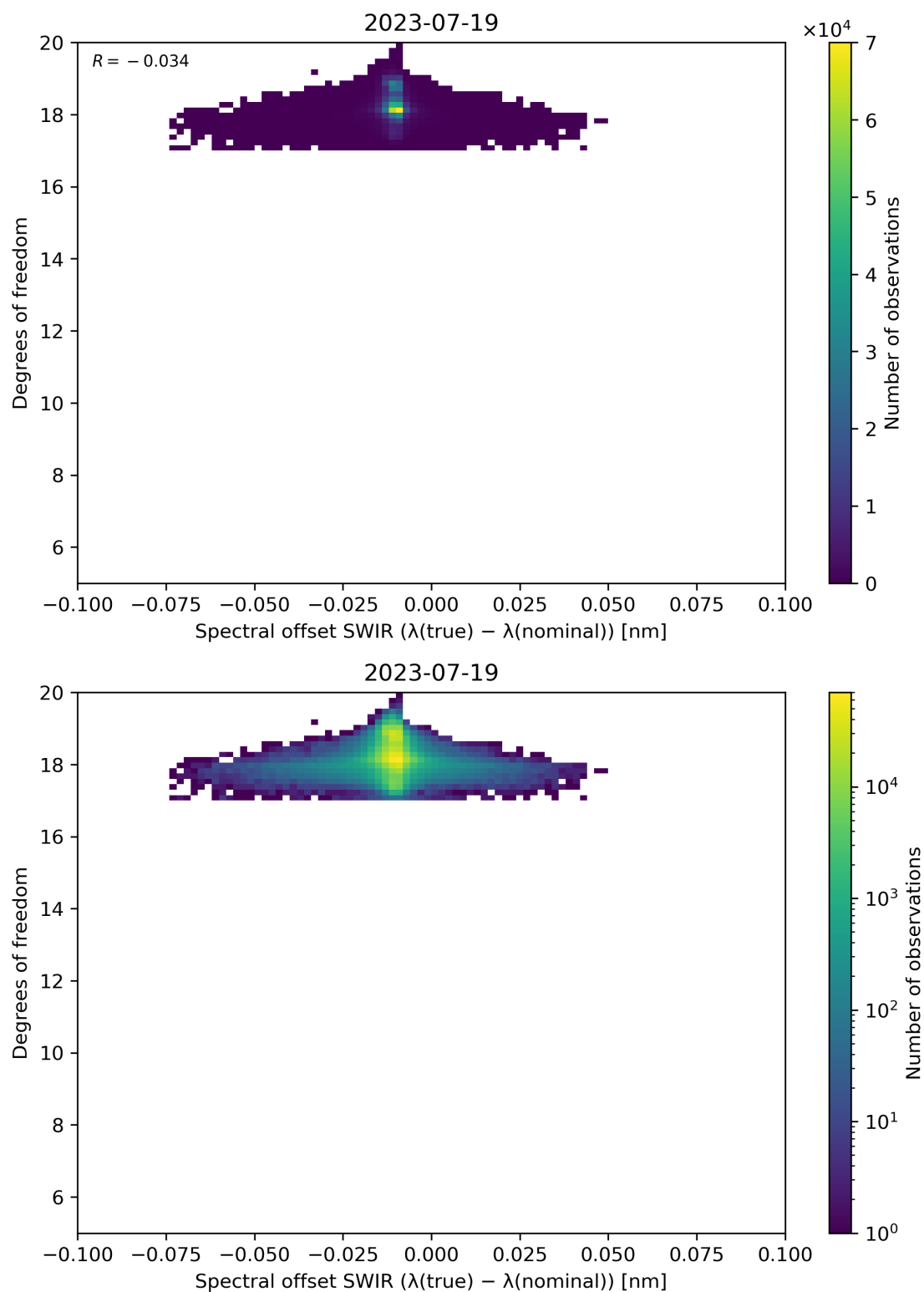
Figure 119: Scatter density plot of “Spectral offset SWIR ( \lambda(\text{true}) - \lambda(\text{nominal}) )” against “Degrees of freedom” for 2023-07-19 to 2023-07-20.
