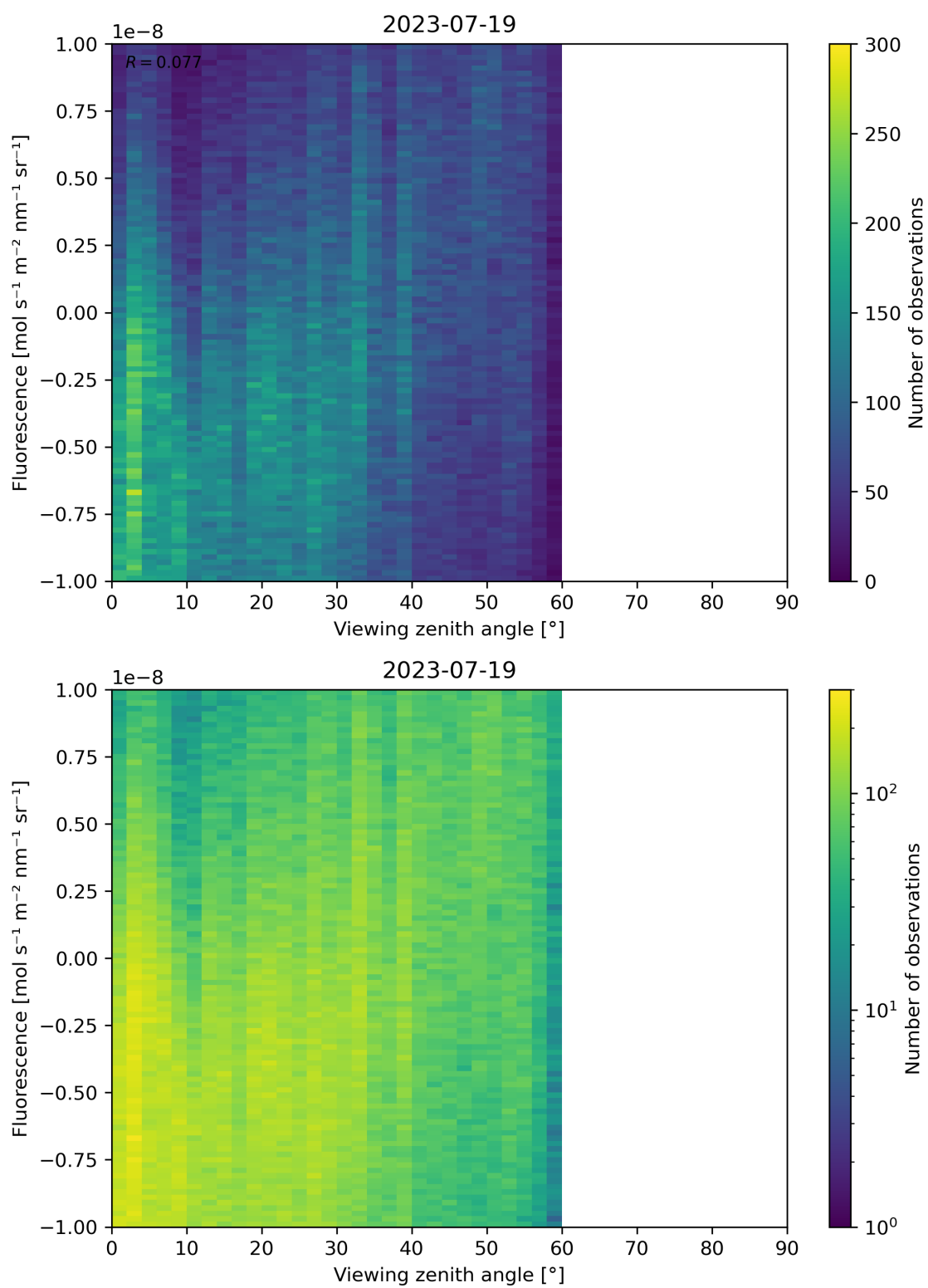
Figure 108: Scatter density plot of “Viewing zenith angle” against “Fluorescence” for 2023-07-19 to 2023-07-20.
