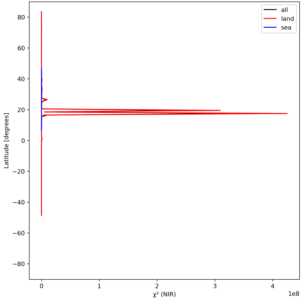
Figure 18: Zonal average of “ \chi^2 (NIR)” for 2023-07-19 to 2023-07-20.
