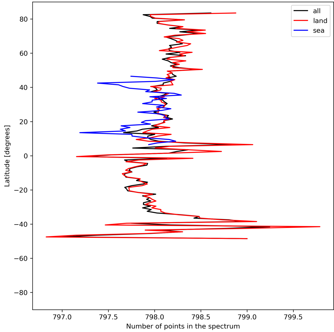
Figure 15: Zonal average of “Number of points in the spectrum” for 2023-07-19 to 2023-07-20.
