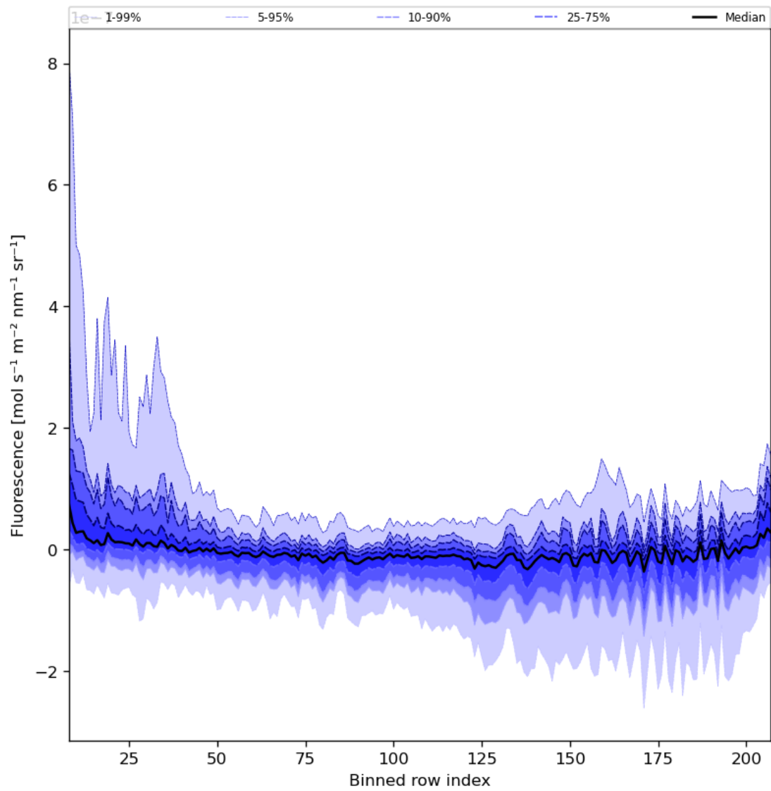
Figure 43: Along track statistics of “Fluorescence” for 2023-07-19 to 2023-07-20
