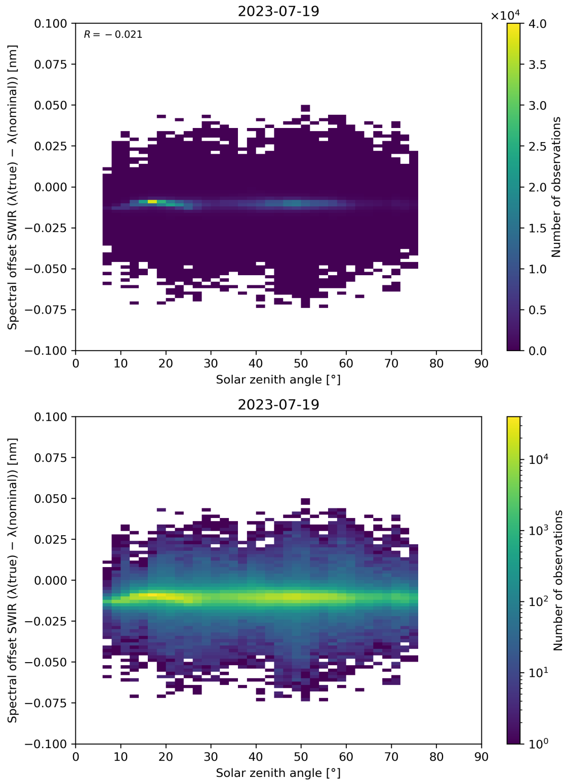
Figure 104: Scatter density plot of “Solar zenith angle” against “Spectral offset SWIR ( \lambda(\text{true}) - \lambda(\text{nominal}) )” for 2023-07-19 to 2023-07-20.
