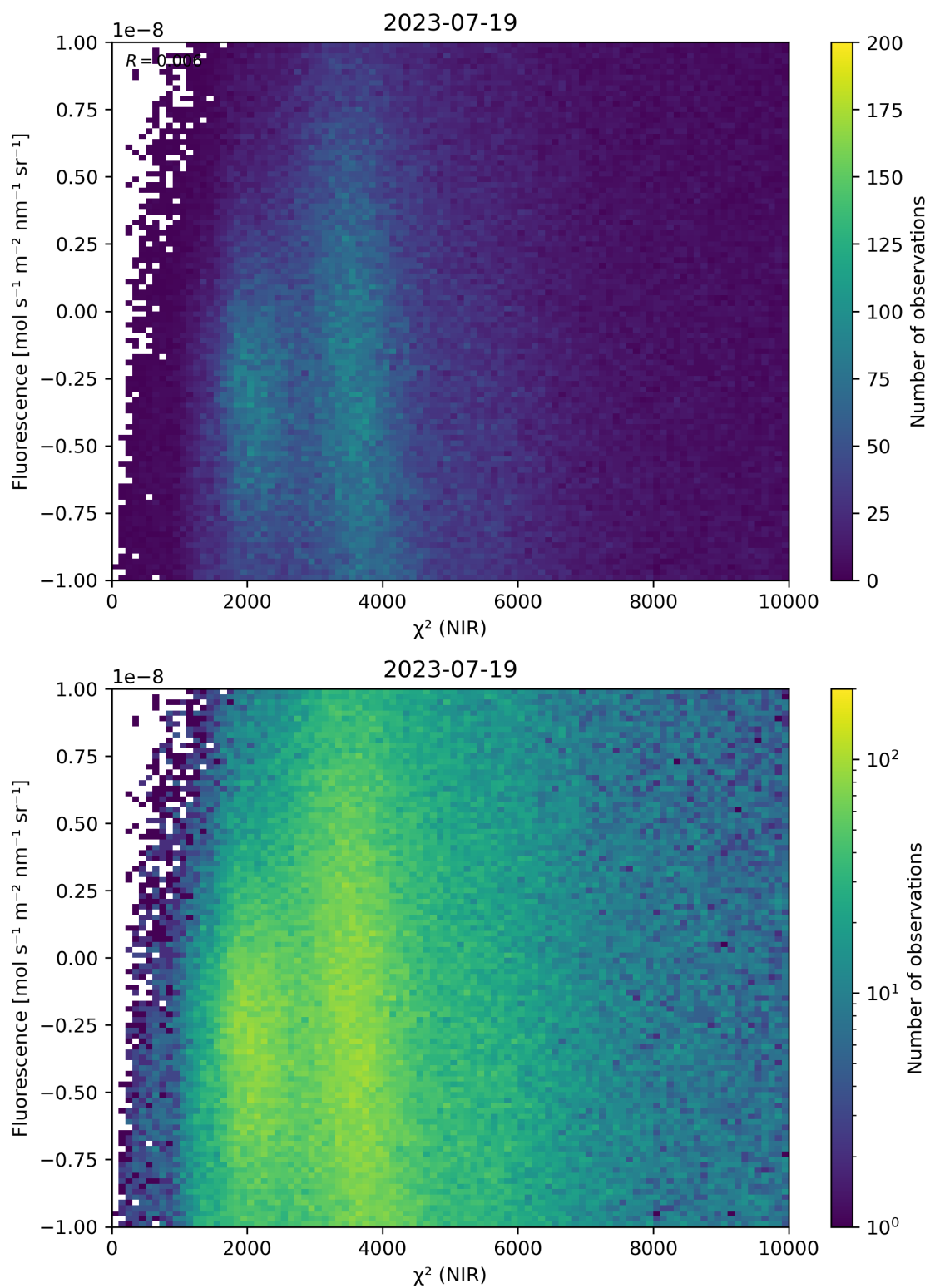
Figure 45: Scatter density plot of “ \chi^2 (NIR)” against “Fluorescence” for 2023-07-19 to 2023-07-20.
