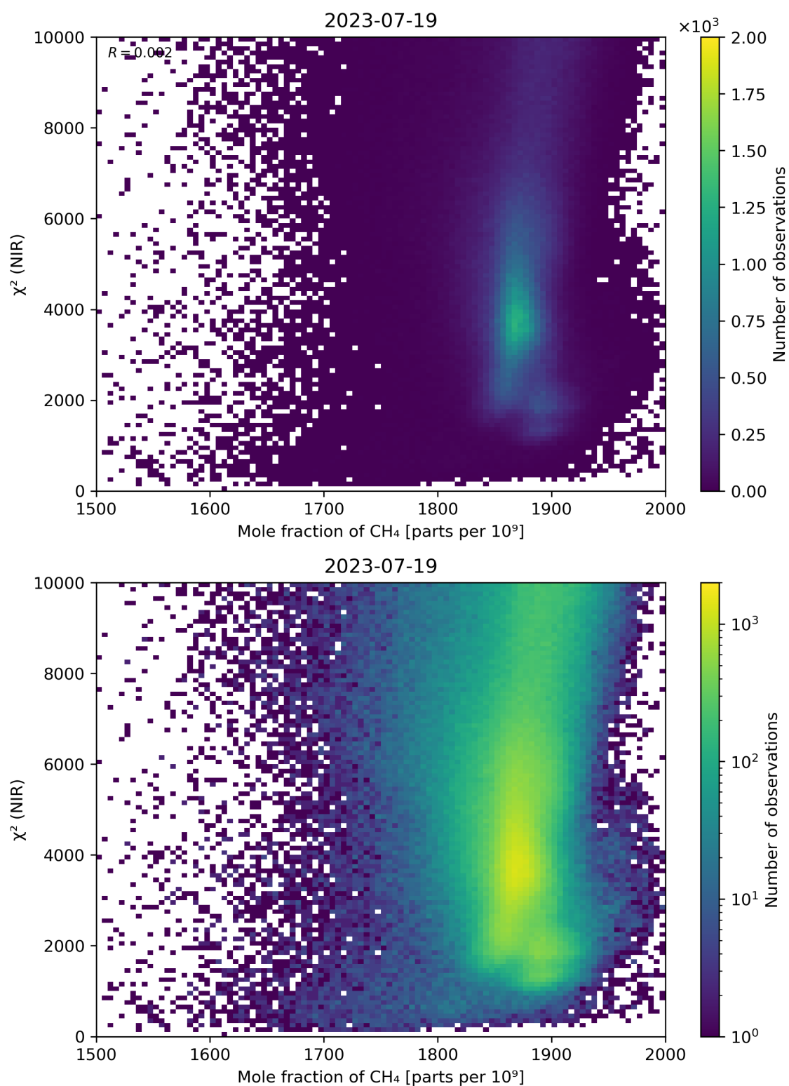
Figure 70: Scatter density plot of “Mole fraction of \text{CH}_4 ” against “ \chi^2 (NIR)” for 2023-07-19 to 2023-07-20.
