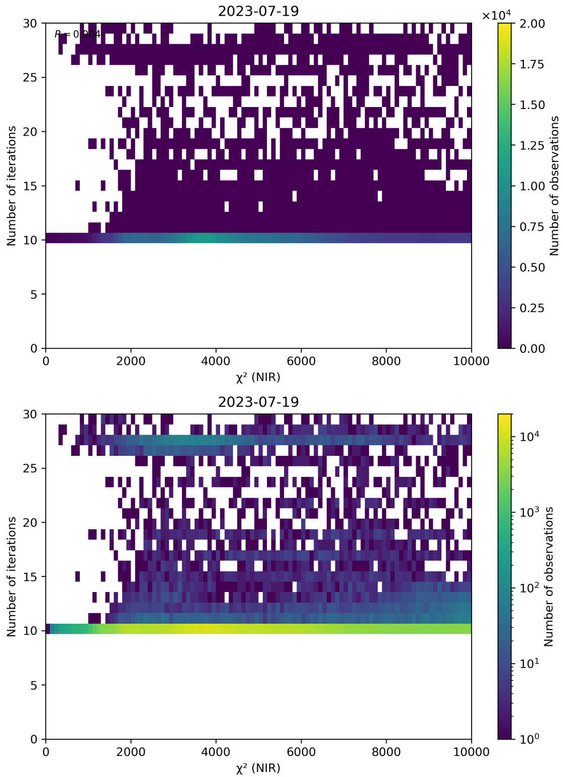
Figure 46: Scatter density plot of “ \chi^2 (NIR)” against “Number of iterations” for 2023-07-19 to 2023-07-20.
