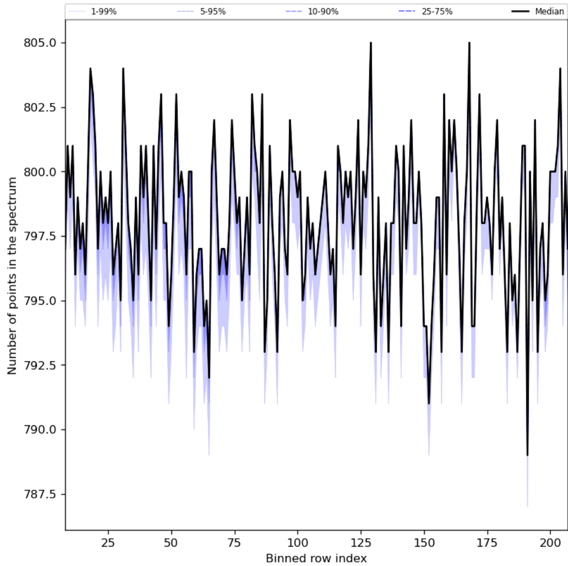
Figure 37: Along track statistics of “Number of points in the spectrum” for 2023-07-19 to 2023-07-20
