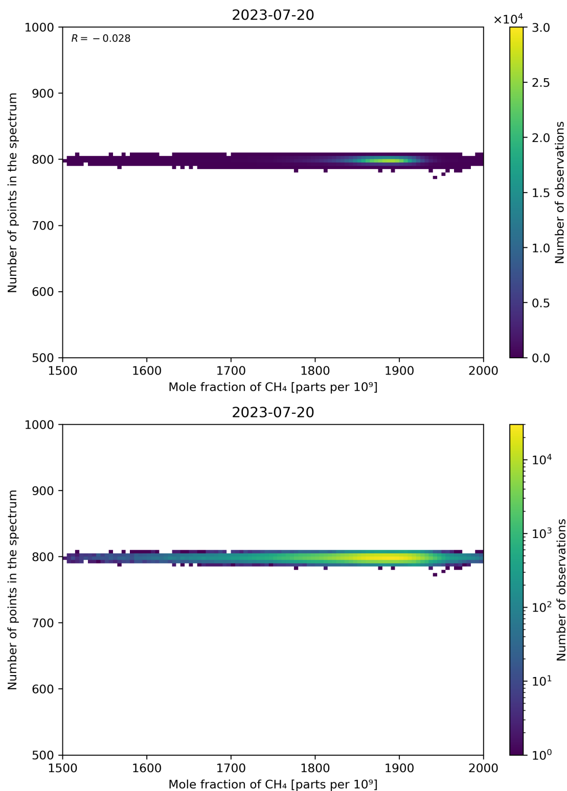
Figure 77: Scatter density plot of “Mole fraction of CH 4 ” against “Number of points in the spectrum” for 2023-07-19 to 2023-07-21.
