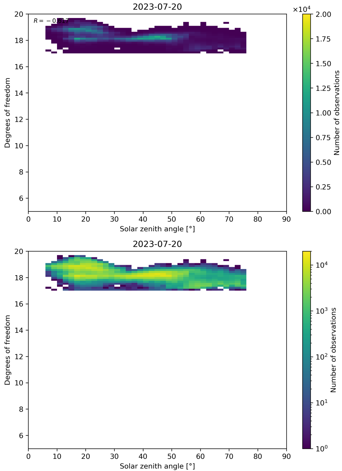
Figure 96: Scatter density plot of “Solar zenith angle” against “Degrees of freedom” for 2023-07-19 to 2023-07-21.
