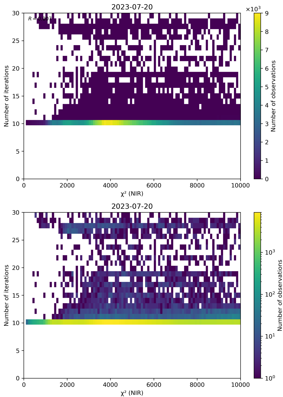
Figure 46: Scatter density plot of “ \chi^2 (NIR)” against “Number of iterations” for 2023-07-19 to 2023-07-21.
