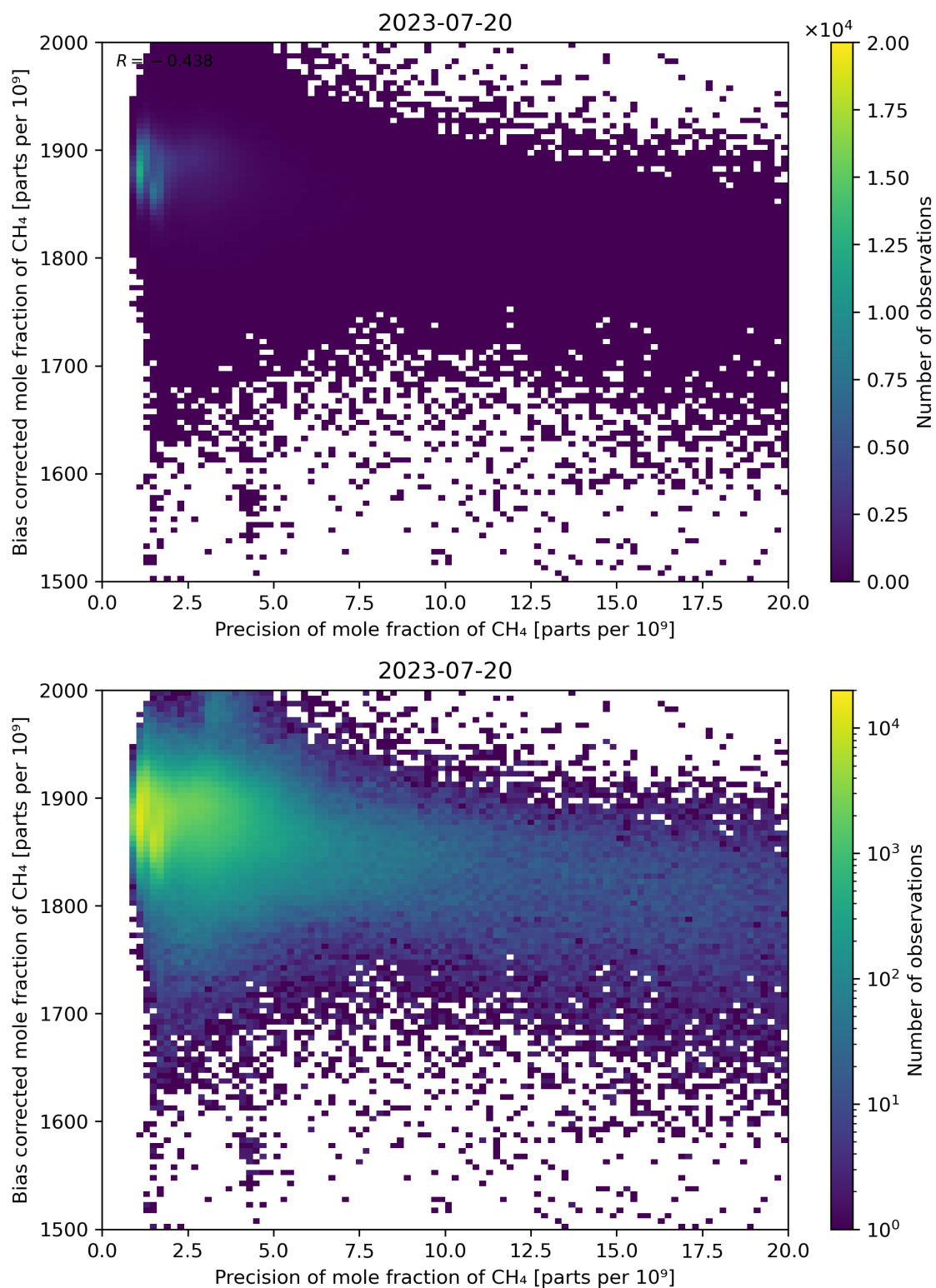
Figure 82: Scatter density plot of “Precision of mole fraction of CH 4 ” against “Bias corrected mole fraction of CH 4 ” for 2023-07-19 to 2023-07-21.
