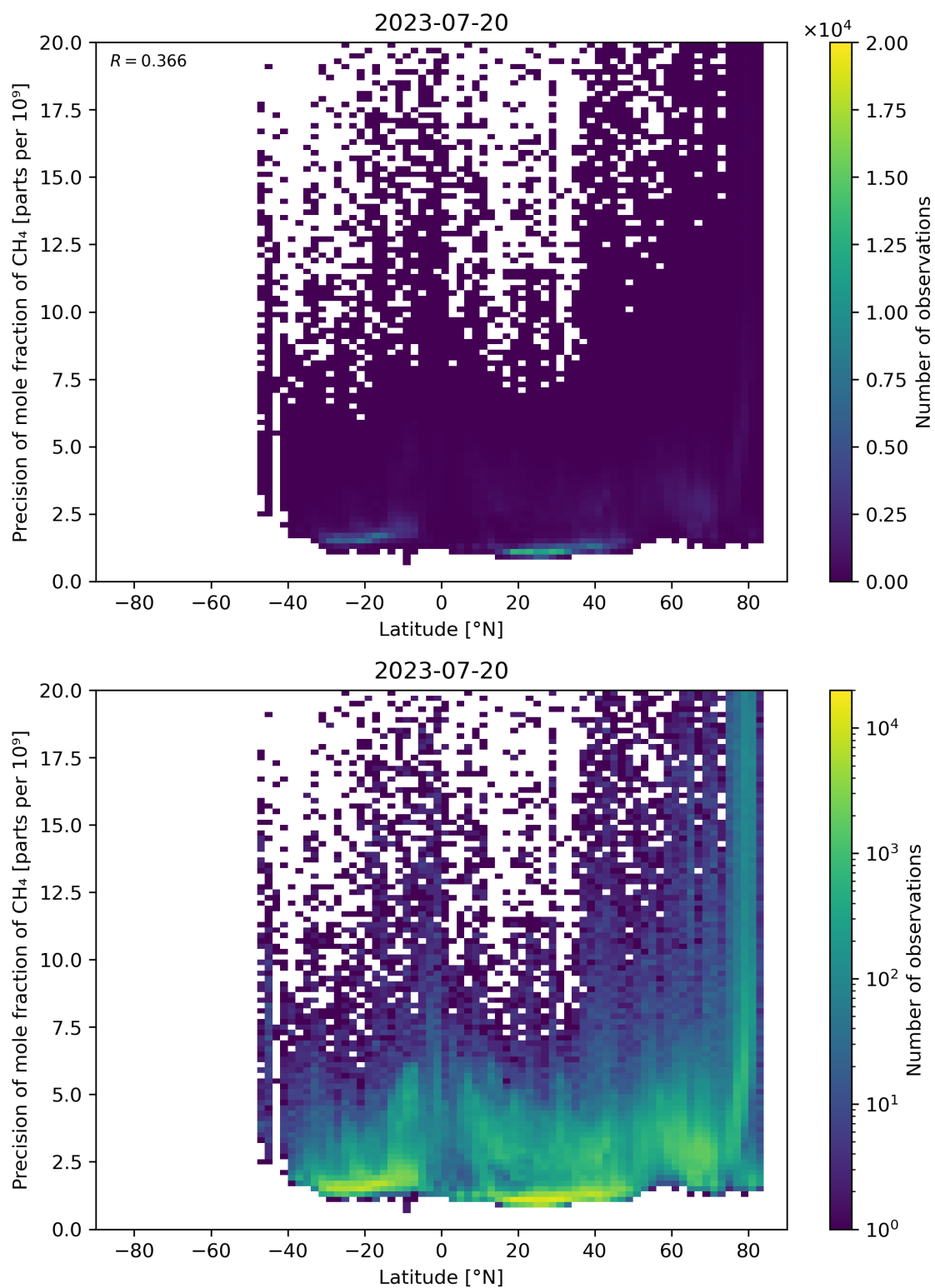
Figure 59: Scatter density plot of “Latitude” against “Precision of mole fraction of \text{CH}_4 ” for 2023-07-19 to 2023-07-21.
