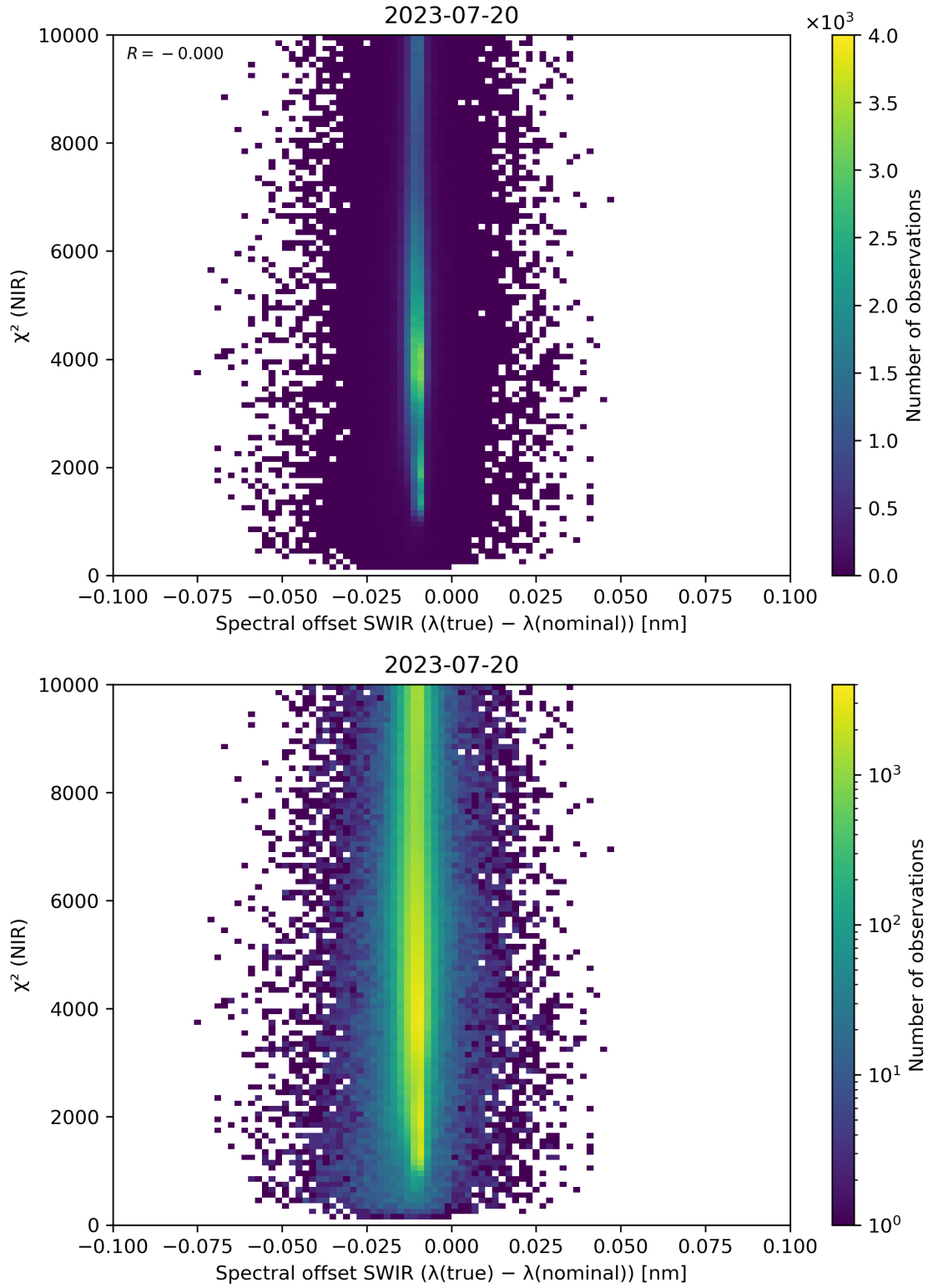
Figure 117: Scatter density plot of “Spectral offset SWIR ( \lambda(\text{true}) - \lambda(\text{nominal}) )” against “ \chi^2 (NIR)” for 2023-07-19 to 2023-07-21.
