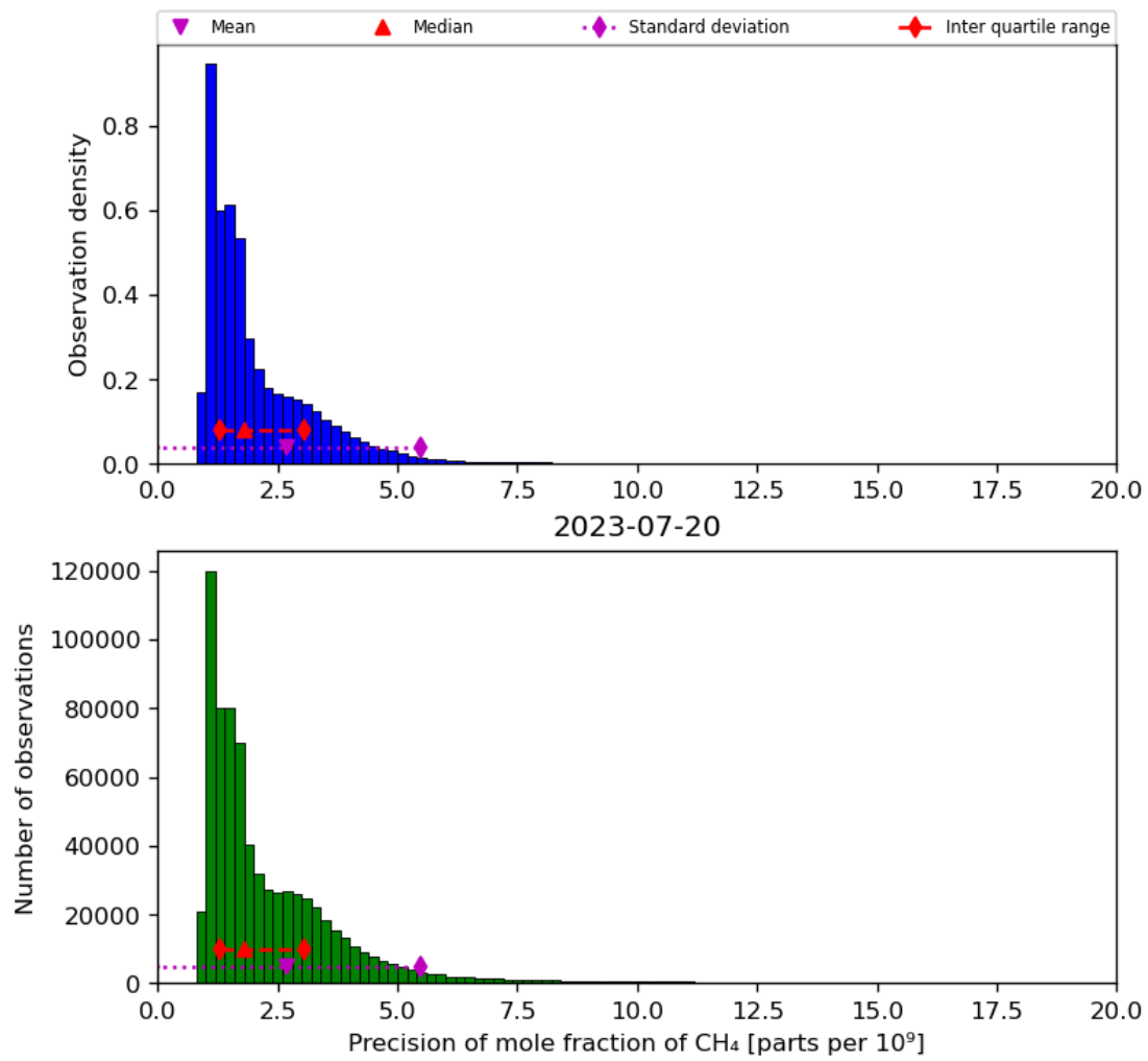
Figure 24: Histogram of “Precision of mole fraction of CH 4 ” for 2023-07-19 to 2023-07-21
