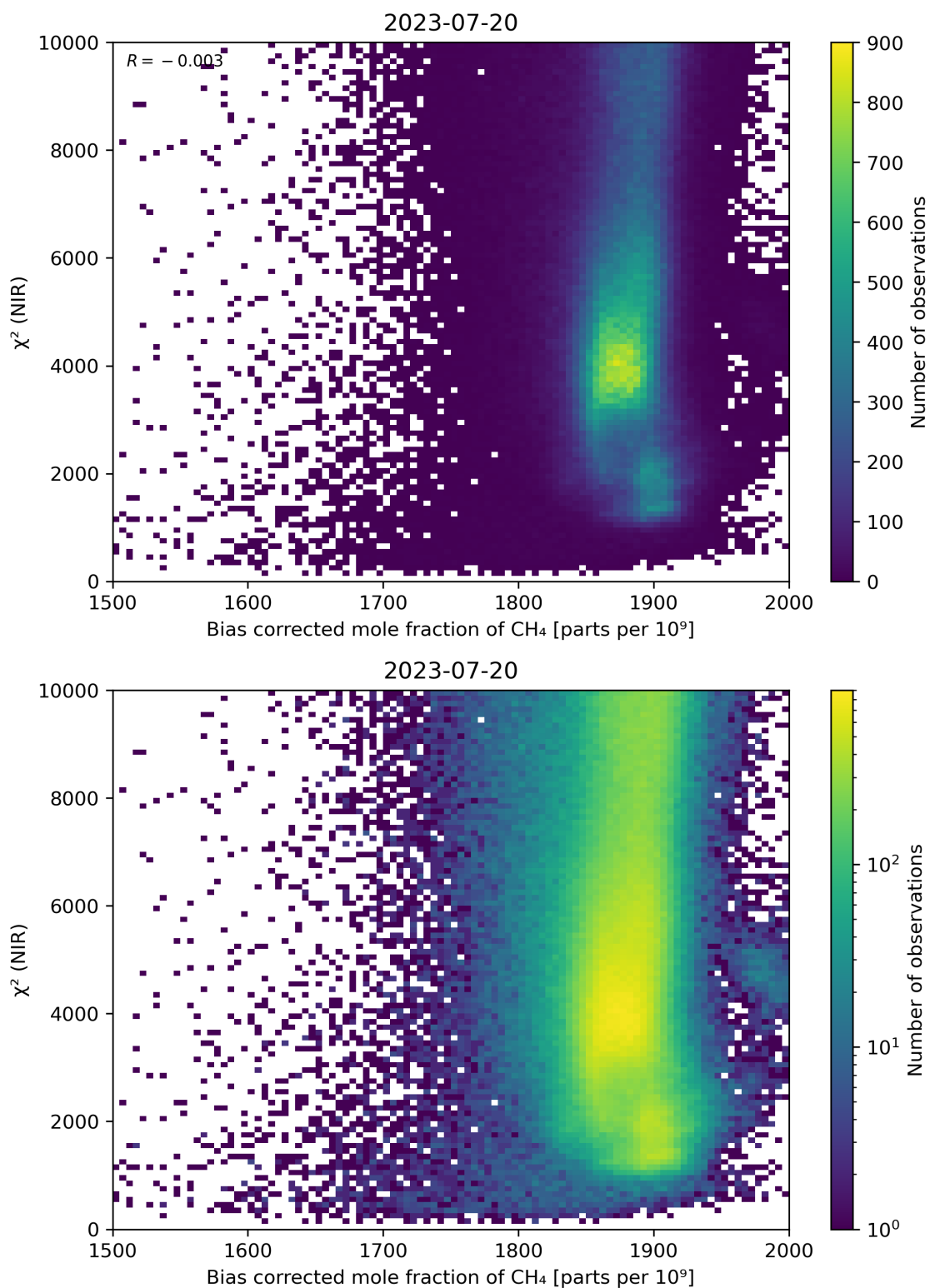
Figure 63: Scatter density plot of “Bias corrected mole fraction of CH 4 ” against “ \chi^2 (NIR)” for 2023-07-19 to 2023-07-21.
