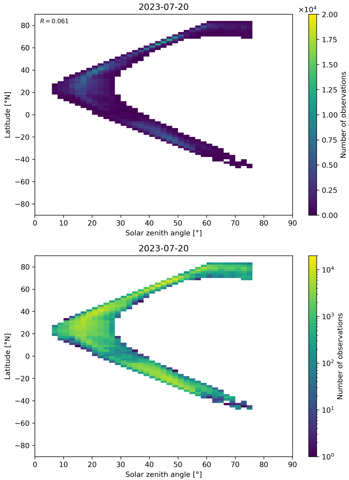
Figure 98: Scatter density plot of “Solar zenith angle” against “Latitude” for 2023-07-19 to 2023-07-21.
