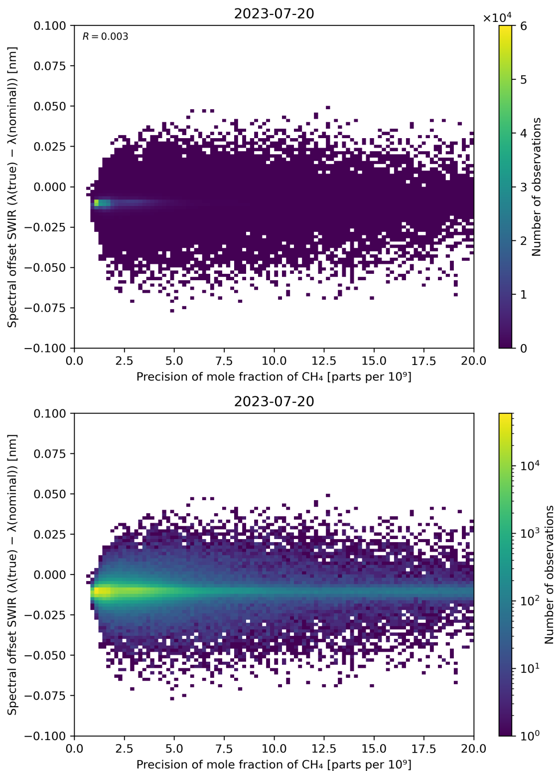
Figure 85: Scatter density plot of “Precision of mole fraction of CH 4 ” against “Spectral offset SWIR ( \lambda(\text{true}) - \lambda(\text{nominal}) )” for 2023-07-19 to 2023-07-21.
