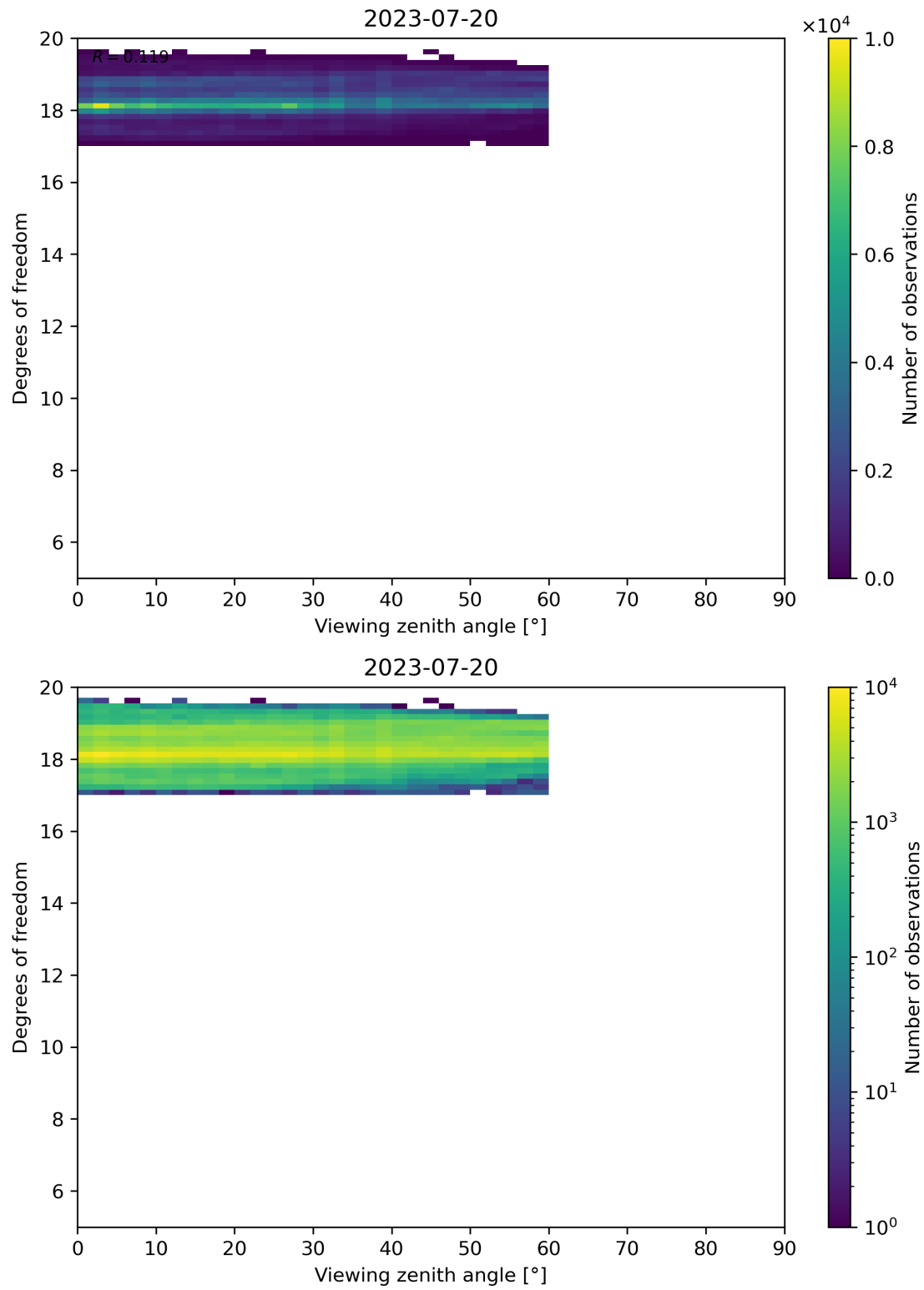
Figure 107: Scatter density plot of “Viewing zenith angle” against “Degrees of freedom” for 2023-07-19 to 2023-07-21.
