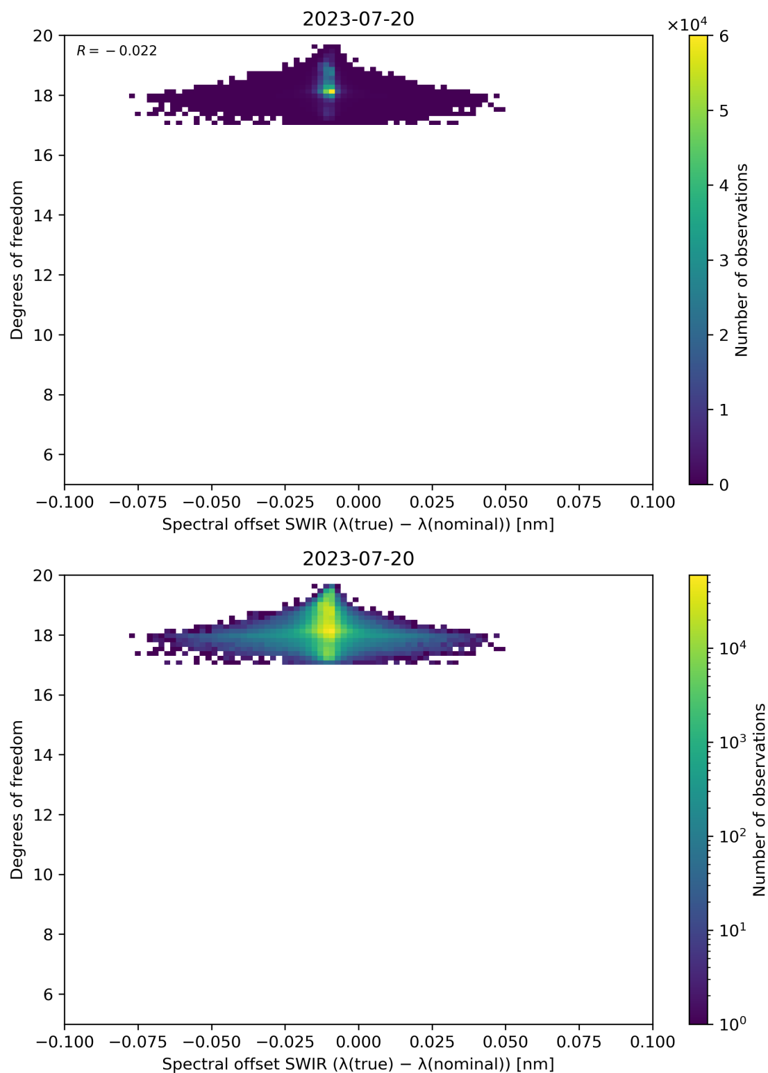
Figure 119: Scatter density plot of “Spectral offset SWIR ( \lambda(\text{true}) - \lambda(\text{nominal}) )” against “Degrees of freedom” for 2023-07-19 to 2023-07-21.
