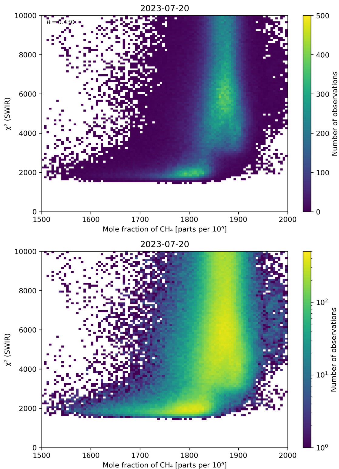
Figure 71: Scatter density plot of “Mole fraction of \text{CH}_4 ” against “ \chi^2 (SWIR)” for 2023-07-19 to 2023-07-21.
