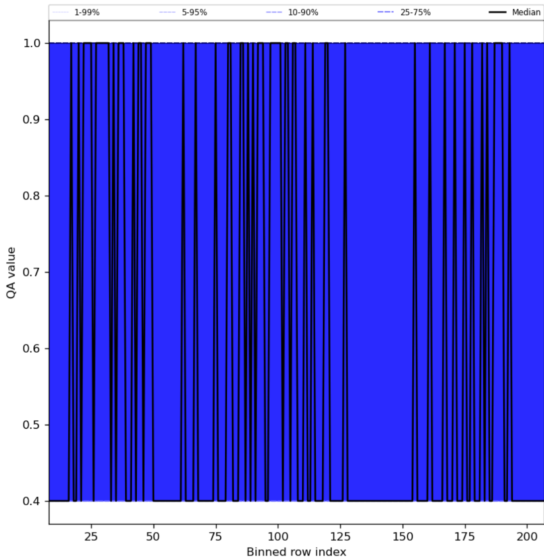
Figure 33: Along track statistics of “QA value” for 2023-07-19 to 2023-07-21
