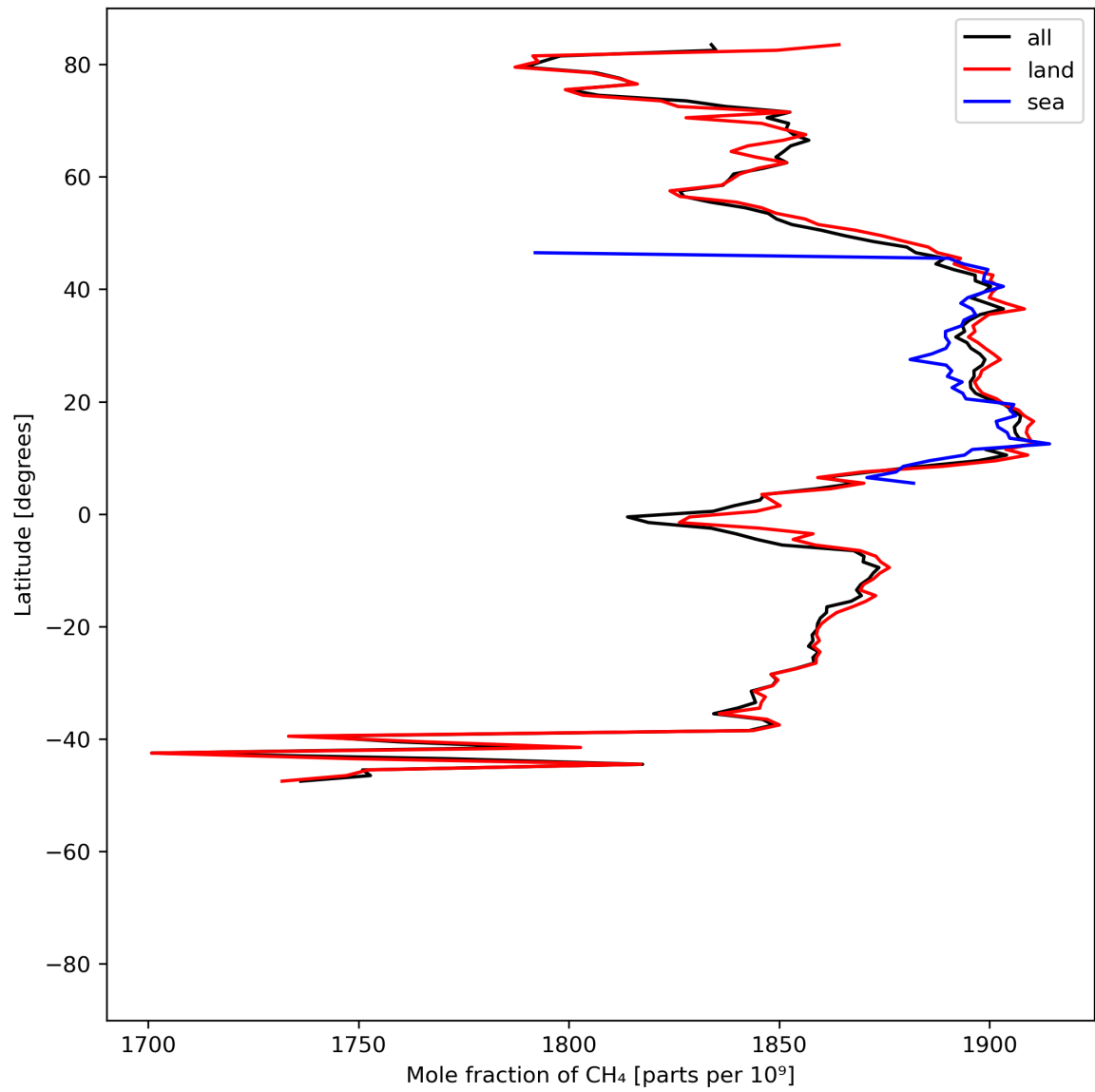
Figure 12: Zonal average of “Mole fraction of \text{CH}_4 ” for 2023-07-19 to 2023-07-21.
