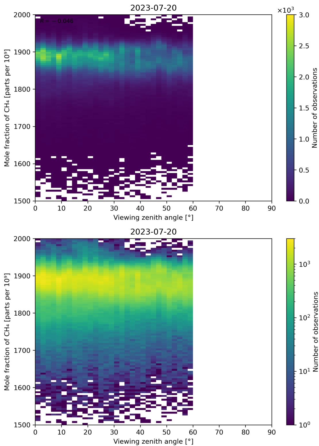
Figure 110: Scatter density plot of “Viewing zenith angle” against “Mole fraction of CH 4 ” for 2023-07-19 to 2023-07-21.
