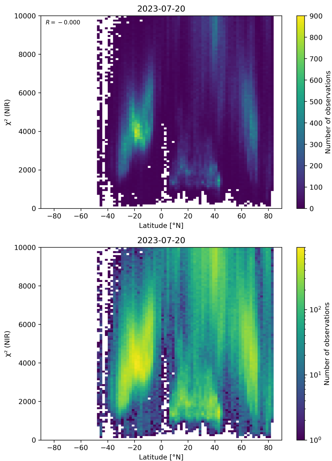
Figure 53: Scatter density plot of “Latitude” against “ \chi^2 (NIR)” for 2023-07-19 to 2023-07-21.
