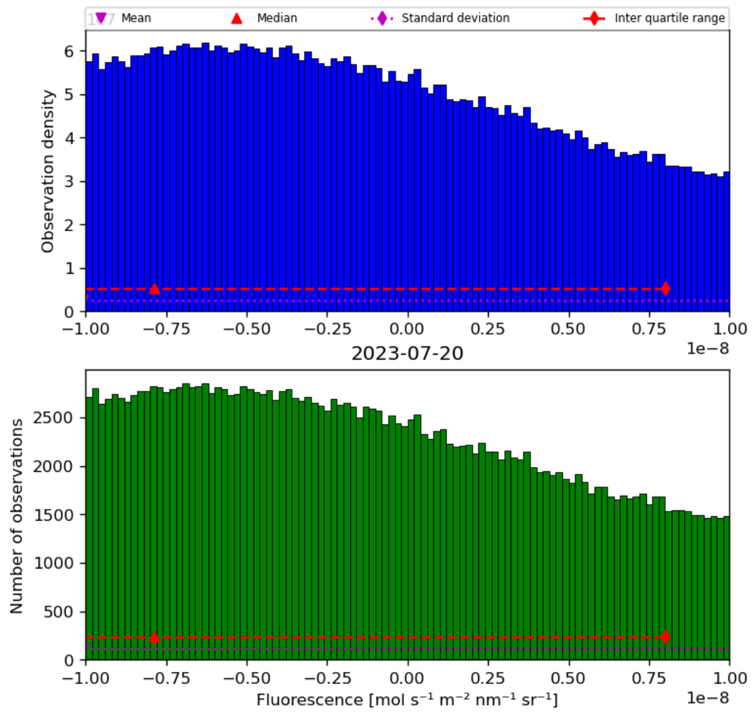
Figure 32: Histogram of “Fluorescence” for 2023-07-19 to 2023-07-21
