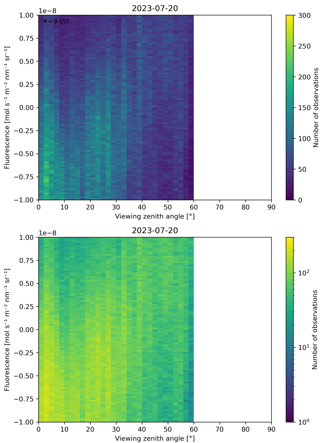
Figure 108: Scatter density plot of “Viewing zenith angle” against “Fluorescence” for 2023-07-19 to 2023-07-21.
