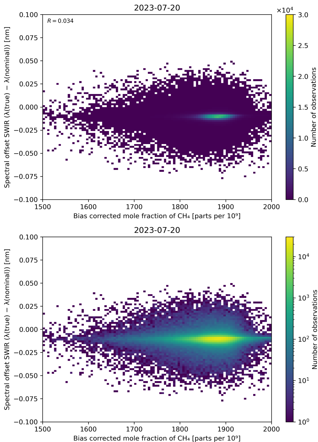
Figure 69: Scatter density plot of “Bias corrected mole fraction of \text{CH}_4 ” against “Spectral offset SWIR ( \lambda(\text{true}) - \lambda(\text{nominal}) )” for 2023-07-19 to 2023-07-21.
