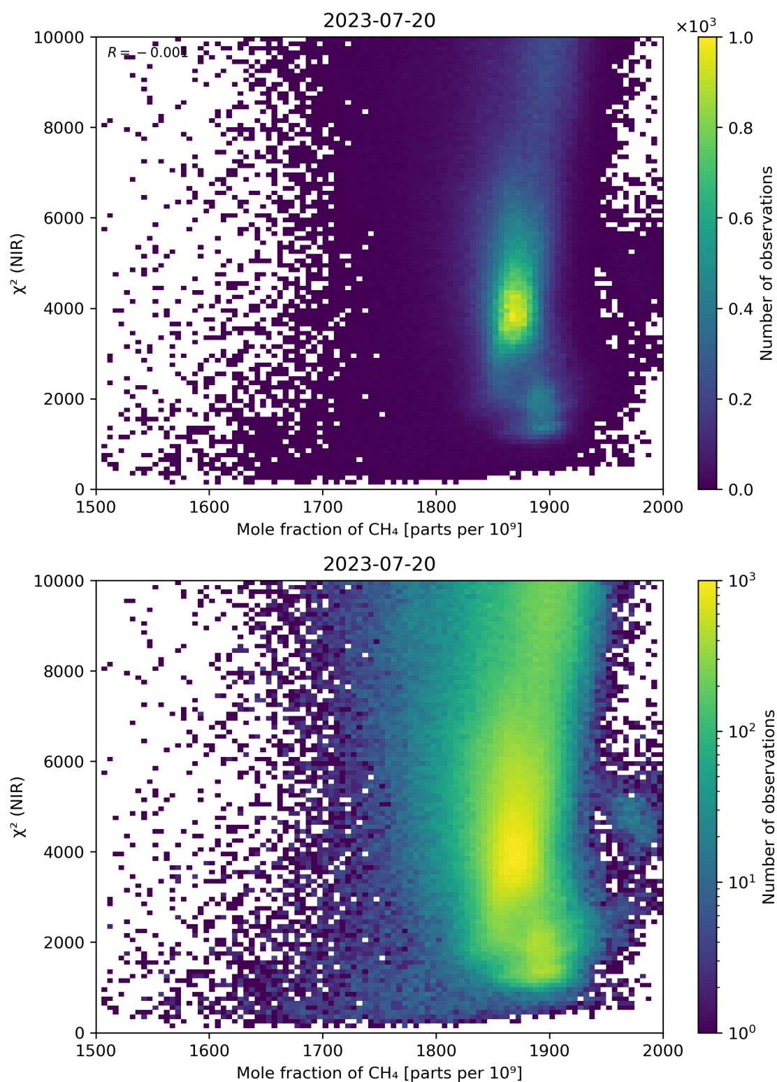
Figure 70: Scatter density plot of “Mole fraction of \text{CH}_4 ” against “ \chi^2 (NIR)” for 2023-07-19 to 2023-07-21.
