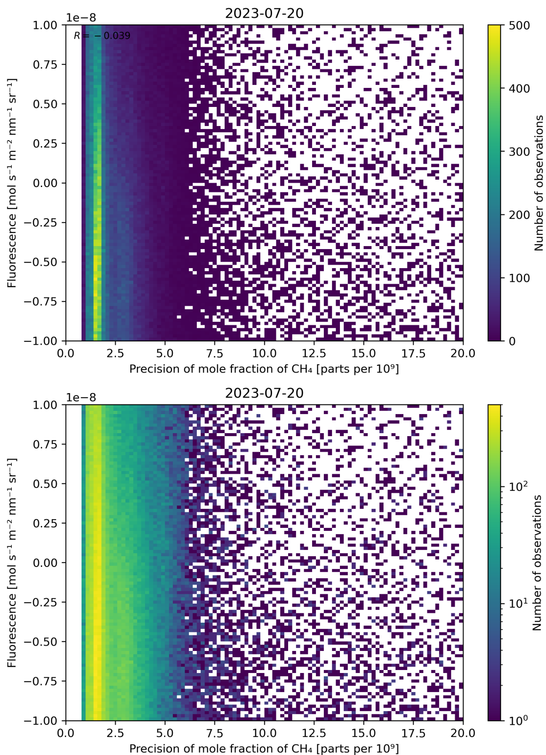
Figure 81: Scatter density plot of “Precision of mole fraction of \text{CH}_4 ” against “Fluorescence” for 2023-07-19 to 2023-07-21.
