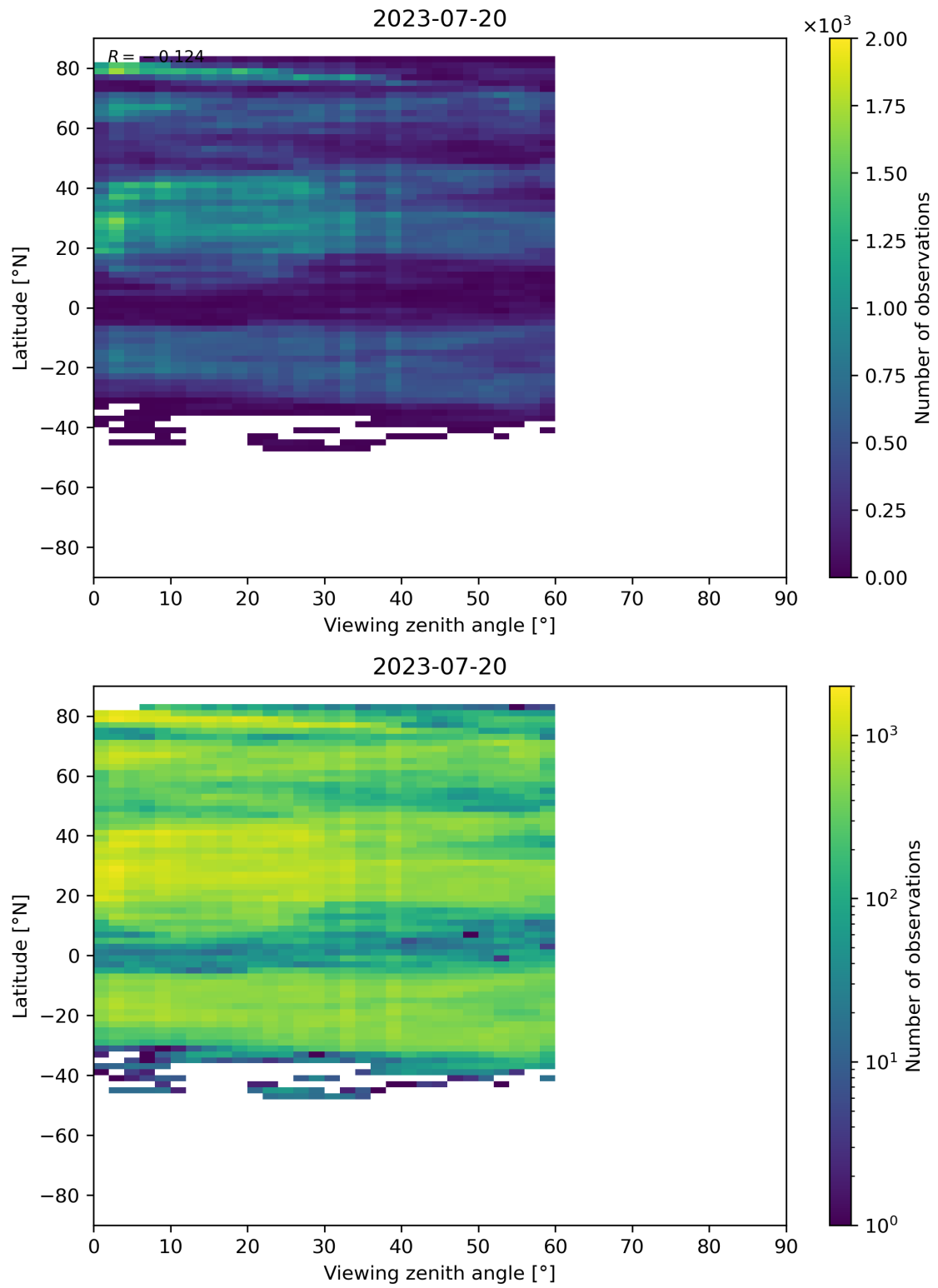
Figure 109: Scatter density plot of “Viewing zenith angle” against “Latitude” for 2023-07-19 to 2023-07-21.
