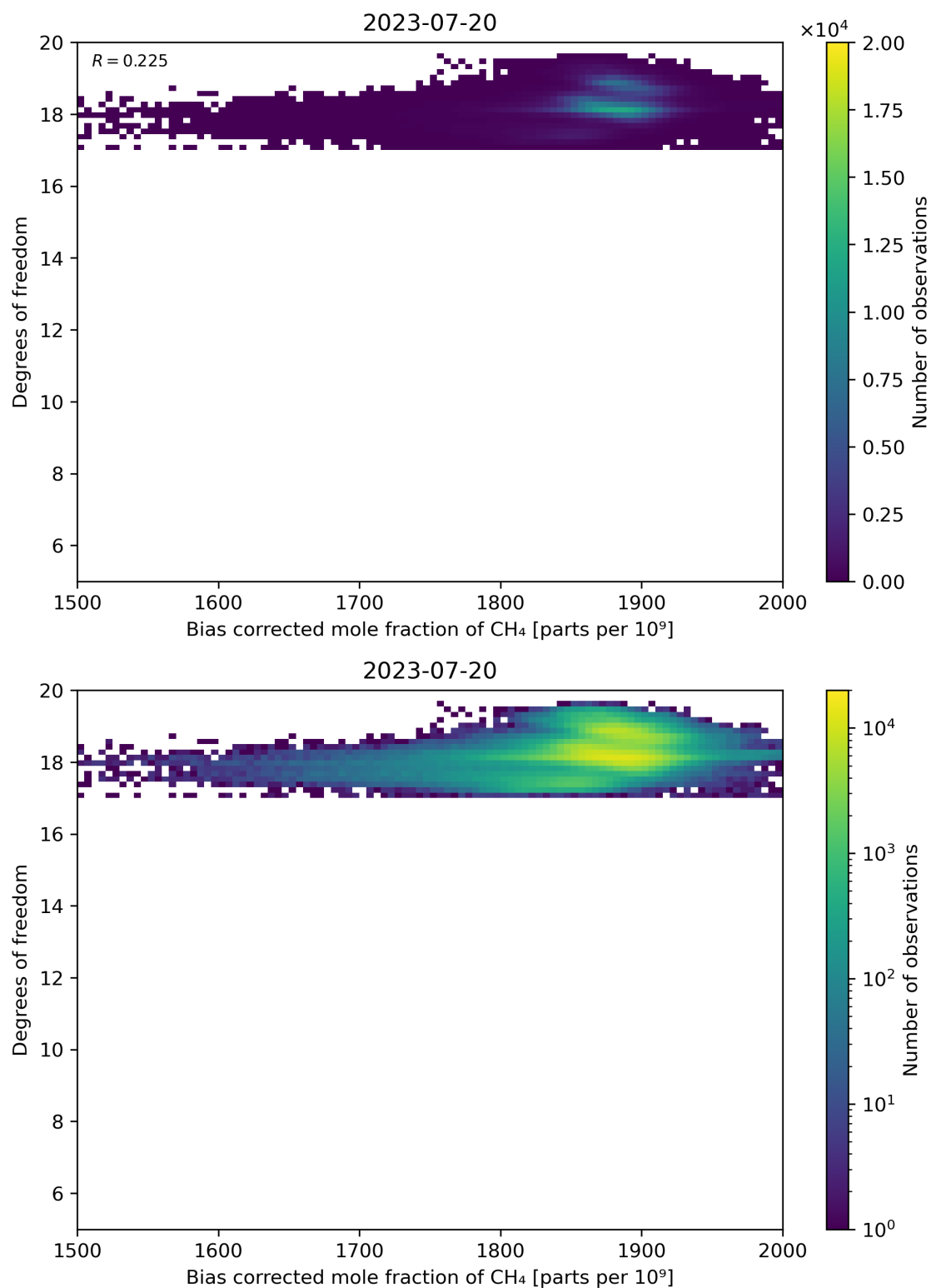
Figure 65: Scatter density plot of “Bias corrected mole fraction of CH 4 ” against “Degrees of freedom” for 2023-07-19 to 2023-07-21.
