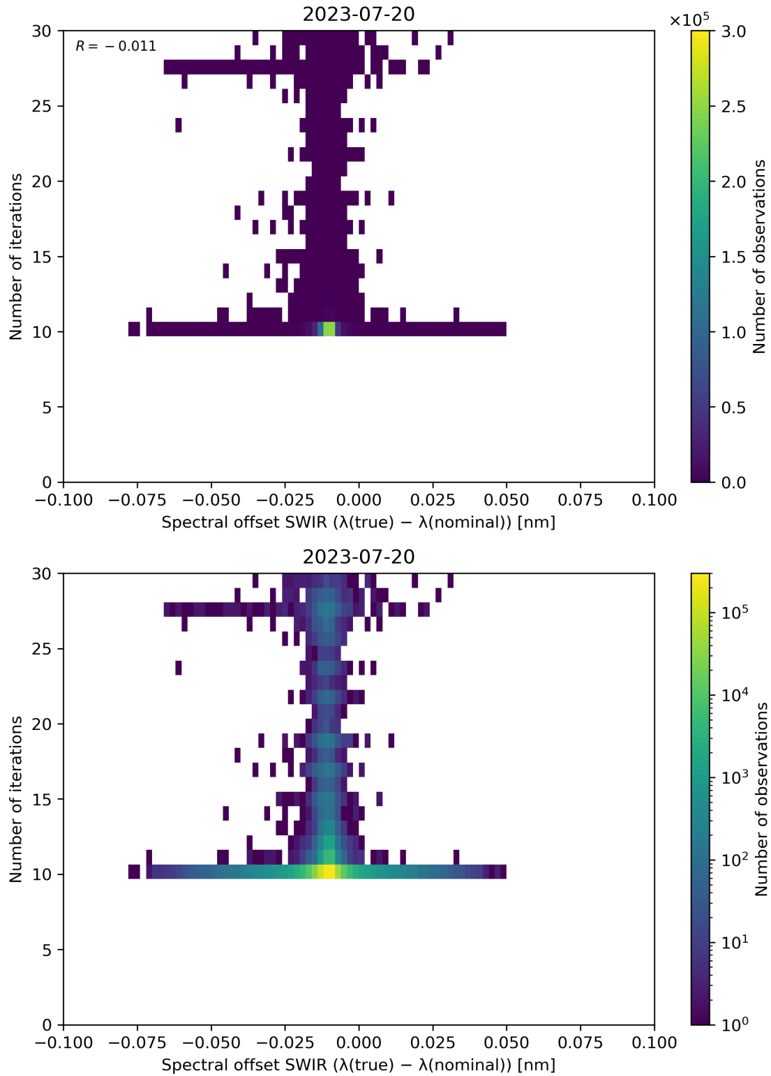
Figure 121: Scatter density plot of “Spectral offset SWIR ( \lambda(\text{true}) - \lambda(\text{nominal}) )” against “Number of iterations” for 2023-07-19 to 2023-07-21.
