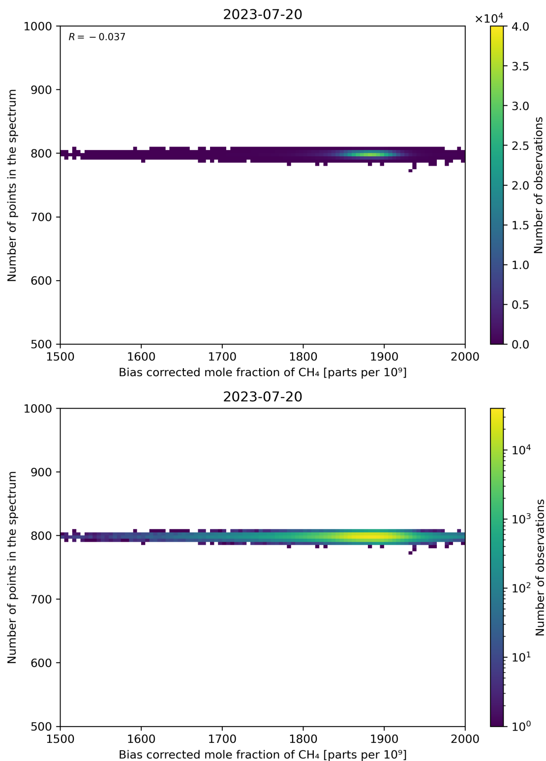
Figure 68: Scatter density plot of “Bias corrected mole fraction of CH 4 ” against “Number of points in the spectrum” for 2023-07-19 to 2023-07-21.
