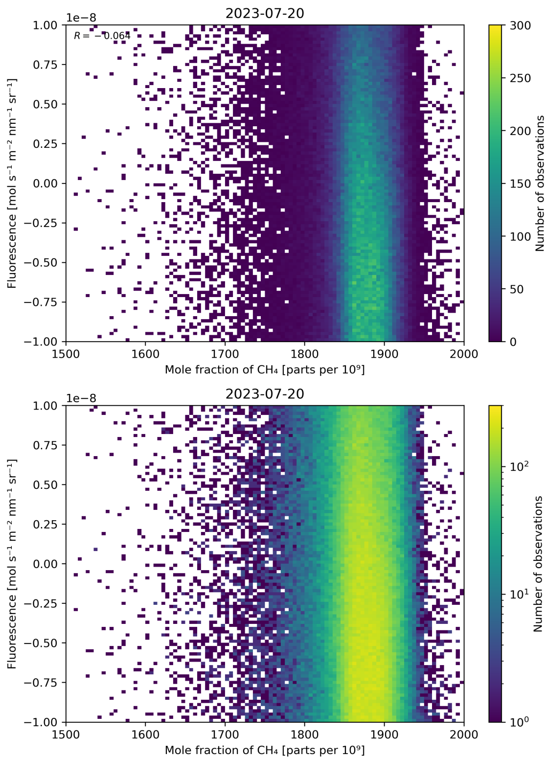
Figure 73: Scatter density plot of “Mole fraction of \text{CH}_4 ” against “Fluorescence” for 2023-07-19 to 2023-07-21.
