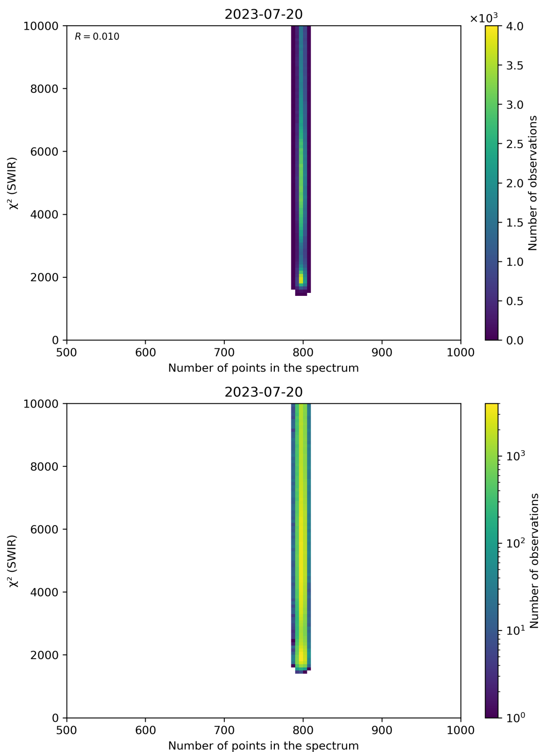
Figure 89: Scatter density plot of “Number of points in the spectrum” against “ \chi^2 (SWIR)” for 2023-07-19 to 2023-07-21.
