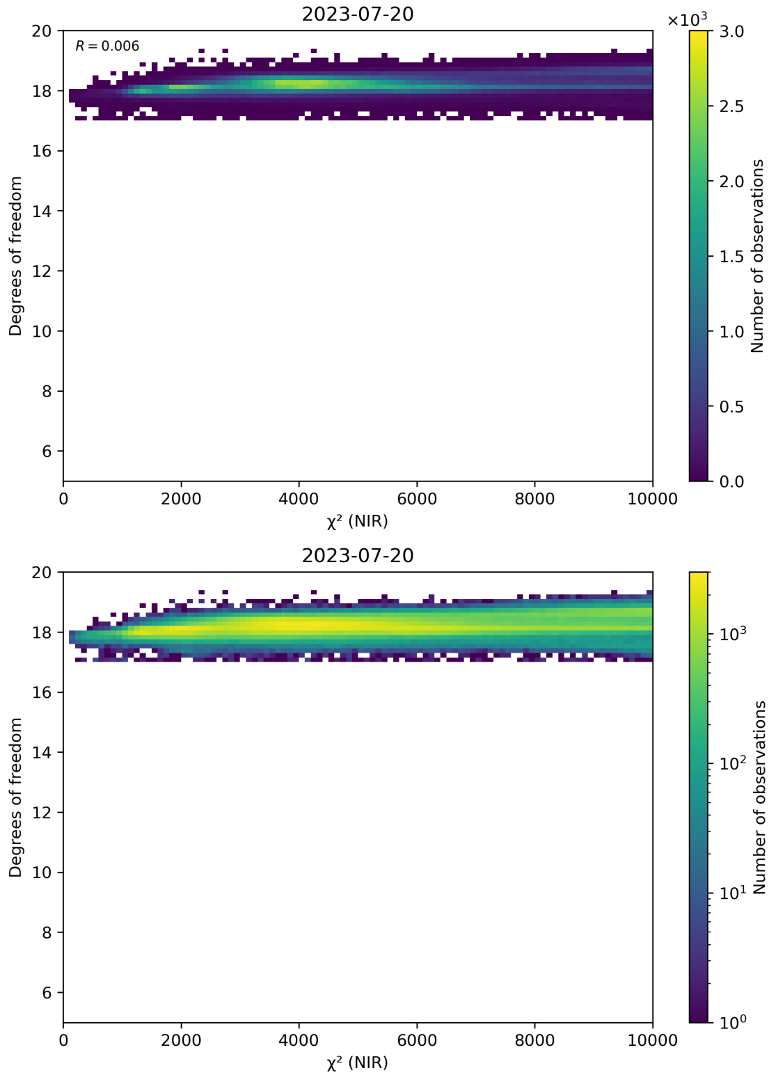
Figure 44: Scatter density plot of “ \chi^2 (NIR)” against “Degrees of freedom” for 2023-07-19 to 2023-07-21.
