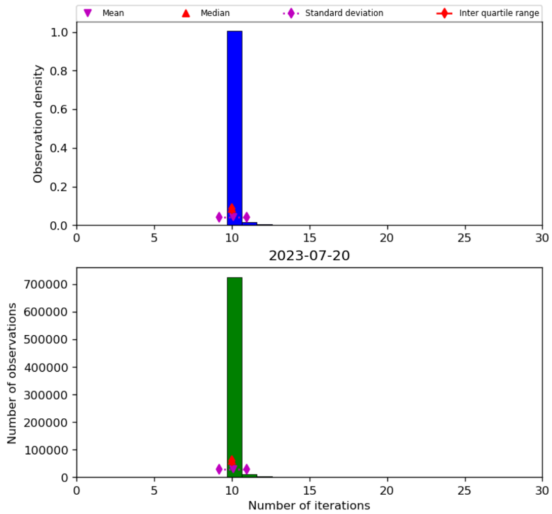
Figure 31: Histogram of “Number of iterations” for 2023-07-19 to 2023-07-21
