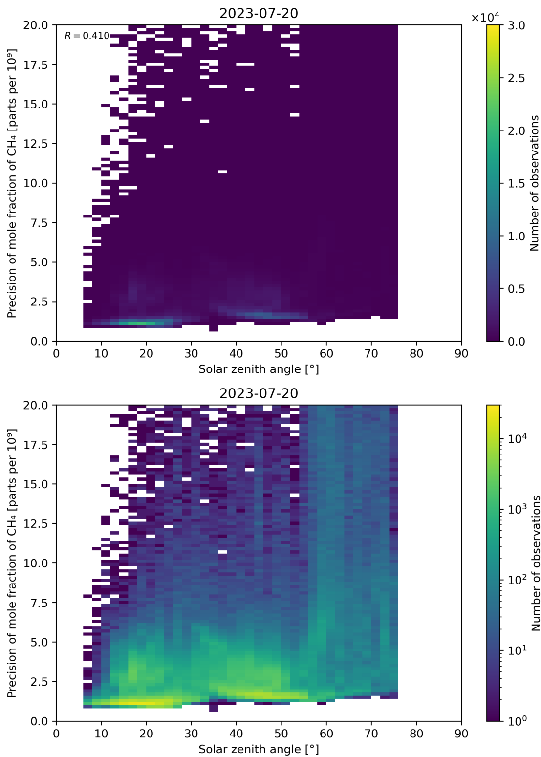
Figure 101: Scatter density plot of “Solar zenith angle” against “Precision of mole fraction of CH 4 ” for 2023-07-19 to 2023-07-21.
