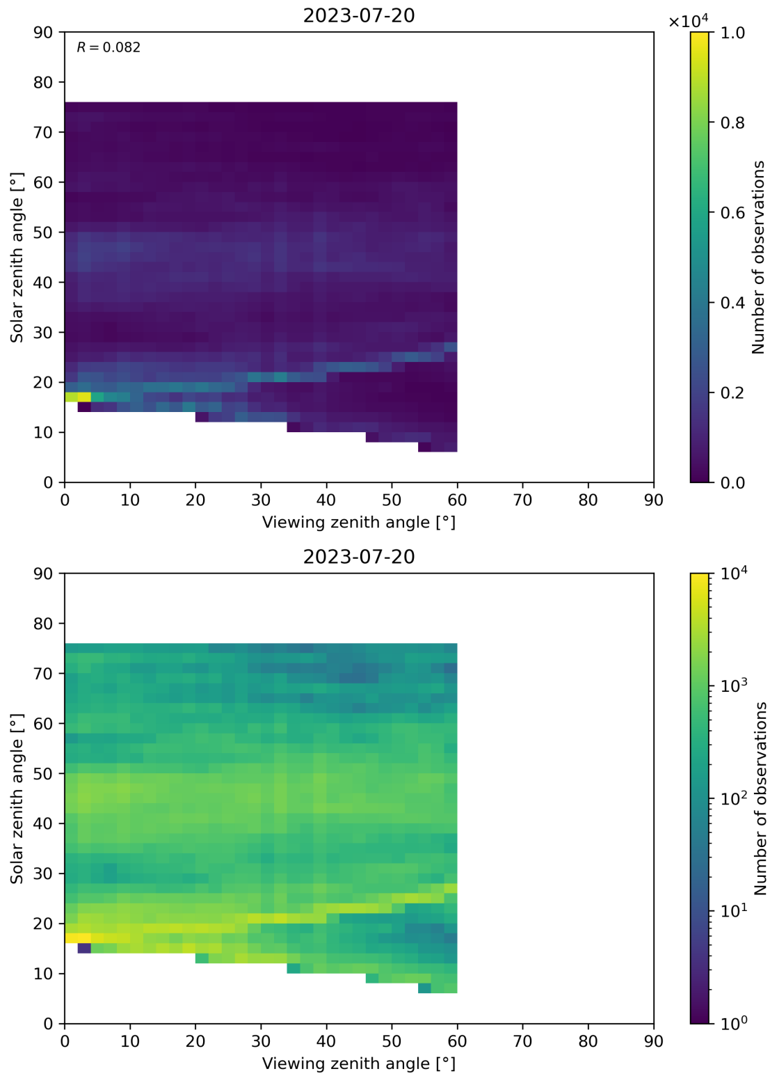
Figure 115: Scatter density plot of “Viewing zenith angle” against “Solar zenith angle” for 2023-07-19 to 2023-07-21.
