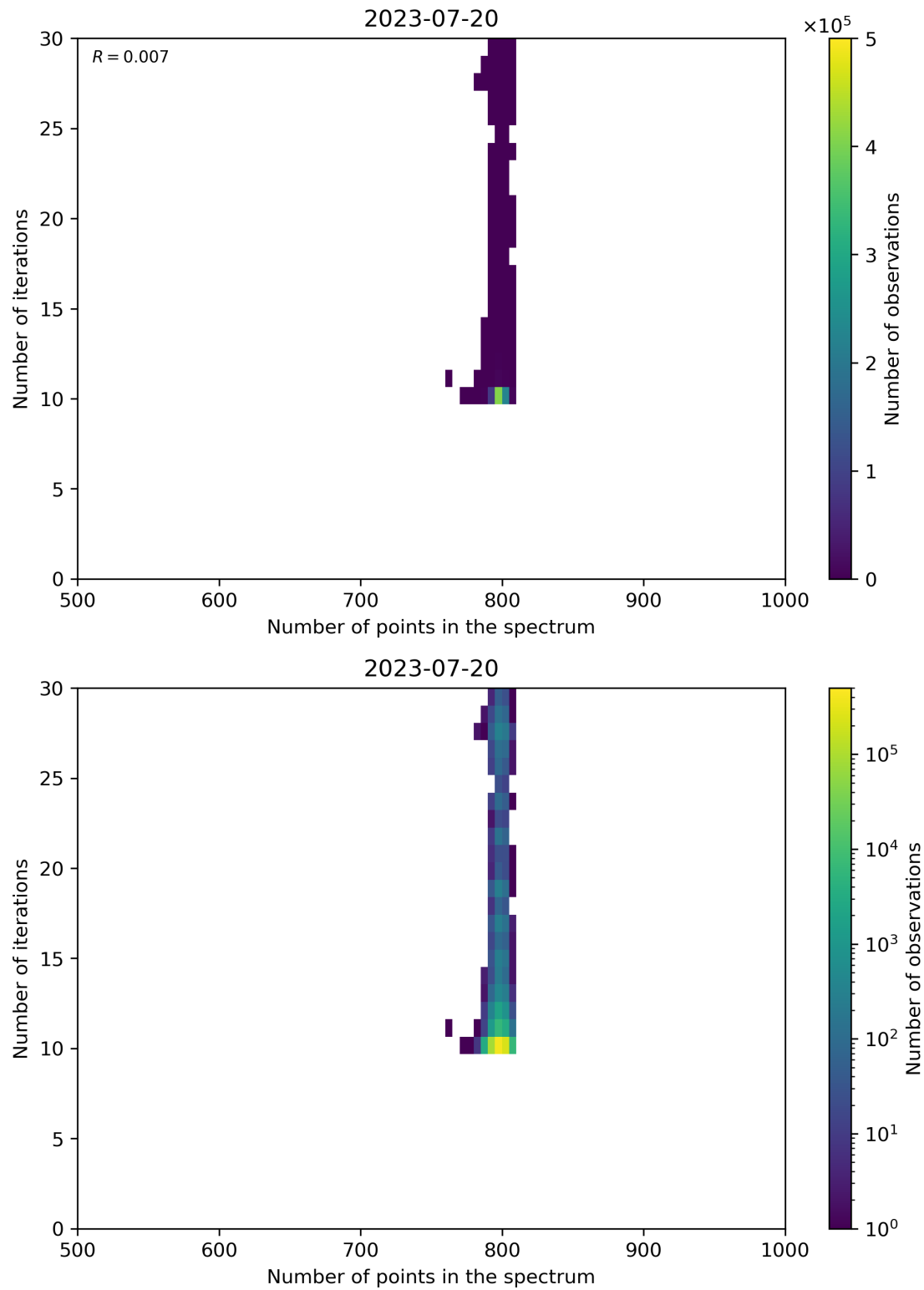
Figure 92: Scatter density plot of “Number of points in the spectrum” against “Number of iterations” for 2023-07-19 to 2023-07-21.
