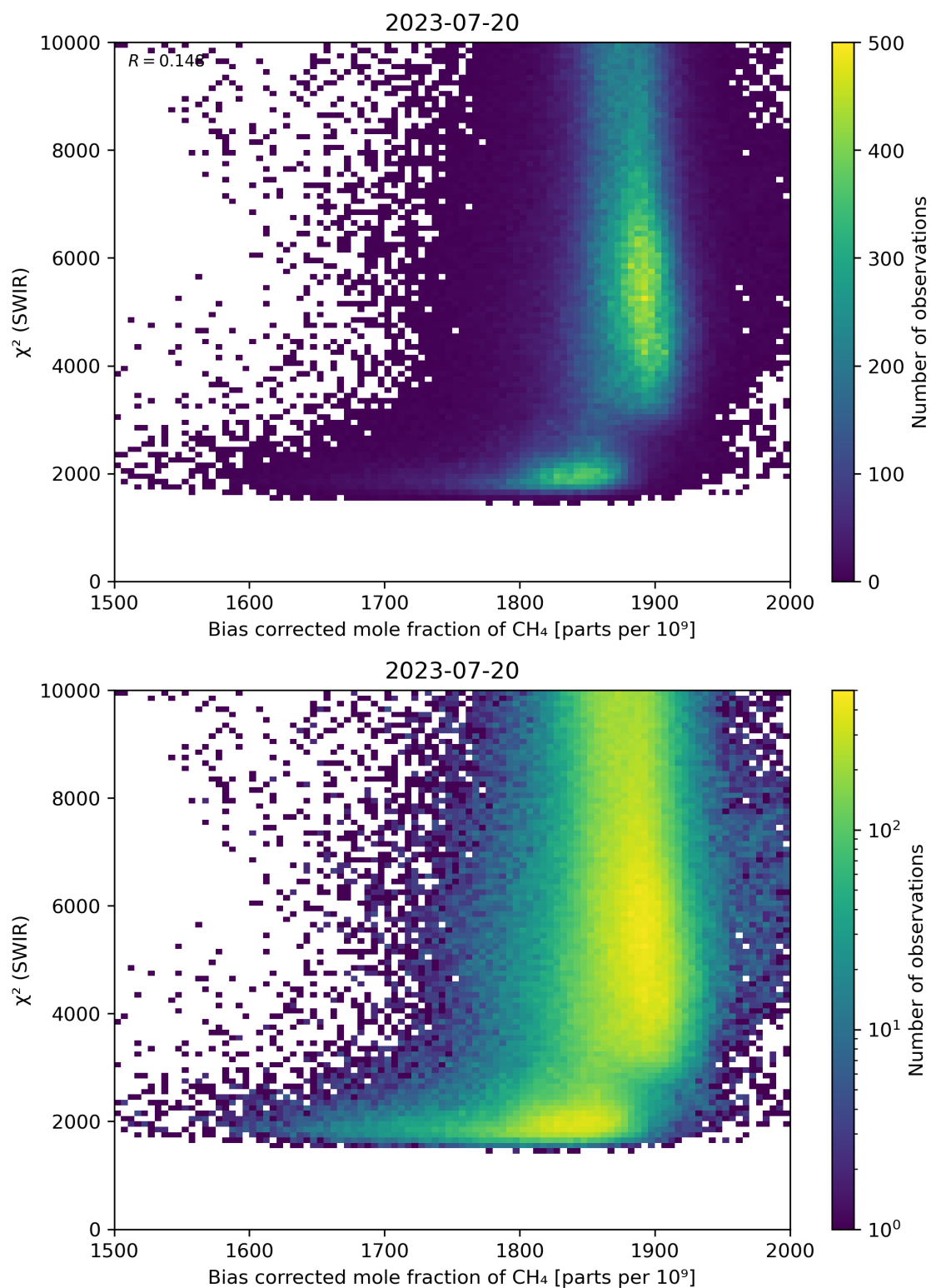
Figure 64: Scatter density plot of “Bias corrected mole fraction of \text{CH}_4 ” against “ \chi^2 (SWIR)” for 2023-07-19 to 2023-07-21.
