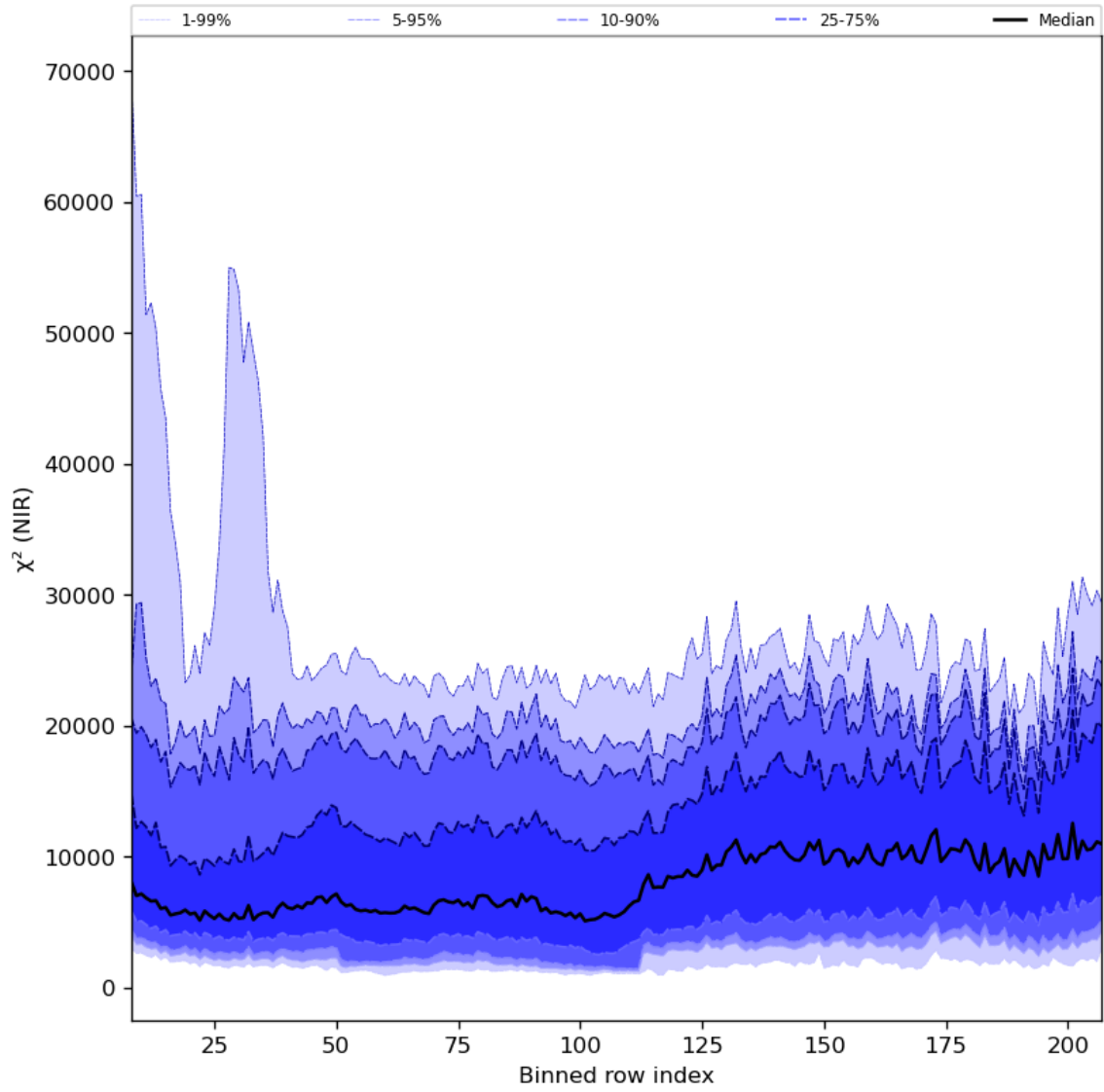
Figure 40: Along track statistics of “ \chi^2 (NIR)” for 2023-07-19 to 2023-07-21
