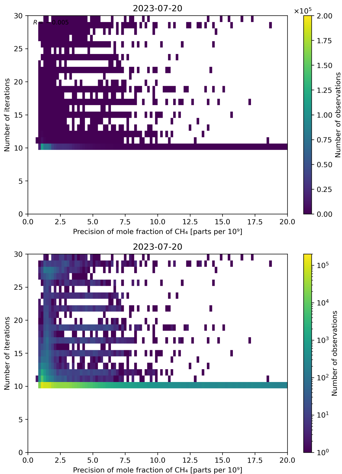
Figure 83: Scatter density plot of “Precision of mole fraction of CH 4 ” against “Number of iterations” for 2023-07-19 to 2023-07-21.
