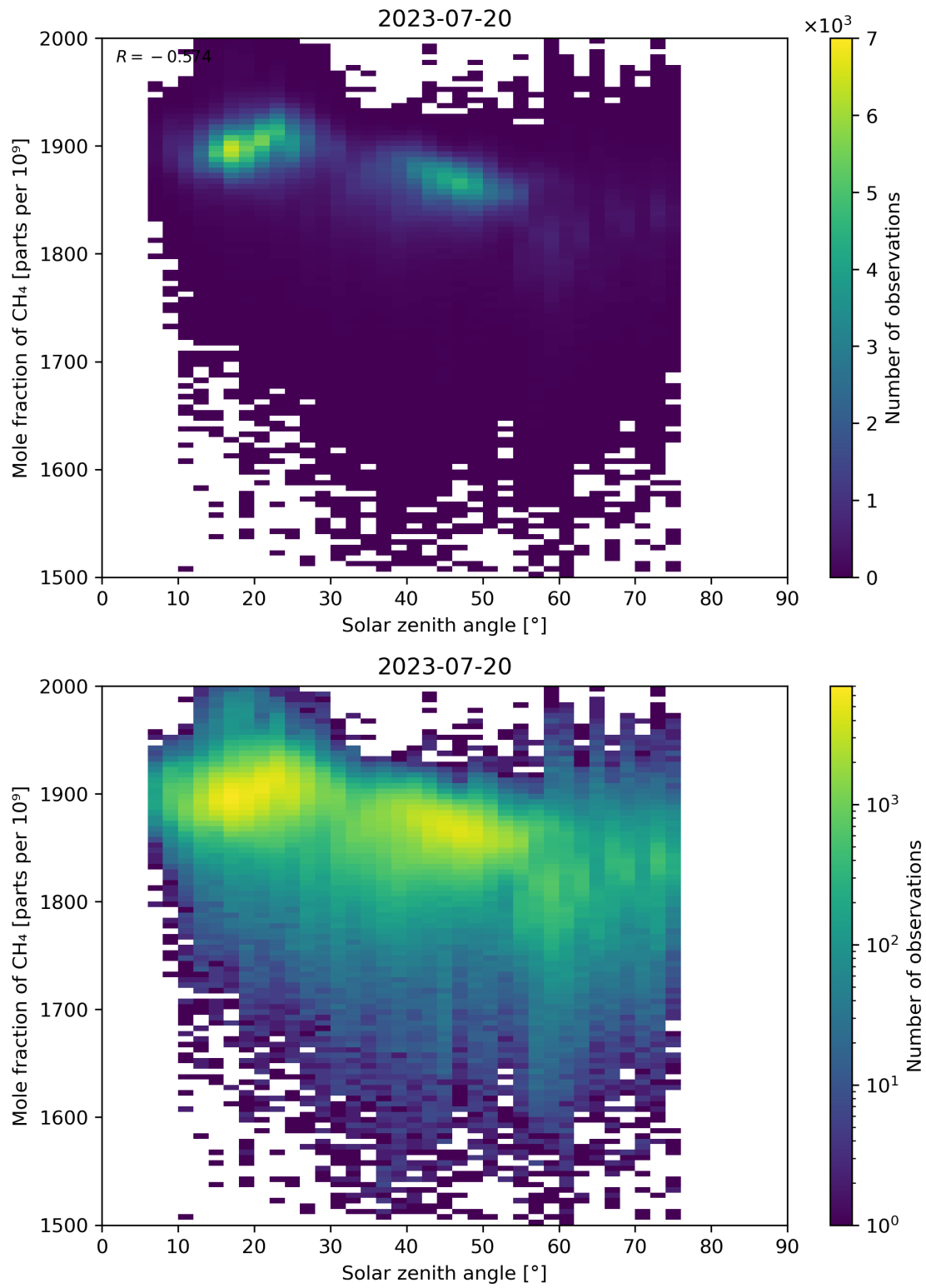
Figure 99: Scatter density plot of “Solar zenith angle” against “Mole fraction of \text{CH}_4 ” for 2023-07-19 to 2023-07-21.
