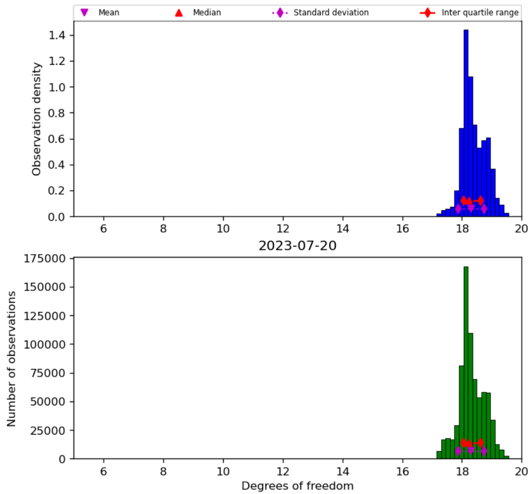
Figure 30: Histogram of “Degrees of freedom” for 2023-07-19 to 2023-07-21
