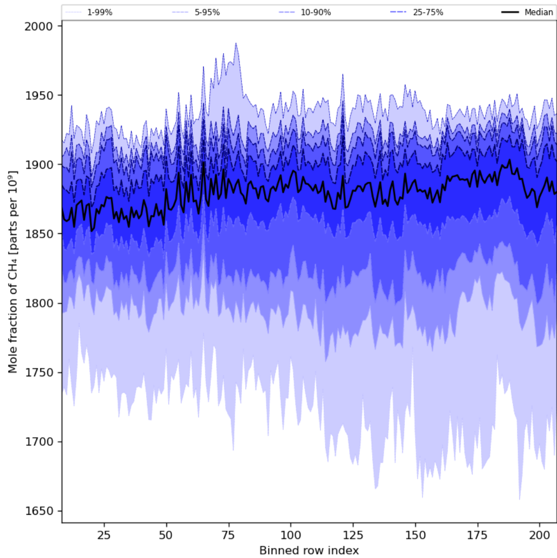
Figure 34: Along track statistics of “Mole fraction of CH 4 ” for 2023-07-19 to 2023-07-21
