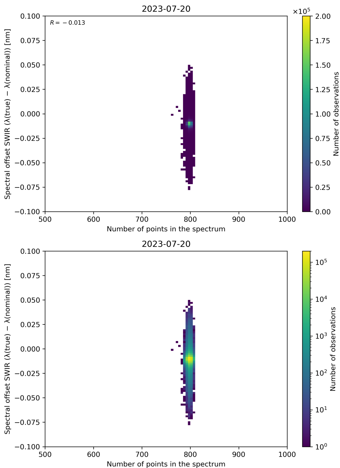
Figure 93: Scatter density plot of “Number of points in the spectrum” against “Spectral offset SWIR ( \lambda(\text{true}) - \lambda(\text{nominal}) )” for 2023-07-19 to 2023-07-21.
