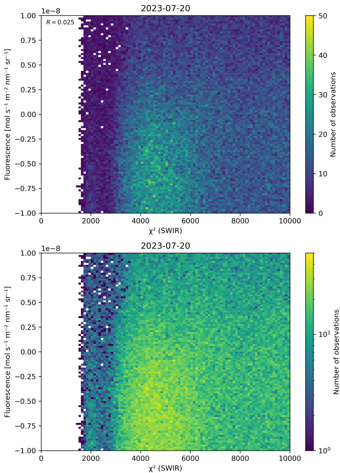
Figure 49: Scatter density plot of “ \chi^2 (SWIR)” against “Fluorescence” for 2023-07-19 to 2023-07-21.
