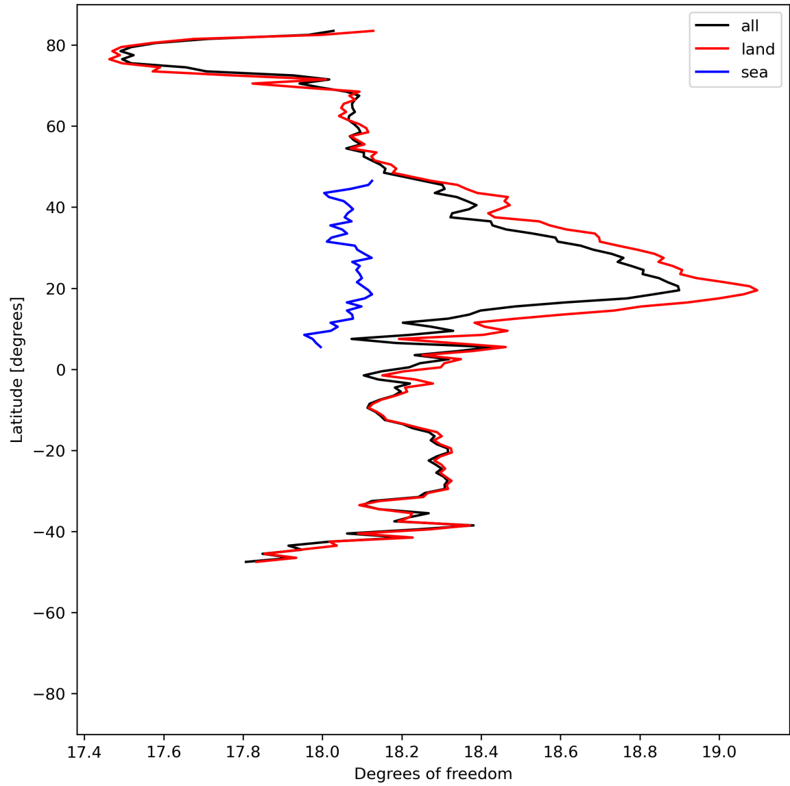
Figure 19: Zonal average of “Degrees of freedom” for 2023-07-19 to 2023-07-21.
