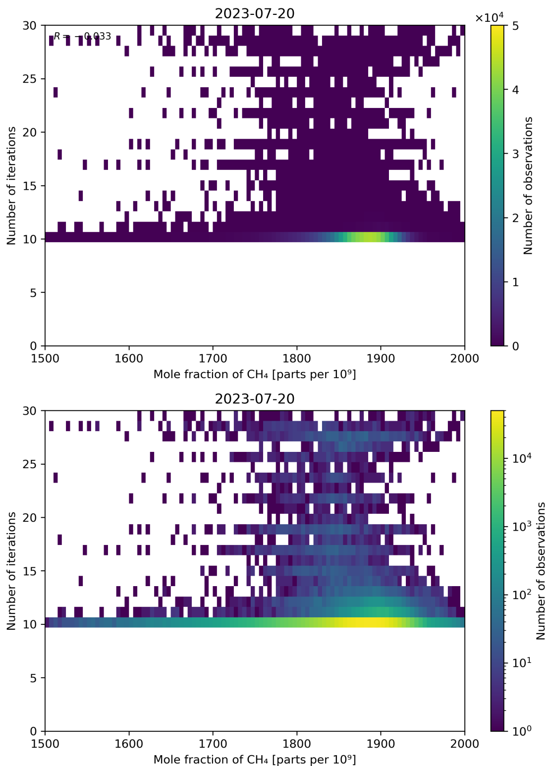
Figure 76: Scatter density plot of “Mole fraction of CH 4 ” against “Number of iterations” for 2023-07-19 to 2023-07-21.
