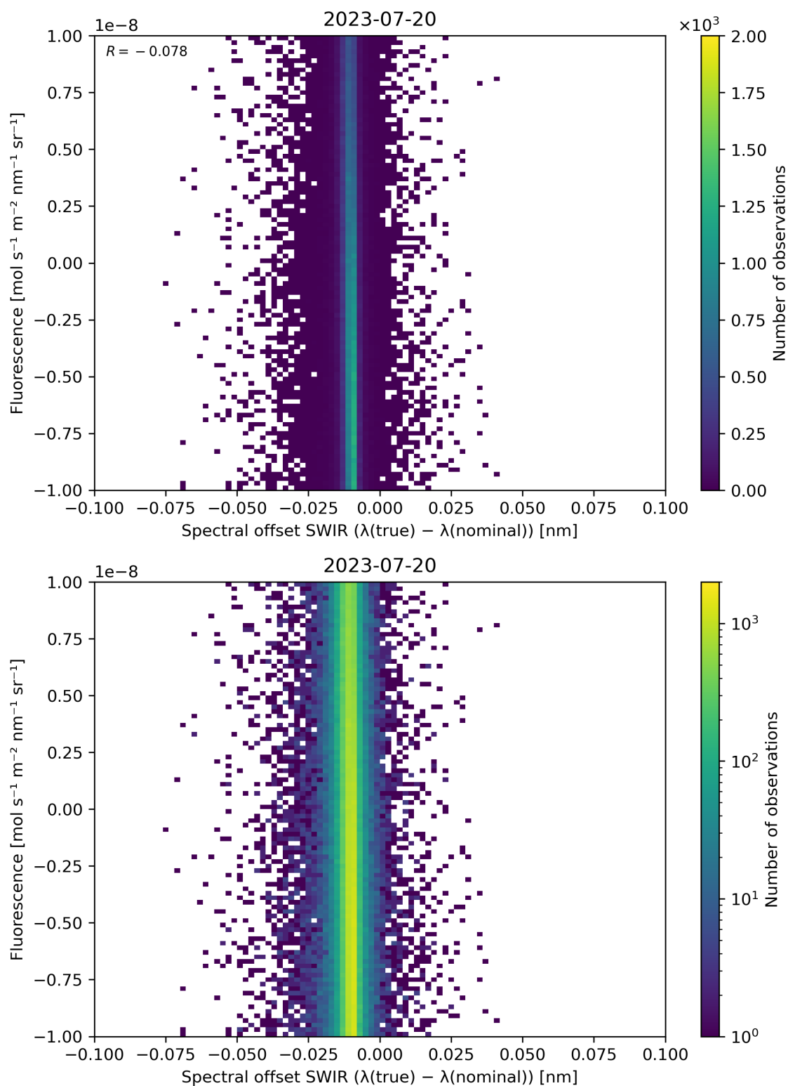
Figure 120: Scatter density plot of “Spectral offset SWIR ( \lambda(\text{true}) - \lambda(\text{nominal}) )” against “Fluorescence” for 2023-07-19 to 2023-07-21.
