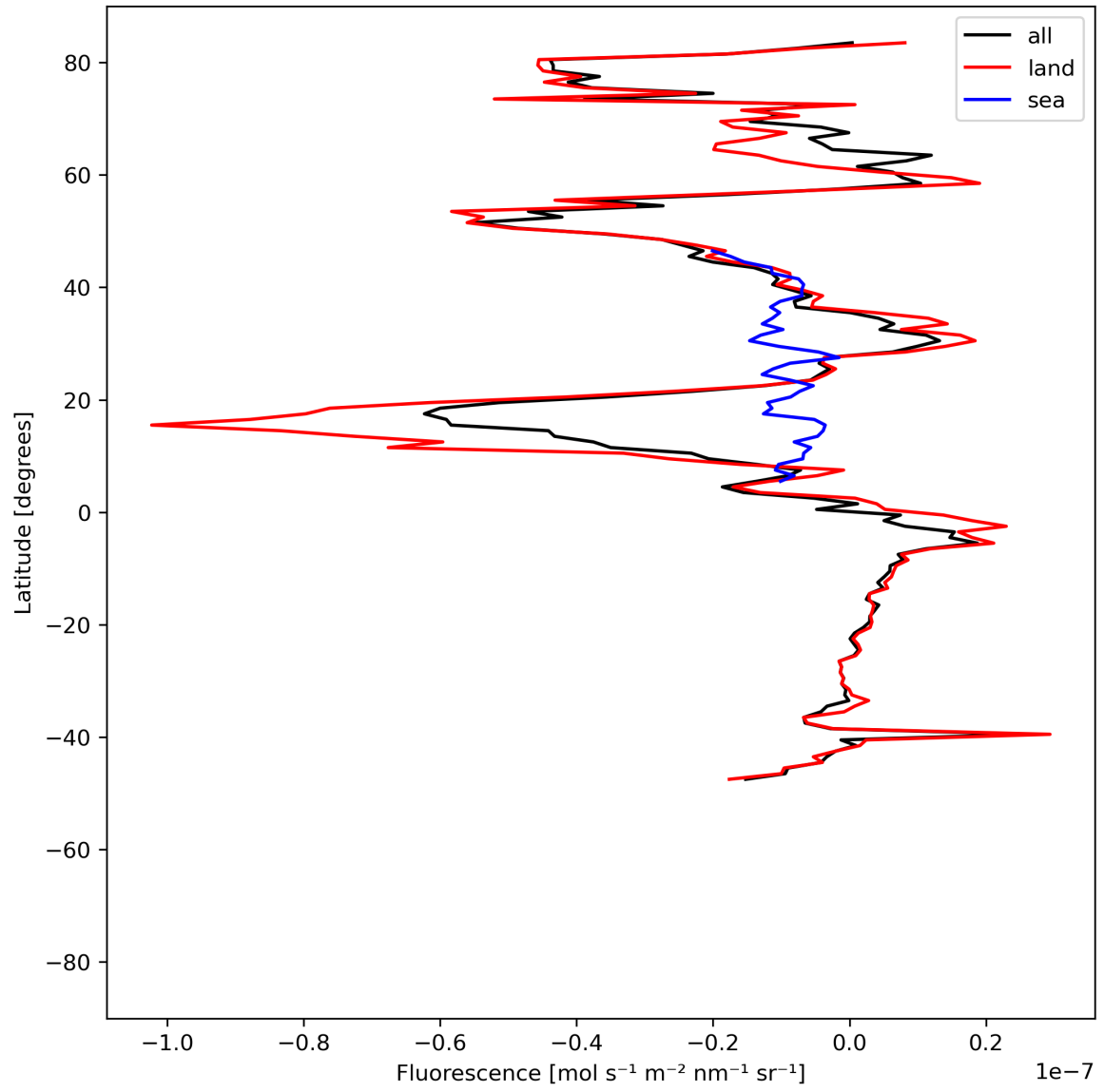
Figure 21: Zonal average of “Fluorescence” for 2023-07-19 to 2023-07-21.
