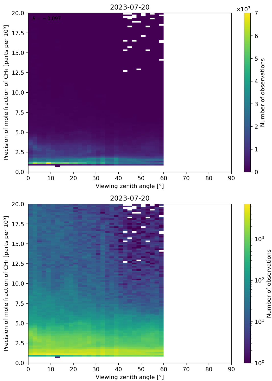
Figure 112: Scatter density plot of “Viewing zenith angle” against “Precision of mole fraction of CH 4 ” for 2023-07-19 to 2023-07-21.
