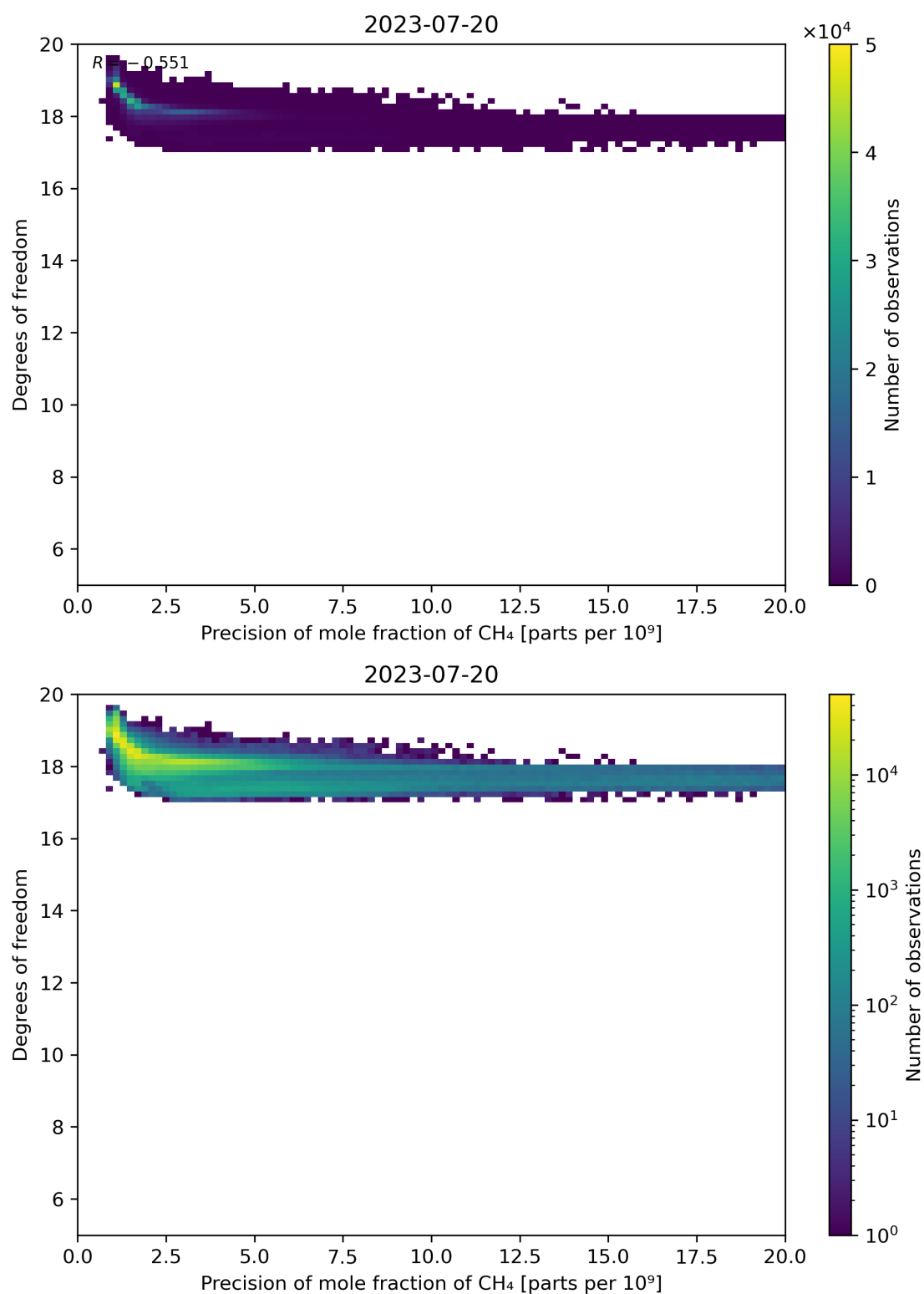
Figure 80: Scatter density plot of “Precision of mole fraction of CH 4 ” against “Degrees of freedom” for 2023-07-19 to 2023-07-21.
