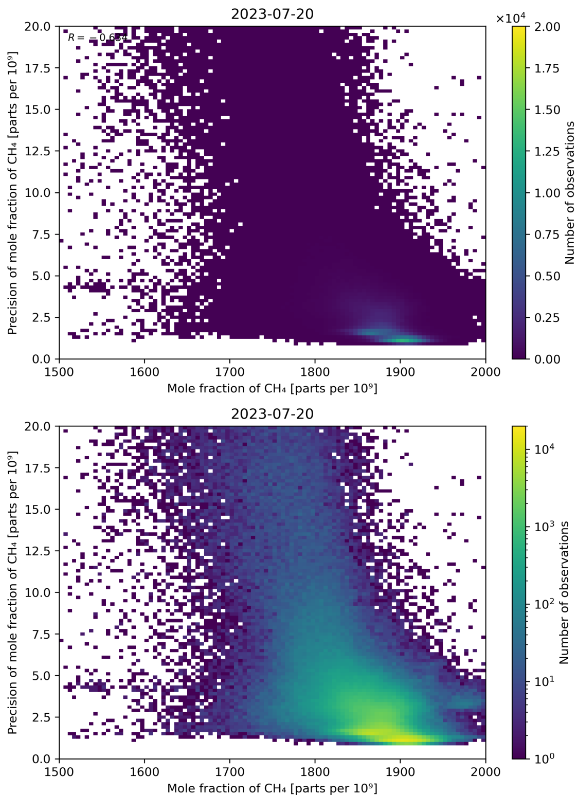
Figure 75: Scatter density plot of “Mole fraction of CH 4 ” against “Precision of mole fraction of CH 4 ” for 2023-07-19 to 2023-07-21.
