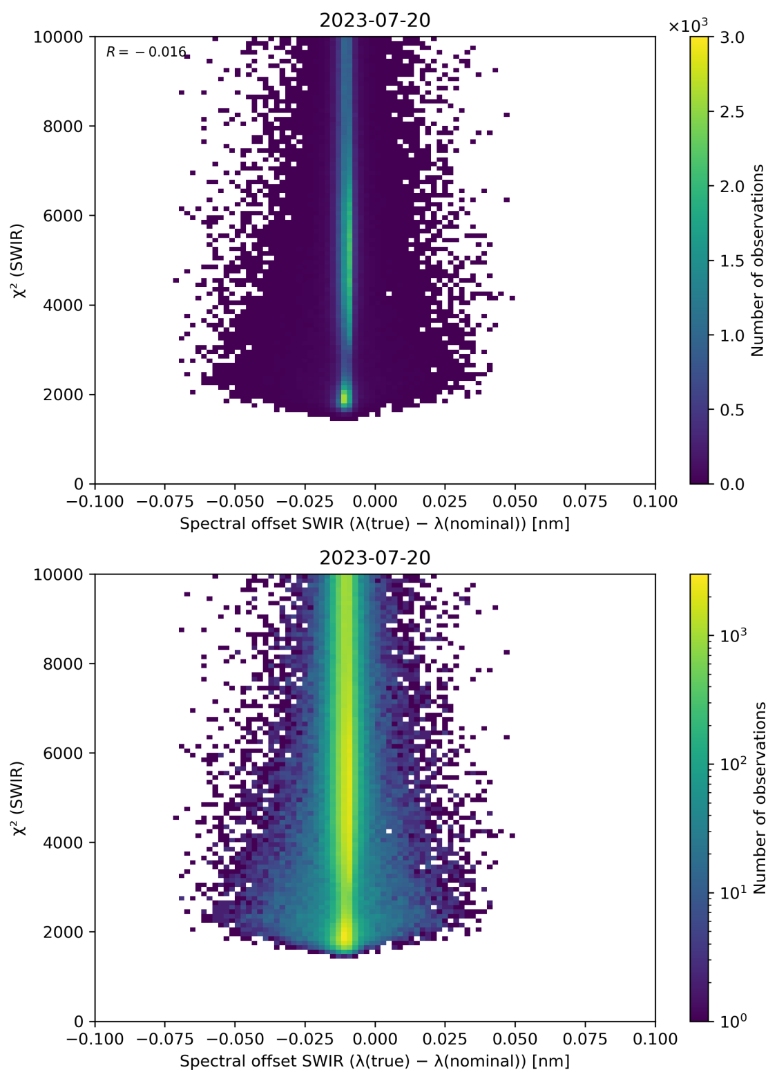
Figure 118: Scatter density plot of “Spectral offset SWIR ( \lambda(\text{true}) - \lambda(\text{nominal}) )” against “ \chi^2 (SWIR)” for 2023-07-19 to 2023-07-21.
