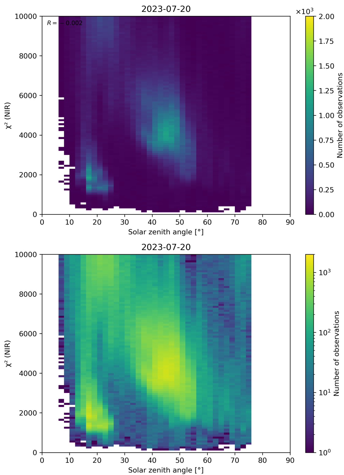
Figure 94: Scatter density plot of “Solar zenith angle” against “ \chi^2 (NIR)” for 2023-07-19 to 2023-07-21.
