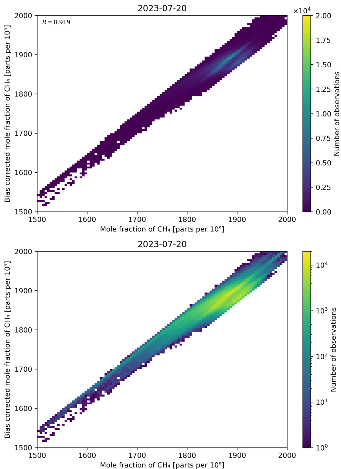
Figure 74: Scatter density plot of “Mole fraction of CH 4 ” against “Bias corrected mole fraction of CH 4 ” for 2023-07-19 to 2023-07-21.
