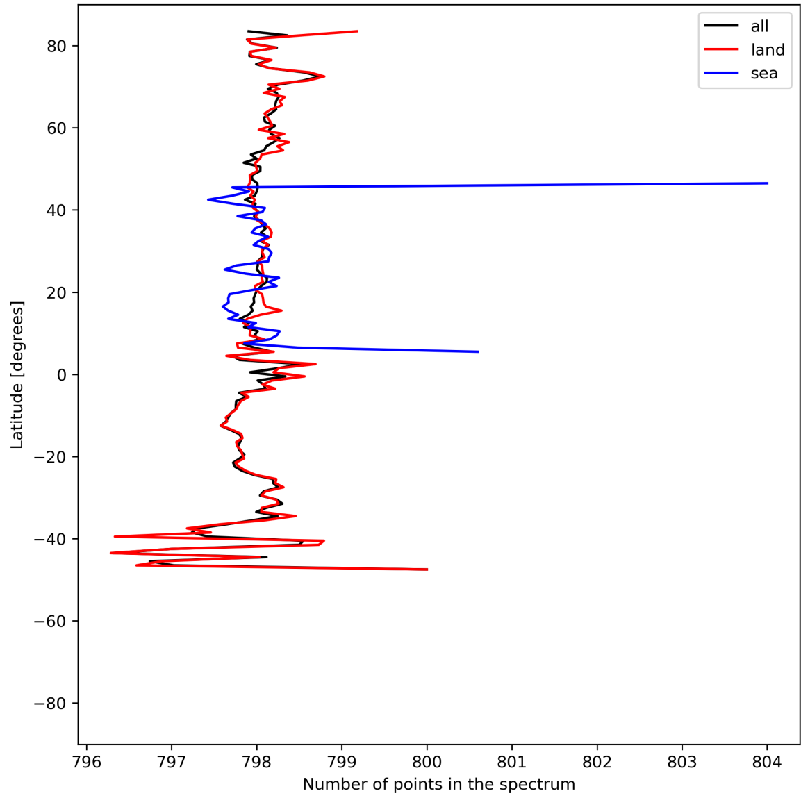
Figure 15: Zonal average of “Number of points in the spectrum” for 2023-07-19 to 2023-07-21.
