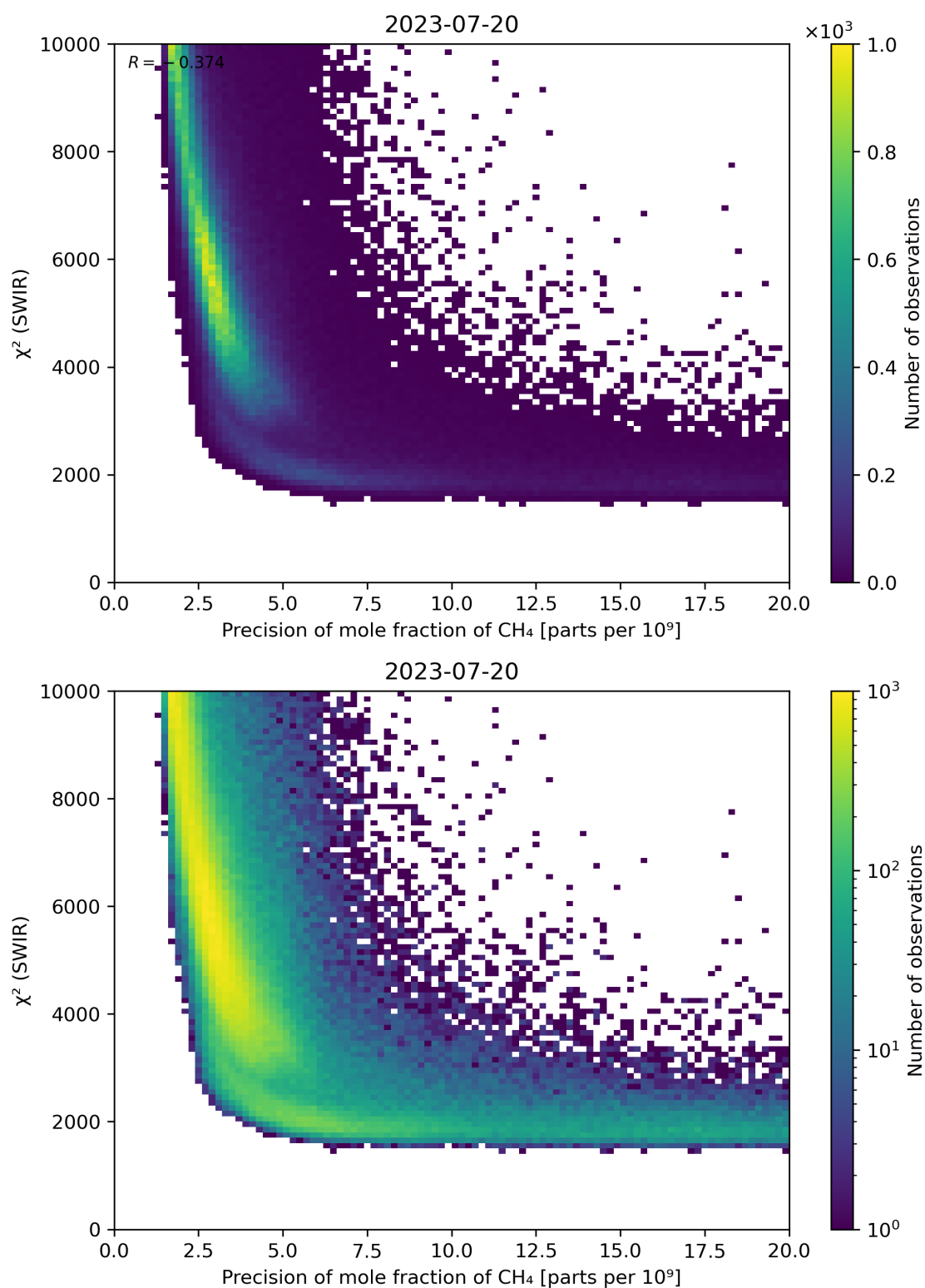
Figure 79: Scatter density plot of “Precision of mole fraction of CH 4 ” against “ \chi^2 (SWIR)” for 2023-07-19 to 2023-07-21.
