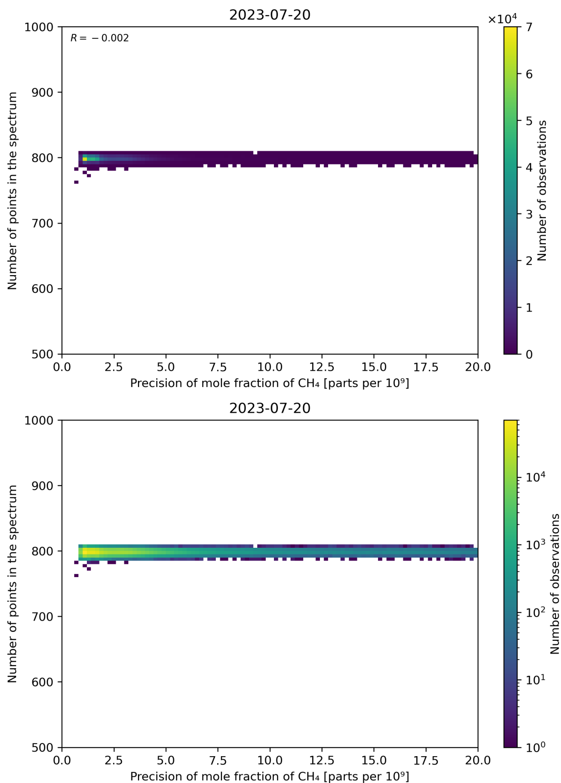
Figure 84: Scatter density plot of “Precision of mole fraction of CH 4 ” against “Number of points in the spectrum” for 2023-07-19 to 2023-07-21.
