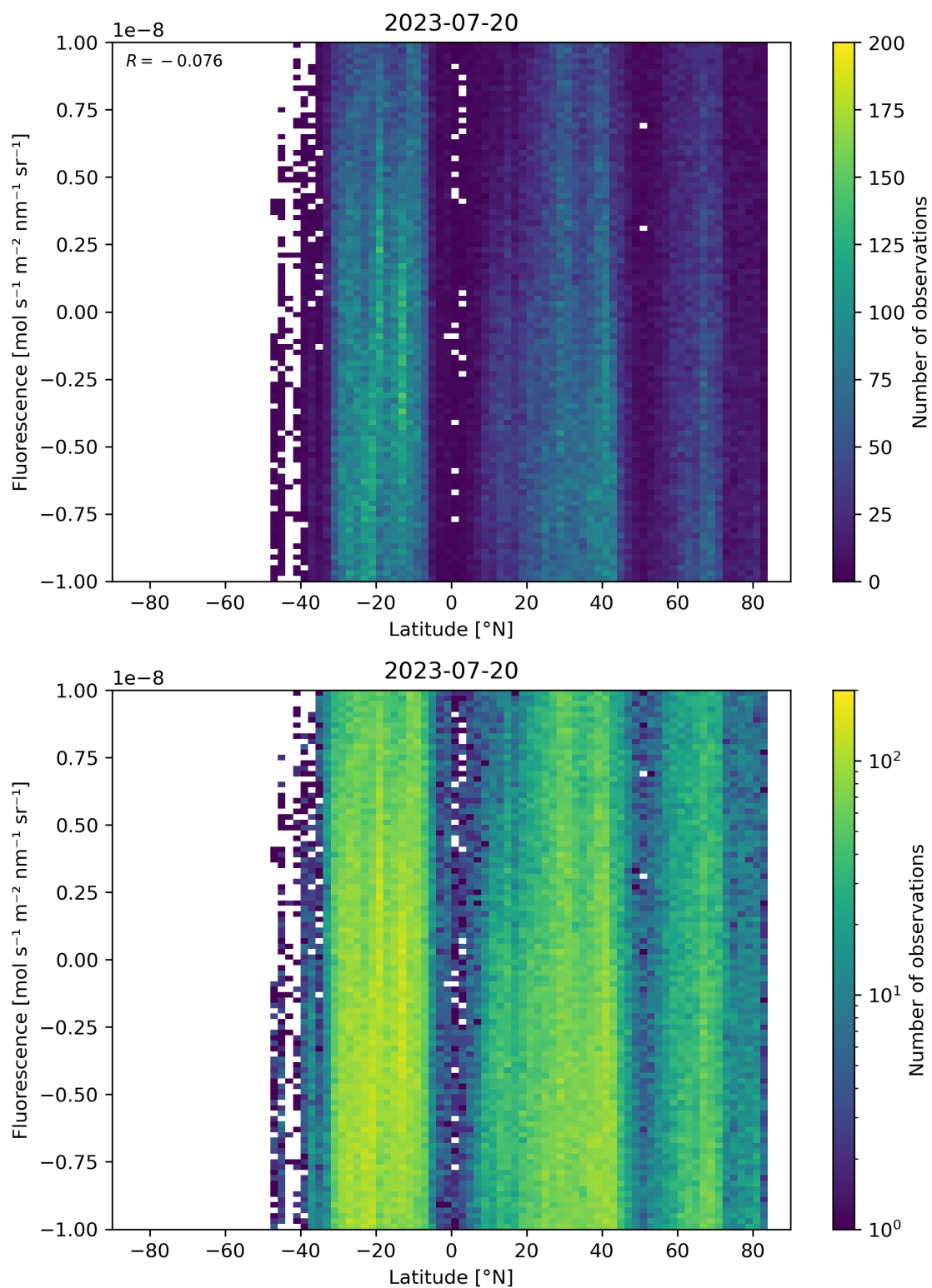
Figure 56: Scatter density plot of “Latitude” against “Fluorescence” for 2023-07-19 to 2023-07-21.
