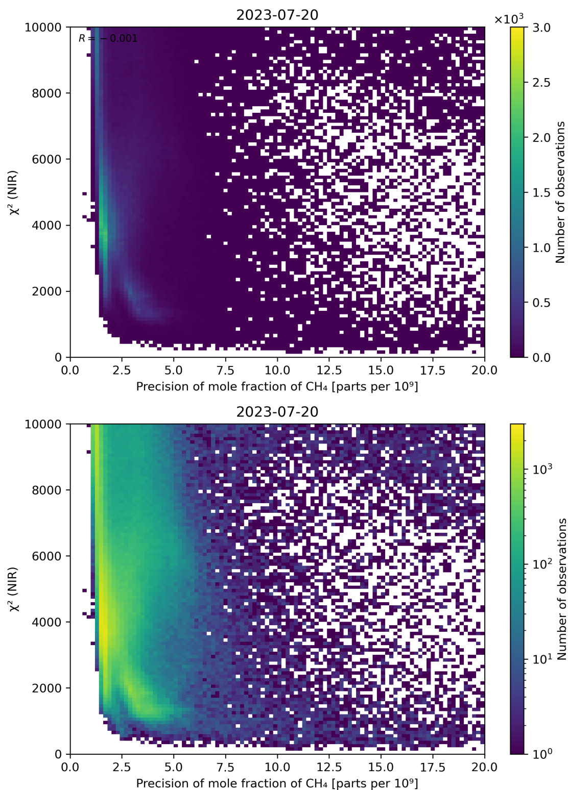
Figure 78: Scatter density plot of “Precision of mole fraction of CH 4 ” against “ \chi^2 (NIR)” for 2023-07-19 to 2023-07-21.
