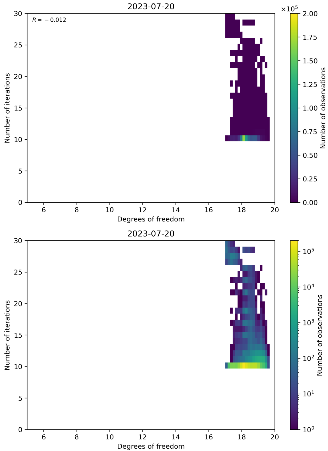
Figure 52: Scatter density plot of “Degrees of freedom” against “Number of iterations” for 2023-07-19 to 2023-07-21.
