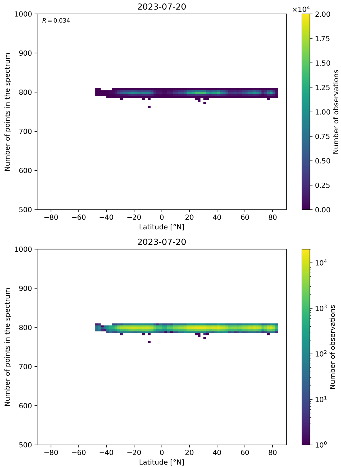
Figure 61: Scatter density plot of “Latitude” against “Number of points in the spectrum” for 2023-07-19 to 2023-07-21.
