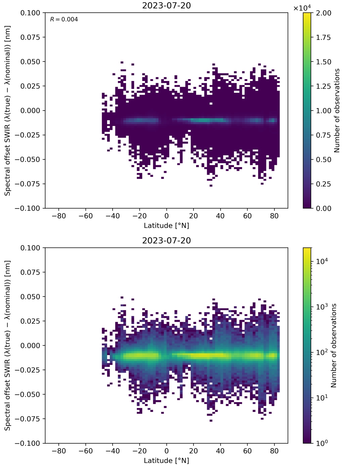
Figure 62: Scatter density plot of “Latitude” against “Spectral offset SWIR ( \lambda(\text{true}) - \lambda(\text{nominal}) )” for 2023-07-19 to 2023-07-21.
