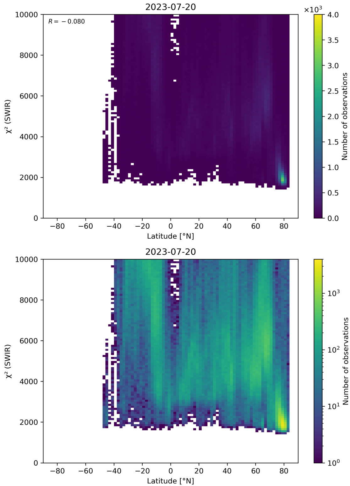
Figure 54: Scatter density plot of “Latitude” against “ \chi^2 (SWIR)” for 2023-07-19 to 2023-07-21.
