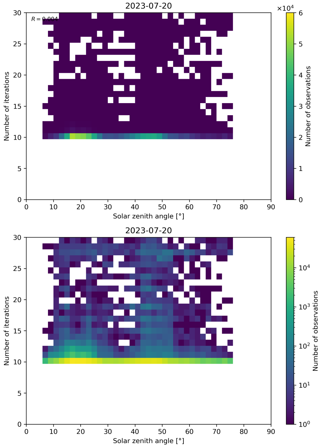
Figure 102: Scatter density plot of “Solar zenith angle” against “Number of iterations” for 2023-07-19 to 2023-07-21.
