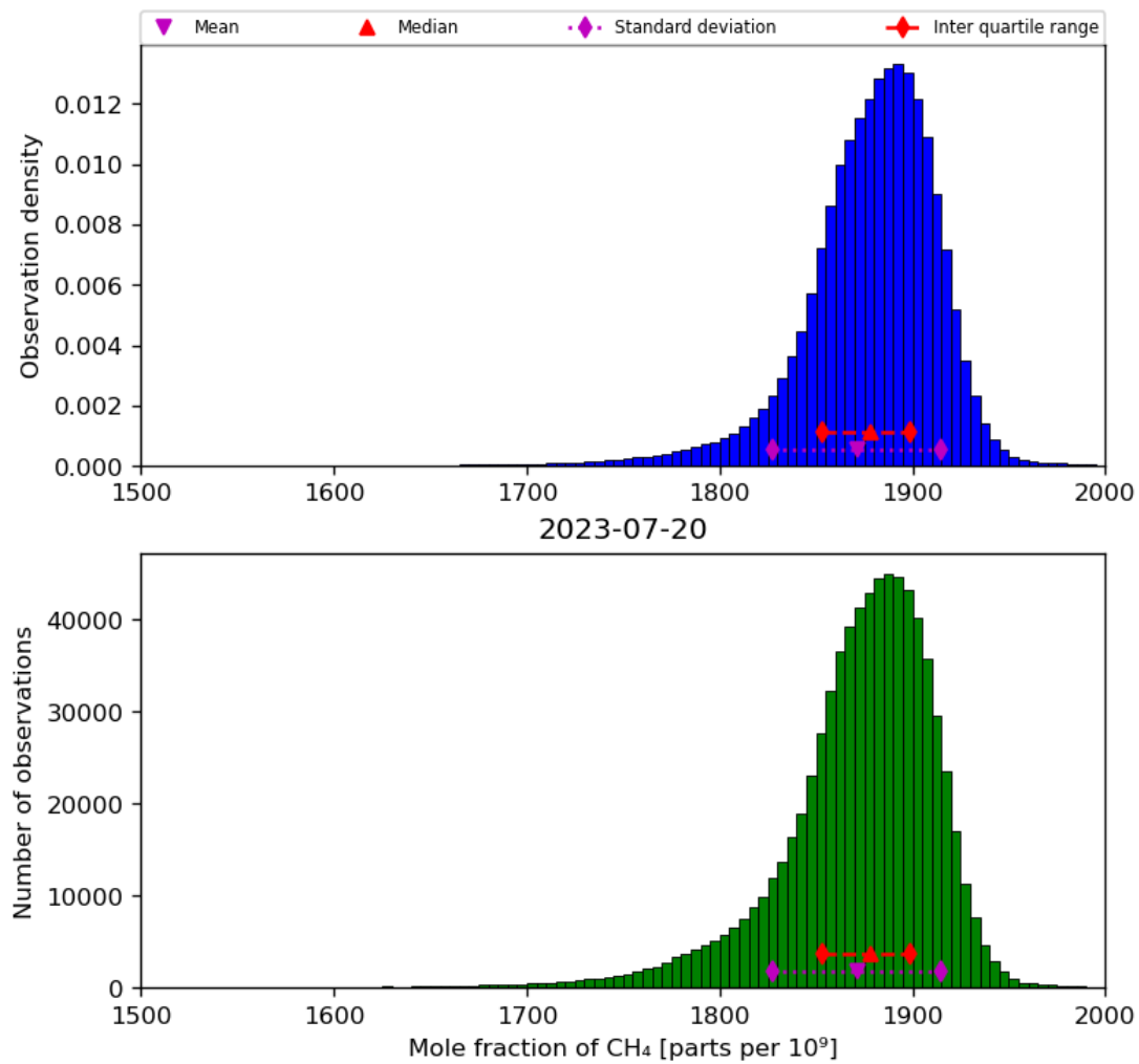
Figure 23: Histogram of “Mole fraction of CH 4 ” for 2023-07-19 to 2023-07-21
