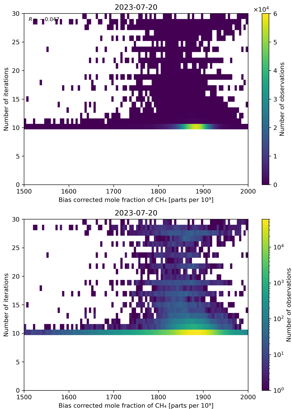
Figure 67: Scatter density plot of “Bias corrected mole fraction of CH 4 ” against “Number of iterations” for 2023-07-19 to 2023-07-21.
