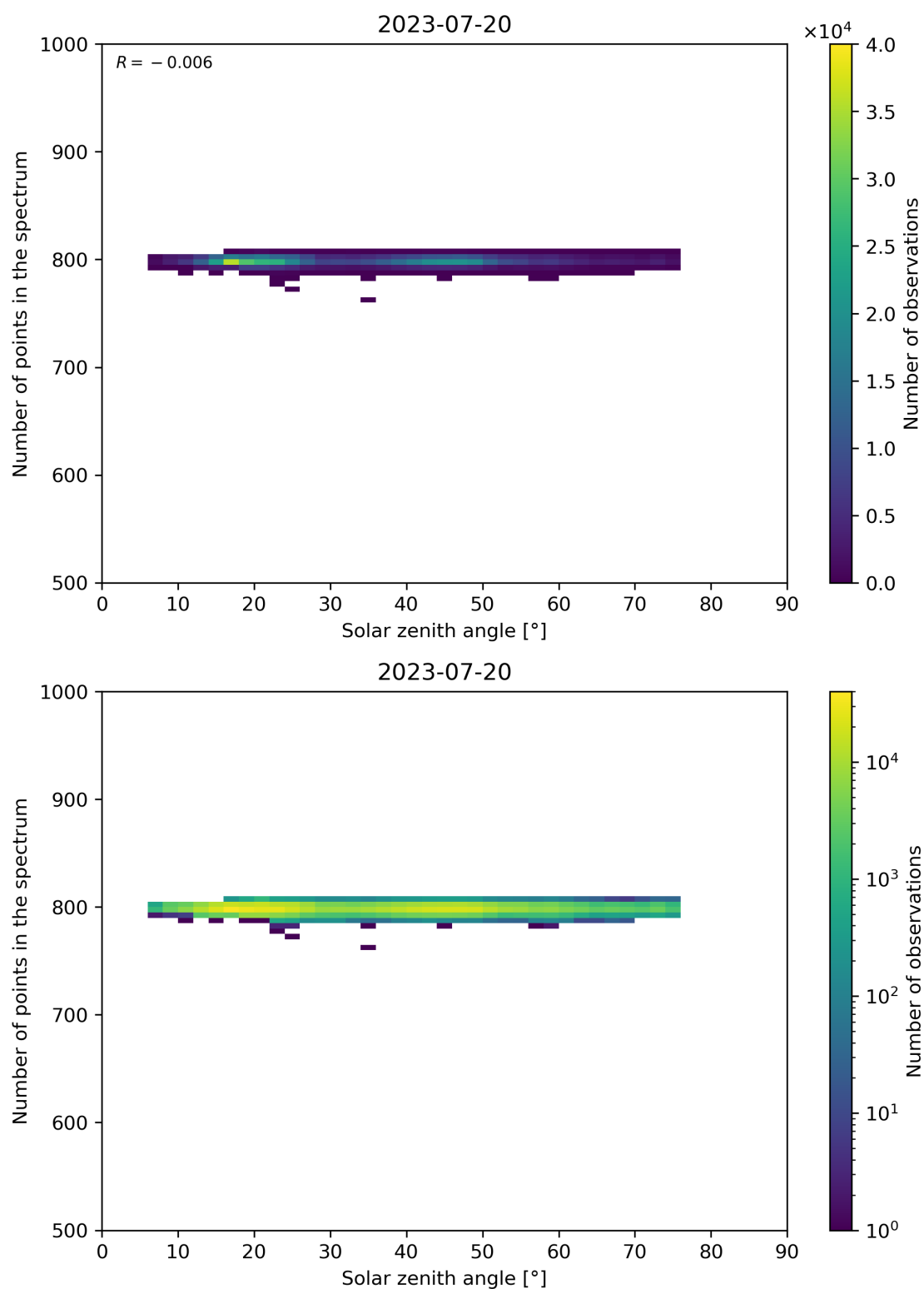
Figure 103: Scatter density plot of “Solar zenith angle” against “Number of points in the spectrum” for 2023-07-19 to 2023-07-21.
