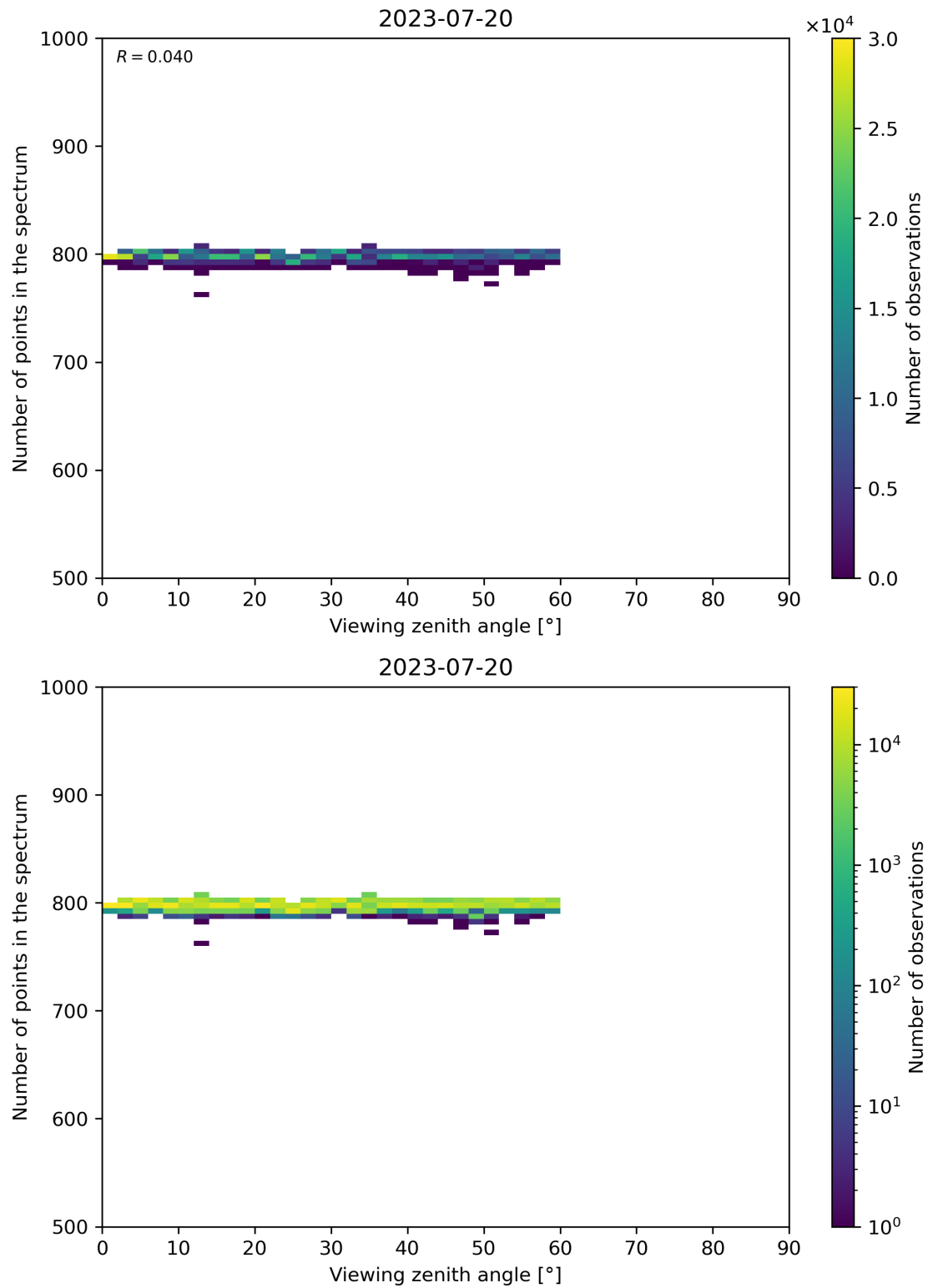
Figure 114: Scatter density plot of “Viewing zenith angle” against “Number of points in the spectrum” for 2023-07-19 to 2023-07-21.
