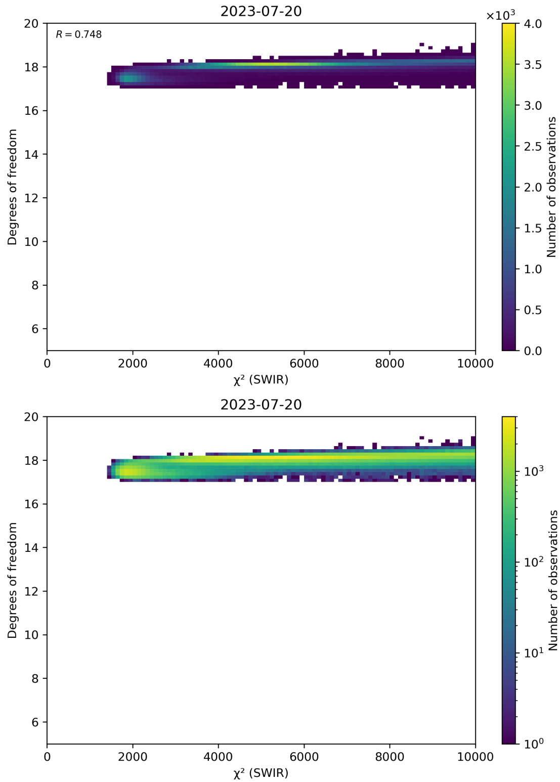
Figure 48: Scatter density plot of “ \chi^2 (SWIR)” against “Degrees of freedom” for 2023-07-19 to 2023-07-21.
