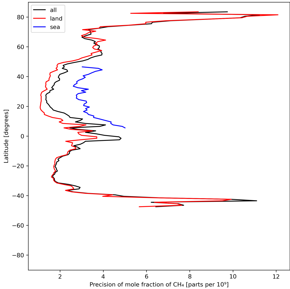
Figure 13: Zonal average of “Precision of mole fraction of \text{CH}_4 ” for 2023-07-19 to 2023-07-21.
