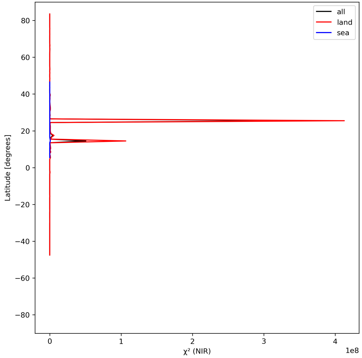
Figure 18: Zonal average of “ \chi^2 (NIR)” for 2023-07-19 to 2023-07-21.
