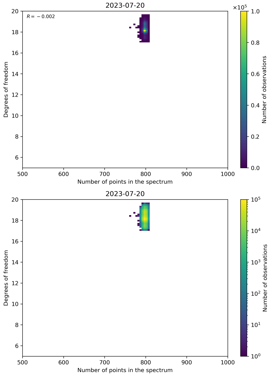
Figure 90: Scatter density plot of “Number of points in the spectrum” against “Degrees of freedom” for 2023-07-19 to 2023-07-21.
