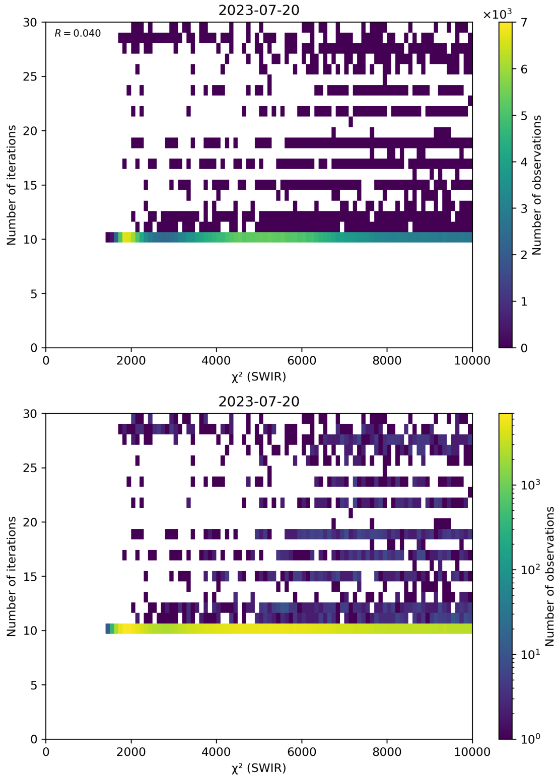
Figure 50: Scatter density plot of “ \chi^2 (SWIR)” against “Number of iterations” for 2023-07-19 to 2023-07-21.
