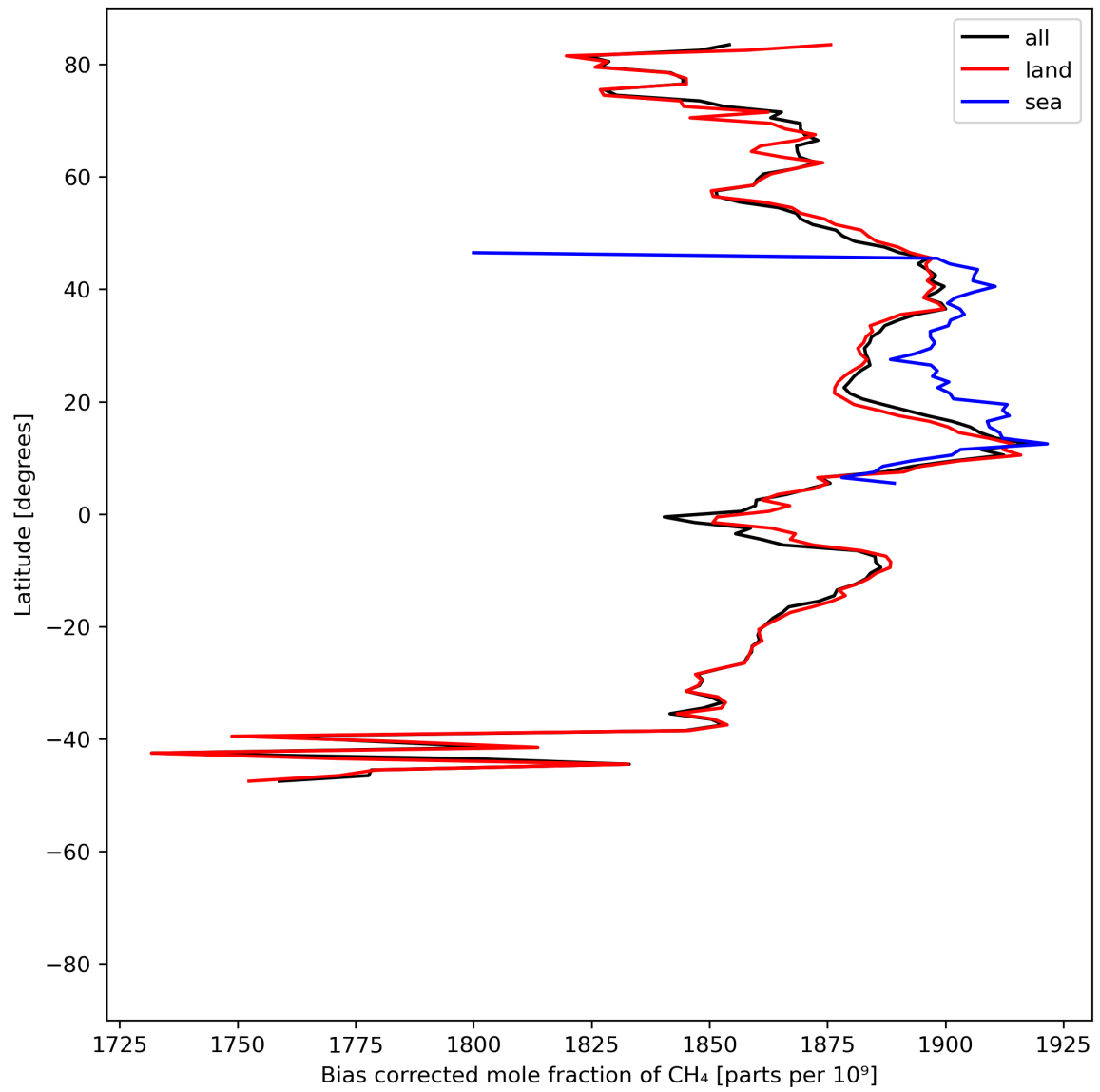
Figure 14: Zonal average of “Bias corrected mole fraction of CH 4 ” for 2023-07-19 to 2023-07-21.
