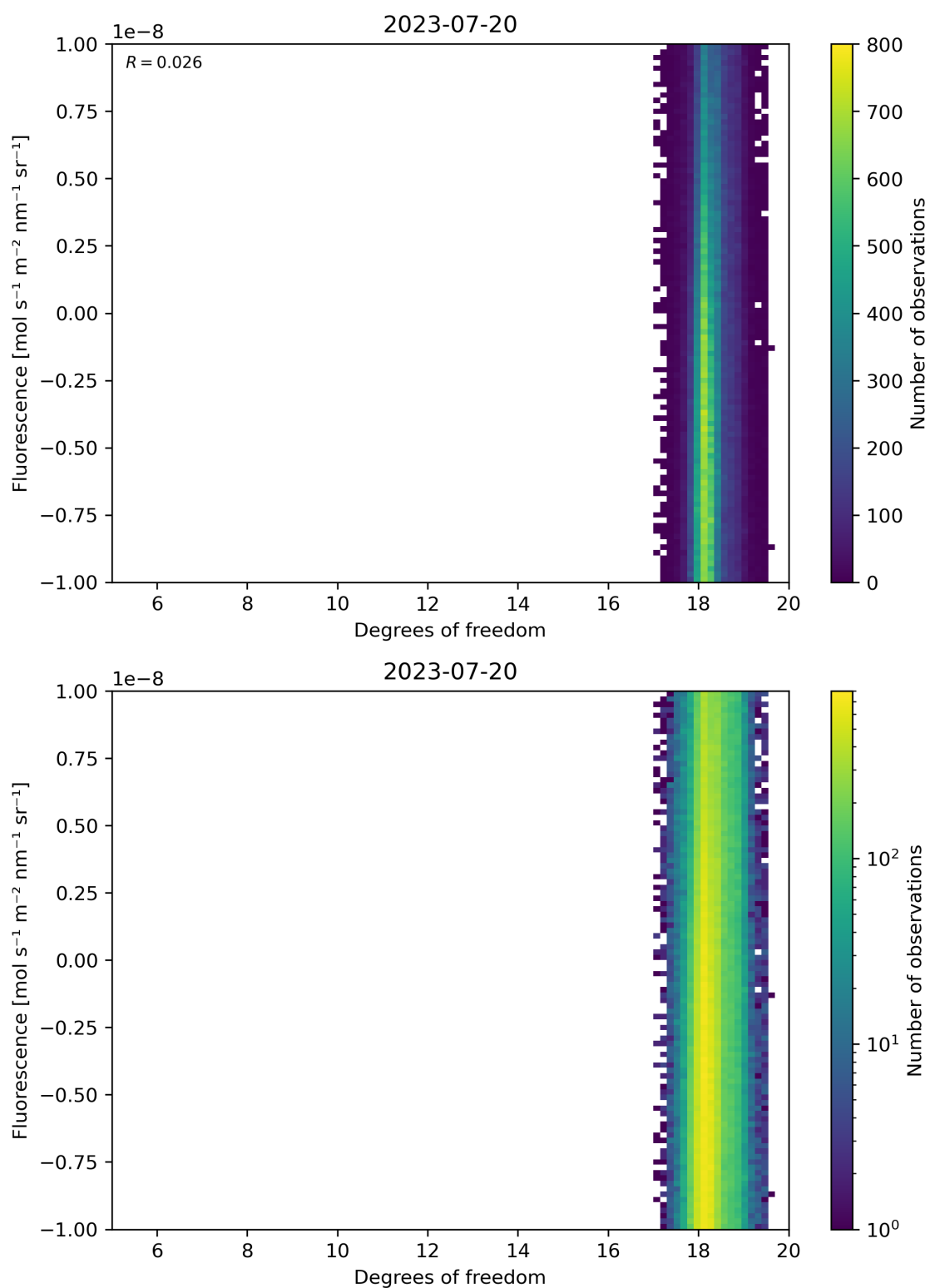
Figure 51: Scatter density plot of “Degrees of freedom” against “Fluorescence” for 2023-07-19 to 2023-07-21.
