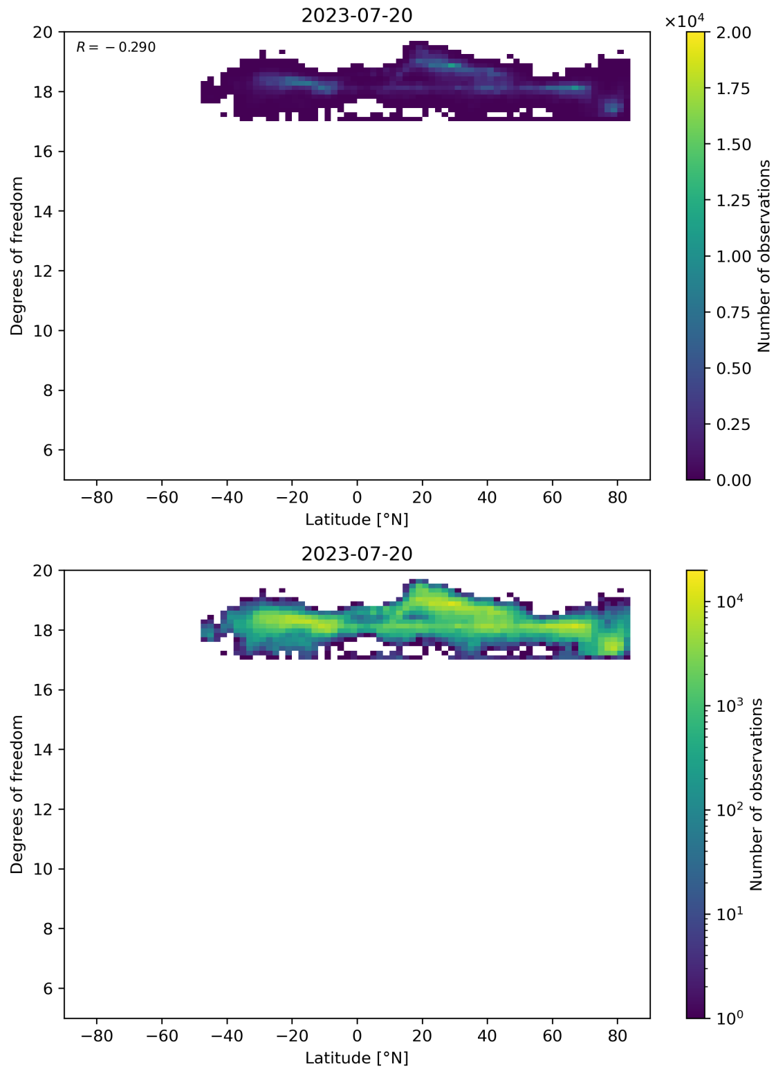
Figure 55: Scatter density plot of “Latitude” against “Degrees of freedom” for 2023-07-19 to 2023-07-21.
