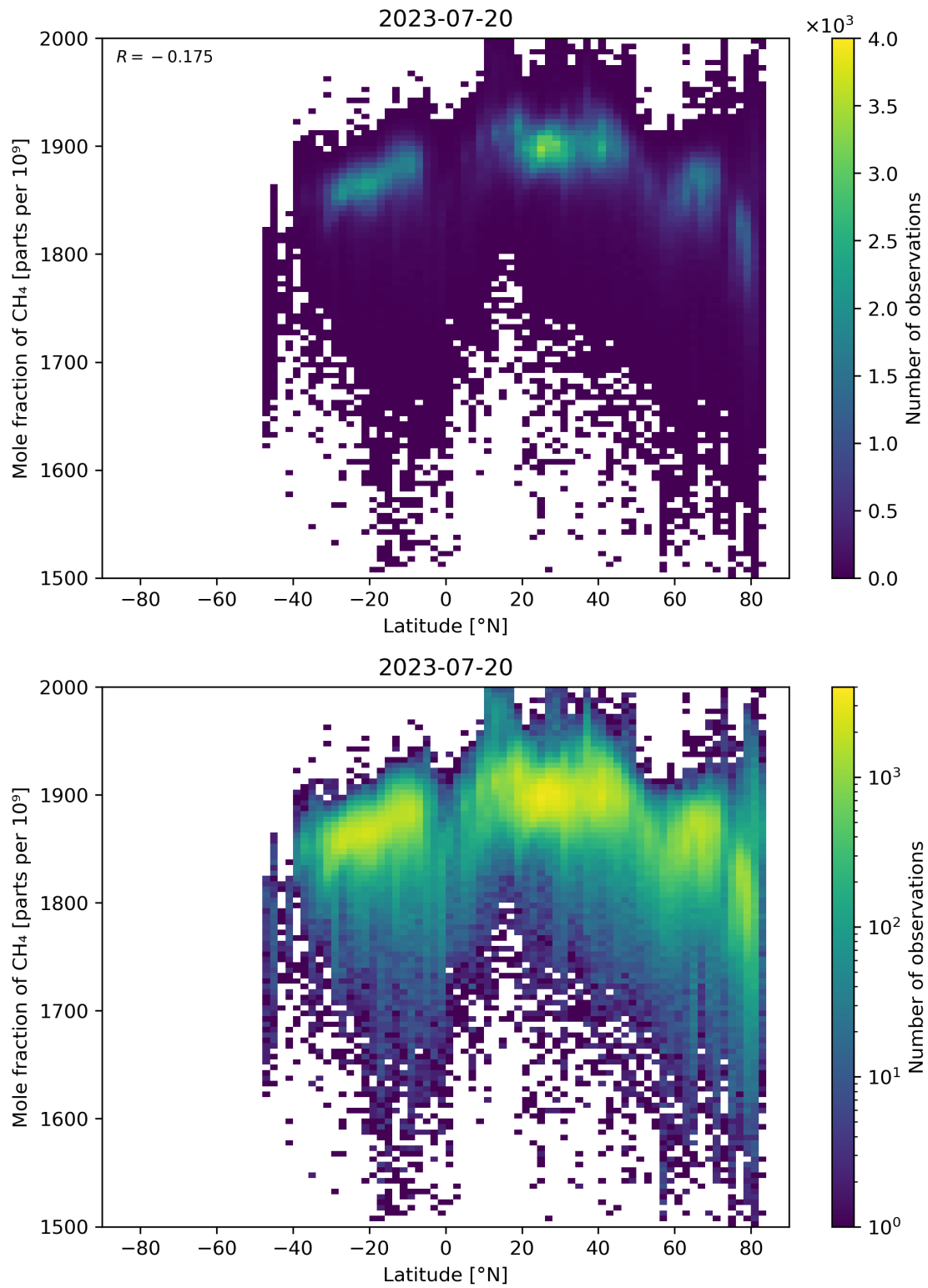
Figure 57: Scatter density plot of “Latitude” against “Mole fraction of CH 4 ” for 2023-07-19 to 2023-07-21.
