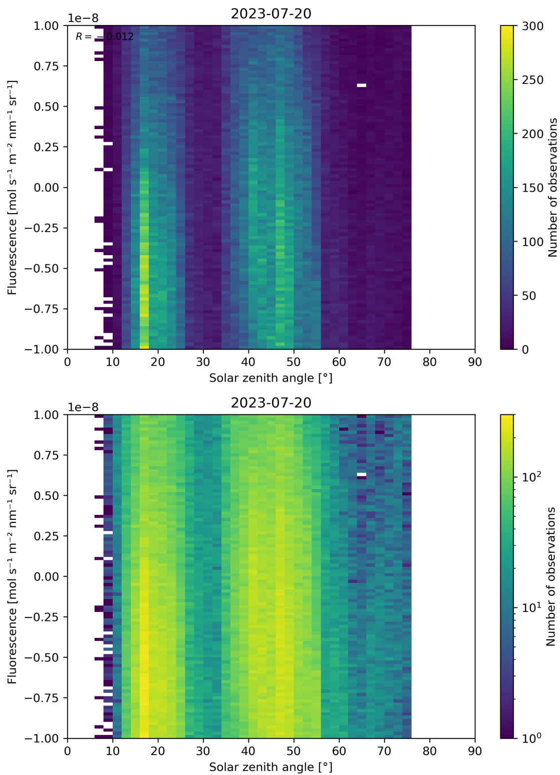
Figure 97: Scatter density plot of “Solar zenith angle” against “Fluorescence” for 2023-07-19 to 2023-07-21.
