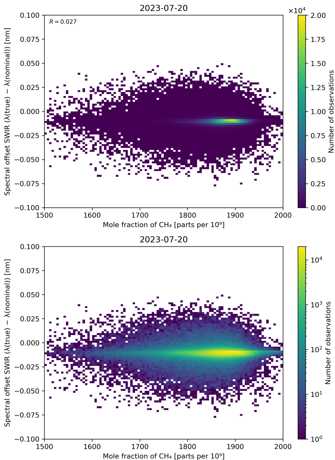
Figure 86: Scatter density plot of “Mole fraction of CH 4 ” against “Spectral offset SWIR ( \lambda(\text{true}) - \lambda(\text{nominal}) )” for 2023-07-19 to 2023-07-21.
