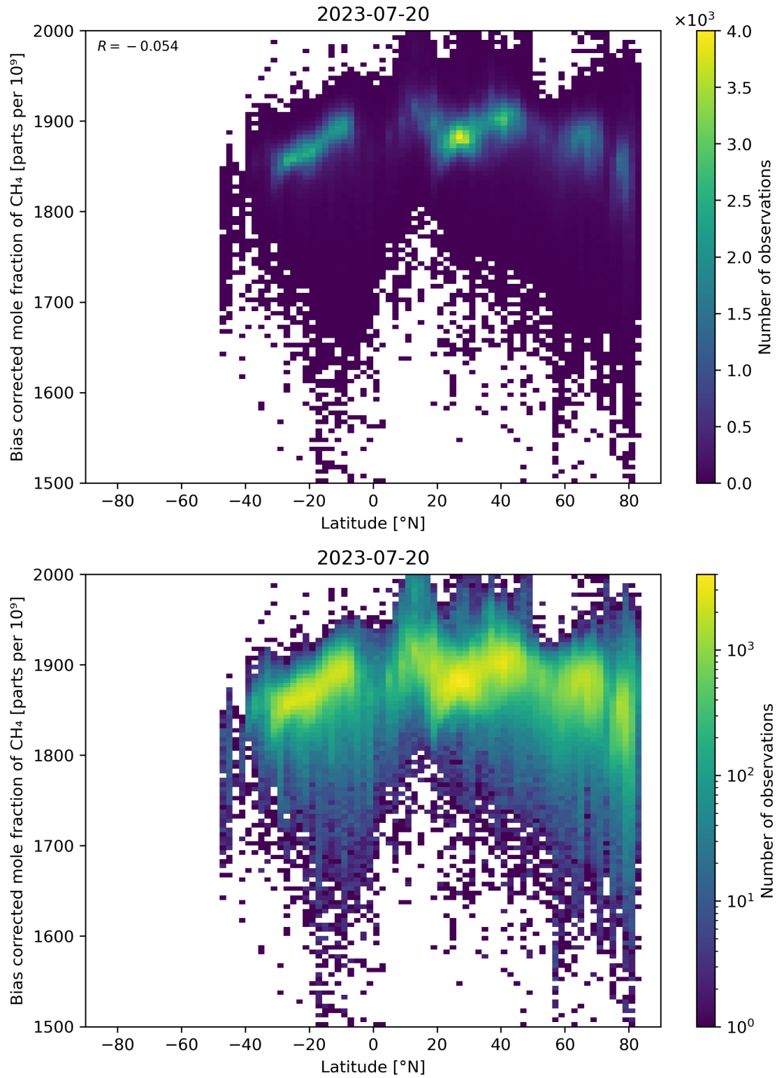
Figure 58: Scatter density plot of “Latitude” against “Bias corrected mole fraction of \text{CH}_4 ” for 2023-07-19 to 2023-07-21.
