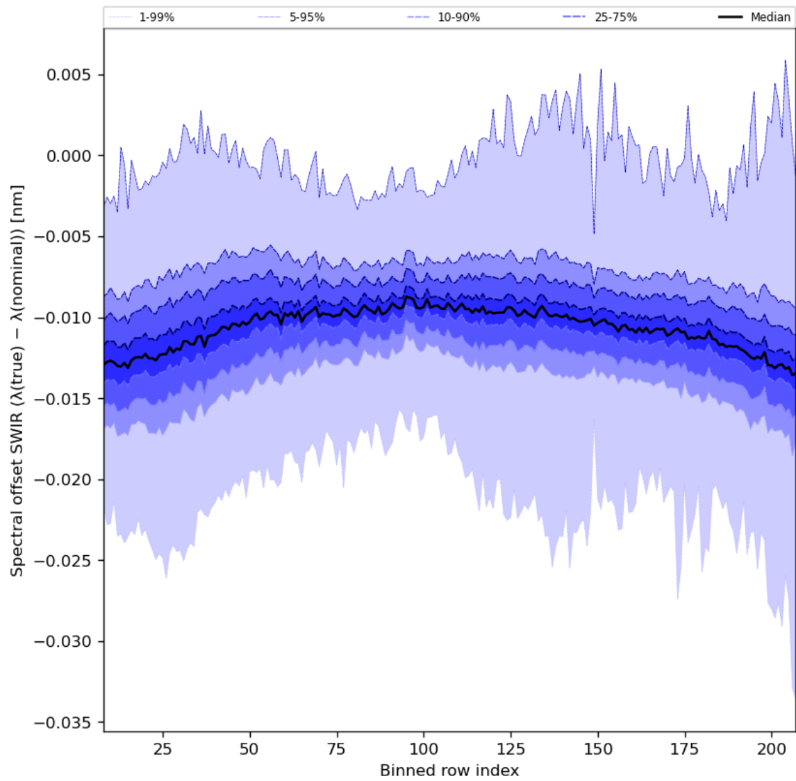
Figure 38: Along track statistics of “Spectral offset SWIR ( \lambda(\text{true}) - \lambda(\text{nominal}) )” for 2023-07-19 to 2023-07-21
