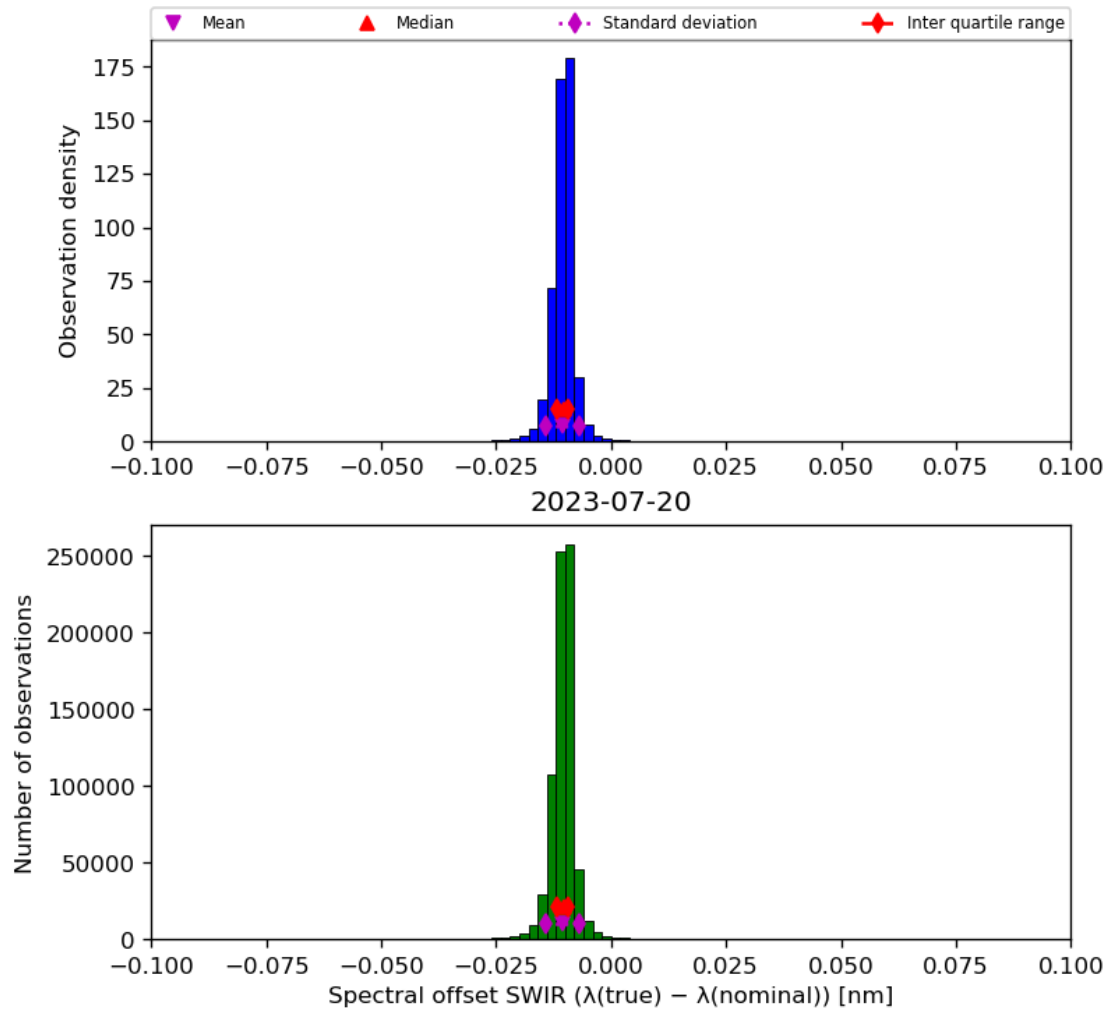
Figure 27: Histogram of “Spectral offset SWIR ( \lambda(\text{true}) - \lambda(\text{nominal}) )” for 2023-07-19 to 2023-07-21
