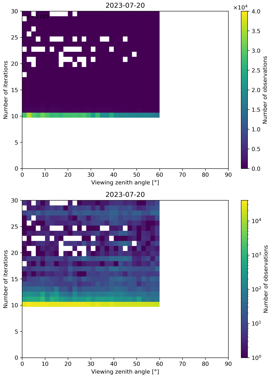
Figure 113: Scatter density plot of “Viewing zenith angle” against “Number of iterations” for 2023-07-19 to 2023-07-21.
