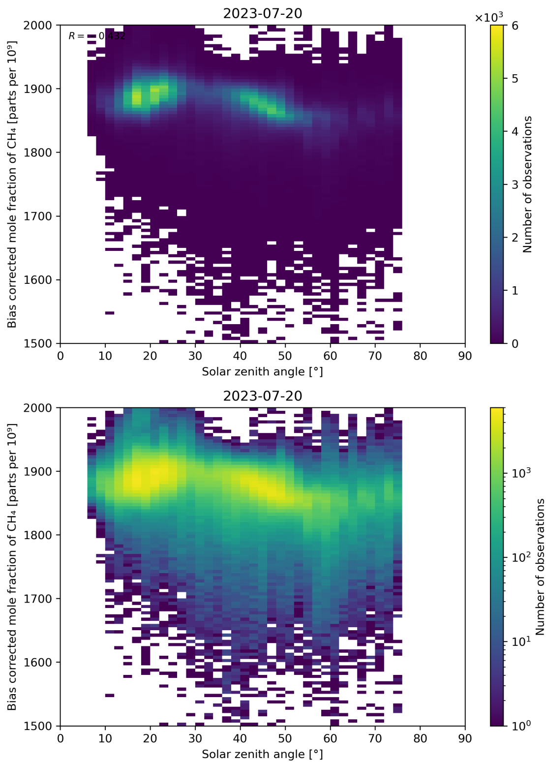
Figure 100: Scatter density plot of “Solar zenith angle” against “Bias corrected mole fraction of CH 4 ” for 2023-07-19 to 2023-07-21.
