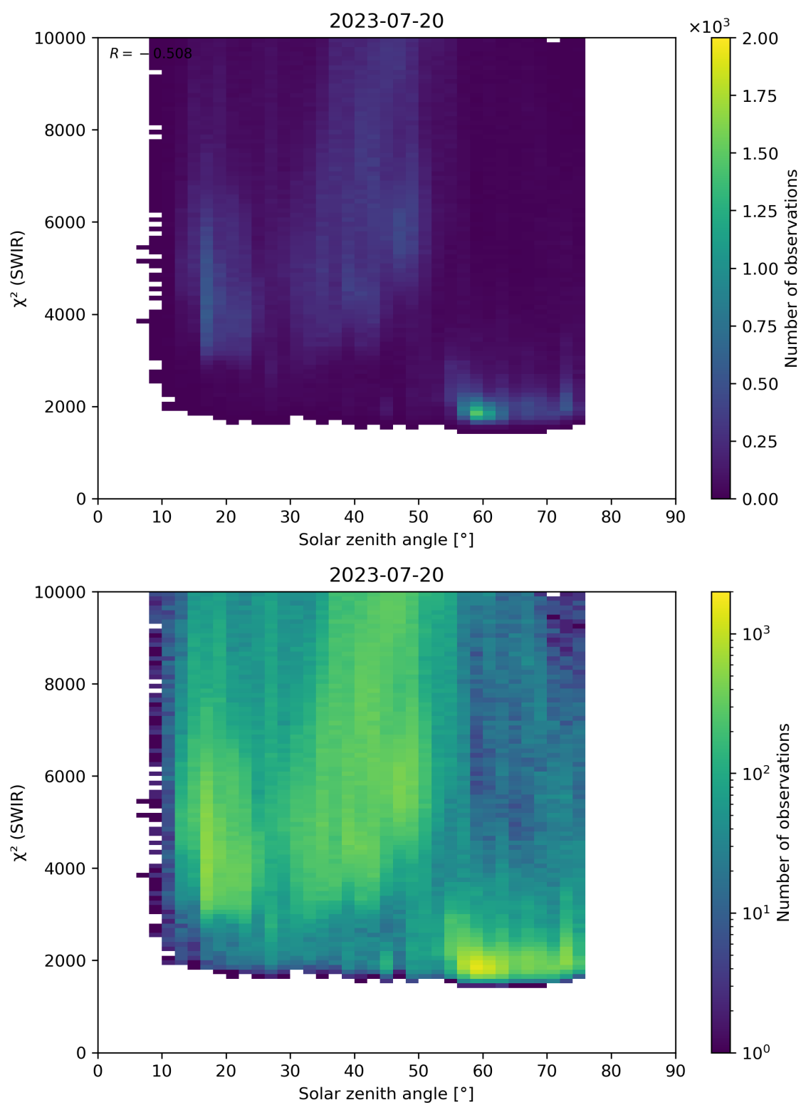
Figure 95: Scatter density plot of “Solar zenith angle” against “ \chi^2 (SWIR)” for 2023-07-19 to 2023-07-21.
