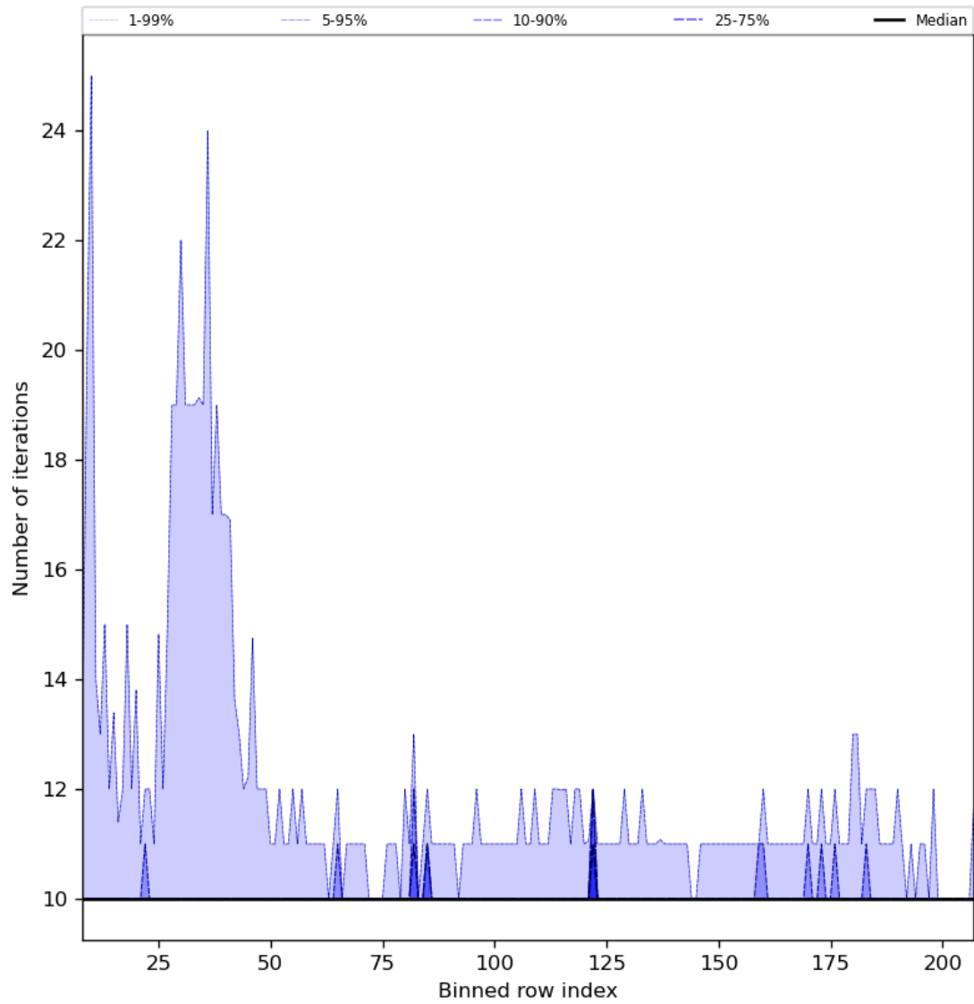
Figure 42: Along track statistics of “Number of iterations” for 2023-07-19 to 2023-07-21
