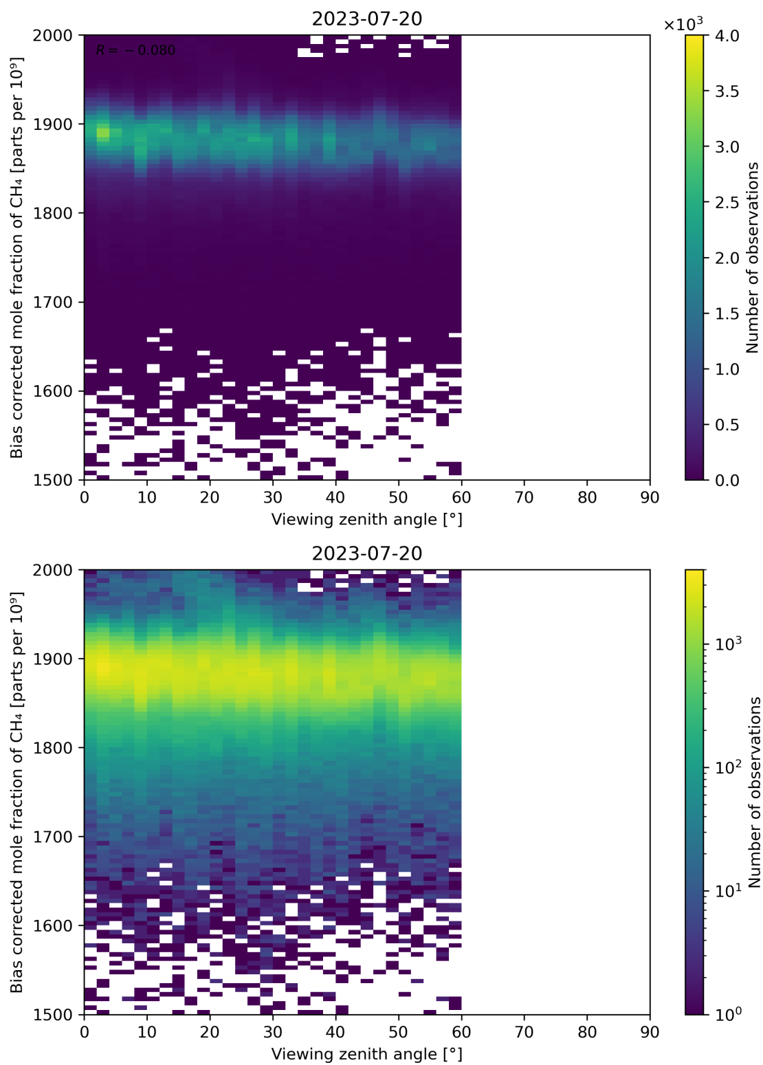
Figure 111: Scatter density plot of “Viewing zenith angle” against “Bias corrected mole fraction of CH 4 ” for 2023-07-19 to 2023-07-21.
