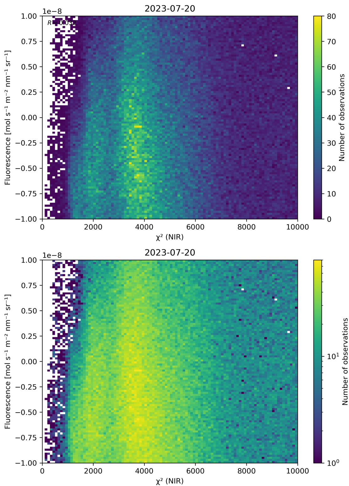
Figure 45: Scatter density plot of “ \chi^2 (NIR)” against “Fluorescence” for 2023-07-19 to 2023-07-21.
