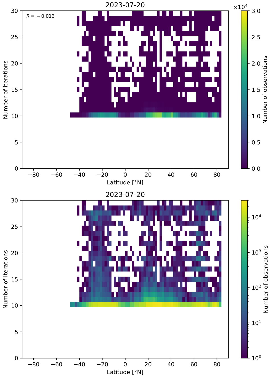
Figure 60: Scatter density plot of “Latitude” against “Number of iterations” for 2023-07-19 to 2023-07-21.
