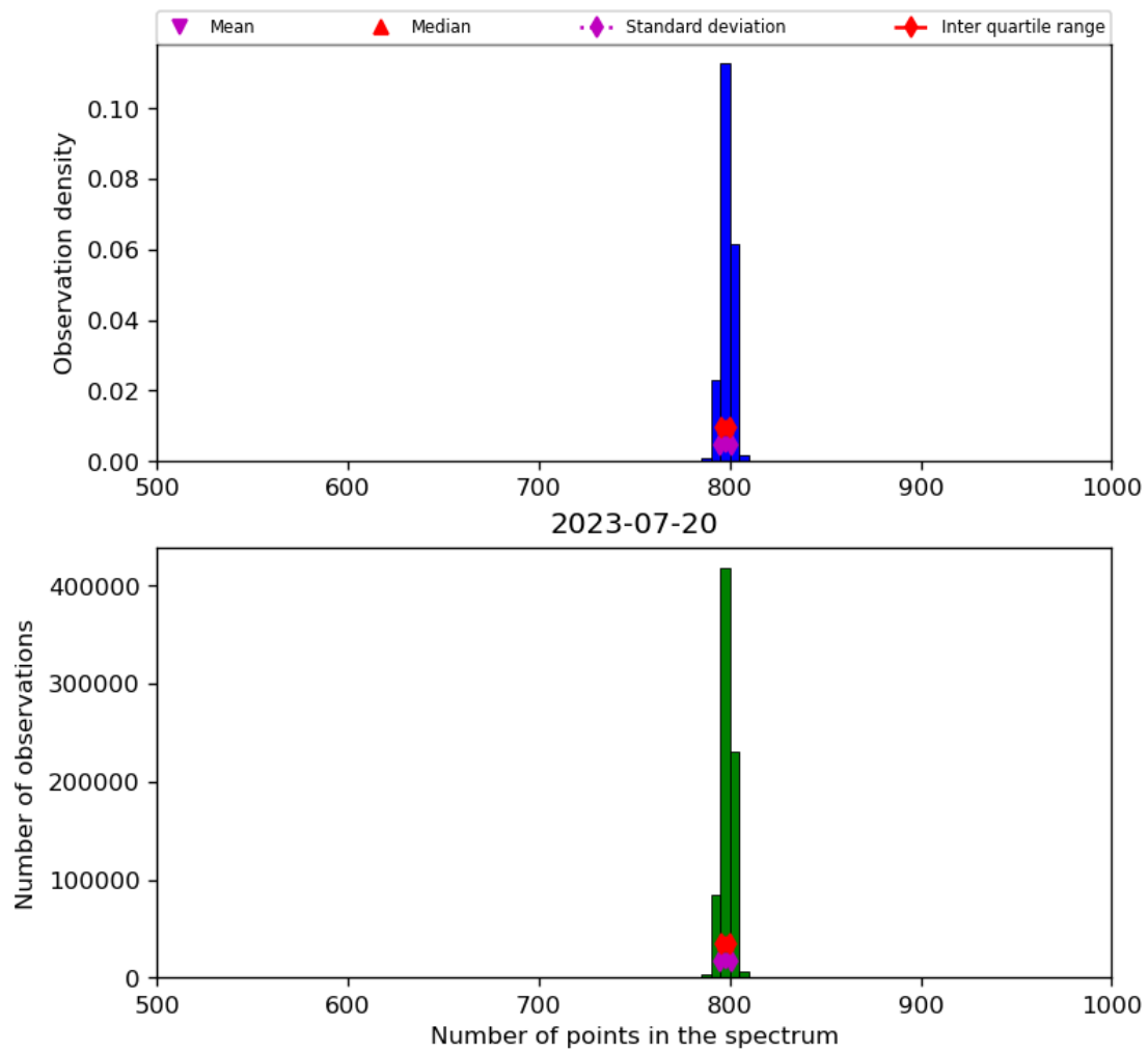
Figure 26: Histogram of “Number of points in the spectrum” for 2023-07-19 to 2023-07-21
