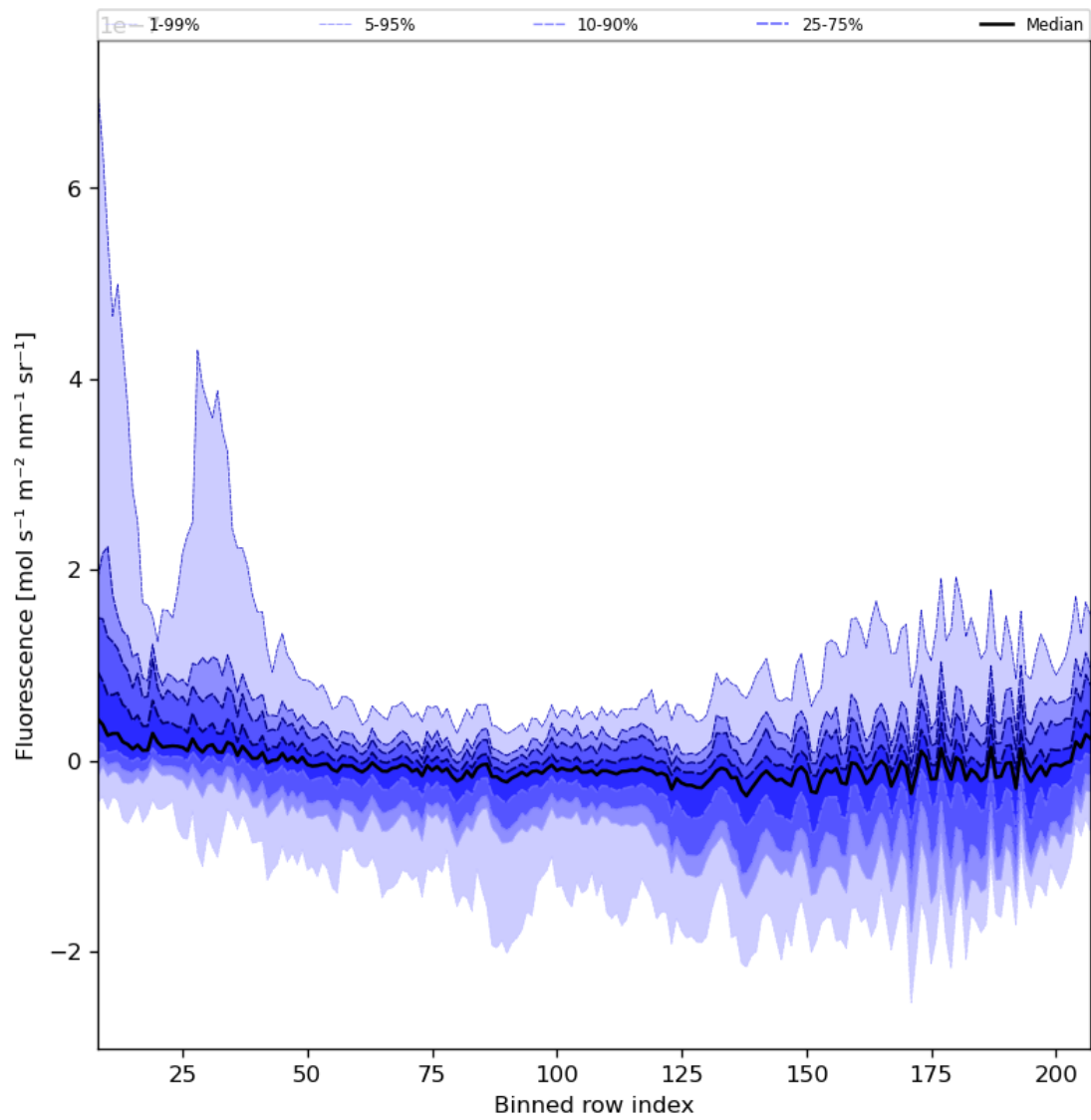
Figure 43: Along track statistics of “Fluorescence” for 2023-07-19 to 2023-07-21
