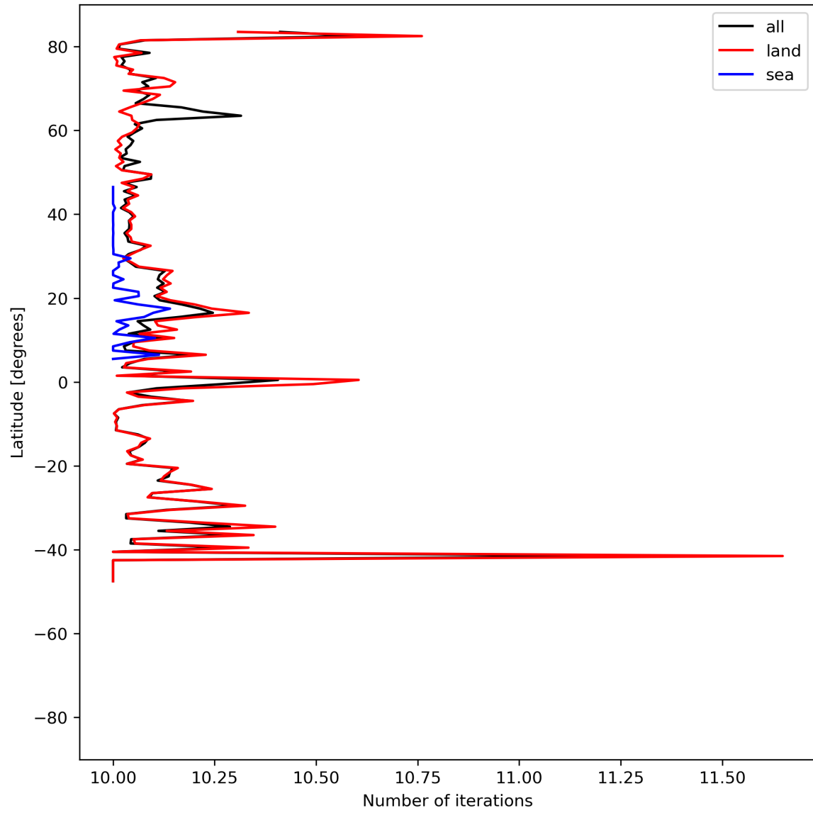
Figure 20: Zonal average of “Number of iterations” for 2023-07-19 to 2023-07-21.
