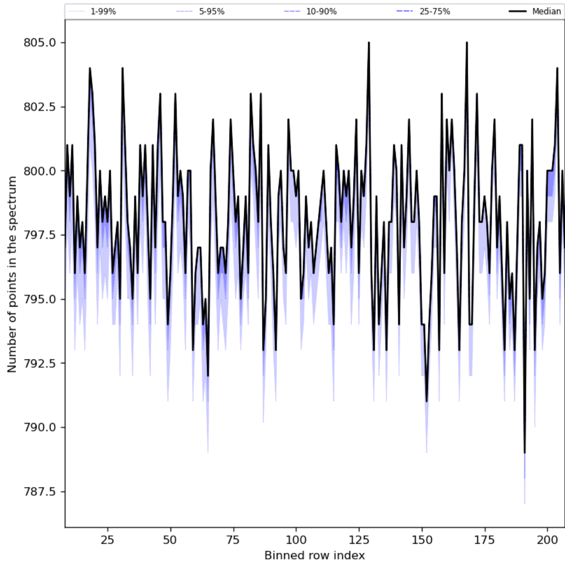
Figure 37: Along track statistics of “Number of points in the spectrum” for 2023-07-19 to 2023-07-21
