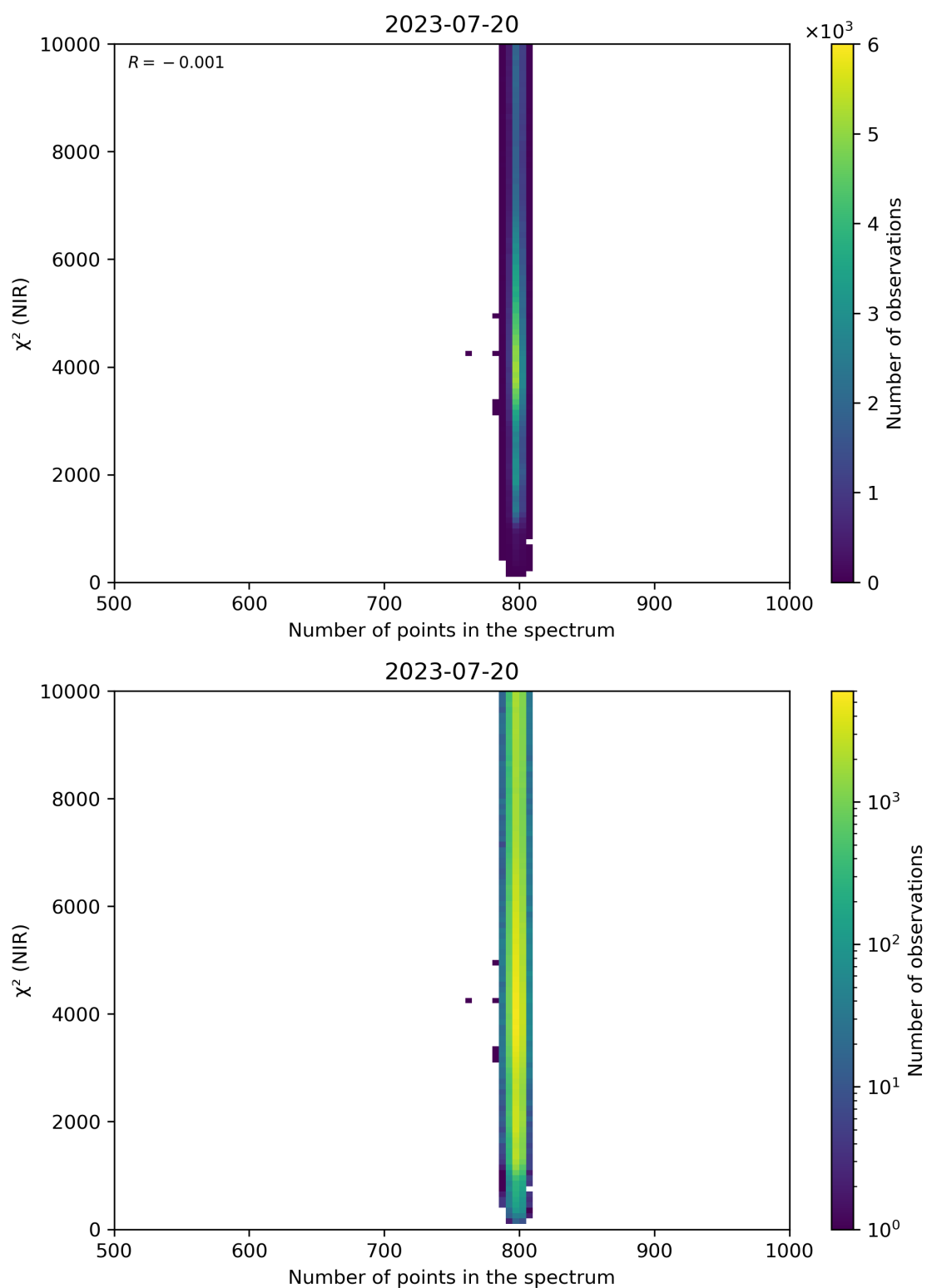
Figure 88: Scatter density plot of “Number of points in the spectrum” against “ \chi^2 (NIR)” for 2023-07-19 to 2023-07-21.
