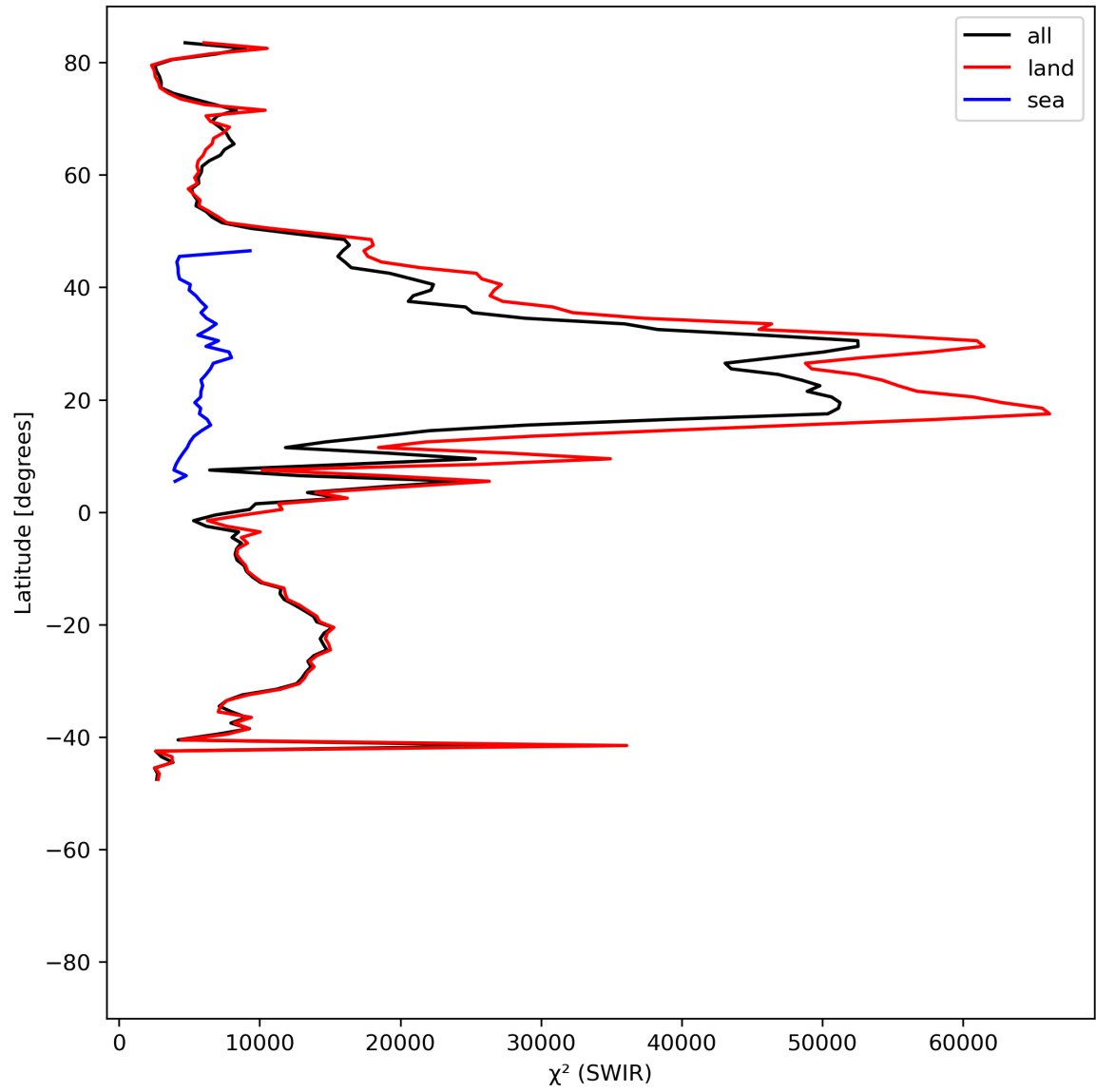
Figure 17: Zonal average of “ \chi^2 (SWIR)” for 2023-07-19 to 2023-07-21.
