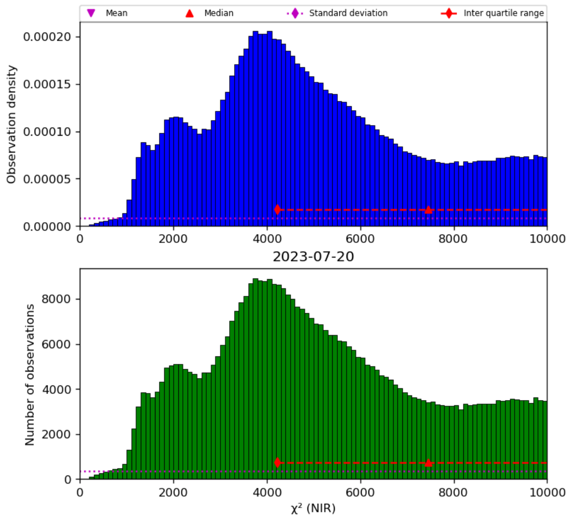
Figure 29: Histogram of “ \chi^2 (NIR)” for 2023-07-19 to 2023-07-21
