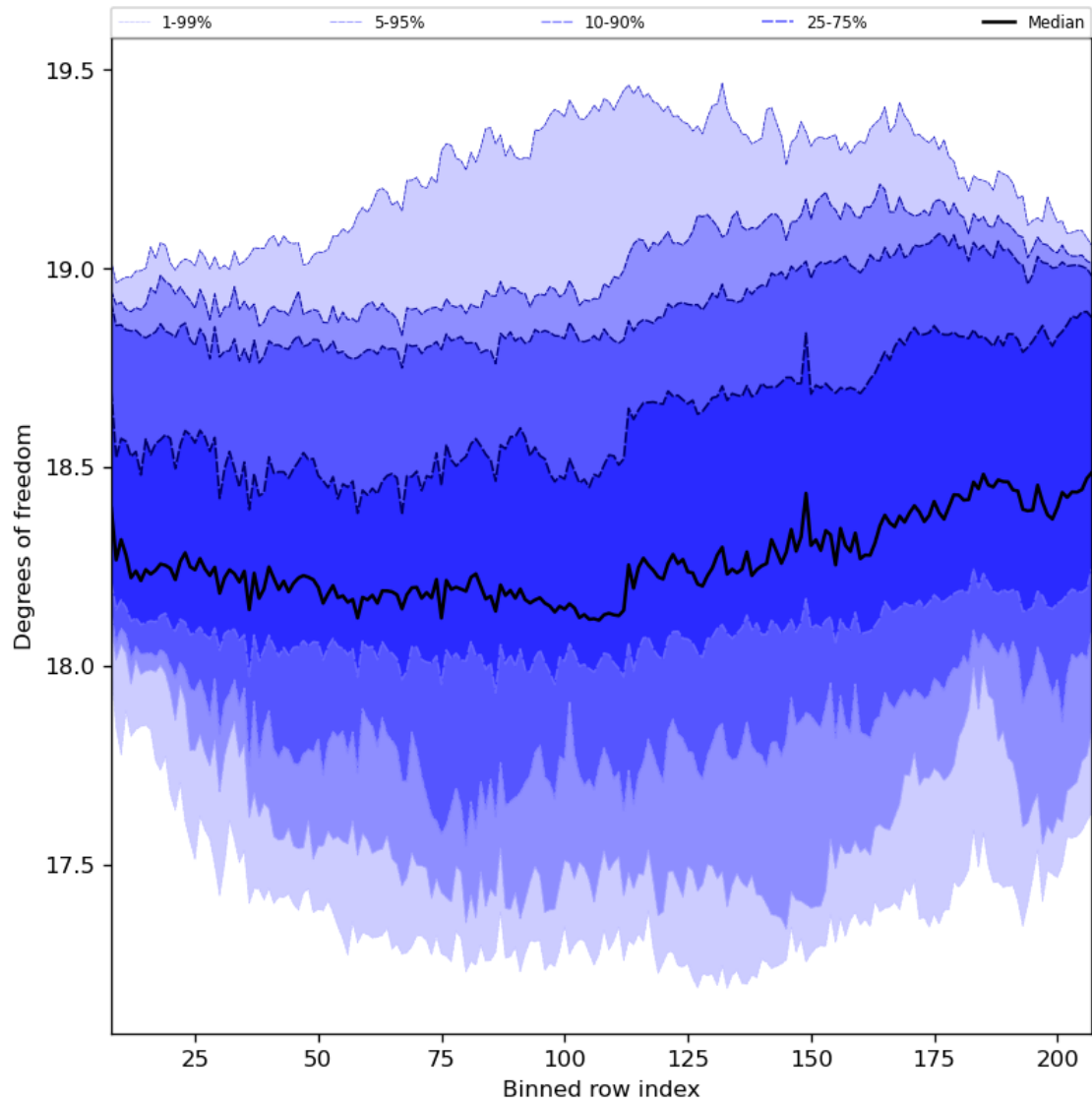
Figure 41: Along track statistics of “Degrees of freedom” for 2023-07-19 to 2023-07-21
