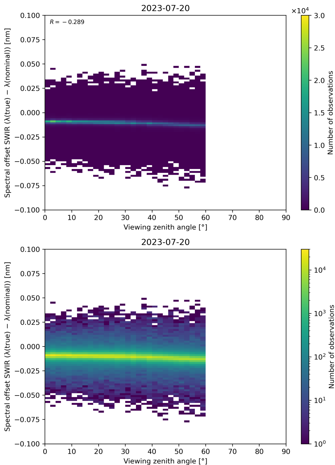
Figure 116: Scatter density plot of “Viewing zenith angle” against “Spectral offset SWIR ( \lambda(\text{true}) - \lambda(\text{nominal}) )” for 2023-07-19 to 2023-07-21.
