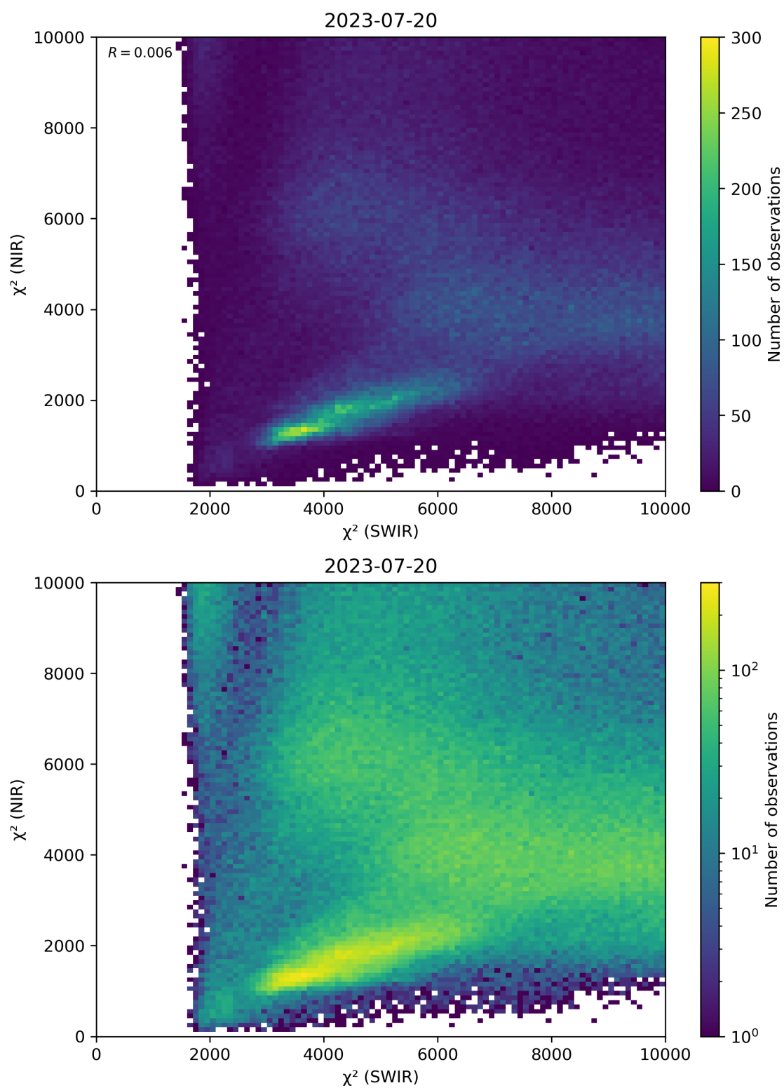
Figure 47: Scatter density plot of “ \chi^2 (SWIR)” against “ \chi^2 (NIR)” for 2023-07-19 to 2023-07-21.
