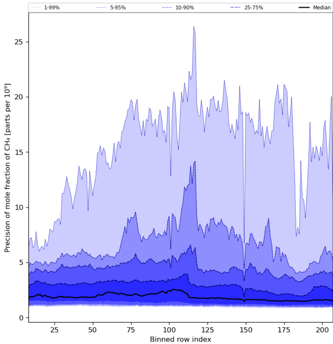
Figure 35: Along track statistics of “Precision of mole fraction of CH 4 ” for 2023-07-19 to 2023-07-21
