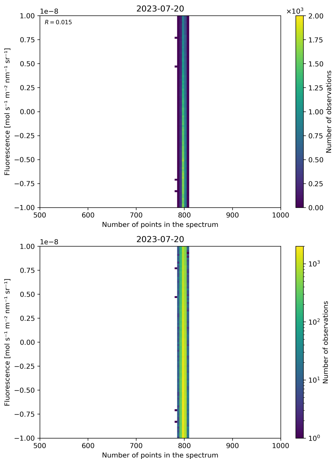
Figure 91: Scatter density plot of “Number of points in the spectrum” against “Fluorescence” for 2023-07-19 to 2023-07-21.
