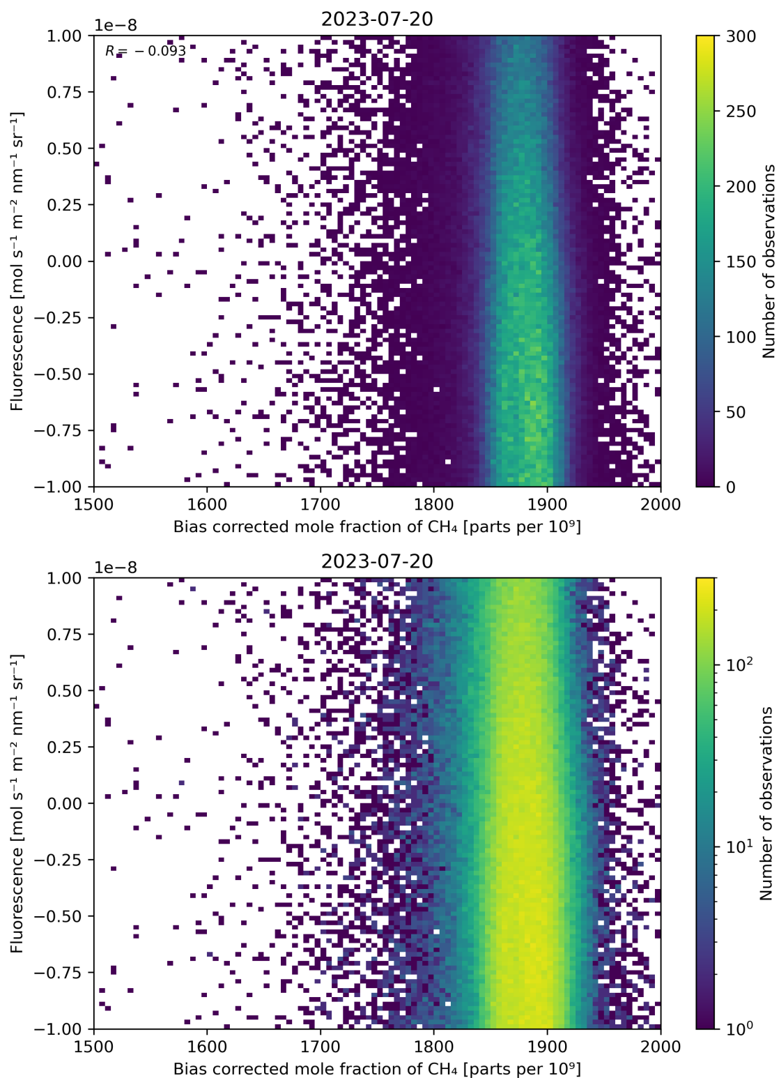
Figure 66: Scatter density plot of “Bias corrected mole fraction of CH 4 ” against “Fluorescence” for 2023-07-19 to 2023-07-21.
