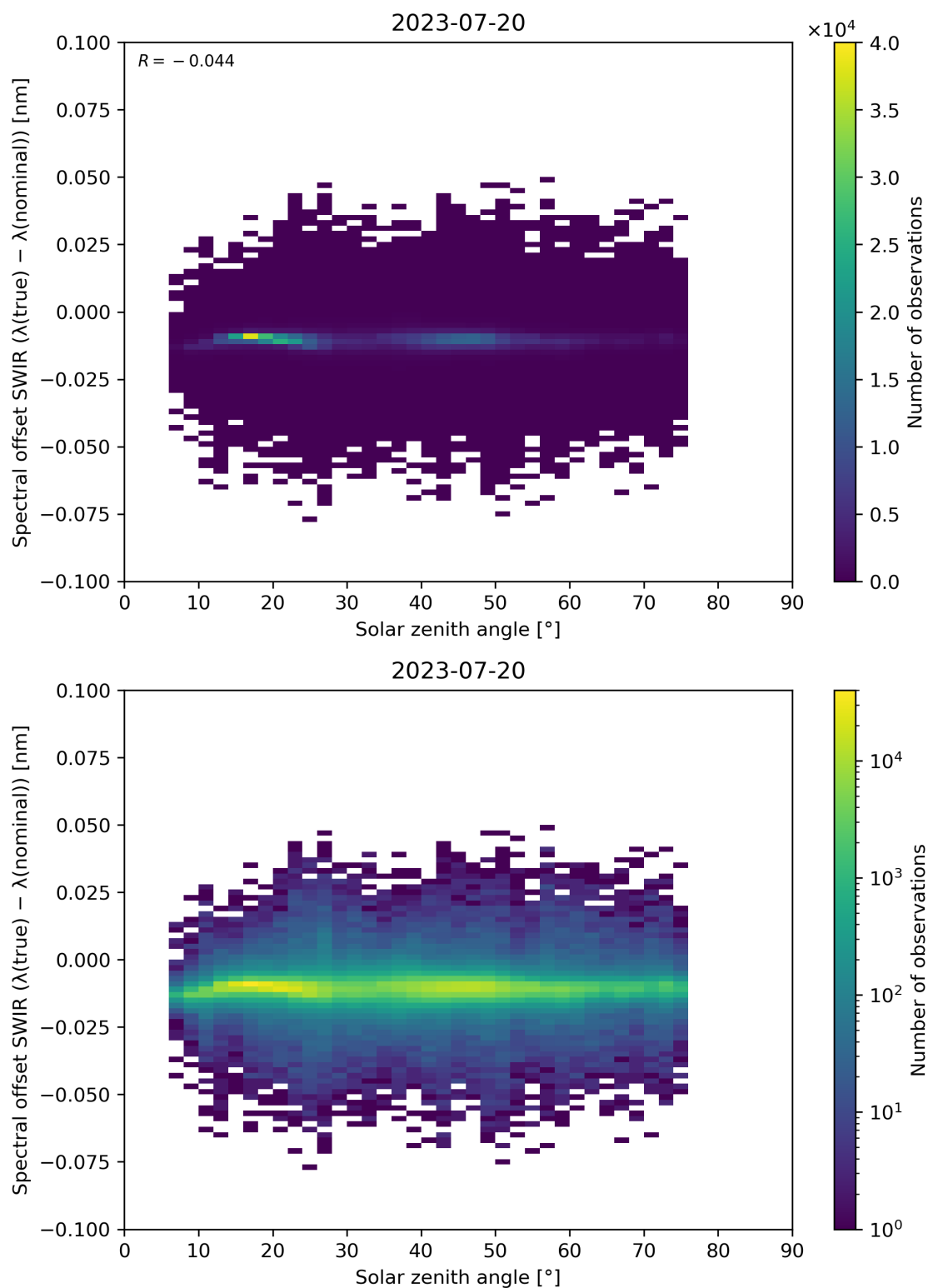
Figure 104: Scatter density plot of “Solar zenith angle” against “Spectral offset SWIR ( \lambda(\text{true}) - \lambda(\text{nominal}) )” for 2023-07-19 to 2023-07-21.
