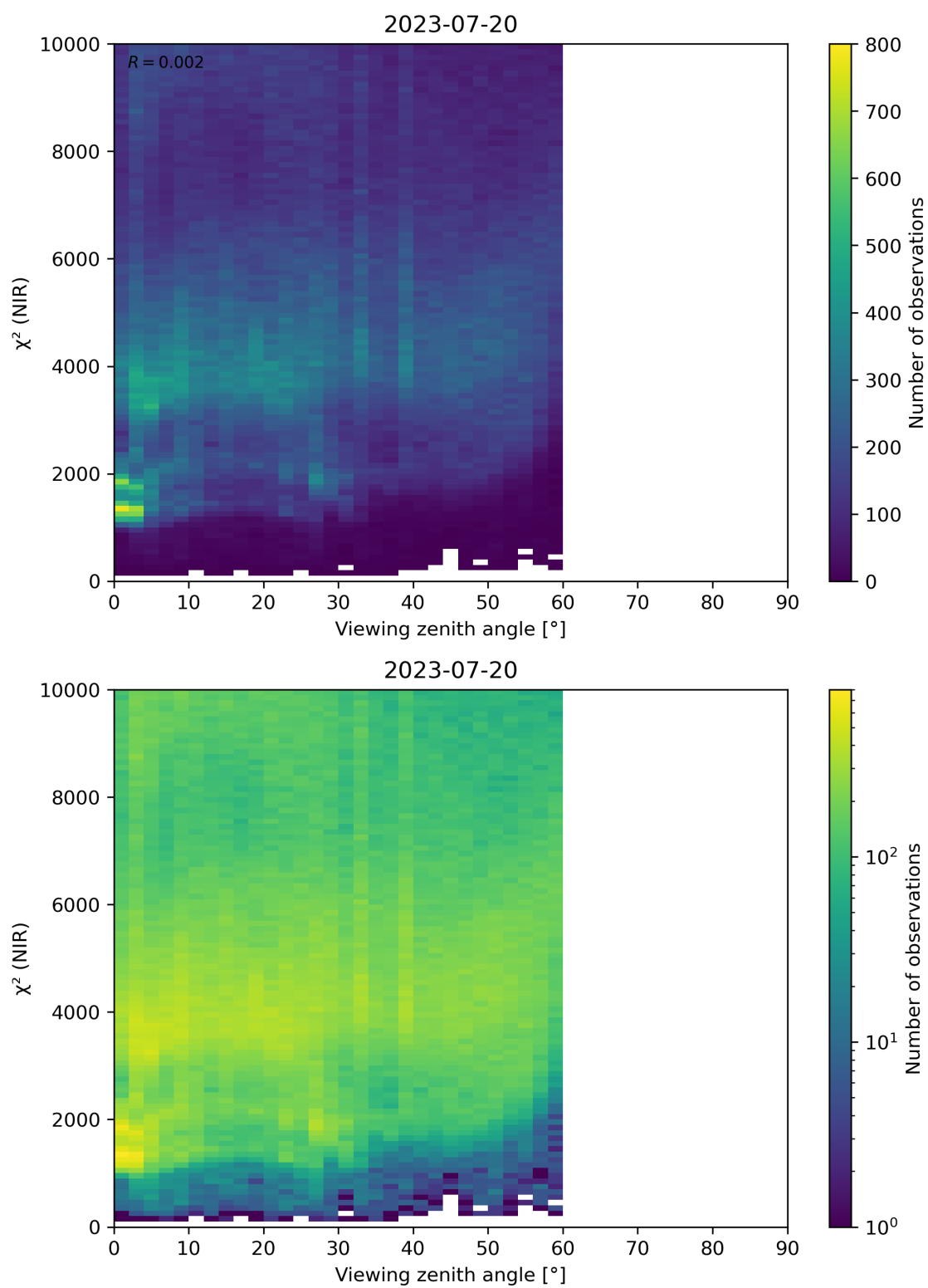
Figure 105: Scatter density plot of “Viewing zenith angle” against “ \chi^2 (NIR)” for 2023-07-19 to 2023-07-21.
