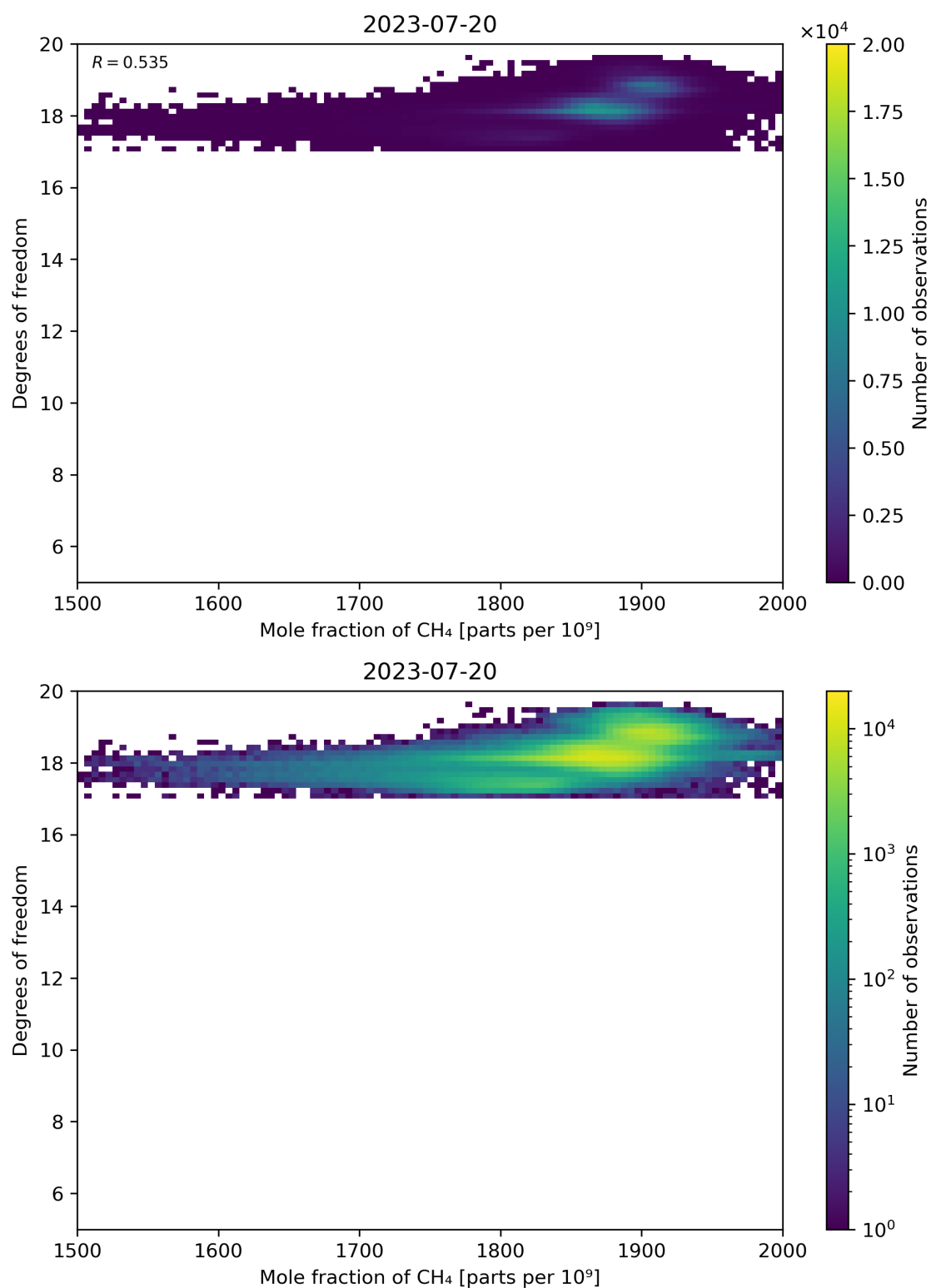
Figure 72: Scatter density plot of “Mole fraction of CH 4 ” against “Degrees of freedom” for 2023-07-19 to 2023-07-21.
