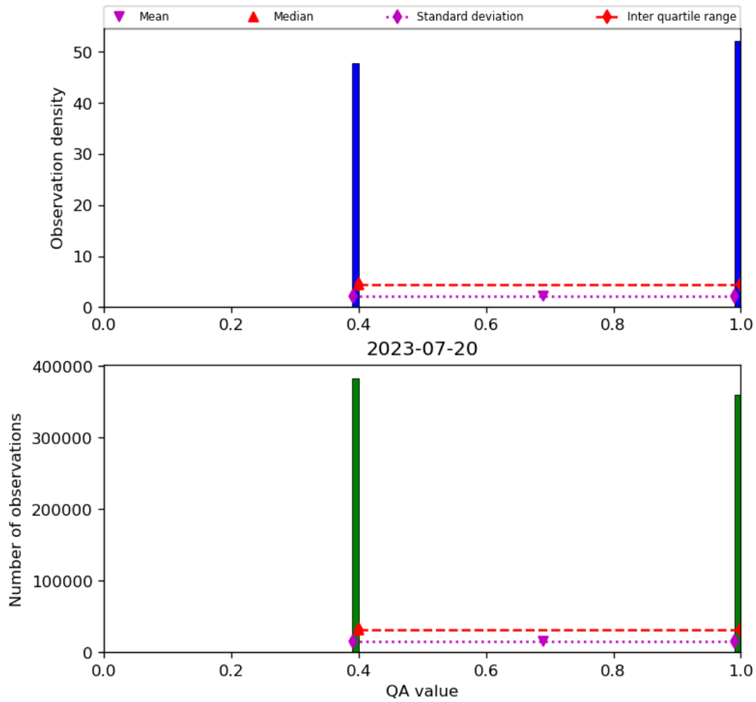
Figure 22: Histogram of “QA value” for 2023-07-19 to 2023-07-21
