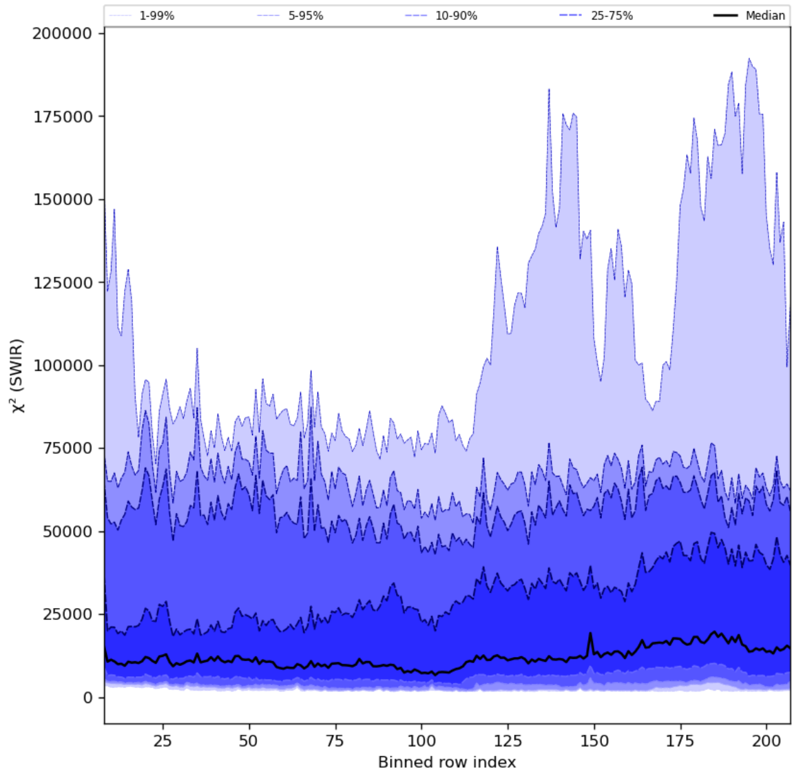
Figure 39: Along track statistics of " \chi^2 (SWIR)" for 2023-07-19 to 2023-07-21
