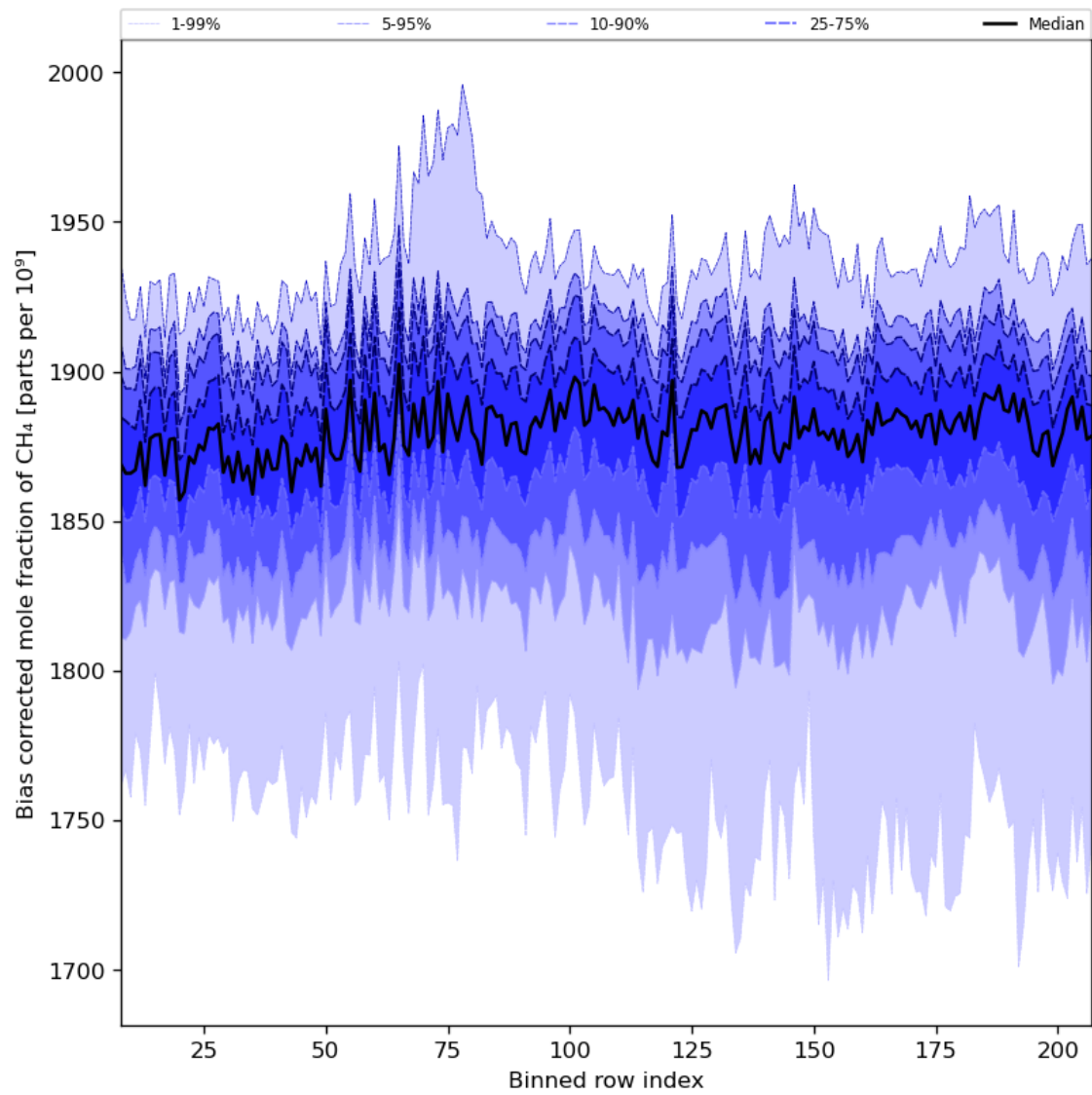
Figure 36: Along track statistics of “Bias corrected mole fraction of CH 4 ” for 2023-07-19 to 2023-07-21
