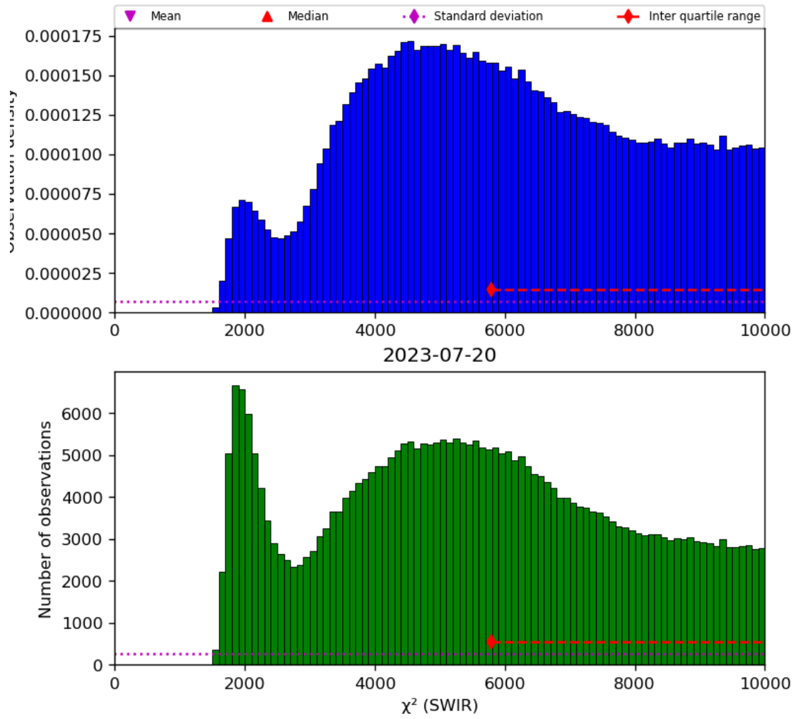
Figure 28: Histogram of “ \chi^2 (SWIR)” for 2023-07-19 to 2023-07-21
