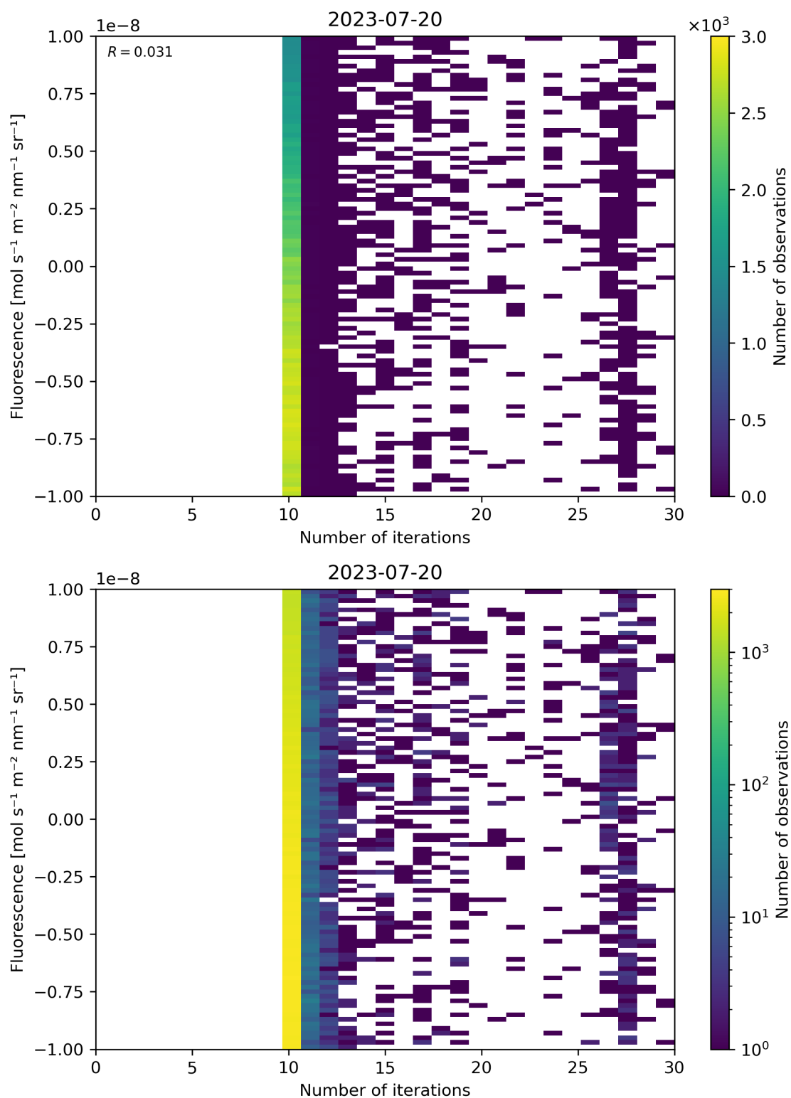
Figure 87: Scatter density plot of “Number of iterations” against “Fluorescence” for 2023-07-19 to 2023-07-21.
