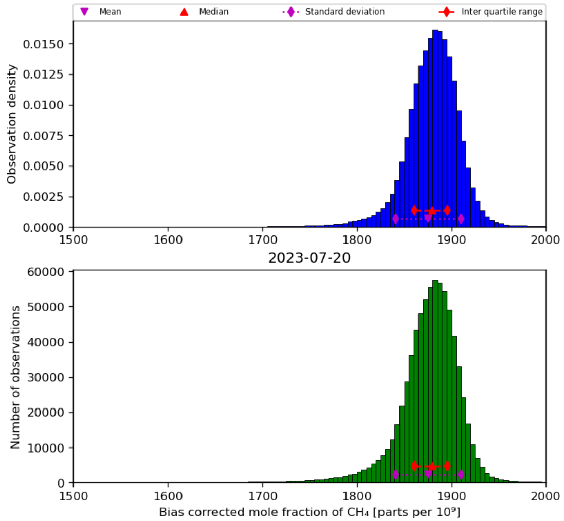
Figure 25: Histogram of “Bias corrected mole fraction of CH 4 ” for 2023-07-19 to 2023-07-21
