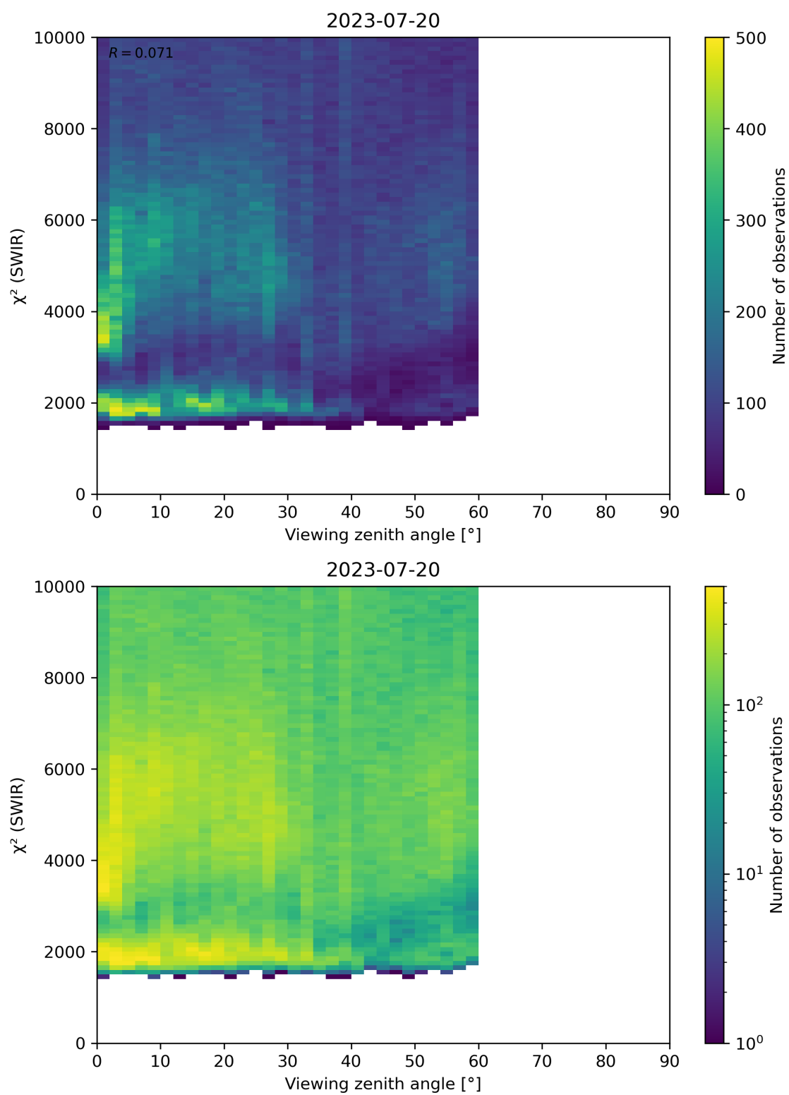
Figure 106: Scatter density plot of “Viewing zenith angle” against “ \chi^2 (SWIR)” for 2023-07-19 to 2023-07-21.
