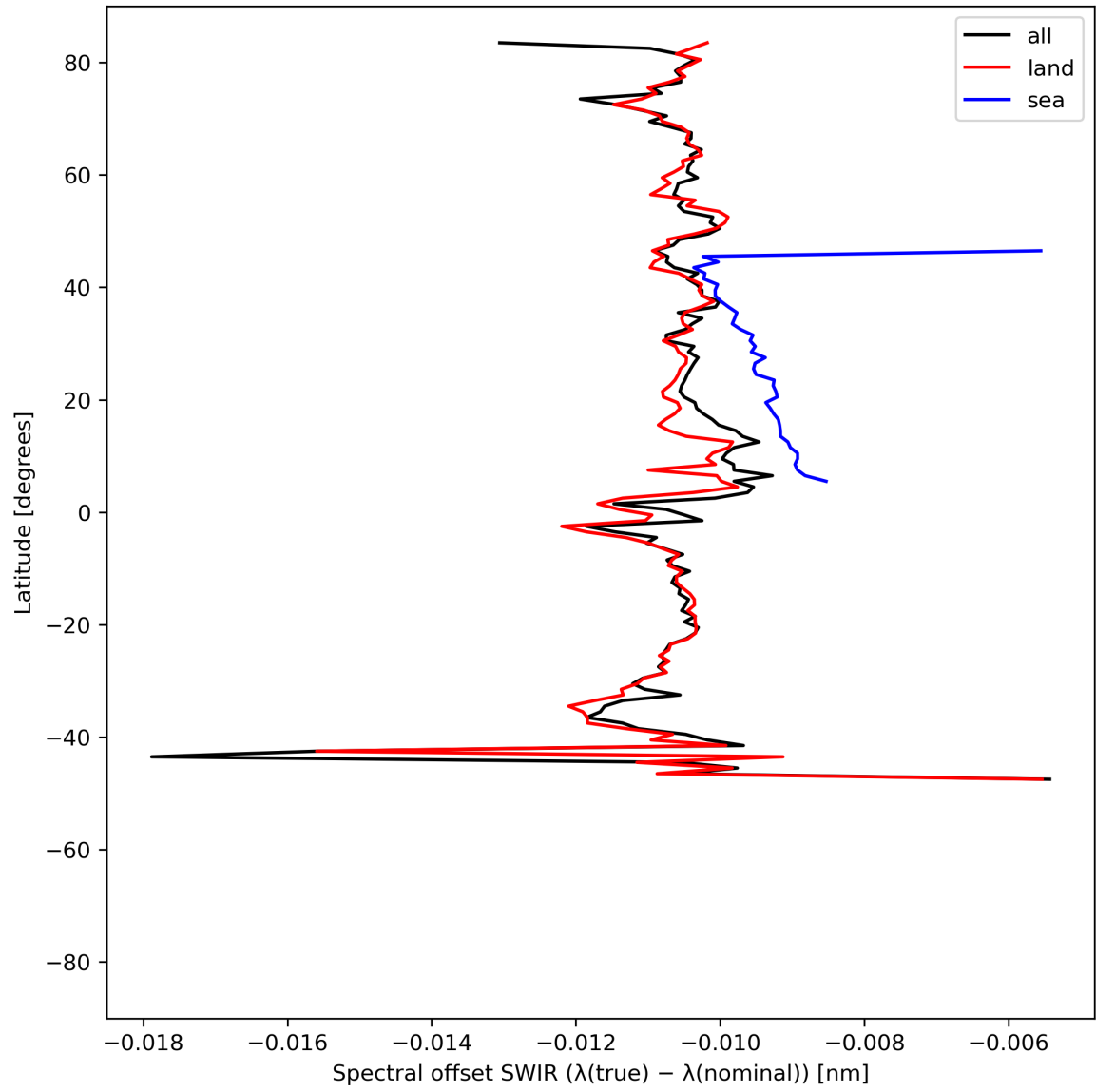
Figure 16: Zonal average of “Spectral offset SWIR ( \lambda(\text{true}) - \lambda(\text{nominal}) )” for 2023-07-19 to 2023-07-21.
