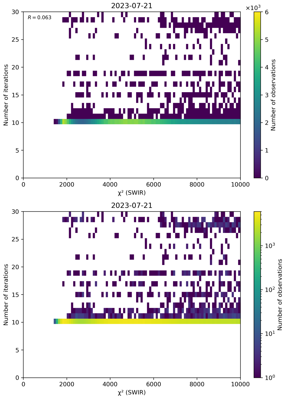
Figure 50: Scatter density plot of “ \chi^2 (SWIR)” against “Number of iterations” for 2023-07-20 to 2023-07-22.
