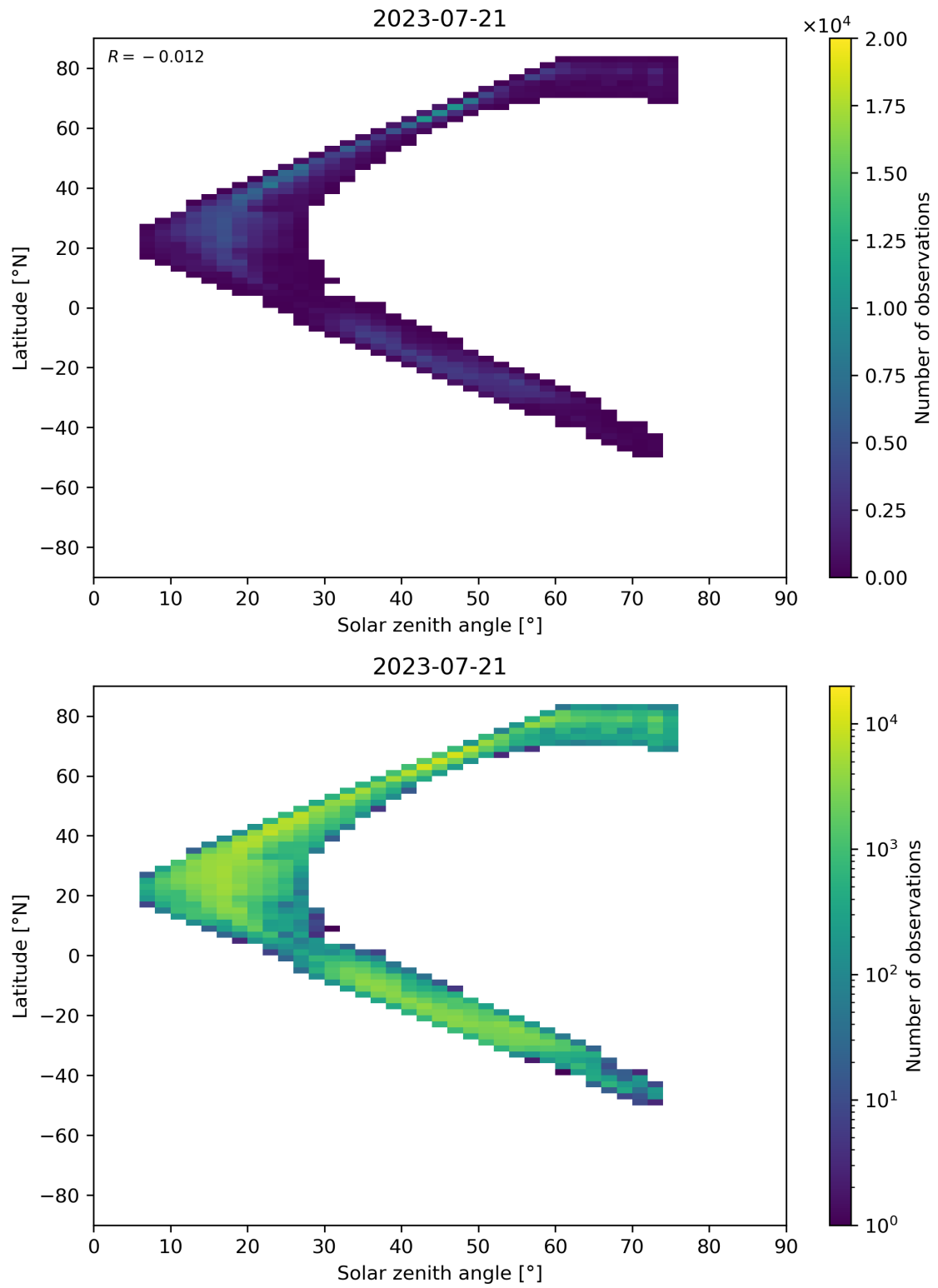
Figure 98: Scatter density plot of “Solar zenith angle” against “Latitude” for 2023-07-20 to 2023-07-22.
