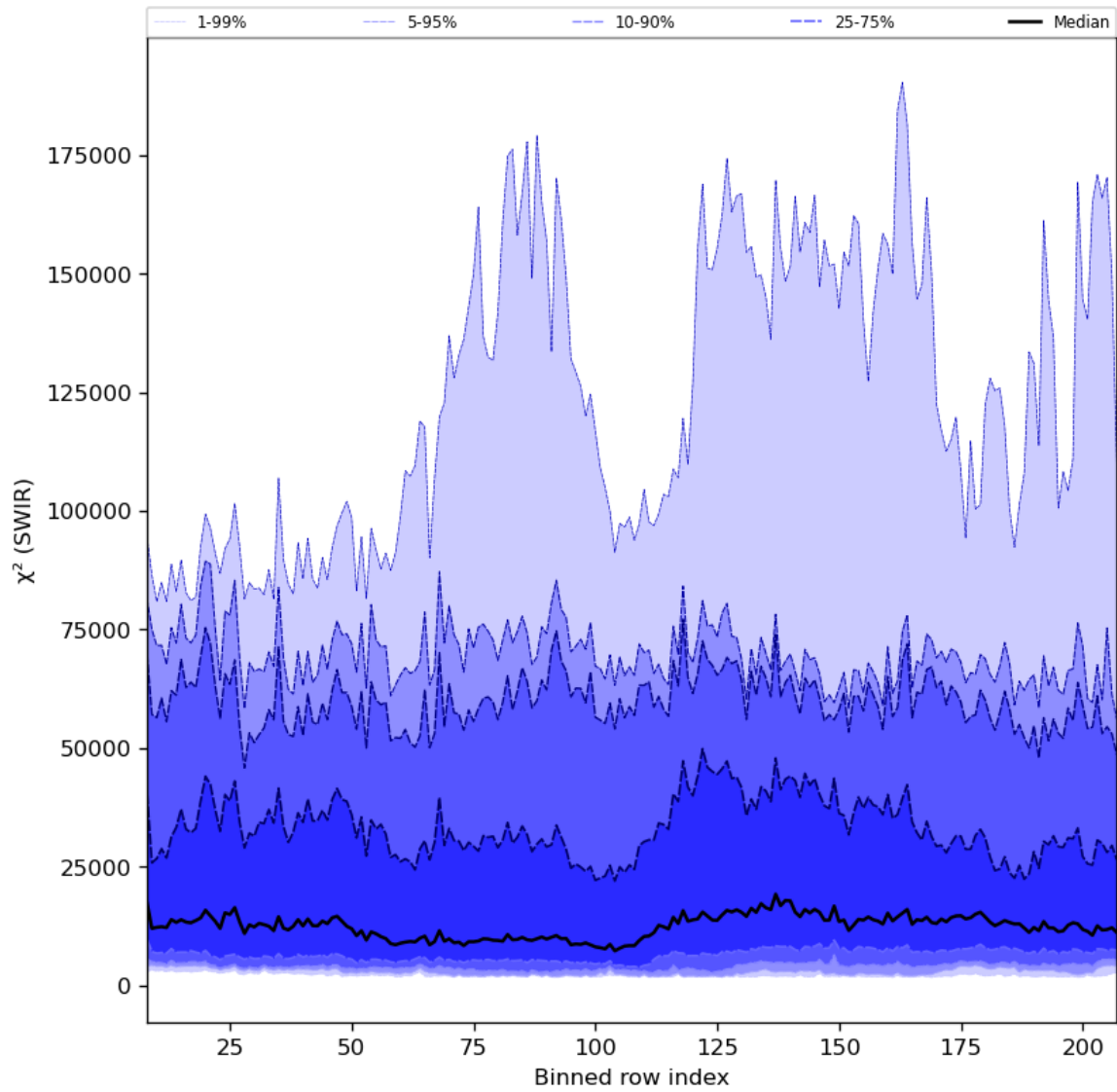
Figure 39: Along track statistics of “ \chi^2 (SWIR)” for 2023-07-20 to 2023-07-22
