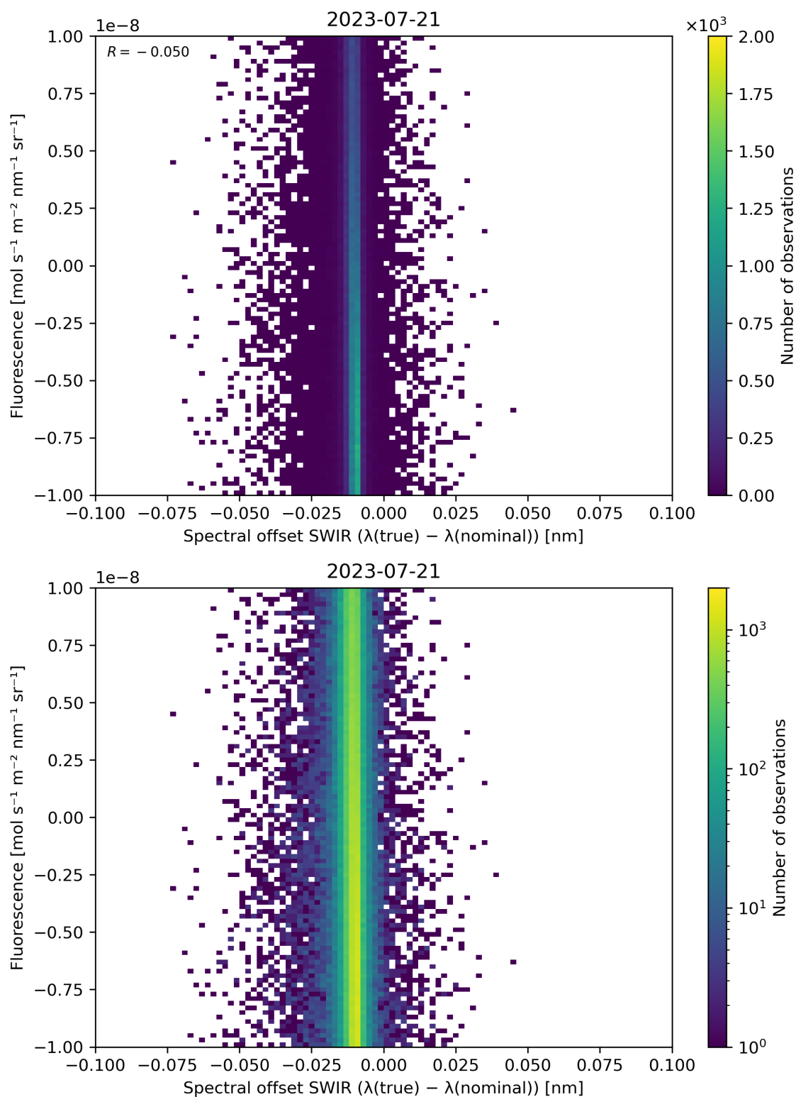
Figure 120: Scatter density plot of “Spectral offset SWIR ( \lambda(\text{true}) - \lambda(\text{nominal}) )” against “Fluorescence” for 2023-07-20 to 2023-07-22.
