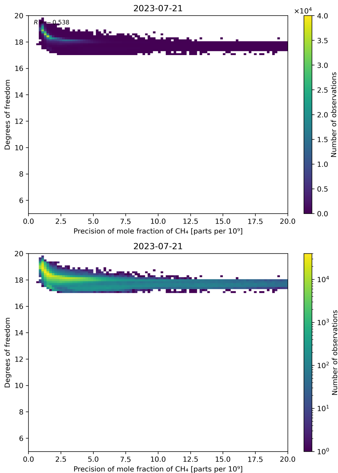
Figure 80: Scatter density plot of “Precision of mole fraction of CH 4 ” against “Degrees of freedom” for 2023-07-20 to 2023-07-22.
