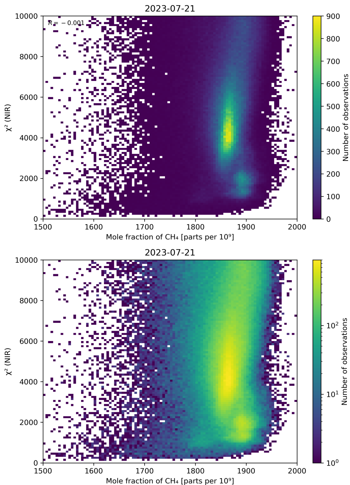
Figure 70: Scatter density plot of “Mole fraction of CH 4 ” against “ \chi^2 (NIR)” for 2023-07-20 to 2023-07-22.
