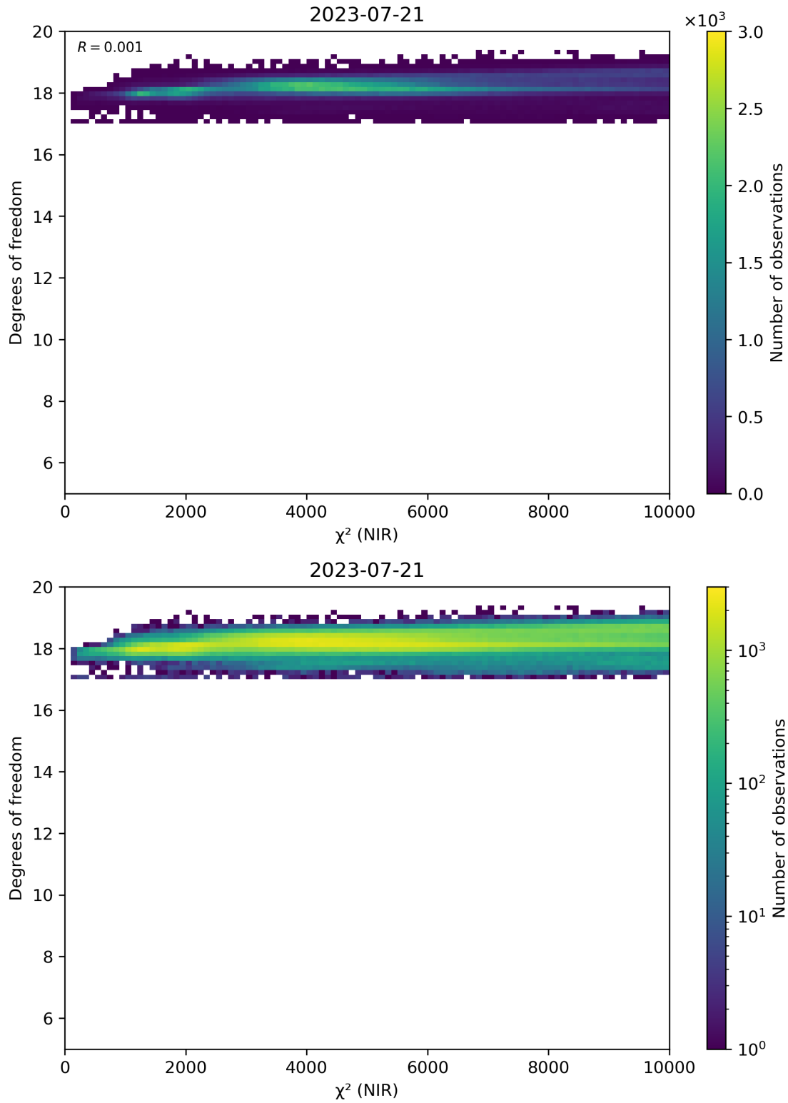
Figure 44: Scatter density plot of “ \chi^2 (NIR)” against “Degrees of freedom” for 2023-07-20 to 2023-07-22.
