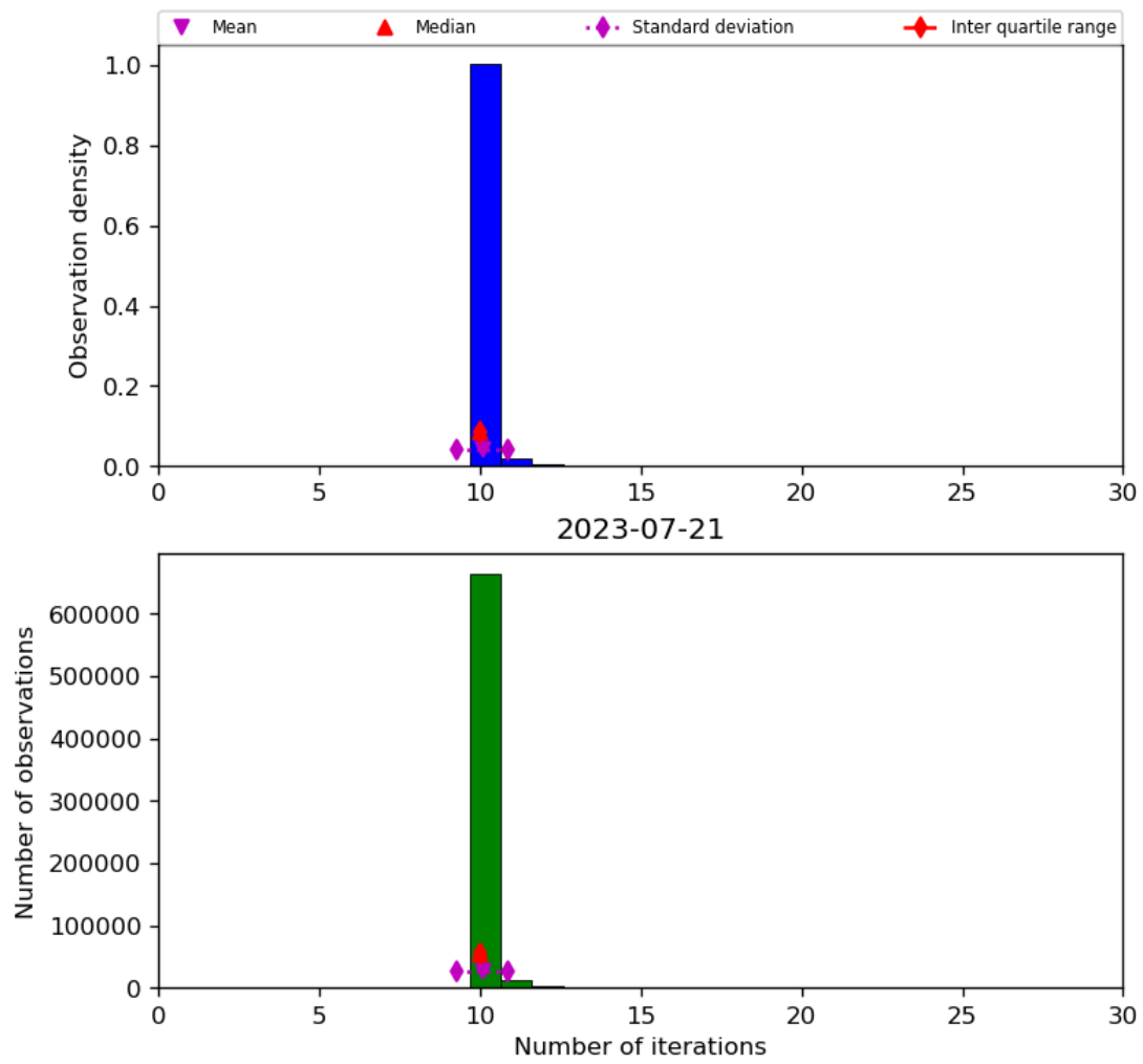
Figure 31: Histogram of “Number of iterations” for 2023-07-20 to 2023-07-22
