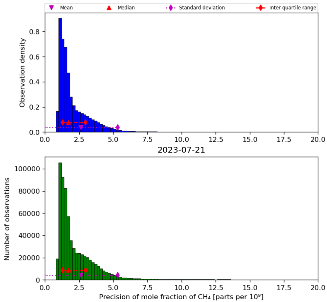
Figure 24: Histogram of “Precision of mole fraction of CH 4 ” for 2023-07-20 to 2023-07-22
