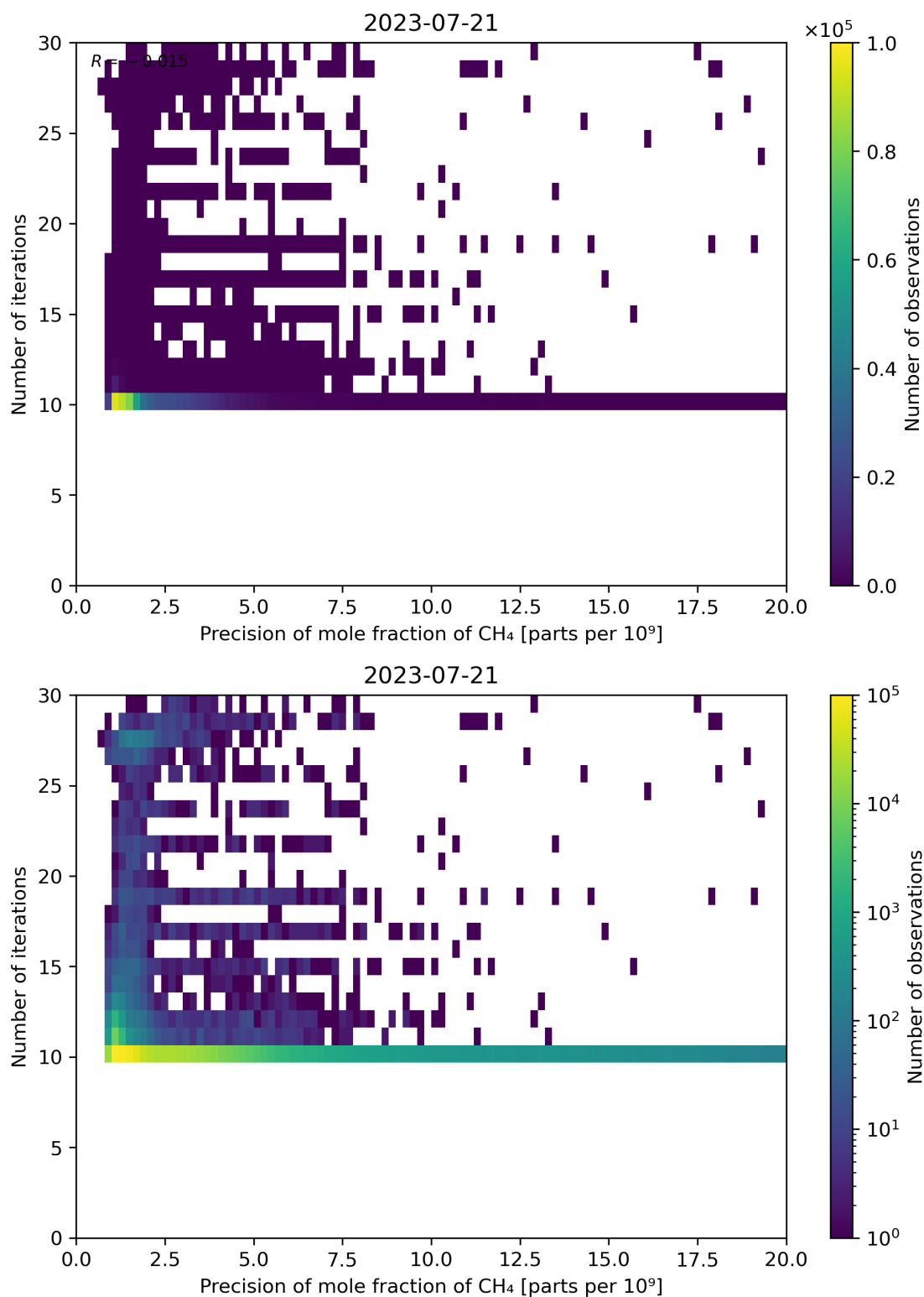
Figure 83: Scatter density plot of “Precision of mole fraction of \text{CH}_4 ” against “Number of iterations” for 2023-07-20 to 2023-07-22.
