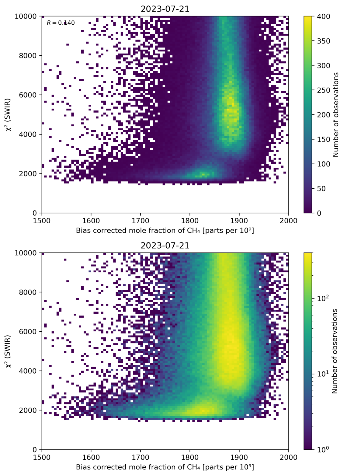
Figure 64: Scatter density plot of “Bias corrected mole fraction of CH 4 ” against “ \chi^2 (SWIR)” for 2023-07-20 to 2023-07-22.
