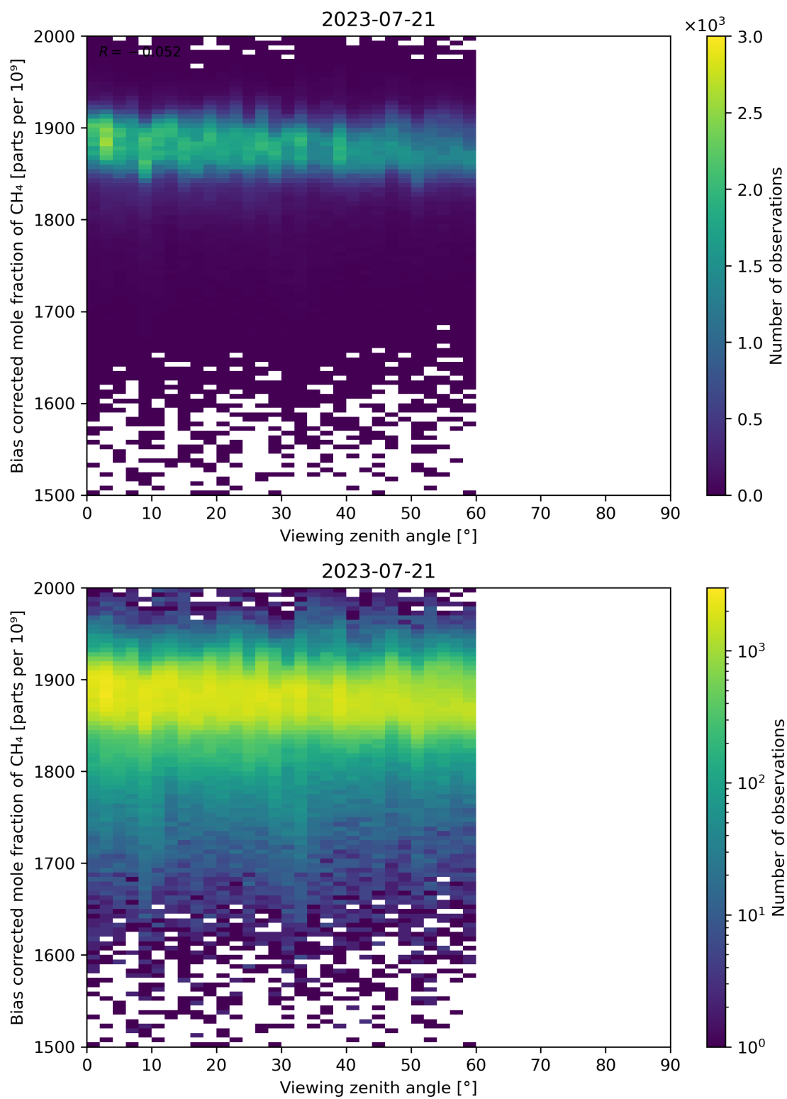
Figure 111: Scatter density plot of “Viewing zenith angle” against “Bias corrected mole fraction of CH 4 ” for 2023-07-20 to 2023-07-22.
