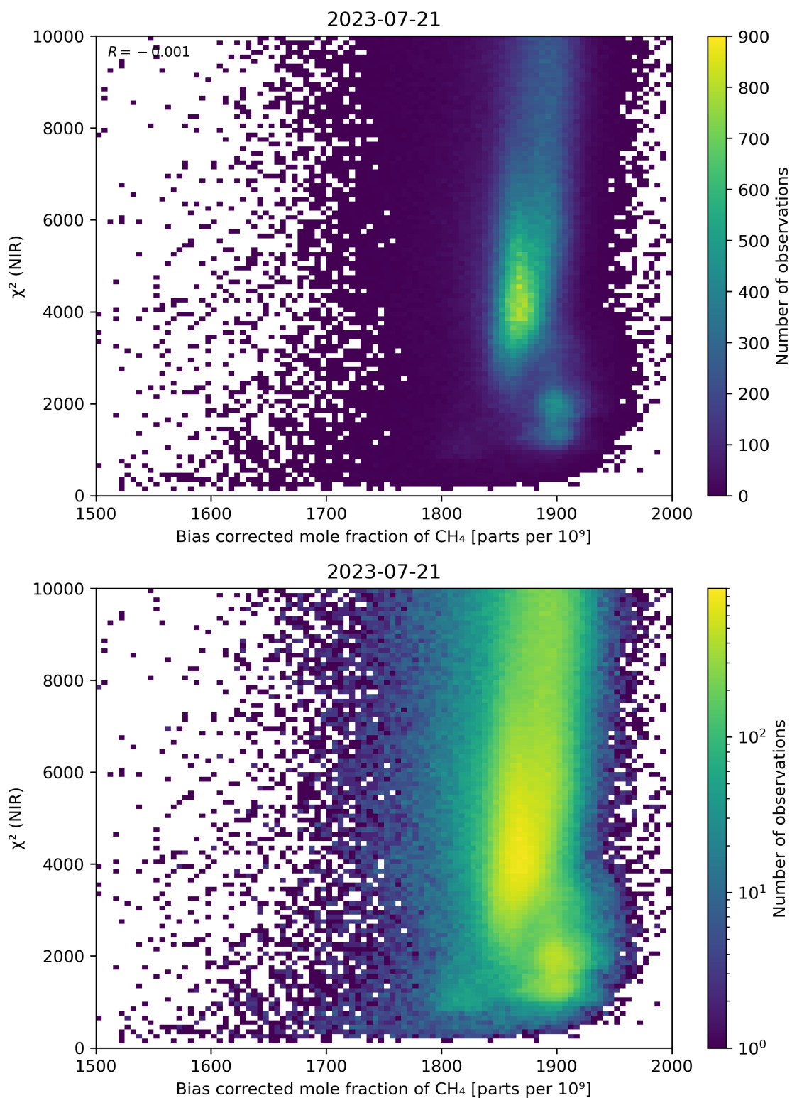
Figure 63: Scatter density plot of “Bias corrected mole fraction of CH 4 ” against “ \chi^2 (NIR)” for 2023-07-20 to 2023-07-22.
