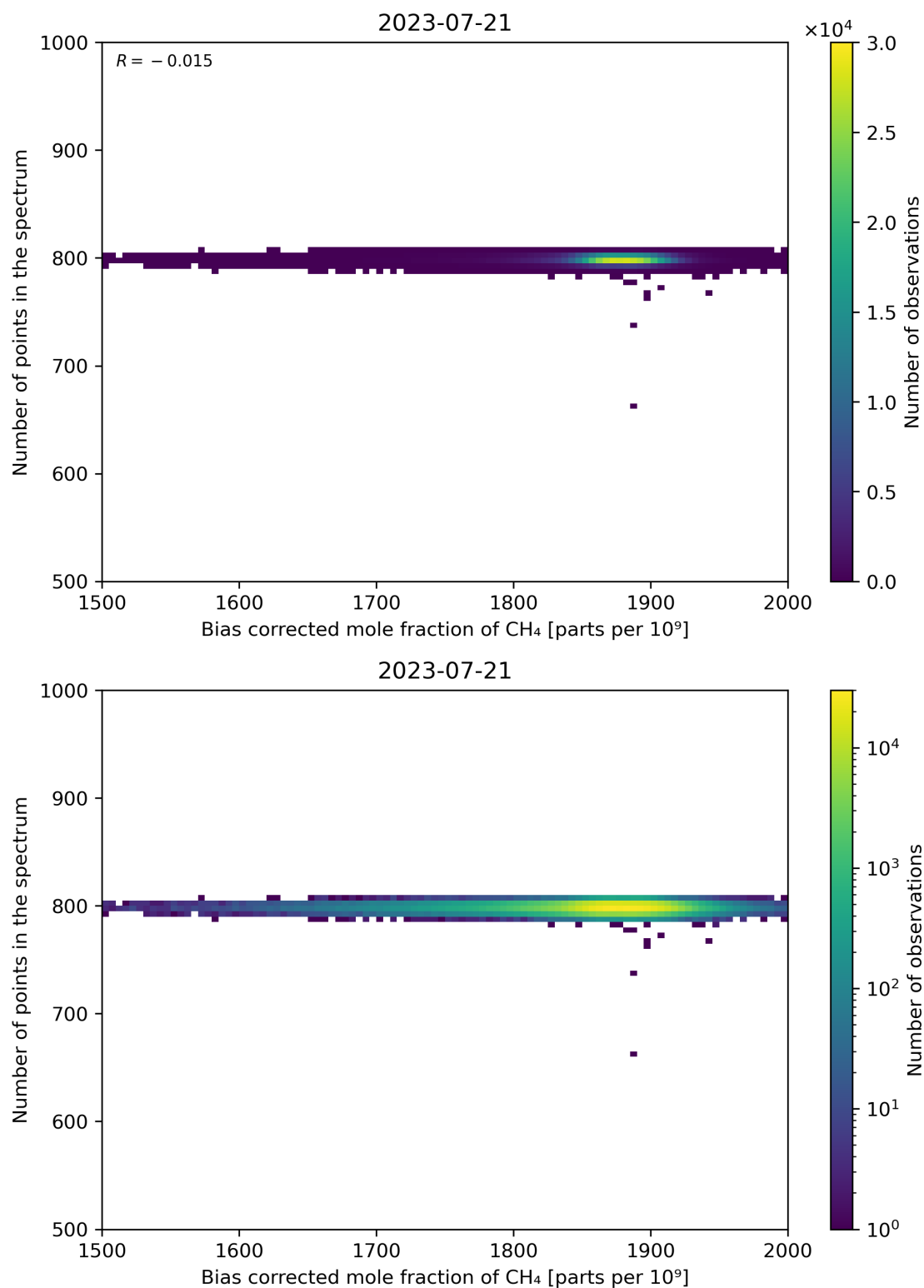
Figure 68: Scatter density plot of “Bias corrected mole fraction of CH 4 ” against “Number of points in the spectrum” for 2023-07-20 to 2023-07-22.
