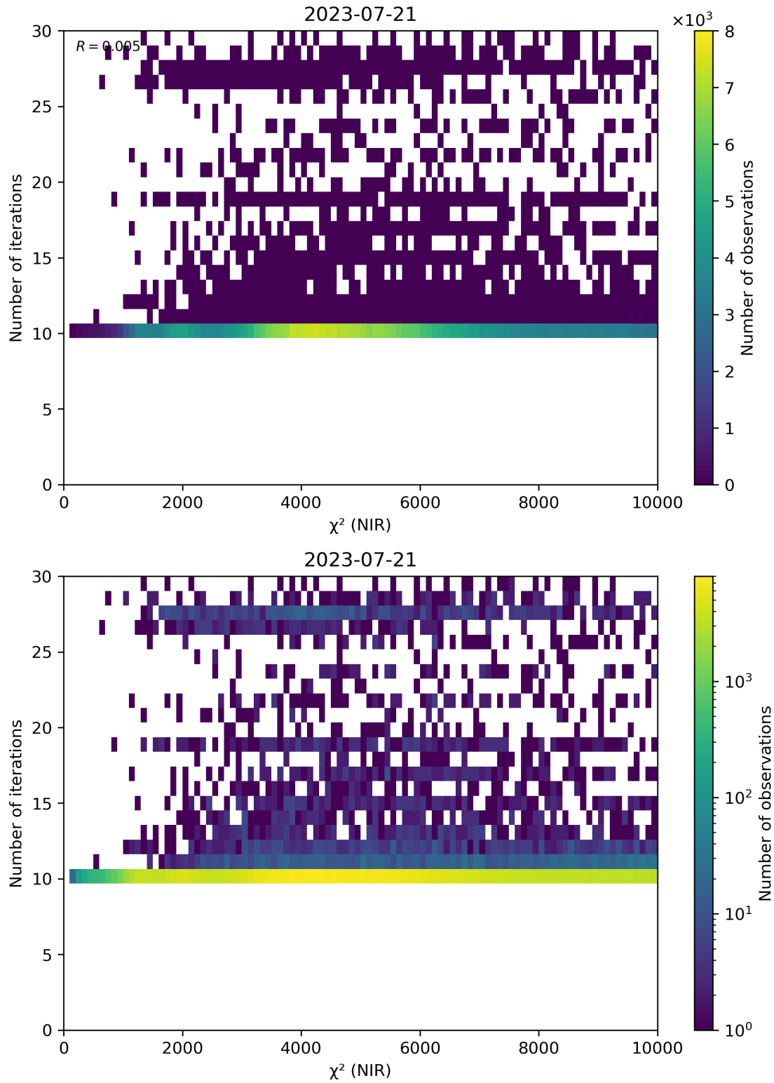
Figure 46: Scatter density plot of “ \chi^2 (NIR)” against “Number of iterations” for 2023-07-20 to 2023-07-22.
