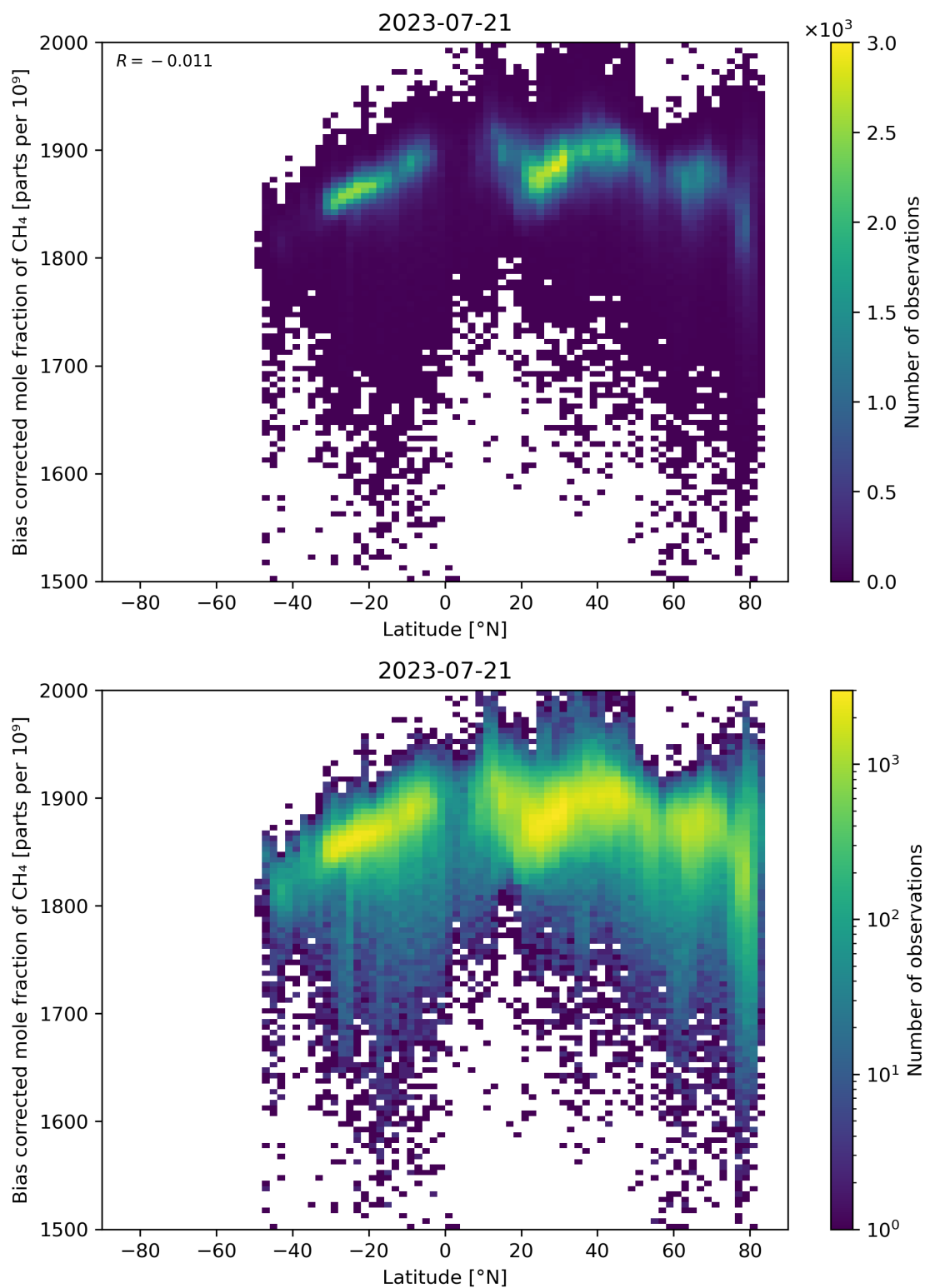
Figure 58: Scatter density plot of “Latitude” against “Bias corrected mole fraction of \text{CH}_4 ” for 2023-07-20 to 2023-07-22.
