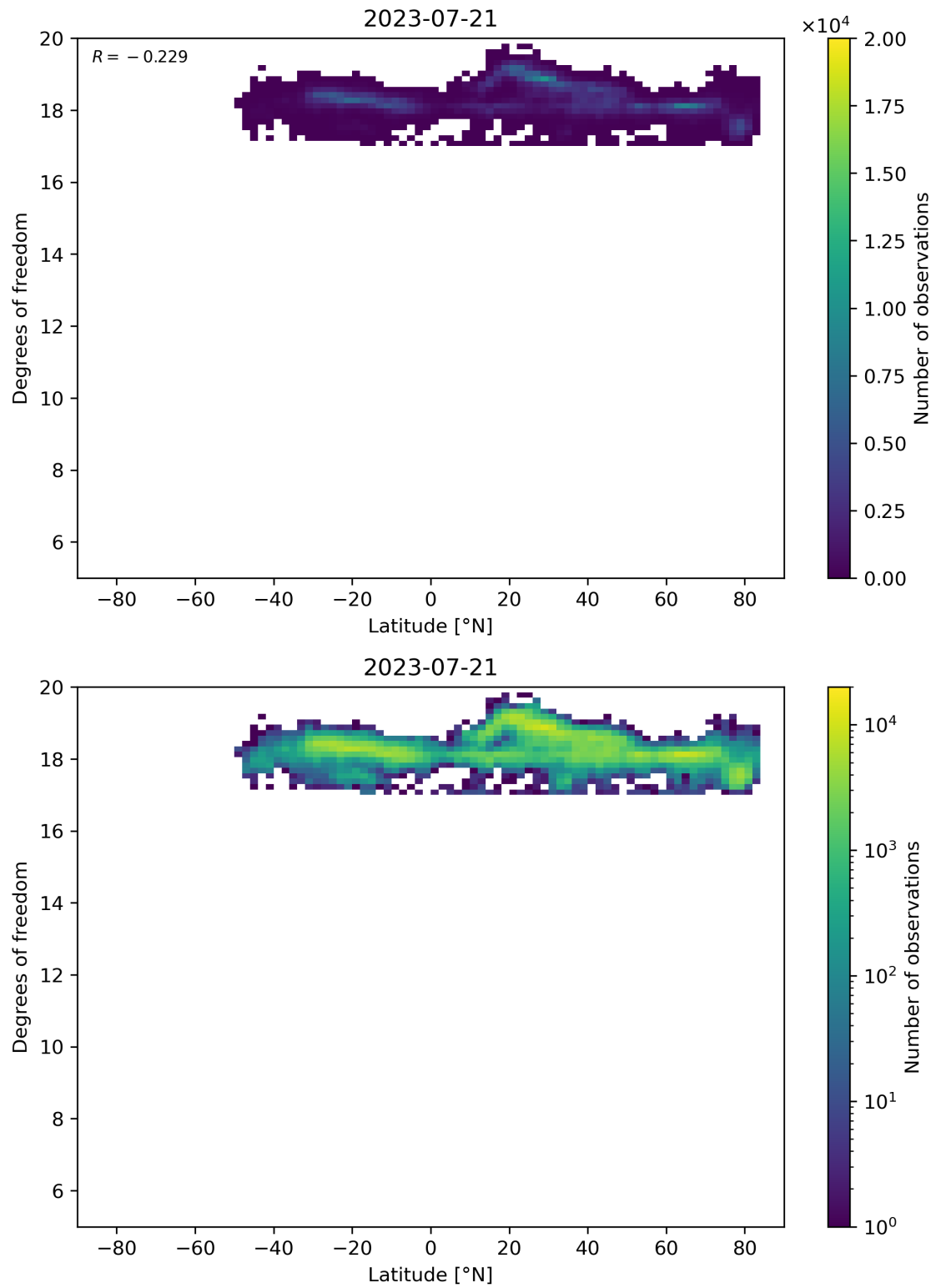
Figure 55: Scatter density plot of “Latitude” against “Degrees of freedom” for 2023-07-20 to 2023-07-22.
