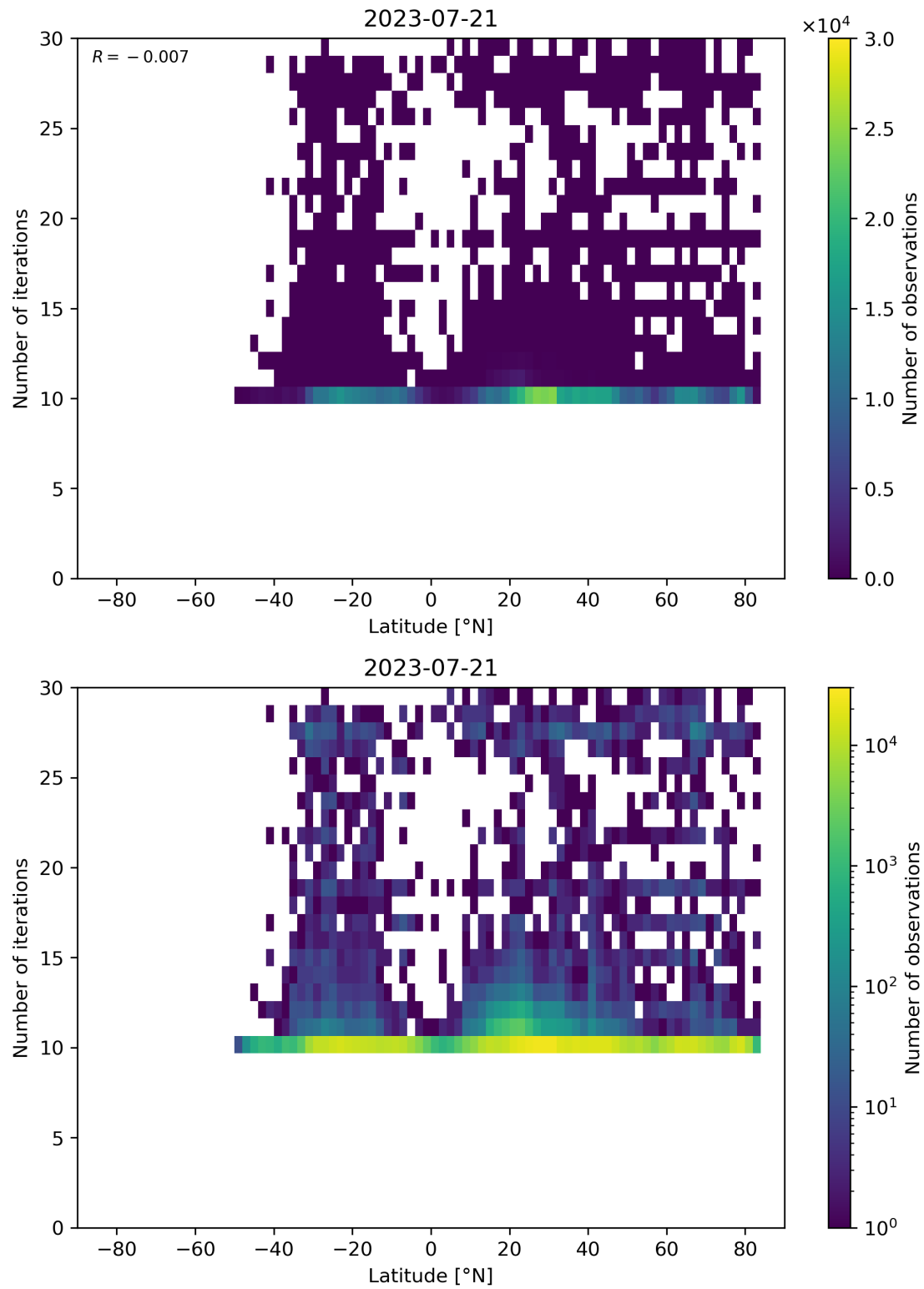
Figure 60: Scatter density plot of “Latitude” against “Number of iterations” for 2023-07-20 to 2023-07-22.
