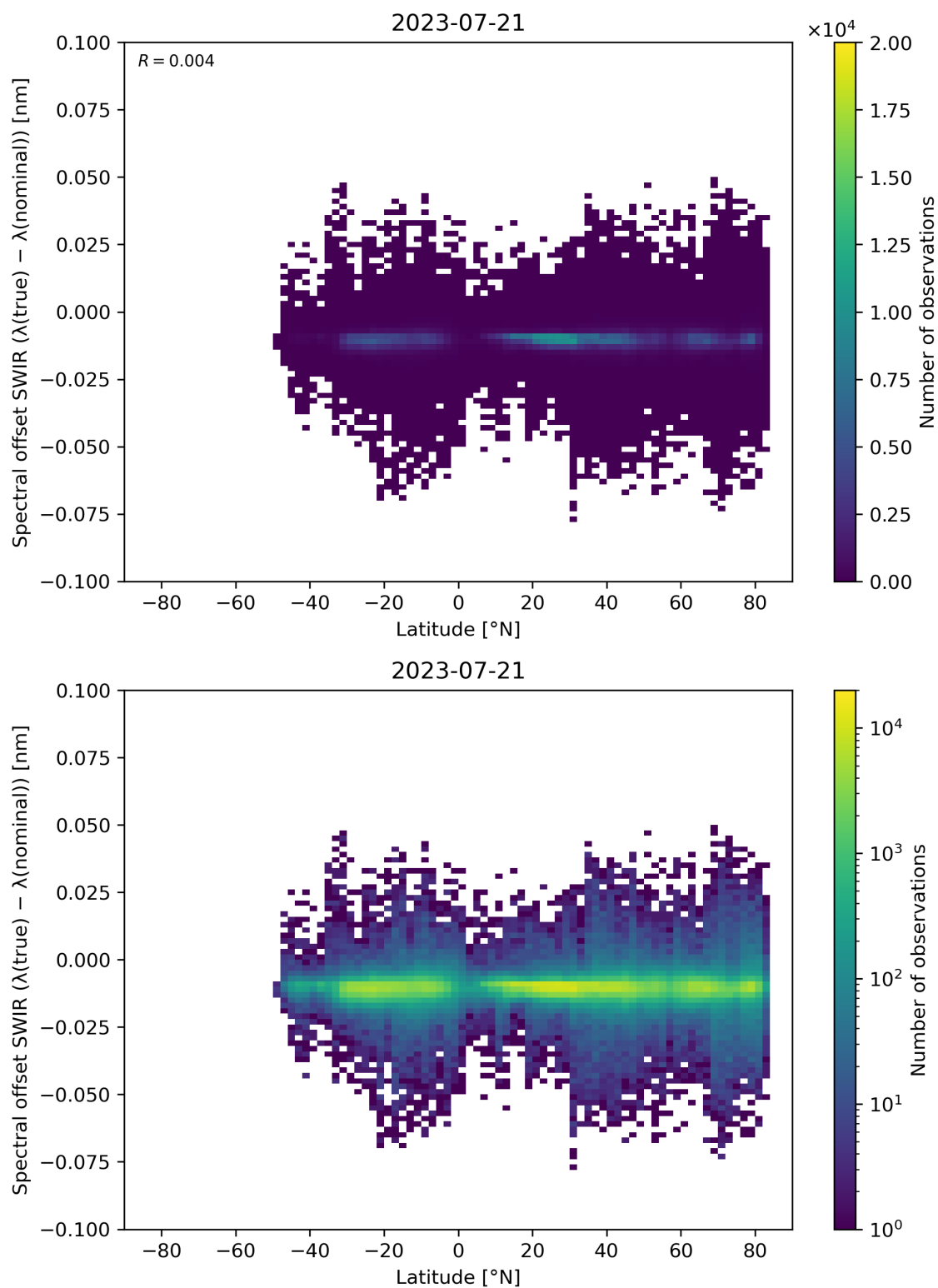
Figure 62: Scatter density plot of “Latitude” against “Spectral offset SWIR ( \lambda(\text{true}) - \lambda(\text{nominal}) )” for 2023-07-20 to 2023-07-22.
