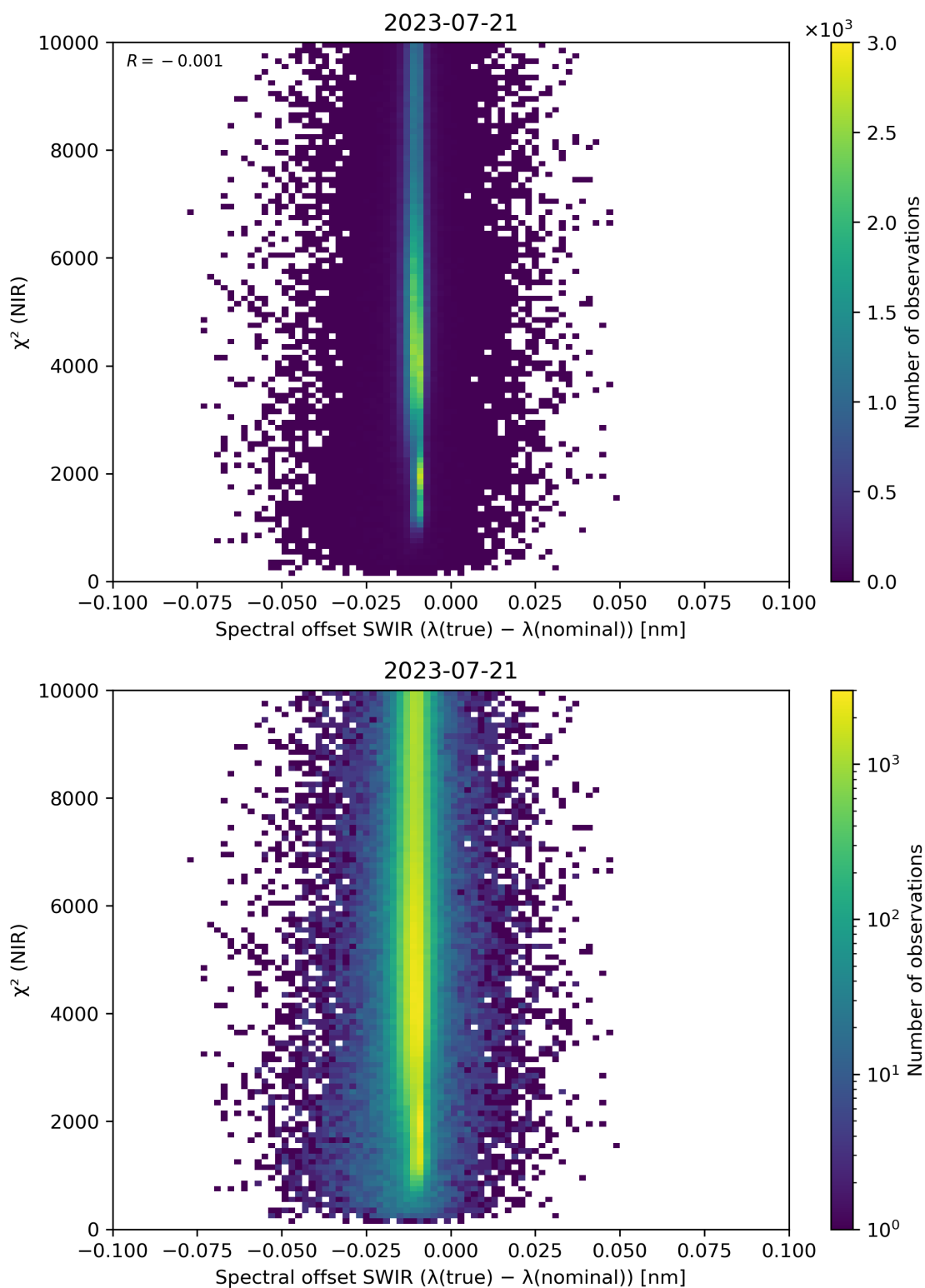
Figure 117: Scatter density plot of “Spectral offset SWIR ( \lambda(\text{true}) - \lambda(\text{nominal}) )” against “ \chi^2 (NIR)” for 2023-07-20 to 2023-07-22.
