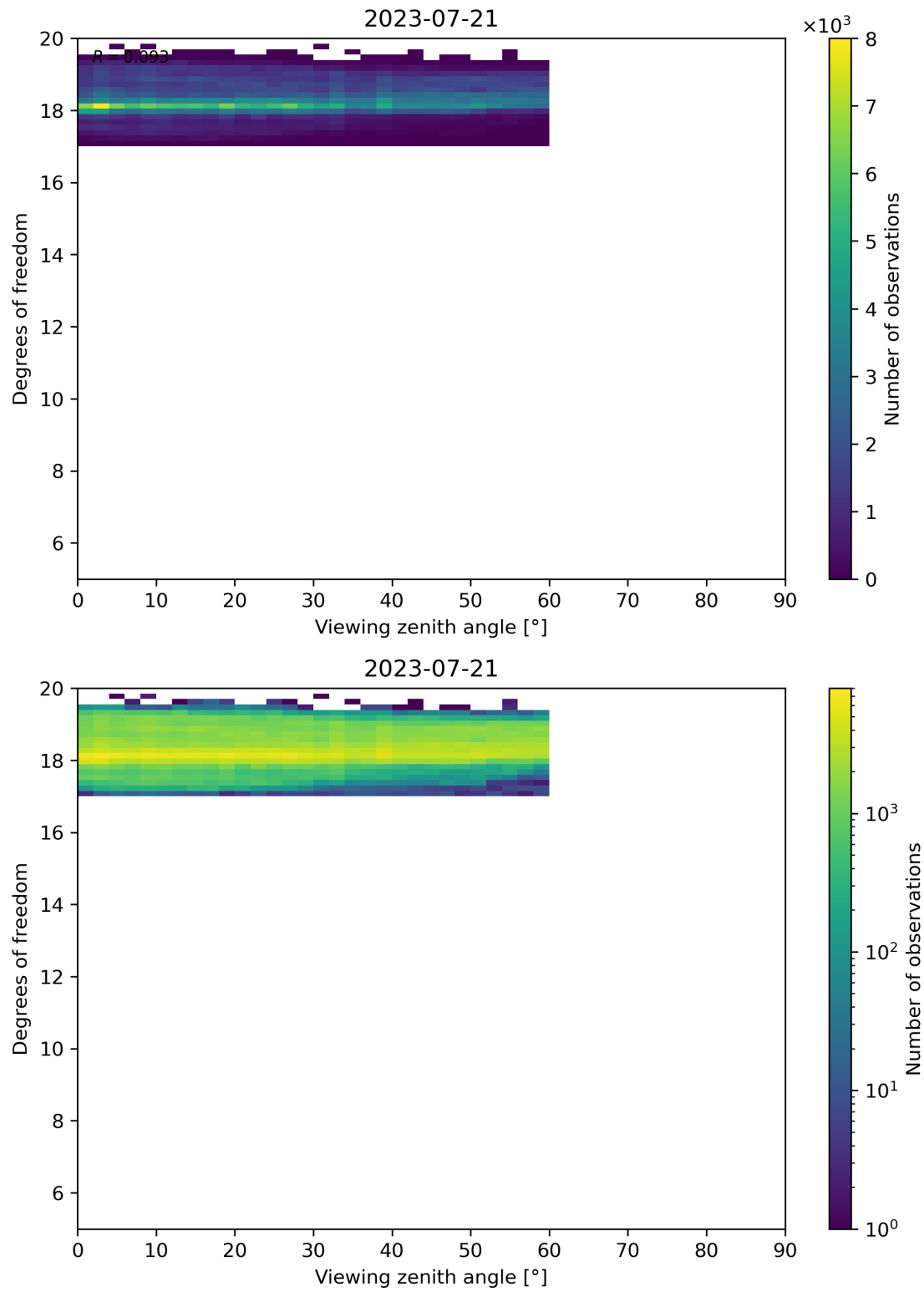
Figure 107: Scatter density plot of “Viewing zenith angle” against “Degrees of freedom” for 2023-07-20 to 2023-07-22.
