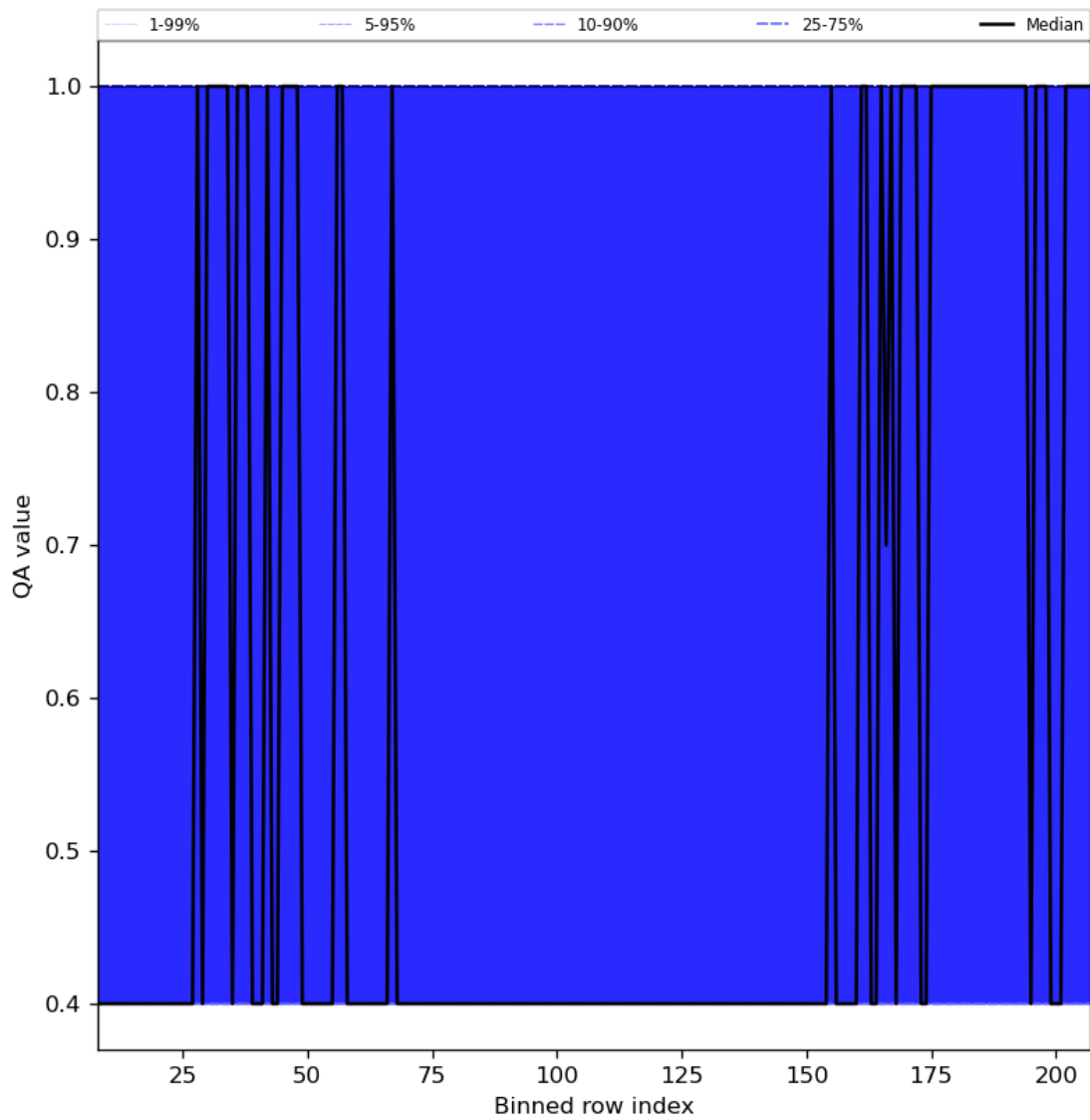
Figure 33: Along track statistics of “QA value” for 2023-07-20 to 2023-07-22
