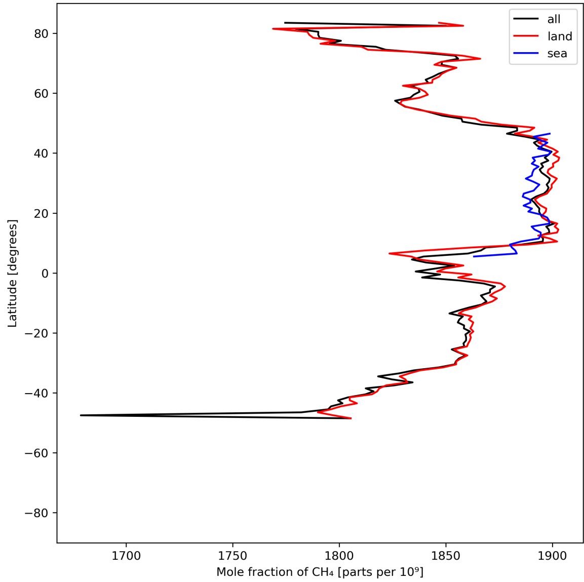
Figure 12: Zonal average of “Mole fraction of \text{CH}_4 ” for 2023-07-20 to 2023-07-22.
