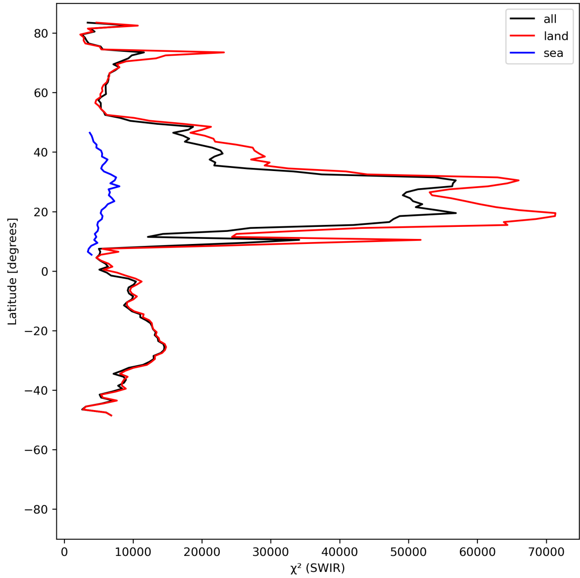
Figure 17: Zonal average of “ \chi^2 (SWIR)” for 2023-07-20 to 2023-07-22.
