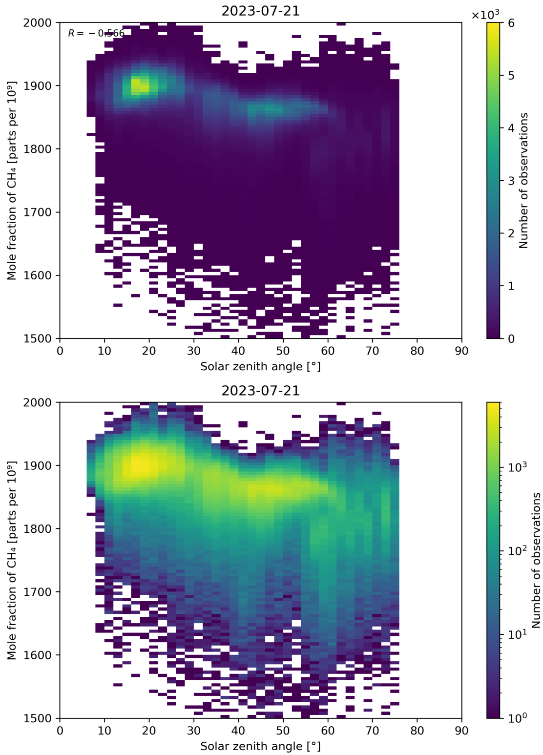
Figure 99: Scatter density plot of “Solar zenith angle” against “Mole fraction of CH 4 ” for 2023-07-20 to 2023-07-22.
