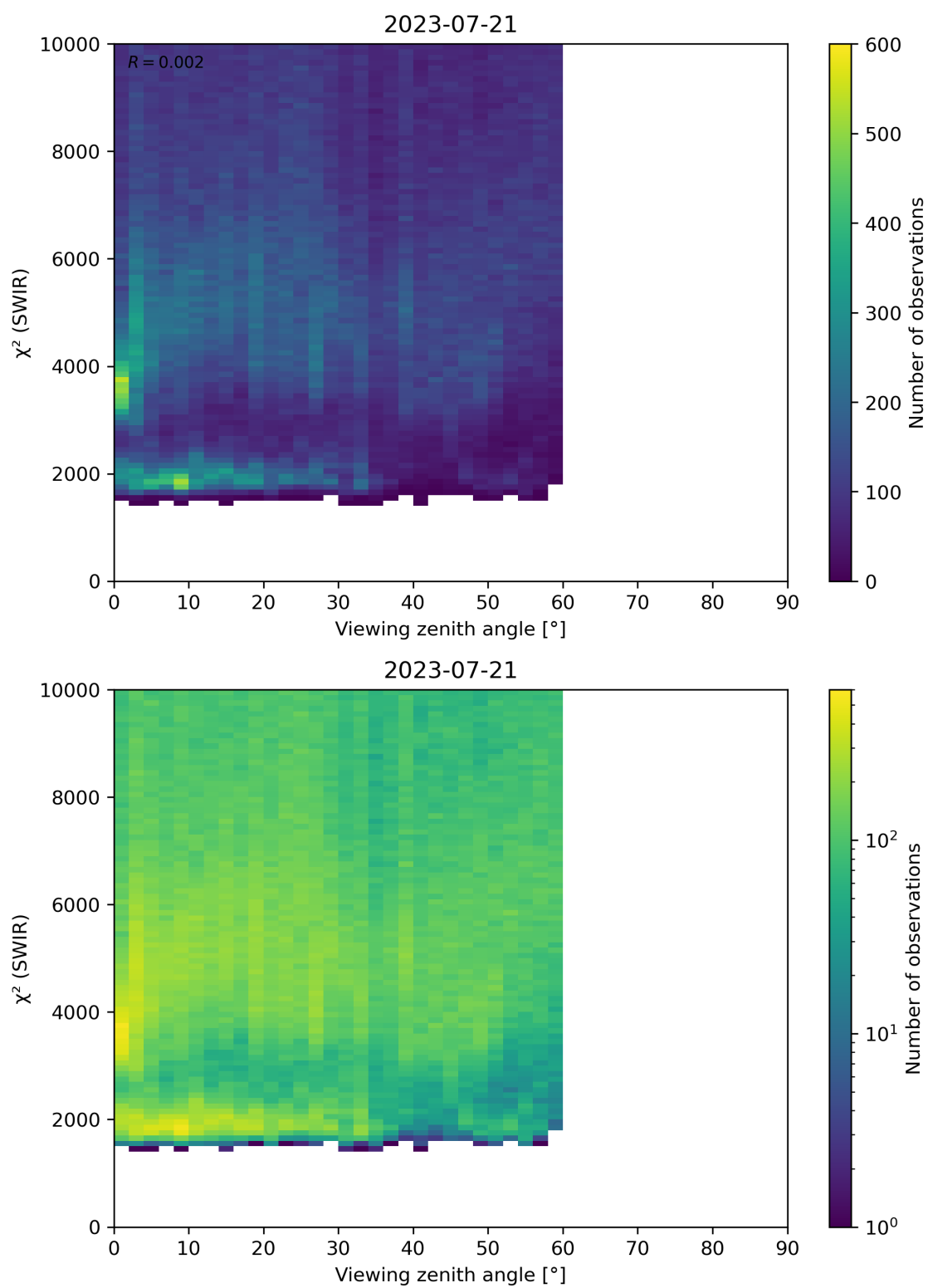
Figure 106: Scatter density plot of “Viewing zenith angle” against “ \chi^2 (SWIR)” for 2023-07-20 to 2023-07-22.
