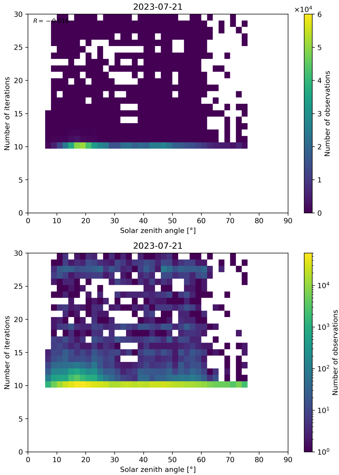
Figure 102: Scatter density plot of “Solar zenith angle” against “Number of iterations” for 2023-07-20 to 2023-07-22.
