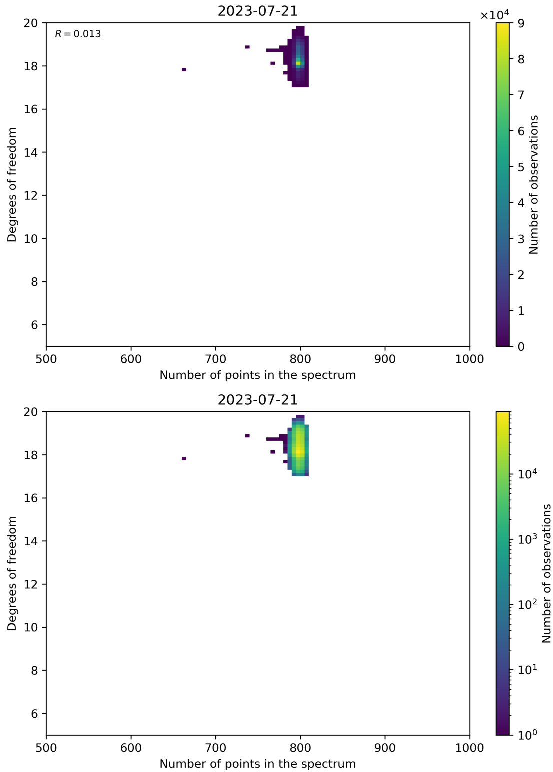
Figure 90: Scatter density plot of “Number of points in the spectrum” against “Degrees of freedom” for 2023-07-20 to 2023-07-22.
