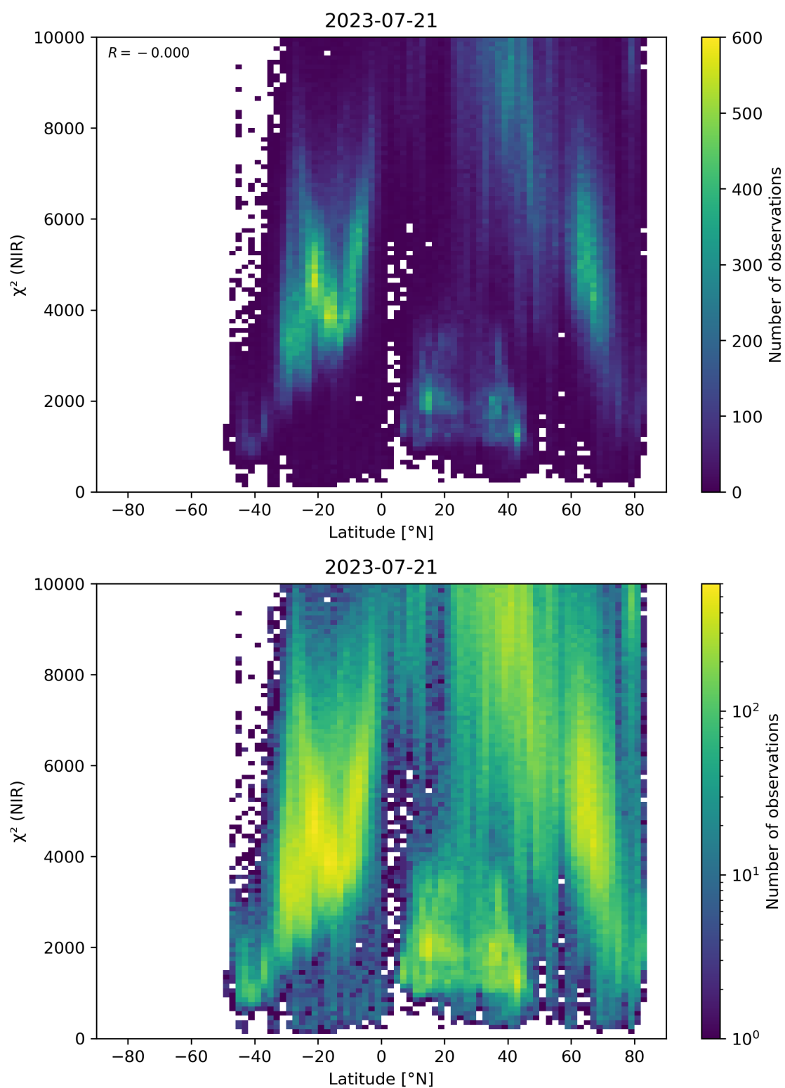
Figure 53: Scatter density plot of “Latitude” against “ \chi^2 (NIR)” for 2023-07-20 to 2023-07-22.
