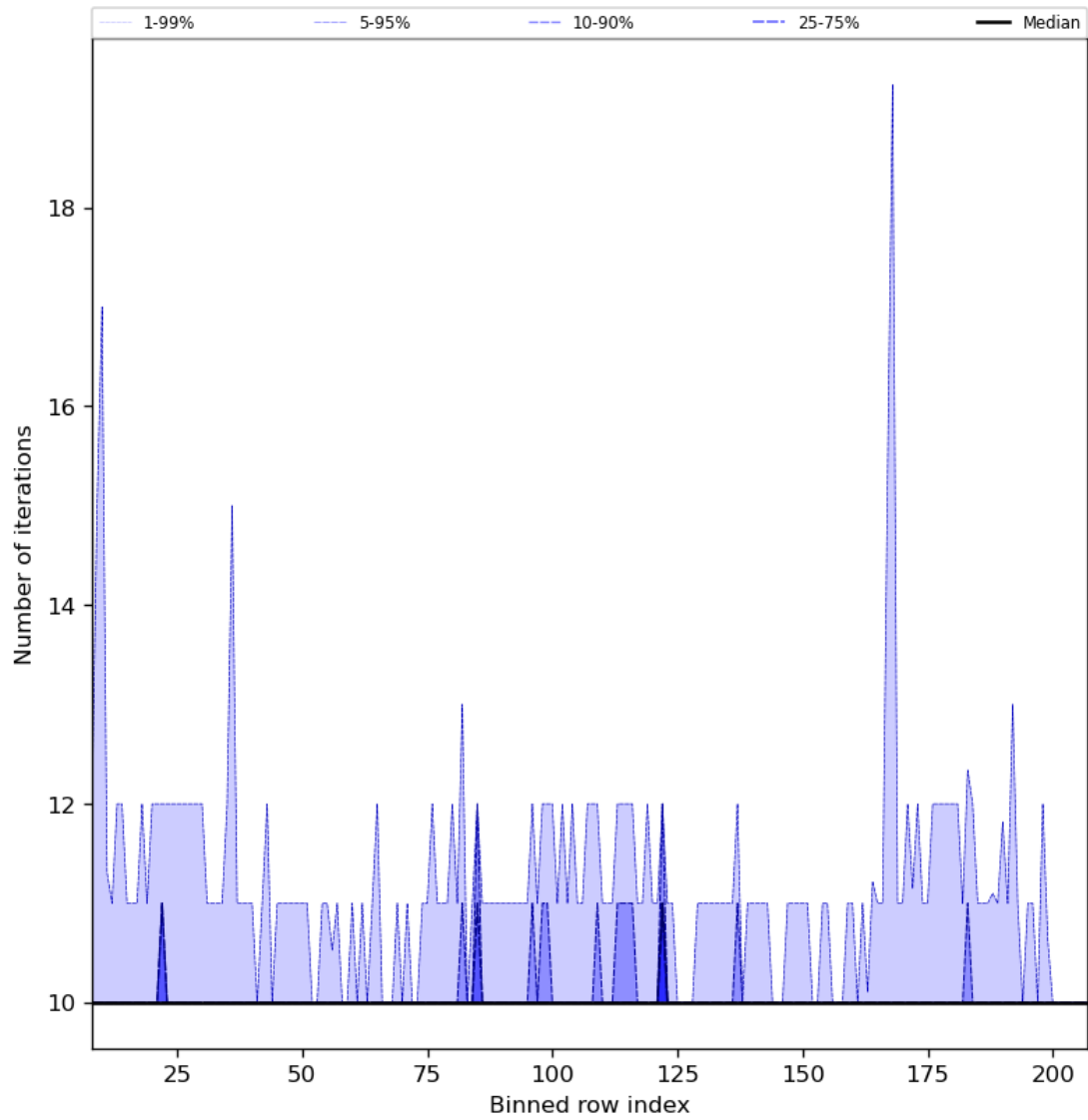
Figure 42: Along track statistics of “Number of iterations” for 2023-07-20 to 2023-07-22
