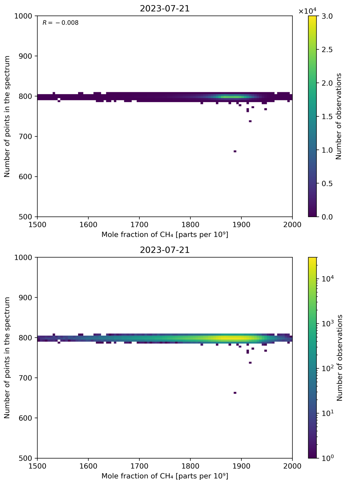
Figure 77: Scatter density plot of “Mole fraction of CH 4 ” against “Number of points in the spectrum” for 2023-07-20 to 2023-07-22.
