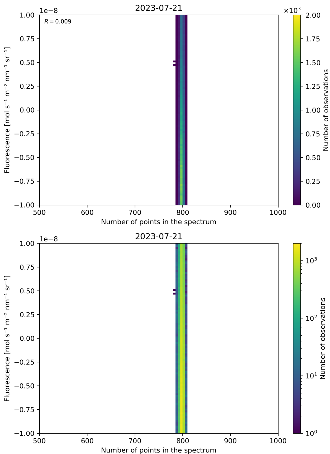
Figure 91: Scatter density plot of “Number of points in the spectrum” against “Fluorescence” for 2023-07-20 to 2023-07-22.
