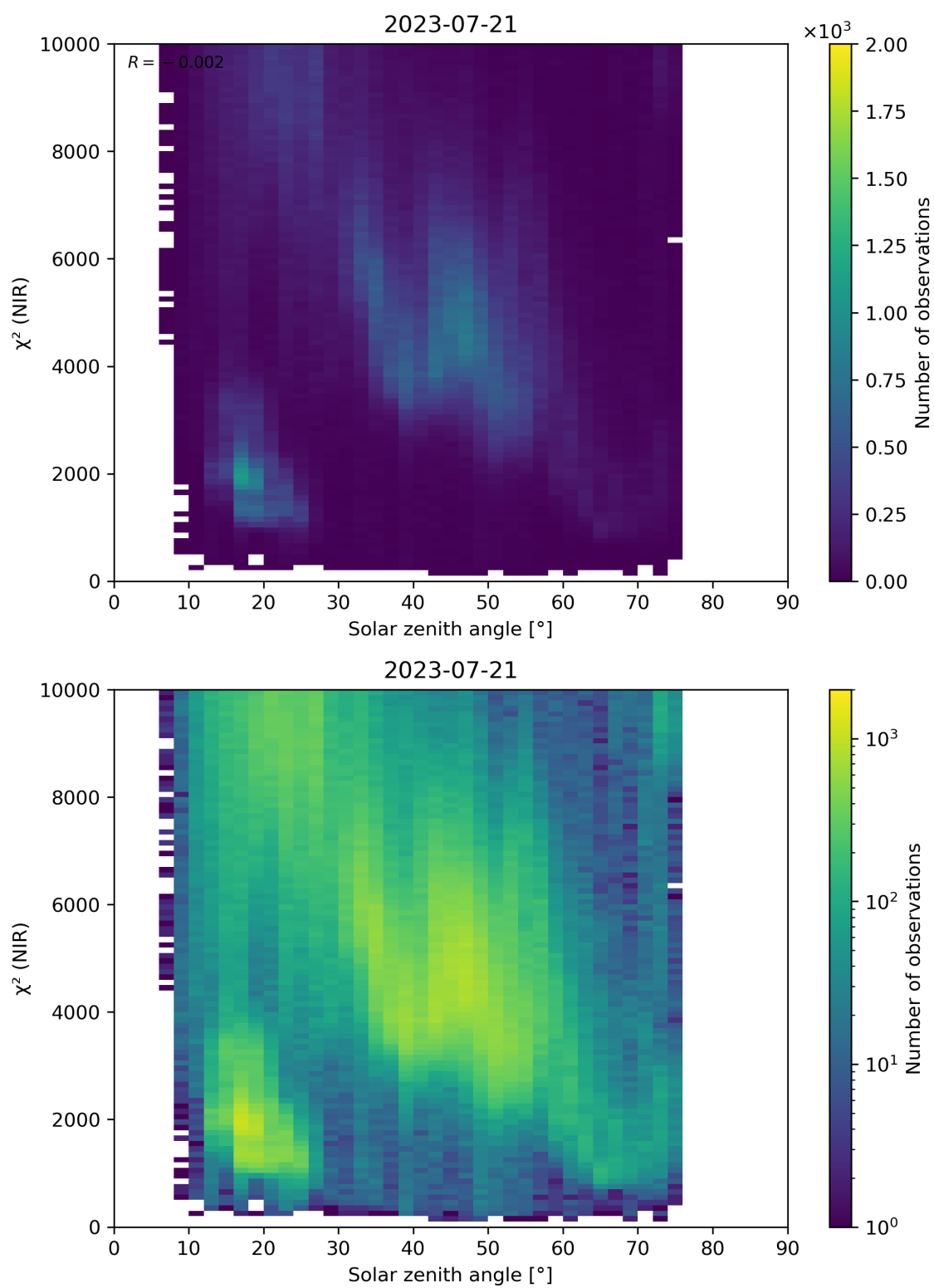
Figure 94: Scatter density plot of “Solar zenith angle” against “ \chi^2 (NIR)” for 2023-07-20 to 2023-07-22.
