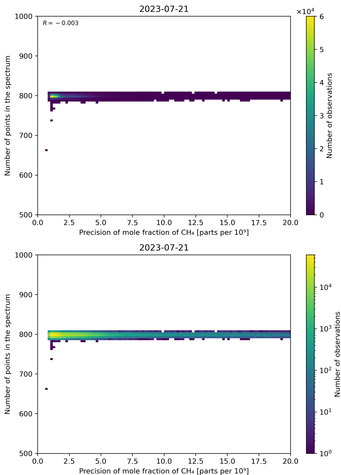
Figure 84: Scatter density plot of “Precision of mole fraction of CH 4 ” against “Number of points in the spectrum” for 2023-07-20 to 2023-07-22.
