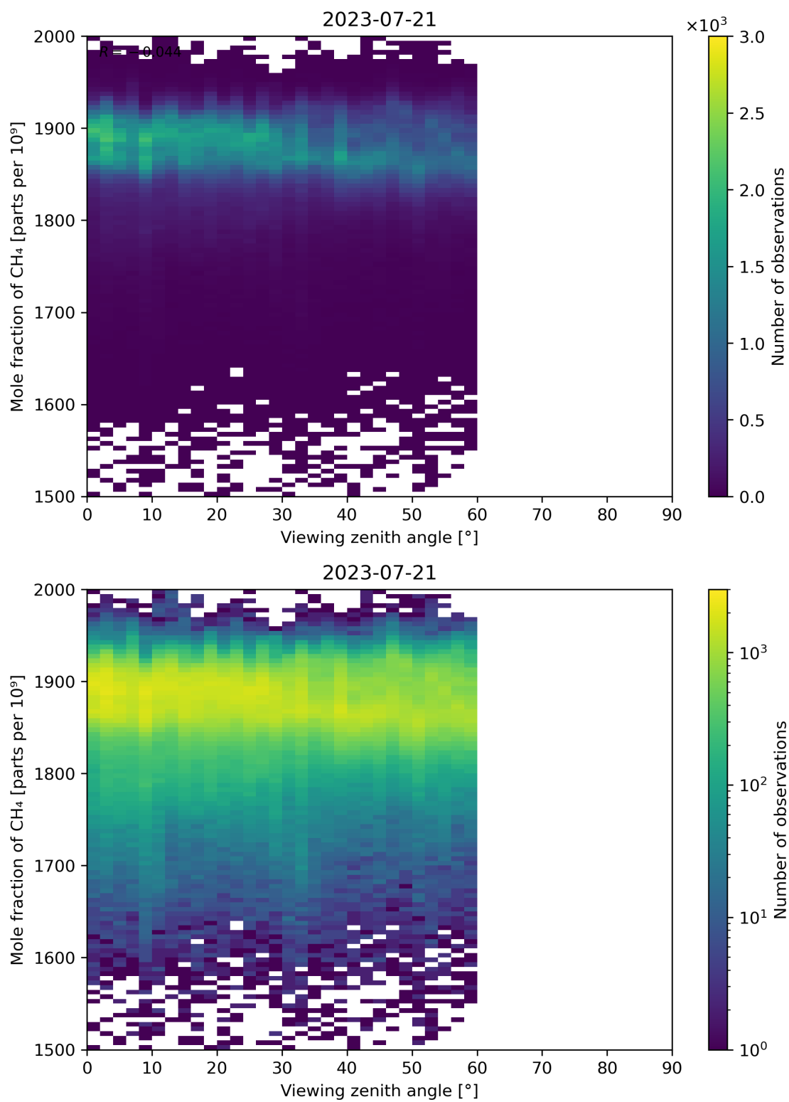
Figure 110: Scatter density plot of “Viewing zenith angle” against “Mole fraction of CH 4 ” for 2023-07-20 to 2023-07-22.
