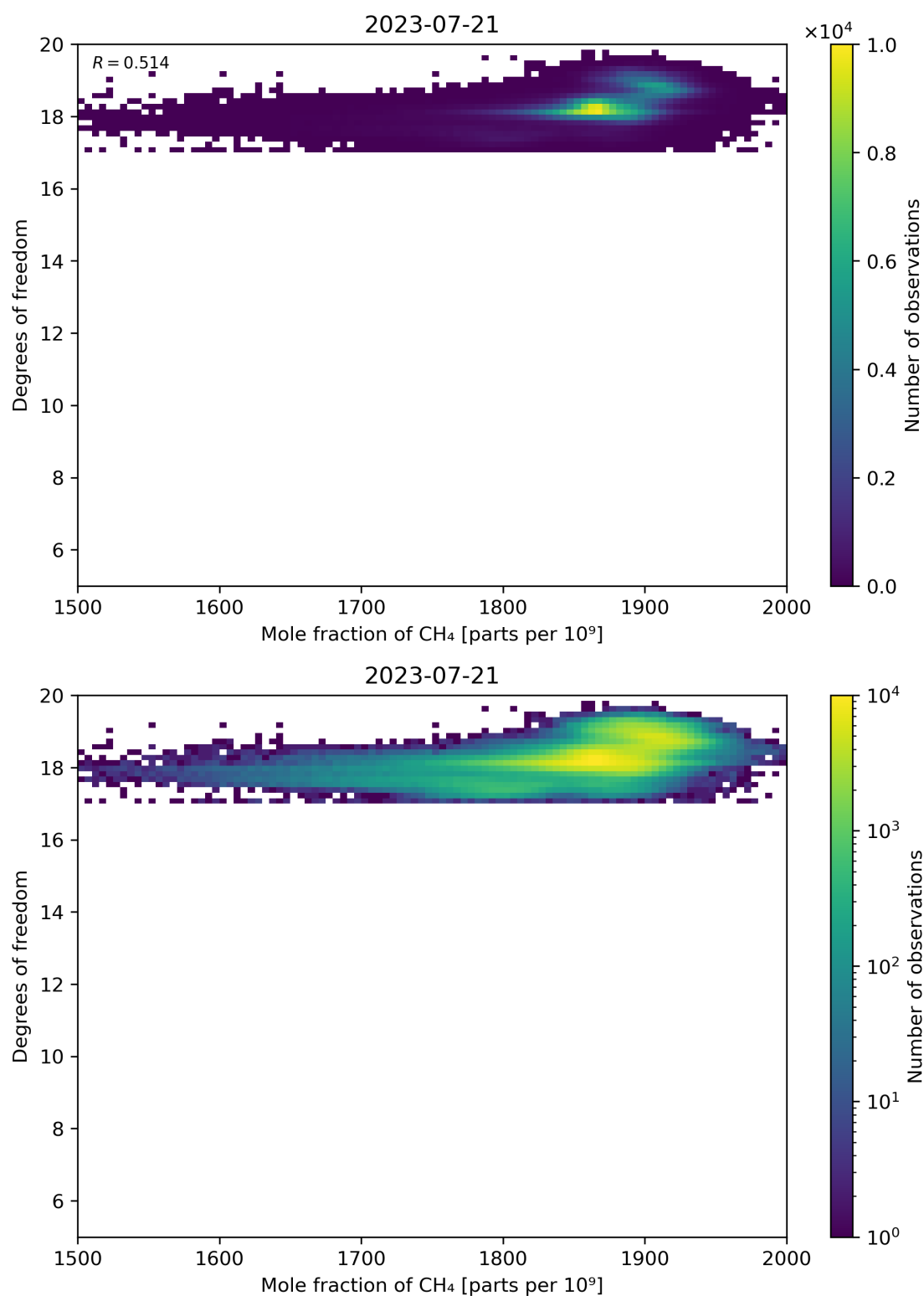
Figure 72: Scatter density plot of “Mole fraction of CH 4 ” against “Degrees of freedom” for 2023-07-20 to 2023-07-22.
