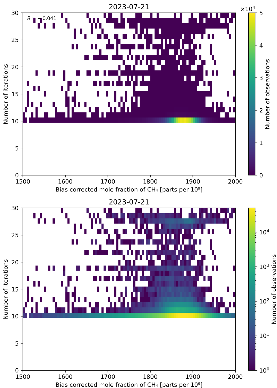
Figure 67: Scatter density plot of “Bias corrected mole fraction of CH 4 ” against “Number of iterations” for 2023-07-20 to 2023-07-22.
