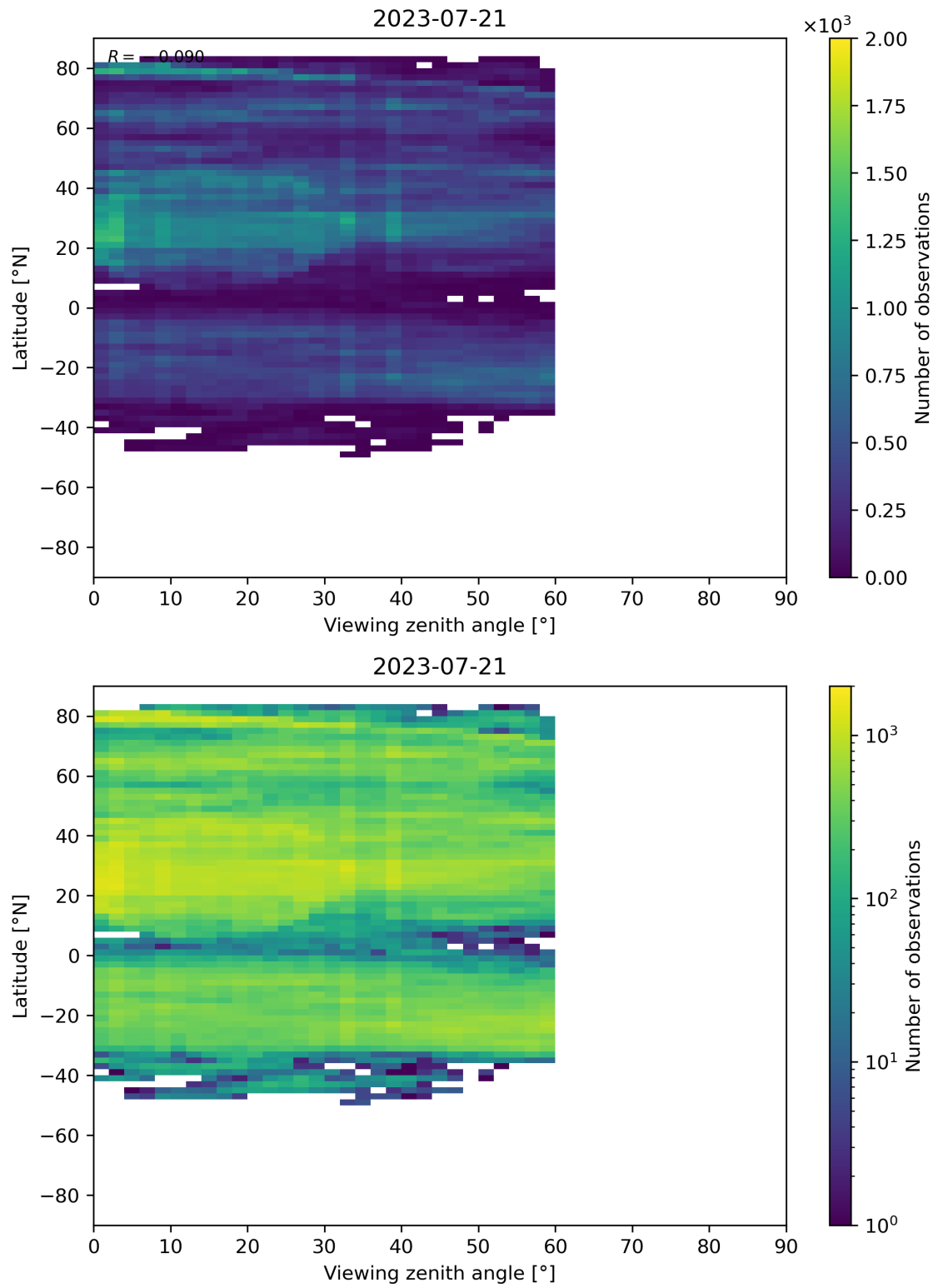
Figure 109: Scatter density plot of “Viewing zenith angle” against “Latitude” for 2023-07-20 to 2023-07-22.
