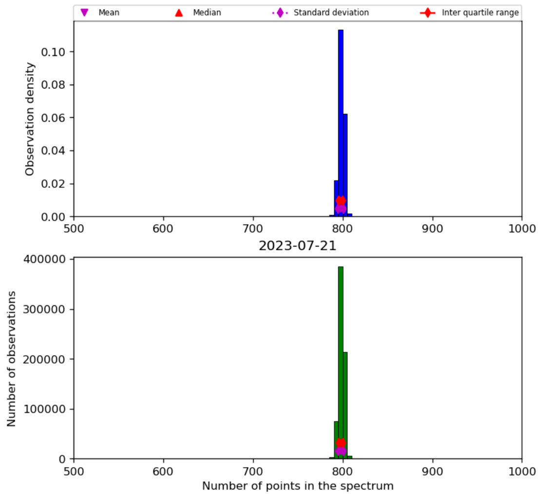
Figure 26: Histogram of “Number of points in the spectrum” for 2023-07-20 to 2023-07-22
