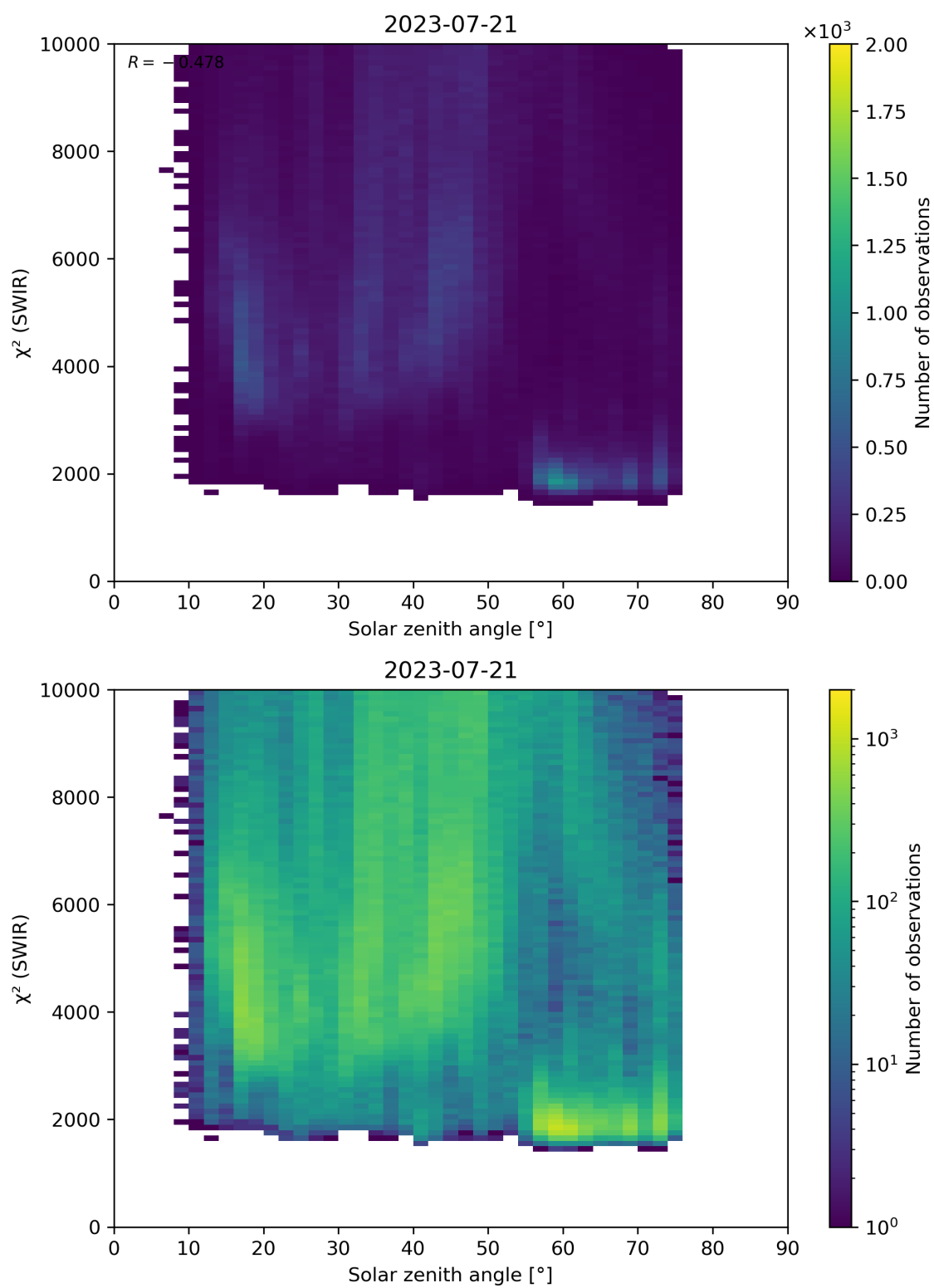
Figure 95: Scatter density plot of “Solar zenith angle” against “ \chi^2 (SWIR)” for 2023-07-20 to 2023-07-22.
