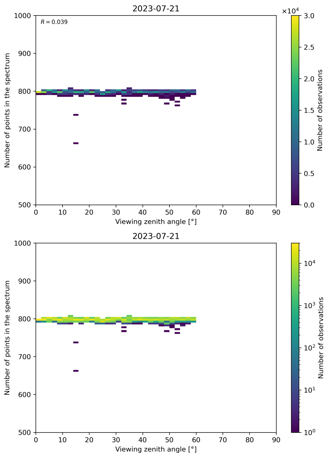
Figure 114: Scatter density plot of “Viewing zenith angle” against “Number of points in the spectrum” for 2023-07-20 to 2023-07-22.
