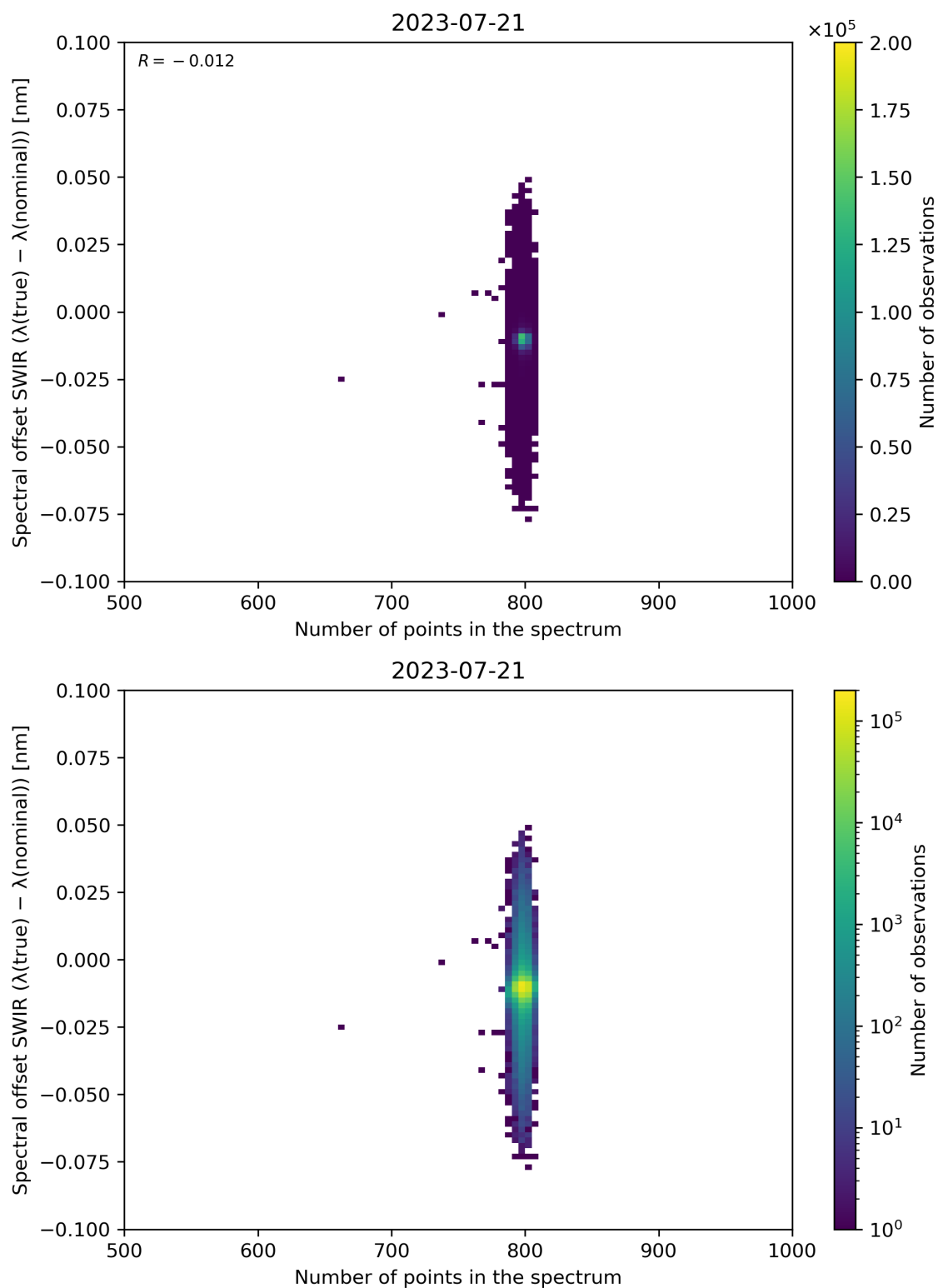
Figure 93: Scatter density plot of “Number of points in the spectrum” against “Spectral offset SWIR ( \lambda(\text{true}) - \lambda(\text{nominal}) )” for 2023-07-20 to 2023-07-22.
