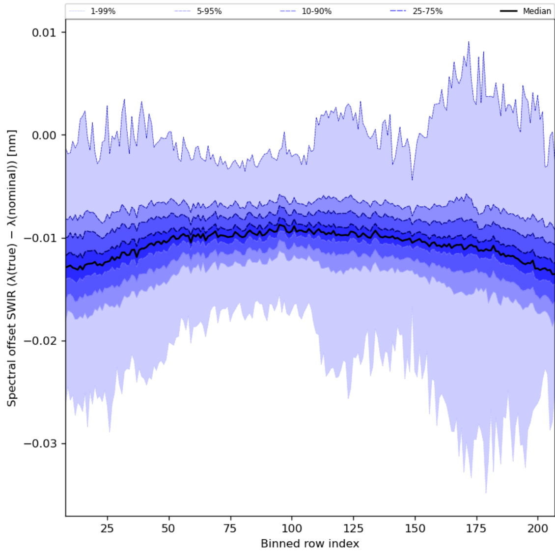
Figure 38: Along track statistics of “Spectral offset SWIR ( \lambda(\text{true}) - \lambda(\text{nominal}) )” for 2023-07-20 to 2023-07-22
