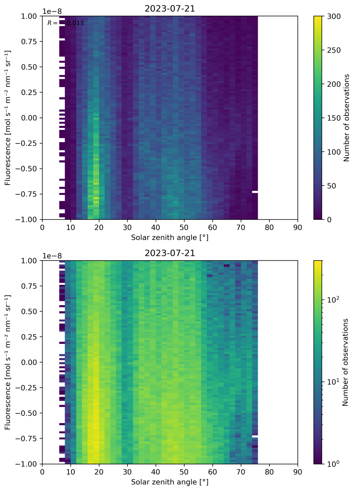
Figure 97: Scatter density plot of “Solar zenith angle” against “Fluorescence” for 2023-07-20 to 2023-07-22.
