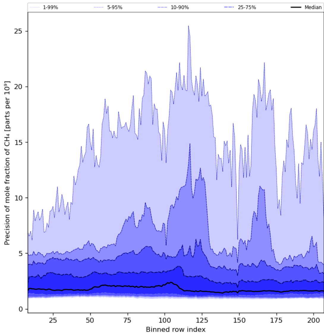
Figure 35: Along track statistics of “Precision of mole fraction of CH 4 ” for 2023-07-20 to 2023-07-22
