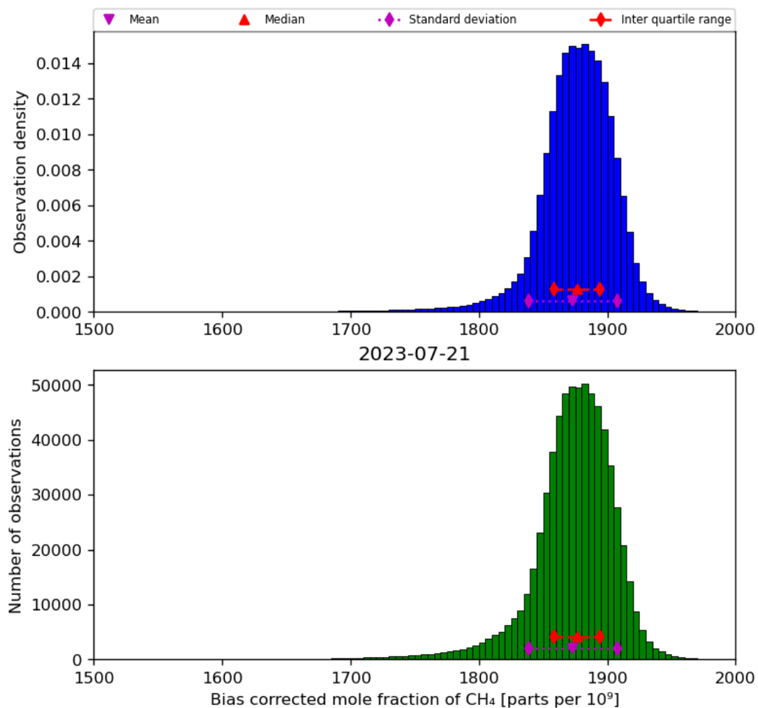
Figure 25: Histogram of “Bias corrected mole fraction of CH 4 ” for 2023-07-20 to 2023-07-22
