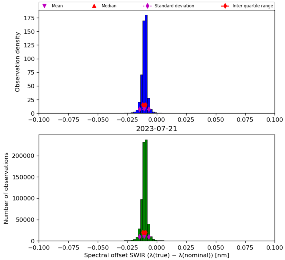
Figure 27: Histogram of “Spectral offset SWIR ( \lambda(\text{true}) - \lambda(\text{nominal}) )” for 2023-07-20 to 2023-07-22
