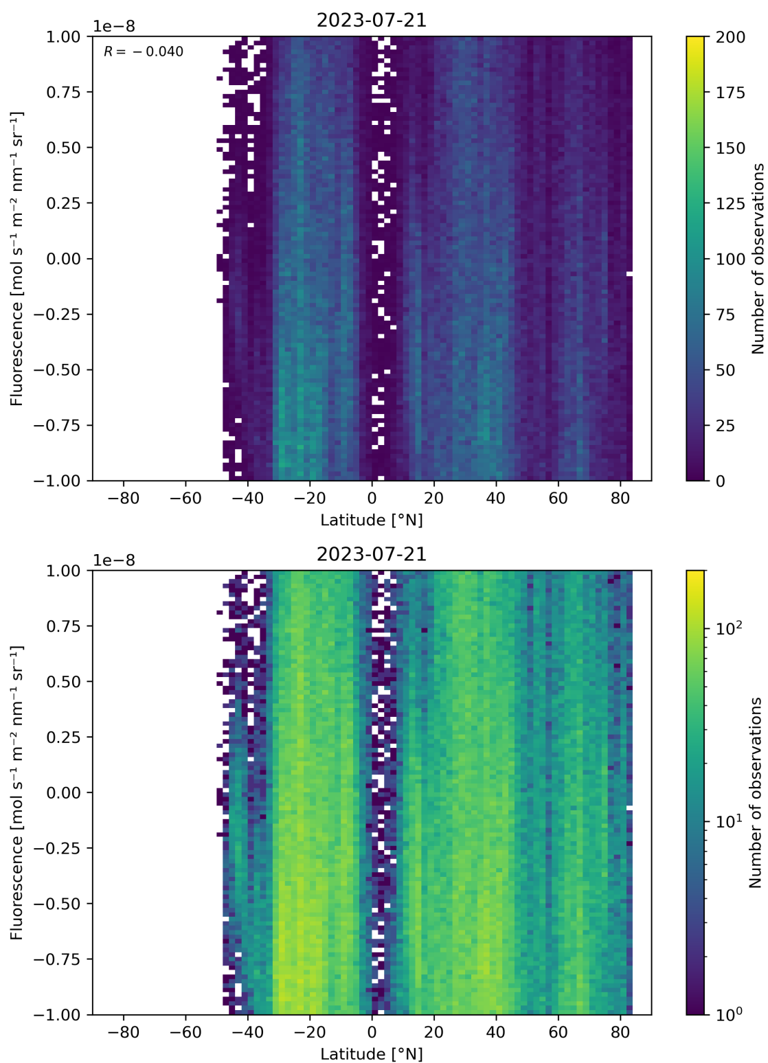
Figure 56: Scatter density plot of “Latitude” against “Fluorescence” for 2023-07-20 to 2023-07-22.
