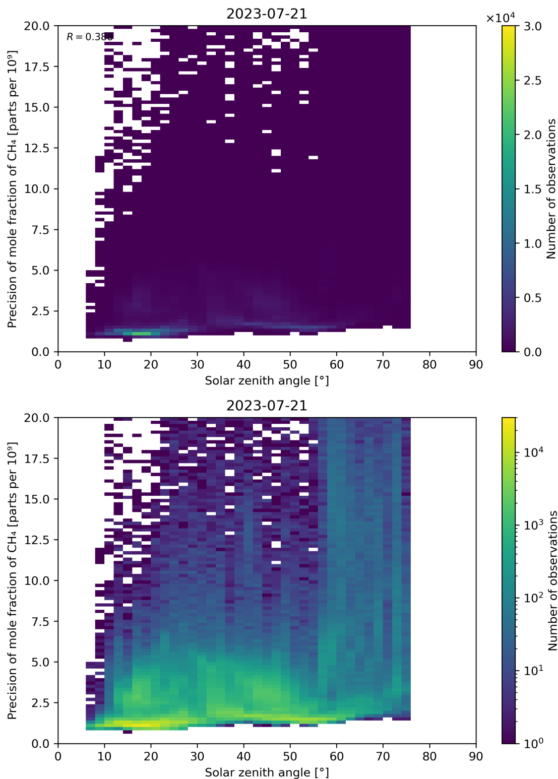
Figure 101: Scatter density plot of “Solar zenith angle” against “Precision of mole fraction of CH 4 ” for 2023-07-20 to 2023-07-22.
