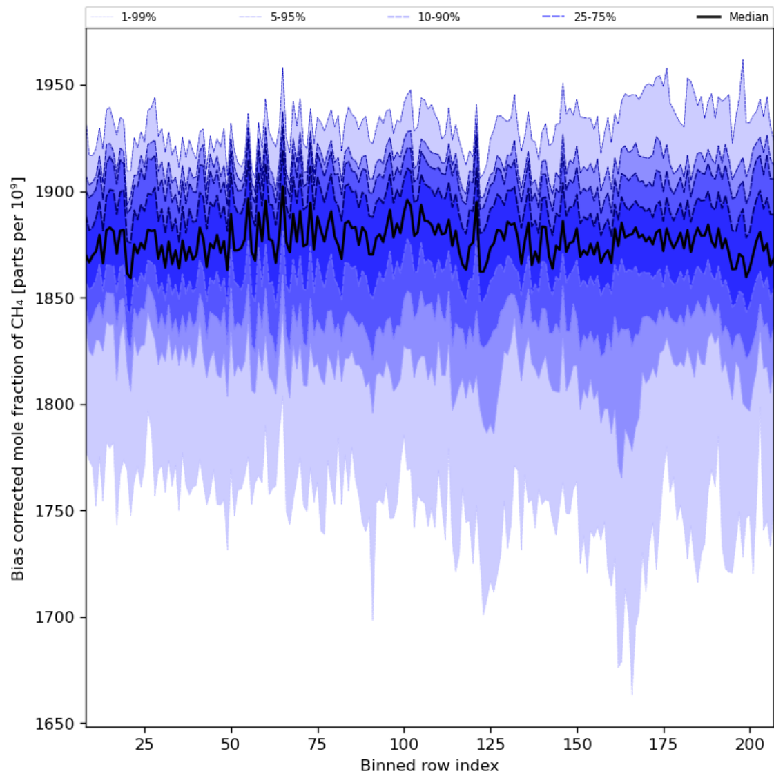
Figure 36: Along track statistics of “Bias corrected mole fraction of CH 4 ” for 2023-07-20 to 2023-07-22
