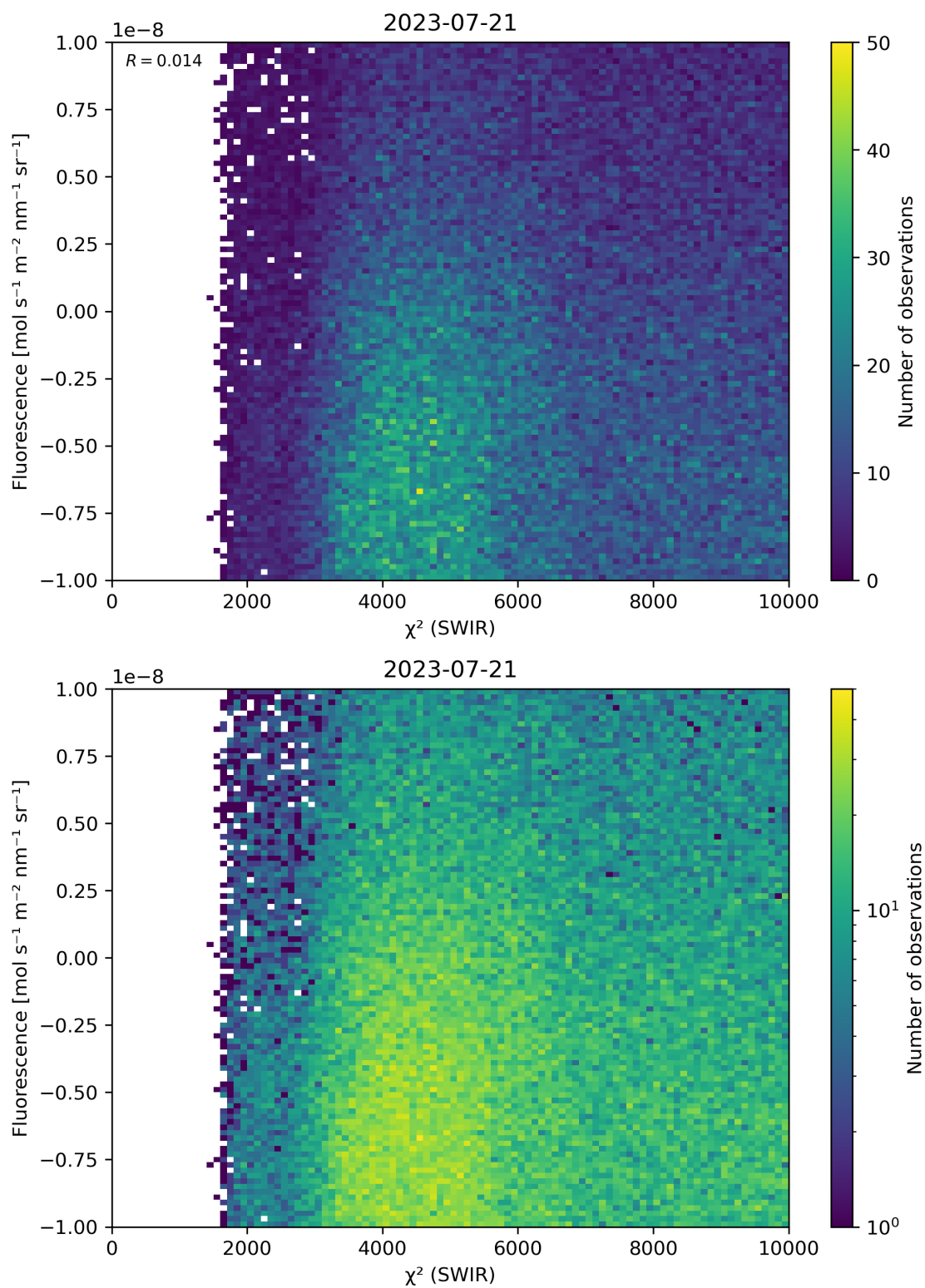
Figure 49: Scatter density plot of “ \chi^2 (SWIR)” against “Fluorescence” for 2023-07-20 to 2023-07-22.
