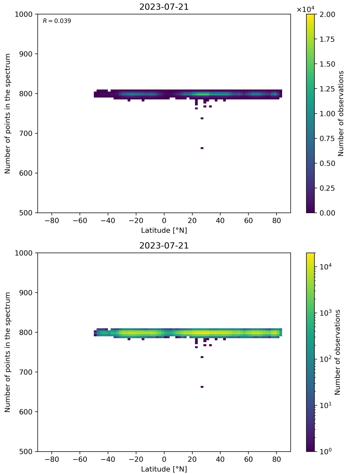
Figure 61: Scatter density plot of “Latitude” against “Number of points in the spectrum” for 2023-07-20 to 2023-07-22.
