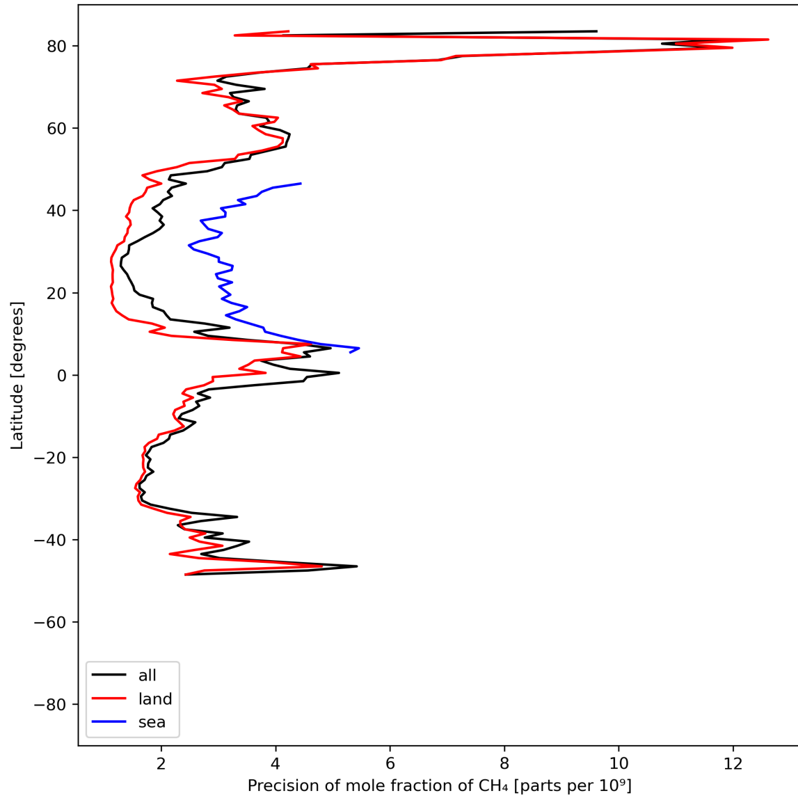
Figure 13: Zonal average of “Precision of mole fraction of CH 4 ” for 2023-07-20 to 2023-07-22.
