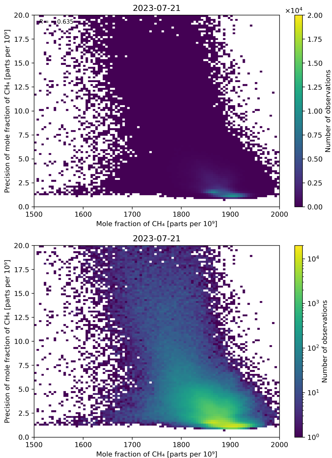
Figure 75: Scatter density plot of “Mole fraction of CH 4 ” against “Precision of mole fraction of CH 4 ” for 2023-07-20 to 2023-07-22.
