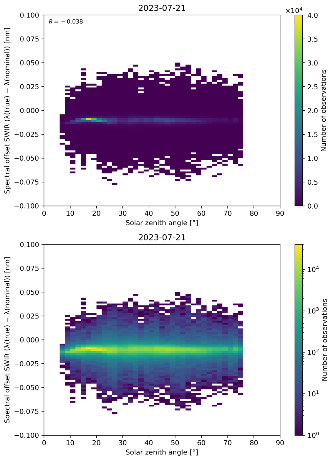
Figure 104: Scatter density plot of “Solar zenith angle” against “Spectral offset SWIR ( \lambda(\text{true}) - \lambda(\text{nominal}) )” for 2023-07-20 to 2023-07-22.
