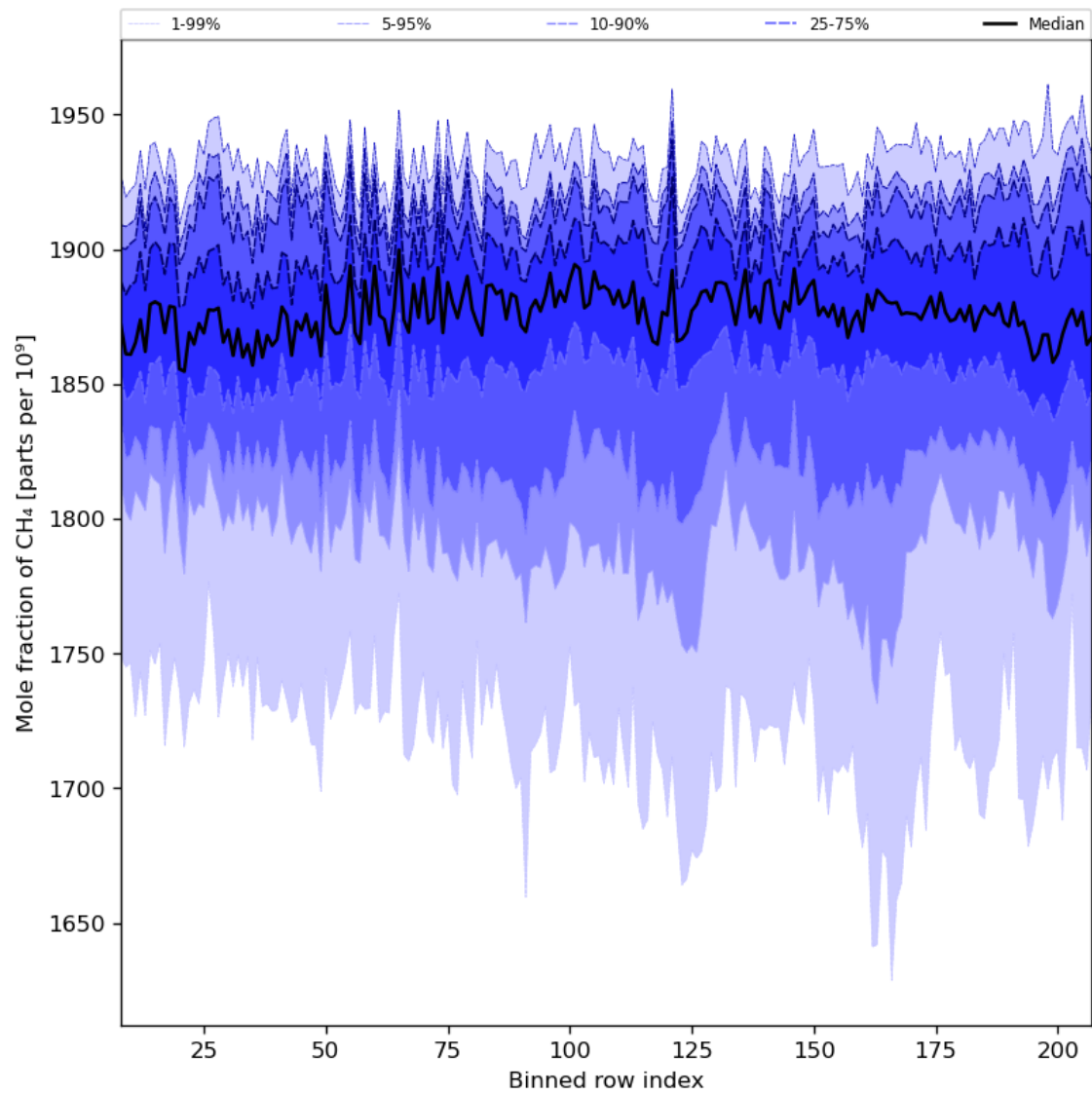
Figure 34: Along track statistics of “Mole fraction of CH 4 ” for 2023-07-20 to 2023-07-22
