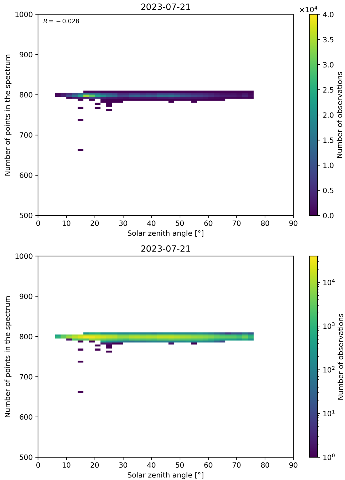
Figure 103: Scatter density plot of “Solar zenith angle” against “Number of points in the spectrum” for 2023-07-20 to 2023-07-22.
