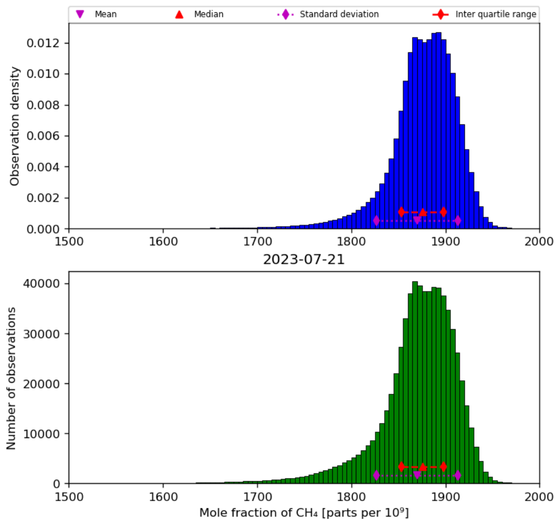
Figure 23: Histogram of “Mole fraction of CH 4 ” for 2023-07-20 to 2023-07-22
