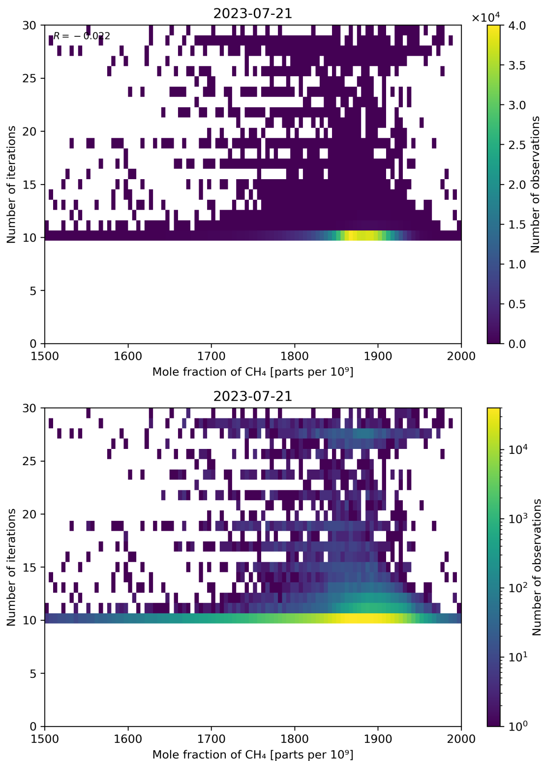
Figure 76: Scatter density plot of “Mole fraction of CH 4 ” against “Number of iterations” for 2023-07-20 to 2023-07-22.
