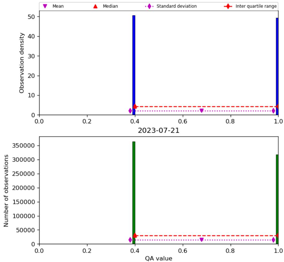
Figure 22: Histogram of "QA value" for 2023-07-20 to 2023-07-22
