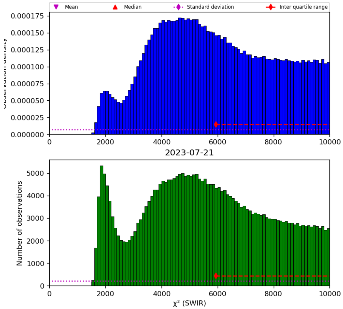
Figure 28: Histogram of “ \chi^2 (SWIR)” for 2023-07-20 to 2023-07-22
