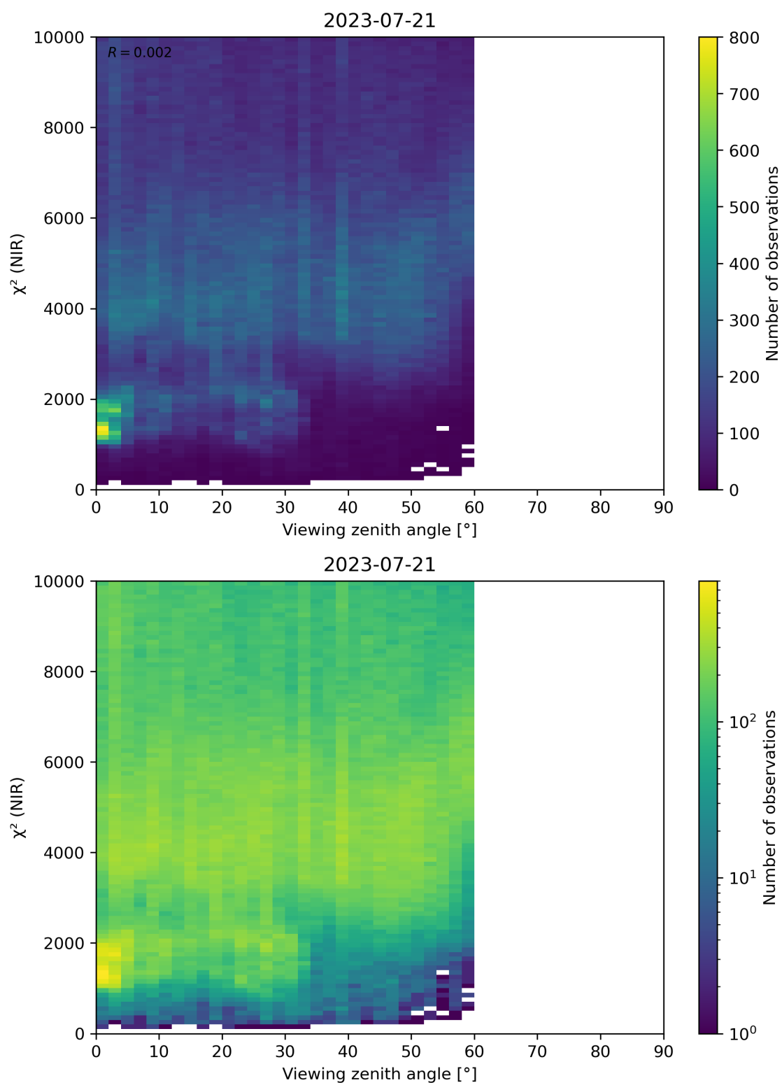
Figure 105: Scatter density plot of “Viewing zenith angle” against “ \chi^2 (NIR)” for 2023-07-20 to 2023-07-22.
