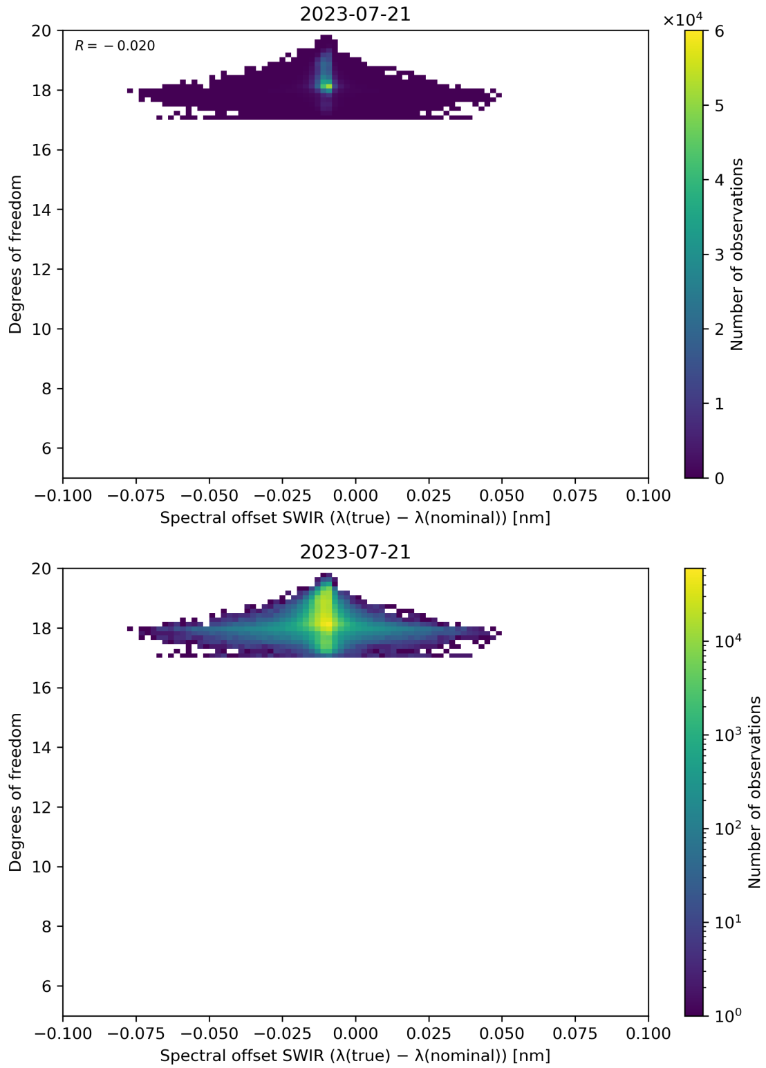
Figure 119: Scatter density plot of “Spectral offset SWIR ( \lambda(\text{true}) - \lambda(\text{nominal}) )” against “Degrees of freedom” for 2023-07-20 to 2023-07-22.
