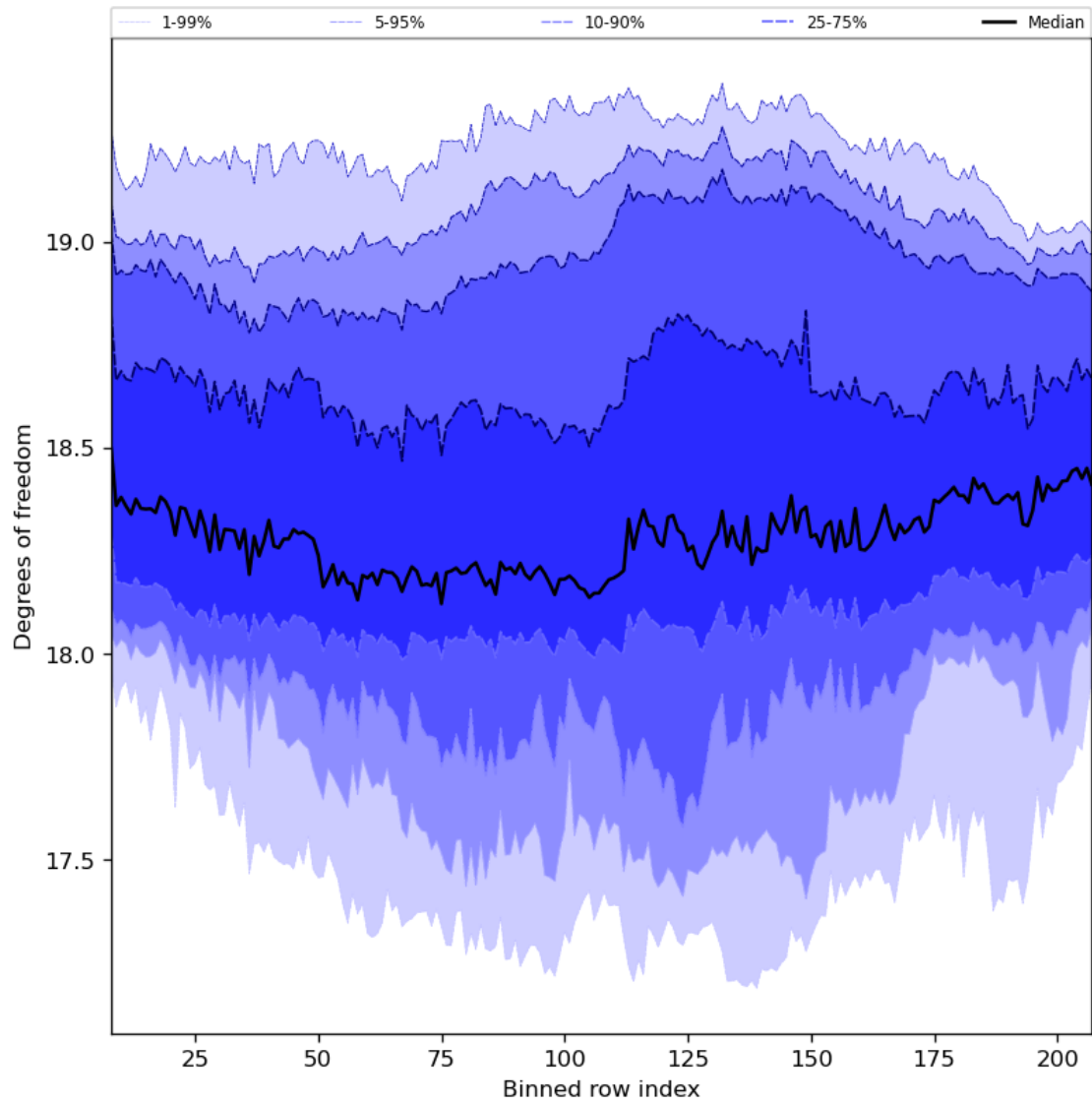
Figure 41: Along track statistics of “Degrees of freedom” for 2023-07-20 to 2023-07-22
