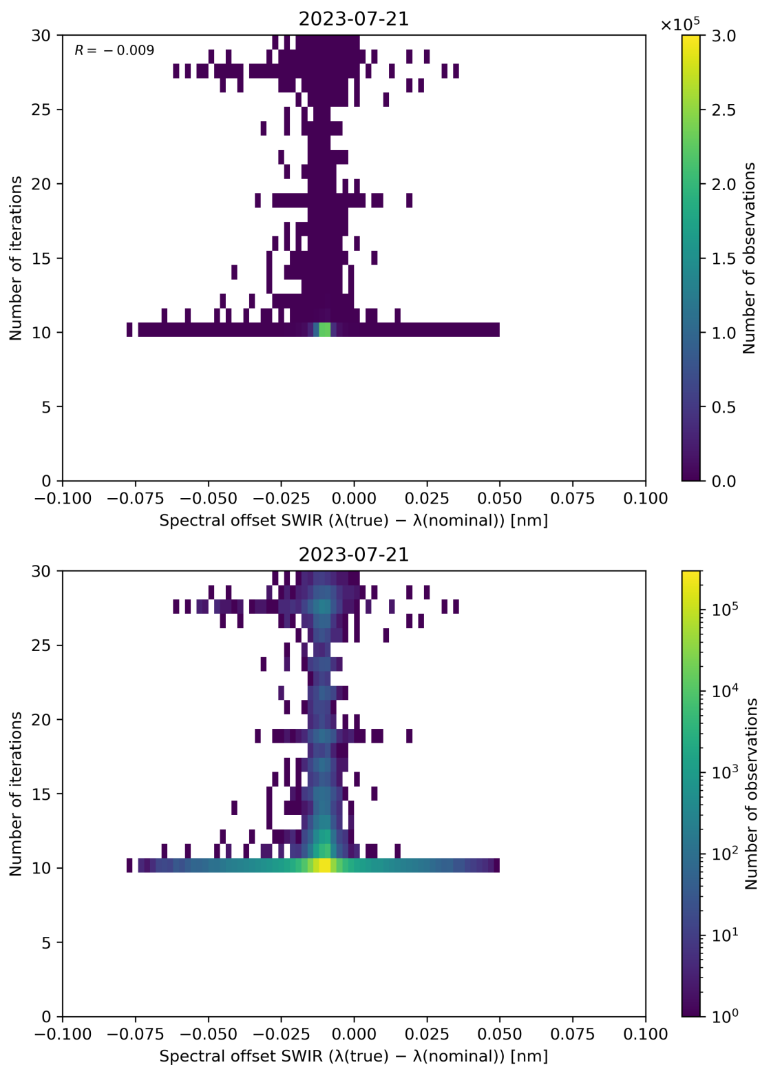
Figure 121: Scatter density plot of “Spectral offset SWIR ( \lambda(\text{true}) - \lambda(\text{nominal}) )” against “Number of iterations” for 2023-07-20 to 2023-07-22.
