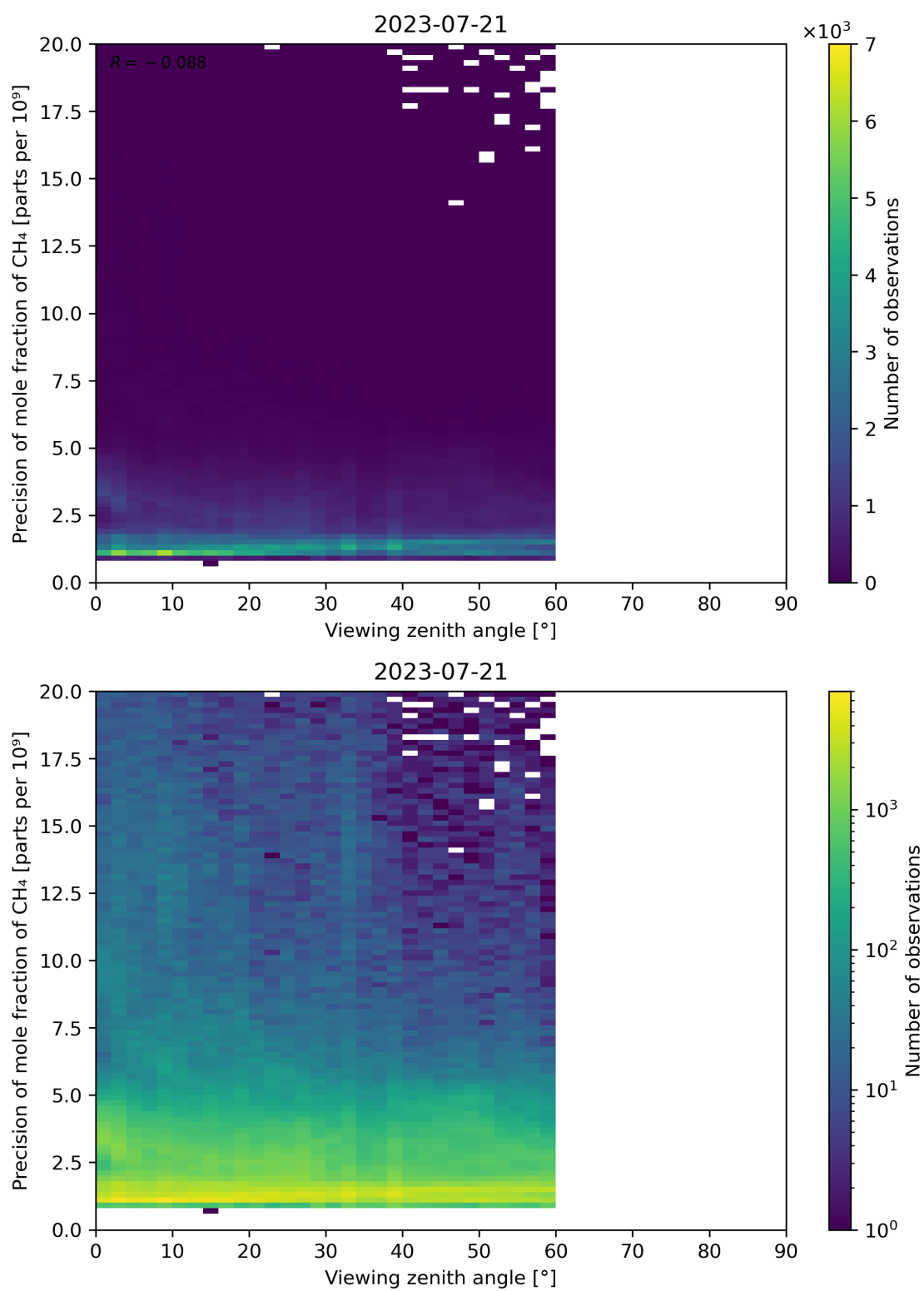
Figure 112: Scatter density plot of “Viewing zenith angle” against “Precision of mole fraction of CH 4 ” for 2023-07-20 to 2023-07-22.
