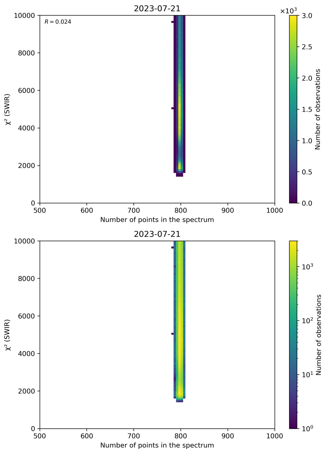
Figure 89: Scatter density plot of “Number of points in the spectrum” against “ \chi^2 (SWIR)” for 2023-07-20 to 2023-07-22.
