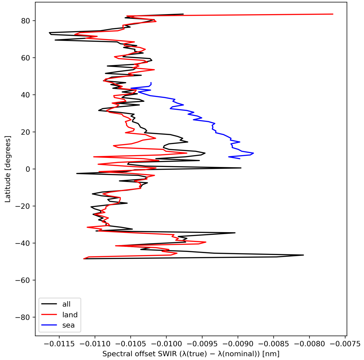
Figure 16: Zonal average of “Spectral offset SWIR ( \lambda(\text{true}) - \lambda(\text{nominal}) )” for 2023-07-20 to 2023-07-22.
