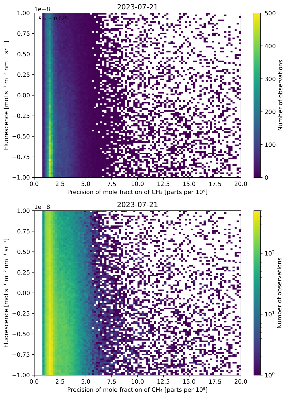
Figure 81: Scatter density plot of “Precision of mole fraction of \text{CH}_4 ” against “Fluorescence” for 2023-07-20 to 2023-07-22.
