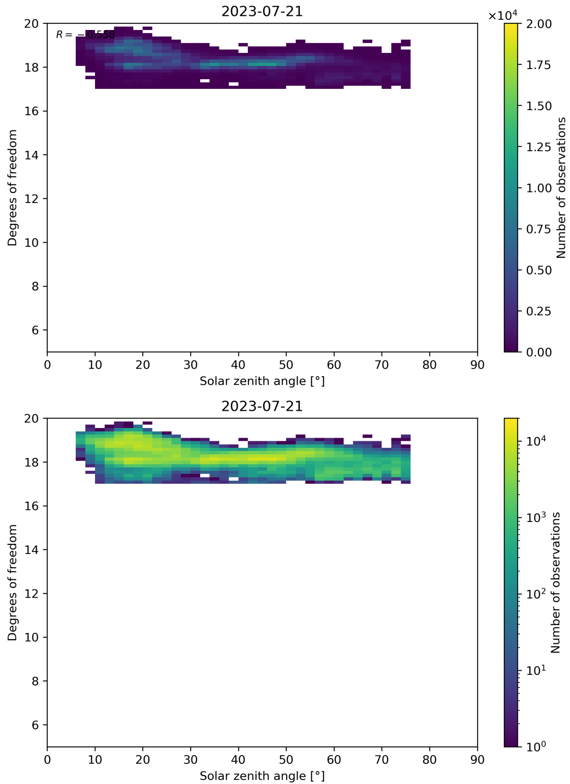
Figure 96: Scatter density plot of “Solar zenith angle” against “Degrees of freedom” for 2023-07-20 to 2023-07-22.
