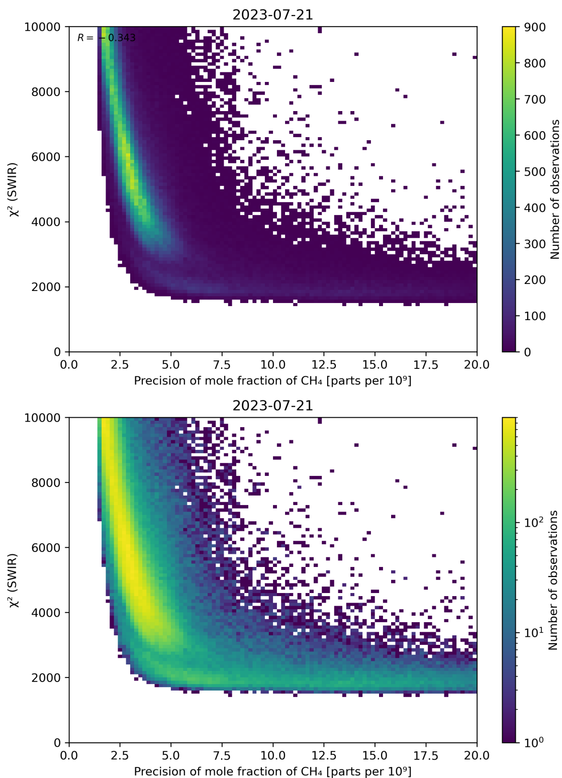
Figure 79: Scatter density plot of “Precision of mole fraction of \text{CH}_4 ” against “ \chi^2 (SWIR)” for 2023-07-20 to 2023-07-22.
