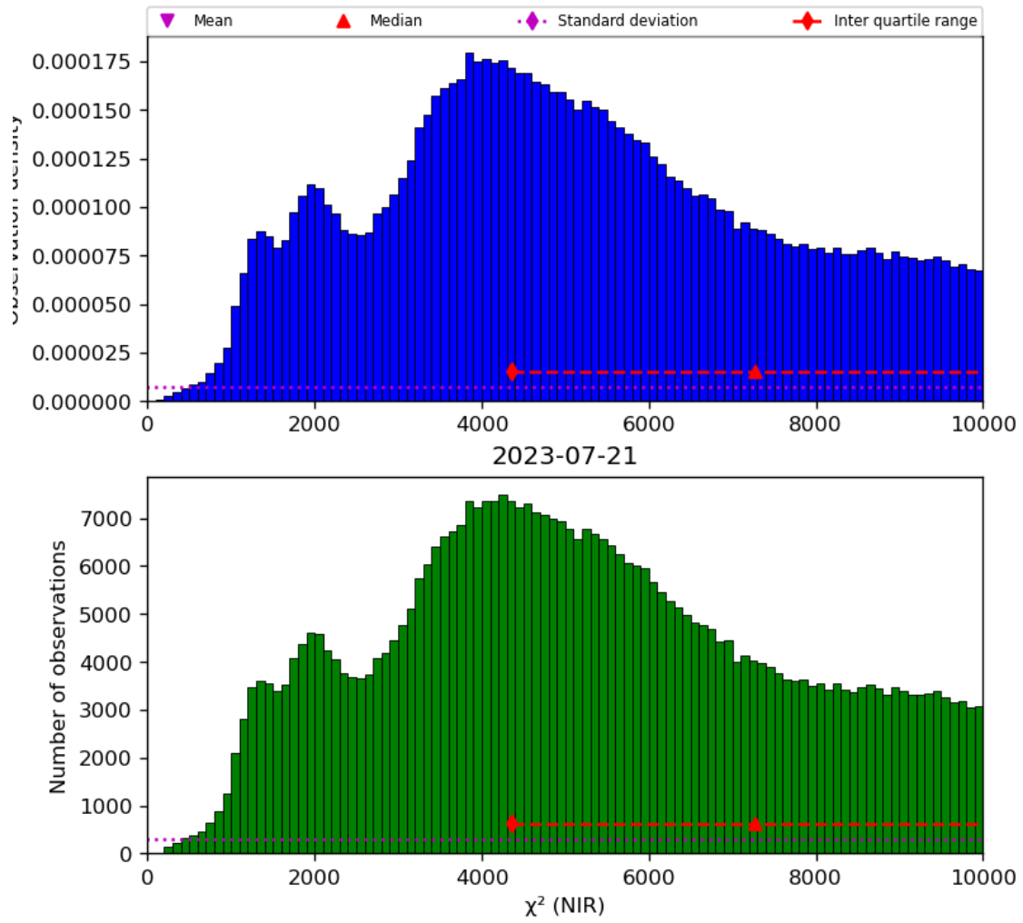
Figure 29: Histogram of “ \chi^2 (NIR)” for 2023-07-20 to 2023-07-22
