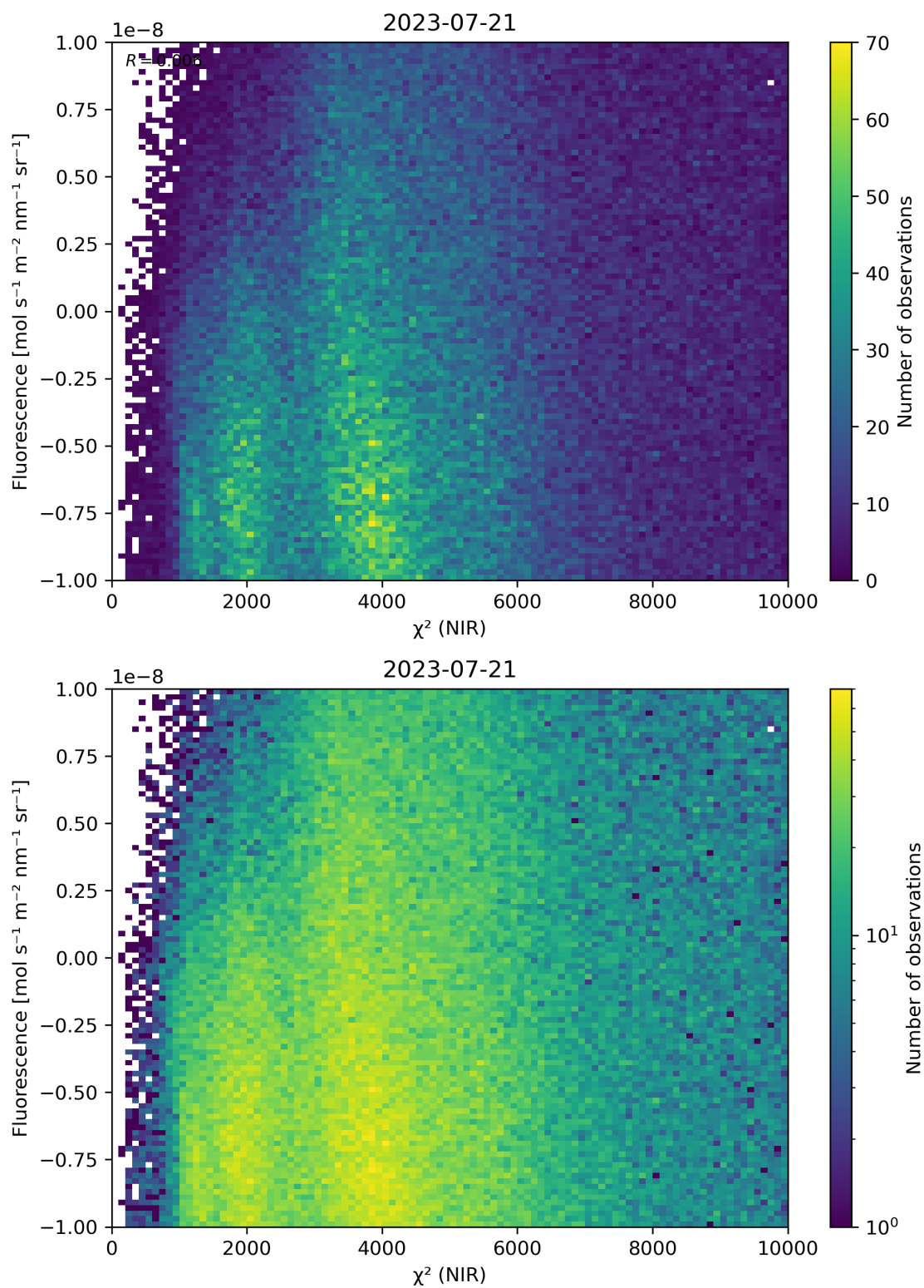
Figure 45: Scatter density plot of “ \chi^2 (NIR)” against “Fluorescence” for 2023-07-20 to 2023-07-22.
