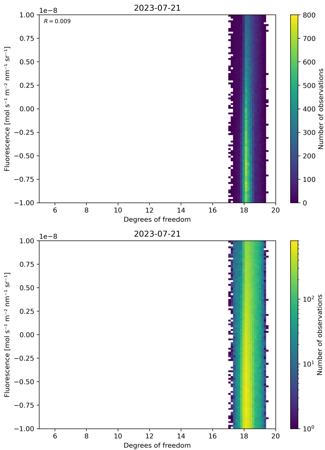
Figure 51: Scatter density plot of “Degrees of freedom” against “Fluorescence” for 2023-07-20 to 2023-07-22.
