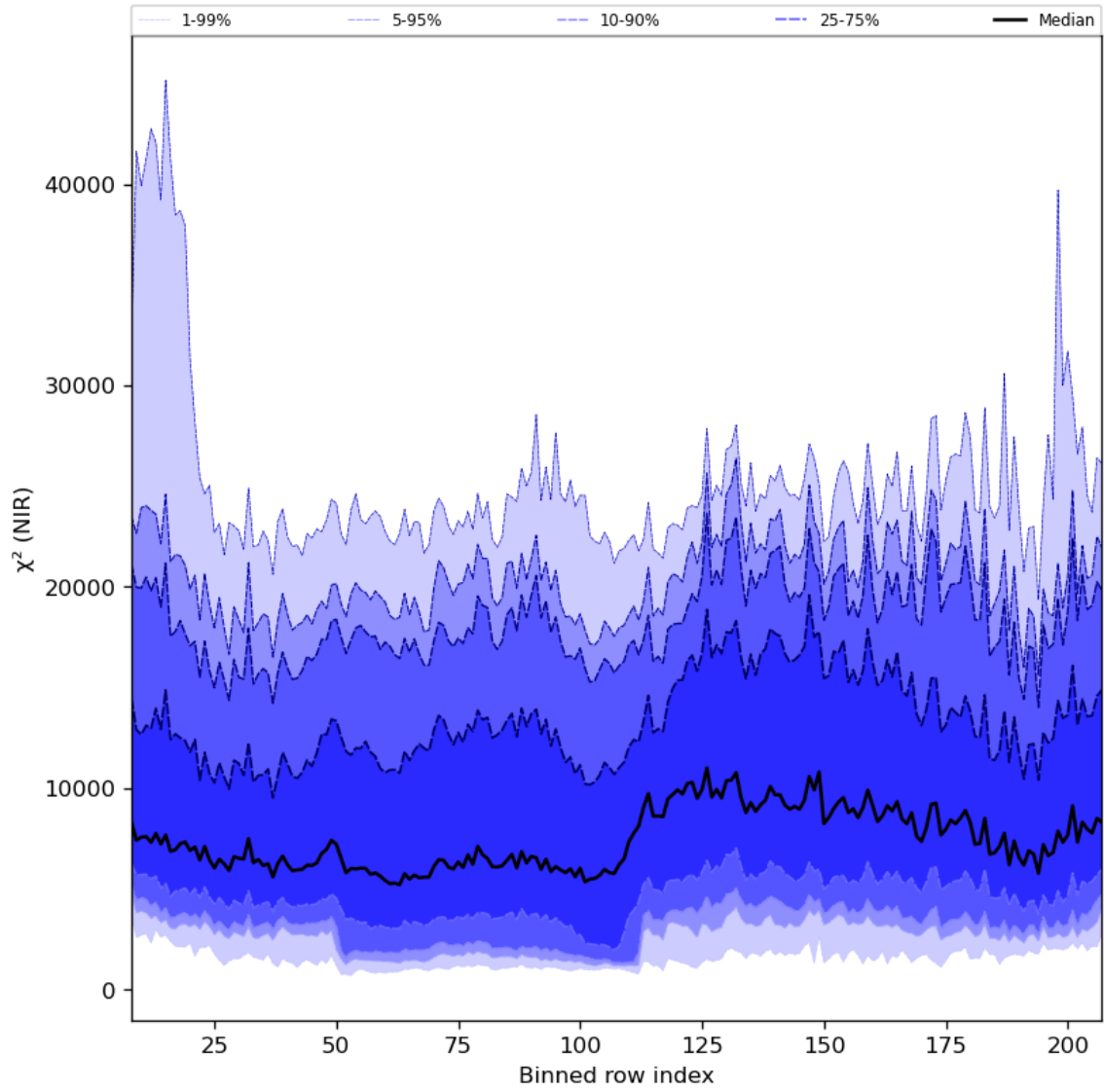
Figure 40: Along track statistics of " \chi^2 (NIR)" for 2023-07-20 to 2023-07-22
