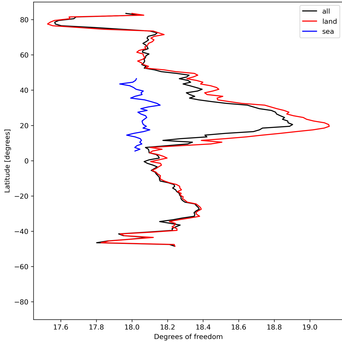
Figure 19: Zonal average of “Degrees of freedom” for 2023-07-20 to 2023-07-22.
