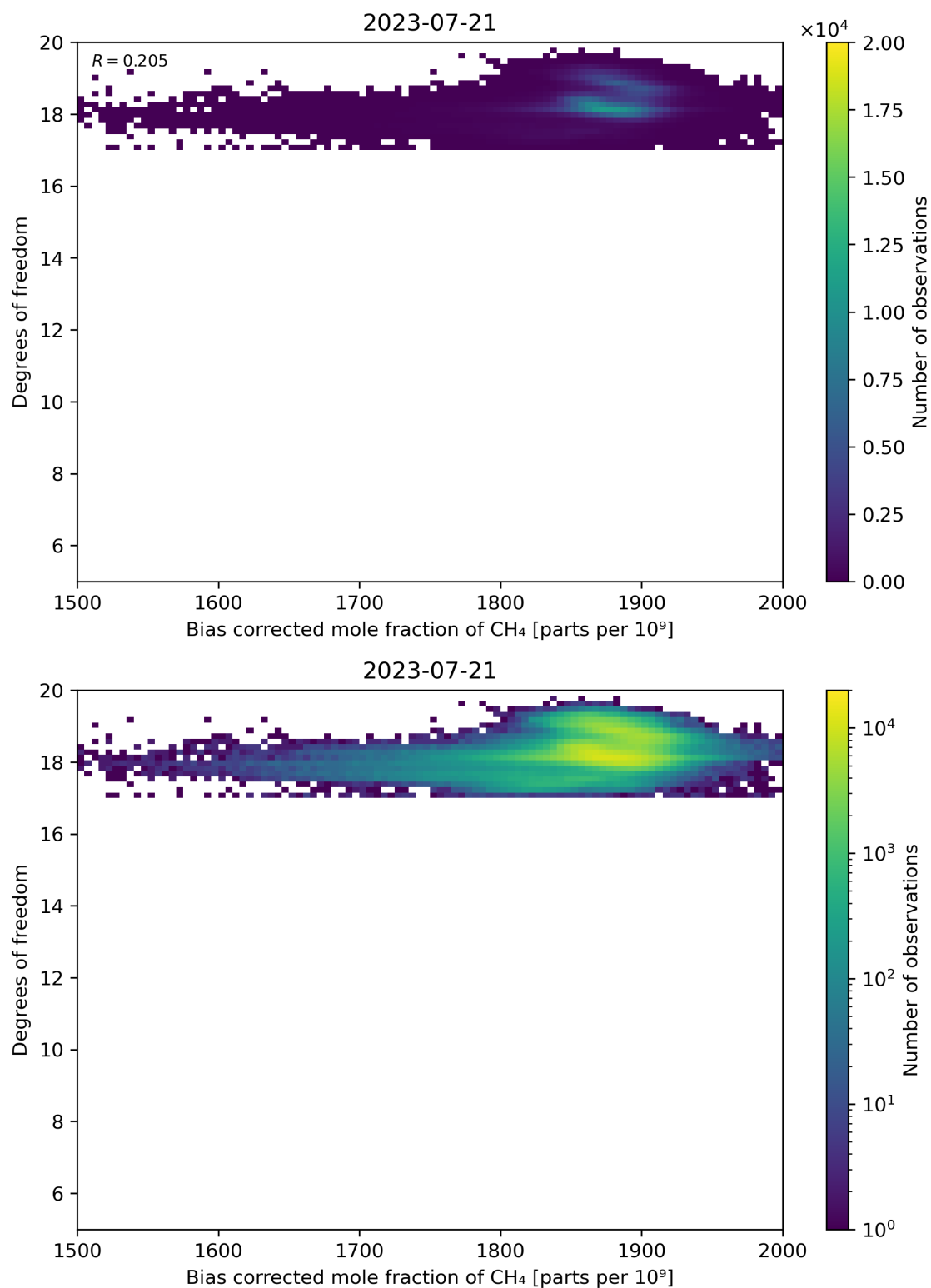
Figure 65: Scatter density plot of “Bias corrected mole fraction of CH 4 ” against “Degrees of freedom” for 2023-07-20 to 2023-07-22.
