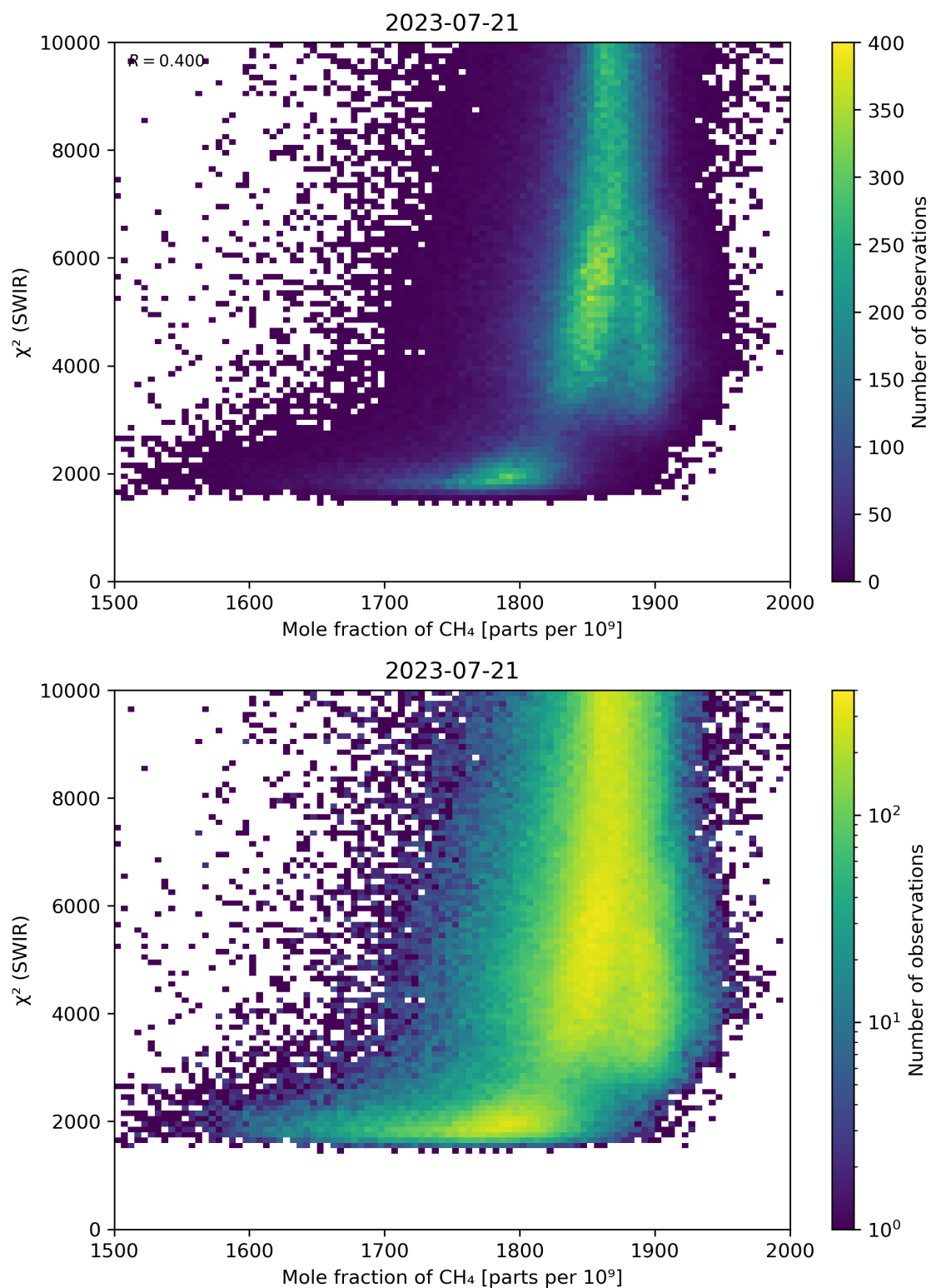
Figure 71: Scatter density plot of “Mole fraction of \text{CH}_4 ” against “ \chi^2 (SWIR)” for 2023-07-20 to 2023-07-22.
