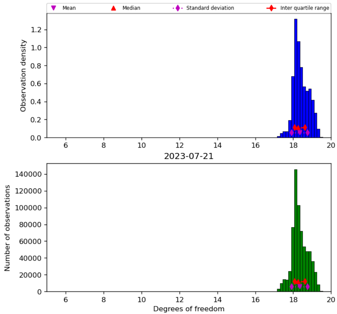
Figure 30: Histogram of “Degrees of freedom” for 2023-07-20 to 2023-07-22
