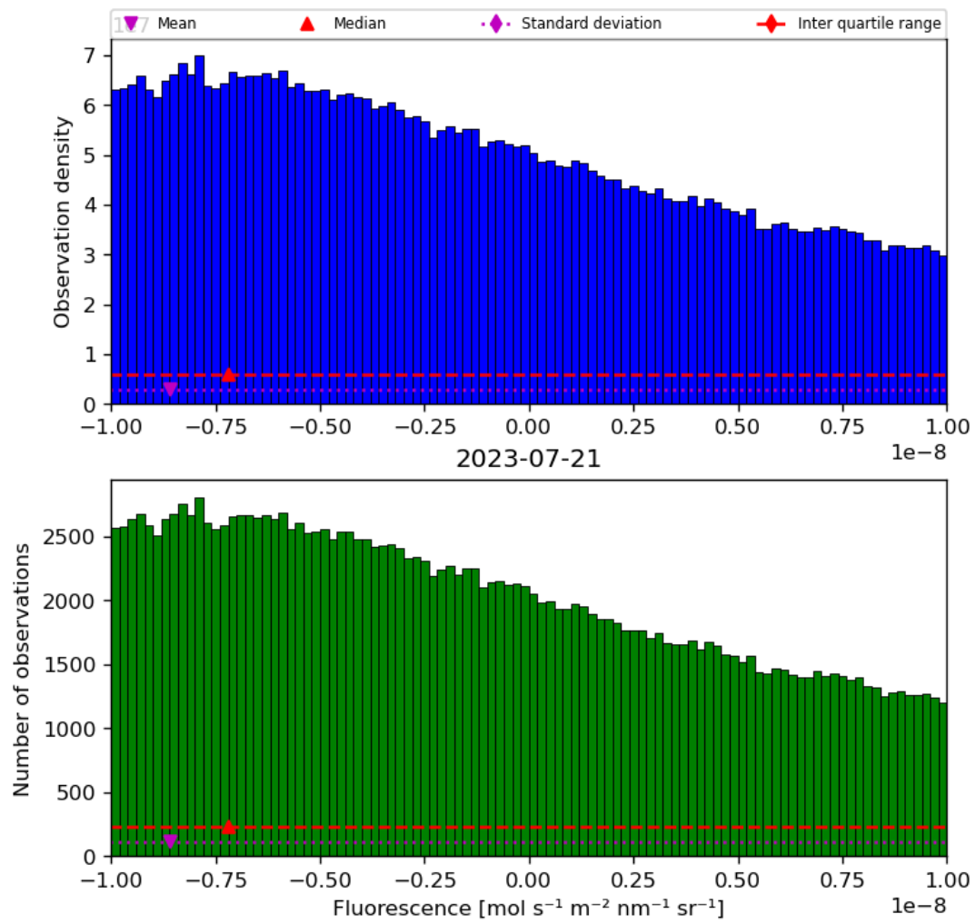
Figure 32: Histogram of “Fluorescence” for 2023-07-20 to 2023-07-22
