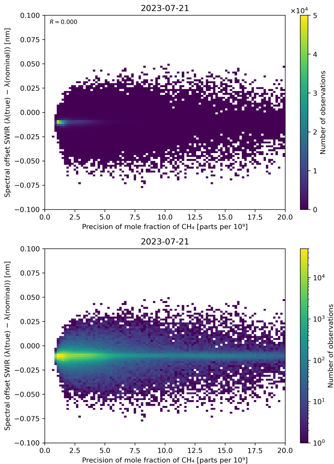
Figure 85: Scatter density plot of “Precision of mole fraction of CH 4 ” against “Spectral offset SWIR ( \lambda(\text{true}) - \lambda(\text{nominal}) )” for 2023-07-20 to 2023-07-22.
