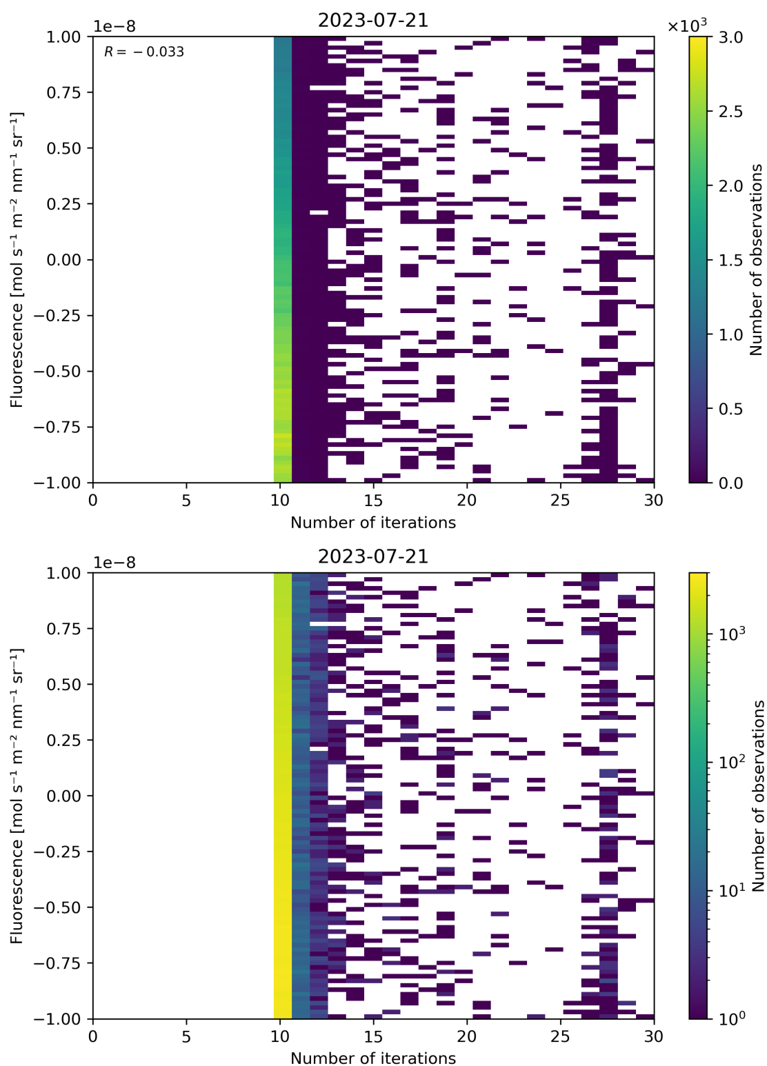
Figure 87: Scatter density plot of “Number of iterations” against “Fluorescence” for 2023-07-20 to 2023-07-22.
