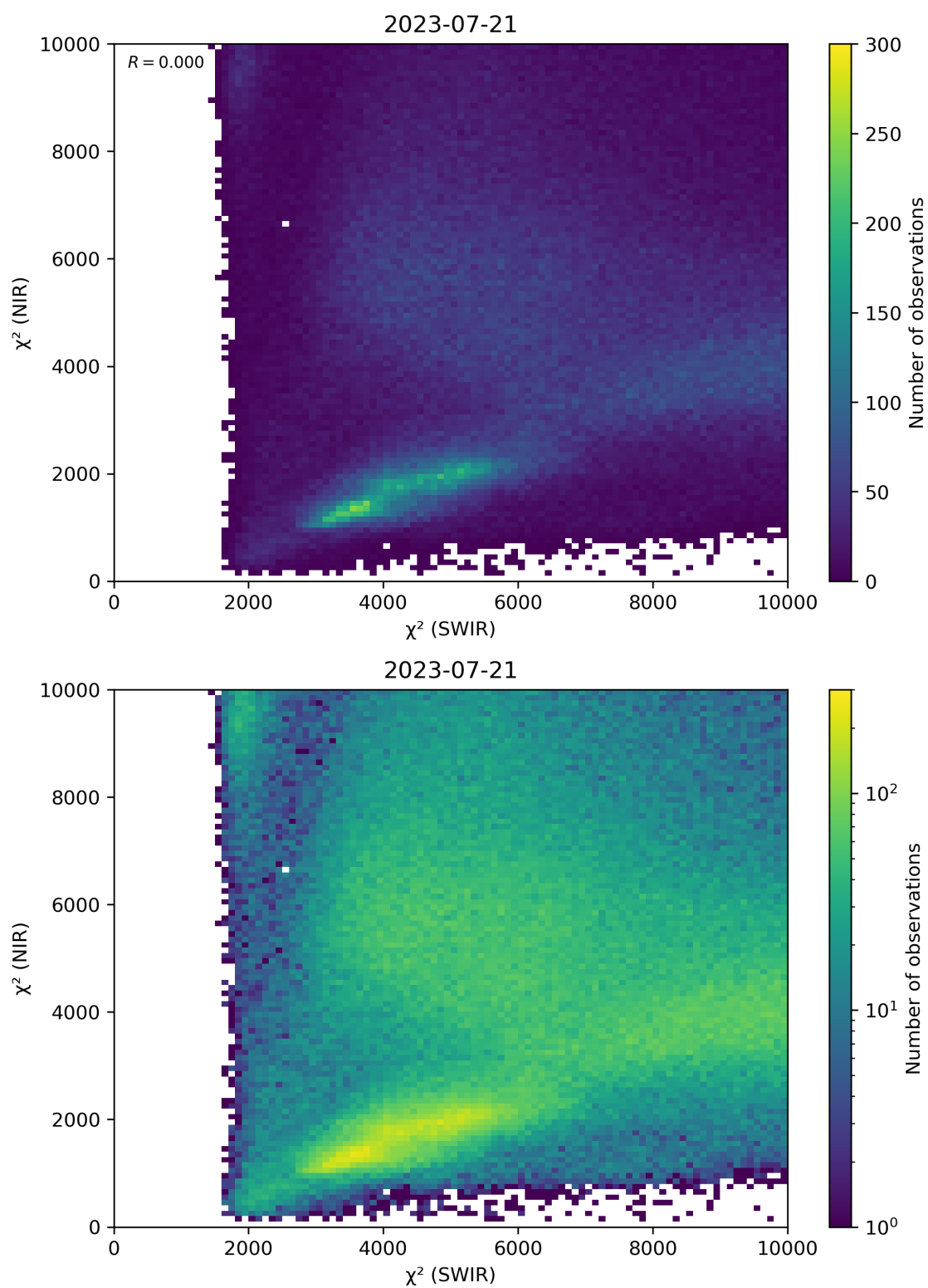
Figure 47: Scatter density plot of “ \chi^2 (SWIR)” against “ \chi^2 (NIR)” for 2023-07-20 to 2023-07-22.
