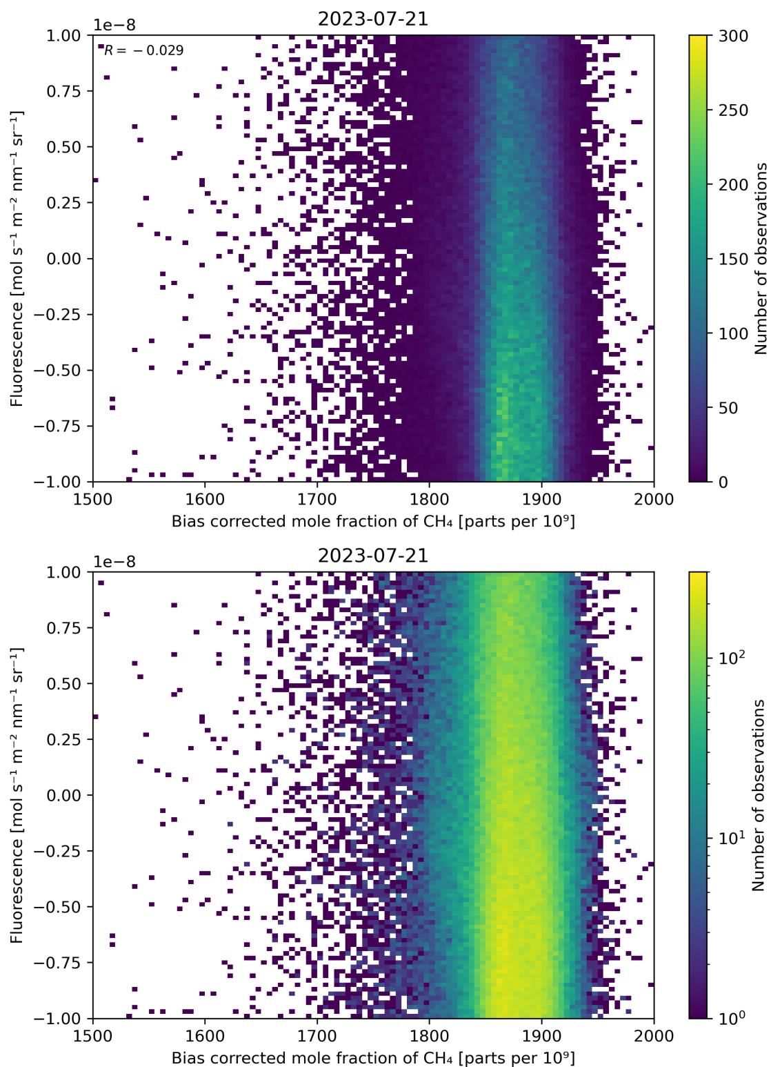
Figure 66: Scatter density plot of “Bias corrected mole fraction of \text{CH}_4 ” against “Fluorescence” for 2023-07-20 to 2023-07-22.
