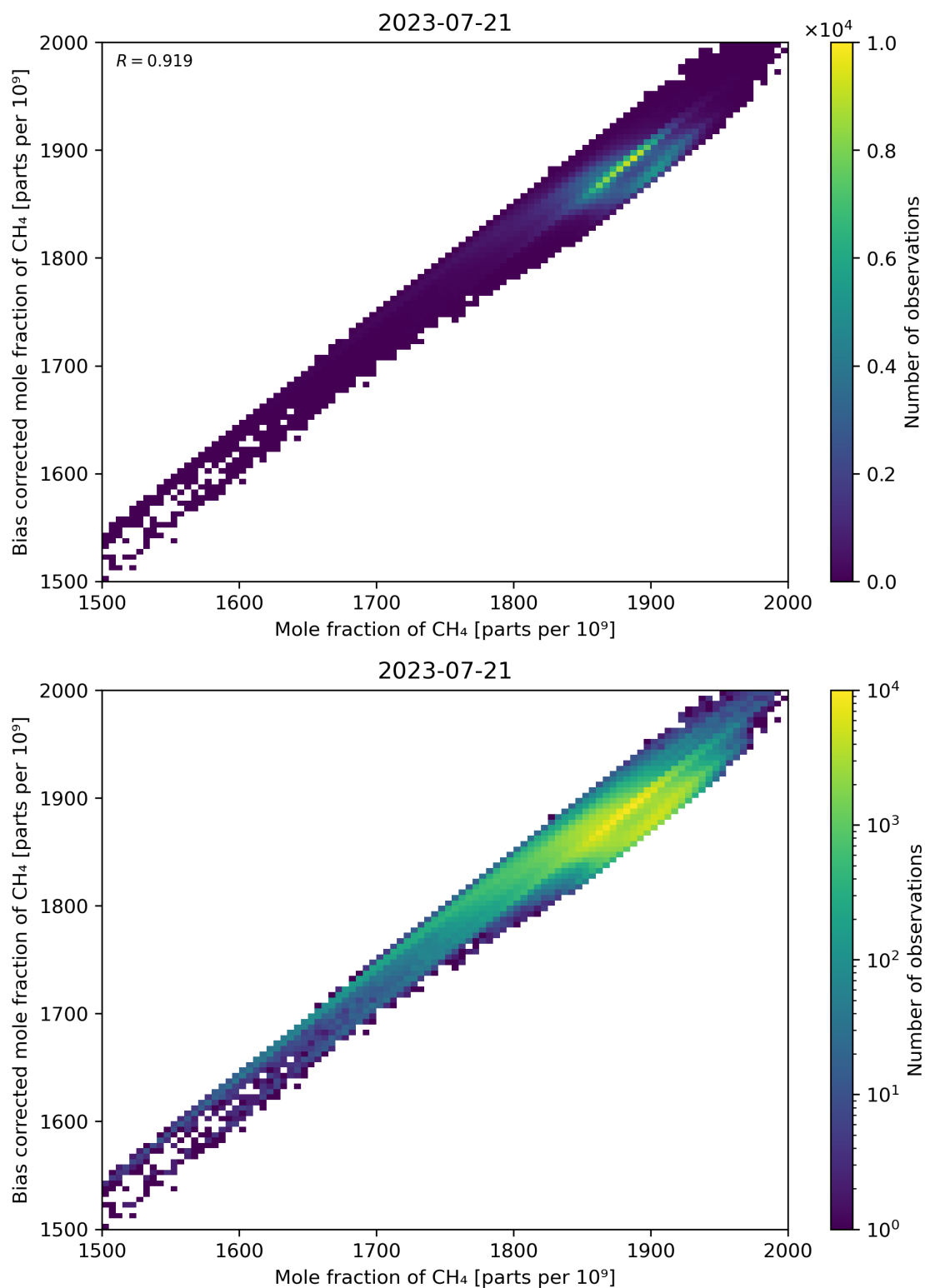
Figure 74: Scatter density plot of “Mole fraction of CH 4 ” against “Bias corrected mole fraction of CH 4 ” for 2023-07-20 to 2023-07-22.
