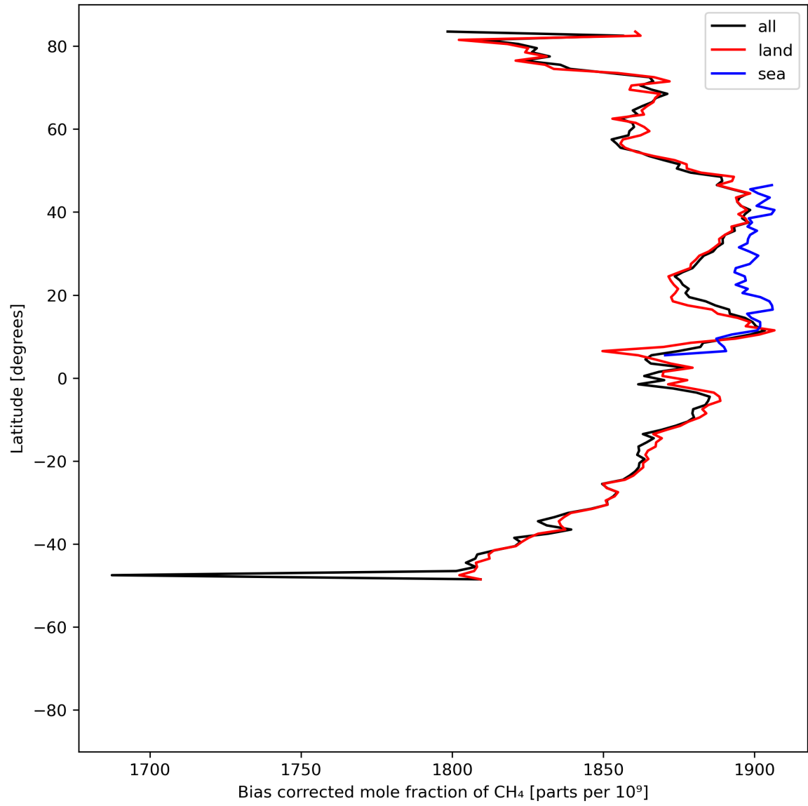
Figure 14: Zonal average of “Bias corrected mole fraction of CH 4 ” for 2023-07-20 to 2023-07-22.
