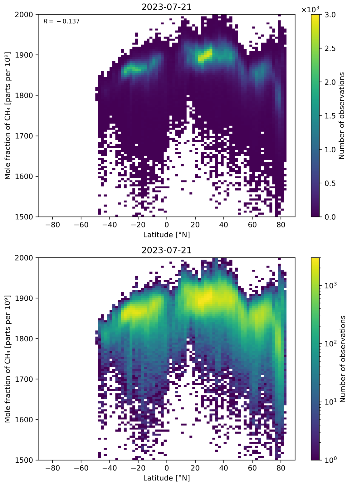
Figure 57: Scatter density plot of “Latitude” against “Mole fraction of \text{CH}_4 ” for 2023-07-20 to 2023-07-22.
