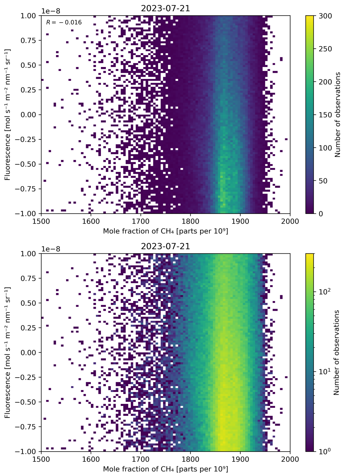
Figure 73: Scatter density plot of “Mole fraction of \text{CH}_4 ” against “Fluorescence” for 2023-07-20 to 2023-07-22.
