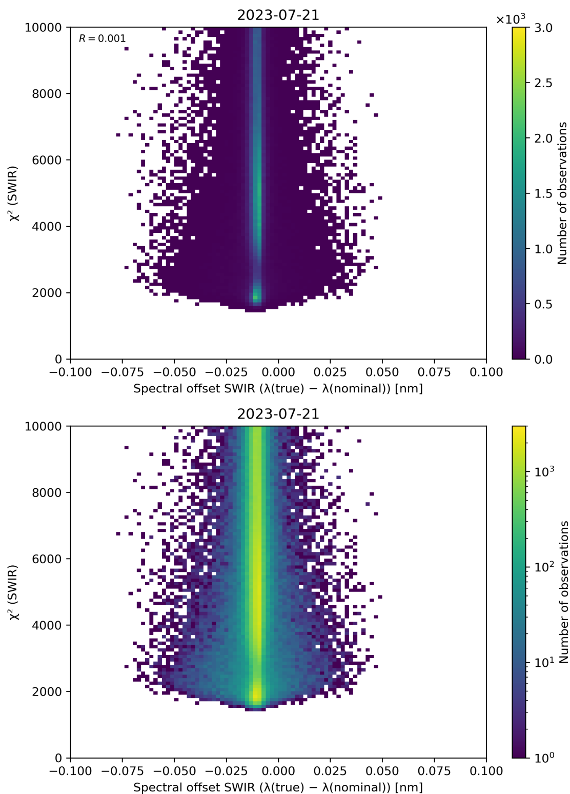
Figure 118: Scatter density plot of “Spectral offset SWIR ( \lambda(\text{true}) - \lambda(\text{nominal}) )” against “ \chi^2 (SWIR)” for 2023-07-20 to 2023-07-22.
