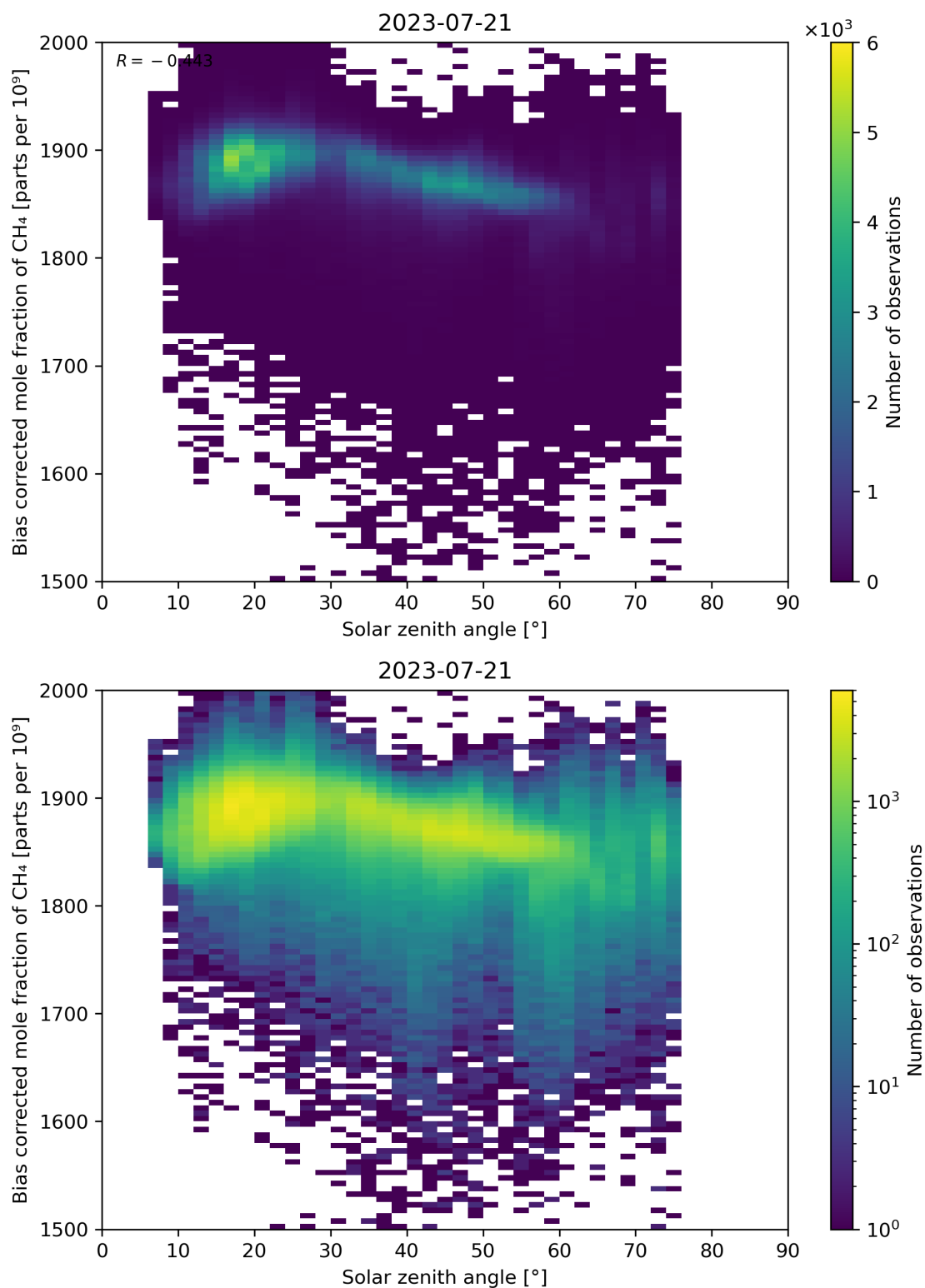
Figure 100: Scatter density plot of “Solar zenith angle” against “Bias corrected mole fraction of CH 4 ” for 2023-07-20 to 2023-07-22.
