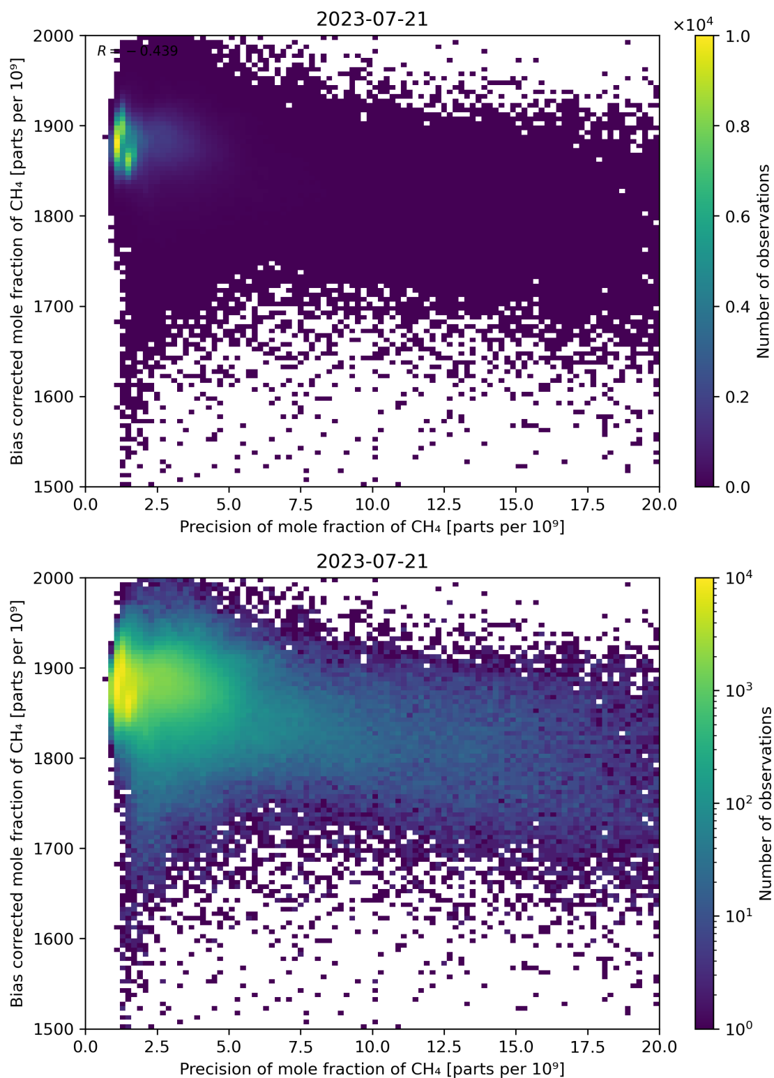
Figure 82: Scatter density plot of “Precision of mole fraction of CH 4 ” against “Bias corrected mole fraction of CH 4 ” for 2023-07-20 to 2023-07-22.
