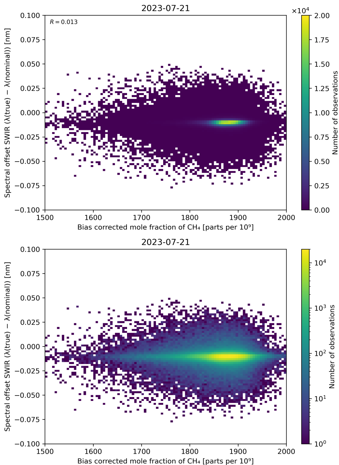
Figure 69: Scatter density plot of “Bias corrected mole fraction of \text{CH}_4 ” against “Spectral offset SWIR ( \lambda(\text{true}) - \lambda(\text{nominal}) )” for 2023-07-20 to 2023-07-22.
