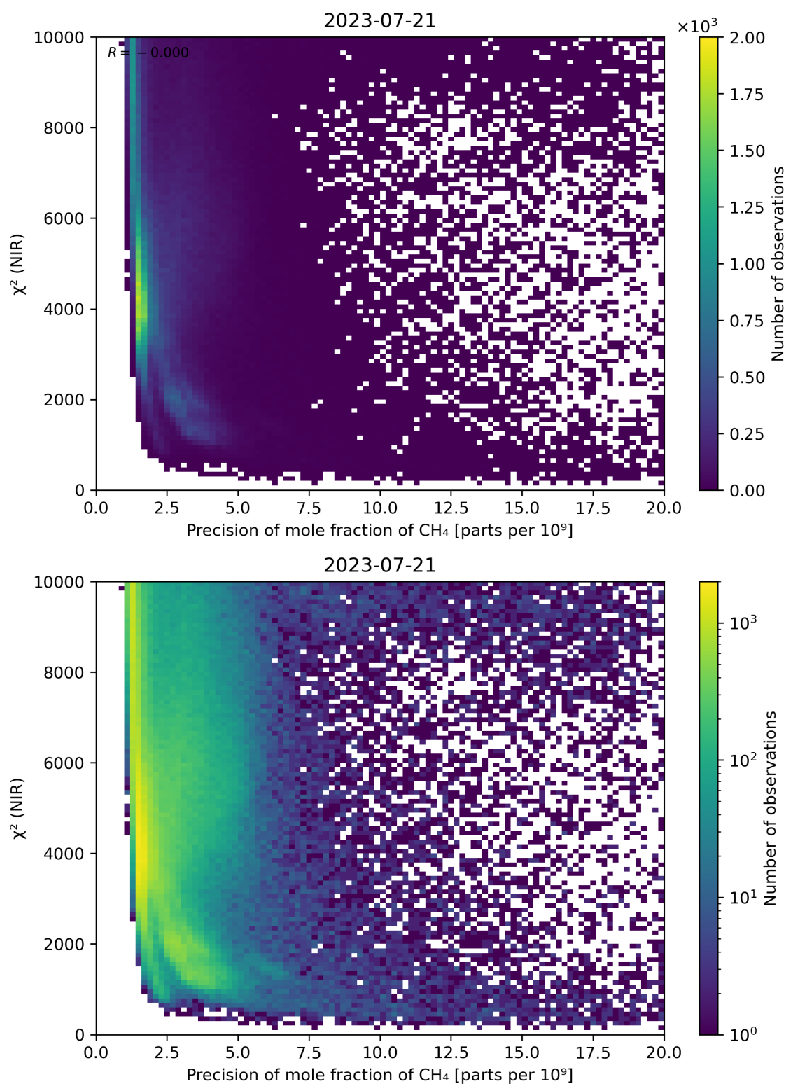
Figure 78: Scatter density plot of “Precision of mole fraction of CH 4 ” against “ \chi^2 (NIR)” for 2023-07-20 to 2023-07-22.
