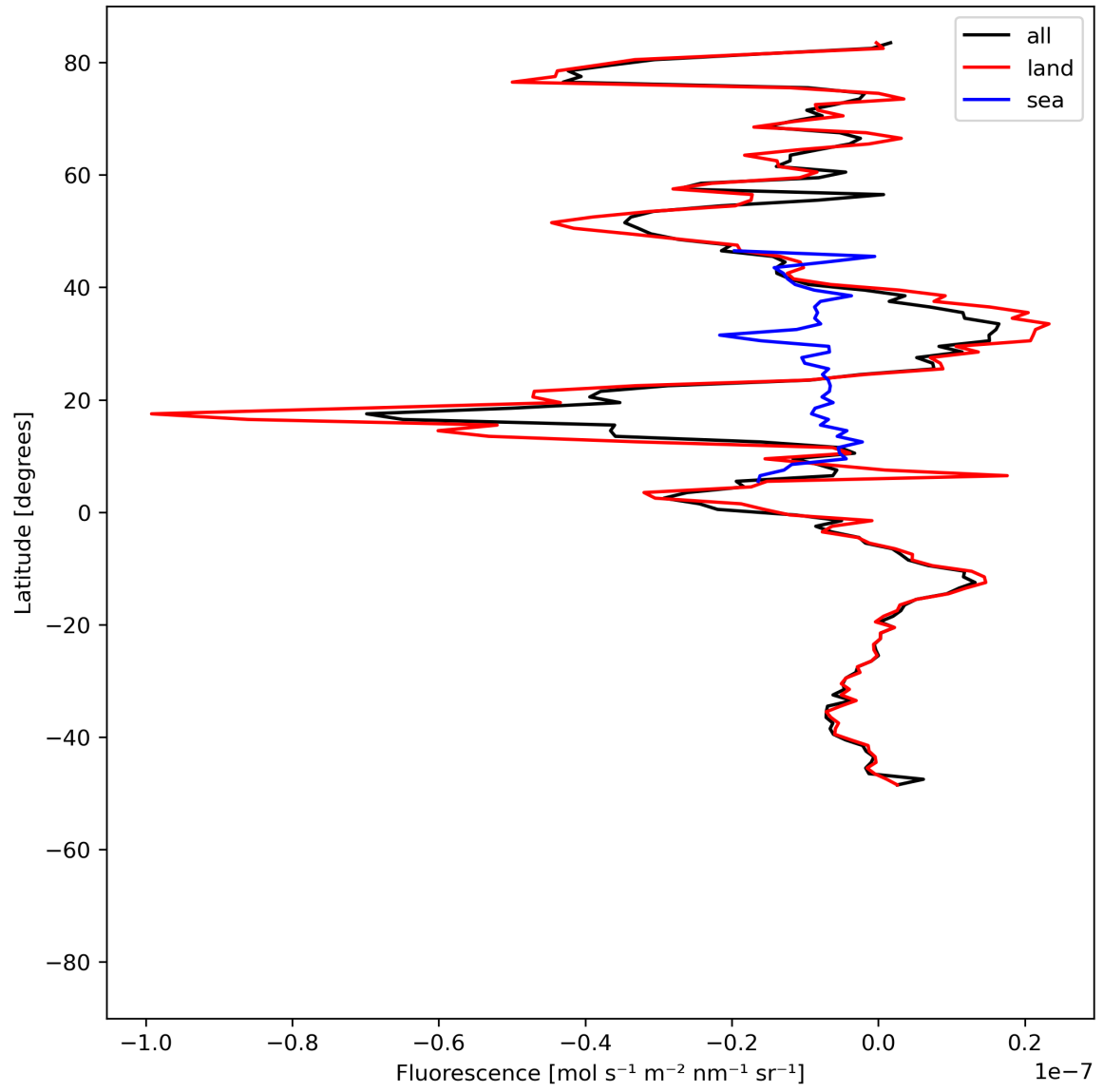
Figure 21: Zonal average of “Fluorescence” for 2023-07-20 to 2023-07-22.
