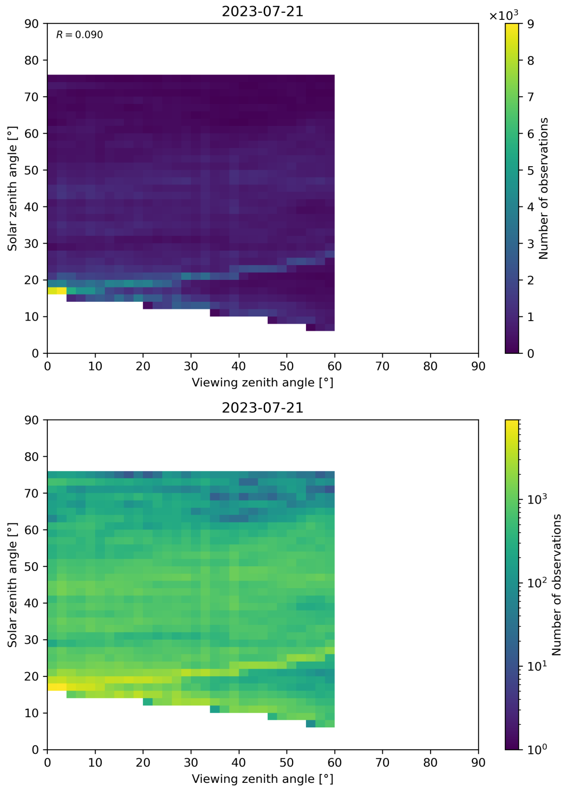
Figure 115: Scatter density plot of “Viewing zenith angle” against “Solar zenith angle” for 2023-07-20 to 2023-07-22.
