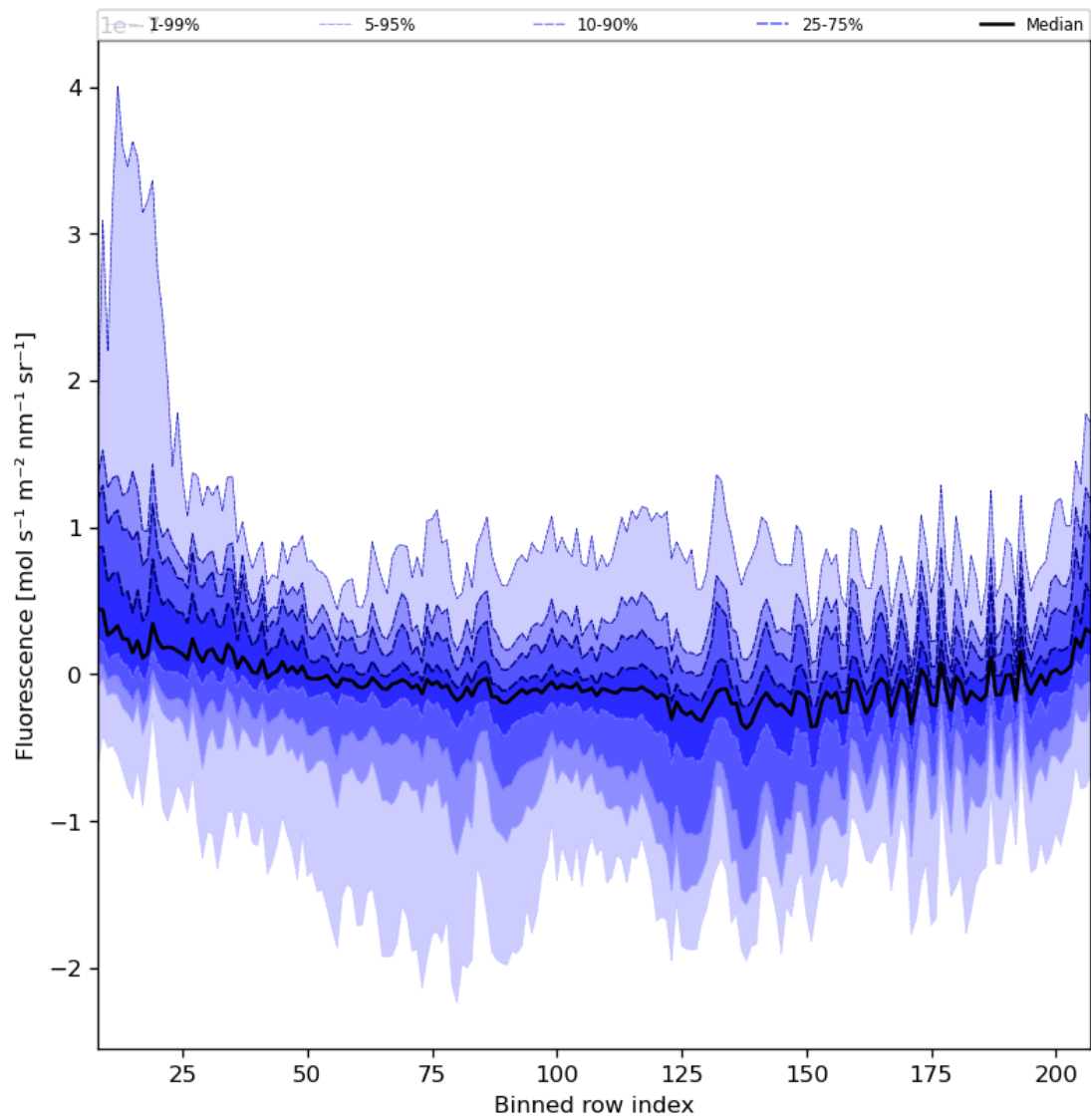
Figure 43: Along track statistics of "Fluorescence" for 2023-07-20 to 2023-07-22
