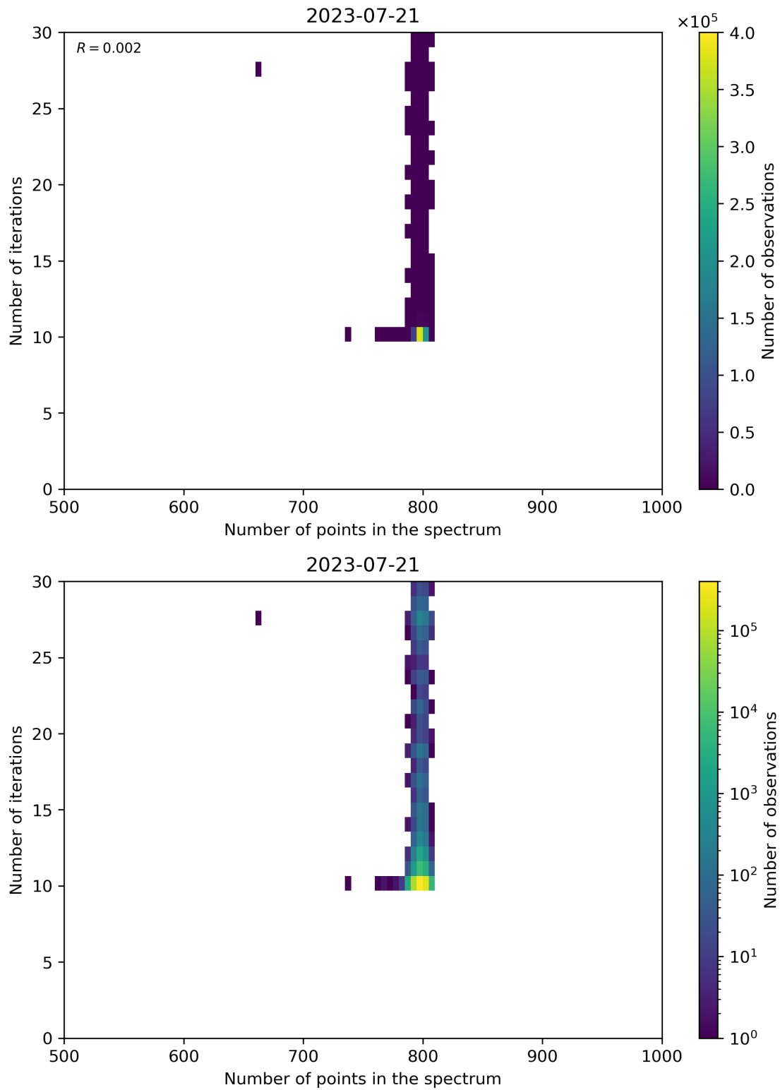
Figure 92: Scatter density plot of “Number of points in the spectrum” against “Number of iterations” for 2023-07-20 to 2023-07-22.
