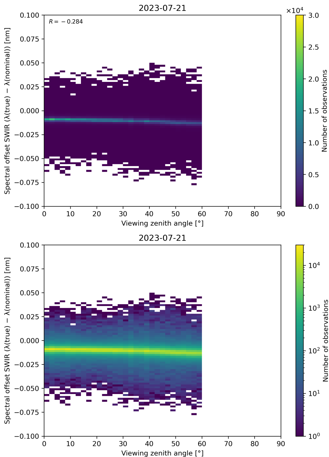
Figure 116: Scatter density plot of “Viewing zenith angle” against “Spectral offset SWIR ( \lambda(\text{true}) - \lambda(\text{nominal}) )” for 2023-07-20 to 2023-07-22.
