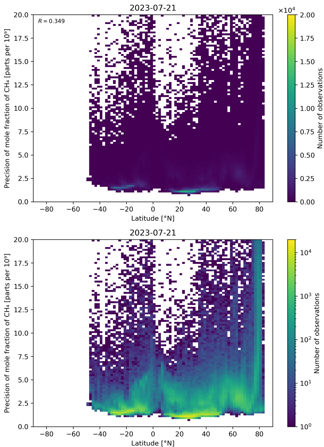
Figure 59: Scatter density plot of “Latitude” against “Precision of mole fraction of \text{CH}_4 ” for 2023-07-20 to 2023-07-22.
