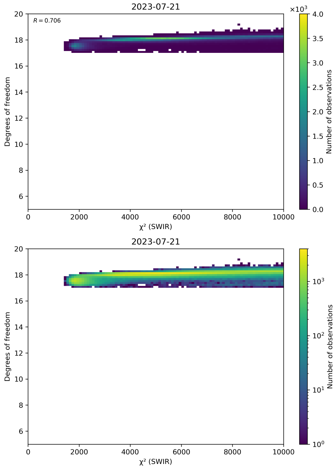
Figure 48: Scatter density plot of “ \chi^2 (SWIR)” against “Degrees of freedom” for 2023-07-20 to 2023-07-22.
