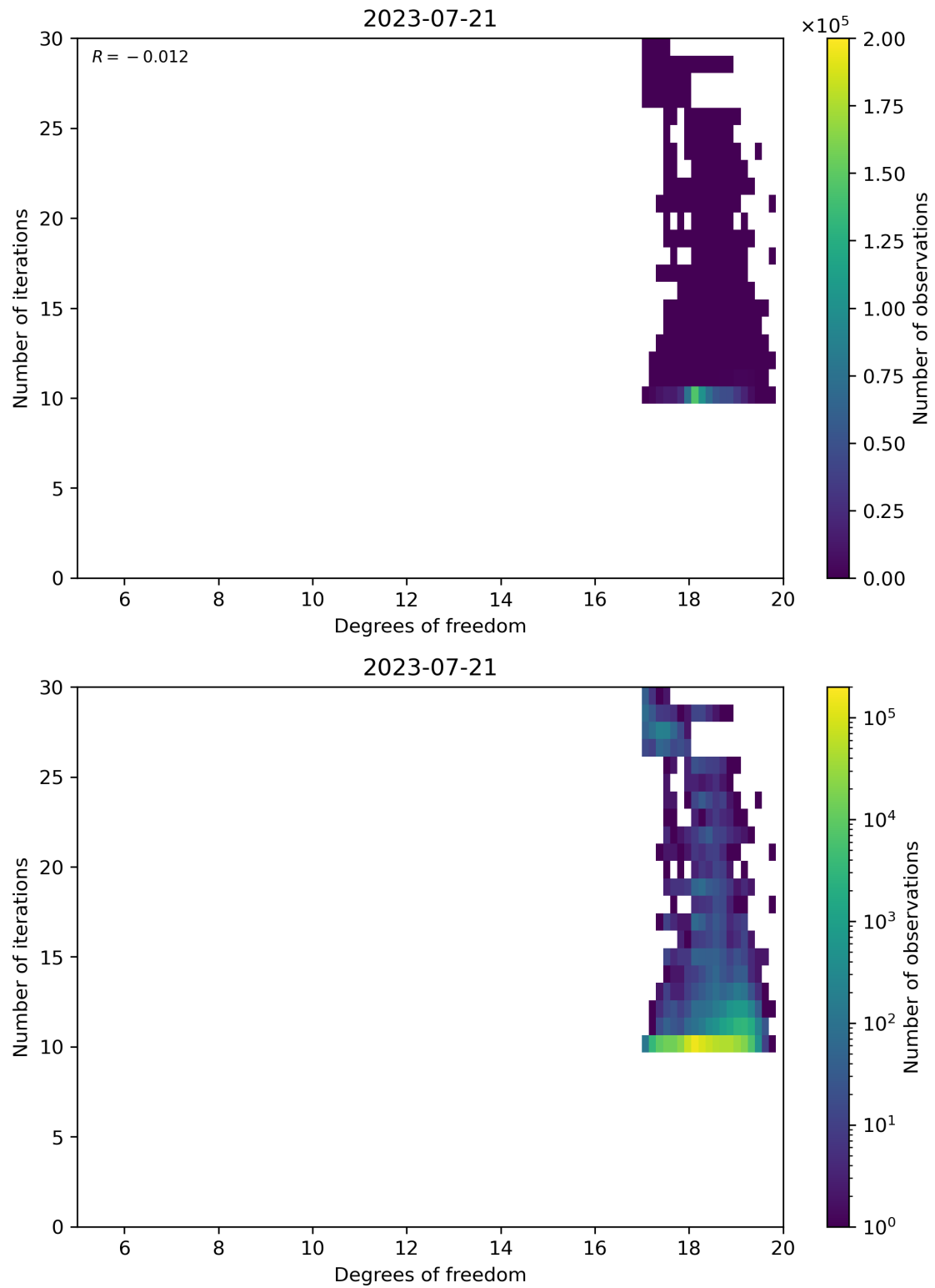
Figure 52: Scatter density plot of “Degrees of freedom” against “Number of iterations” for 2023-07-20 to 2023-07-22.
