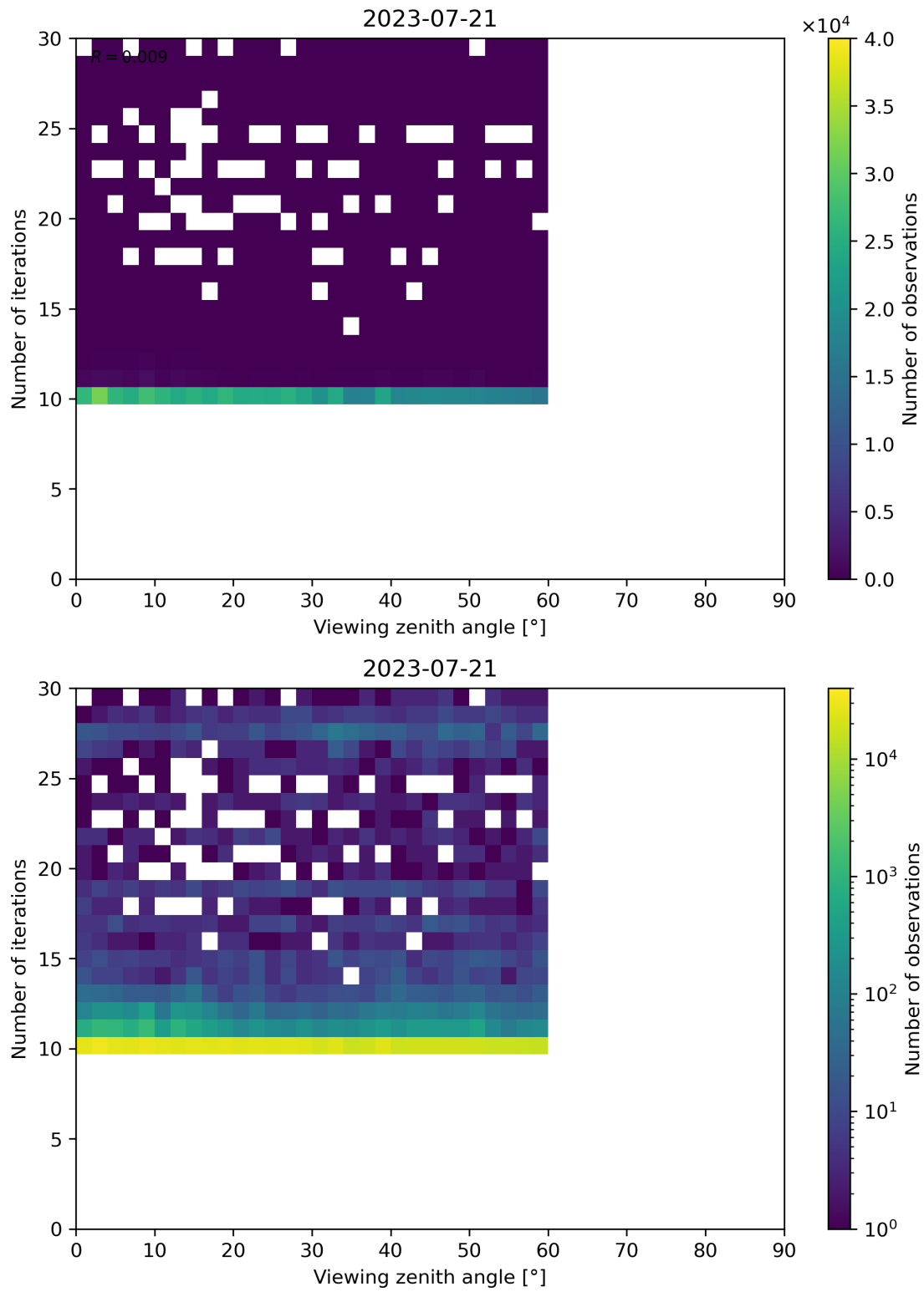
Figure 113: Scatter density plot of “Viewing zenith angle” against “Number of iterations” for 2023-07-20 to 2023-07-22.
