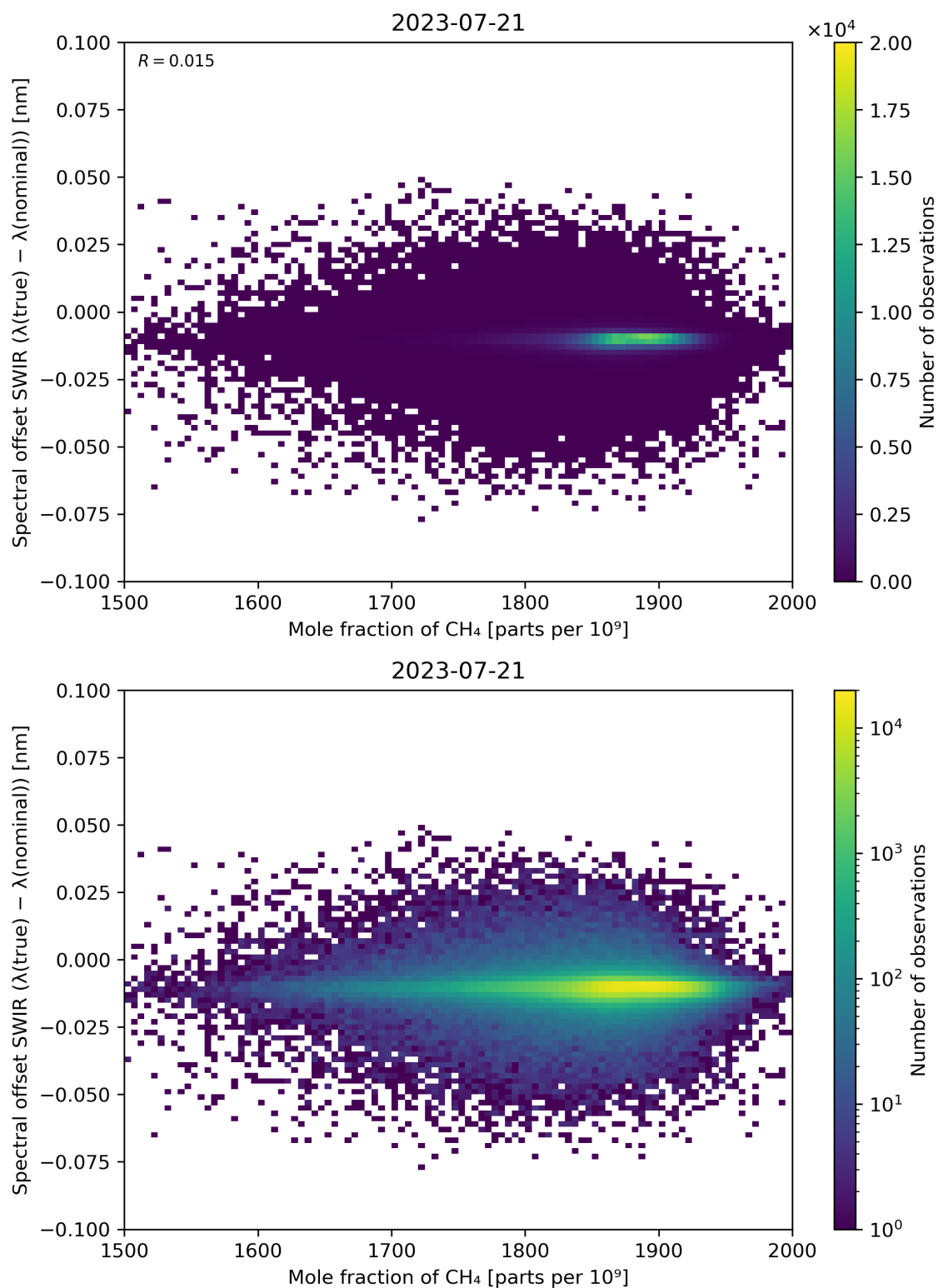
Figure 86: Scatter density plot of “Mole fraction of CH 4 ” against “Spectral offset SWIR ( \lambda(\text{true}) - \lambda(\text{nominal}) )” for 2023-07-20 to 2023-07-22.
