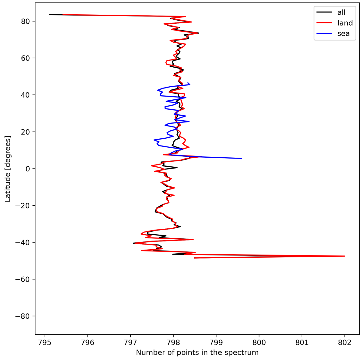
Figure 15: Zonal average of “Number of points in the spectrum” for 2023-07-20 to 2023-07-22.
