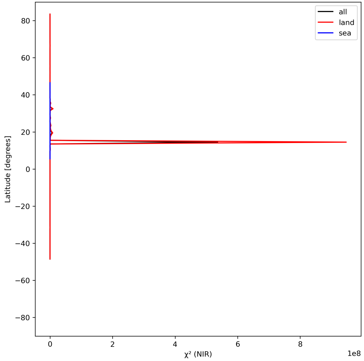
Figure 18: Zonal average of “ \chi^2 (NIR)” for 2023-07-20 to 2023-07-22.
