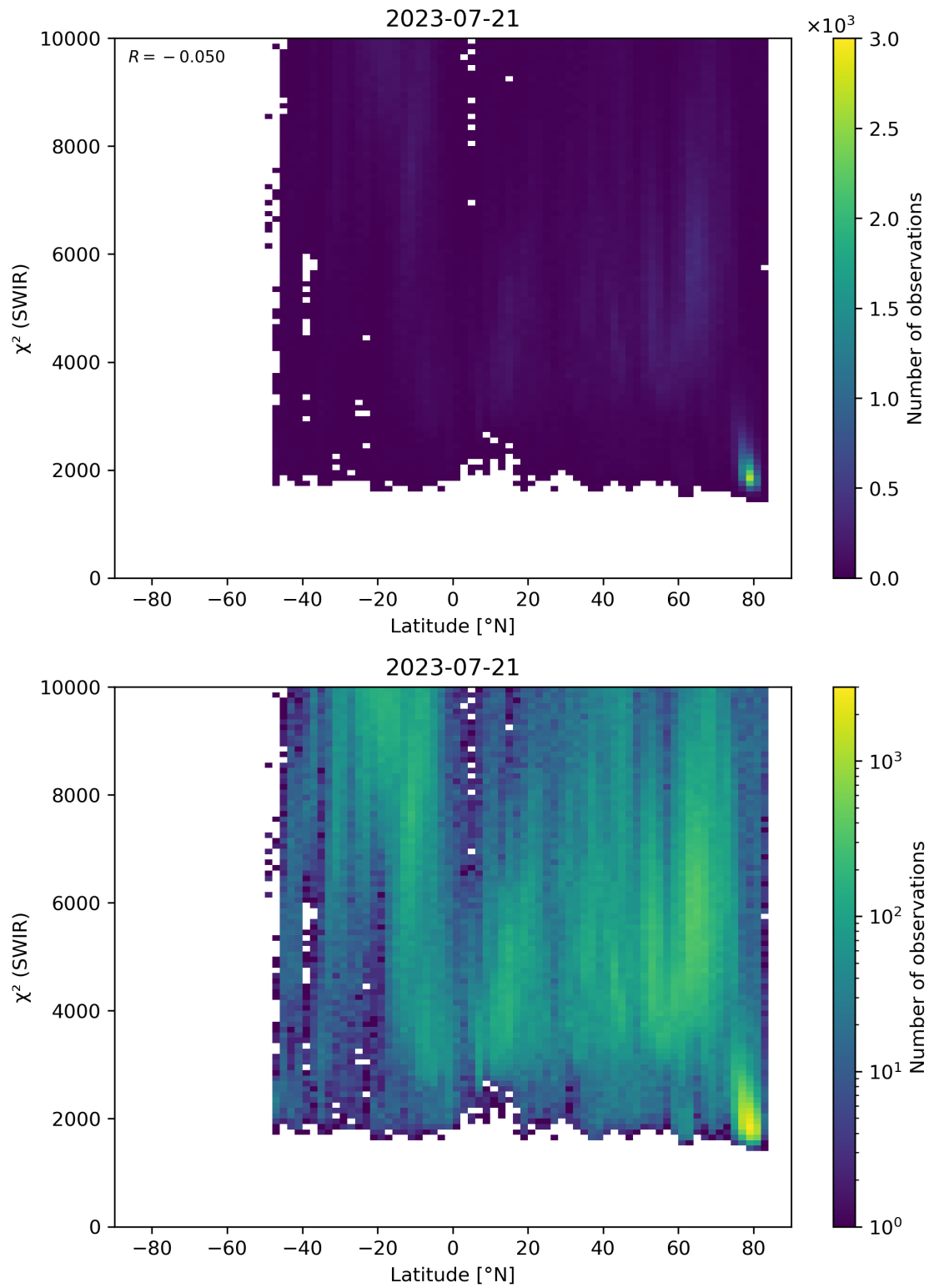
Figure 54: Scatter density plot of “Latitude” against “ \chi^2 (SWIR)” for 2023-07-20 to 2023-07-22.
