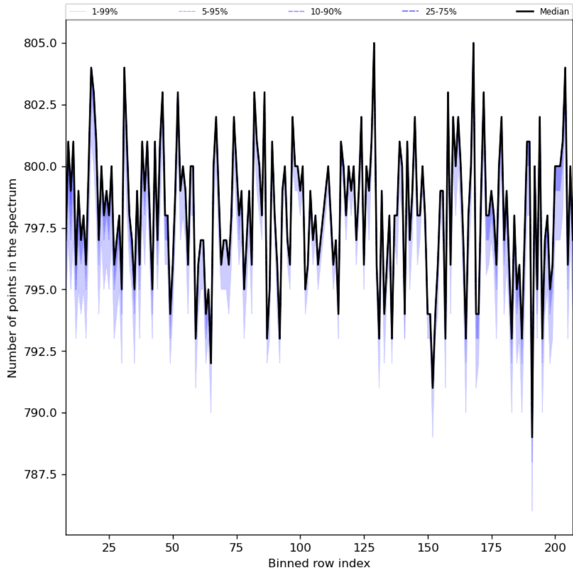
Figure 37: Along track statistics of “Number of points in the spectrum” for 2023-07-20 to 2023-07-22
