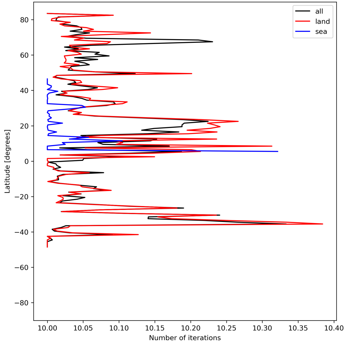
Figure 20: Zonal average of “Number of iterations” for 2023-07-20 to 2023-07-22.
