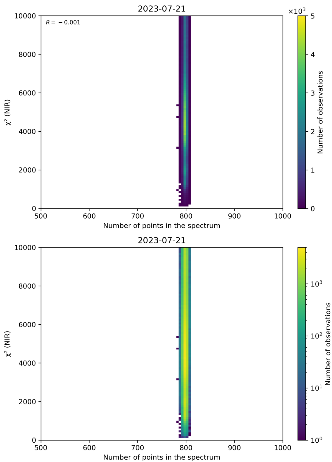
Figure 88: Scatter density plot of “Number of points in the spectrum” against “ \chi^2 (NIR)” for 2023-07-20 to 2023-07-22.
