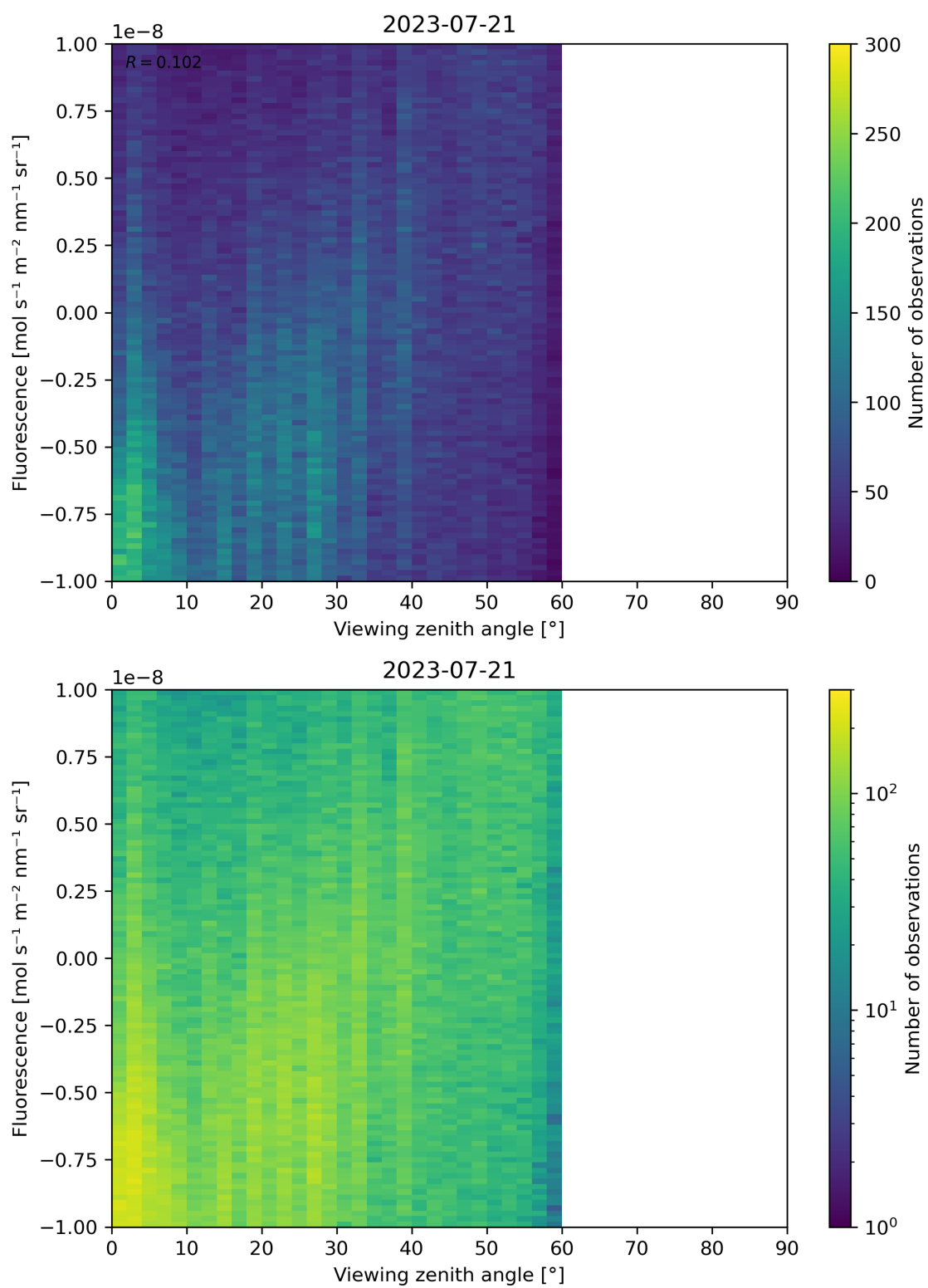
Figure 108: Scatter density plot of “Viewing zenith angle” against “Fluorescence” for 2023-07-20 to 2023-07-22.
