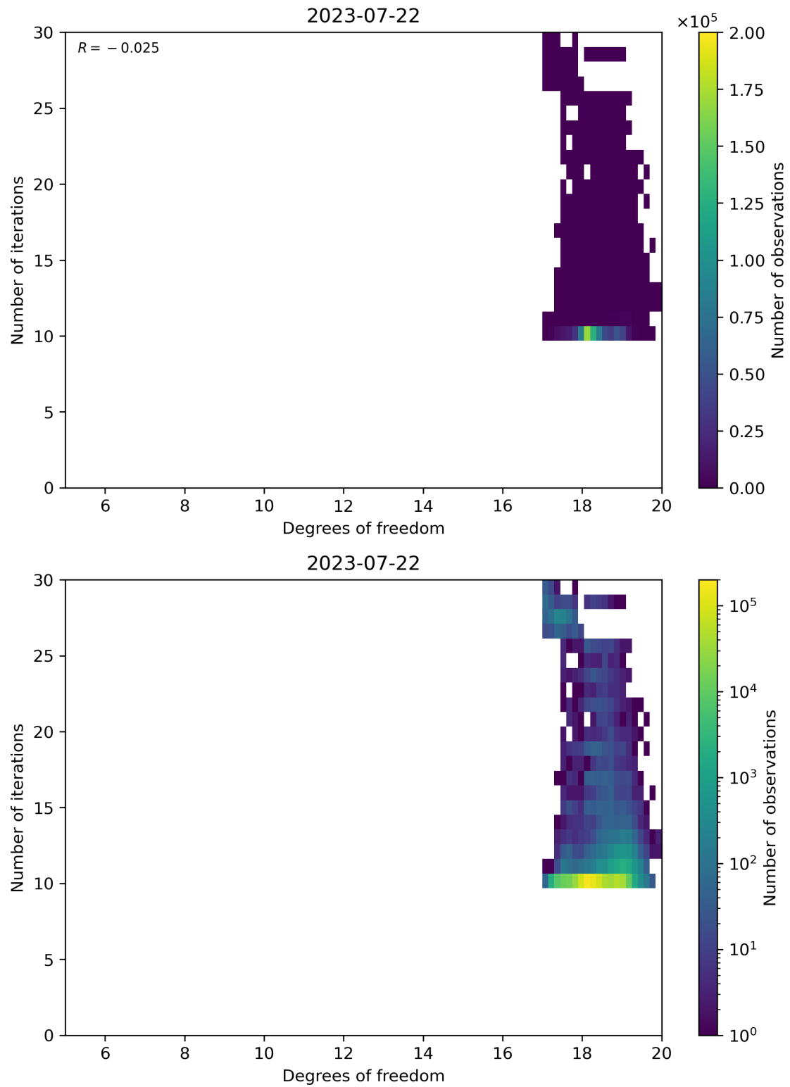
Figure 52: Scatter density plot of “Degrees of freedom” against “Number of iterations” for 2023-07-21 to 2023-07-23.
