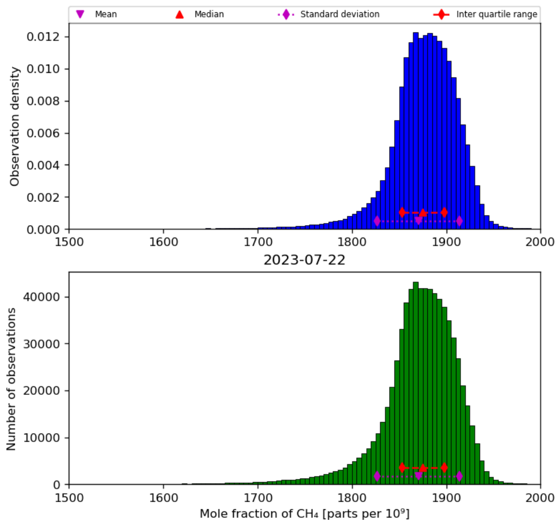
Figure 23: Histogram of “Mole fraction of CH 4 ” for 2023-07-21 to 2023-07-23
