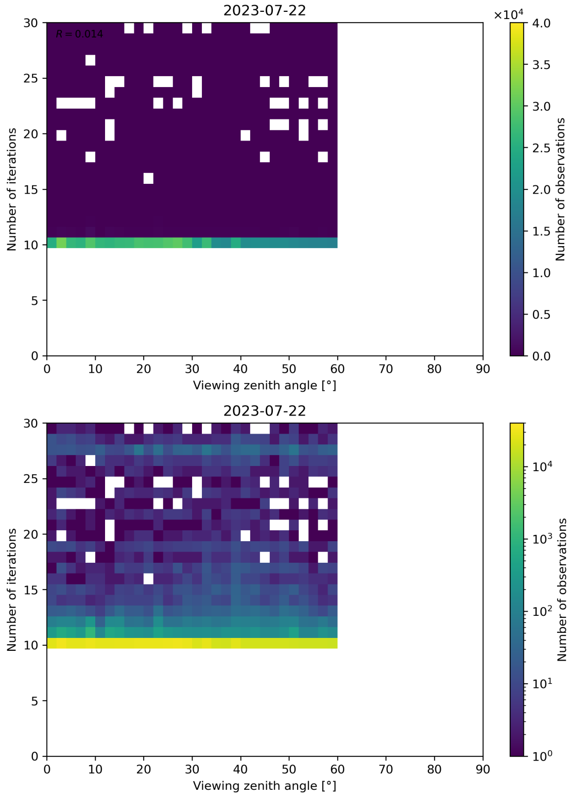
Figure 113: Scatter density plot of “Viewing zenith angle” against “Number of iterations” for 2023-07-21 to 2023-07-23.
