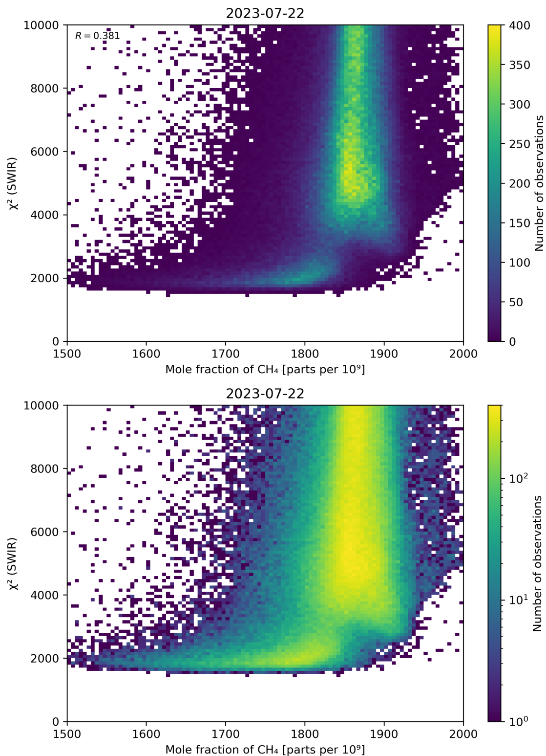
Figure 71: Scatter density plot of “Mole fraction of CH 4 ” against “ \chi^2 (SWIR)” for 2023-07-21 to 2023-07-23.
