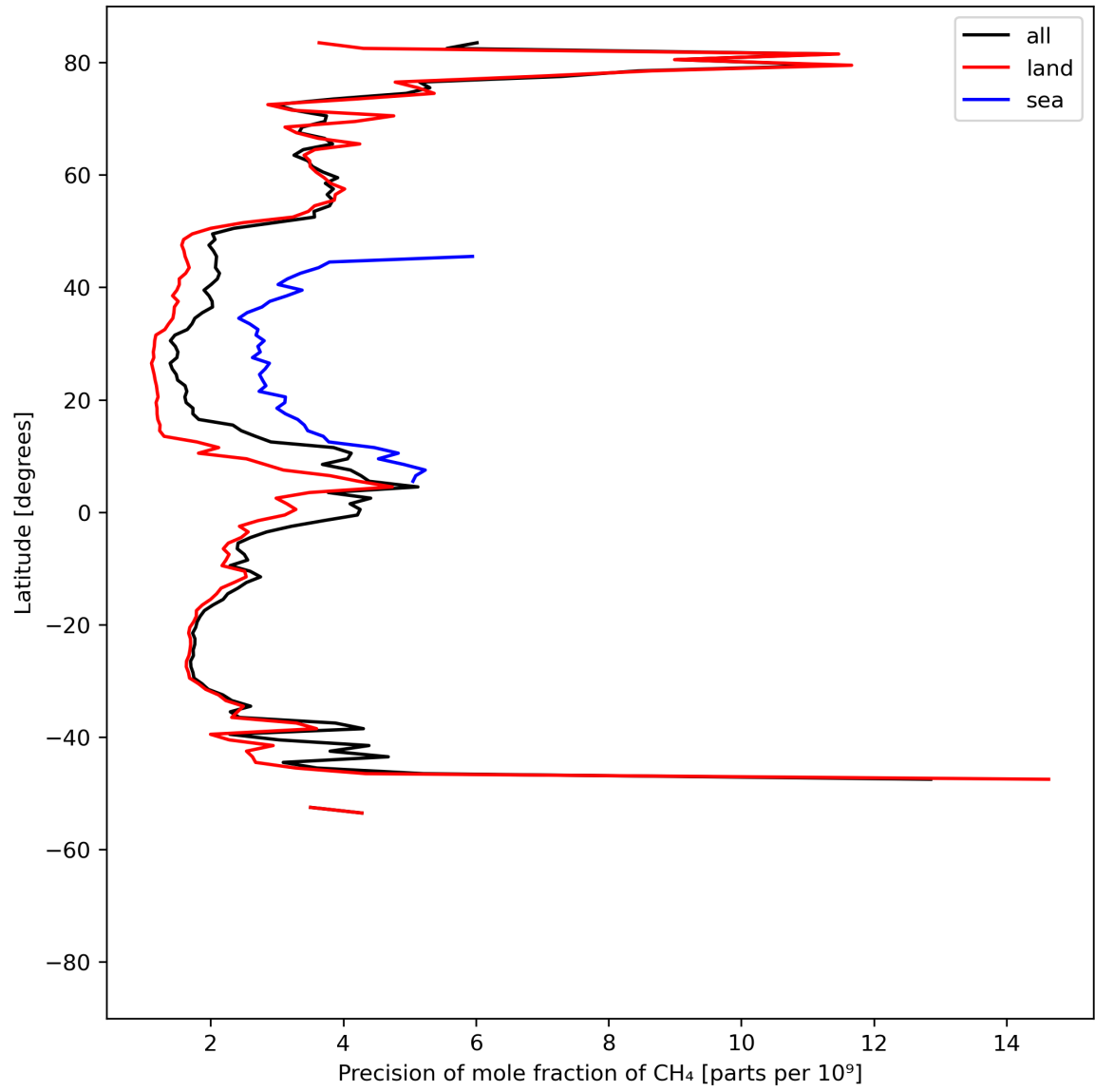
Figure 13: Zonal average of “Precision of mole fraction of CH 4 ” for 2023-07-21 to 2023-07-23.
