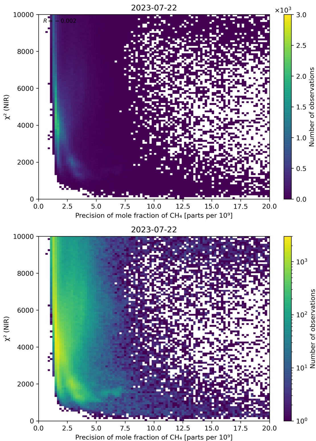
Figure 78: Scatter density plot of “Precision of mole fraction of CH 4 ” against “ \chi^2 (NIR)” for 2023-07-21 to 2023-07-23.
