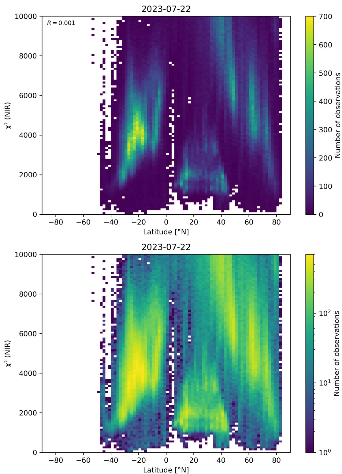
Figure 53: Scatter density plot of “Latitude” against “ \chi^2 (NIR)” for 2023-07-21 to 2023-07-23.
