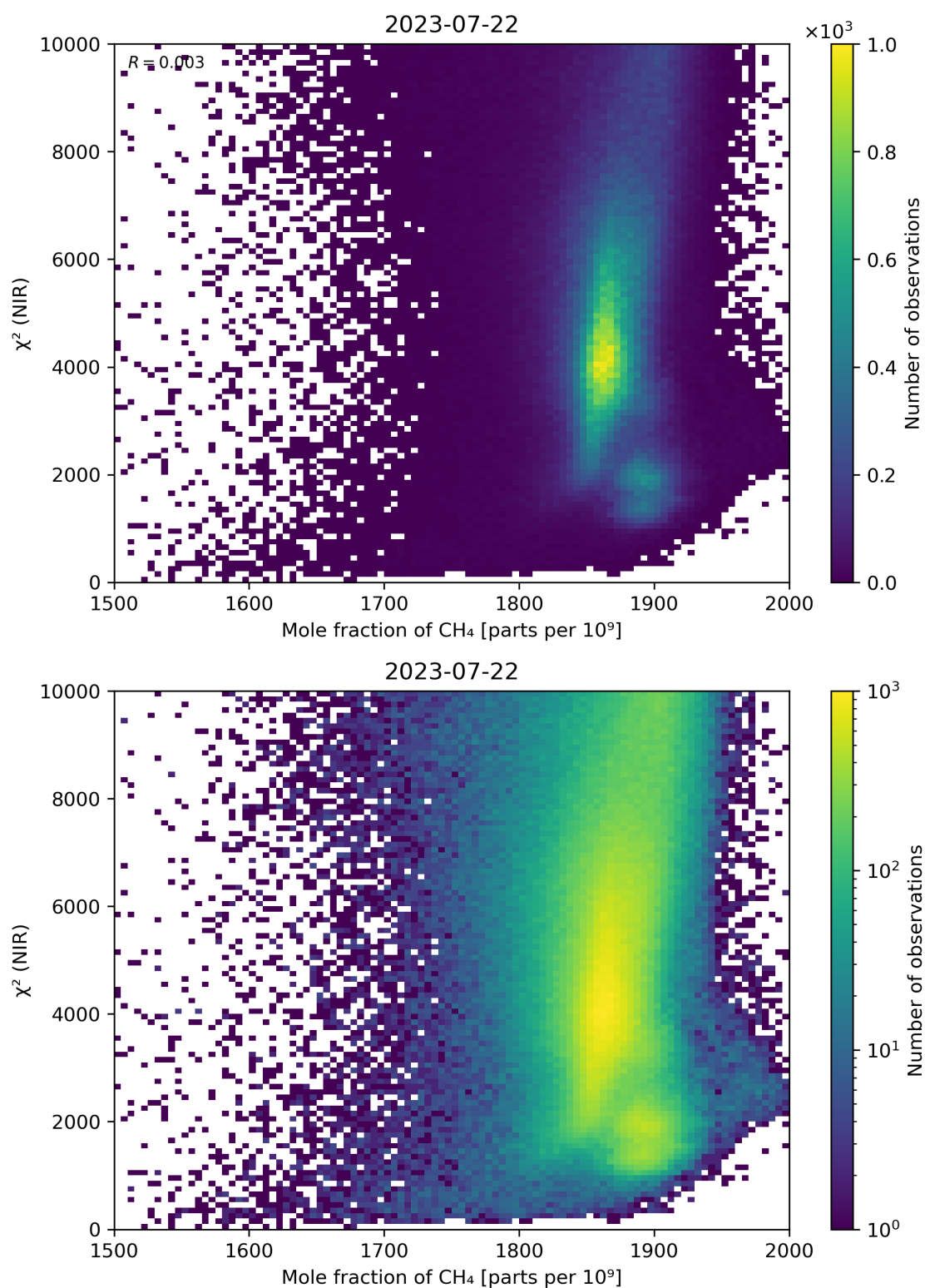
Figure 70: Scatter density plot of “Mole fraction of CH 4 ” against “ \chi^2 (NIR)” for 2023-07-21 to 2023-07-23.
