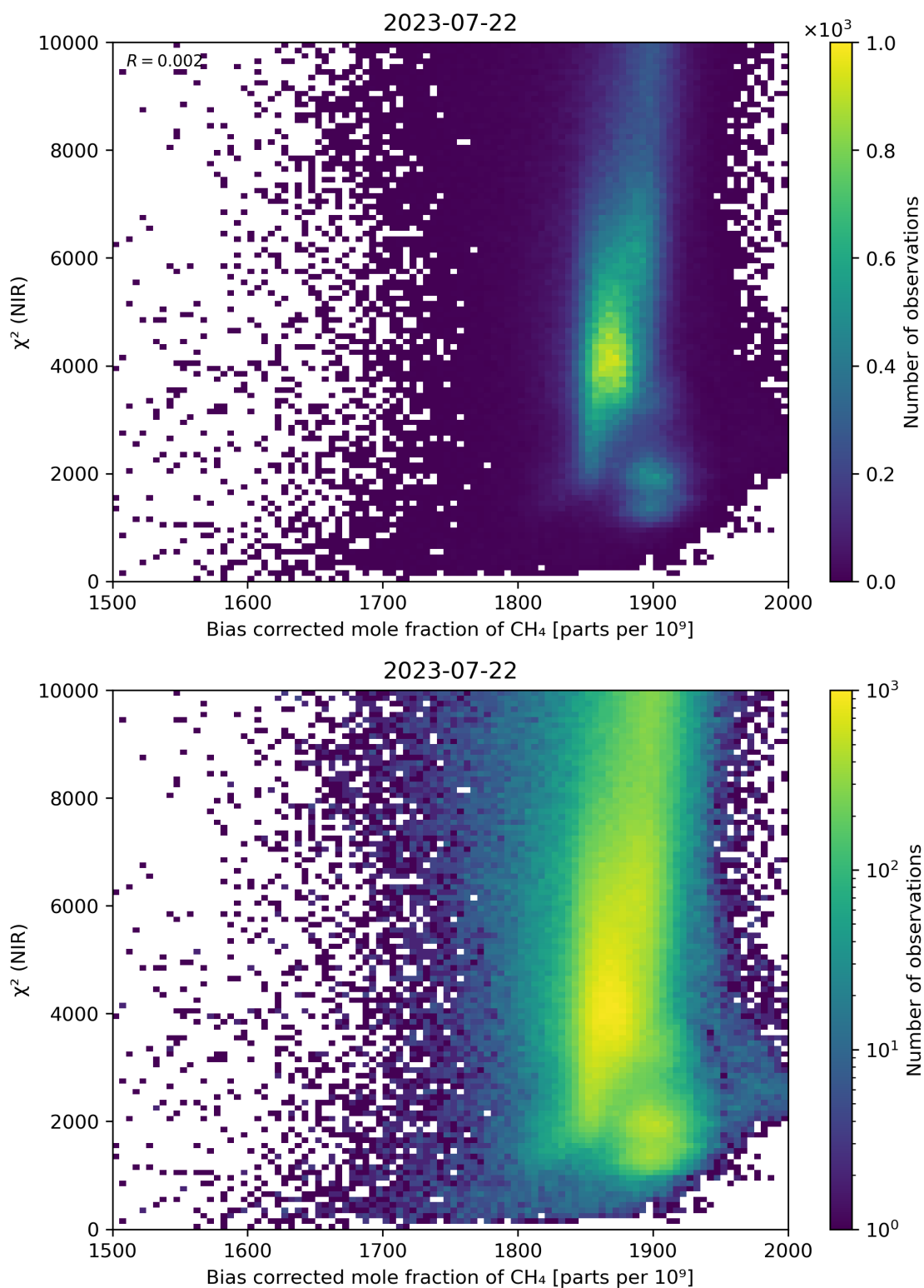
Figure 63: Scatter density plot of “Bias corrected mole fraction of \text{CH}_4 ” against “ \chi^2 (NIR)” for 2023-07-21 to 2023-07-23.
