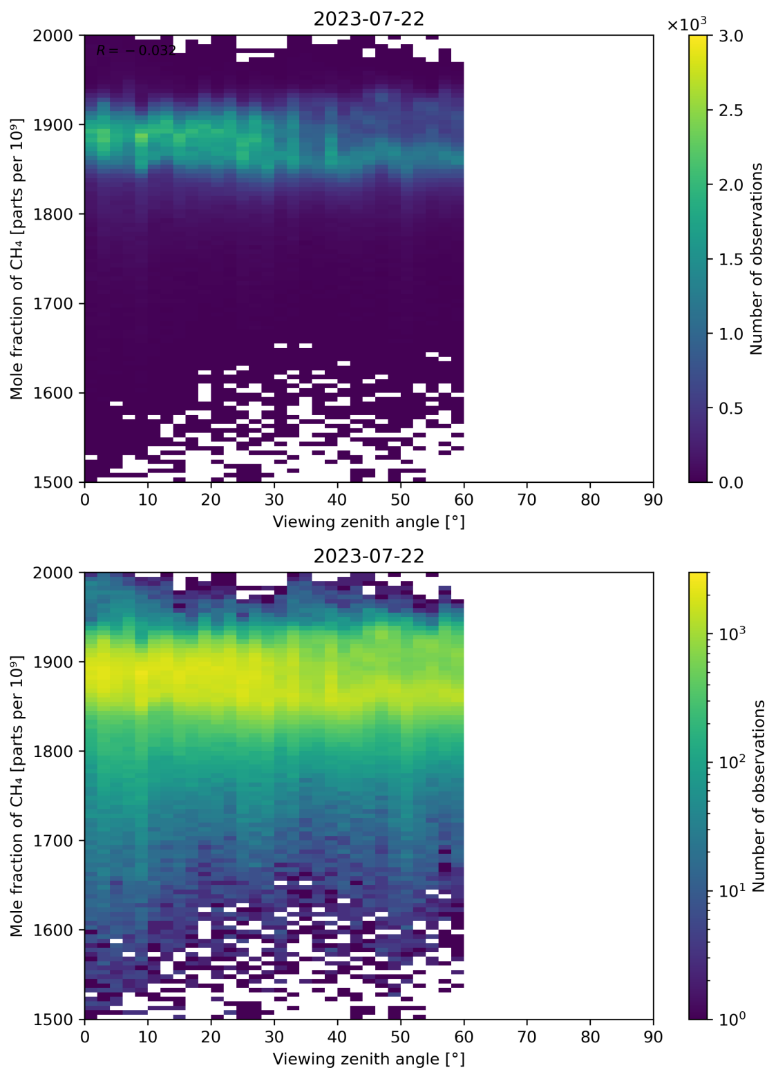
Figure 110: Scatter density plot of “Viewing zenith angle” against “Mole fraction of CH 4 ” for 2023-07-21 to 2023-07-23.
