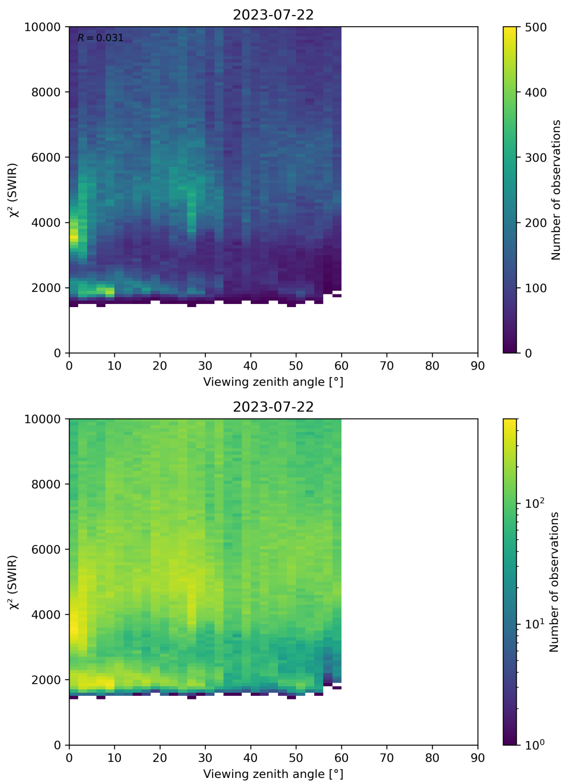
Figure 106: Scatter density plot of “Viewing zenith angle” against “ \chi^2 (SWIR)” for 2023-07-21 to 2023-07-23.
