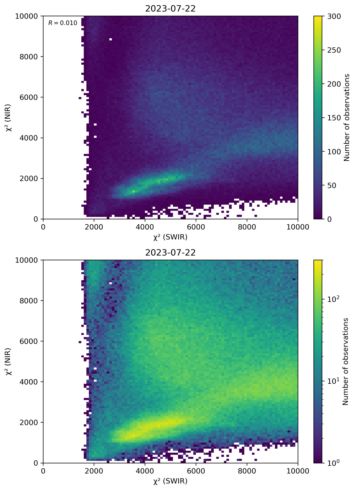
Figure 47: Scatter density plot of “ \chi^2 (SWIR)” against “ \chi^2 (NIR)” for 2023-07-21 to 2023-07-23.
