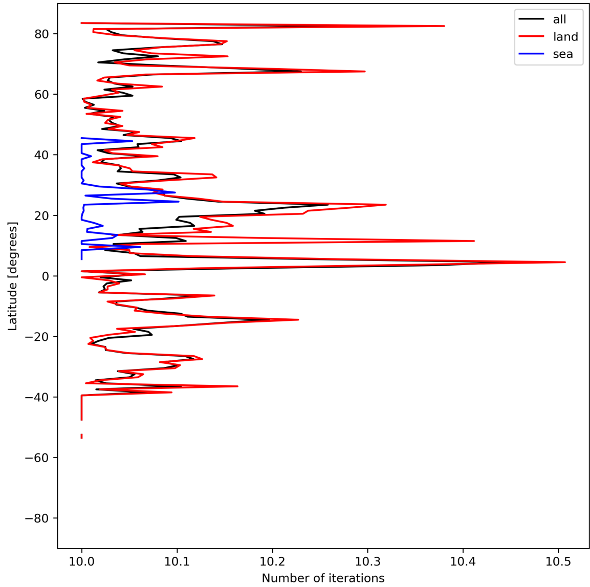
Figure 20: Zonal average of “Number of iterations” for 2023-07-21 to 2023-07-23.
