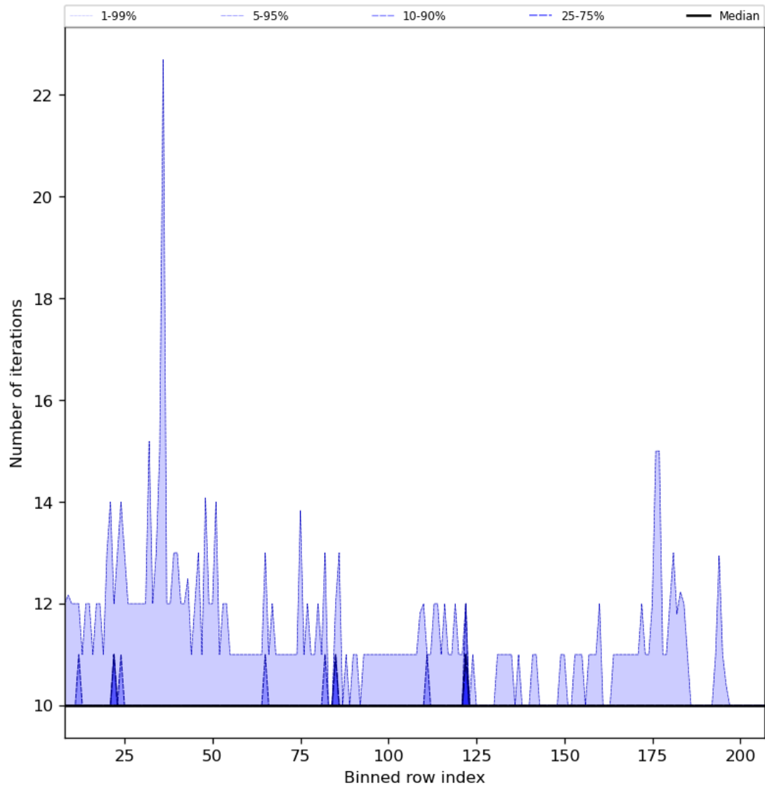
Figure 42: Along track statistics of “Number of iterations” for 2023-07-21 to 2023-07-23
