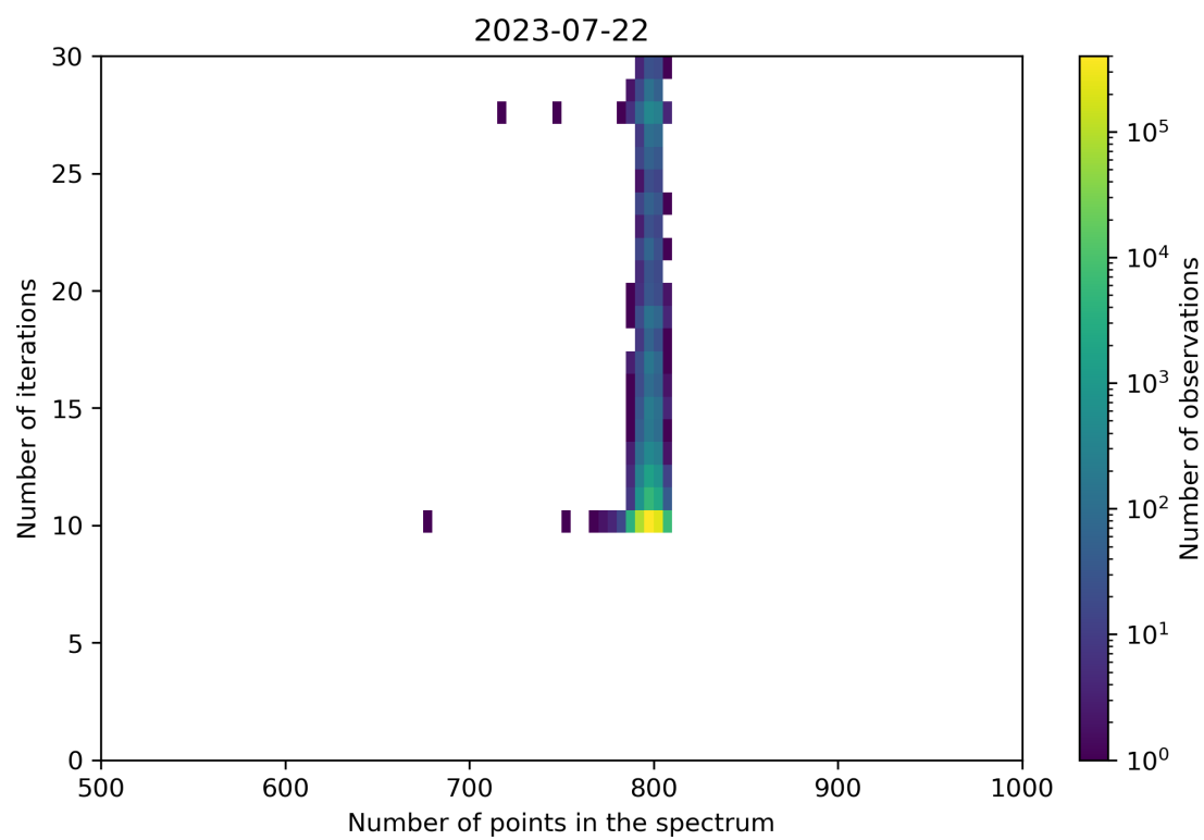
Figure 92: Scatter density plot of “Number of points in the spectrum” against “Number of iterations” for 2023-07-21 to 2023-07-23.
