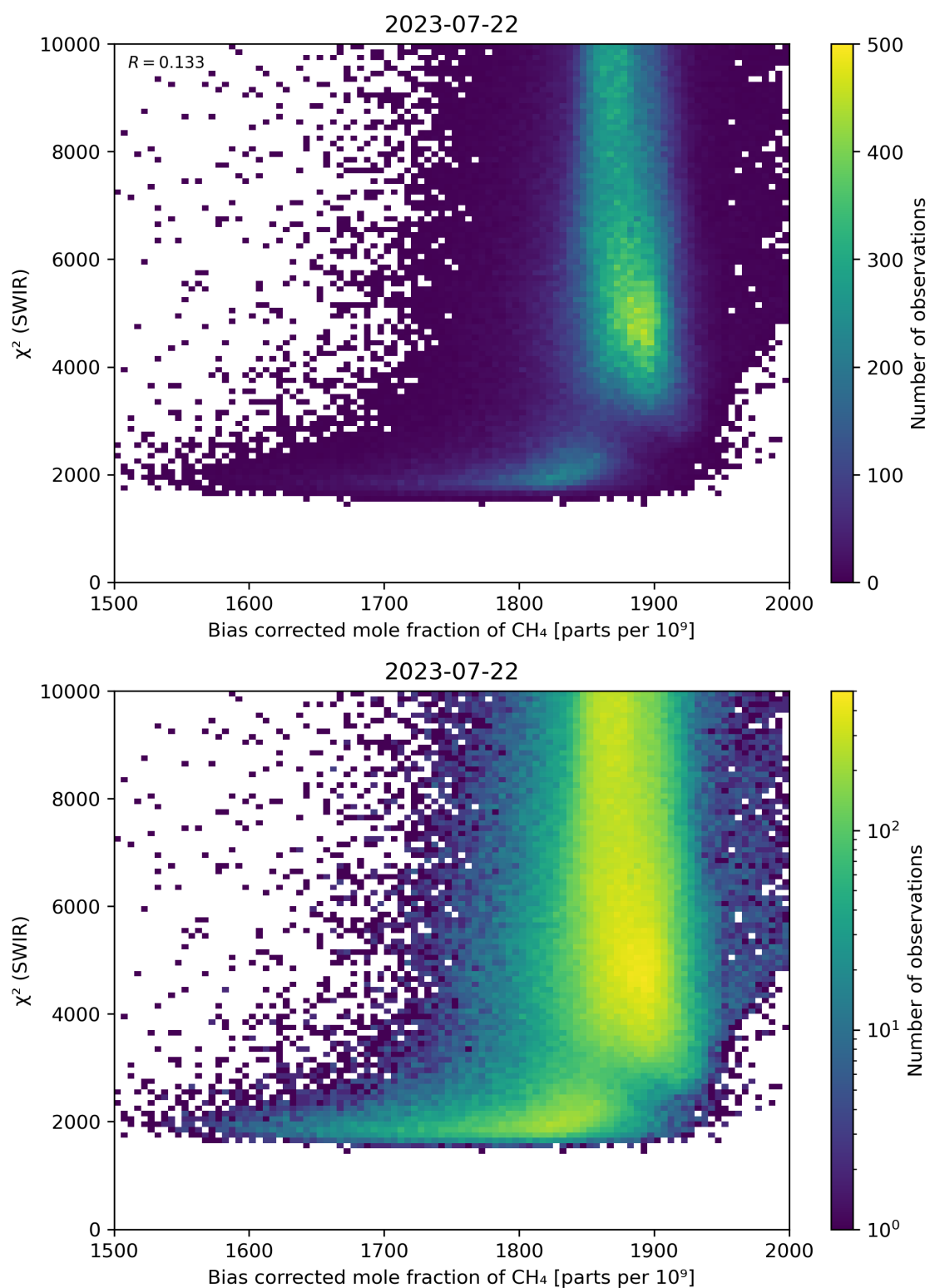
Figure 64: Scatter density plot of “Bias corrected mole fraction of CH 4 ” against “ \chi^2 (SWIR)” for 2023-07-21 to 2023-07-23.
