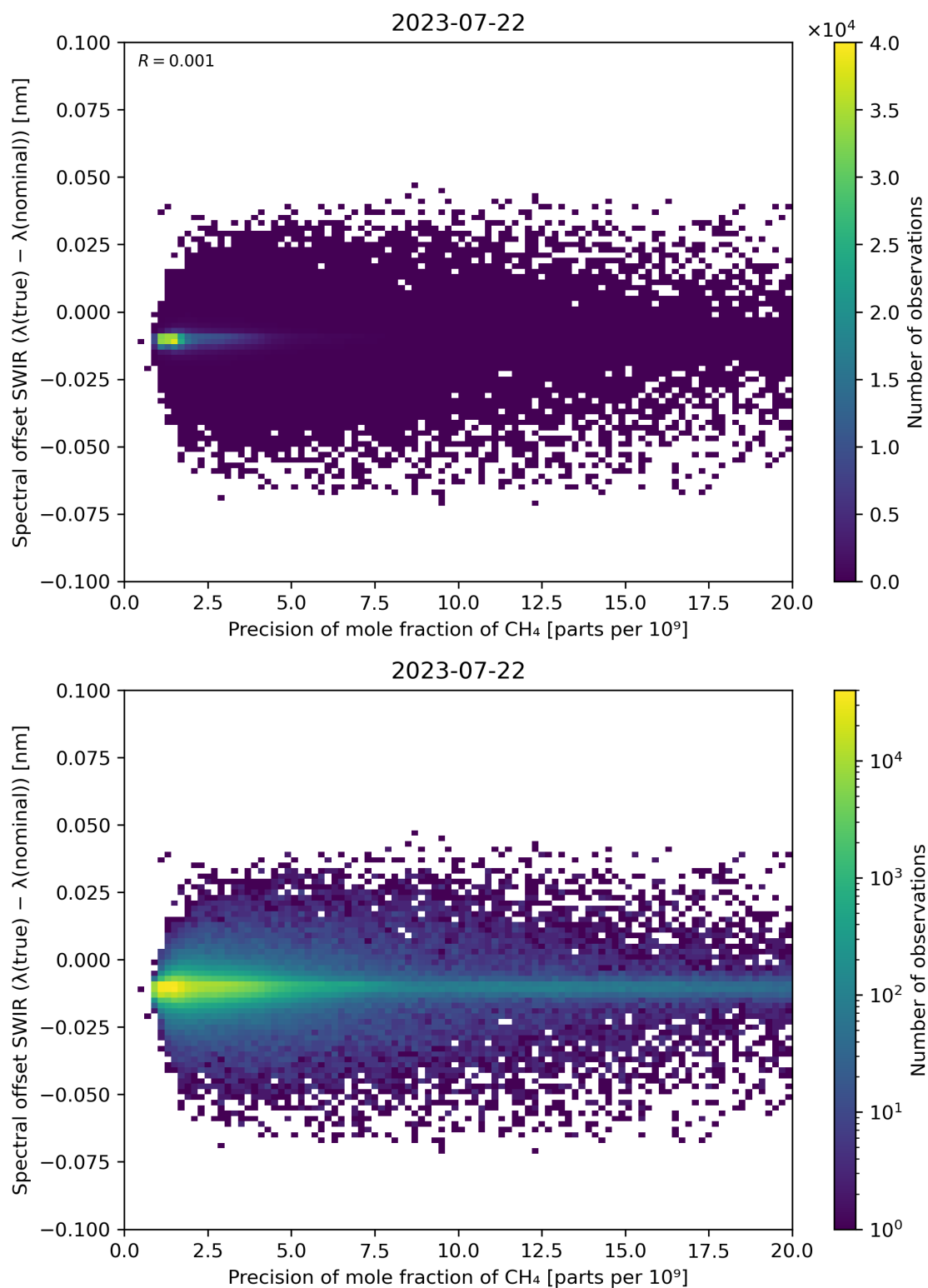
Figure 85: Scatter density plot of “Precision of mole fraction of CH 4 ” against “Spectral offset SWIR ( \lambda(\text{true}) - \lambda(\text{nominal}) )” for 2023-07-21 to 2023-07-23.
