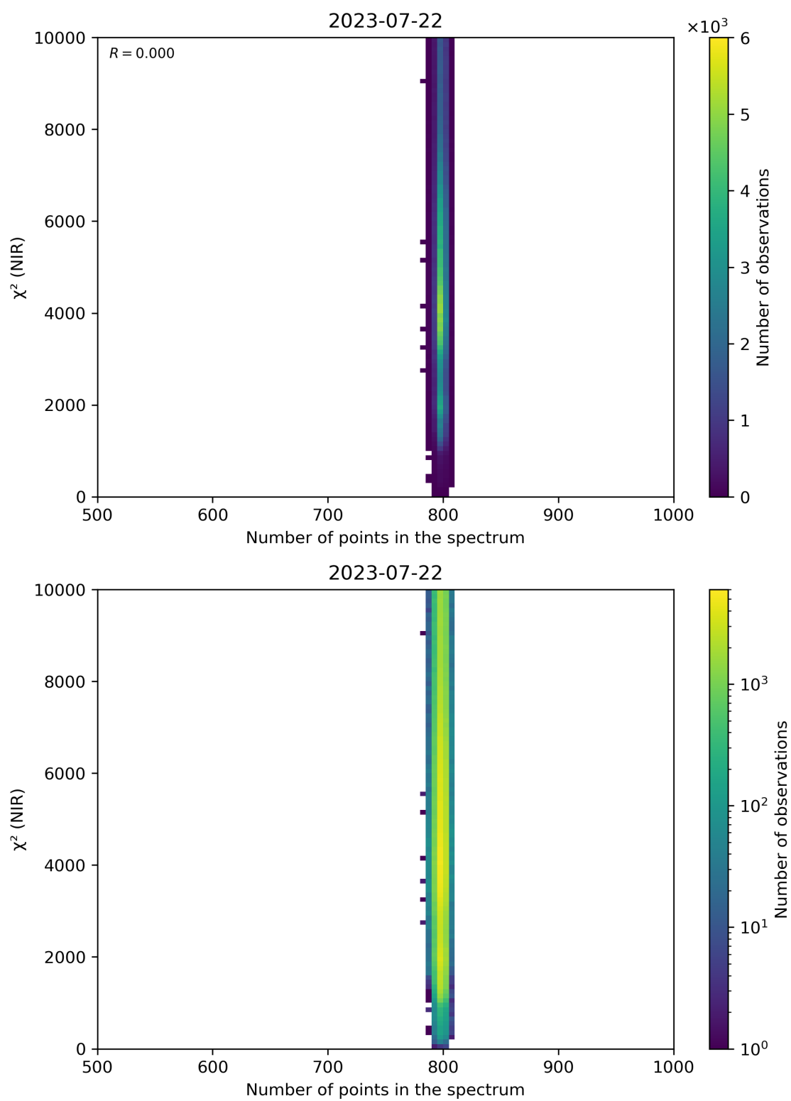
Figure 88: Scatter density plot of “Number of points in the spectrum” against “ \chi^2 (NIR)” for 2023-07-21 to 2023-07-23.
