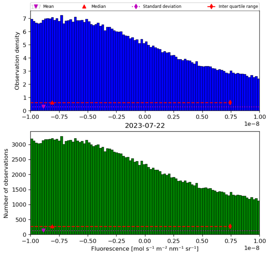
Figure 32: Histogram of “Fluorescence” for 2023-07-21 to 2023-07-23
