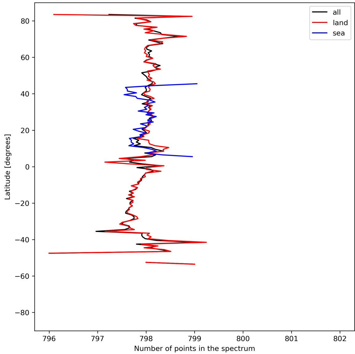
Figure 15: Zonal average of “Number of points in the spectrum” for 2023-07-21 to 2023-07-23.
