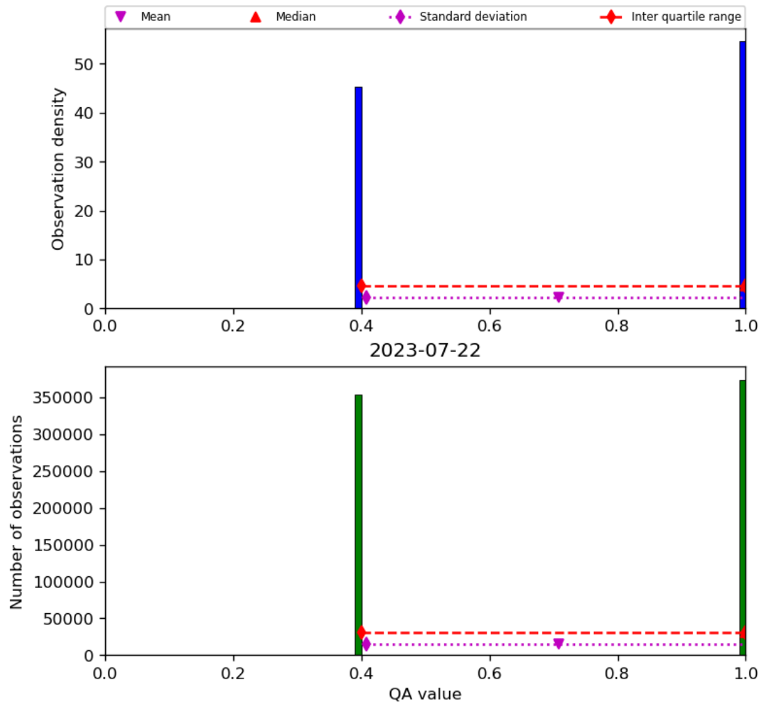
Figure 22: Histogram of “QA value” for 2023-07-21 to 2023-07-23
