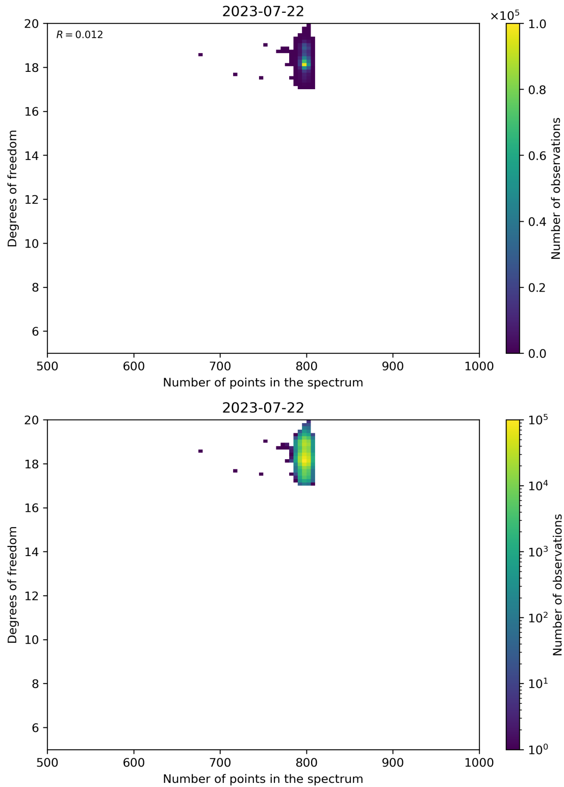
Figure 90: Scatter density plot of “Number of points in the spectrum” against “Degrees of freedom” for 2023-07-21 to 2023-07-23.
