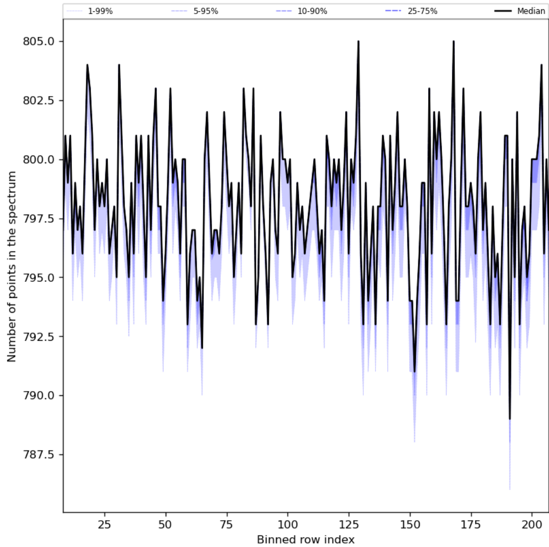
Figure 37: Along track statistics of “Number of points in the spectrum” for 2023-07-21 to 2023-07-23
