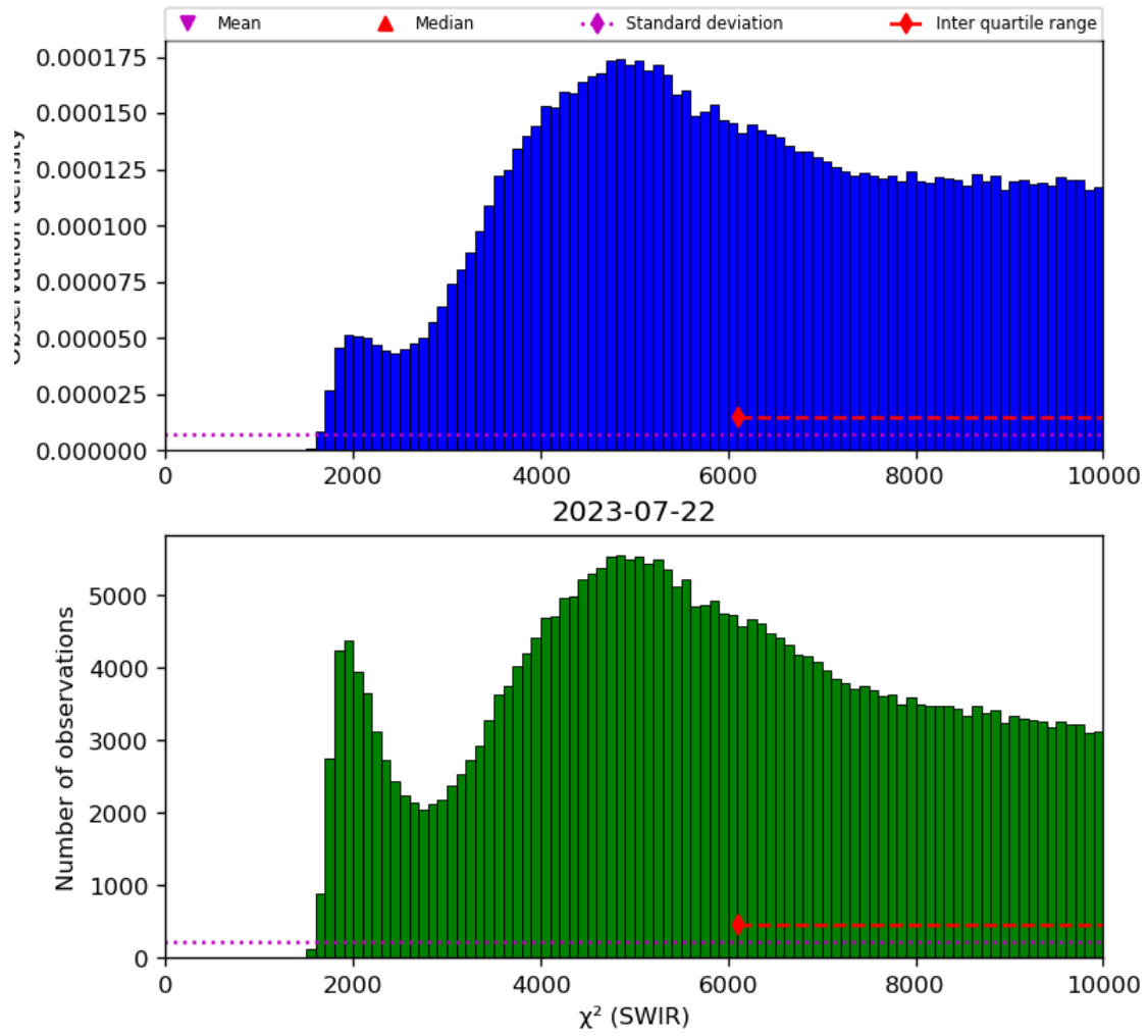
Figure 28: Histogram of “ \chi^2 (SWIR)” for 2023-07-21 to 2023-07-23
