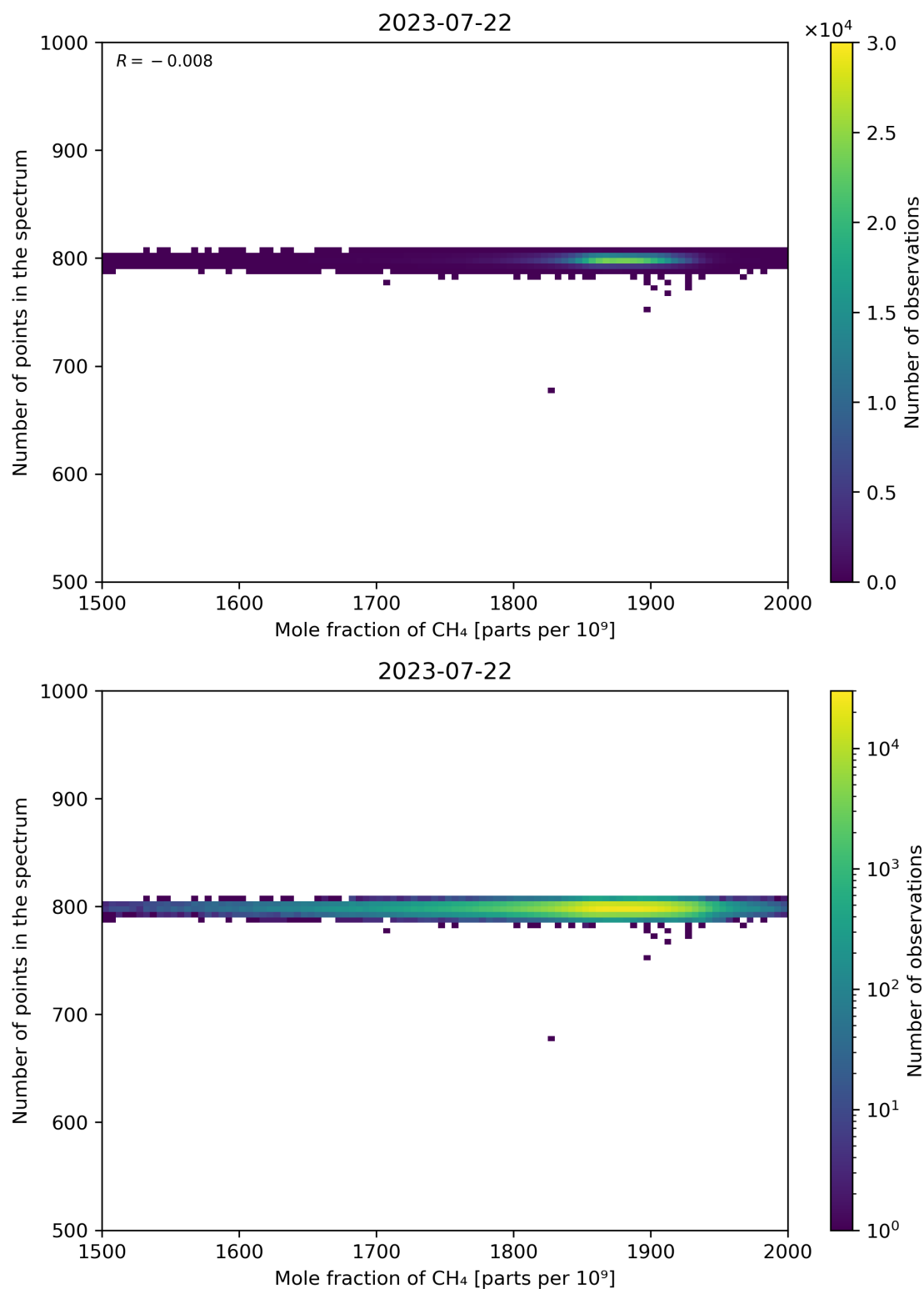
Figure 77: Scatter density plot of “Mole fraction of CH 4 ” against “Number of points in the spectrum” for 2023-07-21 to 2023-07-23.
