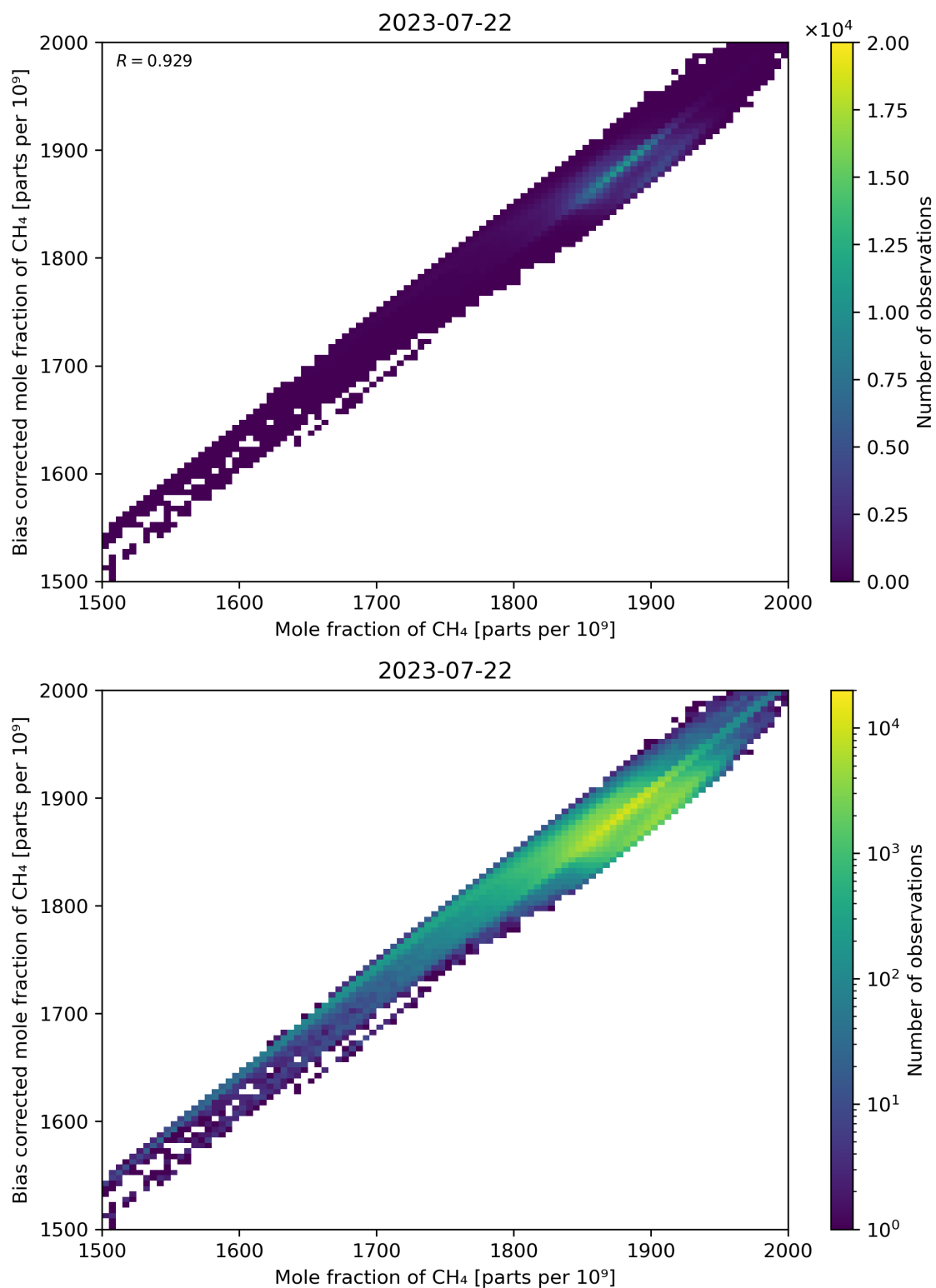
Figure 74: Scatter density plot of “Mole fraction of CH 4 ” against “Bias corrected mole fraction of CH 4 ” for 2023-07-21 to 2023-07-23.
