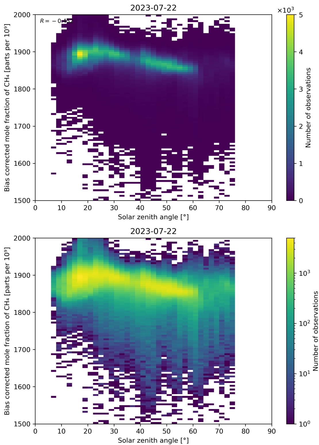
Figure 100: Scatter density plot of “Solar zenith angle” against “Bias corrected mole fraction of \text{CH}_4 ” for 2023-07-21 to 2023-07-23.
