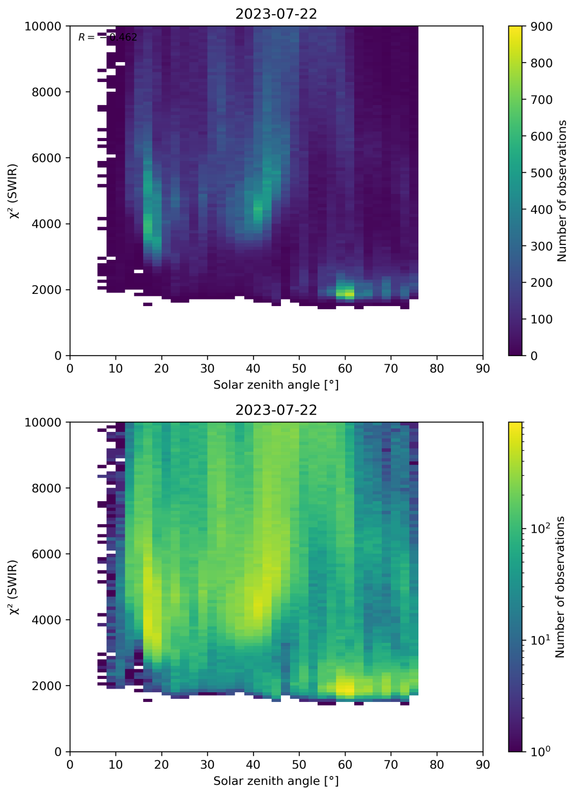
Figure 95: Scatter density plot of “Solar zenith angle” against “ \chi^2 (SWIR)” for 2023-07-21 to 2023-07-23.
