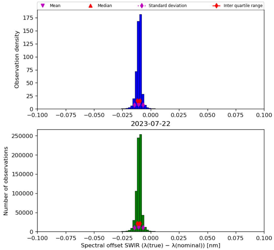
Figure 27: Histogram of “Spectral offset SWIR ( \lambda(\text{true}) - \lambda(\text{nominal}) )” for 2023-07-21 to 2023-07-23
