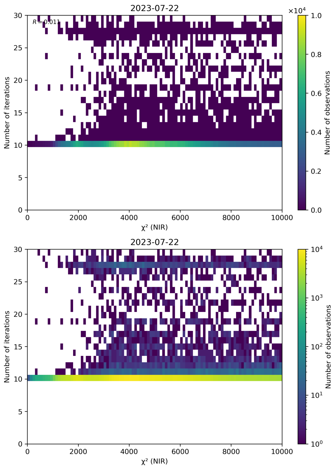
Figure 46: Scatter density plot of “ \chi^2 (NIR)” against “Number of iterations” for 2023-07-21 to 2023-07-23.
