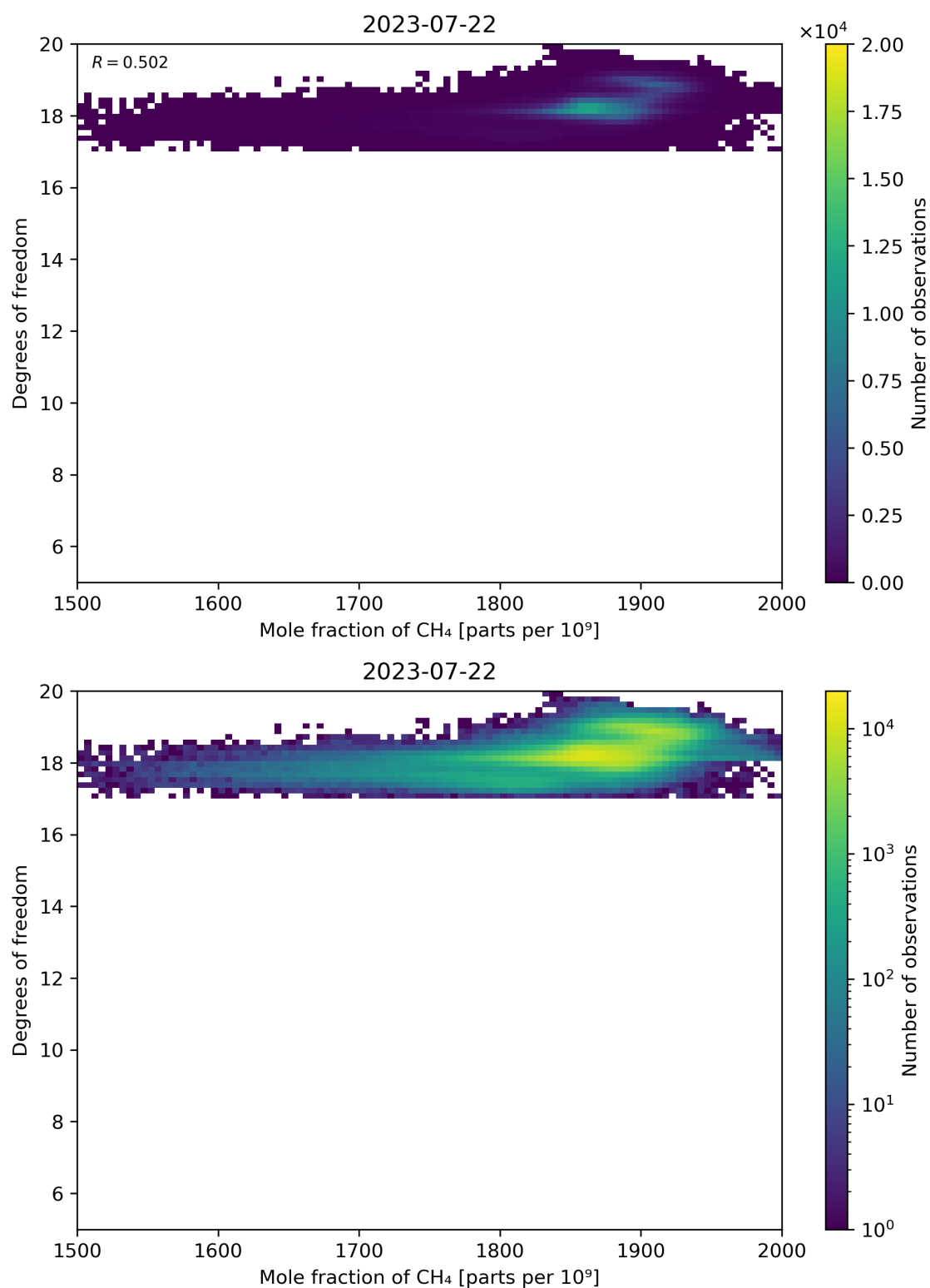
Figure 72: Scatter density plot of “Mole fraction of CH 4 ” against “Degrees of freedom” for 2023-07-21 to 2023-07-23.
