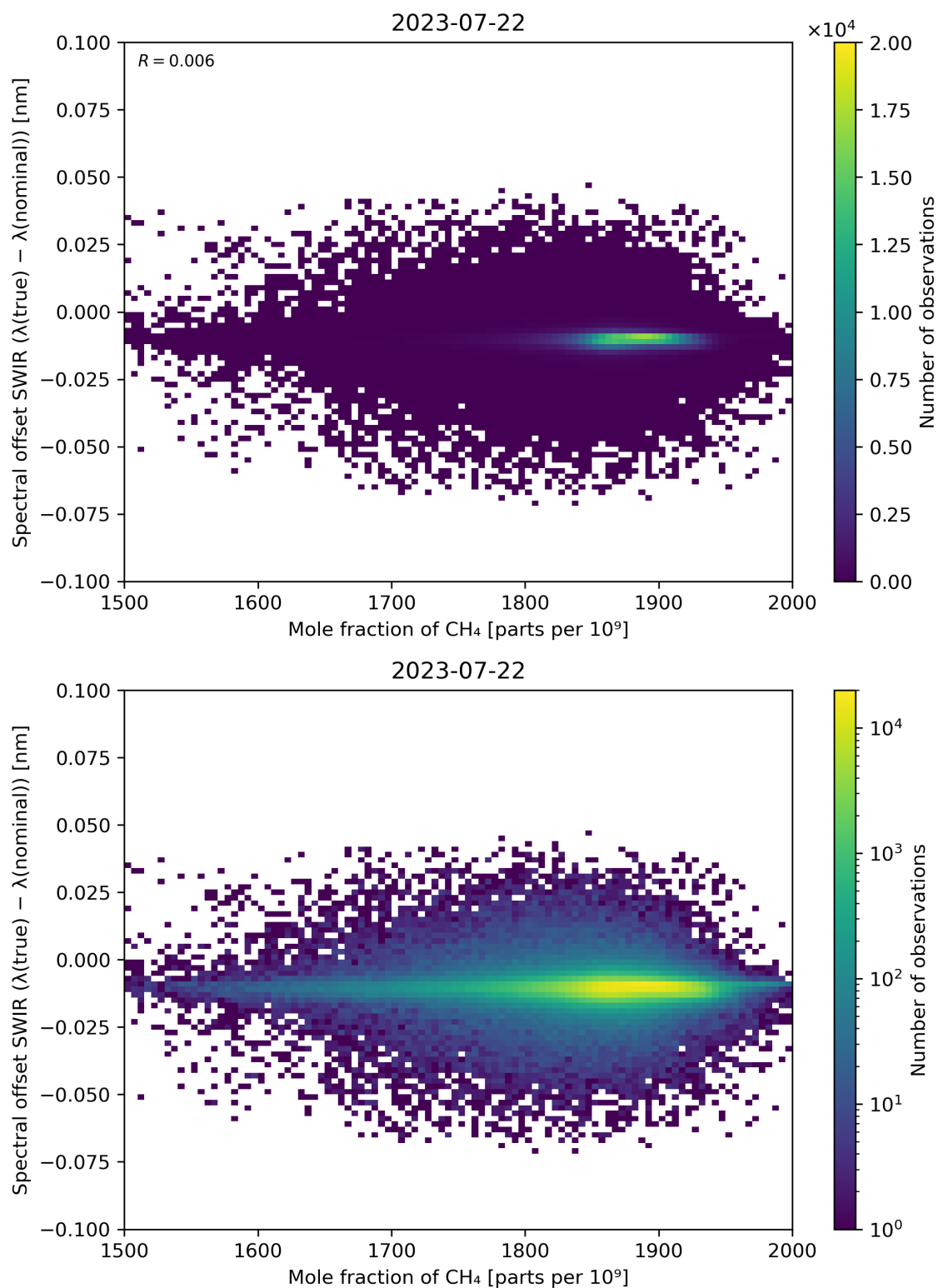
Figure 86: Scatter density plot of “Mole fraction of CH 4 ” against “Spectral offset SWIR ( \lambda(\text{true}) - \lambda(\text{nominal}) )” for 2023-07-21 to 2023-07-23.
