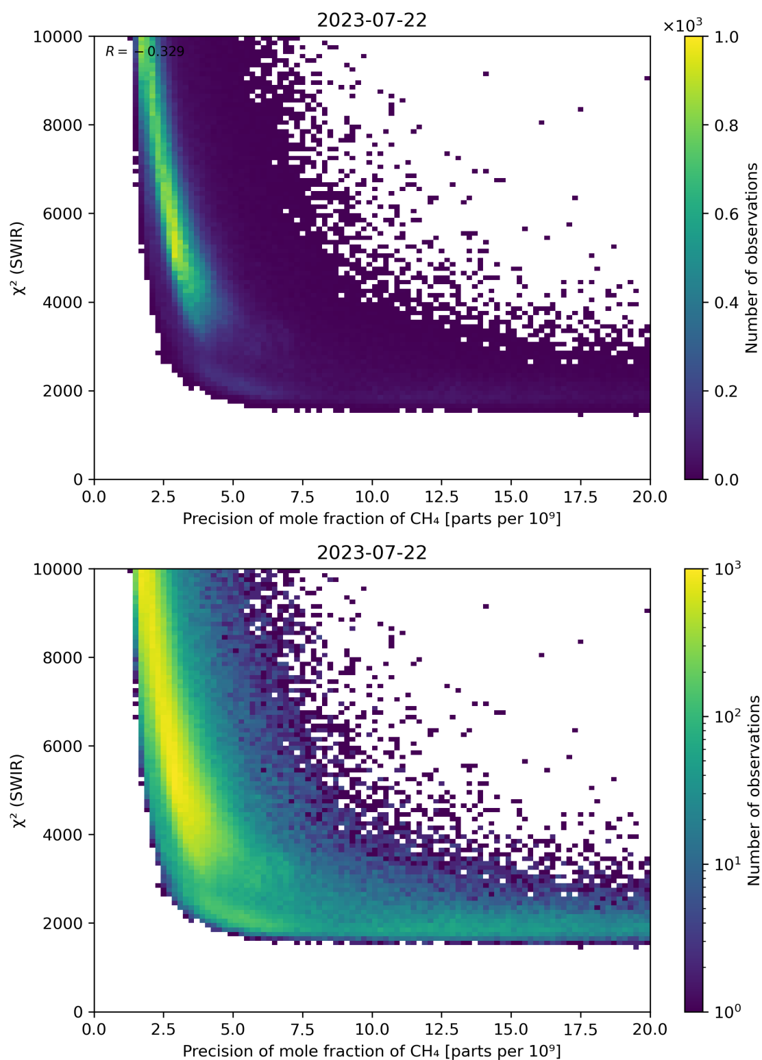
Figure 79: Scatter density plot of “Precision of mole fraction of \text{CH}_4 ” against “ \chi^2 (SWIR)” for 2023-07-21 to 2023-07-23.
