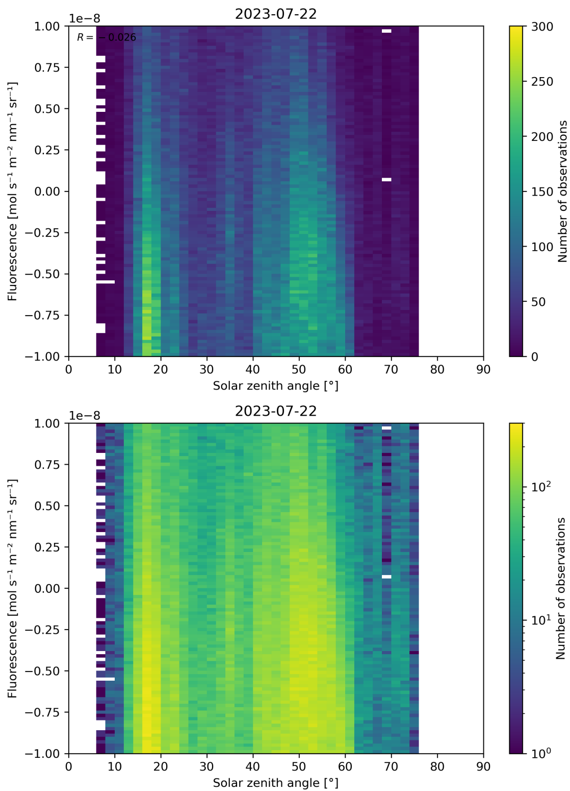
Figure 97: Scatter density plot of “Solar zenith angle” against “Fluorescence” for 2023-07-21 to 2023-07-23.
