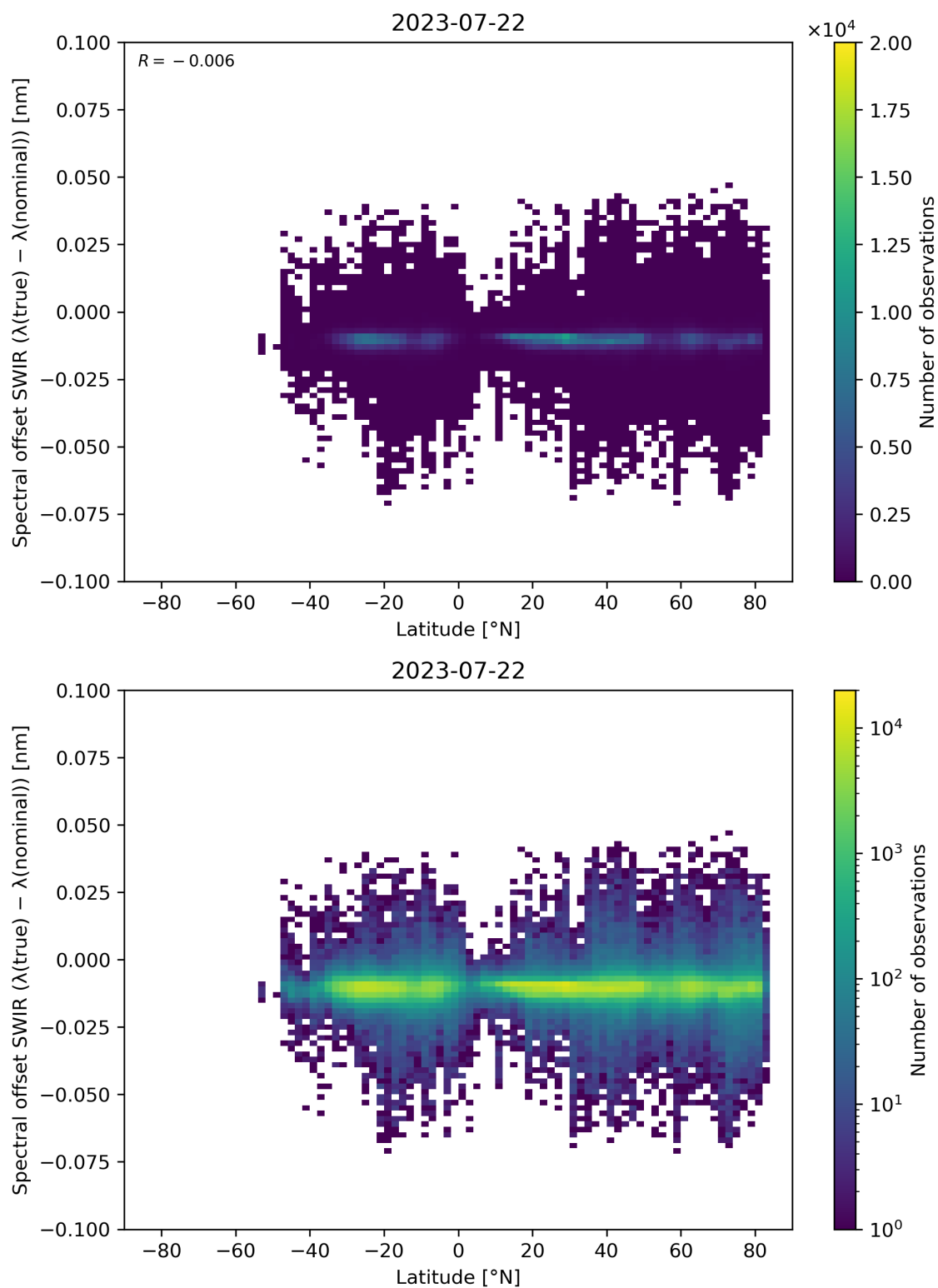
Figure 62: Scatter density plot of “Latitude” against “Spectral offset SWIR ( \lambda(\text{true}) - \lambda(\text{nominal}) )” for 2023-07-21 to 2023-07-23.
