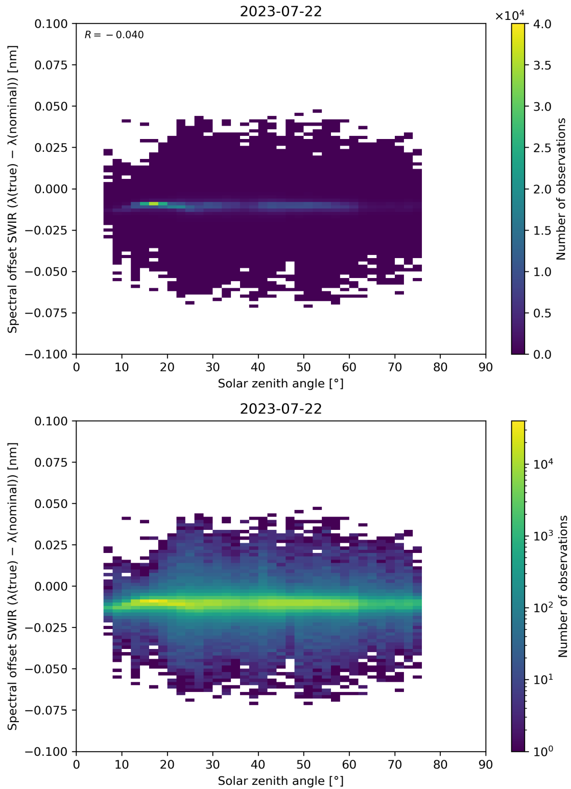
Figure 104: Scatter density plot of “Solar zenith angle” against “Spectral offset SWIR ( \lambda(\text{true}) - \lambda(\text{nominal}) )” for 2023-07-21 to 2023-07-23.
