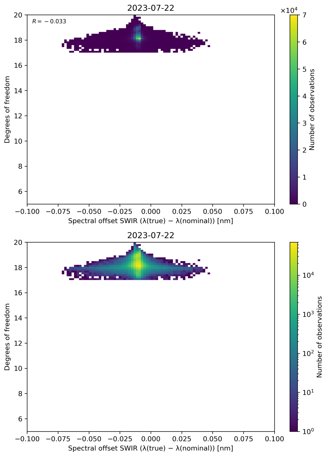
Figure 119: Scatter density plot of “Spectral offset SWIR ( \lambda(\text{true}) - \lambda(\text{nominal}) )” against “Degrees of freedom” for 2023-07-21 to 2023-07-23.
