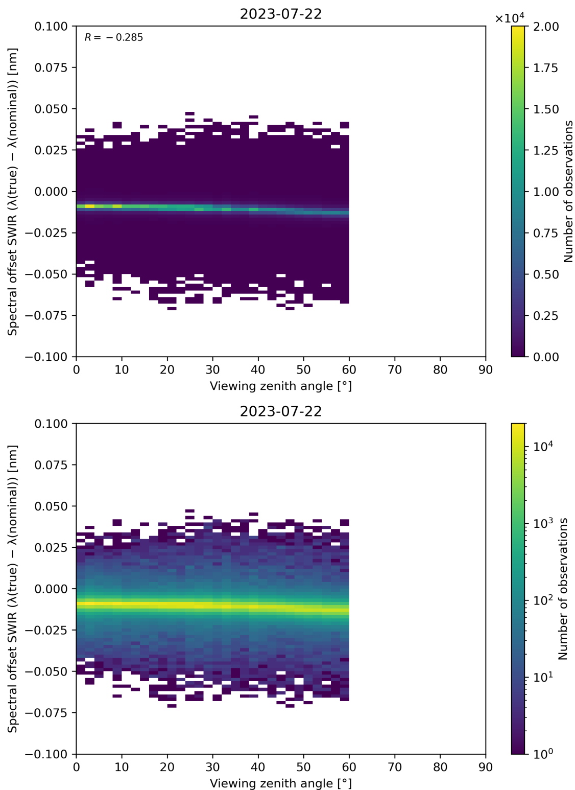
Figure 116: Scatter density plot of “Viewing zenith angle” against “Spectral offset SWIR ( \lambda(\text{true}) - \lambda(\text{nominal}) )” for 2023-07-21 to 2023-07-23.
