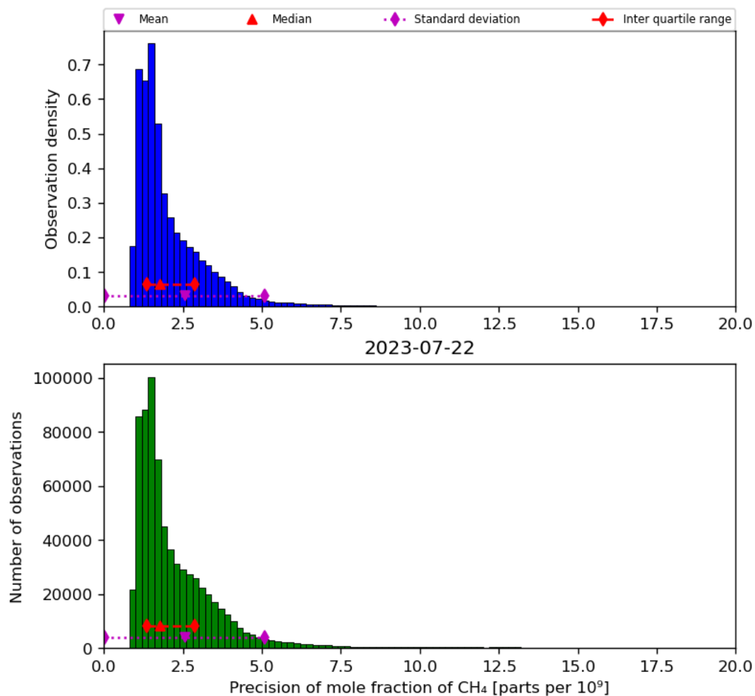
Figure 24: Histogram of “Precision of mole fraction of CH 4 ” for 2023-07-21 to 2023-07-23
