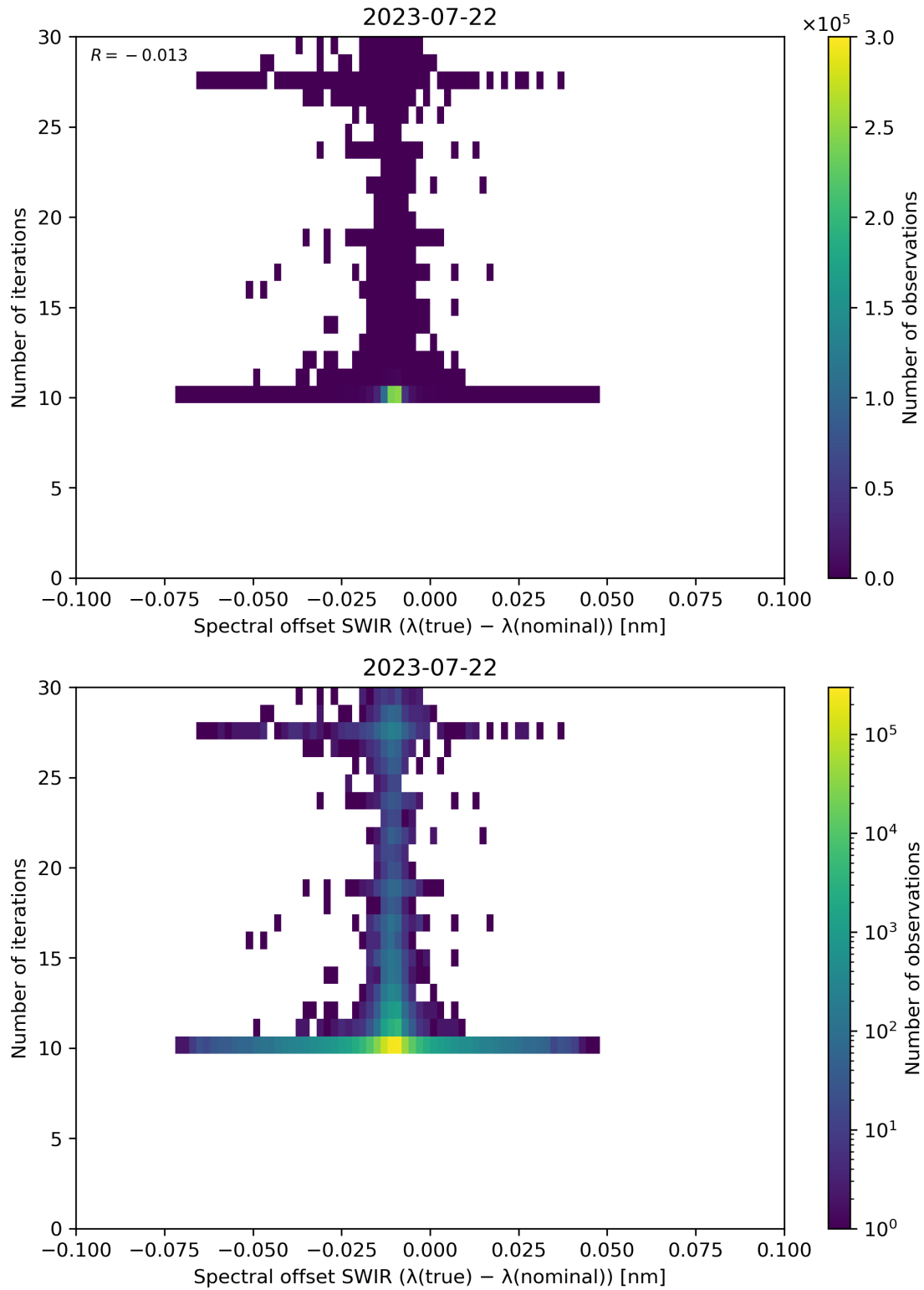
Figure 121: Scatter density plot of “Spectral offset SWIR ( \lambda(\text{true}) - \lambda(\text{nominal}) )” against “Number of iterations” for 2023-07-21 to 2023-07-23.
