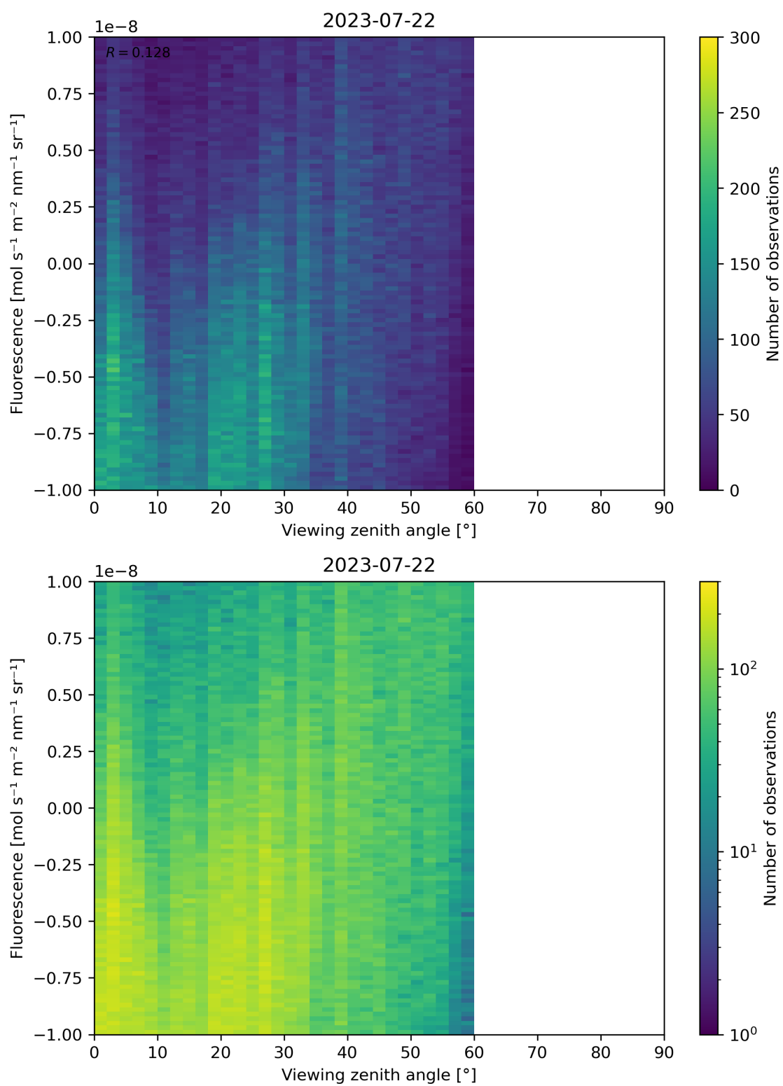
Figure 108: Scatter density plot of “Viewing zenith angle” against “Fluorescence” for 2023-07-21 to 2023-07-23.
