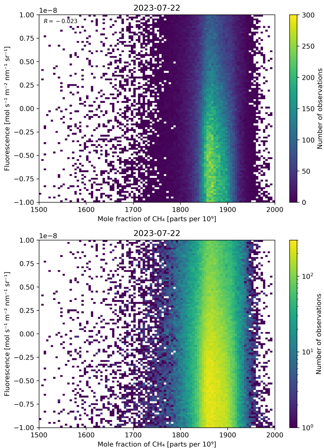
Figure 73: Scatter density plot of “Mole fraction of \text{CH}_4 ” against “Fluorescence” for 2023-07-21 to 2023-07-23.
