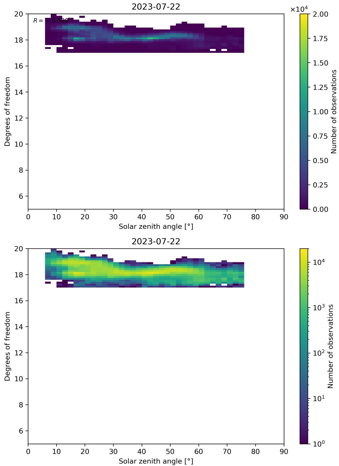
Figure 96: Scatter density plot of “Solar zenith angle” against “Degrees of freedom” for 2023-07-21 to 2023-07-23.
