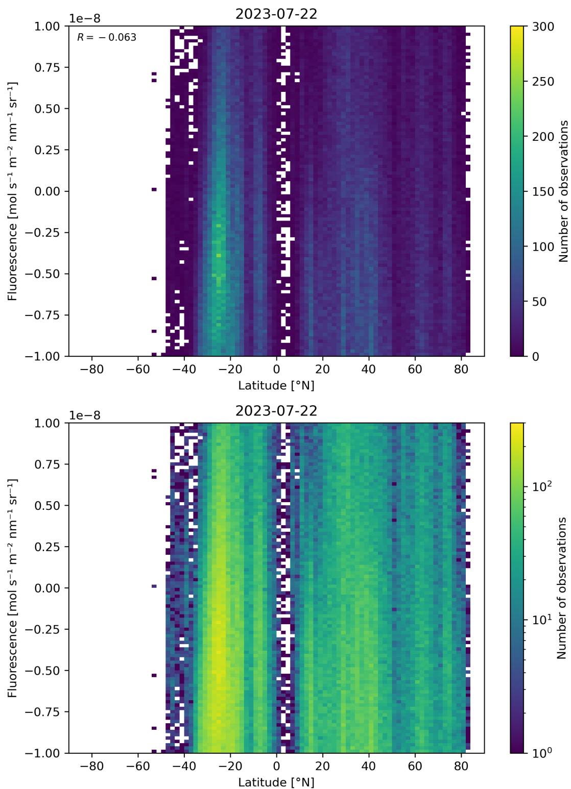
Figure 56: Scatter density plot of “Latitude” against “Fluorescence” for 2023-07-21 to 2023-07-23.
