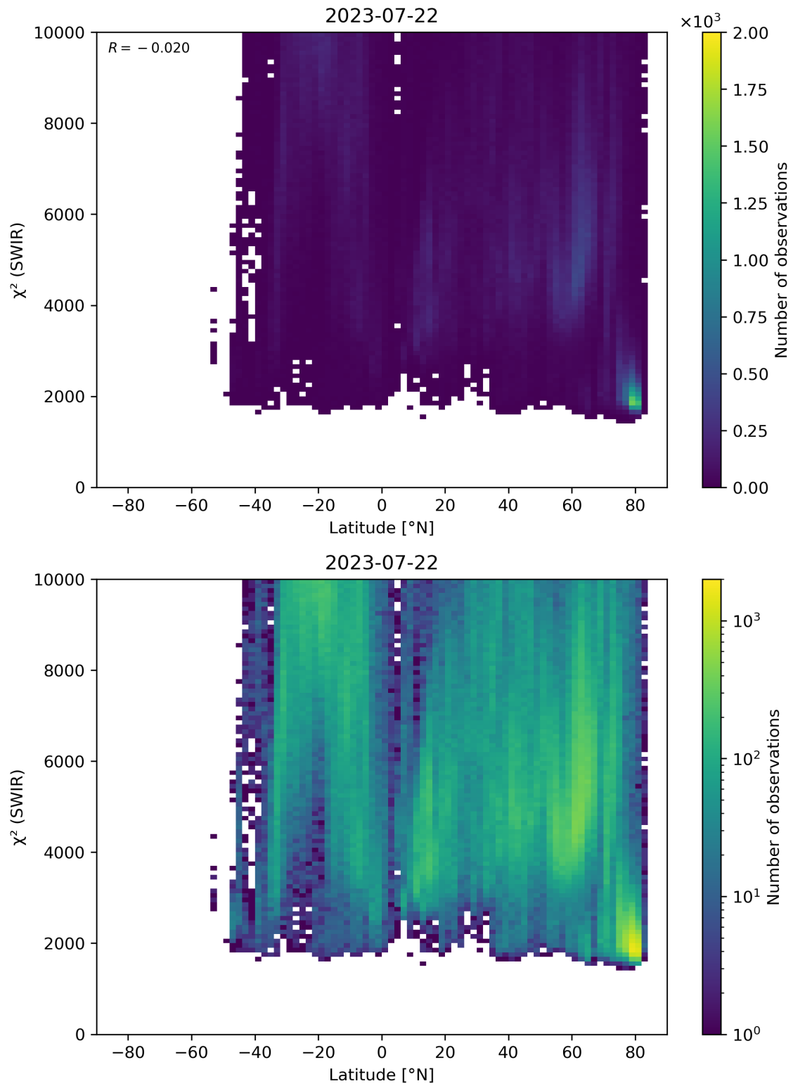
Figure 54: Scatter density plot of “Latitude” against “ \chi^2 (SWIR)” for 2023-07-21 to 2023-07-23.
