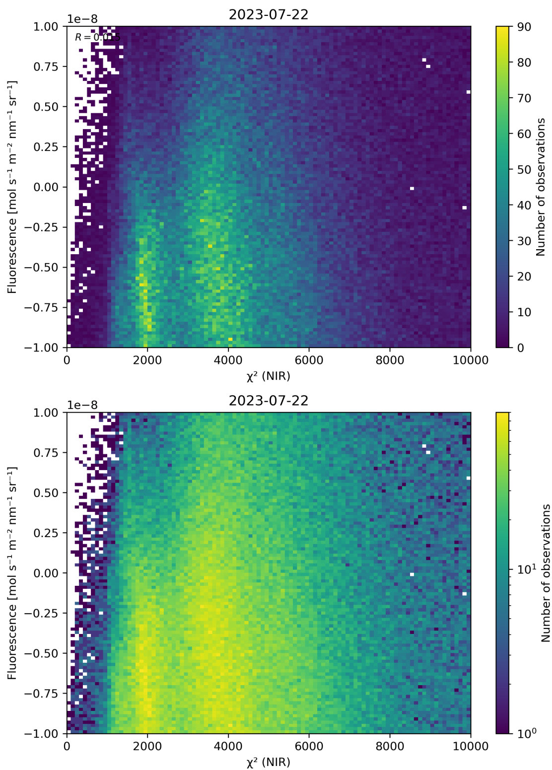
Figure 45: Scatter density plot of “ \chi^2 (NIR)” against “Fluorescence” for 2023-07-21 to 2023-07-23.
