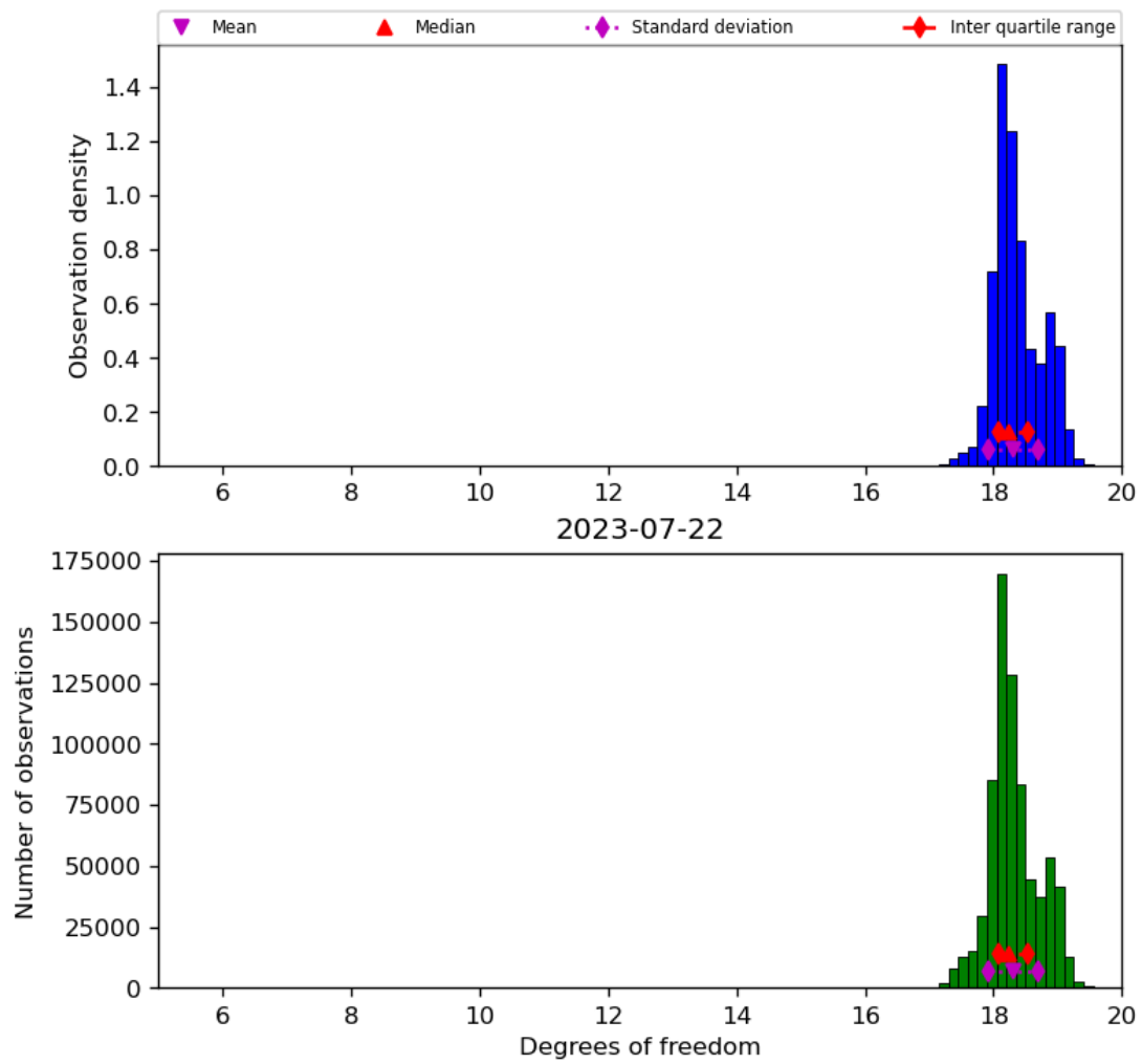
Figure 30: Histogram of “Degrees of freedom” for 2023-07-21 to 2023-07-23
