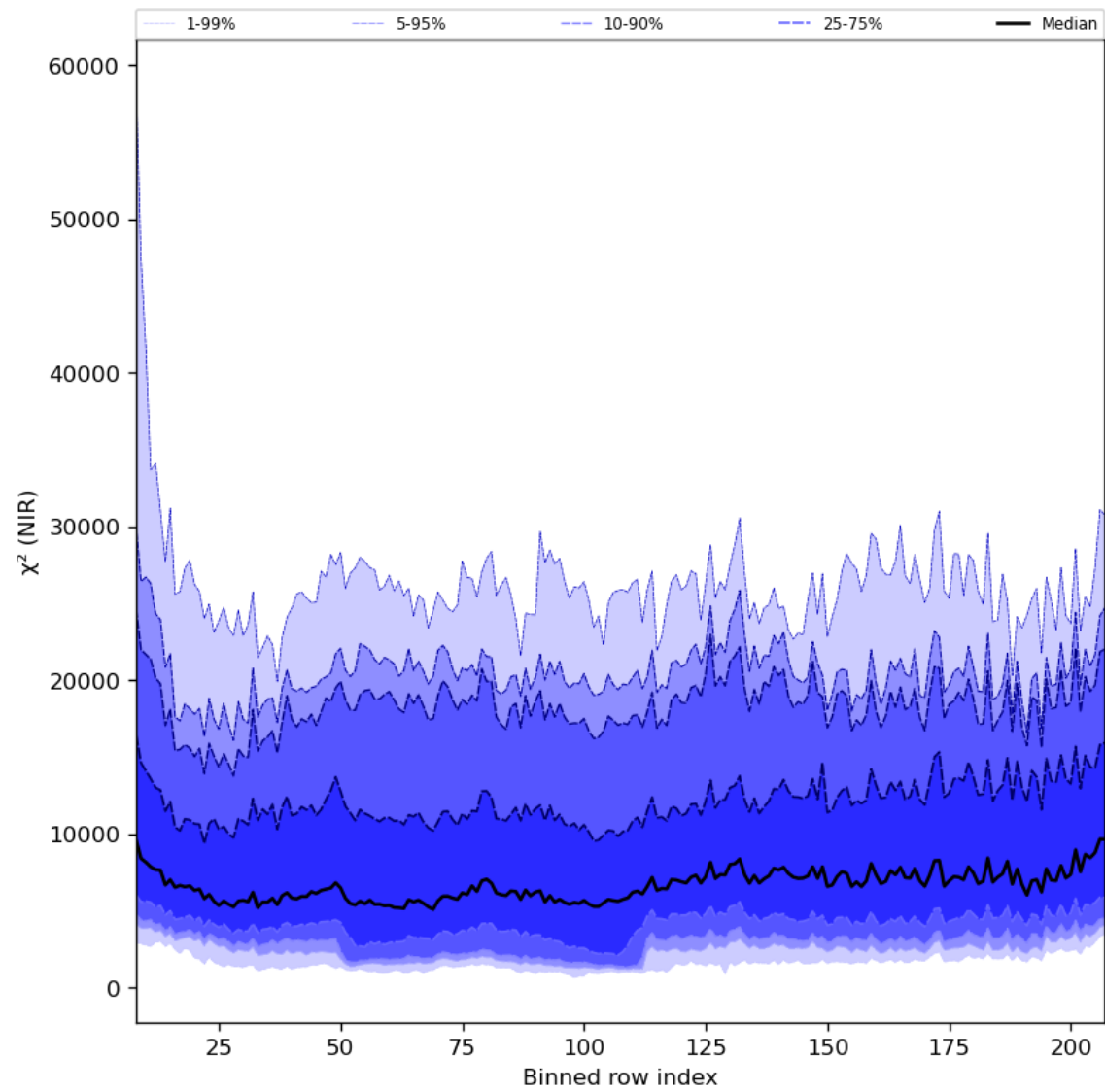
Figure 40: Along track statistics of “ \chi^2 (NIR)” for 2023-07-21 to 2023-07-23
