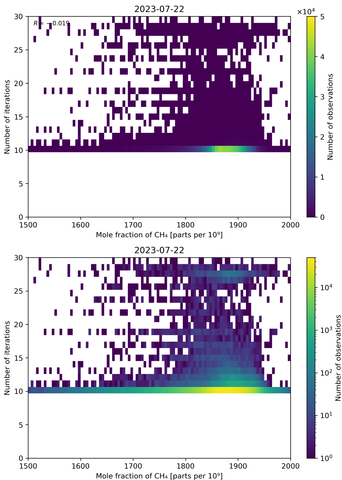
Figure 76: Scatter density plot of “Mole fraction of CH 4 ” against “Number of iterations” for 2023-07-21 to 2023-07-23.
