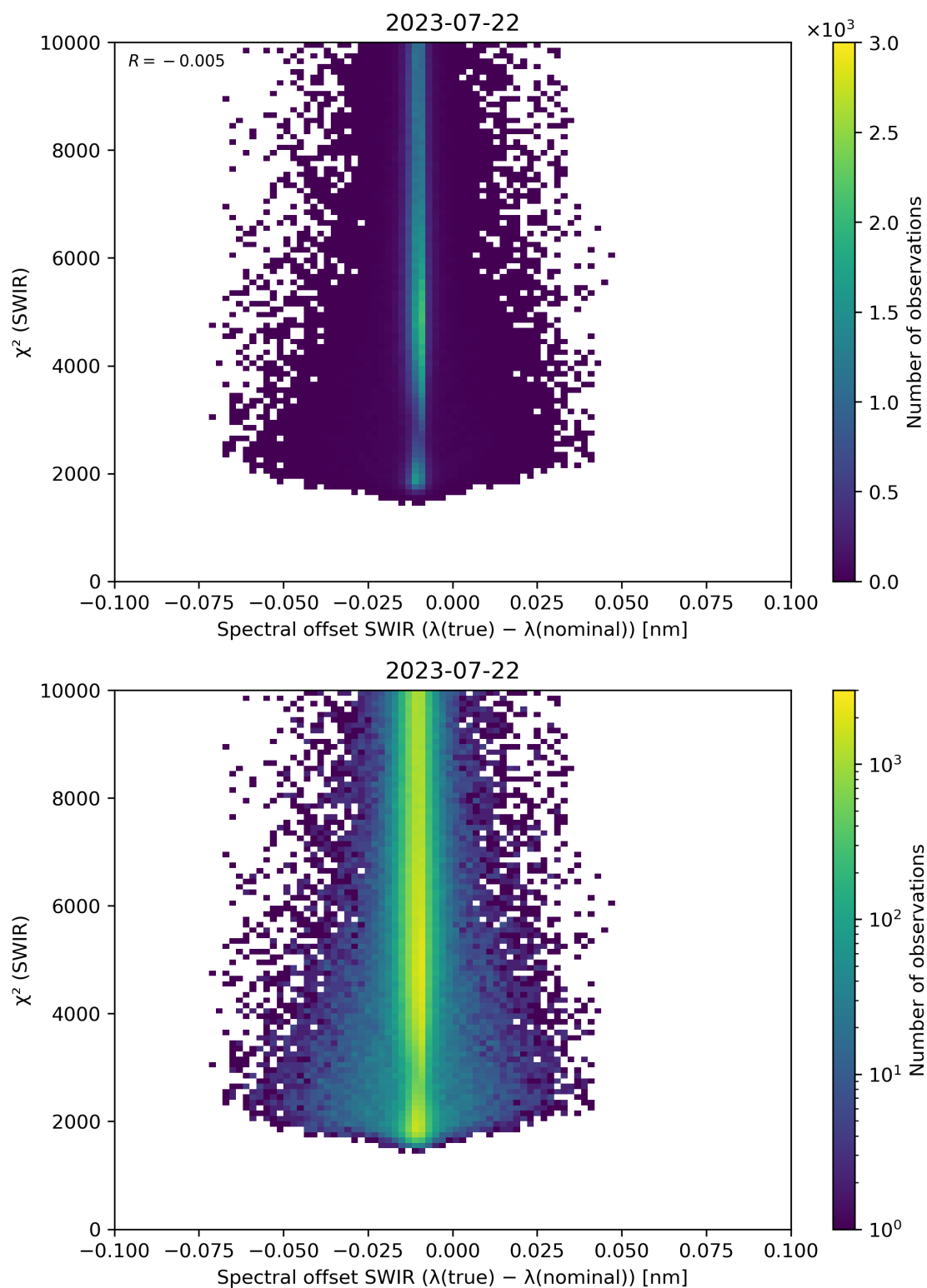
Figure 118: Scatter density plot of “Spectral offset SWIR ( \lambda(\text{true}) - \lambda(\text{nominal}) )” against “ \chi^2 (SWIR)” for 2023-07-21 to 2023-07-23.
