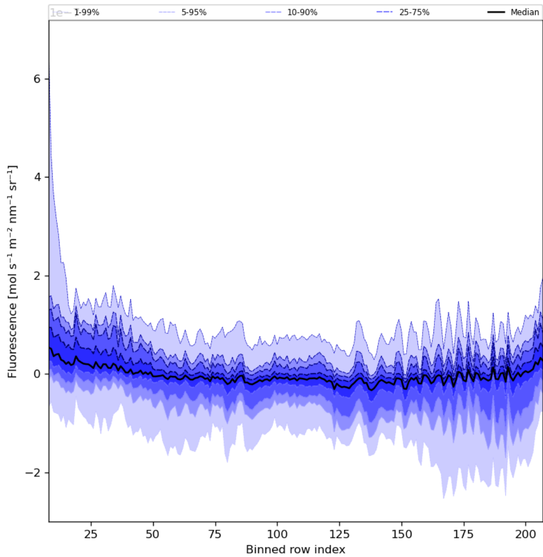
Figure 43: Along track statistics of “Fluorescence” for 2023-07-21 to 2023-07-23
