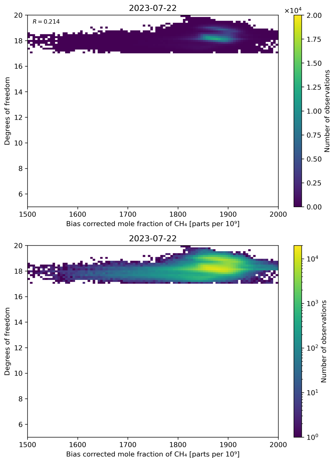
Figure 65: Scatter density plot of “Bias corrected mole fraction of CH 4 ” against “Degrees of freedom” for 2023-07-21 to 2023-07-23.
