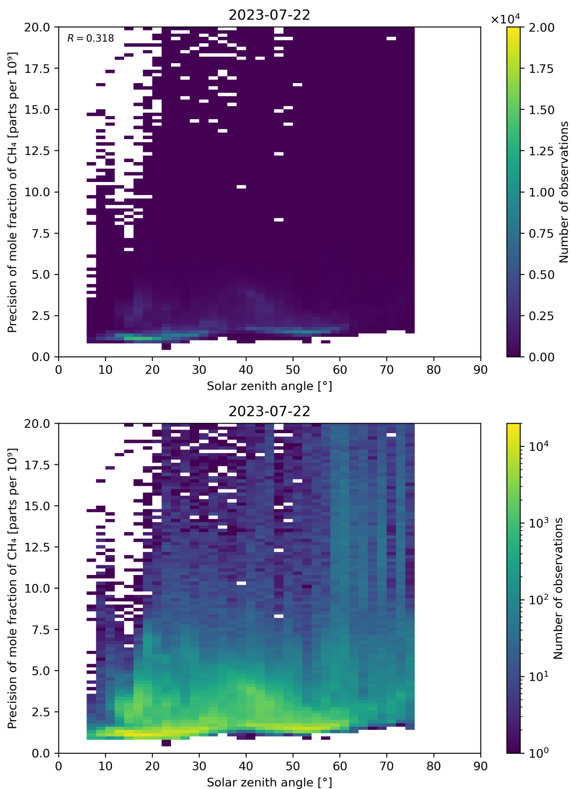
Figure 101: Scatter density plot of “Solar zenith angle” against “Precision of mole fraction of CH 4 ” for 2023-07-21 to 2023-07-23.
