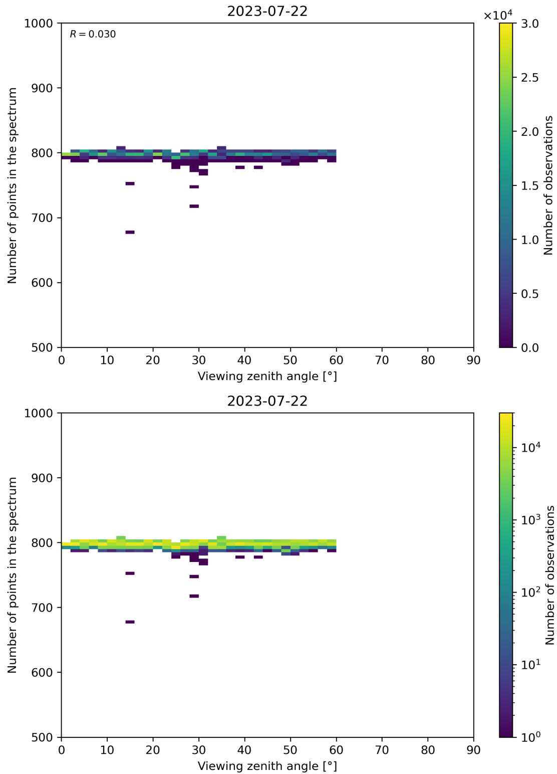
Figure 114: Scatter density plot of “Viewing zenith angle” against “Number of points in the spectrum” for 2023-07-21 to 2023-07-23.
