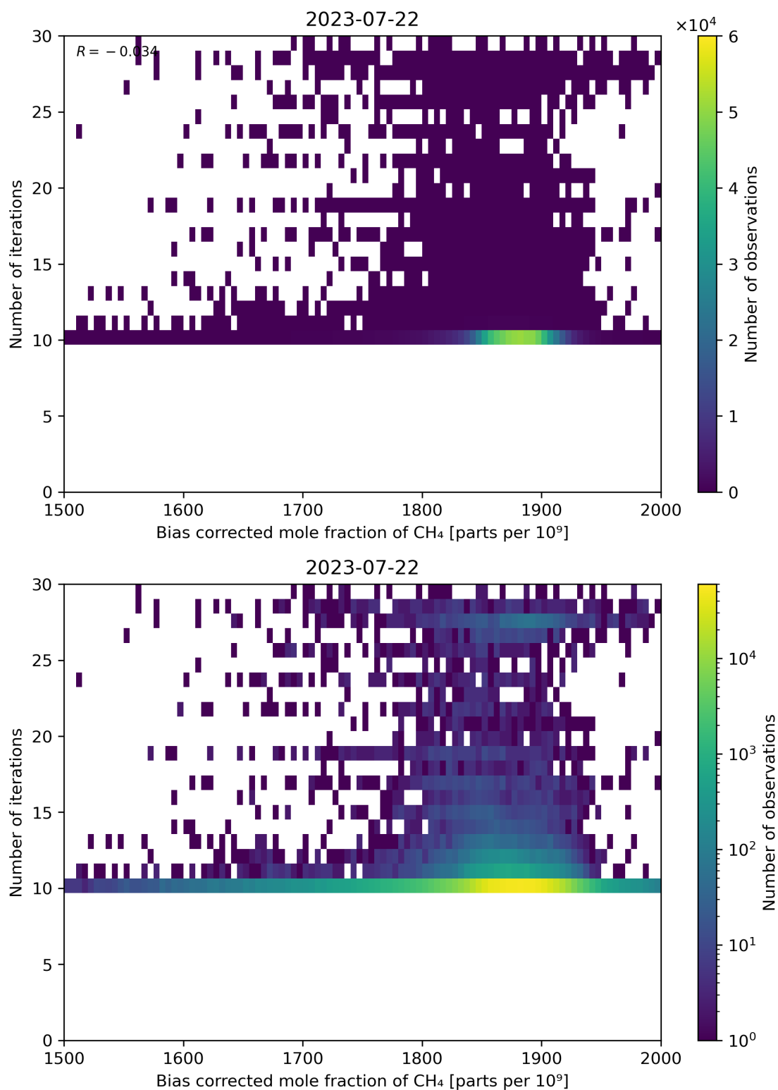
Figure 67: Scatter density plot of “Bias corrected mole fraction of \text{CH}_4 ” against “Number of iterations” for 2023-07-21 to 2023-07-23.
