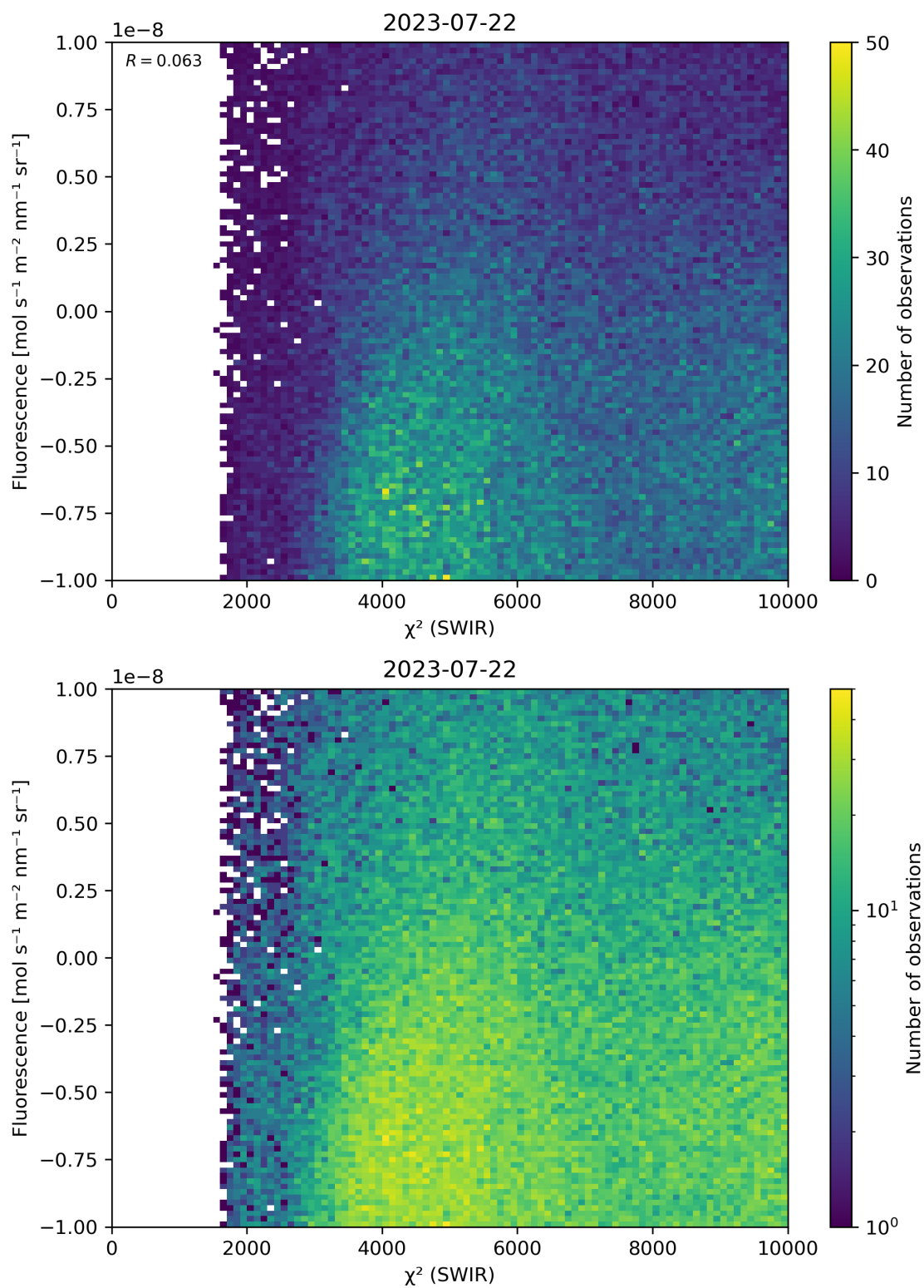
Figure 49: Scatter density plot of “ \chi^2 (SWIR)” against “Fluorescence” for 2023-07-21 to 2023-07-23.
