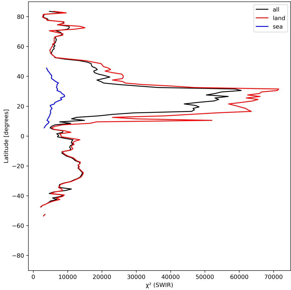
Figure 17: Zonal average of “ \chi^2 (SWIR)” for 2023-07-21 to 2023-07-23.
