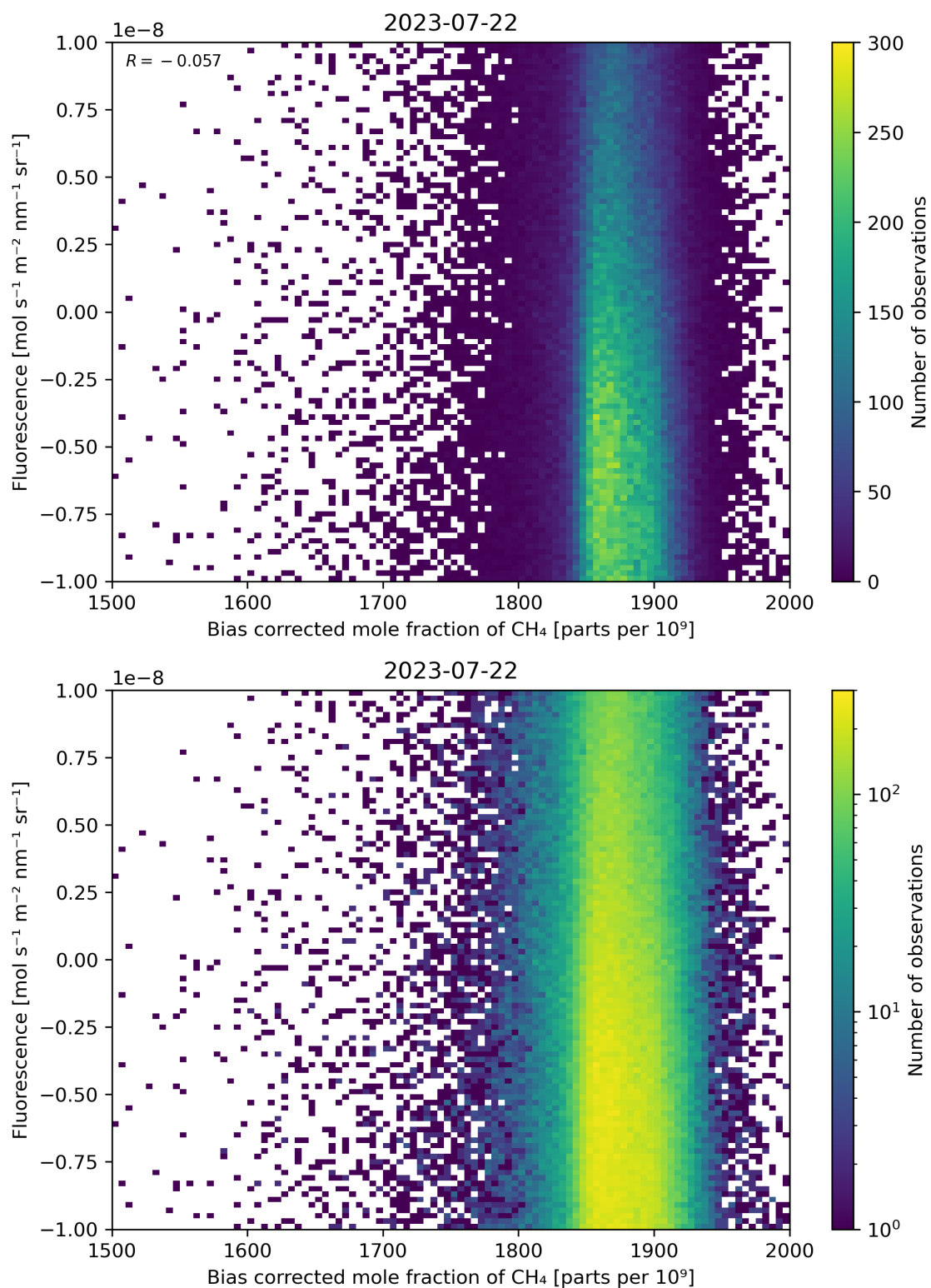
Figure 66: Scatter density plot of “Bias corrected mole fraction of \text{CH}_4 ” against “Fluorescence” for 2023-07-21 to 2023-07-23.
