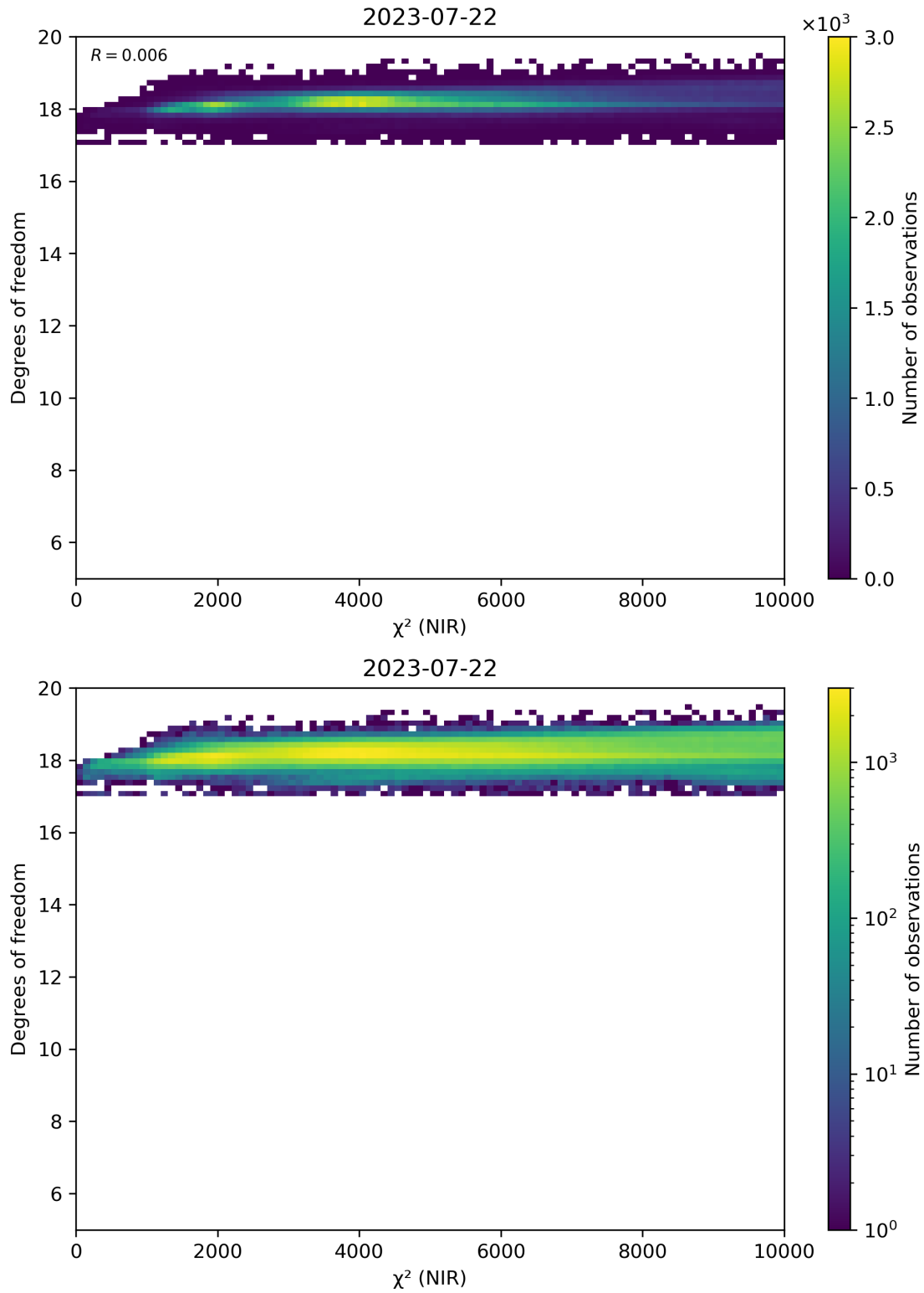
Figure 44: Scatter density plot of “ \chi^2 (NIR)” against “Degrees of freedom” for 2023-07-21 to 2023-07-23.
