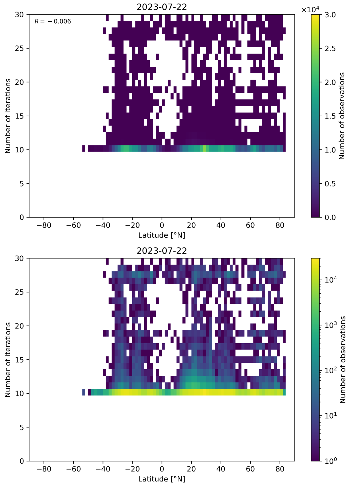
Figure 60: Scatter density plot of “Latitude” against “Number of iterations” for 2023-07-21 to 2023-07-23.
