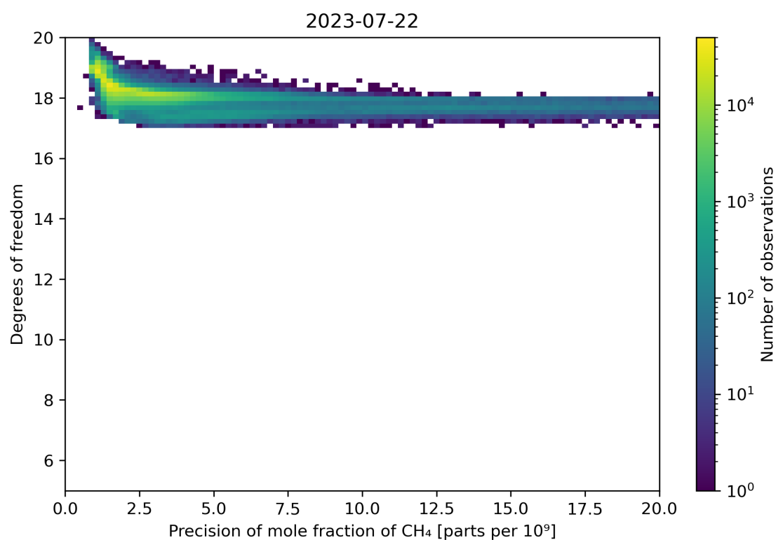
Figure 80: Scatter density plot of “Precision of mole fraction of CH 4 ” against “Degrees of freedom” for 2023-07-21 to 2023-07-23.
