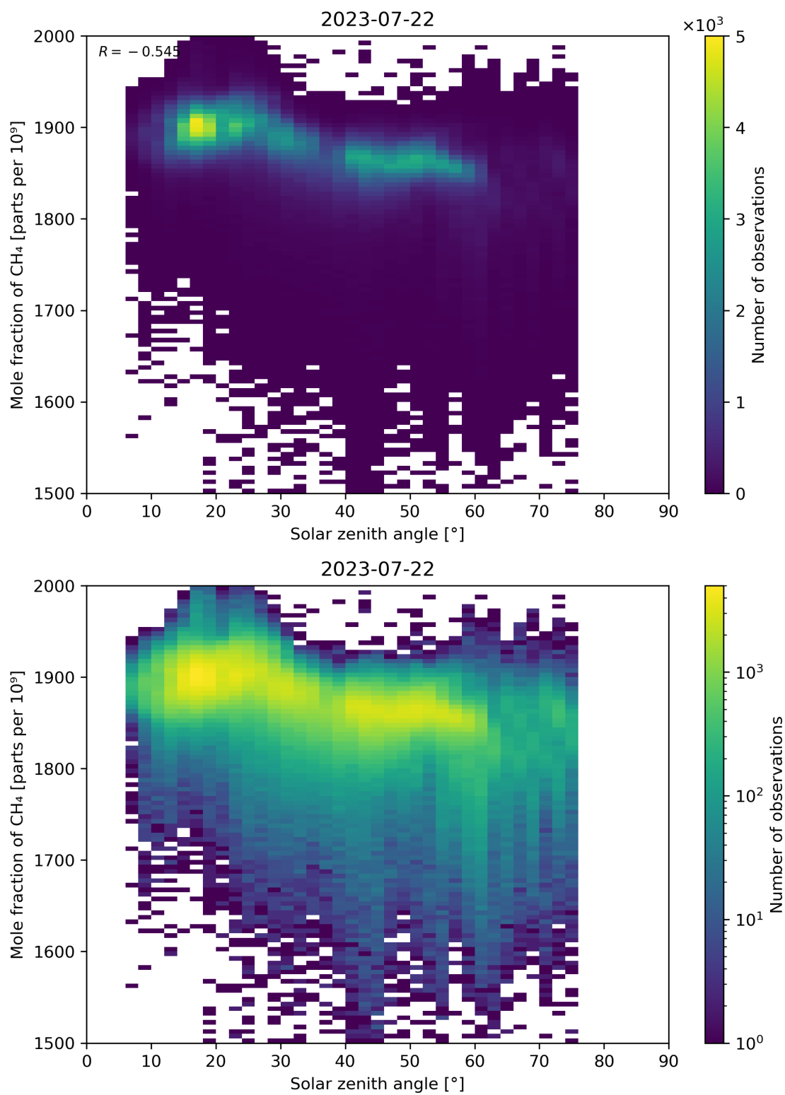
Figure 99: Scatter density plot of “Solar zenith angle” against “Mole fraction of CH 4 ” for 2023-07-21 to 2023-07-23.
