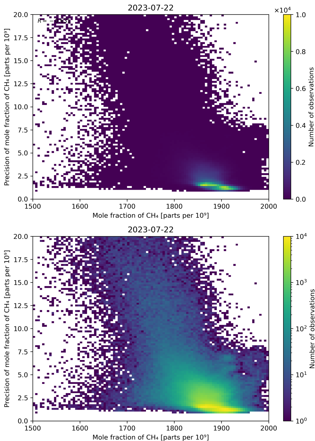
Figure 75: Scatter density plot of “Mole fraction of CH 4 ” against “Precision of mole fraction of CH 4 ” for 2023-07-21 to 2023-07-23.
