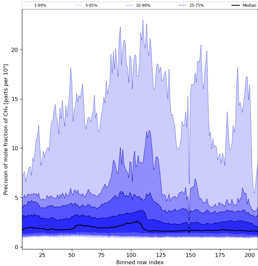
Figure 35: Along track statistics of “Precision of mole fraction of CH 4 ” for 2023-07-21 to 2023-07-23
