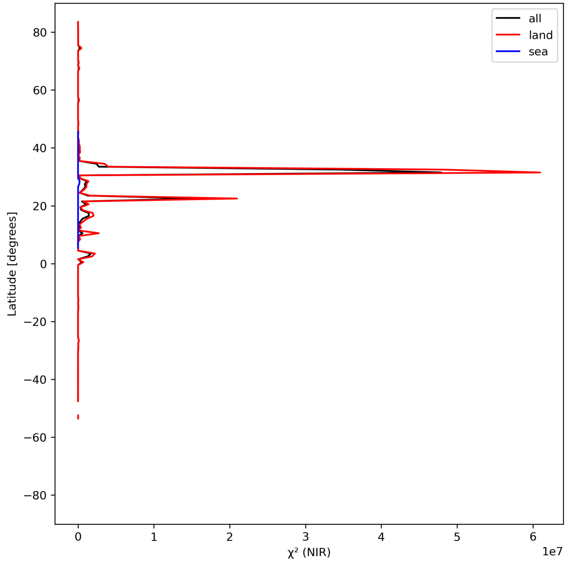
Figure 18: Zonal average of “ \chi^2 (NIR)” for 2023-07-21 to 2023-07-23.
