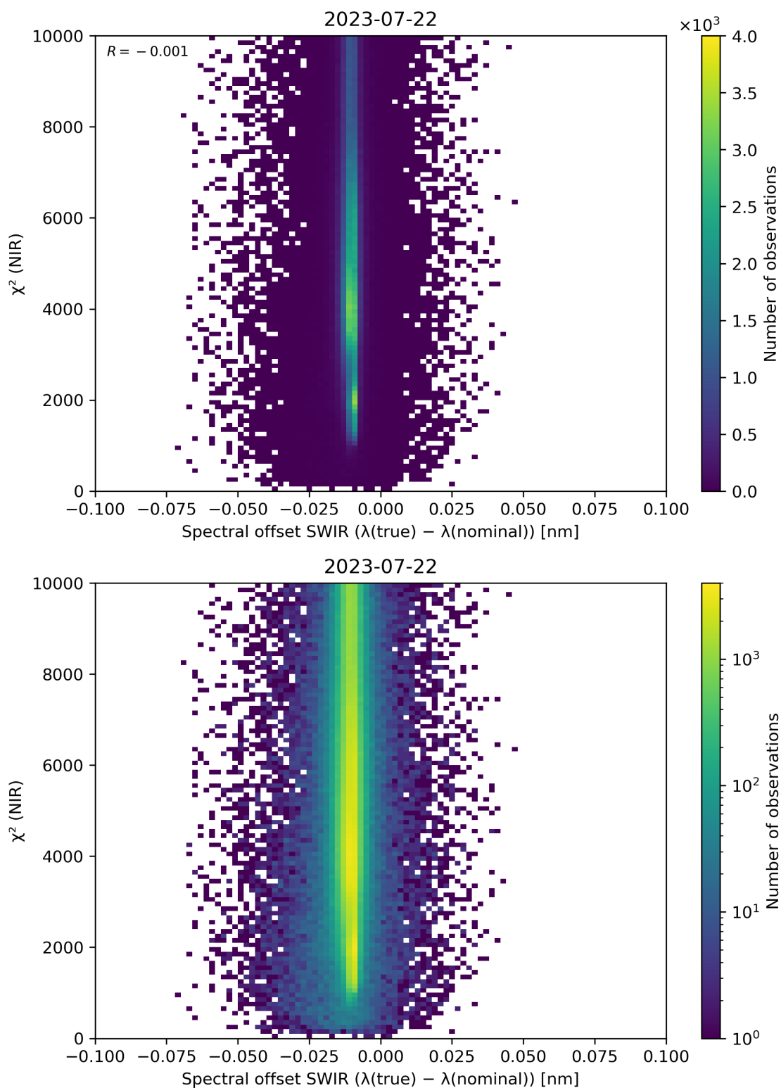
Figure 117: Scatter density plot of “Spectral offset SWIR ( \lambda(\text{true}) - \lambda(\text{nominal}) )” against “ \chi^2 (NIR)” for 2023-07-21 to 2023-07-23.
