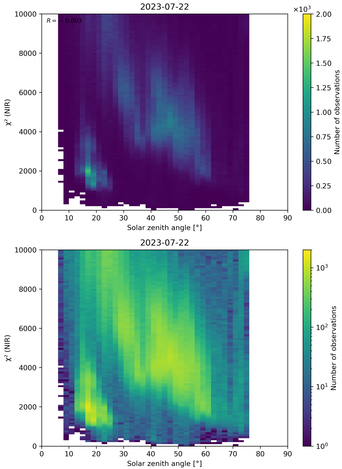
Figure 94: Scatter density plot of “Solar zenith angle” against “ \chi^2 (NIR)” for 2023-07-21 to 2023-07-23.
