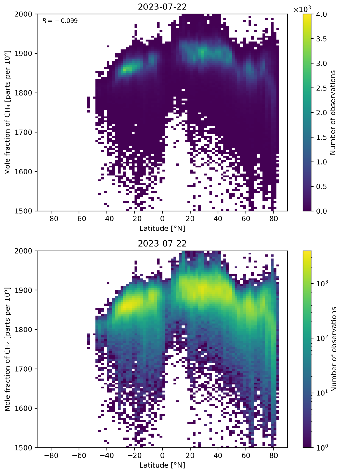
Figure 57: Scatter density plot of “Latitude” against “Mole fraction of CH 4 ” for 2023-07-21 to 2023-07-23.
