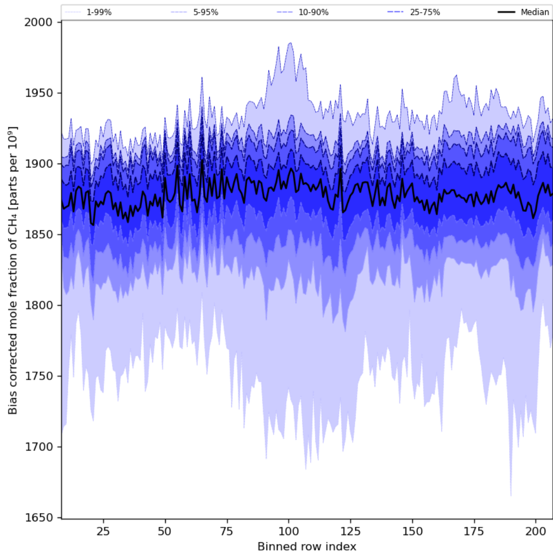
Figure 36: Along track statistics of “Bias corrected mole fraction of CH 4 ” for 2023-07-21 to 2023-07-23
