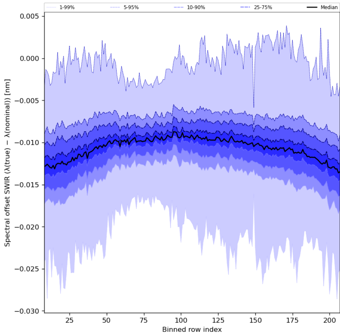
Figure 38: Along track statistics of “Spectral offset SWIR ( \lambda(\text{true}) - \lambda(\text{nominal}) )” for 2023-07-21 to 2023-07-23
