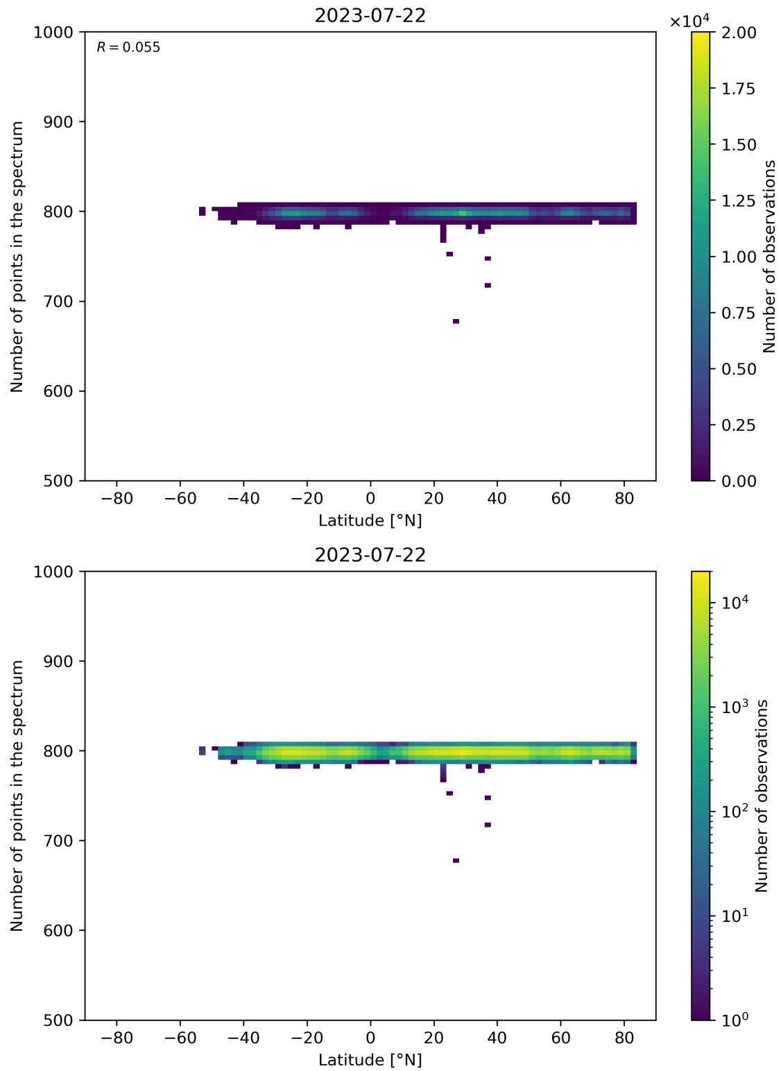
Figure 61: Scatter density plot of “Latitude” against “Number of points in the spectrum” for 2023-07-21 to 2023-07-23.
