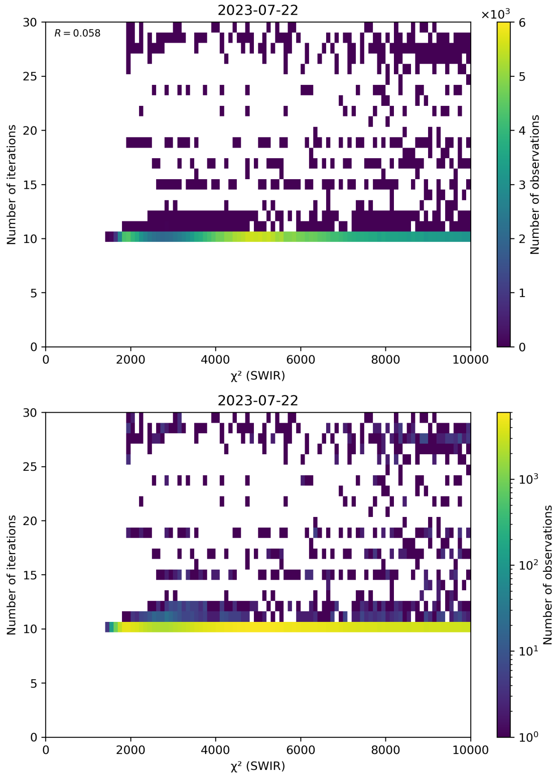
Figure 50: Scatter density plot of “ \chi^2 (SWIR)” against “Number of iterations” for 2023-07-21 to 2023-07-23.
