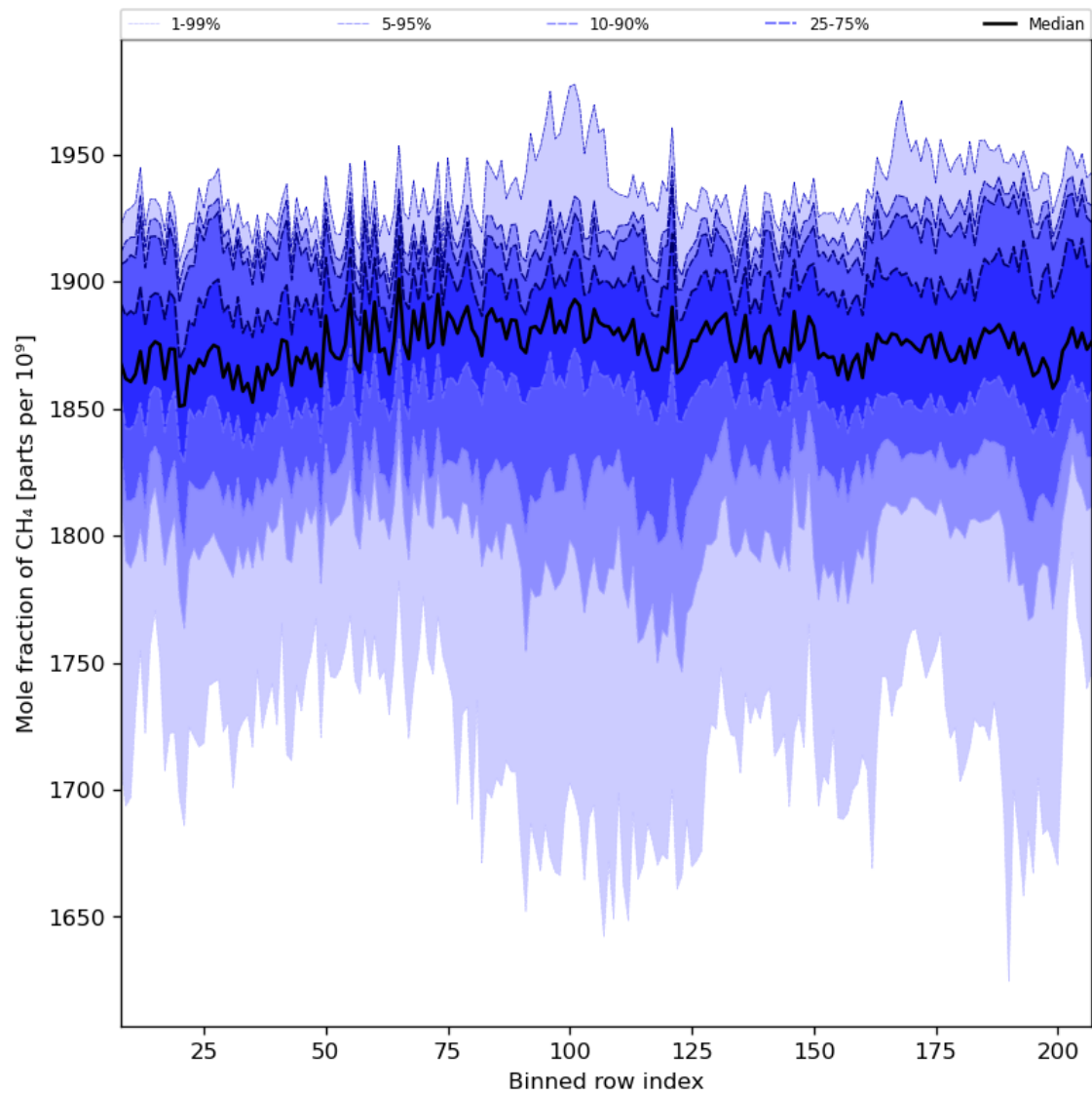
Figure 34: Along track statistics of “Mole fraction of CH 4 ” for 2023-07-21 to 2023-07-23
