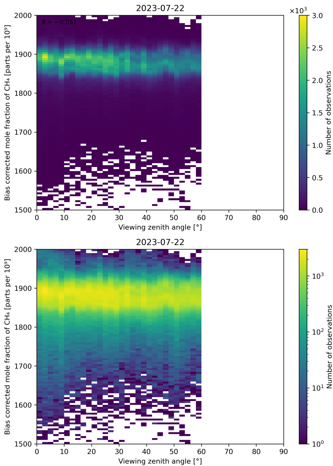
Figure 111: Scatter density plot of “Viewing zenith angle” against “Bias corrected mole fraction of CH 4 ” for 2023-07-21 to 2023-07-23.
