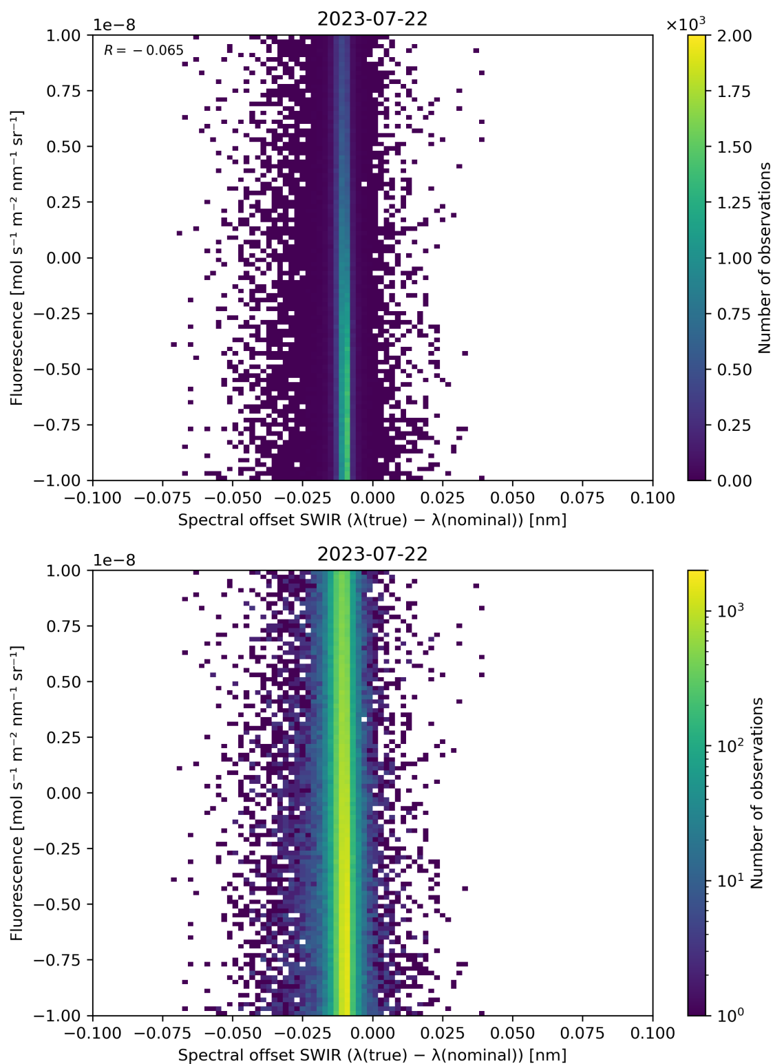
Figure 120: Scatter density plot of “Spectral offset SWIR ( \lambda(\text{true}) - \lambda(\text{nominal}) )” against “Fluorescence” for 2023-07-21 to 2023-07-23.
