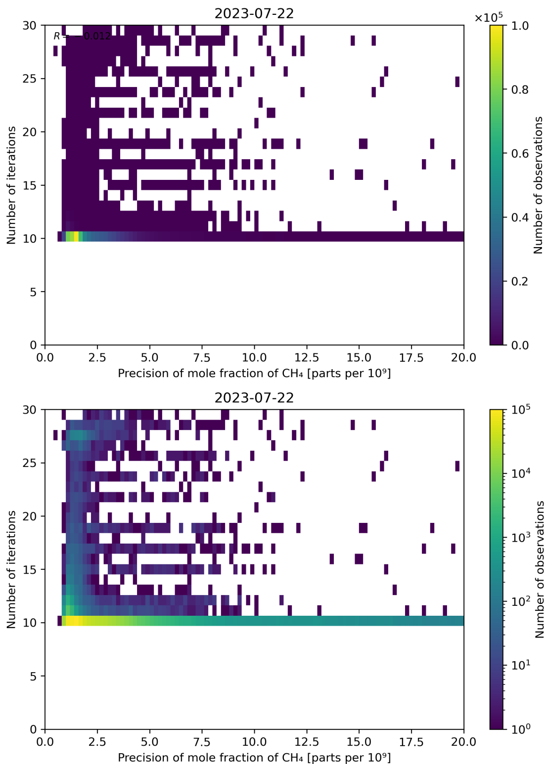
Figure 83: Scatter density plot of “Precision of mole fraction of CH 4 ” against “Number of iterations” for 2023-07-21 to 2023-07-23.
