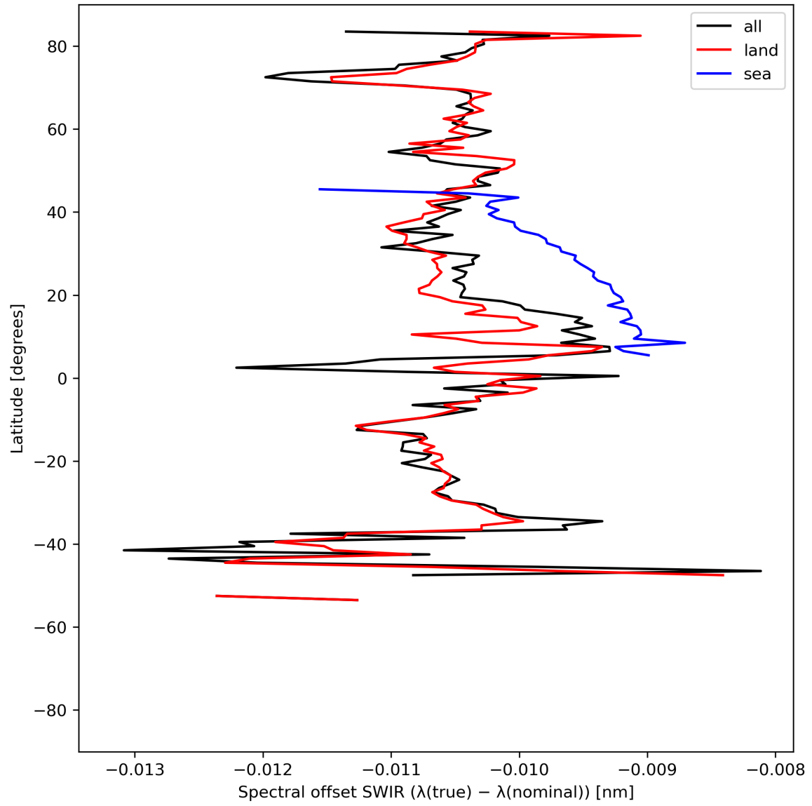
Figure 16: Zonal average of “Spectral offset SWIR ( \lambda(\text{true}) - \lambda(\text{nominal}) )” for 2023-07-21 to 2023-07-23.
