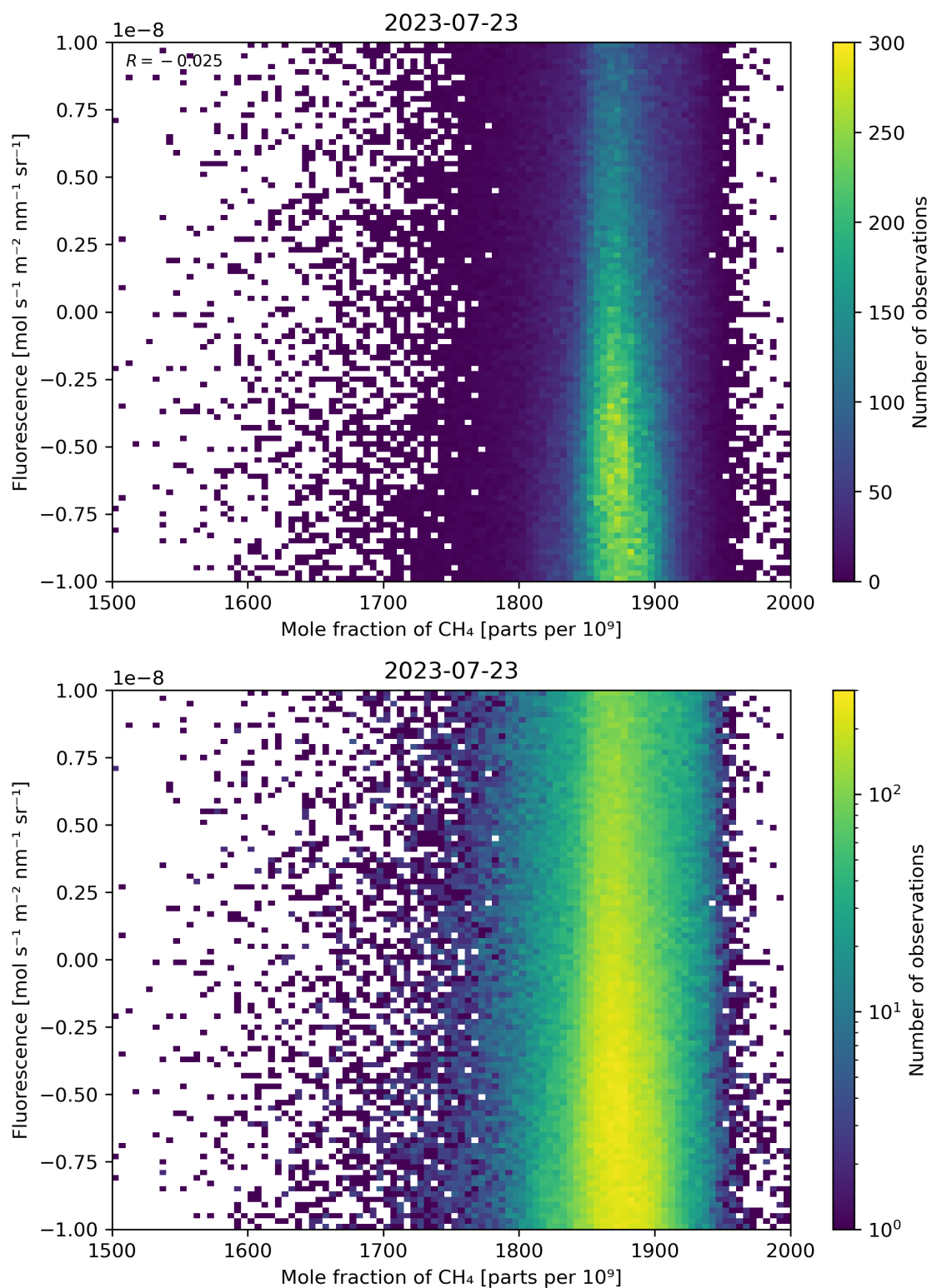
Figure 73: Scatter density plot of “Mole fraction of \text{CH}_4 ” against “Fluorescence” for 2023-07-22 to 2023-07-24.
