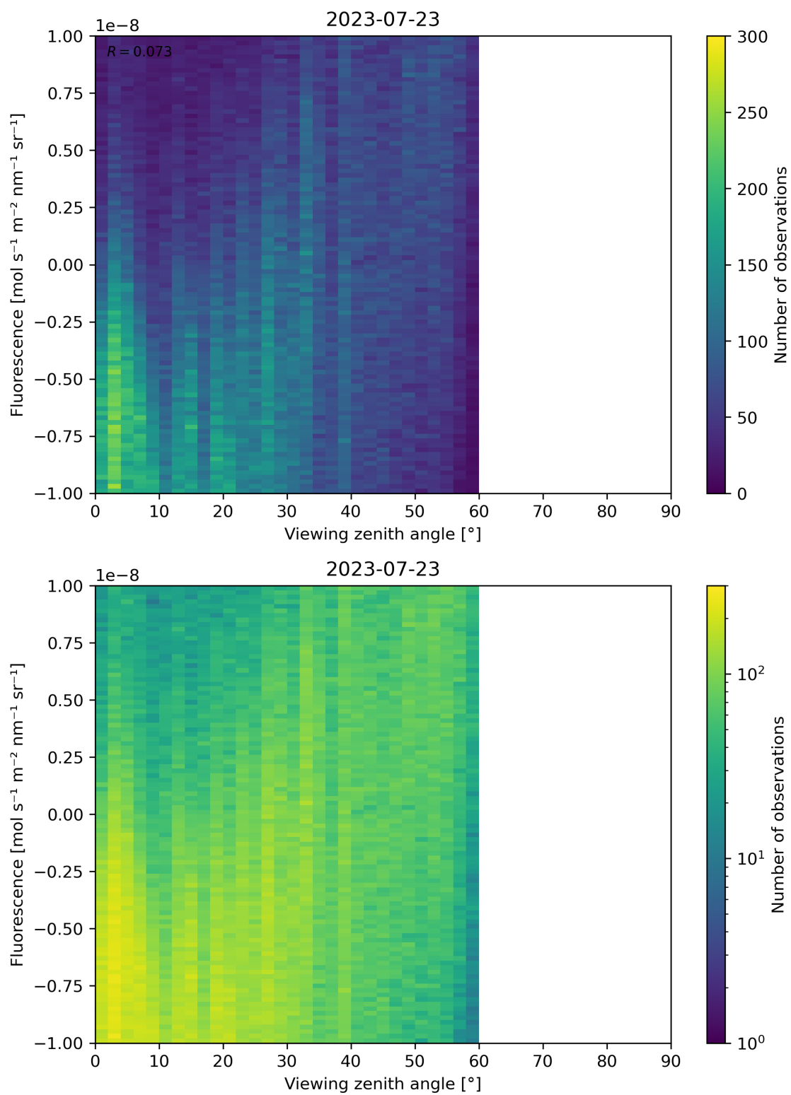
Figure 108: Scatter density plot of “Viewing zenith angle” against “Fluorescence” for 2023-07-22 to 2023-07-24.
