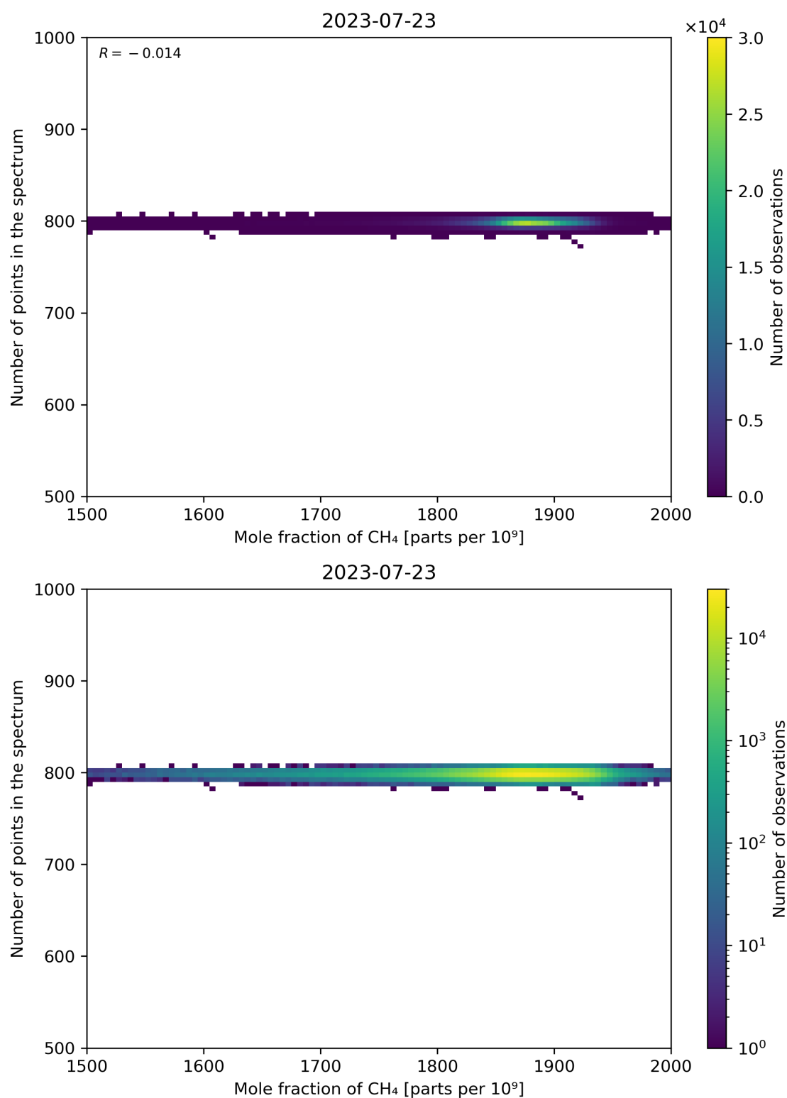
Figure 77: Scatter density plot of “Mole fraction of CH 4 ” against “Number of points in the spectrum” for 2023-07-22 to 2023-07-24.
