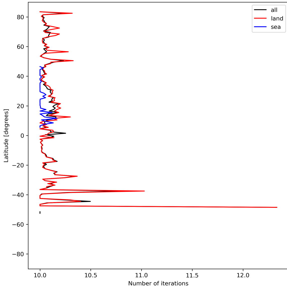
Figure 20: Zonal average of “Number of iterations” for 2023-07-22 to 2023-07-24.
