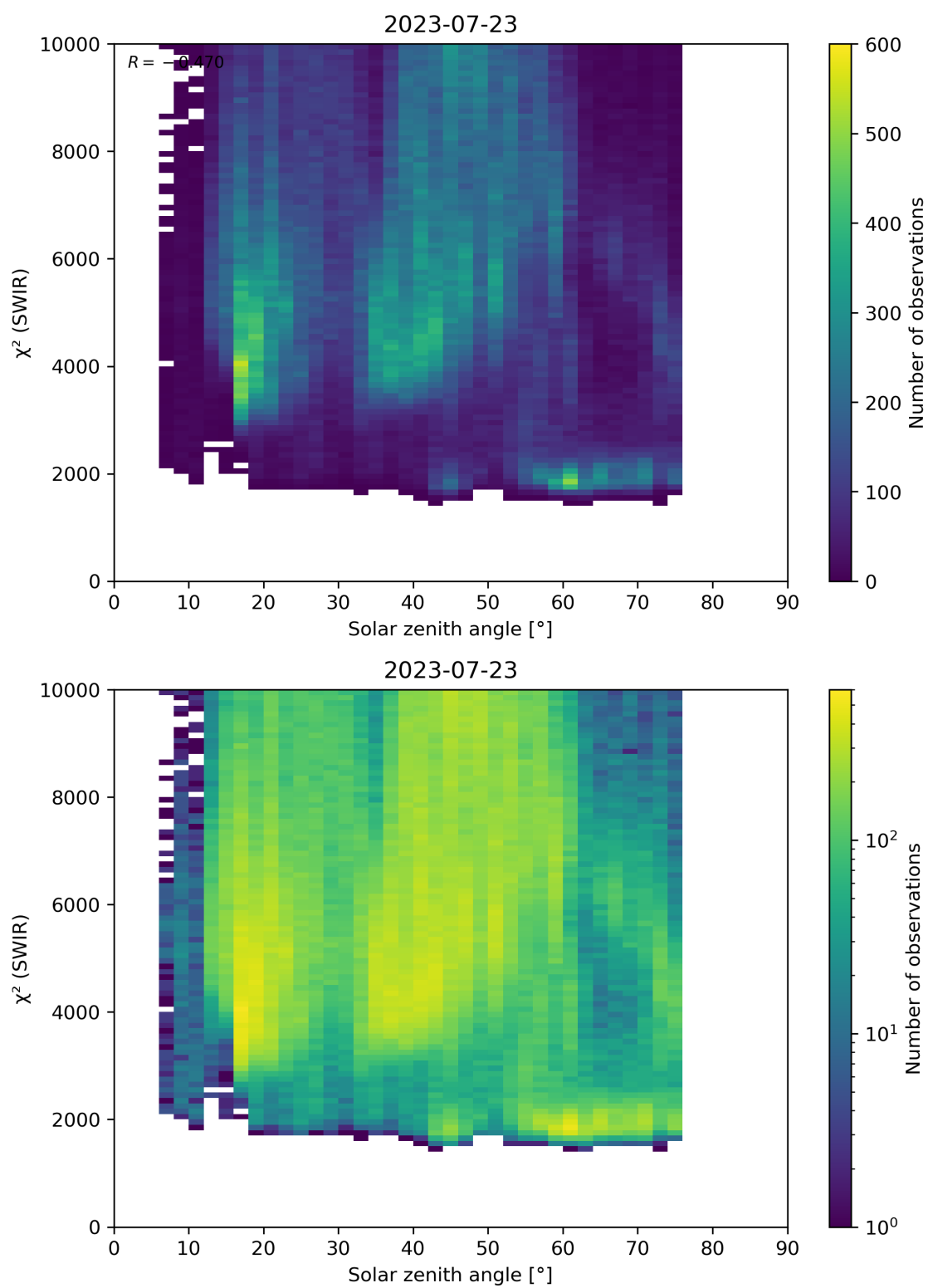
Figure 95: Scatter density plot of “Solar zenith angle” against “ \chi^2 (SWIR)” for 2023-07-22 to 2023-07-24.
