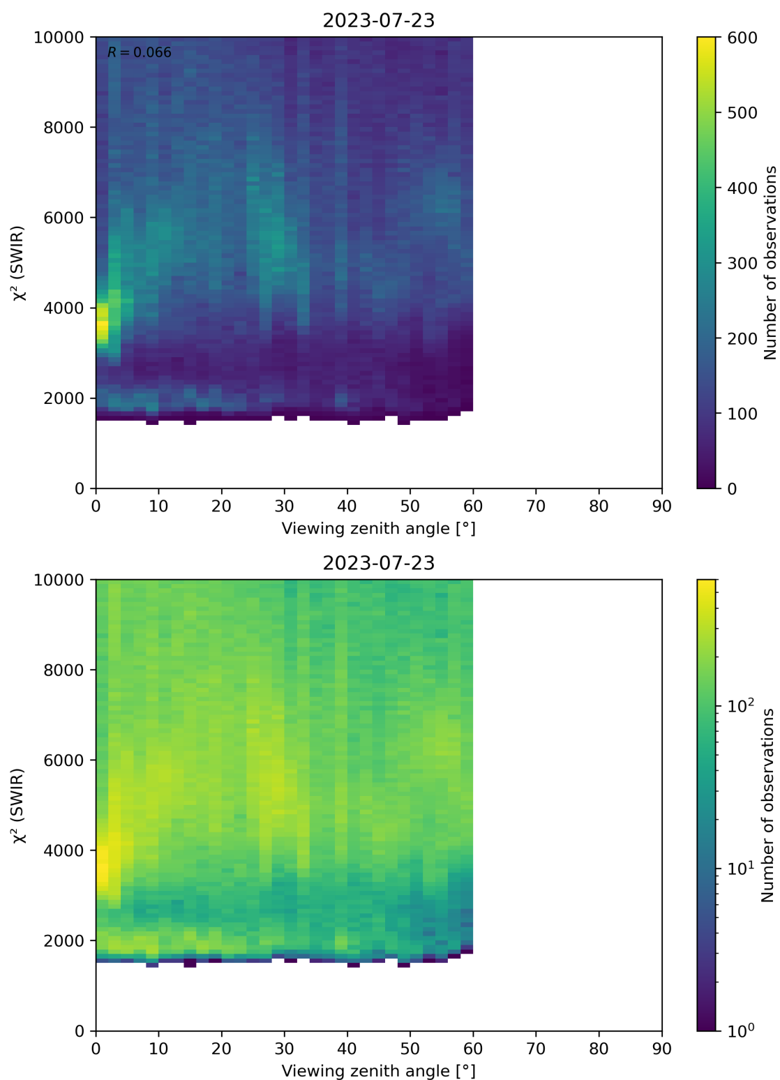
Figure 106: Scatter density plot of “Viewing zenith angle” against “ \chi^2 (SWIR)” for 2023-07-22 to 2023-07-24.
