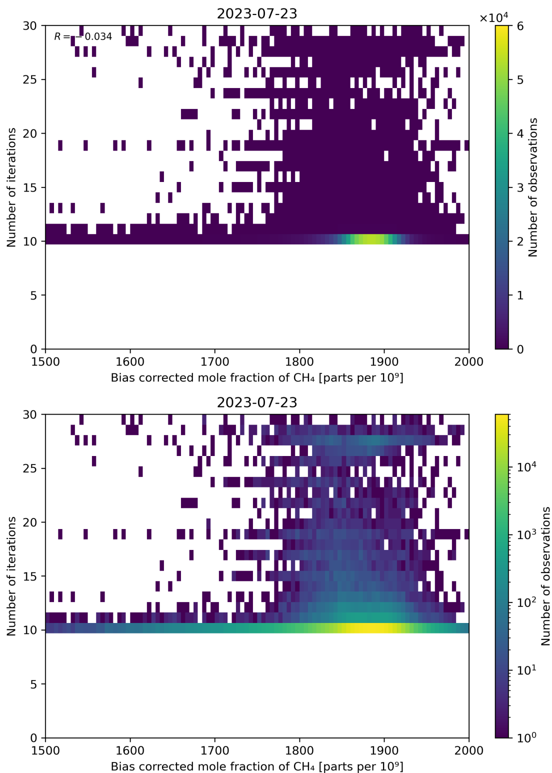
Figure 67: Scatter density plot of “Bias corrected mole fraction of CH 4 ” against “Number of iterations” for 2023-07-22 to 2023-07-24.
