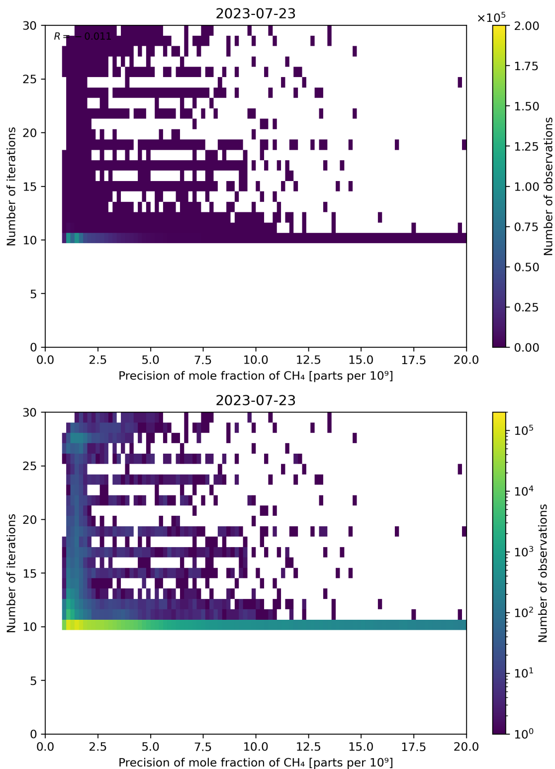
Figure 83: Scatter density plot of “Precision of mole fraction of CH 4 ” against “Number of iterations” for 2023-07-22 to 2023-07-24.
