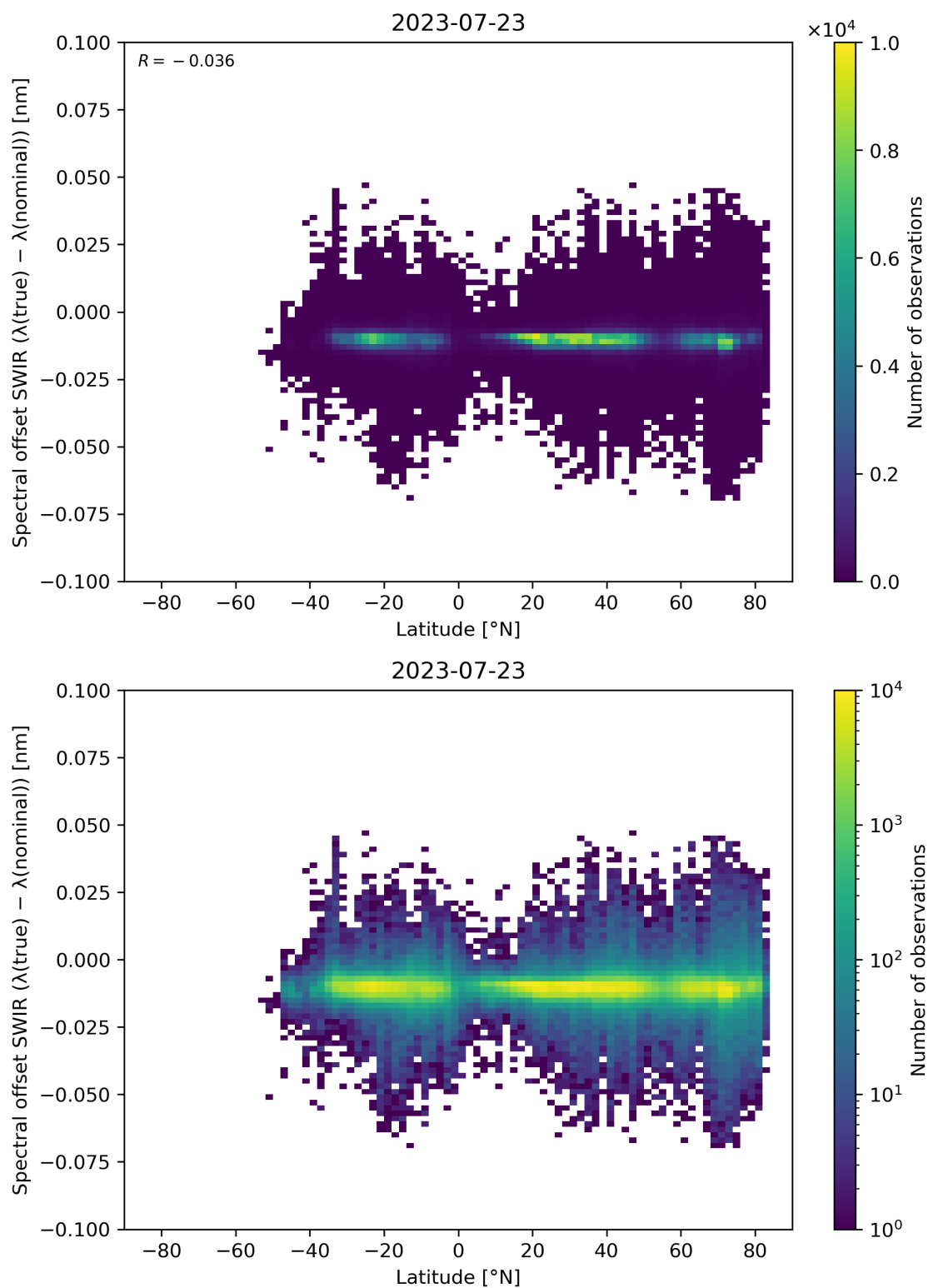
Figure 62: Scatter density plot of “Latitude” against “Spectral offset SWIR ( \lambda(\text{true}) - \lambda(\text{nominal}) )” for 2023-07-22 to 2023-07-24.
