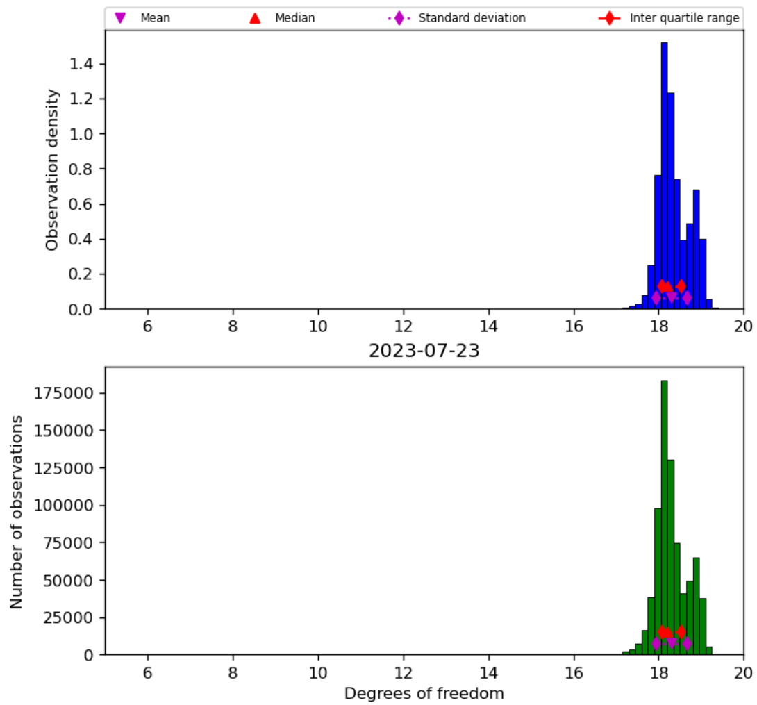
Figure 30: Histogram of “Degrees of freedom” for 2023-07-22 to 2023-07-24
