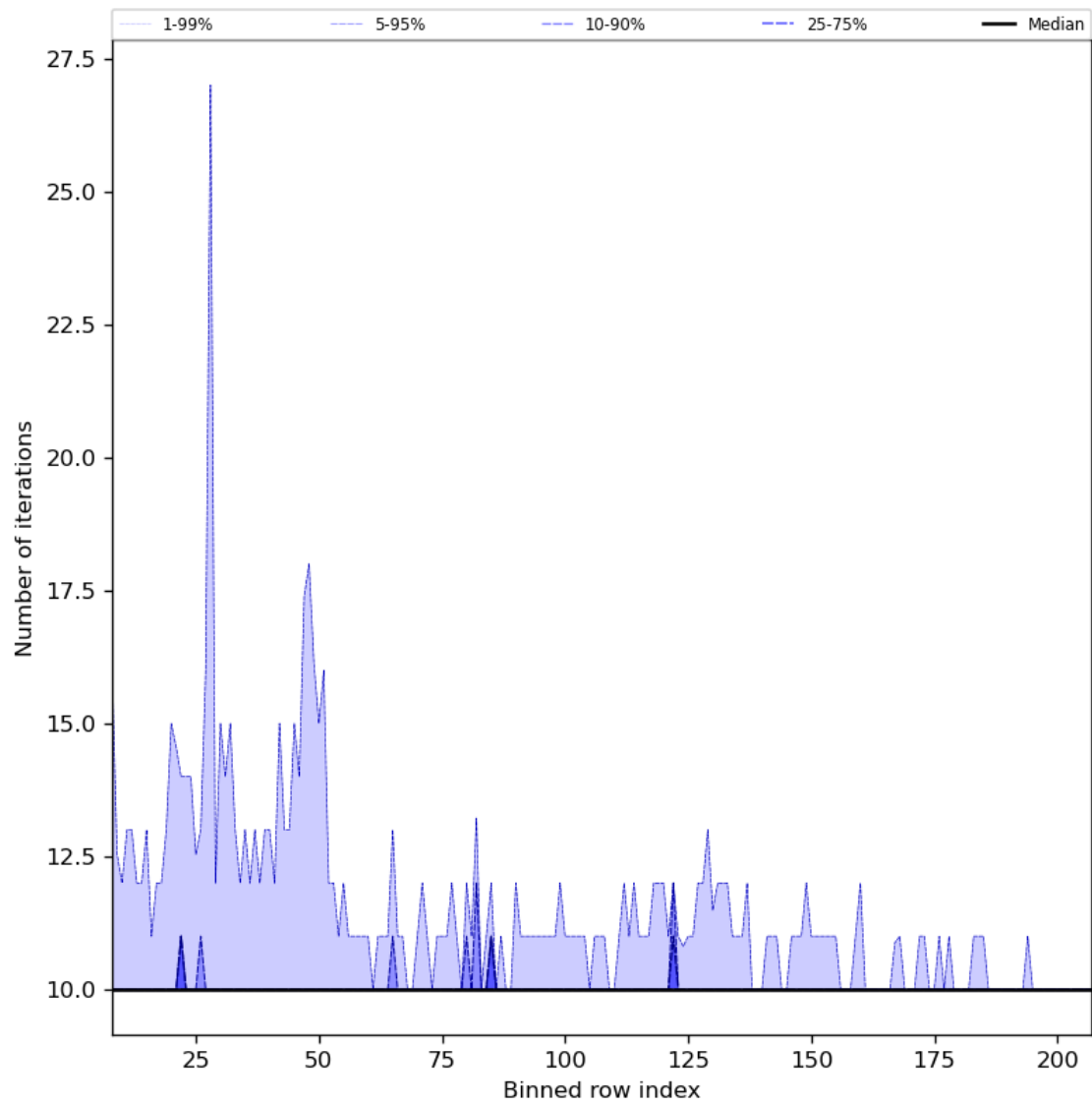
Figure 42: Along track statistics of “Number of iterations” for 2023-07-22 to 2023-07-24
