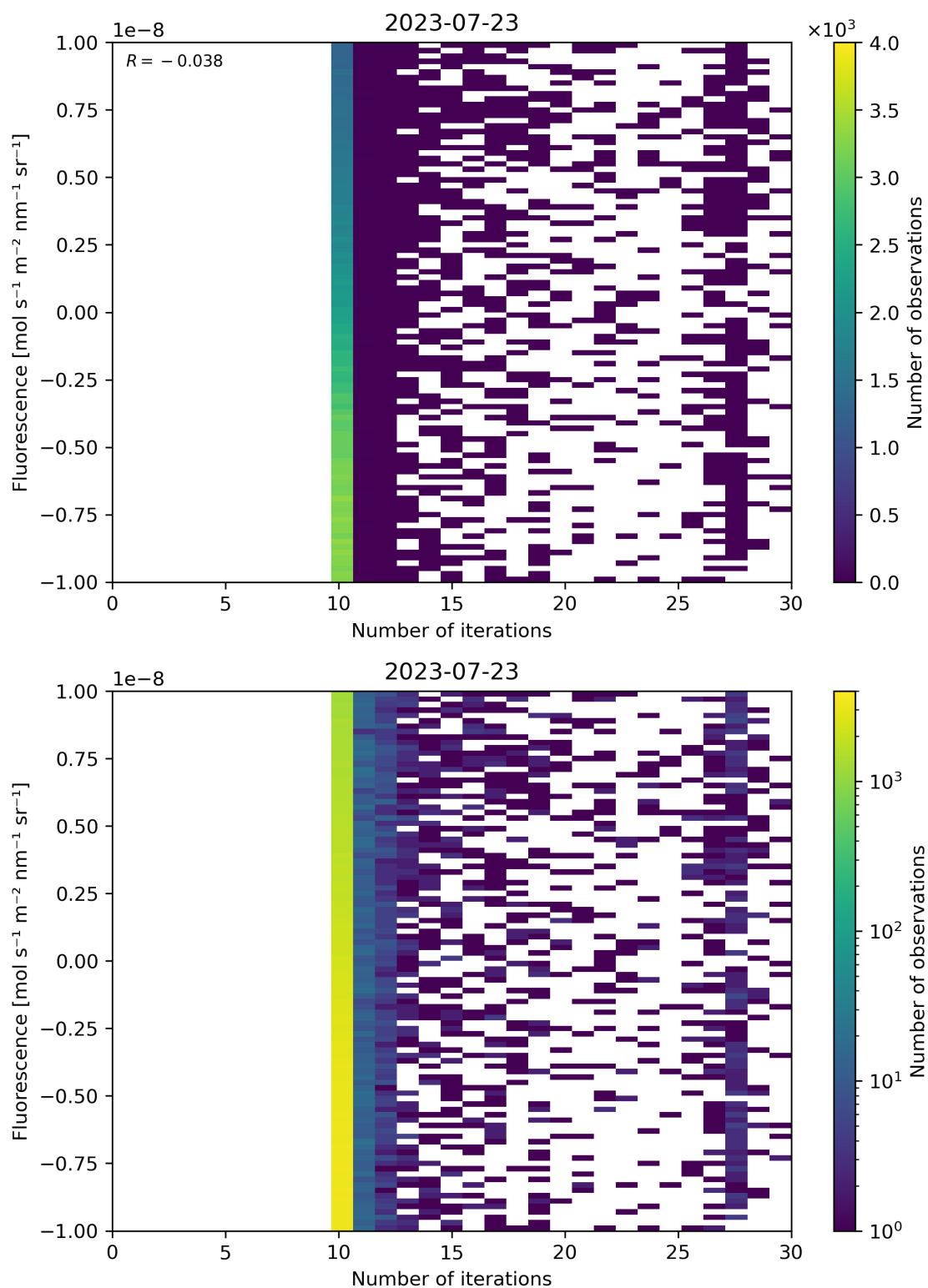
Figure 87: Scatter density plot of “Number of iterations” against “Fluorescence” for 2023-07-22 to 2023-07-24.
