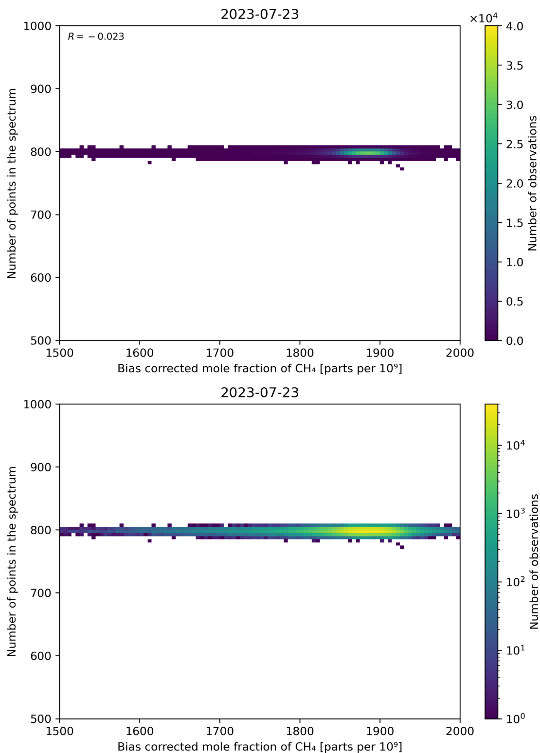
Figure 68: Scatter density plot of “Bias corrected mole fraction of CH 4 ” against “Number of points in the spectrum” for 2023-07-22 to 2023-07-24.
