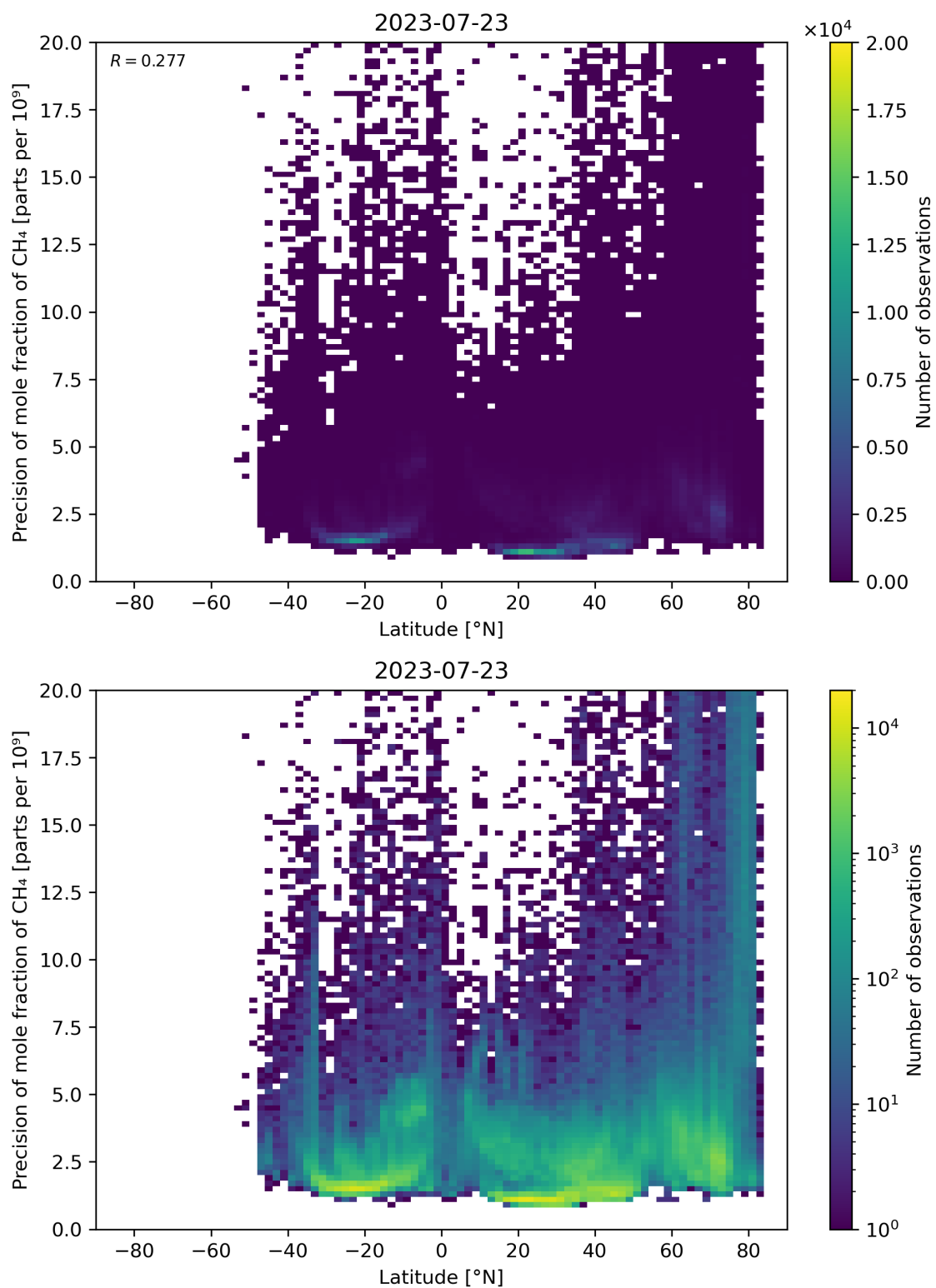
Figure 59: Scatter density plot of “Latitude” against “Precision of mole fraction of \text{CH}_4 ” for 2023-07-22 to 2023-07-24.
