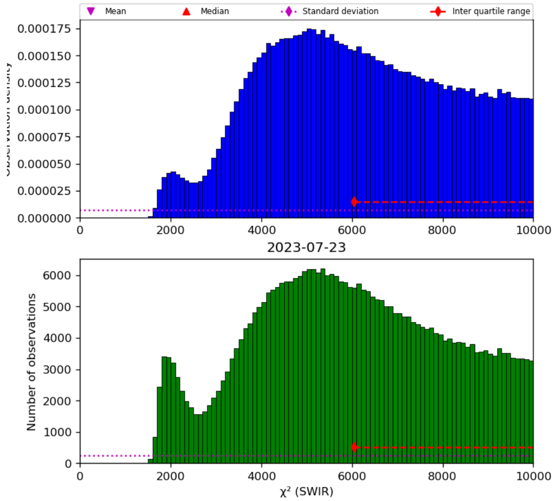
Figure 28: Histogram of “ \chi^2 (SWIR)” for 2023-07-22 to 2023-07-24
