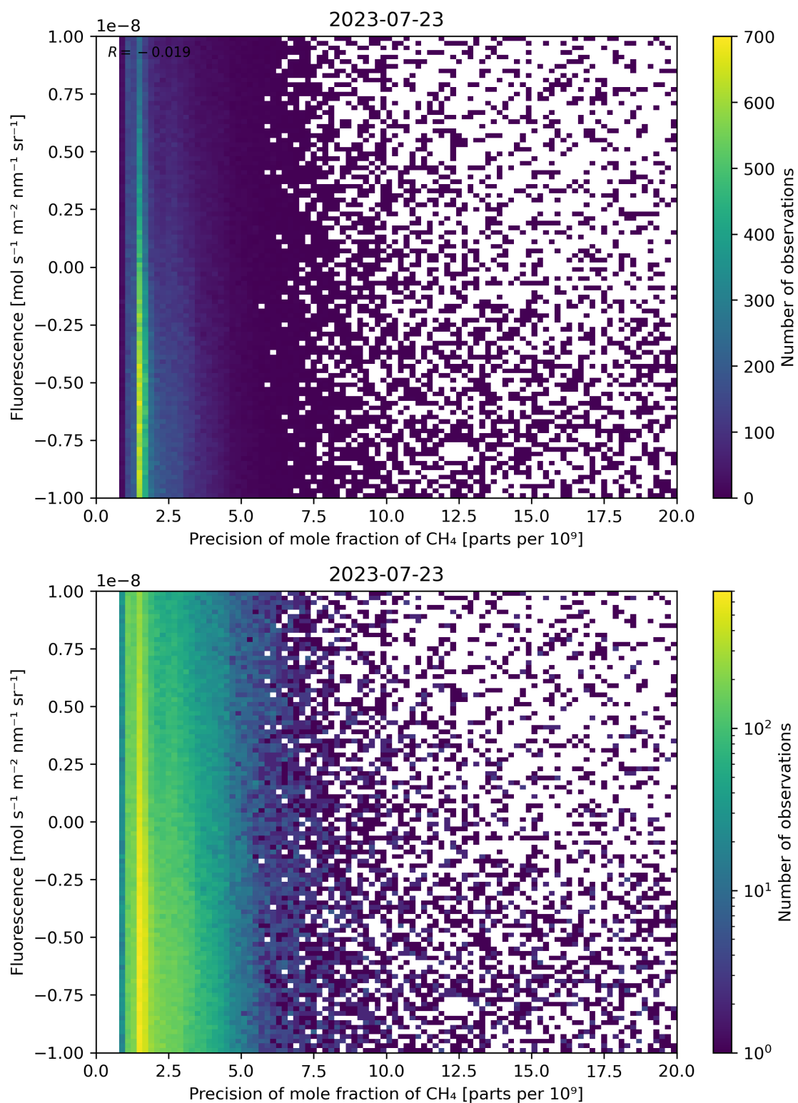
Figure 81: Scatter density plot of “Precision of mole fraction of \text{CH}_4 ” against “Fluorescence” for 2023-07-22 to 2023-07-24.
