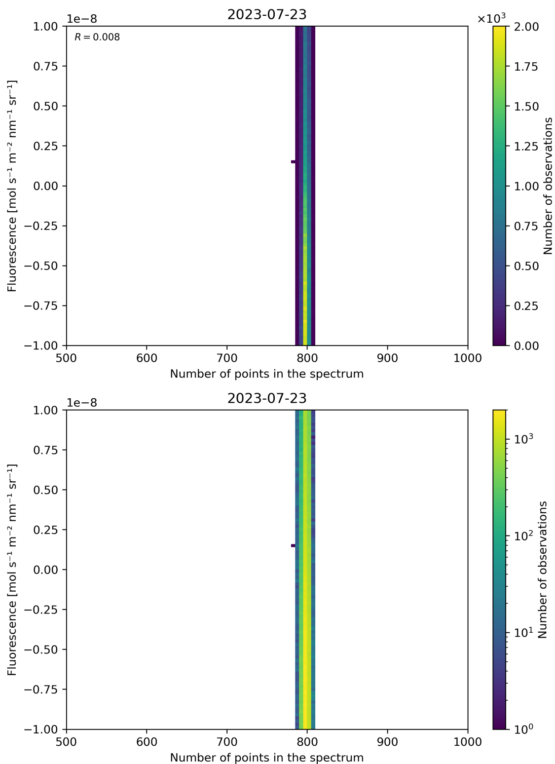
Figure 91: Scatter density plot of “Number of points in the spectrum” against “Fluorescence” for 2023-07-22 to 2023-07-24.
