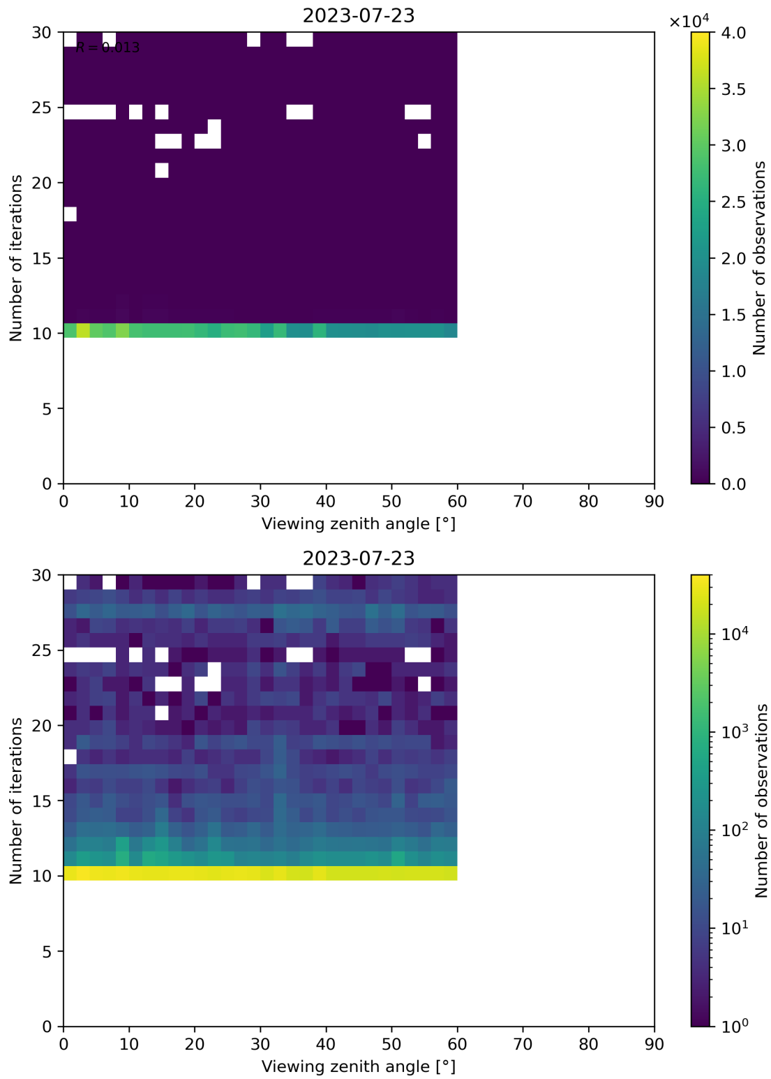
Figure 113: Scatter density plot of “Viewing zenith angle” against “Number of iterations” for 2023-07-22 to 2023-07-24.
