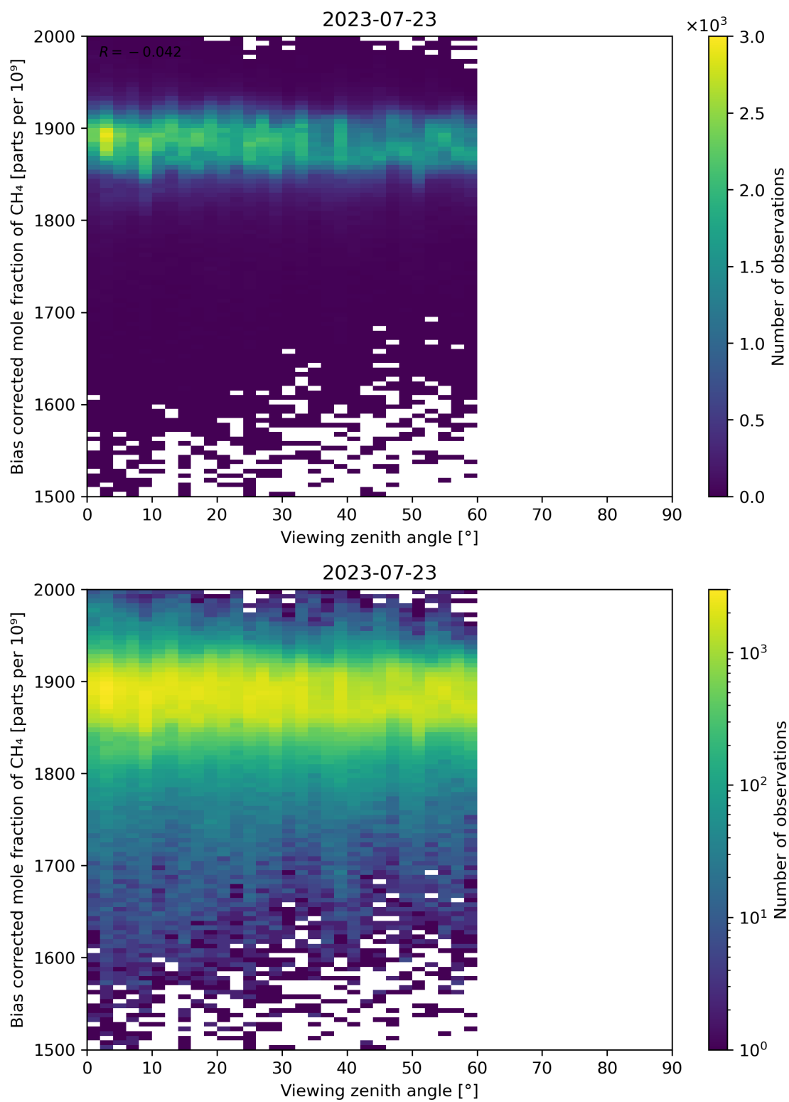
Figure 111: Scatter density plot of “Viewing zenith angle” against “Bias corrected mole fraction of CH 4 ” for 2023-07-22 to 2023-07-24.
