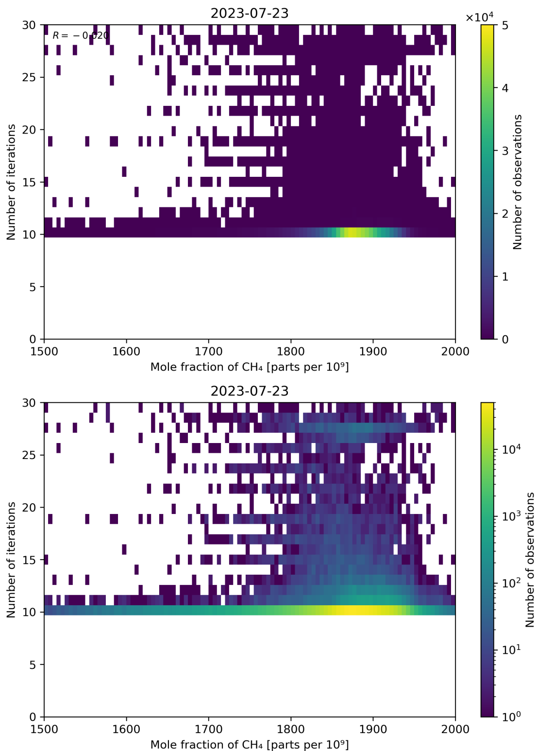
Figure 76: Scatter density plot of “Mole fraction of CH 4 ” against “Number of iterations” for 2023-07-22 to 2023-07-24.
