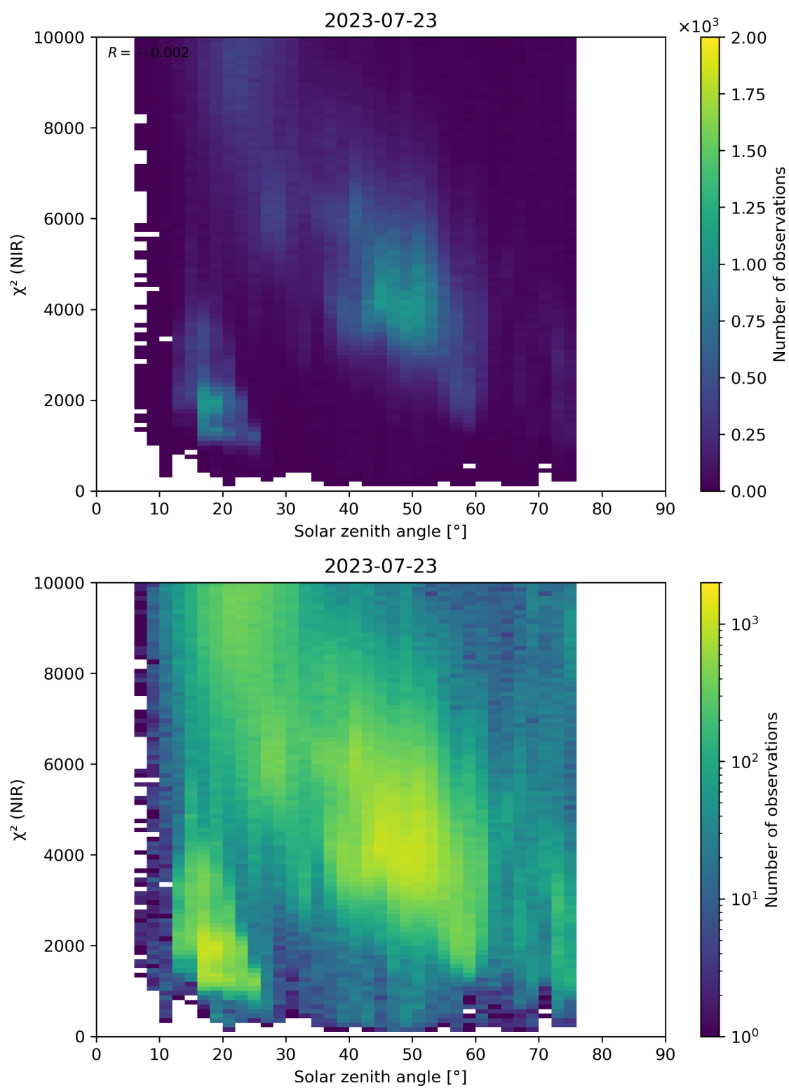
Figure 94: Scatter density plot of “Solar zenith angle” against “ \chi^2 (NIR)” for 2023-07-22 to 2023-07-24.
