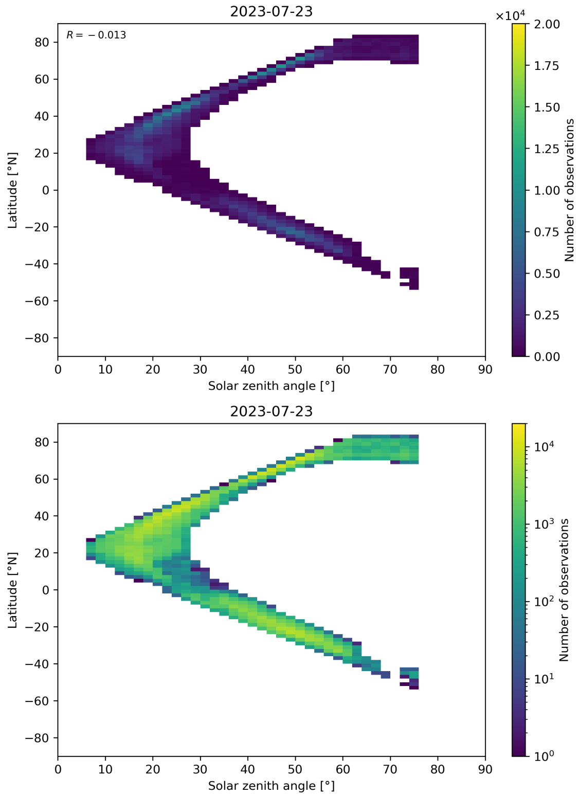
Figure 98: Scatter density plot of “Solar zenith angle” against “Latitude” for 2023-07-22 to 2023-07-24.
