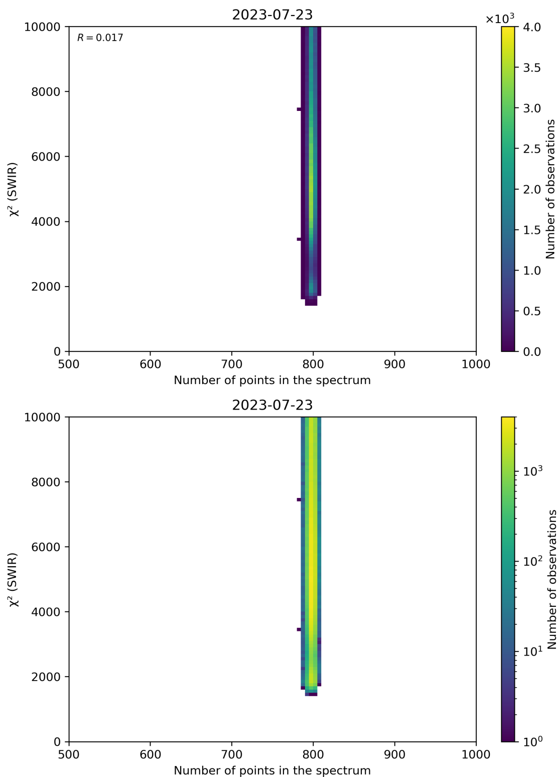
Figure 89: Scatter density plot of “Number of points in the spectrum” against “ \chi^2 (SWIR)” for 2023-07-22 to 2023-07-24.
