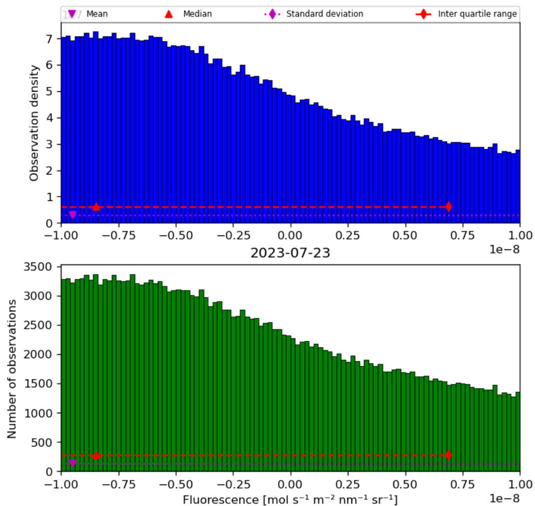
Figure 32: Histogram of “Fluorescence” for 2023-07-22 to 2023-07-24
