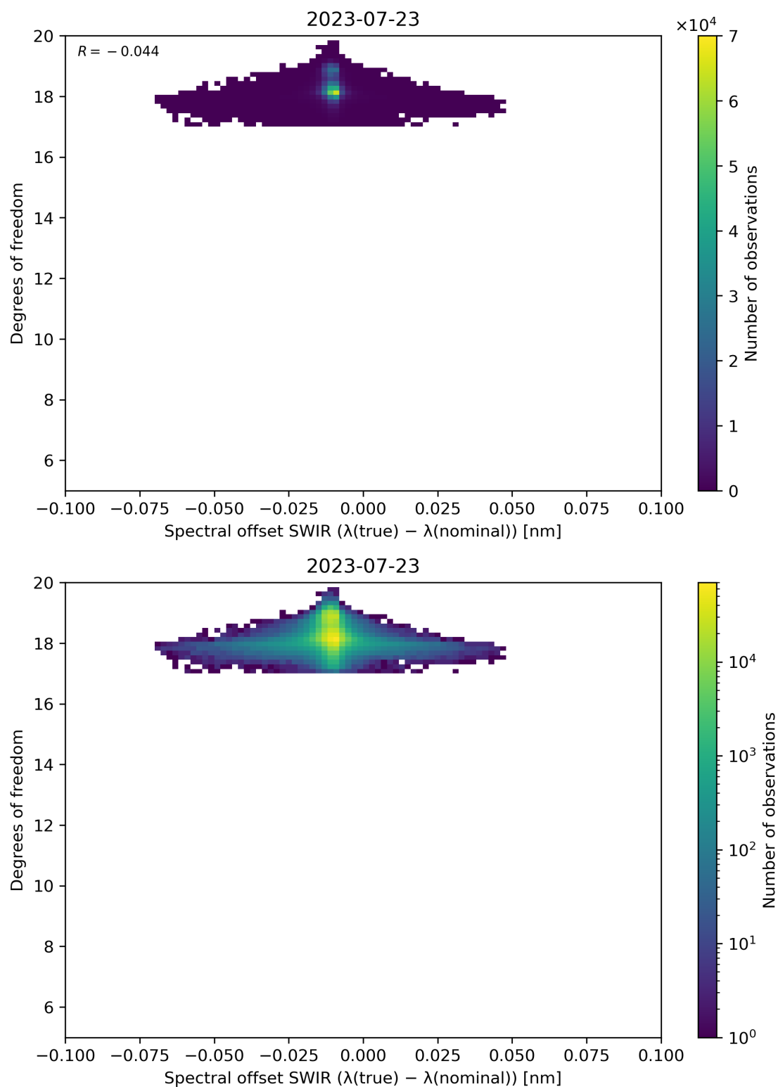
Figure 119: Scatter density plot of “Spectral offset SWIR ( \lambda(\text{true}) - \lambda(\text{nominal}) )” against “Degrees of freedom” for 2023-07-22 to 2023-07-24.
