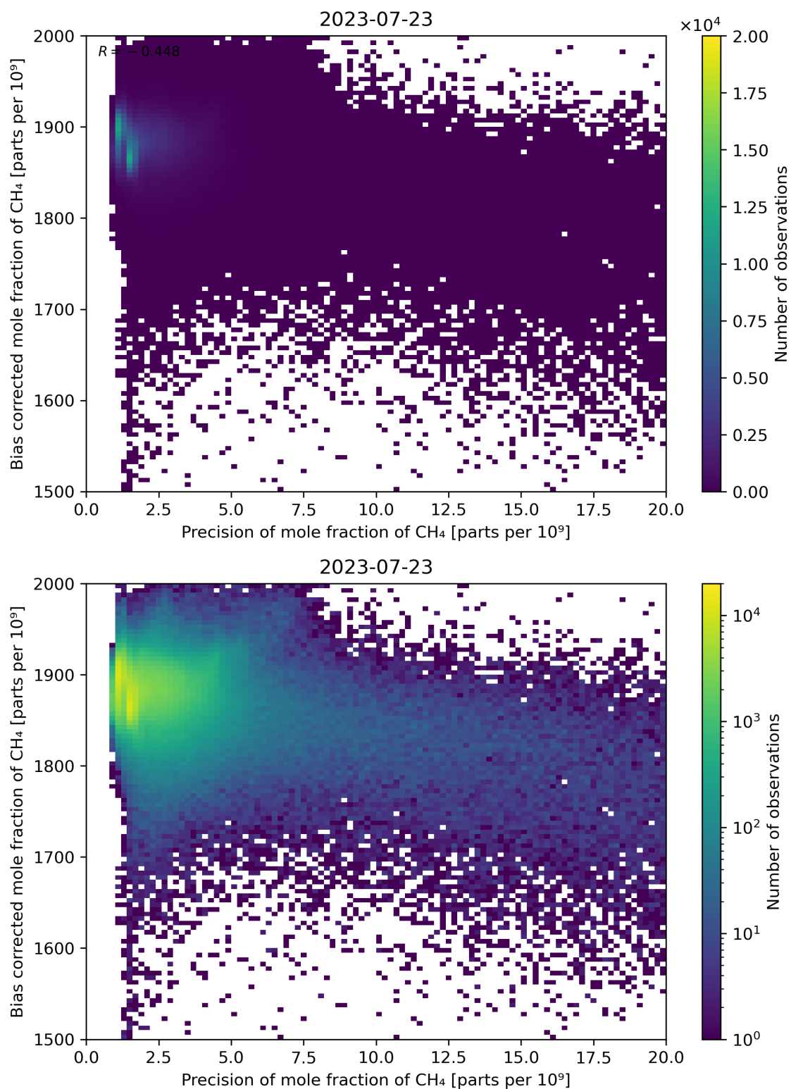
Figure 82: Scatter density plot of “Precision of mole fraction of CH 4 ” against “Bias corrected mole fraction of CH 4 ” for 2023-07-22 to 2023-07-24.
