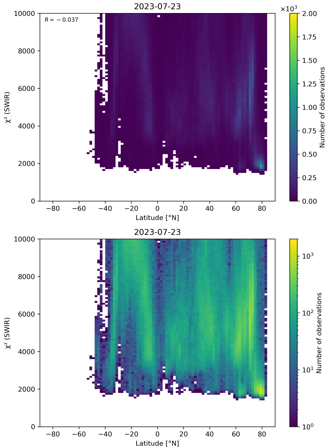
Figure 54: Scatter density plot of “Latitude” against “ \chi^2 (SWIR)” for 2023-07-22 to 2023-07-24.
