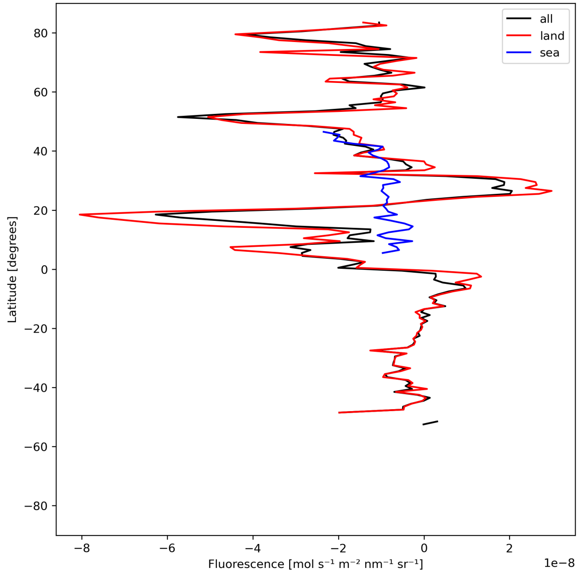
Figure 21: Zonal average of “Fluorescence” for 2023-07-22 to 2023-07-24.
