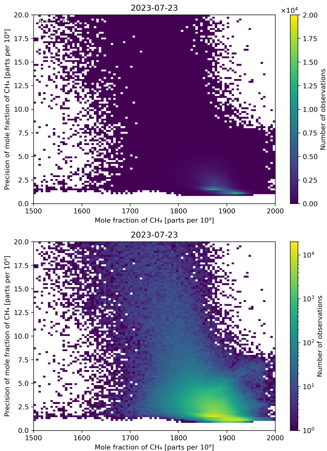
Figure 75: Scatter density plot of “Mole fraction of CH 4 ” against “Precision of mole fraction of CH 4 ” for 2023-07-22 to 2023-07-24.
