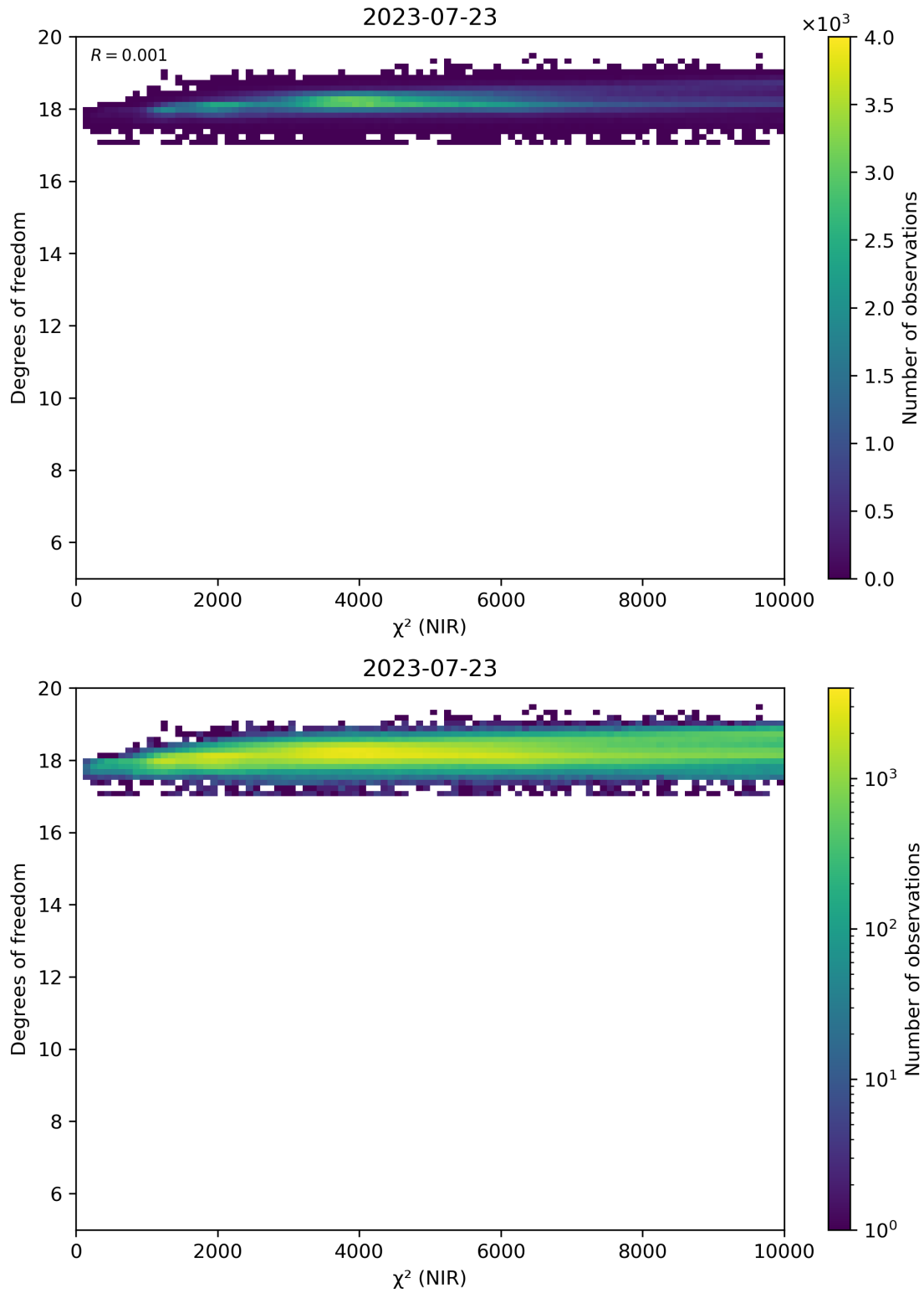
Figure 44: Scatter density plot of “ \chi^2 (NIR)” against “Degrees of freedom” for 2023-07-22 to 2023-07-24.
