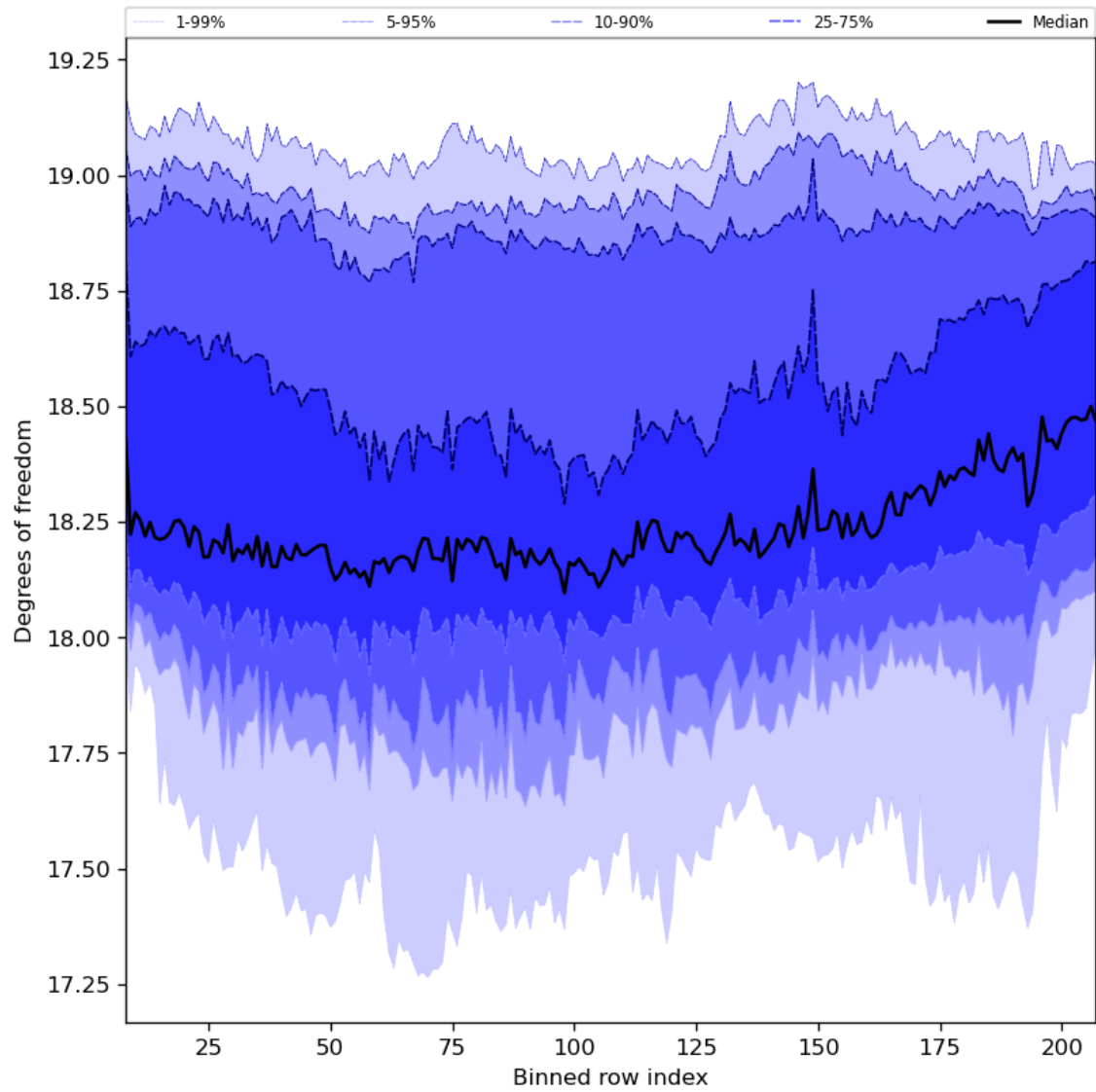
Figure 41: Along track statistics of “Degrees of freedom” for 2023-07-22 to 2023-07-24
