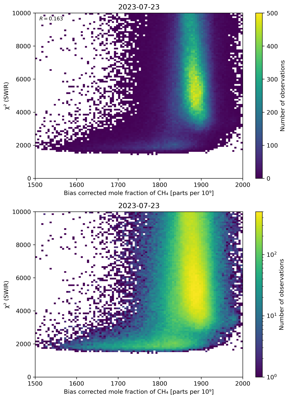
Figure 64: Scatter density plot of “Bias corrected mole fraction of CH 4 ” against “ \chi^2 (SWIR)” for 2023-07-22 to 2023-07-24.
