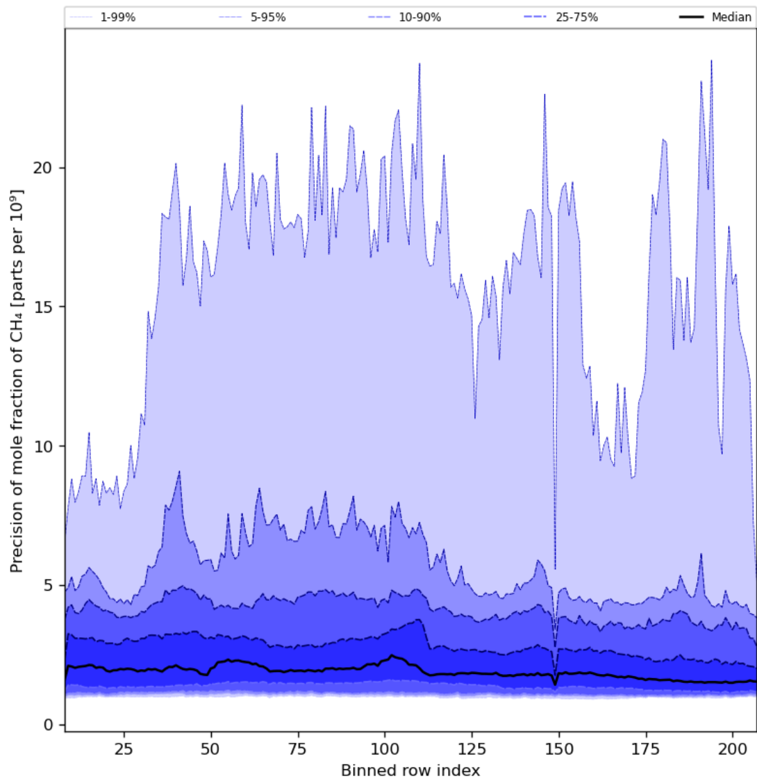
Figure 35: Along track statistics of “Precision of mole fraction of CH 4 ” for 2023-07-22 to 2023-07-24
