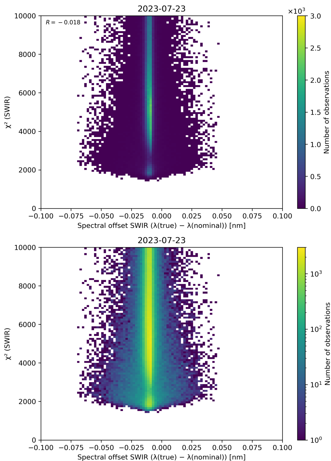
Figure 118: Scatter density plot of “Spectral offset SWIR ( \lambda(\text{true}) - \lambda(\text{nominal}) )” against “ \chi^2 (SWIR)” for 2023-07-22 to 2023-07-24.
