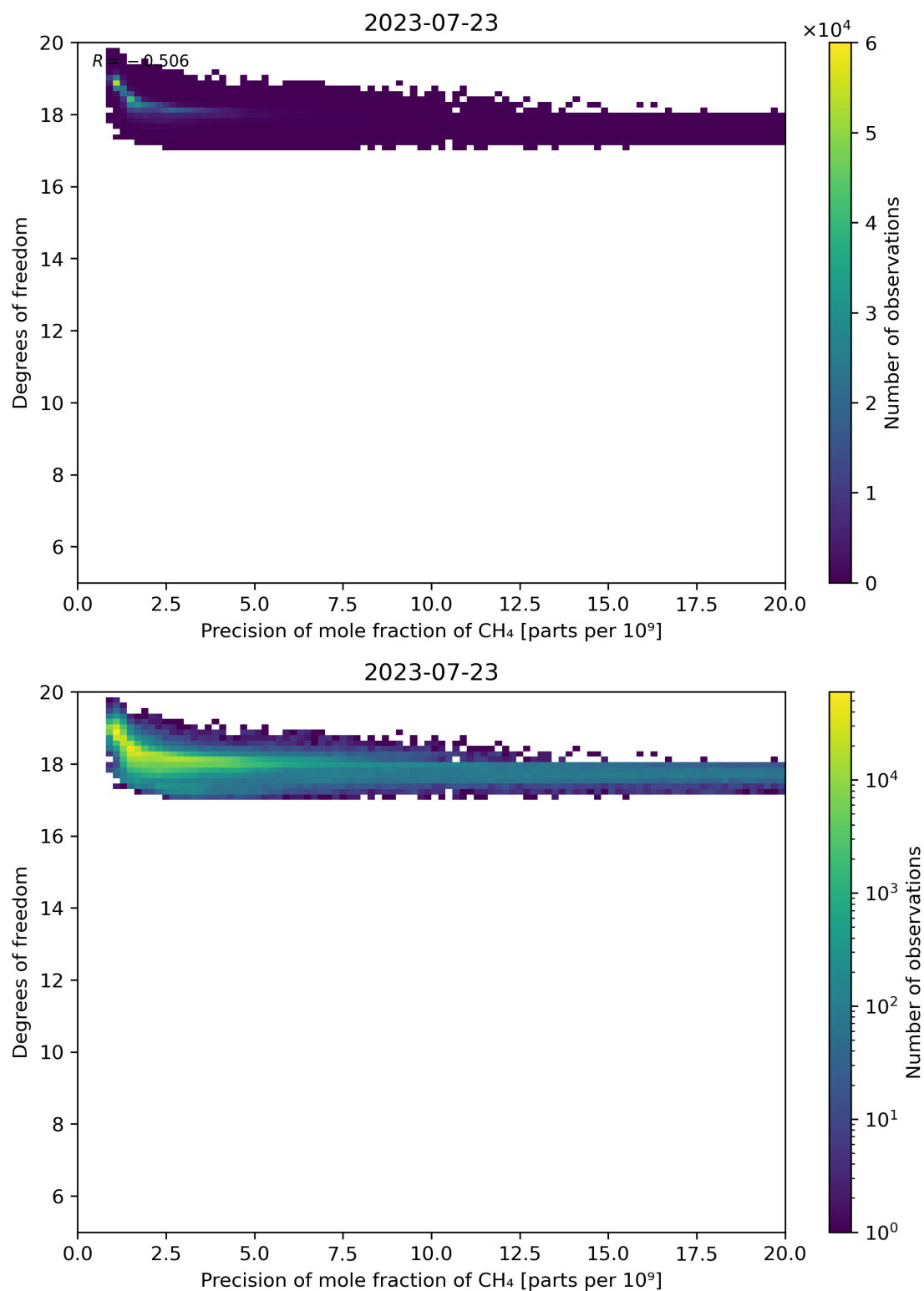
Figure 80: Scatter density plot of “Precision of mole fraction of CH 4 ” against “Degrees of freedom” for 2023-07-22 to 2023-07-24.
