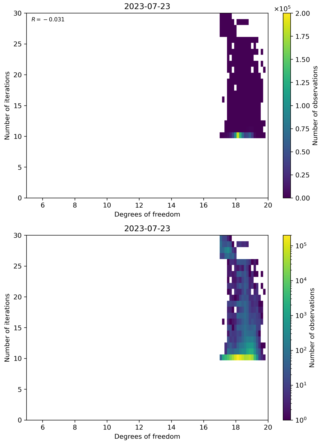
Figure 52: Scatter density plot of “Degrees of freedom” against “Number of iterations” for 2023-07-22 to 2023-07-24.
