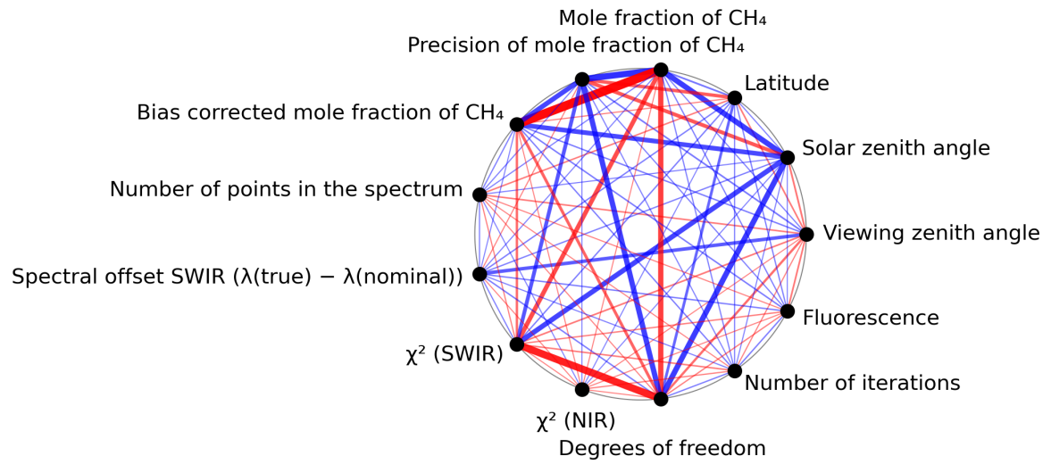
Figure 1: Map of correlation graph for 2023-07-22 to 2023-07-24.
