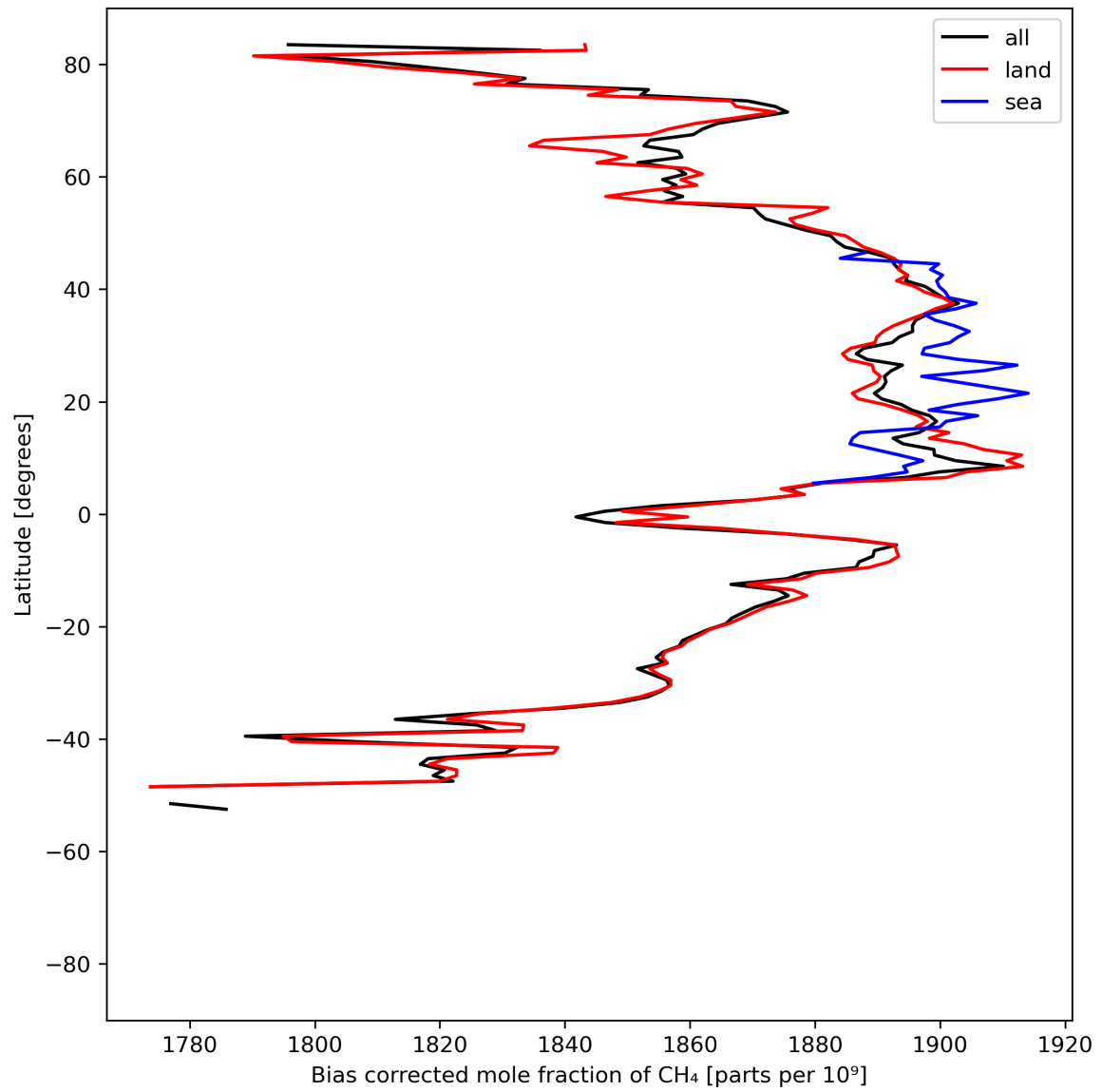
Figure 14: Zonal average of “Bias corrected mole fraction of CH 4 ” for 2023-07-22 to 2023-07-24.
