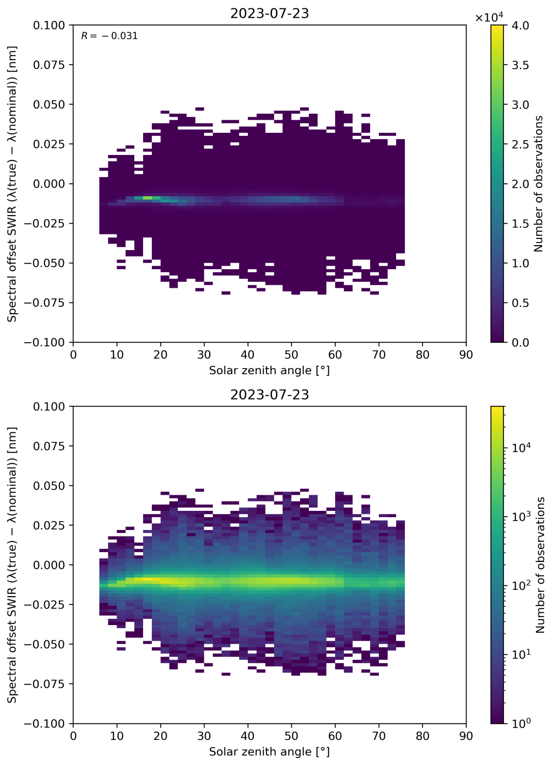
Figure 104: Scatter density plot of “Solar zenith angle” against “Spectral offset SWIR ( \lambda(\text{true}) - \lambda(\text{nominal}) )” for 2023-07-22 to 2023-07-24.
