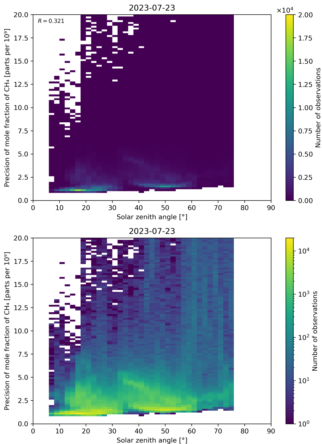
Figure 101: Scatter density plot of “Solar zenith angle” against “Precision of mole fraction of CH 4 ” for 2023-07-22 to 2023-07-24.
