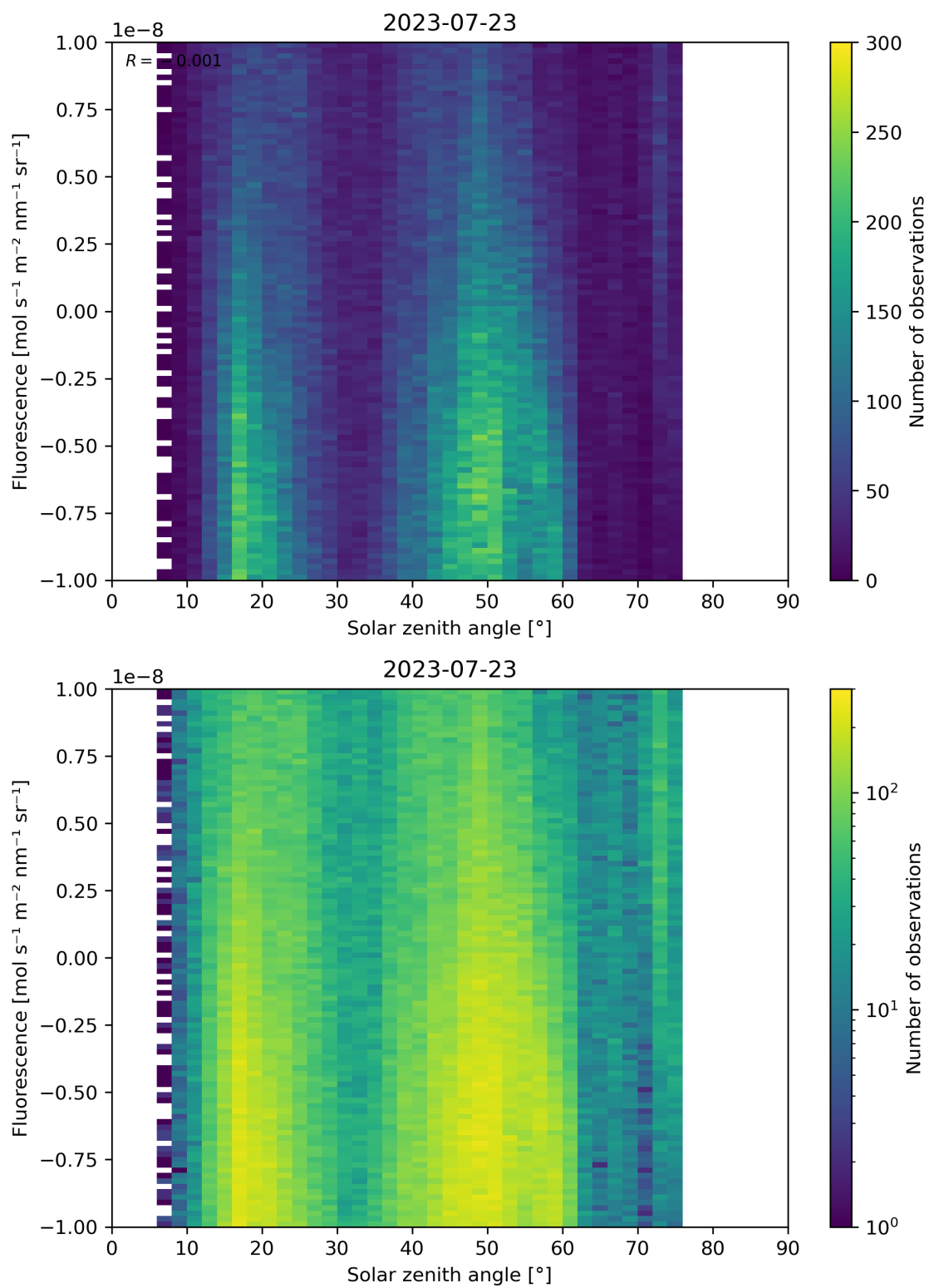
Figure 97: Scatter density plot of “Solar zenith angle” against “Fluorescence” for 2023-07-22 to 2023-07-24.
