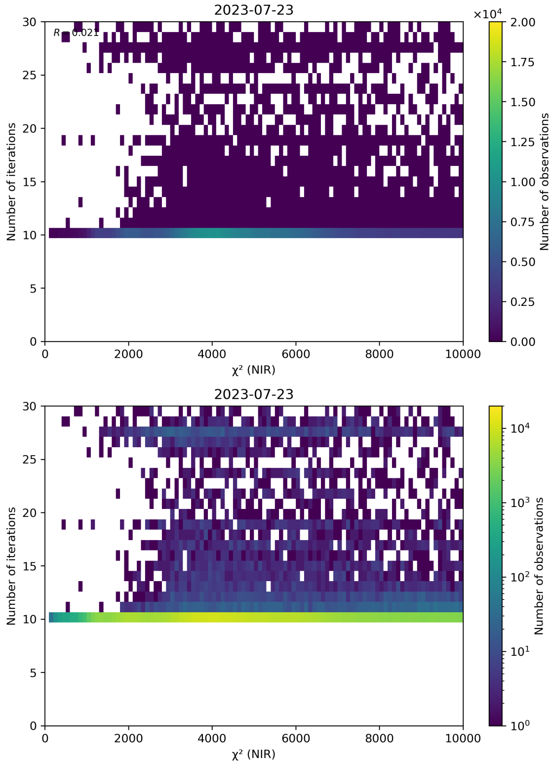
Figure 46: Scatter density plot of “ \chi^2 (NIR)” against “Number of iterations” for 2023-07-22 to 2023-07-24.
