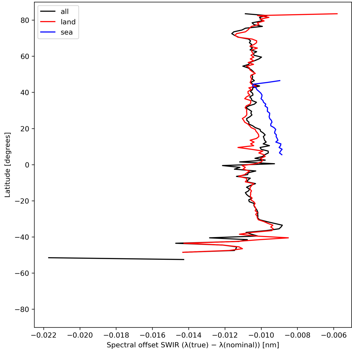
Figure 16: Zonal average of “Spectral offset SWIR ( \lambda(\text{true}) - \lambda(\text{nominal}) )” for 2023-07-22 to 2023-07-24.
