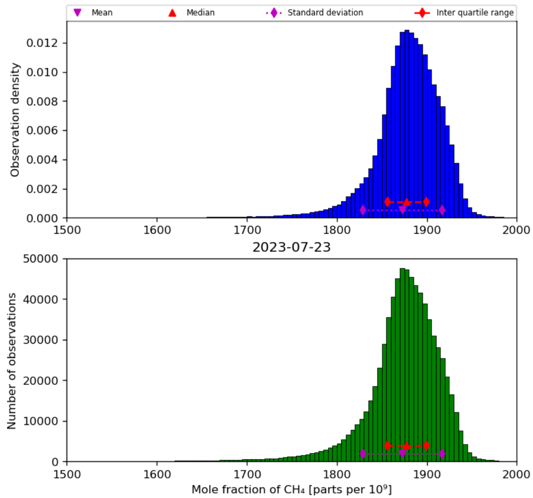
Figure 23: Histogram of “Mole fraction of CH 4 ” for 2023-07-22 to 2023-07-24
