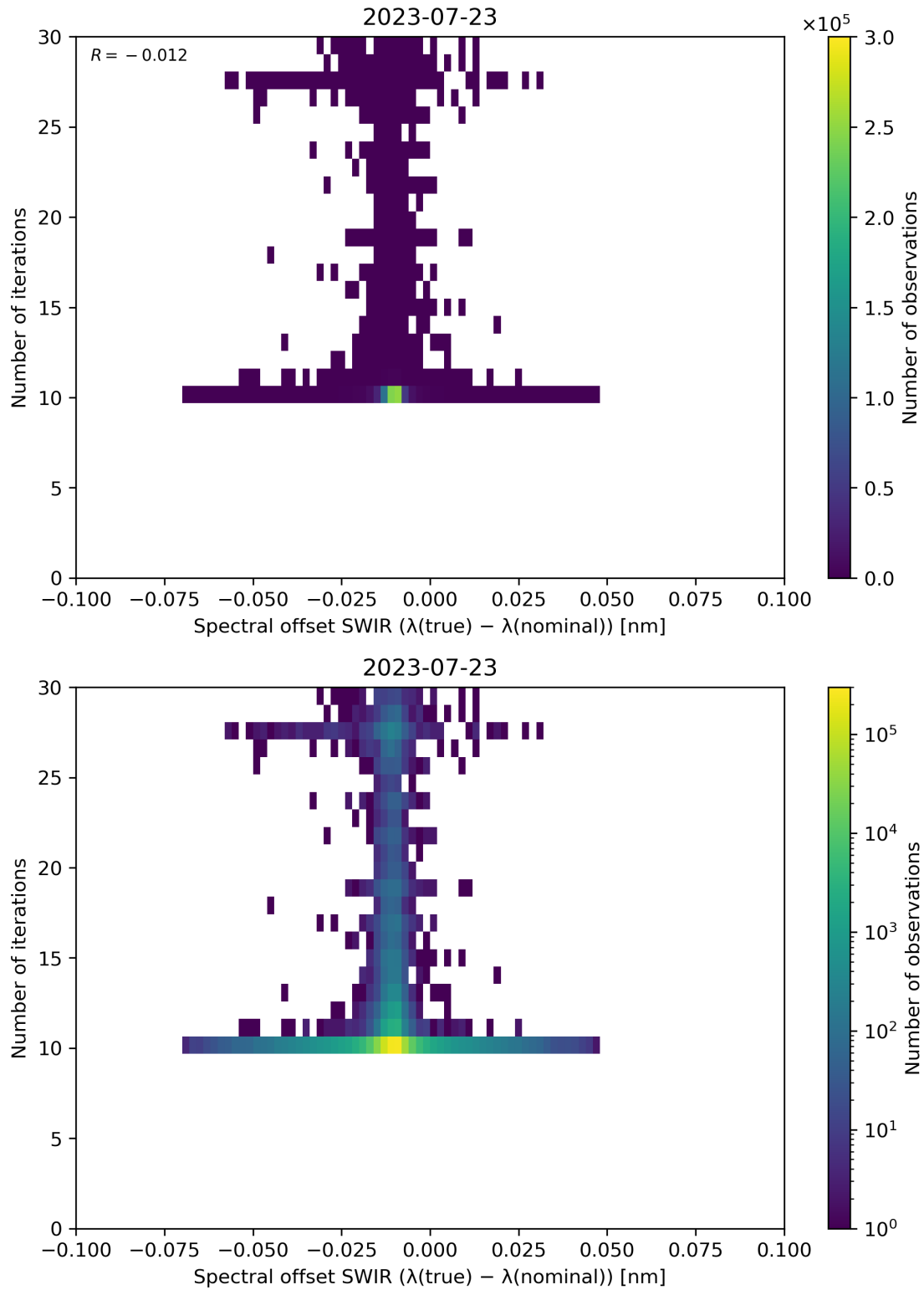
Figure 121: Scatter density plot of “Spectral offset SWIR ( \lambda(\text{true}) - \lambda(\text{nominal}) )” against “Number of iterations” for 2023-07-22 to 2023-07-24.
