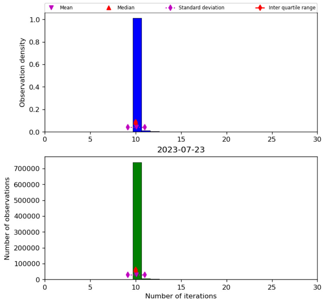
Figure 31: Histogram of “Number of iterations” for 2023-07-22 to 2023-07-24
