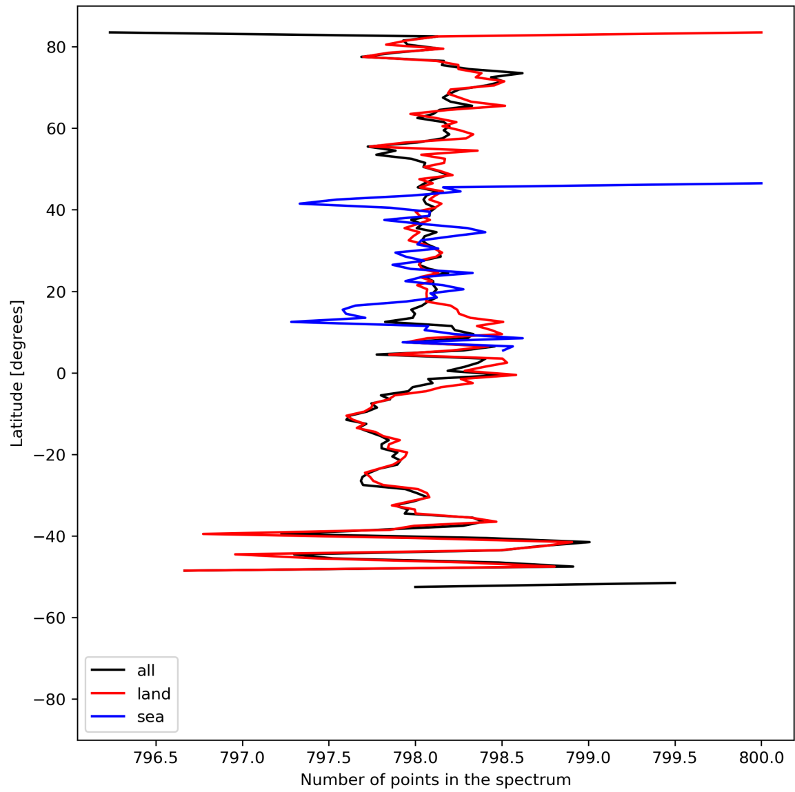
Figure 15: Zonal average of “Number of points in the spectrum” for 2023-07-22 to 2023-07-24.
