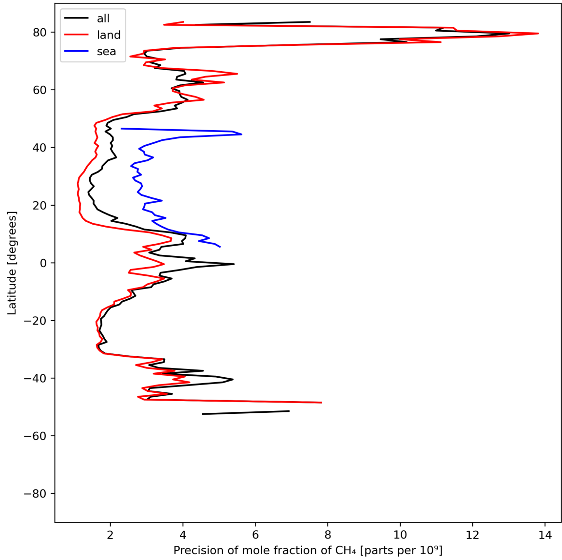
Figure 13: Zonal average of “Precision of mole fraction of CH 4 ” for 2023-07-22 to 2023-07-24.
