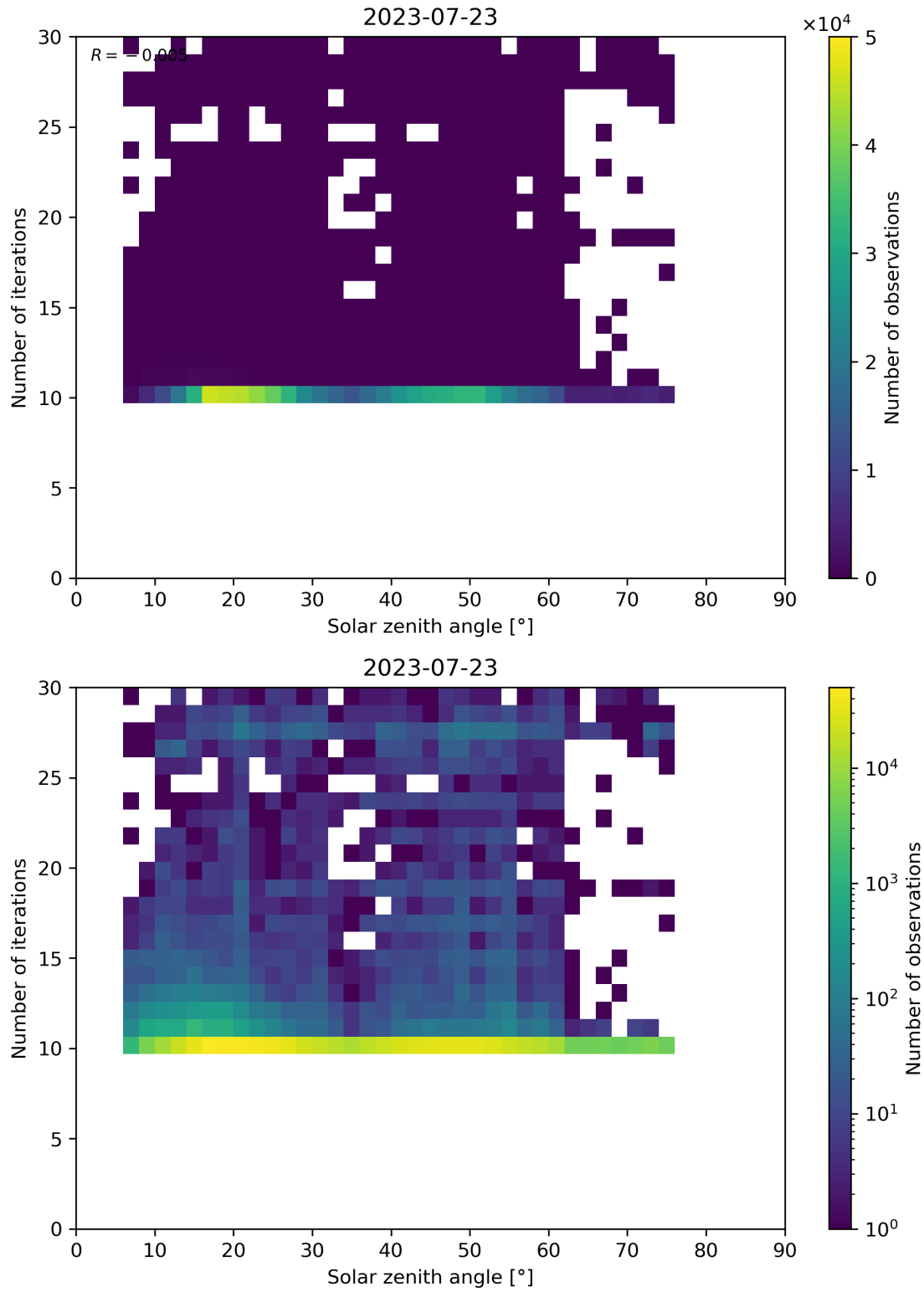
Figure 102: Scatter density plot of “Solar zenith angle” against “Number of iterations” for 2023-07-22 to 2023-07-24.
