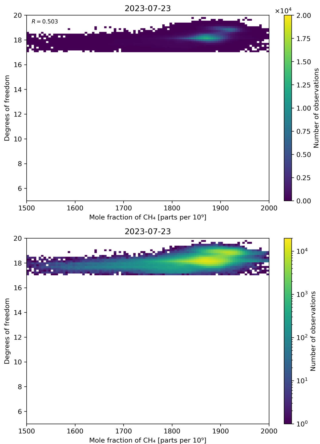
Figure 72: Scatter density plot of “Mole fraction of CH 4 ” against “Degrees of freedom” for 2023-07-22 to 2023-07-24.
