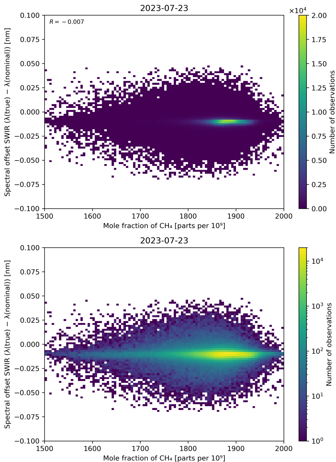
Figure 86: Scatter density plot of “Mole fraction of CH 4 ” against “Spectral offset SWIR ( \lambda(\text{true}) - \lambda(\text{nominal}) )” for 2023-07-22 to 2023-07-24.
