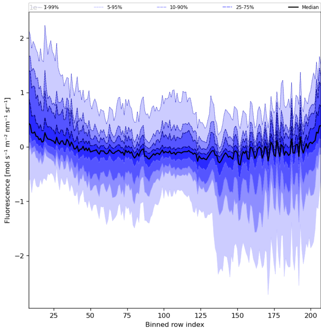
Figure 43: Along track statistics of “Fluorescence” for 2023-07-22 to 2023-07-24
