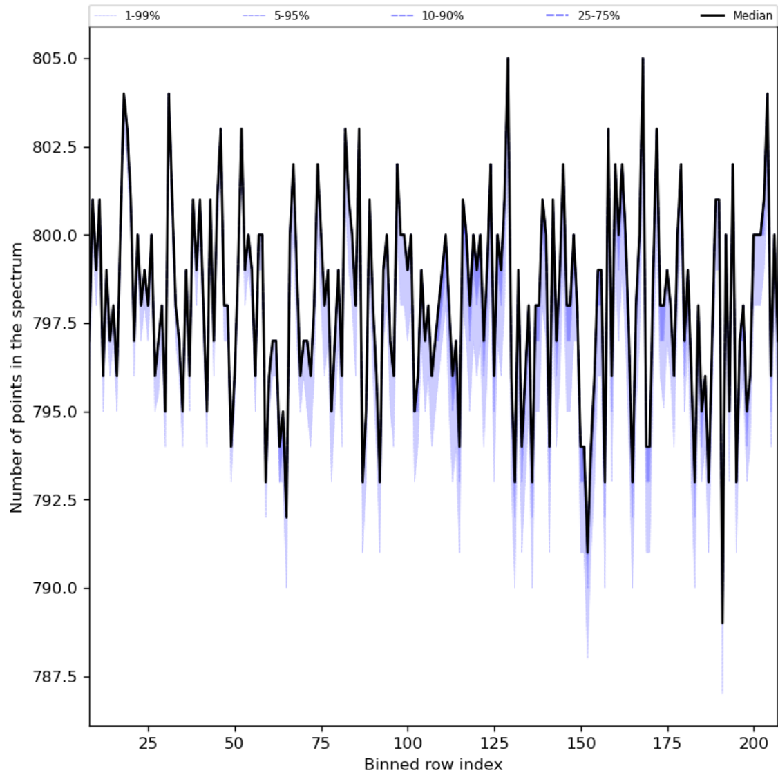
Figure 37: Along track statistics of “Number of points in the spectrum” for 2023-07-22 to 2023-07-24
