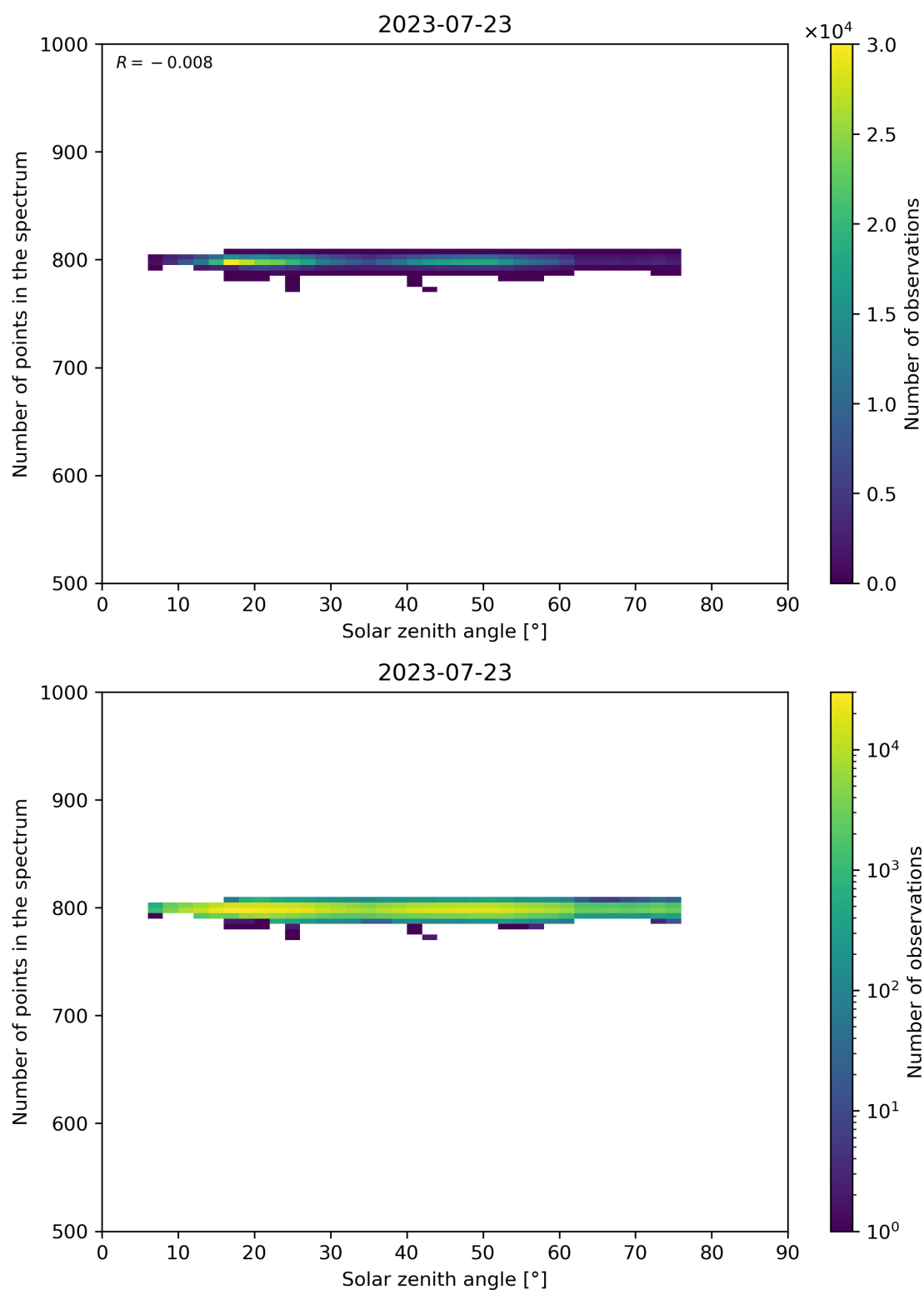
Figure 103: Scatter density plot of “Solar zenith angle” against “Number of points in the spectrum” for 2023-07-22 to 2023-07-24.
