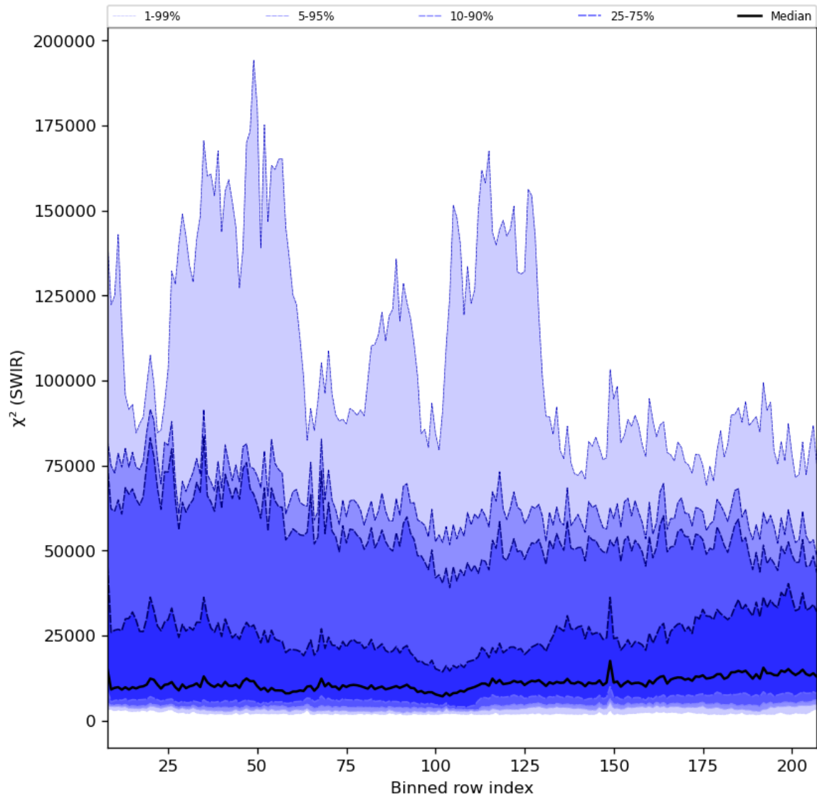
Figure 39: Along track statistics of “ \chi^2 (SWIR)” for 2023-07-22 to 2023-07-24
