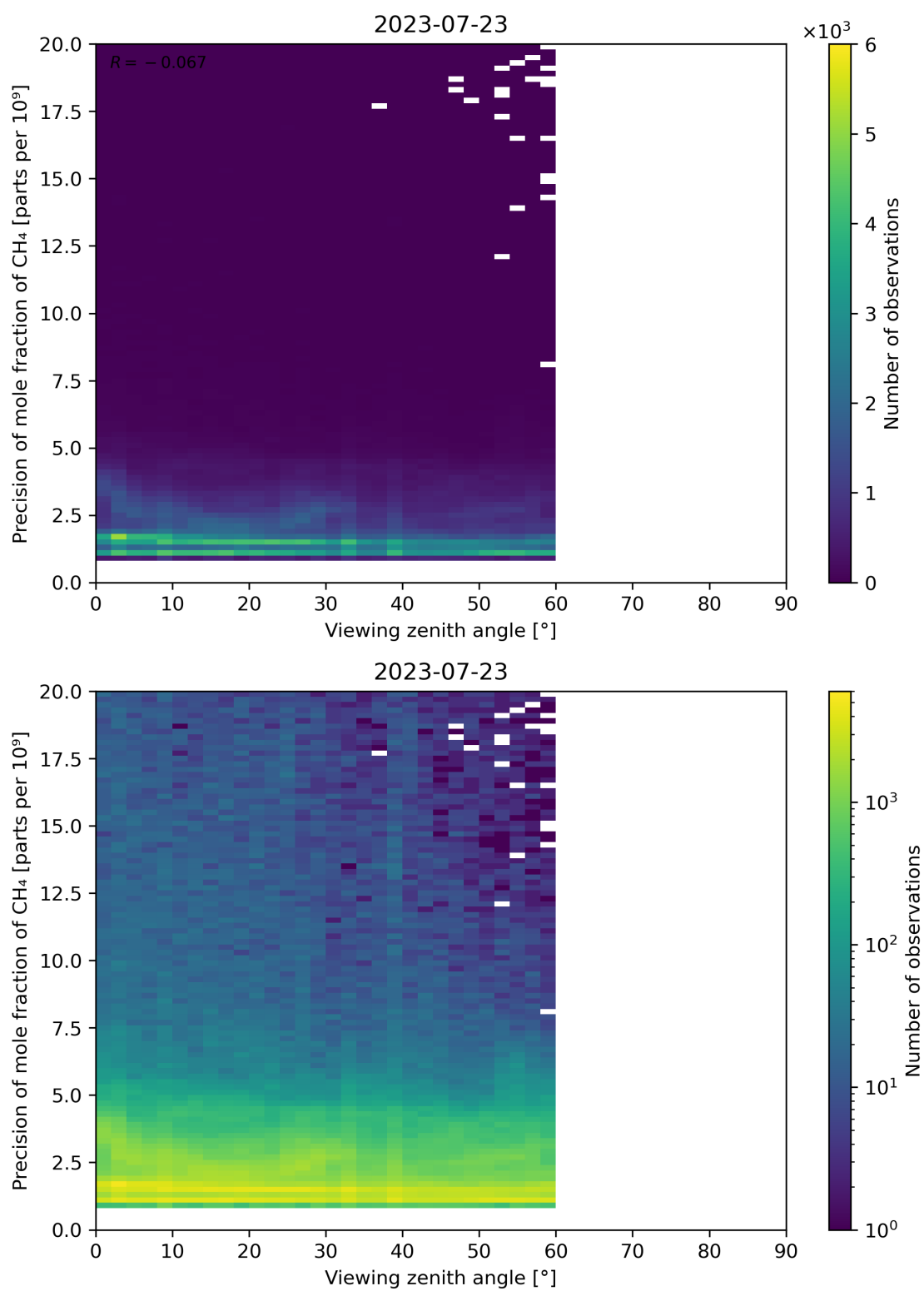
Figure 112: Scatter density plot of “Viewing zenith angle” against “Precision of mole fraction of CH 4 ” for 2023-07-22 to 2023-07-24.
