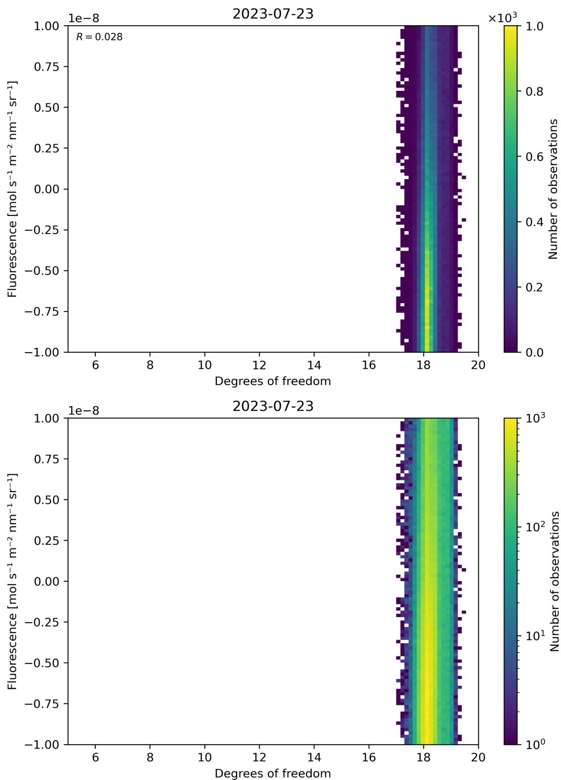
Figure 51: Scatter density plot of “Degrees of freedom” against “Fluorescence” for 2023-07-22 to 2023-07-24.
