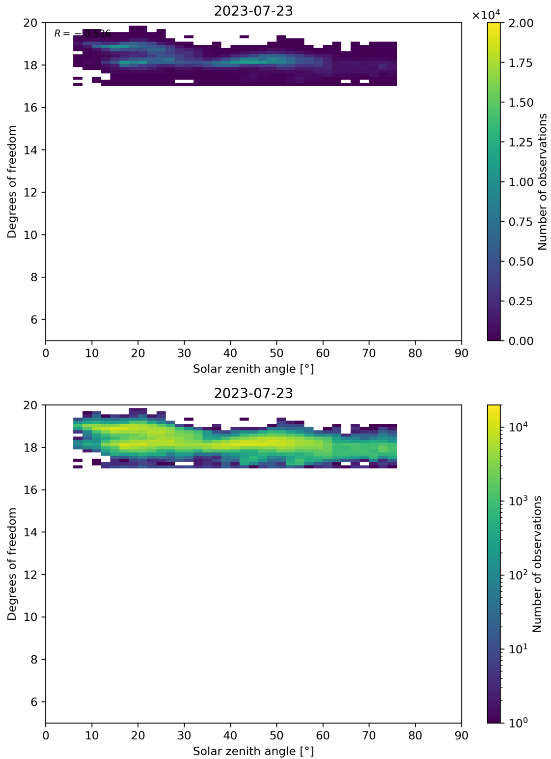
Figure 96: Scatter density plot of “Solar zenith angle” against “Degrees of freedom” for 2023-07-22 to 2023-07-24.
