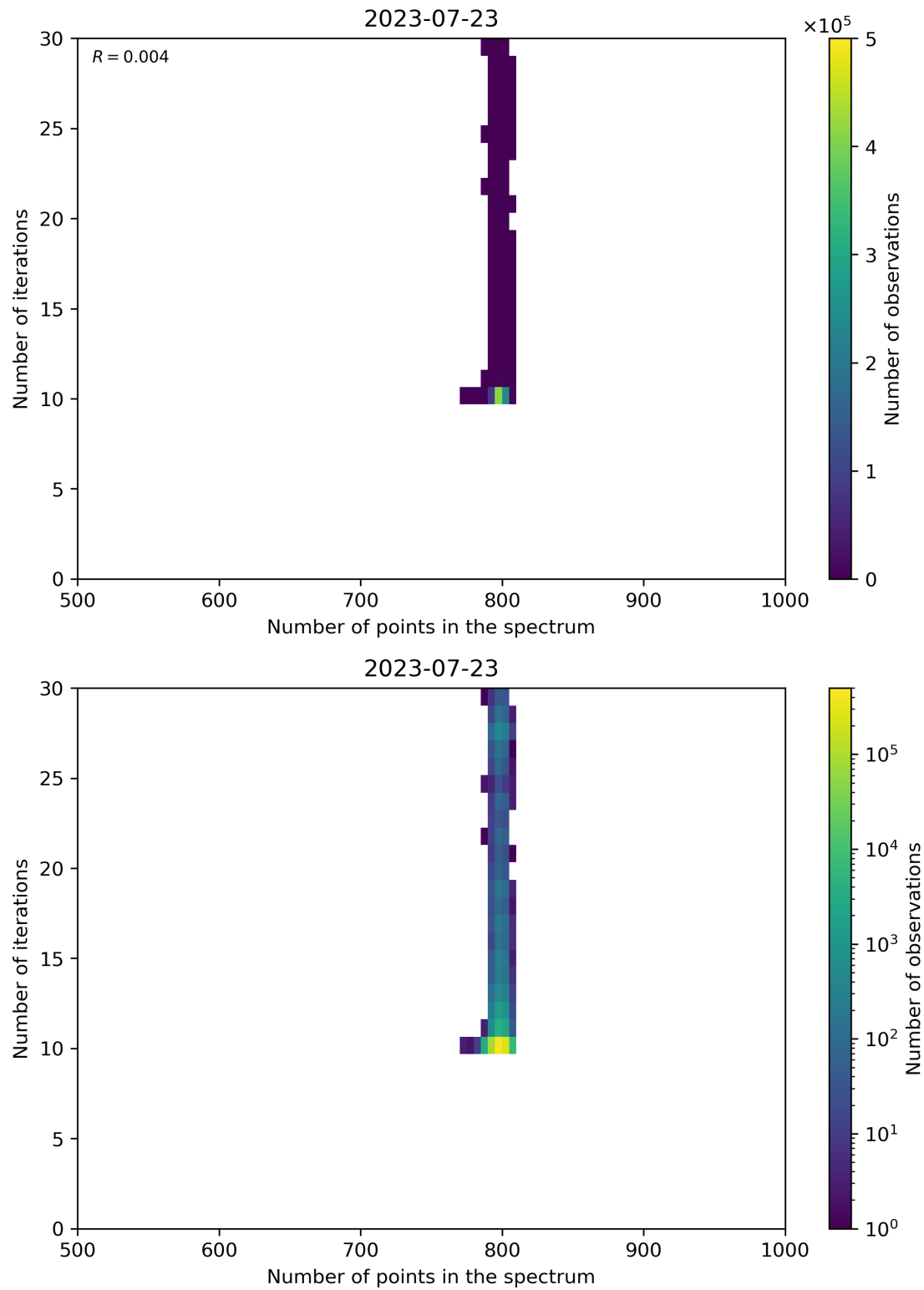
Figure 92: Scatter density plot of “Number of points in the spectrum” against “Number of iterations” for 2023-07-22 to 2023-07-24.
