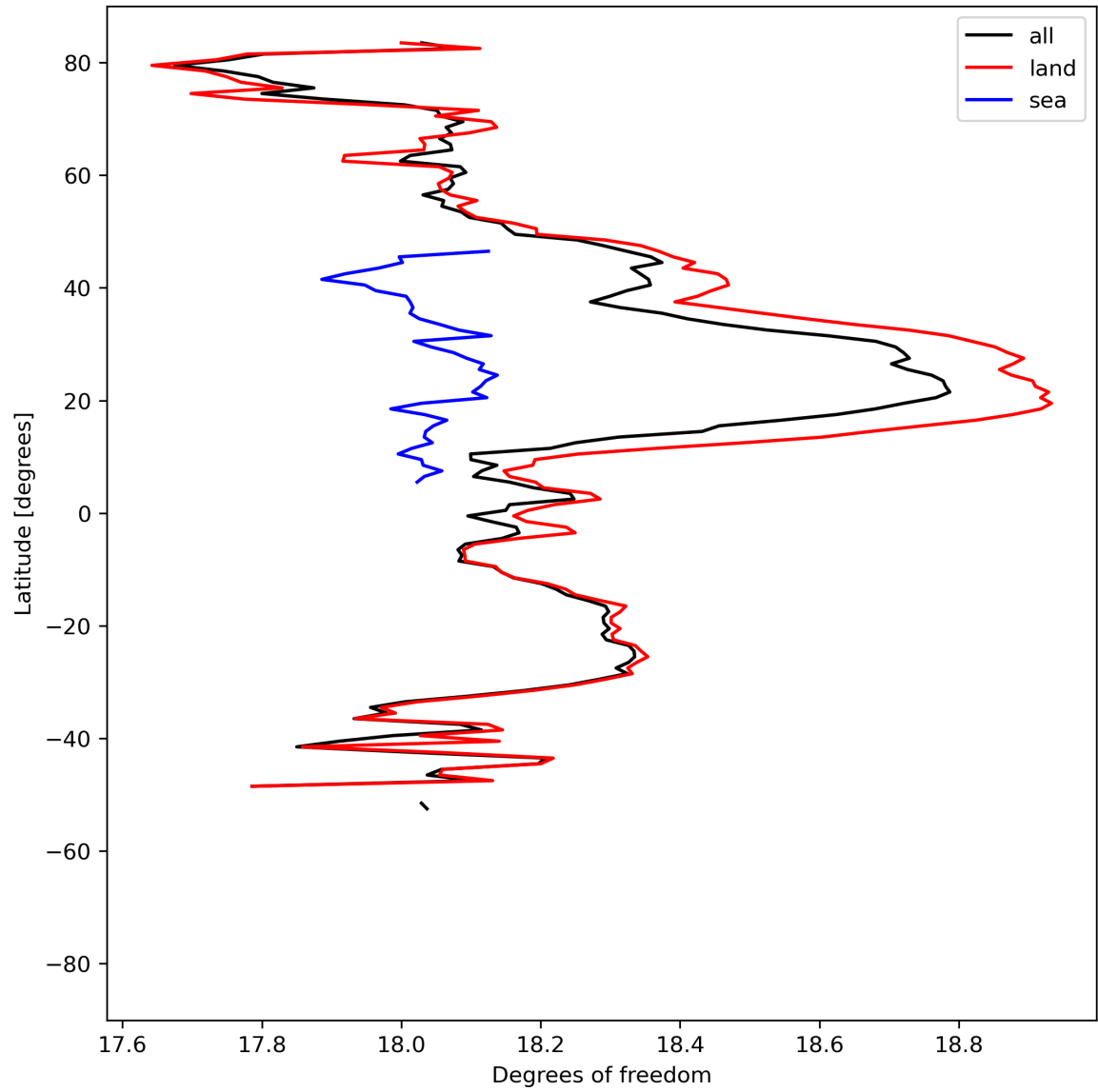
Figure 19: Zonal average of “Degrees of freedom” for 2023-07-22 to 2023-07-24.
