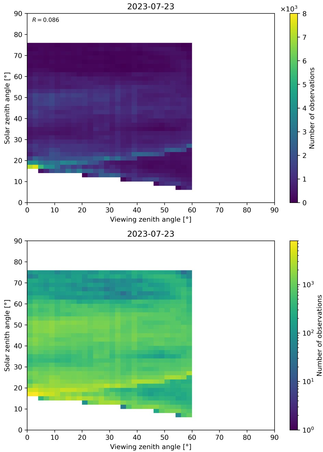
Figure 115: Scatter density plot of “Viewing zenith angle” against “Solar zenith angle” for 2023-07-22 to 2023-07-24.
