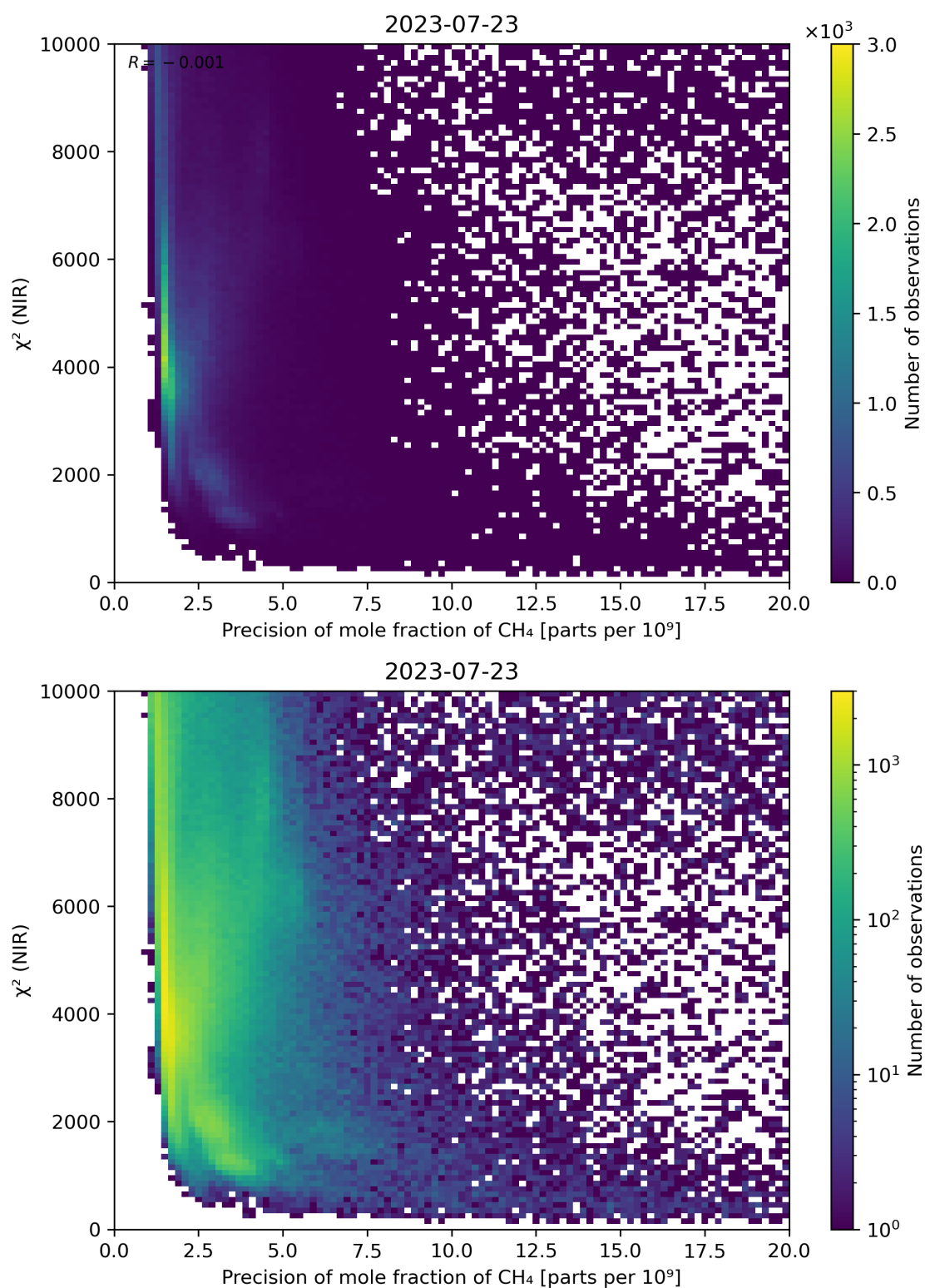
Figure 78: Scatter density plot of “Precision of mole fraction of CH 4 ” against “ \chi^2 (NIR)” for 2023-07-22 to 2023-07-24.
