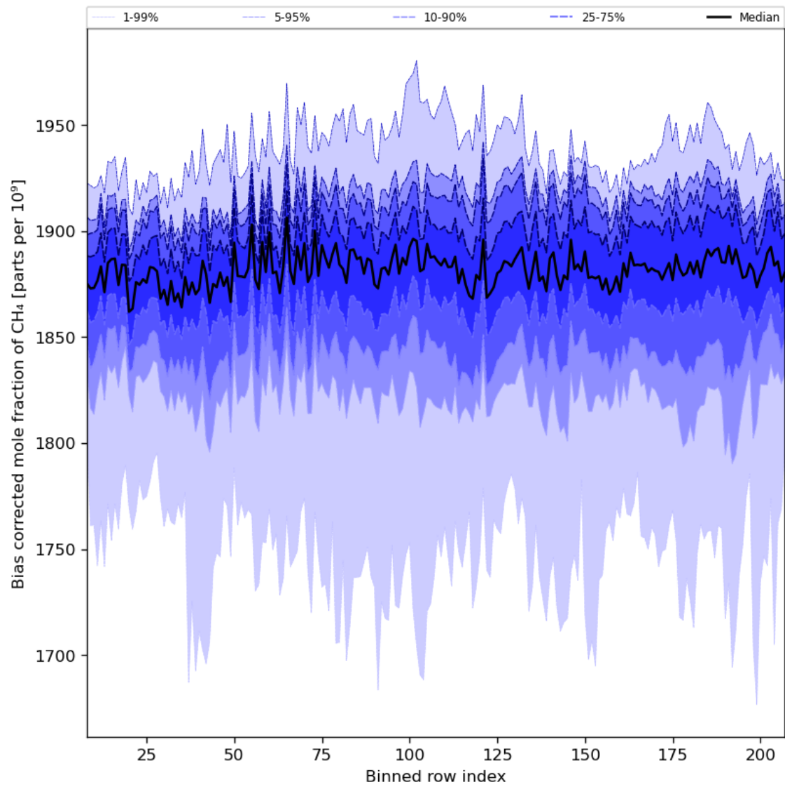
Figure 36: Along track statistics of “Bias corrected mole fraction of CH 4 ” for 2023-07-22 to 2023-07-24
