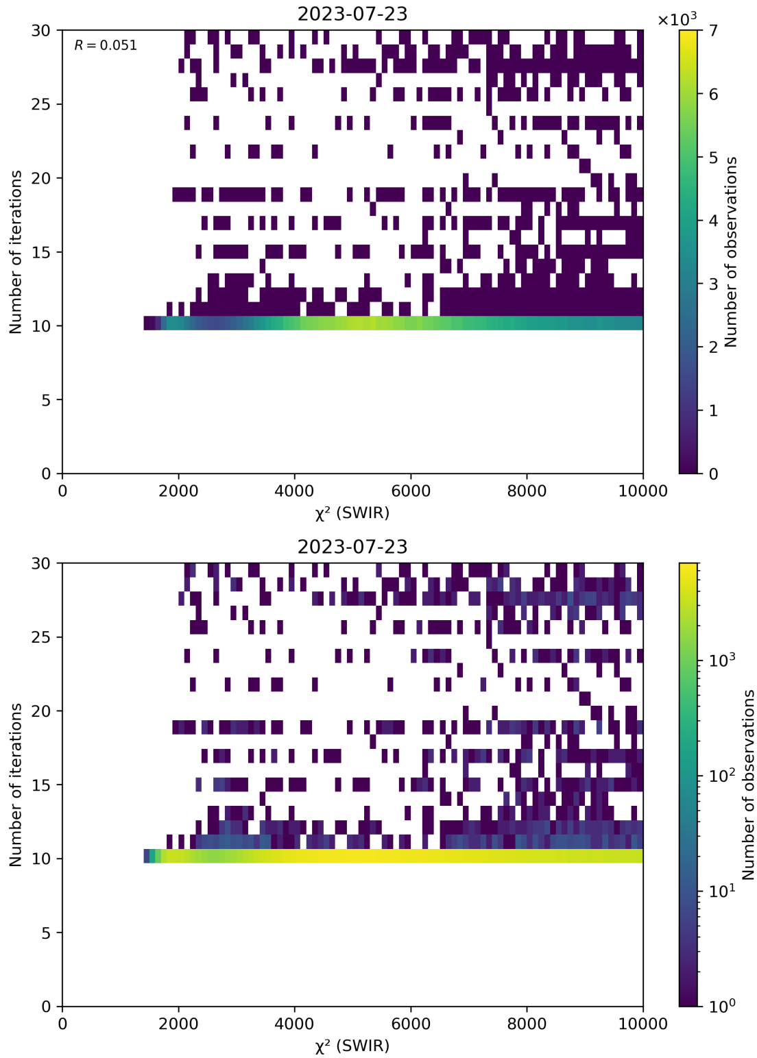
Figure 50: Scatter density plot of “ \chi^2 (SWIR)” against “Number of iterations” for 2023-07-22 to 2023-07-24.
