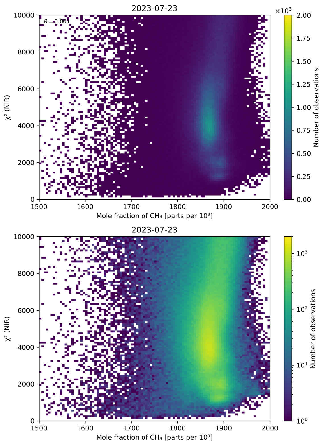
Figure 70: Scatter density plot of “Mole fraction of CH 4 ” against “ \chi^2 (NIR)” for 2023-07-22 to 2023-07-24.
