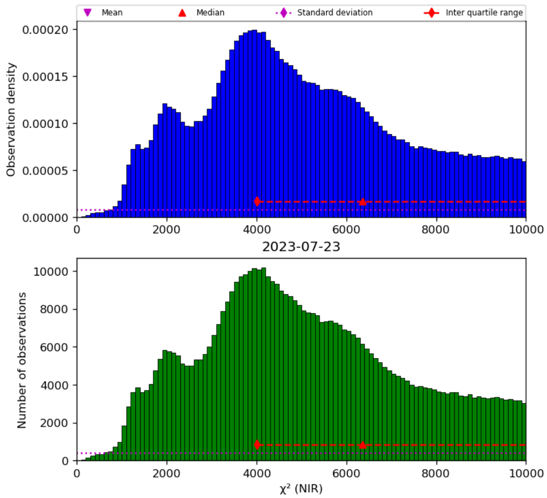
Figure 29: Histogram of “ \chi^2 (NIR)” for 2023-07-22 to 2023-07-24
