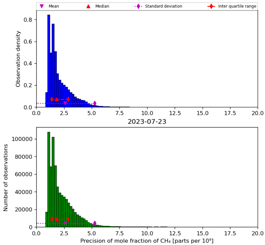
Figure 24: Histogram of “Precision of mole fraction of CH 4 ” for 2023-07-22 to 2023-07-24
