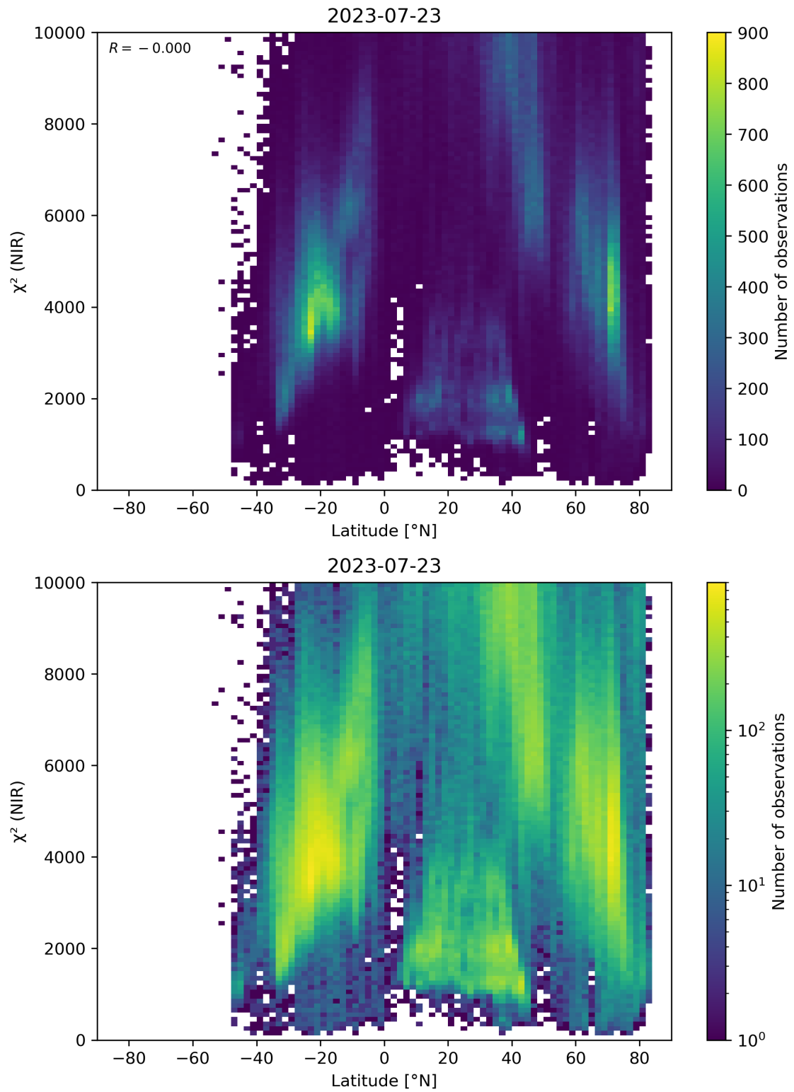
Figure 53: Scatter density plot of “Latitude” against “ \chi^2 (NIR)” for 2023-07-22 to 2023-07-24.
