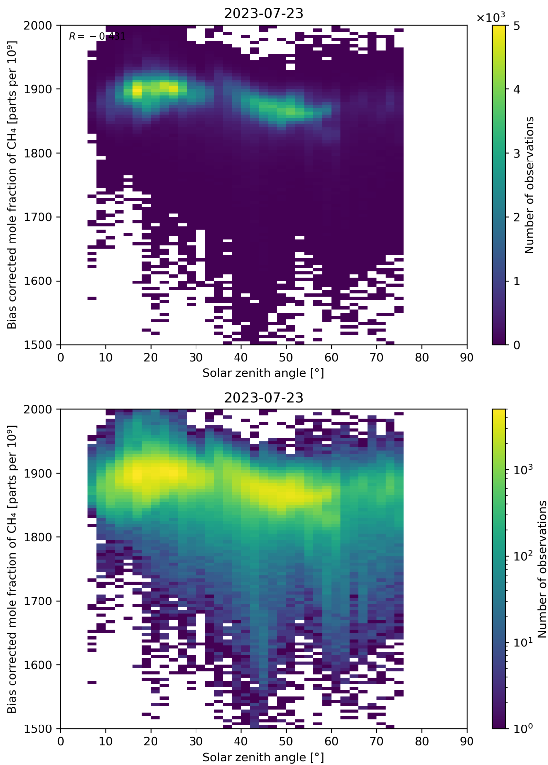
Figure 100: Scatter density plot of “Solar zenith angle” against “Bias corrected mole fraction of CH 4 ” for 2023-07-22 to 2023-07-24.
