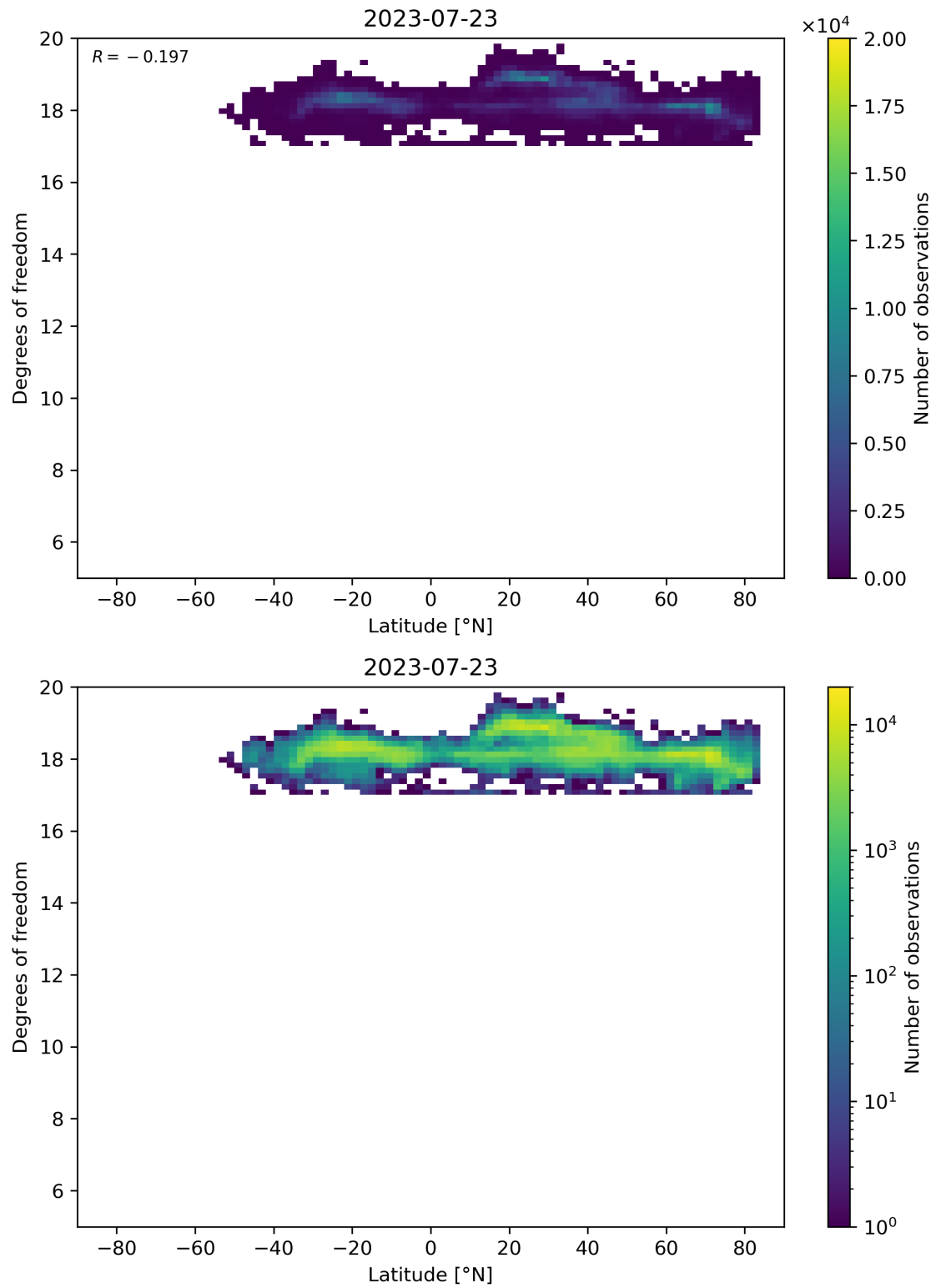
Figure 55: Scatter density plot of “Latitude” against “Degrees of freedom” for 2023-07-22 to 2023-07-24.
