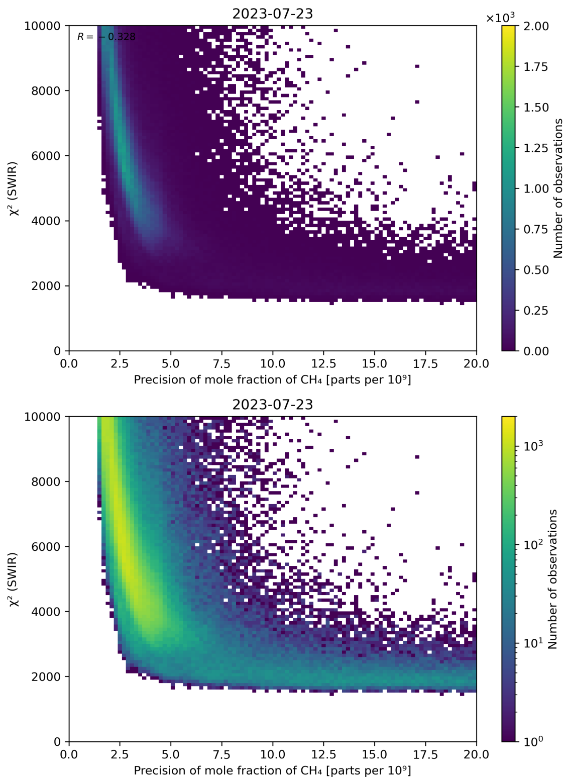
Figure 79: Scatter density plot of “Precision of mole fraction of \text{CH}_4 ” against “ \chi^2 (SWIR)” for 2023-07-22 to 2023-07-24.
