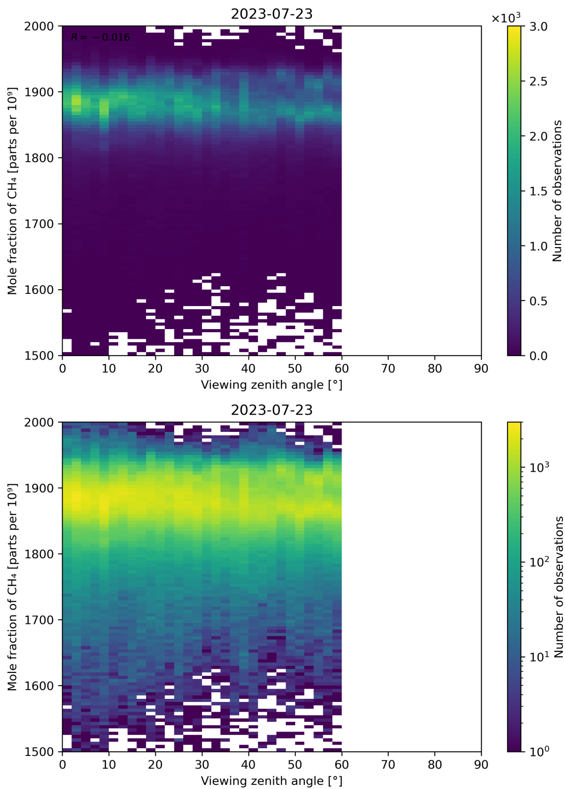
Figure 110: Scatter density plot of “Viewing zenith angle” against “Mole fraction of \text{CH}_4 ” for 2023-07-22 to 2023-07-24.
