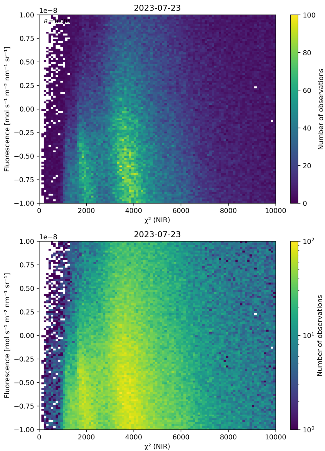
Figure 45: Scatter density plot of “ \chi^2 (NIR)” against “Fluorescence” for 2023-07-22 to 2023-07-24.
