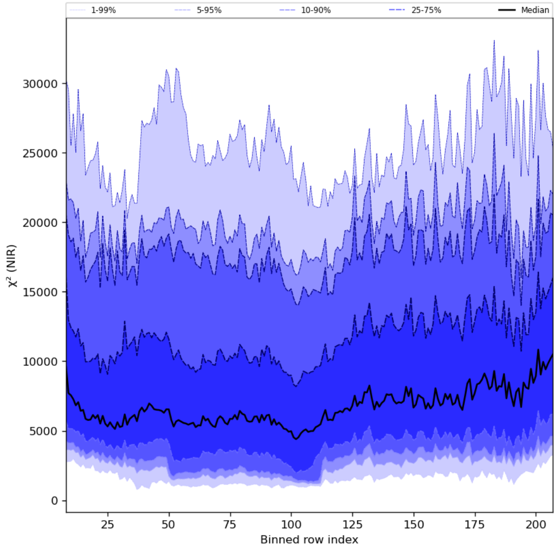
Figure 40: Along track statistics of “ \chi^2 (NIR)” for 2023-07-22 to 2023-07-24
