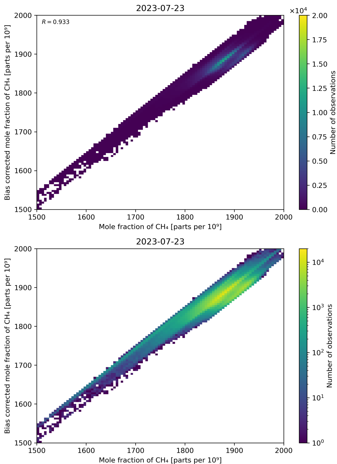
Figure 74: Scatter density plot of “Mole fraction of CH 4 ” against “Bias corrected mole fraction of CH 4 ” for 2023-07-22 to 2023-07-24.
