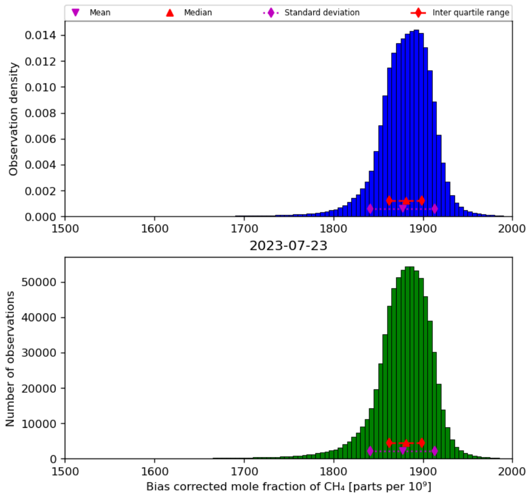
Figure 25: Histogram of “Bias corrected mole fraction of CH 4 ” for 2023-07-22 to 2023-07-24
