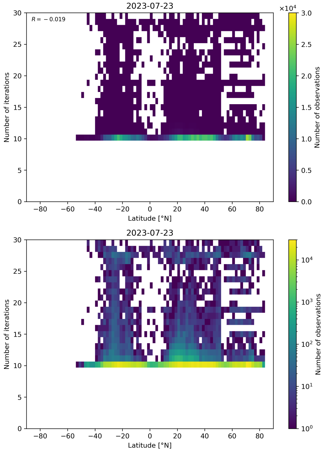
Figure 60: Scatter density plot of “Latitude” against “Number of iterations” for 2023-07-22 to 2023-07-24.
