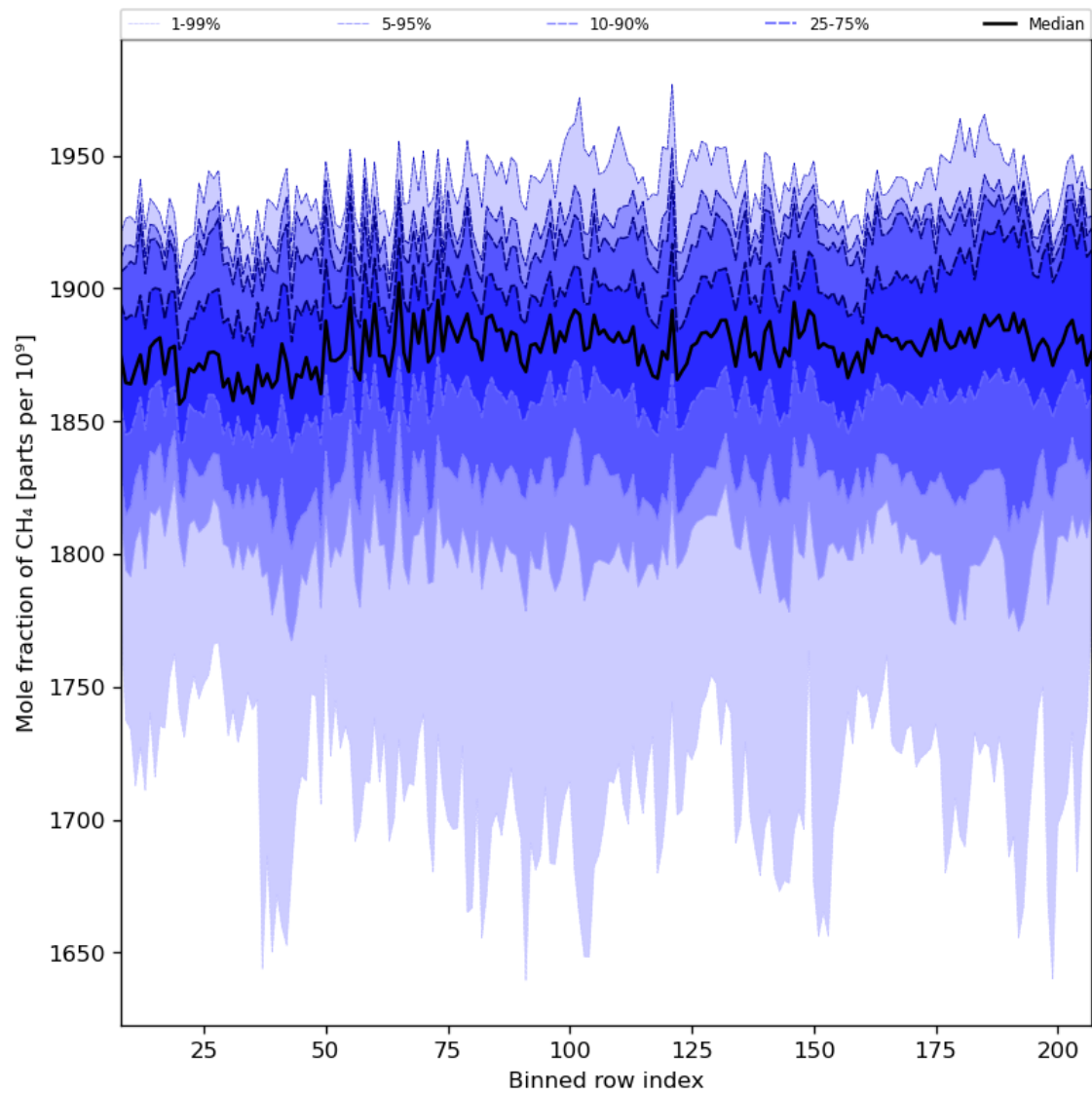
Figure 34: Along track statistics of “Mole fraction of CH 4 ” for 2023-07-22 to 2023-07-24
