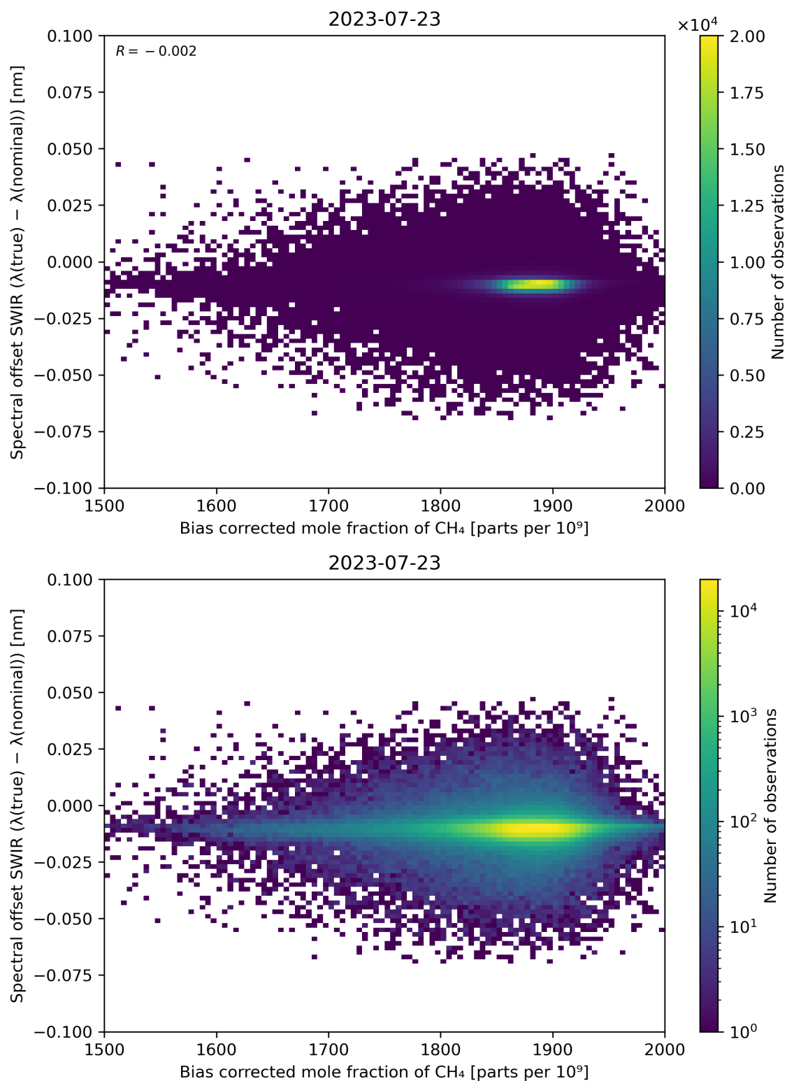
Figure 69: Scatter density plot of “Bias corrected mole fraction of \text{CH}_4 ” against “Spectral offset SWIR ( \lambda(\text{true}) - \lambda(\text{nominal}) )” for 2023-07-22 to 2023-07-24.
