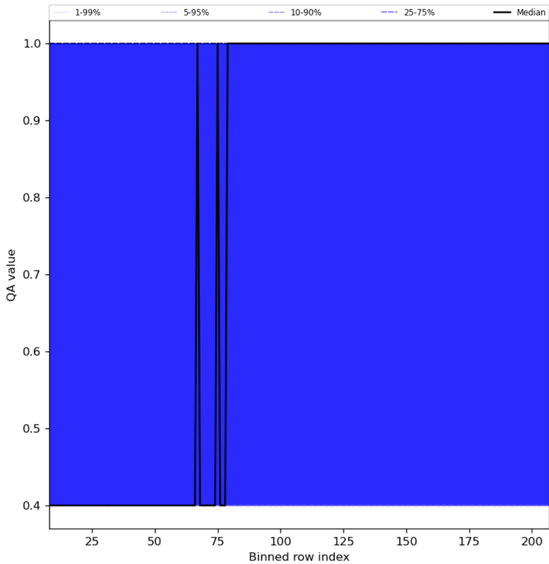
Figure 33: Along track statistics of “QA value” for 2023-07-22 to 2023-07-24
