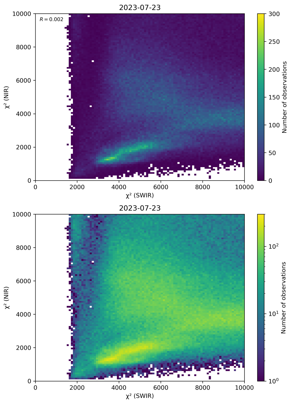
Figure 47: Scatter density plot of “ \chi^2 (SWIR)” against “ \chi^2 (NIR)” for 2023-07-22 to 2023-07-24.
