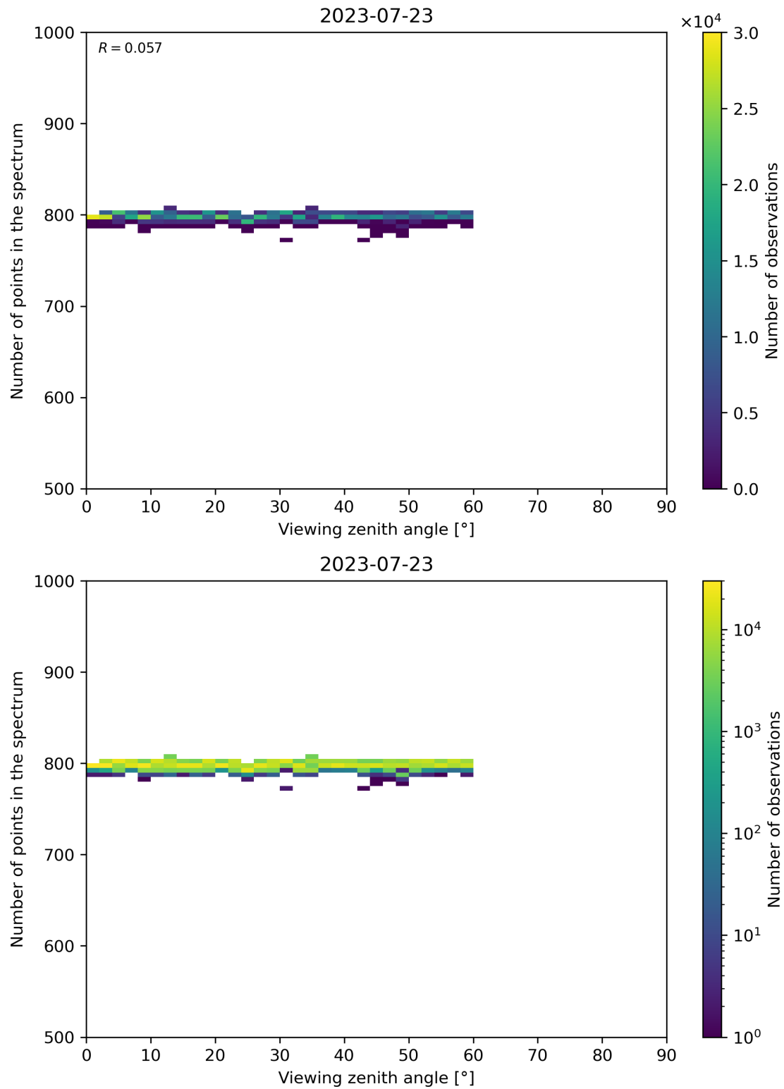
Figure 114: Scatter density plot of “Viewing zenith angle” against “Number of points in the spectrum” for 2023-07-22 to 2023-07-24.
