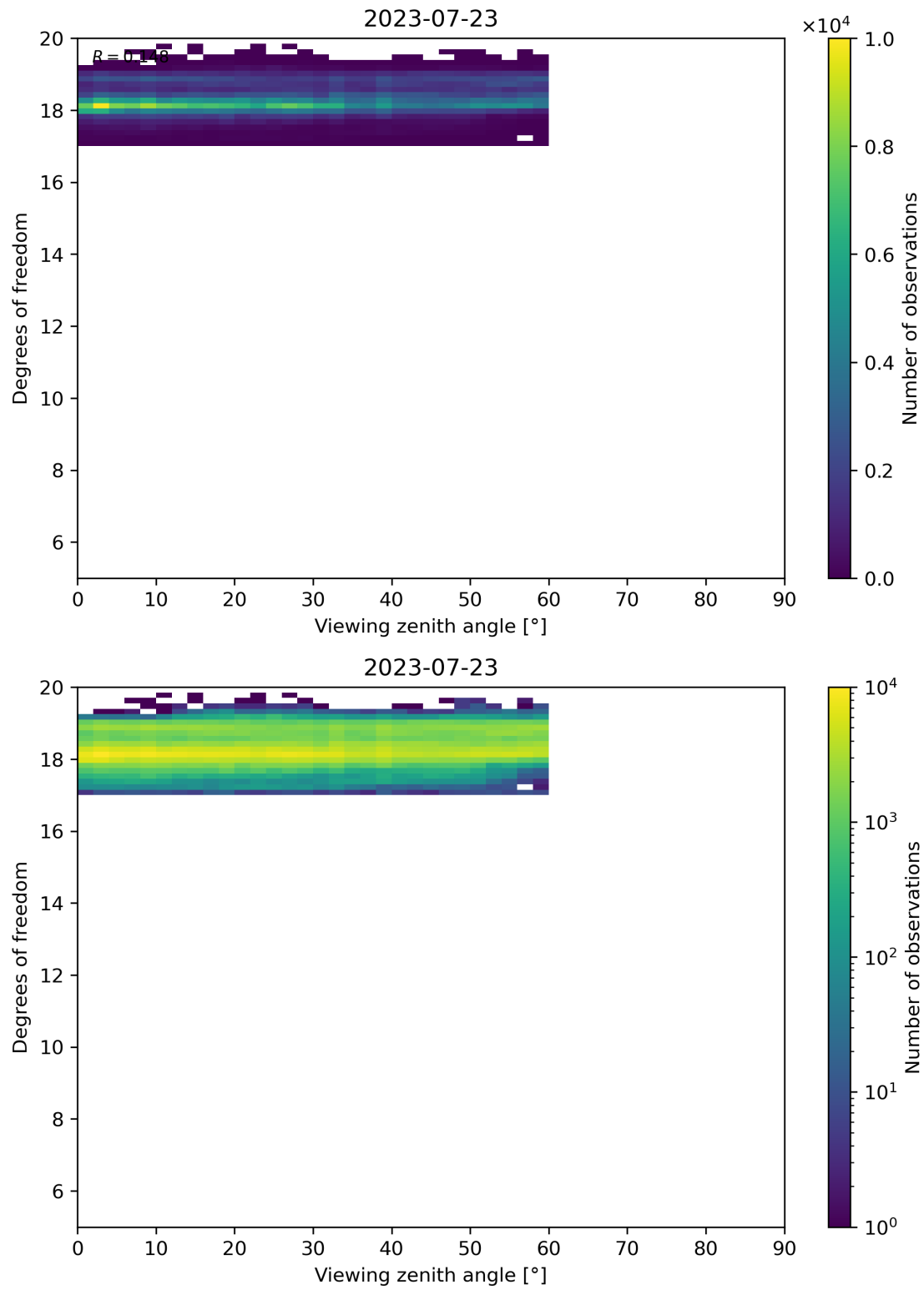
Figure 107: Scatter density plot of “Viewing zenith angle” against “Degrees of freedom” for 2023-07-22 to 2023-07-24.
