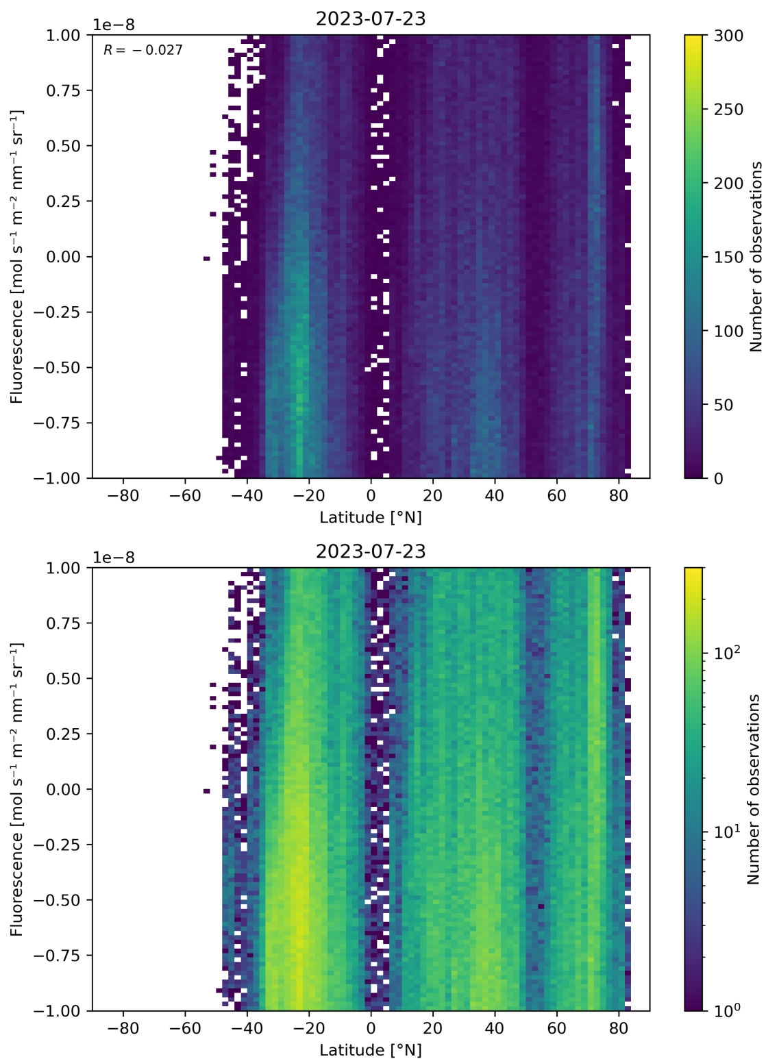
Figure 56: Scatter density plot of “Latitude” against “Fluorescence” for 2023-07-22 to 2023-07-24.
