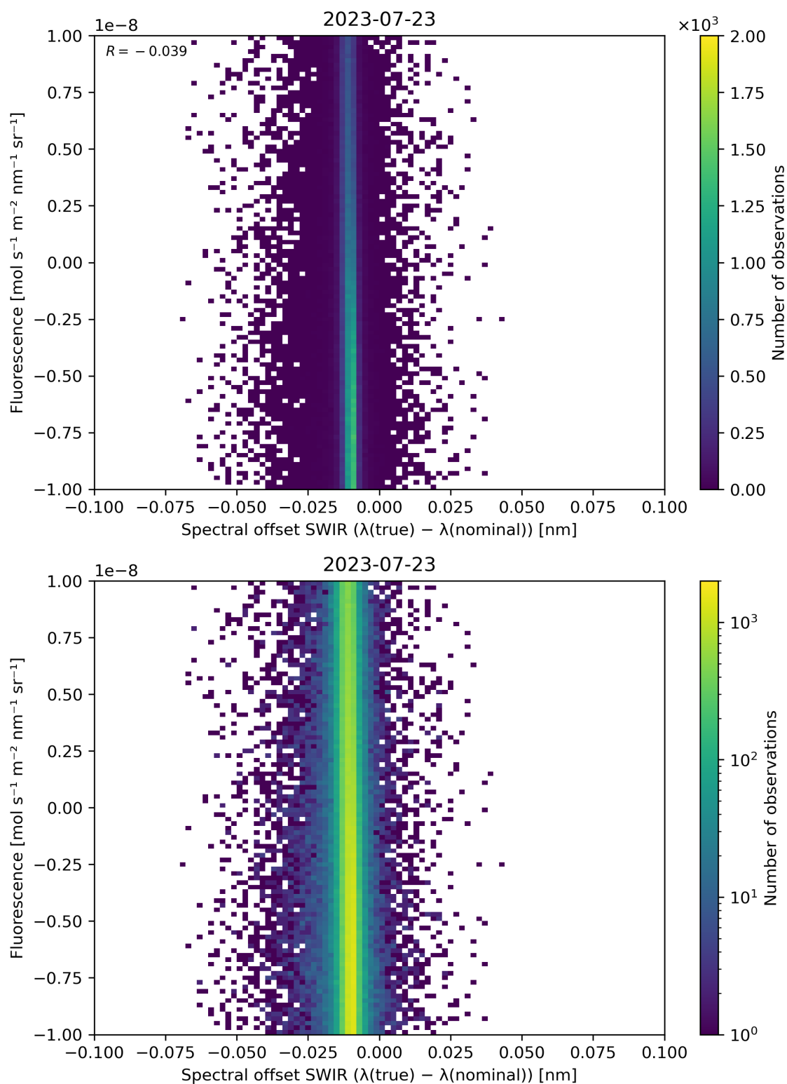
Figure 120: Scatter density plot of “Spectral offset SWIR ( \lambda(\text{true}) - \lambda(\text{nominal}) )” against “Fluorescence” for 2023-07-22 to 2023-07-24.
