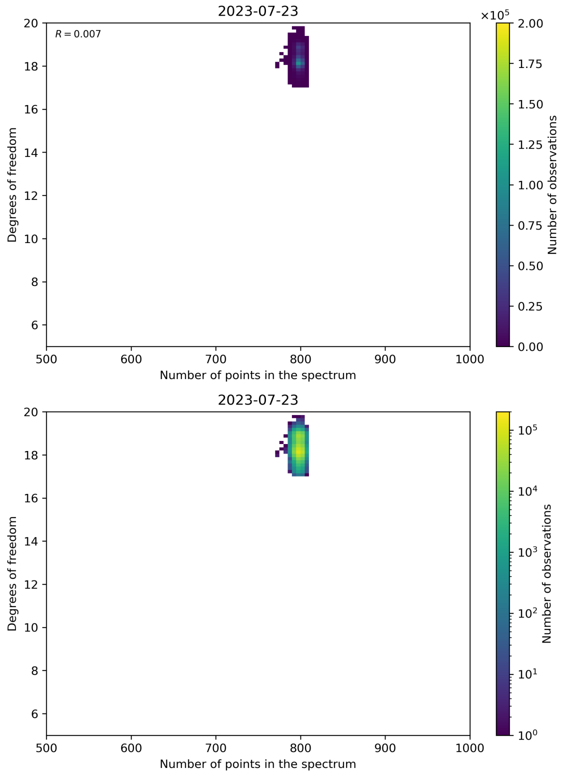
Figure 90: Scatter density plot of “Number of points in the spectrum” against “Degrees of freedom” for 2023-07-22 to 2023-07-24.
