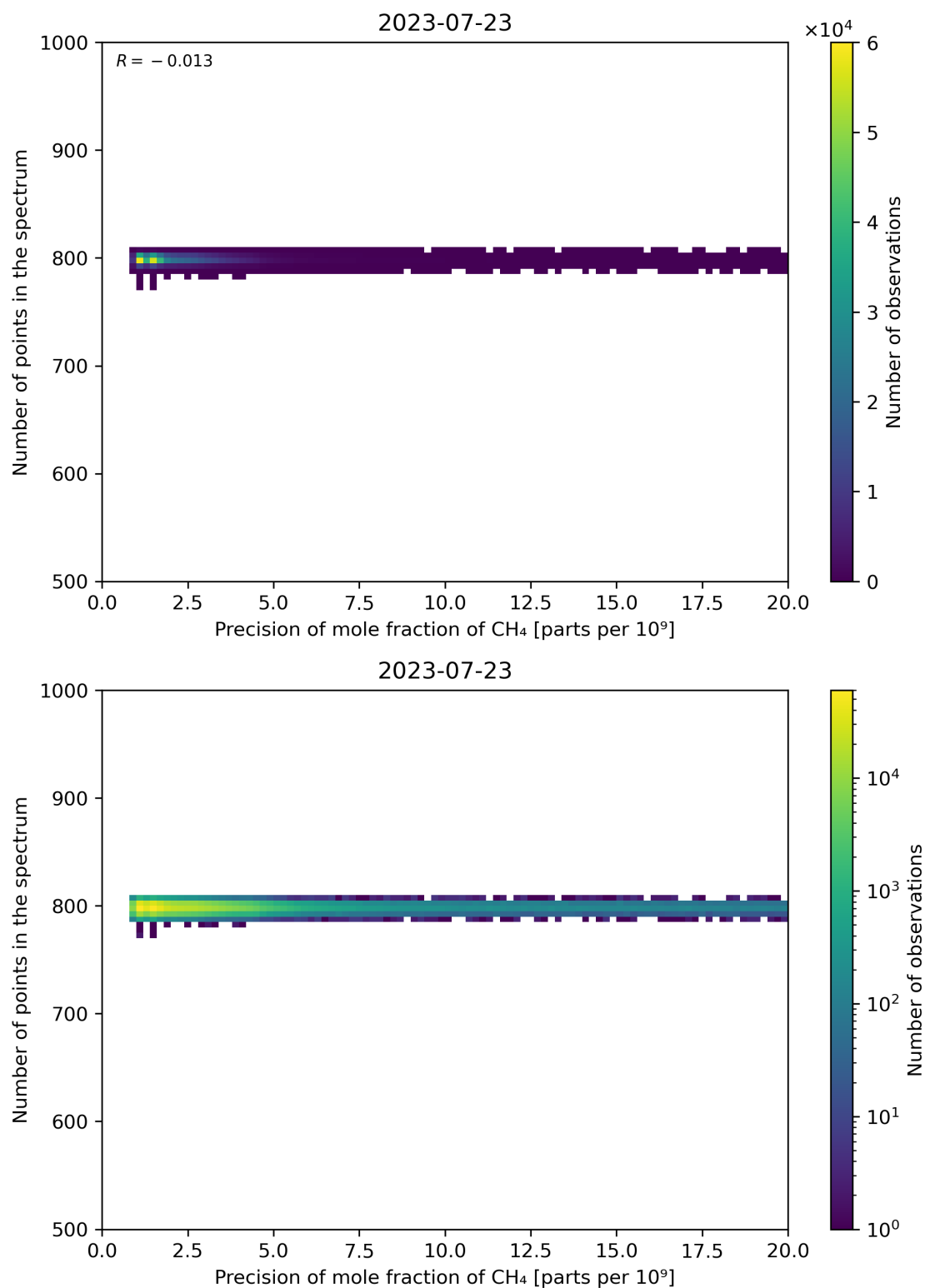
Figure 84: Scatter density plot of “Precision of mole fraction of CH 4 ” against “Number of points in the spectrum” for 2023-07-22 to 2023-07-24.
