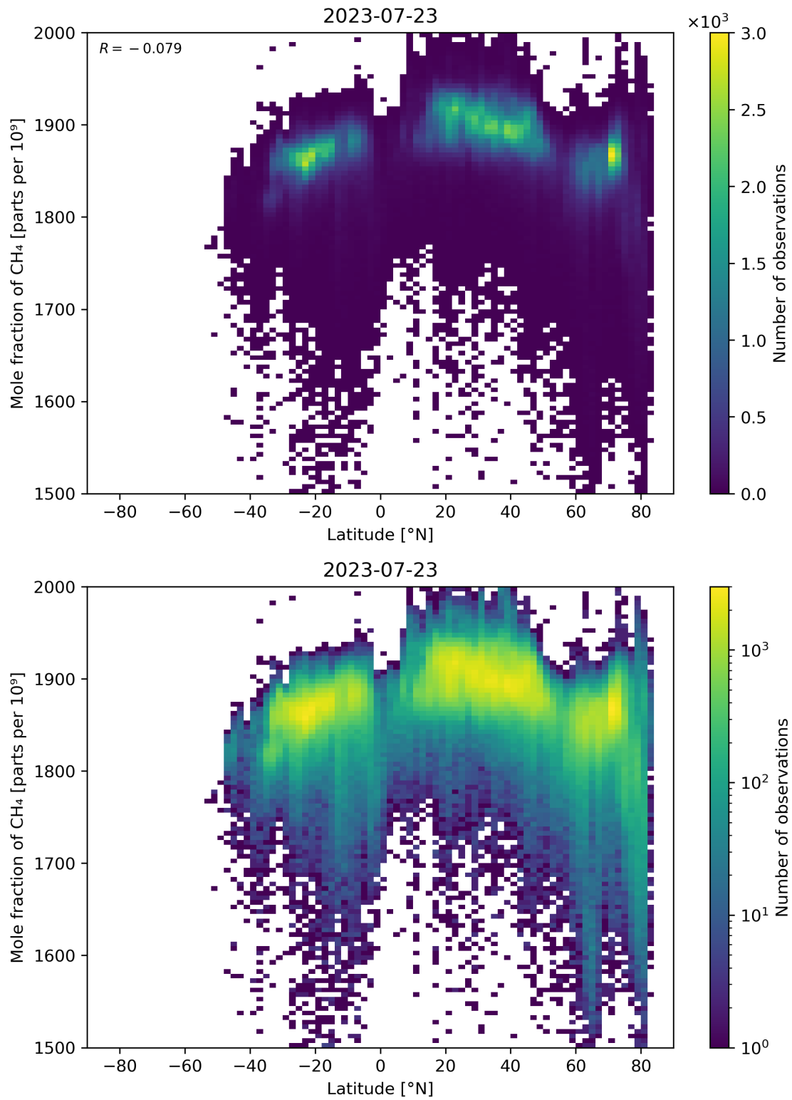
Figure 57: Scatter density plot of “Latitude” against “Mole fraction of CH 4 ” for 2023-07-22 to 2023-07-24.
