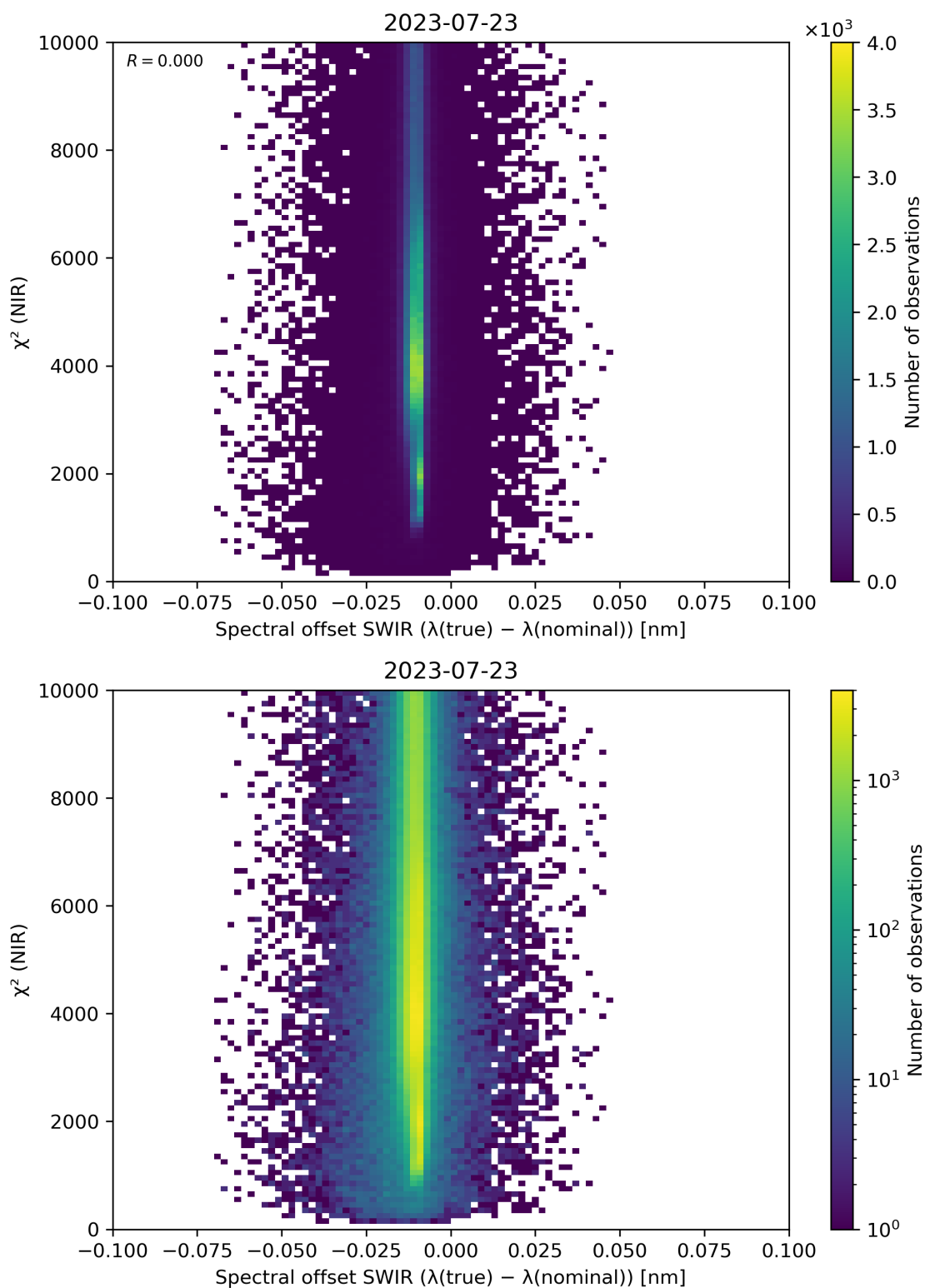
Figure 117: Scatter density plot of “Spectral offset SWIR ( \lambda(\text{true}) - \lambda(\text{nominal}) )” against “ \chi^2 (NIR)” for 2023-07-22 to 2023-07-24.
