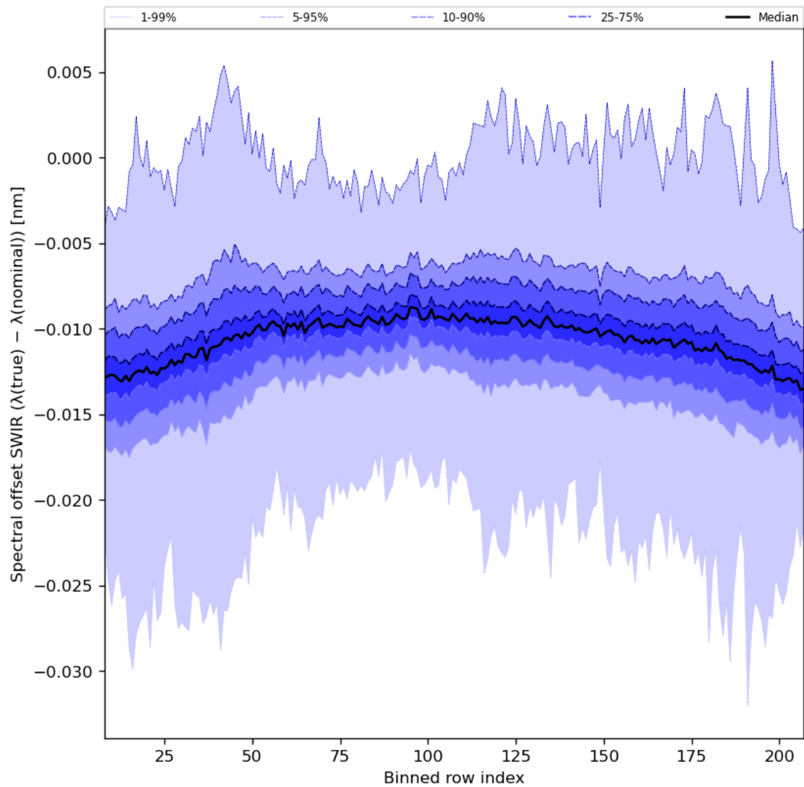
Figure 38: Along track statistics of “Spectral offset SWIR ( \lambda(\text{true}) - \lambda(\text{nominal}) )” for 2023-07-22 to 2023-07-24
