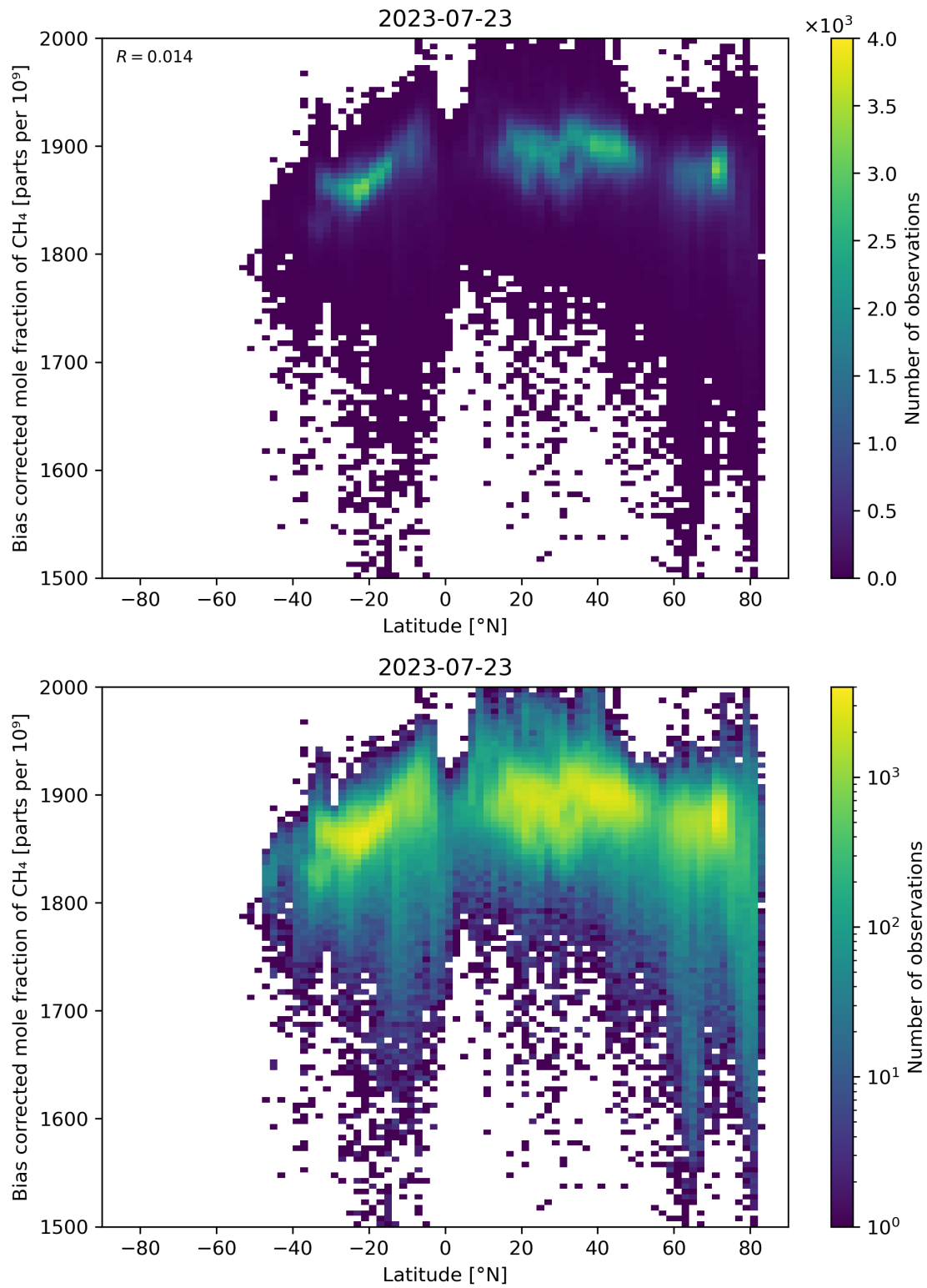
Figure 58: Scatter density plot of “Latitude” against “Bias corrected mole fraction of CH 4 ” for 2023-07-22 to 2023-07-24.
