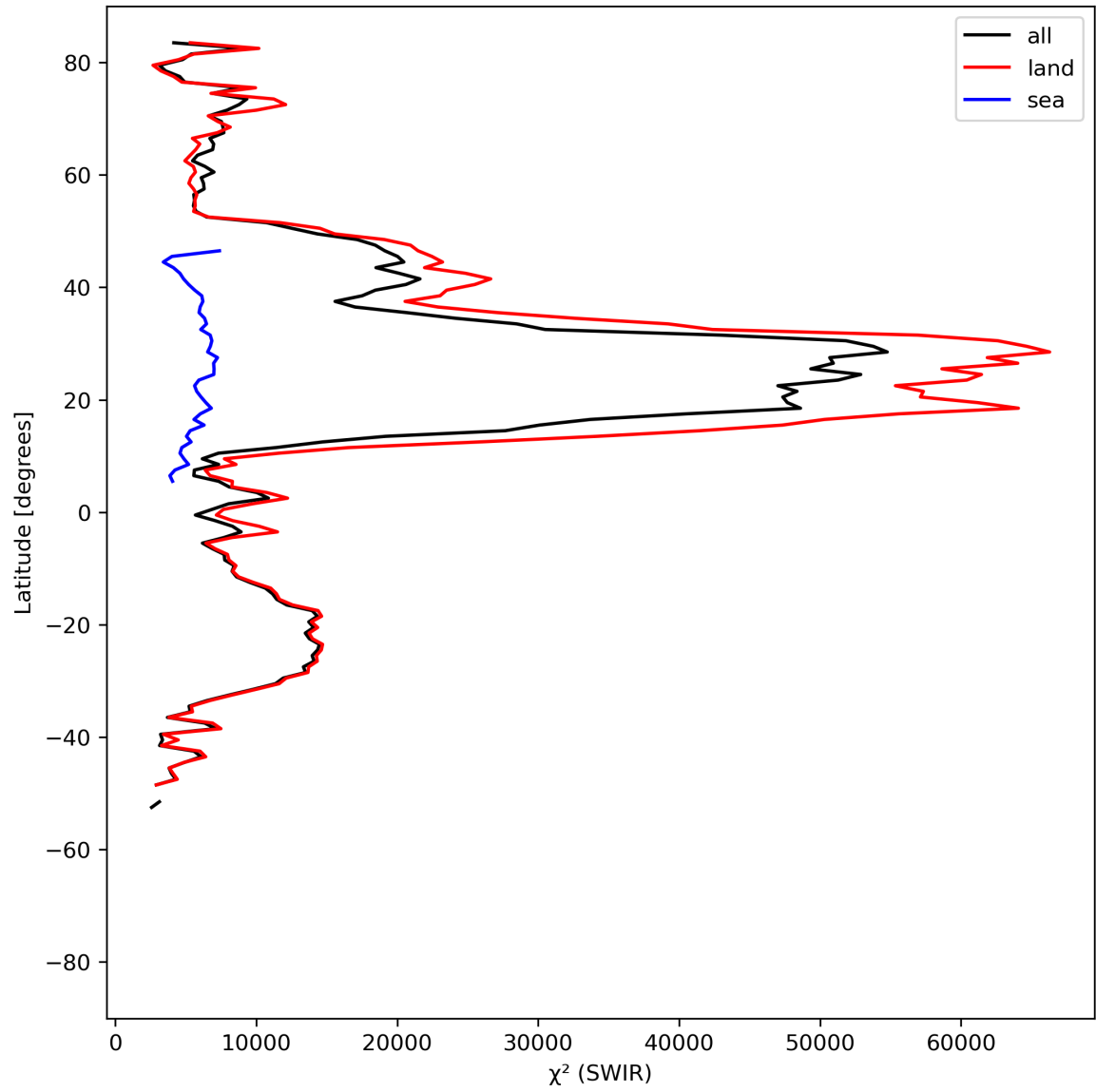
Figure 17: Zonal average of “ \chi^2 (SWIR)” for 2023-07-22 to 2023-07-24.
