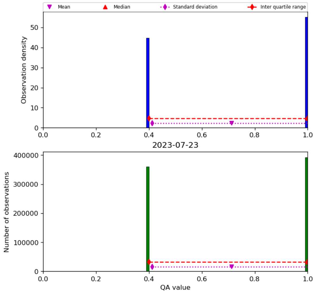
Figure 22: Histogram of “QA value” for 2023-07-22 to 2023-07-24
