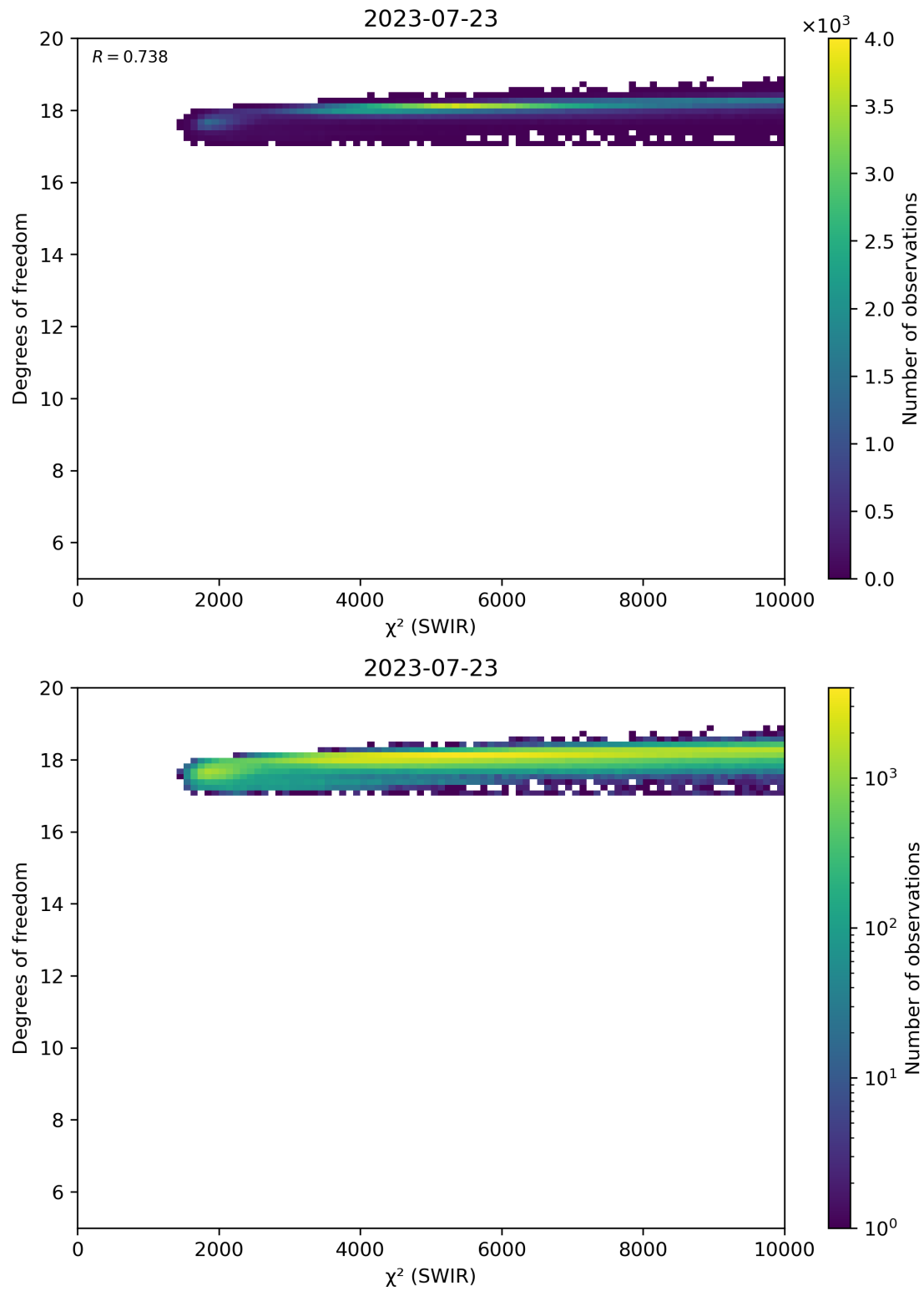
Figure 48: Scatter density plot of “ \chi^2 (SWIR)” against “Degrees of freedom” for 2023-07-22 to 2023-07-24.
