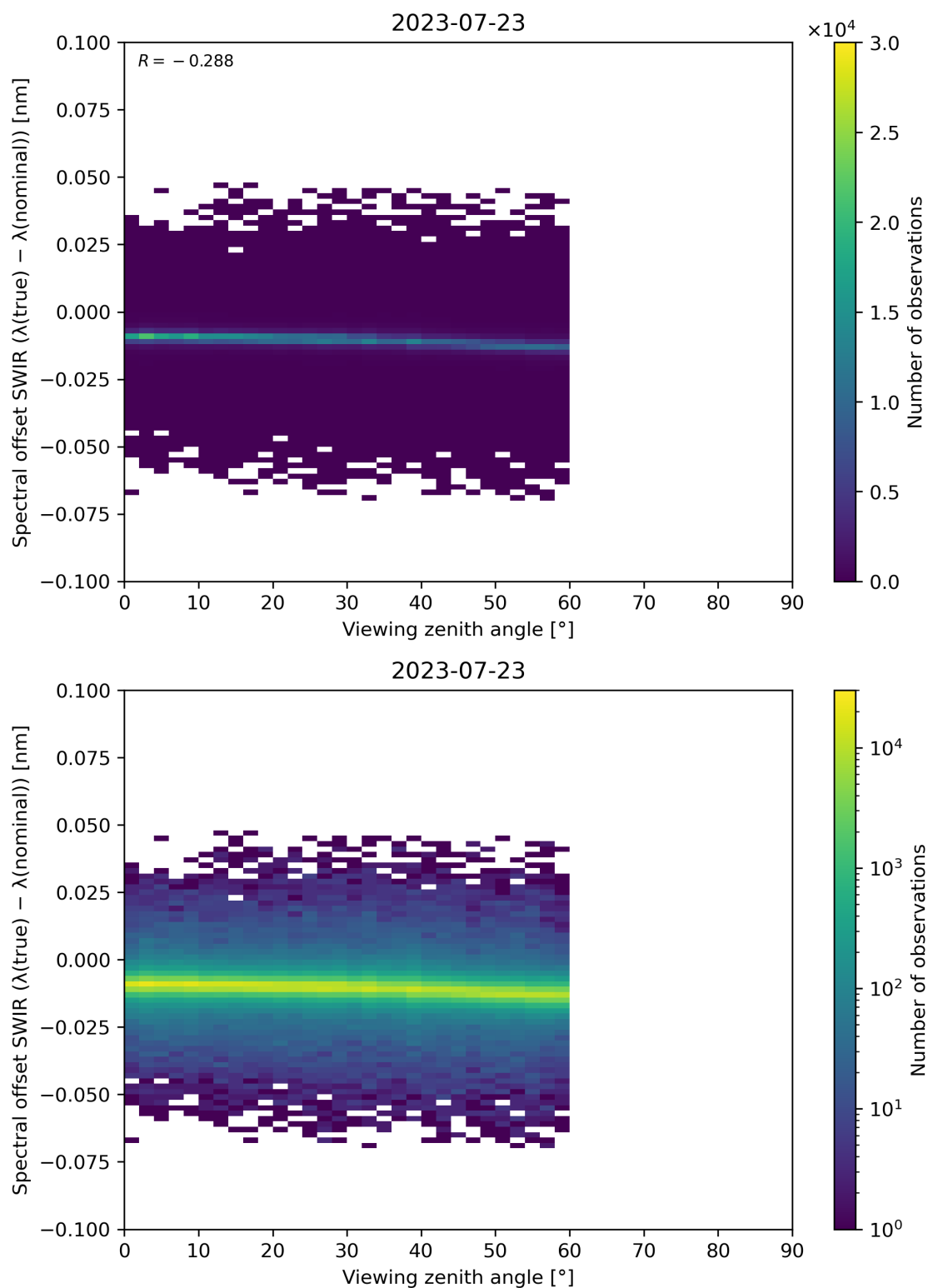
Figure 116: Scatter density plot of “Viewing zenith angle” against “Spectral offset SWIR ( \lambda(\text{true}) - \lambda(\text{nominal}) )” for 2023-07-22 to 2023-07-24.
