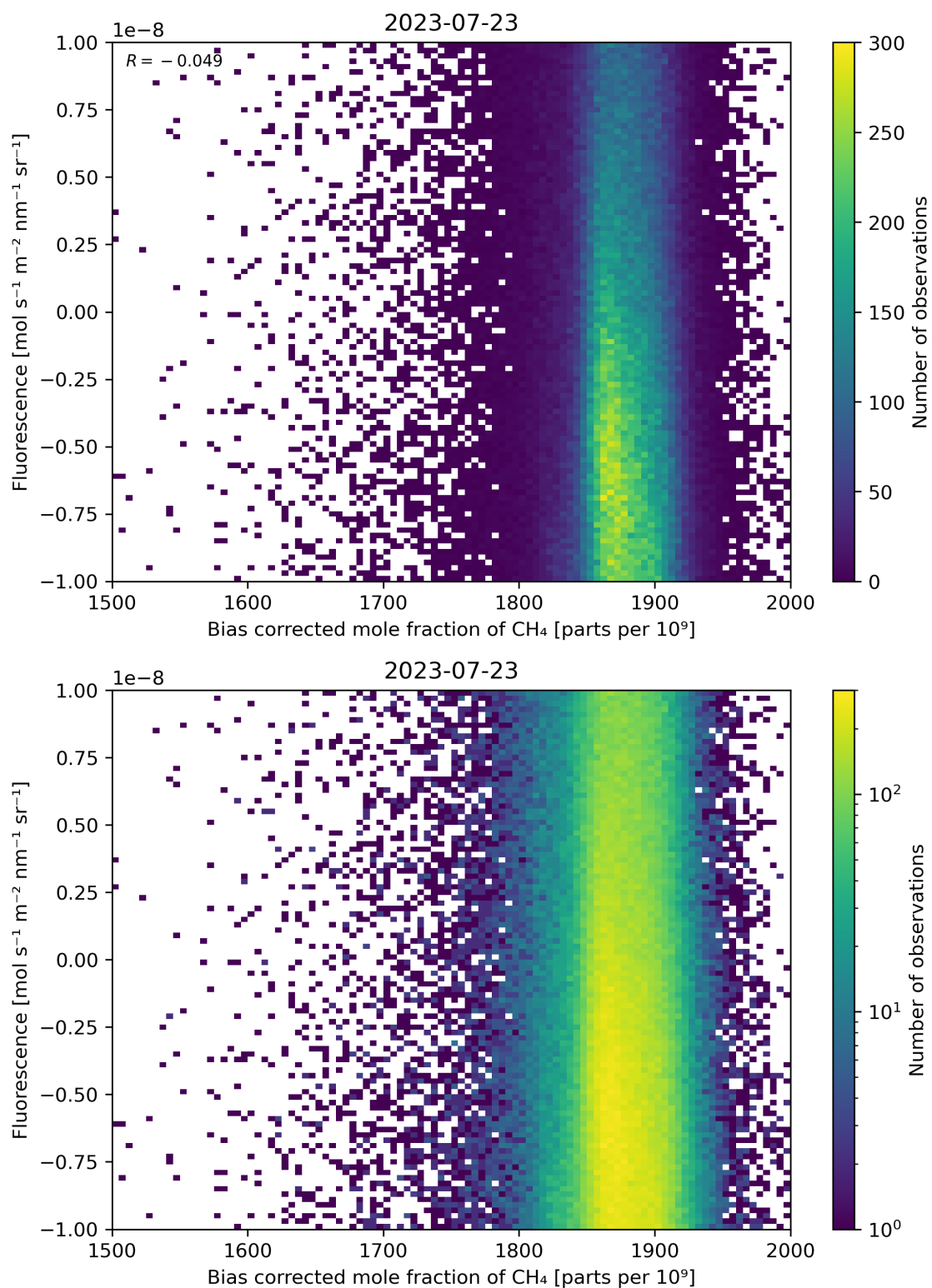
Figure 66: Scatter density plot of “Bias corrected mole fraction of \text{CH}_4 ” against “Fluorescence” for 2023-07-22 to 2023-07-24.
