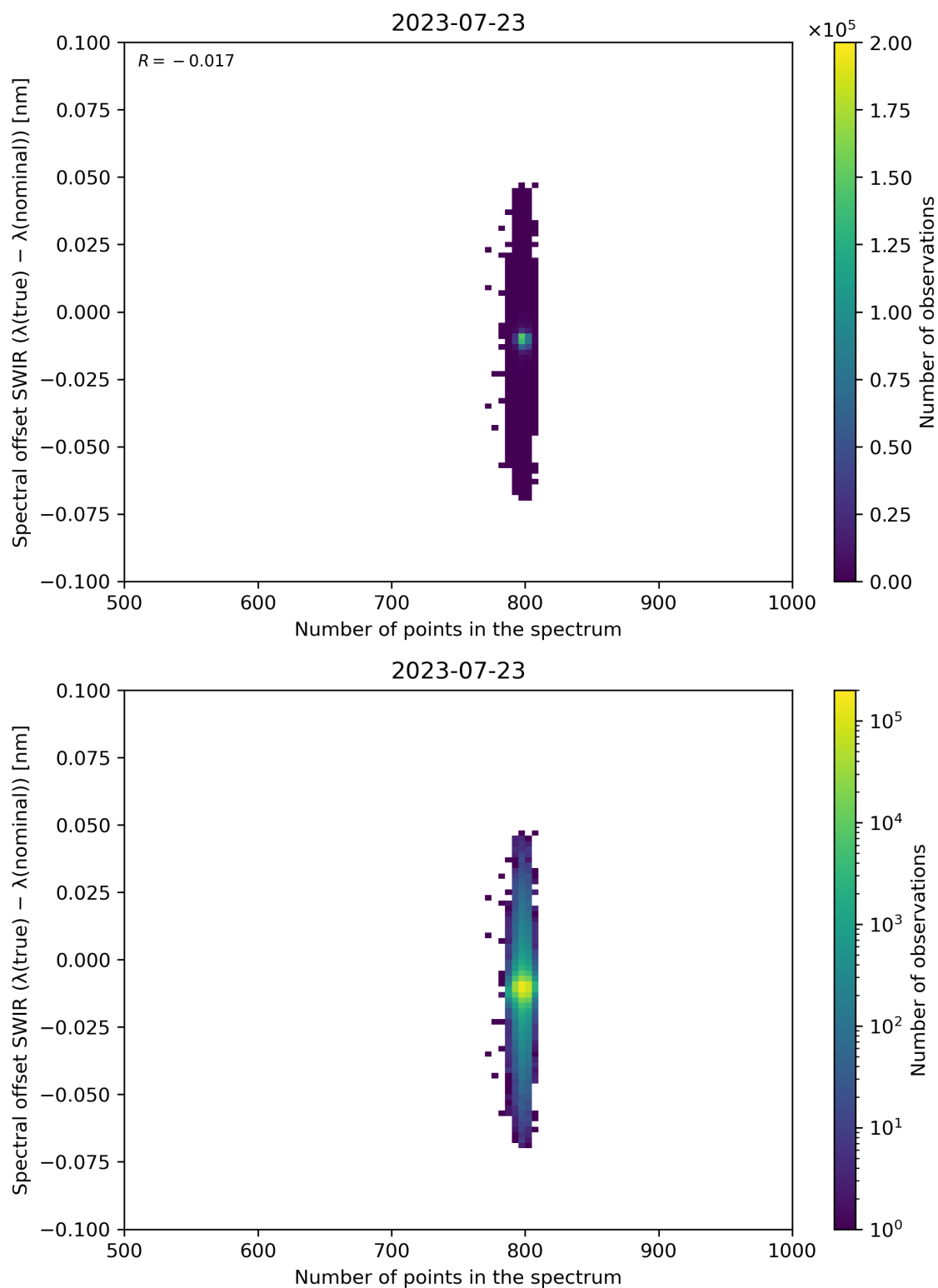
Figure 93: Scatter density plot of “Number of points in the spectrum” against “Spectral offset SWIR ( \lambda(\text{true}) - \lambda(\text{nominal}) )” for 2023-07-22 to 2023-07-24.
