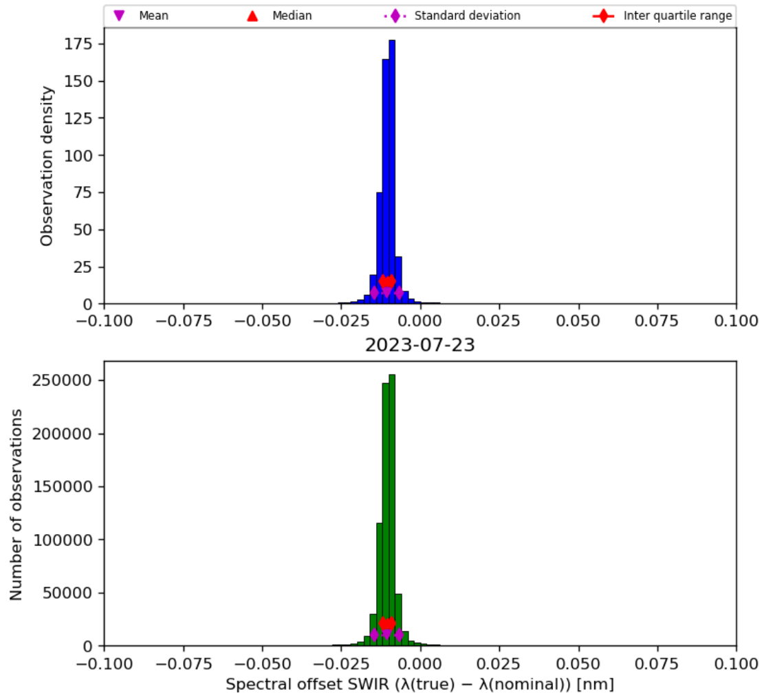
Figure 27: Histogram of “Spectral offset SWIR ( \lambda(\text{true}) - \lambda(\text{nominal}) )” for 2023-07-22 to 2023-07-24
