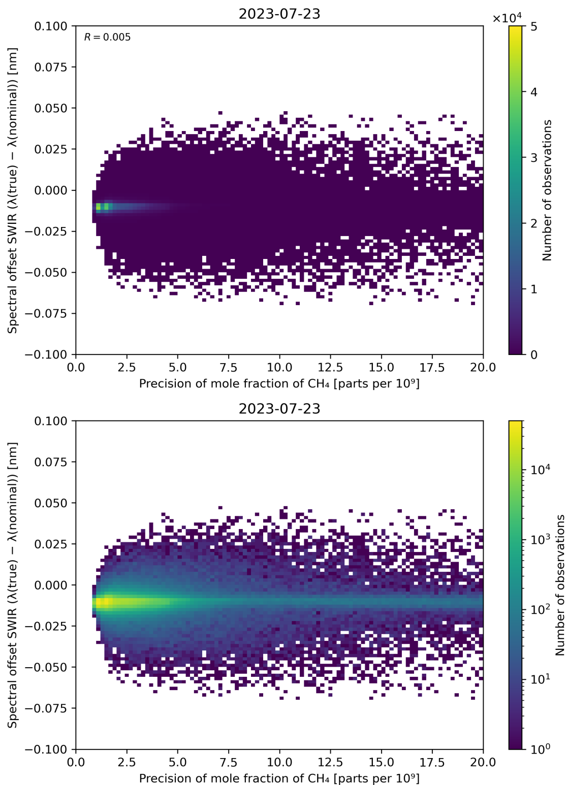
Figure 85: Scatter density plot of “Precision of mole fraction of CH 4 ” against “Spectral offset SWIR ( \lambda(\text{true}) - \lambda(\text{nominal}) )” for 2023-07-22 to 2023-07-24.
