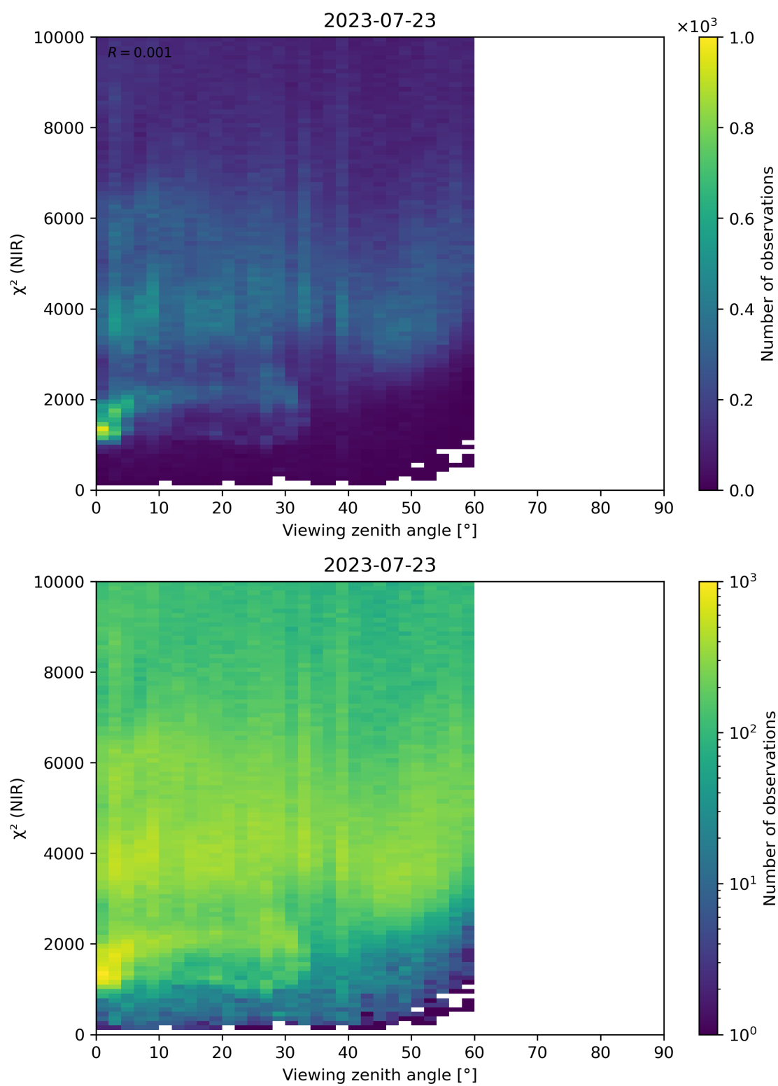
Figure 105: Scatter density plot of “Viewing zenith angle” against “ \chi^2 (NIR)” for 2023-07-22 to 2023-07-24.
