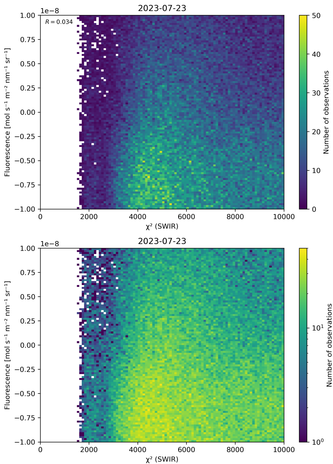
Figure 49: Scatter density plot of “ \chi^2 (SWIR)” against “Fluorescence” for 2023-07-22 to 2023-07-24.
