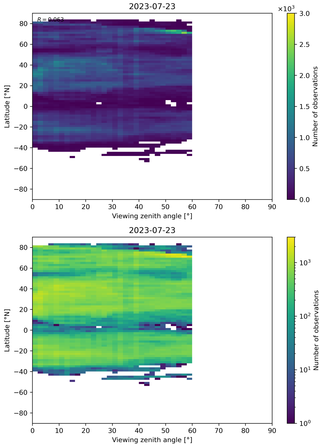
Figure 109: Scatter density plot of “Viewing zenith angle” against “Latitude” for 2023-07-22 to 2023-07-24.
