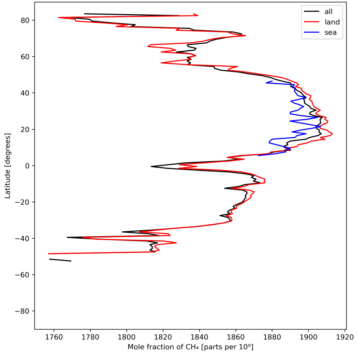
Figure 12: Zonal average of “Mole fraction of \text{CH}_4 ” for 2023-07-22 to 2023-07-24.
