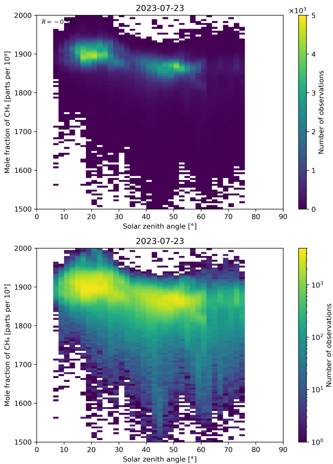
Figure 99: Scatter density plot of “Solar zenith angle” against “Mole fraction of CH 4 ” for 2023-07-22 to 2023-07-24.
