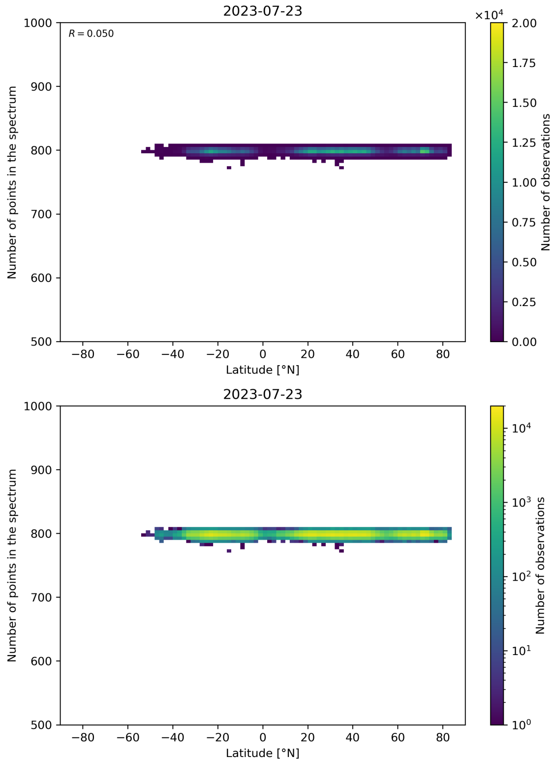
Figure 61: Scatter density plot of “Latitude” against “Number of points in the spectrum” for 2023-07-22 to 2023-07-24.
