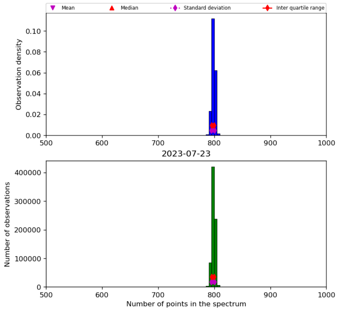
Figure 26: Histogram of “Number of points in the spectrum” for 2023-07-22 to 2023-07-24
