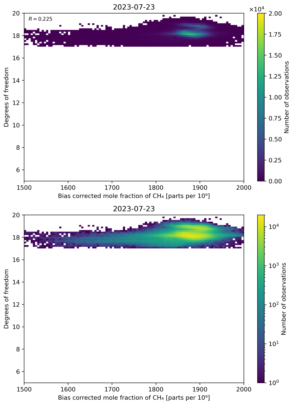
Figure 65: Scatter density plot of “Bias corrected mole fraction of \text{CH}_4 ” against “Degrees of freedom” for 2023-07-22 to 2023-07-24.
