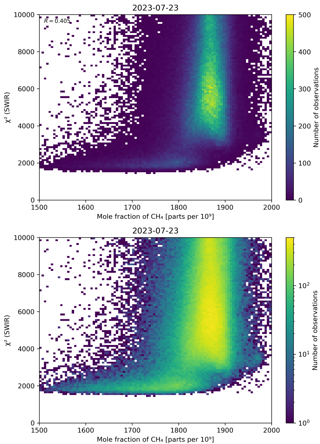
Figure 71: Scatter density plot of “Mole fraction of \text{CH}_4 ” against “ \chi^2 (SWIR)” for 2023-07-22 to 2023-07-24.
