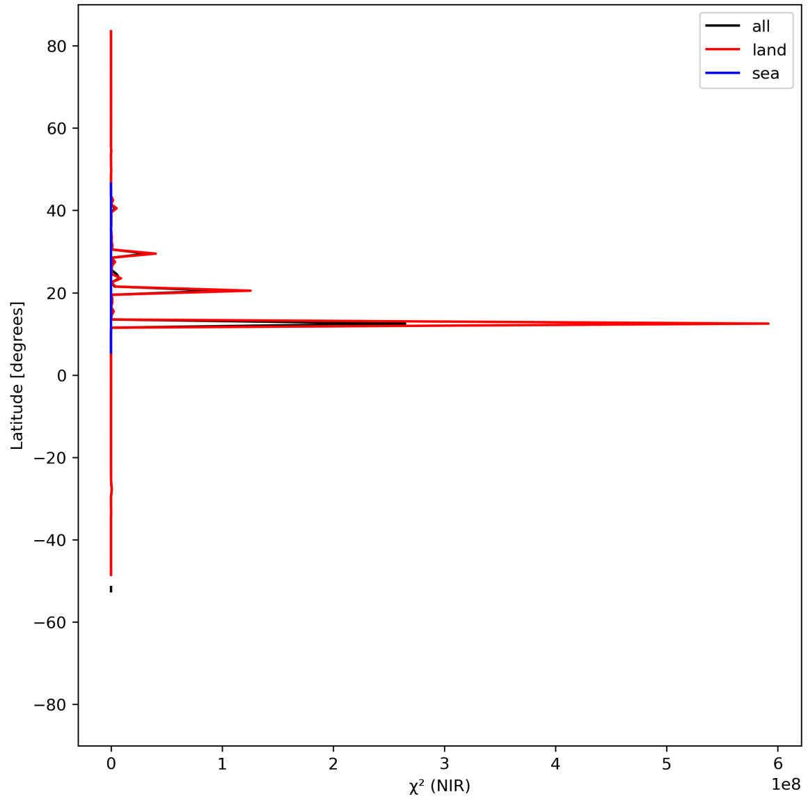
Figure 18: Zonal average of “ \chi^2 (NIR)” for 2023-07-22 to 2023-07-24.
