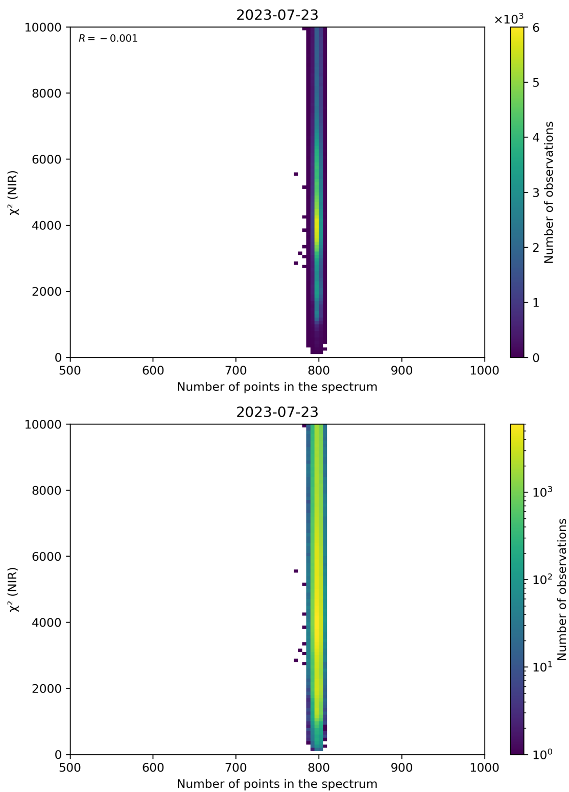
Figure 88: Scatter density plot of “Number of points in the spectrum” against “ \chi^2 (NIR)” for 2023-07-22 to 2023-07-24.
