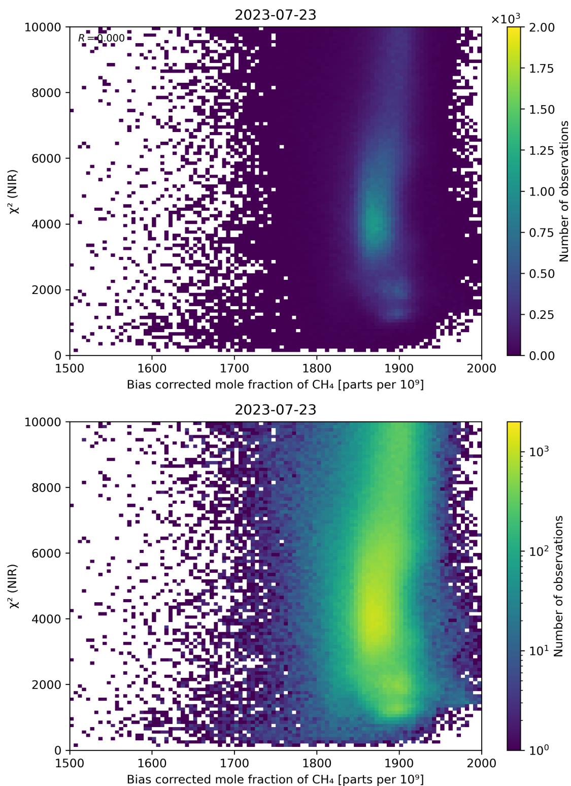
Figure 63: Scatter density plot of “Bias corrected mole fraction of CH 4 ” against “ \chi^2 (NIR)” for 2023-07-22 to 2023-07-24.
