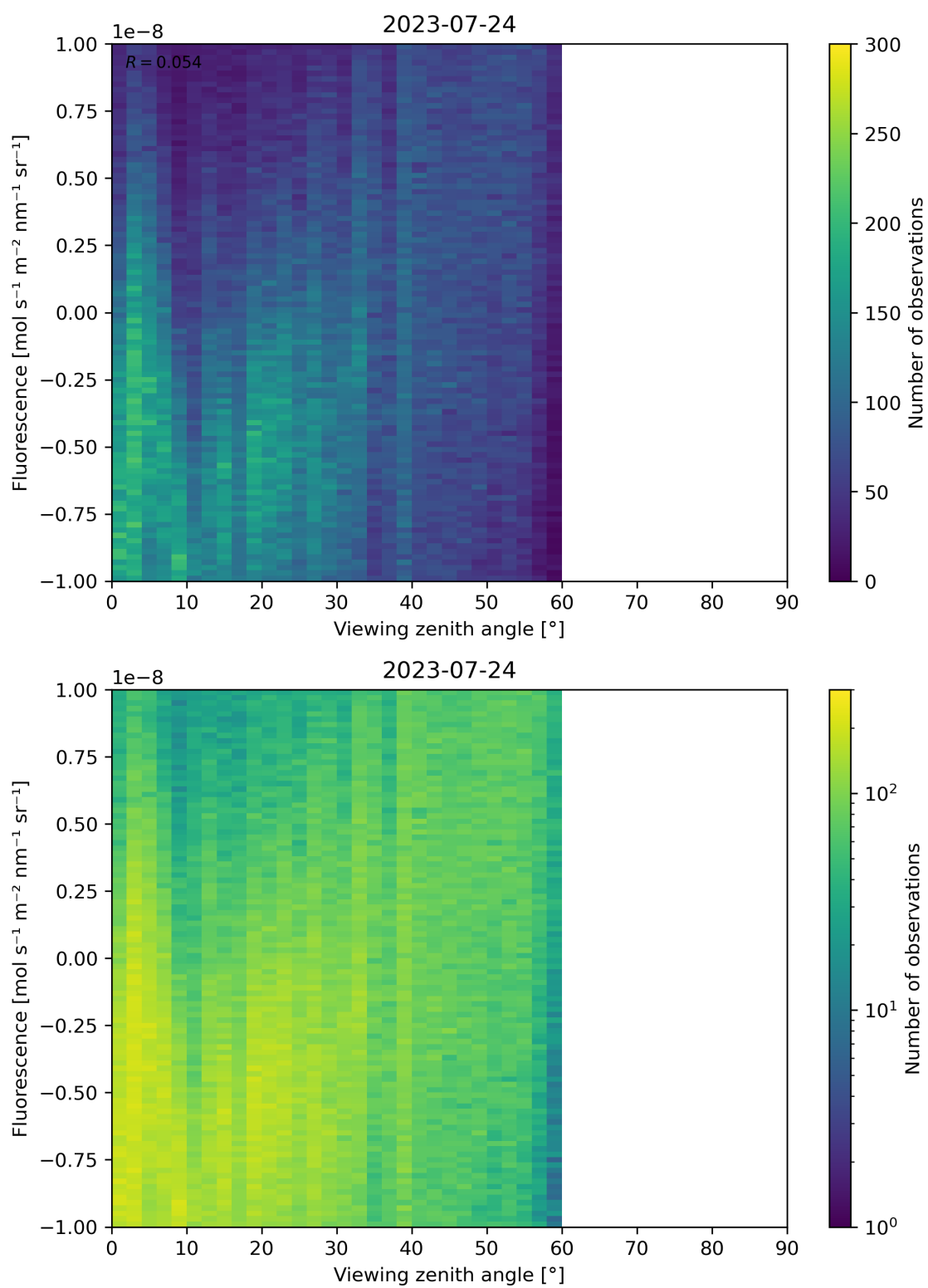
Figure 108: Scatter density plot of “Viewing zenith angle” against “Fluorescence” for 2023-07-24 to 2023-07-25.
