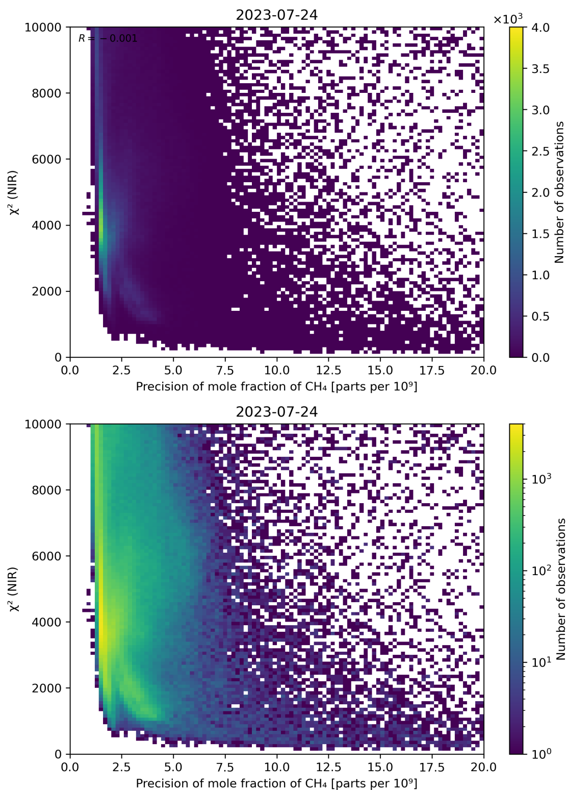
Figure 78: Scatter density plot of “Precision of mole fraction of CH 4 ” against “ \chi^2 (NIR)” for 2023-07-24 to 2023-07-25.
