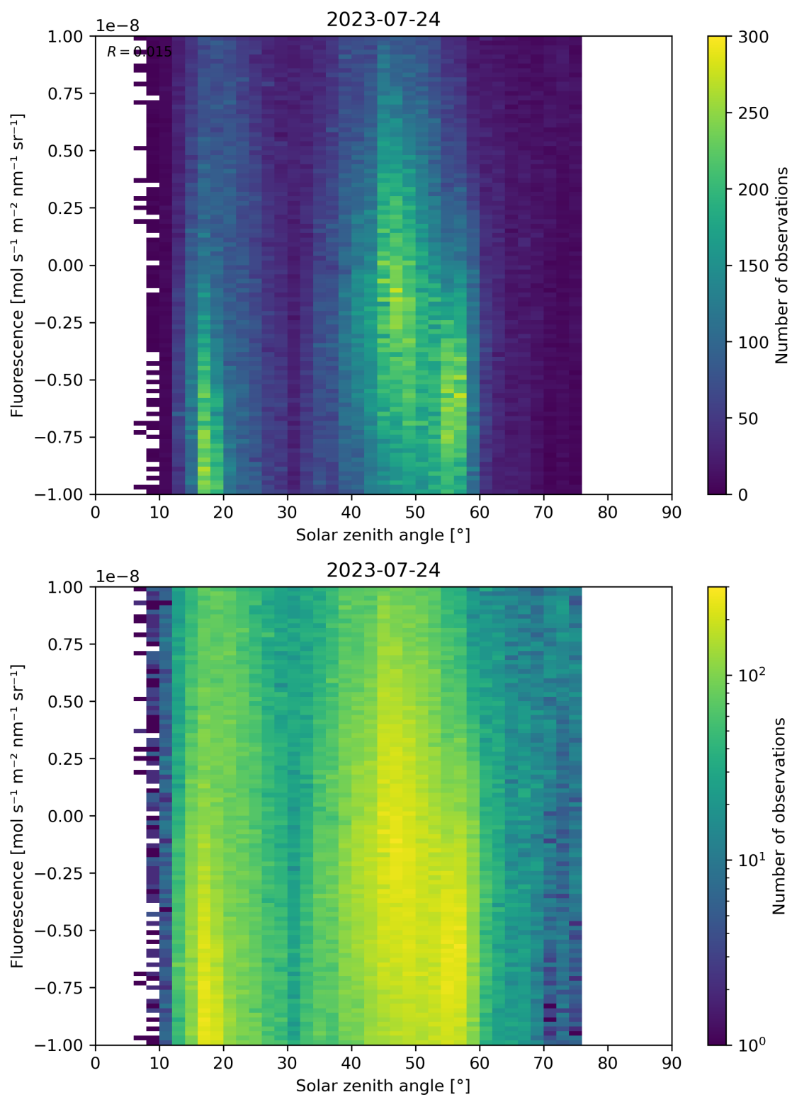
Figure 97: Scatter density plot of “Solar zenith angle” against “Fluorescence” for 2023-07-24 to 2023-07-25.
