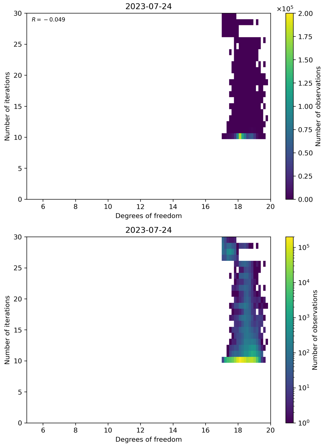
Figure 52: Scatter density plot of “Degrees of freedom” against “Number of iterations” for 2023-07-24 to 2023-07-25.
