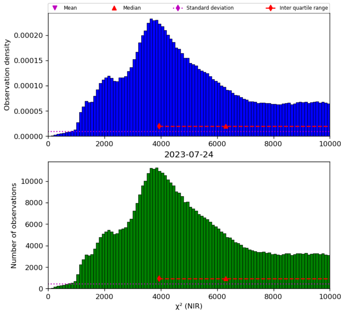
Figure 29: Histogram of “ \chi^2 (NIR)” for 2023-07-24 to 2023-07-25
