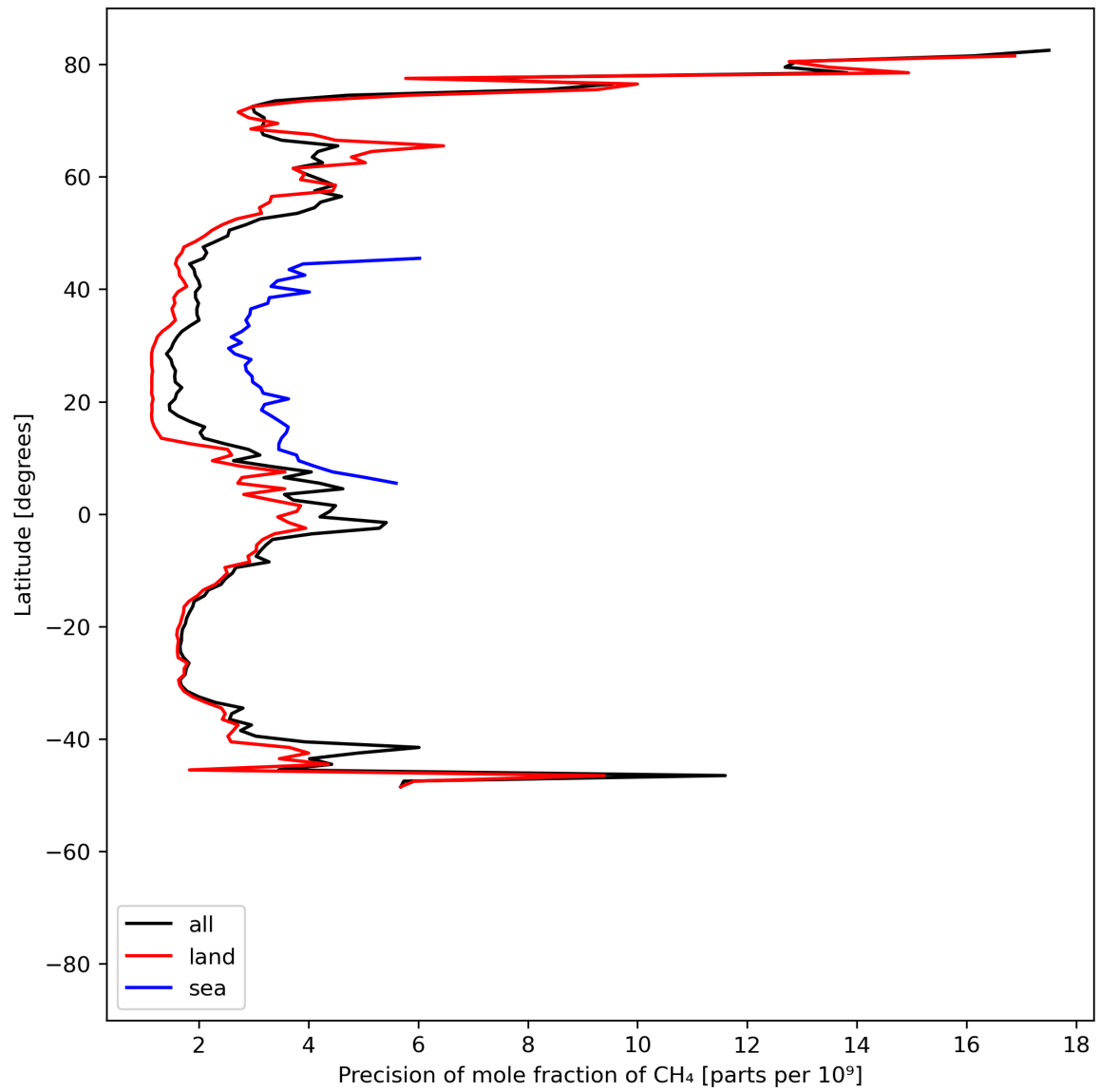
Figure 13: Zonal average of “Precision of mole fraction of CH 4 ” for 2023-07-24 to 2023-07-25.
