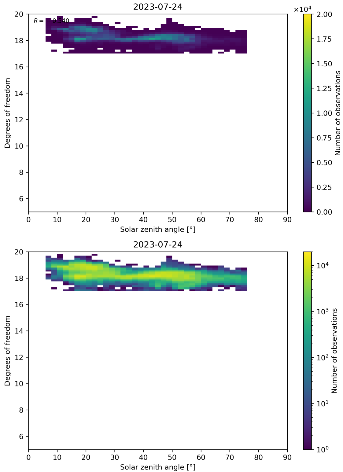
Figure 96: Scatter density plot of “Solar zenith angle” against “Degrees of freedom” for 2023-07-24 to 2023-07-25.
