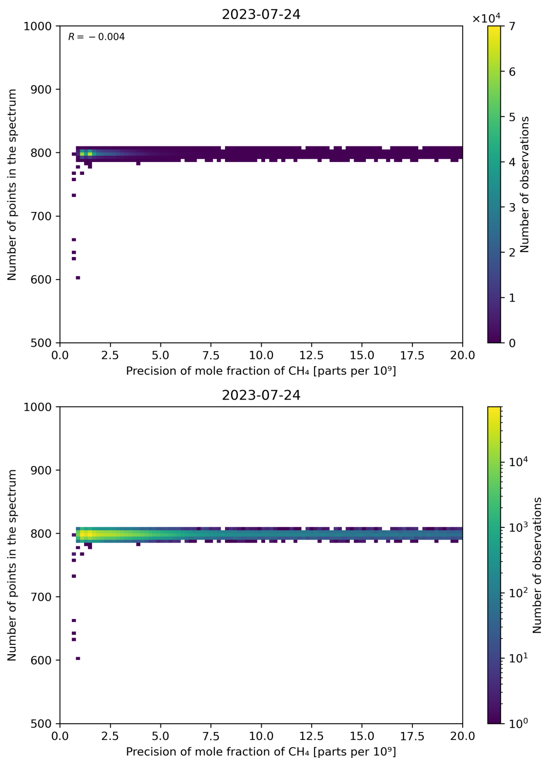
Figure 84: Scatter density plot of “Precision of mole fraction of CH 4 ” against “Number of points in the spectrum” for 2023-07-24 to 2023-07-25.
