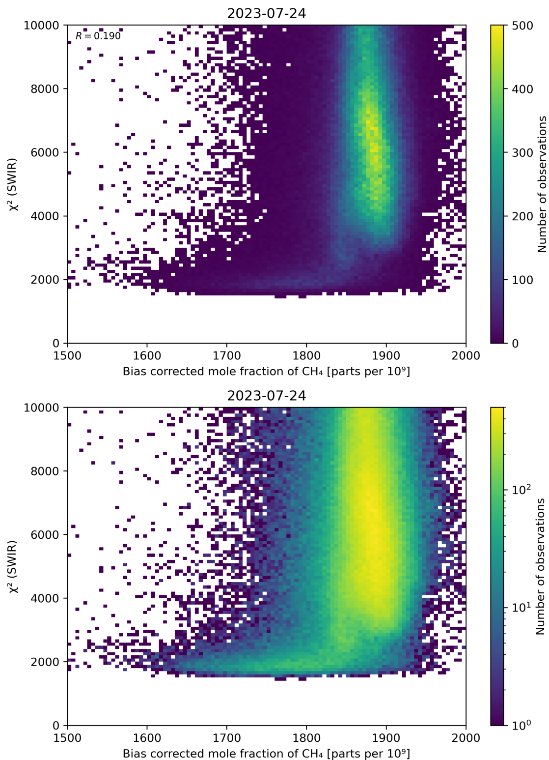
Figure 64: Scatter density plot of “Bias corrected mole fraction of \text{CH}_4 ” against “ \chi^2 (SWIR)” for 2023-07-24 to 2023-07-25.
