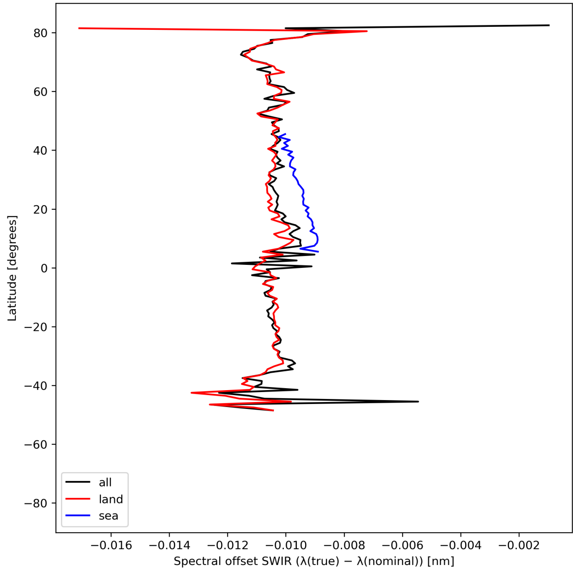
Figure 16: Zonal average of “Spectral offset SWIR ( \lambda(\text{true}) - \lambda(\text{nominal}) )” for 2023-07-24 to 2023-07-25.
