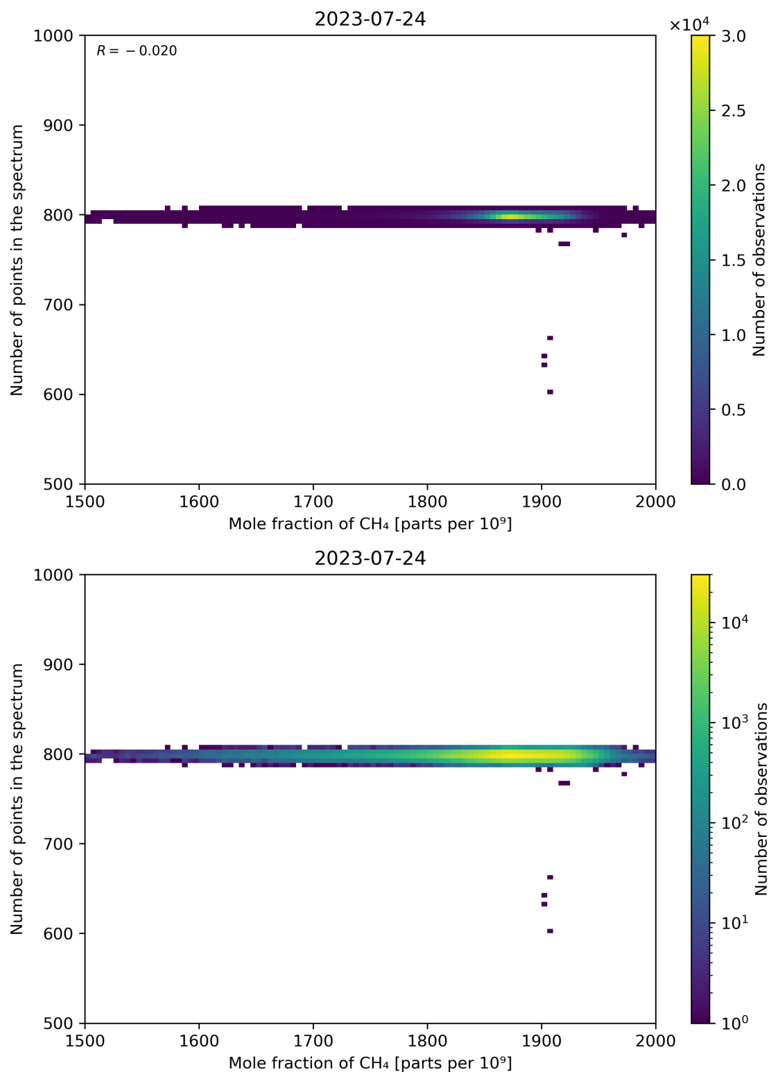
Figure 77: Scatter density plot of “Mole fraction of CH 4 ” against “Number of points in the spectrum” for 2023-07-24 to 2023-07-25.
