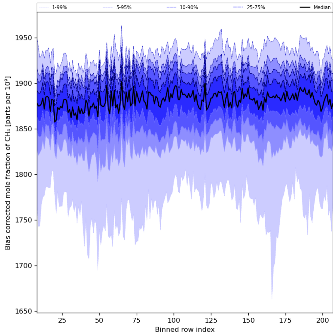
Figure 36: Along track statistics of “Bias corrected mole fraction of CH 4 ” for 2023-07-24 to 2023-07-25
