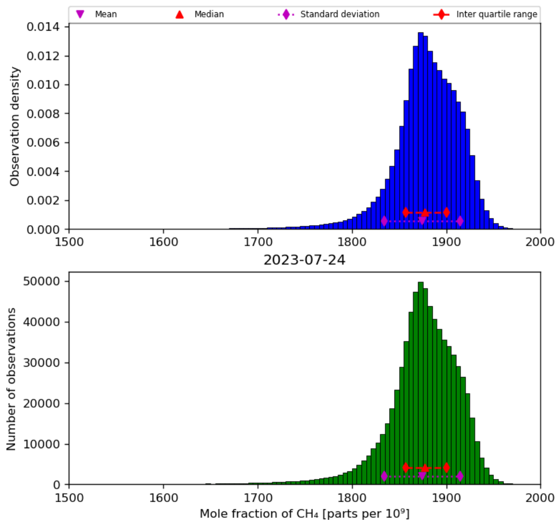
Figure 23: Histogram of “Mole fraction of CH 4 ” for 2023-07-24 to 2023-07-25
