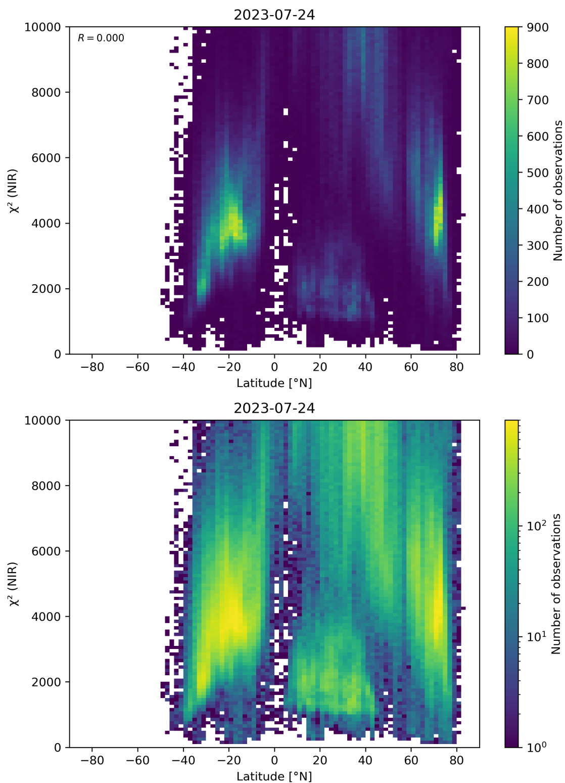
Figure 53: Scatter density plot of “Latitude” against “ \chi^2 (NIR)” for 2023-07-24 to 2023-07-25.
