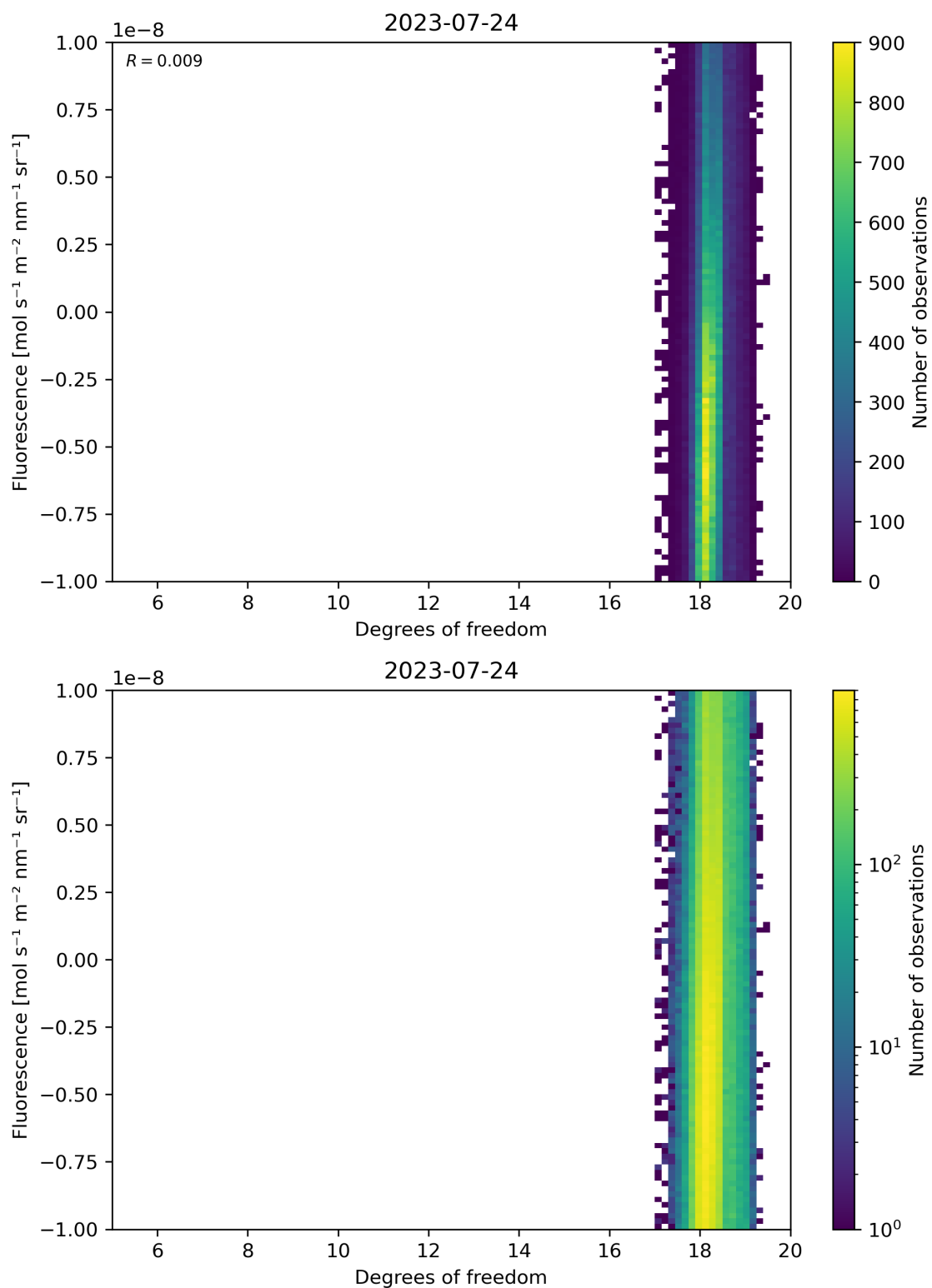
Figure 51: Scatter density plot of “Degrees of freedom” against “Fluorescence” for 2023-07-24 to 2023-07-25.
