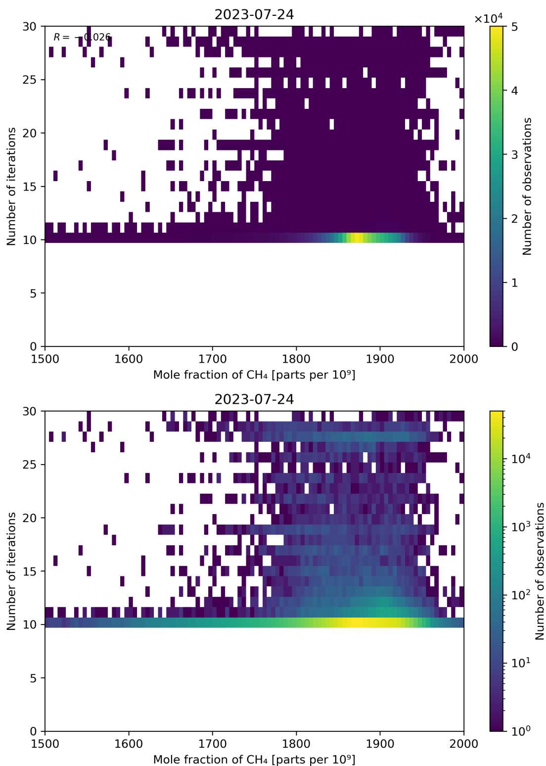
Figure 76: Scatter density plot of “Mole fraction of CH 4 ” against “Number of iterations” for 2023-07-24 to 2023-07-25.
