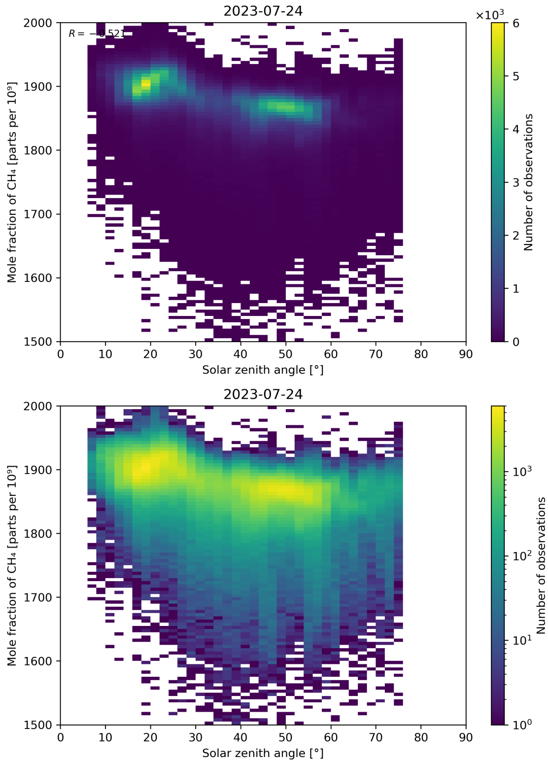
Figure 99: Scatter density plot of “Solar zenith angle” against “Mole fraction of CH 4 ” for 2023-07-24 to 2023-07-25.
