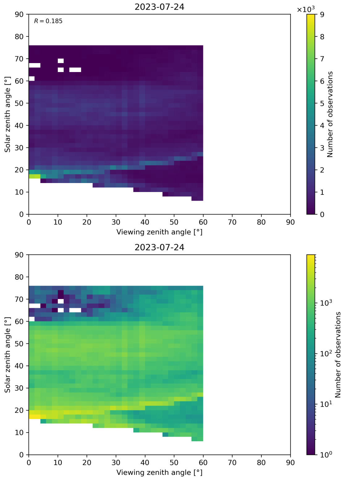
Figure 115: Scatter density plot of “Viewing zenith angle” against “Solar zenith angle” for 2023-07-24 to 2023-07-25.
