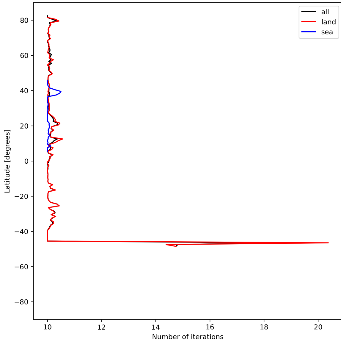
Figure 20: Zonal average of “Number of iterations” for 2023-07-24 to 2023-07-25.
