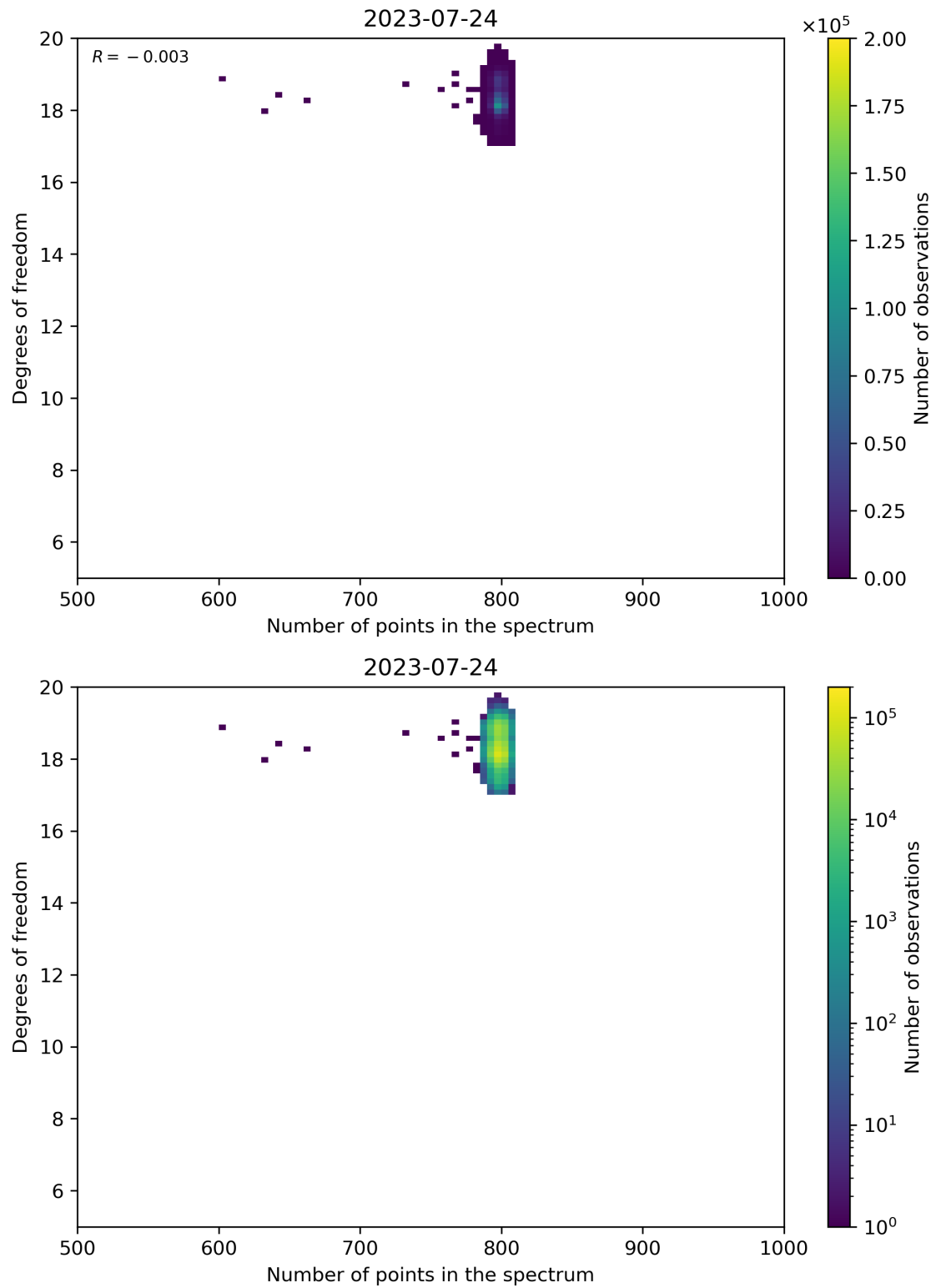
Figure 90: Scatter density plot of “Number of points in the spectrum” against “Degrees of freedom” for 2023-07-24 to 2023-07-25.
