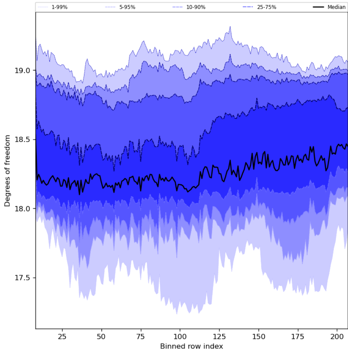
Figure 41: Along track statistics of “Degrees of freedom” for 2023-07-24 to 2023-07-25
