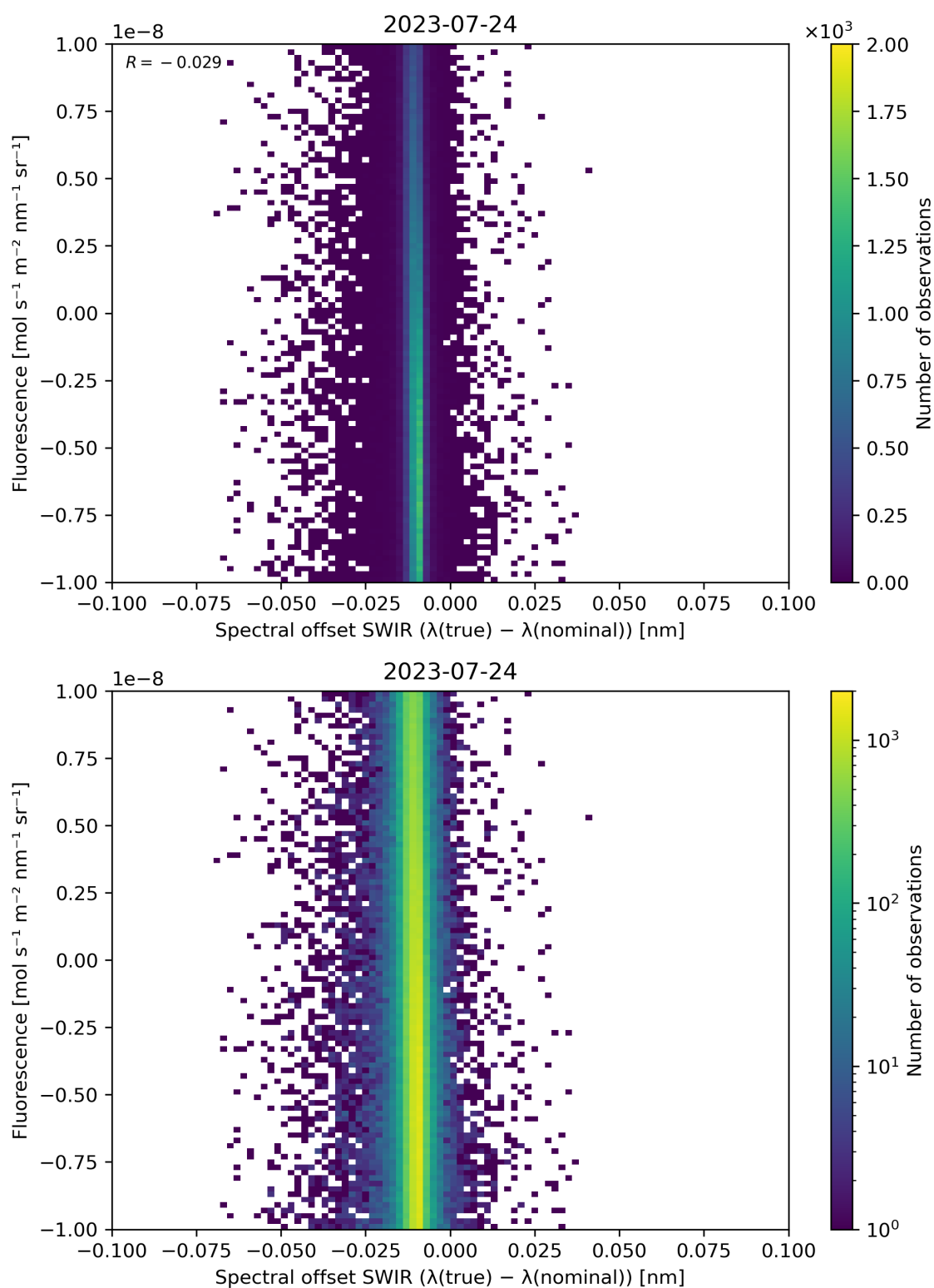
Figure 120: Scatter density plot of “Spectral offset SWIR ( \lambda(\text{true}) - \lambda(\text{nominal}) )” against “Fluorescence” for 2023-07-24 to 2023-07-25.
