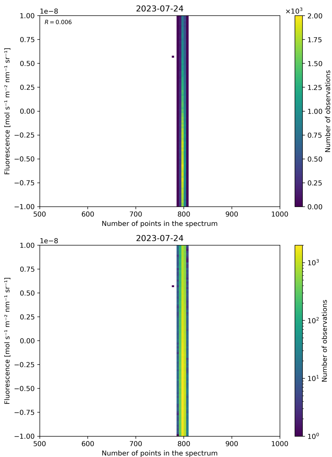
Figure 91: Scatter density plot of “Number of points in the spectrum” against “Fluorescence” for 2023-07-24 to 2023-07-25.
