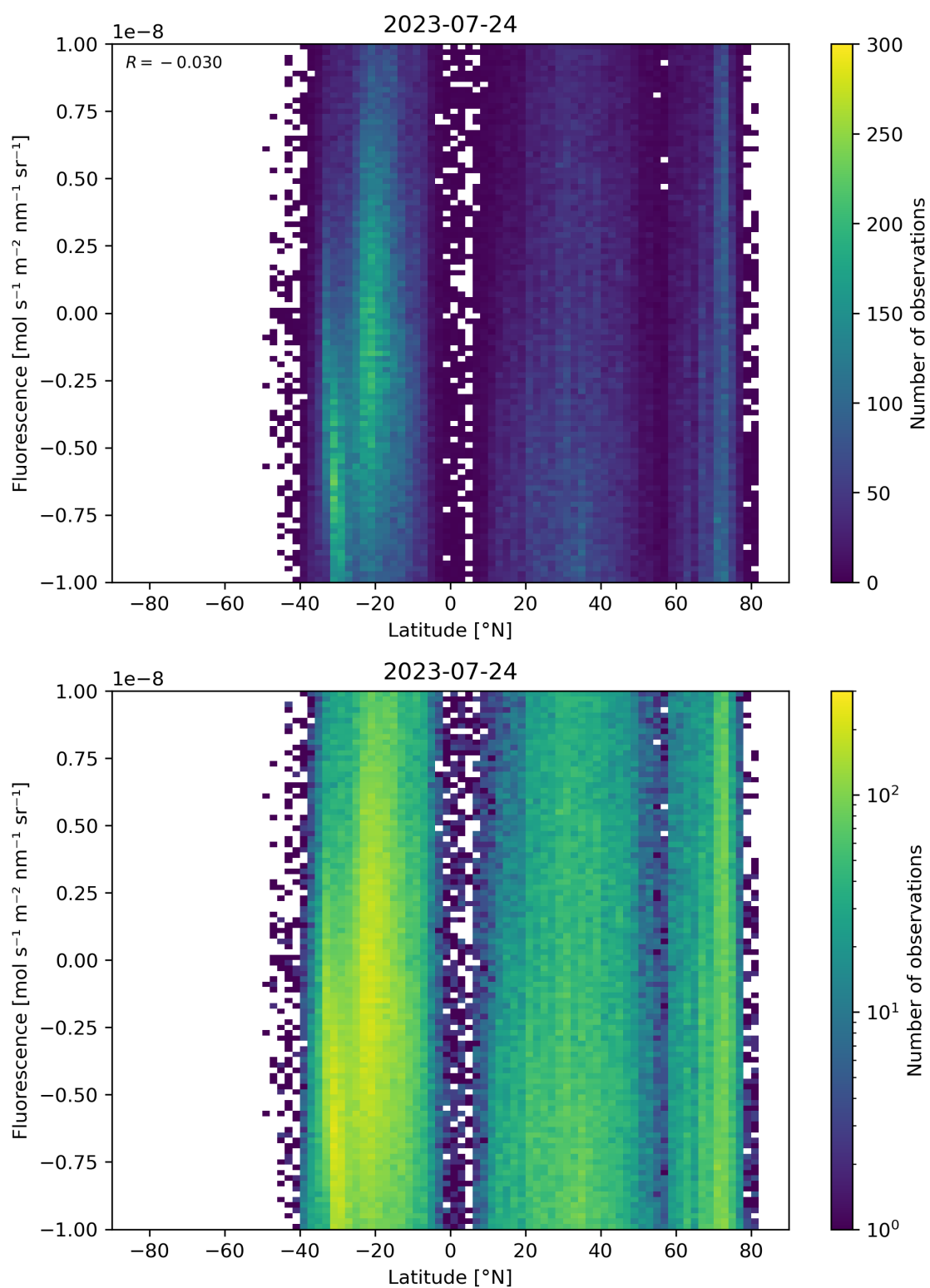
Figure 56: Scatter density plot of “Latitude” against “Fluorescence” for 2023-07-24 to 2023-07-25.
