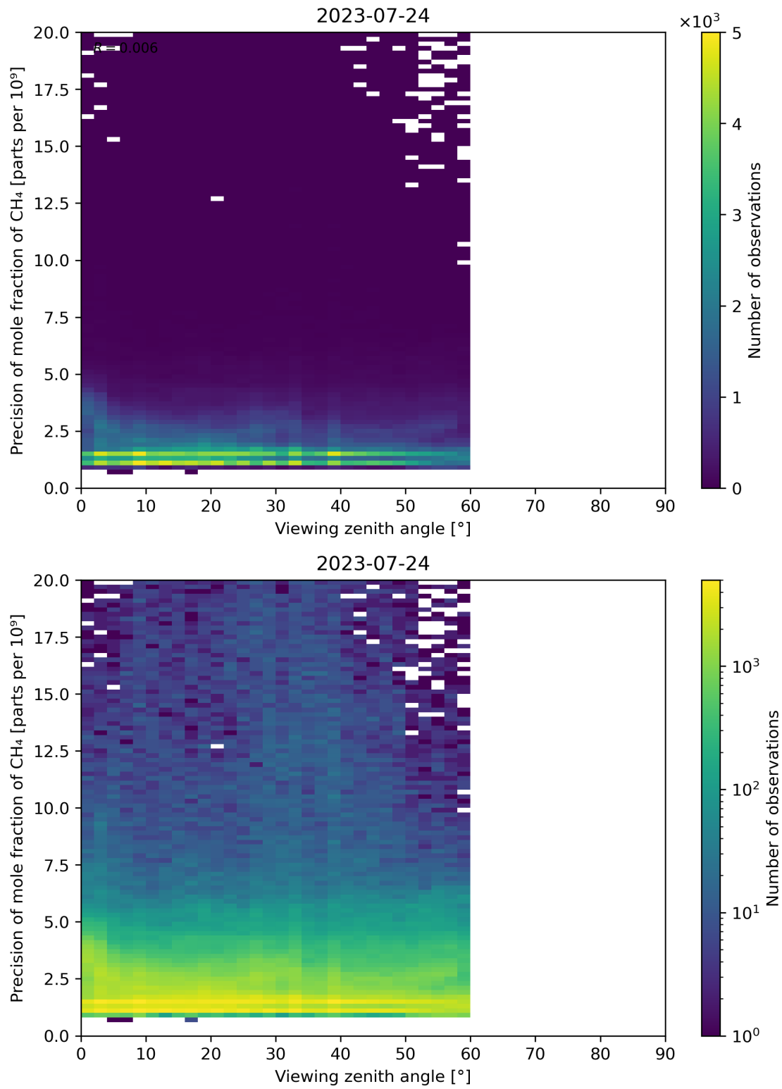
Figure 112: Scatter density plot of “Viewing zenith angle” against “Precision of mole fraction of CH 4 ” for 2023-07-24 to 2023-07-25.
