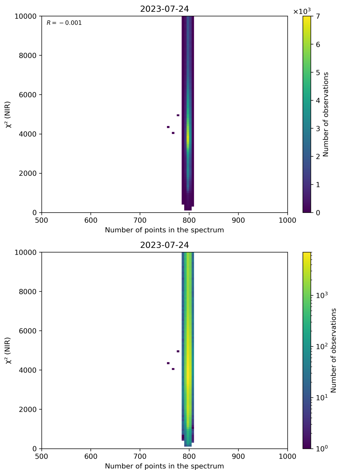
Figure 88: Scatter density plot of “Number of points in the spectrum” against “ \chi^2 (NIR)” for 2023-07-24 to 2023-07-25.
