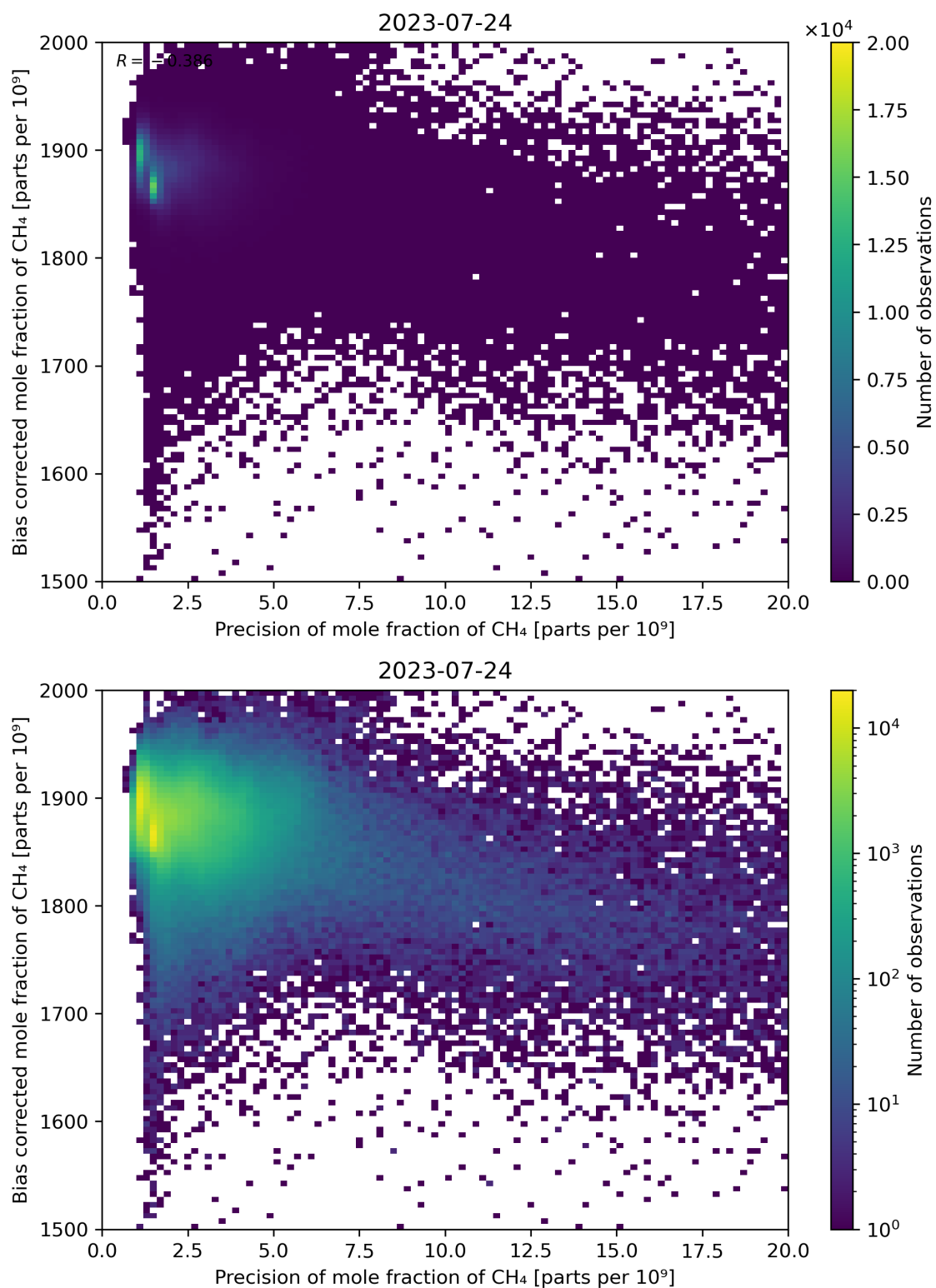
Figure 82: Scatter density plot of “Precision of mole fraction of \text{CH}_4 ” against “Bias corrected mole fraction of \text{CH}_4 ” for 2023-07-24 to 2023-07-25.
