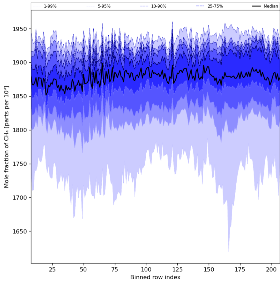
Figure 34: Along track statistics of “Mole fraction of CH 4 ” for 2023-07-24 to 2023-07-25
