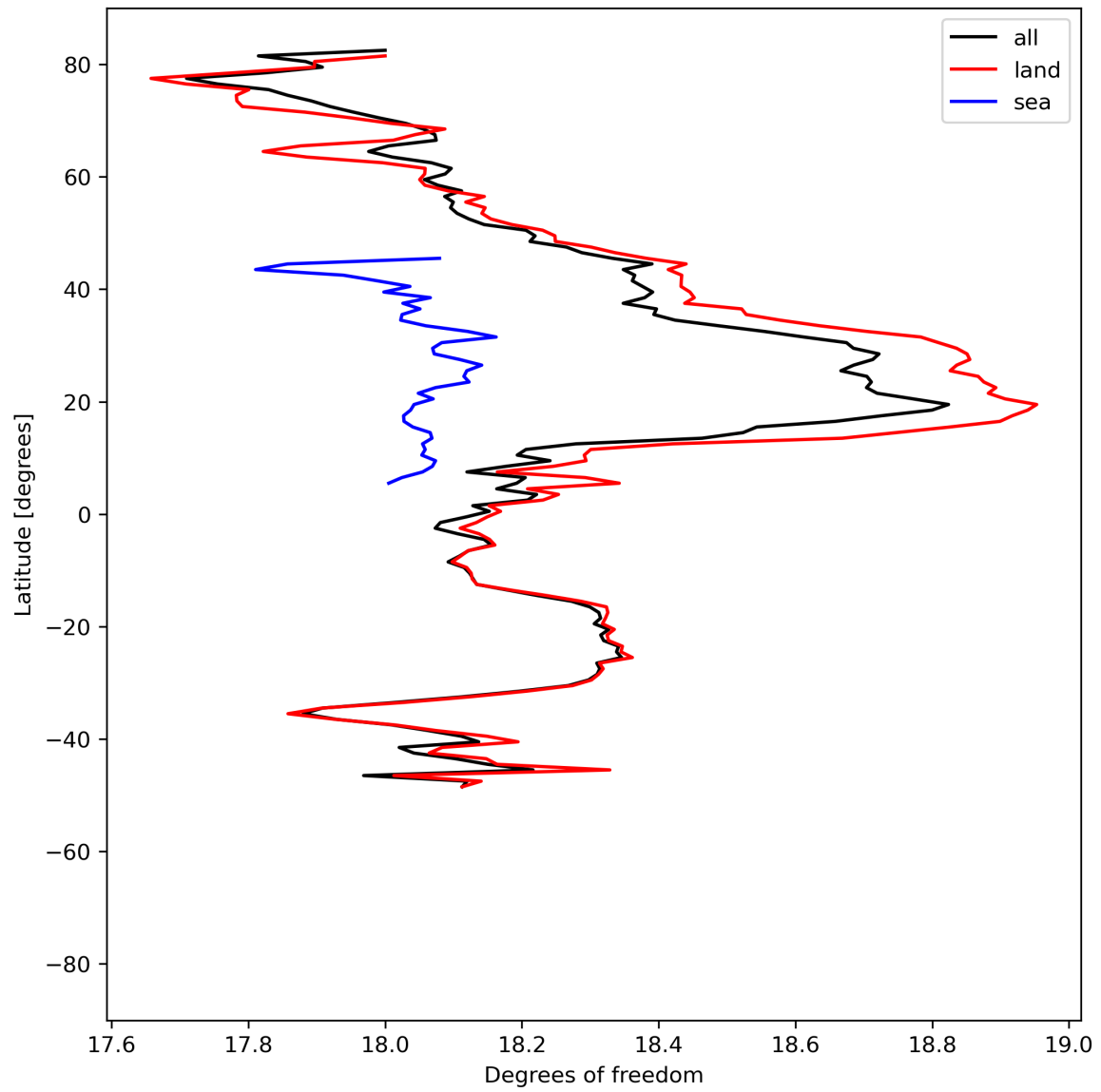
Figure 19: Zonal average of “Degrees of freedom” for 2023-07-24 to 2023-07-25.
