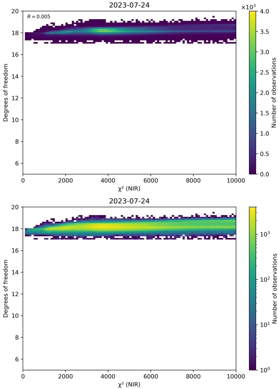
Figure 44: Scatter density plot of “ \chi^2 (NIR)” against “Degrees of freedom” for 2023-07-24 to 2023-07-25.
