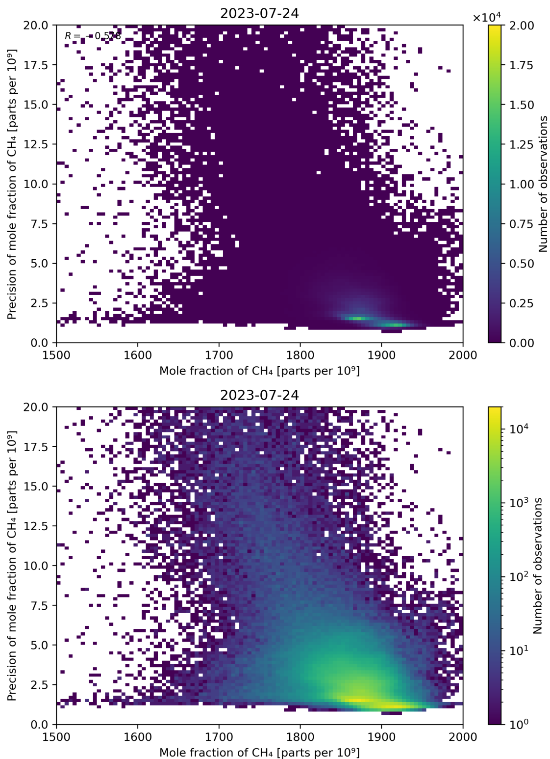
Figure 75: Scatter density plot of “Mole fraction of CH 4 ” against “Precision of mole fraction of CH 4 ” for 2023-07-24 to 2023-07-25.
