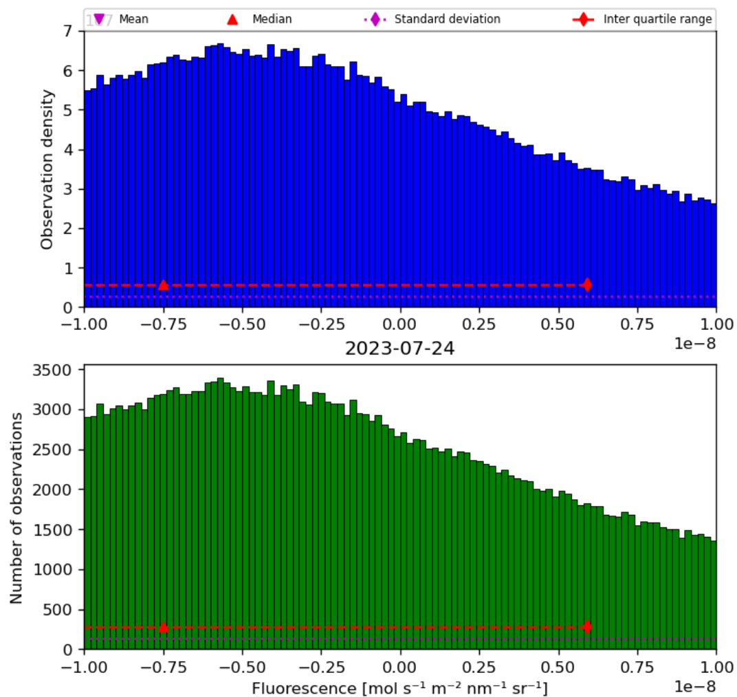
Figure 32: Histogram of “Fluorescence” for 2023-07-24 to 2023-07-25
