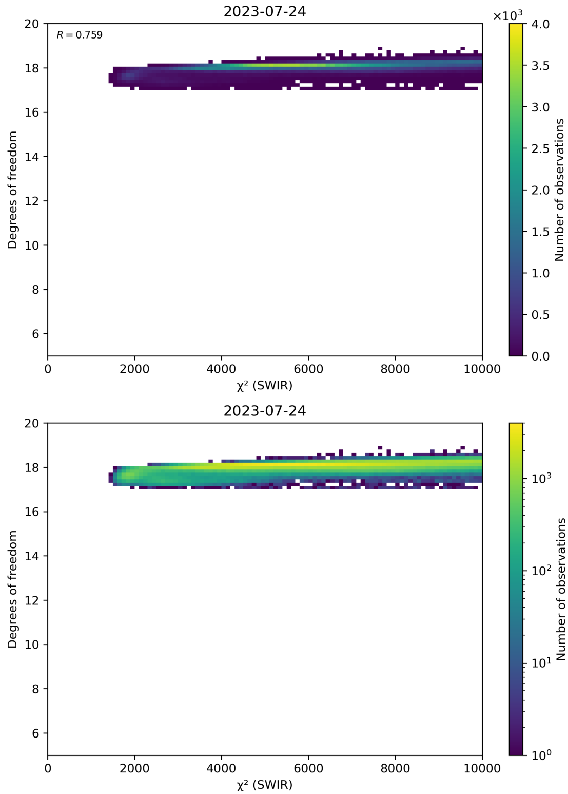
Figure 48: Scatter density plot of “ \chi^2 (SWIR)” against “Degrees of freedom” for 2023-07-24 to 2023-07-25.
