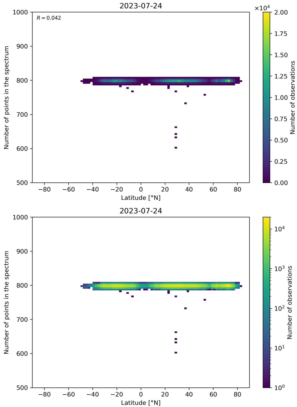
Figure 61: Scatter density plot of “Latitude” against “Number of points in the spectrum” for 2023-07-24 to 2023-07-25.
