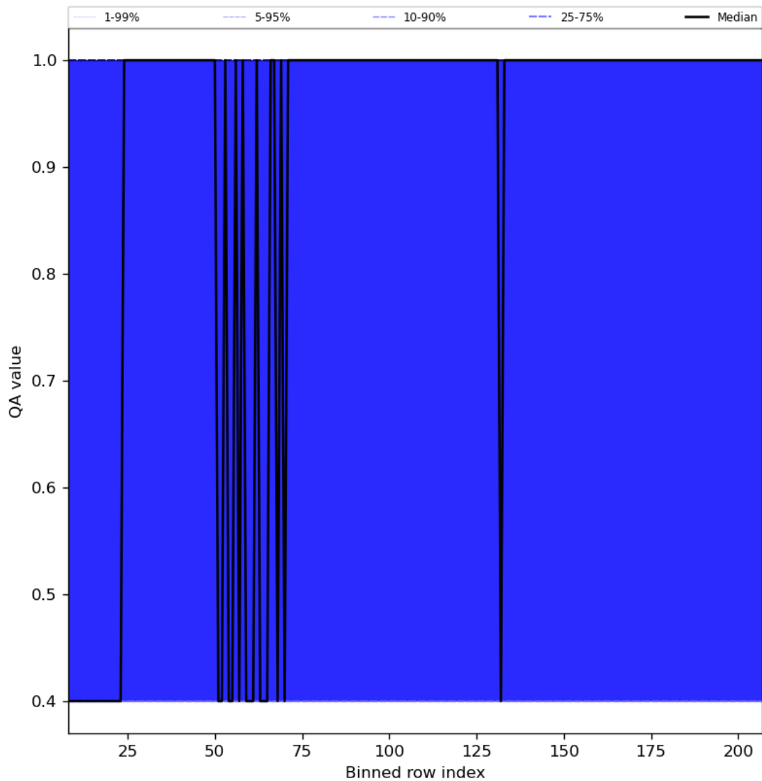
Figure 33: Along track statistics of “QA value” for 2023-07-24 to 2023-07-25
