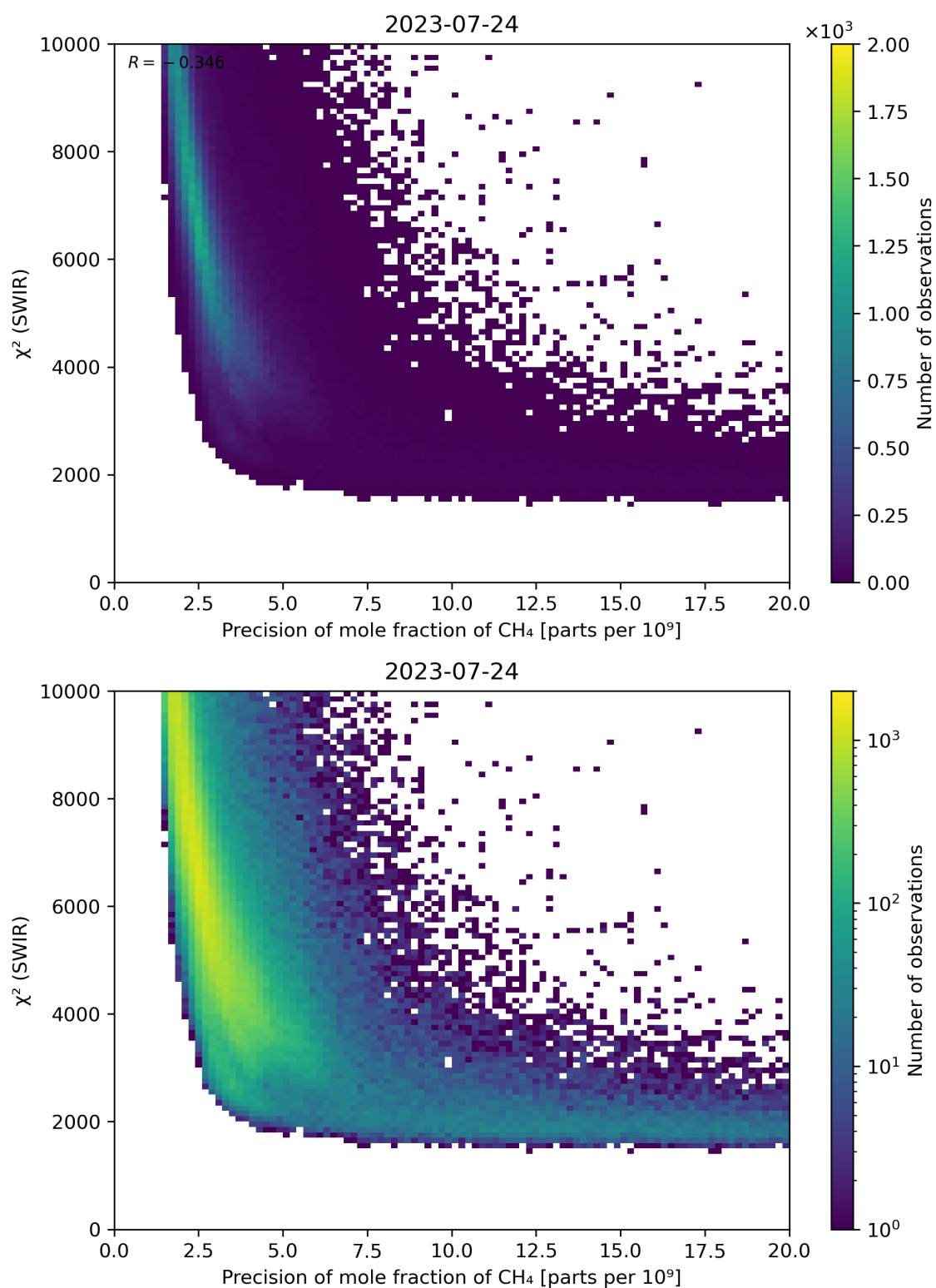
Figure 79: Scatter density plot of “Precision of mole fraction of \text{CH}_4 ” against “ \chi^2 (SWIR)” for 2023-07-24 to 2023-07-25.
