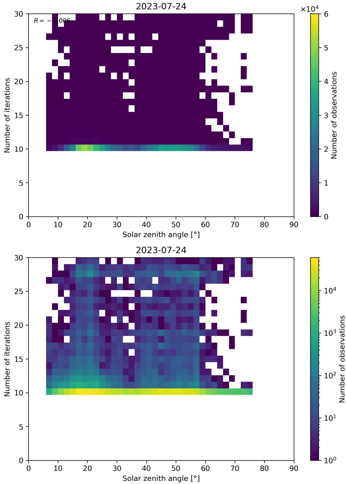
Figure 102: Scatter density plot of “Solar zenith angle” against “Number of iterations” for 2023-07-24 to 2023-07-25.
