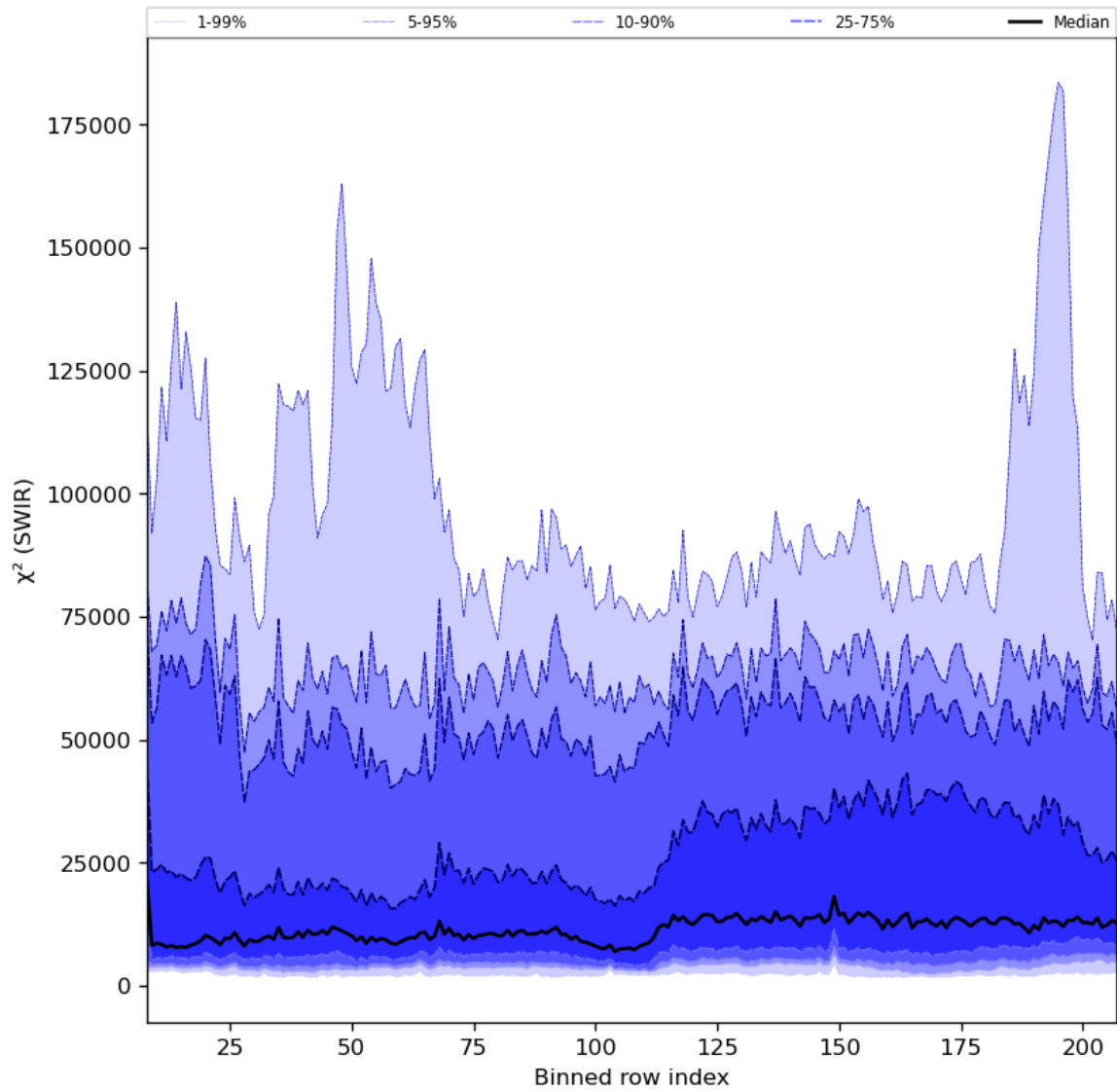
Figure 39: Along track statistics of “ \chi^2 (SWIR)” for 2023-07-24 to 2023-07-25
