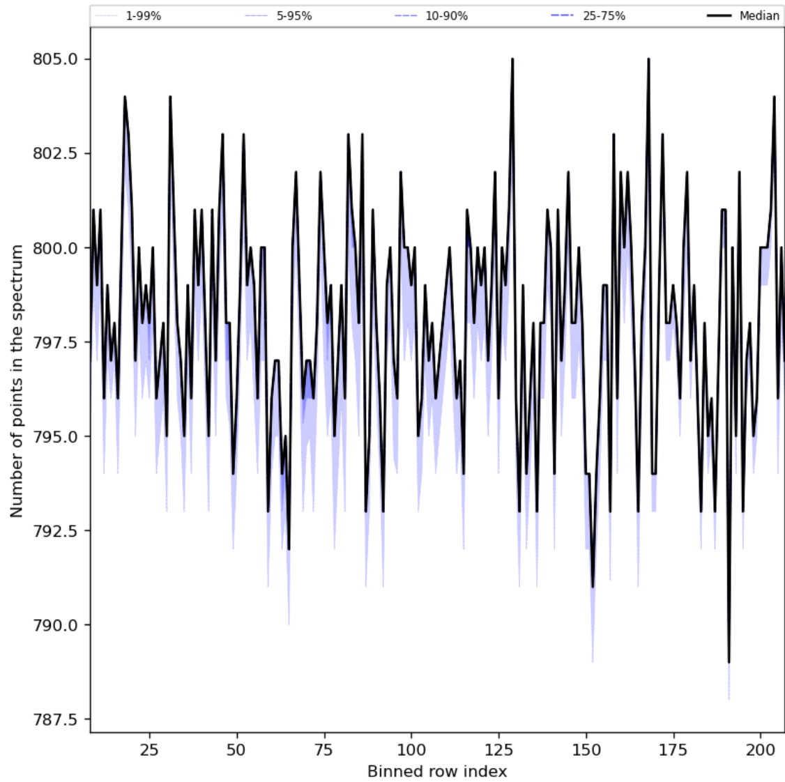
Figure 37: Along track statistics of “Number of points in the spectrum” for 2023-07-24 to 2023-07-25
