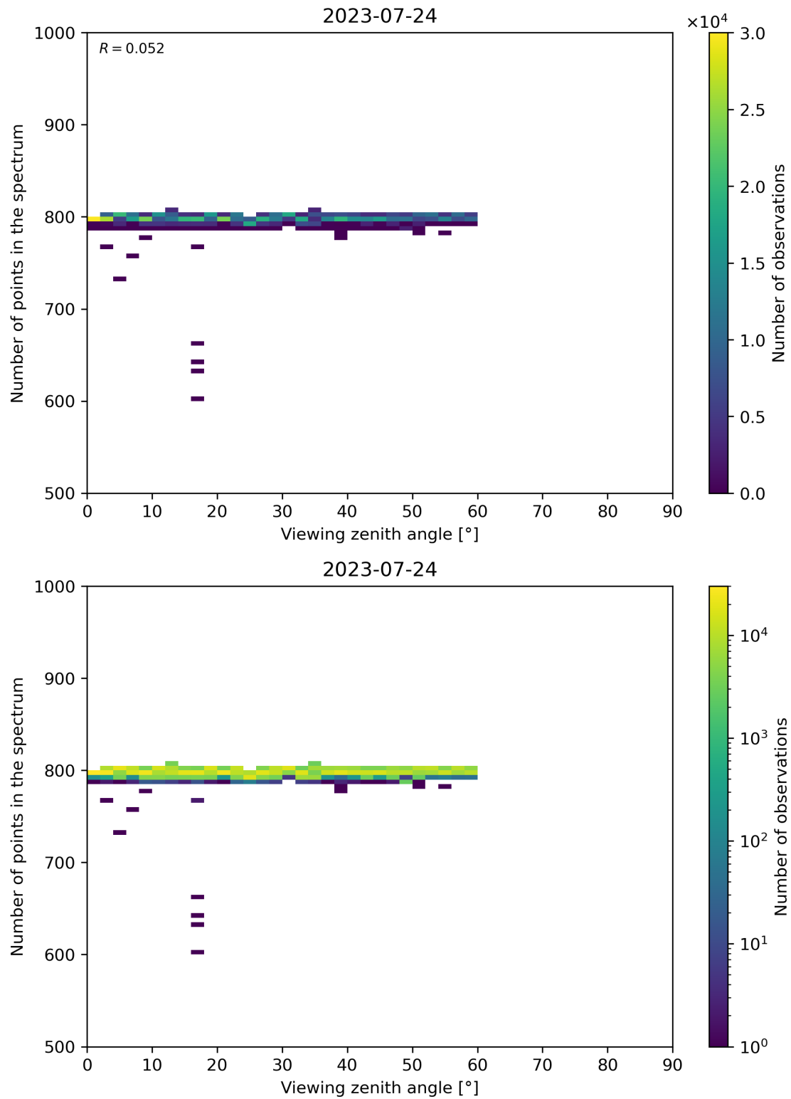
Figure 114: Scatter density plot of “Viewing zenith angle” against “Number of points in the spectrum” for 2023-07-24 to 2023-07-25.
