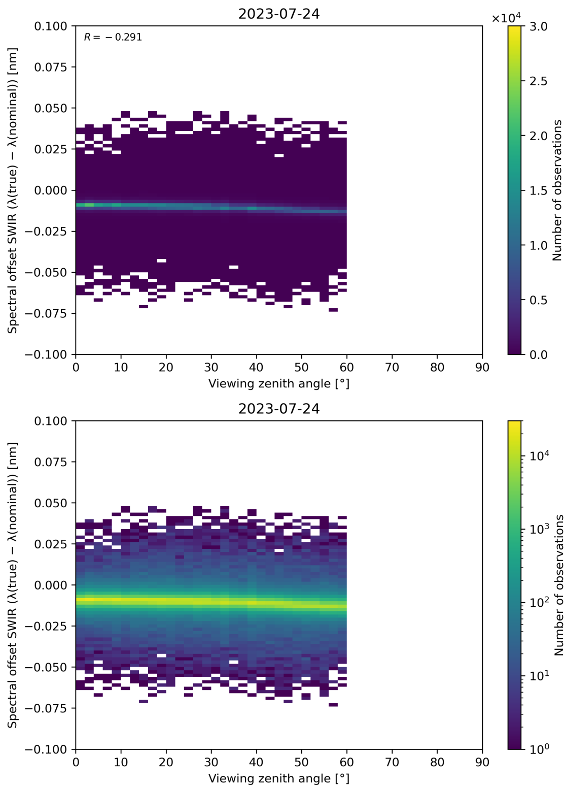
Figure 116: Scatter density plot of “Viewing zenith angle” against “Spectral offset SWIR ( \lambda(\text{true}) - \lambda(\text{nominal}) )” for 2023-07-24 to 2023-07-25.
