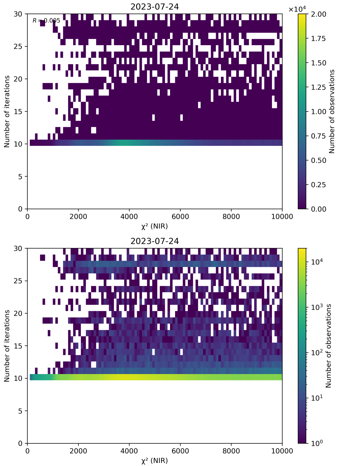
Figure 46: Scatter density plot of “ \chi^2 (NIR)” against “Number of iterations” for 2023-07-24 to 2023-07-25.
