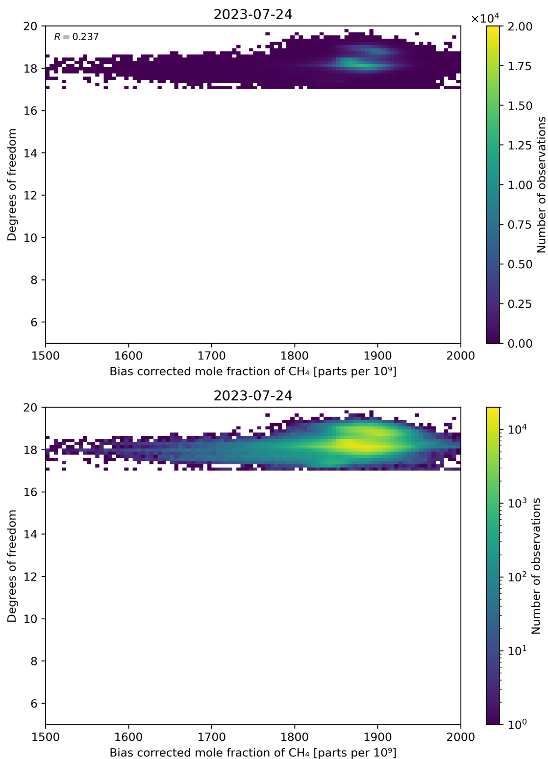
Figure 65: Scatter density plot of “Bias corrected mole fraction of CH 4 ” against “Degrees of freedom” for 2023-07-24 to 2023-07-25.
