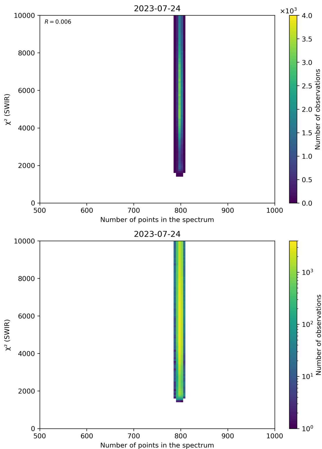
Figure 89: Scatter density plot of “Number of points in the spectrum” against “ \chi^2 (SWIR)” for 2023-07-24 to 2023-07-25.
