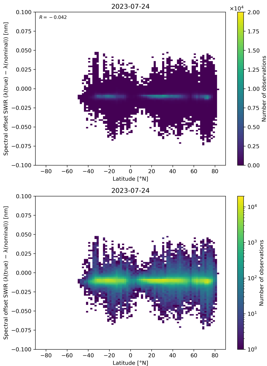
Figure 62: Scatter density plot of “Latitude” against “Spectral offset SWIR ( \lambda(\text{true}) - \lambda(\text{nominal}) )” for 2023-07-24 to 2023-07-25.
