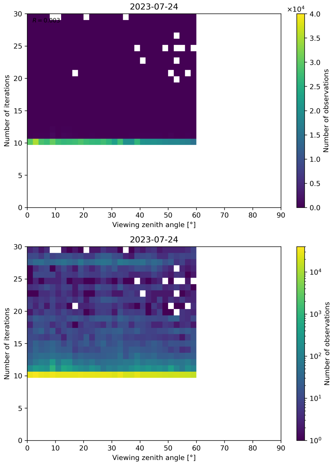
Figure 113: Scatter density plot of “Viewing zenith angle” against “Number of iterations” for 2023-07-24 to 2023-07-25.
