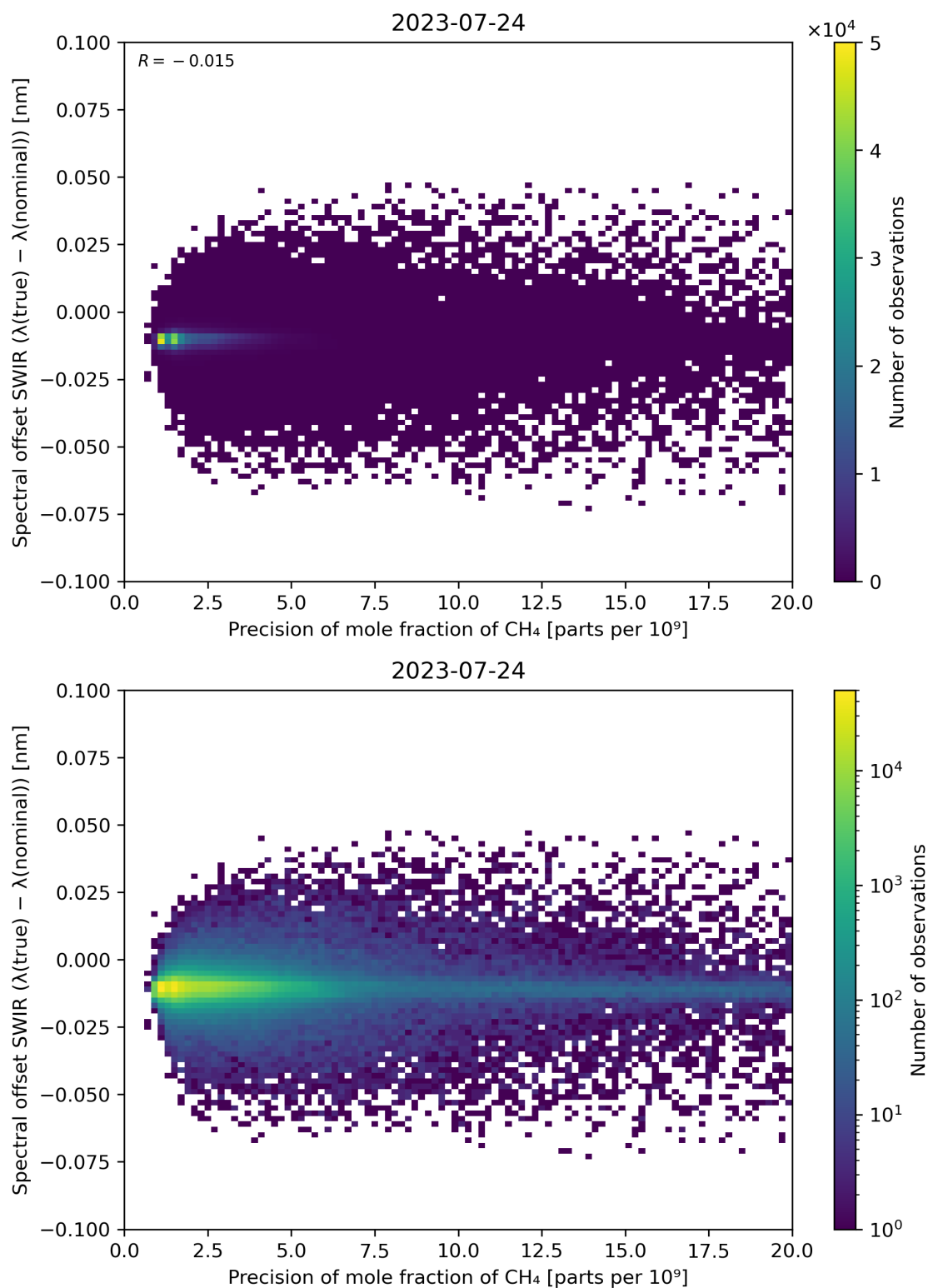
Figure 85: Scatter density plot of “Precision of mole fraction of CH 4 ” against “Spectral offset SWIR ( \lambda(\text{true}) - \lambda(\text{nominal}) )” for 2023-07-24 to 2023-07-25.
