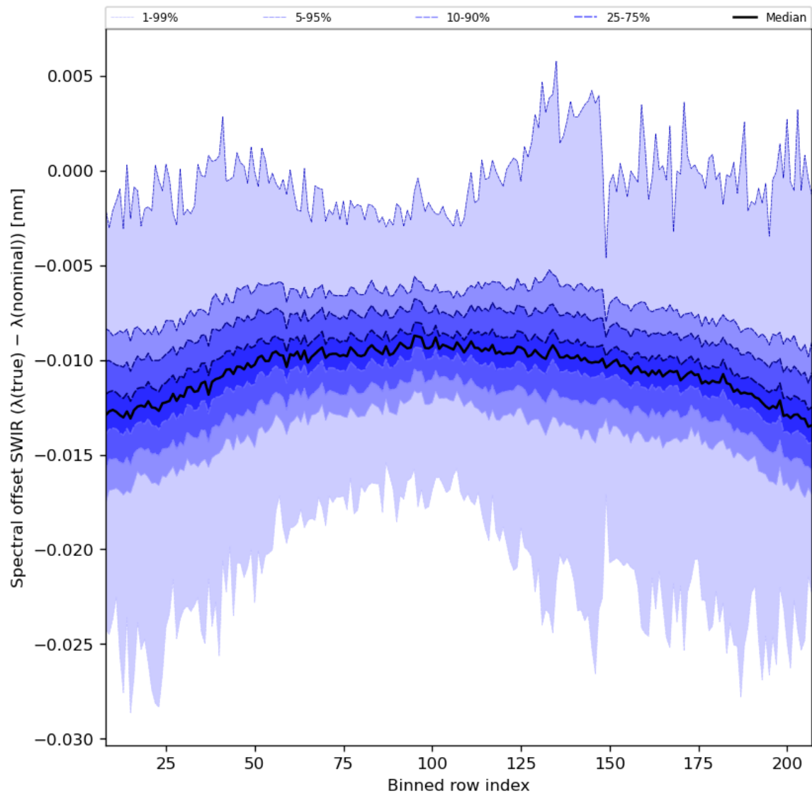
Figure 38: Along track statistics of "Spectral offset SWIR ( \lambda(\text{true}) - \lambda(\text{nominal}) )" for 2023-07-24 to 2023-07-25
