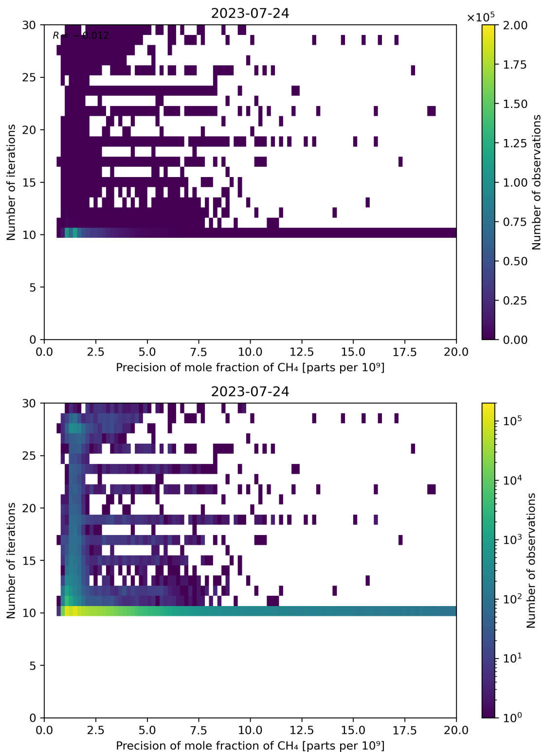
Figure 83: Scatter density plot of “Precision of mole fraction of CH 4 ” against “Number of iterations” for 2023-07-24 to 2023-07-25.
