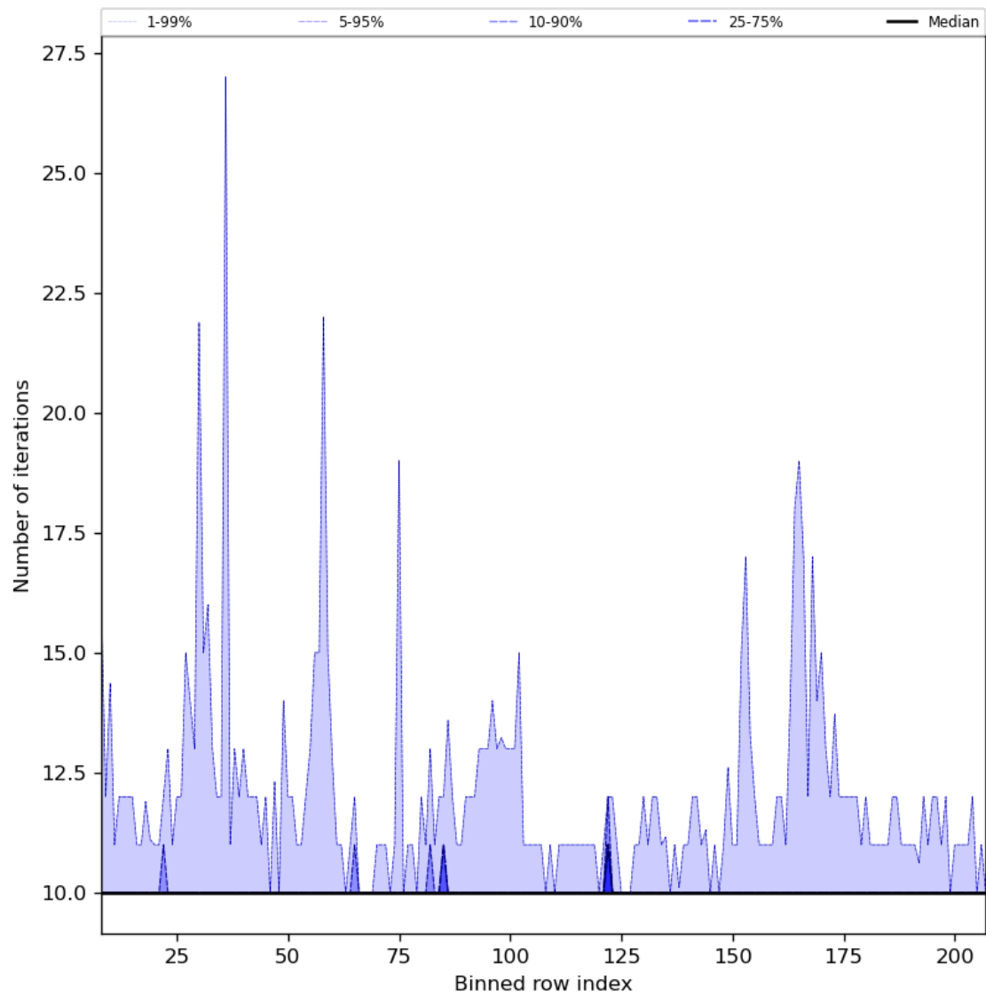
Figure 42: Along track statistics of “Number of iterations” for 2023-07-24 to 2023-07-25
