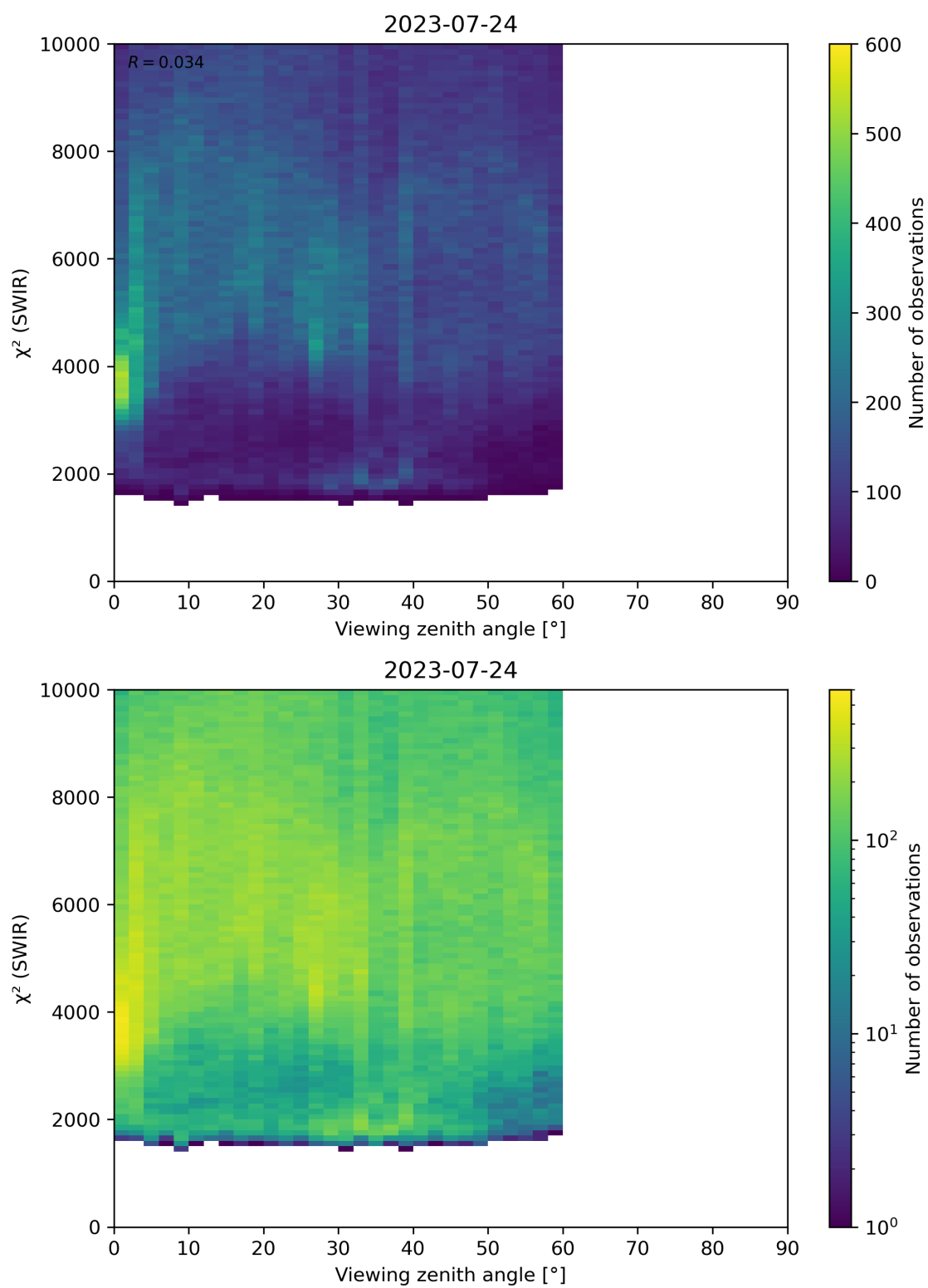
Figure 106: Scatter density plot of “Viewing zenith angle” against “ \chi^2 (SWIR)” for 2023-07-24 to 2023-07-25.
