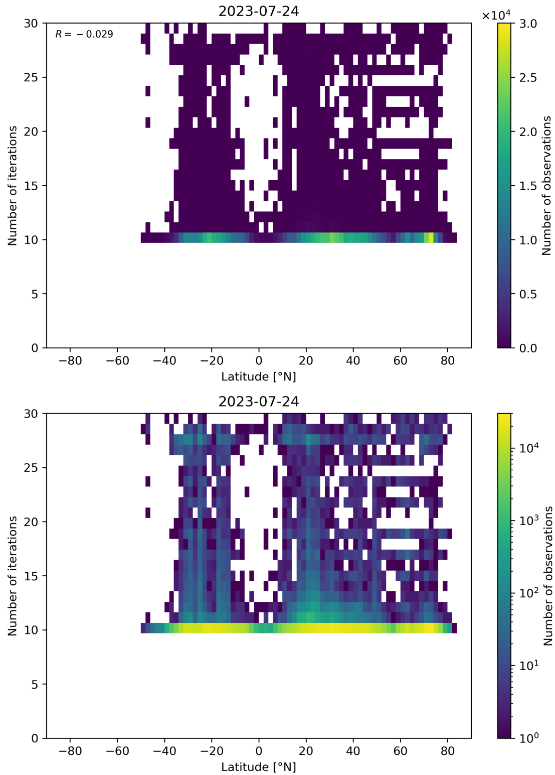
Figure 60: Scatter density plot of “Latitude” against “Number of iterations” for 2023-07-24 to 2023-07-25.
