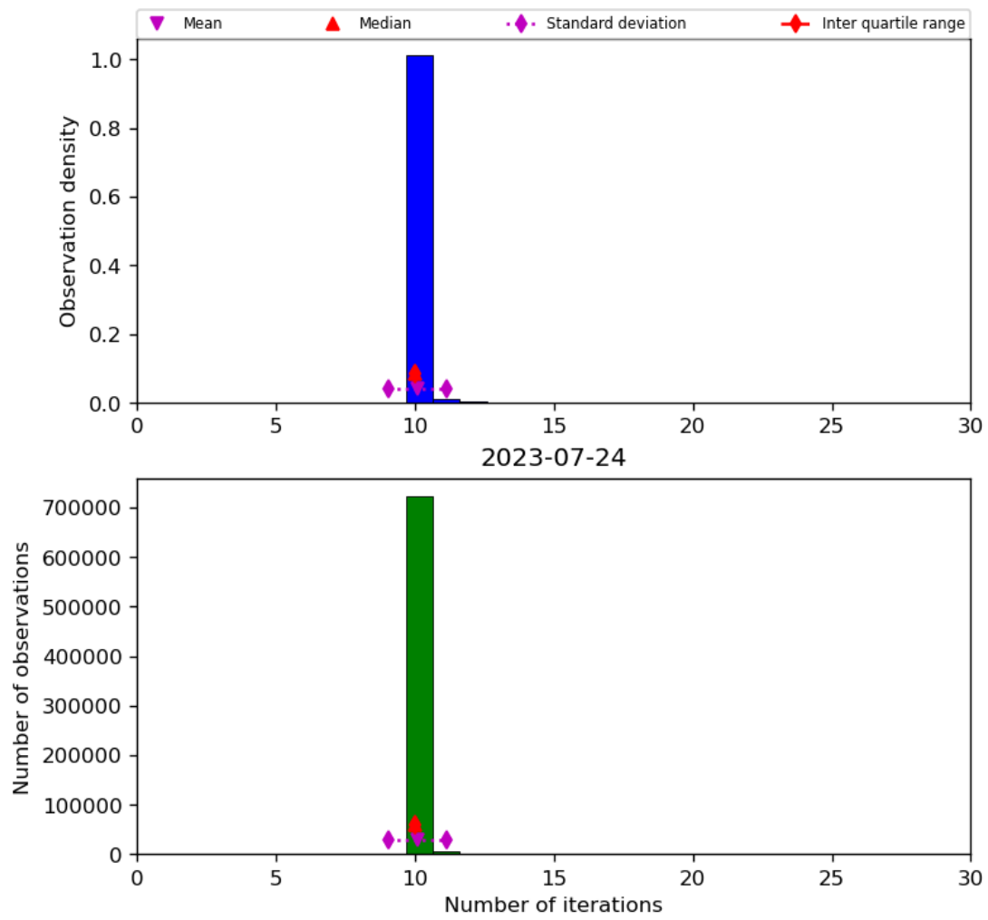
Figure 31: Histogram of “Number of iterations” for 2023-07-24 to 2023-07-25
