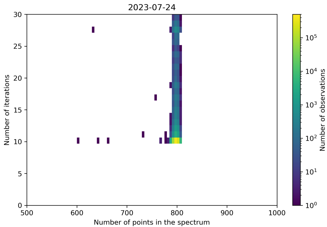
Figure 92: Scatter density plot of “Number of points in the spectrum” against “Number of iterations” for 2023-07-24 to 2023-07-25.
