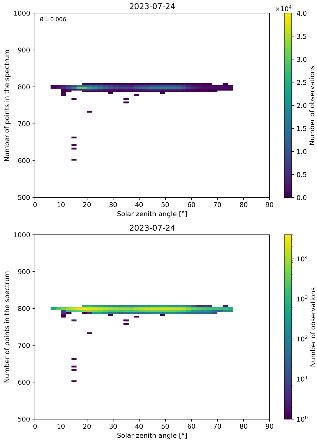
Figure 103: Scatter density plot of “Solar zenith angle” against “Number of points in the spectrum” for 2023-07-24 to 2023-07-25.
