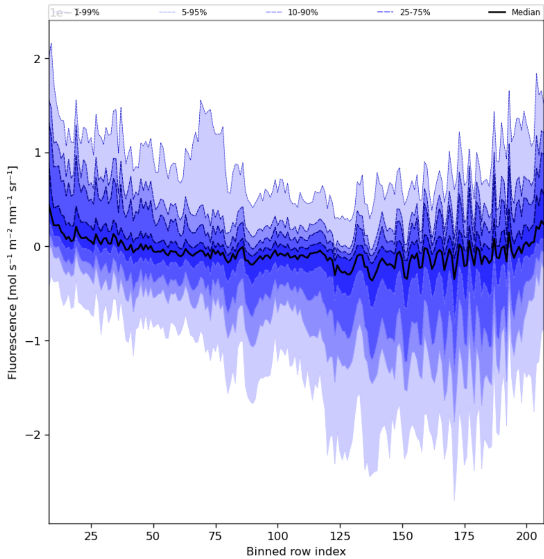
Figure 43: Along track statistics of “Fluorescence” for 2023-07-24 to 2023-07-25
