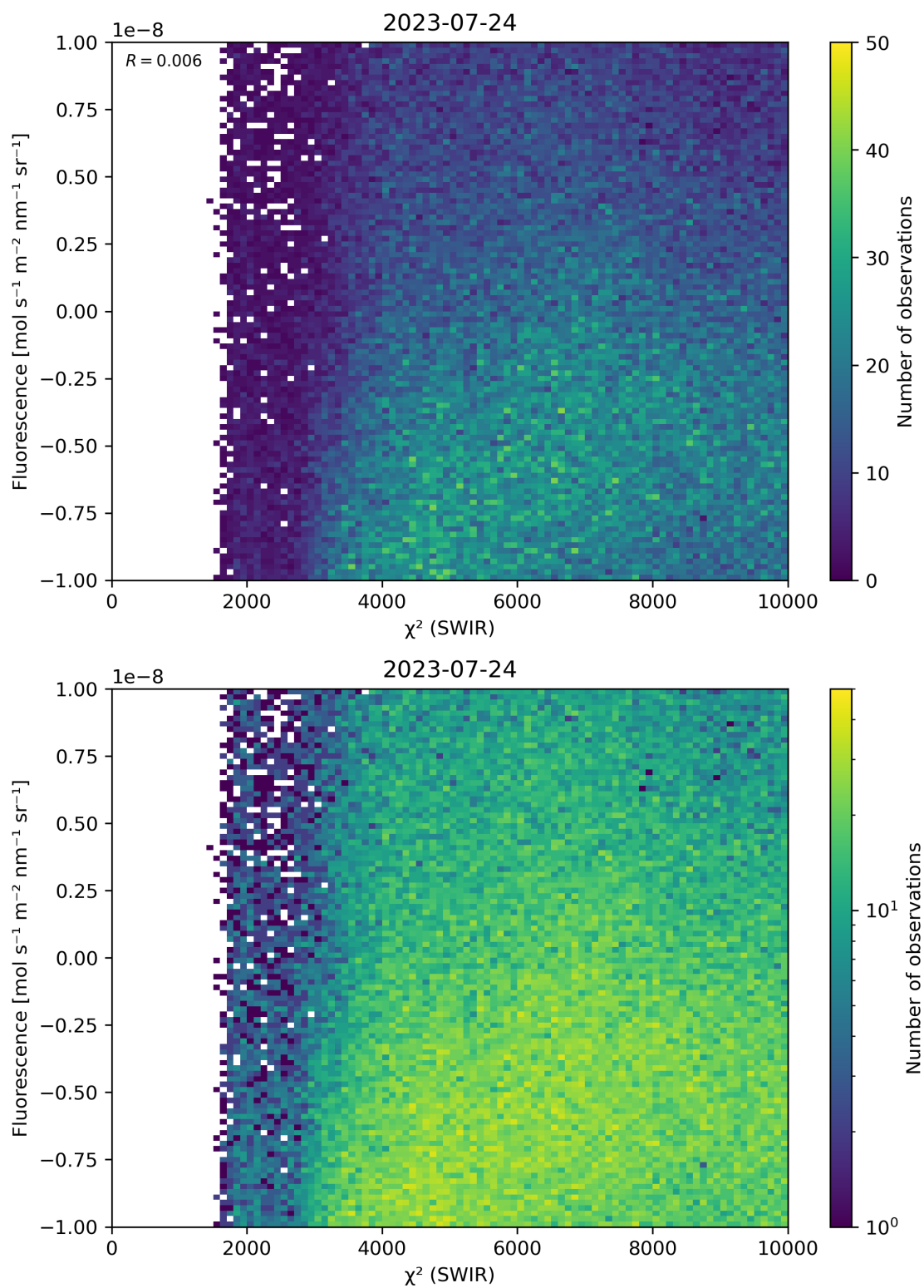
Figure 49: Scatter density plot of “ \chi^2 (SWIR)” against “Fluorescence” for 2023-07-24 to 2023-07-25.
