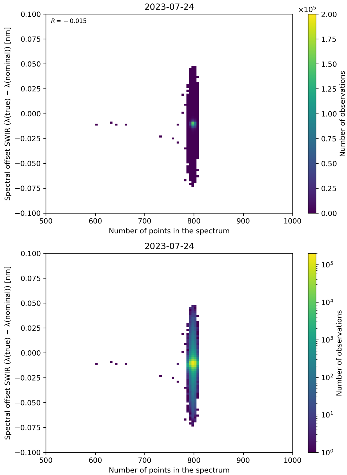
Figure 93: Scatter density plot of “Number of points in the spectrum” against “Spectral offset SWIR ( \lambda(\text{true}) - \lambda(\text{nominal}) )” for 2023-07-24 to 2023-07-25.
