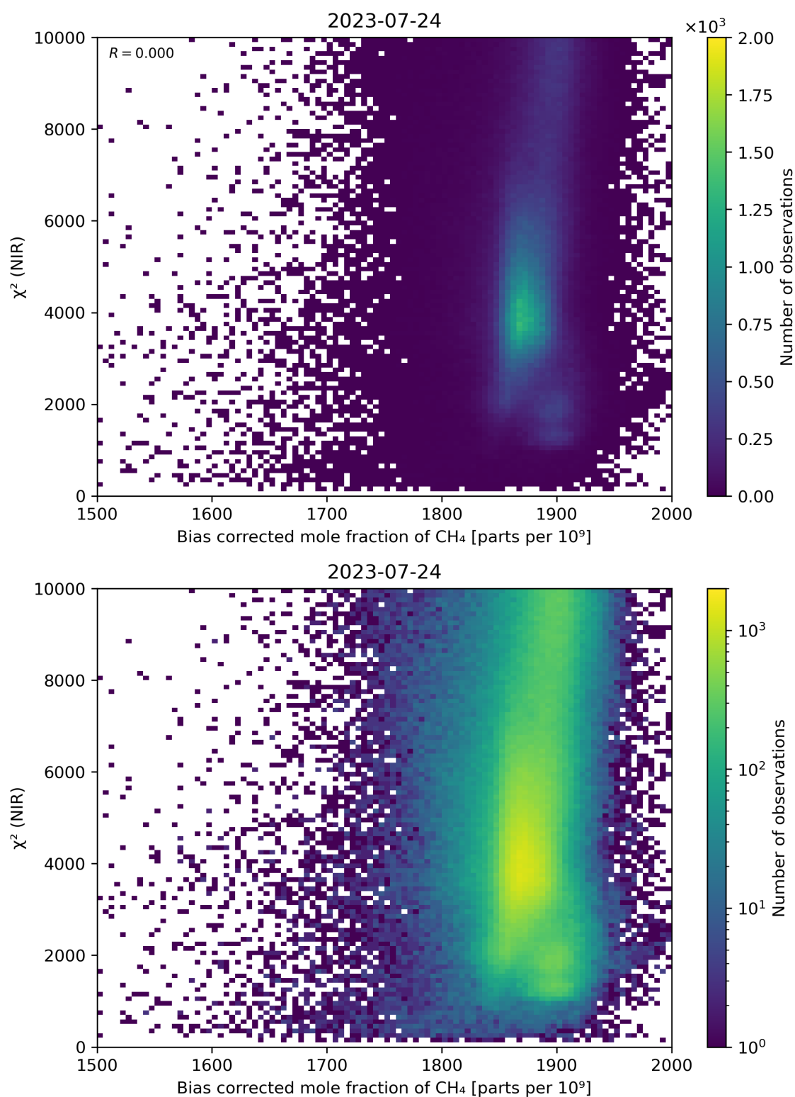
Figure 63: Scatter density plot of “Bias corrected mole fraction of \text{CH}_4 ” against “ \chi^2 (NIR)” for 2023-07-24 to 2023-07-25.
