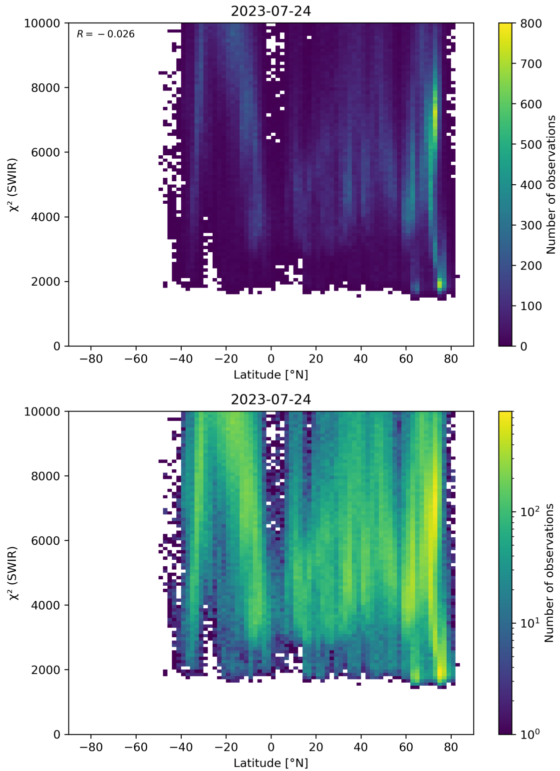
Figure 54: Scatter density plot of “Latitude” against “ \chi^2 (SWIR)” for 2023-07-24 to 2023-07-25.
