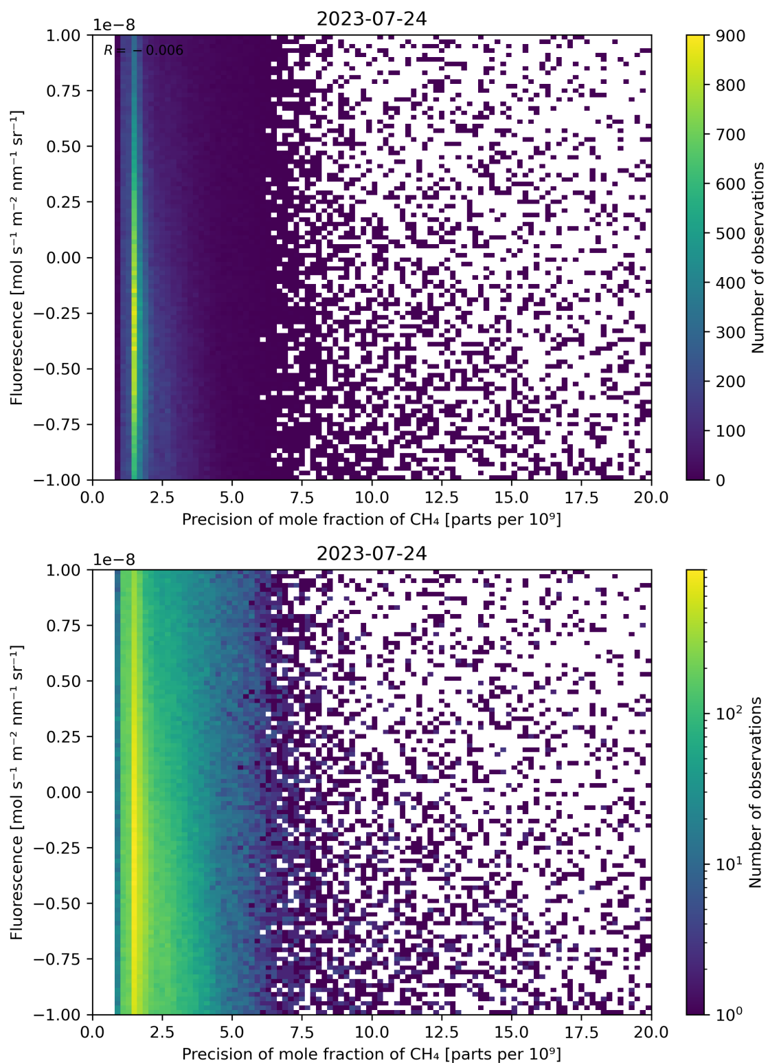
Figure 81: Scatter density plot of “Precision of mole fraction of \text{CH}_4 ” against “Fluorescence” for 2023-07-24 to 2023-07-25.
