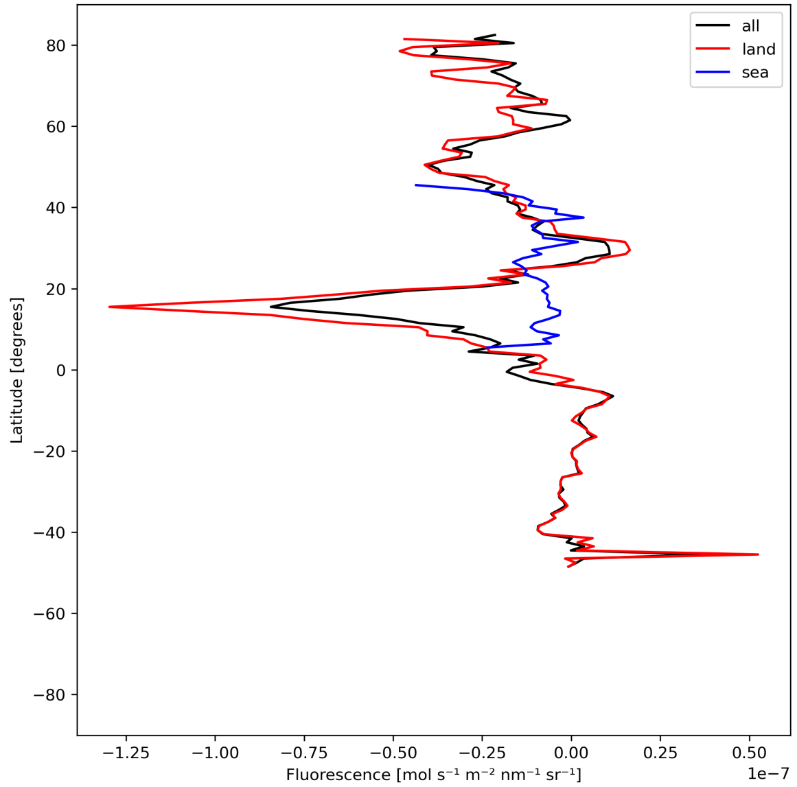
Figure 21: Zonal average of “Fluorescence” for 2023-07-24 to 2023-07-25.
