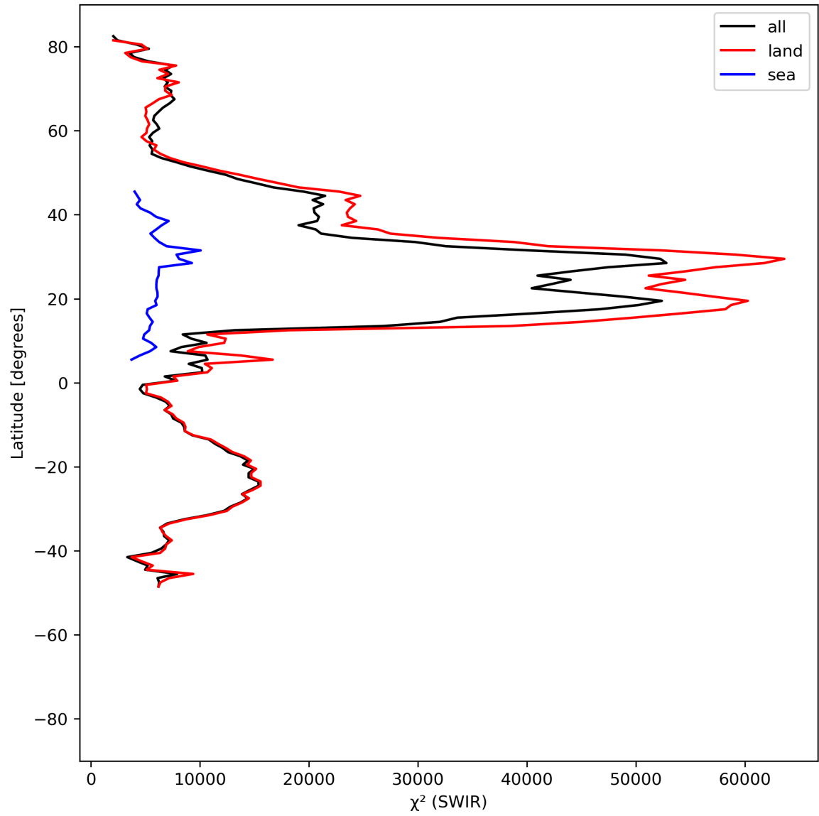
Figure 17: Zonal average of “ \chi^2 (SWIR)” for 2023-07-24 to 2023-07-25.
