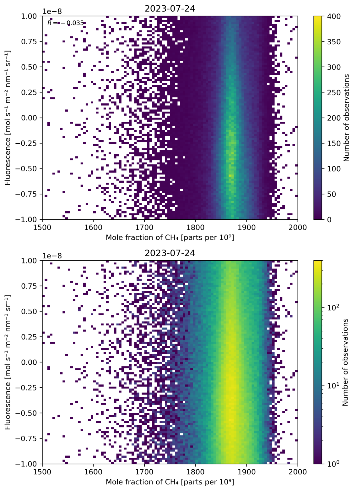
Figure 73: Scatter density plot of “Mole fraction of \text{CH}_4 ” against “Fluorescence” for 2023-07-24 to 2023-07-25.
