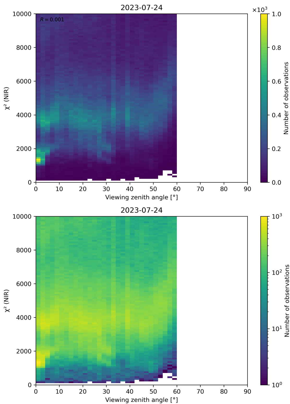
Figure 105: Scatter density plot of “Viewing zenith angle” against “ \chi^2 (NIR)” for 2023-07-24 to 2023-07-25.
