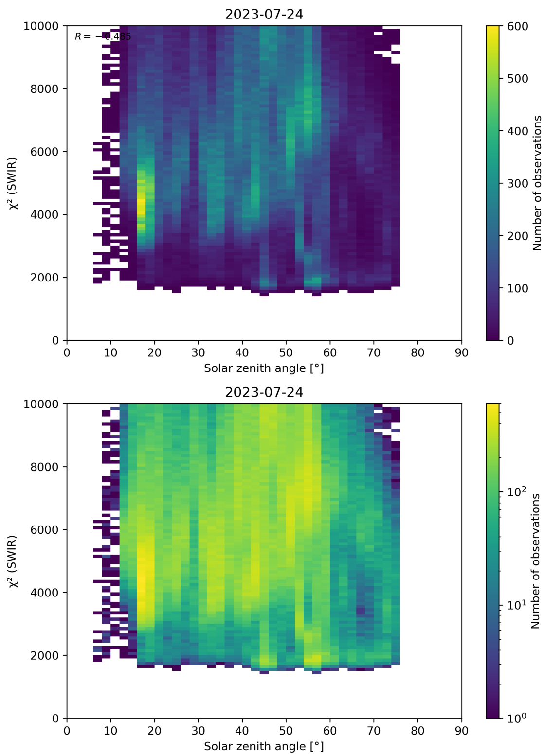
Figure 95: Scatter density plot of “Solar zenith angle” against “ \chi^2 (SWIR)” for 2023-07-24 to 2023-07-25.
