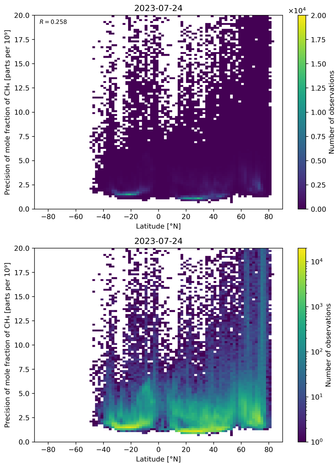
Figure 59: Scatter density plot of “Latitude” against “Precision of mole fraction of \text{CH}_4 ” for 2023-07-24 to 2023-07-25.
