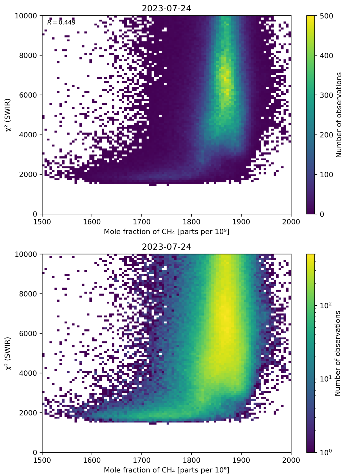
Figure 71: Scatter density plot of “Mole fraction of \text{CH}_4 ” against “ \chi^2 (SWIR)” for 2023-07-24 to 2023-07-25.
