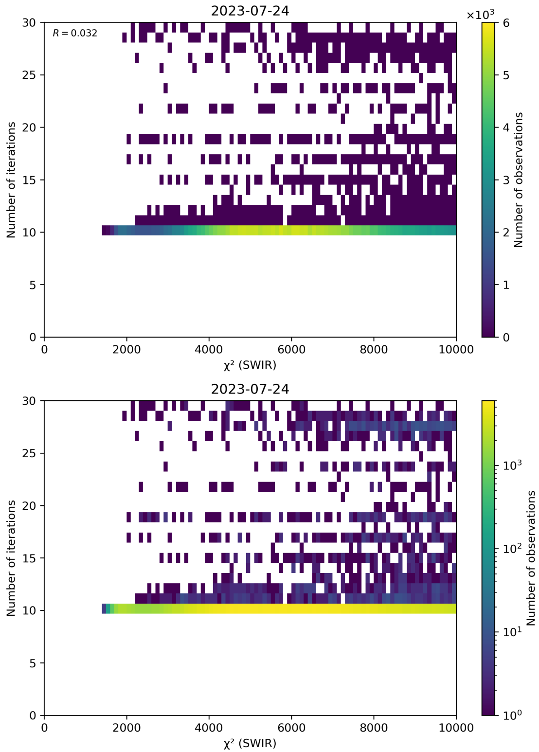
Figure 50: Scatter density plot of “ \chi^2 (SWIR)” against “Number of iterations” for 2023-07-24 to 2023-07-25.
