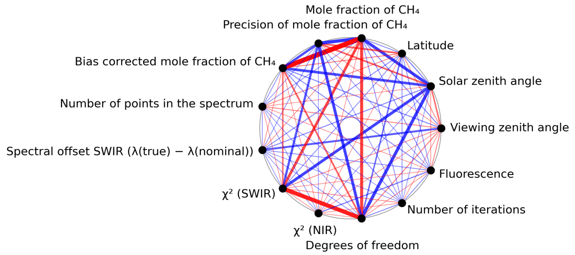
Figure 1: Map of correlation graph for 2023-07-24 to 2023-07-25.
