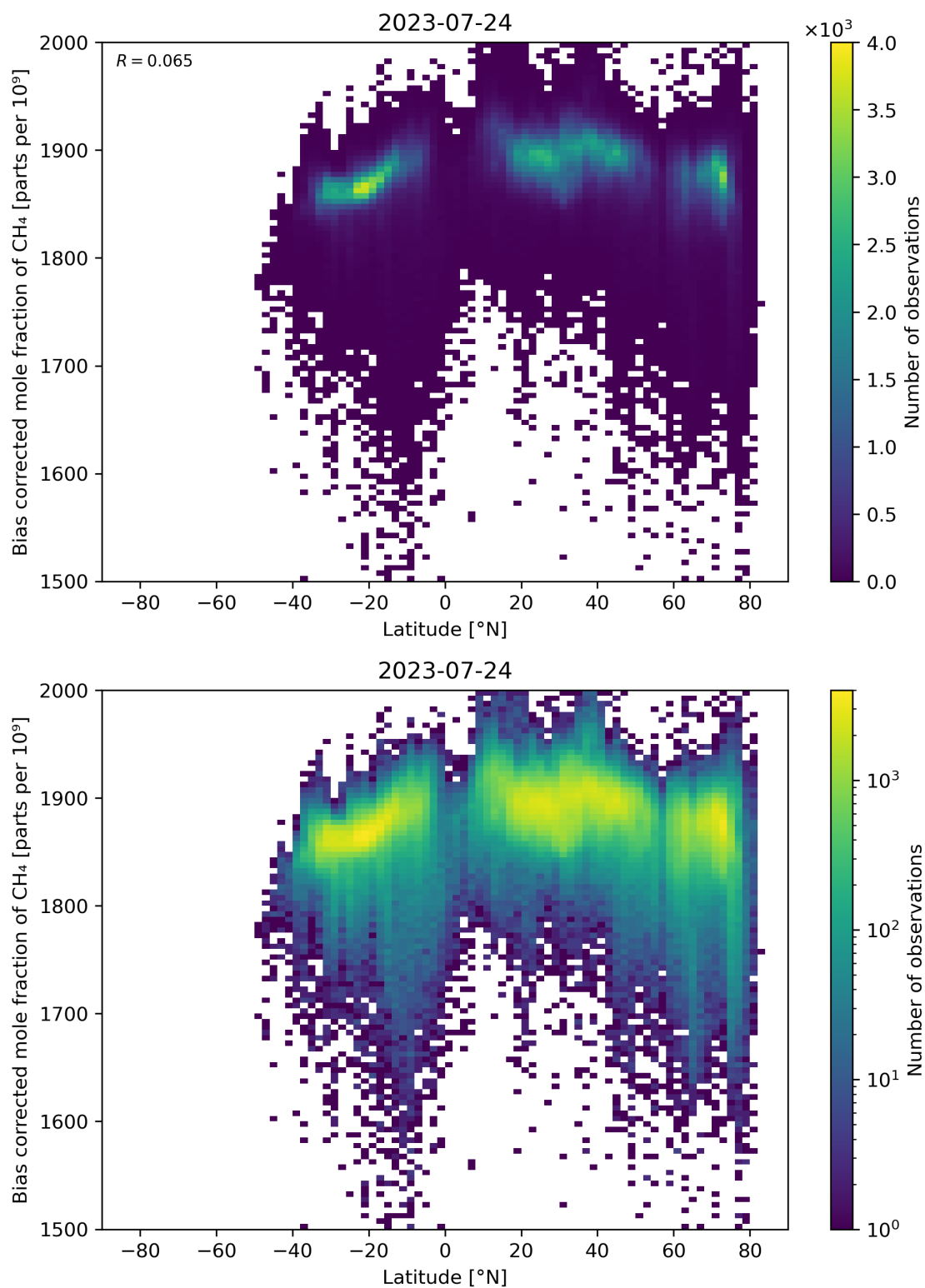
Figure 58: Scatter density plot of “Latitude” against “Bias corrected mole fraction of \text{CH}_4 ” for 2023-07-24 to 2023-07-25.
