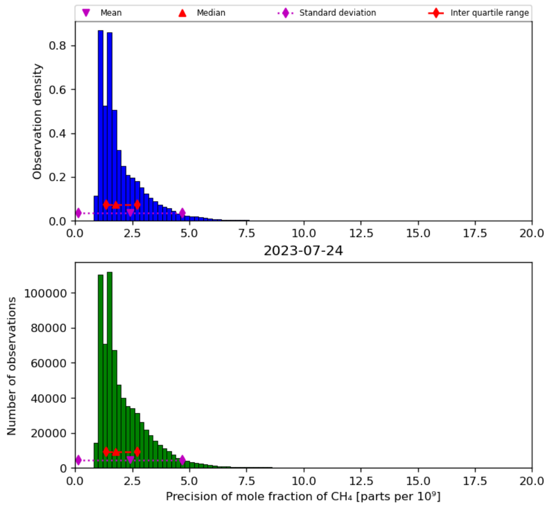
Figure 24: Histogram of “Precision of mole fraction of CH 4 ” for 2023-07-24 to 2023-07-25
