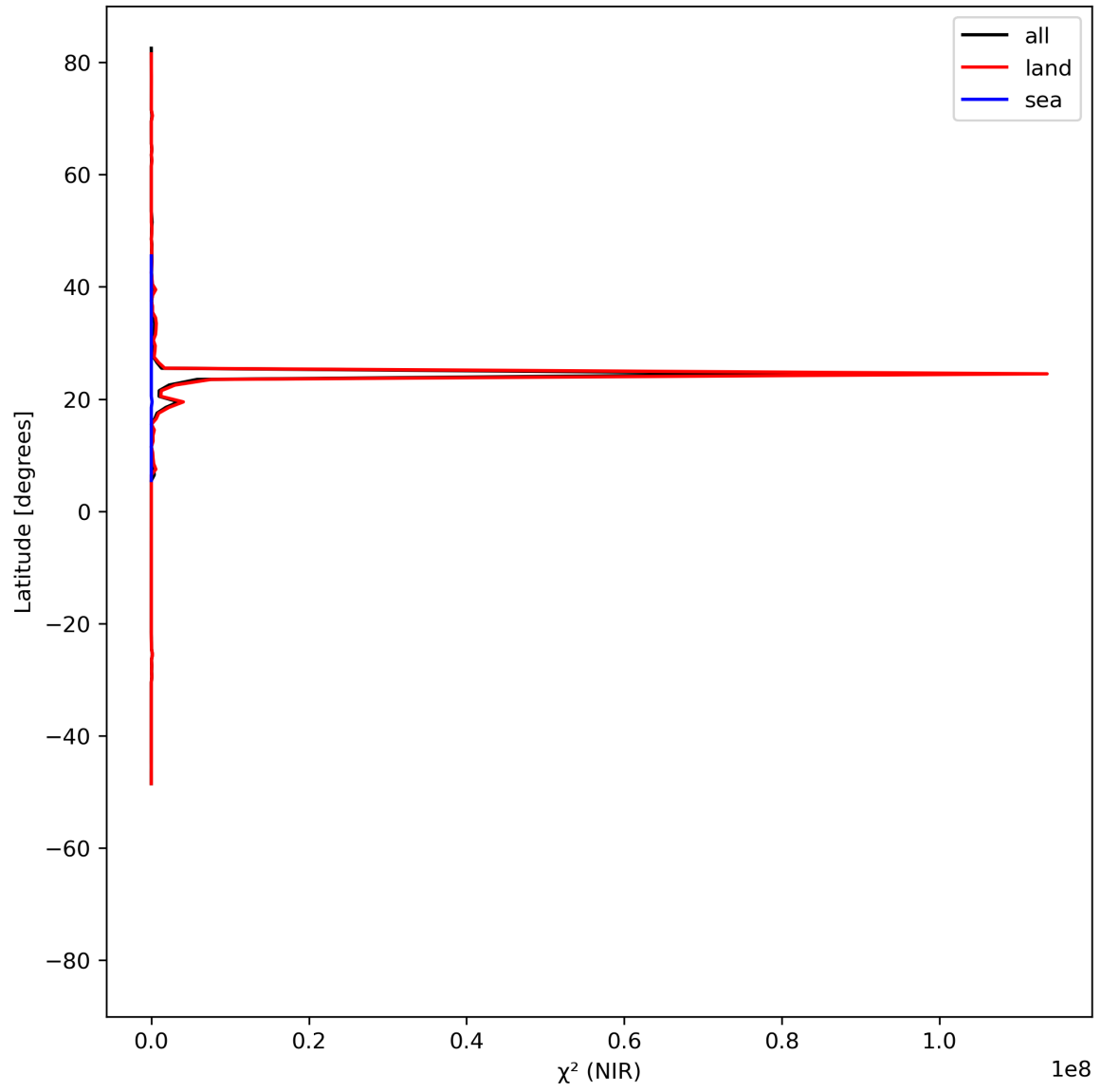
Figure 18: Zonal average of “ \chi^2 (NIR)” for 2023-07-24 to 2023-07-25.
