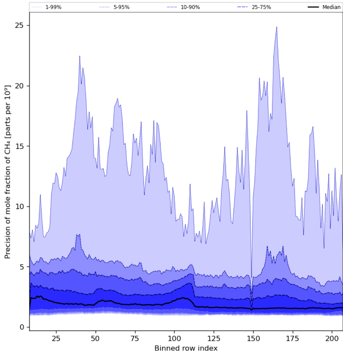
Figure 35: Along track statistics of "Precision of mole fraction of CH 4 " for 2023-07-24 to 2023-07-25
