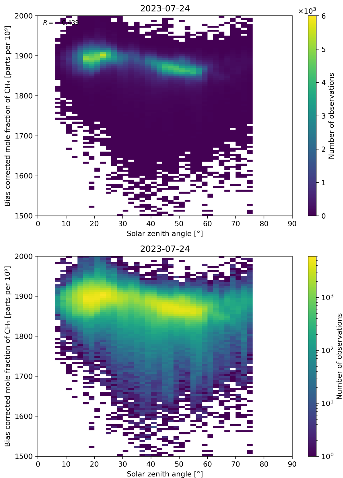
Figure 100: Scatter density plot of “Solar zenith angle” against “Bias corrected mole fraction of CH 4 ” for 2023-07-24 to 2023-07-25.
