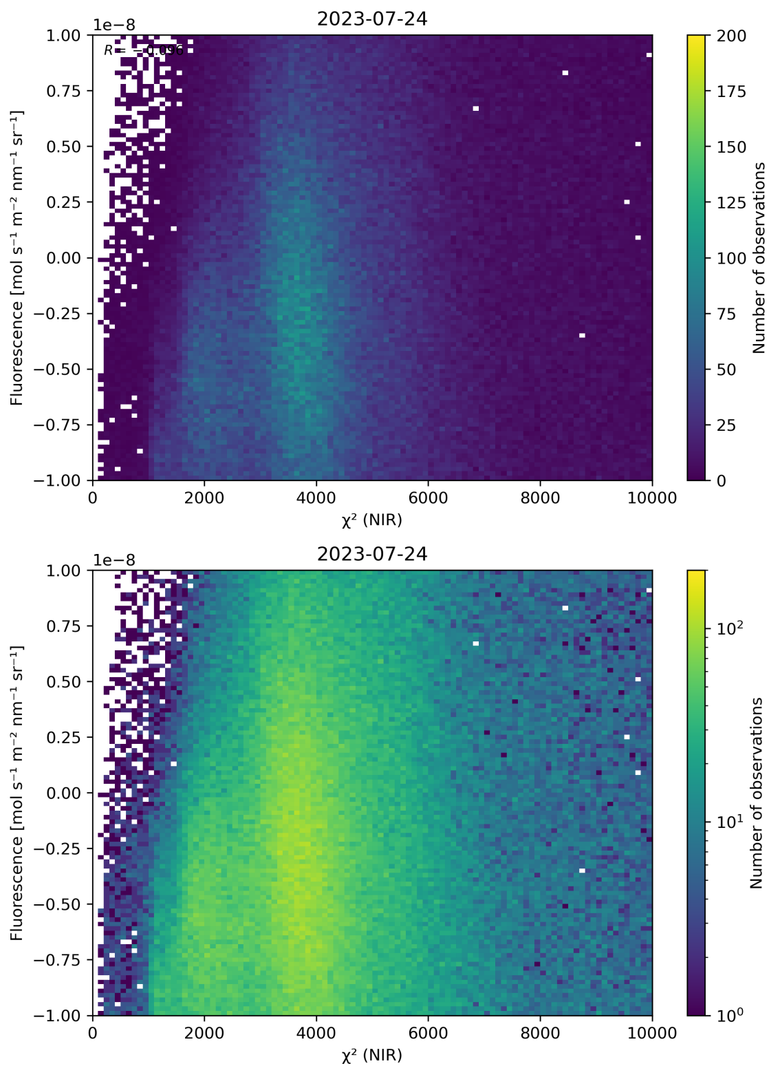
Figure 45: Scatter density plot of “ \chi^2 (NIR)” against “Fluorescence” for 2023-07-24 to 2023-07-25.
