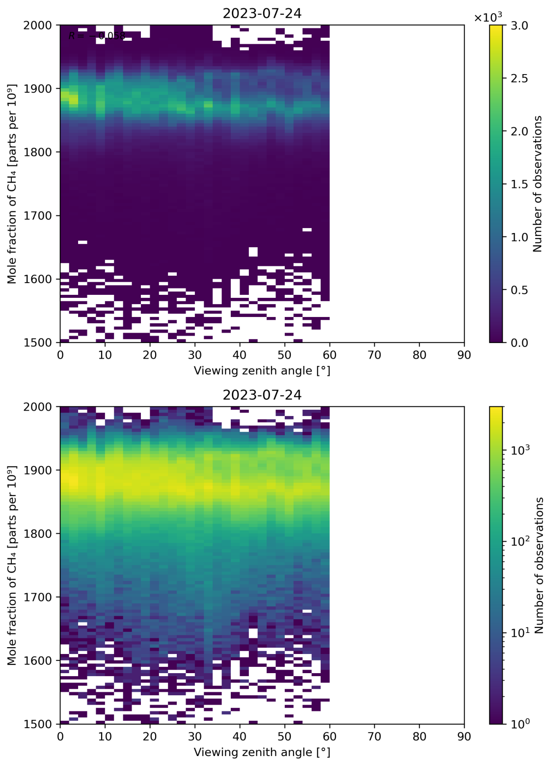
Figure 110: Scatter density plot of “Viewing zenith angle” against “Mole fraction of CH 4 ” for 2023-07-24 to 2023-07-25.
