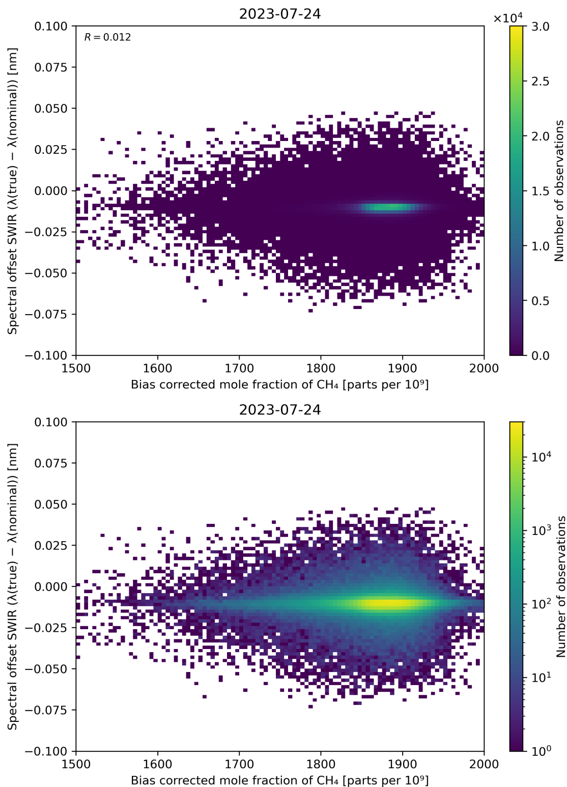
Figure 69: Scatter density plot of “Bias corrected mole fraction of \text{CH}_4 ” against “Spectral offset SWIR ( \lambda(\text{true}) - \lambda(\text{nominal}) )” for 2023-07-24 to 2023-07-25.
