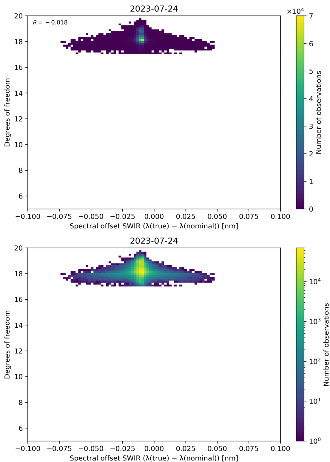
Figure 119: Scatter density plot of “Spectral offset SWIR ( \lambda(\text{true}) - \lambda(\text{nominal}) )” against “Degrees of freedom” for 2023-07-24 to 2023-07-25.
