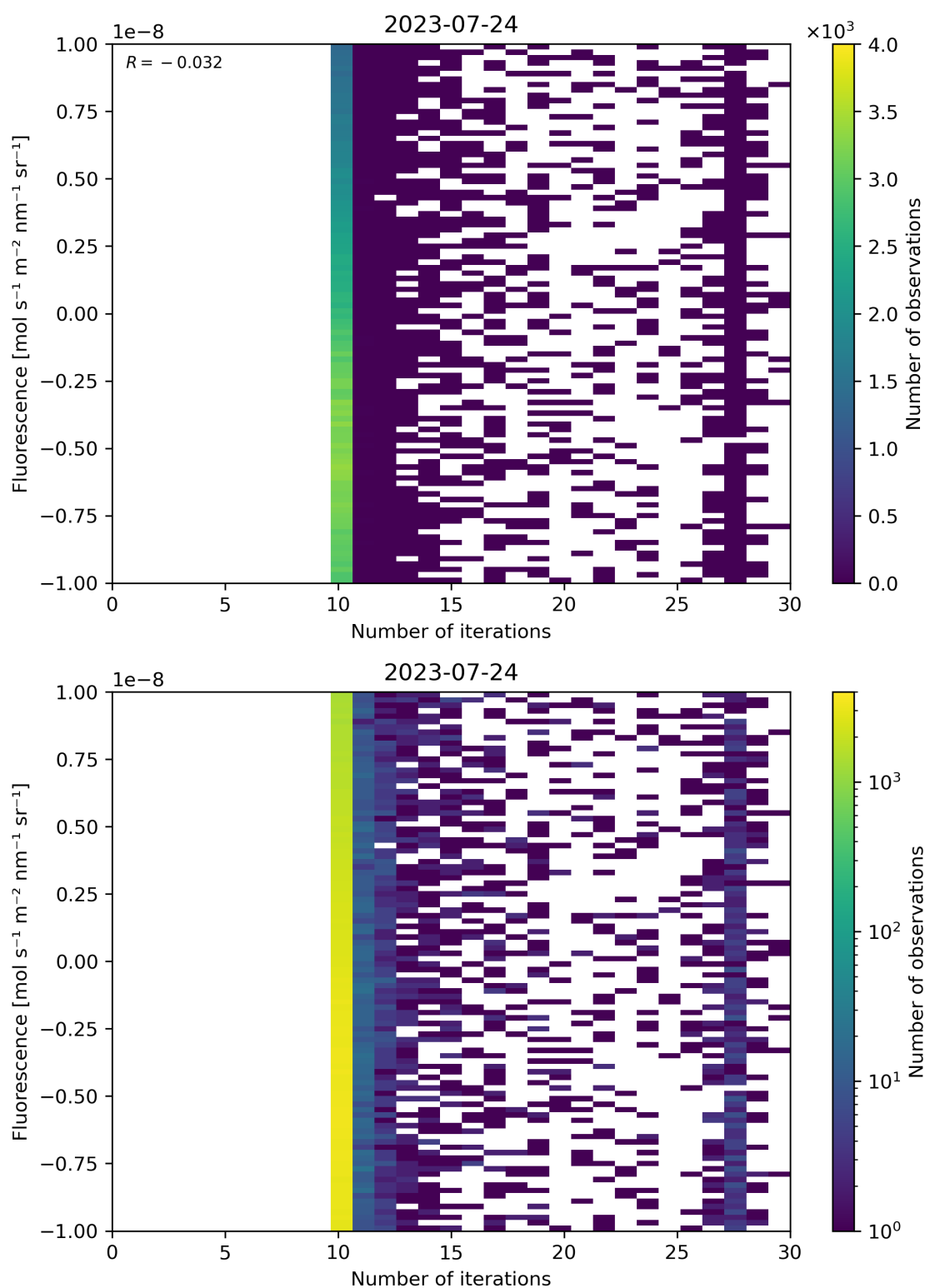
Figure 87: Scatter density plot of “Number of iterations” against “Fluorescence” for 2023-07-24 to 2023-07-25.
