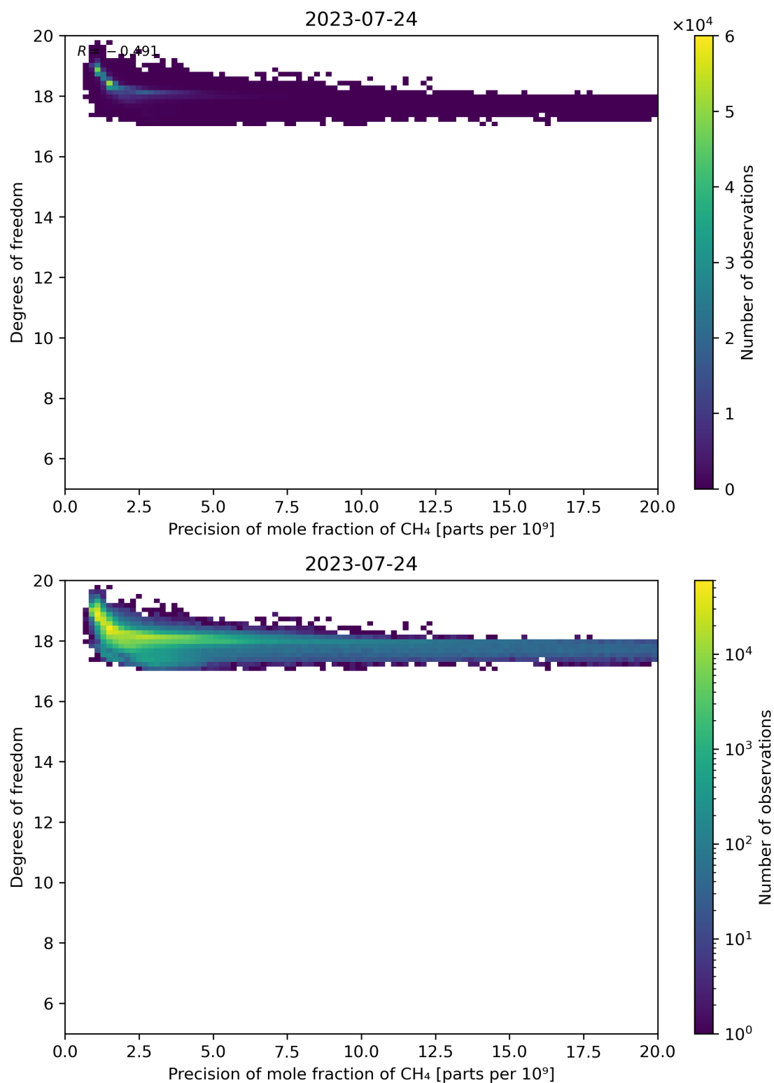
Figure 80: Scatter density plot of “Precision of mole fraction of CH 4 ” against “Degrees of freedom” for 2023-07-24 to 2023-07-25.
