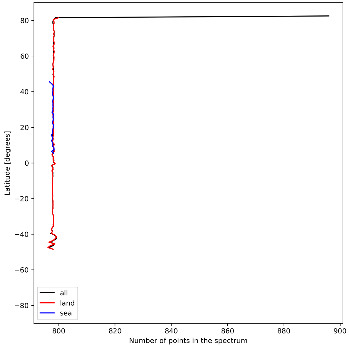
Figure 15: Zonal average of “Number of points in the spectrum” for 2023-07-24 to 2023-07-25.
