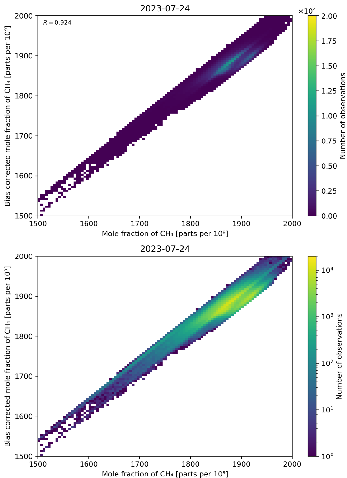
Figure 74: Scatter density plot of “Mole fraction of CH 4 ” against “Bias corrected mole fraction of CH 4 ” for 2023-07-24 to 2023-07-25.
