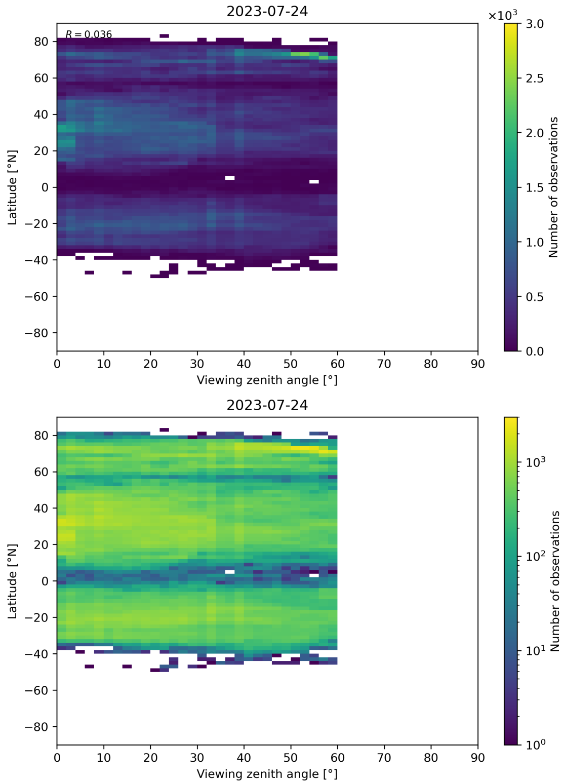
Figure 109: Scatter density plot of “Viewing zenith angle” against “Latitude” for 2023-07-24 to 2023-07-25.
