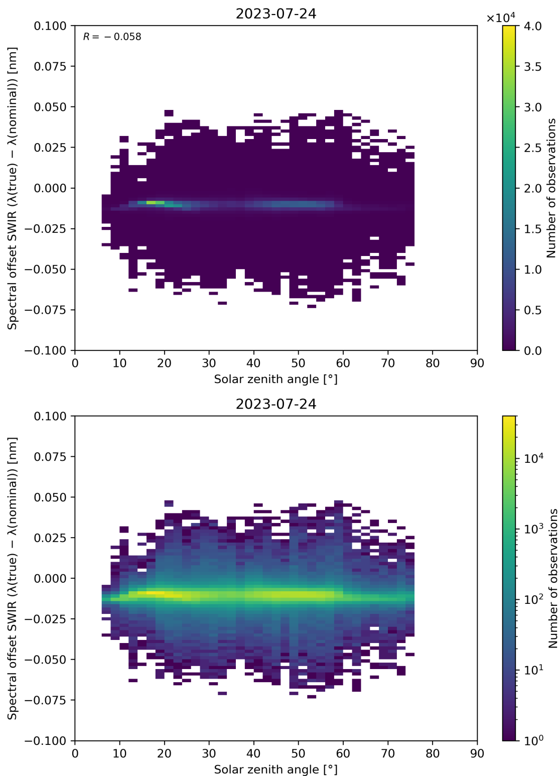
Figure 104: Scatter density plot of “Solar zenith angle” against “Spectral offset SWIR ( \lambda(\text{true}) - \lambda(\text{nominal}) )” for 2023-07-24 to 2023-07-25.
