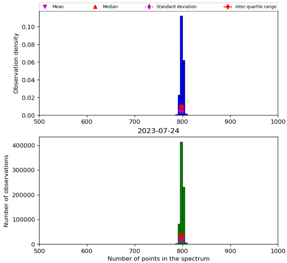
Figure 26: Histogram of “Number of points in the spectrum” for 2023-07-24 to 2023-07-25
