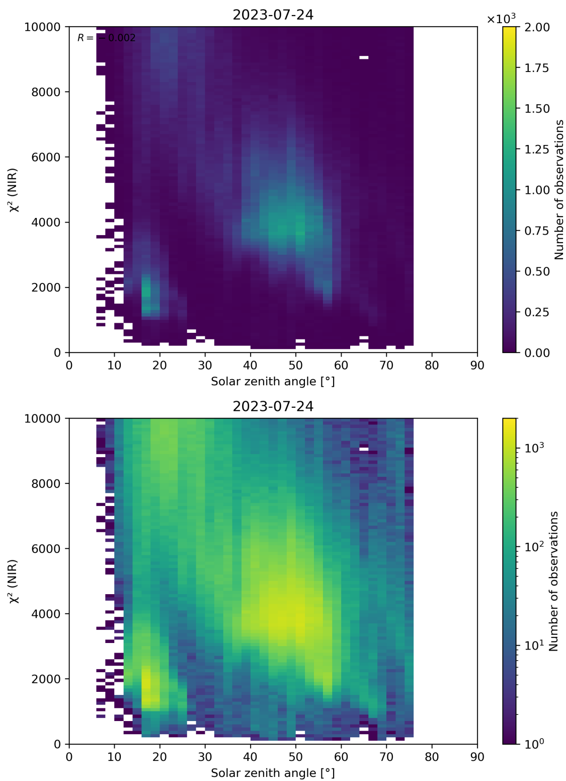
Figure 94: Scatter density plot of “Solar zenith angle” against “ \chi^2 (NIR)” for 2023-07-24 to 2023-07-25.
