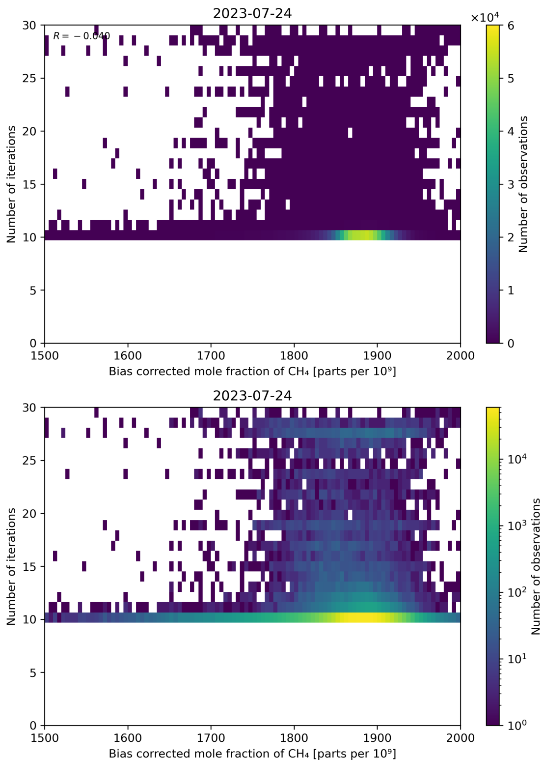
Figure 67: Scatter density plot of “Bias corrected mole fraction of \text{CH}_4 ” against “Number of iterations” for 2023-07-24 to 2023-07-25.
