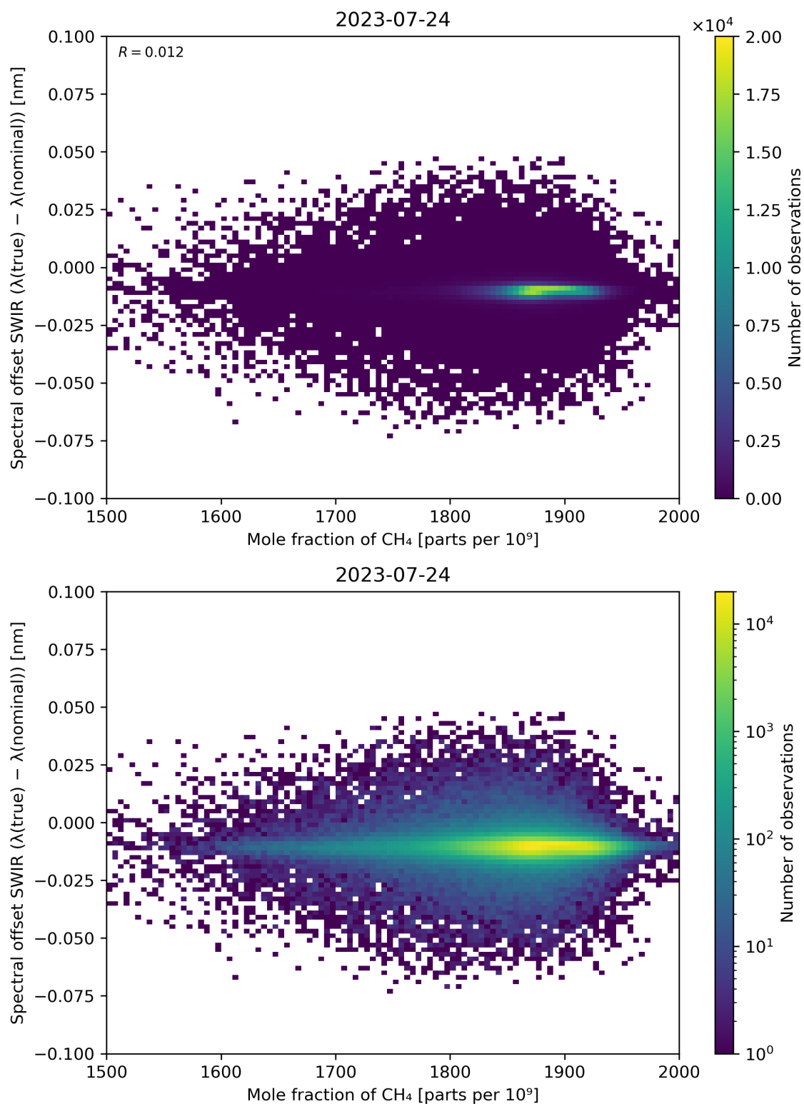
Figure 86: Scatter density plot of “Mole fraction of CH 4 ” against “Spectral offset SWIR ( \lambda(\text{true}) - \lambda(\text{nominal}) )” for 2023-07-24 to 2023-07-25.
