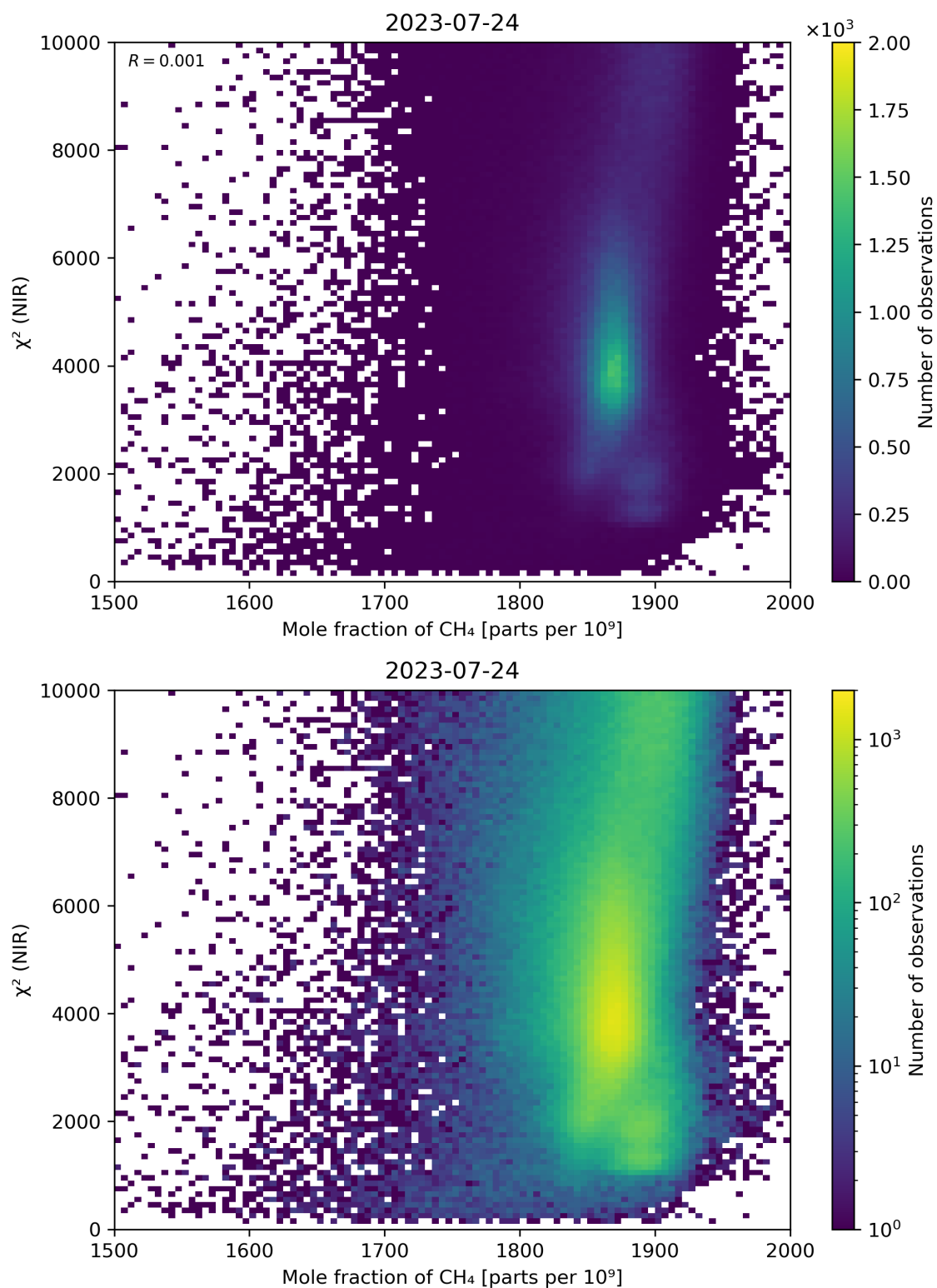
Figure 70: Scatter density plot of “Mole fraction of \text{CH}_4 ” against “ \chi^2 (NIR)” for 2023-07-24 to 2023-07-25.
