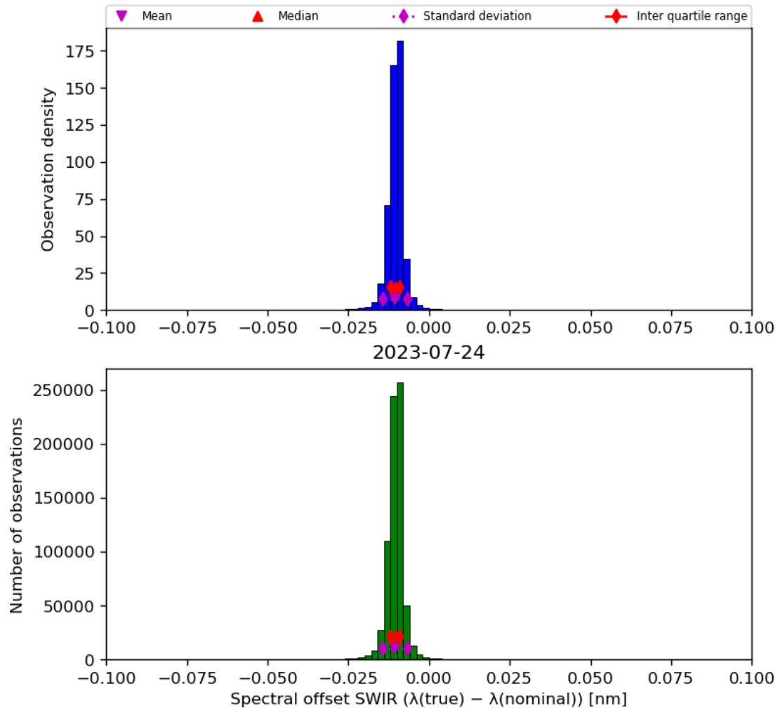
Figure 27: Histogram of “Spectral offset SWIR ( \lambda(\text{true}) - \lambda(\text{nominal}) )” for 2023-07-24 to 2023-07-25
