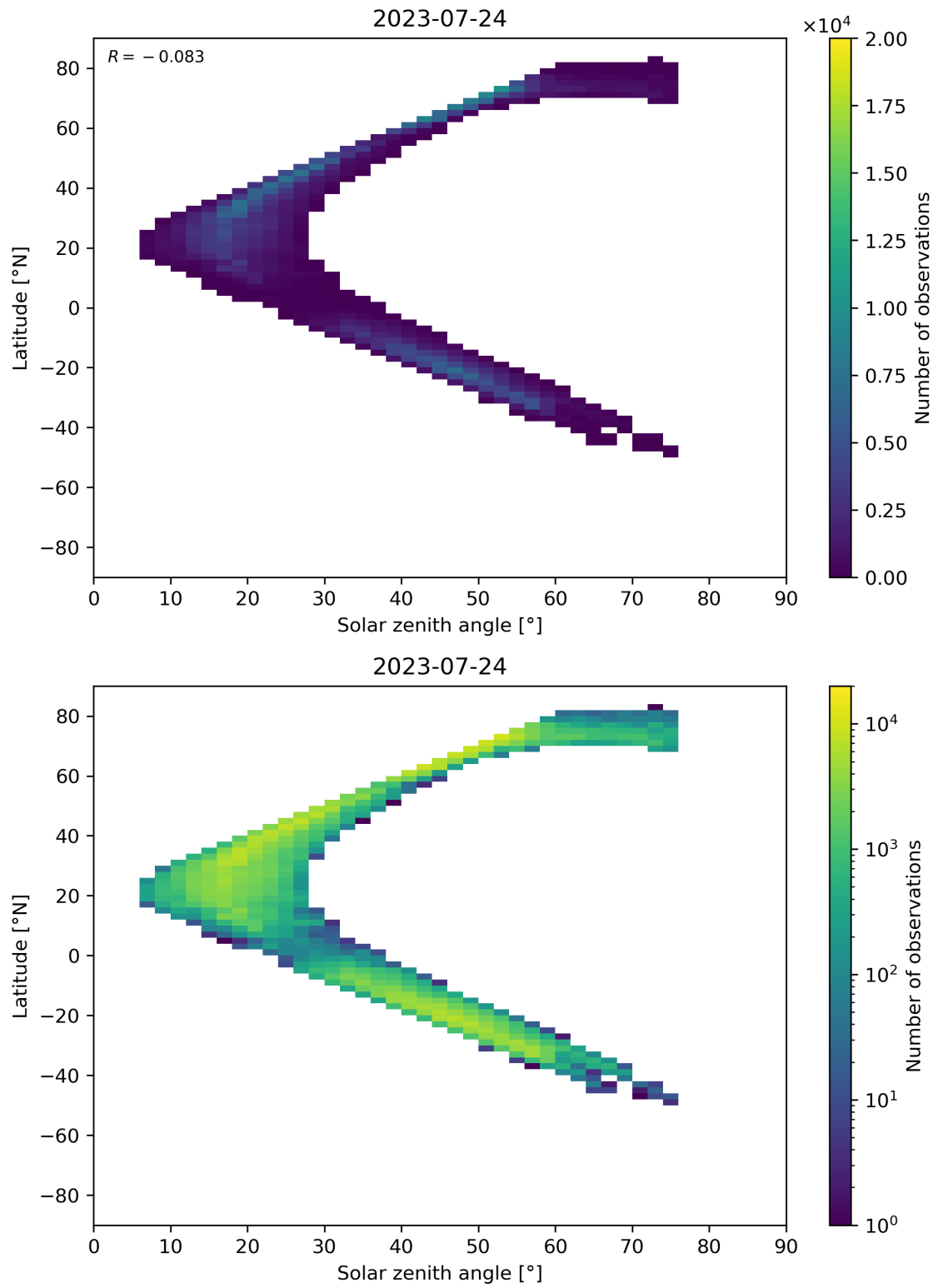
Figure 98: Scatter density plot of “Solar zenith angle” against “Latitude” for 2023-07-24 to 2023-07-25.
