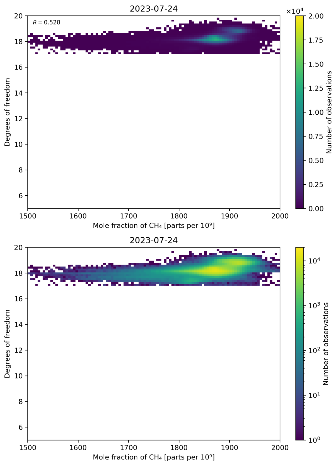
Figure 72: Scatter density plot of “Mole fraction of CH 4 ” against “Degrees of freedom” for 2023-07-24 to 2023-07-25.
