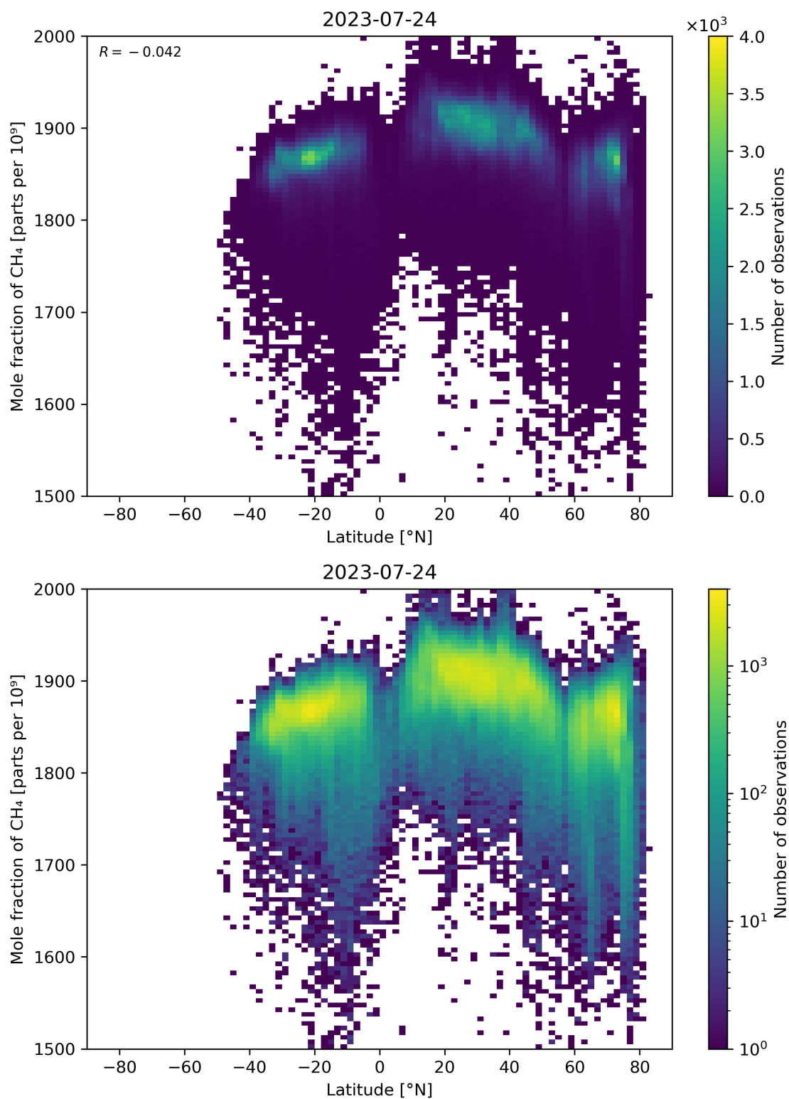
Figure 57: Scatter density plot of “Latitude” against “Mole fraction of \text{CH}_4 ” for 2023-07-24 to 2023-07-25.
