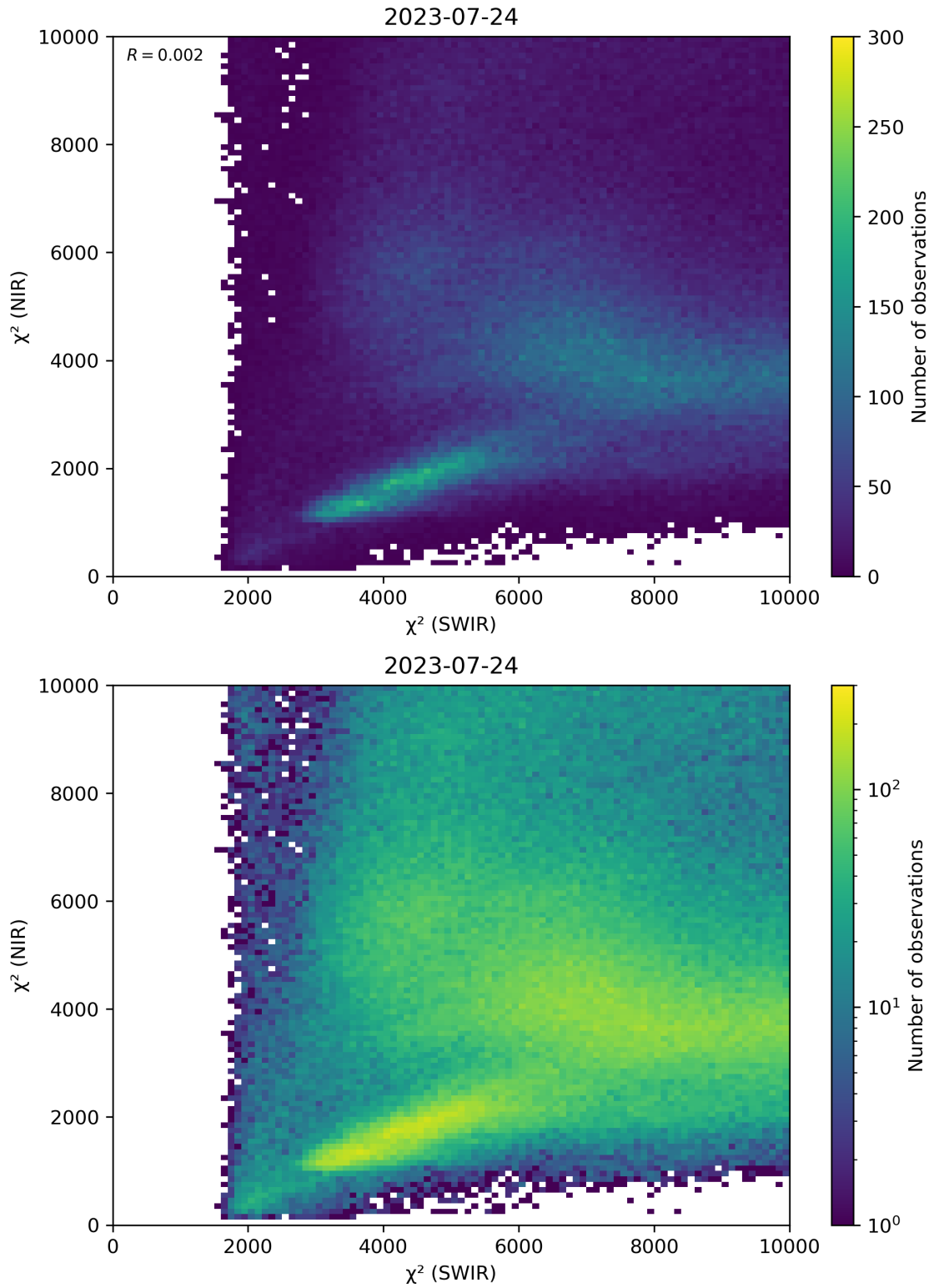
Figure 47: Scatter density plot of “ \chi^2 (SWIR)” against “ \chi^2 (NIR)” for 2023-07-24 to 2023-07-25.
