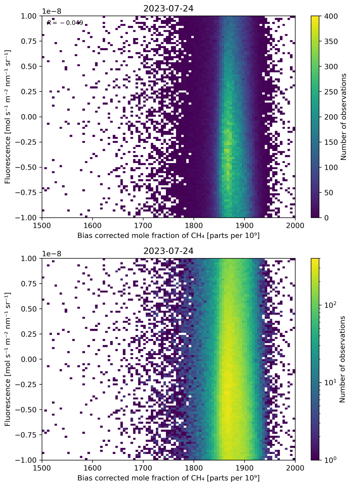
Figure 66: Scatter density plot of “Bias corrected mole fraction of \text{CH}_4 ” against “Fluorescence” for 2023-07-24 to 2023-07-25.
