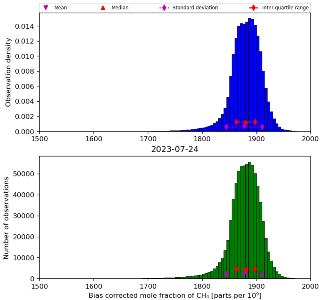
Figure 25: Histogram of “Bias corrected mole fraction of CH 4 ” for 2023-07-24 to 2023-07-25
