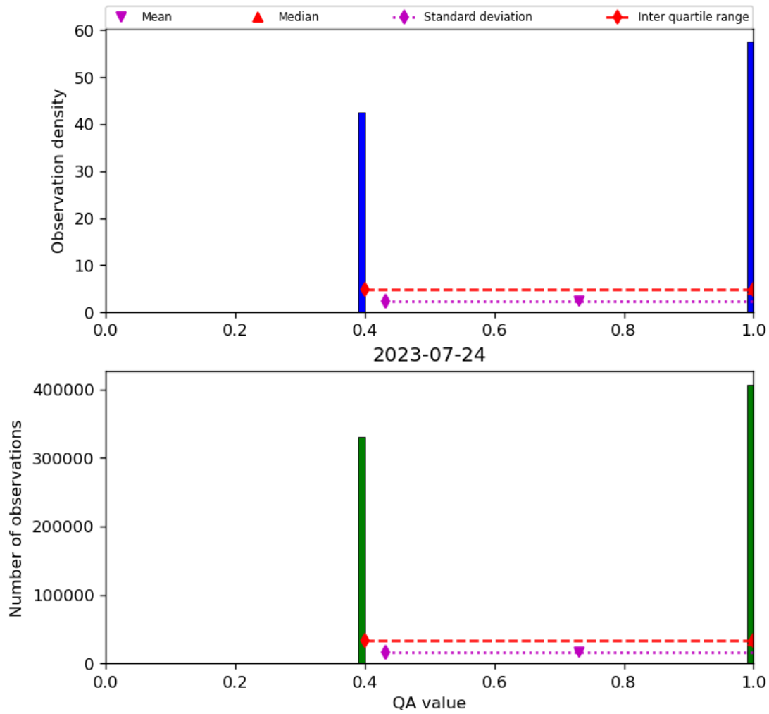
Figure 22: Histogram of “QA value” for 2023-07-24 to 2023-07-25
