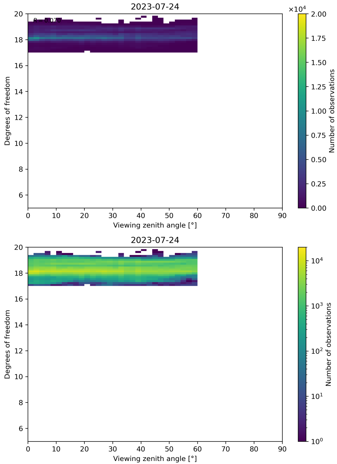
Figure 107: Scatter density plot of “Viewing zenith angle” against “Degrees of freedom” for 2023-07-24 to 2023-07-25.
