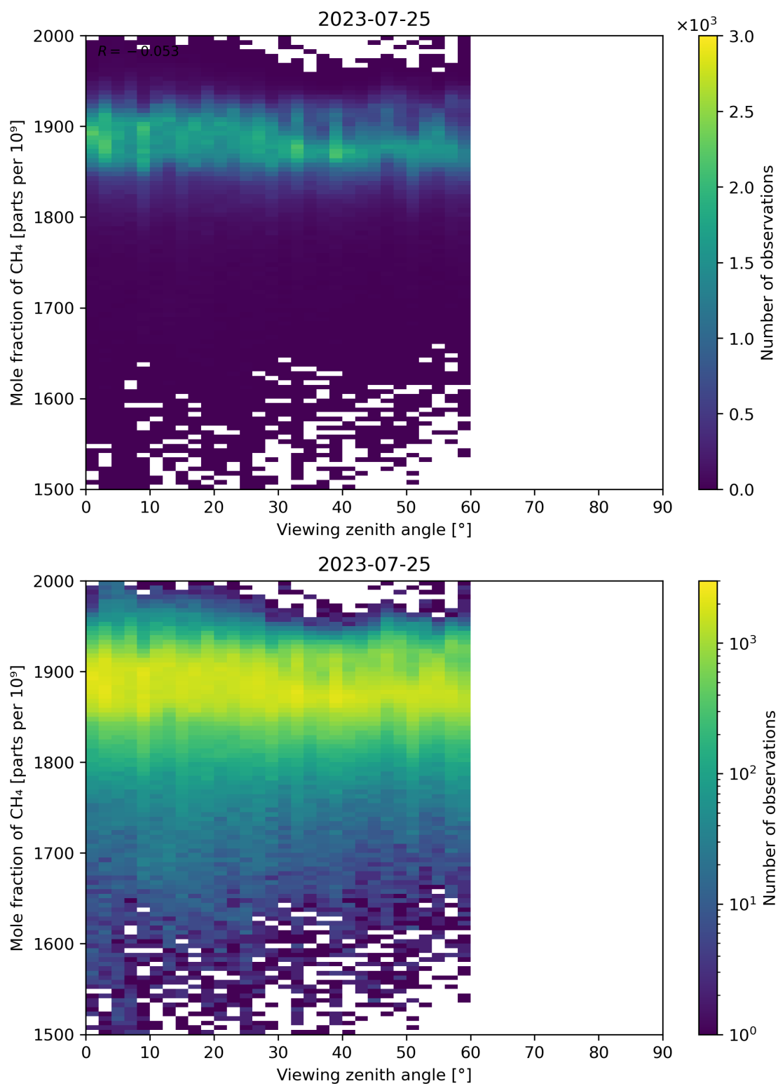
Figure 110: Scatter density plot of “Viewing zenith angle” against “Mole fraction of CH 4 ” for 2023-07-24 to 2023-07-26.
