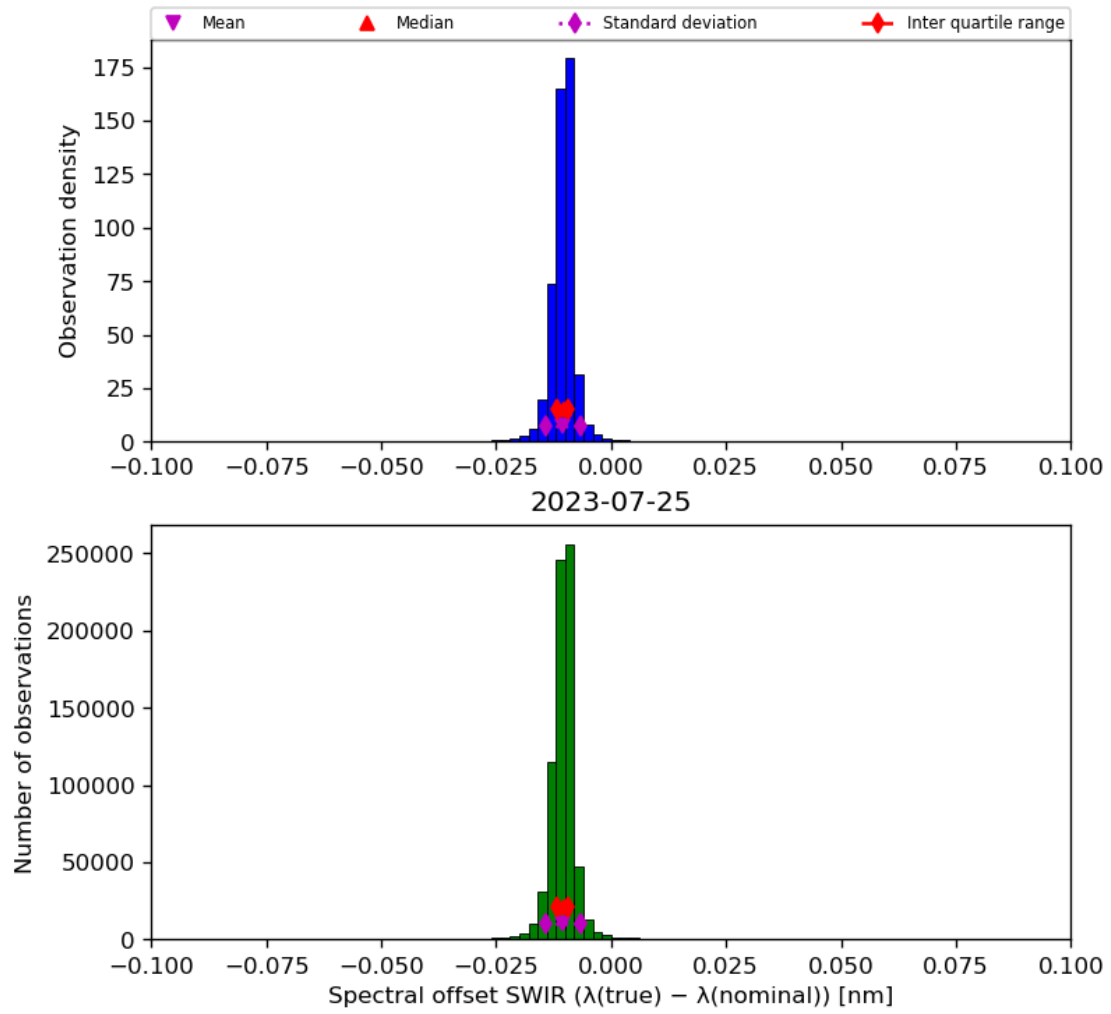
Figure 27: Histogram of “Spectral offset SWIR ( \lambda(\text{true}) - \lambda(\text{nominal}) )” for 2023-07-24 to 2023-07-26
