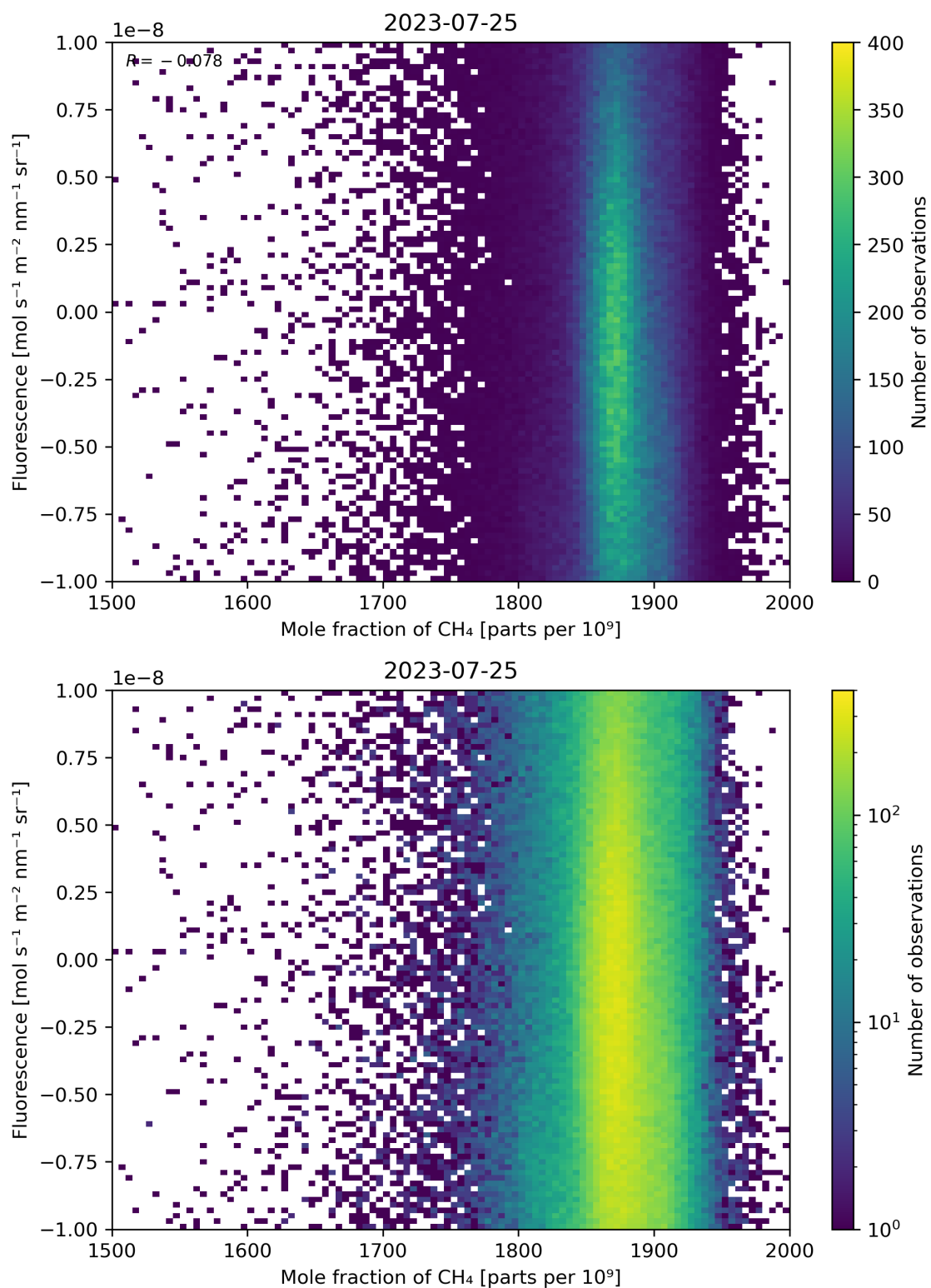
Figure 73: Scatter density plot of “Mole fraction of \text{CH}_4 ” against “Fluorescence” for 2023-07-24 to 2023-07-26.
