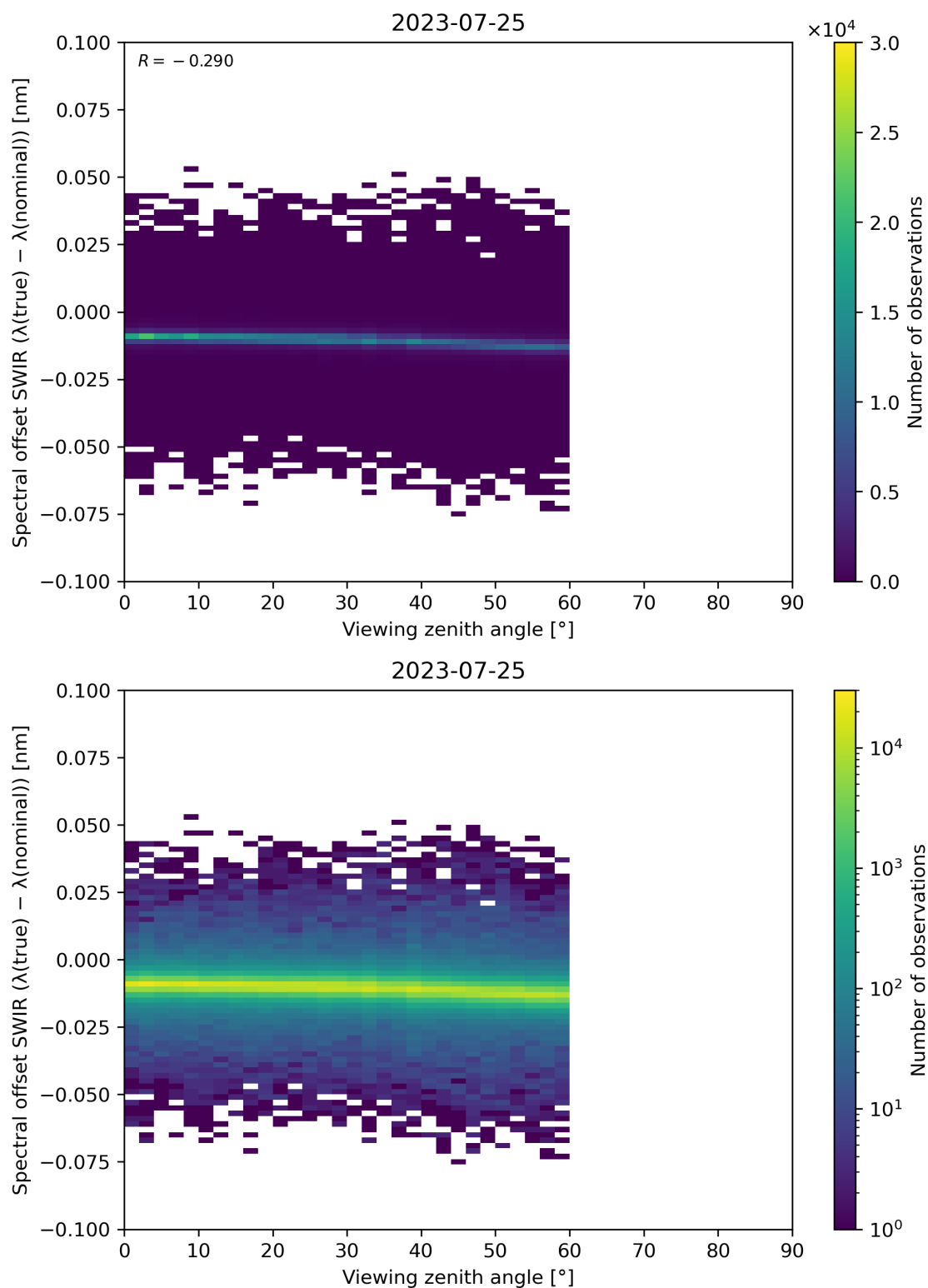
Figure 116: Scatter density plot of “Viewing zenith angle” against “Spectral offset SWIR ( \lambda(\text{true}) - \lambda(\text{nominal}) )” for 2023-07-24 to 2023-07-26.
