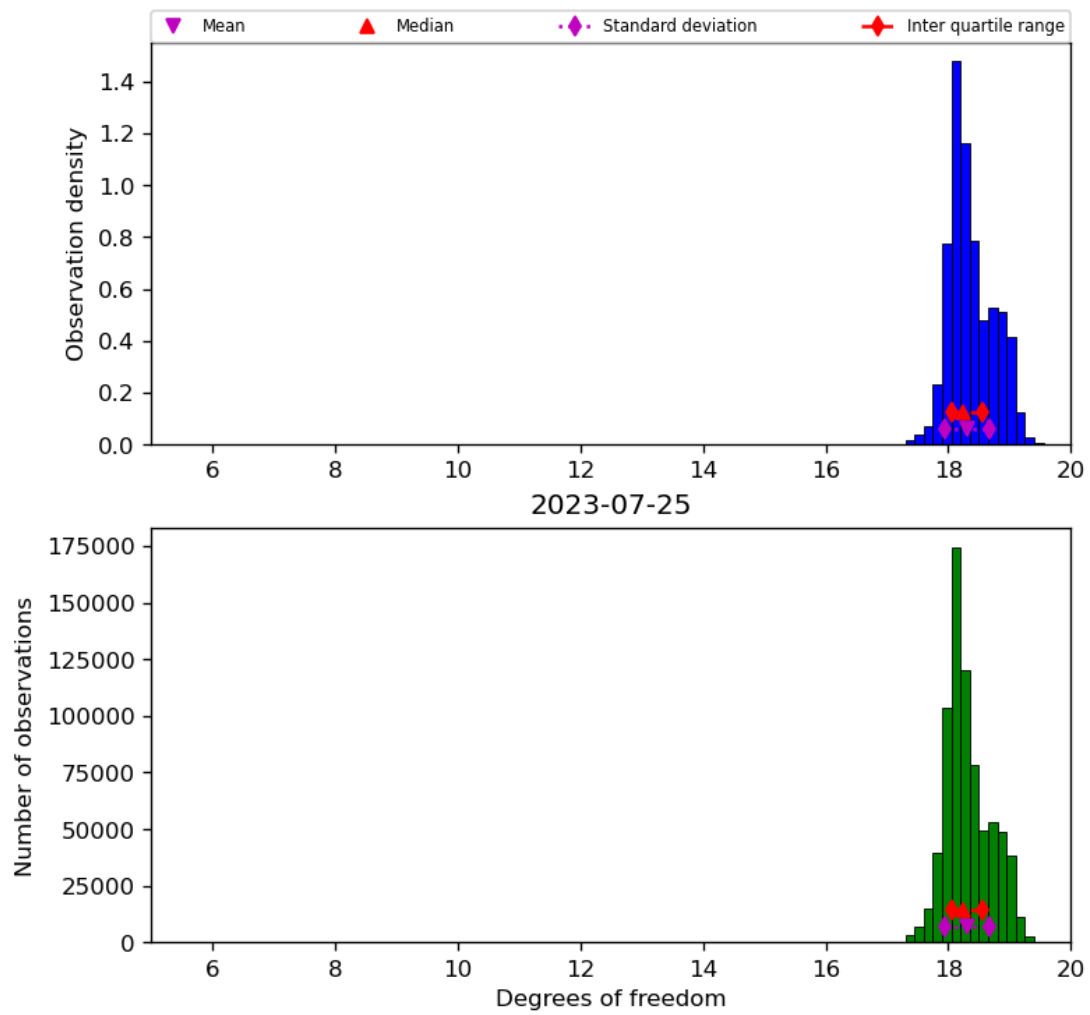
Figure 30: Histogram of “Degrees of freedom” for 2023-07-24 to 2023-07-26
