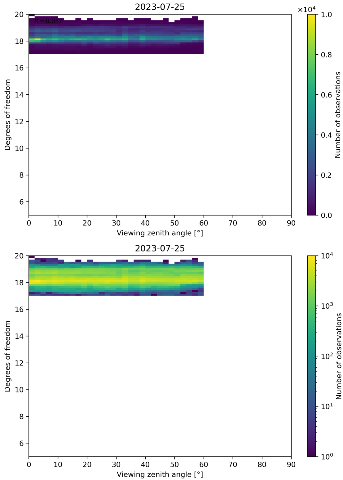
Figure 107: Scatter density plot of “Viewing zenith angle” against “Degrees of freedom” for 2023-07-24 to 2023-07-26.
