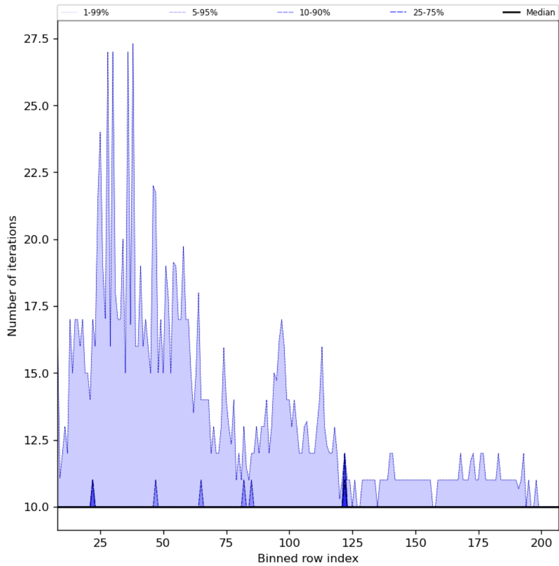
Figure 42: Along track statistics of “Number of iterations” for 2023-07-24 to 2023-07-26
