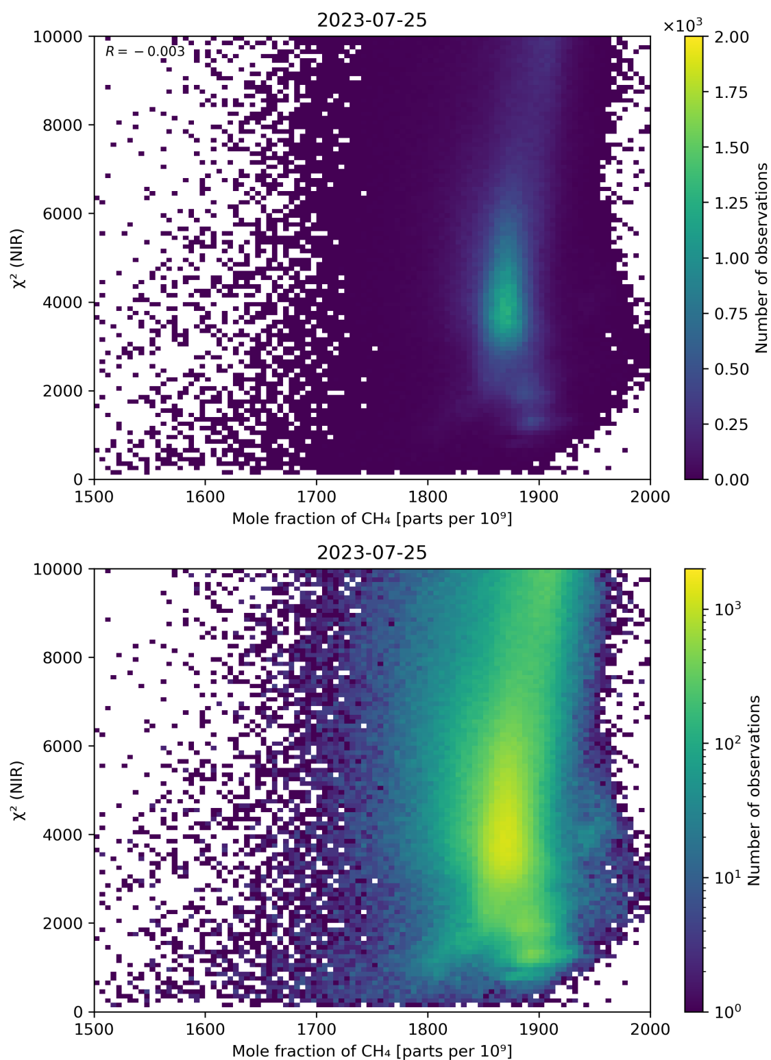
Figure 70: Scatter density plot of “Mole fraction of CH 4 ” against “ \chi^2 (NIR)” for 2023-07-24 to 2023-07-26.
