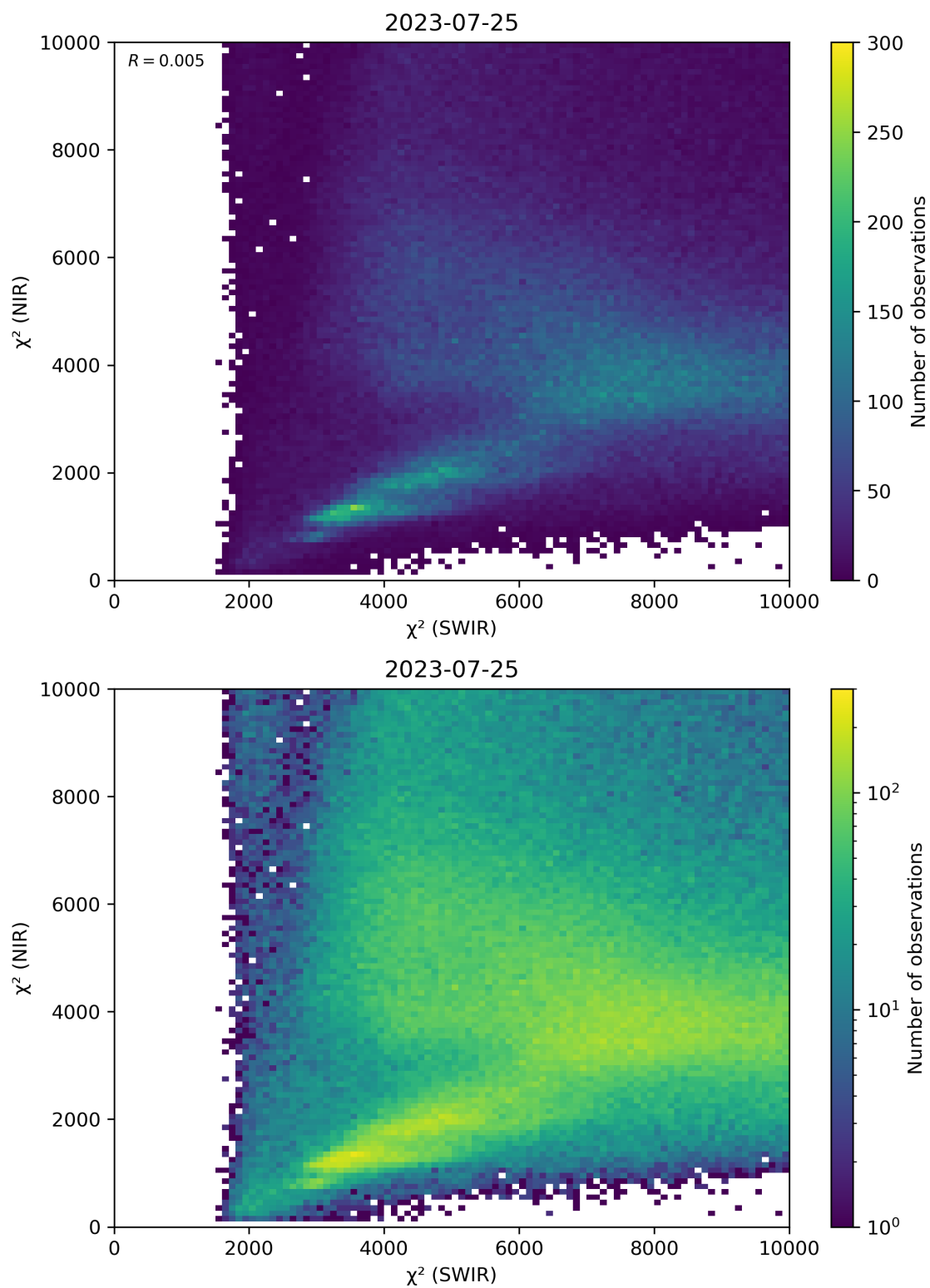
Figure 47: Scatter density plot of “ \chi^2 (SWIR)” against “ \chi^2 (NIR)” for 2023-07-24 to 2023-07-26.
