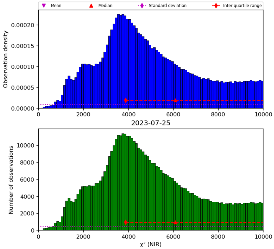
Figure 29: Histogram of “ \chi^2 (NIR)” for 2023-07-24 to 2023-07-26
