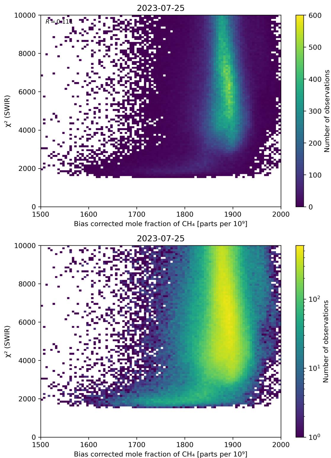
Figure 64: Scatter density plot of “Bias corrected mole fraction of CH 4 ” against “ \chi^2 (SWIR)” for 2023-07-24 to 2023-07-26.
