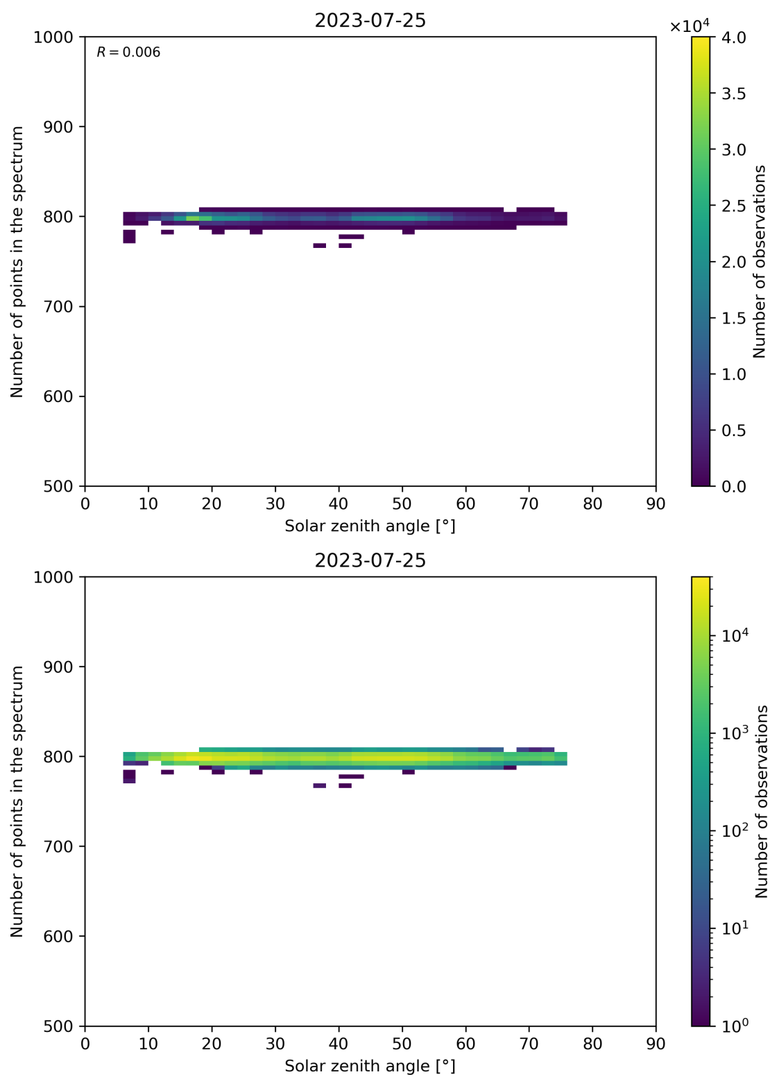
Figure 103: Scatter density plot of “Solar zenith angle” against “Number of points in the spectrum” for 2023-07-24 to 2023-07-26.
