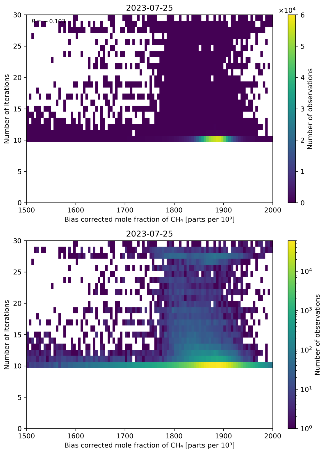
Figure 67: Scatter density plot of “Bias corrected mole fraction of CH 4 ” against “Number of iterations” for 2023-07-24 to 2023-07-26.
