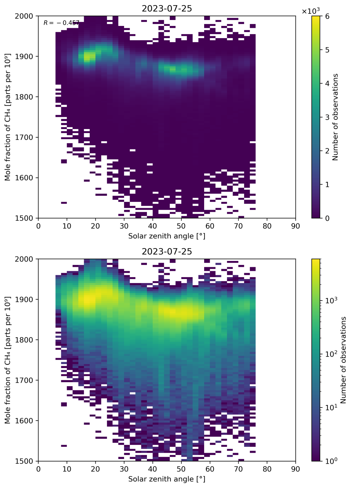
Figure 99: Scatter density plot of “Solar zenith angle” against “Mole fraction of CH 4 ” for 2023-07-24 to 2023-07-26.
