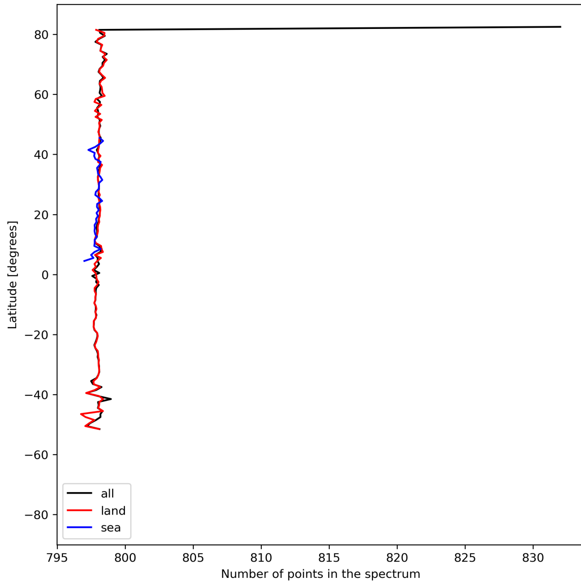
Figure 15: Zonal average of “Number of points in the spectrum” for 2023-07-24 to 2023-07-26.
