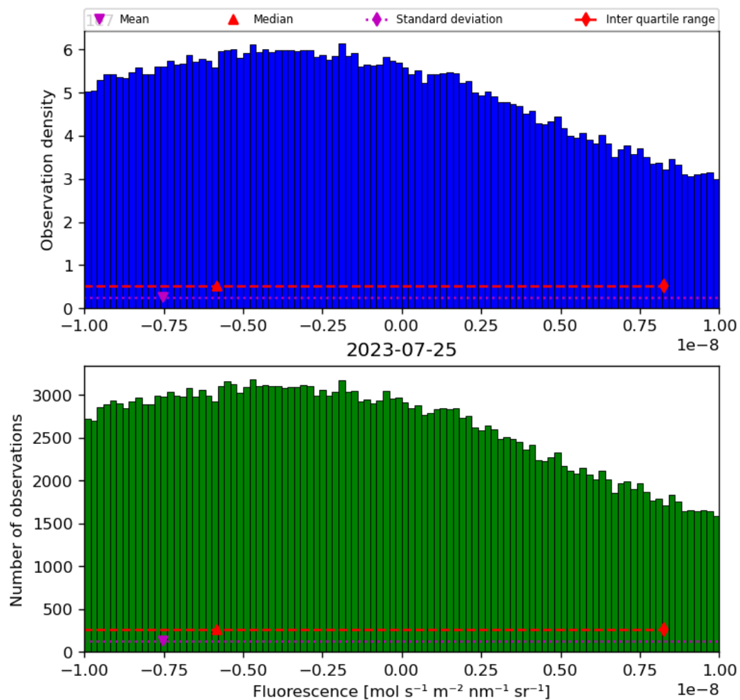
Figure 32: Histogram of “Fluorescence” for 2023-07-24 to 2023-07-26
