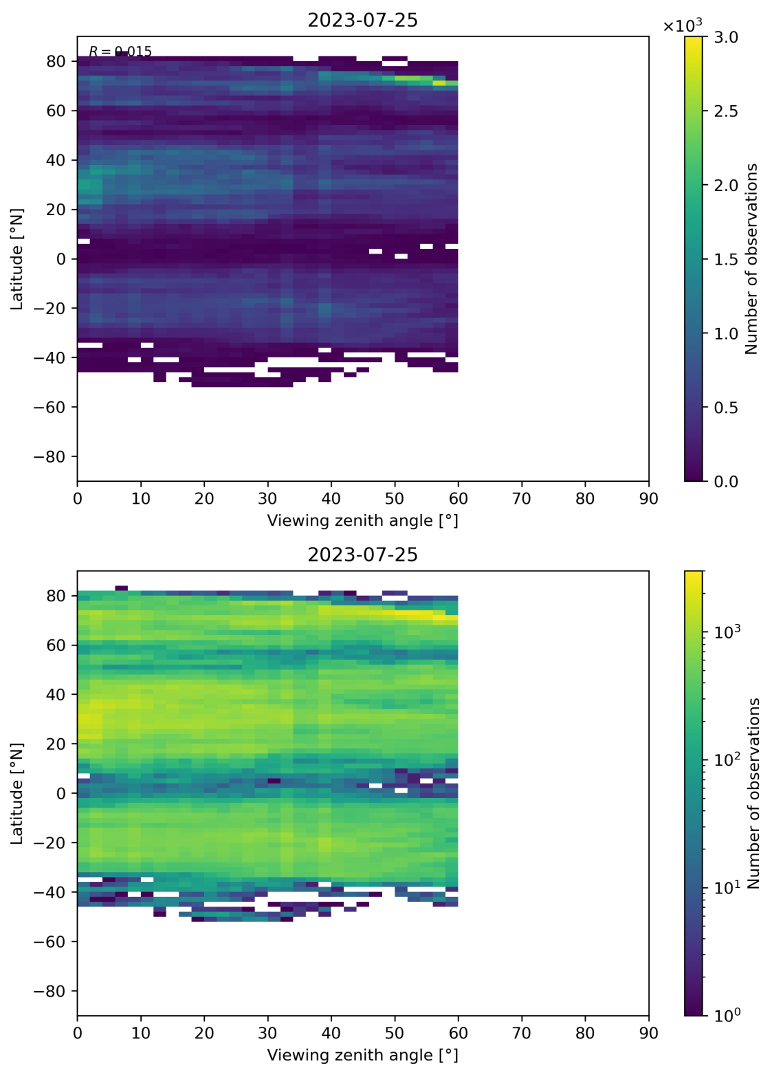
Figure 109: Scatter density plot of “Viewing zenith angle” against “Latitude” for 2023-07-24 to 2023-07-26.
