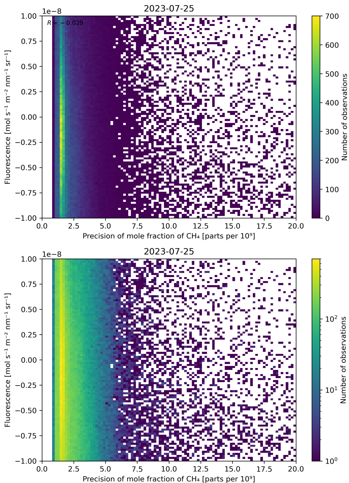
Figure 81: Scatter density plot of “Precision of mole fraction of \text{CH}_4 ” against “Fluorescence” for 2023-07-24 to 2023-07-26.
