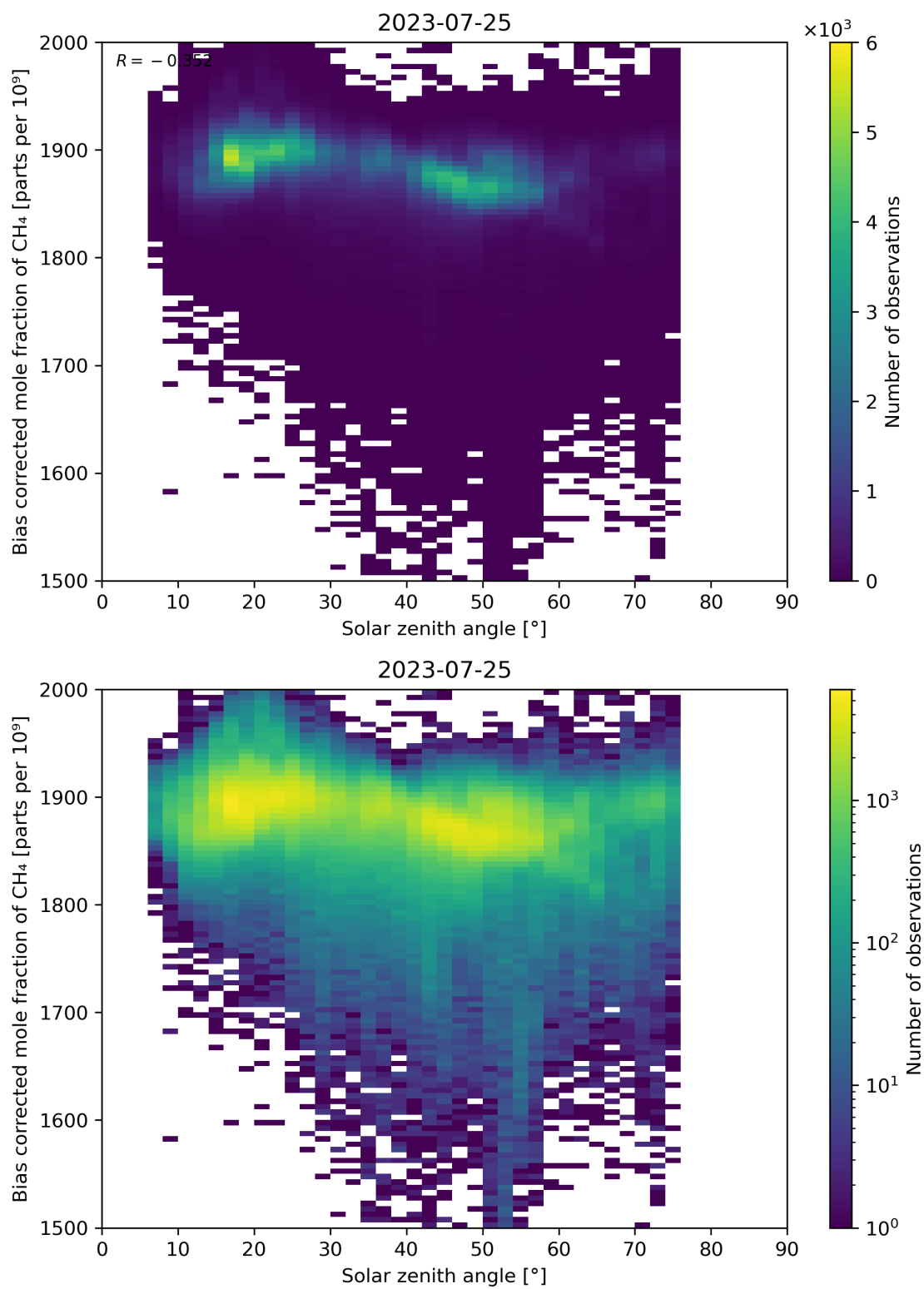
Figure 100: Scatter density plot of “Solar zenith angle” against “Bias corrected mole fraction of \text{CH}_4 ” for 2023-07-24 to 2023-07-26.
