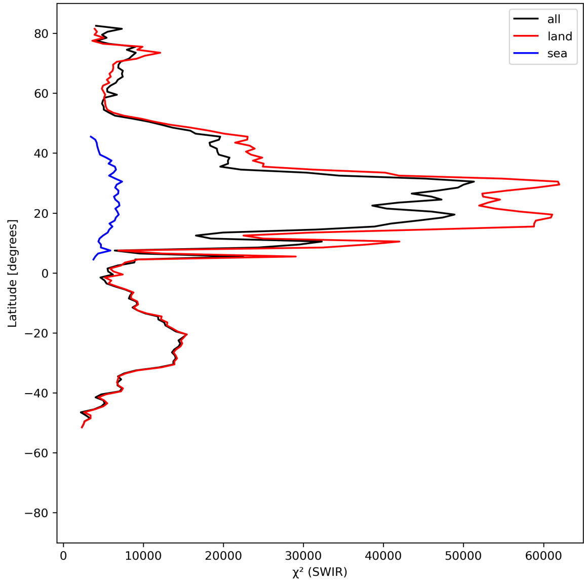
Figure 17: Zonal average of “ \chi^2 (SWIR)” for 2023-07-24 to 2023-07-26.
