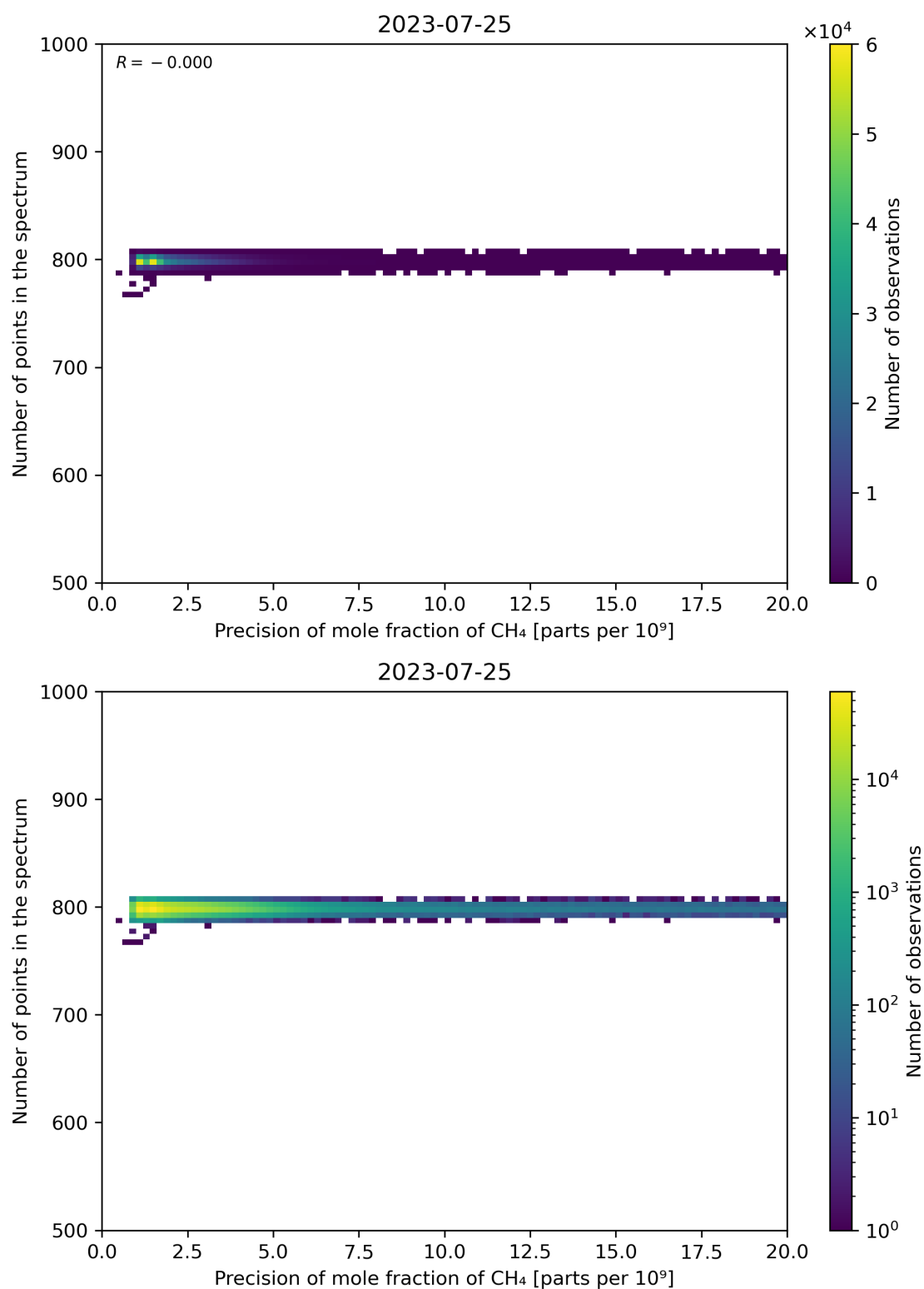
Figure 84: Scatter density plot of “Precision of mole fraction of CH 4 ” against “Number of points in the spectrum” for 2023-07-24 to 2023-07-26.
