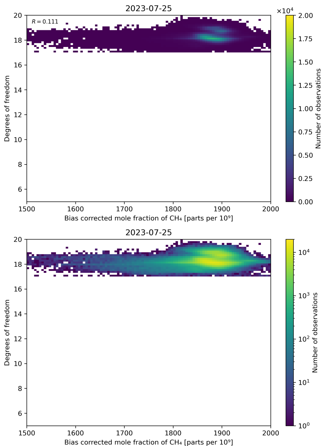
Figure 65: Scatter density plot of “Bias corrected mole fraction of CH 4 ” against “Degrees of freedom” for 2023-07-24 to 2023-07-26.
