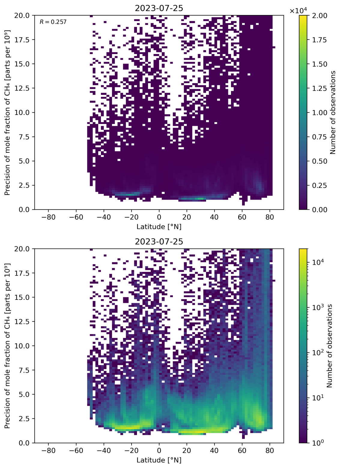
Figure 59: Scatter density plot of “Latitude” against “Precision of mole fraction of \text{CH}_4 ” for 2023-07-24 to 2023-07-26.
