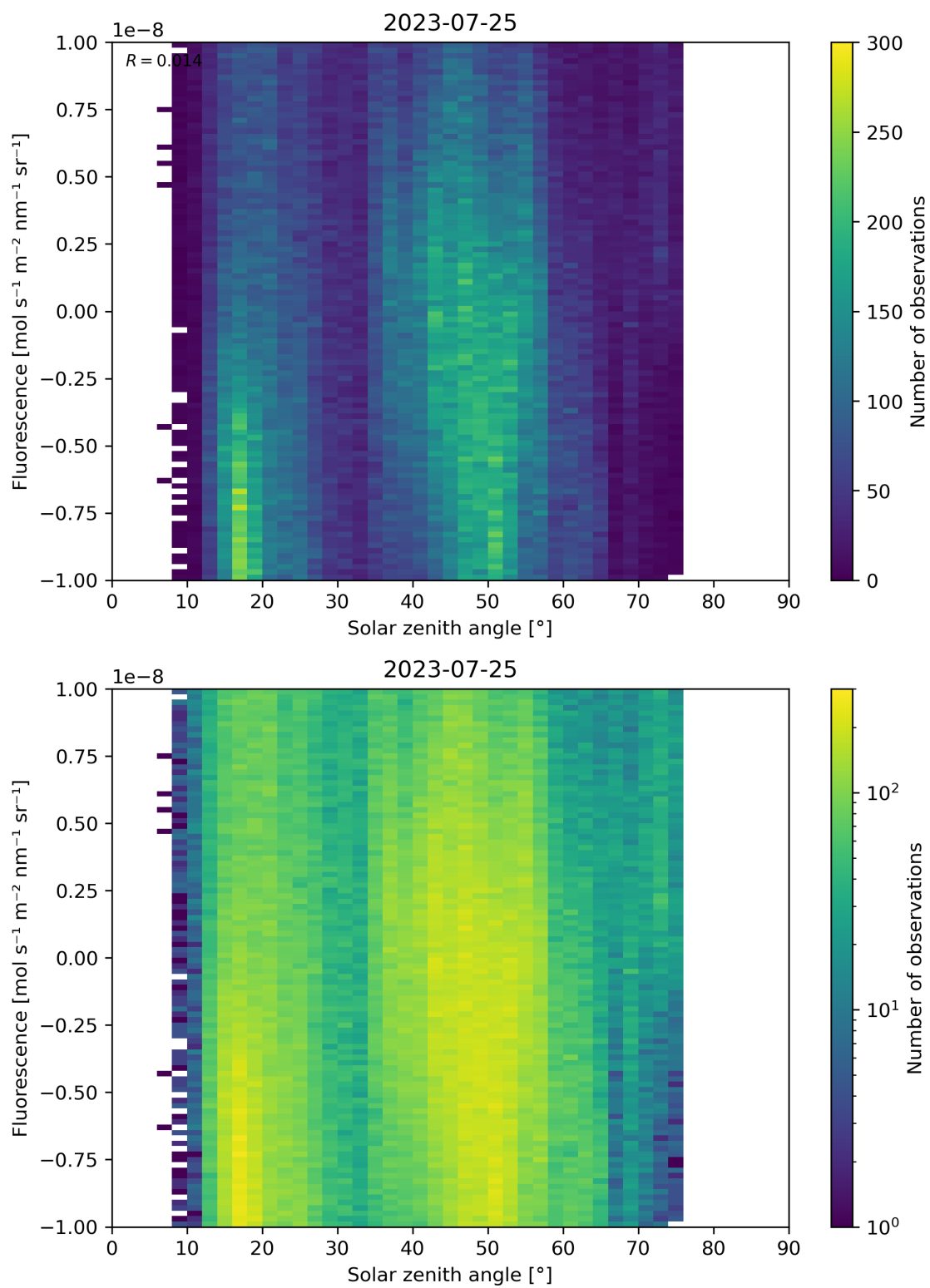
Figure 97: Scatter density plot of “Solar zenith angle” against “Fluorescence” for 2023-07-24 to 2023-07-26.
