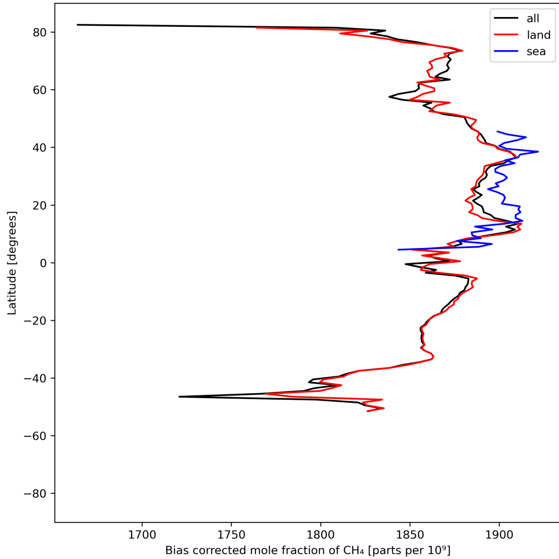
Figure 14: Zonal average of “Bias corrected mole fraction of CH 4 ” for 2023-07-24 to 2023-07-26.
