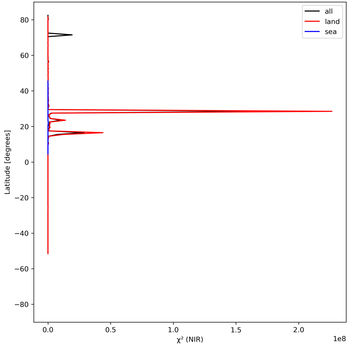
Figure 18: Zonal average of “ \chi^2 (NIR)” for 2023-07-24 to 2023-07-26.
