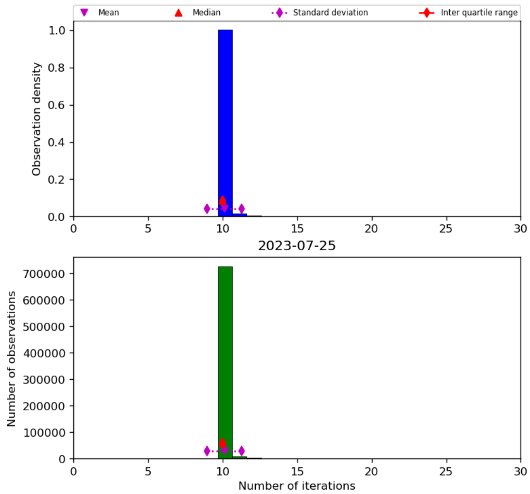
Figure 31: Histogram of “Number of iterations” for 2023-07-24 to 2023-07-26
