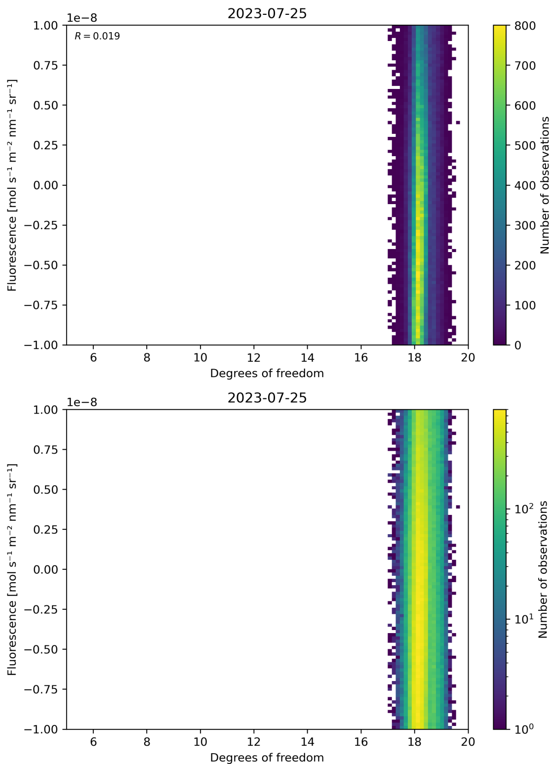
Figure 51: Scatter density plot of “Degrees of freedom” against “Fluorescence” for 2023-07-24 to 2023-07-26.
