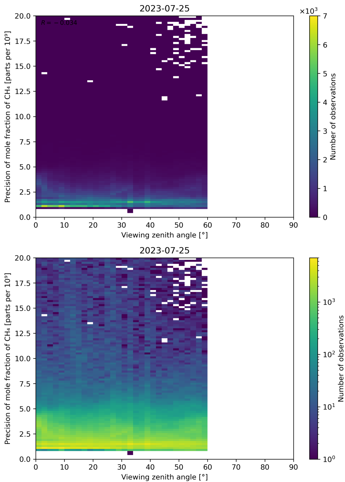
Figure 112: Scatter density plot of “Viewing zenith angle” against “Precision of mole fraction of \text{CH}_4 ” for 2023-07-24 to 2023-07-26.
