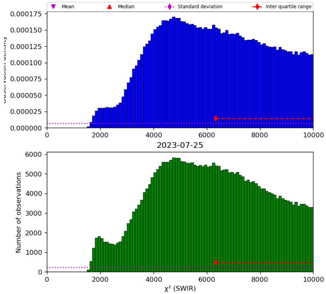
Figure 28: Histogram of “ \chi^2 (SWIR)” for 2023-07-24 to 2023-07-26
