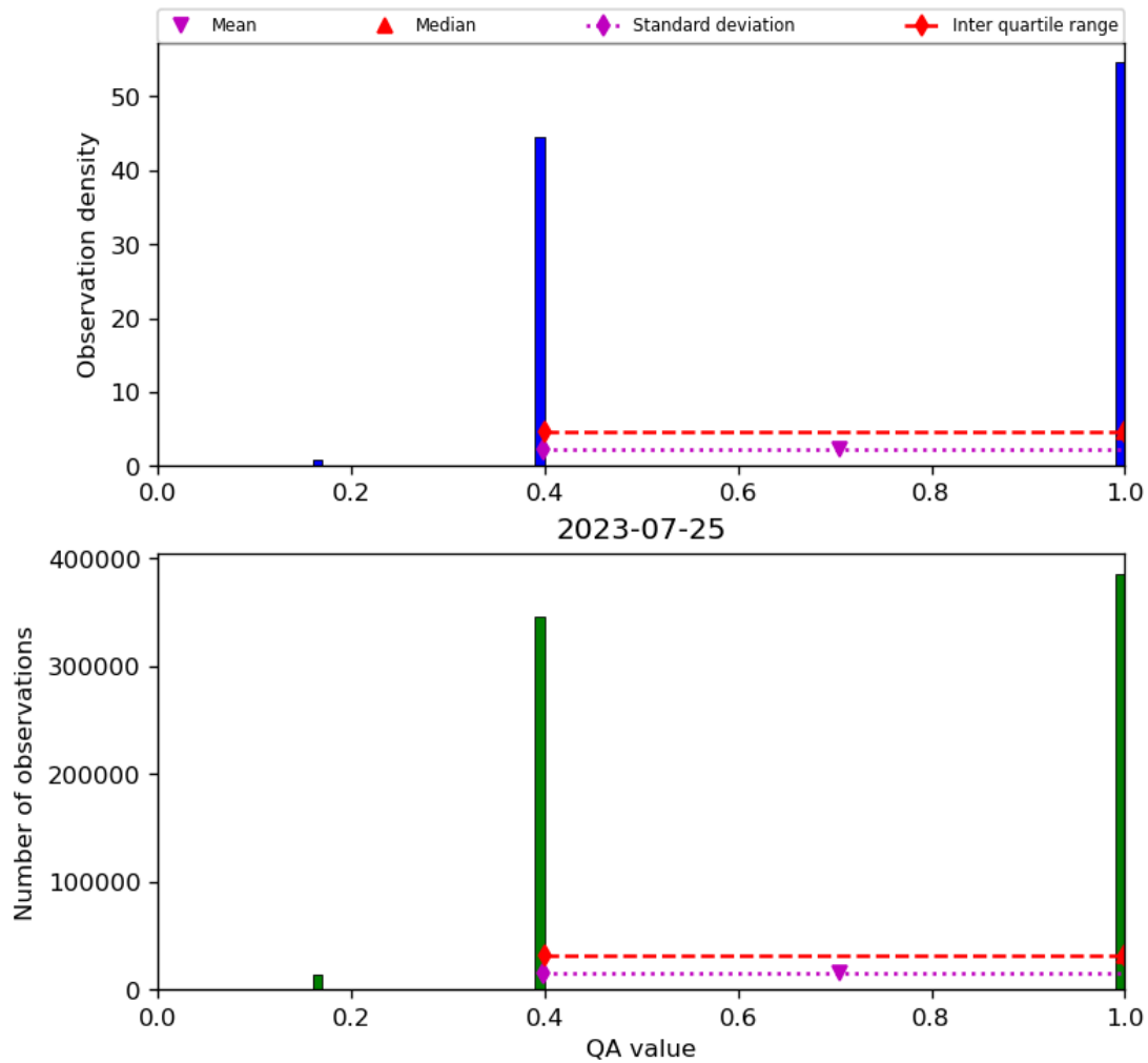
Figure 22: Histogram of “QA value” for 2023-07-24 to 2023-07-26
