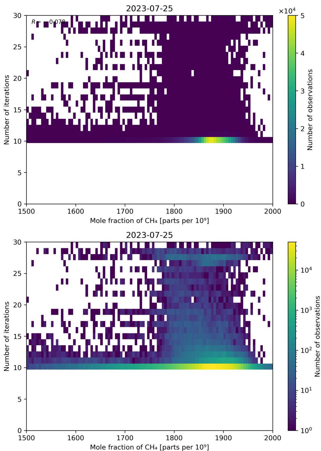
Figure 76: Scatter density plot of “Mole fraction of CH 4 ” against “Number of iterations” for 2023-07-24 to 2023-07-26.
