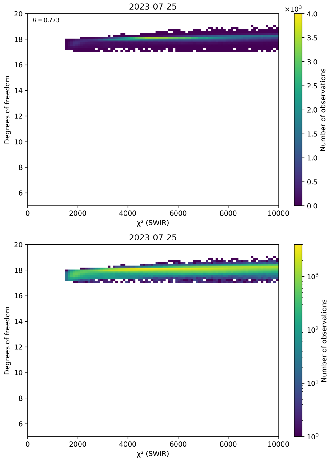
Figure 48: Scatter density plot of “ \chi^2 (SWIR)” against “Degrees of freedom” for 2023-07-24 to 2023-07-26.
