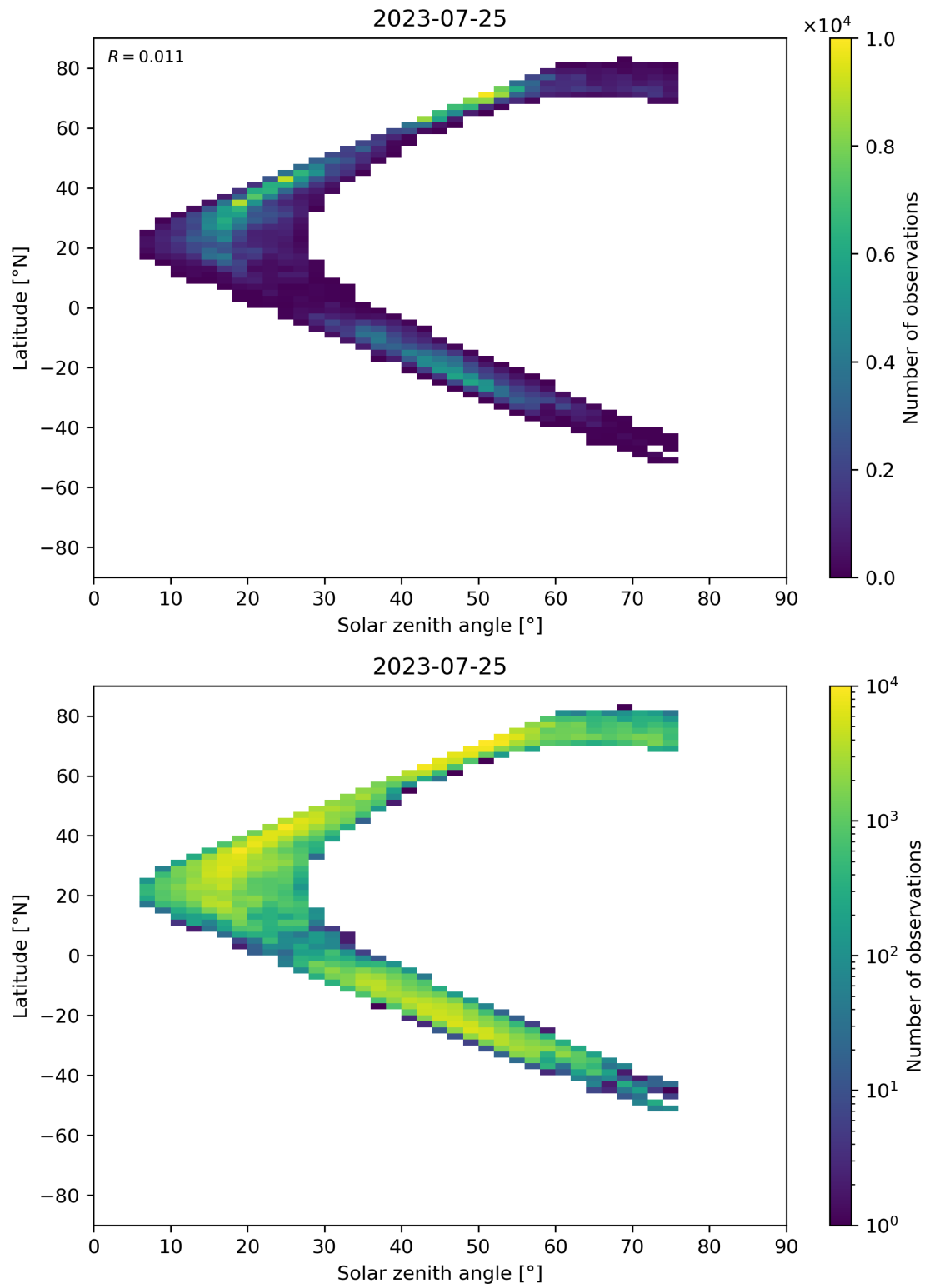
Figure 98: Scatter density plot of “Solar zenith angle” against “Latitude” for 2023-07-24 to 2023-07-26.
