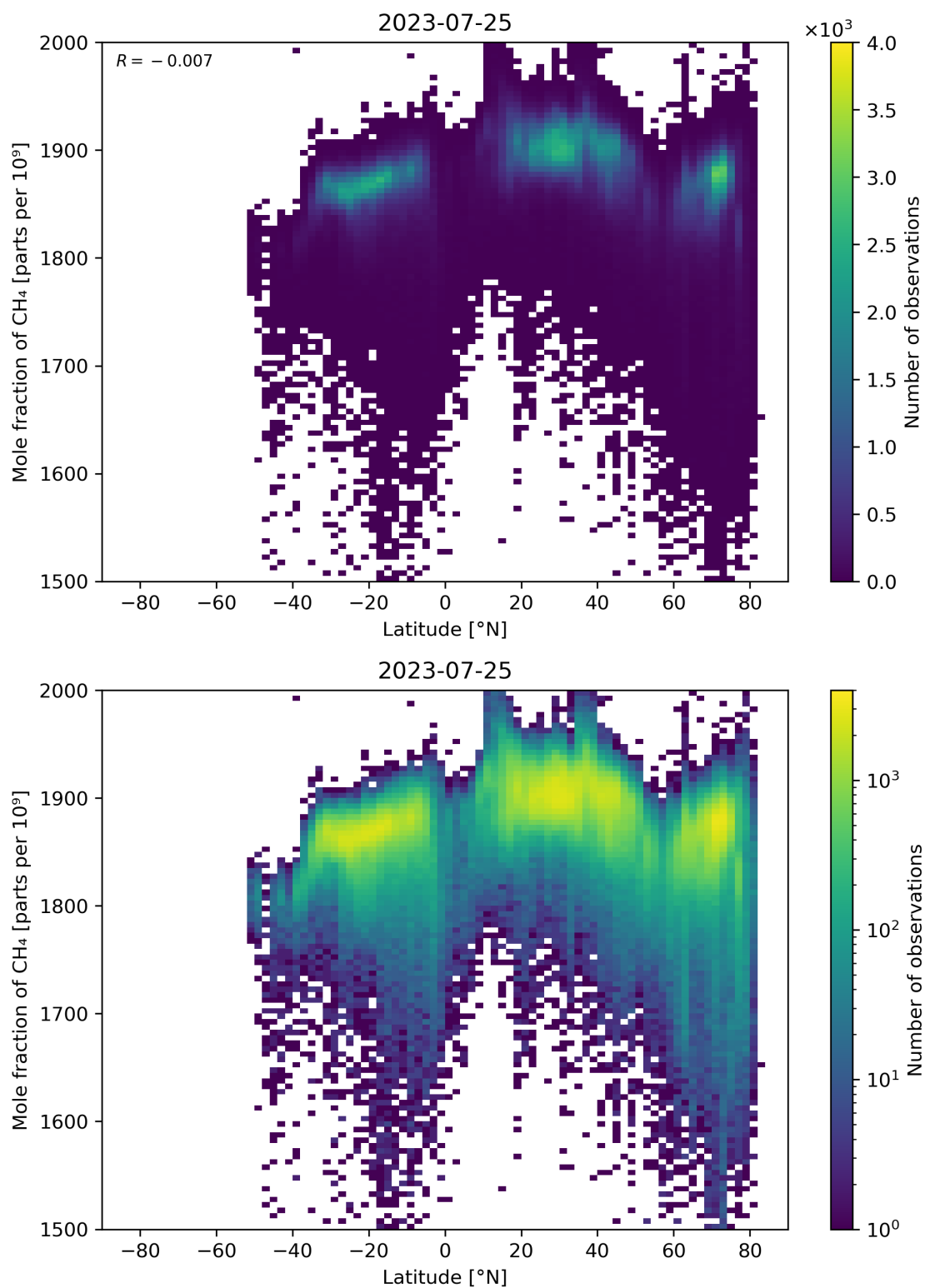
Figure 57: Scatter density plot of “Latitude” against “Mole fraction of CH 4 ” for 2023-07-24 to 2023-07-26.
