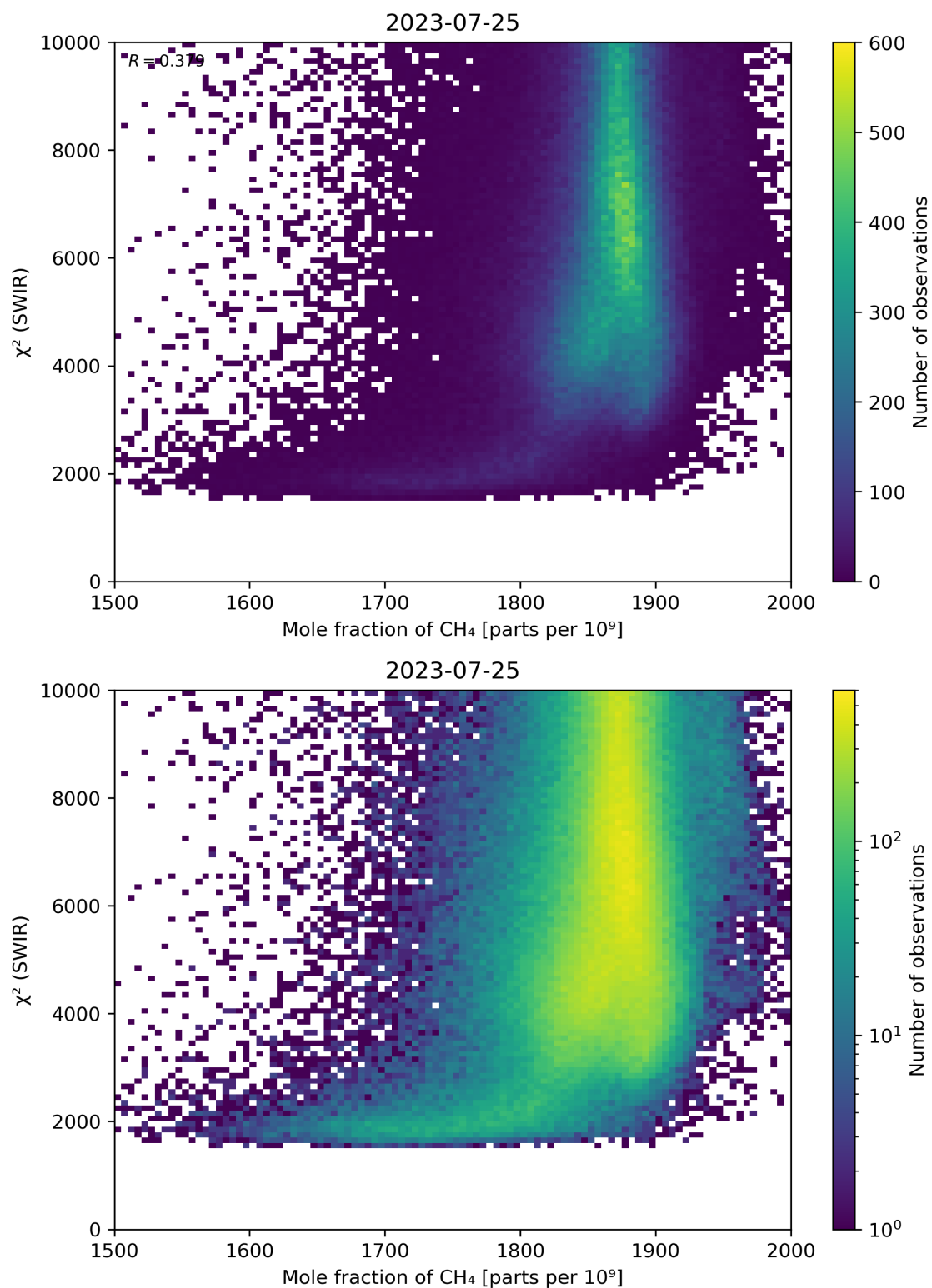
Figure 71: Scatter density plot of “Mole fraction of CH 4 ” against “ \chi^2 (SWIR)” for 2023-07-24 to 2023-07-26.
