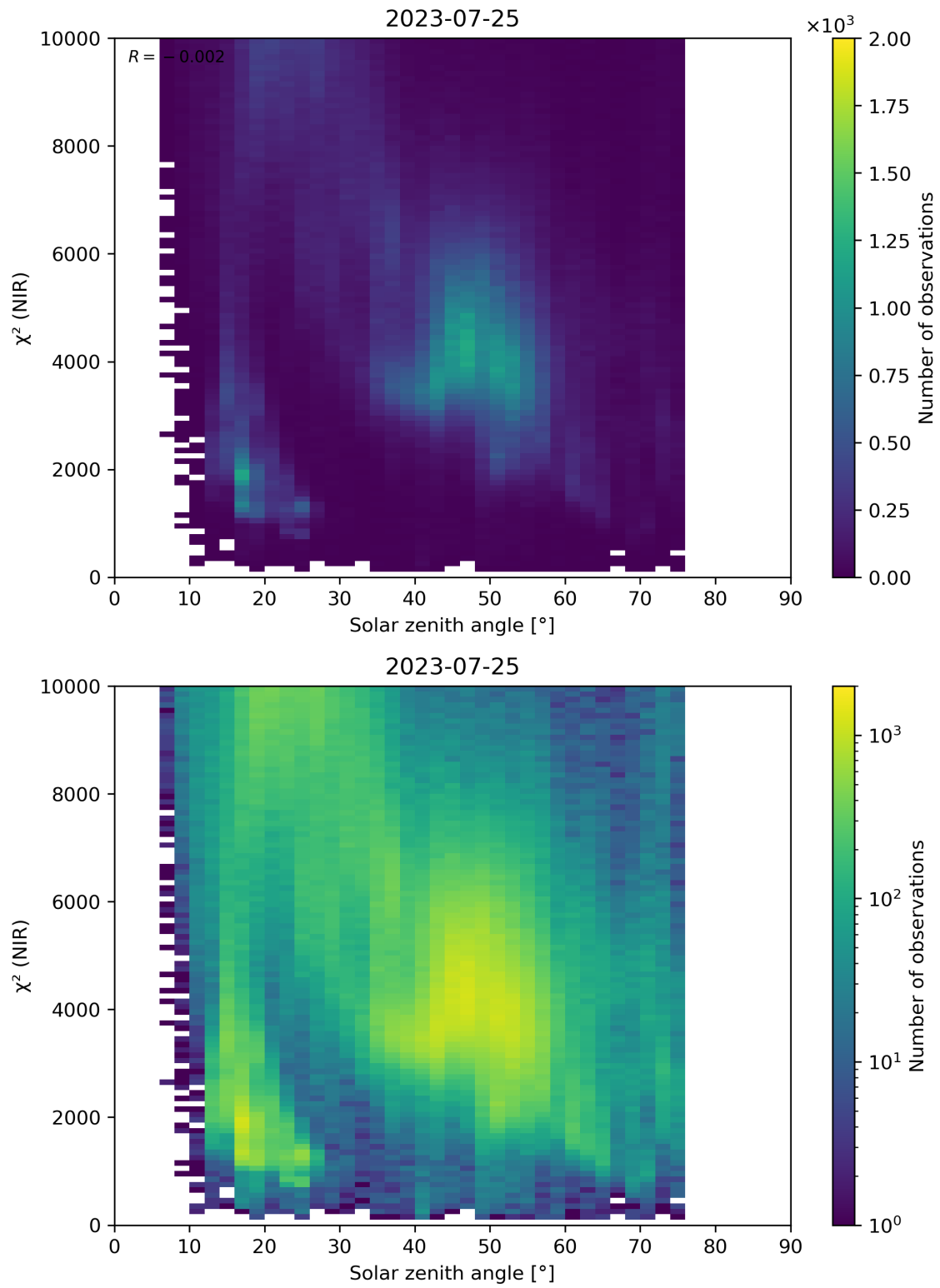
Figure 94: Scatter density plot of “Solar zenith angle” against “ \chi^2 (NIR)” for 2023-07-24 to 2023-07-26.
