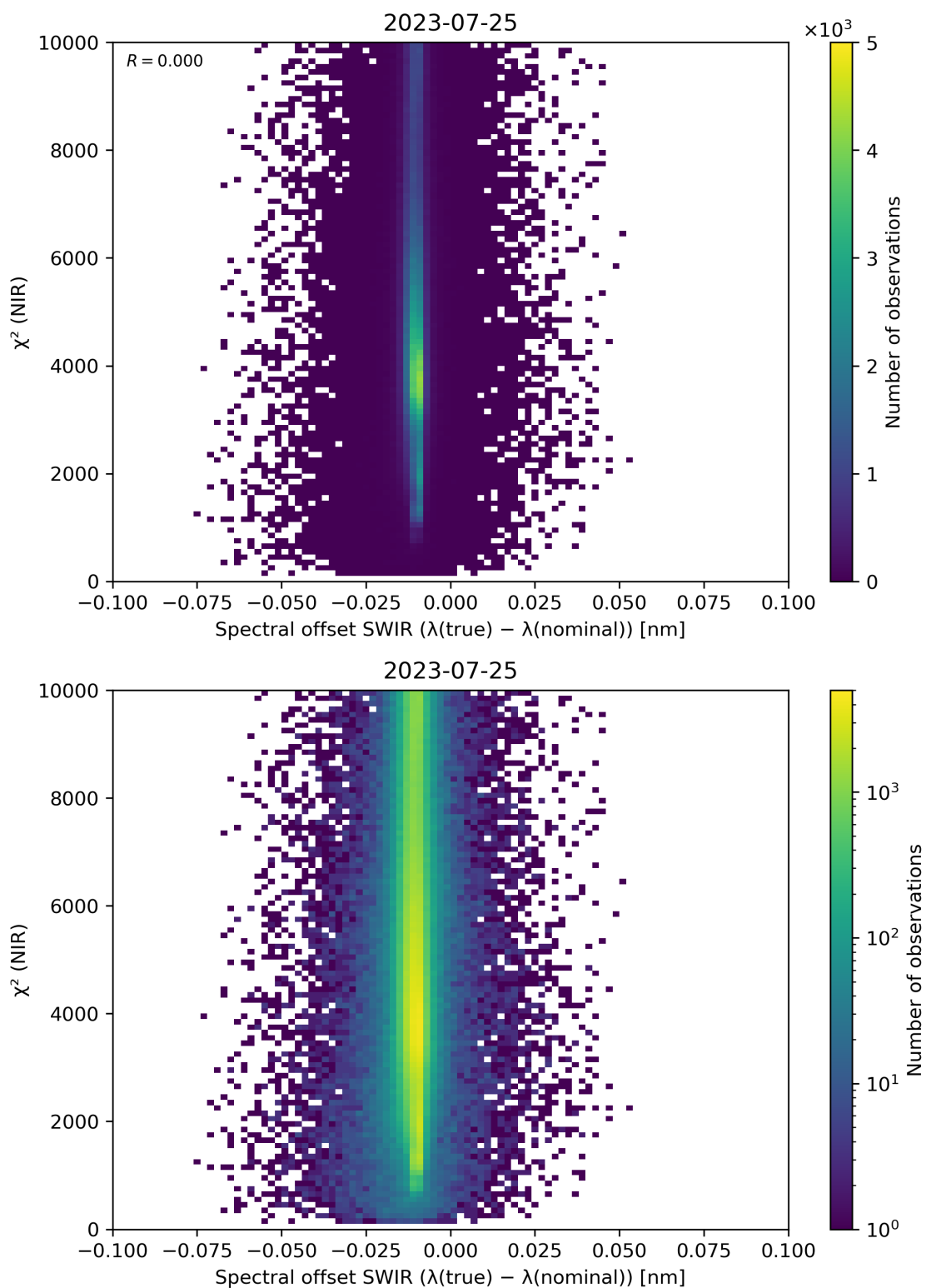
Figure 117: Scatter density plot of “Spectral offset SWIR ( \lambda(\text{true}) - \lambda(\text{nominal}) )” against “ \chi^2 (NIR)” for 2023-07-24 to 2023-07-26.
