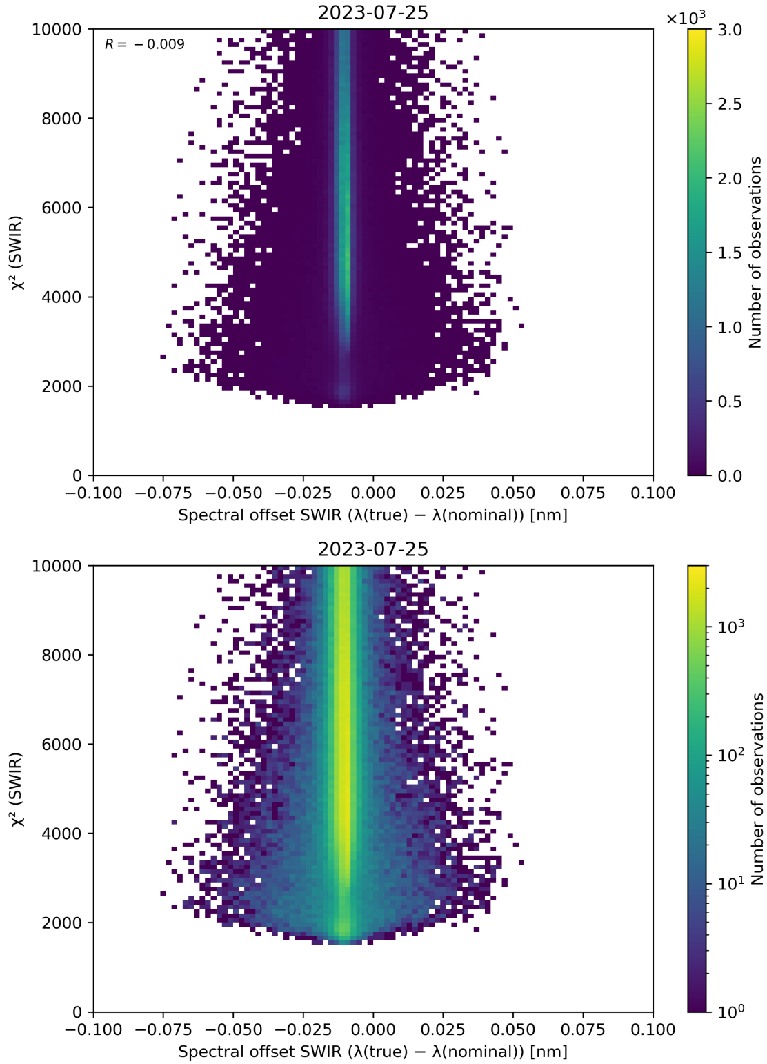
Figure 118: Scatter density plot of “Spectral offset SWIR ( \lambda(\text{true}) - \lambda(\text{nominal}) )” against “ \chi^2 (SWIR)” for 2023-07-24 to 2023-07-26.
