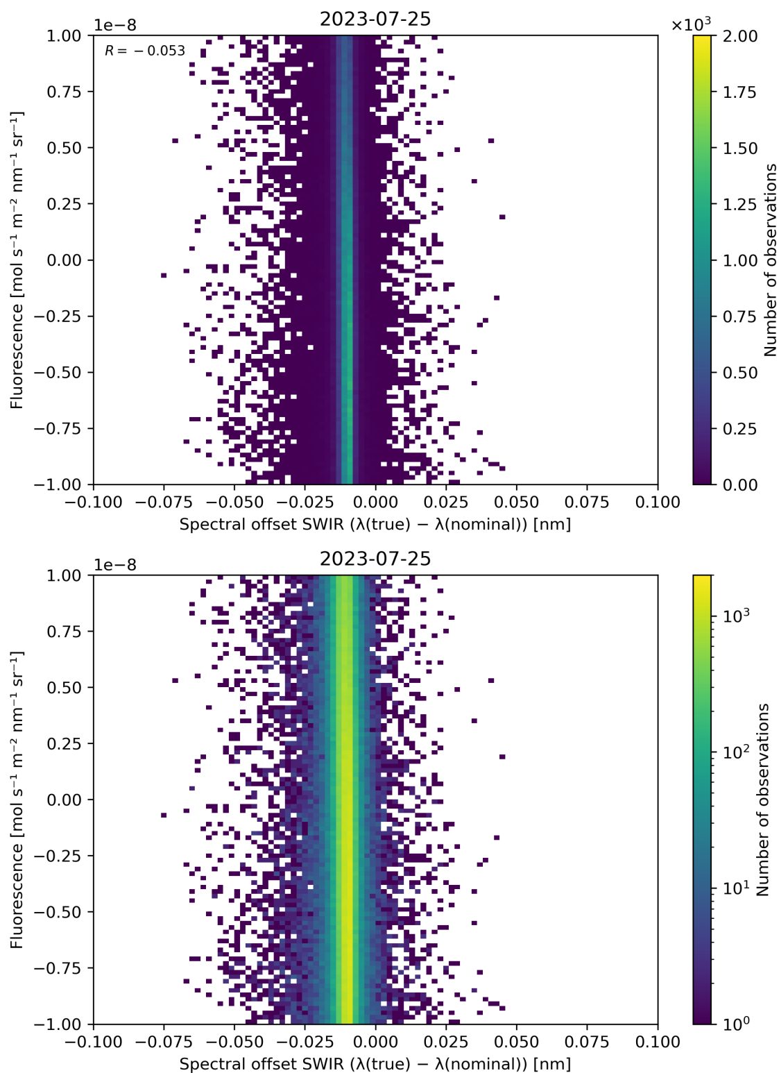
Figure 120: Scatter density plot of “Spectral offset SWIR ( \lambda(\text{true}) - \lambda(\text{nominal}) )” against “Fluorescence” for 2023-07-24 to 2023-07-26.
