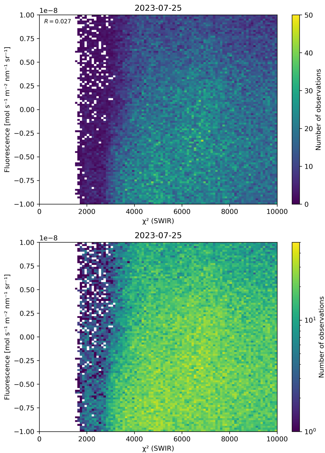
Figure 49: Scatter density plot of “ \chi^2 (SWIR)” against “Fluorescence” for 2023-07-24 to 2023-07-26.
