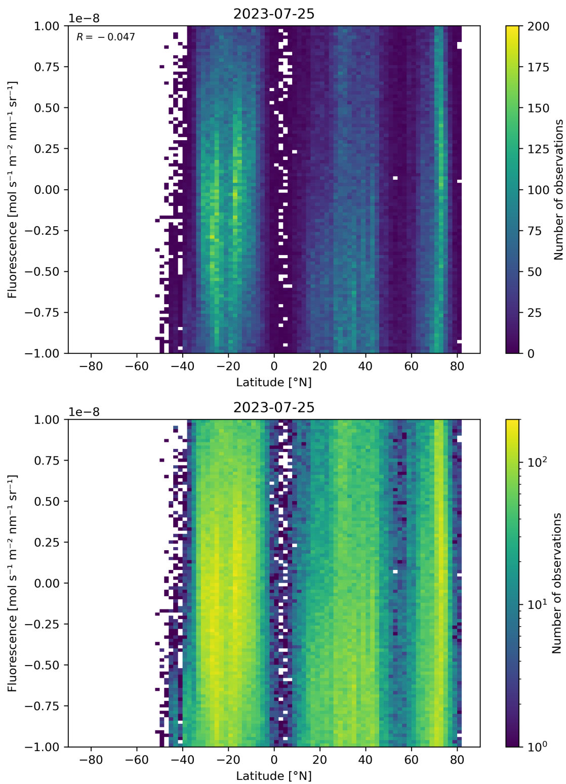
Figure 56: Scatter density plot of “Latitude” against “Fluorescence” for 2023-07-24 to 2023-07-26.
