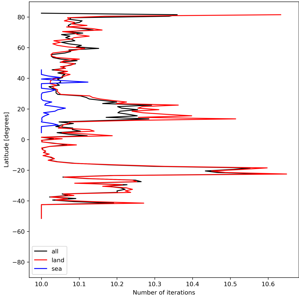
Figure 20: Zonal average of “Number of iterations” for 2023-07-24 to 2023-07-26.
