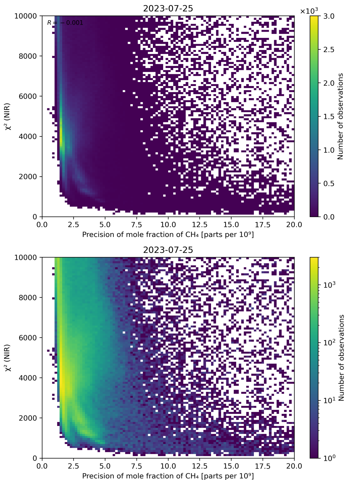
Figure 78: Scatter density plot of “Precision of mole fraction of CH 4 ” against “ \chi^2 (NIR)” for 2023-07-24 to 2023-07-26.
