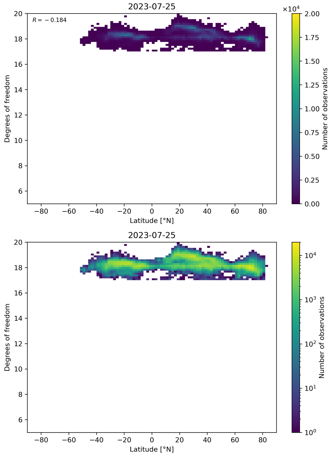
Figure 55: Scatter density plot of “Latitude” against “Degrees of freedom” for 2023-07-24 to 2023-07-26.
