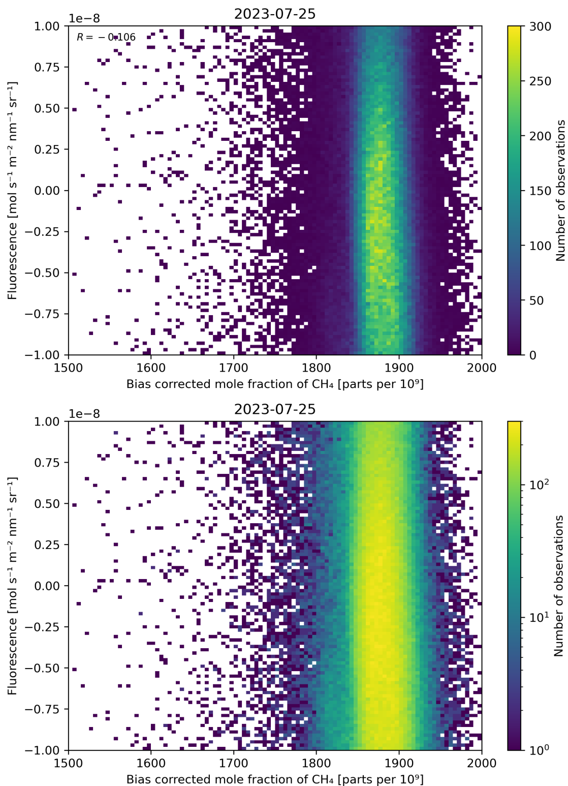
Figure 66: Scatter density plot of “Bias corrected mole fraction of \text{CH}_4 ” against “Fluorescence” for 2023-07-24 to 2023-07-26.
