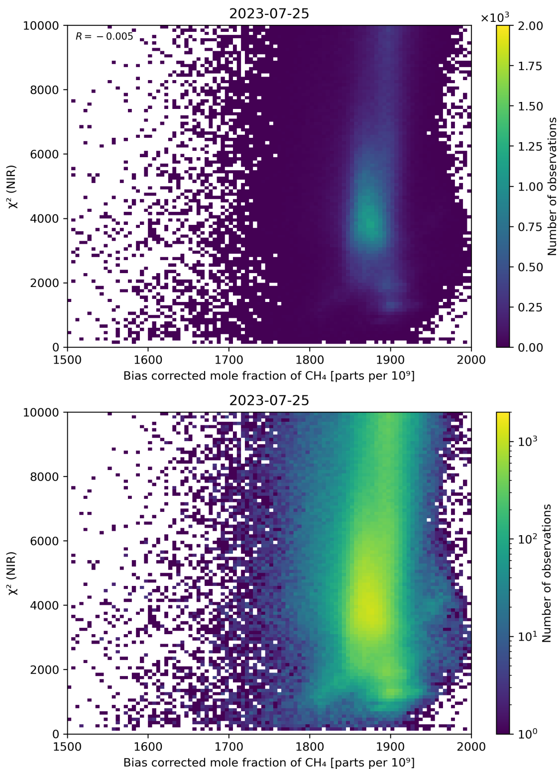
Figure 63: Scatter density plot of “Bias corrected mole fraction of CH 4 ” against “ \chi^2 (NIR)” for 2023-07-24 to 2023-07-26.
