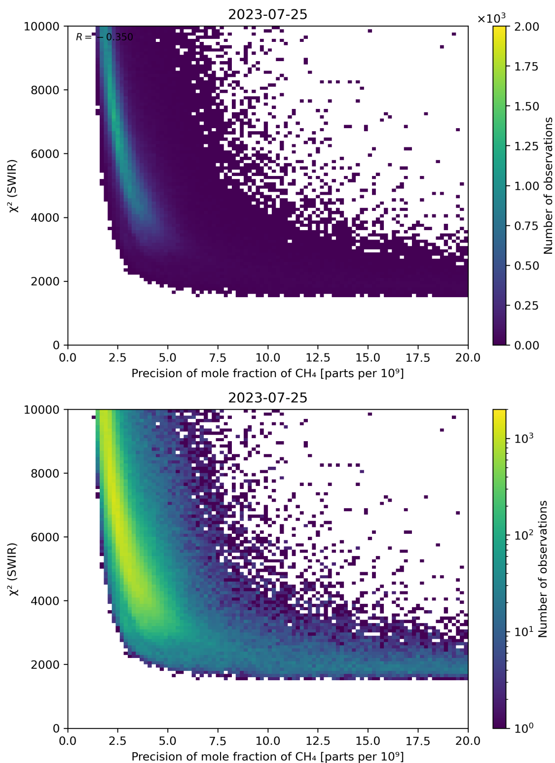
Figure 79: Scatter density plot of “Precision of mole fraction of CH 4 ” against “ \chi^2 (SWIR)” for 2023-07-24 to 2023-07-26.
