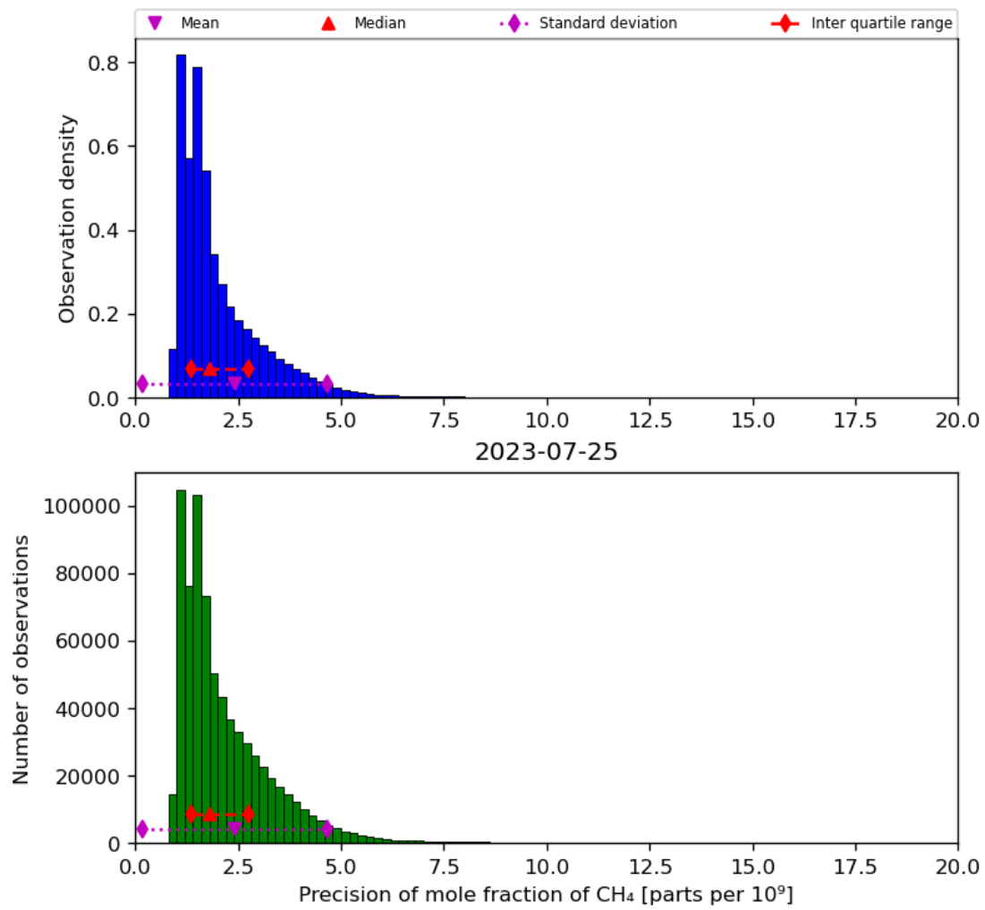
Figure 24: Histogram of “Precision of mole fraction of CH 4 ” for 2023-07-24 to 2023-07-26
