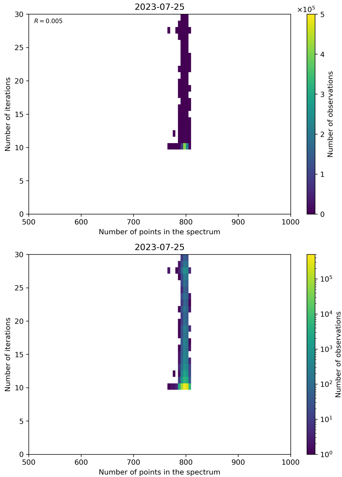
Figure 92: Scatter density plot of “Number of points in the spectrum” against “Number of iterations” for 2023-07-24 to 2023-07-26.
