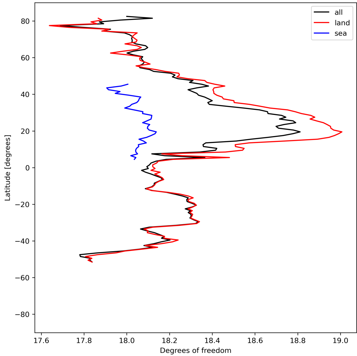
Figure 19: Zonal average of “Degrees of freedom” for 2023-07-24 to 2023-07-26.
