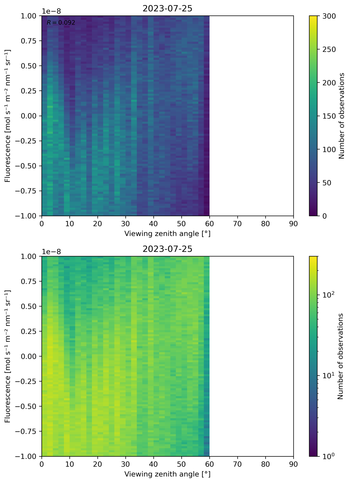
Figure 108: Scatter density plot of “Viewing zenith angle” against “Fluorescence” for 2023-07-24 to 2023-07-26.
