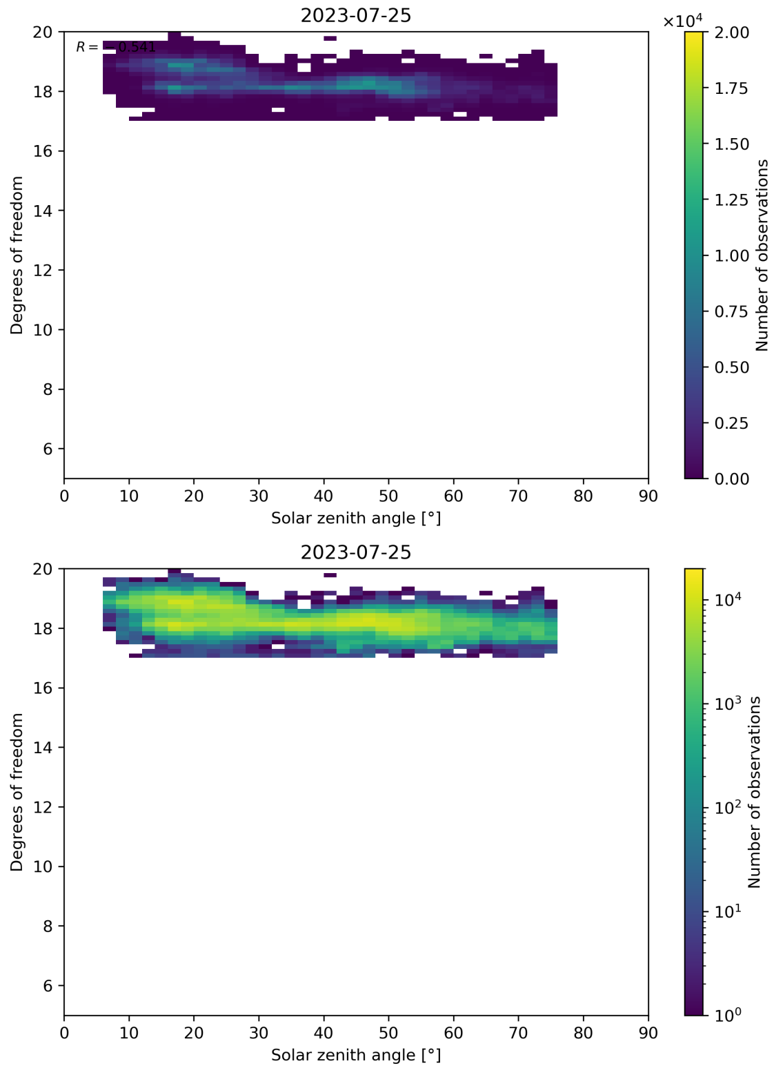
Figure 96: Scatter density plot of “Solar zenith angle” against “Degrees of freedom” for 2023-07-24 to 2023-07-26.
