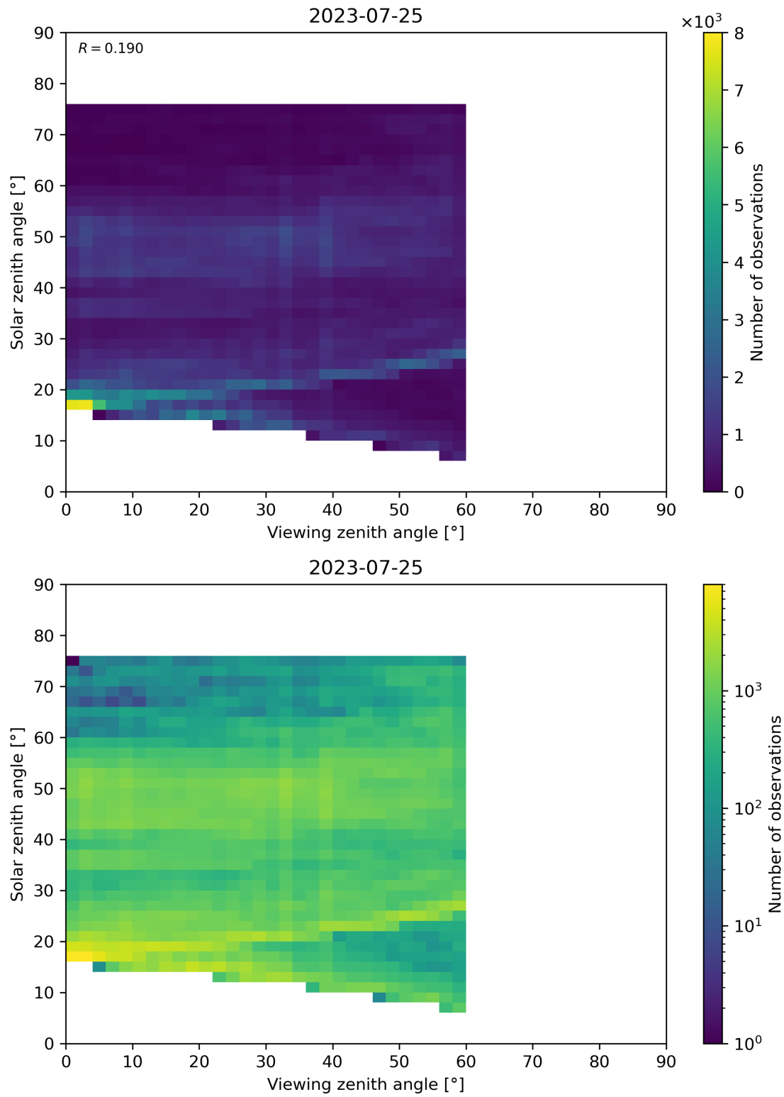
Figure 115: Scatter density plot of “Viewing zenith angle” against “Solar zenith angle” for 2023-07-24 to 2023-07-26.
