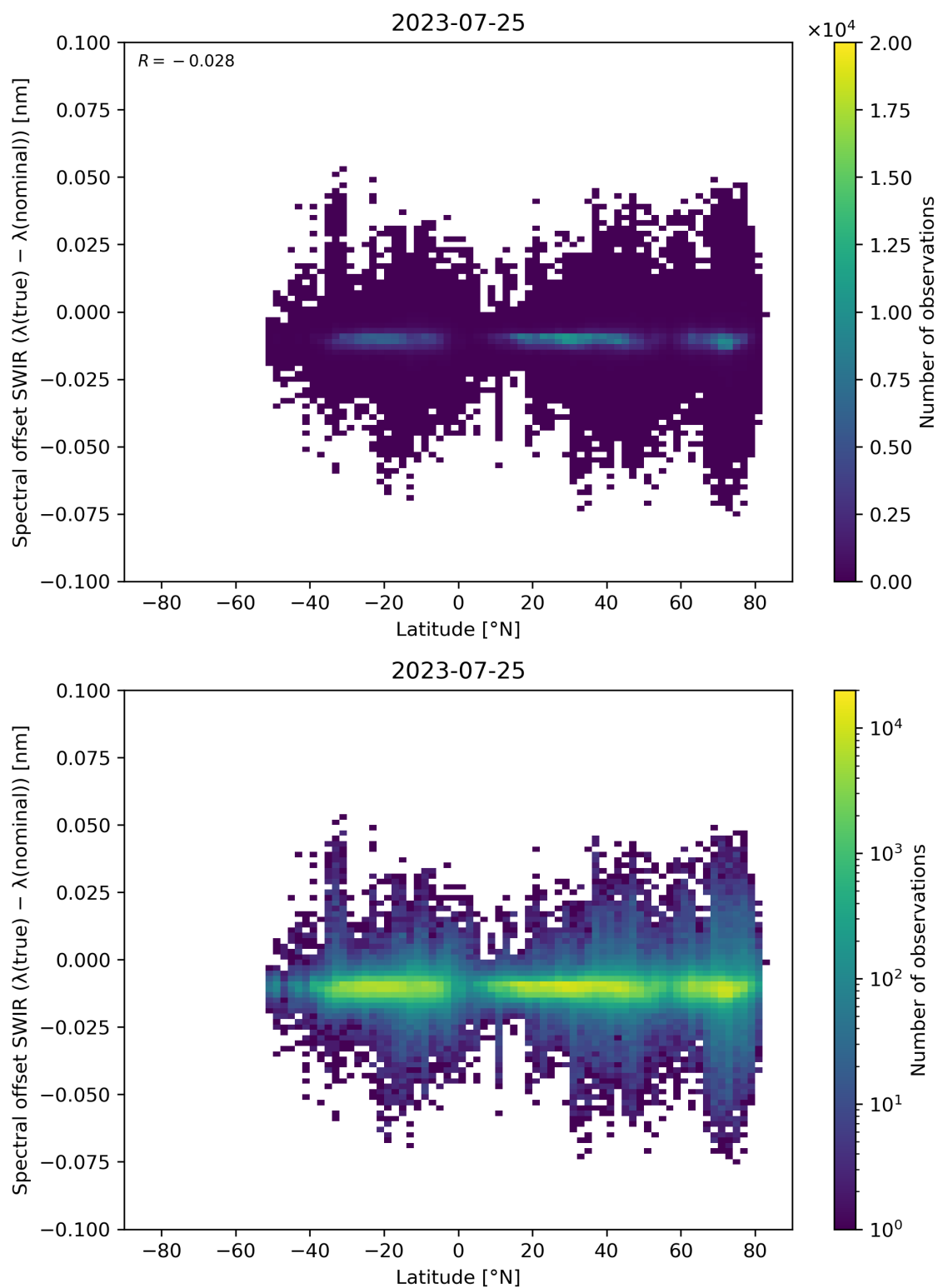
Figure 62: Scatter density plot of “Latitude” against “Spectral offset SWIR ( \lambda(\text{true}) - \lambda(\text{nominal}) )” for 2023-07-24 to 2023-07-26.
