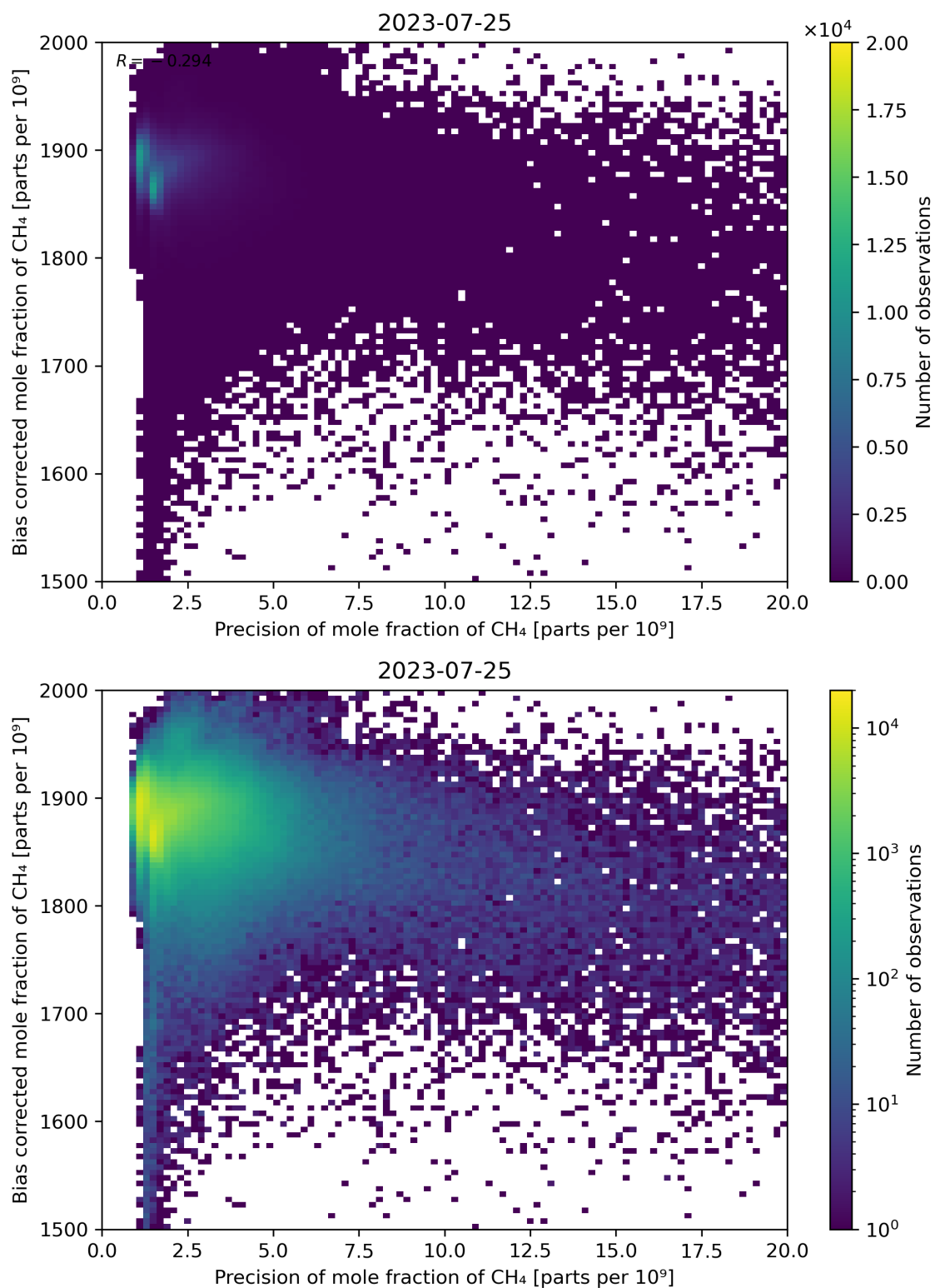
Figure 82: Scatter density plot of “Precision of mole fraction of CH 4 ” against “Bias corrected mole fraction of CH 4 ” for 2023-07-24 to 2023-07-26.
