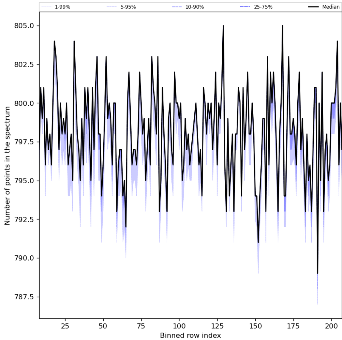
Figure 37: Along track statistics of “Number of points in the spectrum” for 2023-07-24 to 2023-07-26
