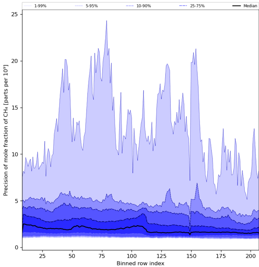
Figure 35: Along track statistics of “Precision of mole fraction of CH 4 ” for 2023-07-24 to 2023-07-26
