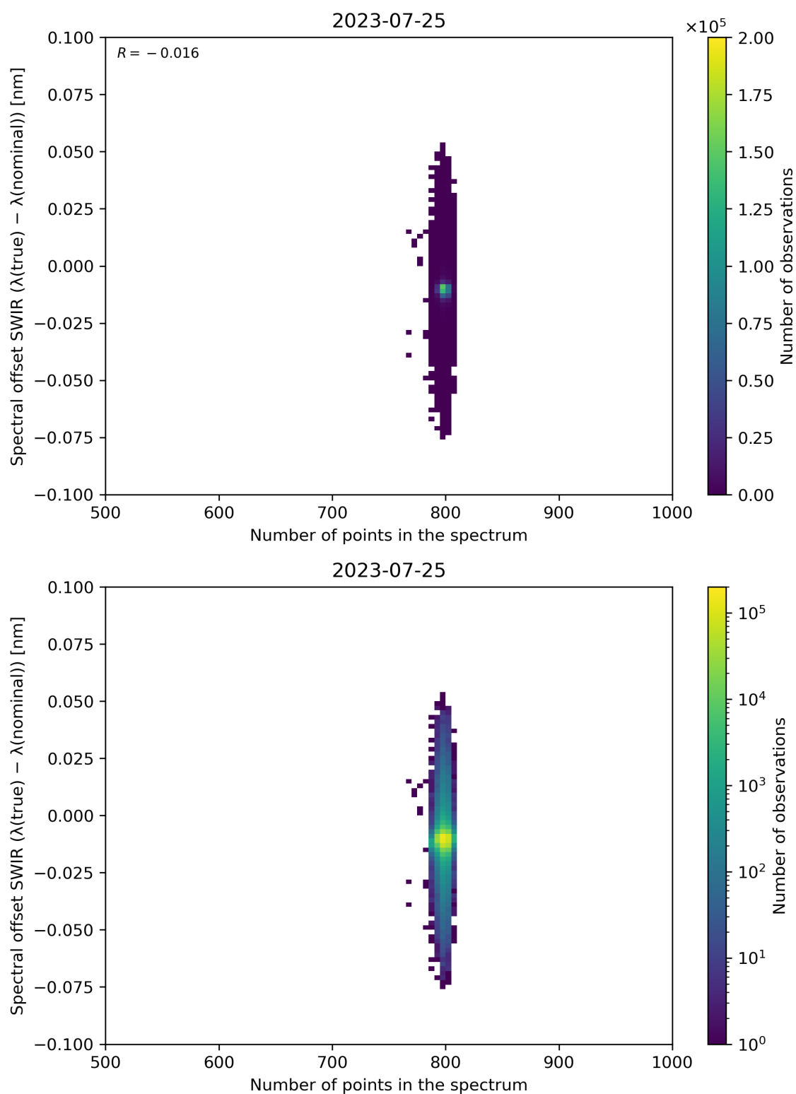
Figure 93: Scatter density plot of “Number of points in the spectrum” against “Spectral offset SWIR ( \lambda(\text{true}) - \lambda(\text{nominal}) )” for 2023-07-24 to 2023-07-26.
