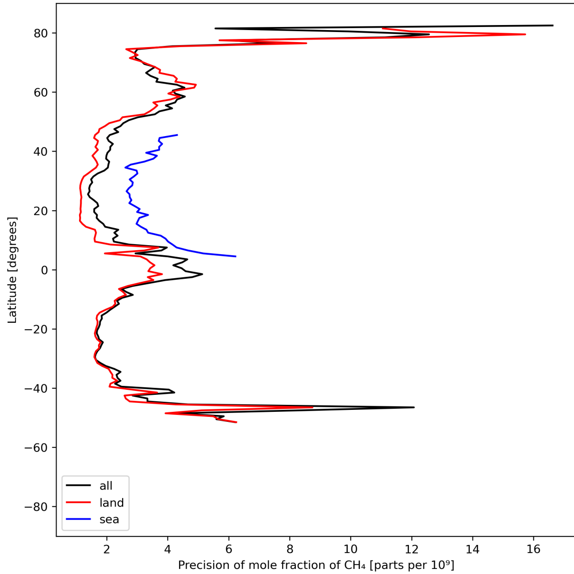
Figure 13: Zonal average of “Precision of mole fraction of CH 4 ” for 2023-07-24 to 2023-07-26.
