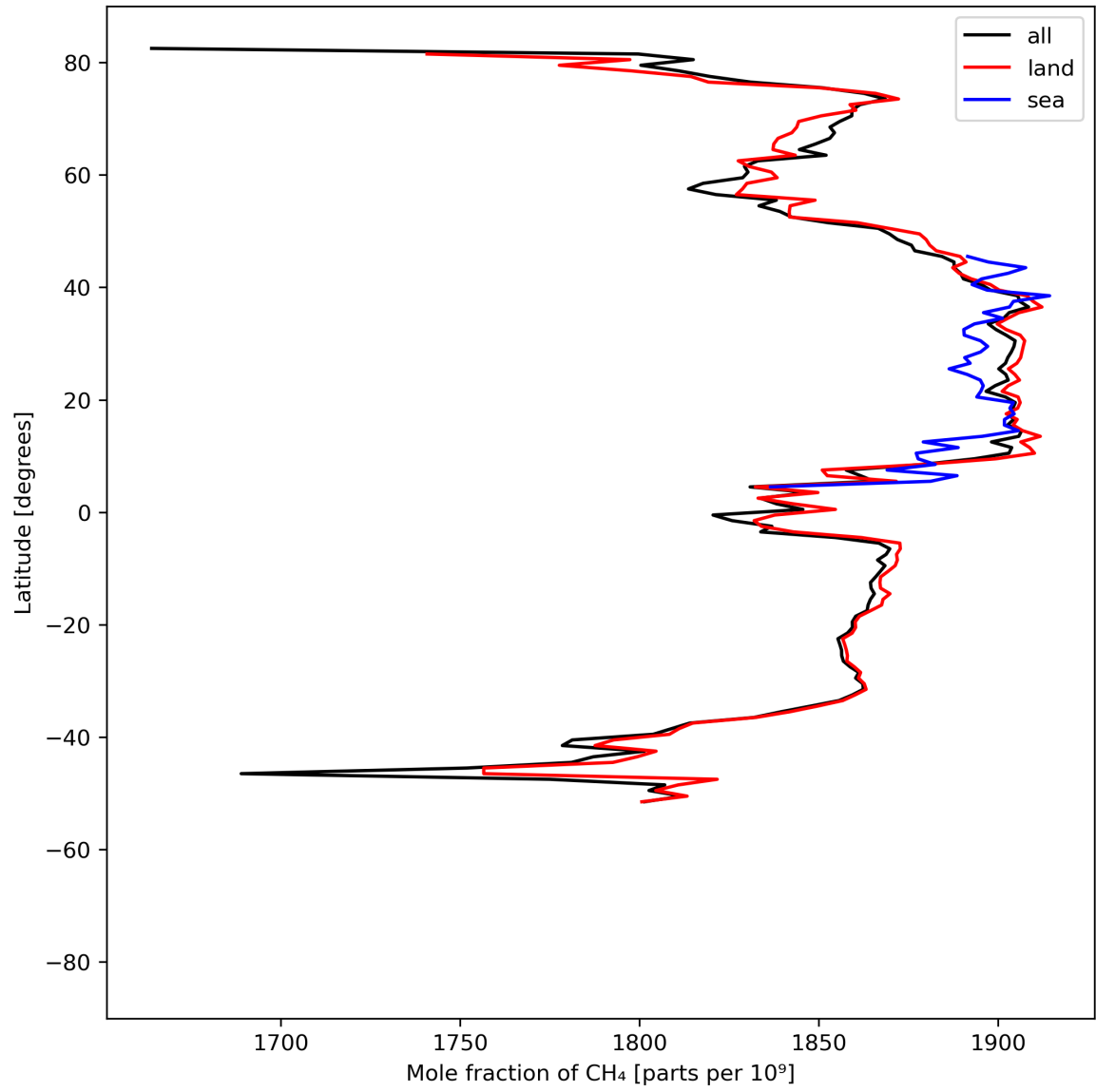
Figure 12: Zonal average of “Mole fraction of \text{CH}_4 ” for 2023-07-24 to 2023-07-26.
