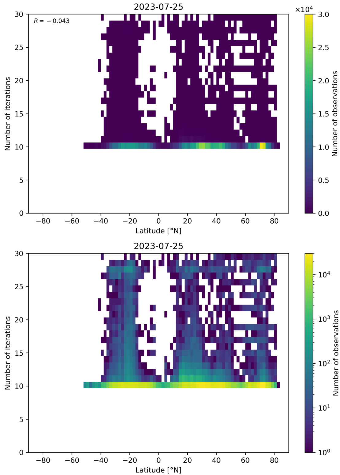
Figure 60: Scatter density plot of “Latitude” against “Number of iterations” for 2023-07-24 to 2023-07-26.
