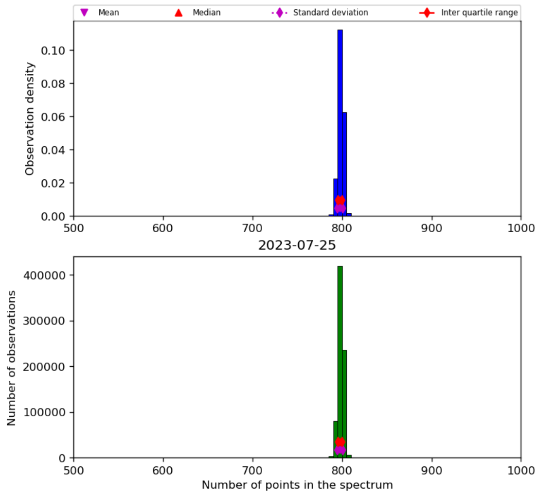
Figure 26: Histogram of “Number of points in the spectrum” for 2023-07-24 to 2023-07-26
