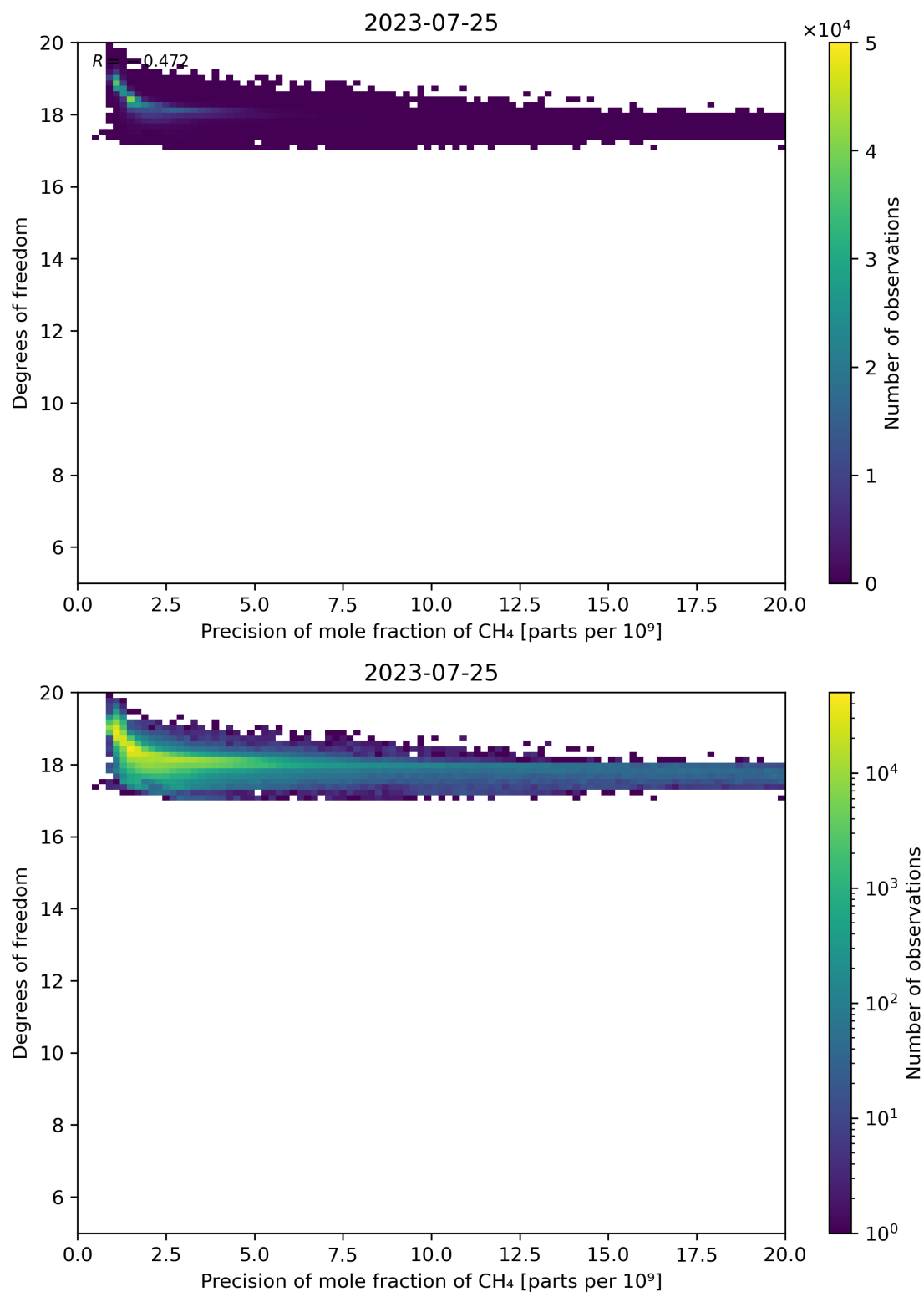
Figure 80: Scatter density plot of “Precision of mole fraction of CH 4 ” against “Degrees of freedom” for 2023-07-24 to 2023-07-26.
