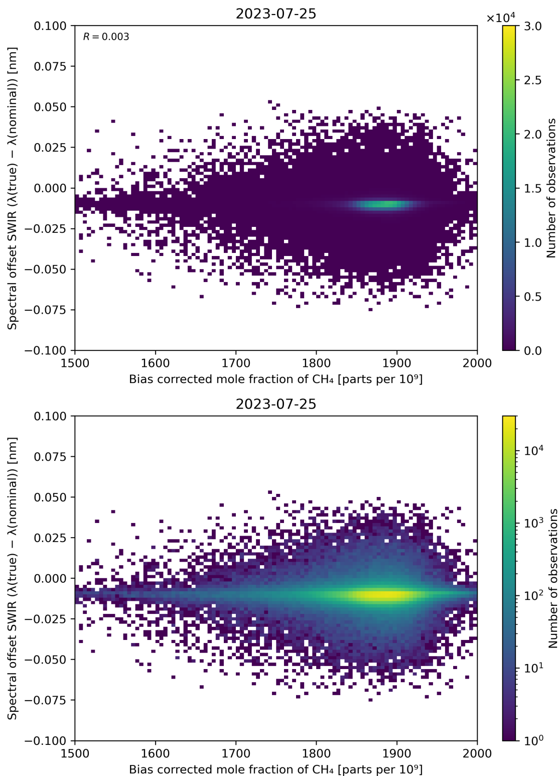
Figure 69: Scatter density plot of “Bias corrected mole fraction of \text{CH}_4 ” against “Spectral offset SWIR ( \lambda(\text{true}) - \lambda(\text{nominal}) )” for 2023-07-24 to 2023-07-26.
