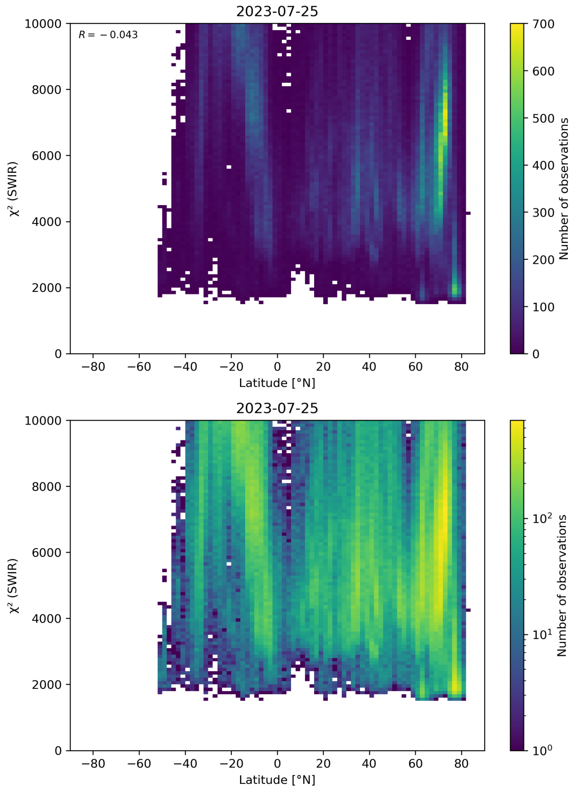
Figure 54: Scatter density plot of “Latitude” against “ \chi^2 (SWIR)” for 2023-07-24 to 2023-07-26.
