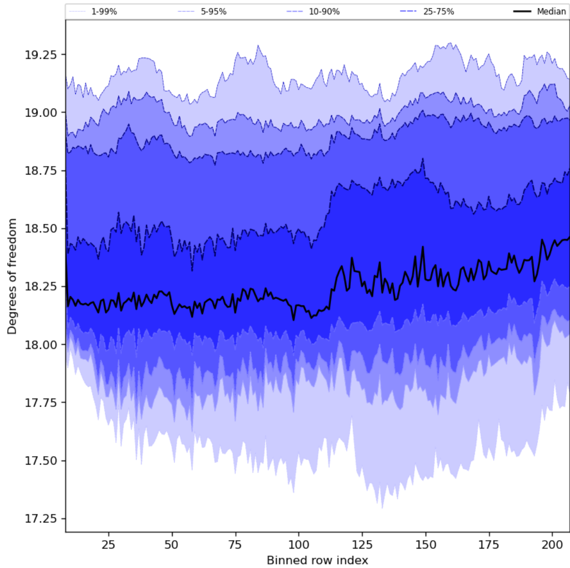
Figure 41: Along track statistics of “Degrees of freedom” for 2023-07-24 to 2023-07-26
