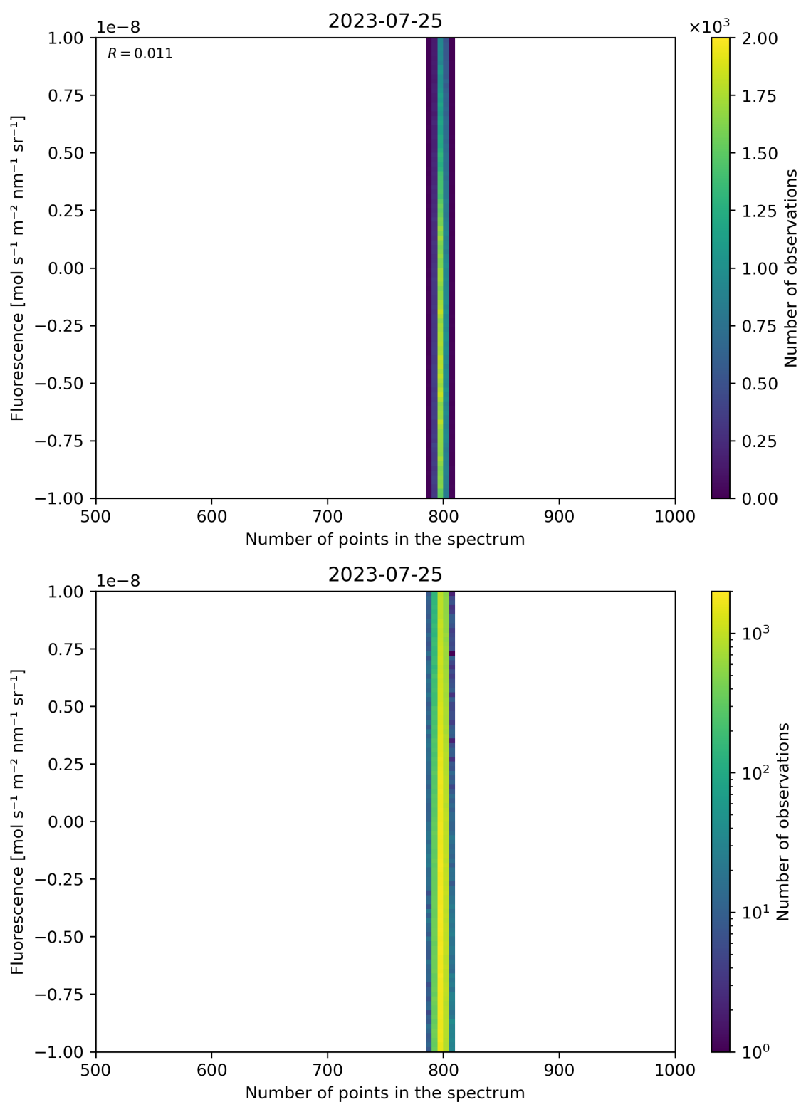
Figure 91: Scatter density plot of “Number of points in the spectrum” against “Fluorescence” for 2023-07-24 to 2023-07-26.
