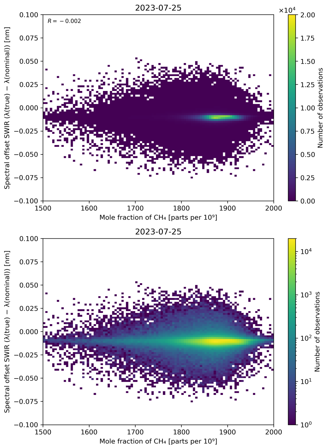
Figure 86: Scatter density plot of “Mole fraction of CH 4 ” against “Spectral offset SWIR ( \lambda(\text{true}) - \lambda(\text{nominal}) )” for 2023-07-24 to 2023-07-26.
