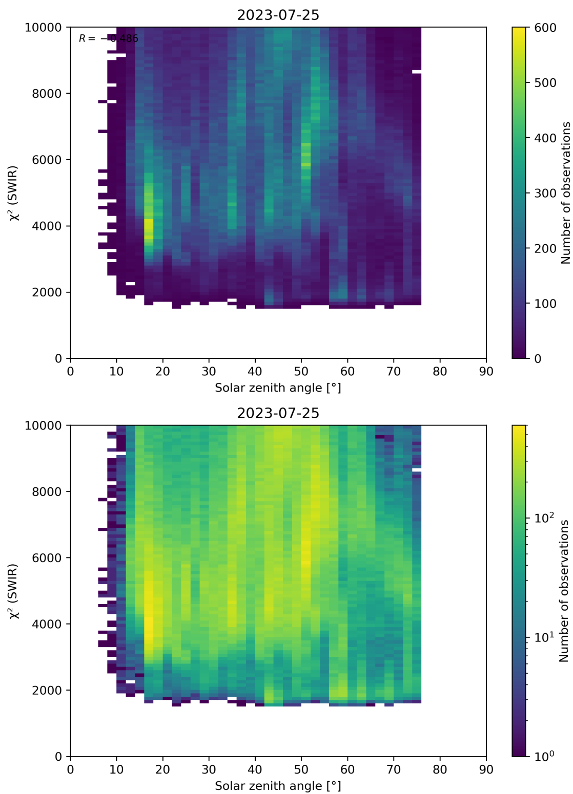
Figure 95: Scatter density plot of “Solar zenith angle” against “ \chi^2 (SWIR)” for 2023-07-24 to 2023-07-26.
