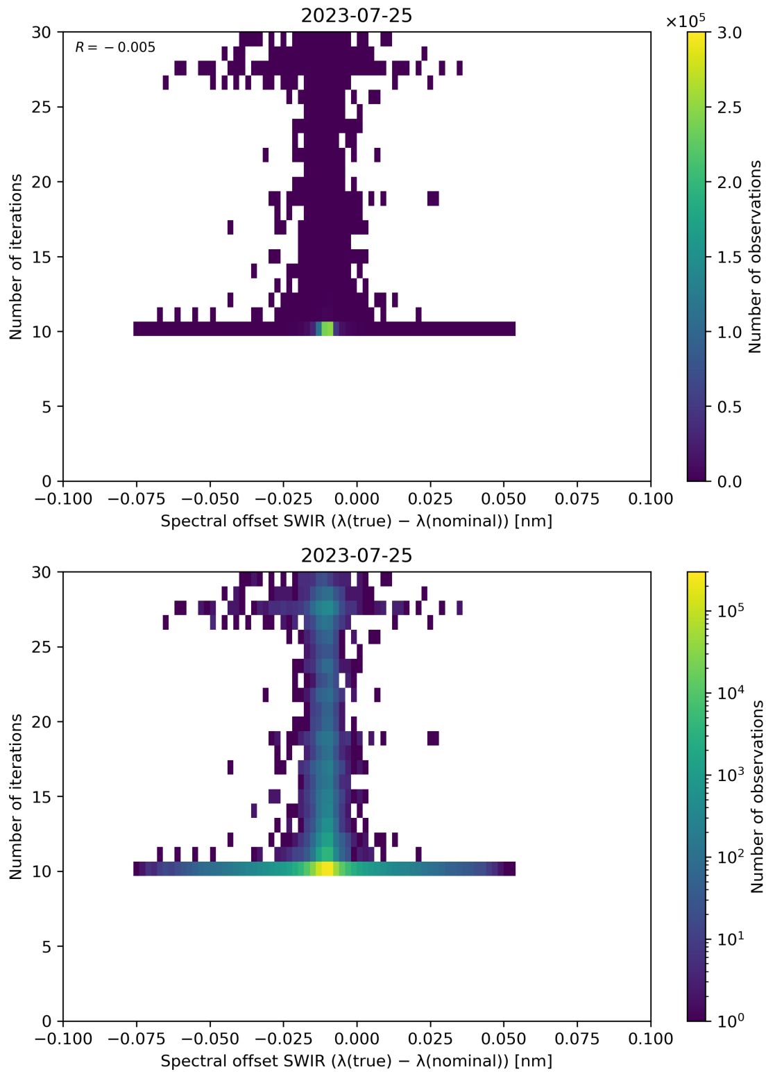
Figure 121: Scatter density plot of “Spectral offset SWIR ( \lambda(\text{true}) - \lambda(\text{nominal}) )” against “Number of iterations” for 2023-07-24 to 2023-07-26.
