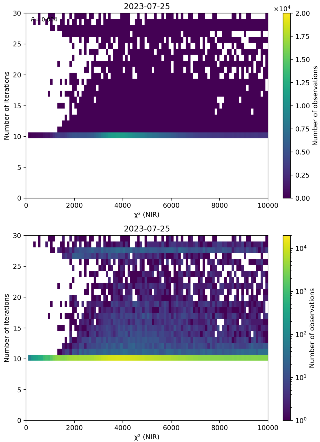
Figure 46: Scatter density plot of “ \chi^2 (NIR)” against “Number of iterations” for 2023-07-24 to 2023-07-26.
