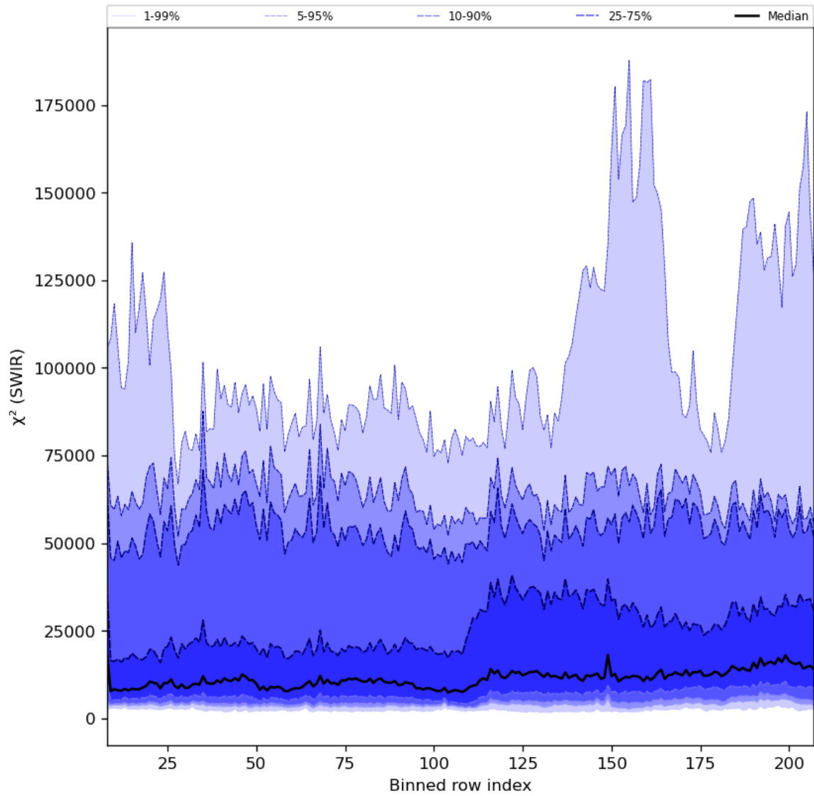
Figure 39: Along track statistics of " \chi^2 (SWIR)" for 2023-07-24 to 2023-07-26
