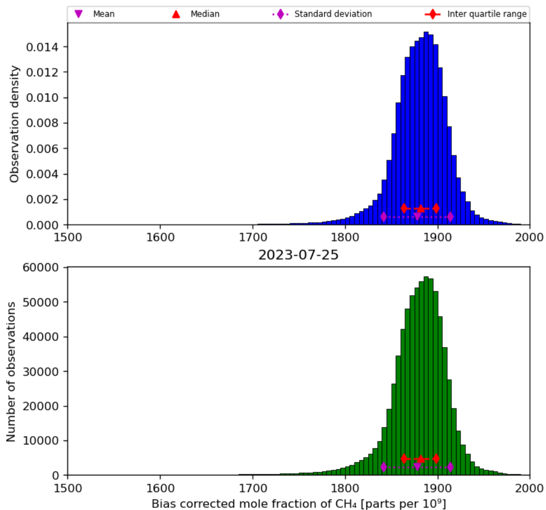
Figure 25: Histogram of “Bias corrected mole fraction of CH 4 ” for 2023-07-24 to 2023-07-26
