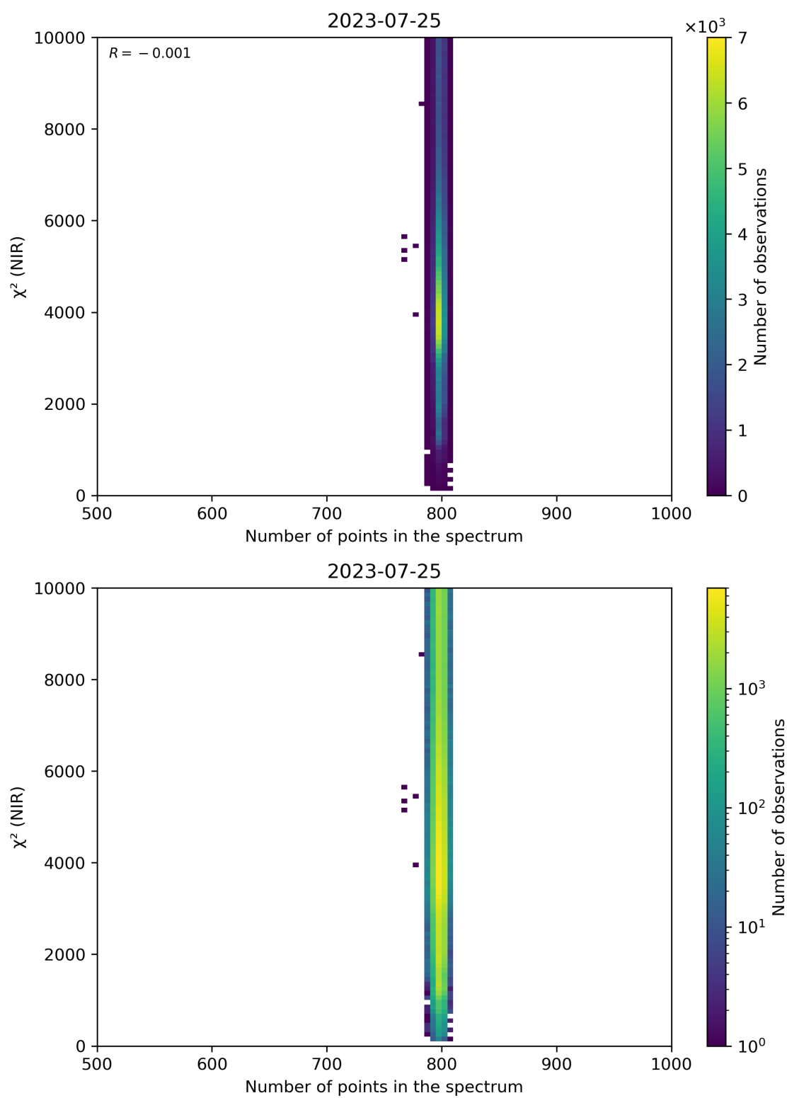
Figure 88: Scatter density plot of “Number of points in the spectrum” against “ \chi^2 (NIR)” for 2023-07-24 to 2023-07-26.
