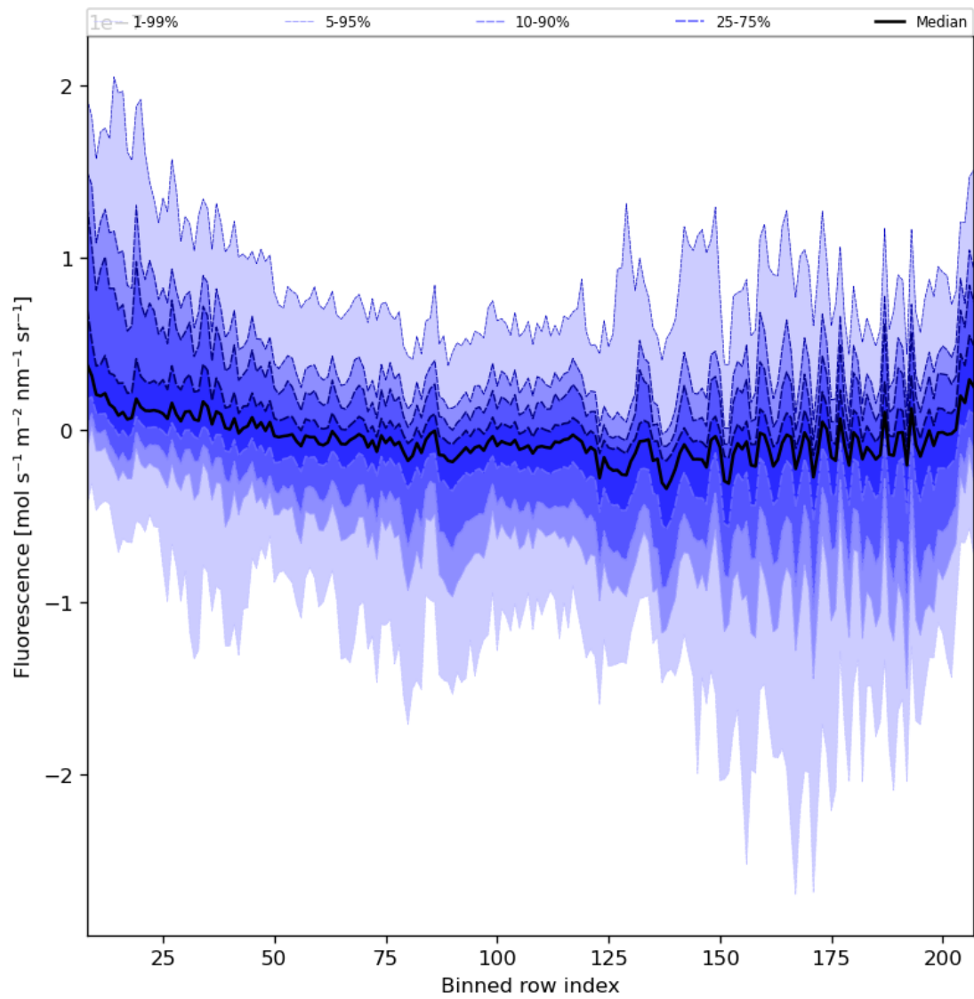
Figure 43: Along track statistics of “Fluorescence” for 2023-07-24 to 2023-07-26
