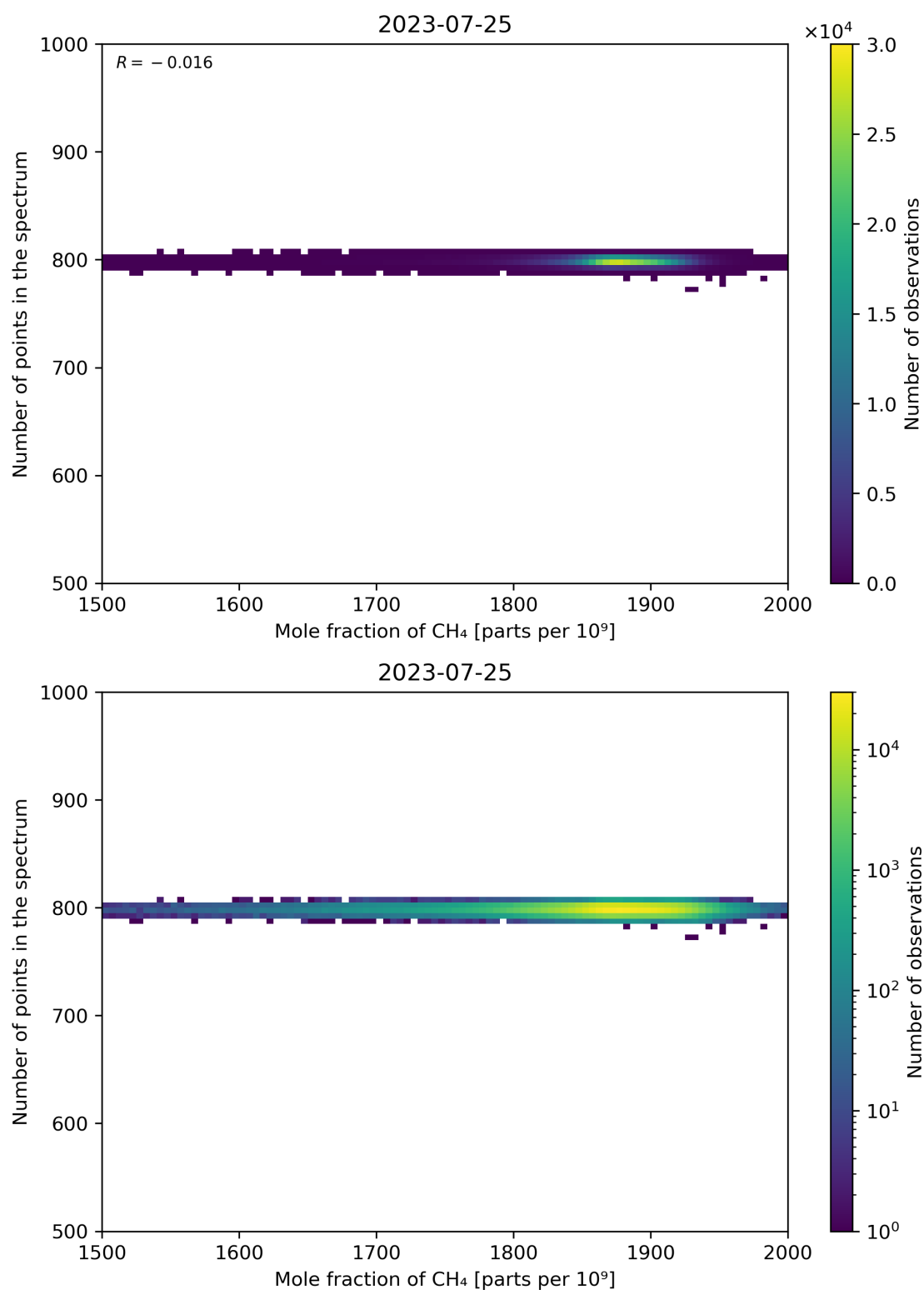
Figure 77: Scatter density plot of “Mole fraction of CH 4 ” against “Number of points in the spectrum” for 2023-07-24 to 2023-07-26.
