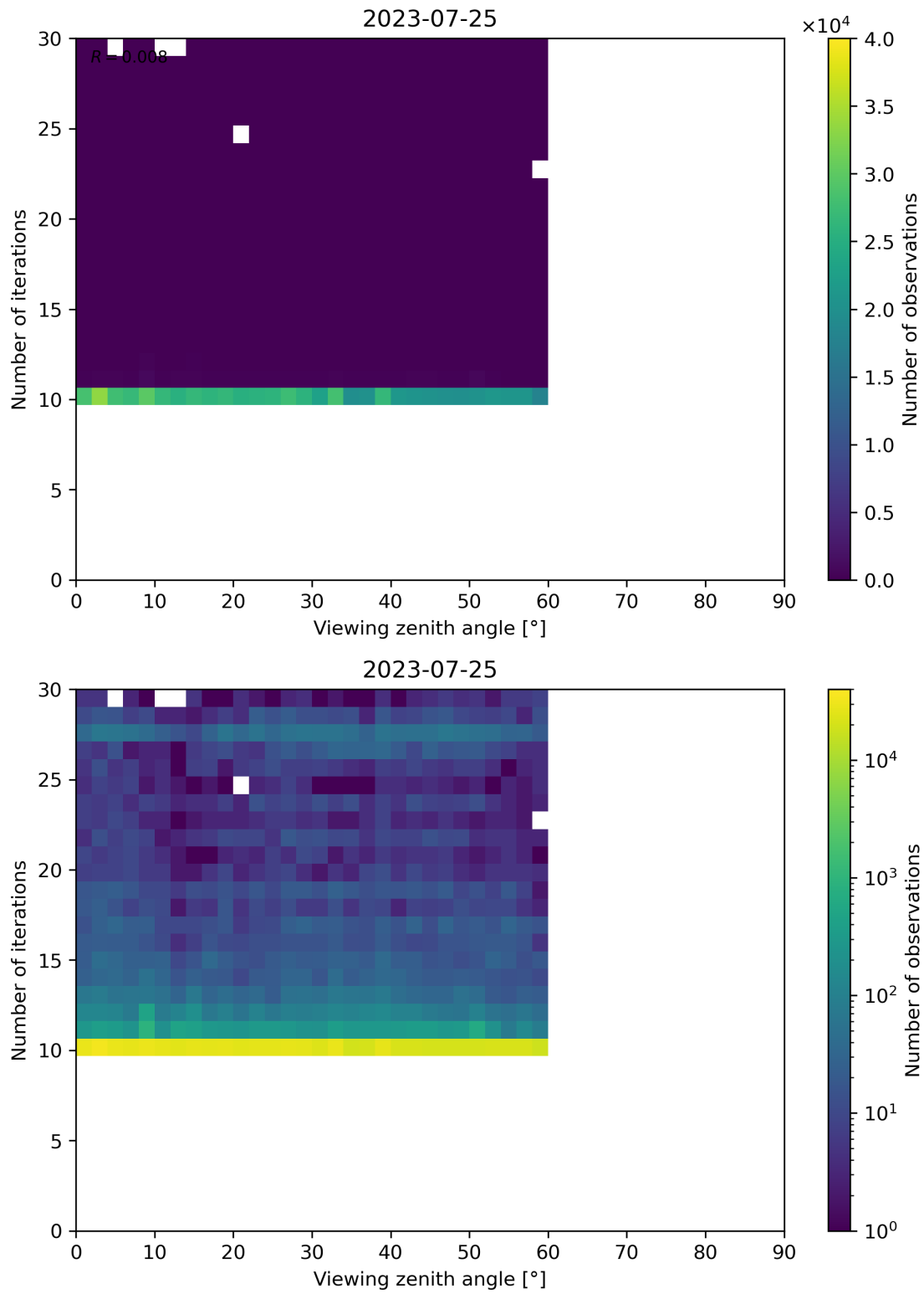
Figure 113: Scatter density plot of “Viewing zenith angle” against “Number of iterations” for 2023-07-24 to 2023-07-26.
