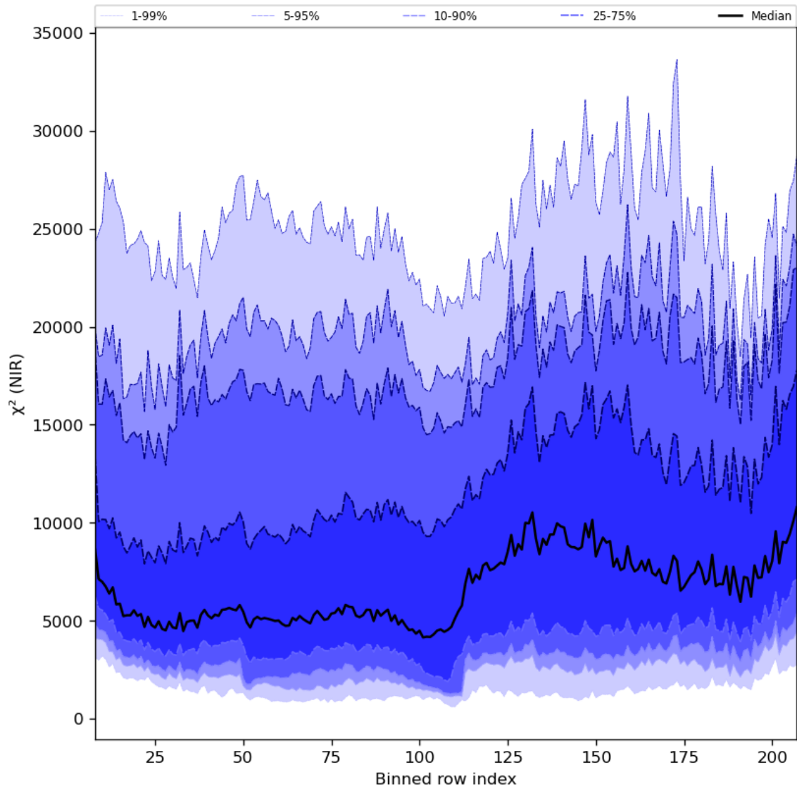
Figure 40: Along track statistics of “ \chi^2 (NIR)” for 2023-07-24 to 2023-07-26
