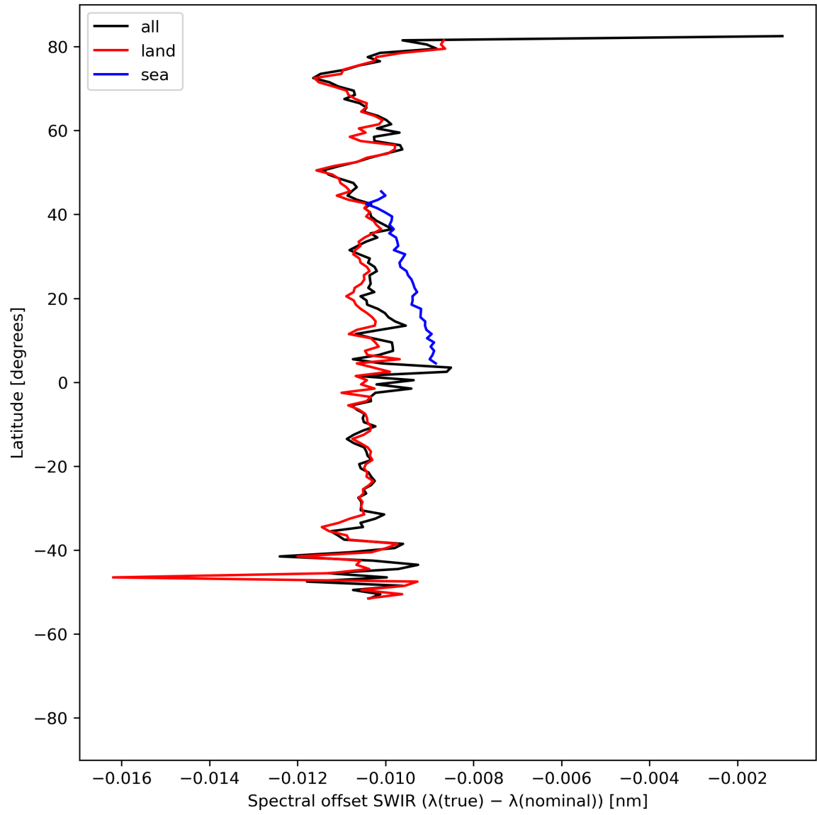
Figure 16: Zonal average of “Spectral offset SWIR ( \lambda(\text{true}) - \lambda(\text{nominal}) )” for 2023-07-24 to 2023-07-26.
