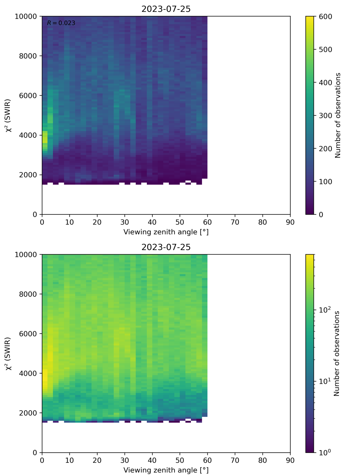
Figure 106: Scatter density plot of “Viewing zenith angle” against “ \chi^2 (SWIR)” for 2023-07-24 to 2023-07-26.
