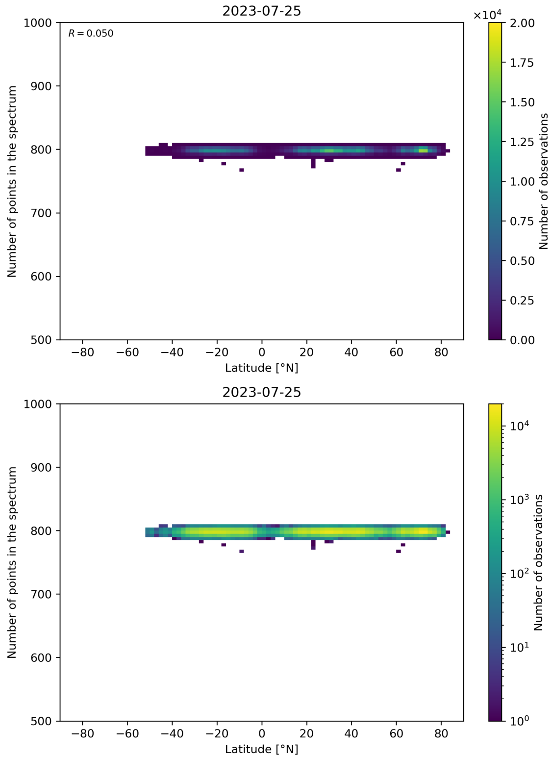
Figure 61: Scatter density plot of “Latitude” against “Number of points in the spectrum” for 2023-07-24 to 2023-07-26.
