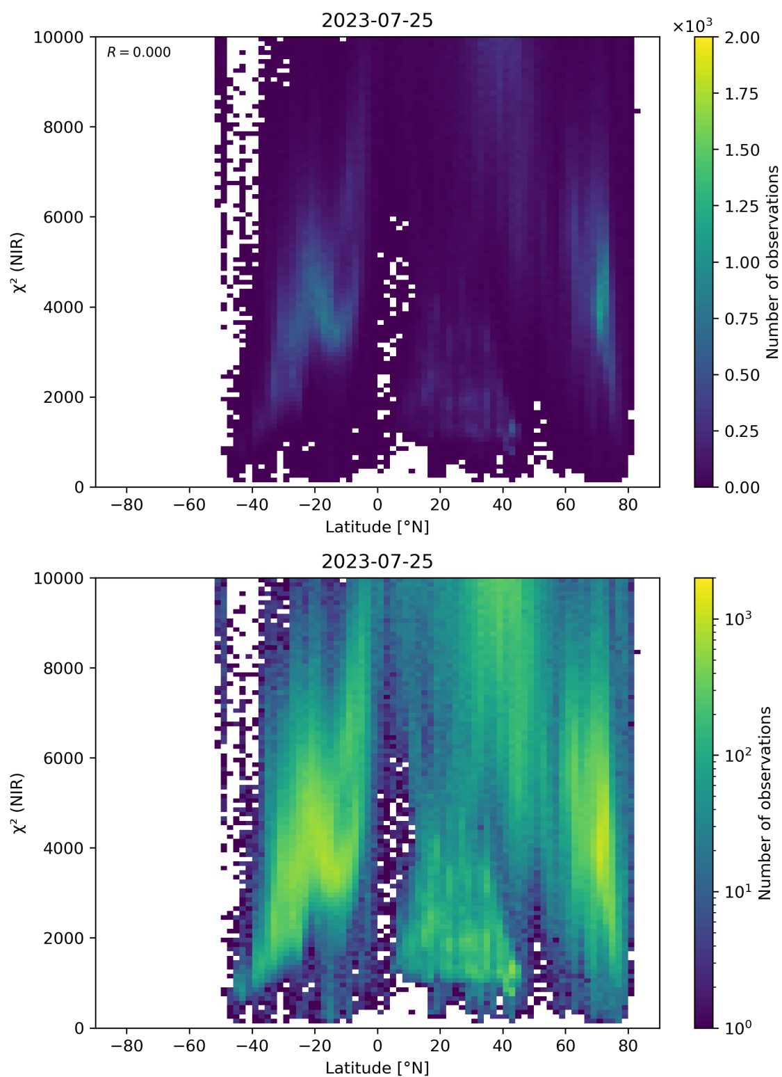
Figure 53: Scatter density plot of “Latitude” against “ \chi^2 (NIR)” for 2023-07-24 to 2023-07-26.
