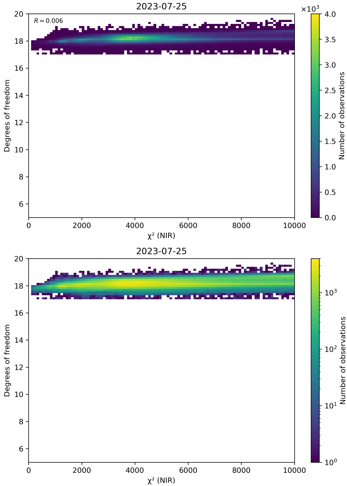
Figure 44: Scatter density plot of “ \chi^2 (NIR)” against “Degrees of freedom” for 2023-07-24 to 2023-07-26.
