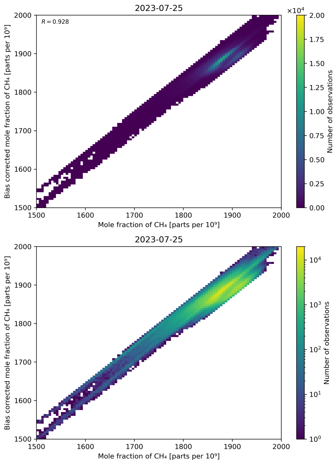
Figure 74: Scatter density plot of “Mole fraction of CH 4 ” against “Bias corrected mole fraction of CH 4 ” for 2023-07-24 to 2023-07-26.
