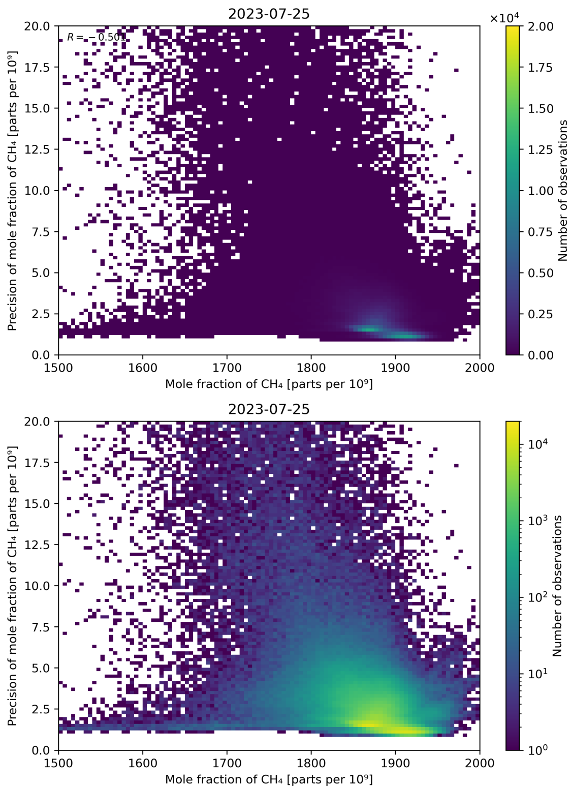
Figure 75: Scatter density plot of “Mole fraction of CH 4 ” against “Precision of mole fraction of CH 4 ” for 2023-07-24 to 2023-07-26.
