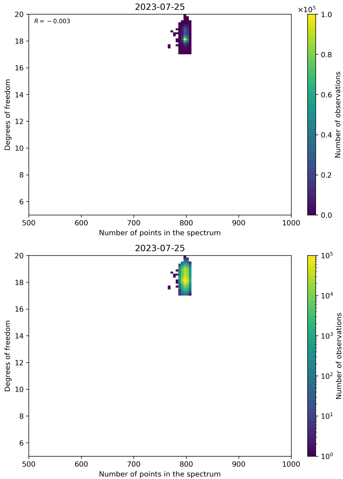
Figure 90: Scatter density plot of “Number of points in the spectrum” against “Degrees of freedom” for 2023-07-24 to 2023-07-26.
