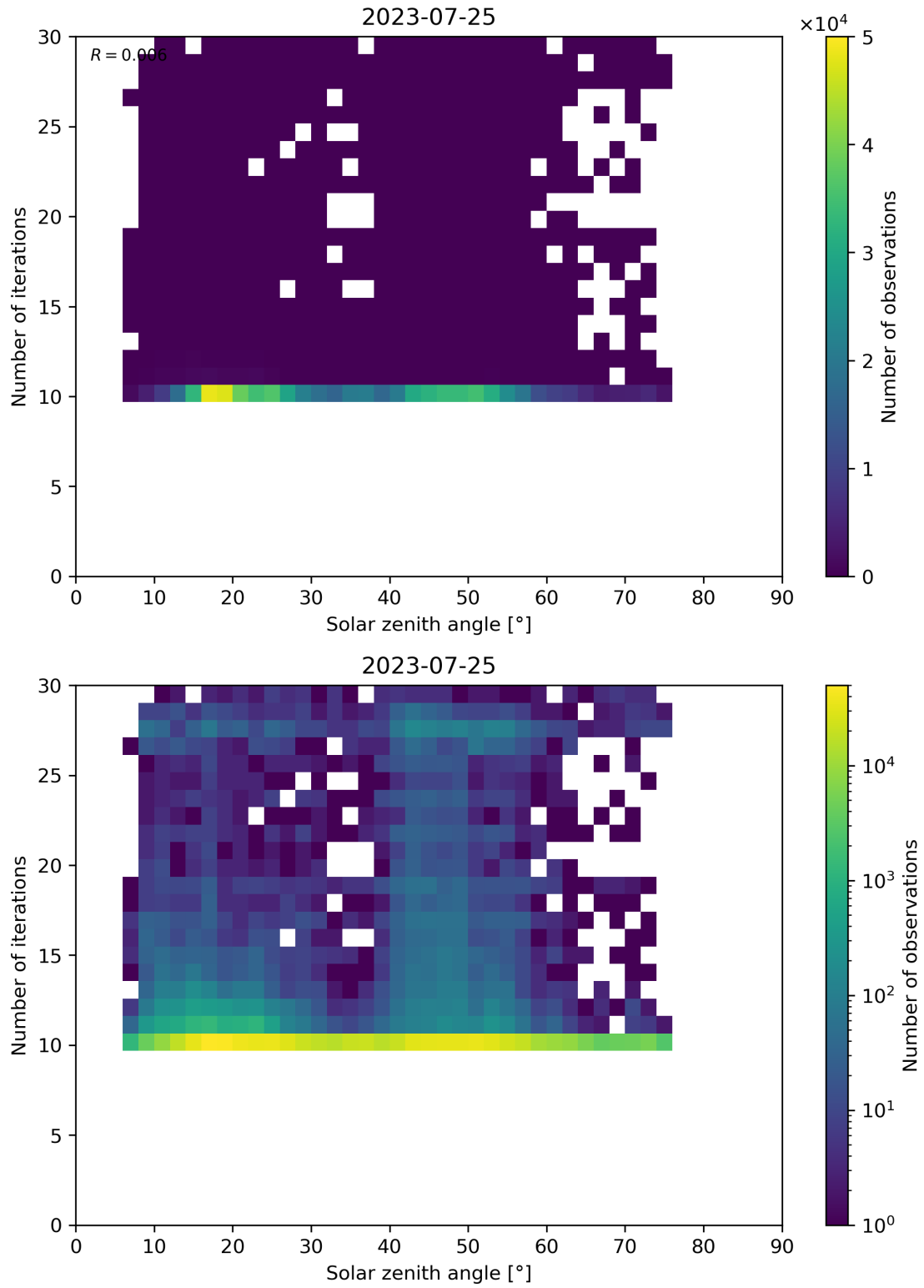
Figure 102: Scatter density plot of “Solar zenith angle” against “Number of iterations” for 2023-07-24 to 2023-07-26.
