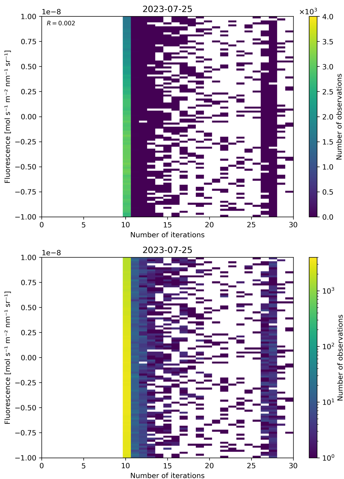
Figure 87: Scatter density plot of “Number of iterations” against “Fluorescence” for 2023-07-24 to 2023-07-26.
