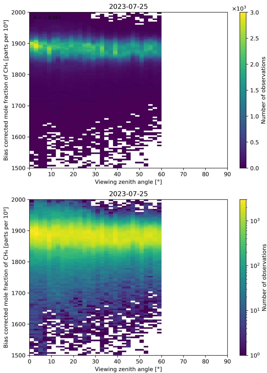
Figure 111: Scatter density plot of “Viewing zenith angle” against “Bias corrected mole fraction of CH 4 ” for 2023-07-24 to 2023-07-26.
