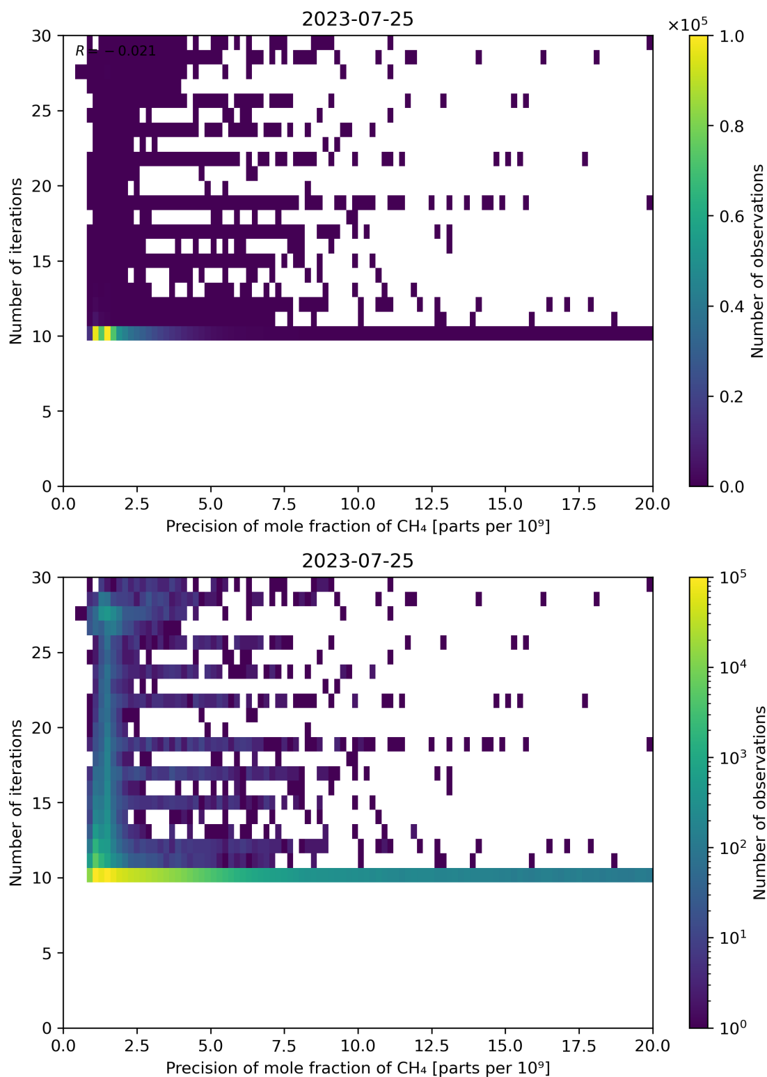
Figure 83: Scatter density plot of “Precision of mole fraction of CH 4 ” against “Number of iterations” for 2023-07-24 to 2023-07-26.
