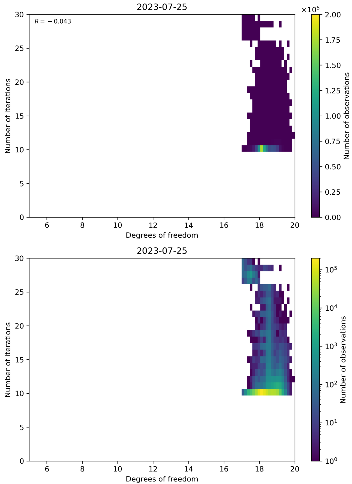
Figure 52: Scatter density plot of “Degrees of freedom” against “Number of iterations” for 2023-07-24 to 2023-07-26.
