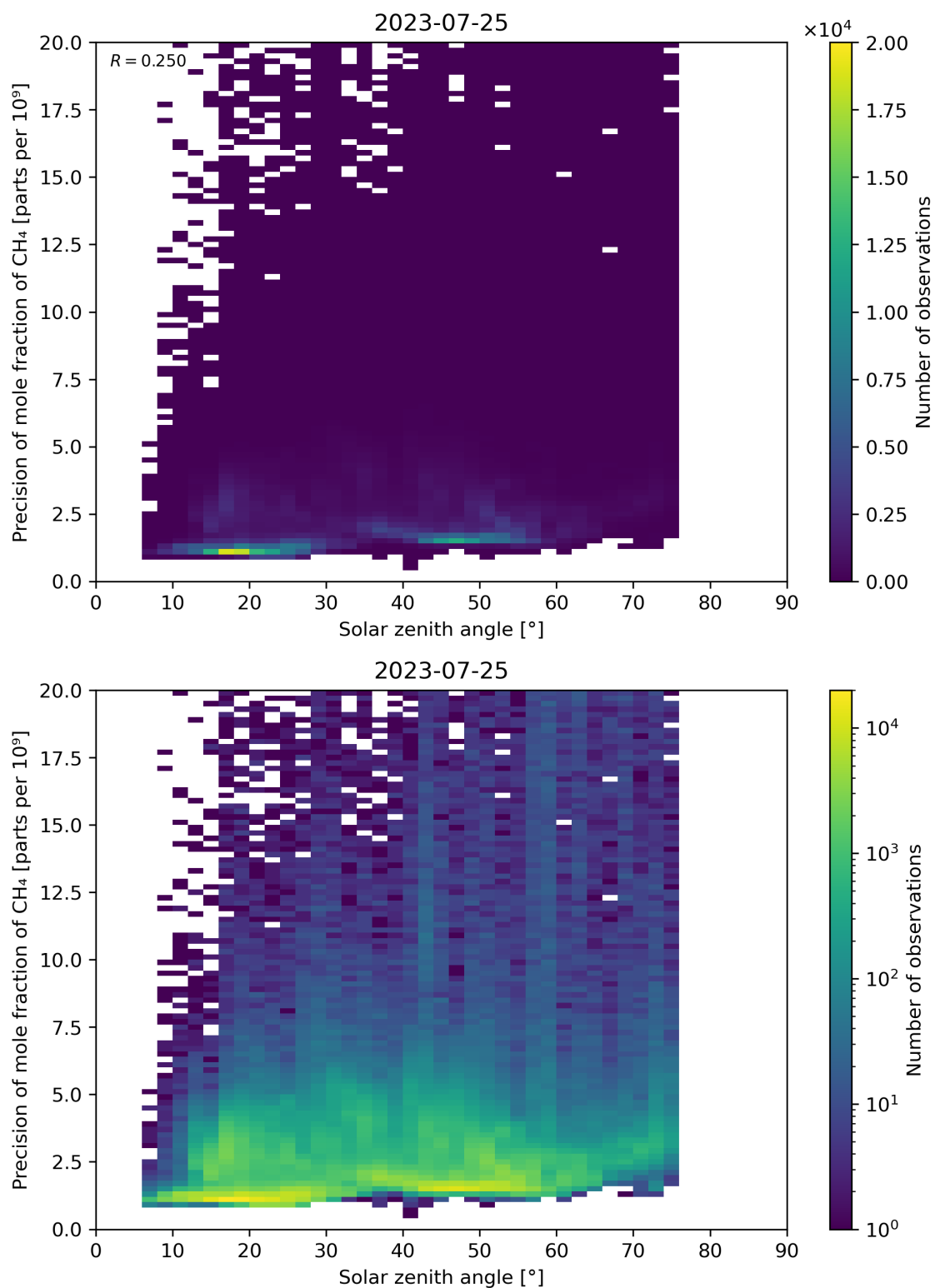
Figure 101: Scatter density plot of “Solar zenith angle” against “Precision of mole fraction of CH 4 ” for 2023-07-24 to 2023-07-26.
