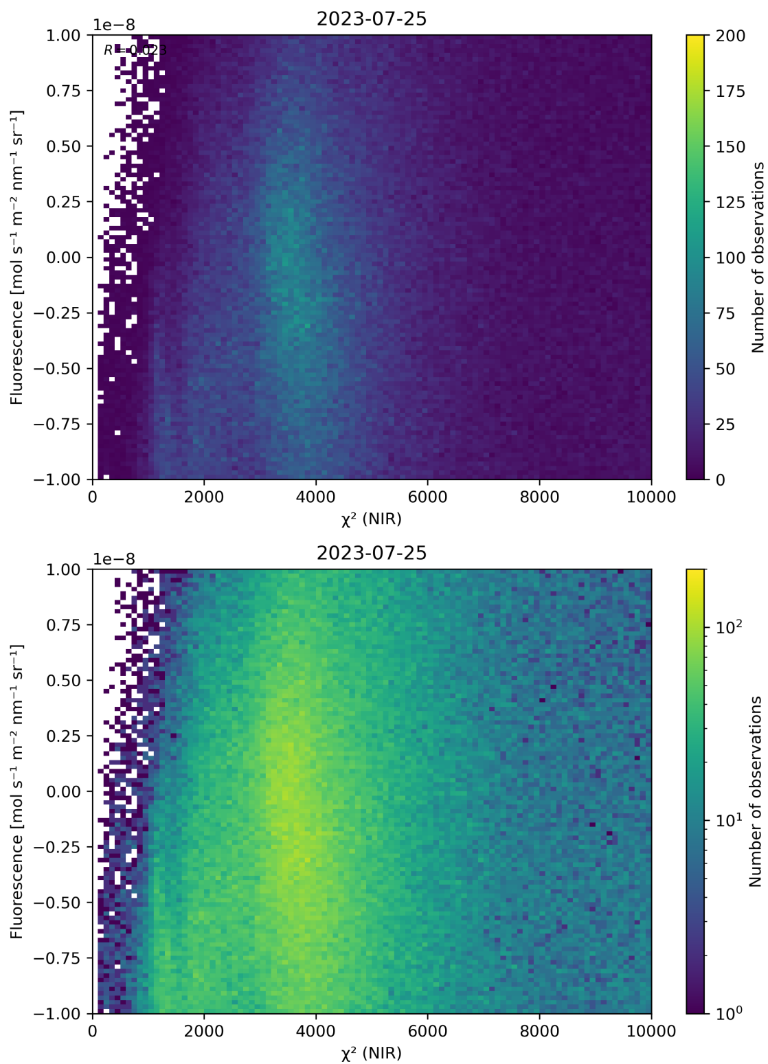
Figure 45: Scatter density plot of “ \chi^2 (NIR)” against “Fluorescence” for 2023-07-24 to 2023-07-26.
