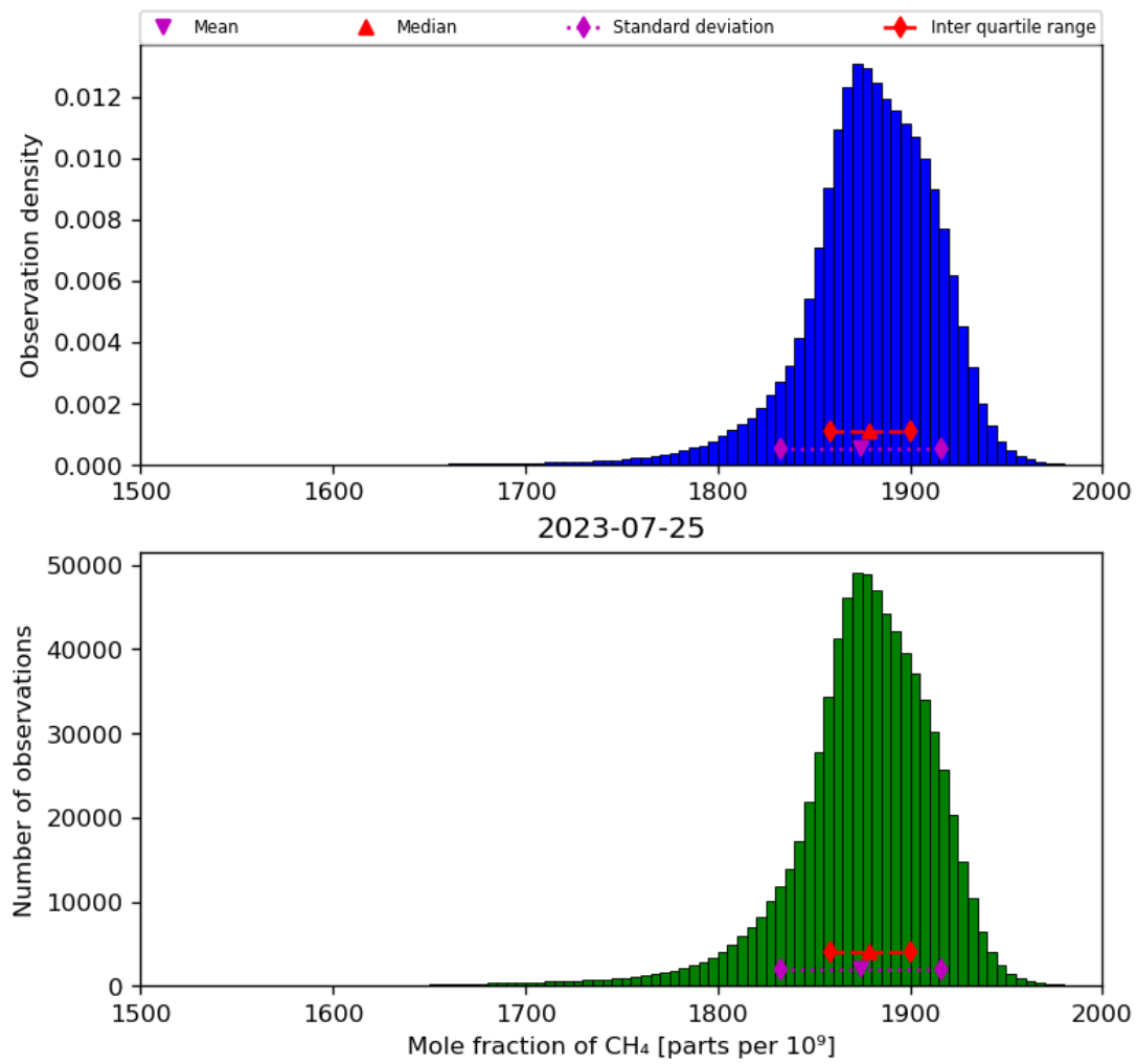
Figure 23: Histogram of "Mole fraction of CH 4 " for 2023-07-24 to 2023-07-26
