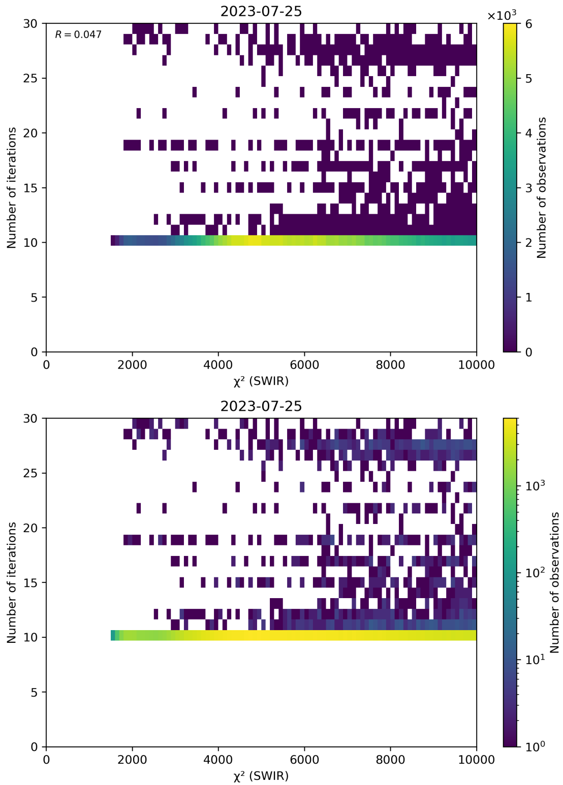
Figure 50: Scatter density plot of “ \chi^2 (SWIR)” against “Number of iterations” for 2023-07-24 to 2023-07-26.
