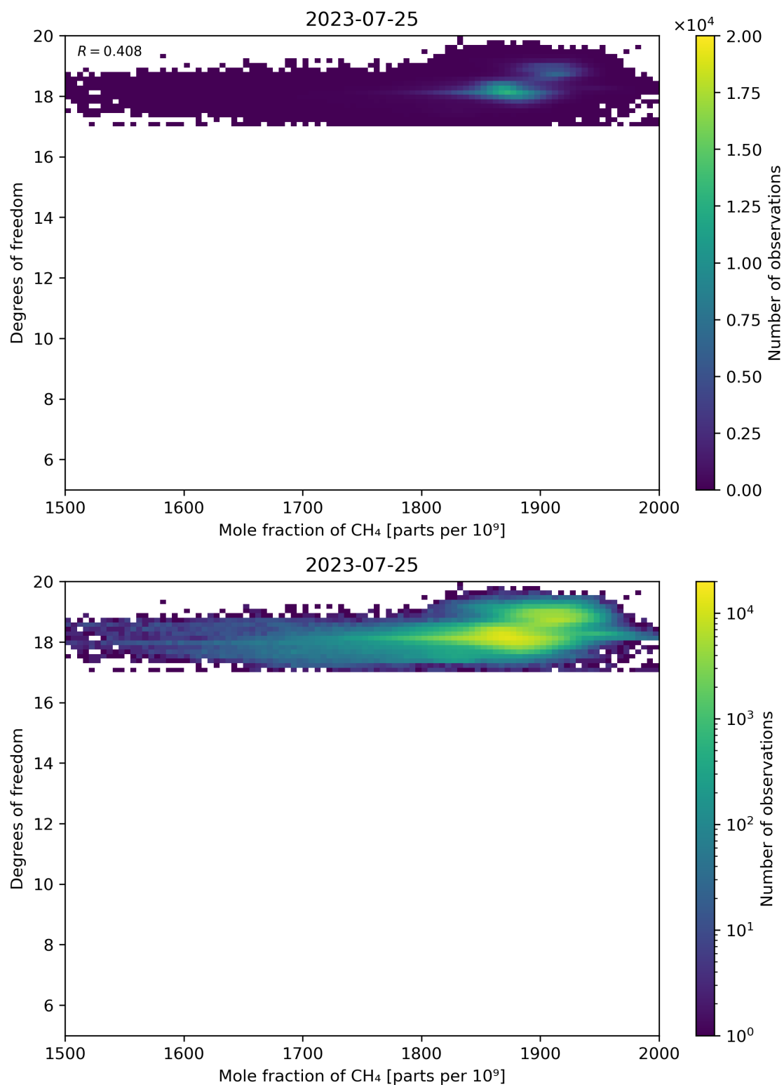
Figure 72: Scatter density plot of “Mole fraction of CH 4 ” against “Degrees of freedom” for 2023-07-24 to 2023-07-26.
