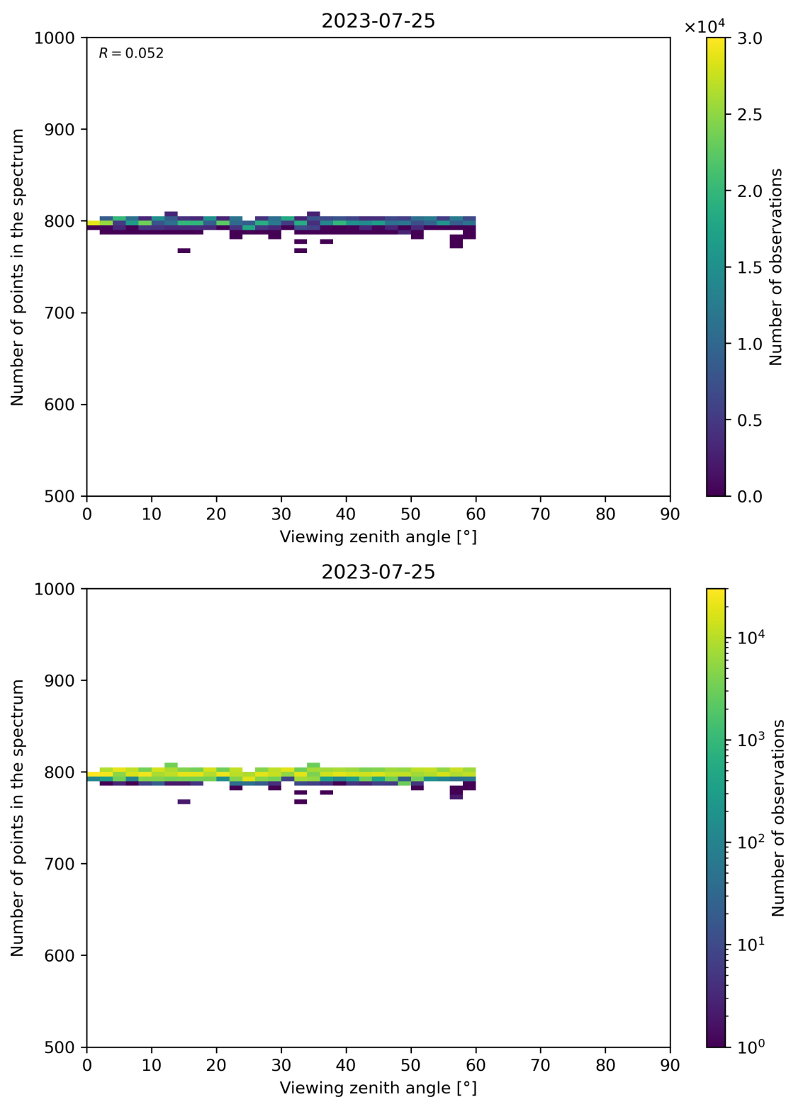
Figure 114: Scatter density plot of “Viewing zenith angle” against “Number of points in the spectrum” for 2023-07-24 to 2023-07-26.
