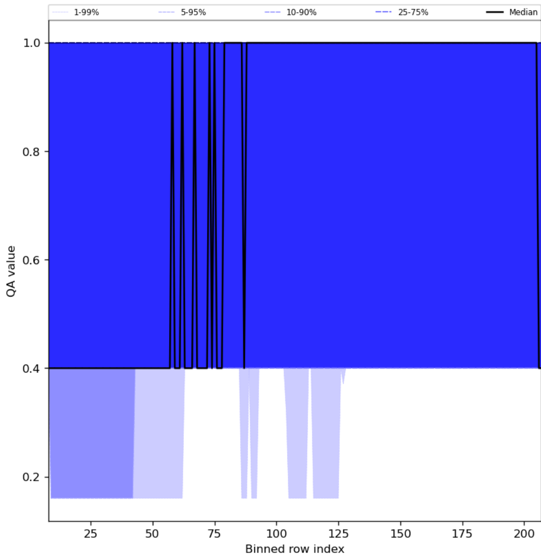
Figure 33: Along track statistics of “QA value” for 2023-07-24 to 2023-07-26
