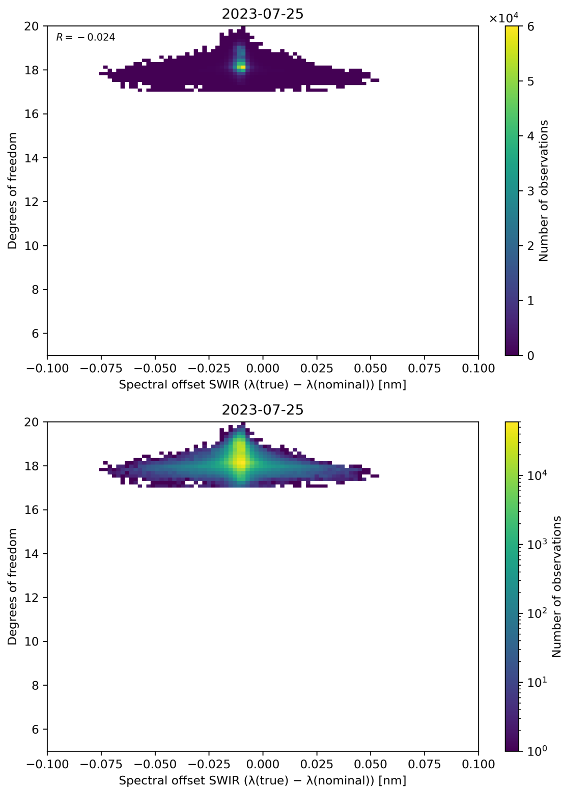
Figure 119: Scatter density plot of “Spectral offset SWIR ( \lambda(\text{true}) - \lambda(\text{nominal}) )” against “Degrees of freedom” for 2023-07-24 to 2023-07-26.
