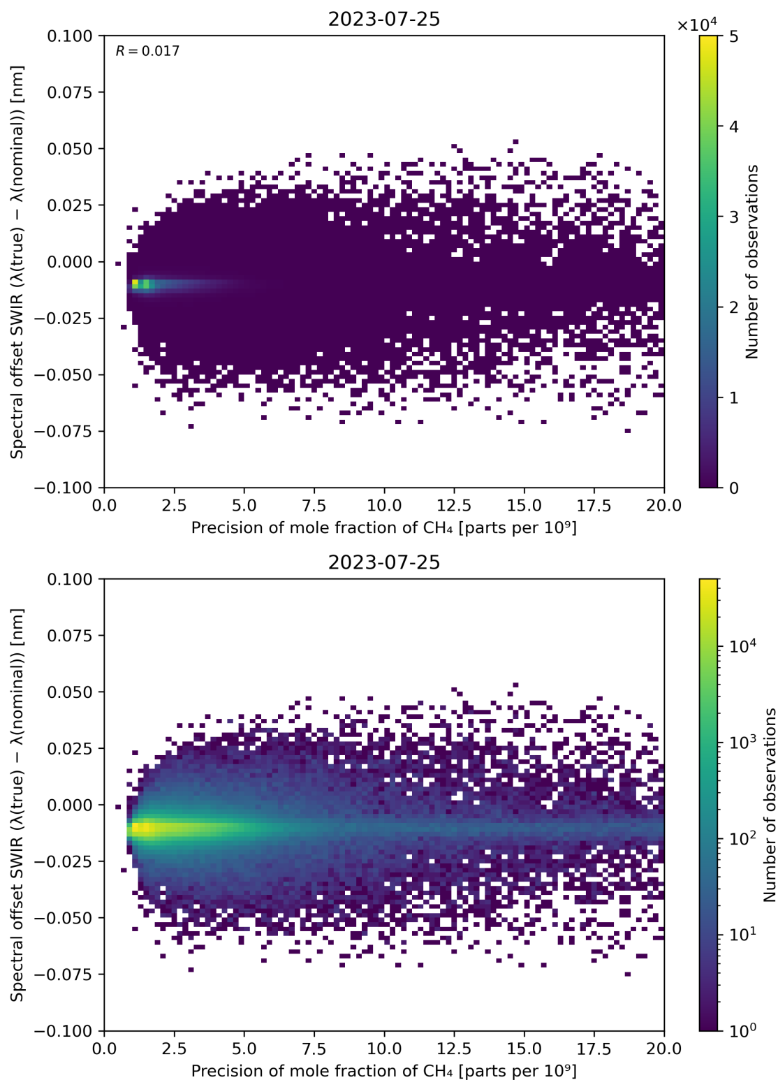
Figure 85: Scatter density plot of “Precision of mole fraction of CH 4 ” against “Spectral offset SWIR ( \lambda(\text{true}) - \lambda(\text{nominal}) )” for 2023-07-24 to 2023-07-26.
