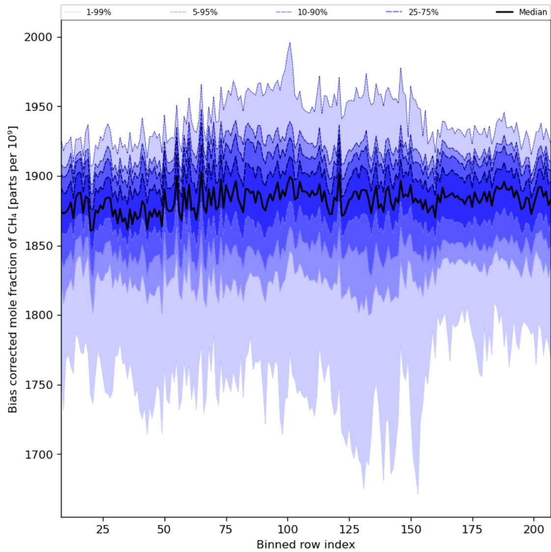
Figure 36: Along track statistics of “Bias corrected mole fraction of CH 4 ” for 2023-07-24 to 2023-07-26
