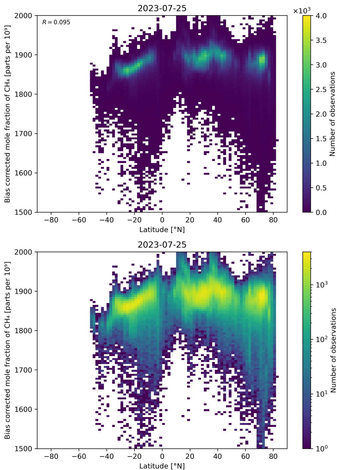
Figure 58: Scatter density plot of “Latitude” against “Bias corrected mole fraction of \text{CH}_4 ” for 2023-07-24 to 2023-07-26.
