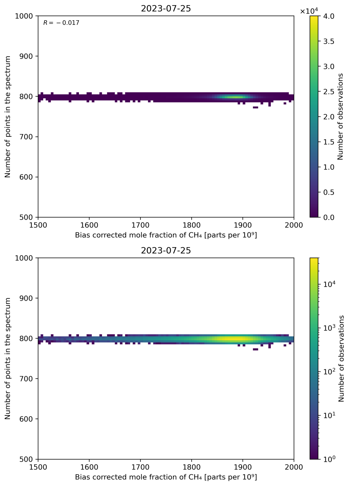
Figure 68: Scatter density plot of “Bias corrected mole fraction of CH 4 ” against “Number of points in the spectrum” for 2023-07-24 to 2023-07-26.
