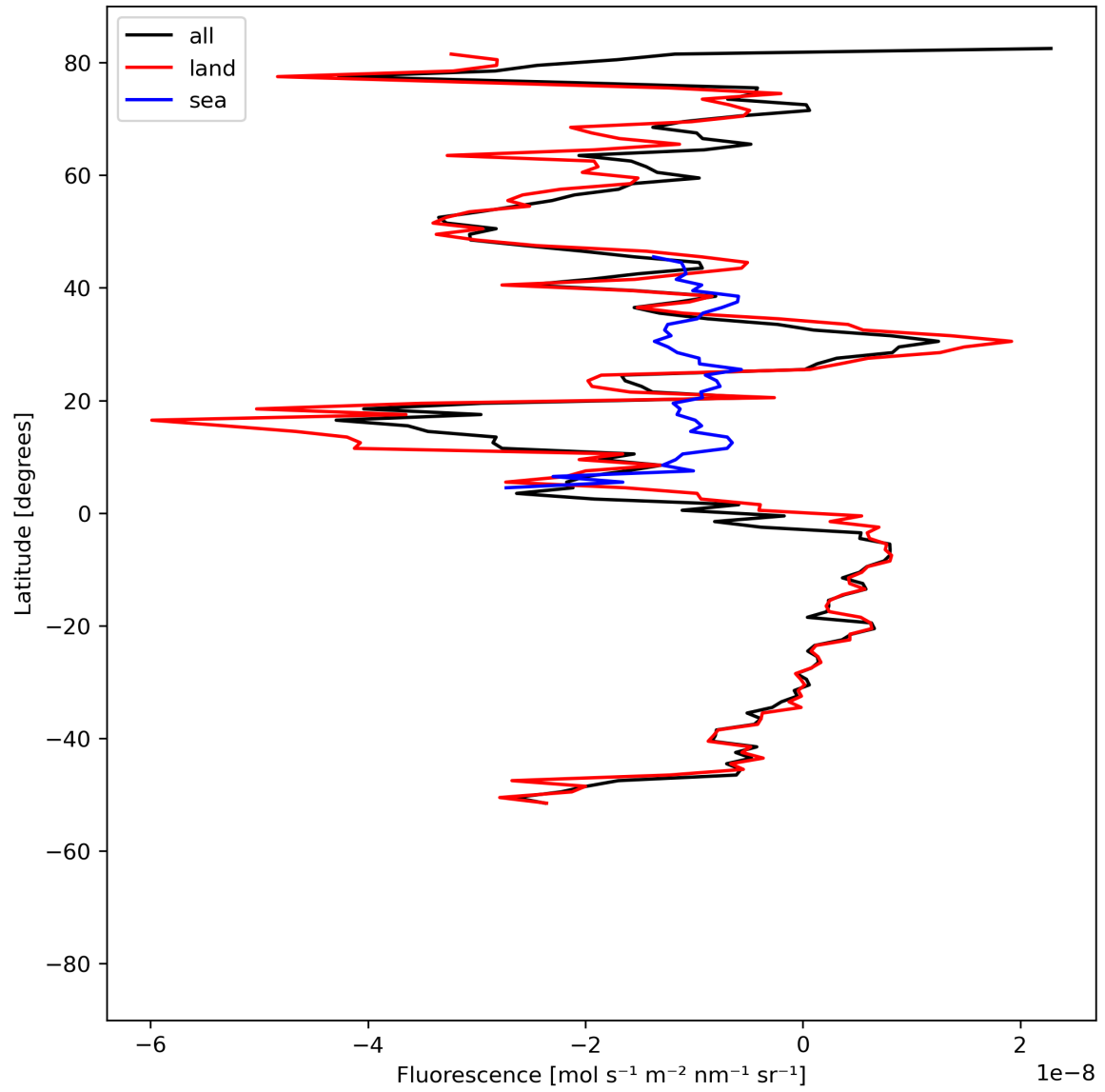
Figure 21: Zonal average of “Fluorescence” for 2023-07-24 to 2023-07-26.
