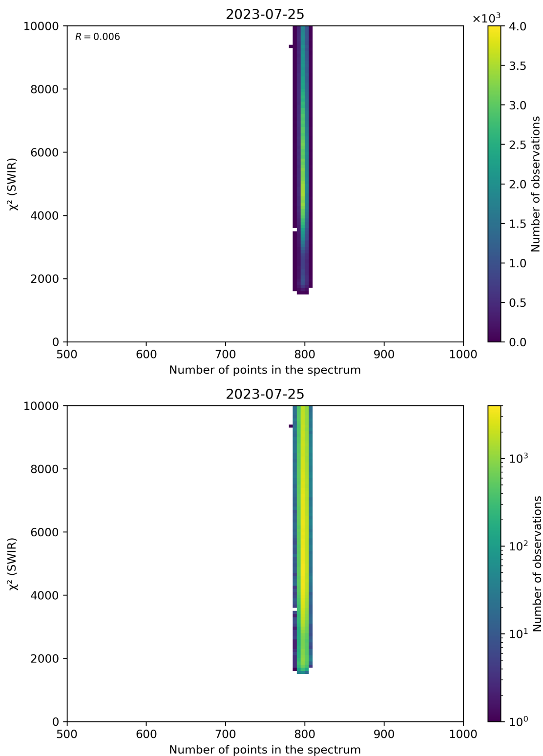
Figure 89: Scatter density plot of “Number of points in the spectrum” against “ \chi^2 (SWIR)” for 2023-07-24 to 2023-07-26.
