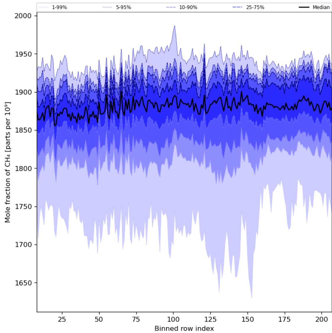
Figure 34: Along track statistics of “Mole fraction of CH 4 ” for 2023-07-24 to 2023-07-26
