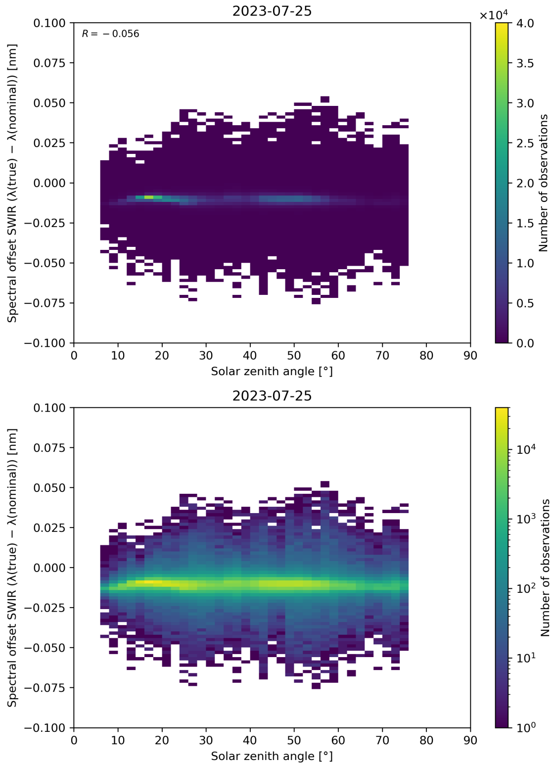
Figure 104: Scatter density plot of “Solar zenith angle” against “Spectral offset SWIR ( \lambda(\text{true}) - \lambda(\text{nominal}) )” for 2023-07-24 to 2023-07-26.
