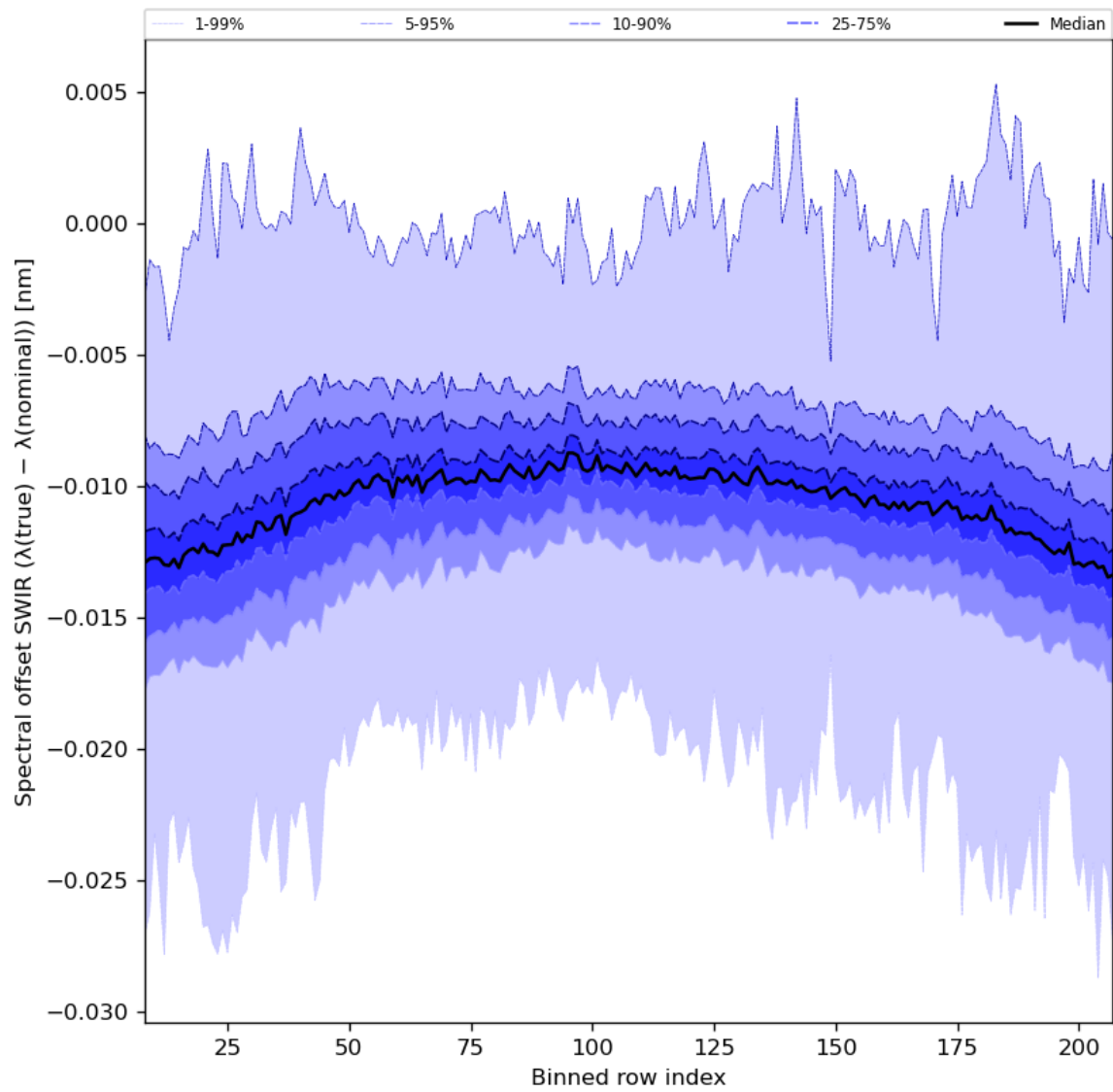
Figure 38: Along track statistics of “Spectral offset SWIR ( \lambda(\text{true}) - \lambda(\text{nominal}) )” for 2023-07-24 to 2023-07-26
