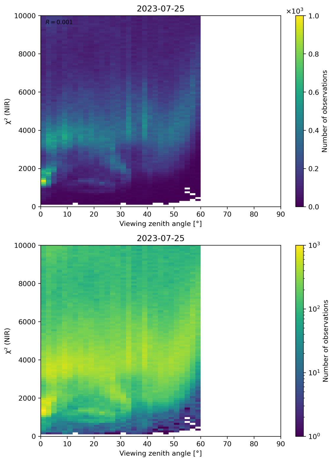
Figure 105: Scatter density plot of “Viewing zenith angle” against “ \chi^2 (NIR)” for 2023-07-24 to 2023-07-26.
