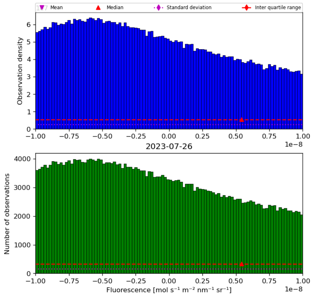
Figure 32: Histogram of “Fluorescence” for 2023-07-25 to 2023-07-27
