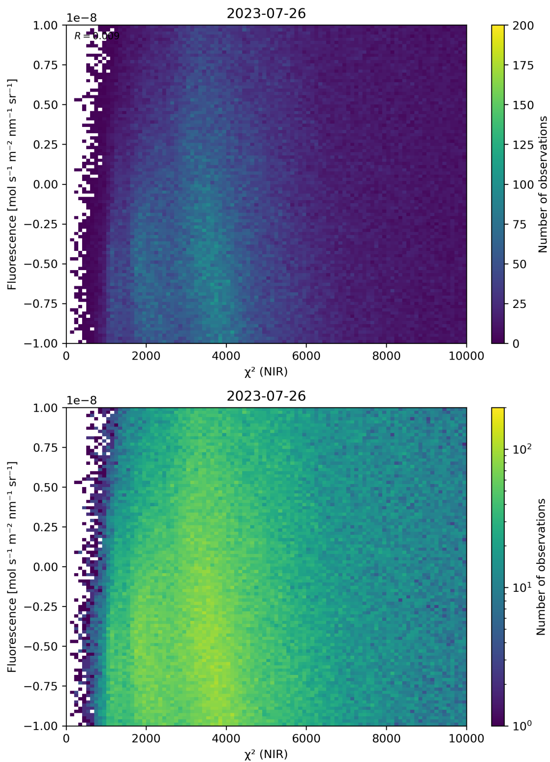
Figure 45: Scatter density plot of “ \chi^2 (NIR)” against “Fluorescence” for 2023-07-25 to 2023-07-27.
