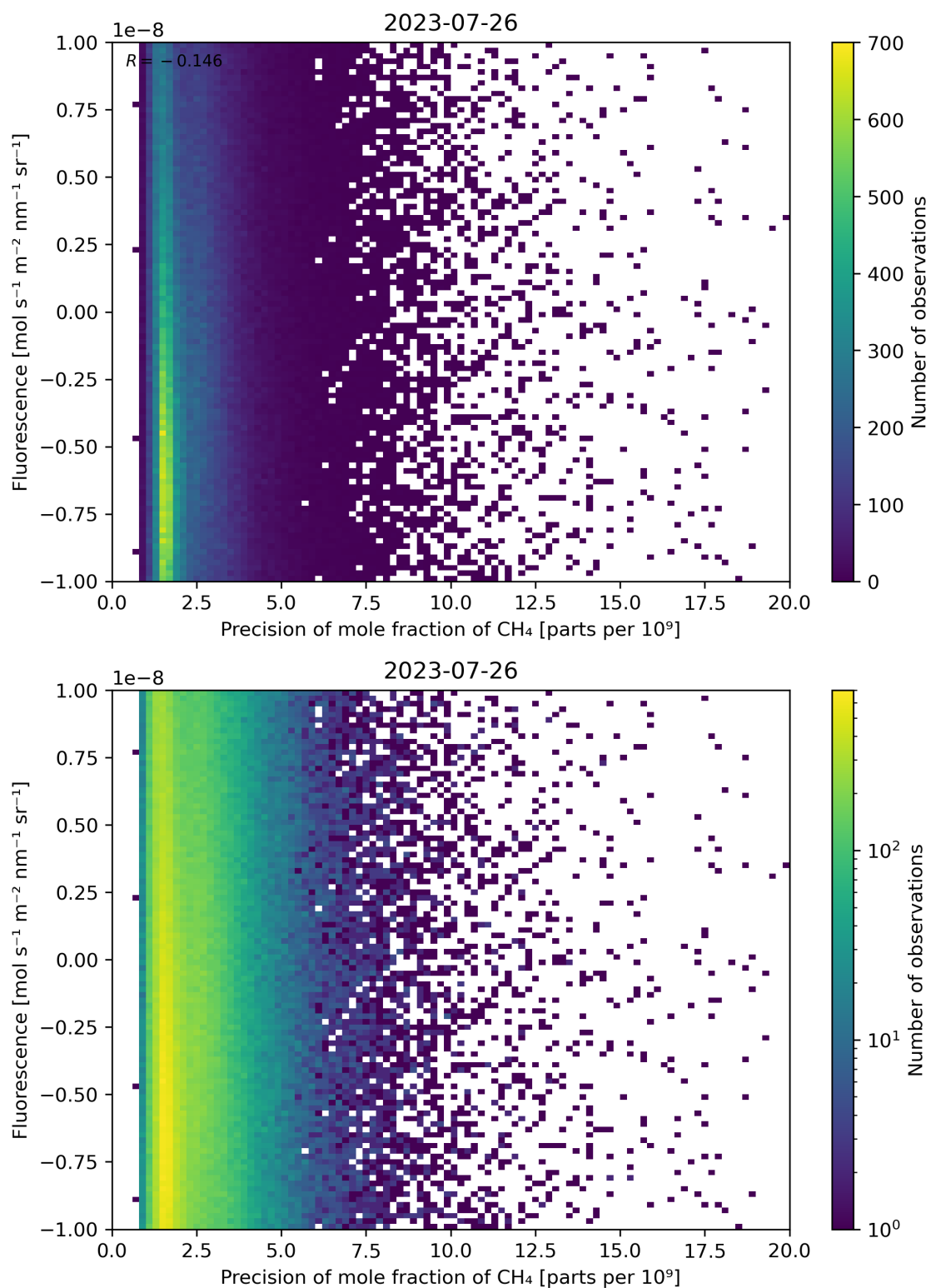
Figure 81: Scatter density plot of “Precision of mole fraction of \text{CH}_4 ” against “Fluorescence” for 2023-07-25 to 2023-07-27.
