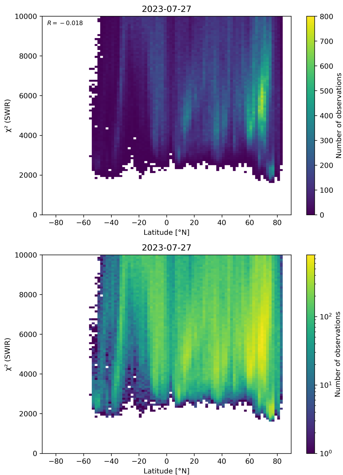
Figure 54: Scatter density plot of “Latitude” against “ \chi^2 (SWIR)” for 2023-07-26 to 2023-07-28.
