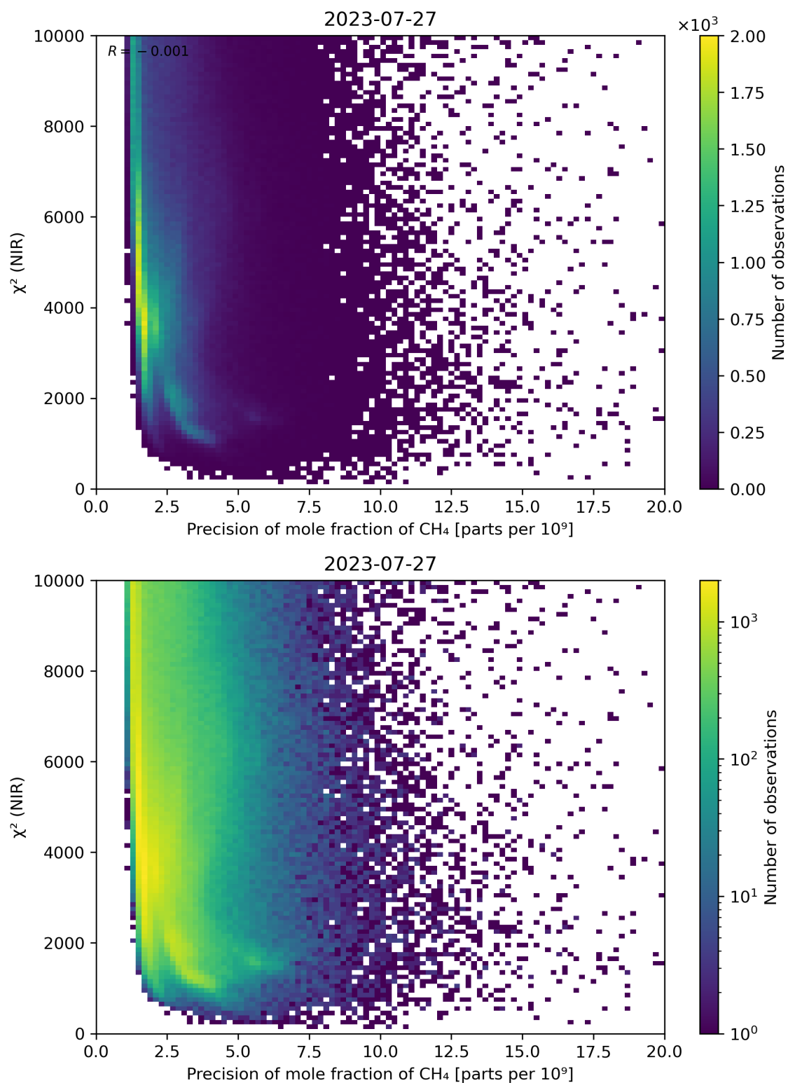
Figure 78: Scatter density plot of “Precision of mole fraction of CH 4 ” against “ \chi^2 (NIR)” for 2023-07-26 to 2023-07-28.
