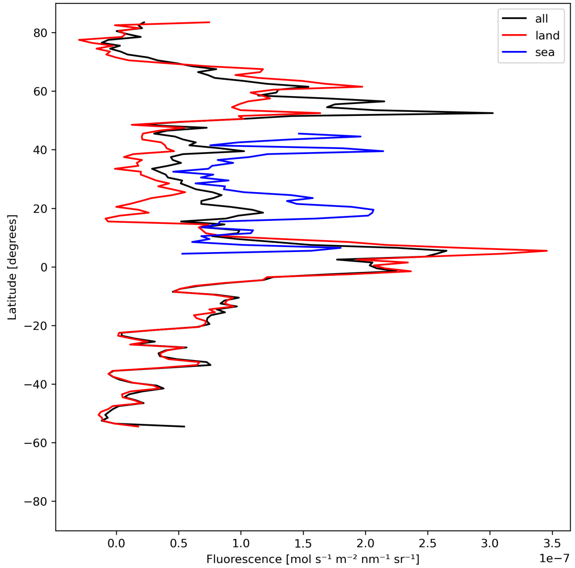
Figure 21: Zonal average of “Fluorescence” for 2023-07-26 to 2023-07-28.
