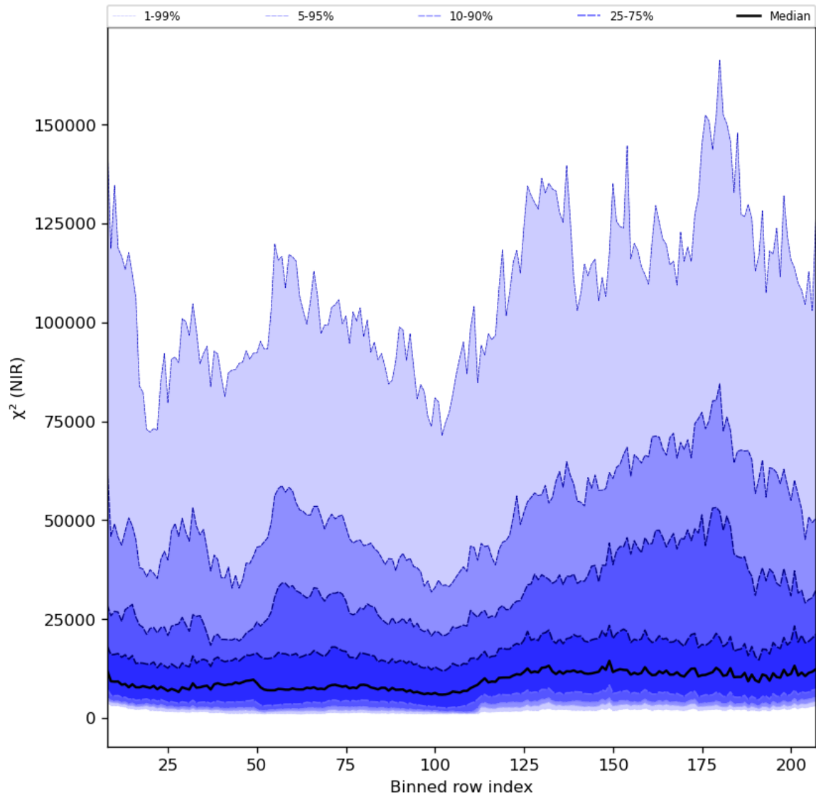
Figure 40: Along track statistics of " \chi^2 (NIR)" for 2023-07-26 to 2023-07-28
