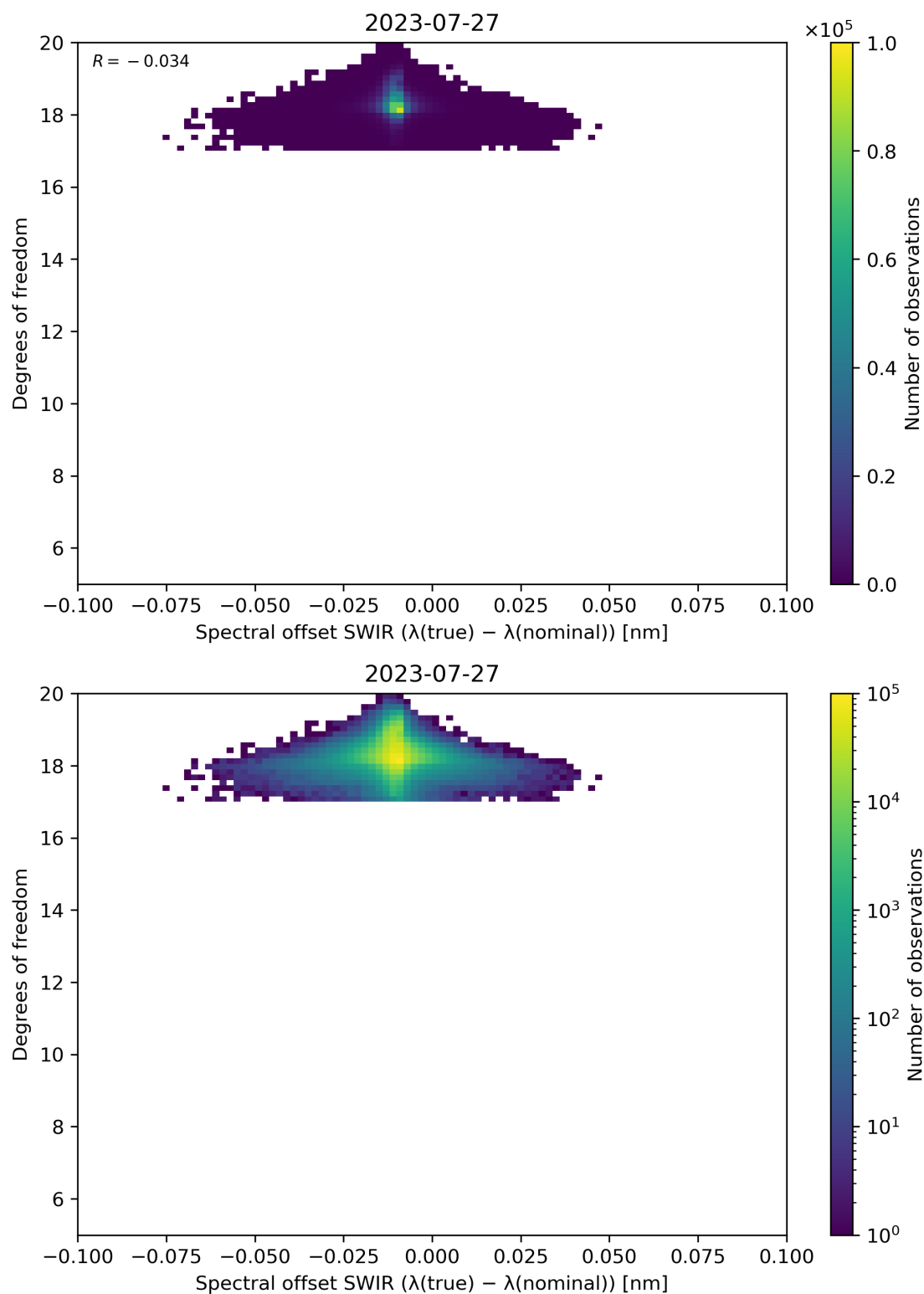
Figure 119: Scatter density plot of “Spectral offset SWIR ( \lambda(\text{true}) - \lambda(\text{nominal}) )” against “Degrees of freedom” for 2023-07-26 to 2023-07-28.
