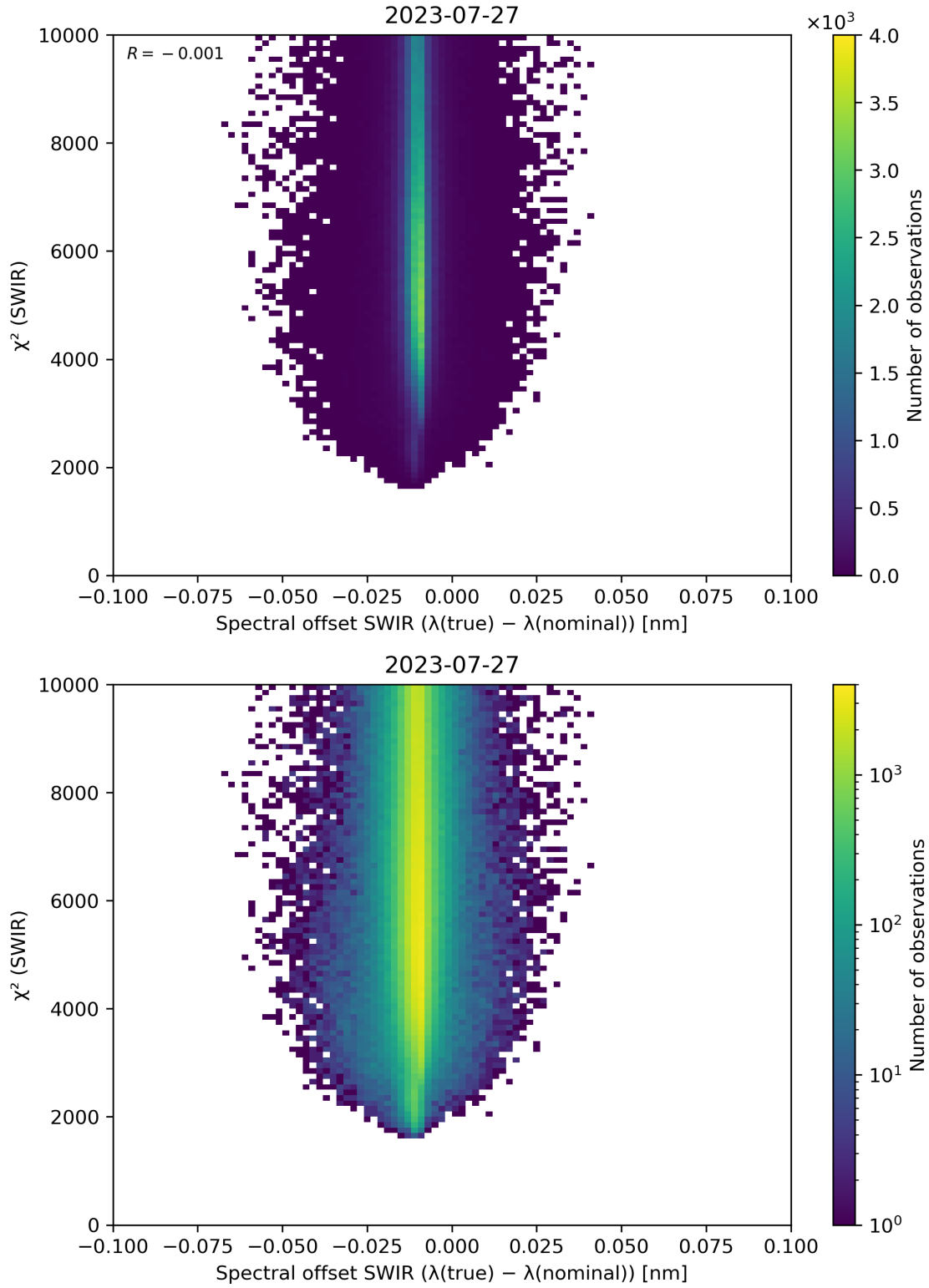
Figure 118: Scatter density plot of “Spectral offset SWIR ( \lambda(\text{true}) - \lambda(\text{nominal}) )” against “ \chi^2 (SWIR)” for 2023-07-26 to 2023-07-28.
