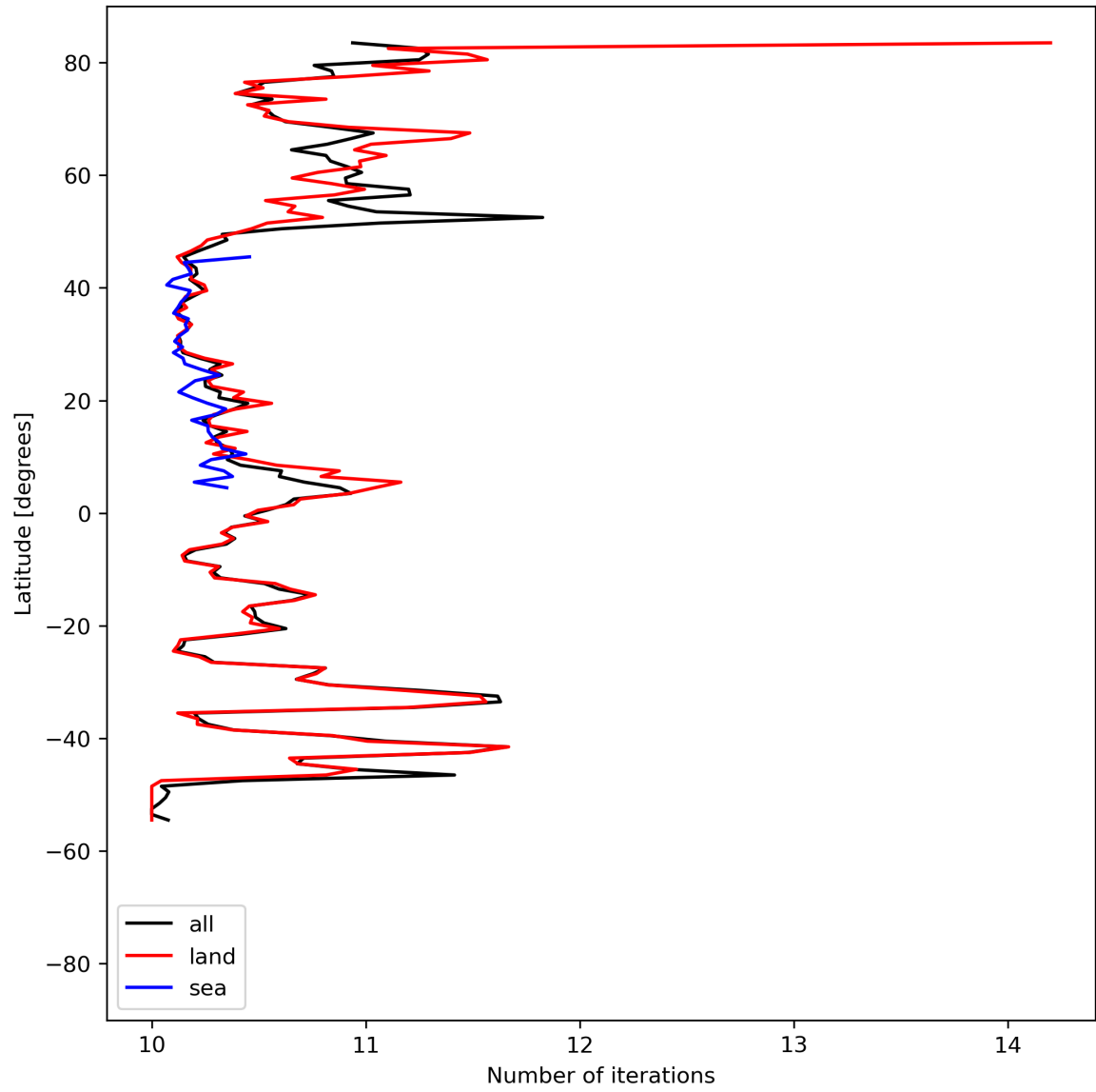
Figure 20: Zonal average of “Number of iterations” for 2023-07-26 to 2023-07-28.
