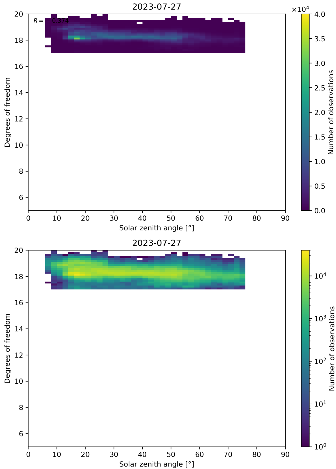
Figure 96: Scatter density plot of “Solar zenith angle” against “Degrees of freedom” for 2023-07-26 to 2023-07-28.
