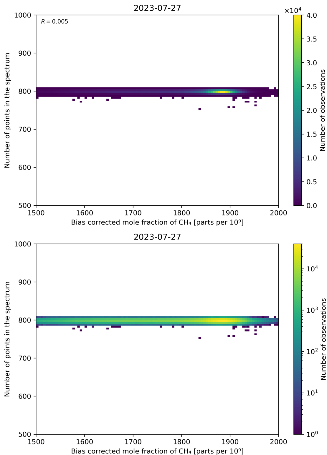
Figure 68: Scatter density plot of “Bias corrected mole fraction of CH 4 ” against “Number of points in the spectrum” for 2023-07-26 to 2023-07-28.
