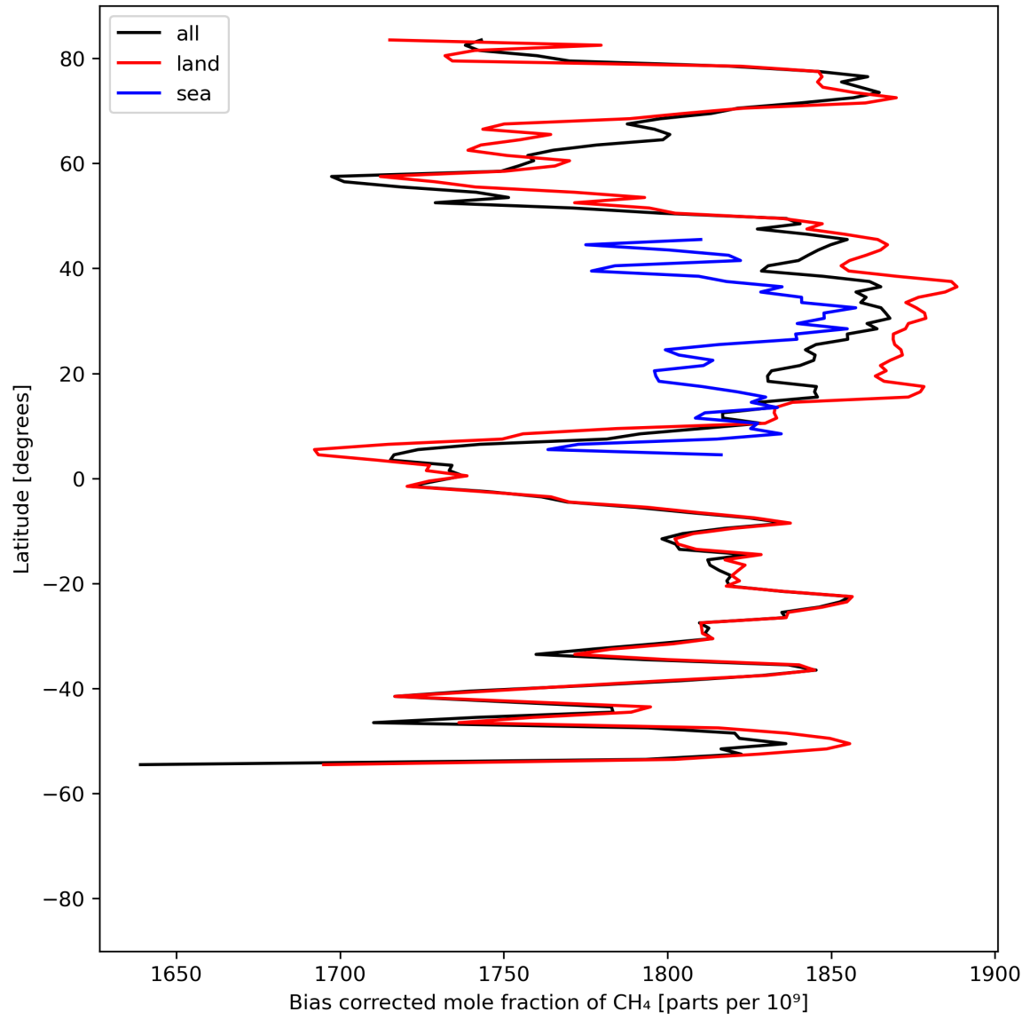
Figure 14: Zonal average of “Bias corrected mole fraction of CH 4 ” for 2023-07-26 to 2023-07-28.
