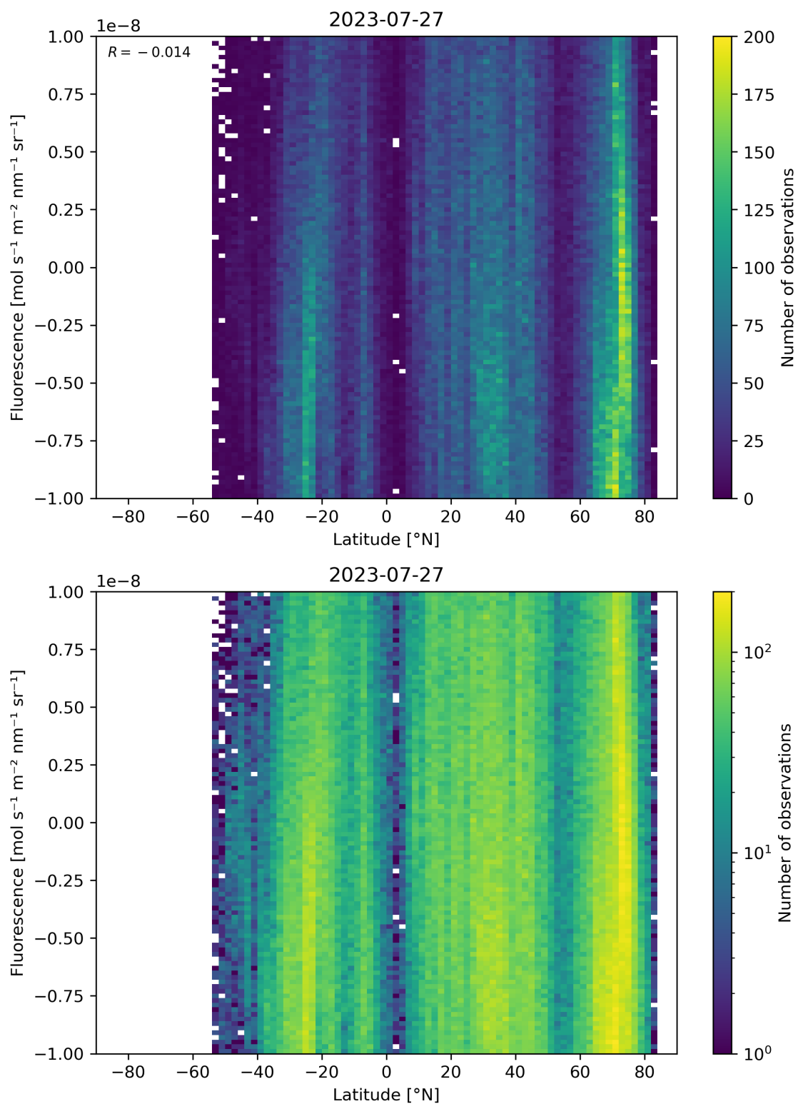
Figure 56: Scatter density plot of “Latitude” against “Fluorescence” for 2023-07-26 to 2023-07-28.
