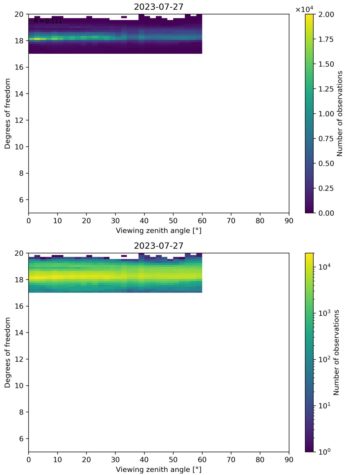
Figure 107: Scatter density plot of “Viewing zenith angle” against “Degrees of freedom” for 2023-07-26 to 2023-07-28.
