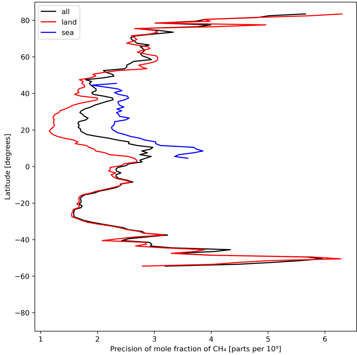
Figure 13: Zonal average of “Precision of mole fraction of CH 4 ” for 2023-07-26 to 2023-07-28.
