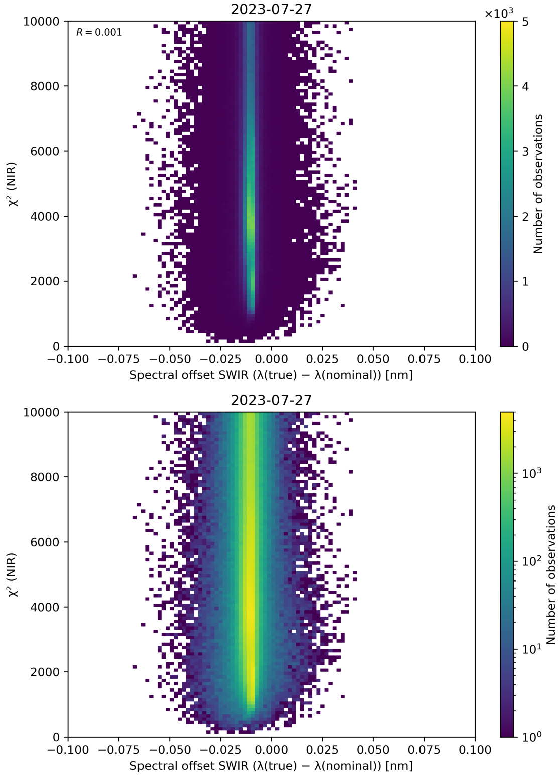
Figure 117: Scatter density plot of “Spectral offset SWIR ( \lambda(\text{true}) - \lambda(\text{nominal}) )” against “ \chi^2 (NIR)” for 2023-07-26 to 2023-07-28.
