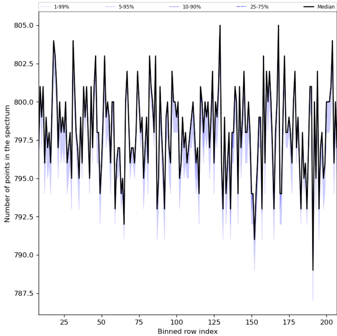
Figure 37: Along track statistics of “Number of points in the spectrum” for 2023-07-26 to 2023-07-28
