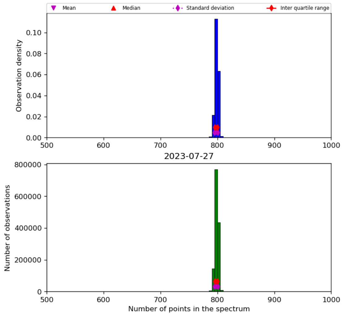
Figure 26: Histogram of “Number of points in the spectrum” for 2023-07-26 to 2023-07-28
