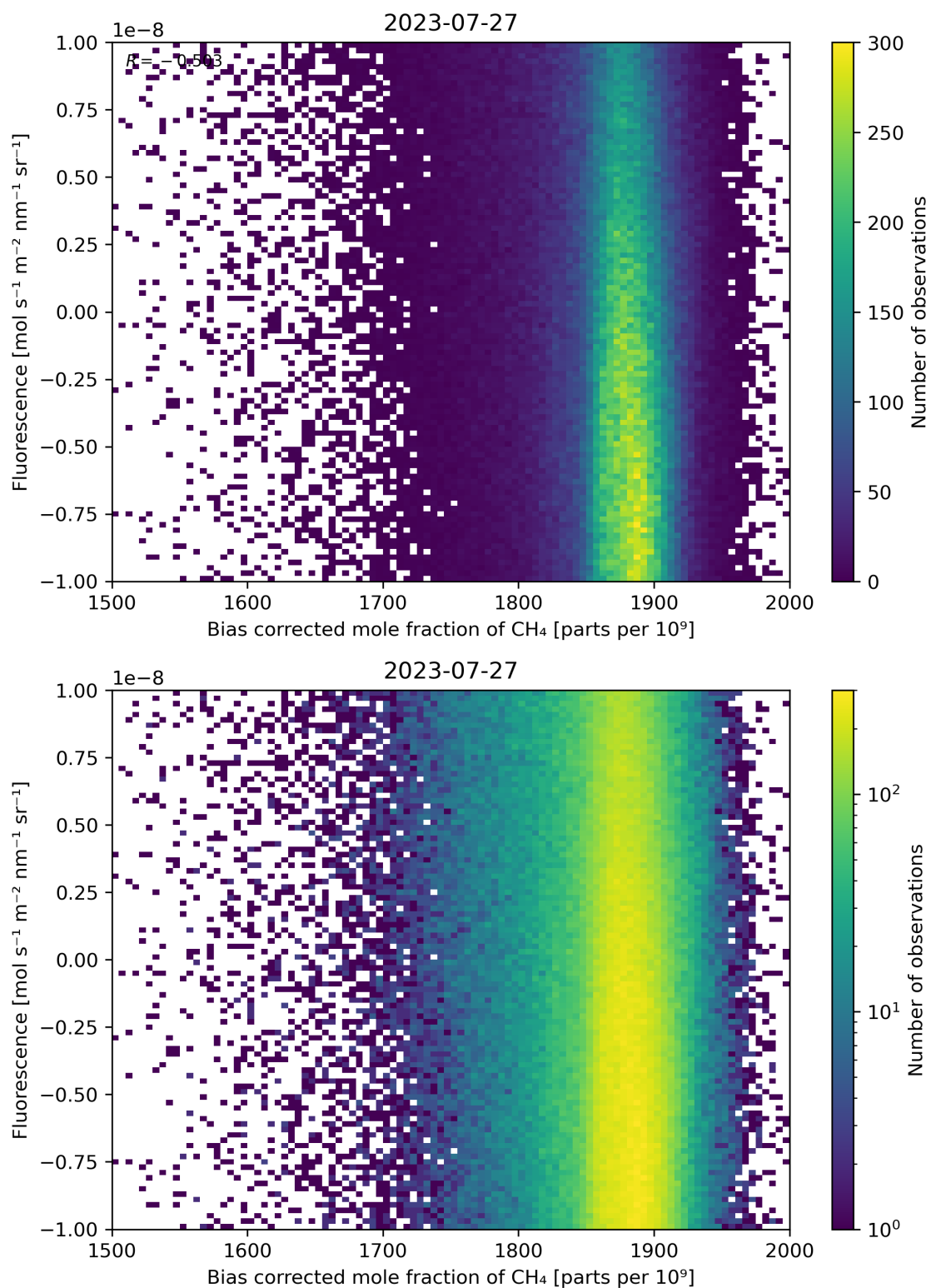
Figure 66: Scatter density plot of “Bias corrected mole fraction of \text{CH}_4 ” against “Fluorescence” for 2023-07-26 to 2023-07-28.
