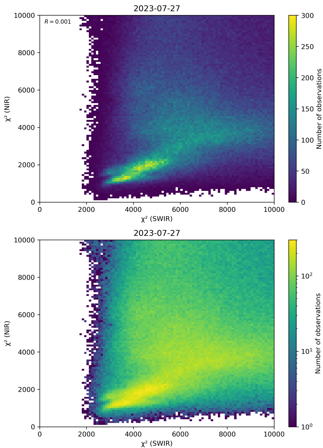
Figure 47: Scatter density plot of “ \chi^2 (SWIR)” against “ \chi^2 (NIR)” for 2023-07-26 to 2023-07-28.
