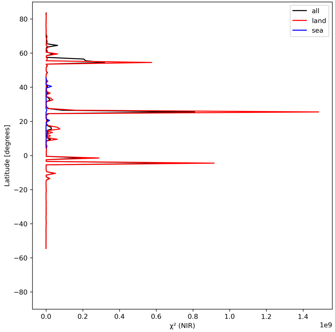
Figure 18: Zonal average of “ \chi^2 (NIR)” for 2023-07-26 to 2023-07-28.
