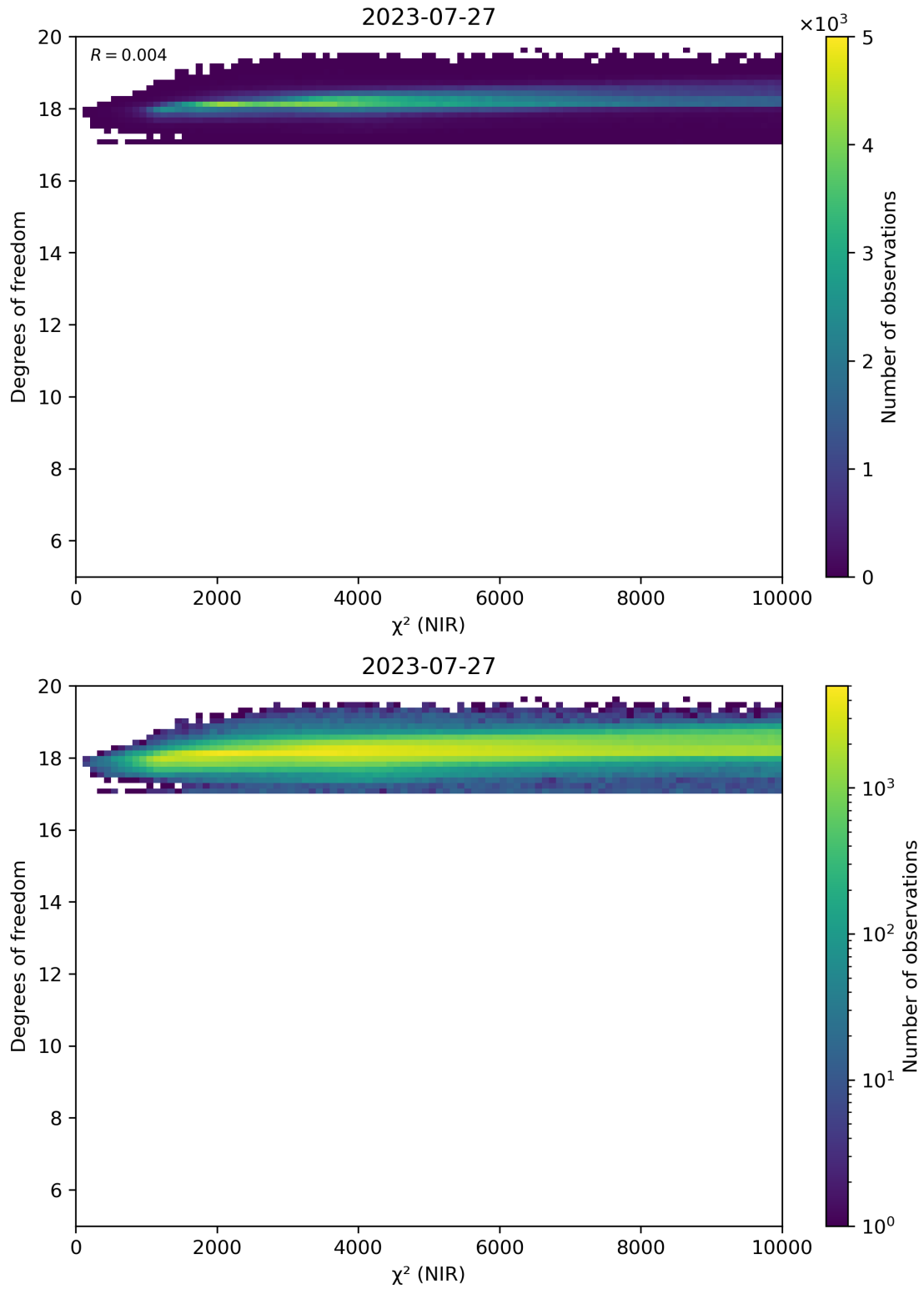
Figure 44: Scatter density plot of “ \chi^2 (NIR)” against “Degrees of freedom” for 2023-07-26 to 2023-07-28.
