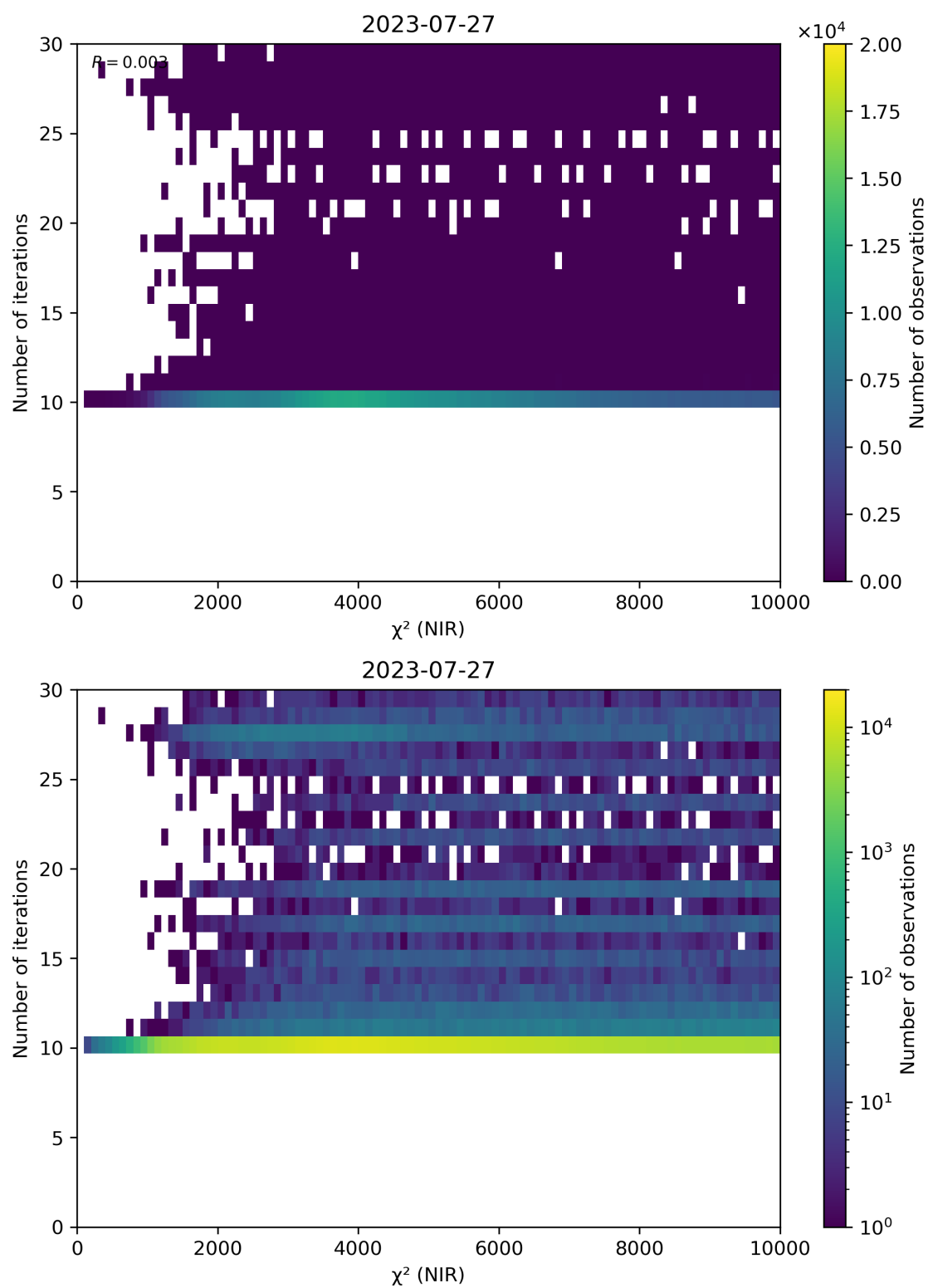
Figure 46: Scatter density plot of “ \chi^2 (NIR)” against “Number of iterations” for 2023-07-26 to 2023-07-28.
