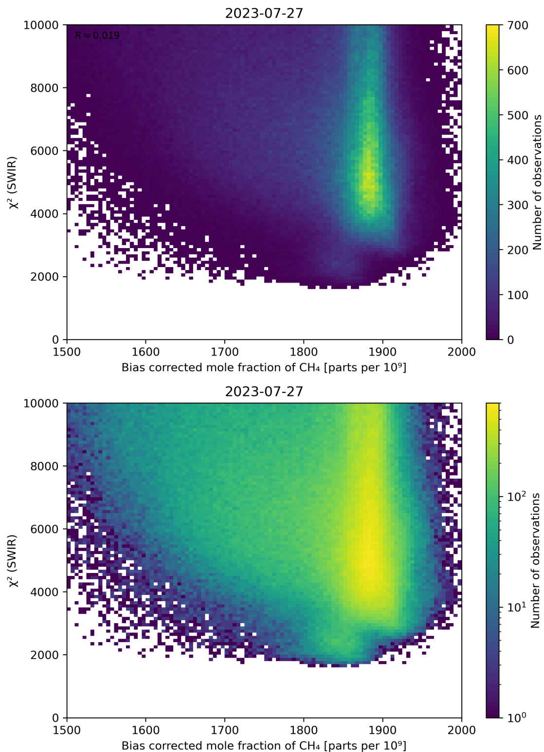
Figure 64: Scatter density plot of “Bias corrected mole fraction of \text{CH}_4 ” against “ \chi^2 (SWIR)” for 2023-07-26 to 2023-07-28.
