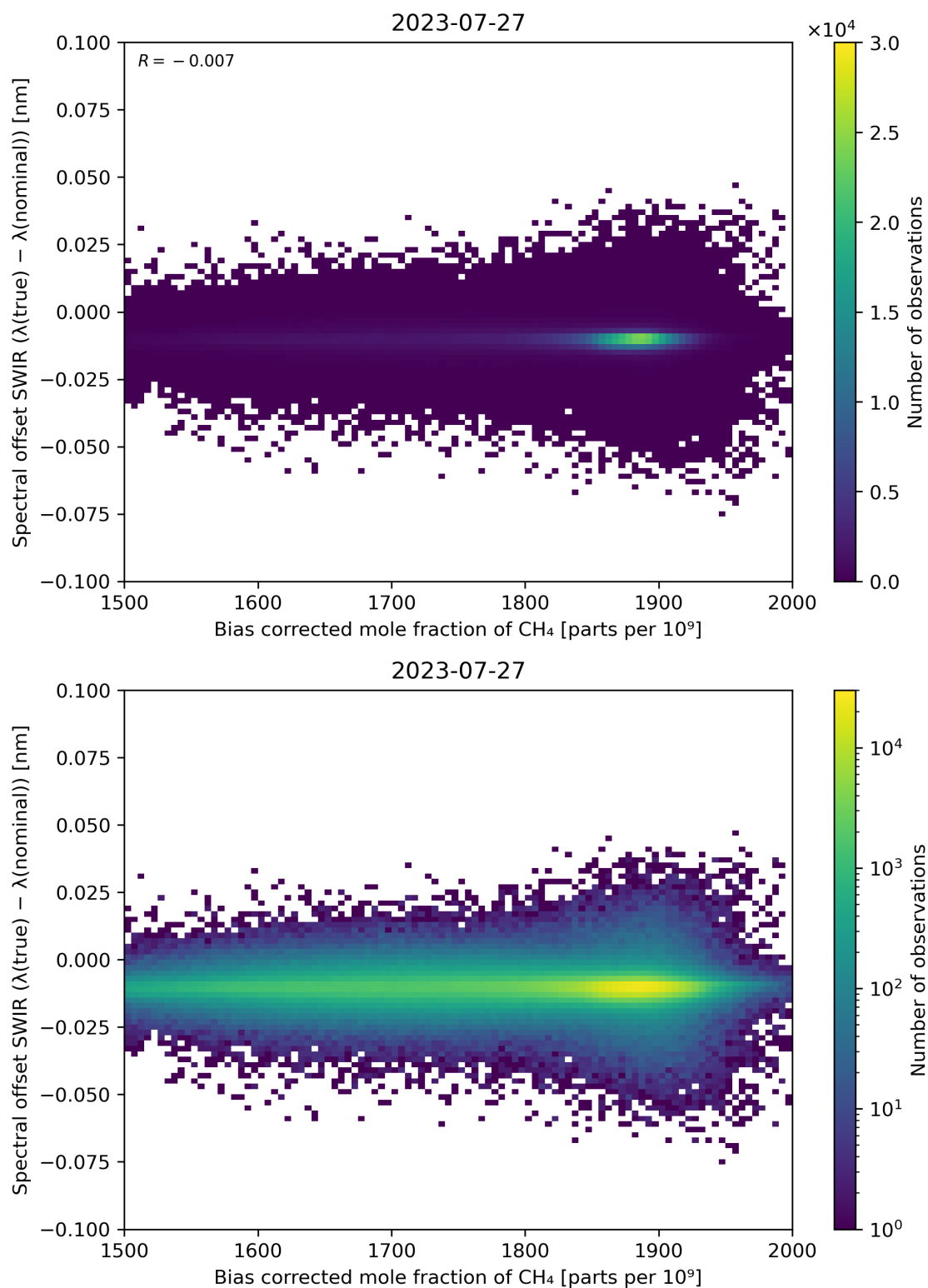
Figure 69: Scatter density plot of “Bias corrected mole fraction of \text{CH}_4 ” against “Spectral offset SWIR ( \lambda(\text{true}) - \lambda(\text{nominal}) )” for 2023-07-26 to 2023-07-28.
