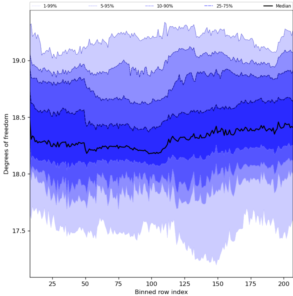
Figure 41: Along track statistics of “Degrees of freedom” for 2023-07-26 to 2023-07-28
