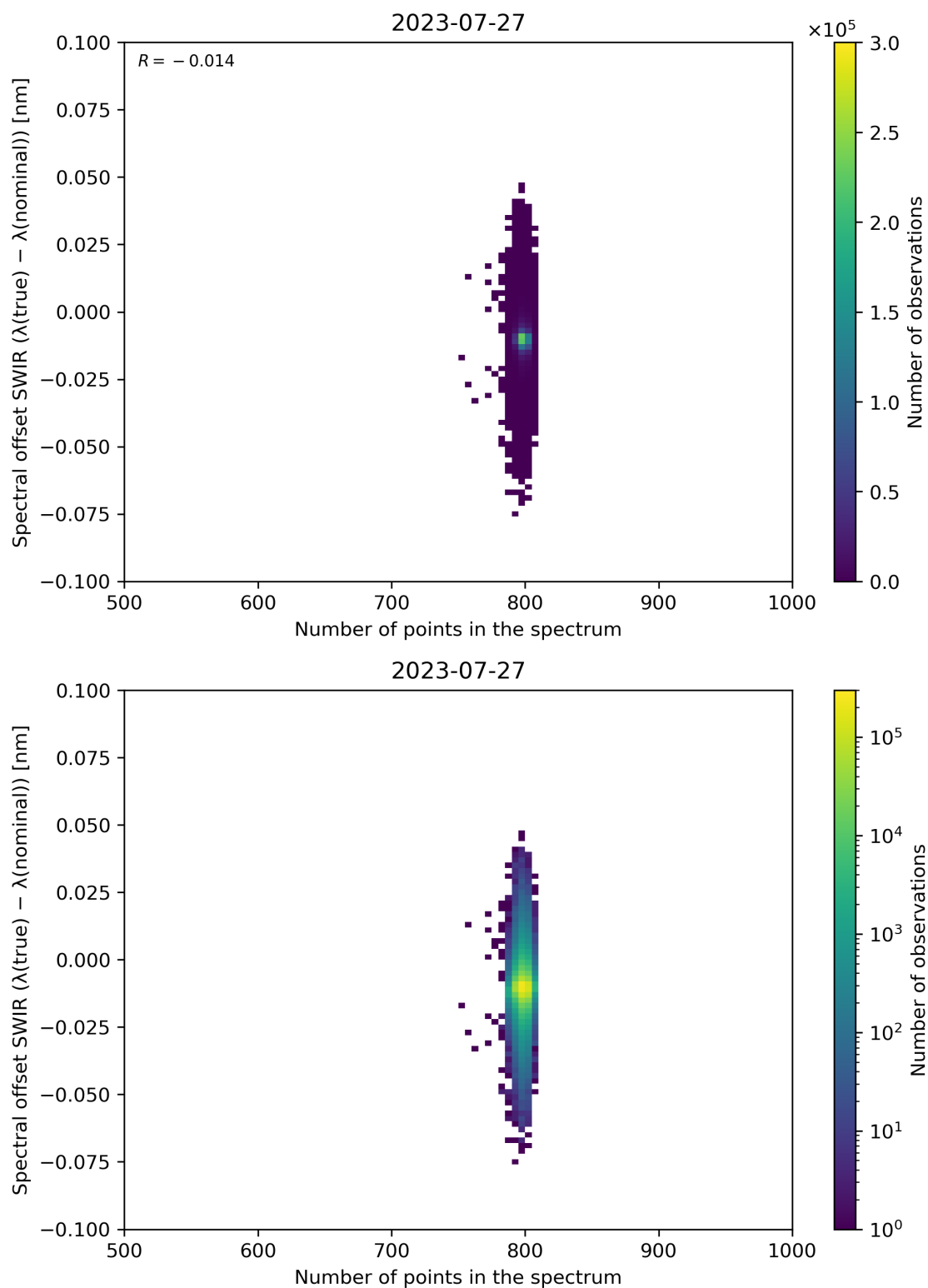
Figure 93: Scatter density plot of “Number of points in the spectrum” against “Spectral offset SWIR ( \lambda(\text{true}) - \lambda(\text{nominal}) )” for 2023-07-26 to 2023-07-28.
