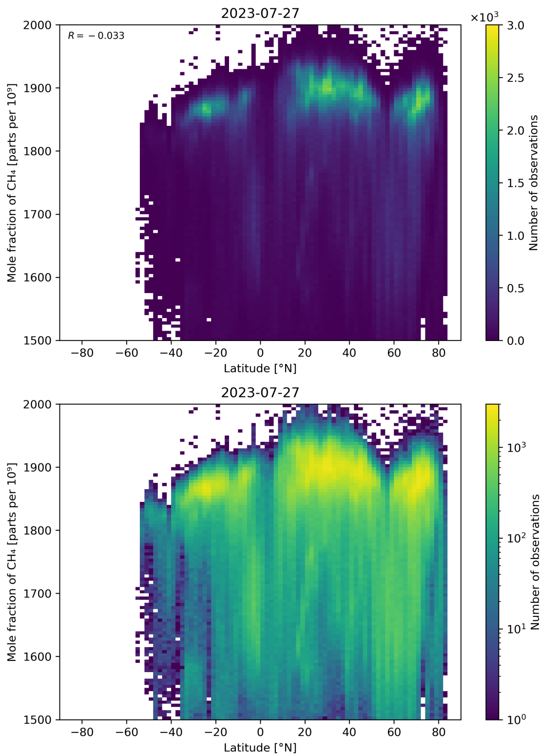
Figure 57: Scatter density plot of “Latitude” against “Mole fraction of CH 4 ” for 2023-07-26 to 2023-07-28.
