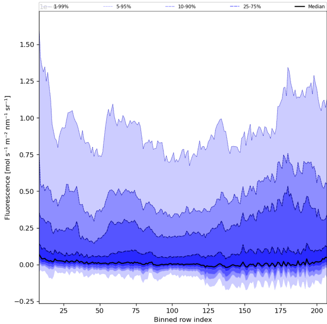
Figure 43: Along track statistics of “Fluorescence” for 2023-07-26 to 2023-07-28
