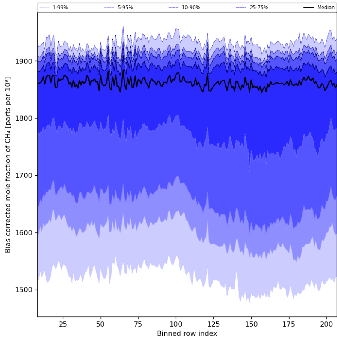
Figure 36: Along track statistics of “Bias corrected mole fraction of CH 4 ” for 2023-07-26 to 2023-07-28
