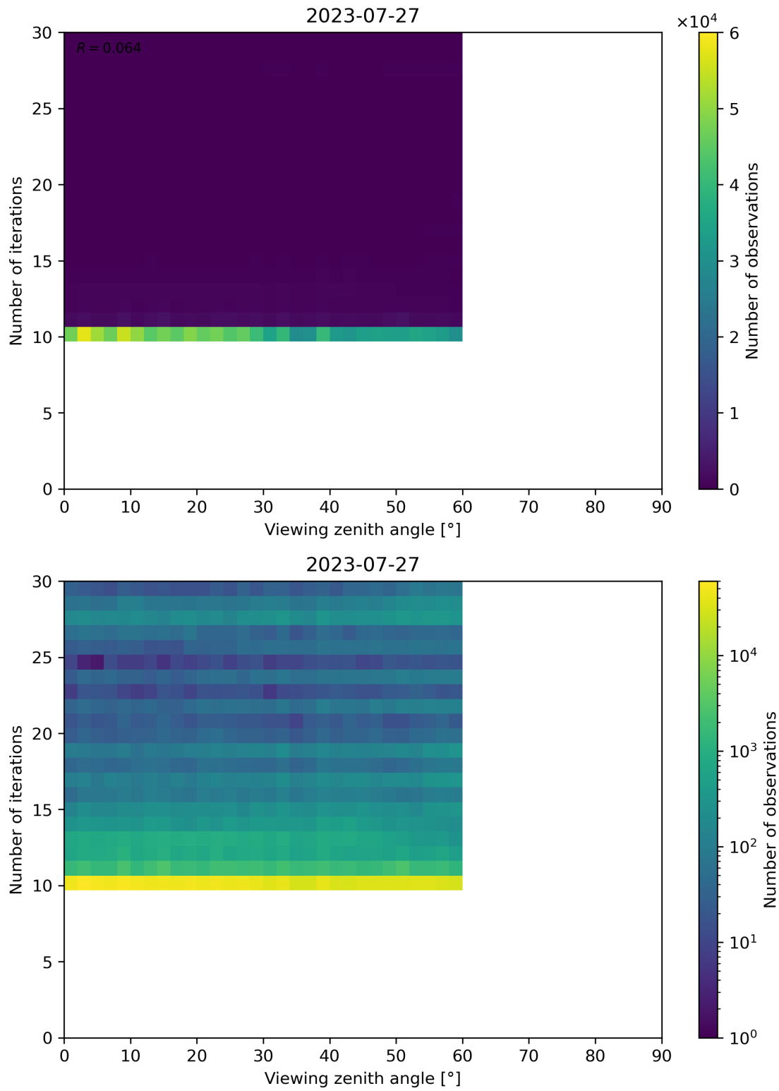
Figure 113: Scatter density plot of “Viewing zenith angle” against “Number of iterations” for 2023-07-26 to 2023-07-28.
