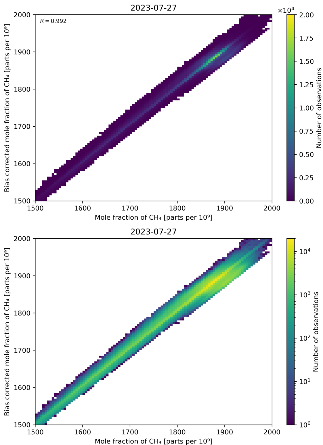
Figure 74: Scatter density plot of “Mole fraction of CH 4 ” against “Bias corrected mole fraction of CH 4 ” for 2023-07-26 to 2023-07-28.
