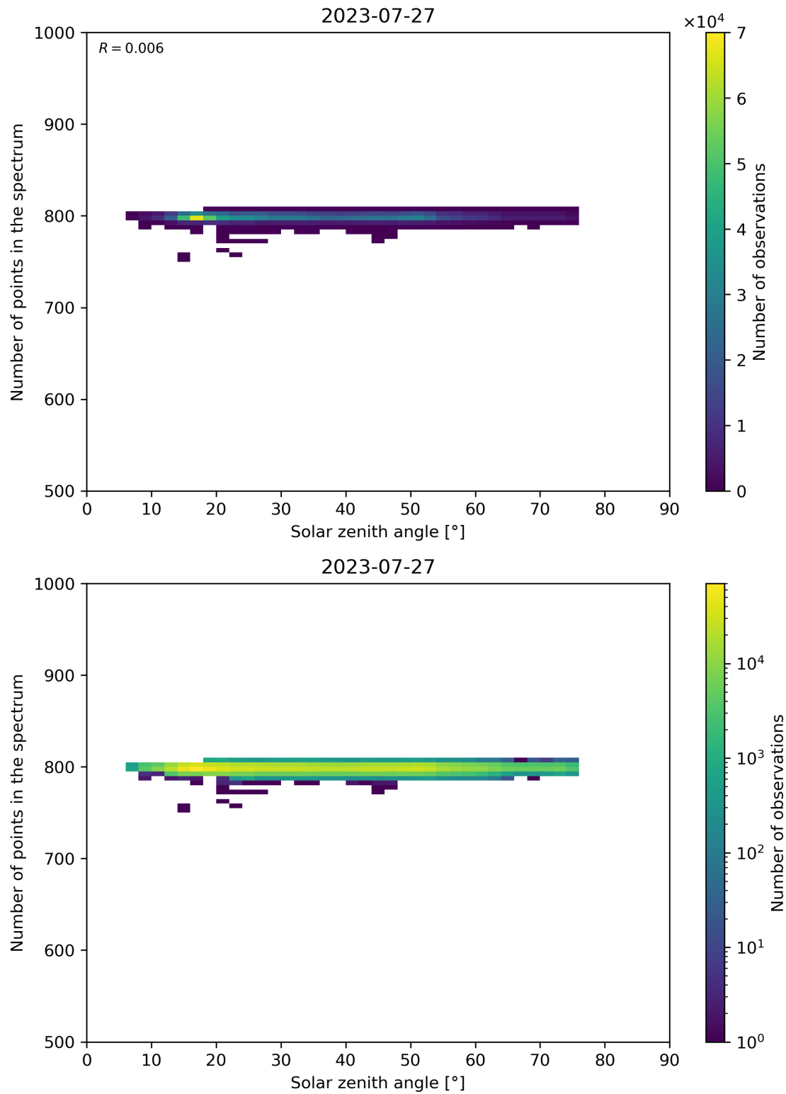
Figure 103: Scatter density plot of “Solar zenith angle” against “Number of points in the spectrum” for 2023-07-26 to 2023-07-28.
