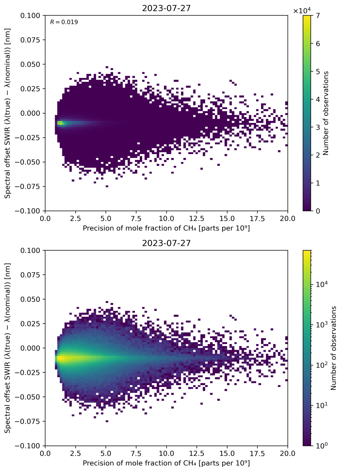
Figure 85: Scatter density plot of “Precision of mole fraction of CH 4 ” against “Spectral offset SWIR ( \lambda(\text{true}) - \lambda(\text{nominal}) )” for 2023-07-26 to 2023-07-28.
