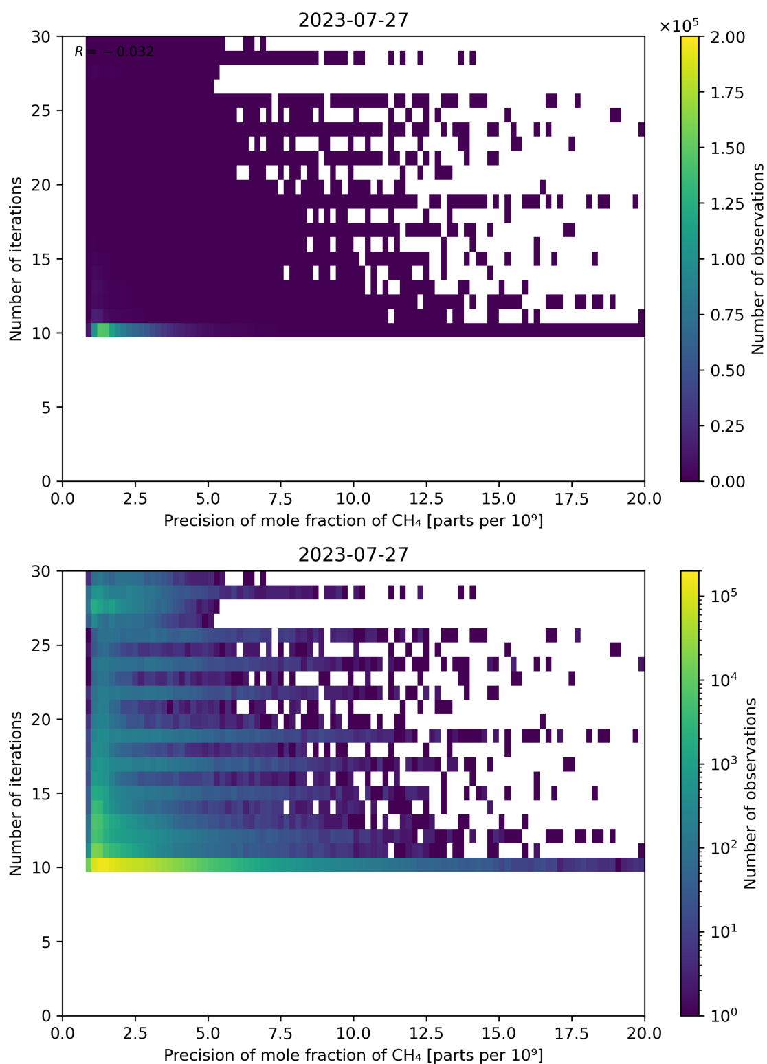
Figure 83: Scatter density plot of “Precision of mole fraction of CH 4 ” against “Number of iterations” for 2023-07-26 to 2023-07-28.
