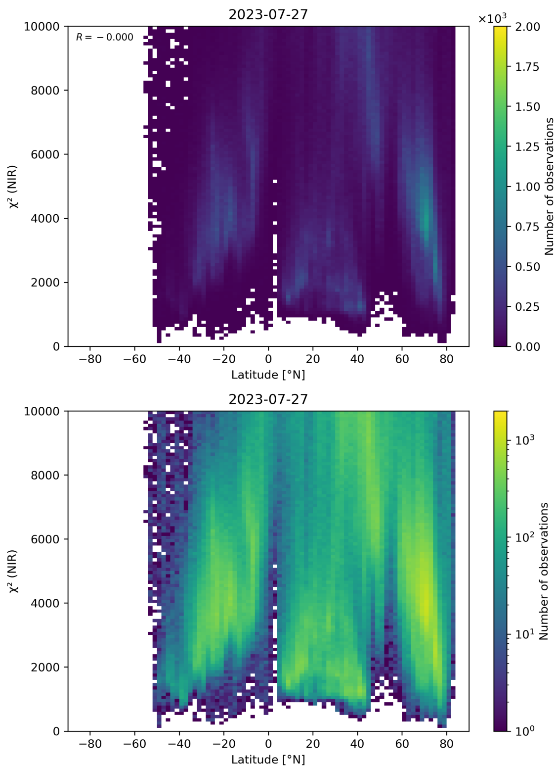
Figure 53: Scatter density plot of “Latitude” against “ \chi^2 (NIR)” for 2023-07-26 to 2023-07-28.
