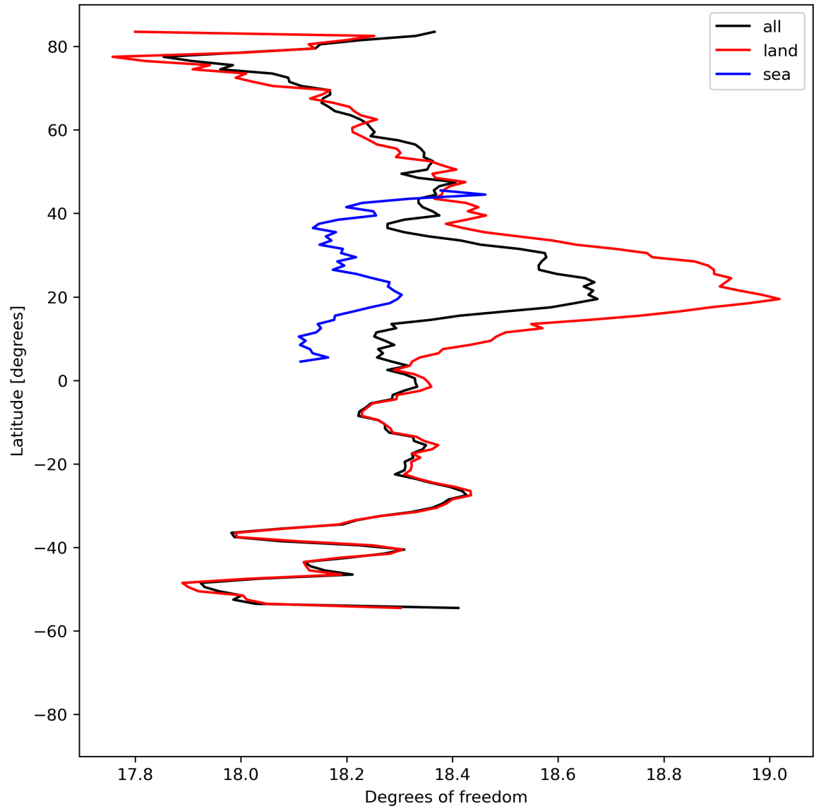
Figure 19: Zonal average of “Degrees of freedom” for 2023-07-26 to 2023-07-28.
