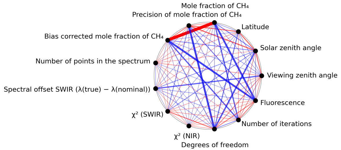
Figure 1: Map of correlation graph for 2023-07-26 to 2023-07-28.
