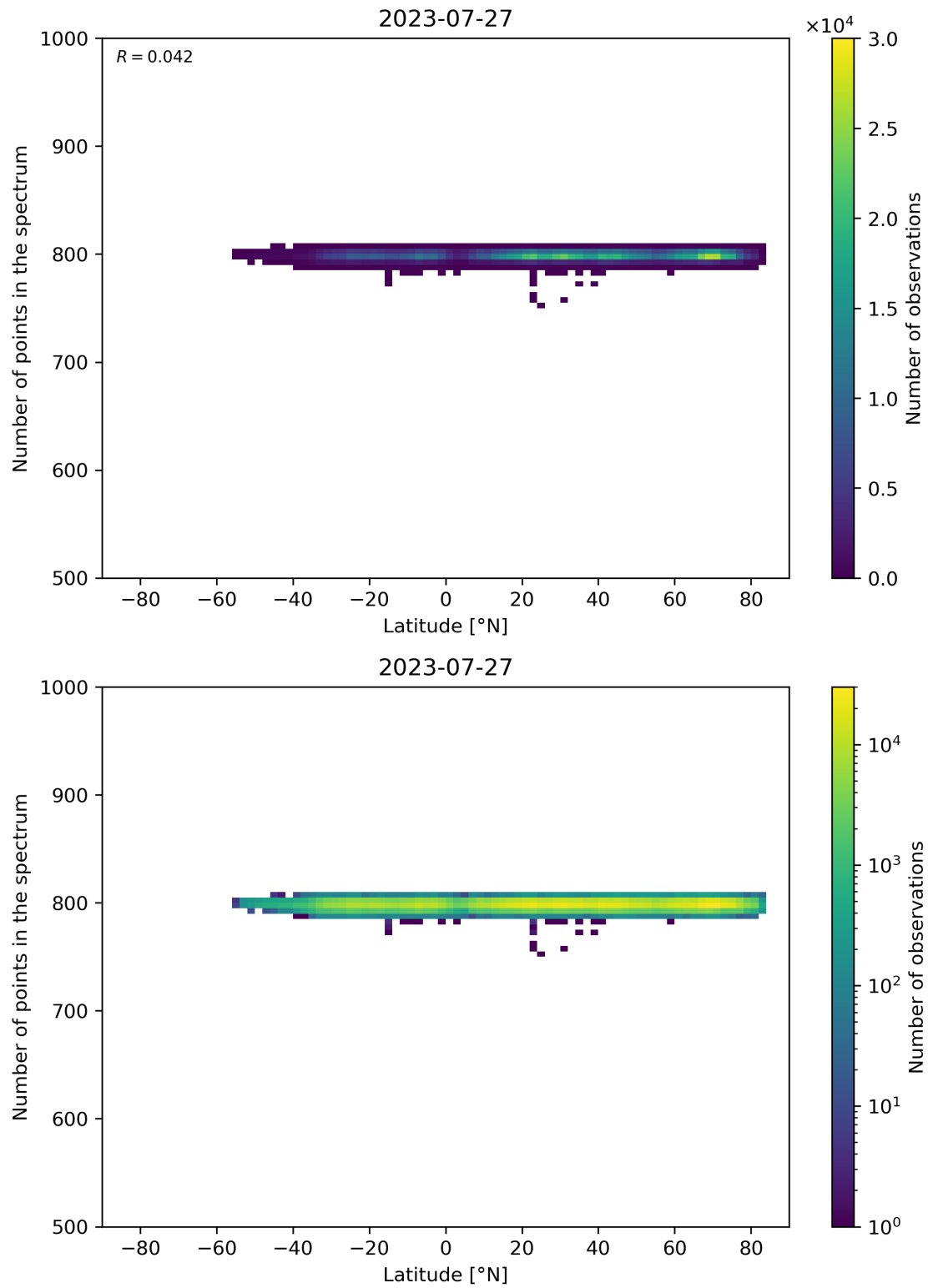
Figure 61: Scatter density plot of “Latitude” against “Number of points in the spectrum” for 2023-07-26 to 2023-07-28.
