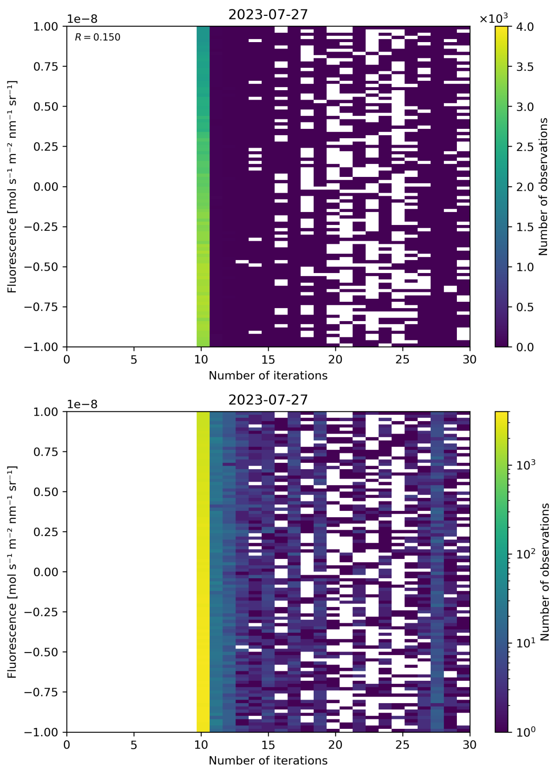
Figure 87: Scatter density plot of “Number of iterations” against “Fluorescence” for 2023-07-26 to 2023-07-28.
