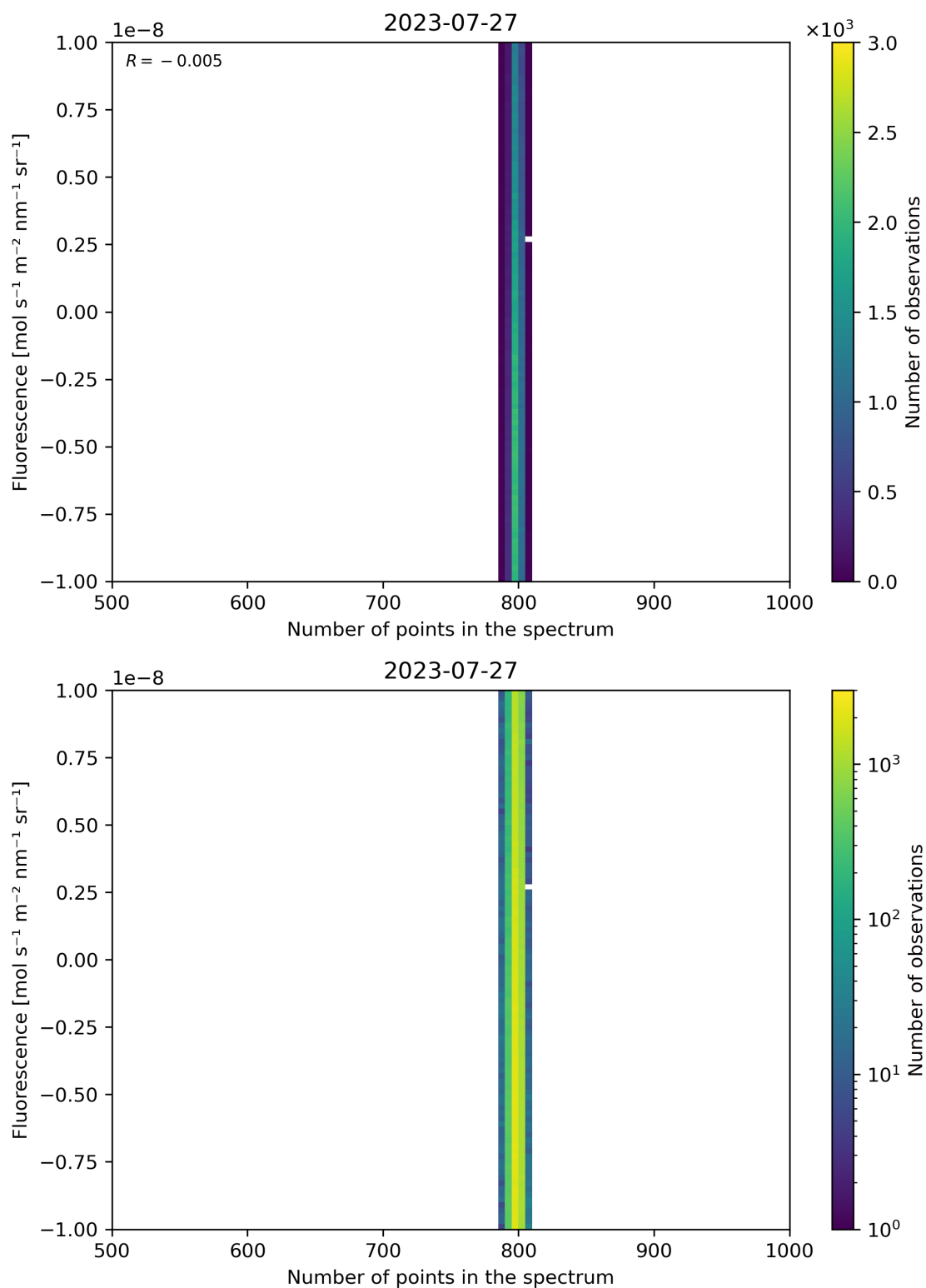
Figure 91: Scatter density plot of “Number of points in the spectrum” against “Fluorescence” for 2023-07-26 to 2023-07-28.
