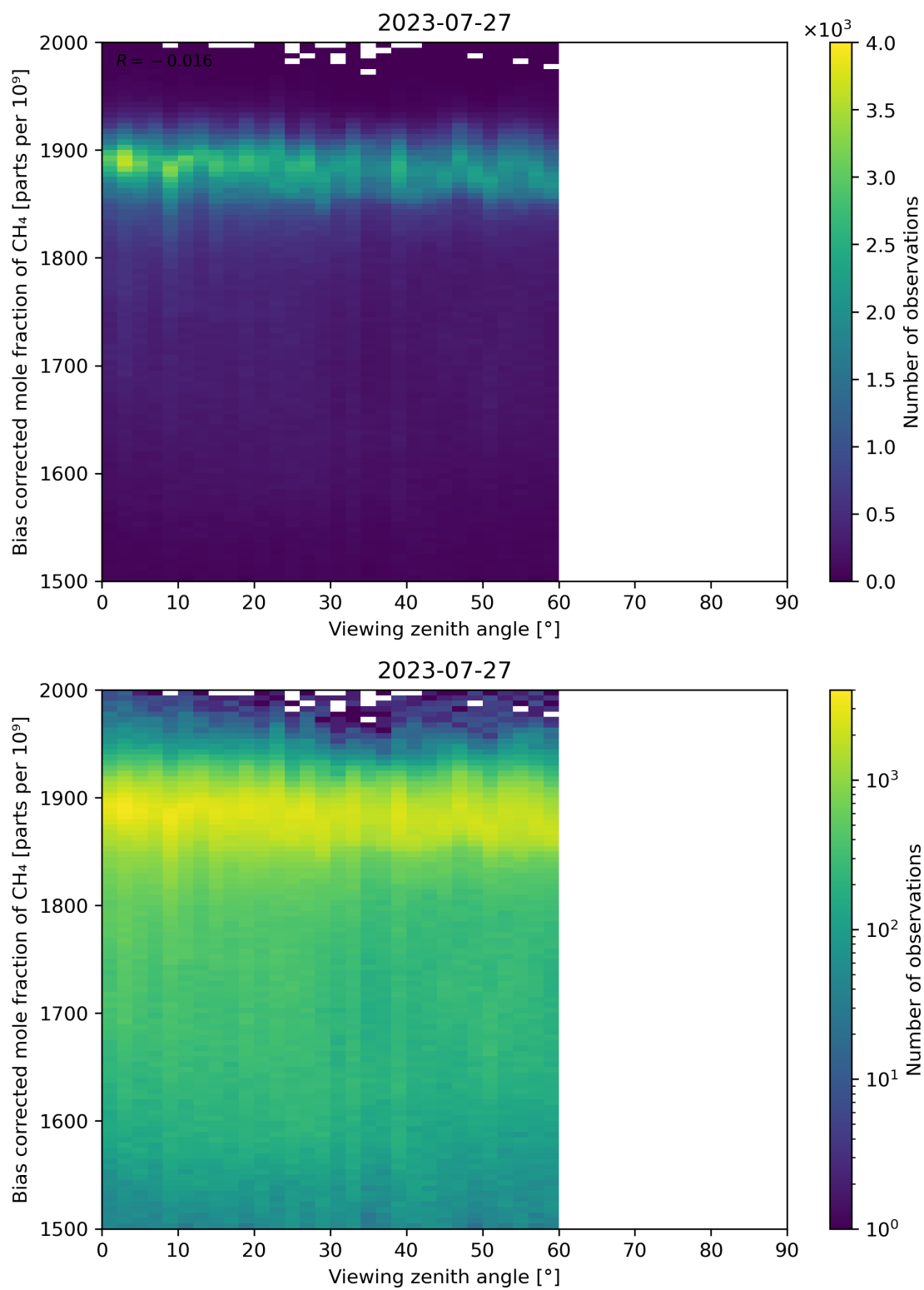
Figure 111: Scatter density plot of “Viewing zenith angle” against “Bias corrected mole fraction of CH 4 ” for 2023-07-26 to 2023-07-28.
