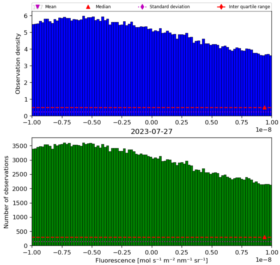
Figure 32: Histogram of “Fluorescence” for 2023-07-26 to 2023-07-28
