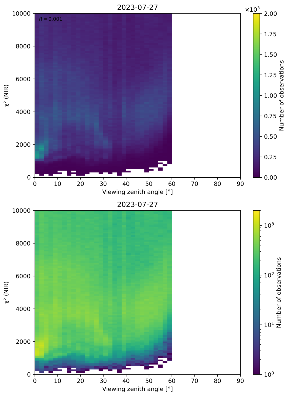
Figure 105: Scatter density plot of “Viewing zenith angle” against “ \chi^2 (NIR)” for 2023-07-26 to 2023-07-28.
