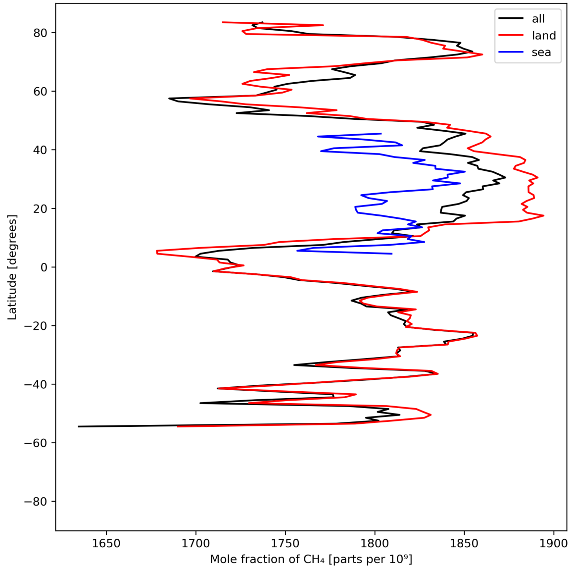
Figure 12: Zonal average of “Mole fraction of CH 4 ” for 2023-07-26 to 2023-07-28.
