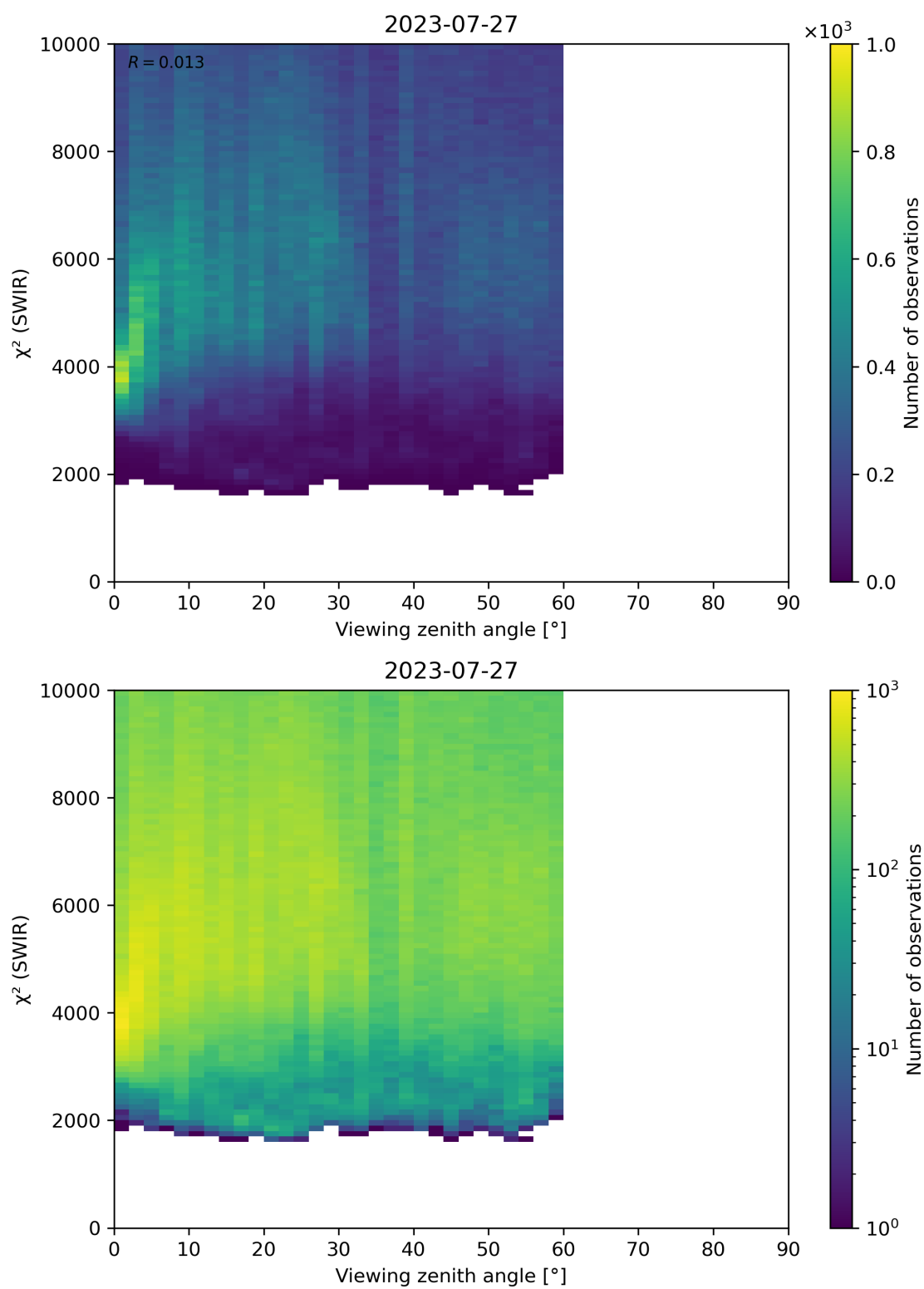
Figure 106: Scatter density plot of “Viewing zenith angle” against “ \chi^2 (SWIR)” for 2023-07-26 to 2023-07-28.
