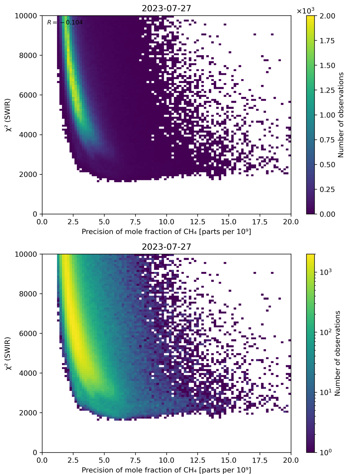
Figure 79: Scatter density plot of “Precision of mole fraction of CH 4 ” against “ \chi^2 (SWIR)” for 2023-07-26 to 2023-07-28.
