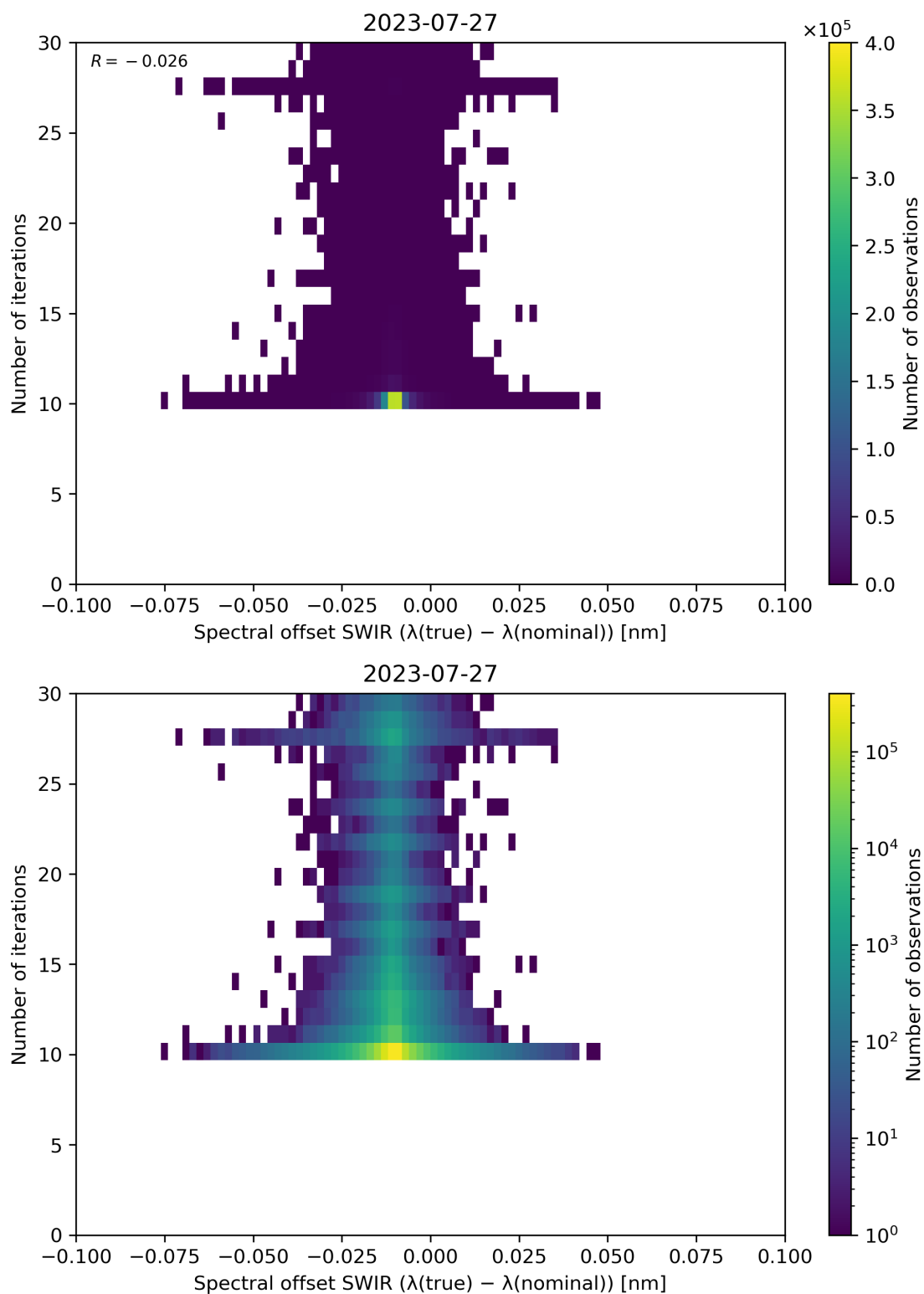
Figure 121: Scatter density plot of “Spectral offset SWIR ( \lambda(\text{true}) - \lambda(\text{nominal}) )” against “Number of iterations” for 2023-07-26 to 2023-07-28.
