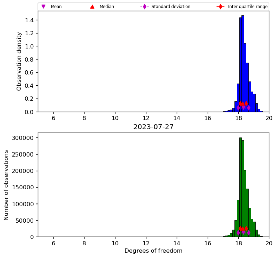
Figure 30: Histogram of “Degrees of freedom” for 2023-07-26 to 2023-07-28
