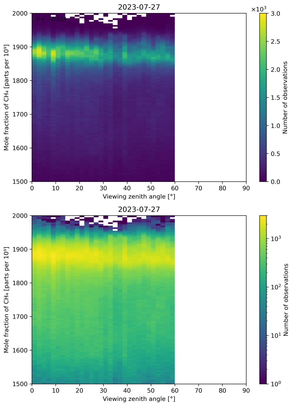
Figure 110: Scatter density plot of “Viewing zenith angle” against “Mole fraction of CH 4 ” for 2023-07-26 to 2023-07-28.
