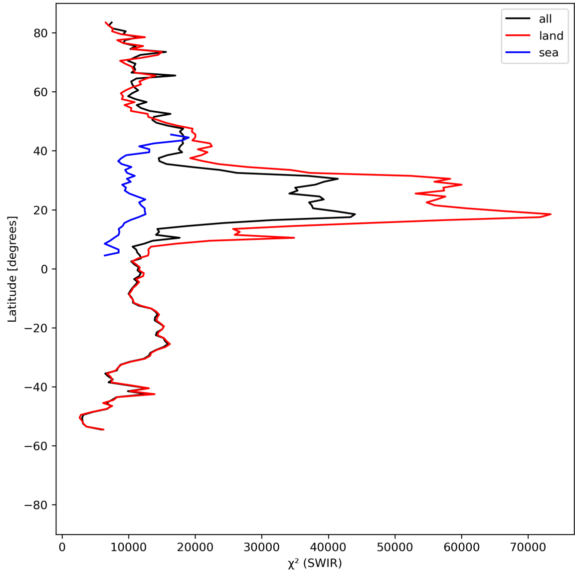
Figure 17: Zonal average of “ \chi^2 (SWIR)” for 2023-07-26 to 2023-07-28.
