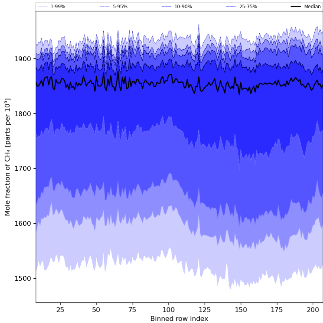
Figure 34: Along track statistics of “Mole fraction of CH 4 ” for 2023-07-26 to 2023-07-28
