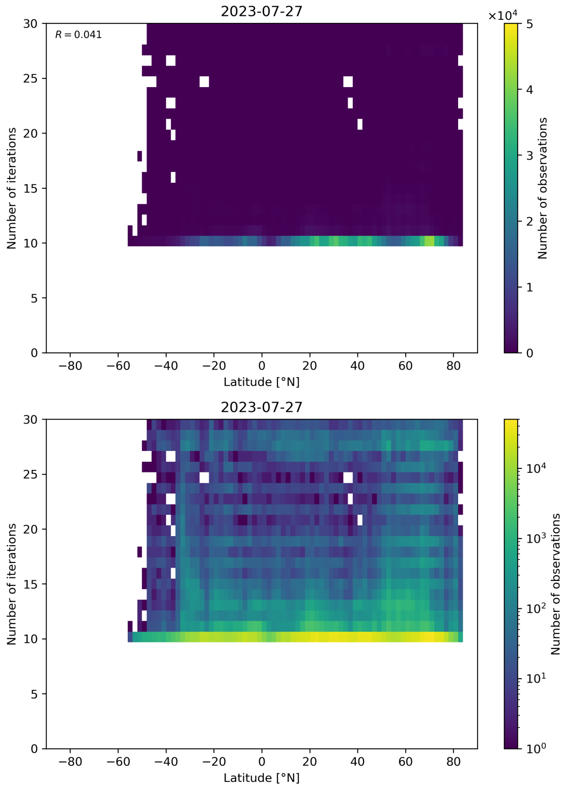
Figure 60: Scatter density plot of “Latitude” against “Number of iterations” for 2023-07-26 to 2023-07-28.
