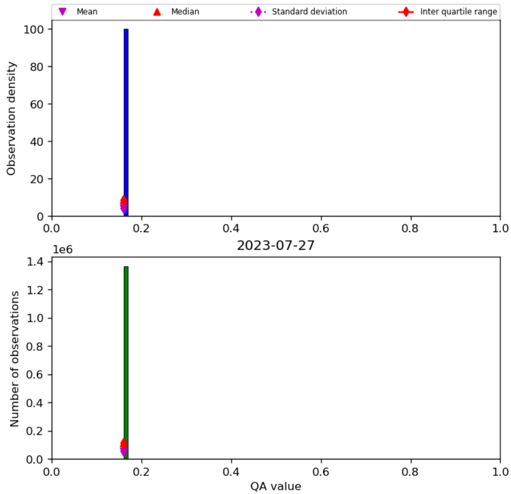
Figure 22: Histogram of “QA value” for 2023-07-26 to 2023-07-28
