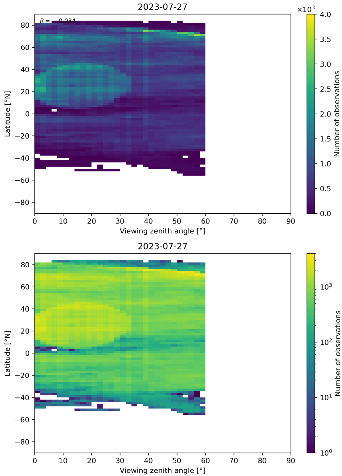
Figure 109: Scatter density plot of “Viewing zenith angle” against “Latitude” for 2023-07-26 to 2023-07-28.
