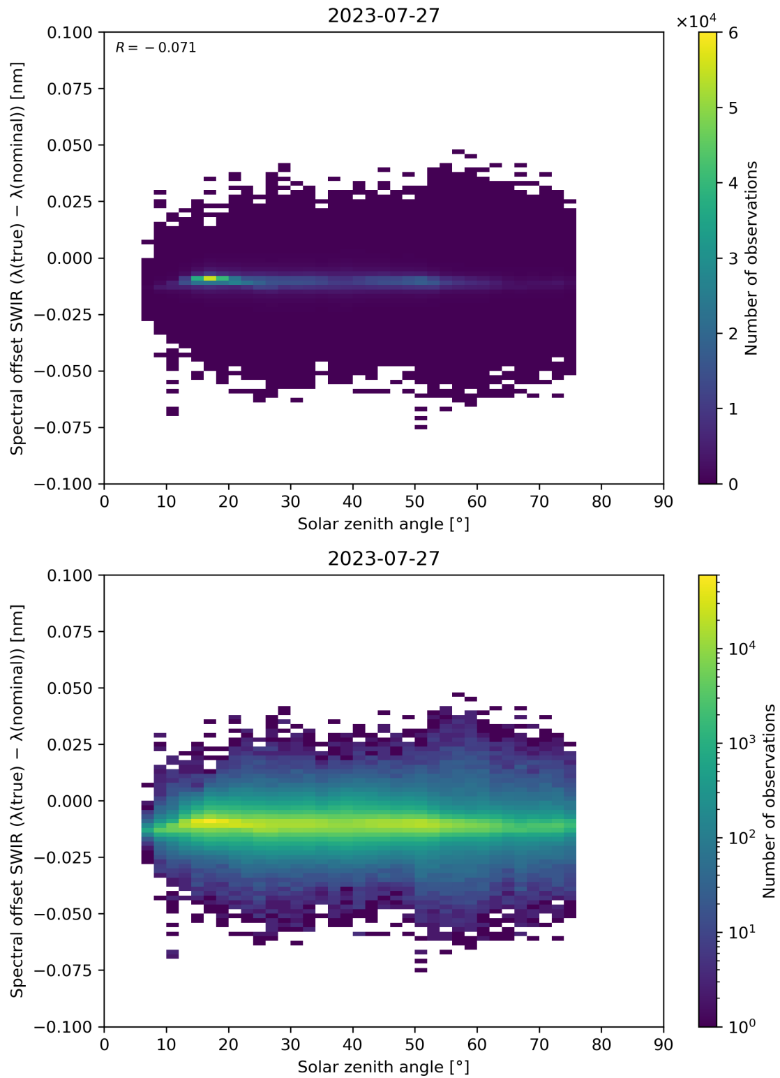
Figure 104: Scatter density plot of “Solar zenith angle” against “Spectral offset SWIR ( \lambda(\text{true}) - \lambda(\text{nominal}) )” for 2023-07-26 to 2023-07-28.
