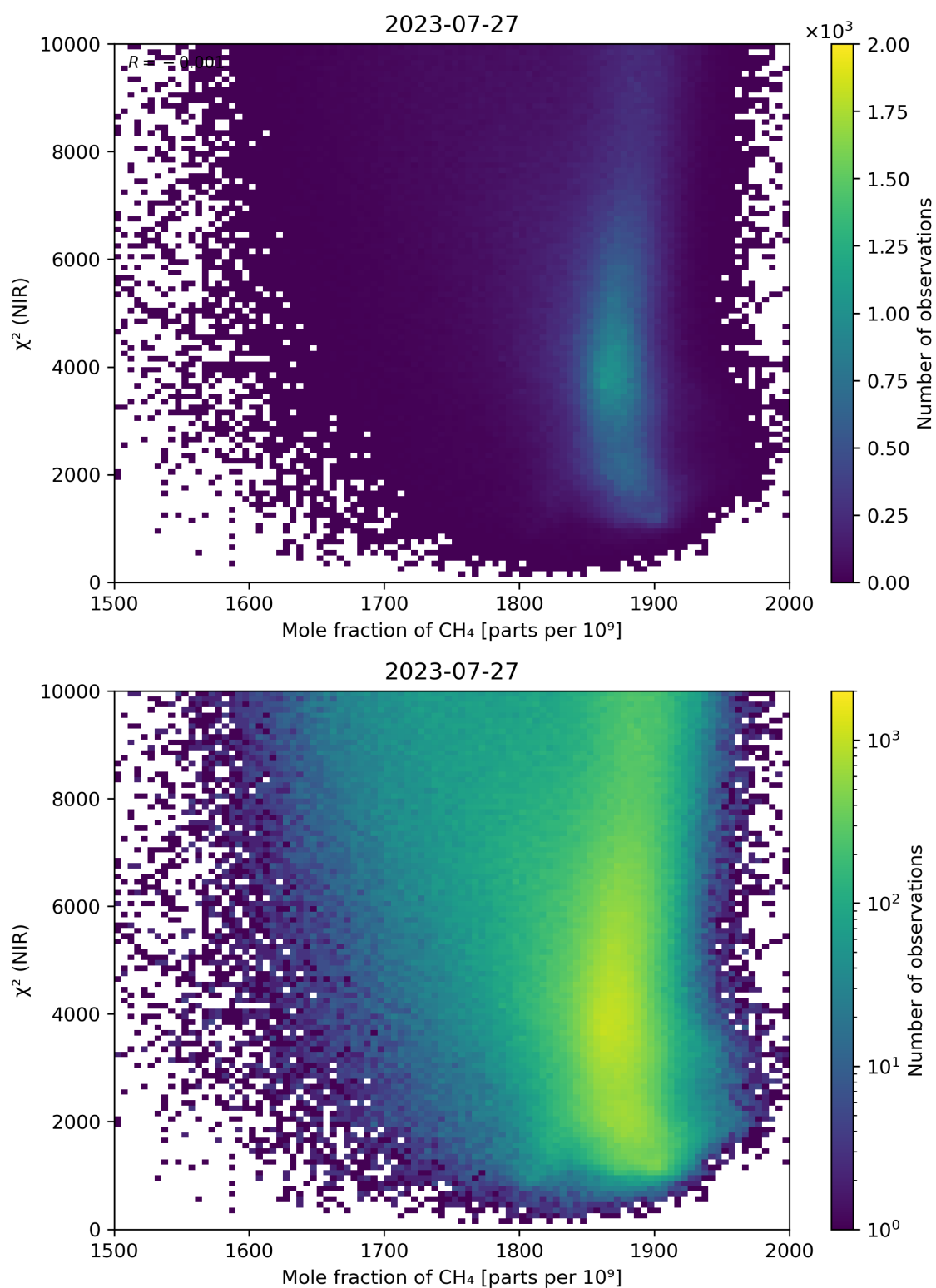
Figure 70: Scatter density plot of “Mole fraction of CH 4 ” against “ \chi^2 (NIR)” for 2023-07-26 to 2023-07-28.
