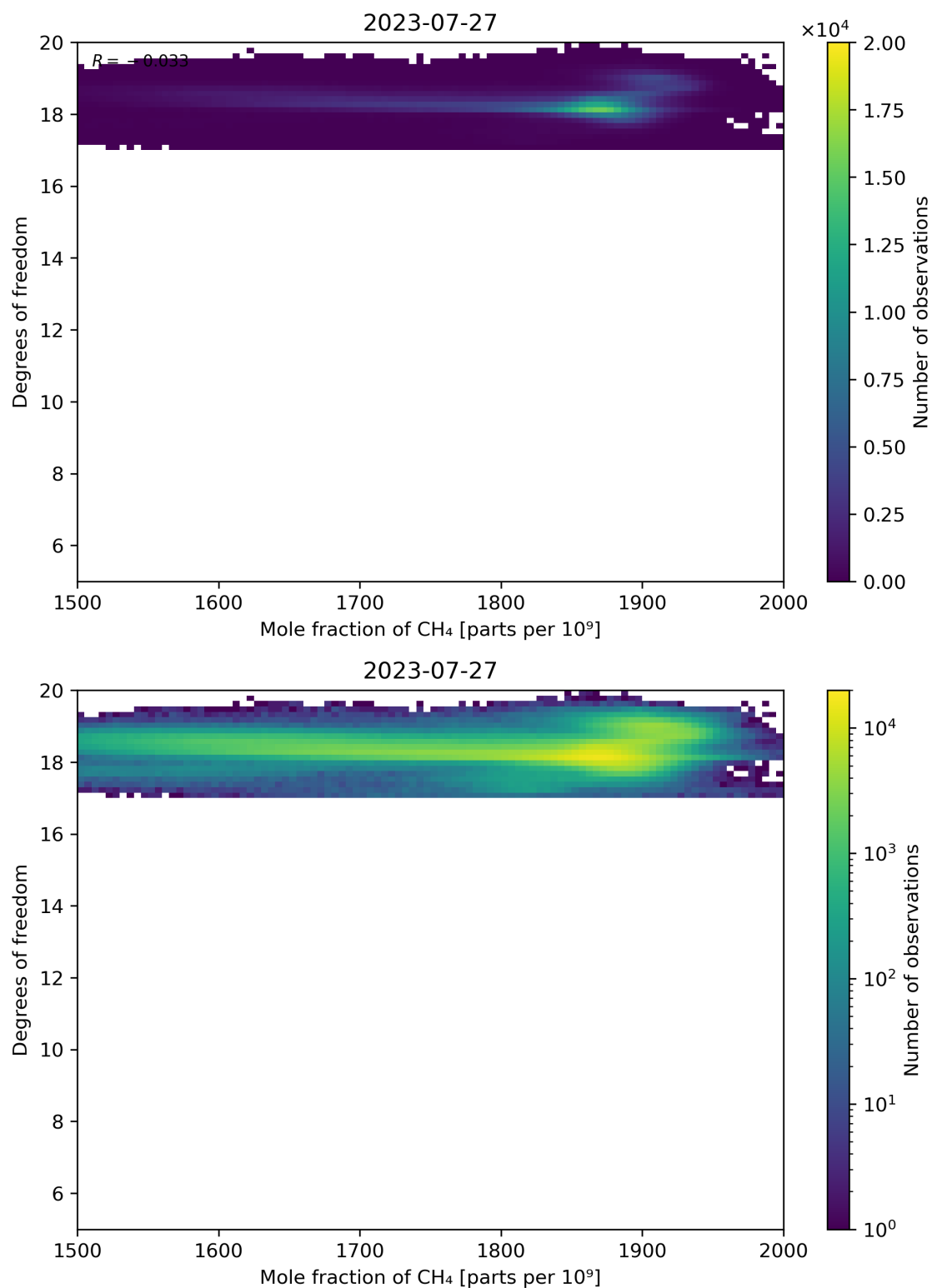
Figure 72: Scatter density plot of “Mole fraction of CH 4 ” against “Degrees of freedom” for 2023-07-26 to 2023-07-28.
