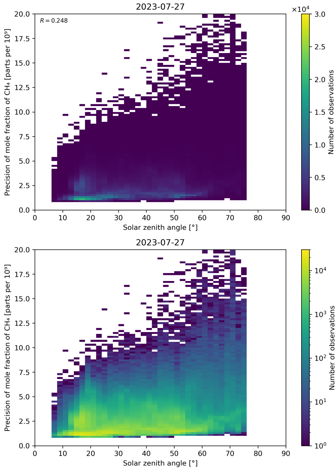
Figure 101: Scatter density plot of “Solar zenith angle” against “Precision of mole fraction of \text{CH}_4 ” for 2023-07-26 to 2023-07-28.
