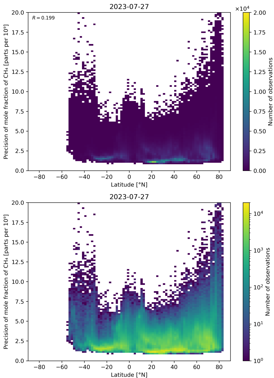
Figure 59: Scatter density plot of “Latitude” against “Precision of mole fraction of CH 4 ” for 2023-07-26 to 2023-07-28.
