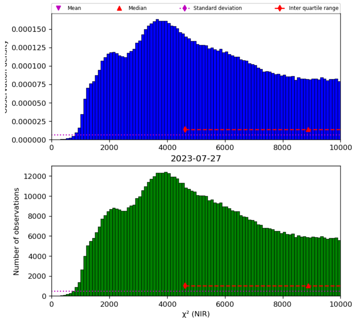
Figure 29: Histogram of “ \chi^2 (NIR)” for 2023-07-26 to 2023-07-28
