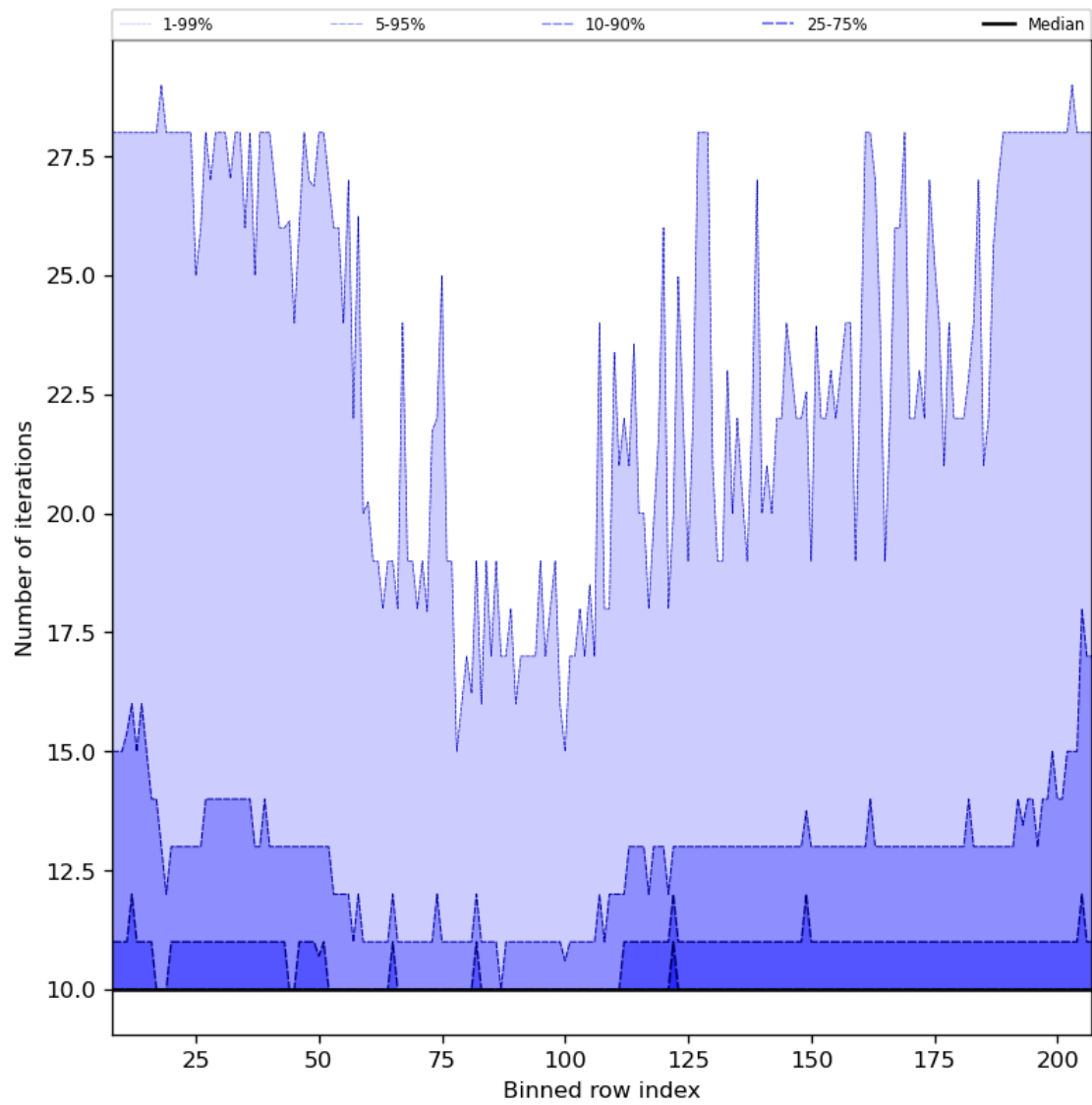
Figure 42: Along track statistics of “Number of iterations” for 2023-07-26 to 2023-07-28
