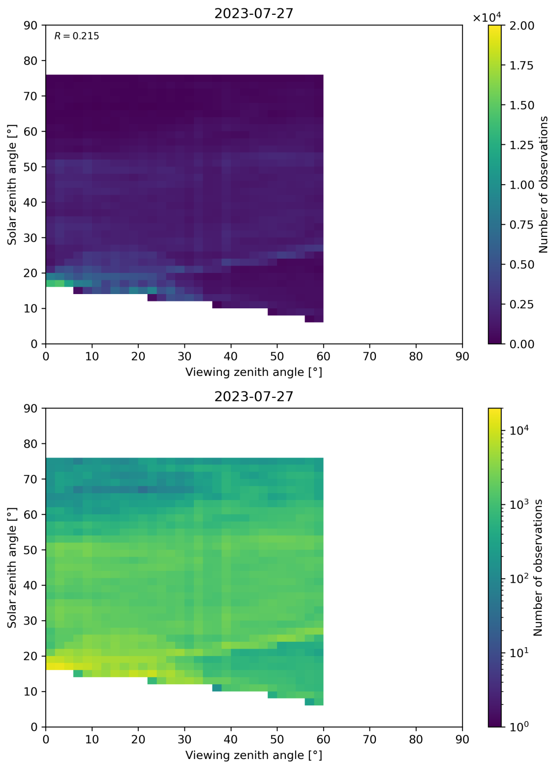
Figure 115: Scatter density plot of “Viewing zenith angle” against “Solar zenith angle” for 2023-07-26 to 2023-07-28.
