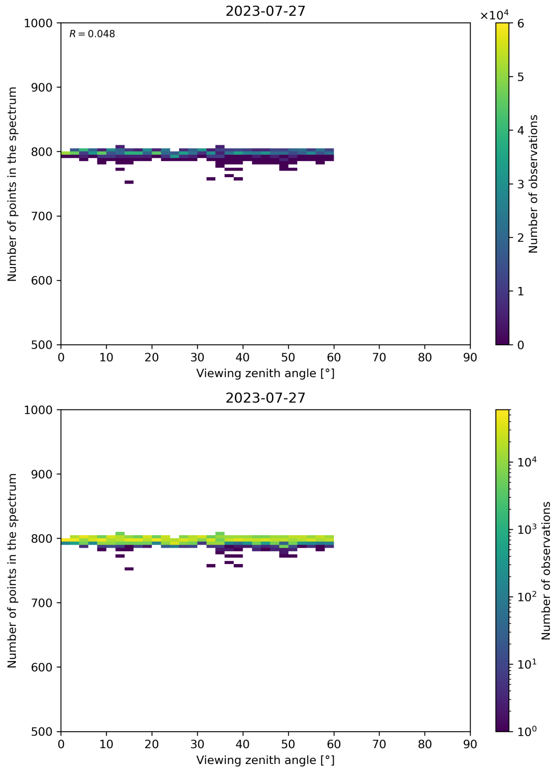
Figure 114: Scatter density plot of “Viewing zenith angle” against “Number of points in the spectrum” for 2023-07-26 to 2023-07-28.
