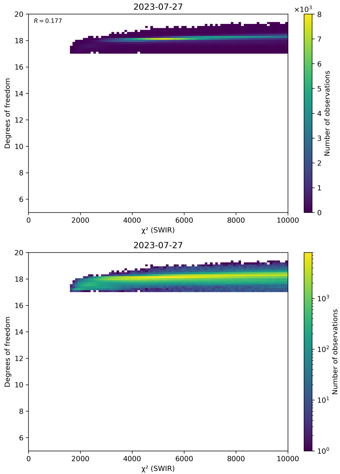
Figure 48: Scatter density plot of “ \chi^2 (SWIR)” against “Degrees of freedom” for 2023-07-26 to 2023-07-28.
