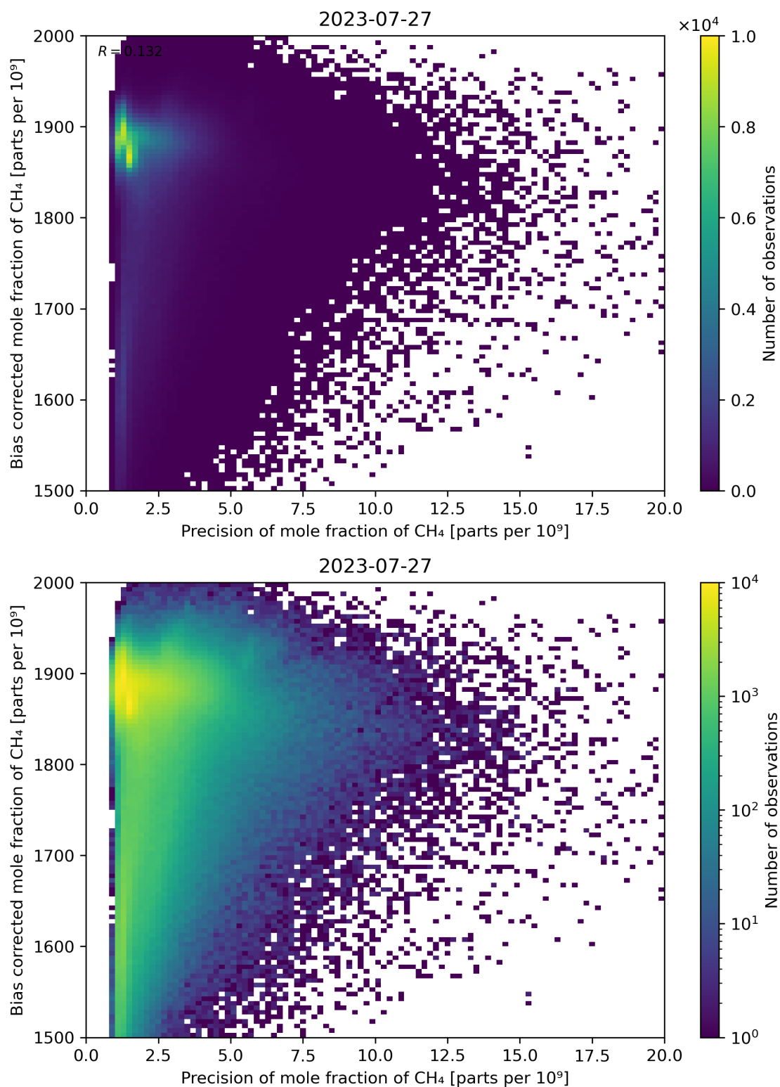
Figure 82: Scatter density plot of “Precision of mole fraction of \text{CH}_4 ” against “Bias corrected mole fraction of \text{CH}_4 ” for 2023-07-26 to 2023-07-28.
