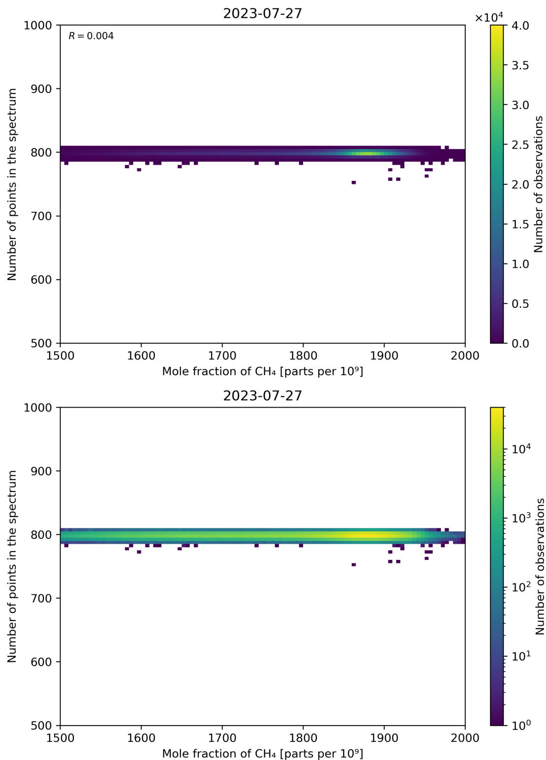
Figure 77: Scatter density plot of “Mole fraction of CH 4 ” against “Number of points in the spectrum” for 2023-07-26 to 2023-07-28.
