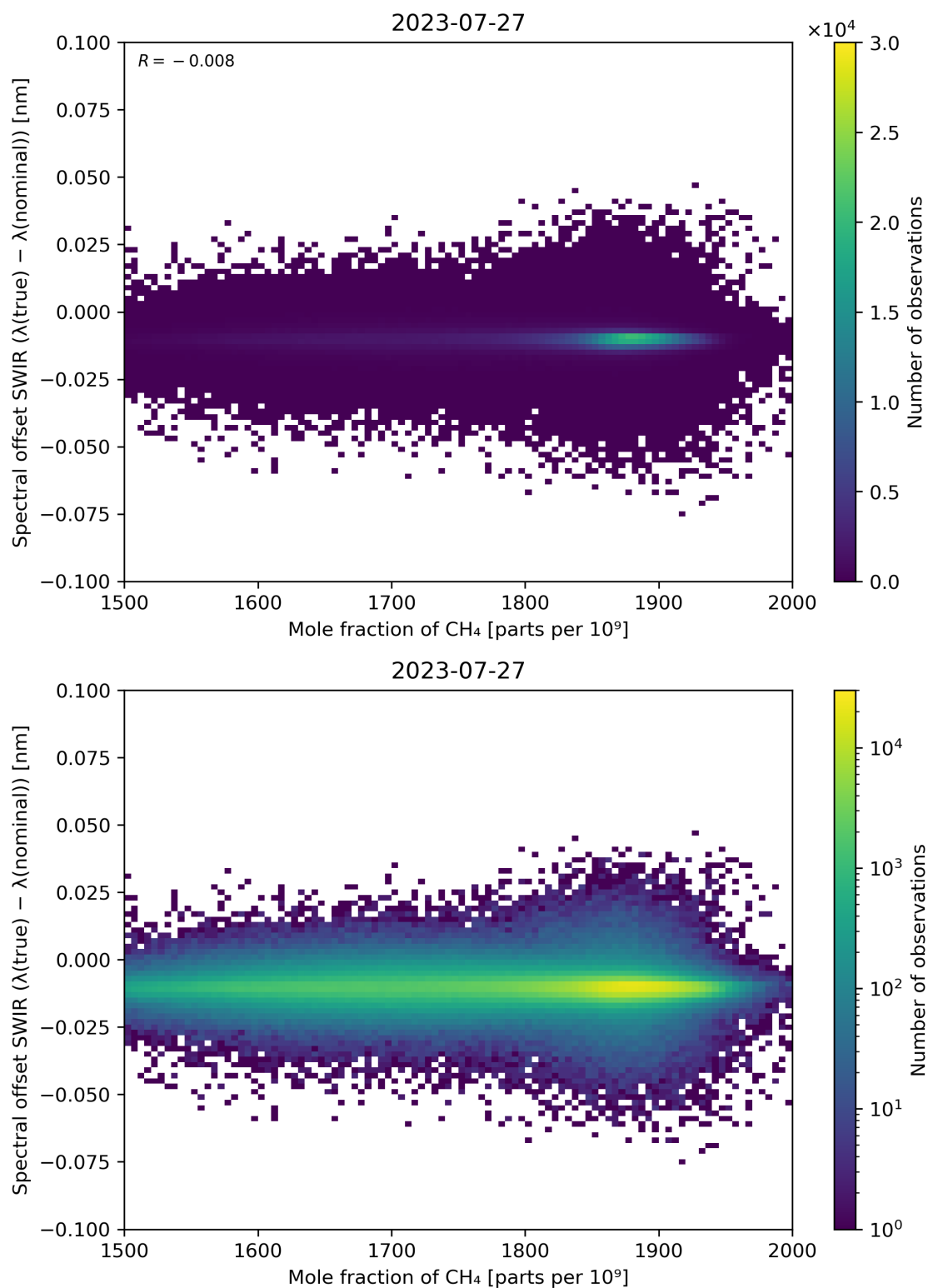
Figure 86: Scatter density plot of “Mole fraction of CH 4 ” against “Spectral offset SWIR ( \lambda(\text{true}) - \lambda(\text{nominal}) )” for 2023-07-26 to 2023-07-28.
