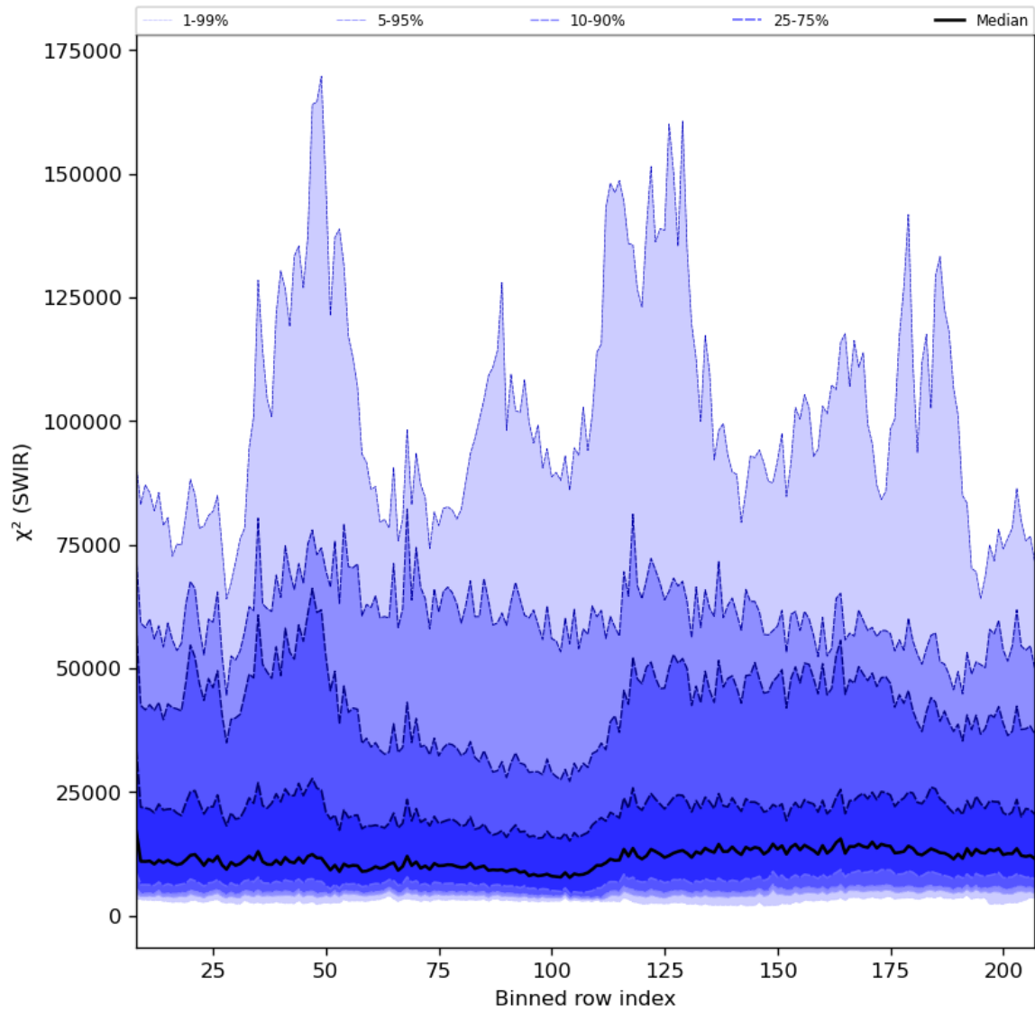
Figure 39: Along track statistics of “ \chi^2 (SWIR)” for 2023-07-26 to 2023-07-28
