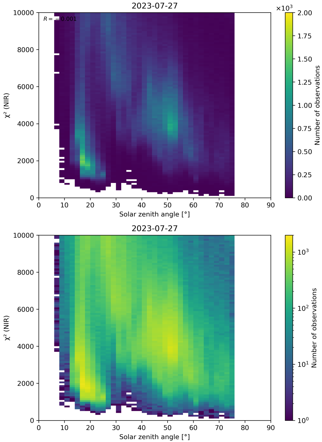
Figure 94: Scatter density plot of “Solar zenith angle” against “ \chi^2 (NIR)” for 2023-07-26 to 2023-07-28.
