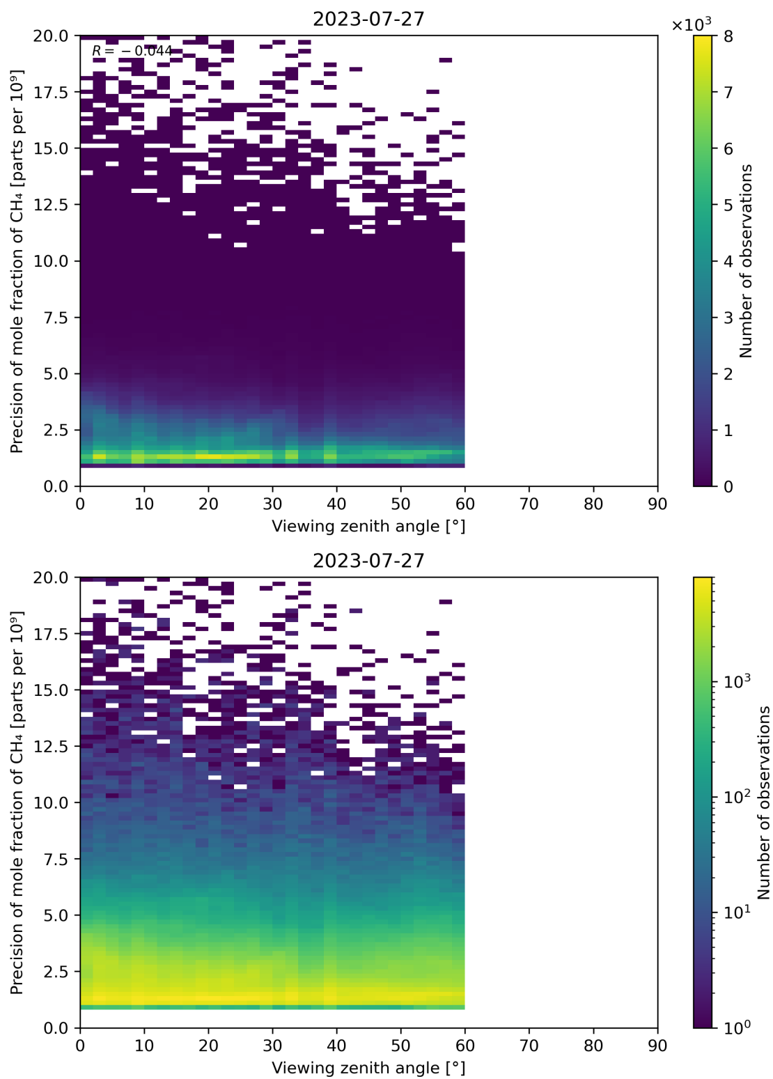
Figure 112: Scatter density plot of “Viewing zenith angle” against “Precision of mole fraction of CH 4 ” for 2023-07-26 to 2023-07-28.
