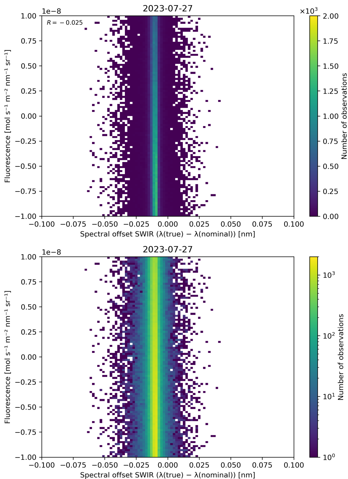
Figure 120: Scatter density plot of “Spectral offset SWIR ( \lambda(\text{true}) - \lambda(\text{nominal}) )” against “Fluorescence” for 2023-07-26 to 2023-07-28.
