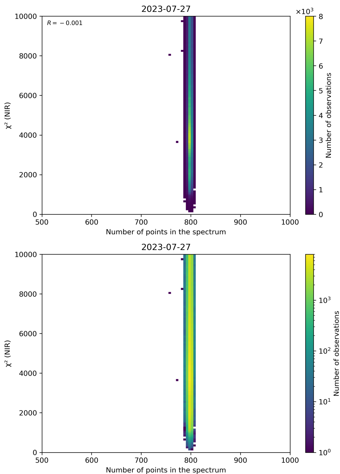
Figure 88: Scatter density plot of “Number of points in the spectrum” against “ \chi^2 (NIR)” for 2023-07-26 to 2023-07-28.
