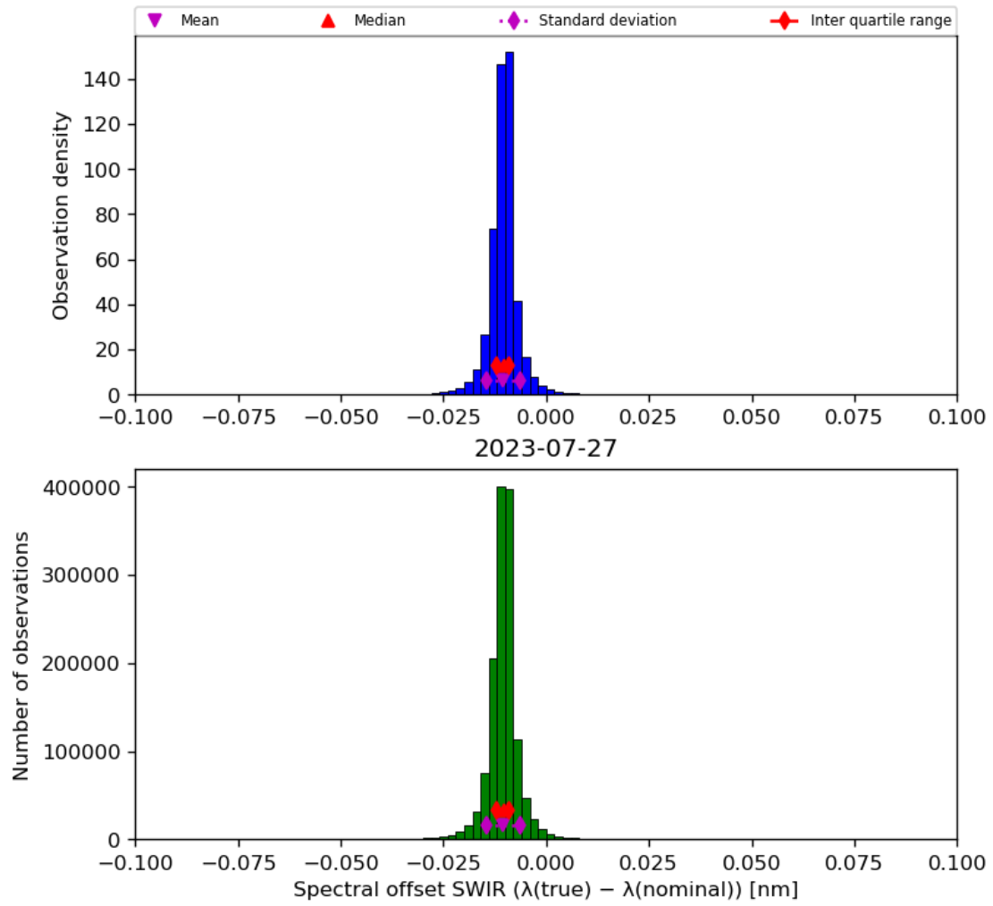
Figure 27: Histogram of “Spectral offset SWIR ( \lambda(\text{true}) - \lambda(\text{nominal}) )” for 2023-07-26 to 2023-07-28
