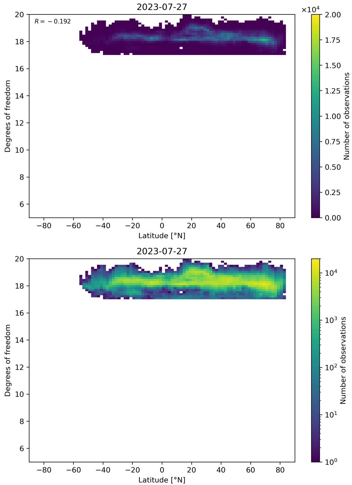
Figure 55: Scatter density plot of “Latitude” against “Degrees of freedom” for 2023-07-26 to 2023-07-28.
