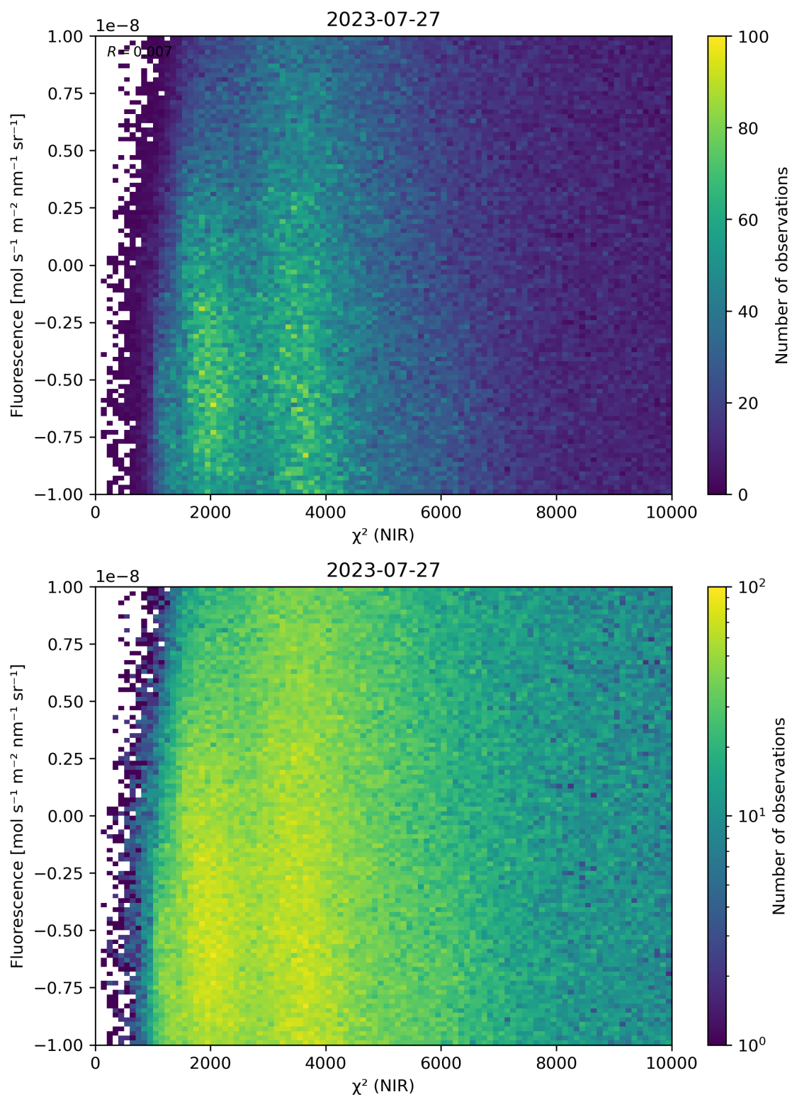
Figure 45: Scatter density plot of “ \chi^2 (NIR)” against “Fluorescence” for 2023-07-26 to 2023-07-28.
