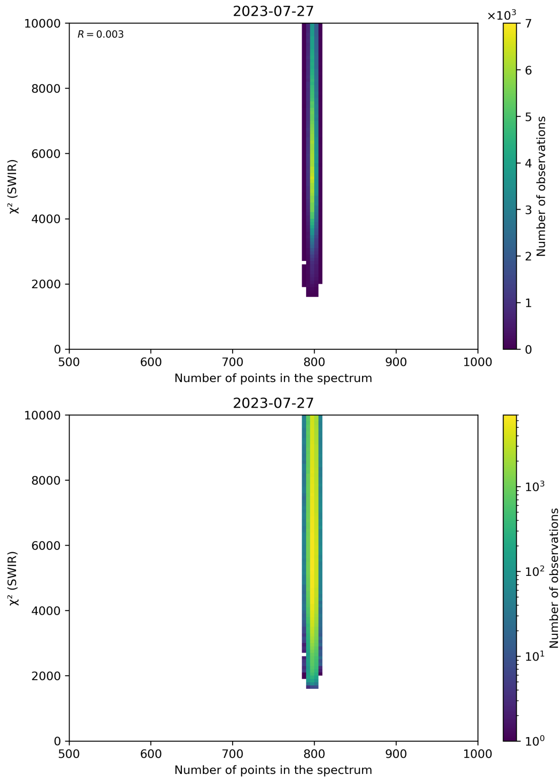
Figure 89: Scatter density plot of “Number of points in the spectrum” against “ \chi^2 (SWIR)” for 2023-07-26 to 2023-07-28.
