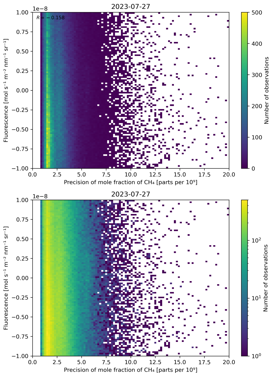
Figure 81: Scatter density plot of “Precision of mole fraction of CH 4 ” against “Fluorescence” for 2023-07-26 to 2023-07-28.
