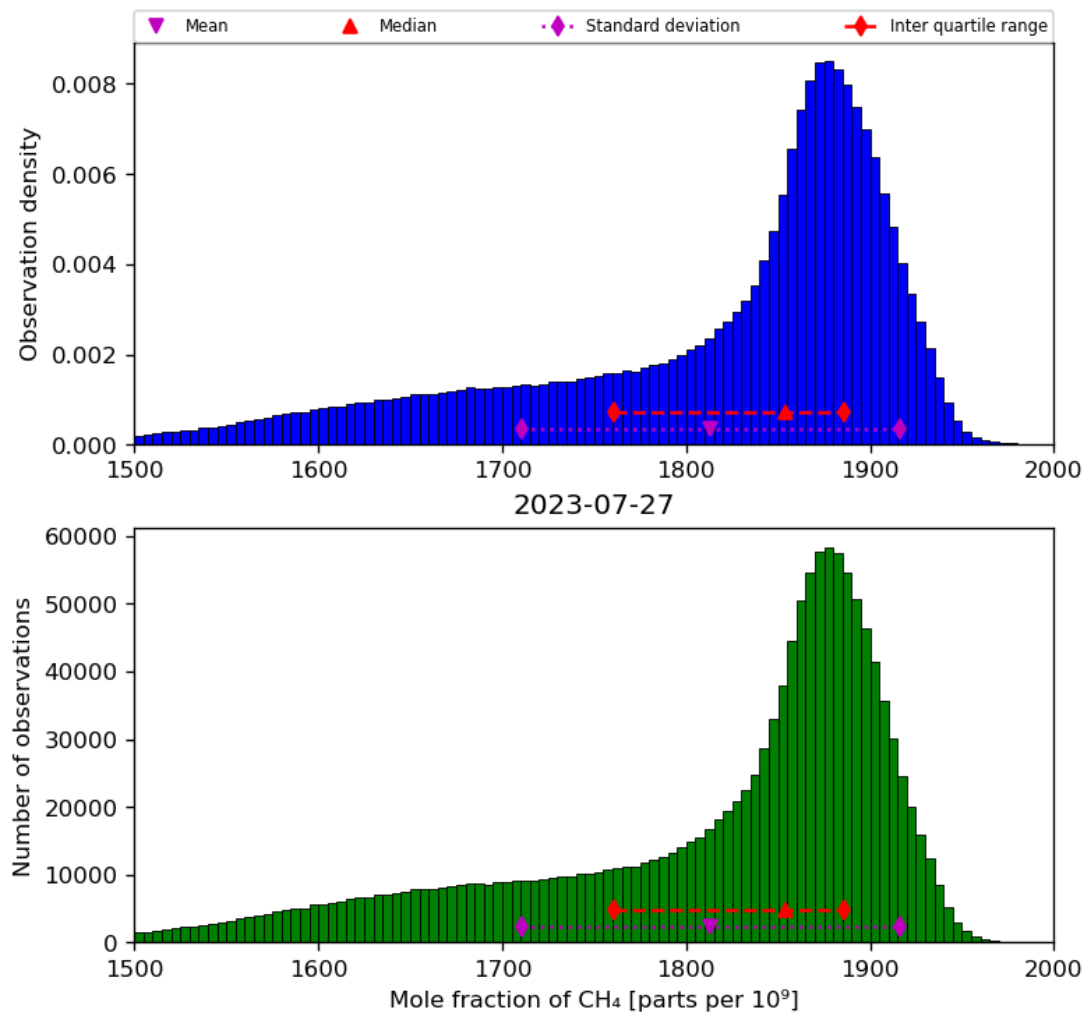
Figure 23: Histogram of “Mole fraction of CH 4 ” for 2023-07-26 to 2023-07-28
