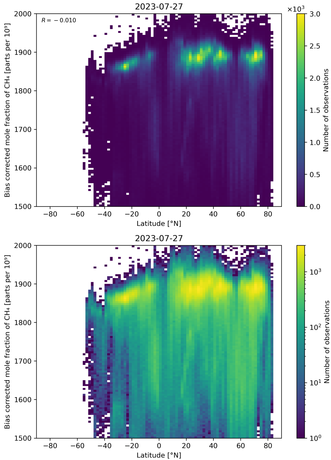
Figure 58: Scatter density plot of “Latitude” against “Bias corrected mole fraction of \text{CH}_4 ” for 2023-07-26 to 2023-07-28.
