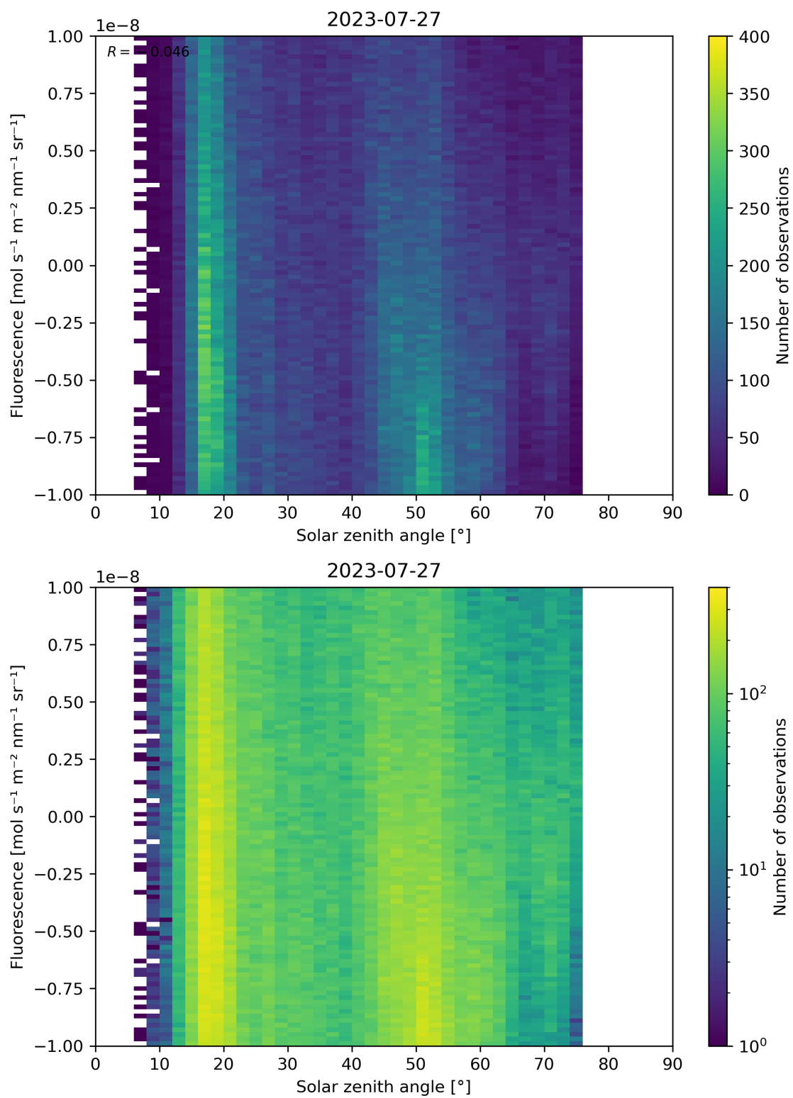
Figure 97: Scatter density plot of “Solar zenith angle” against “Fluorescence” for 2023-07-26 to 2023-07-28.
