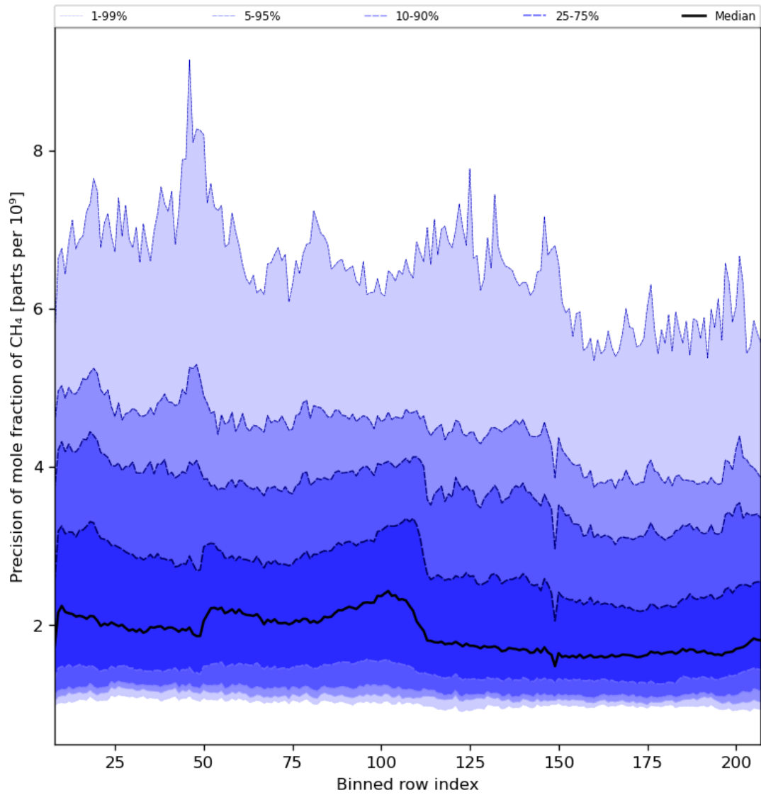
Figure 35: Along track statistics of “Precision of mole fraction of \text{CH}_4 ” for 2023-07-26 to 2023-07-28
