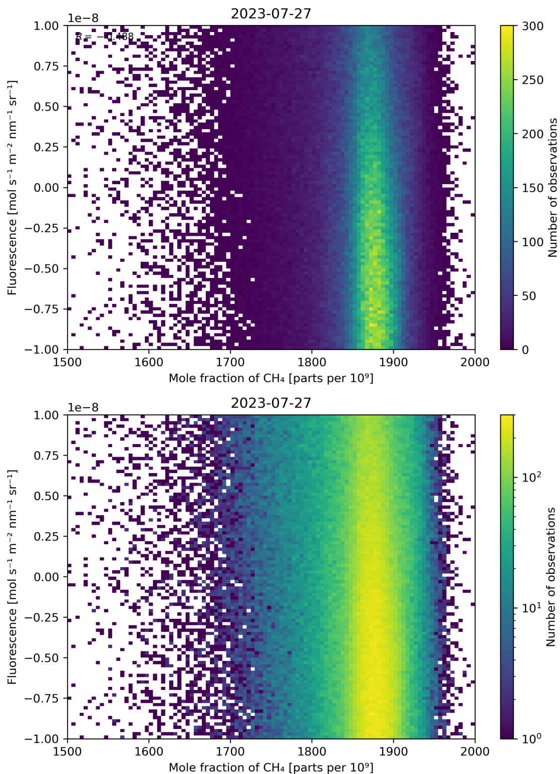
Figure 73: Scatter density plot of “Mole fraction of \text{CH}_4 ” against “Fluorescence” for 2023-07-26 to 2023-07-28.
