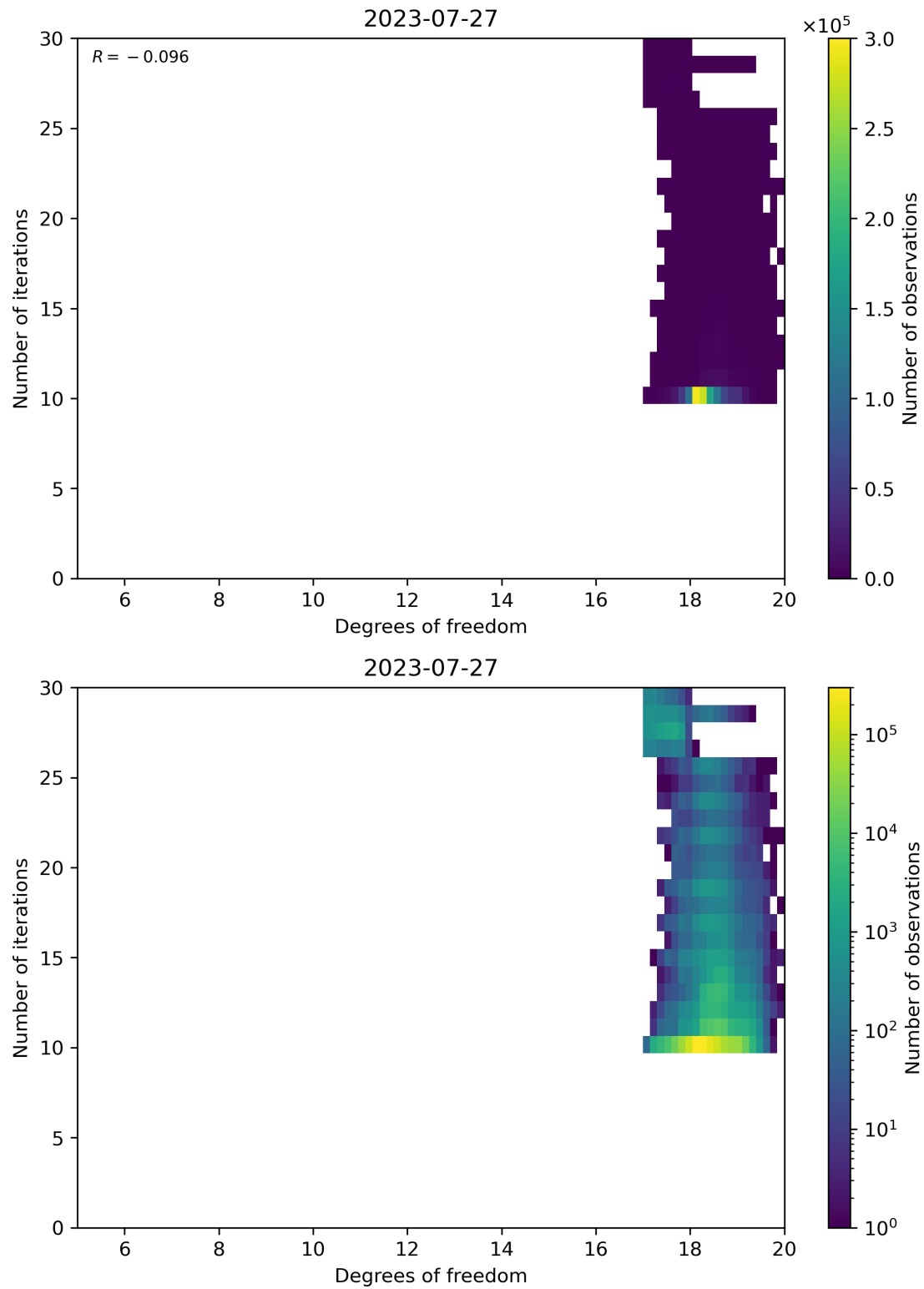
Figure 52: Scatter density plot of “Degrees of freedom” against “Number of iterations” for 2023-07-26 to 2023-07-28.
