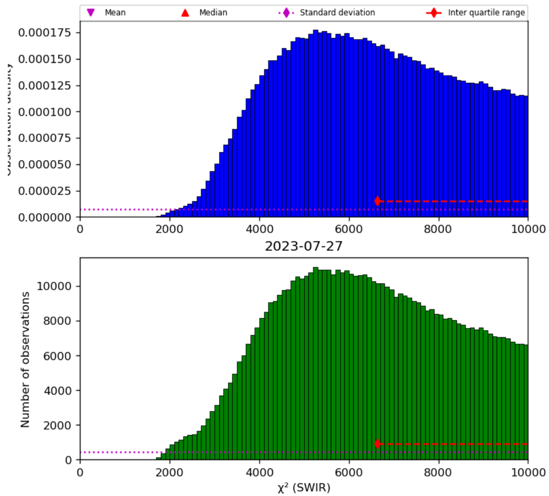
Figure 28: Histogram of “ \chi^2 (SWIR)” for 2023-07-26 to 2023-07-28
