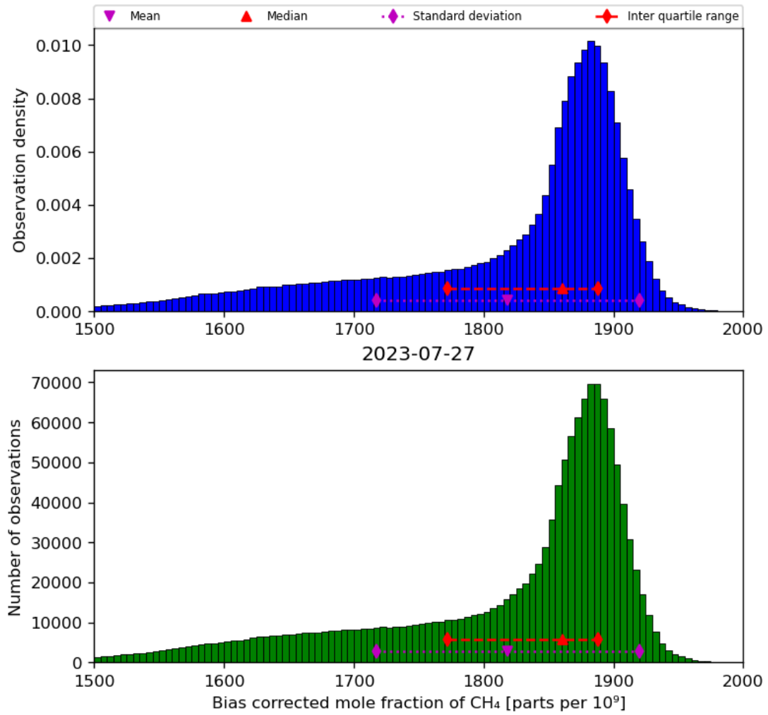
Figure 25: Histogram of “Bias corrected mole fraction of CH 4 ” for 2023-07-26 to 2023-07-28
