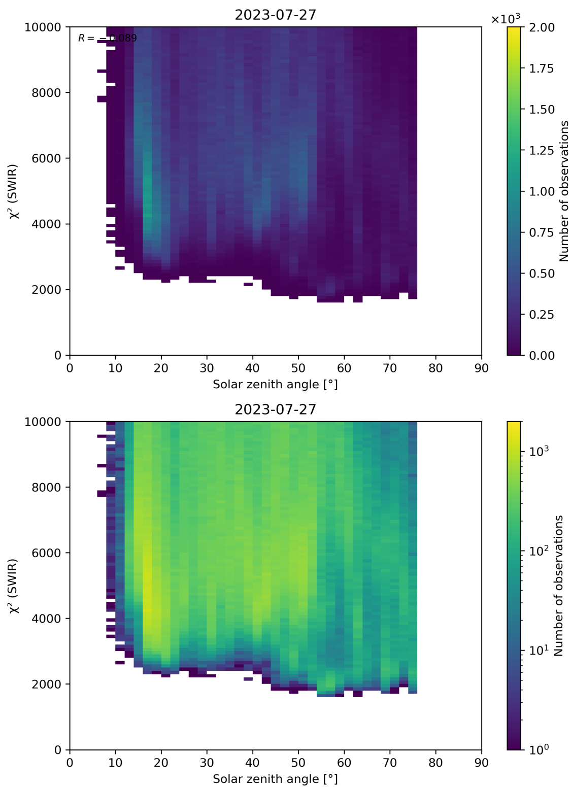
Figure 95: Scatter density plot of “Solar zenith angle” against “ \chi^2 (SWIR)” for 2023-07-26 to 2023-07-28.
