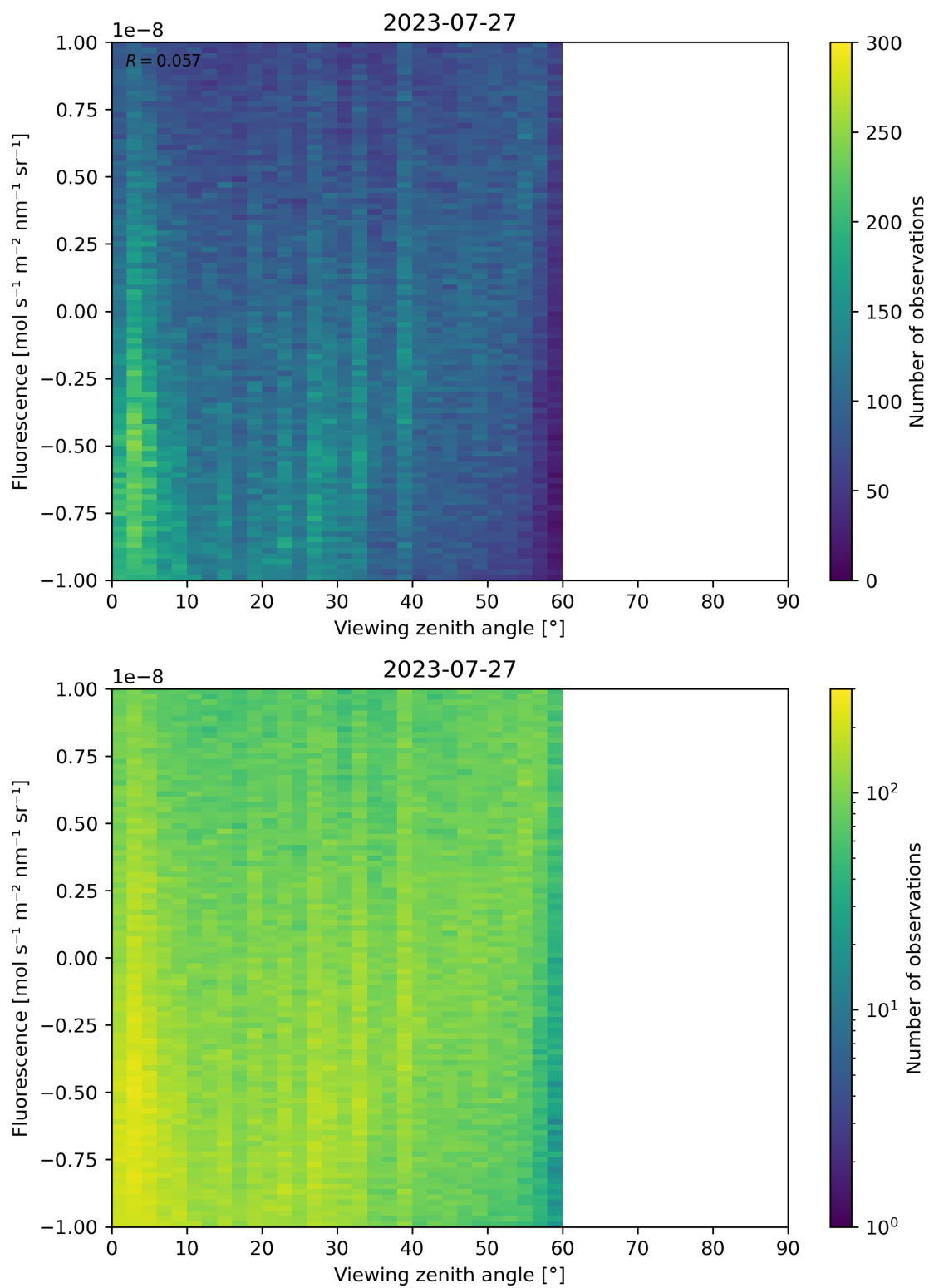
Figure 108: Scatter density plot of “Viewing zenith angle” against “Fluorescence” for 2023-07-26 to 2023-07-28.
