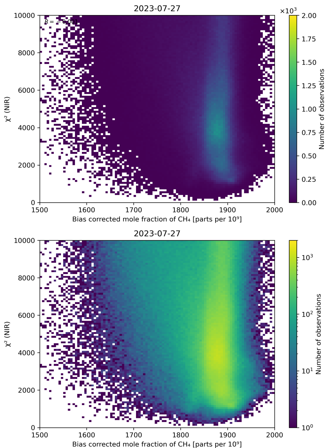
Figure 63: Scatter density plot of “Bias corrected mole fraction of \text{CH}_4 ” against “ \chi^2 (NIR)” for 2023-07-26 to 2023-07-28.
