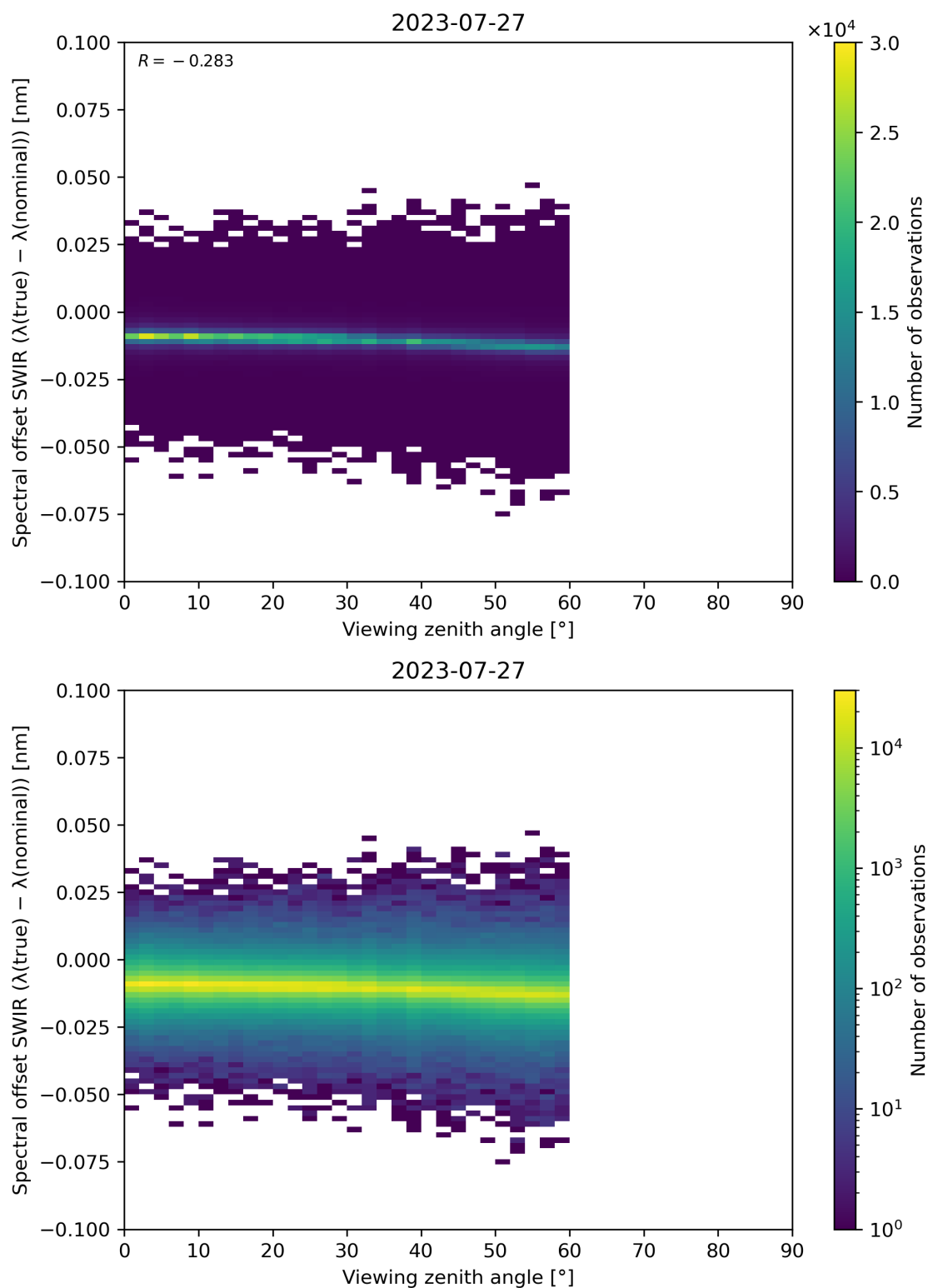
Figure 116: Scatter density plot of “Viewing zenith angle” against “Spectral offset SWIR ( \lambda(\text{true}) - \lambda(\text{nominal}) )” for 2023-07-26 to 2023-07-28.
