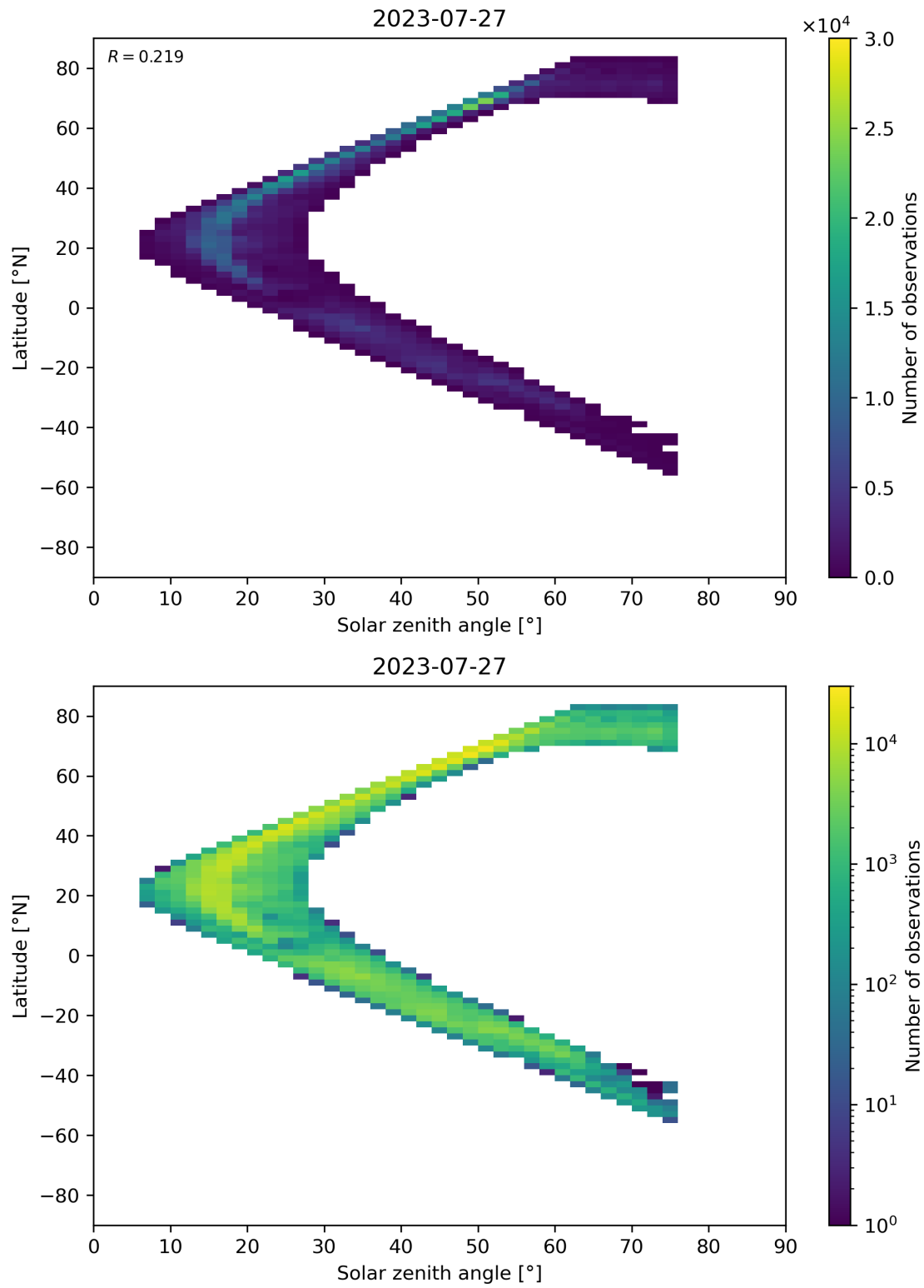
Figure 98: Scatter density plot of “Solar zenith angle” against “Latitude” for 2023-07-26 to 2023-07-28.
