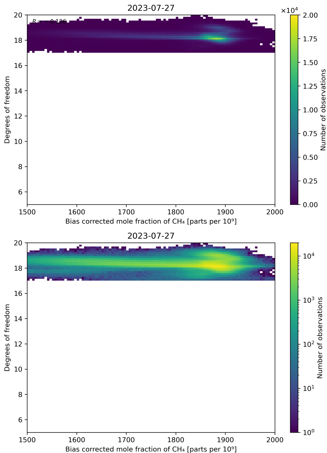
Figure 65: Scatter density plot of “Bias corrected mole fraction of CH 4 ” against “Degrees of freedom” for 2023-07-26 to 2023-07-28.
