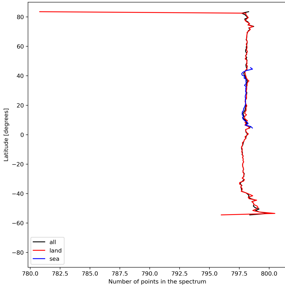
Figure 15: Zonal average of “Number of points in the spectrum” for 2023-07-26 to 2023-07-28.
