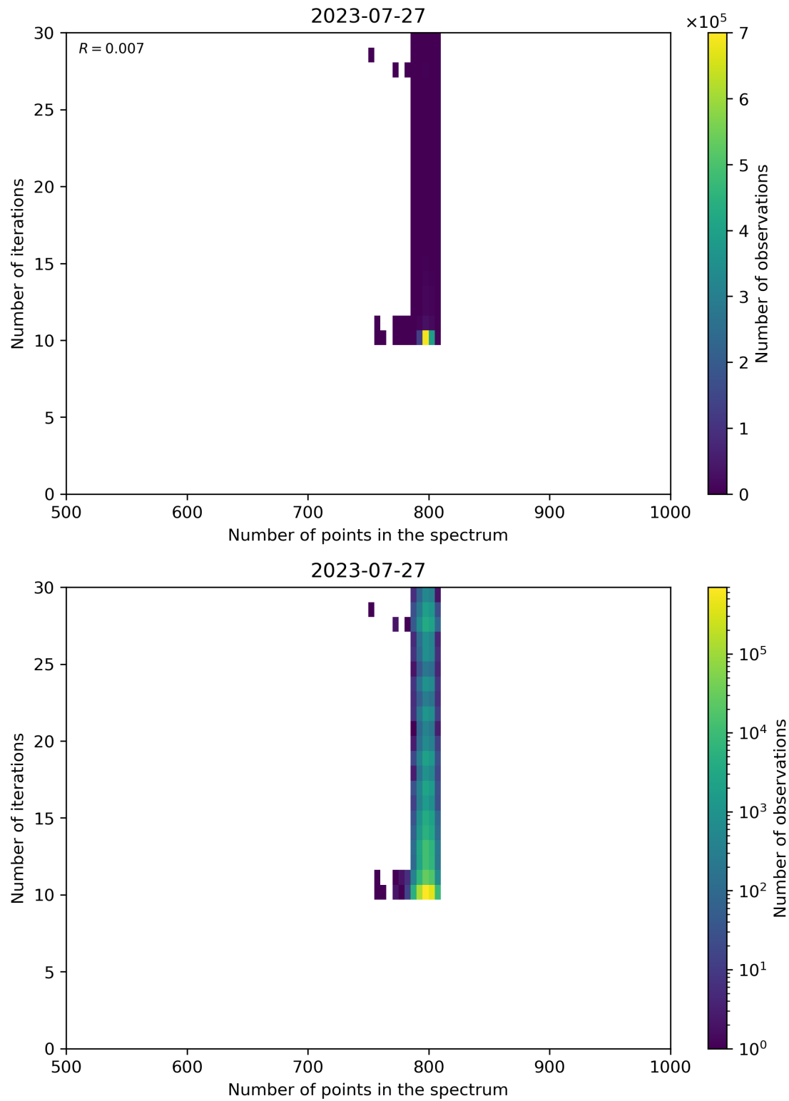
Figure 92: Scatter density plot of “Number of points in the spectrum” against “Number of iterations” for 2023-07-26 to 2023-07-28.
