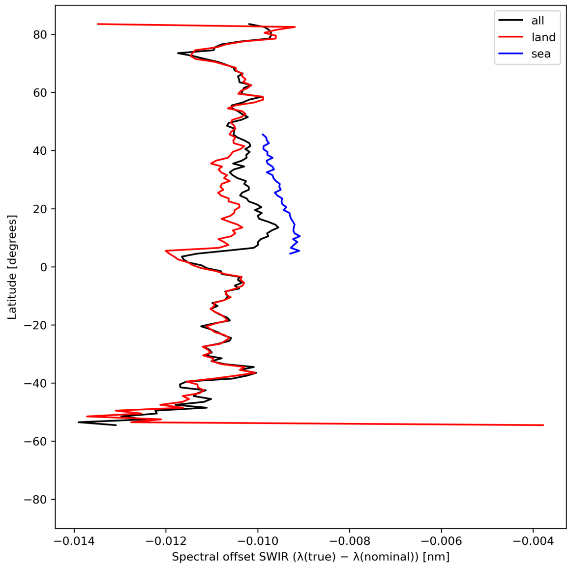
Figure 16: Zonal average of “Spectral offset SWIR ( \lambda(\text{true}) - \lambda(\text{nominal}) )” for 2023-07-26 to 2023-07-28.
