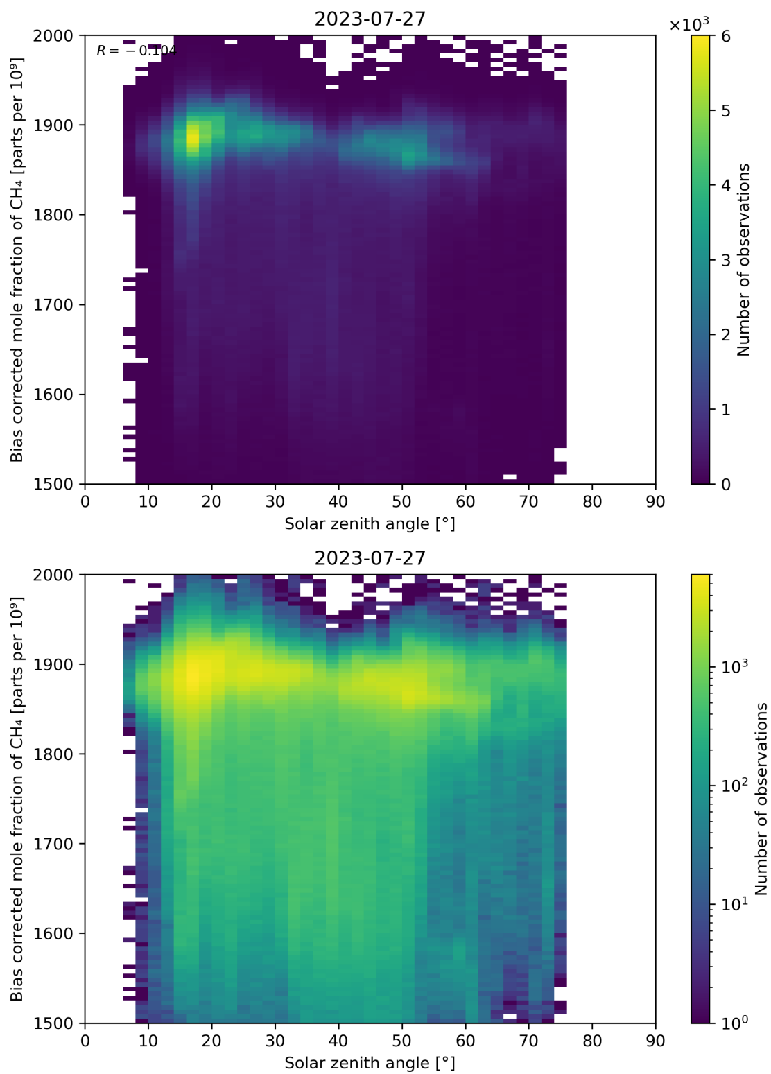
Figure 100: Scatter density plot of “Solar zenith angle” against “Bias corrected mole fraction of \text{CH}_4 ” for 2023-07-26 to 2023-07-28.
