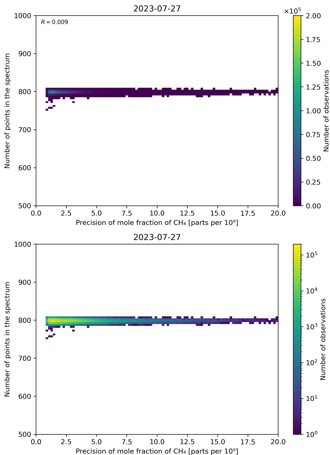
Figure 84: Scatter density plot of “Precision of mole fraction of CH 4 ” against “Number of points in the spectrum” for 2023-07-26 to 2023-07-28.
