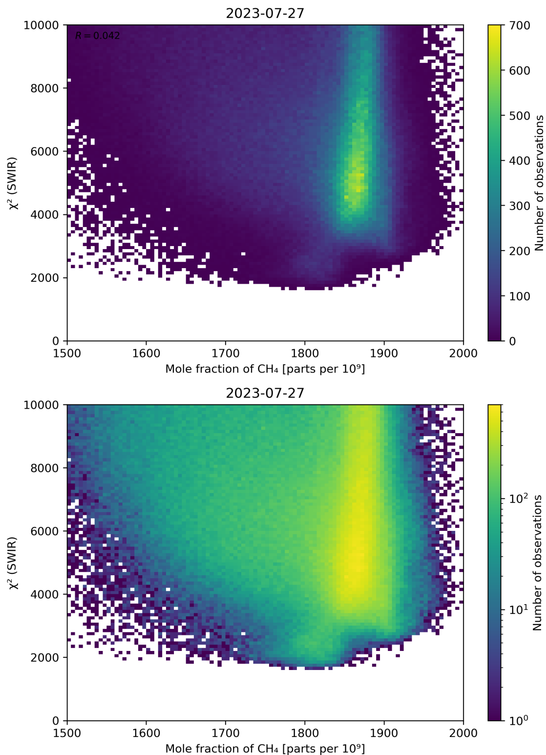
Figure 71: Scatter density plot of “Mole fraction of \text{CH}_4 ” against “ \chi^2 (SWIR)” for 2023-07-26 to 2023-07-28.
