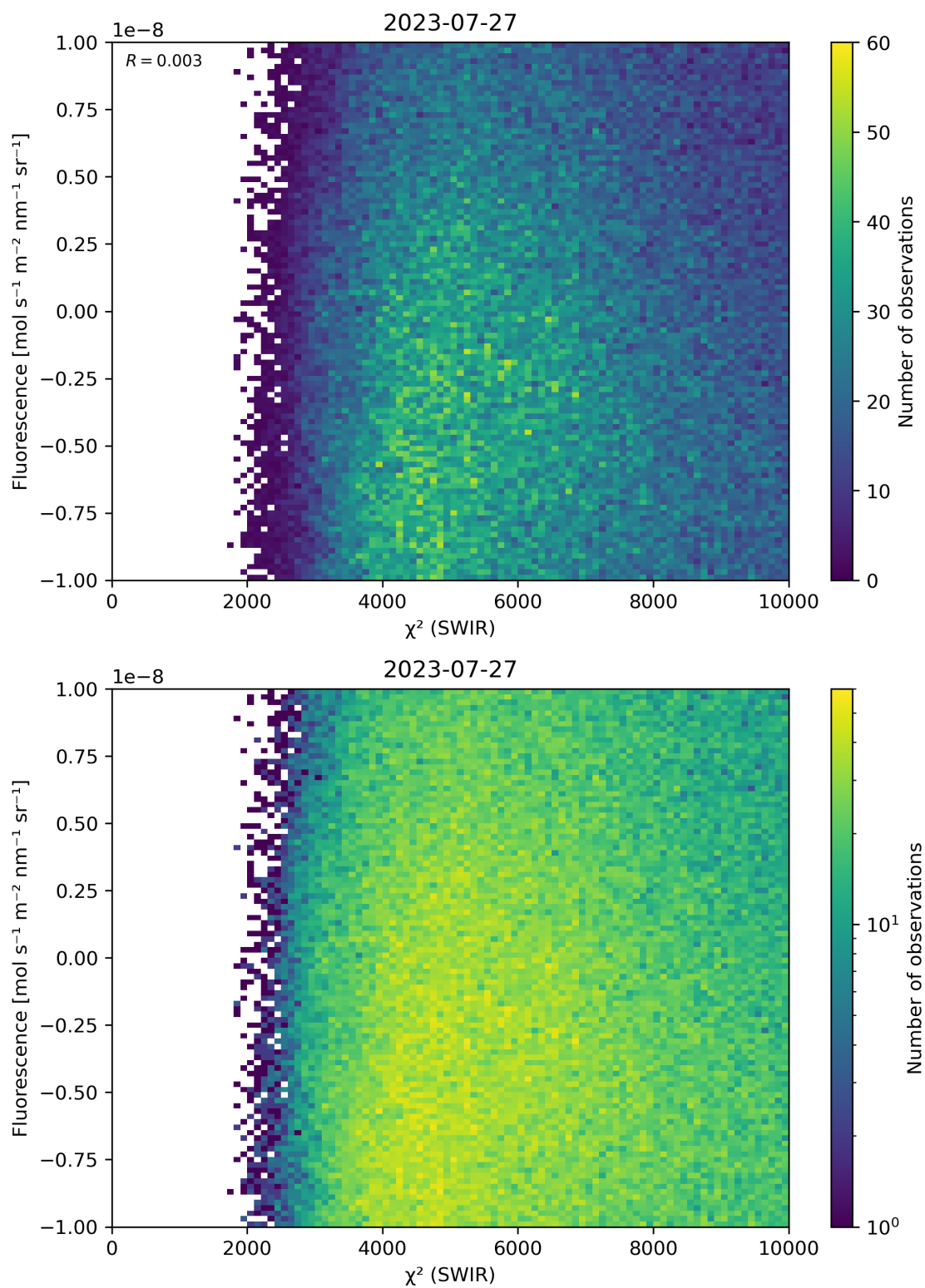
Figure 49: Scatter density plot of “ \chi^2 (SWIR)” against “Fluorescence” for 2023-07-26 to 2023-07-28.
