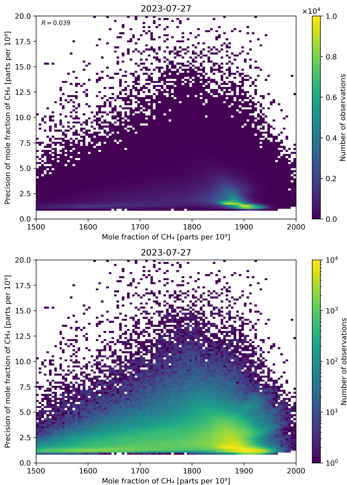
Figure 75: Scatter density plot of “Mole fraction of CH 4 ” against “Precision of mole fraction of CH 4 ” for 2023-07-26 to 2023-07-28.
