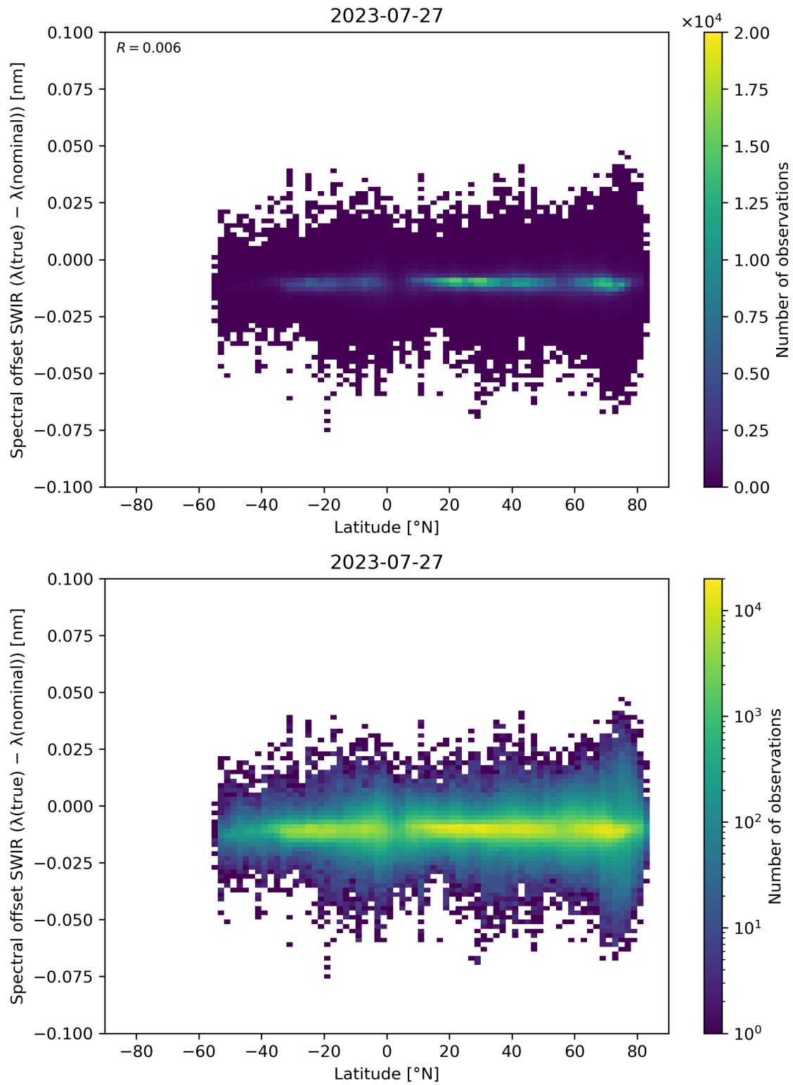
Figure 62: Scatter density plot of “Latitude” against “Spectral offset SWIR ( \lambda(\text{true}) - \lambda(\text{nominal}) )” for 2023-07-26 to 2023-07-28.
