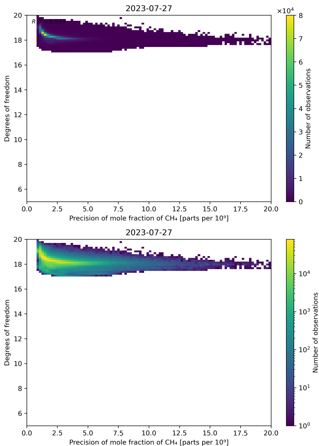
Figure 80: Scatter density plot of “Precision of mole fraction of CH 4 ” against “Degrees of freedom” for 2023-07-26 to 2023-07-28.
