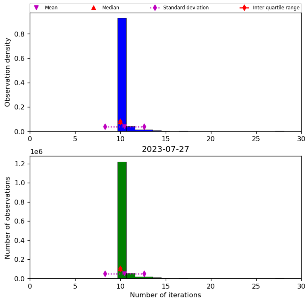
Figure 31: Histogram of “Number of iterations” for 2023-07-26 to 2023-07-28
