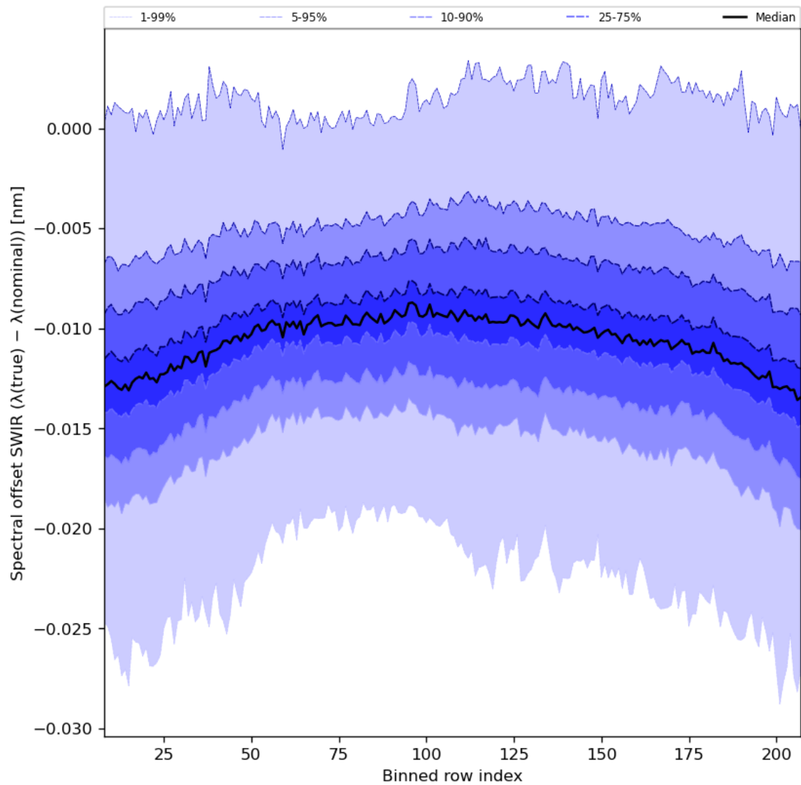
Figure 38: Along track statistics of “Spectral offset SWIR ( \lambda(\text{true}) - \lambda(\text{nominal}) )” for 2023-07-26 to 2023-07-28
