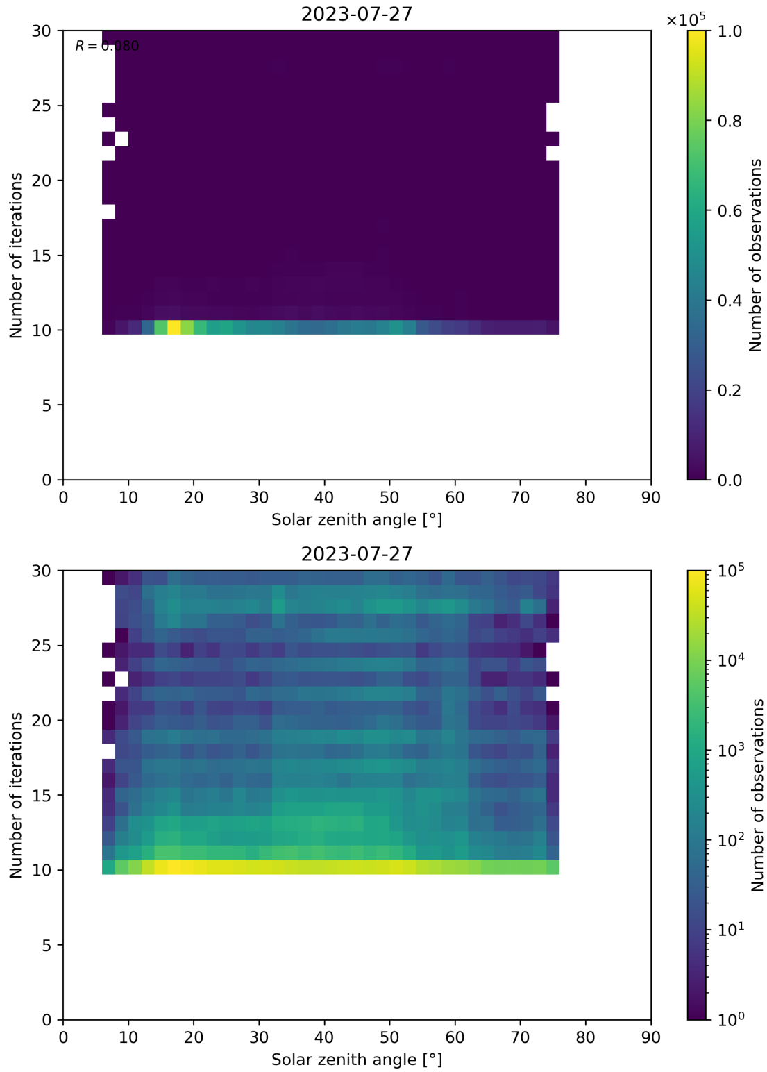
Figure 102: Scatter density plot of “Solar zenith angle” against “Number of iterations” for 2023-07-26 to 2023-07-28.
