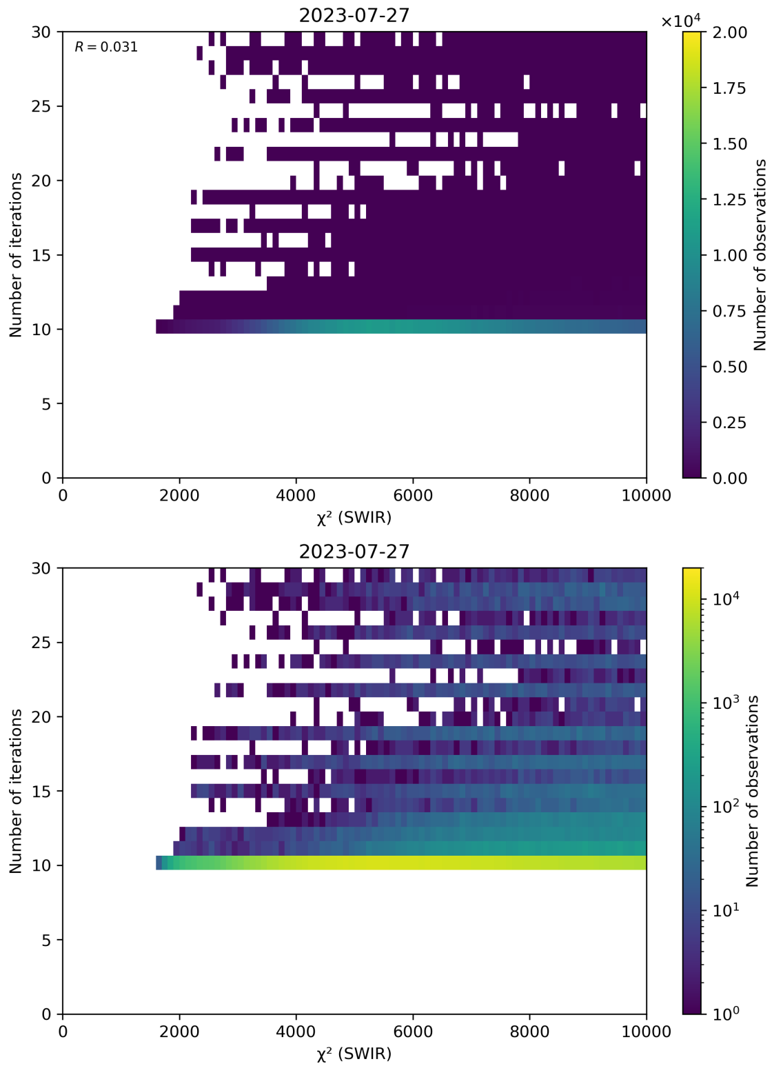
Figure 50: Scatter density plot of “ \chi^2 (SWIR)” against “Number of iterations” for 2023-07-26 to 2023-07-28.
