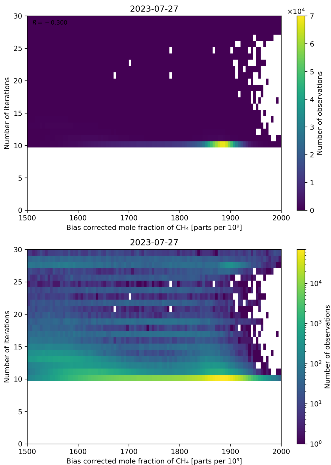
Figure 67: Scatter density plot of “Bias corrected mole fraction of CH 4 ” against “Number of iterations” for 2023-07-26 to 2023-07-28.
