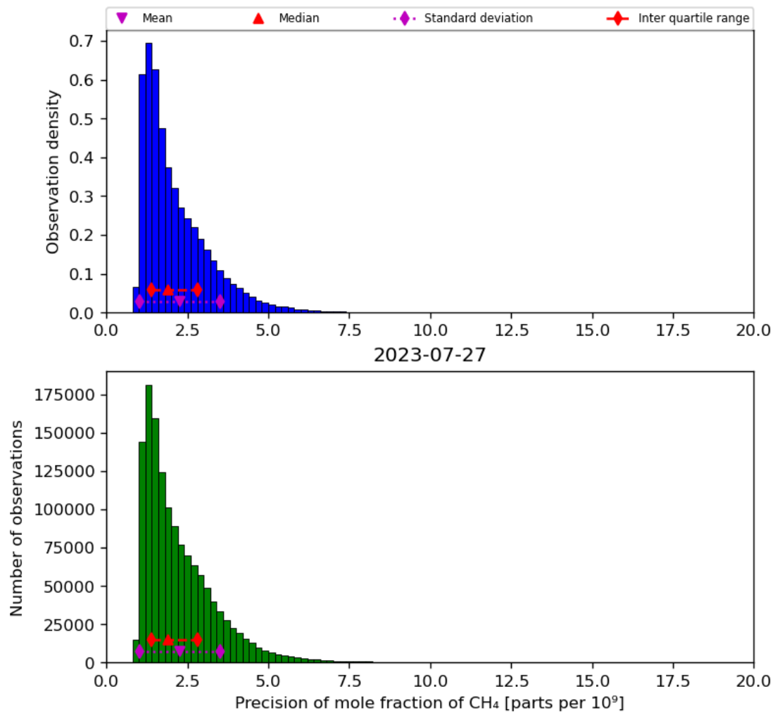
Figure 24: Histogram of “Precision of mole fraction of CH 4 ” for 2023-07-26 to 2023-07-28
