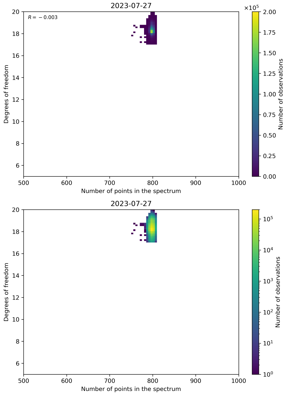
Figure 90: Scatter density plot of “Number of points in the spectrum” against “Degrees of freedom” for 2023-07-26 to 2023-07-28.
