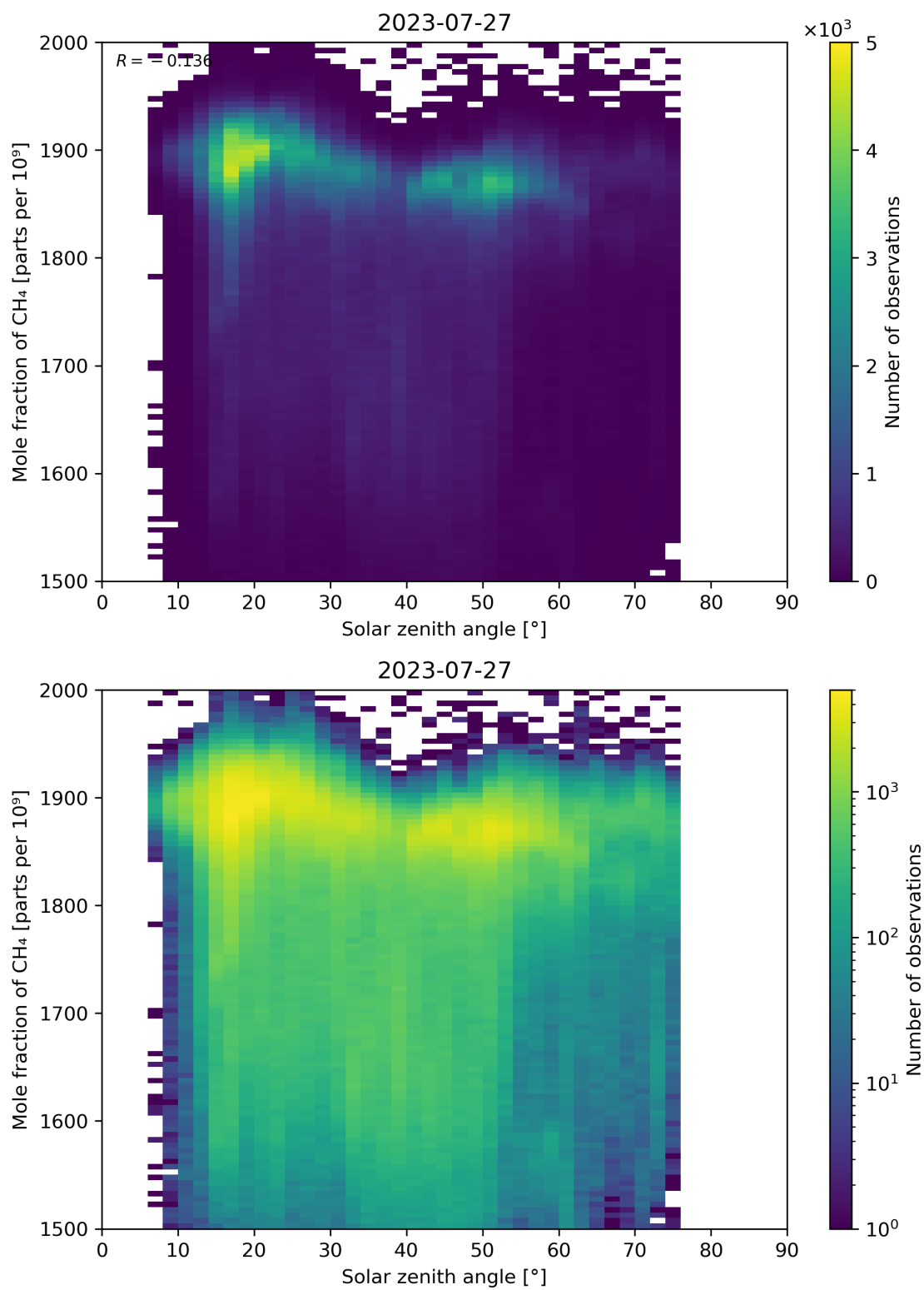
Figure 99: Scatter density plot of “Solar zenith angle” against “Mole fraction of CH 4 ” for 2023-07-26 to 2023-07-28.
