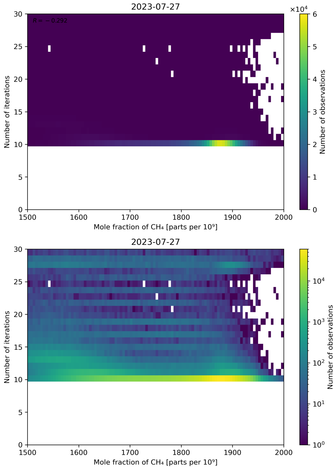
Figure 76: Scatter density plot of “Mole fraction of CH 4 ” against “Number of iterations” for 2023-07-26 to 2023-07-28.
