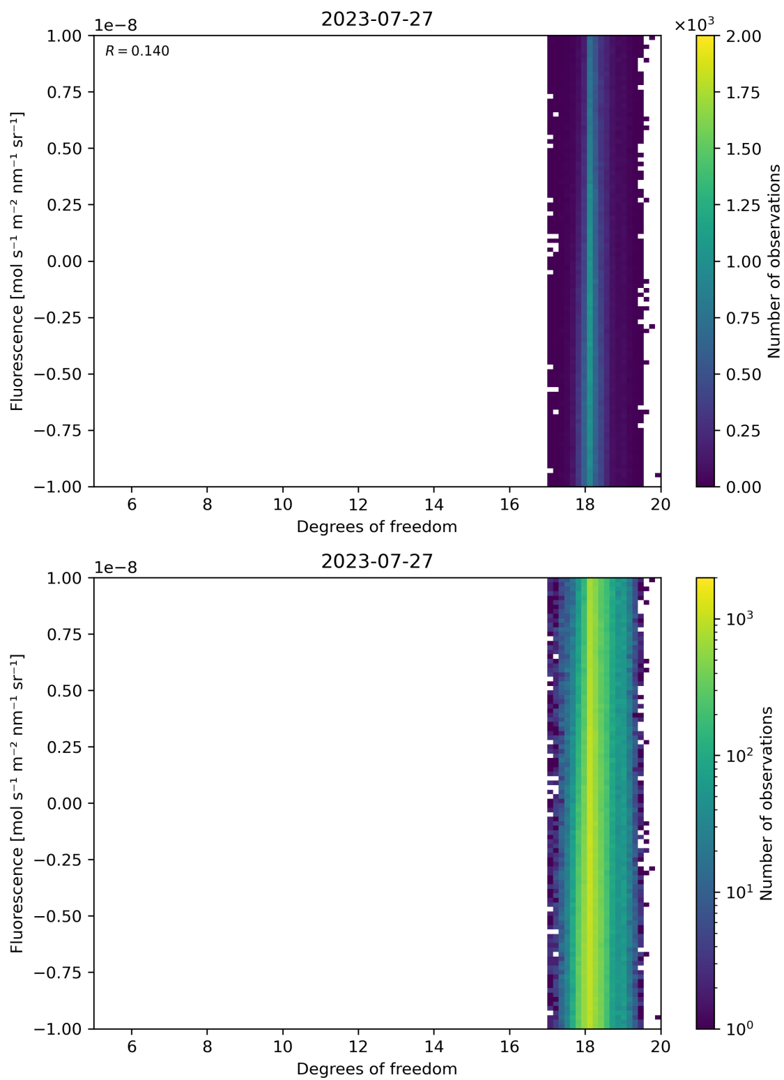
Figure 51: Scatter density plot of “Degrees of freedom” against “Fluorescence” for 2023-07-26 to 2023-07-28.
