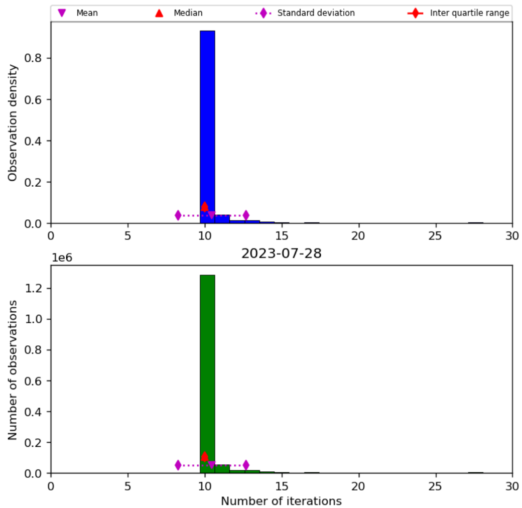
Figure 31: Histogram of “Number of iterations” for 2023-07-27 to 2023-07-29
