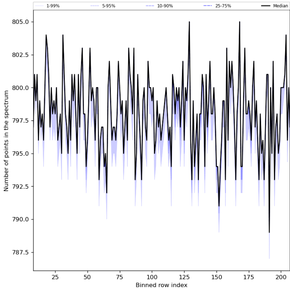
Figure 37: Along track statistics of “Number of points in the spectrum” for 2023-07-27 to 2023-07-29
