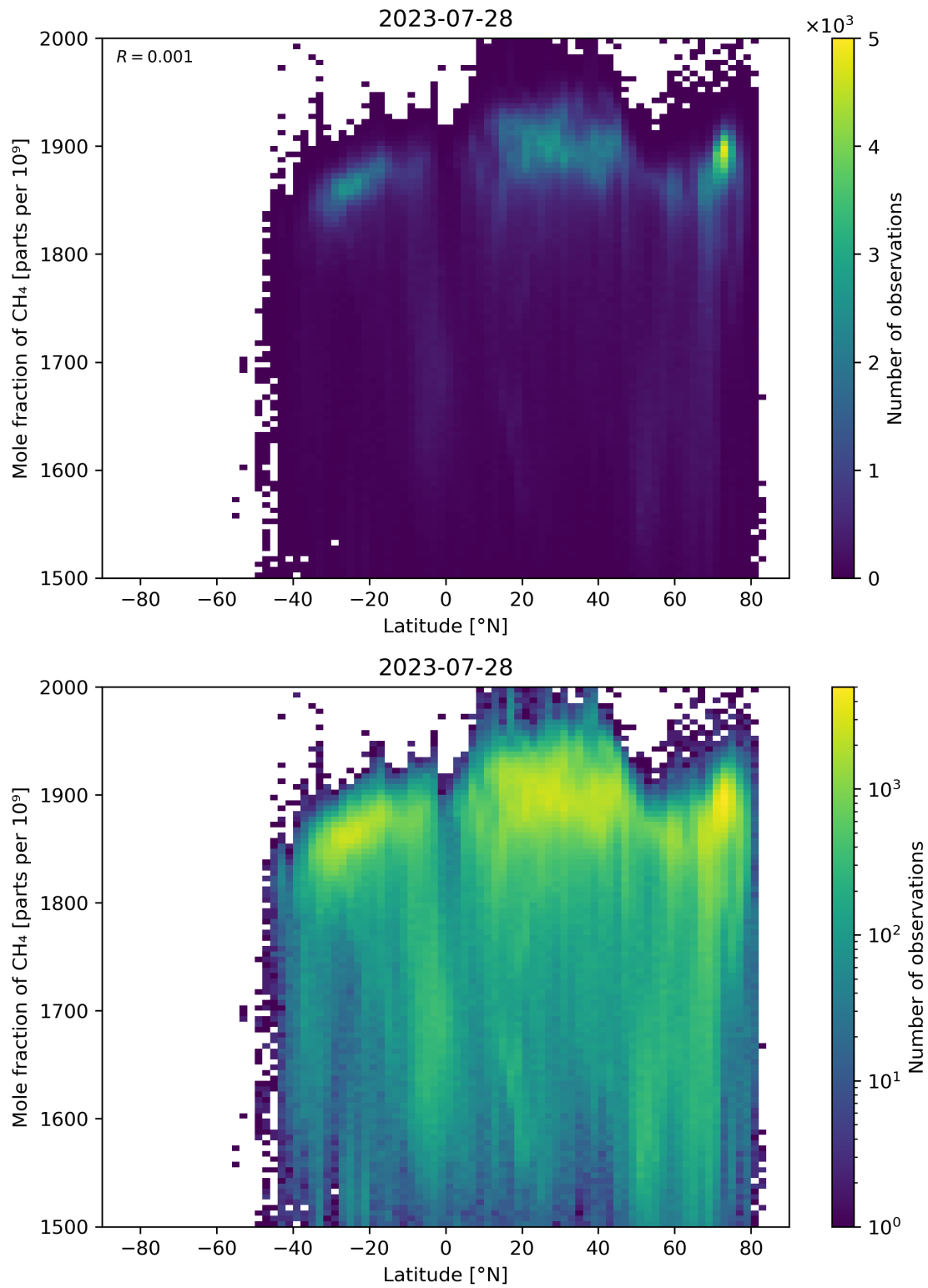
Figure 57: Scatter density plot of “Latitude” against “Mole fraction of CH 4 ” for 2023-07-27 to 2023-07-29.
