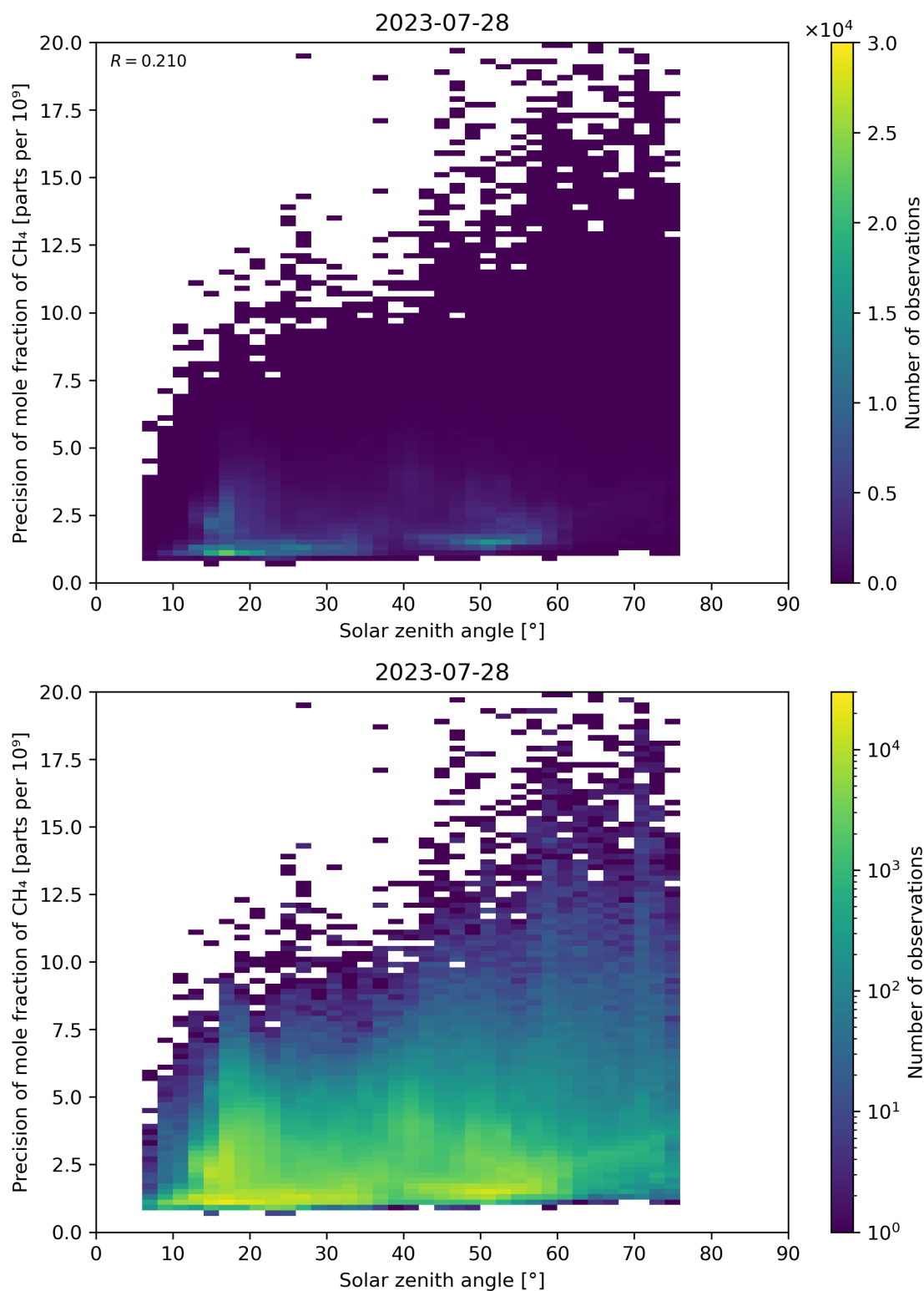
Figure 101: Scatter density plot of “Solar zenith angle” against “Precision of mole fraction of \text{CH}_4 ” for 2023-07-27 to 2023-07-29.
