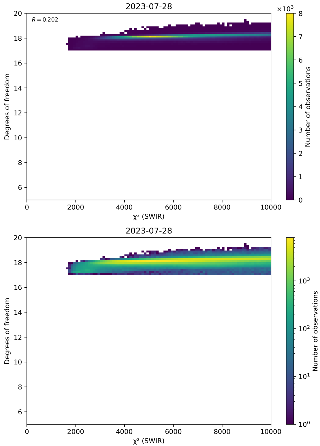
Figure 48: Scatter density plot of “ \chi^2 (SWIR)” against “Degrees of freedom” for 2023-07-27 to 2023-07-29.
