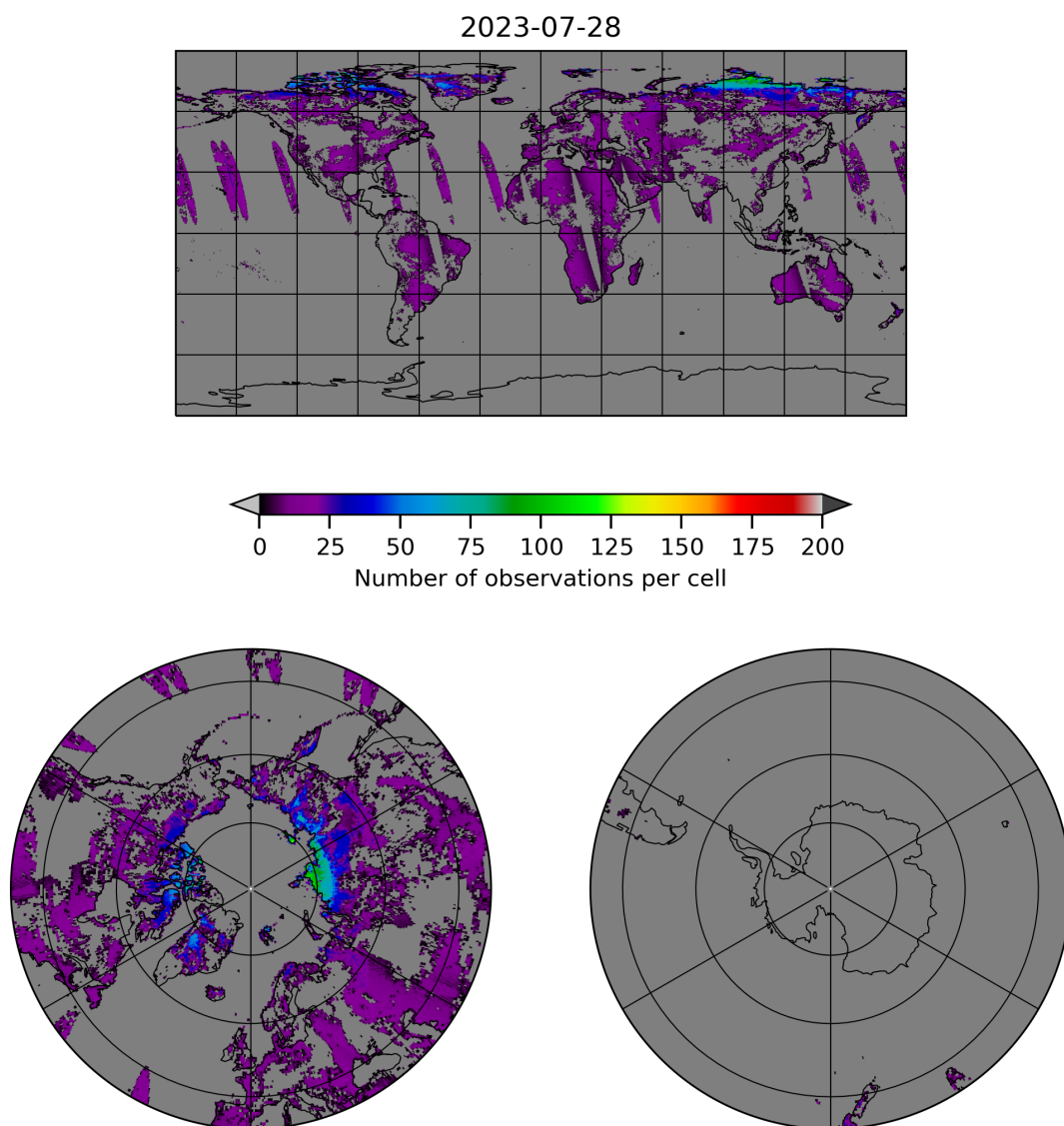
Figure 10: Map of the number of observations for 2023-07-27 to 2023-07-29
