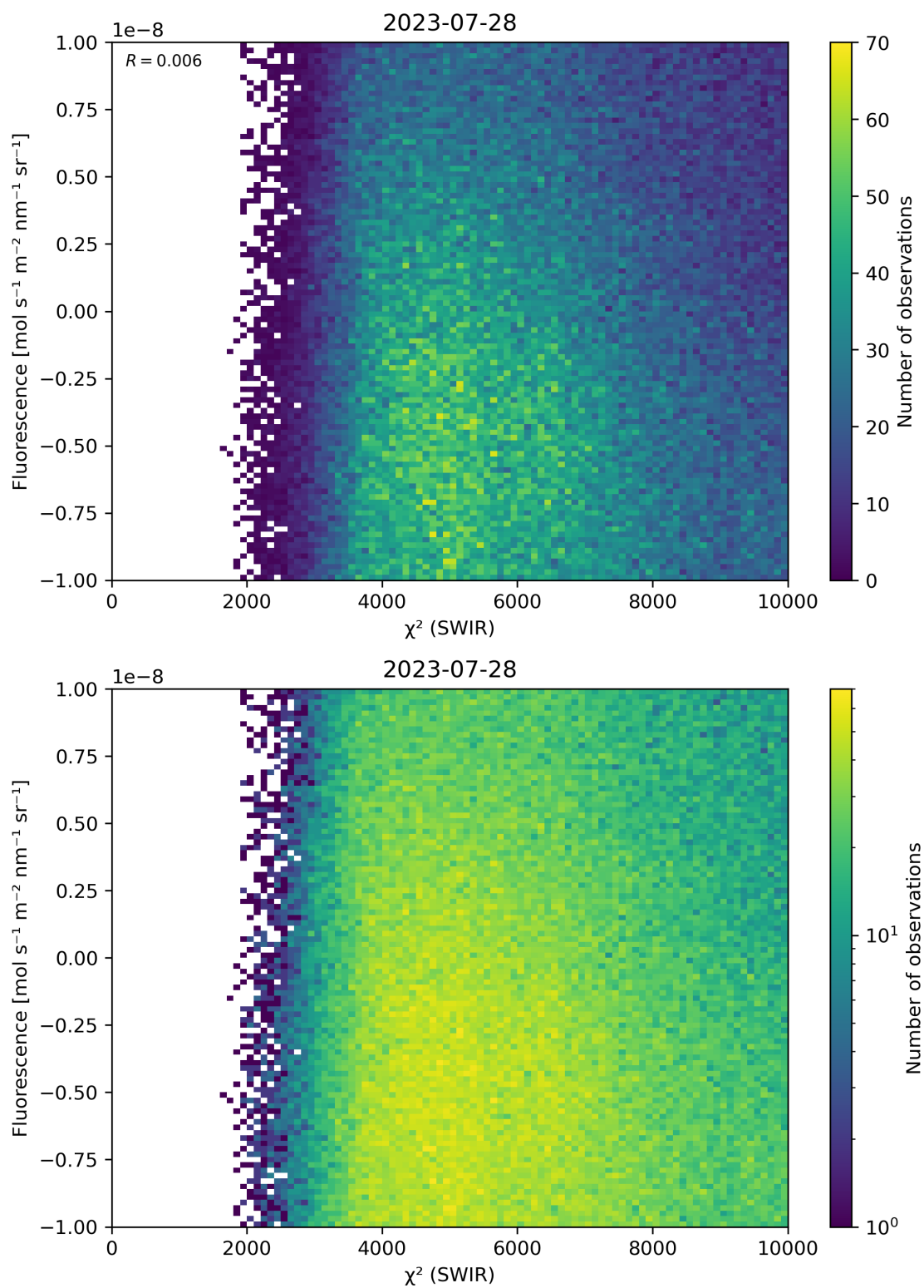
Figure 49: Scatter density plot of “ \chi^2 (SWIR)” against “Fluorescence” for 2023-07-27 to 2023-07-29.
