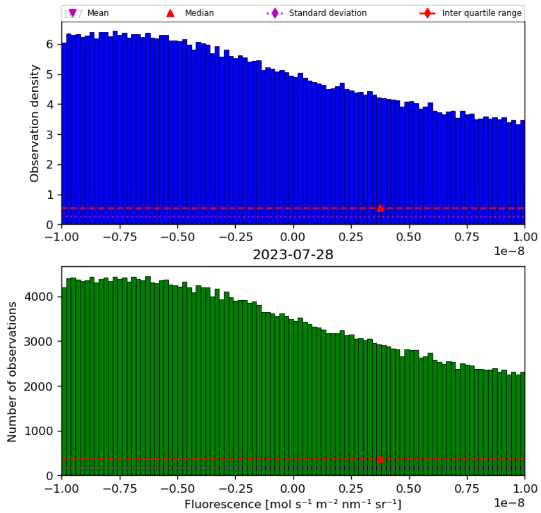
Figure 32: Histogram of “Fluorescence” for 2023-07-27 to 2023-07-29
