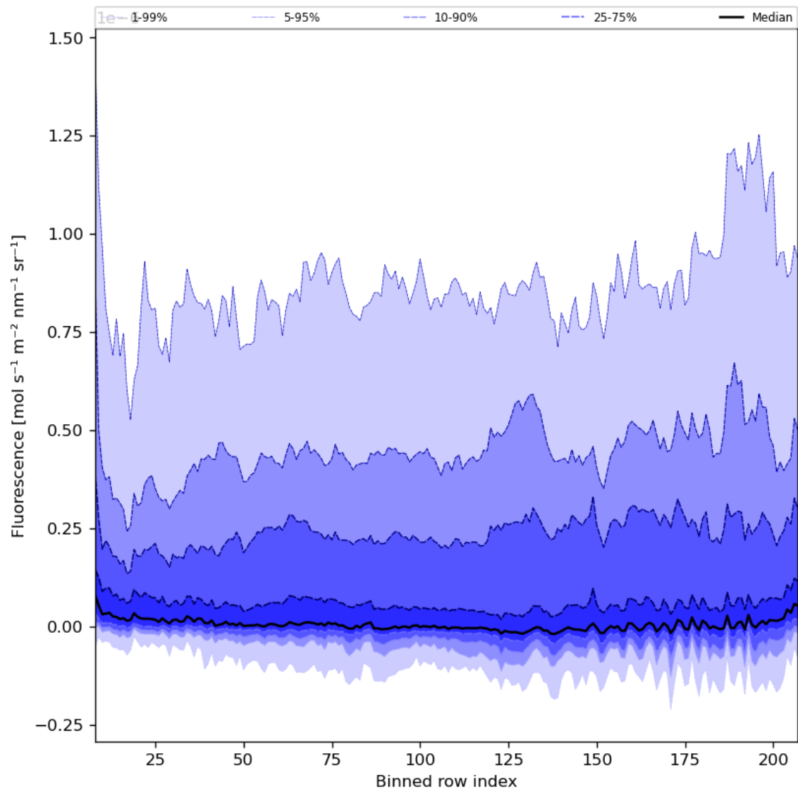
Figure 43: Along track statistics of “Fluorescence” for 2023-07-27 to 2023-07-29
