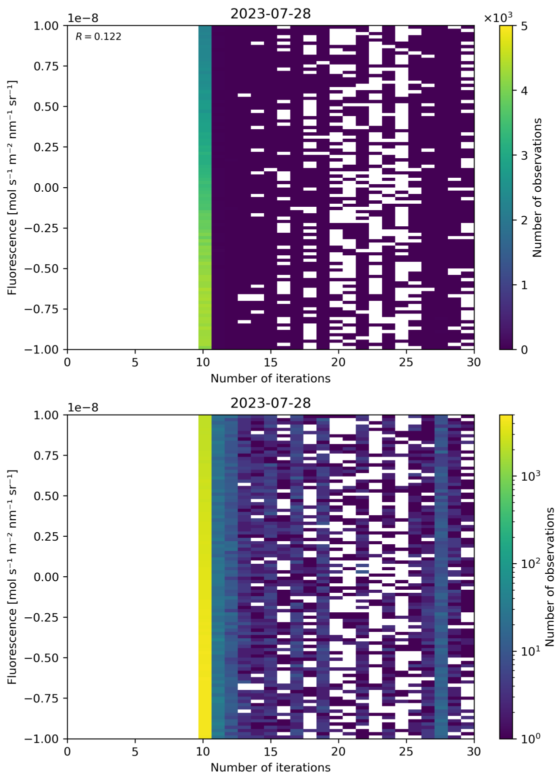
Figure 87: Scatter density plot of “Number of iterations” against “Fluorescence” for 2023-07-27 to 2023-07-29.
