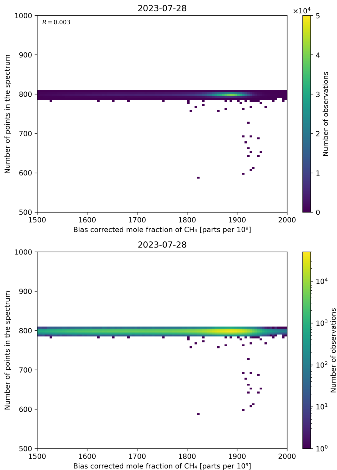
Figure 68: Scatter density plot of “Bias corrected mole fraction of CH 4 ” against “Number of points in the spectrum” for 2023-07-27 to 2023-07-29.
