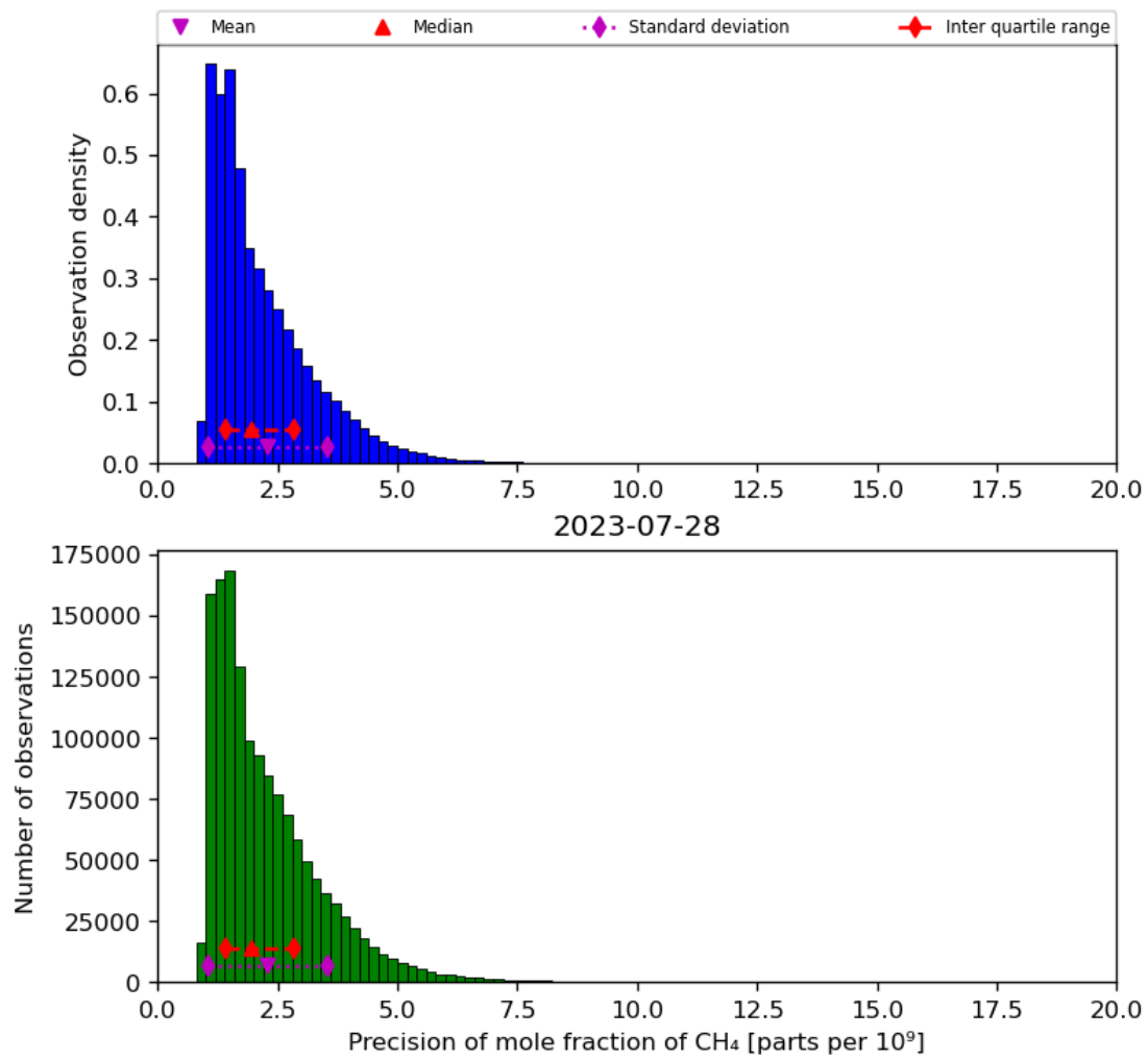
Figure 24: Histogram of “Precision of mole fraction of CH 4 ” for 2023-07-27 to 2023-07-29
