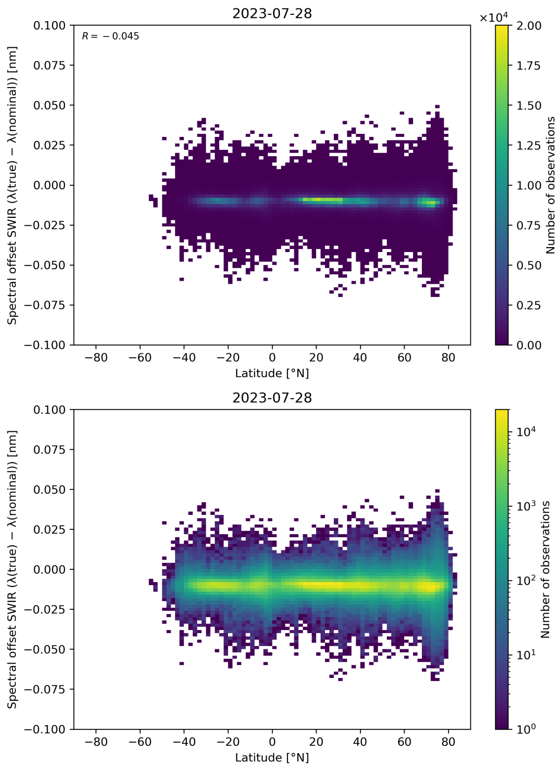
Figure 62: Scatter density plot of “Latitude” against “Spectral offset SWIR ( \lambda(\text{true}) - \lambda(\text{nominal}) )” for 2023-07-27 to 2023-07-29.
