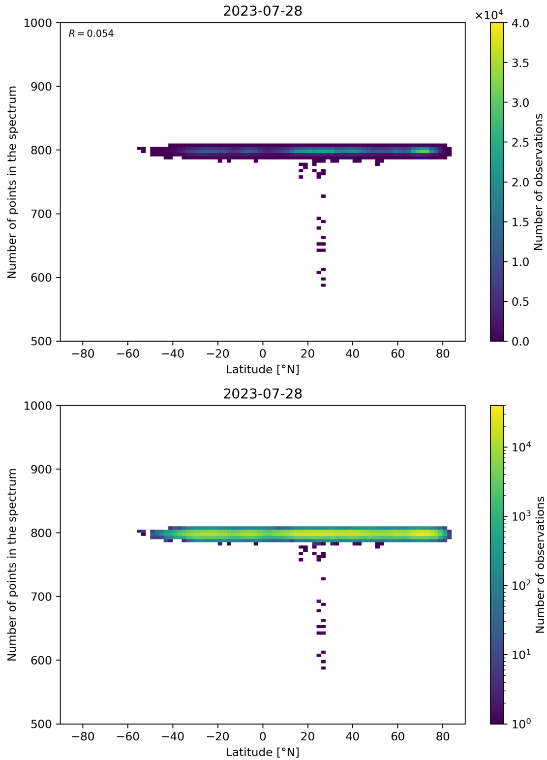
Figure 61: Scatter density plot of “Latitude” against “Number of points in the spectrum” for 2023-07-27 to 2023-07-29.
