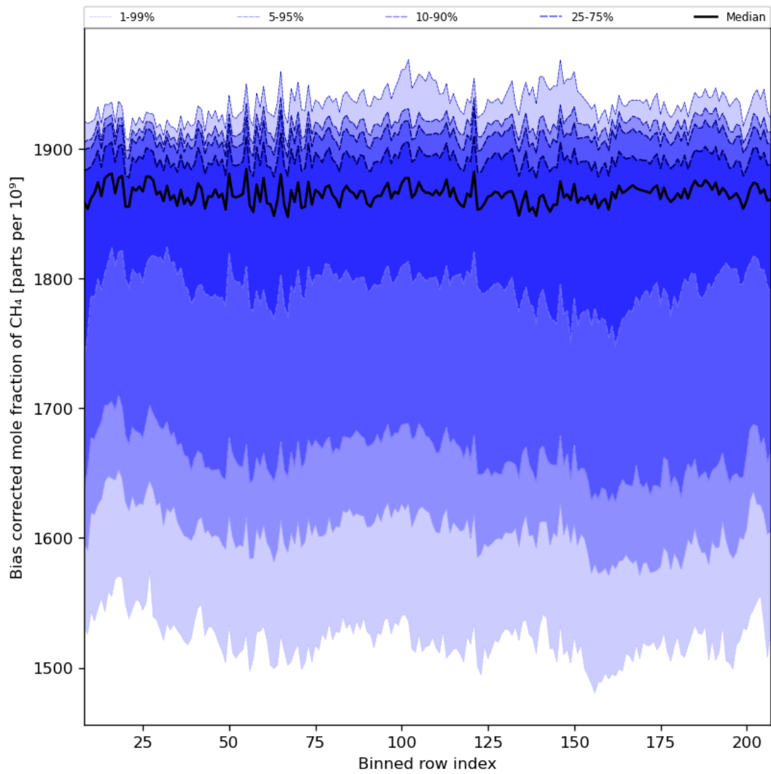
Figure 36: Along track statistics of “Bias corrected mole fraction of CH 4 ” for 2023-07-27 to 2023-07-29
