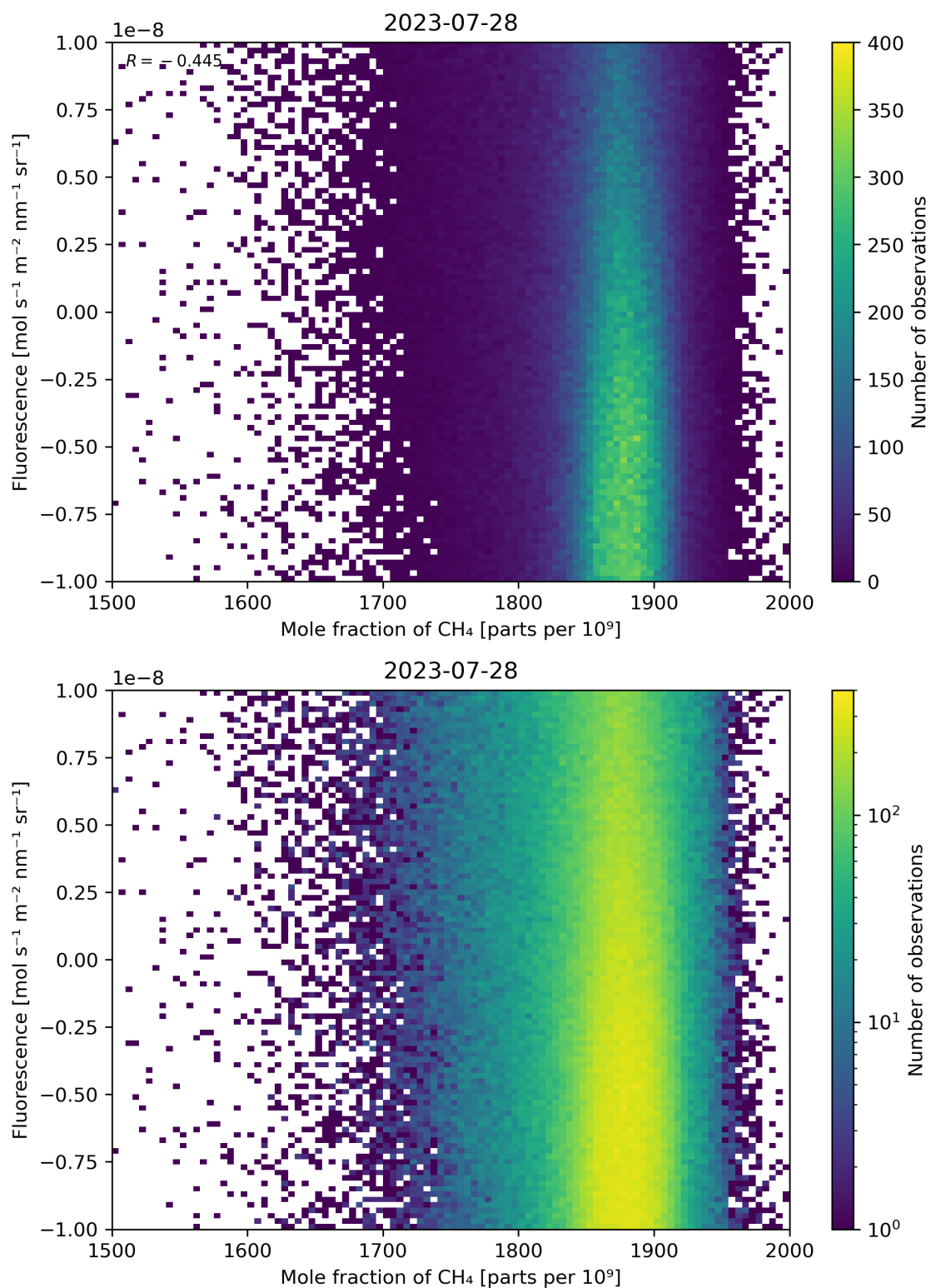
Figure 73: Scatter density plot of “Mole fraction of \text{CH}_4 ” against “Fluorescence” for 2023-07-27 to 2023-07-29.
