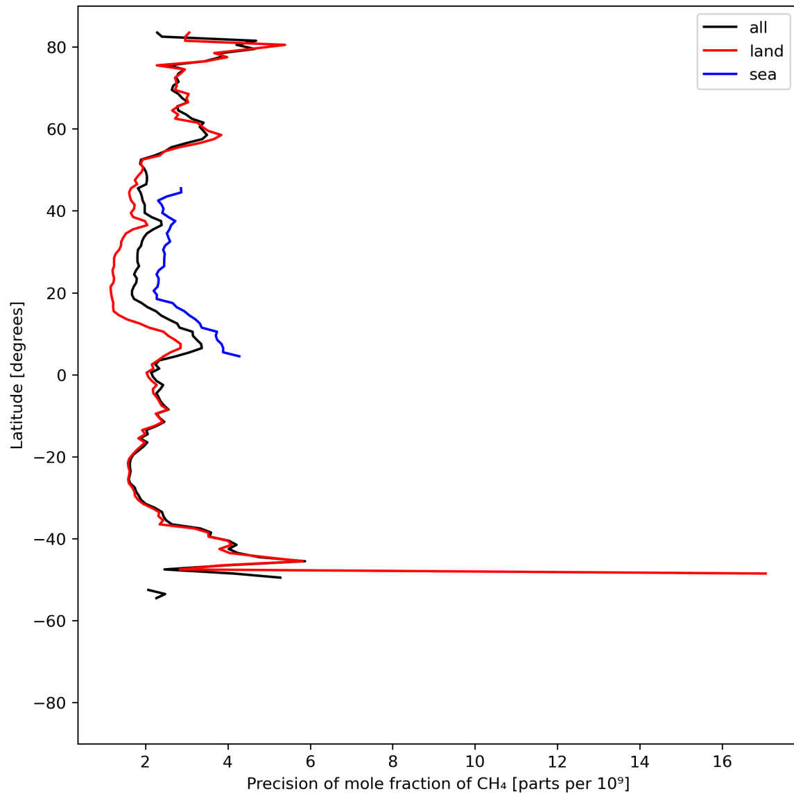
Figure 13: Zonal average of “Precision of mole fraction of \text{CH}_4 ” for 2023-07-27 to 2023-07-29.
