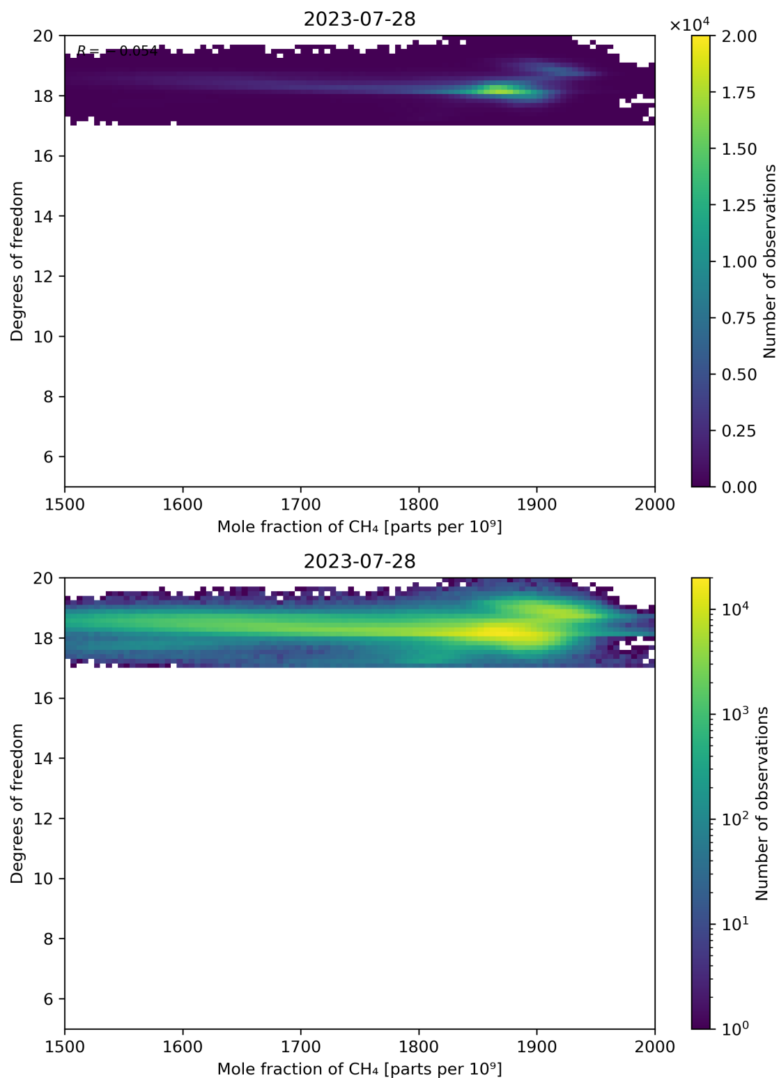
Figure 72: Scatter density plot of “Mole fraction of CH 4 ” against “Degrees of freedom” for 2023-07-27 to 2023-07-29.
