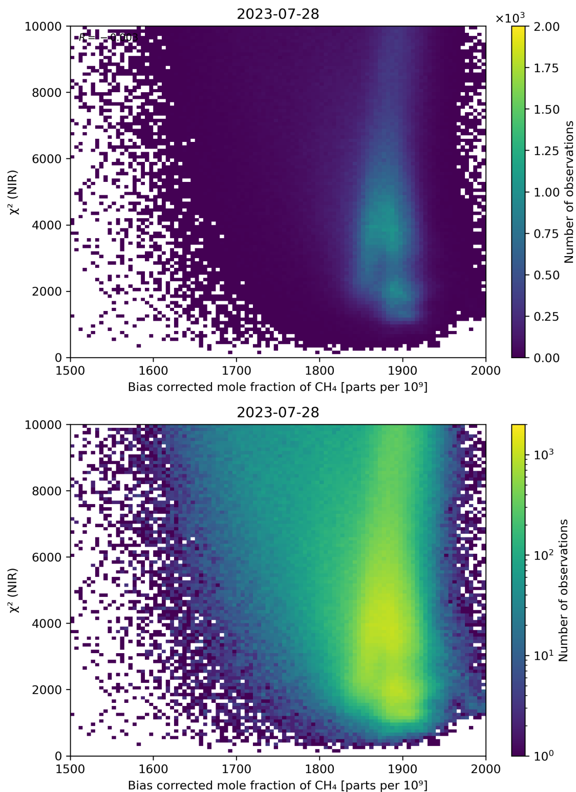
Figure 63: Scatter density plot of “Bias corrected mole fraction of CH 4 ” against “ \chi^2 (NIR)” for 2023-07-27 to 2023-07-29.
