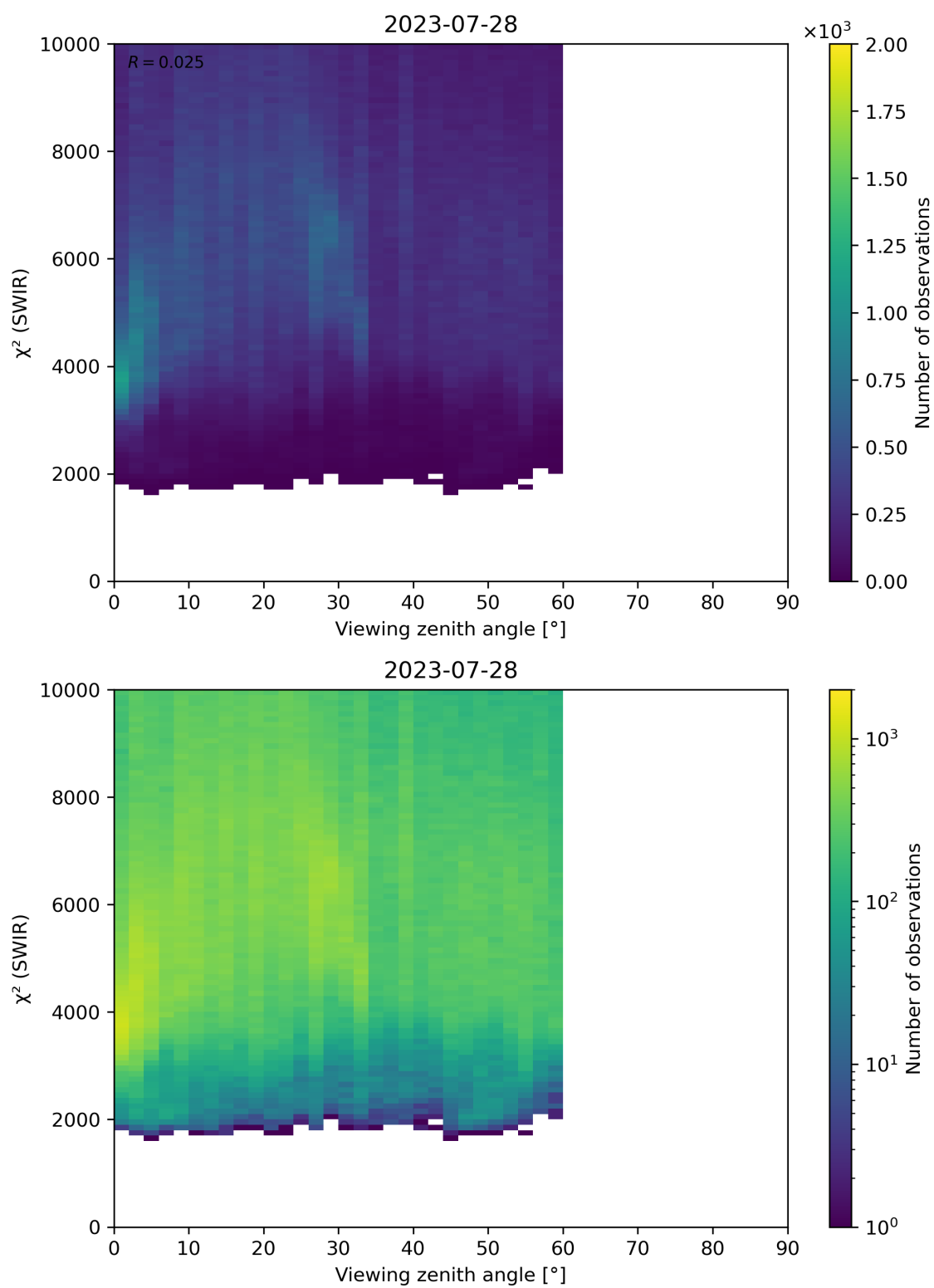
Figure 106: Scatter density plot of “Viewing zenith angle” against “ \chi^2 (SWIR)” for 2023-07-27 to 2023-07-29.
