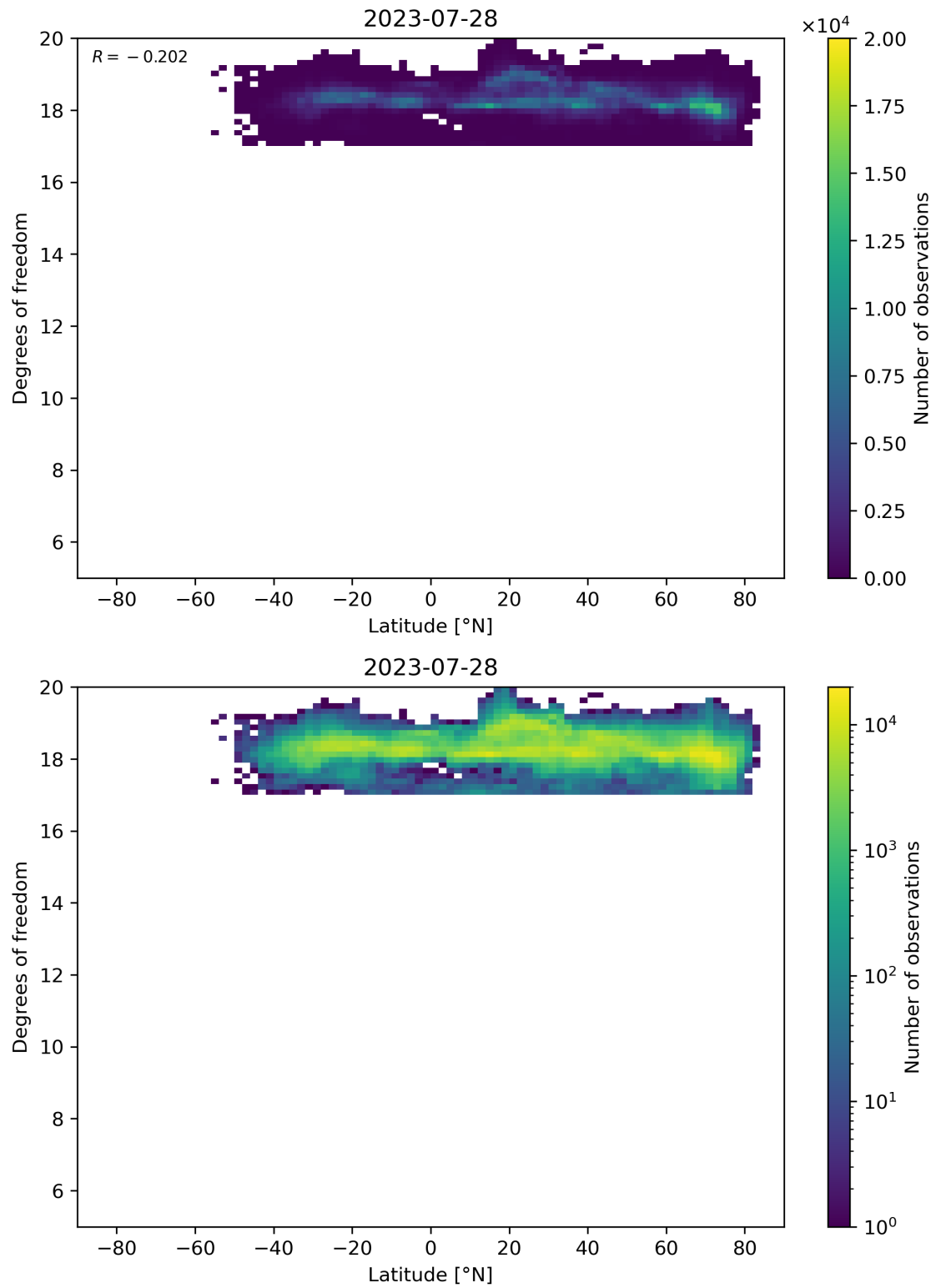
Figure 55: Scatter density plot of “Latitude” against “Degrees of freedom” for 2023-07-27 to 2023-07-29.
