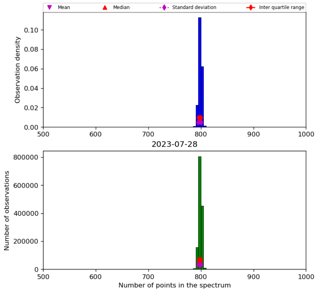
Figure 26: Histogram of “Number of points in the spectrum” for 2023-07-27 to 2023-07-29
