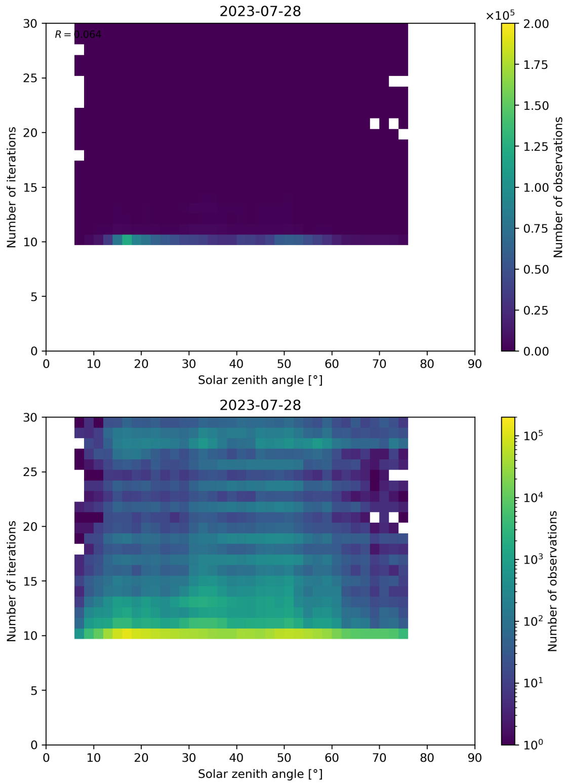
Figure 102: Scatter density plot of “Solar zenith angle” against “Number of iterations” for 2023-07-27 to 2023-07-29.
