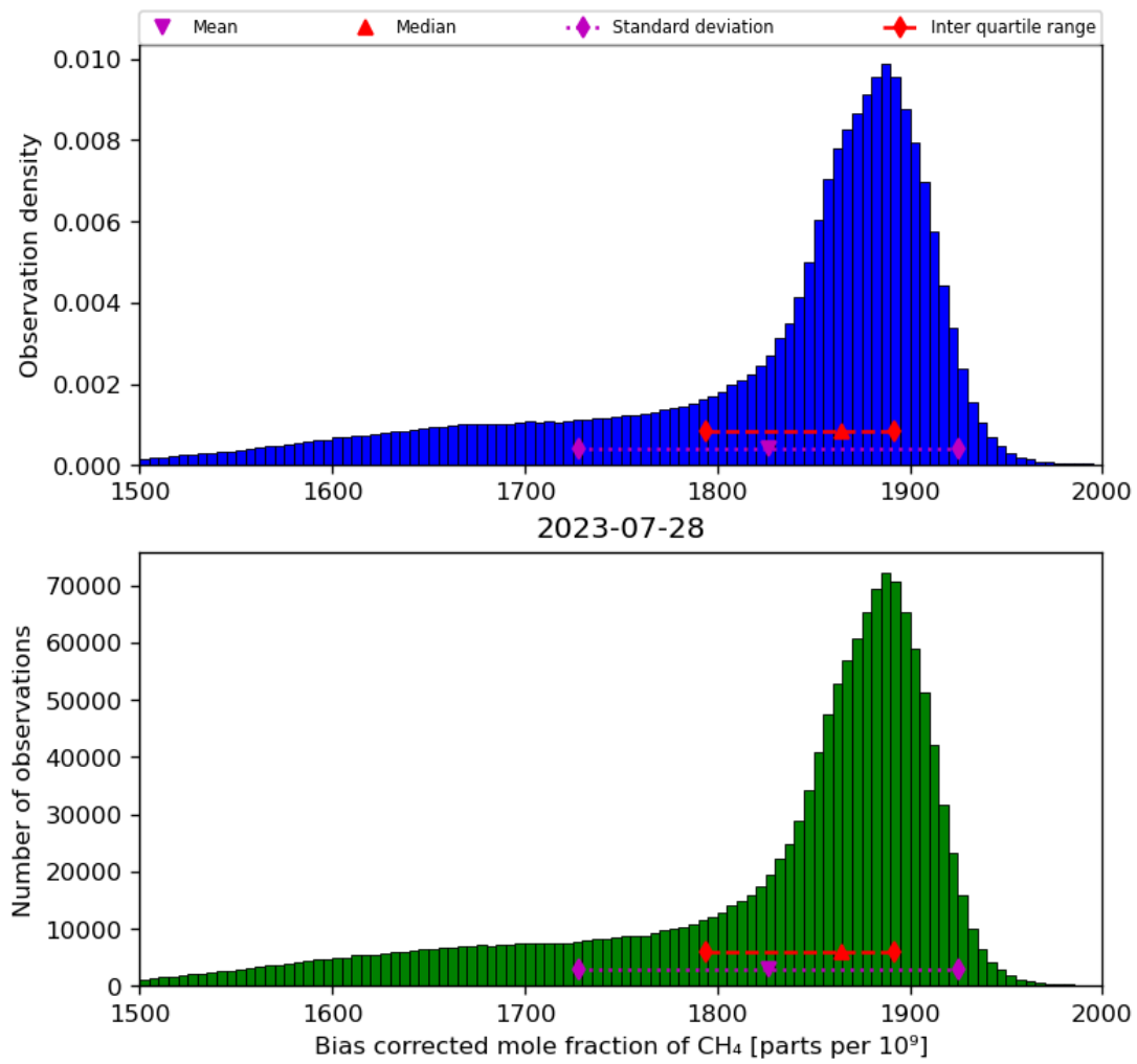
Figure 25: Histogram of “Bias corrected mole fraction of CH 4 ” for 2023-07-27 to 2023-07-29
