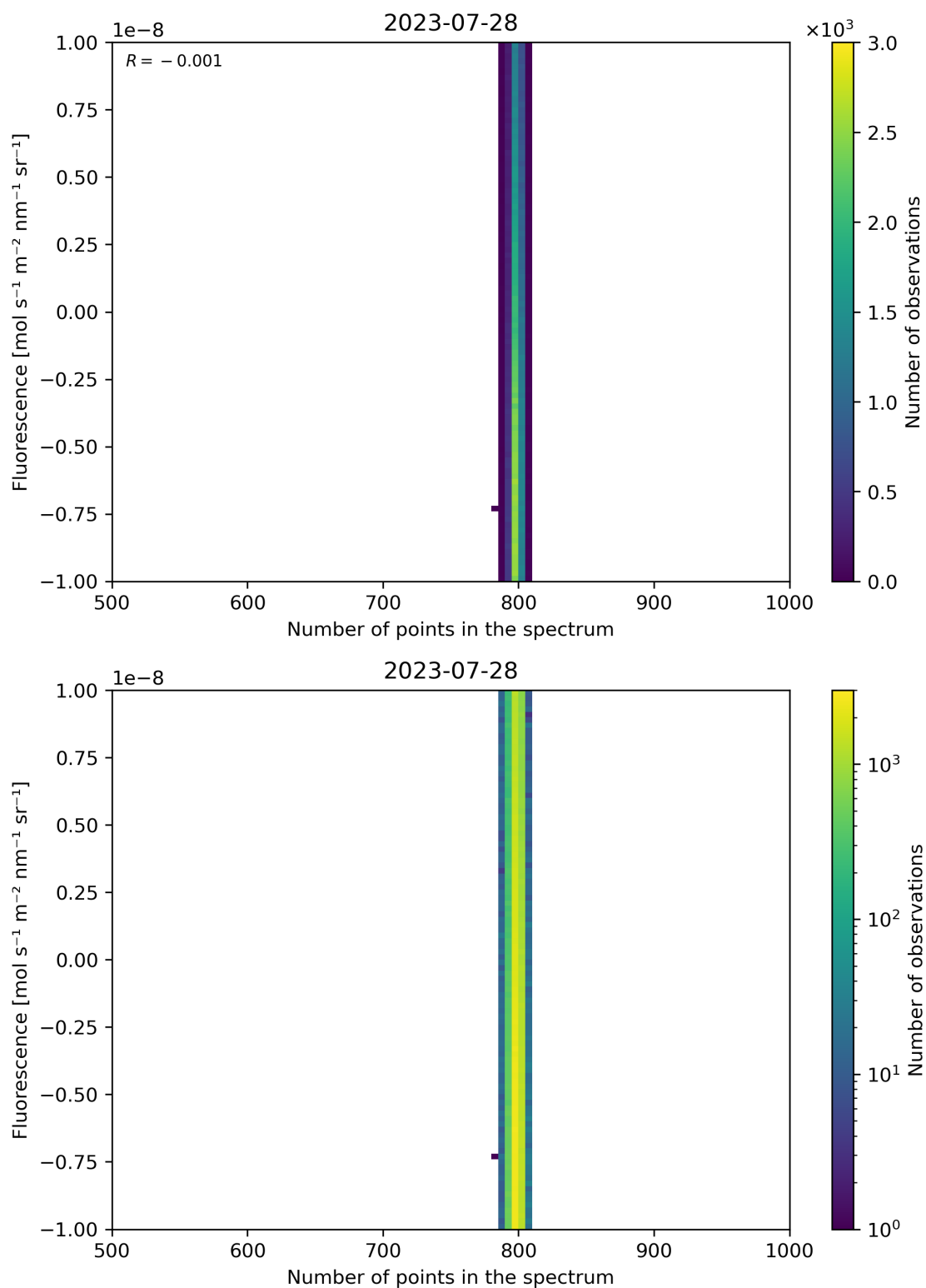
Figure 91: Scatter density plot of “Number of points in the spectrum” against “Fluorescence” for 2023-07-27 to 2023-07-29.
