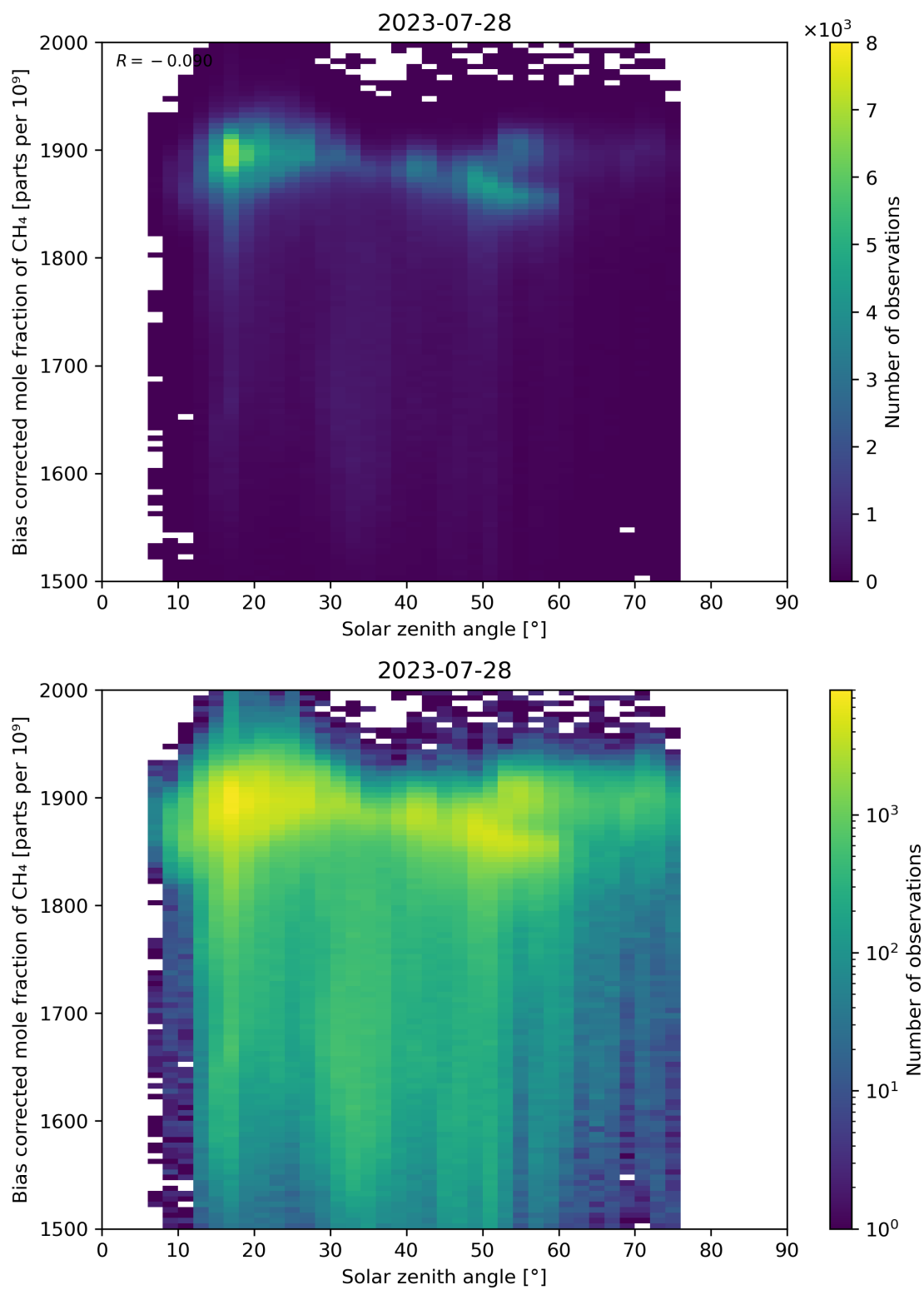
Figure 100: Scatter density plot of “Solar zenith angle” against “Bias corrected mole fraction of CH 4 ” for 2023-07-27 to 2023-07-29.
