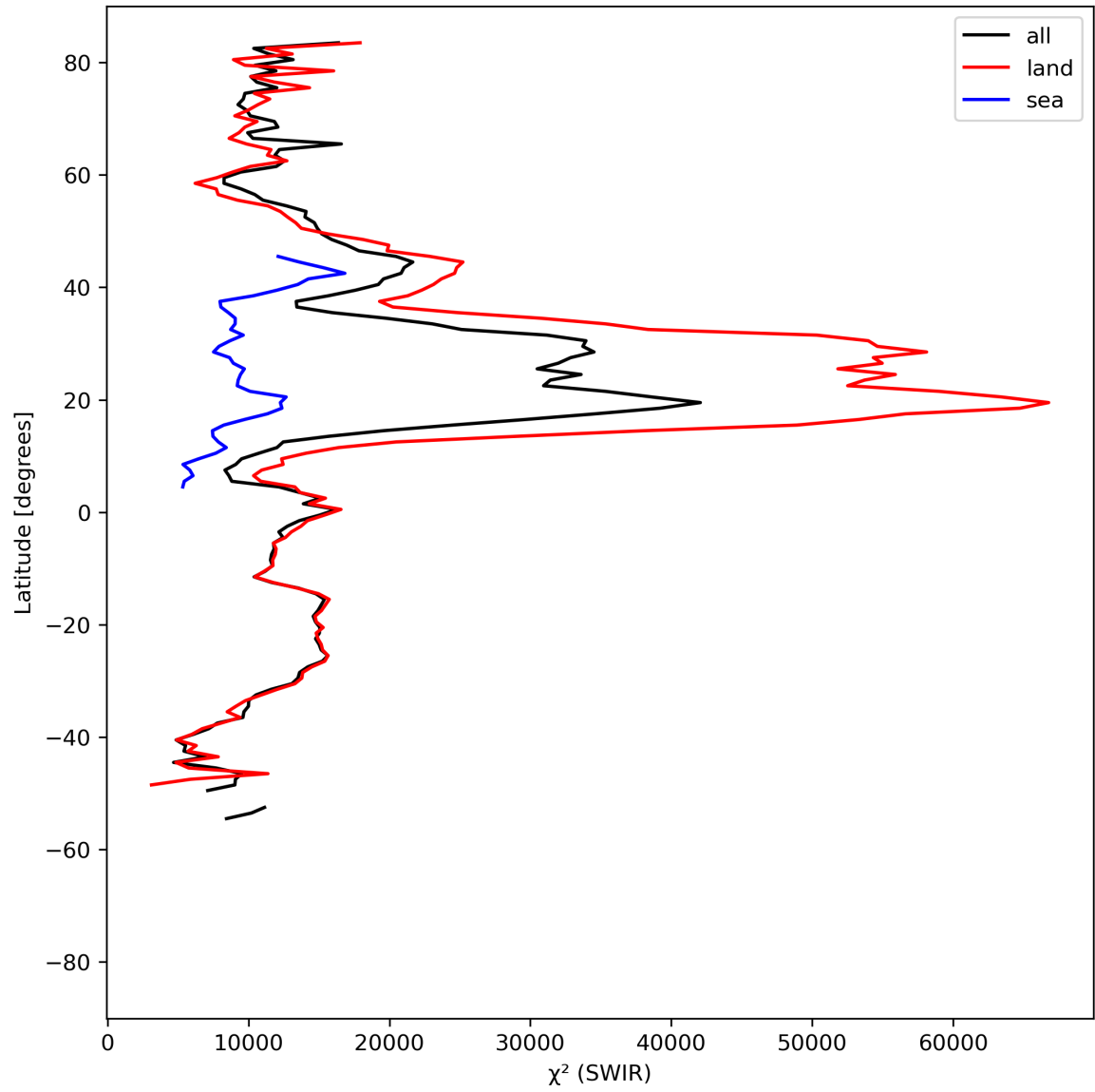
Figure 17: Zonal average of “ \chi^2 (SWIR)” for 2023-07-27 to 2023-07-29.
