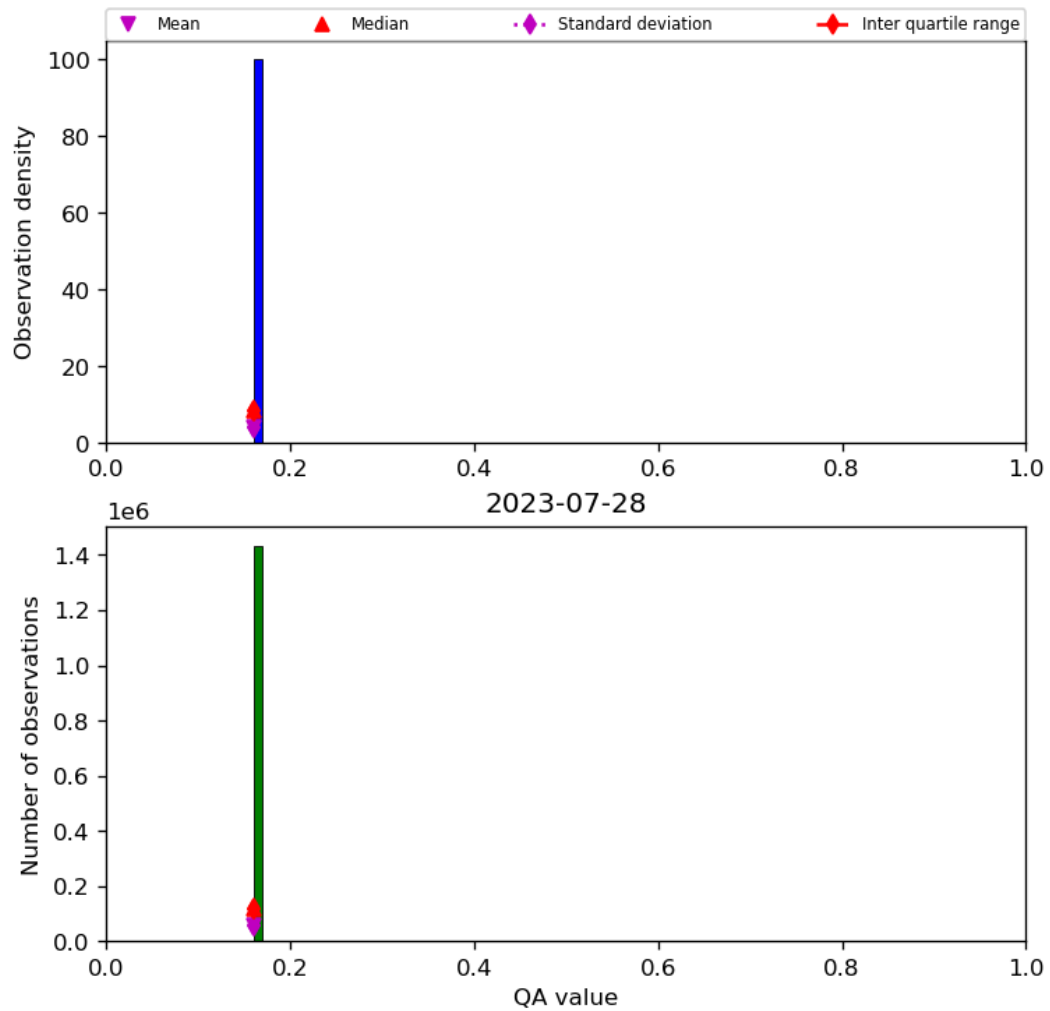
Figure 22: Histogram of “QA value” for 2023-07-27 to 2023-07-29
