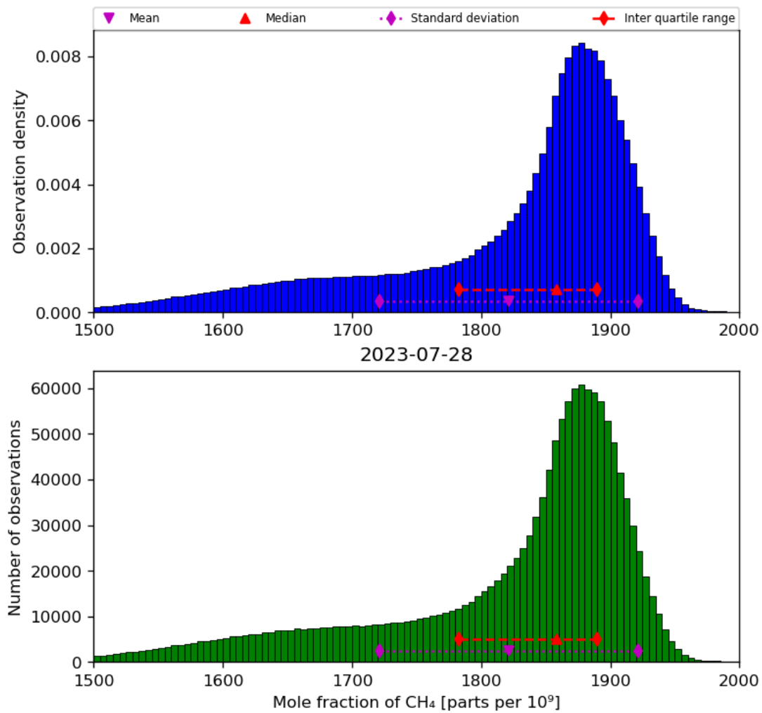
Figure 23: Histogram of “Mole fraction of CH 4 ” for 2023-07-27 to 2023-07-29
