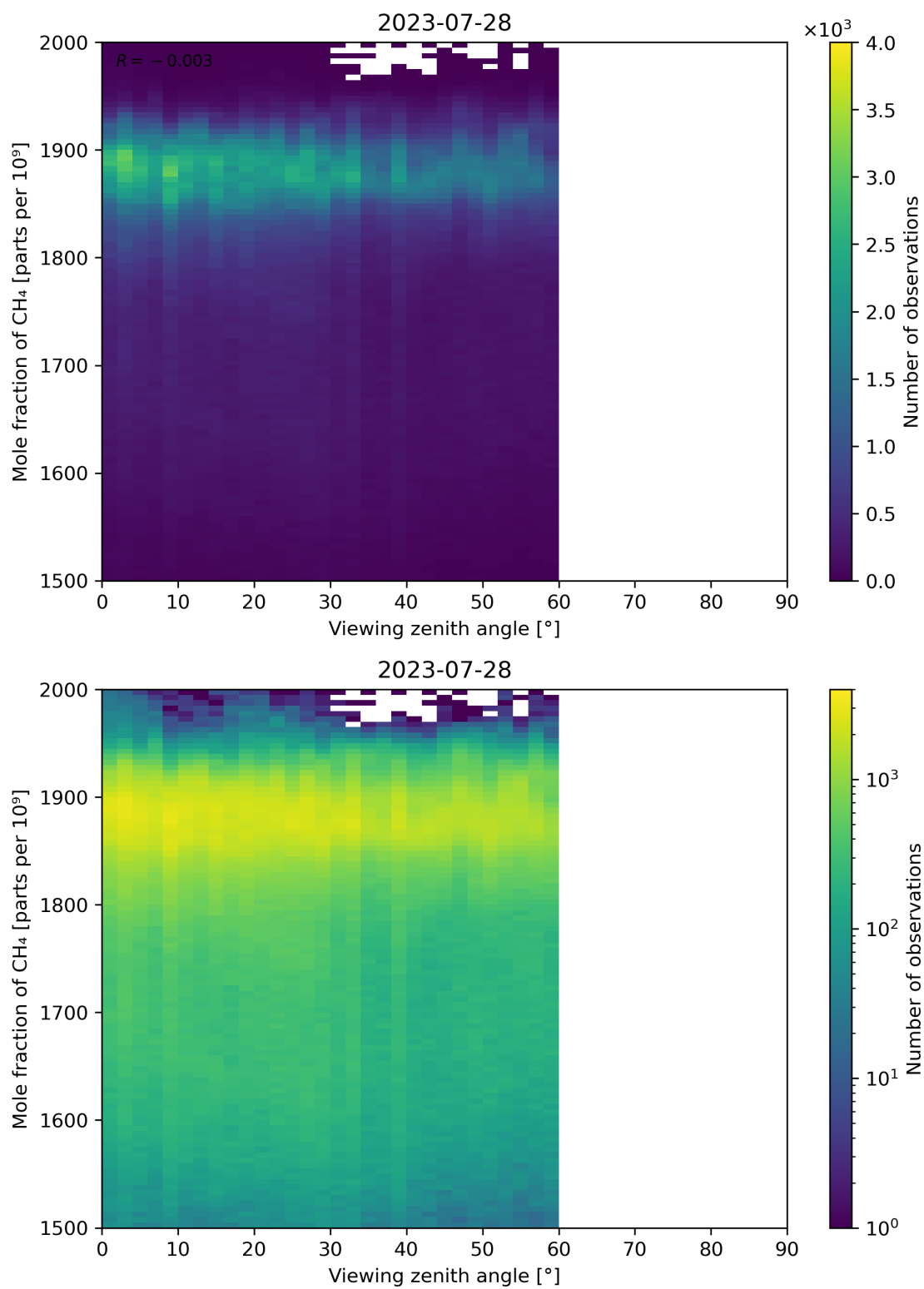
Figure 110: Scatter density plot of “Viewing zenith angle” against “Mole fraction of CH 4 ” for 2023-07-27 to 2023-07-29.
