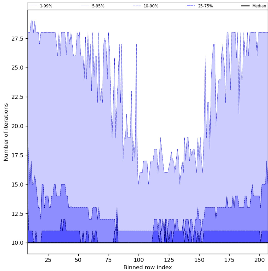
Figure 42: Along track statistics of “Number of iterations” for 2023-07-27 to 2023-07-29
