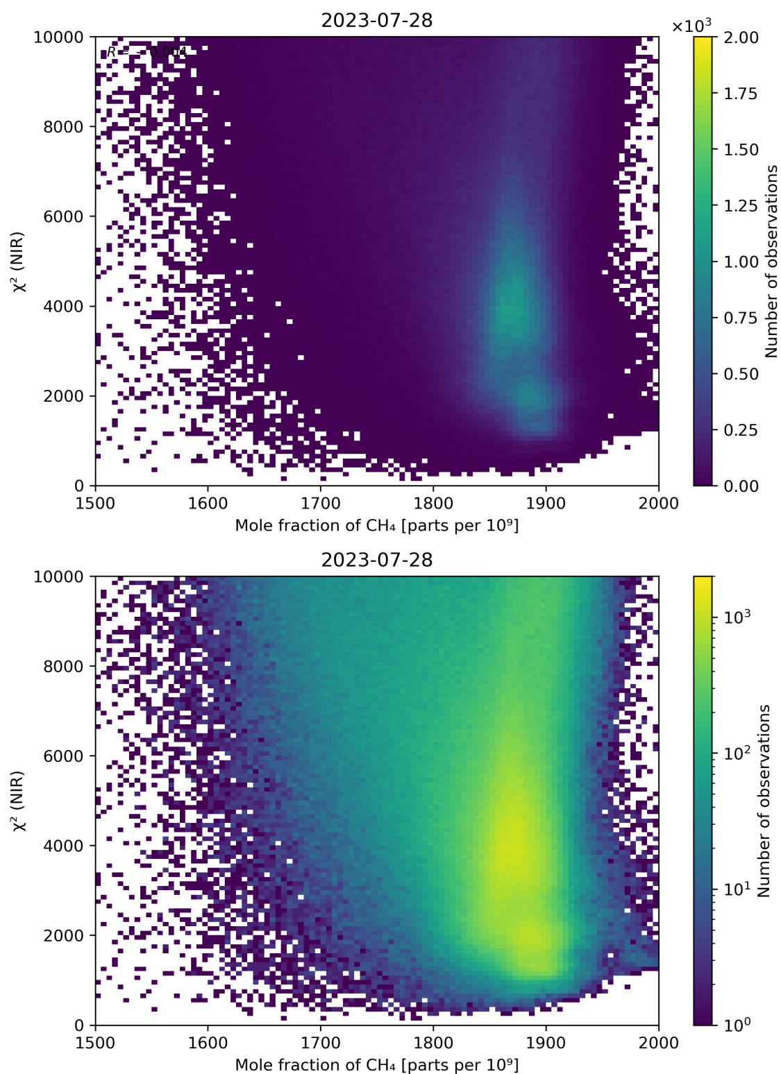
Figure 70: Scatter density plot of “Mole fraction of CH 4 ” against “ \chi^2 (NIR)” for 2023-07-27 to 2023-07-29.
