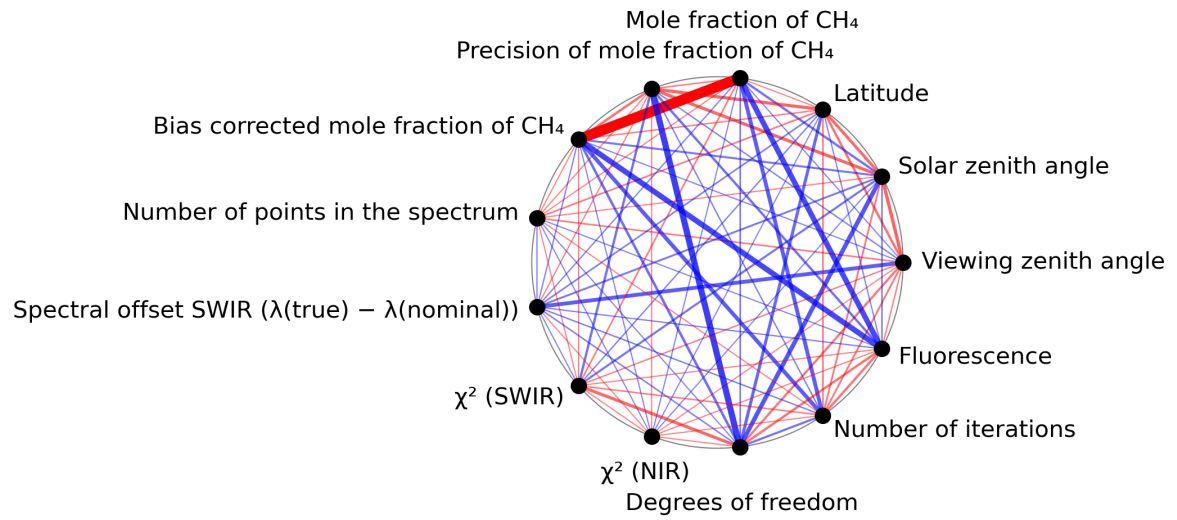
Figure 1: Map of correlation graph for 2023-07-27 to 2023-07-29.
