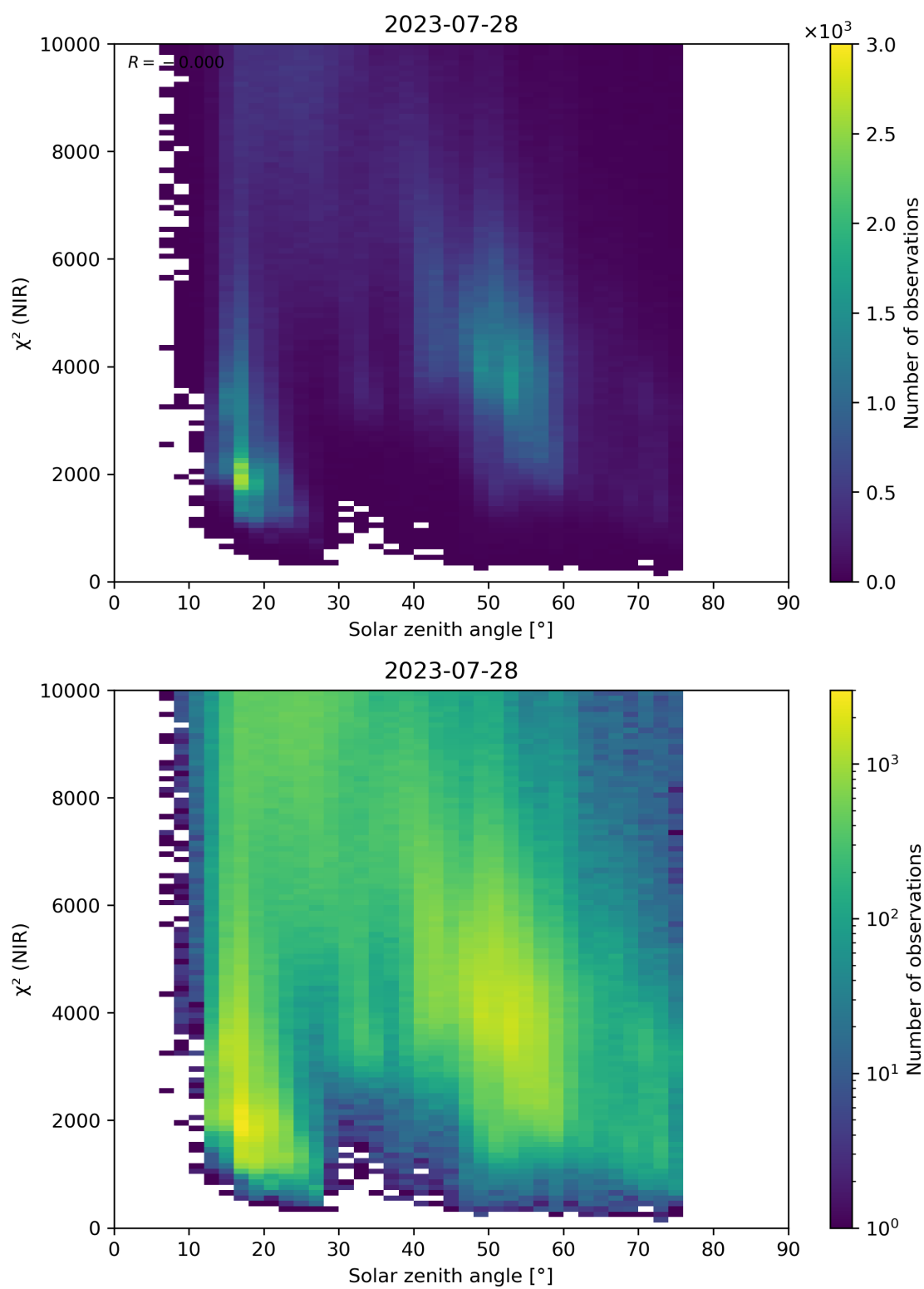
Figure 94: Scatter density plot of “Solar zenith angle” against “ \chi^2 (NIR)” for 2023-07-27 to 2023-07-29.
