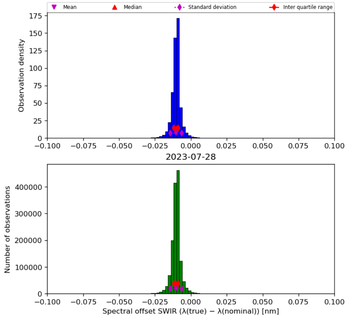
Figure 27: Histogram of “Spectral offset SWIR ( \lambda(\text{true}) - \lambda(\text{nominal}) )” for 2023-07-27 to 2023-07-29
