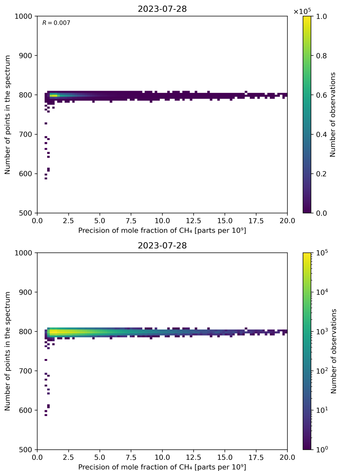
Figure 84: Scatter density plot of “Precision of mole fraction of \text{CH}_4 ” against “Number of points in the spectrum” for 2023-07-27 to 2023-07-29.
