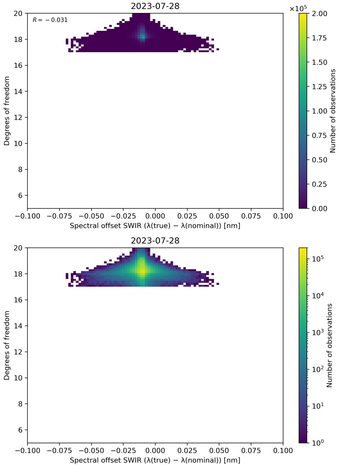
Figure 119: Scatter density plot of “Spectral offset SWIR ( \lambda(\text{true}) - \lambda(\text{nominal}) )” against “Degrees of freedom” for 2023-07-27 to 2023-07-29.
