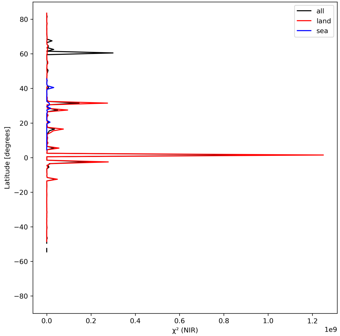
Figure 18: Zonal average of “ \chi^2 (NIR)” for 2023-07-27 to 2023-07-29.
