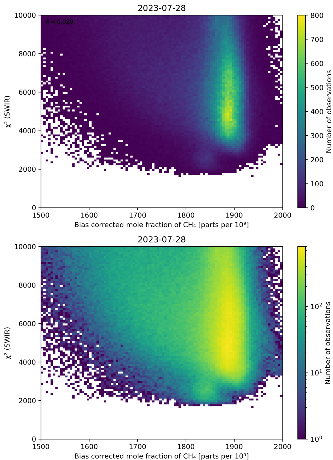
Figure 64: Scatter density plot of “Bias corrected mole fraction of CH 4 ” against “ \chi^2 (SWIR)” for 2023-07-27 to 2023-07-29.
