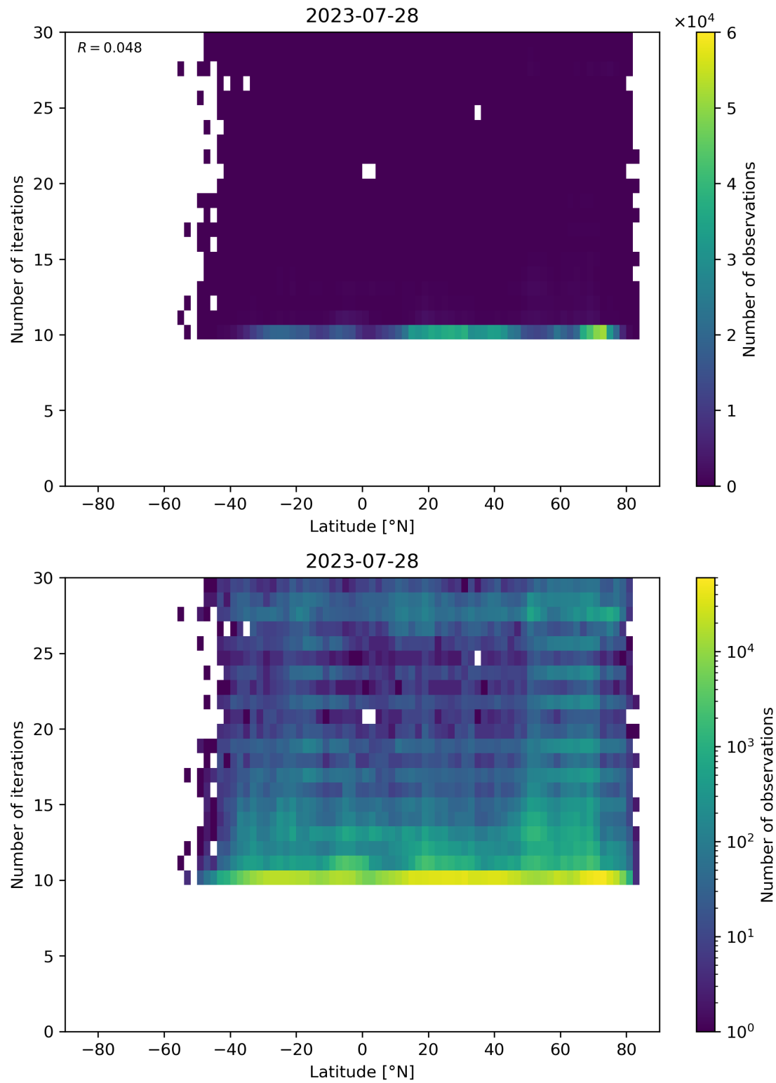
Figure 60: Scatter density plot of “Latitude” against “Number of iterations” for 2023-07-27 to 2023-07-29.
