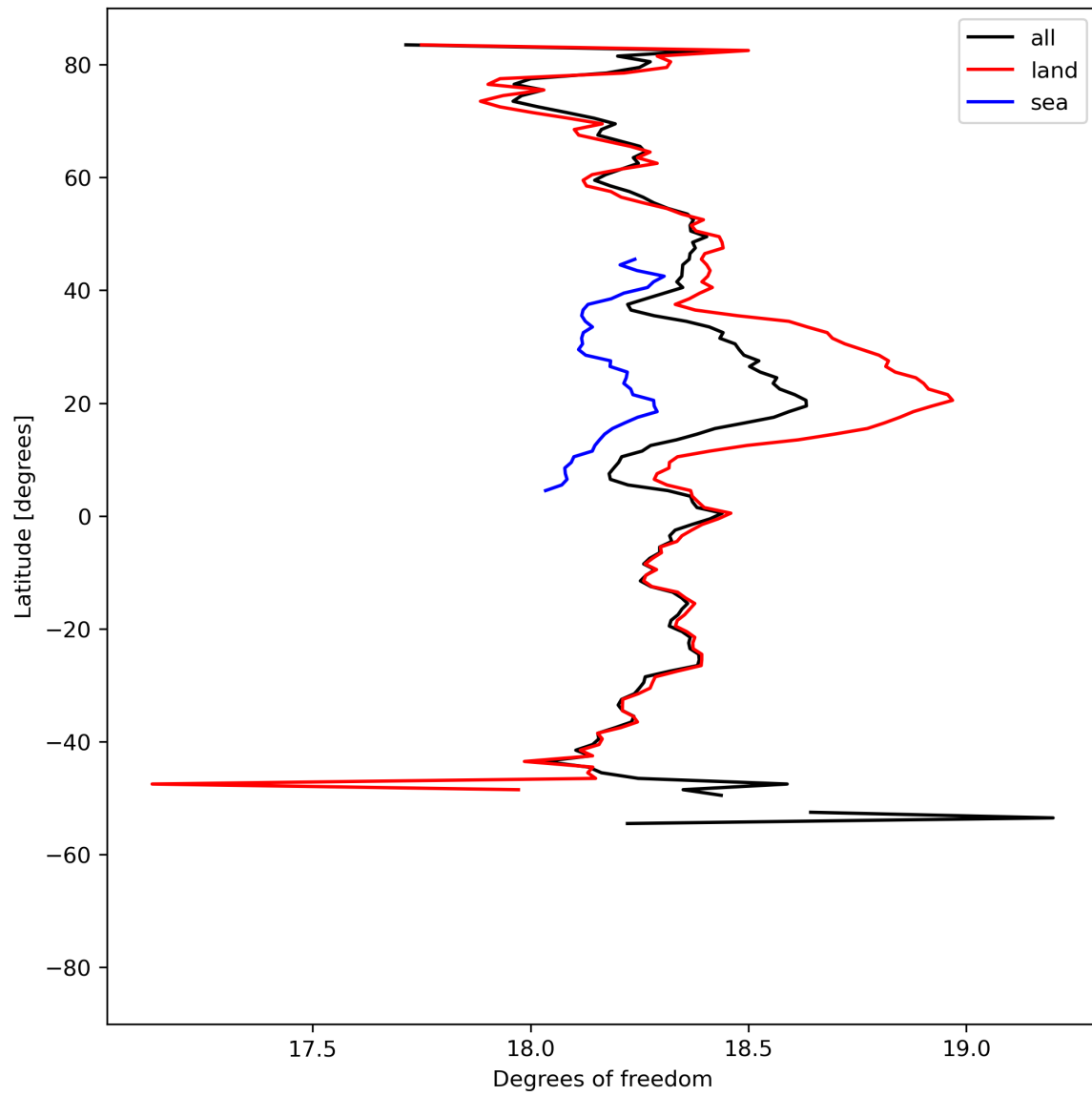
Figure 19: Zonal average of “Degrees of freedom” for 2023-07-27 to 2023-07-29.
