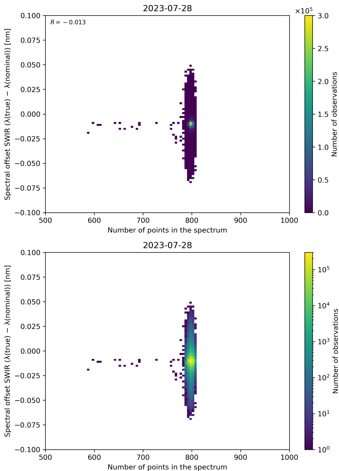
Figure 93: Scatter density plot of “Number of points in the spectrum” against “Spectral offset SWIR ( \lambda(\text{true}) - \lambda(\text{nominal}) )” for 2023-07-27 to 2023-07-29.
