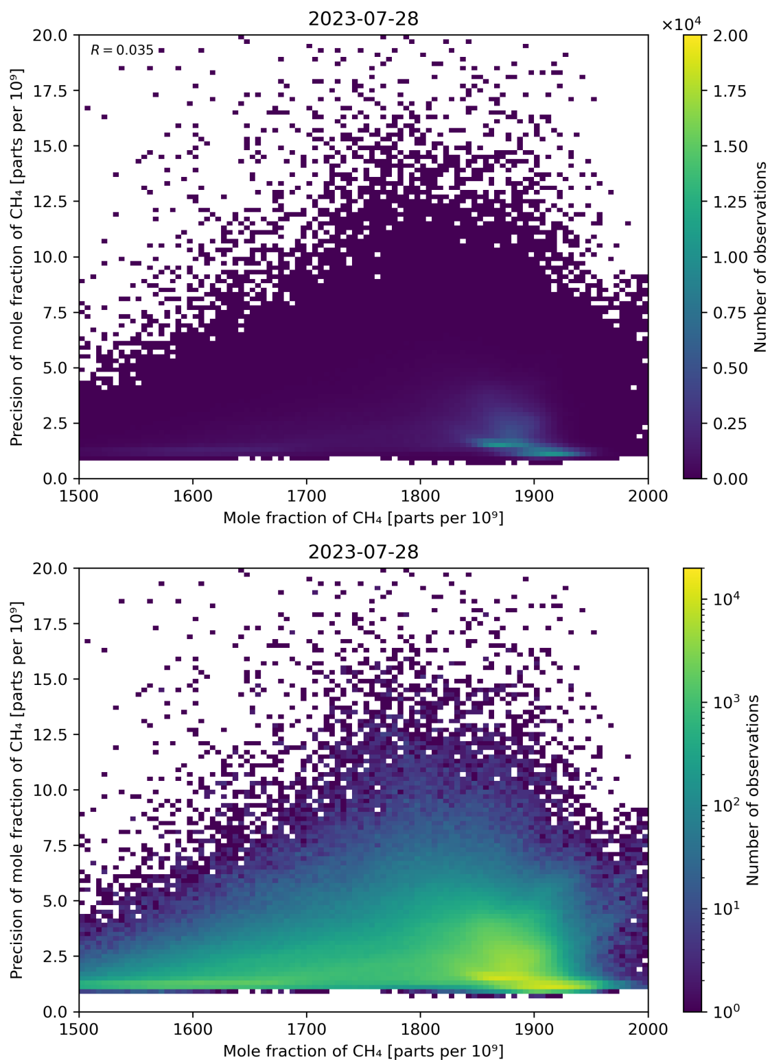
Figure 75: Scatter density plot of “Mole fraction of CH 4 ” against “Precision of mole fraction of CH 4 ” for 2023-07-27 to 2023-07-29.
