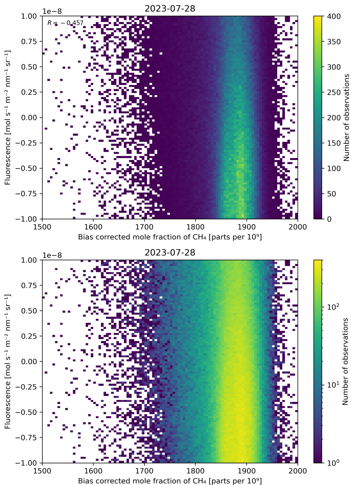
Figure 66: Scatter density plot of “Bias corrected mole fraction of \text{CH}_4 ” against “Fluorescence” for 2023-07-27 to 2023-07-29.
