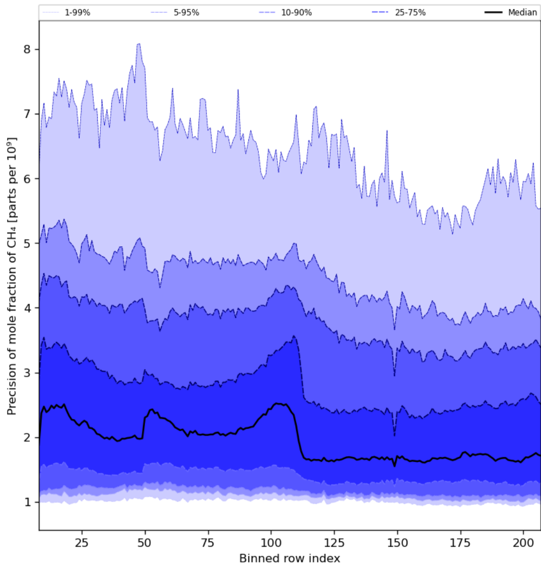
Figure 35: Along track statistics of “Precision of mole fraction of CH 4 ” for 2023-07-27 to 2023-07-29
