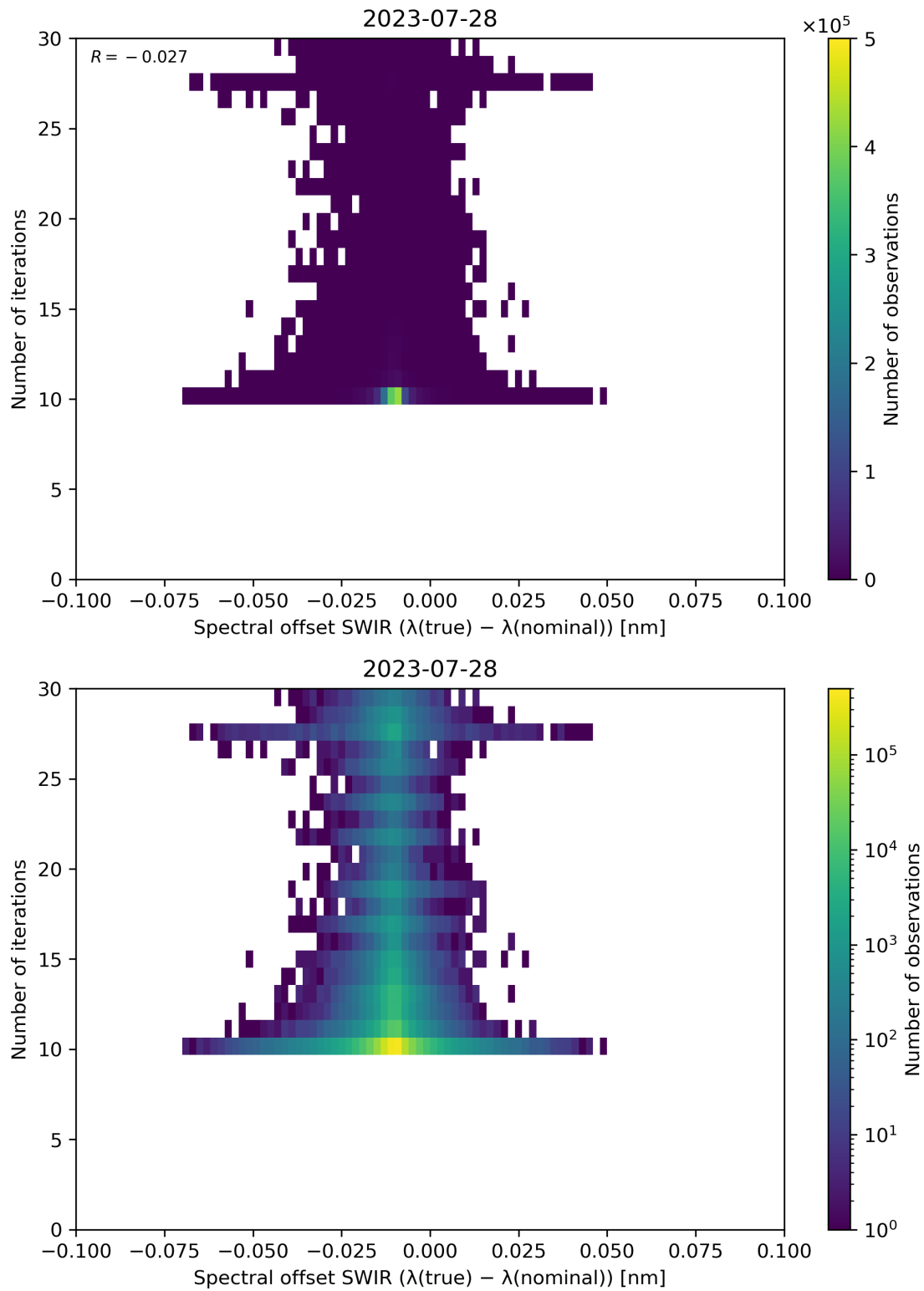
Figure 121: Scatter density plot of “Spectral offset SWIR ( \lambda(\text{true}) - \lambda(\text{nominal}) )” against “Number of iterations” for 2023-07-27 to 2023-07-29.
