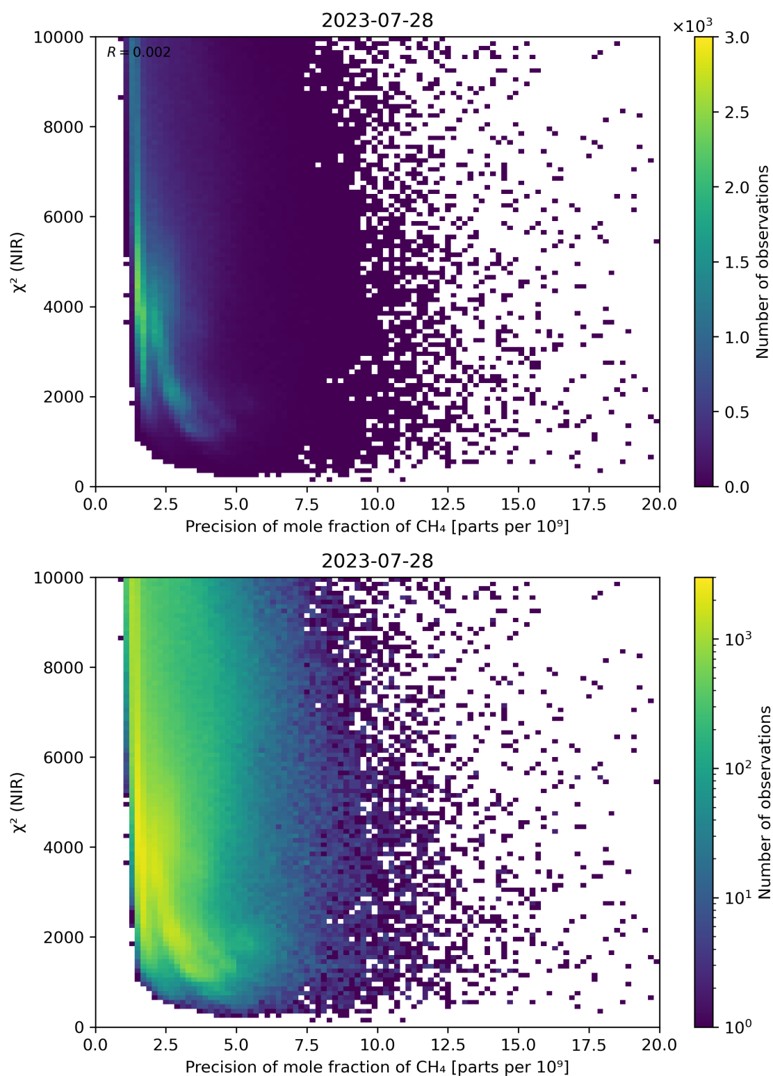
Figure 78: Scatter density plot of “Precision of mole fraction of CH 4 ” against “ \chi^2 (NIR)” for 2023-07-27 to 2023-07-29.
