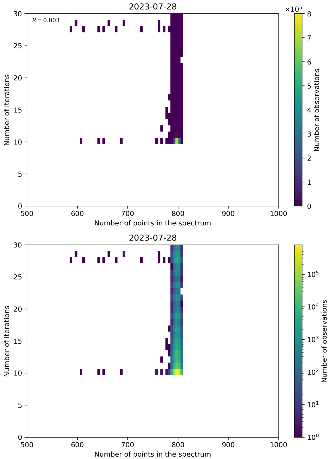
Figure 92: Scatter density plot of “Number of points in the spectrum” against “Number of iterations” for 2023-07-27 to 2023-07-29.
