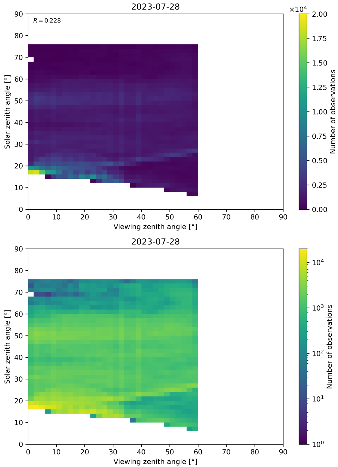
Figure 115: Scatter density plot of “Viewing zenith angle” against “Solar zenith angle” for 2023-07-27 to 2023-07-29.
