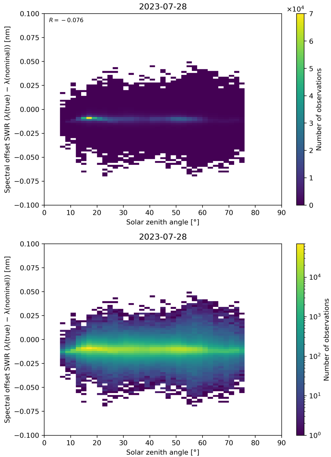
Figure 104: Scatter density plot of “Solar zenith angle” against “Spectral offset SWIR ( \lambda(\text{true}) - \lambda(\text{nominal}) )” for 2023-07-27 to 2023-07-29.
