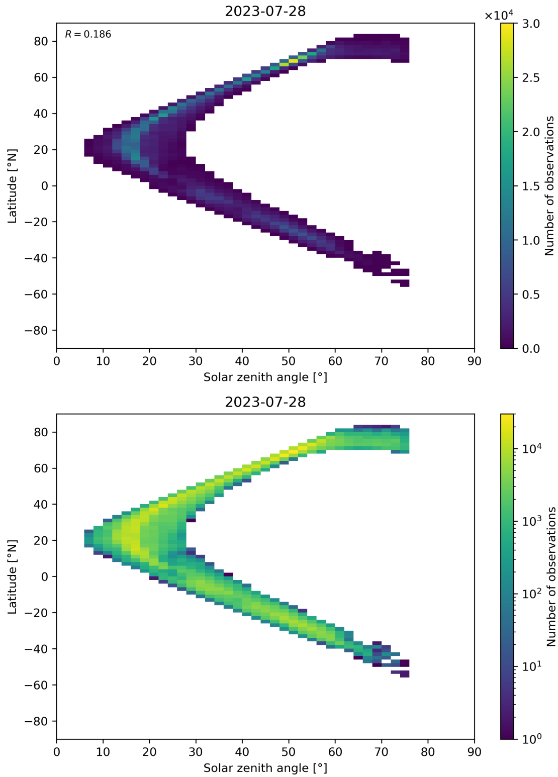
Figure 98: Scatter density plot of “Solar zenith angle” against “Latitude” for 2023-07-27 to 2023-07-29.
