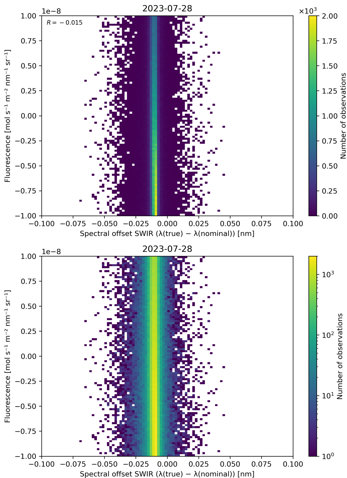
Figure 120: Scatter density plot of “Spectral offset SWIR ( \lambda(\text{true}) - \lambda(\text{nominal}) )” against “Fluorescence” for 2023-07-27 to 2023-07-29.
