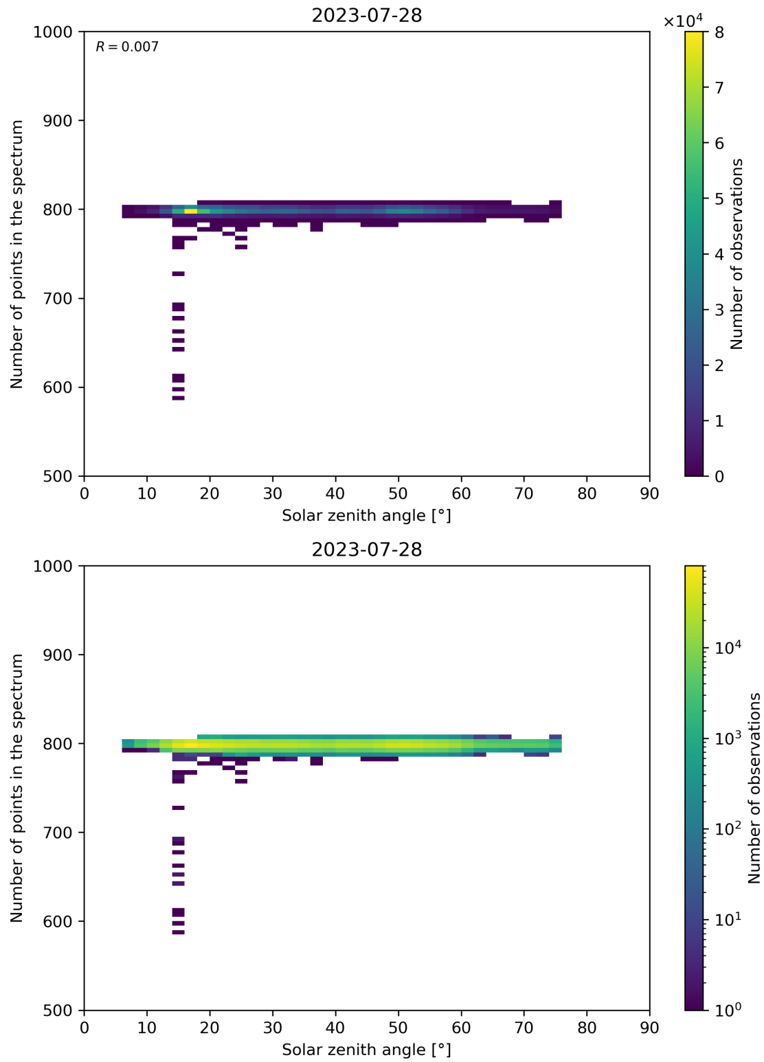
Figure 103: Scatter density plot of “Solar zenith angle” against “Number of points in the spectrum” for 2023-07-27 to 2023-07-29.
