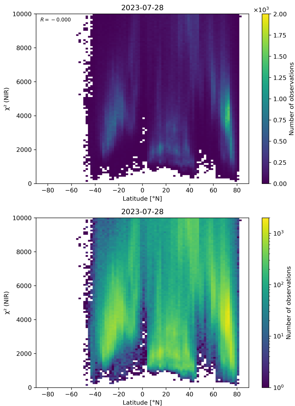
Figure 53: Scatter density plot of “Latitude” against “ \chi^2 (NIR)” for 2023-07-27 to 2023-07-29.
