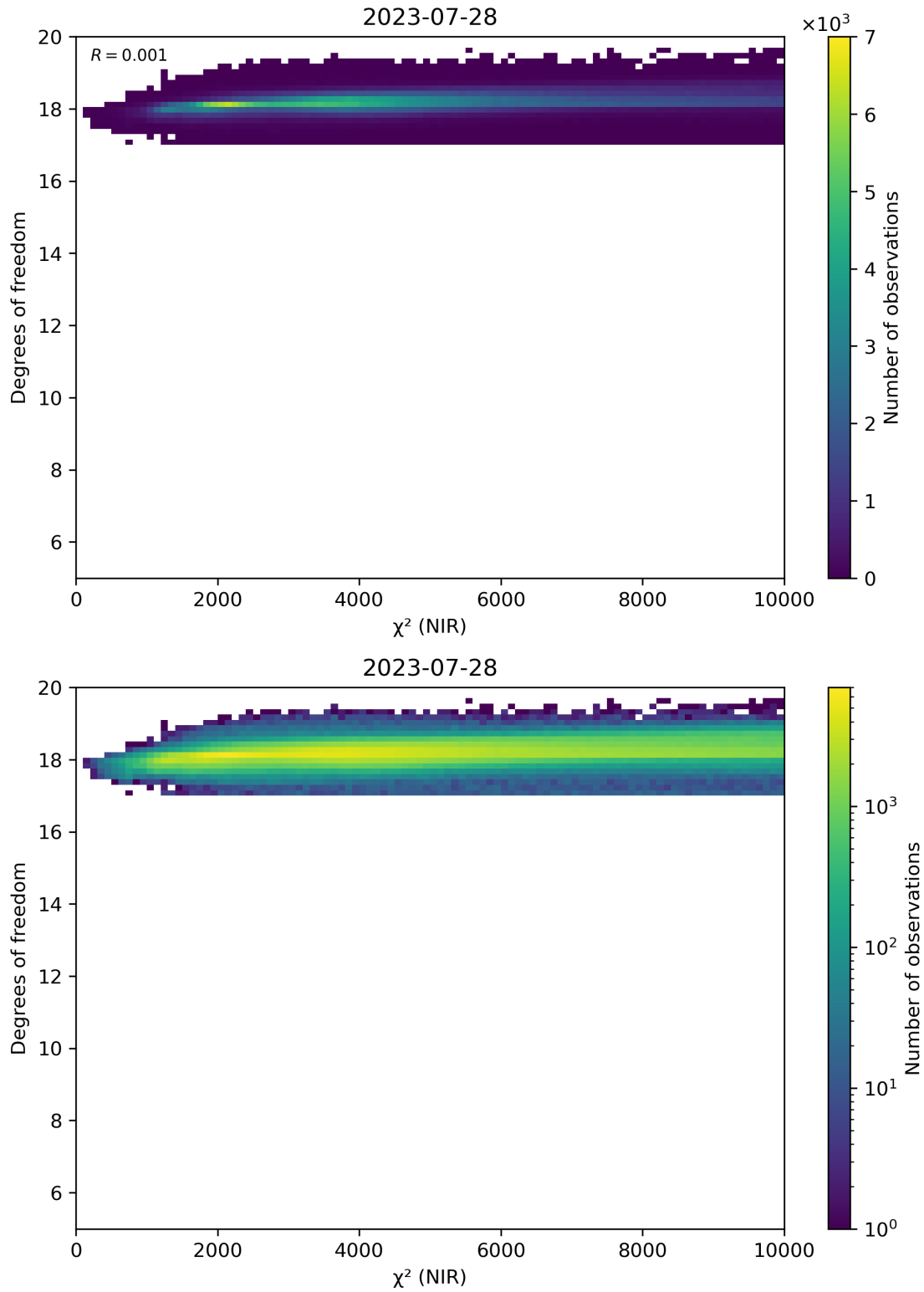
Figure 44: Scatter density plot of “ \chi^2 (NIR)” against “Degrees of freedom” for 2023-07-27 to 2023-07-29.
