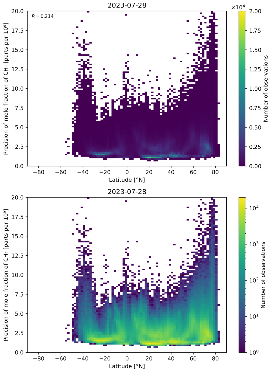
Figure 59: Scatter density plot of “Latitude” against “Precision of mole fraction of \text{CH}_4 ” for 2023-07-27 to 2023-07-29.
