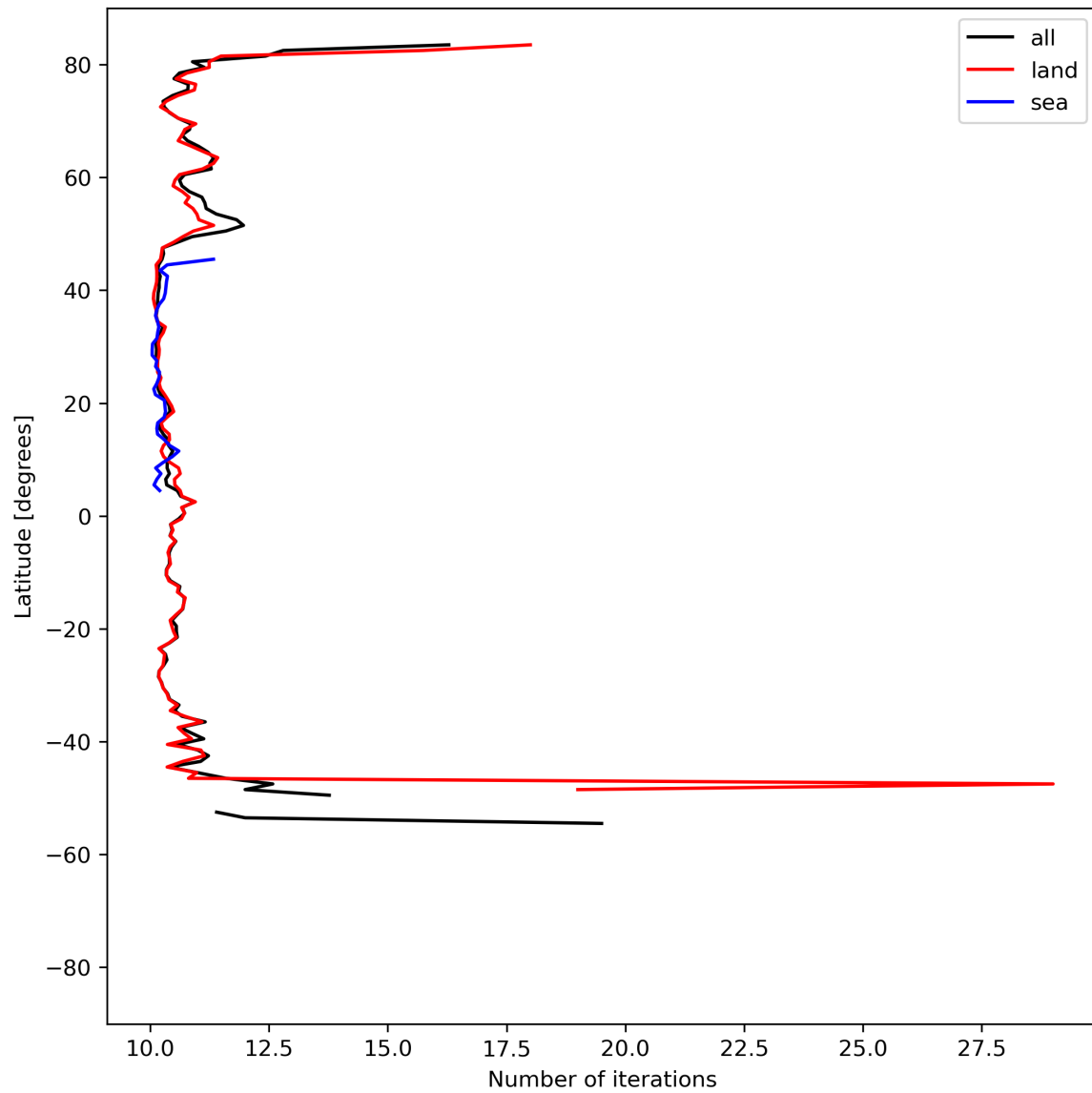
Figure 20: Zonal average of “Number of iterations” for 2023-07-27 to 2023-07-29.
