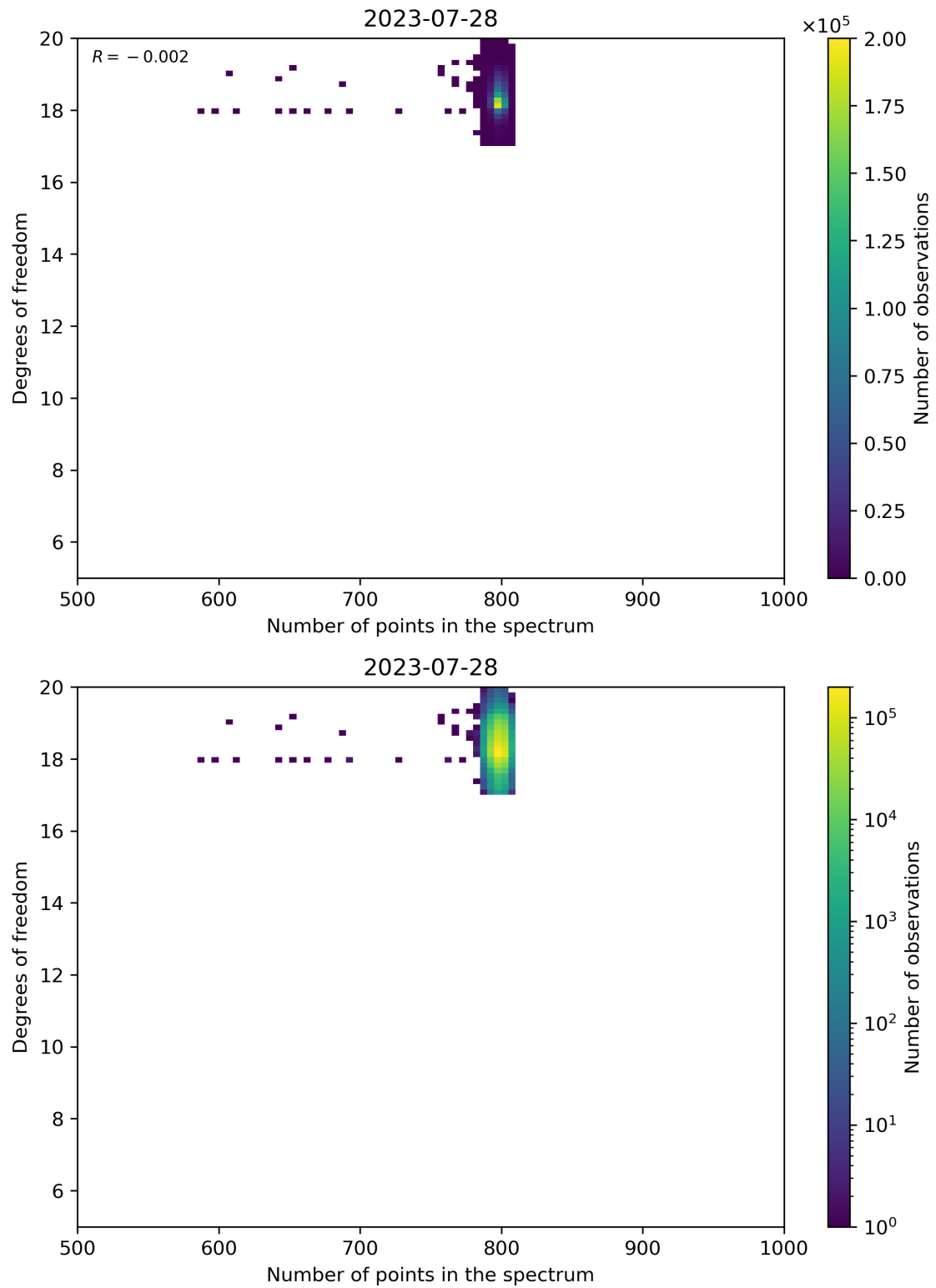
Figure 90: Scatter density plot of “Number of points in the spectrum” against “Degrees of freedom” for 2023-07-27 to 2023-07-29.
