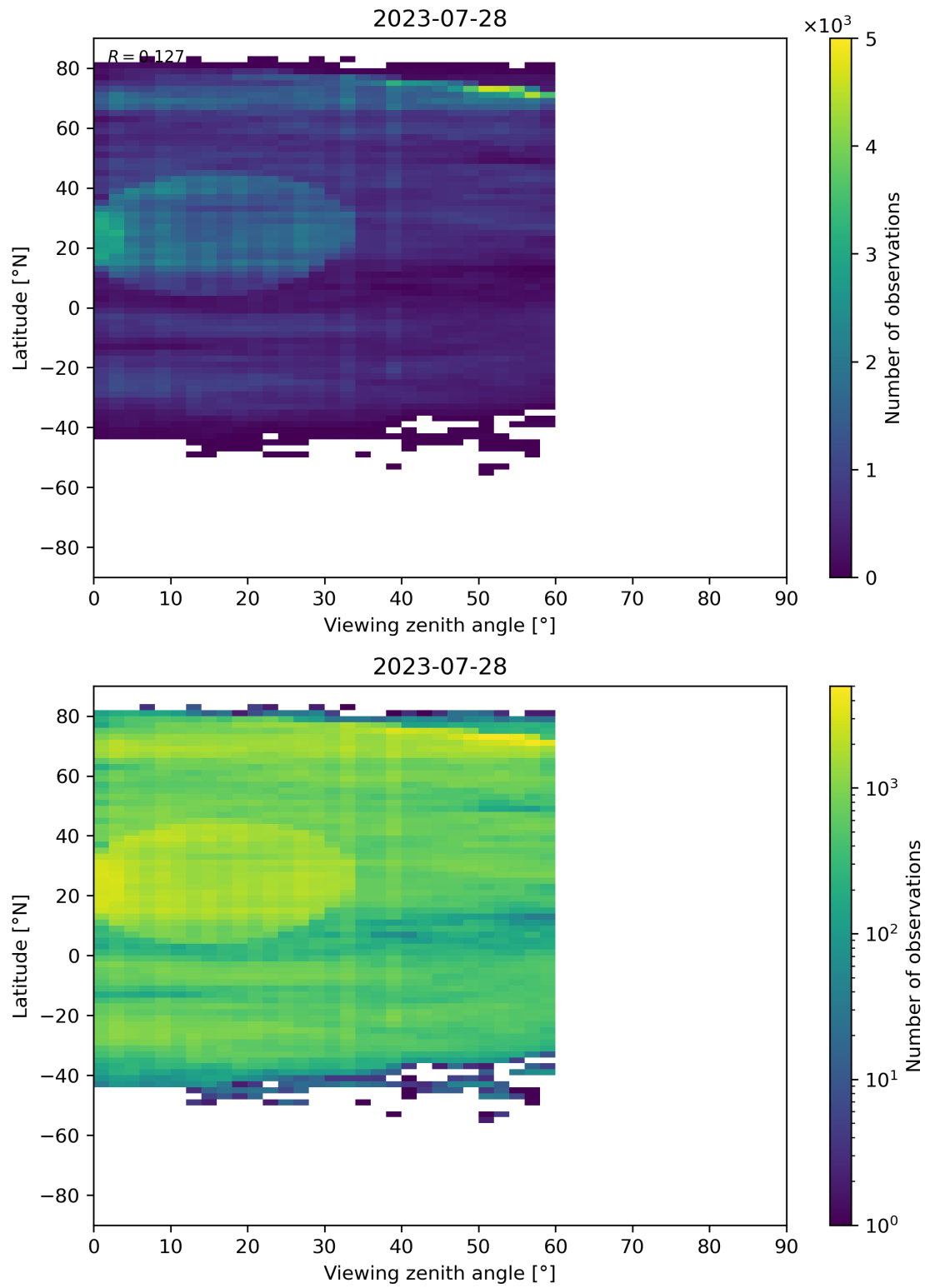
Figure 109: Scatter density plot of “Viewing zenith angle” against “Latitude” for 2023-07-27 to 2023-07-29.
