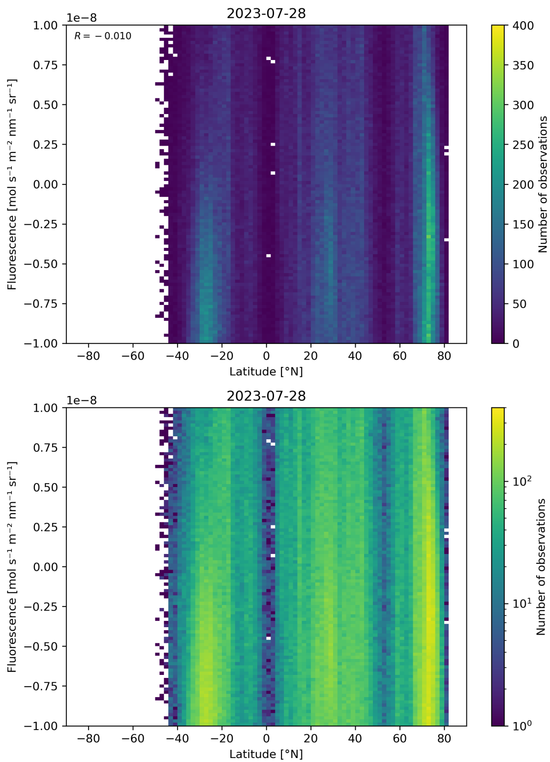
Figure 56: Scatter density plot of “Latitude” against “Fluorescence” for 2023-07-27 to 2023-07-29.
