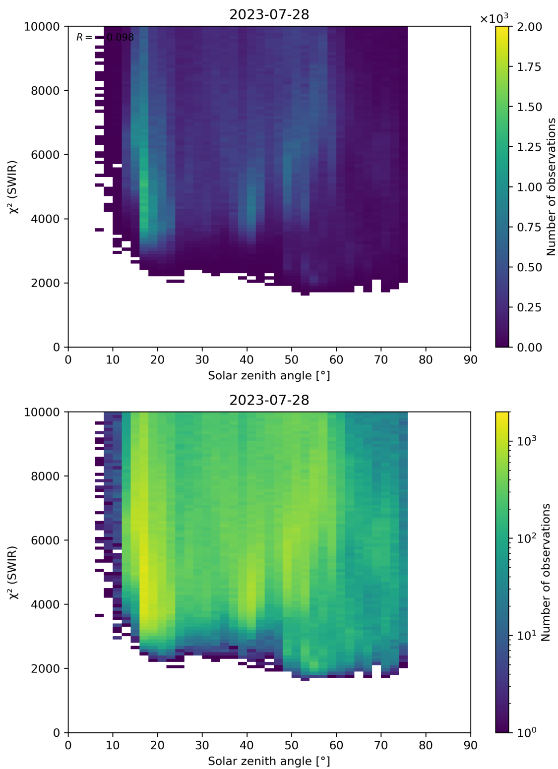
Figure 95: Scatter density plot of “Solar zenith angle” against “ \chi^2 (SWIR)” for 2023-07-27 to 2023-07-29.
