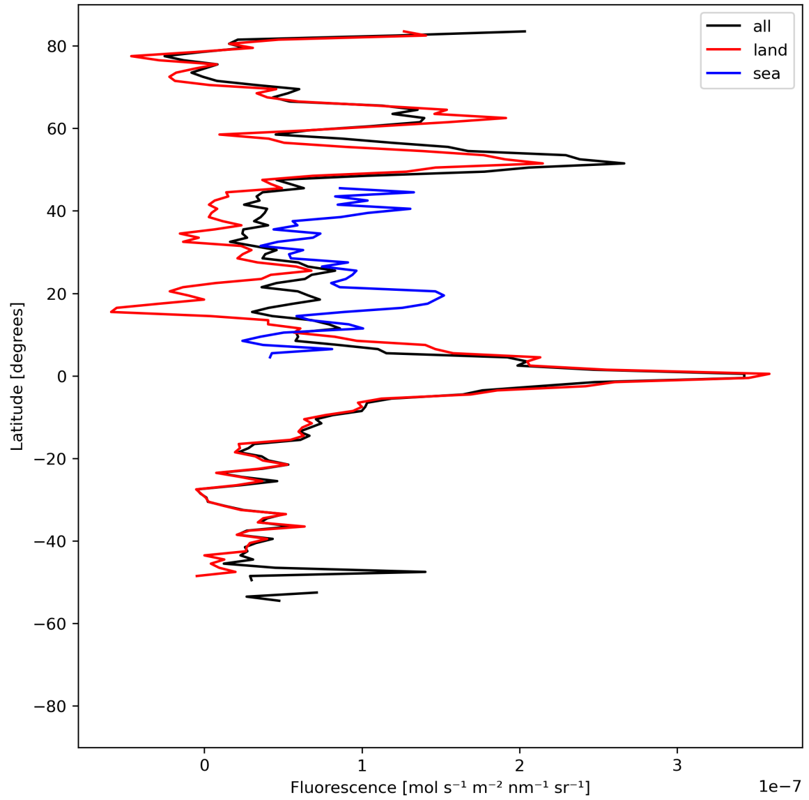
Figure 21: Zonal average of “Fluorescence” for 2023-07-27 to 2023-07-29.
