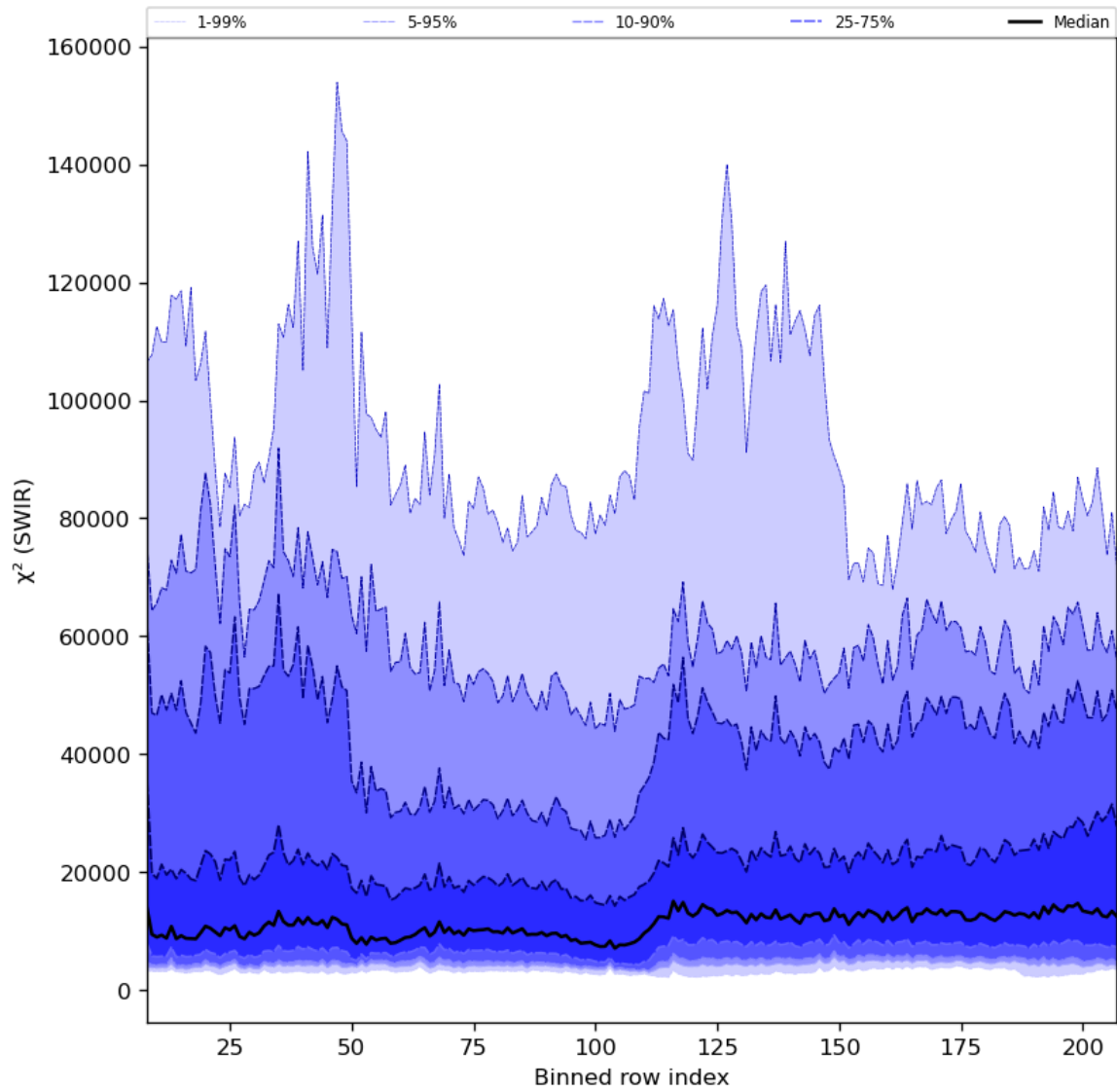
Figure 39: Along track statistics of “ \chi^2 (SWIR)” for 2023-07-27 to 2023-07-29
