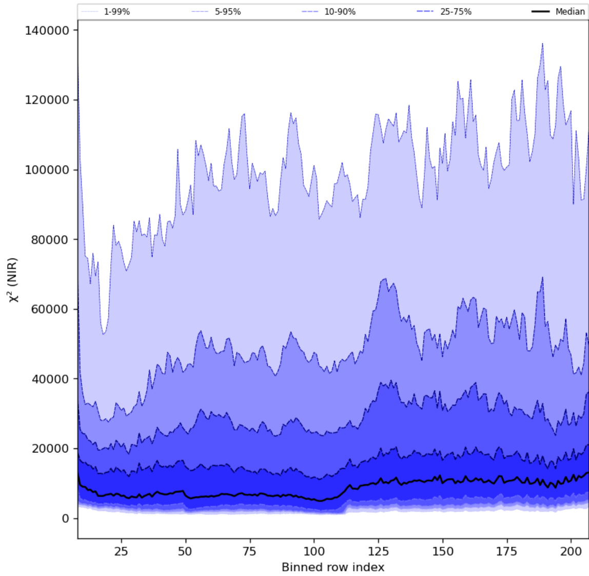
Figure 40: Along track statistics of " \chi^2 (NIR)" for 2023-07-27 to 2023-07-29
