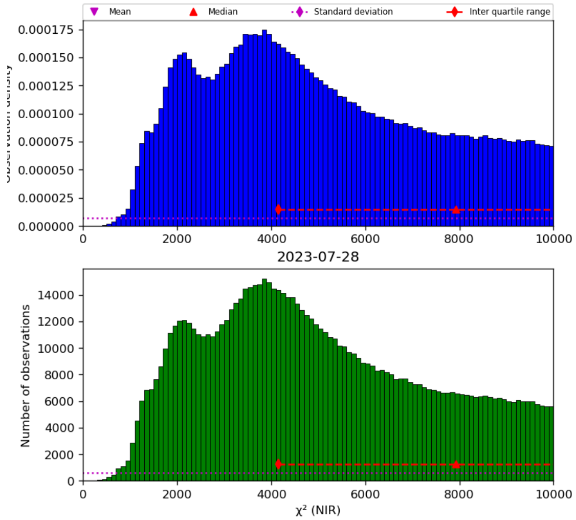
Figure 29: Histogram of “ \chi^2 (NIR)” for 2023-07-27 to 2023-07-29
