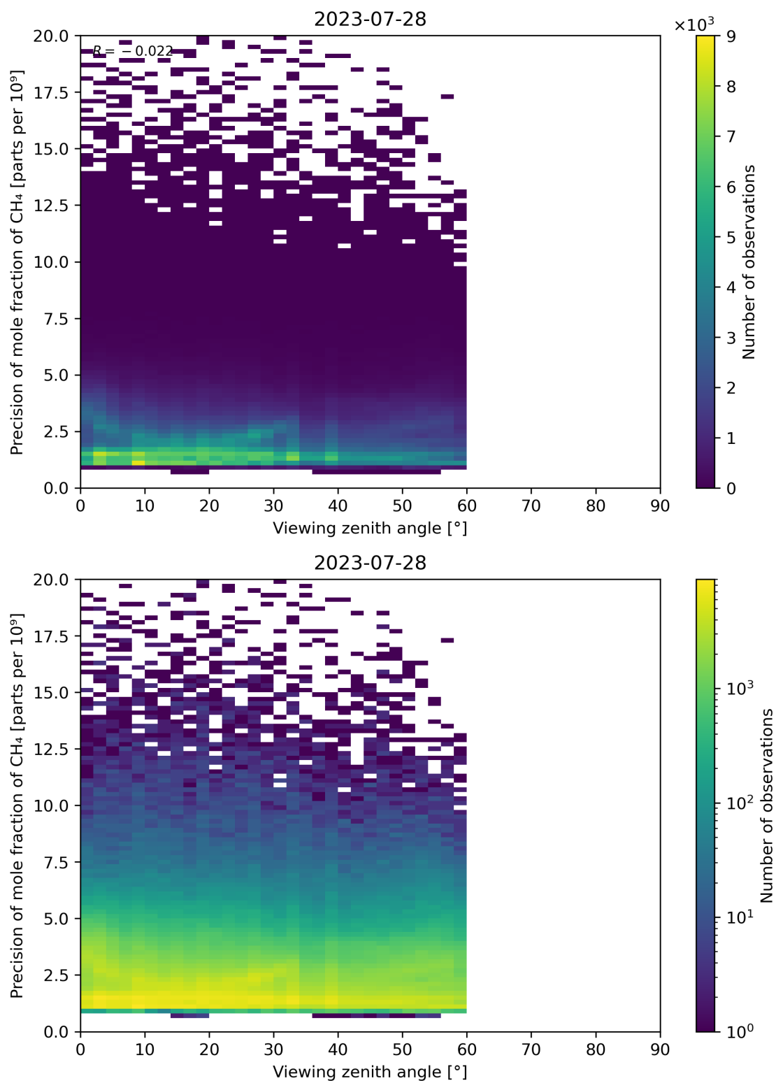
Figure 112: Scatter density plot of “Viewing zenith angle” against “Precision of mole fraction of CH 4 ” for 2023-07-27 to 2023-07-29.
