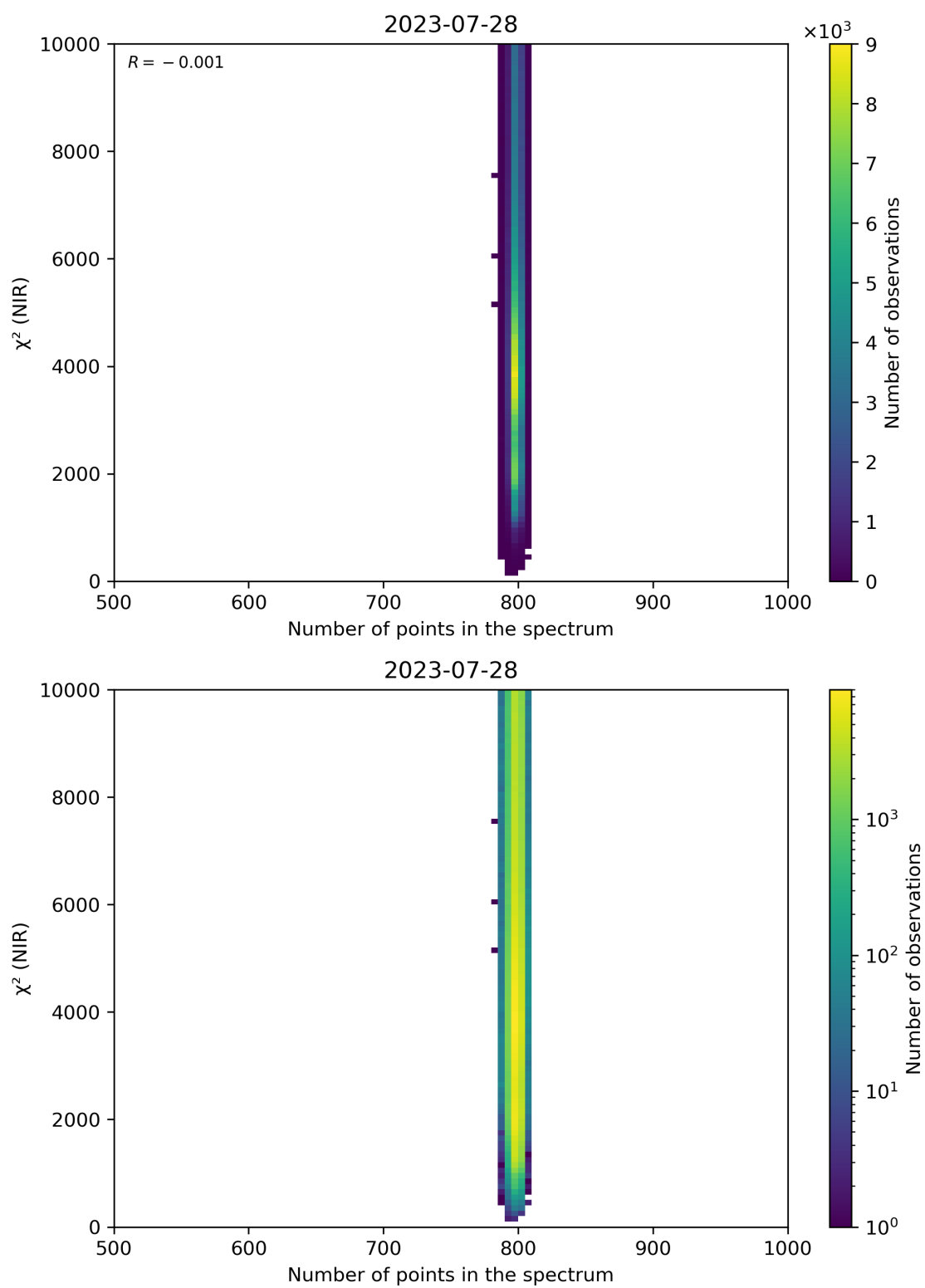
Figure 88: Scatter density plot of “Number of points in the spectrum” against “ \chi^2 (NIR)” for 2023-07-27 to 2023-07-29.
