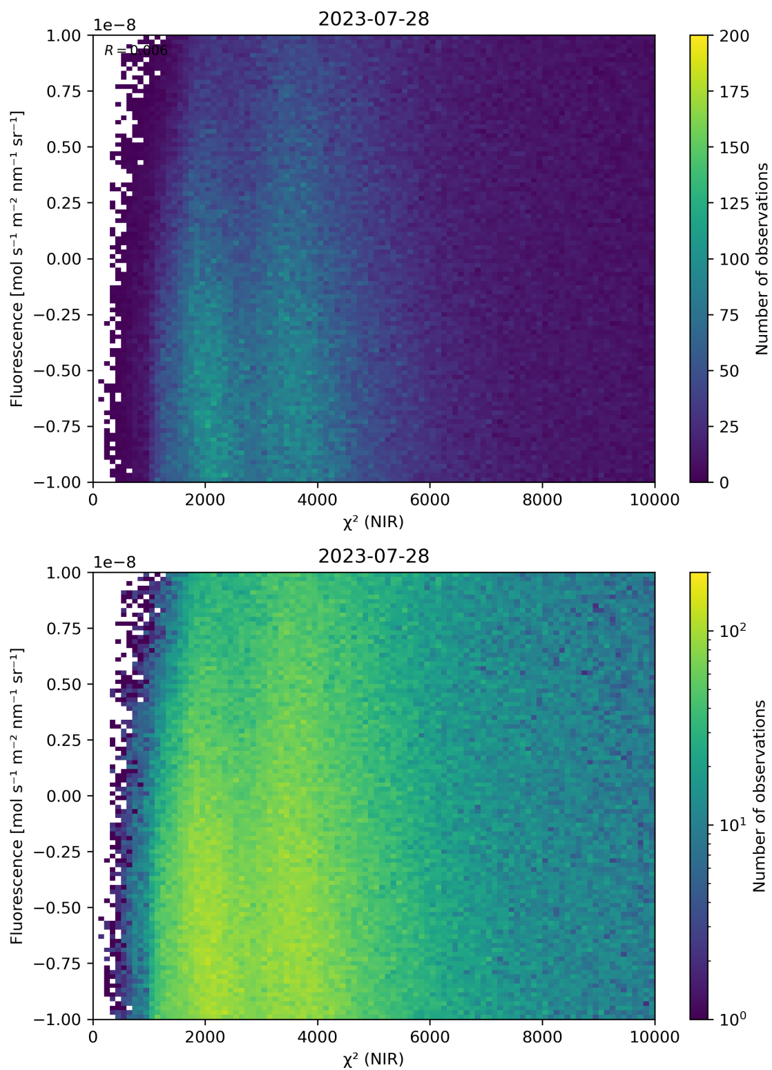
Figure 45: Scatter density plot of “ \chi^2 (NIR)” against “Fluorescence” for 2023-07-27 to 2023-07-29.
