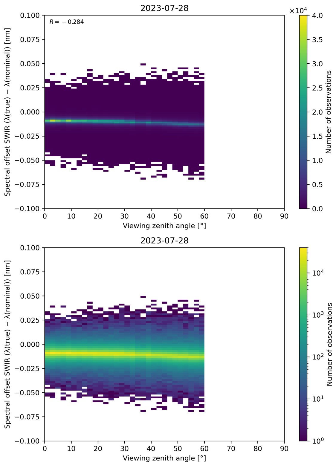
Figure 116: Scatter density plot of “Viewing zenith angle” against “Spectral offset SWIR ( \lambda(\text{true}) - \lambda(\text{nominal}) )” for 2023-07-27 to 2023-07-29.
