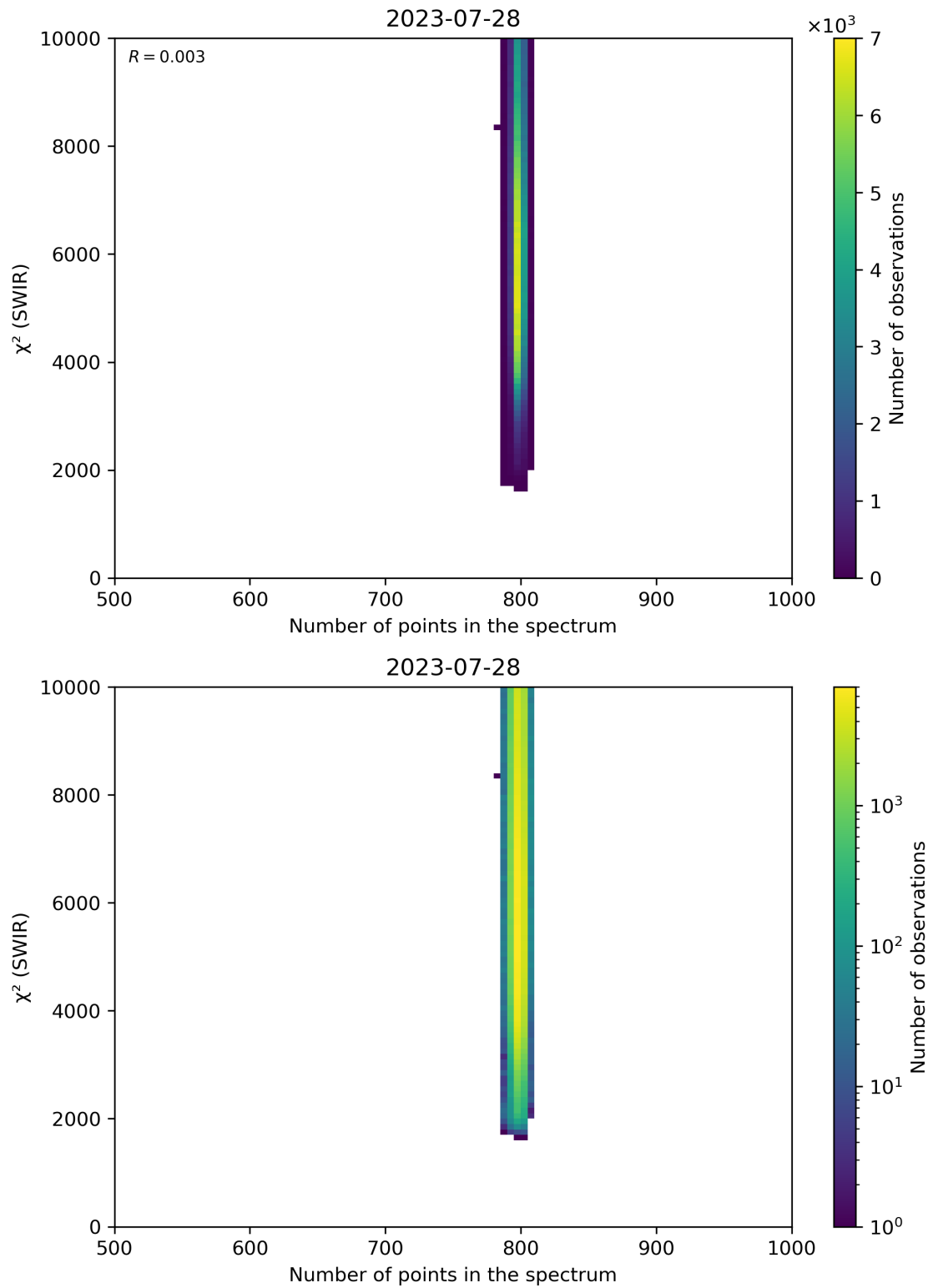
Figure 89: Scatter density plot of “Number of points in the spectrum” against “ \chi^2 (SWIR)” for 2023-07-27 to 2023-07-29.
