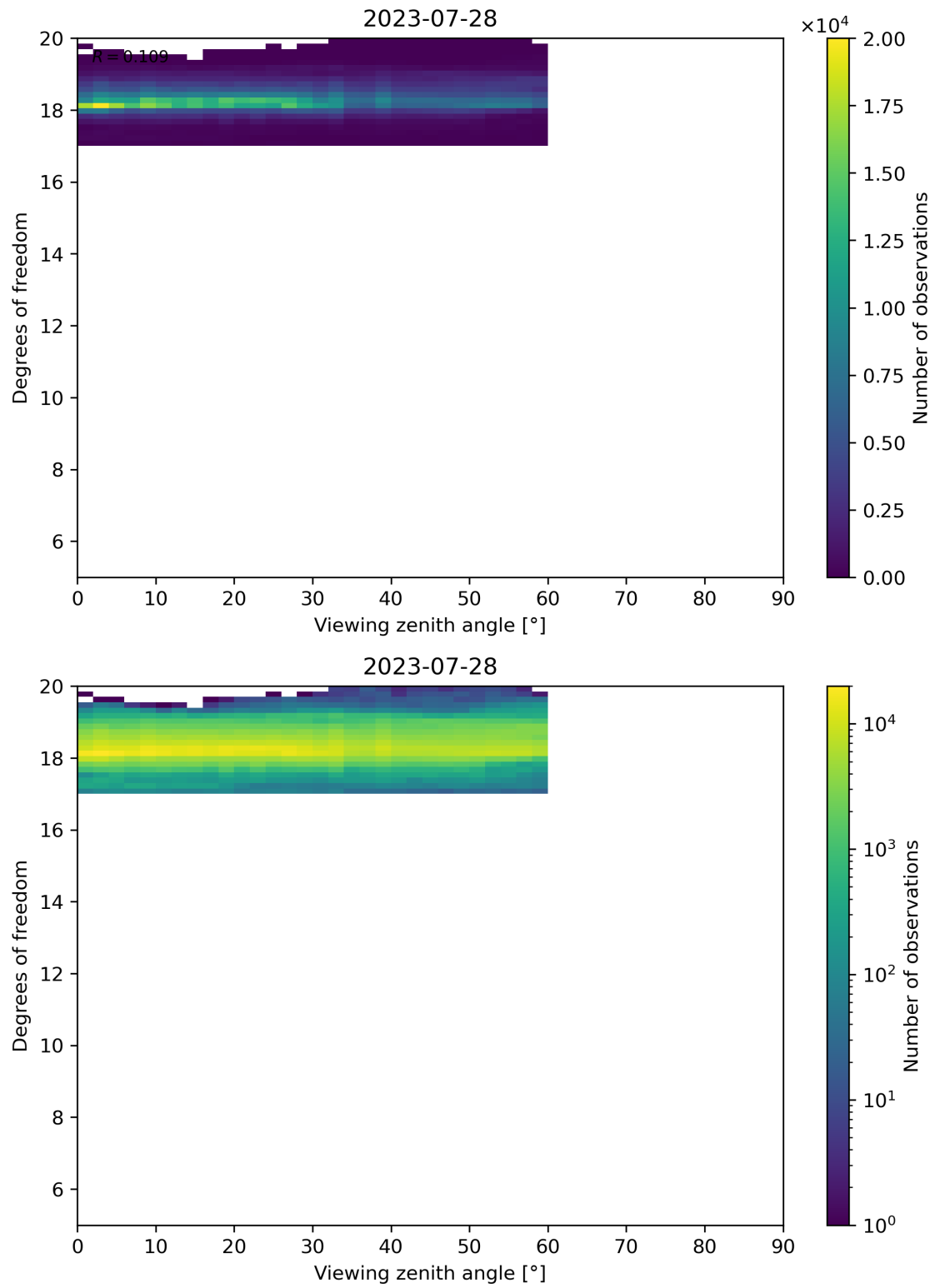
Figure 107: Scatter density plot of “Viewing zenith angle” against “Degrees of freedom” for 2023-07-27 to 2023-07-29.
