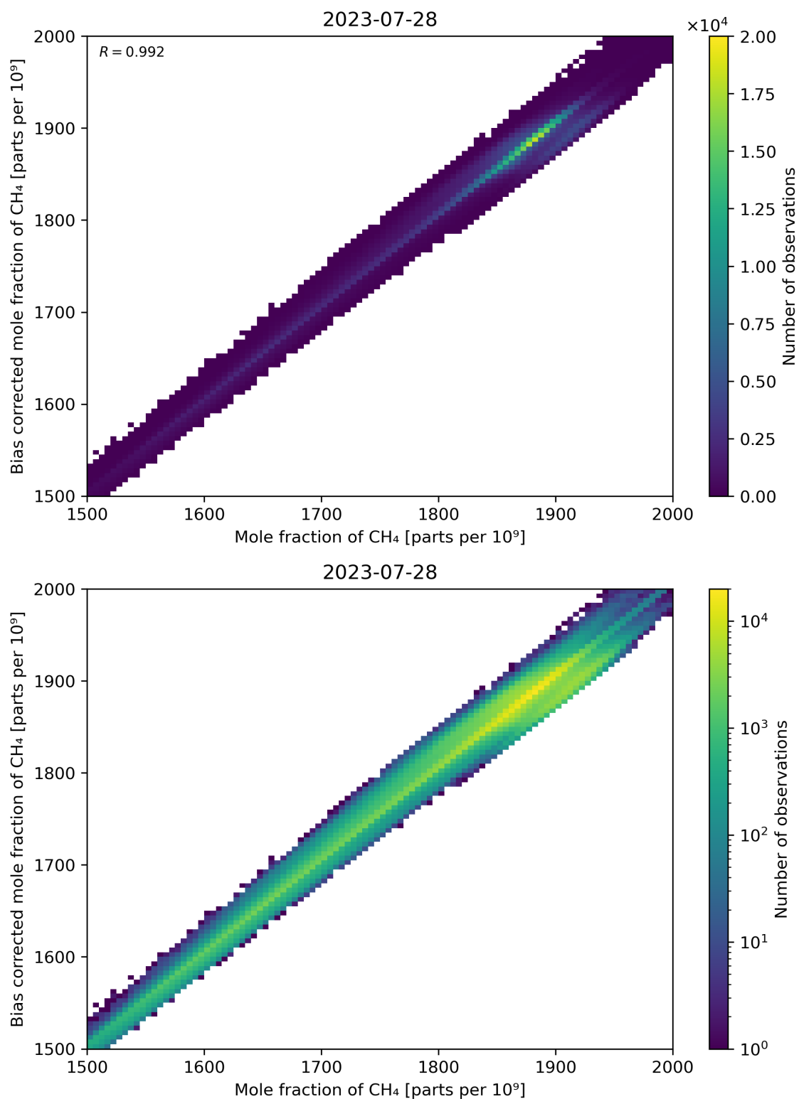
Figure 74: Scatter density plot of “Mole fraction of CH 4 ” against “Bias corrected mole fraction of CH 4 ” for 2023-07-27 to 2023-07-29.
