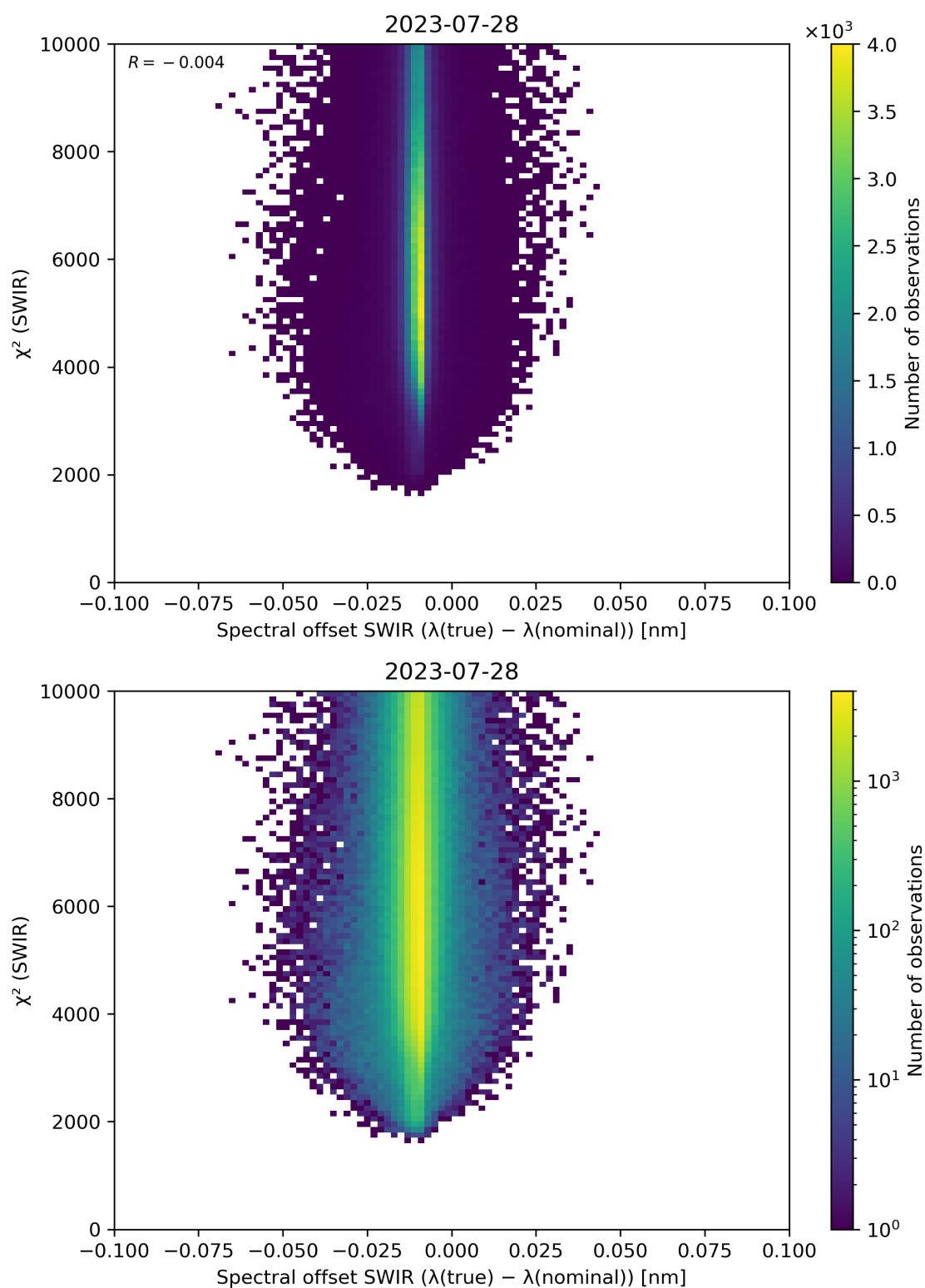
Figure 118: Scatter density plot of “Spectral offset SWIR ( \lambda(\text{true}) - \lambda(\text{nominal}) )” against “ \chi^2 (SWIR)” for 2023-07-27 to 2023-07-29.
