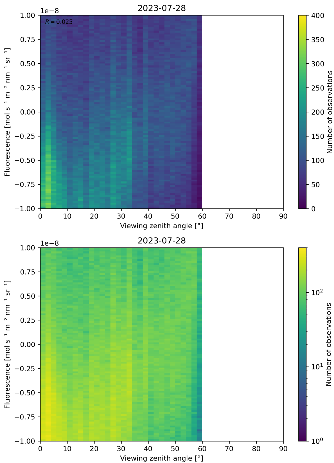
Figure 108: Scatter density plot of “Viewing zenith angle” against “Fluorescence” for 2023-07-27 to 2023-07-29.
