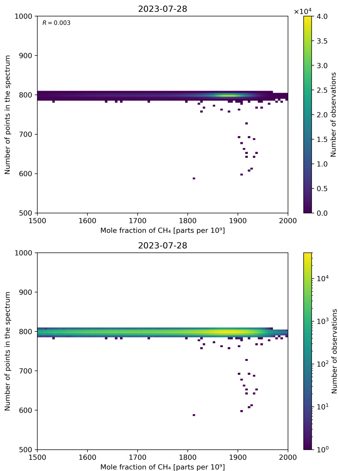
Figure 77: Scatter density plot of “Mole fraction of CH 4 ” against “Number of points in the spectrum” for 2023-07-27 to 2023-07-29.
