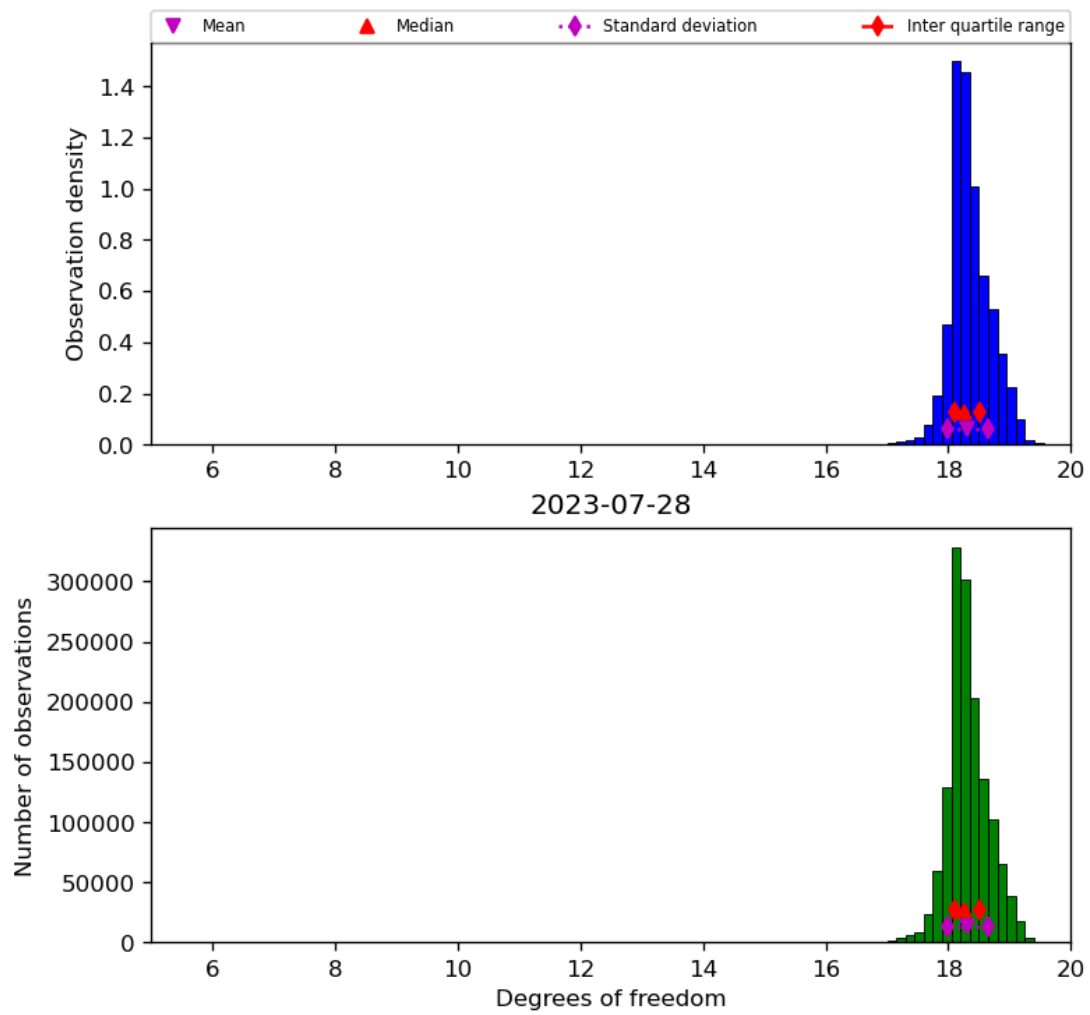
Figure 30: Histogram of “Degrees of freedom” for 2023-07-27 to 2023-07-29
