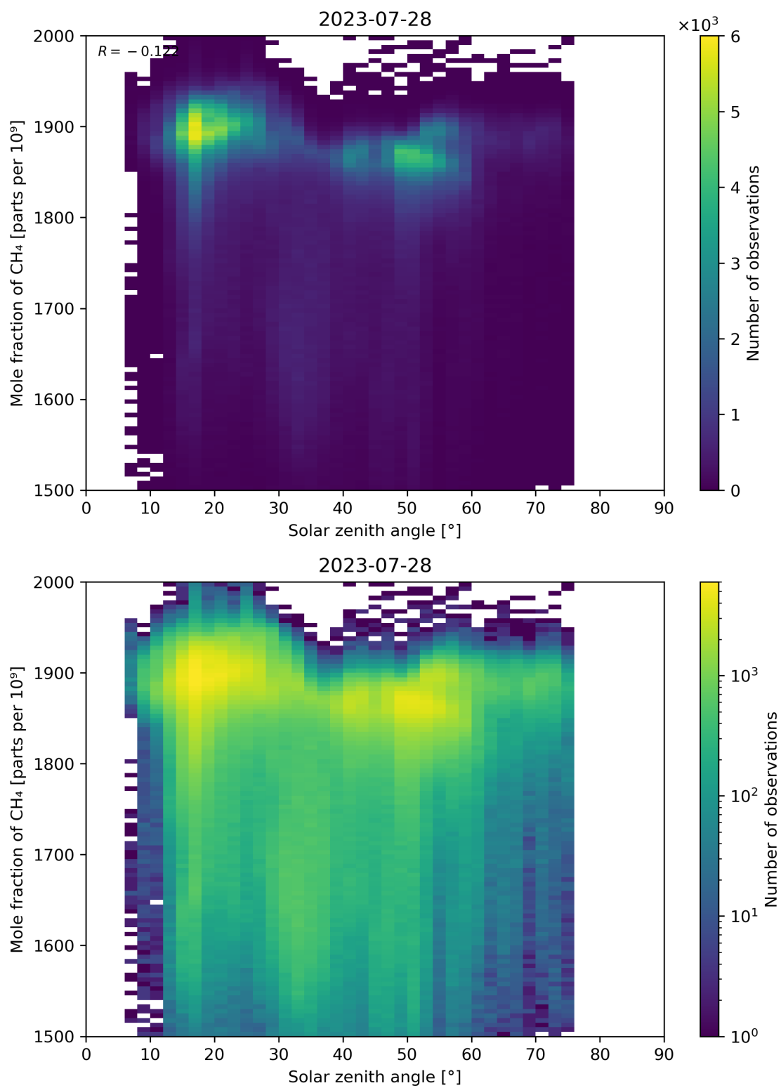
Figure 99: Scatter density plot of “Solar zenith angle” against “Mole fraction of CH 4 ” for 2023-07-27 to 2023-07-29.
