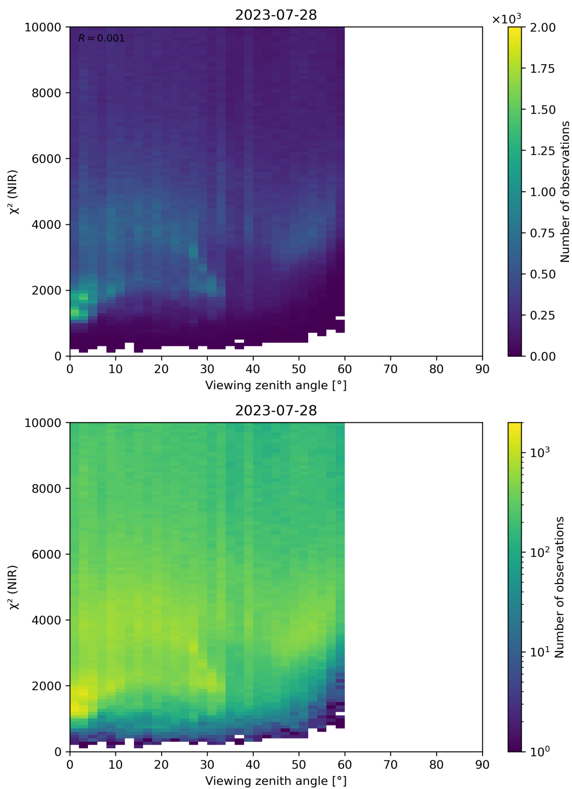
Figure 105: Scatter density plot of “Viewing zenith angle” against “ \chi^2 (NIR)” for 2023-07-27 to 2023-07-29.
