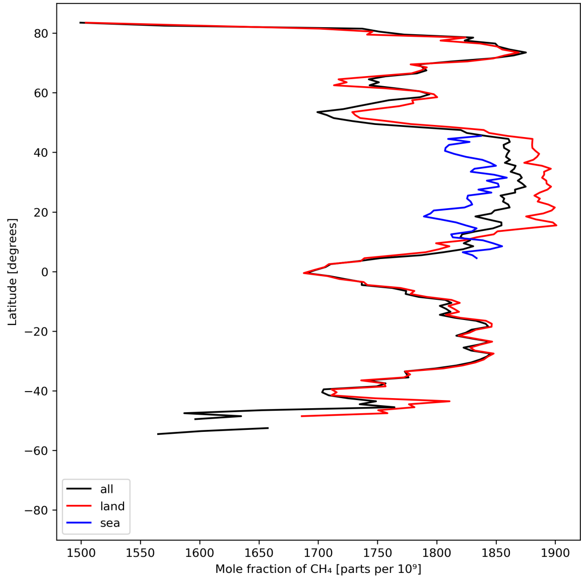
Figure 12: Zonal average of “Mole fraction of \text{CH}_4 ” for 2023-07-27 to 2023-07-29.
