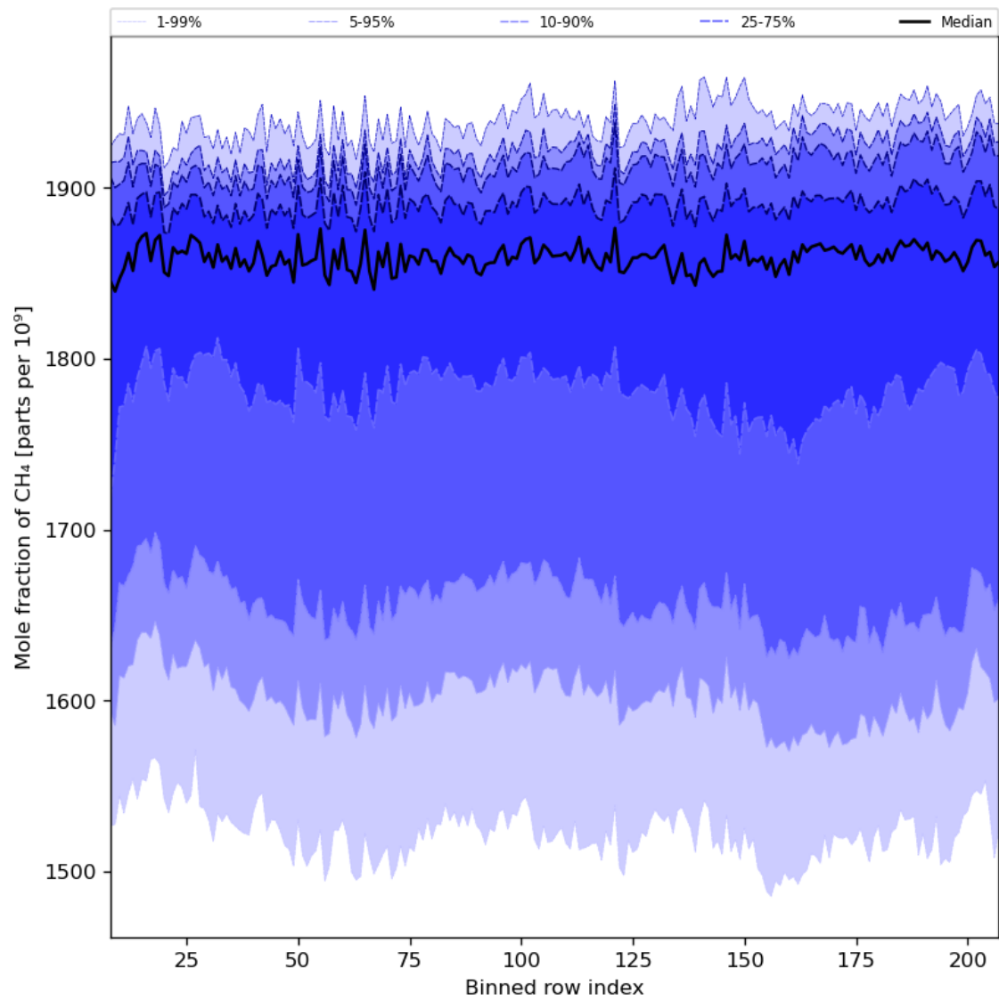
Figure 34: Along track statistics of “Mole fraction of CH 4 ” for 2023-07-27 to 2023-07-29
