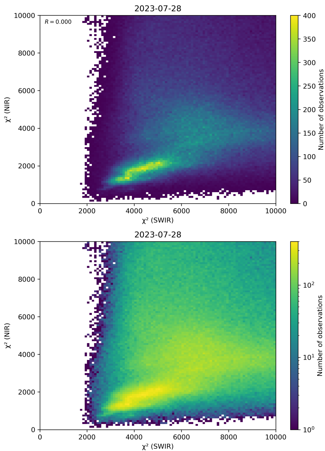
Figure 47: Scatter density plot of “ \chi^2 (SWIR)” against “ \chi^2 (NIR)” for 2023-07-27 to 2023-07-29.
