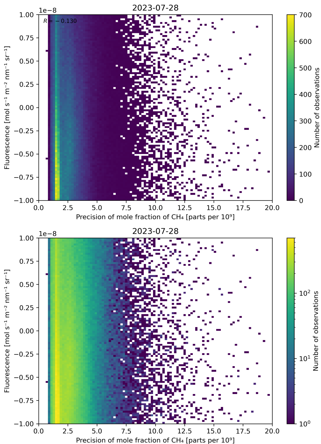
Figure 81: Scatter density plot of “Precision of mole fraction of \text{CH}_4 ” against “Fluorescence” for 2023-07-27 to 2023-07-29.
