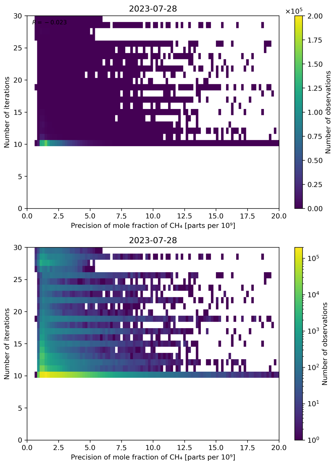
Figure 83: Scatter density plot of “Precision of mole fraction of CH 4 ” against “Number of iterations” for 2023-07-27 to 2023-07-29.
