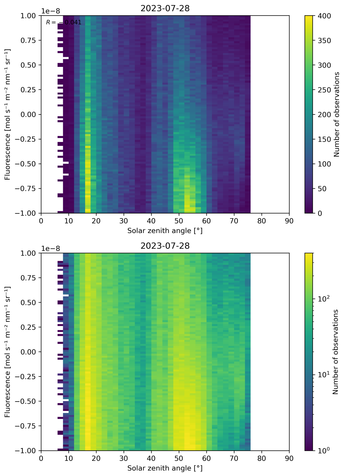
Figure 97: Scatter density plot of “Solar zenith angle” against “Fluorescence” for 2023-07-27 to 2023-07-29.
