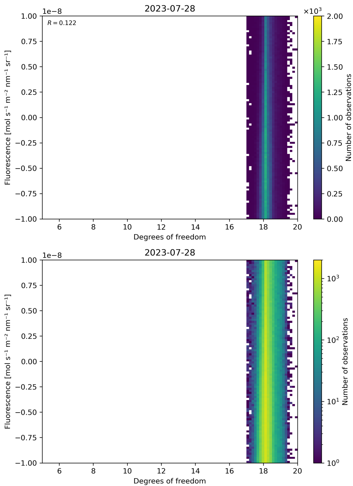
Figure 51: Scatter density plot of “Degrees of freedom” against “Fluorescence” for 2023-07-27 to 2023-07-29.
