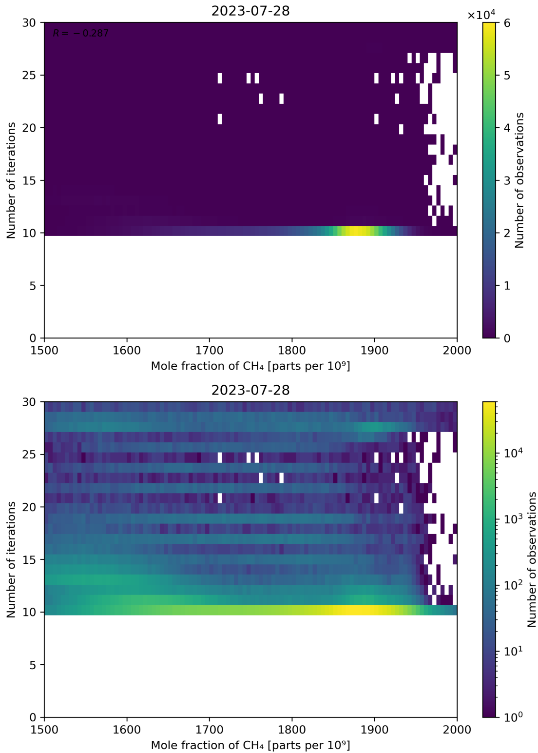
Figure 76: Scatter density plot of “Mole fraction of CH 4 ” against “Number of iterations” for 2023-07-27 to 2023-07-29.
