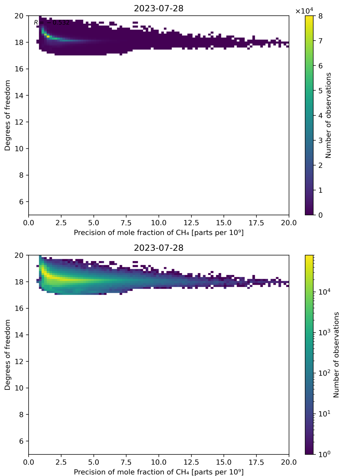
Figure 80: Scatter density plot of “Precision of mole fraction of CH 4 ” against “Degrees of freedom” for 2023-07-27 to 2023-07-29.
