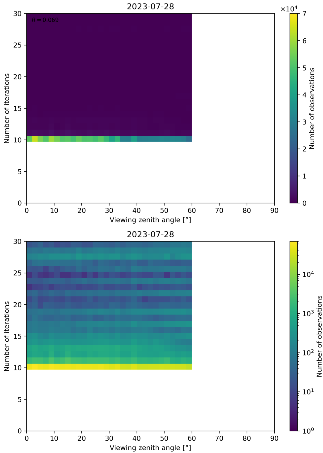
Figure 113: Scatter density plot of “Viewing zenith angle” against “Number of iterations” for 2023-07-27 to 2023-07-29.
