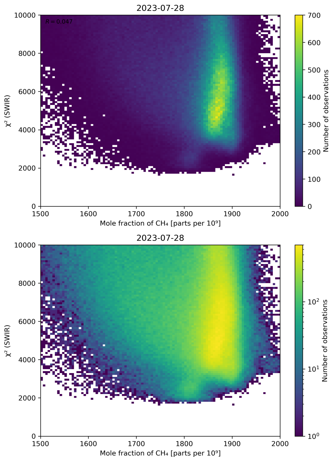
Figure 71: Scatter density plot of “Mole fraction of \text{CH}_4 ” against “ \chi^2 (SWIR)” for 2023-07-27 to 2023-07-29.
