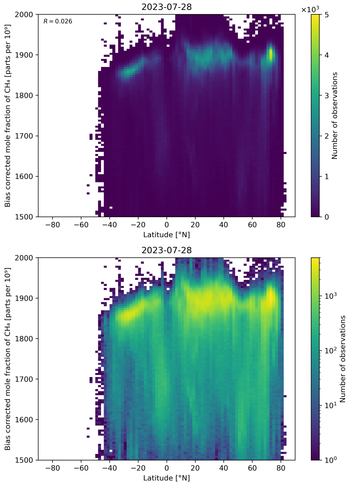
Figure 58: Scatter density plot of “Latitude” against “Bias corrected mole fraction of \text{CH}_4 ” for 2023-07-27 to 2023-07-29.
