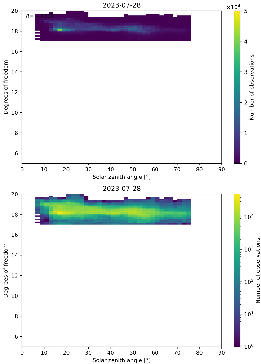
Figure 96: Scatter density plot of “Solar zenith angle” against “Degrees of freedom” for 2023-07-27 to 2023-07-29.
