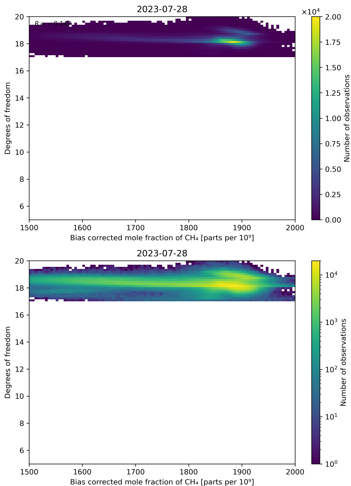
Figure 65: Scatter density plot of “Bias corrected mole fraction of CH 4 ” against “Degrees of freedom” for 2023-07-27 to 2023-07-29.
