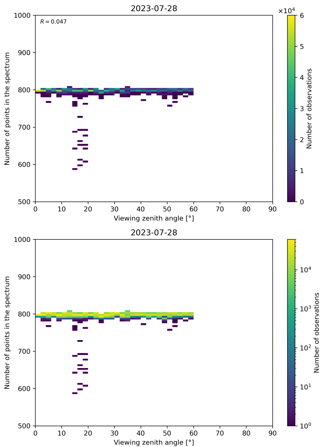
Figure 114: Scatter density plot of “Viewing zenith angle” against “Number of points in the spectrum” for 2023-07-27 to 2023-07-29.
