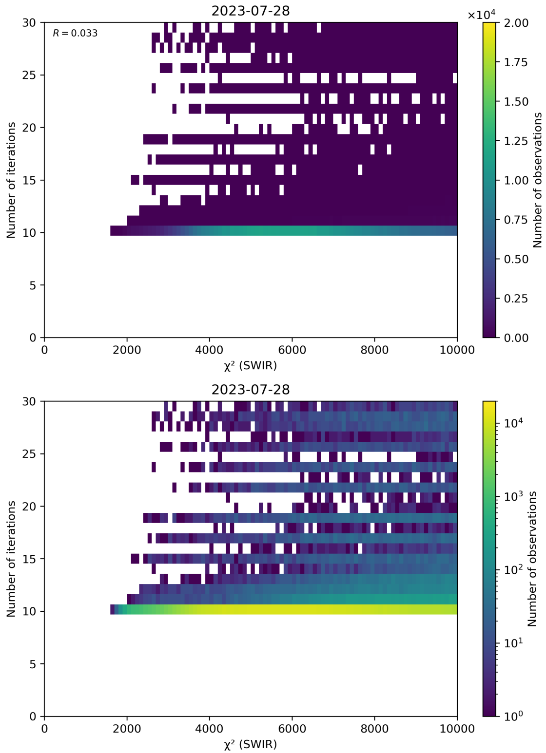
Figure 50: Scatter density plot of “ \chi^2 (SWIR)” against “Number of iterations” for 2023-07-27 to 2023-07-29.
