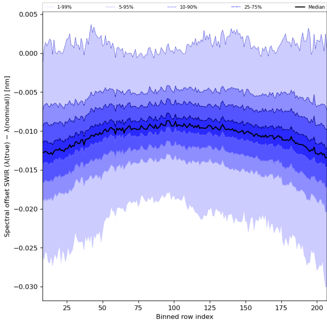
Figure 38: Along track statistics of “Spectral offset SWIR ( \lambda(\text{true}) - \lambda(\text{nominal}) )” for 2023-07-27 to 2023-07-29
