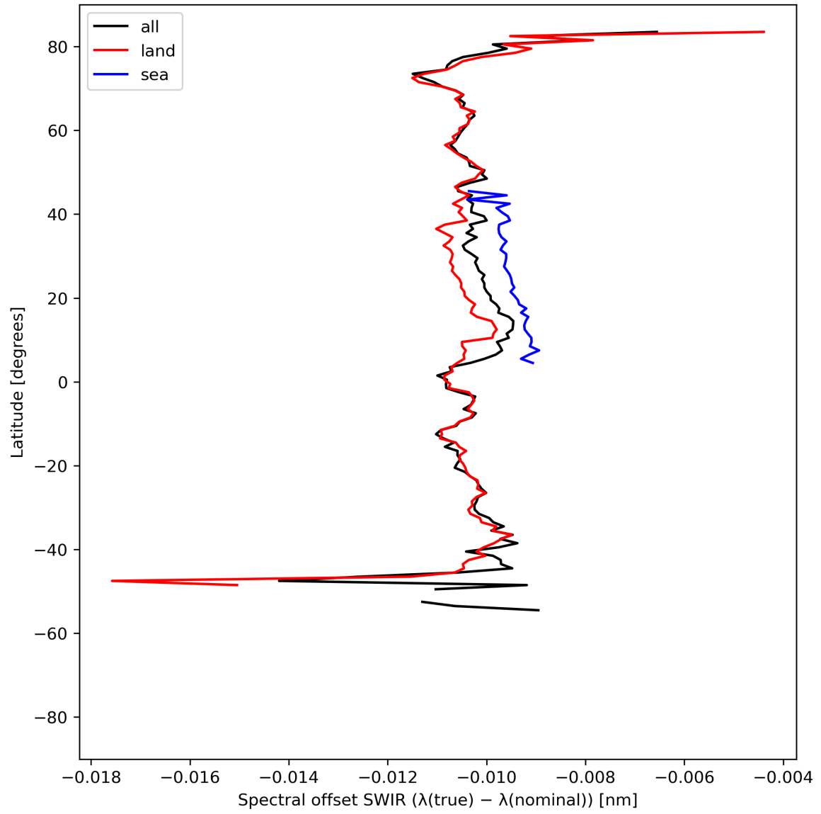
Figure 16: Zonal average of “Spectral offset SWIR ( \lambda(\text{true}) - \lambda(\text{nominal}) )” for 2023-07-27 to 2023-07-29.
