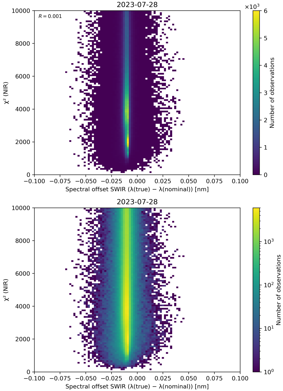
Figure 117: Scatter density plot of “Spectral offset SWIR ( \lambda(\text{true}) - \lambda(\text{nominal}) )” against “ \chi^2 (NIR)” for 2023-07-27 to 2023-07-29.
