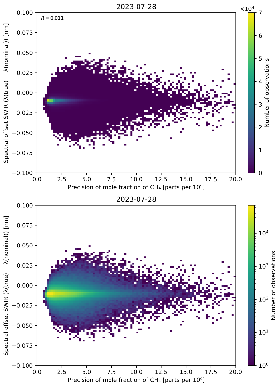
Figure 85: Scatter density plot of “Precision of mole fraction of CH 4 ” against “Spectral offset SWIR ( \lambda(\text{true}) - \lambda(\text{nominal}) )” for 2023-07-27 to 2023-07-29.
