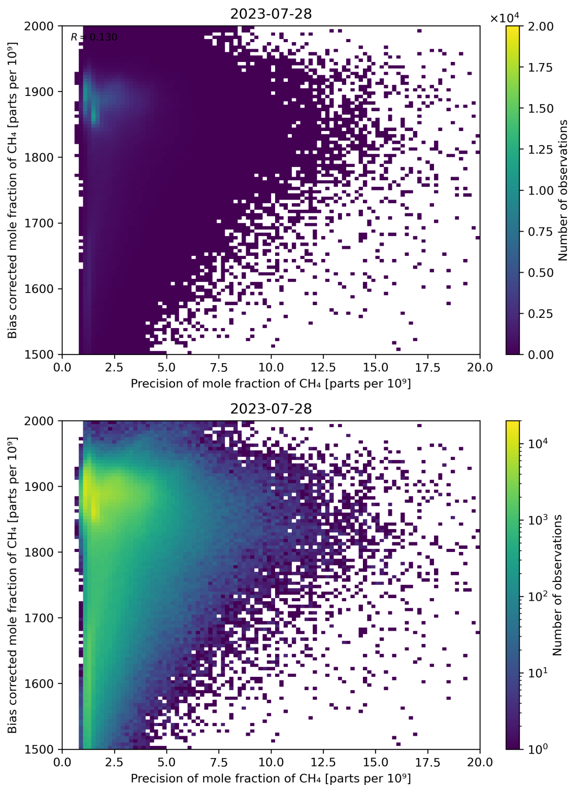
Figure 82: Scatter density plot of “Precision of mole fraction of CH 4 ” against “Bias corrected mole fraction of CH 4 ” for 2023-07-27 to 2023-07-29.
