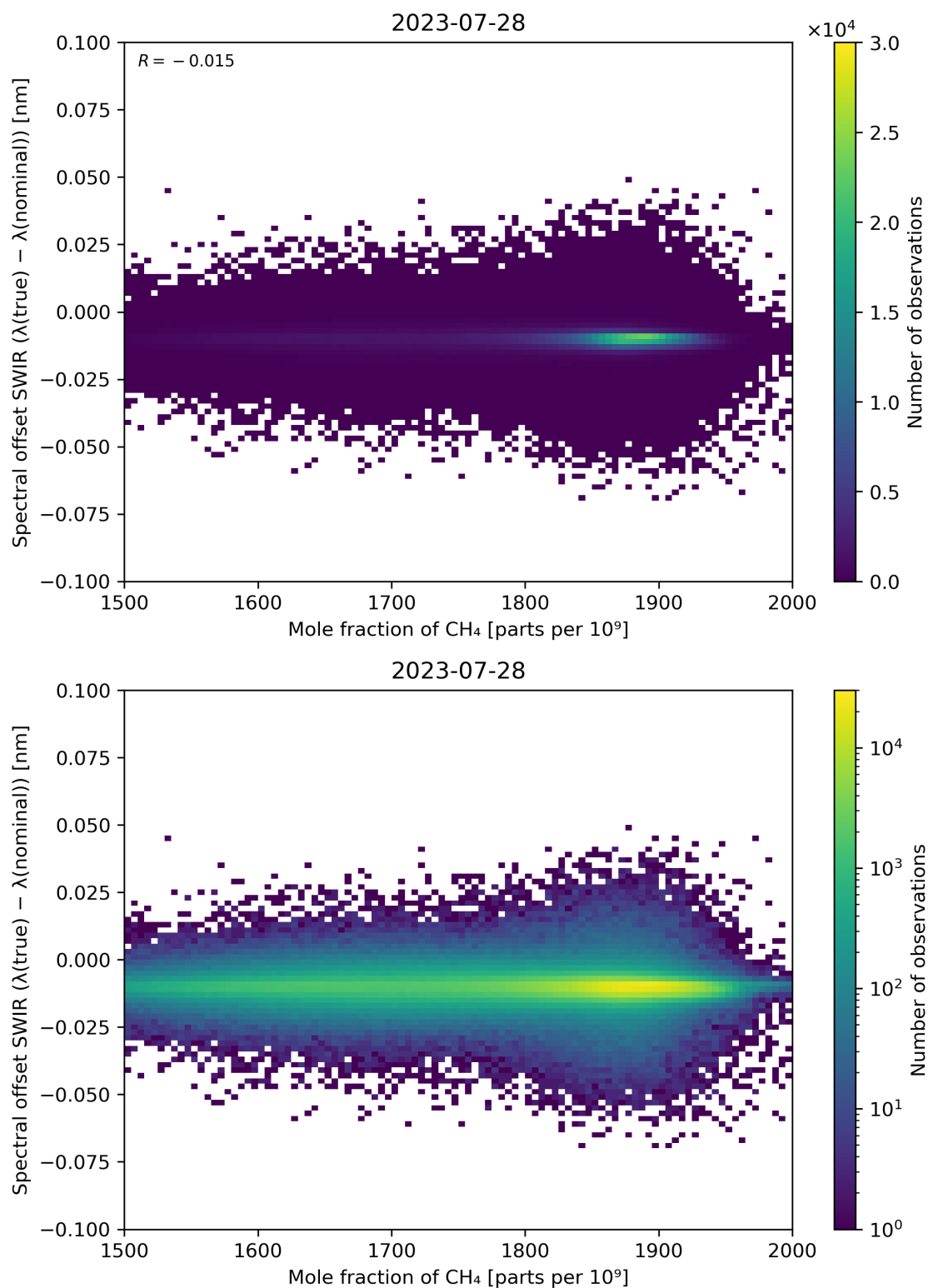
Figure 86: Scatter density plot of “Mole fraction of CH 4 ” against “Spectral offset SWIR ( \lambda(\text{true}) - \lambda(\text{nominal}) )” for 2023-07-27 to 2023-07-29.
