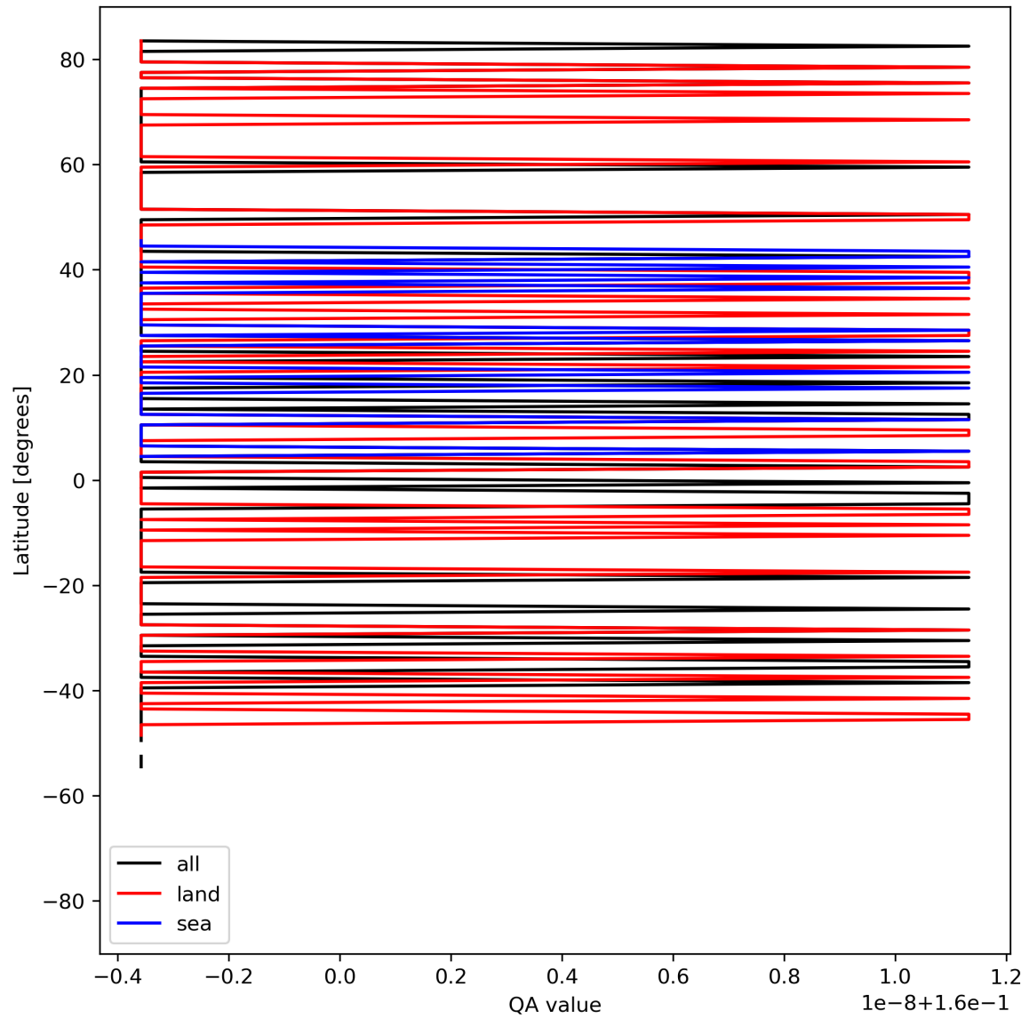
Figure 11: Zonal average of “QA value” for 2023-07-27 to 2023-07-29.
