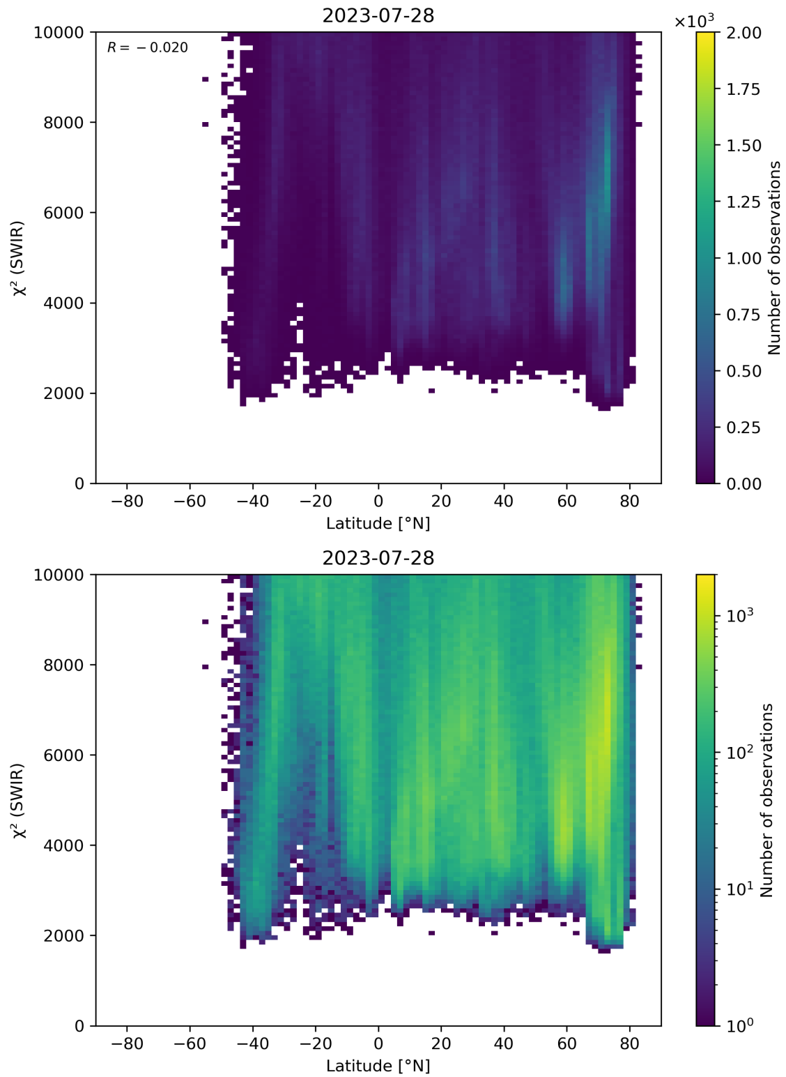
Figure 54: Scatter density plot of “Latitude” against “ \chi^2 (SWIR)” for 2023-07-27 to 2023-07-29.
