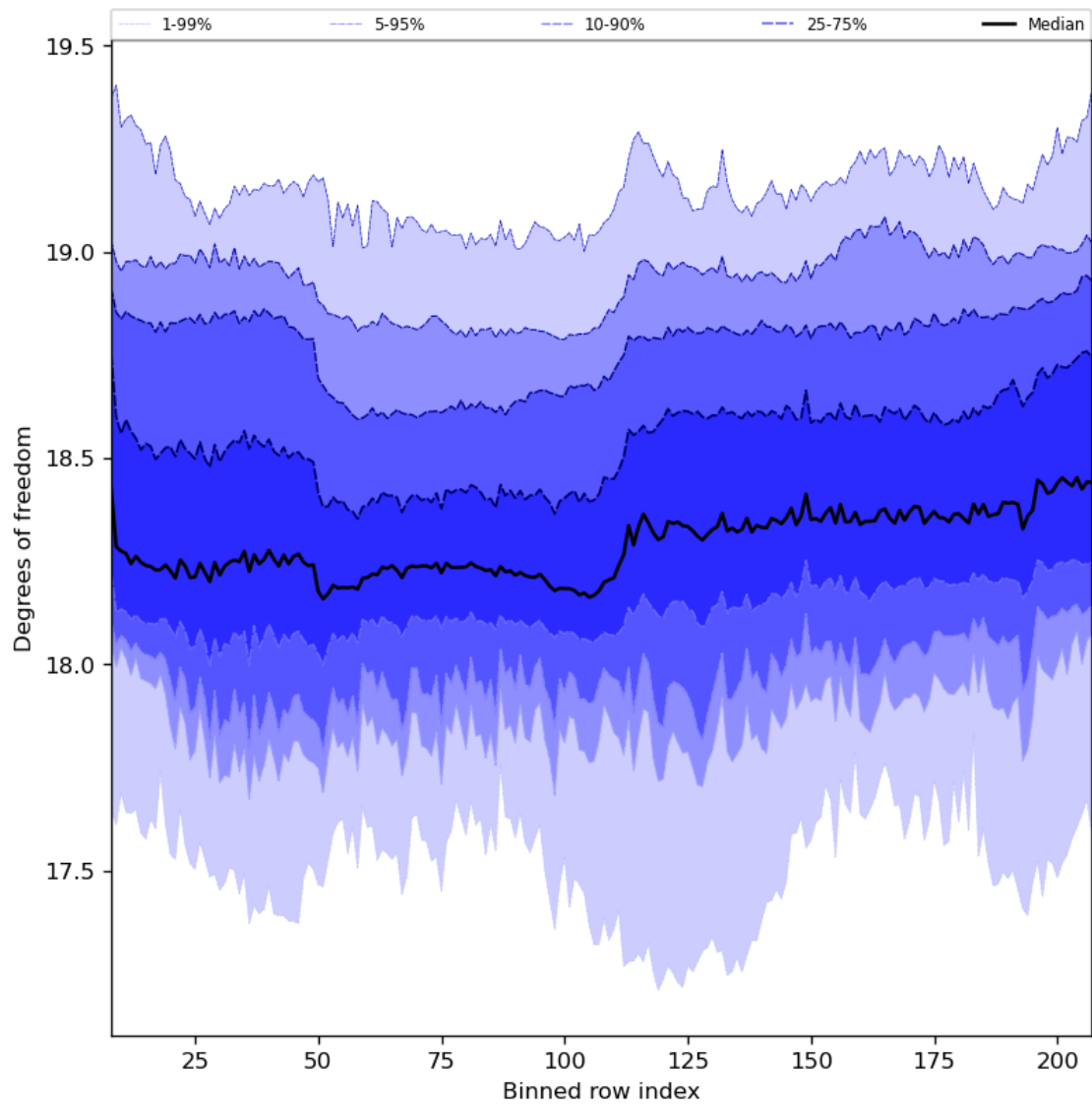
Figure 41: Along track statistics of “Degrees of freedom” for 2023-07-27 to 2023-07-29
