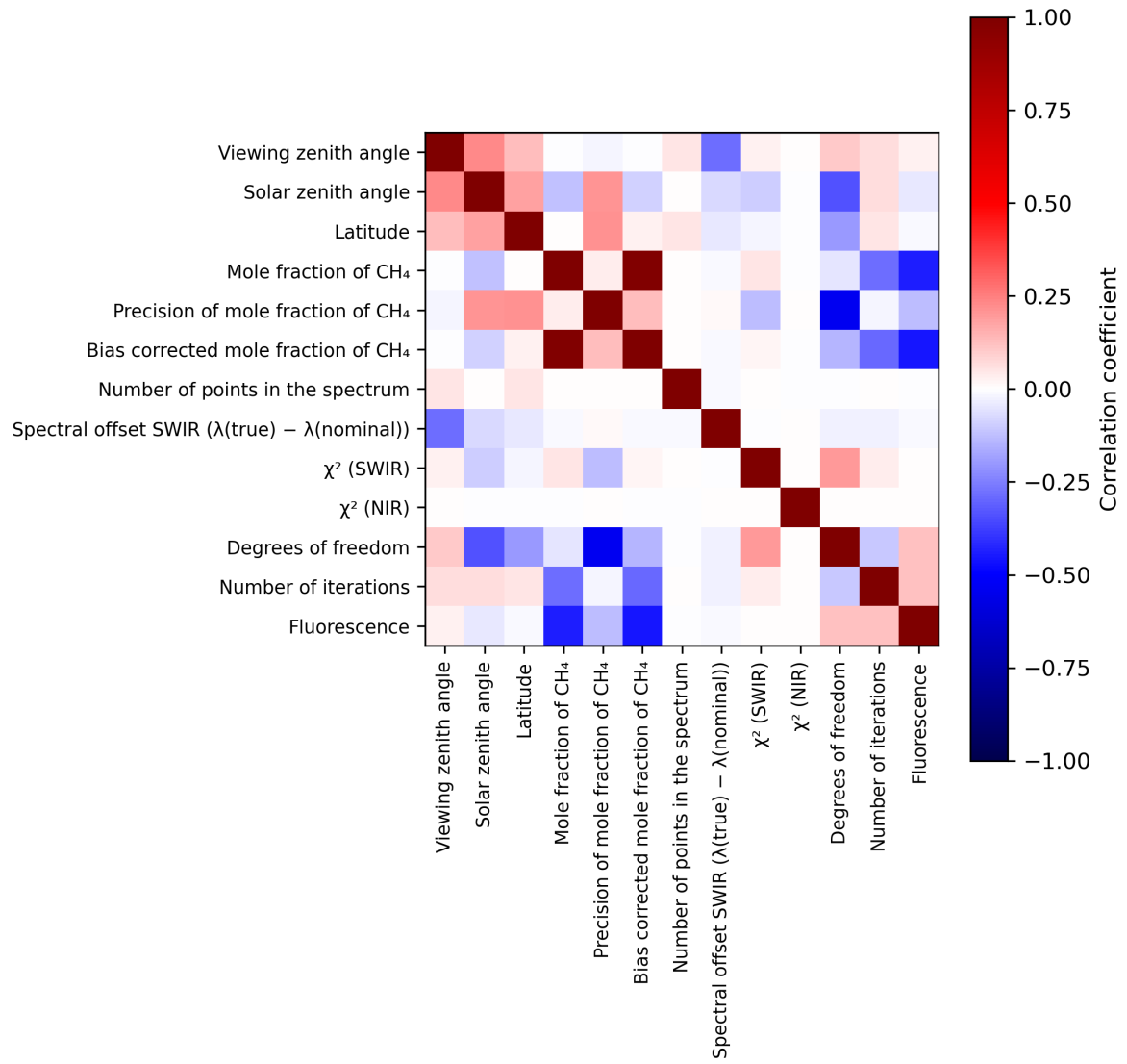
Figure 2: Map of correlation matrix for 2023-07-27 to 2023-07-29.
