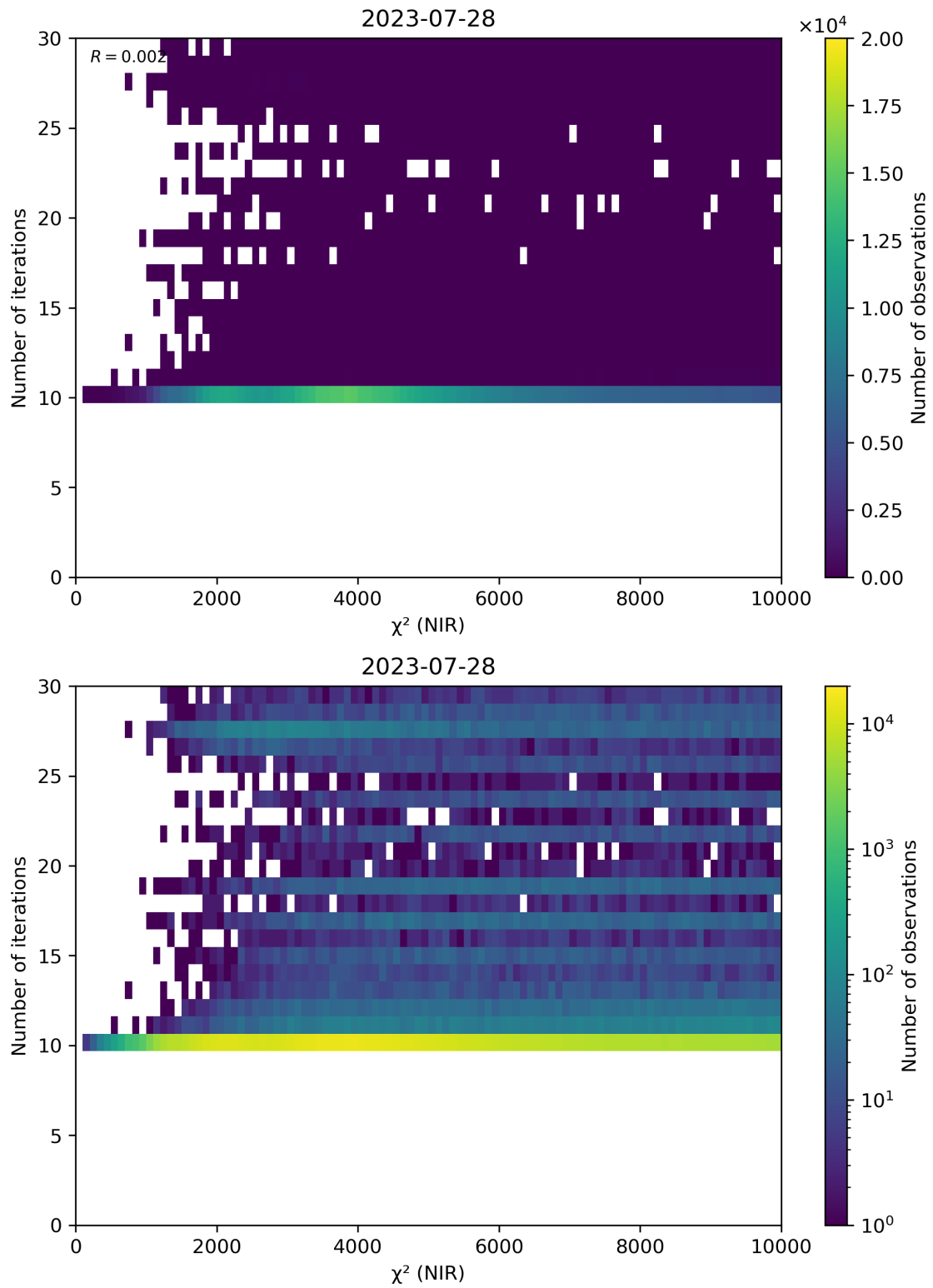
Figure 46: Scatter density plot of “ \chi^2 (NIR)” against “Number of iterations” for 2023-07-27 to 2023-07-29.
