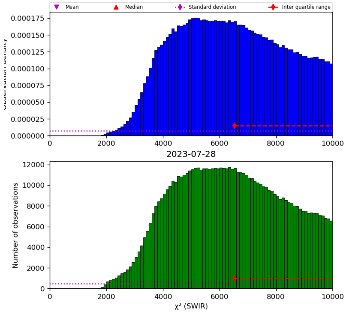
Figure 28: Histogram of “ \chi^2 (SWIR)” for 2023-07-27 to 2023-07-29
