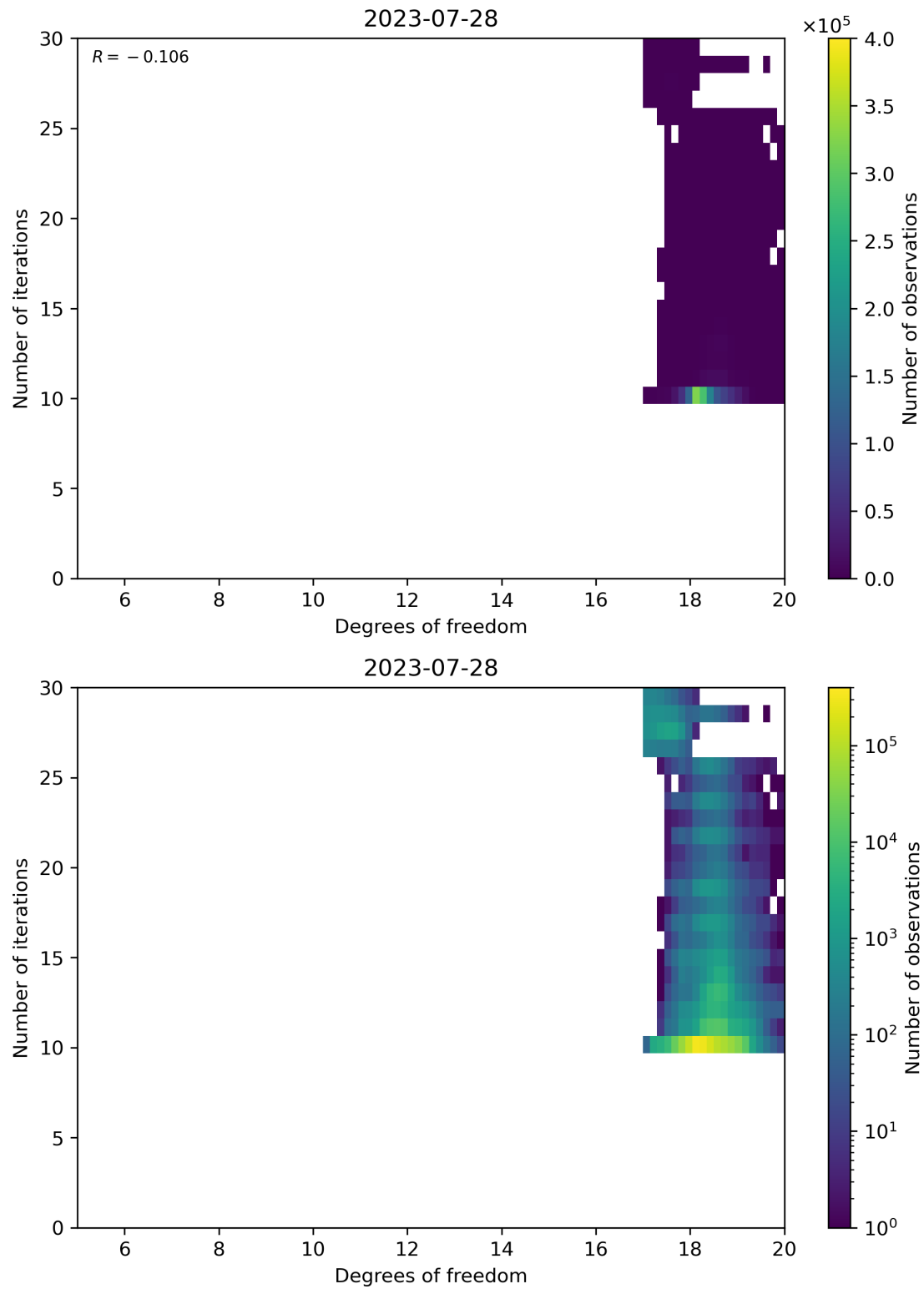
Figure 52: Scatter density plot of “Degrees of freedom” against “Number of iterations” for 2023-07-27 to 2023-07-29.
