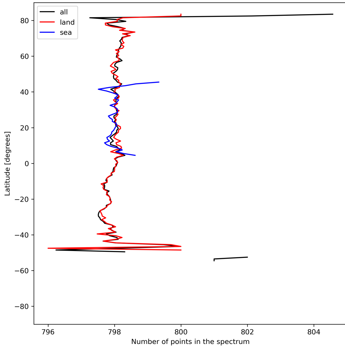
Figure 15: Zonal average of “Number of points in the spectrum” for 2023-07-27 to 2023-07-29.
