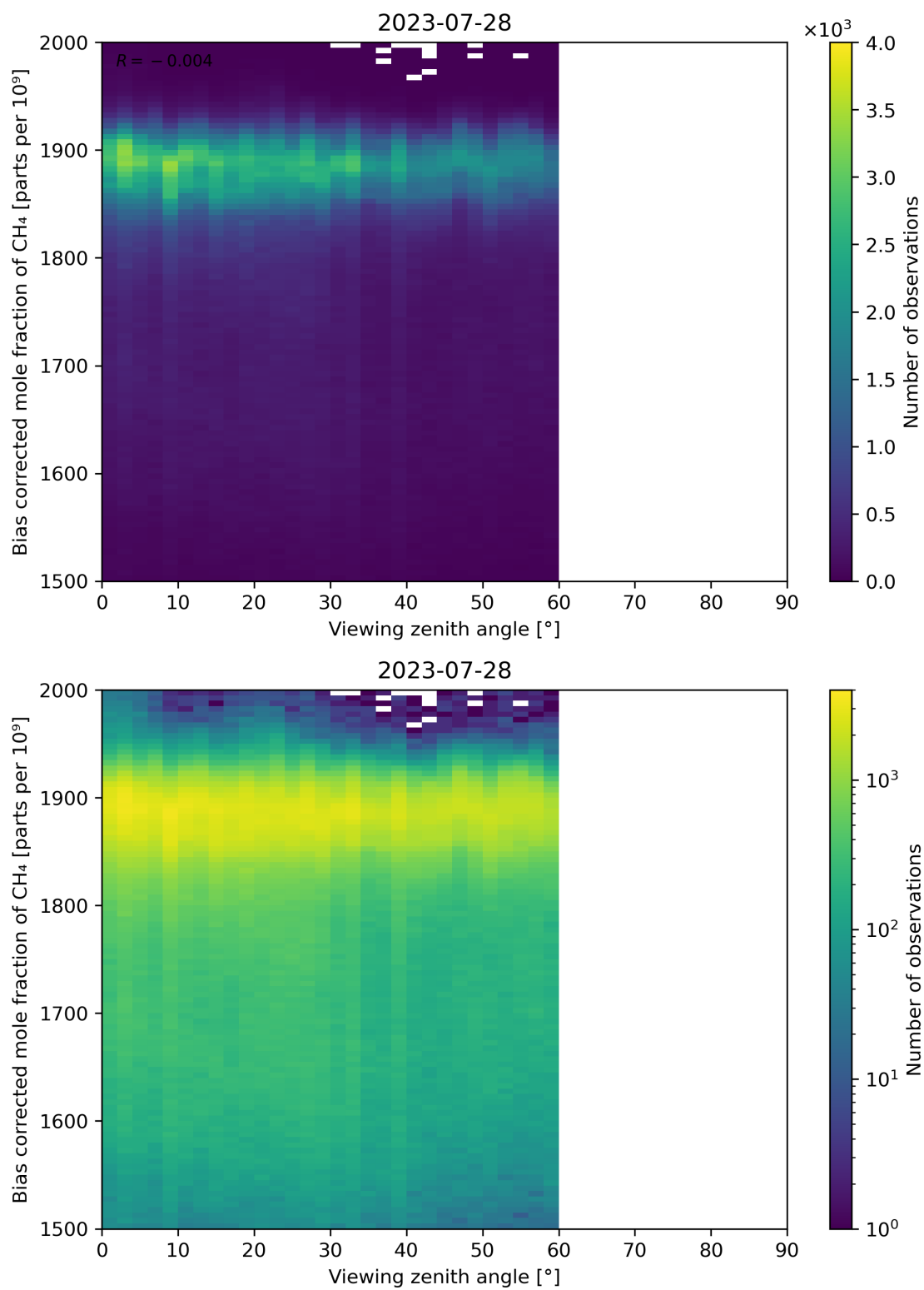
Figure 111: Scatter density plot of “Viewing zenith angle” against “Bias corrected mole fraction of CH 4 ” for 2023-07-27 to 2023-07-29.
