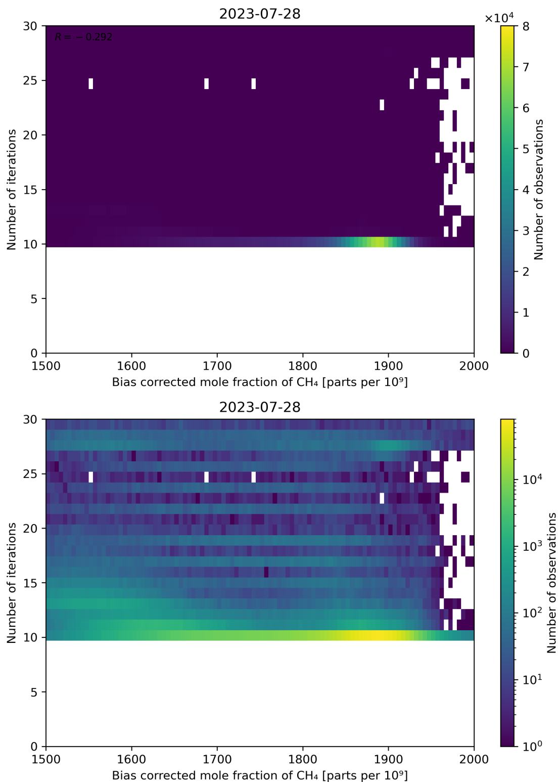
Figure 67: Scatter density plot of “Bias corrected mole fraction of CH 4 ” against “Number of iterations” for 2023-07-27 to 2023-07-29.
