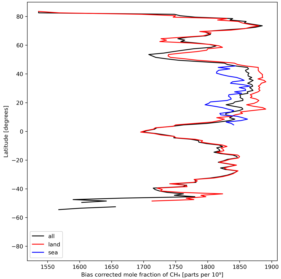
Figure 14: Zonal average of “Bias corrected mole fraction of \text{CH}_4 ” for 2023-07-27 to 2023-07-29.
