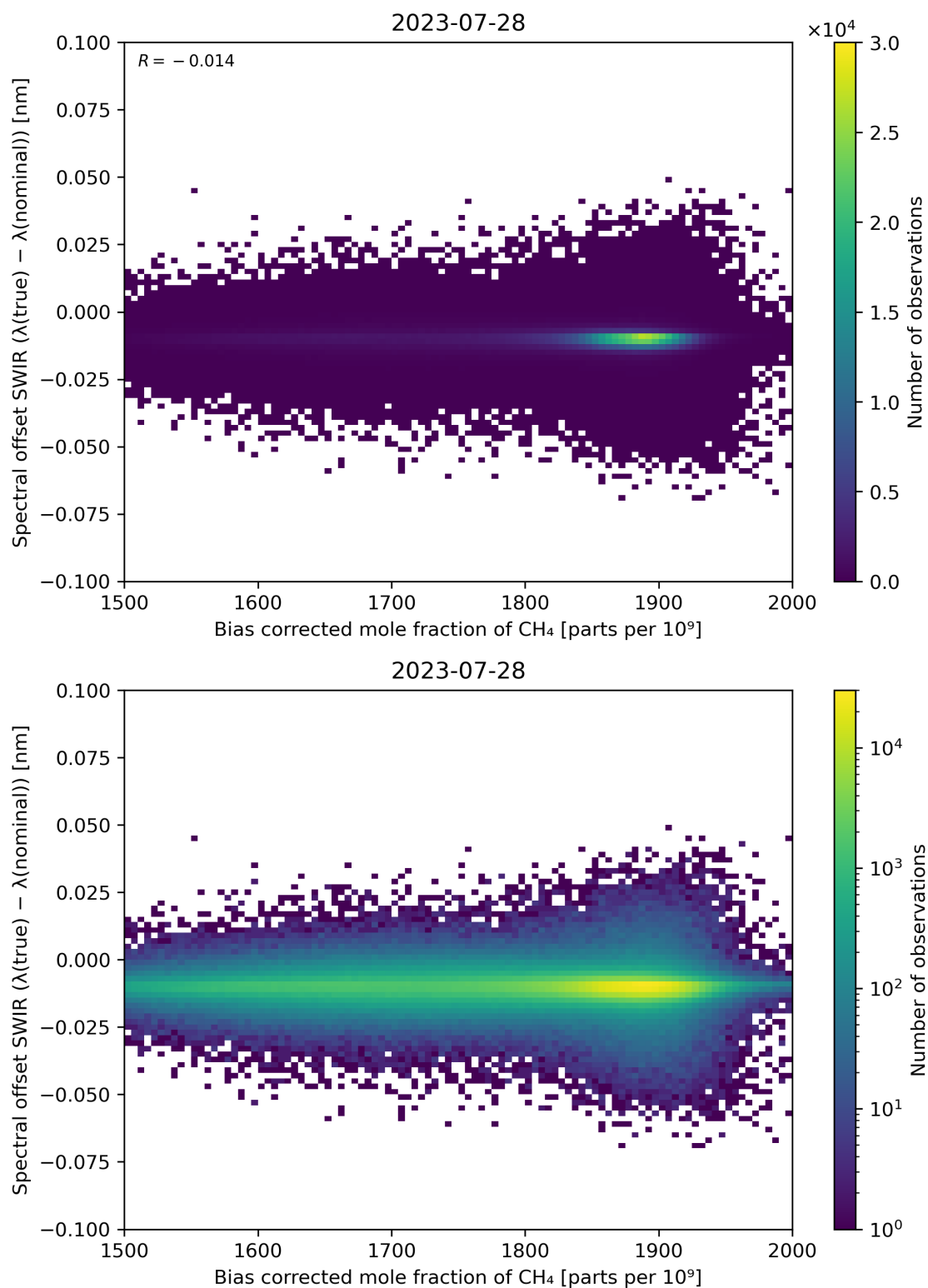
Figure 69: Scatter density plot of “Bias corrected mole fraction of \text{CH}_4 ” against “Spectral offset SWIR ( \lambda(\text{true}) - \lambda(\text{nominal}) )” for 2023-07-27 to 2023-07-29.
