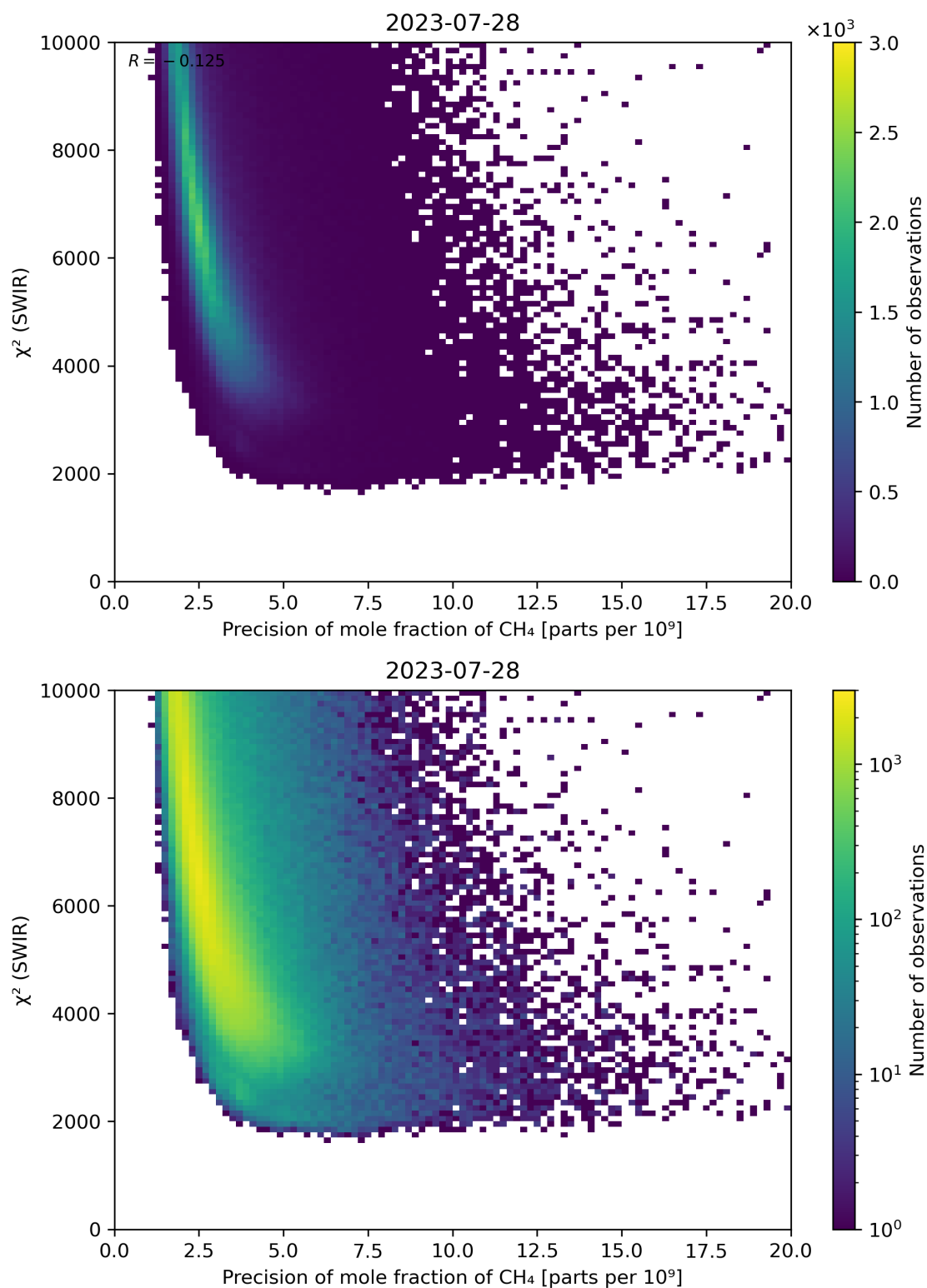
Figure 79: Scatter density plot of “Precision of mole fraction of \text{CH}_4 ” against “ \chi^2 (SWIR)” for 2023-07-27 to 2023-07-29.
