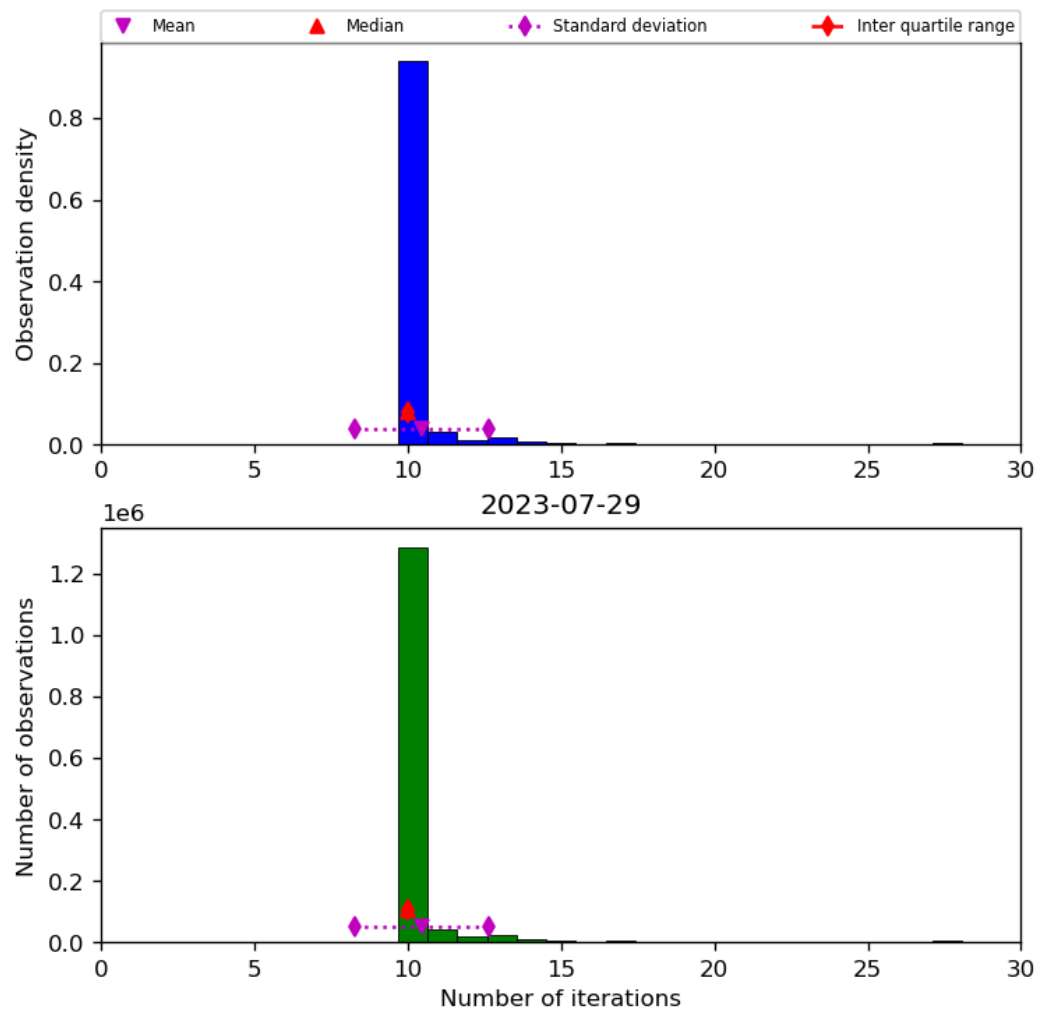
Figure 31: Histogram of “Number of iterations” for 2023-07-29 to 2023-07-30
