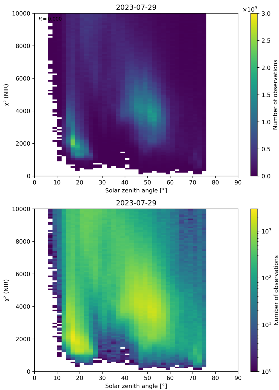
Figure 94: Scatter density plot of “Solar zenith angle” against “ \chi^2 (NIR)” for 2023-07-29 to 2023-07-30.
