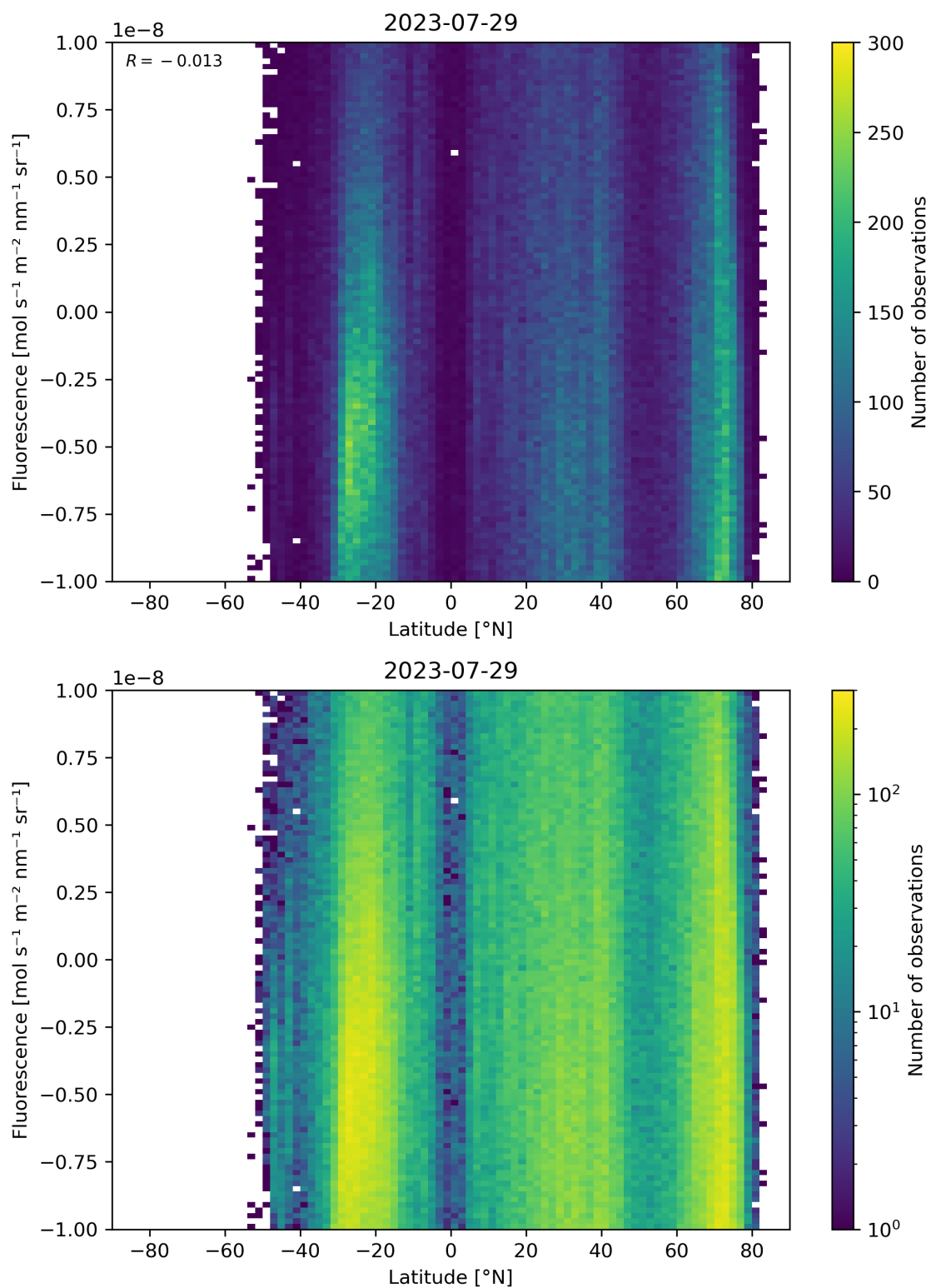
Figure 56: Scatter density plot of “Latitude” against “Fluorescence” for 2023-07-29 to 2023-07-30.
