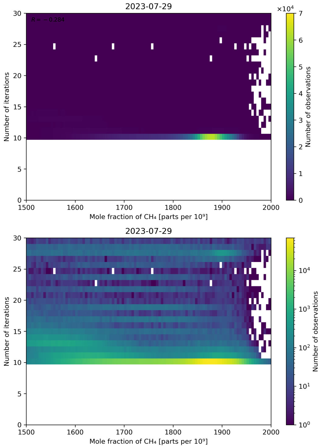
Figure 76: Scatter density plot of “Mole fraction of CH 4 ” against “Number of iterations” for 2023-07-29 to 2023-07-30.
