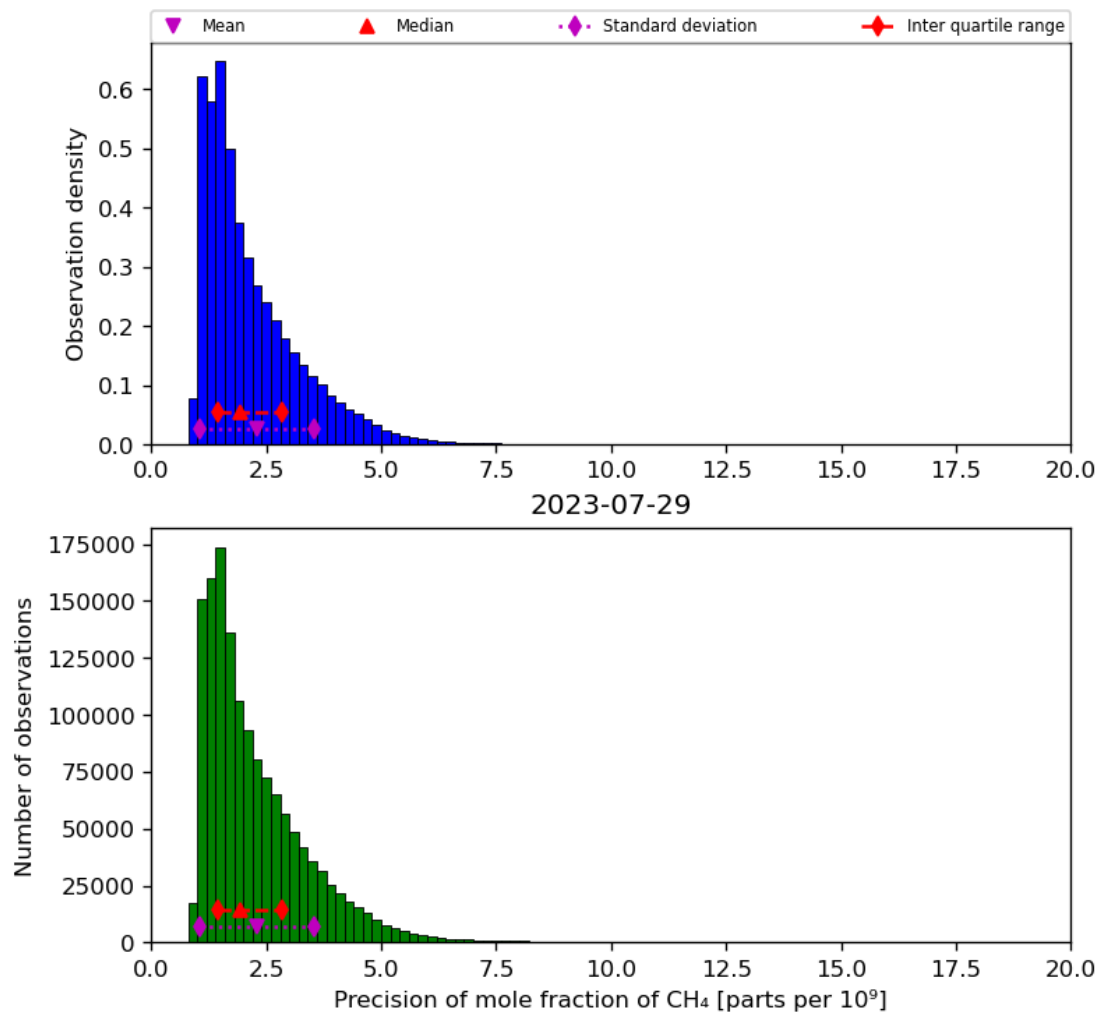
Figure 24: Histogram of “Precision of mole fraction of CH 4 ” for 2023-07-29 to 2023-07-30
