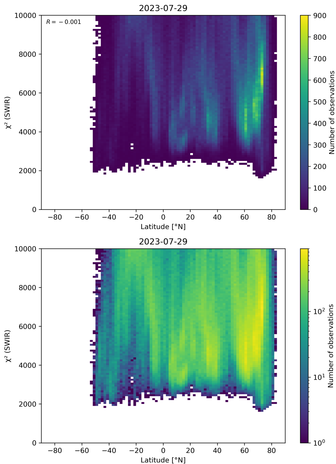
Figure 54: Scatter density plot of “Latitude” against “ \chi^2 (SWIR)” for 2023-07-29 to 2023-07-30.
