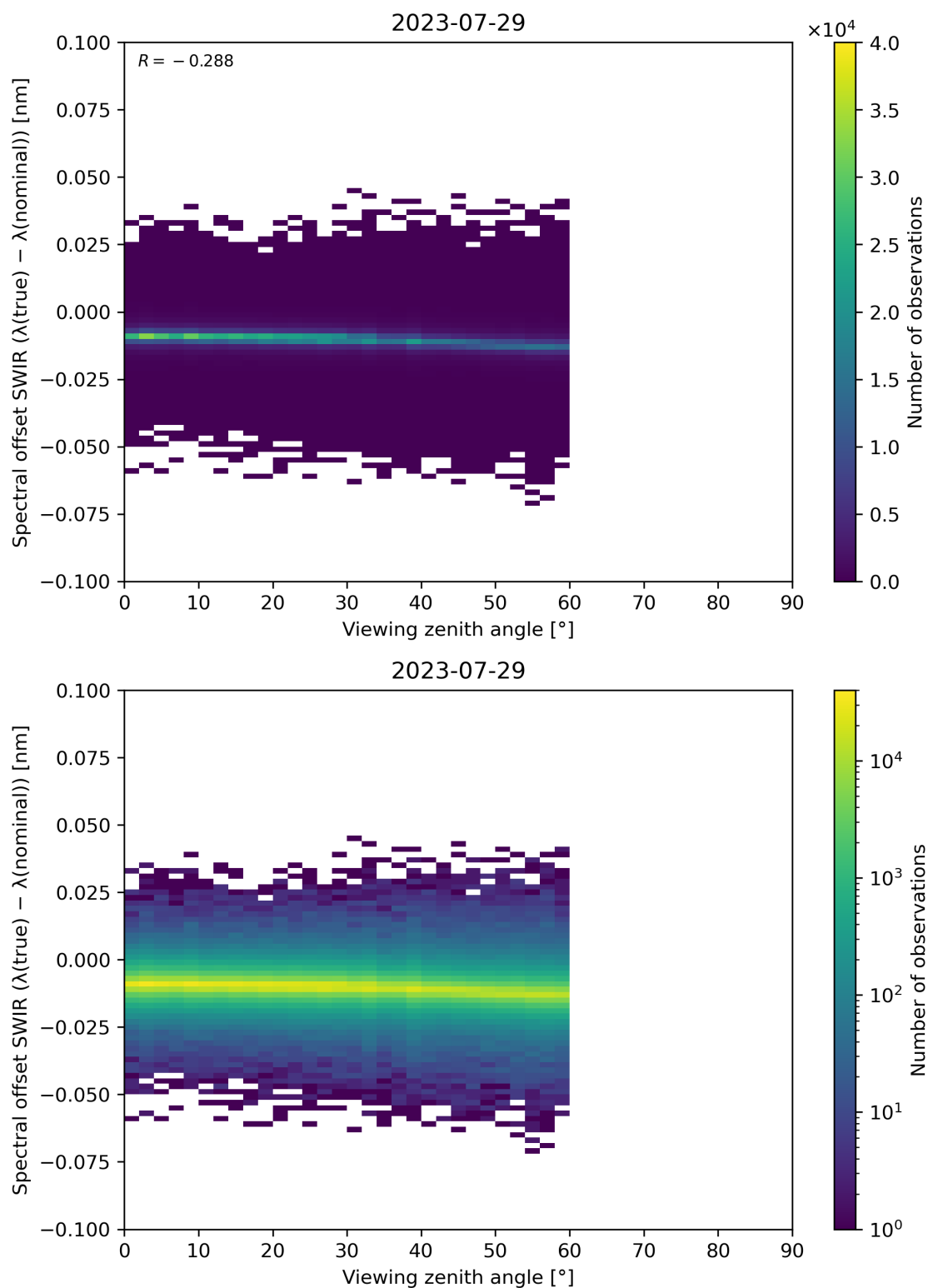
Figure 116: Scatter density plot of “Viewing zenith angle” against “Spectral offset SWIR ( \lambda(\text{true}) - \lambda(\text{nominal}) )” for 2023-07-29 to 2023-07-30.
