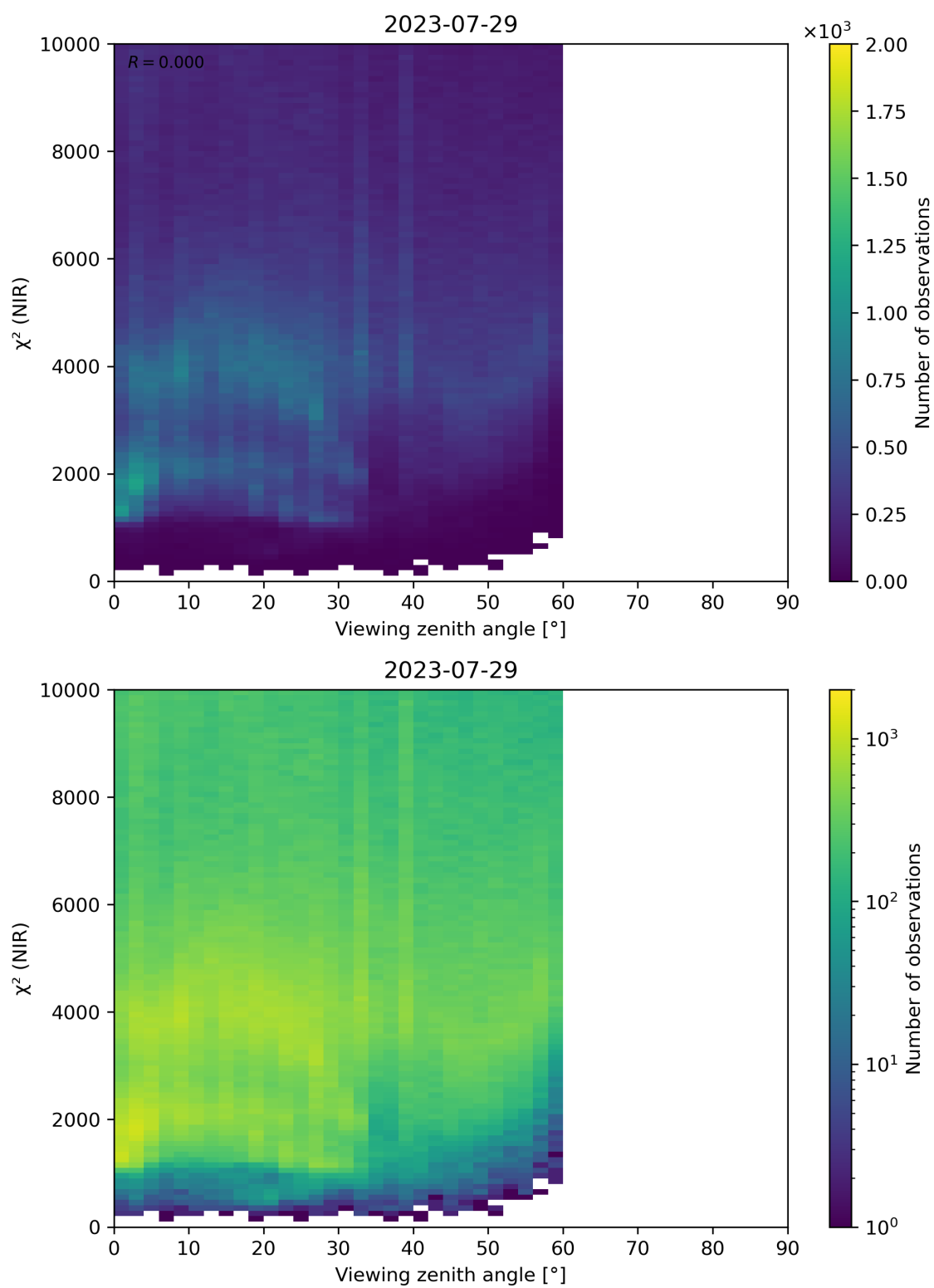
Figure 105: Scatter density plot of “Viewing zenith angle” against “ \chi^2 (NIR)” for 2023-07-29 to 2023-07-30.
