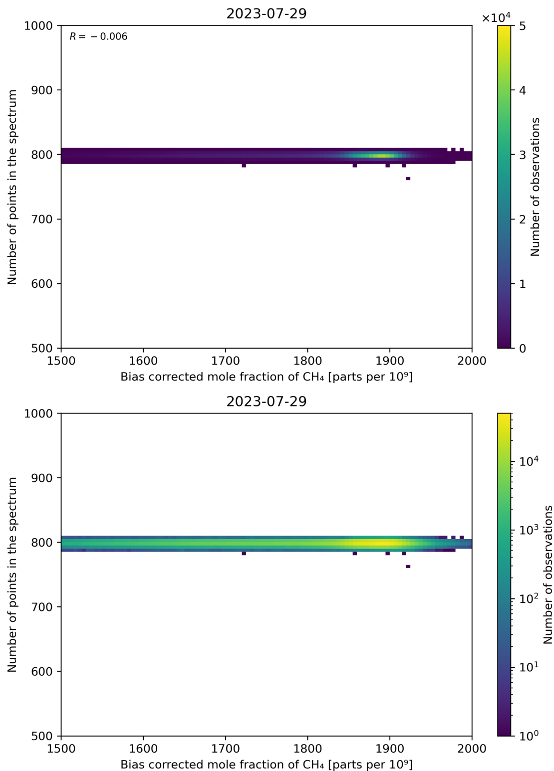
Figure 68: Scatter density plot of “Bias corrected mole fraction of CH 4 ” against “Number of points in the spectrum” for 2023-07-29 to 2023-07-30.
