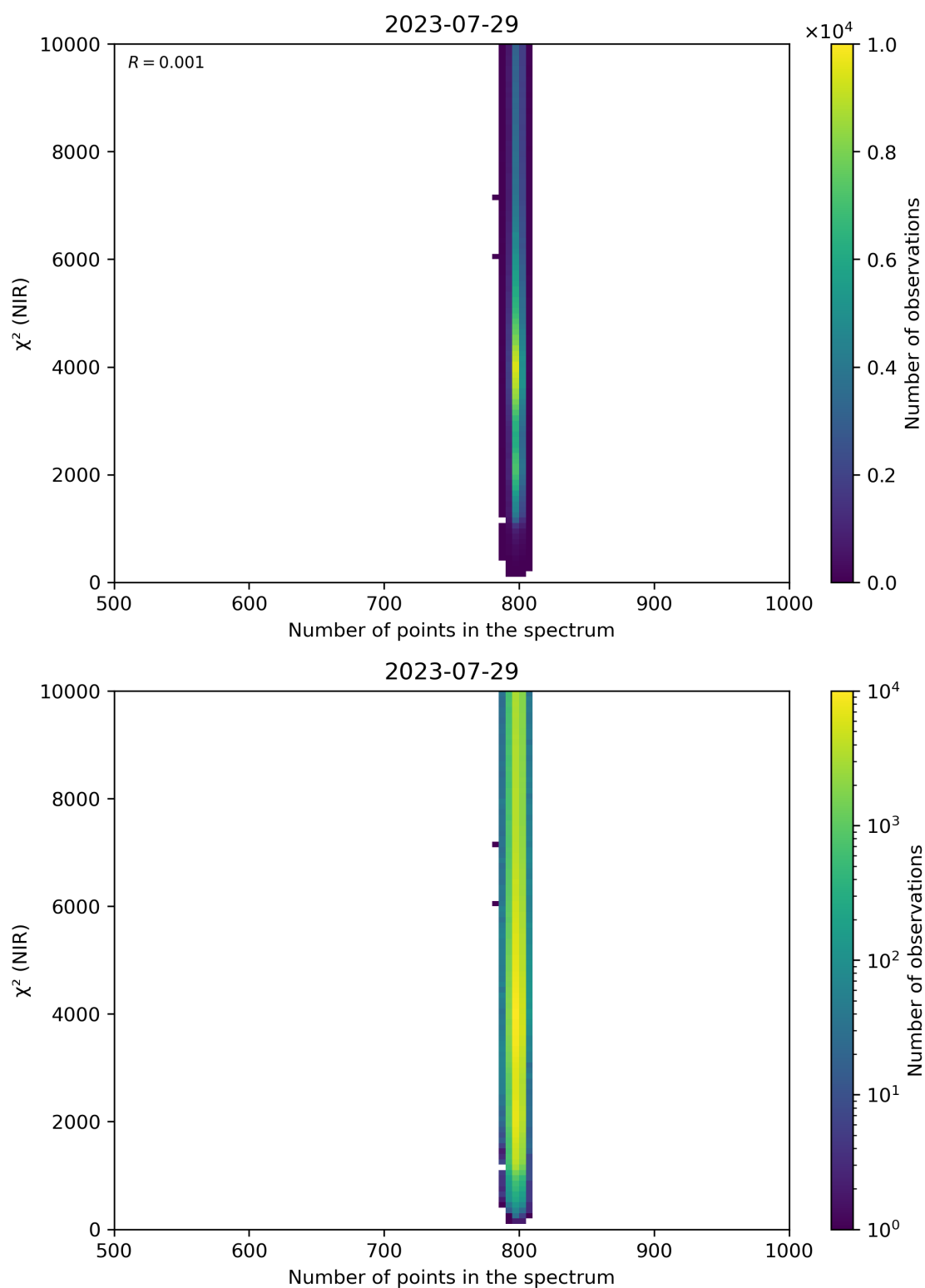
Figure 88: Scatter density plot of “Number of points in the spectrum” against “ \chi^2 (NIR)” for 2023-07-29 to 2023-07-30.
