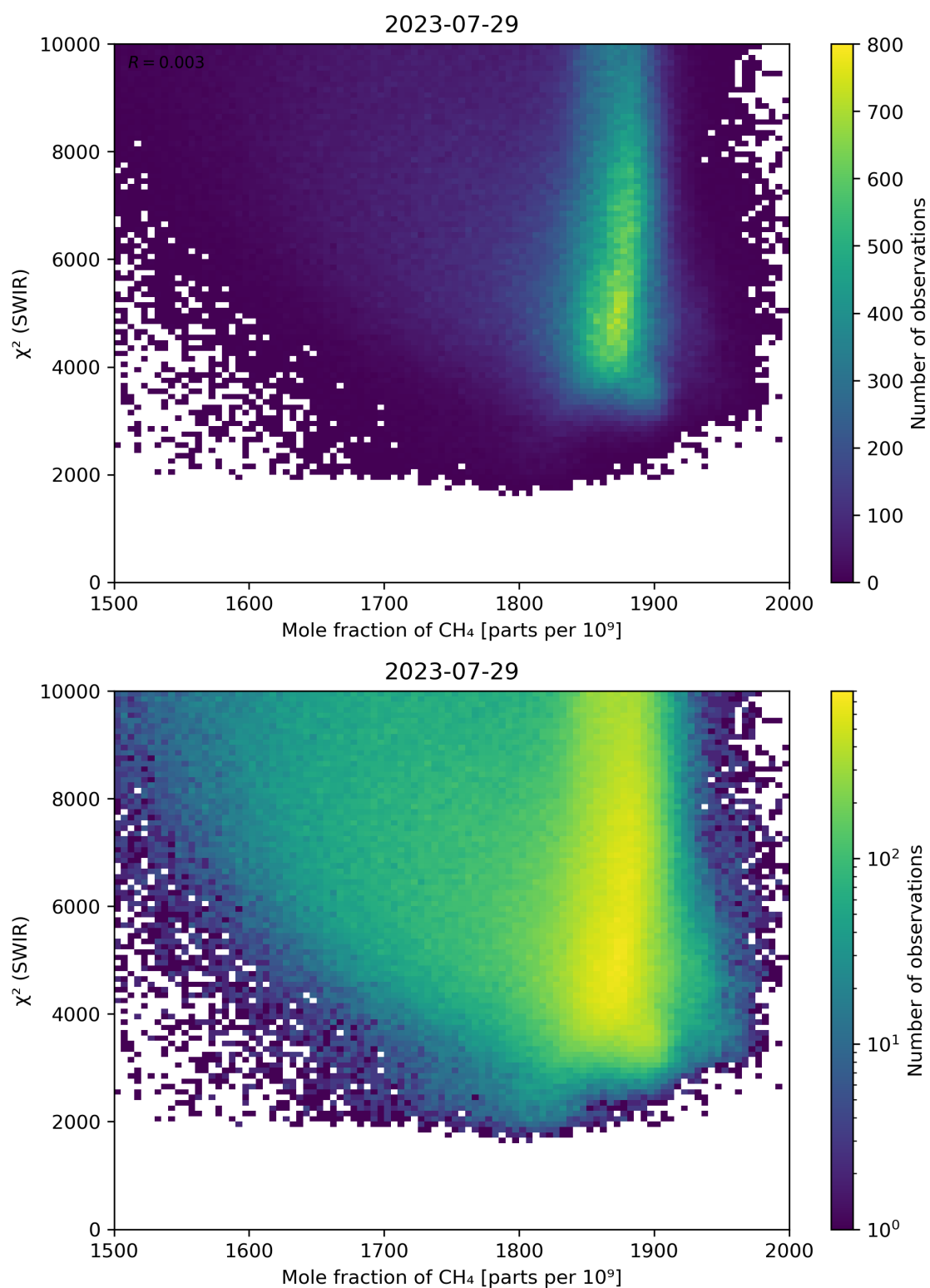
Figure 71: Scatter density plot of “Mole fraction of CH 4 ” against “ \chi^2 (SWIR)” for 2023-07-29 to 2023-07-30.
