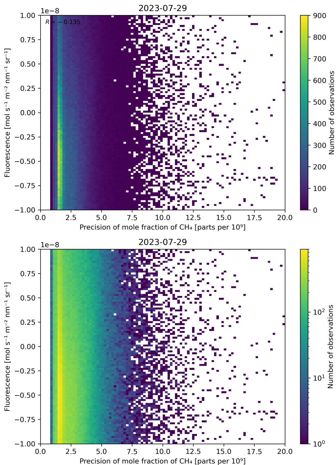
Figure 81: Scatter density plot of “Precision of mole fraction of CH 4 ” against “Fluorescence” for 2023-07-29 to 2023-07-30.
