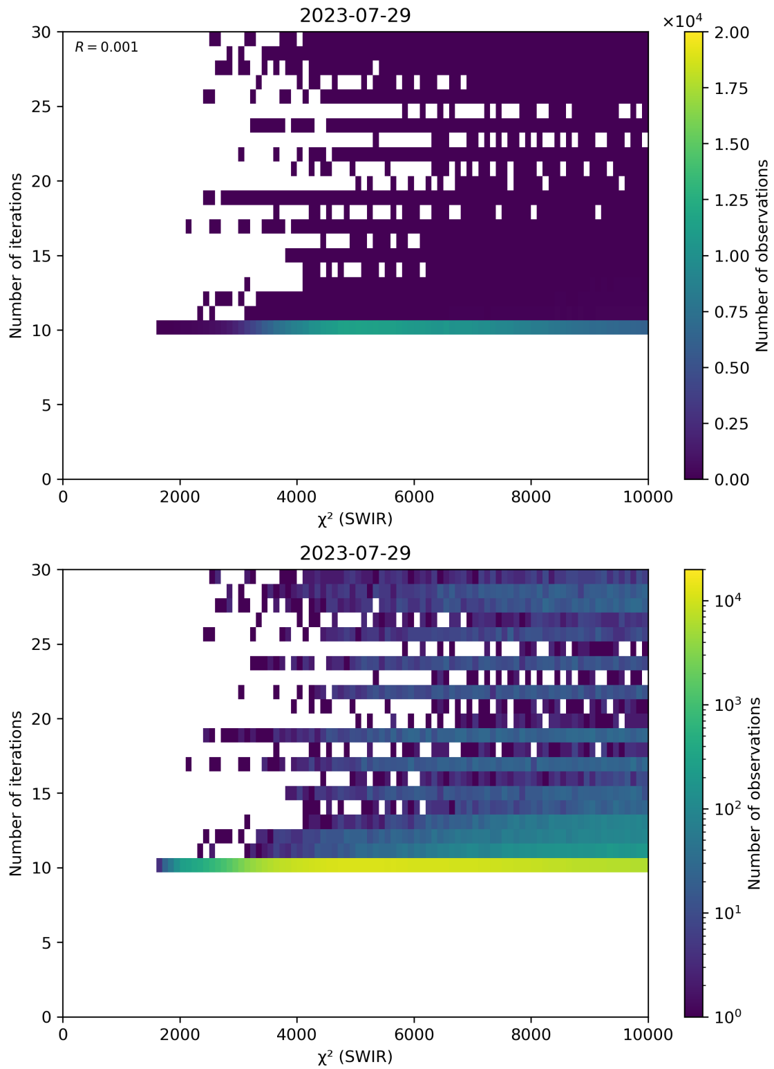
Figure 50: Scatter density plot of “ \chi^2 (SWIR)” against “Number of iterations” for 2023-07-29 to 2023-07-30.
