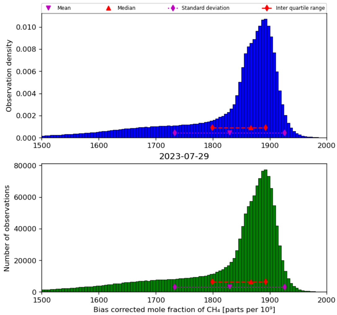
Figure 25: Histogram of “Bias corrected mole fraction of CH 4 ” for 2023-07-29 to 2023-07-30
