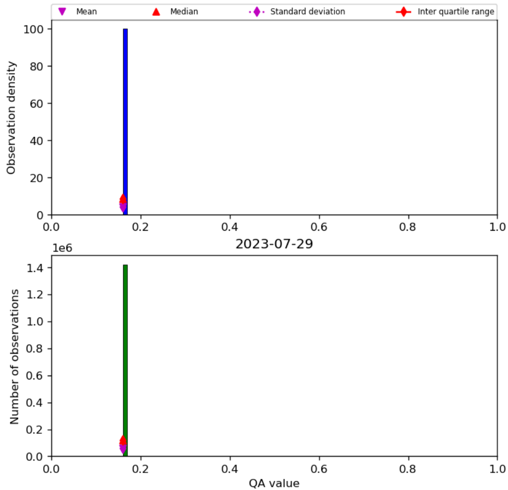
Figure 22: Histogram of “QA value” for 2023-07-29 to 2023-07-30
