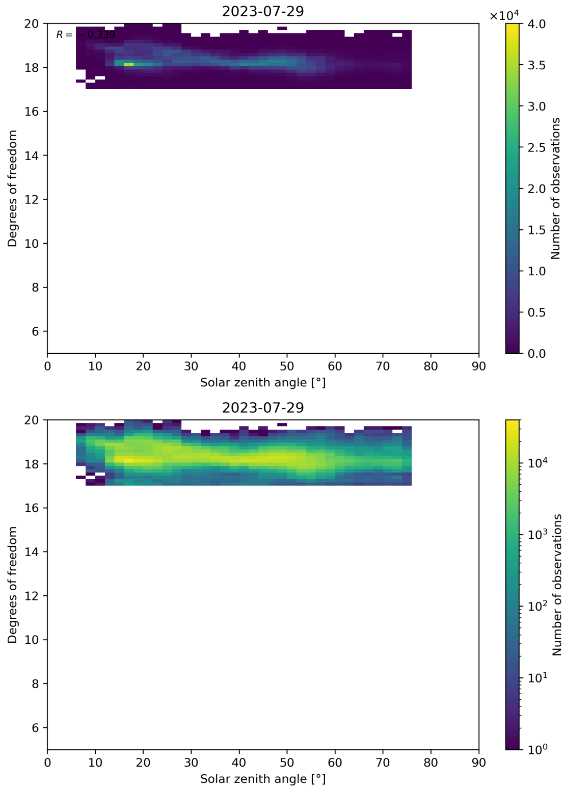
Figure 96: Scatter density plot of “Solar zenith angle” against “Degrees of freedom” for 2023-07-29 to 2023-07-30.
