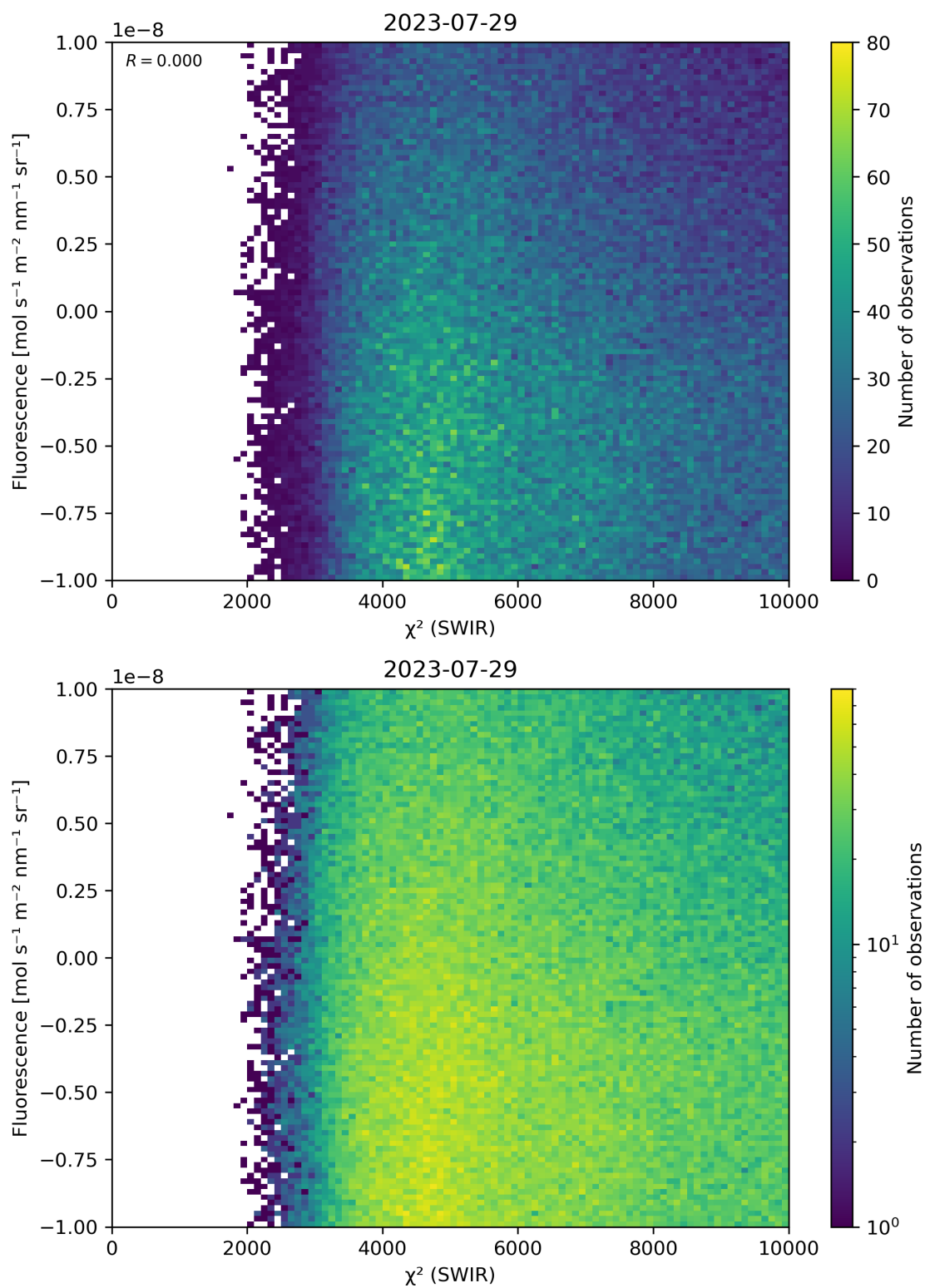
Figure 49: Scatter density plot of “ \chi^2 (SWIR)” against “Fluorescence” for 2023-07-29 to 2023-07-30.
