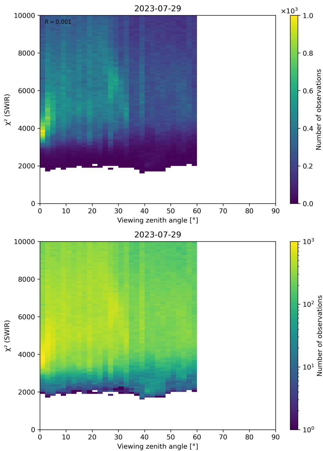
Figure 106: Scatter density plot of “Viewing zenith angle” against “ \chi^2 (SWIR)” for 2023-07-29 to 2023-07-30.
