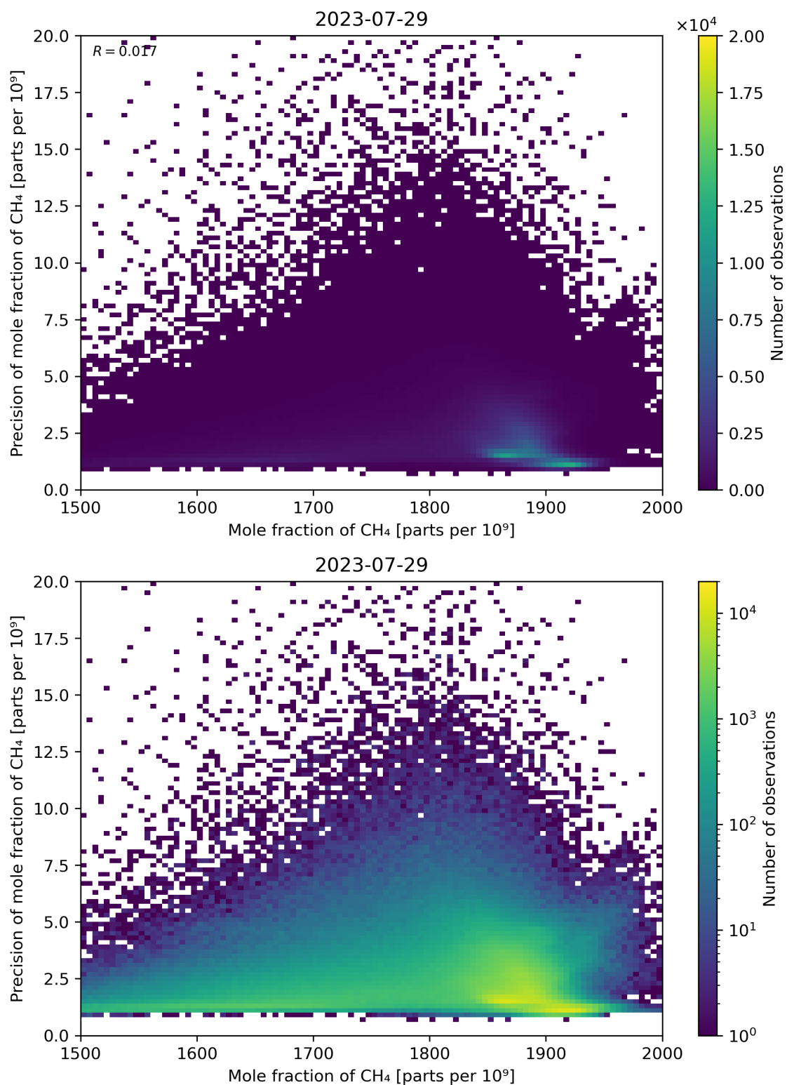
Figure 75: Scatter density plot of “Mole fraction of CH 4 ” against “Precision of mole fraction of CH 4 ” for 2023-07-29 to 2023-07-30.
