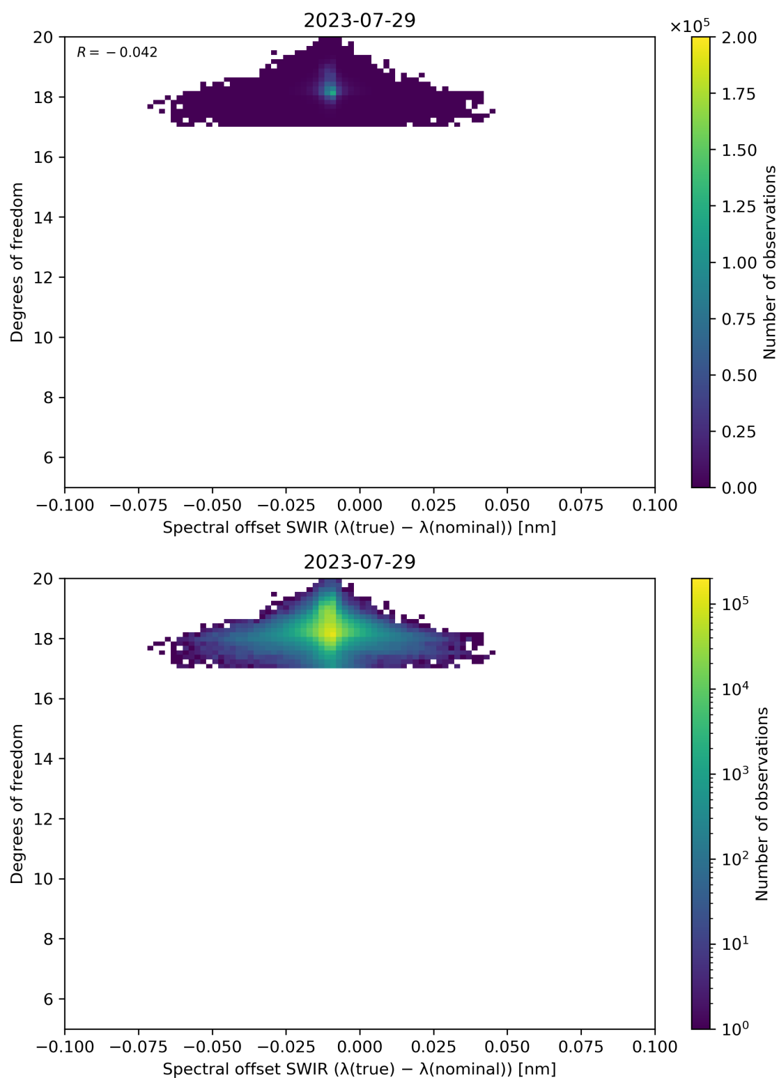
Figure 119: Scatter density plot of “Spectral offset SWIR ( \lambda(\text{true}) - \lambda(\text{nominal}) )” against “Degrees of freedom” for 2023-07-29 to 2023-07-30.
