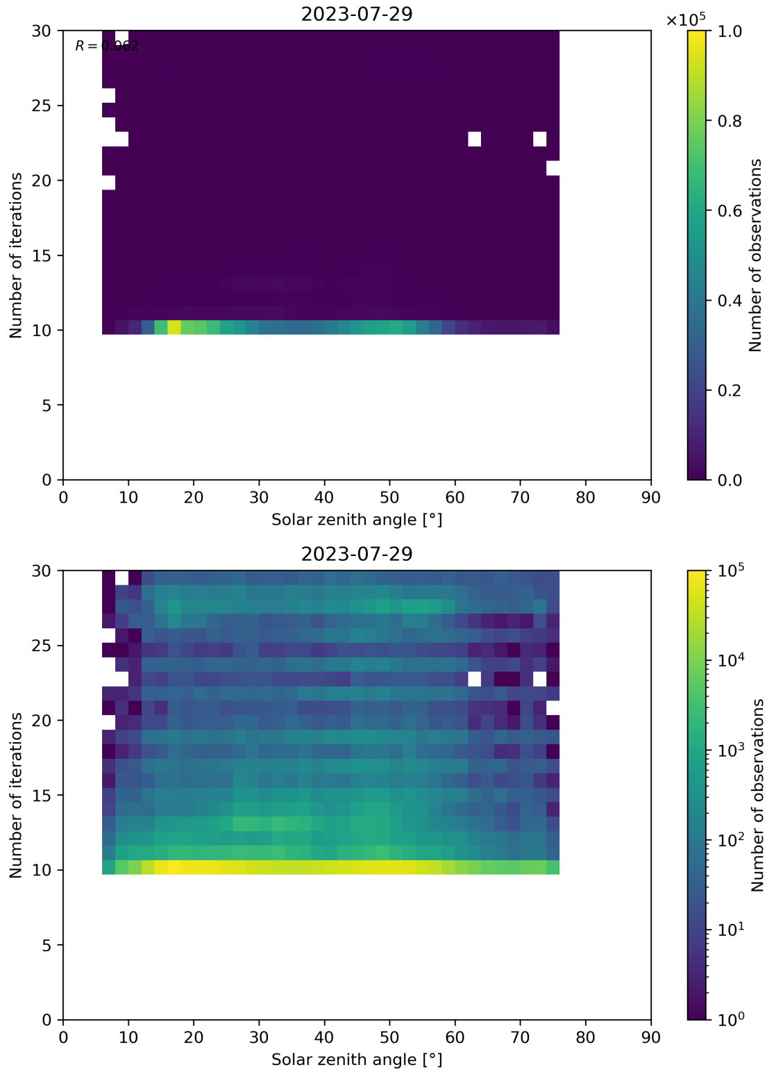
Figure 102: Scatter density plot of “Solar zenith angle” against “Number of iterations” for 2023-07-29 to 2023-07-30.
