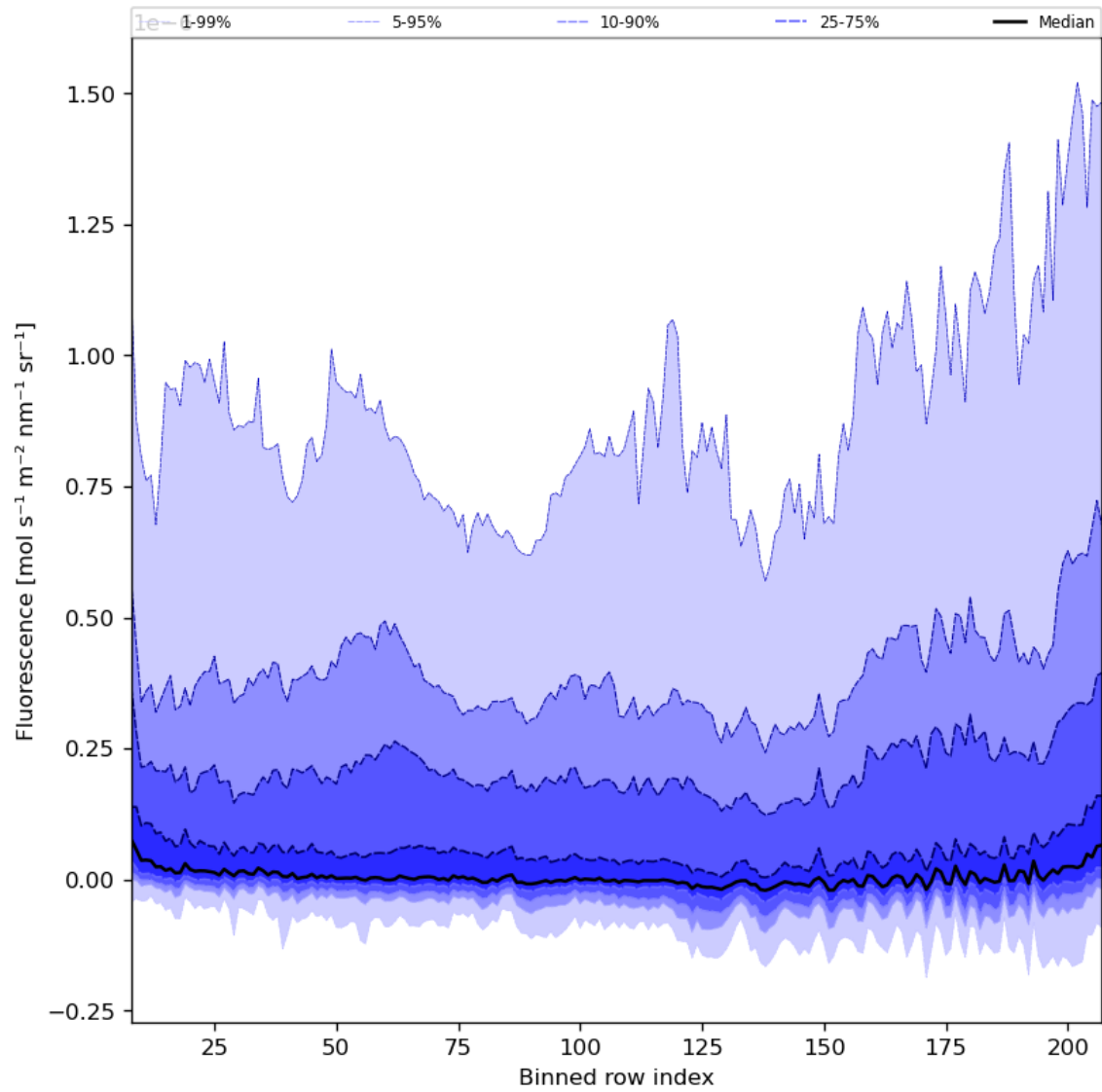
Figure 43: Along track statistics of “Fluorescence” for 2023-07-29 to 2023-07-30
