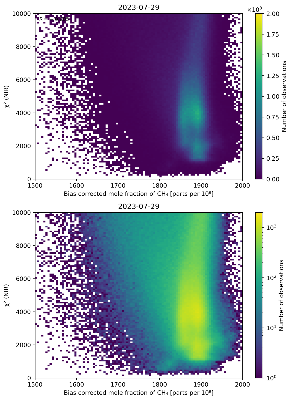
Figure 63: Scatter density plot of “Bias corrected mole fraction of \text{CH}_4 ” against “ \chi^2 (NIR)” for 2023-07-29 to 2023-07-30.
