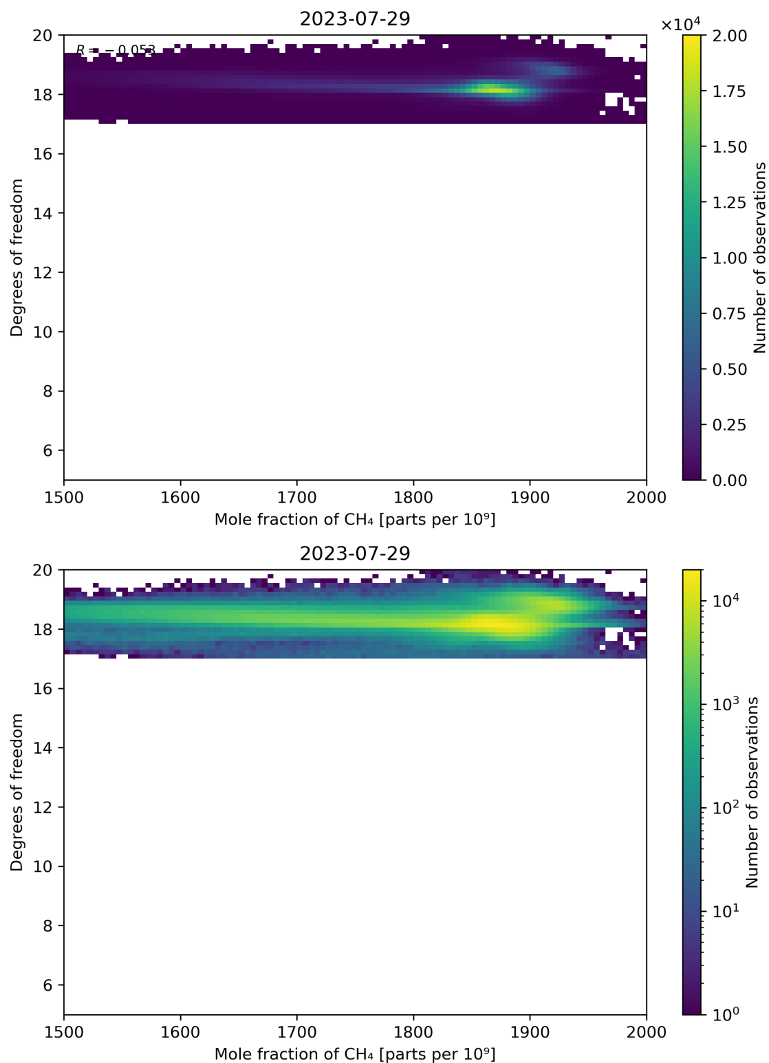
Figure 72: Scatter density plot of “Mole fraction of CH 4 ” against “Degrees of freedom” for 2023-07-29 to 2023-07-30.
