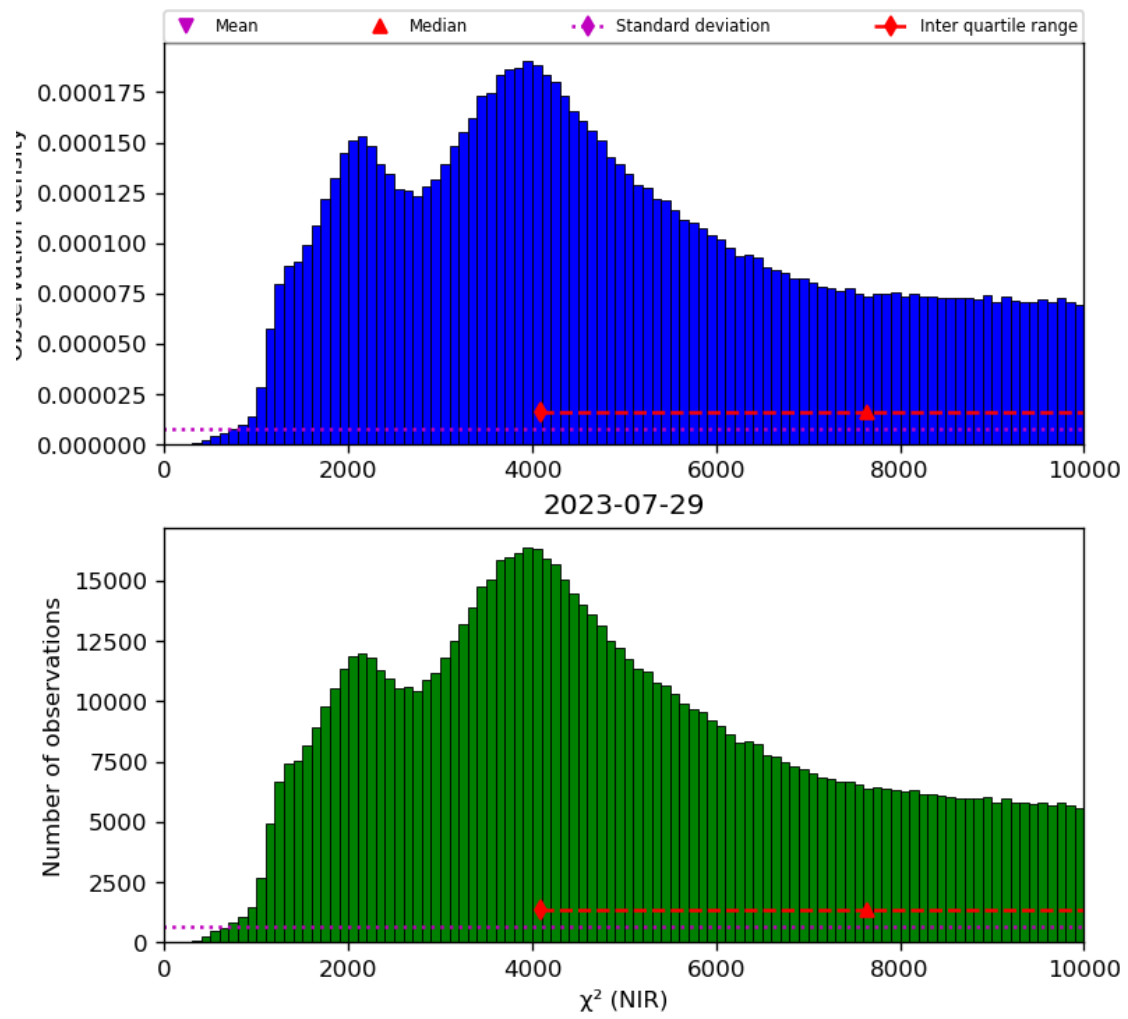
Figure 29: Histogram of “ \chi^2 (NIR)” for 2023-07-29 to 2023-07-30
