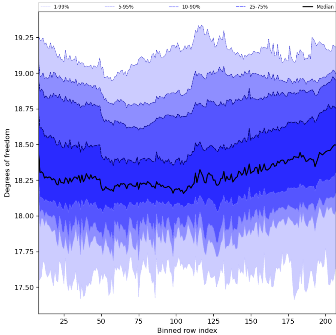
Figure 41: Along track statistics of “Degrees of freedom” for 2023-07-29 to 2023-07-30
