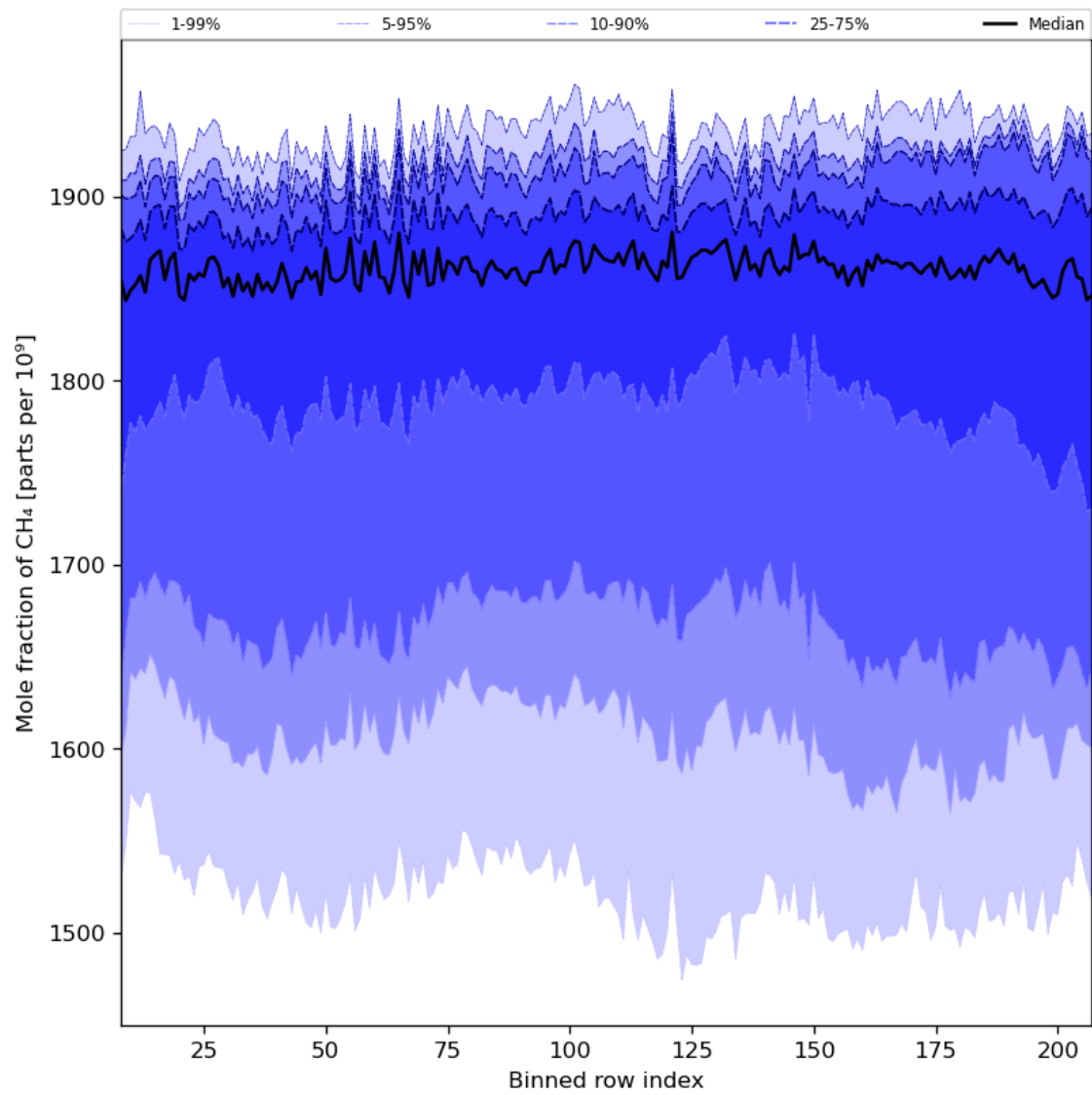
Figure 34: Along track statistics of “Mole fraction of CH 4 ” for 2023-07-29 to 2023-07-30
