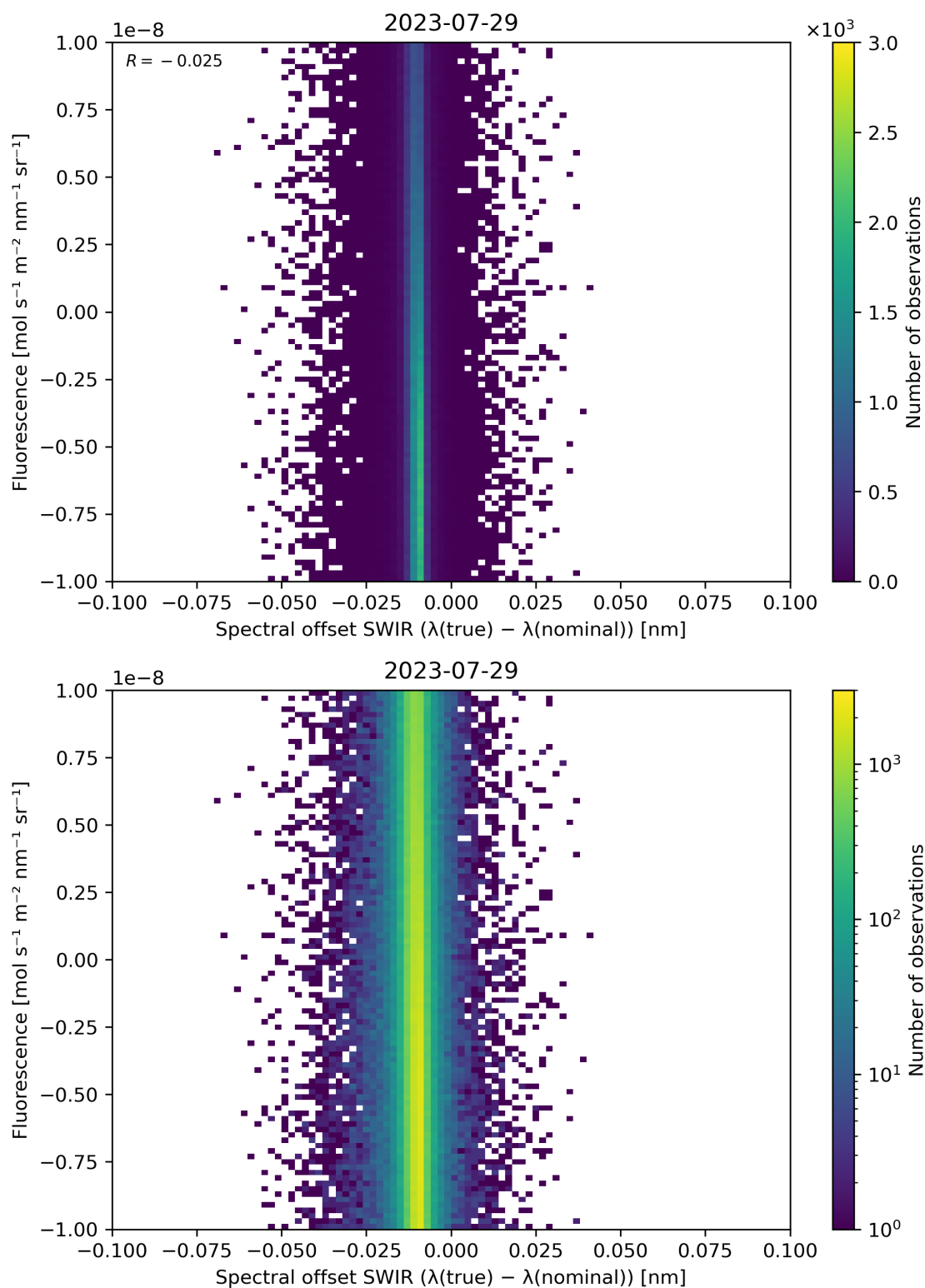
Figure 120: Scatter density plot of “Spectral offset SWIR ( \lambda(\text{true}) - \lambda(\text{nominal}) )” against “Fluorescence” for 2023-07-29 to 2023-07-30.
