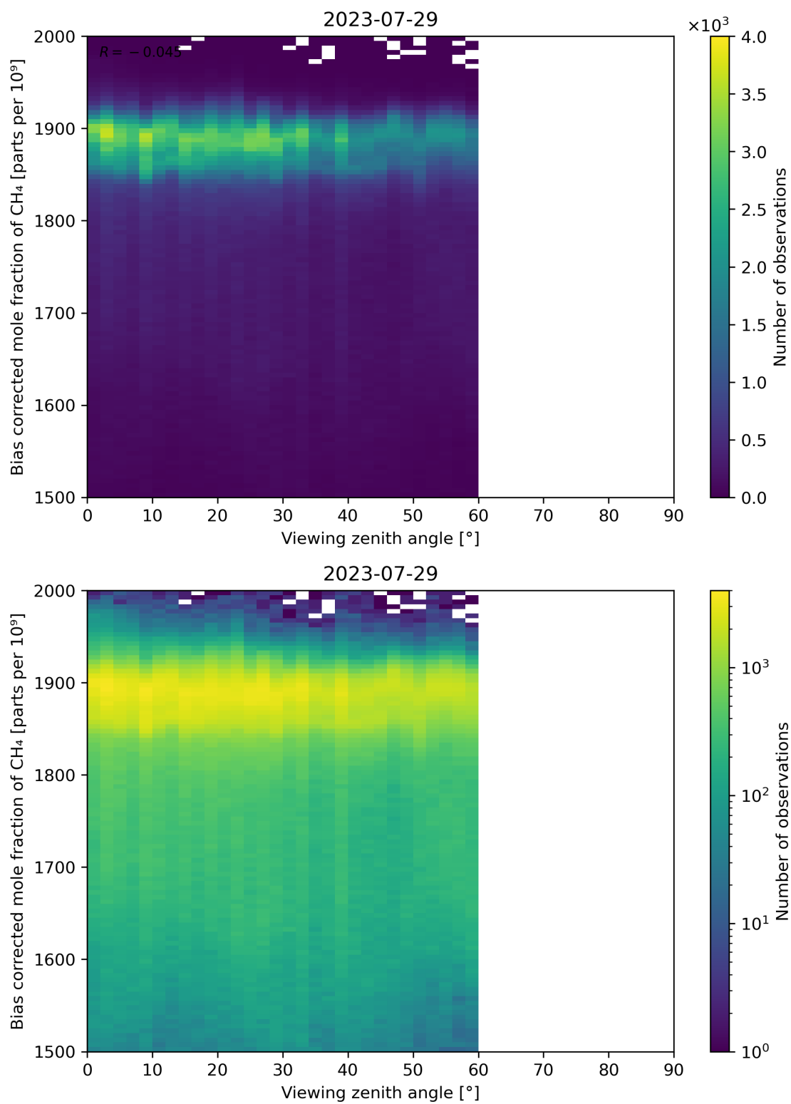
Figure 111: Scatter density plot of “Viewing zenith angle” against “Bias corrected mole fraction of CH 4 ” for 2023-07-29 to 2023-07-30.
