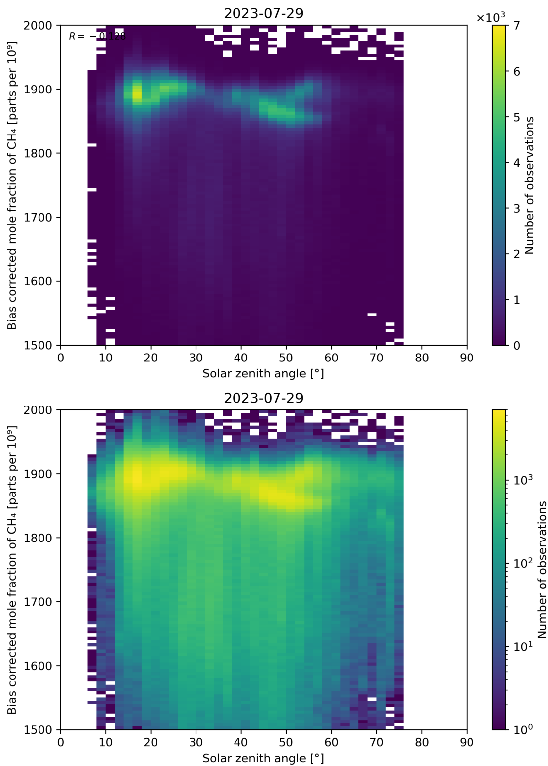
Figure 100: Scatter density plot of “Solar zenith angle” against “Bias corrected mole fraction of \text{CH}_4 ” for 2023-07-29 to 2023-07-30.
