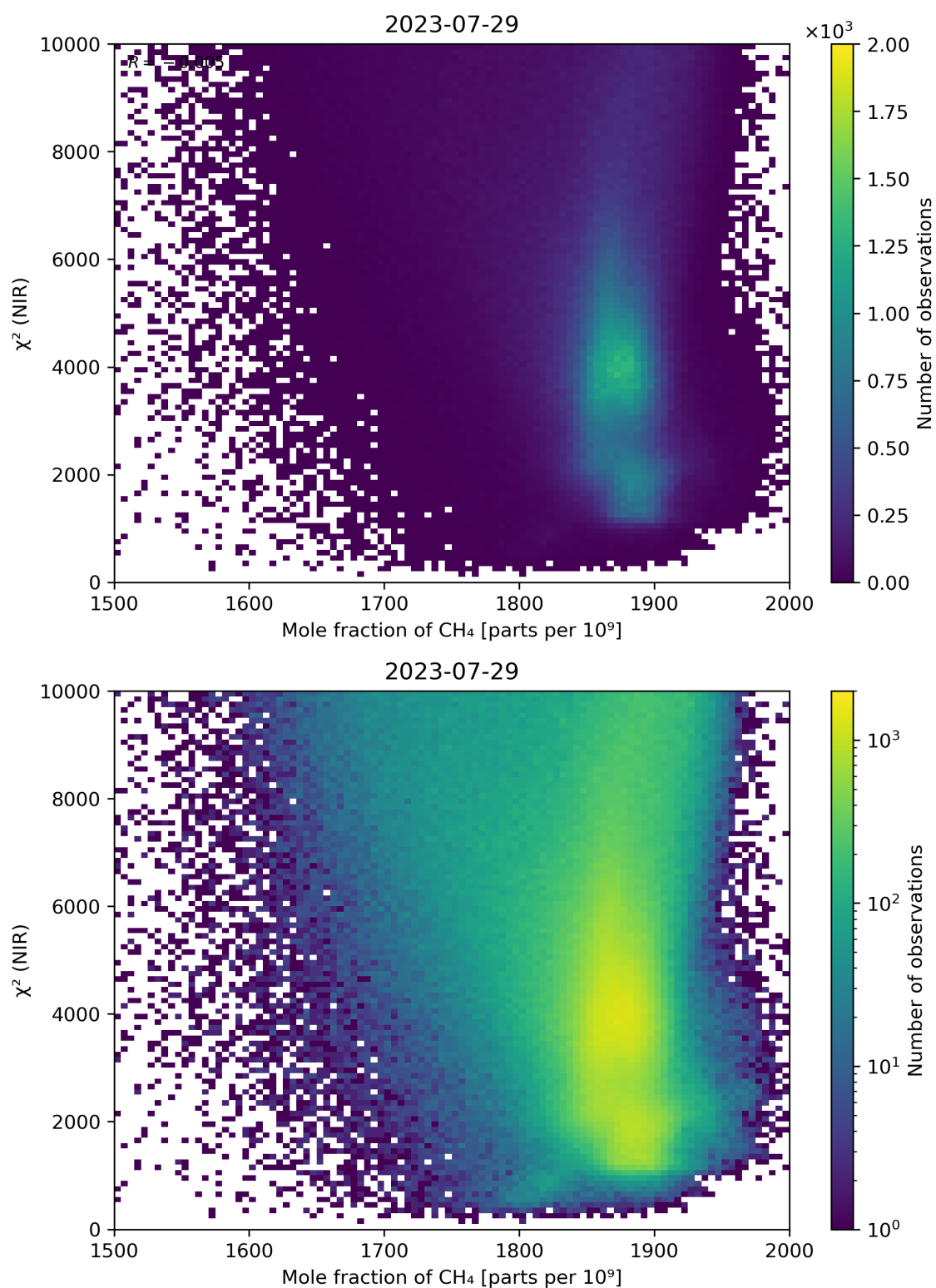
Figure 70: Scatter density plot of “Mole fraction of CH 4 ” against “ \chi^2 (NIR)” for 2023-07-29 to 2023-07-30.
