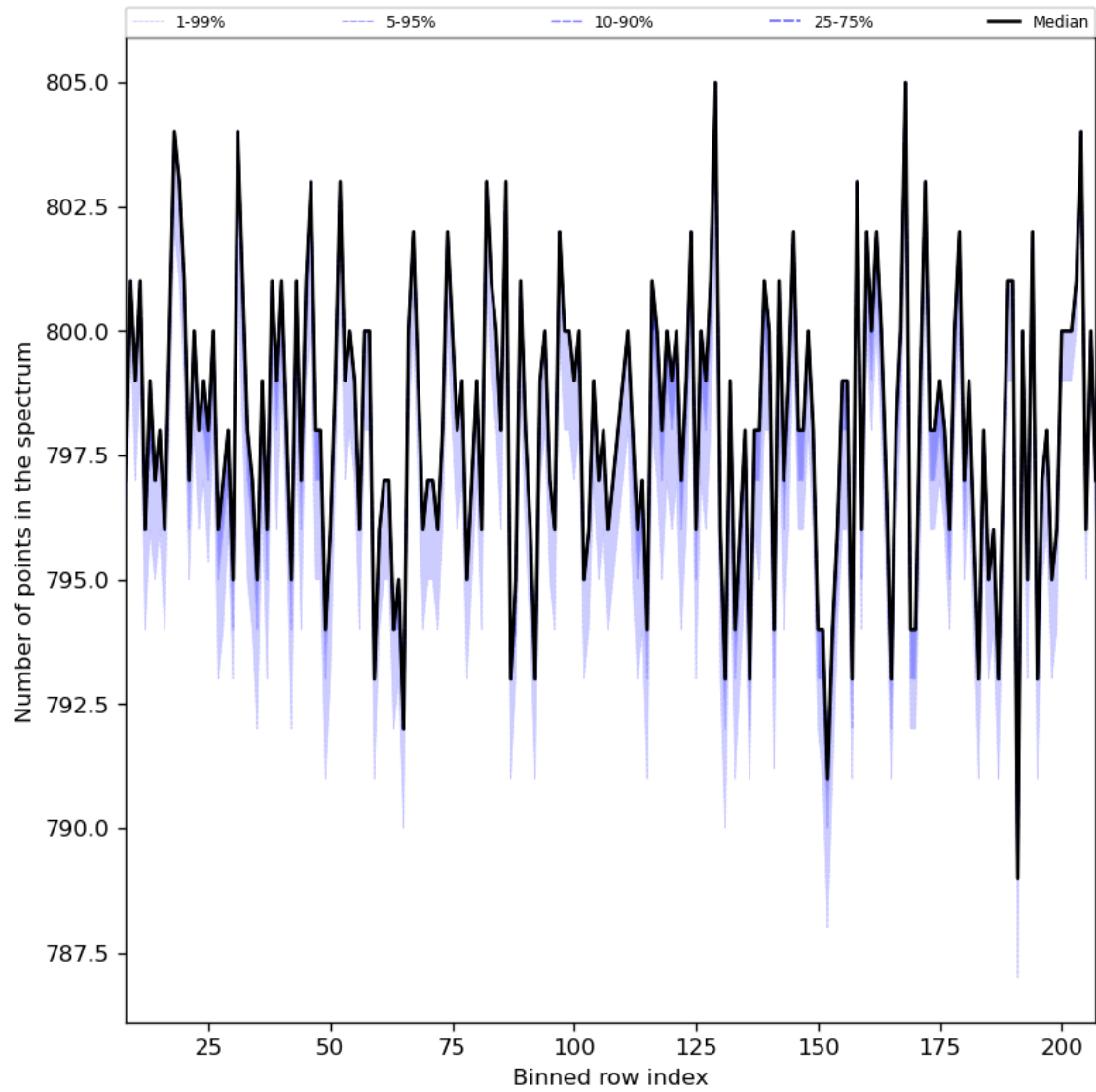
Figure 37: Along track statistics of “Number of points in the spectrum” for 2023-07-29 to 2023-07-30
