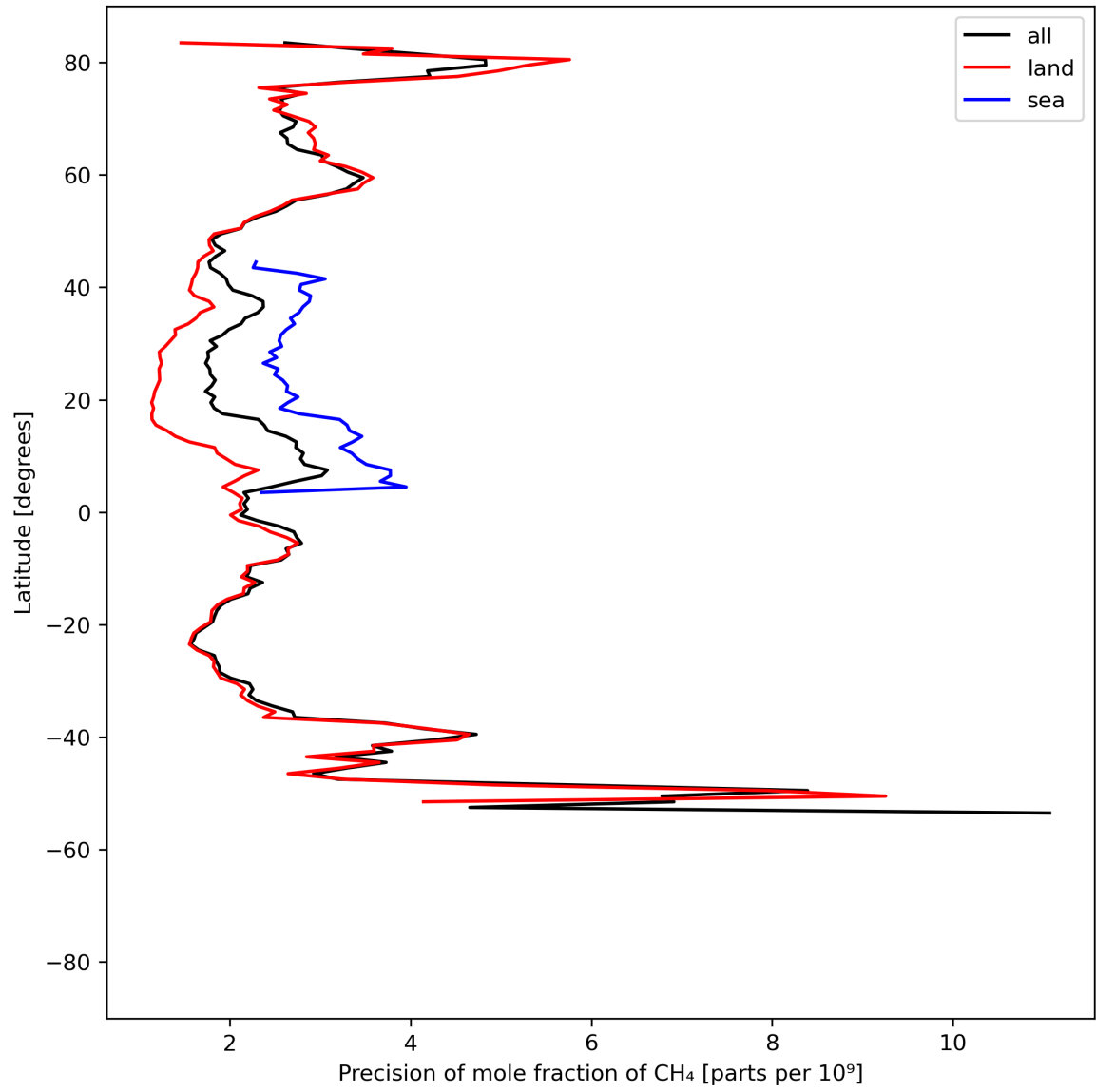
Figure 13: Zonal average of “Precision of mole fraction of CH 4 ” for 2023-07-29 to 2023-07-30.
