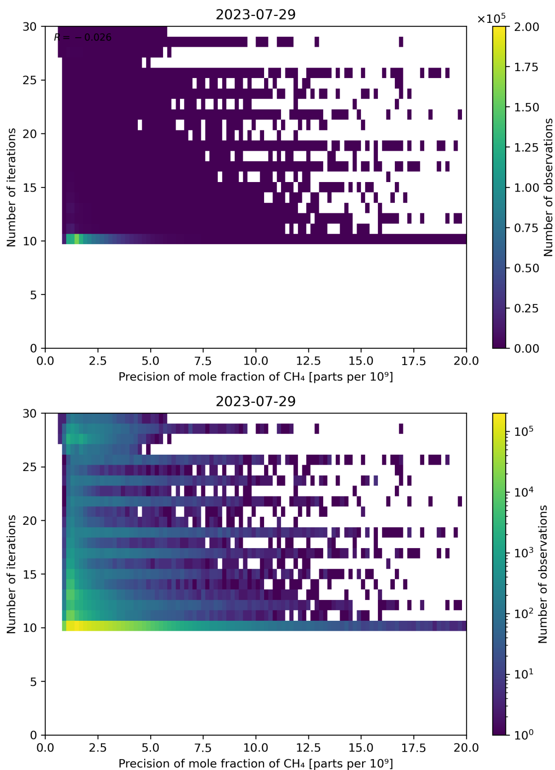
Figure 83: Scatter density plot of “Precision of mole fraction of CH 4 ” against “Number of iterations” for 2023-07-29 to 2023-07-30.
