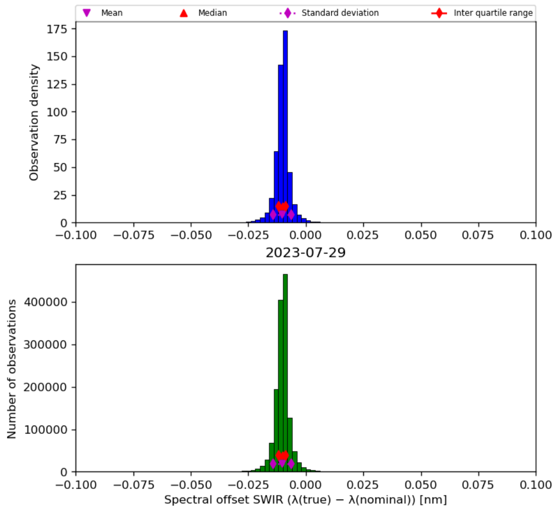
Figure 27: Histogram of “Spectral offset SWIR ( \lambda(\text{true}) - \lambda(\text{nominal}) )” for 2023-07-29 to 2023-07-30
