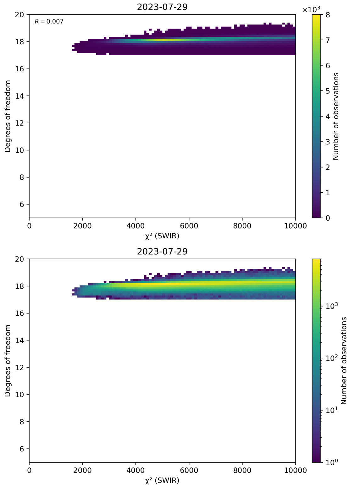
Figure 48: Scatter density plot of “ \chi^2 (SWIR)” against “Degrees of freedom” for 2023-07-29 to 2023-07-30.
