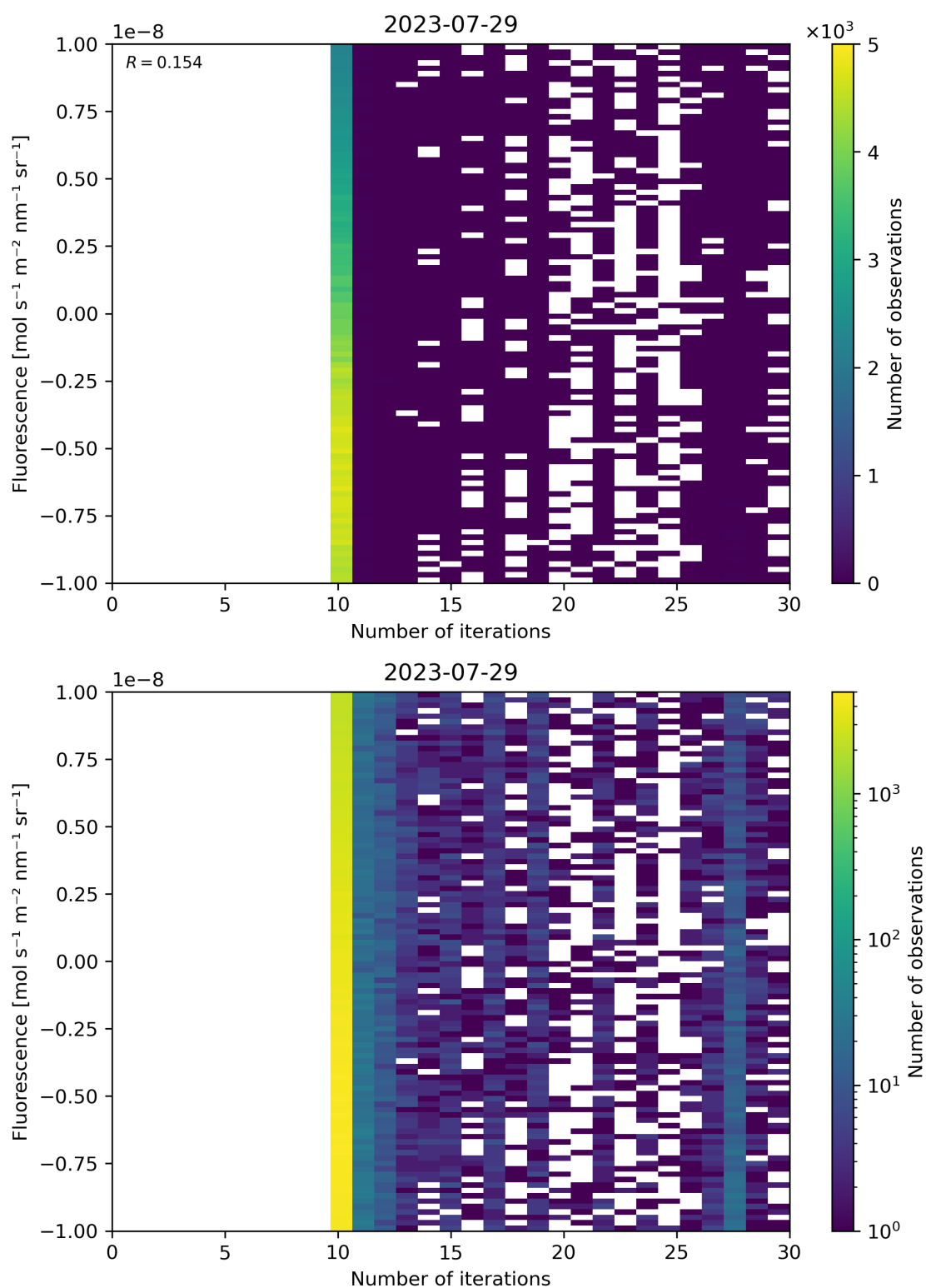
Figure 87: Scatter density plot of “Number of iterations” against “Fluorescence” for 2023-07-29 to 2023-07-30.
