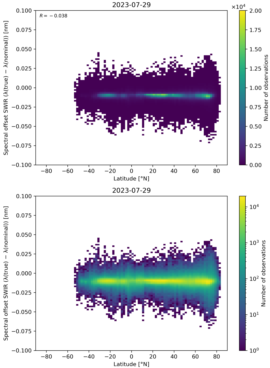
Figure 62: Scatter density plot of “Latitude” against “Spectral offset SWIR ( \lambda(\text{true}) - \lambda(\text{nominal}) )” for 2023-07-29 to 2023-07-30.
