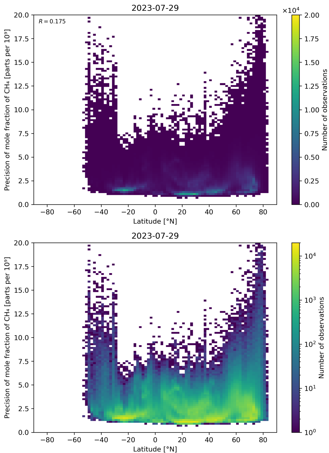
Figure 59: Scatter density plot of “Latitude” against “Precision of mole fraction of CH 4 ” for 2023-07-29 to 2023-07-30.
