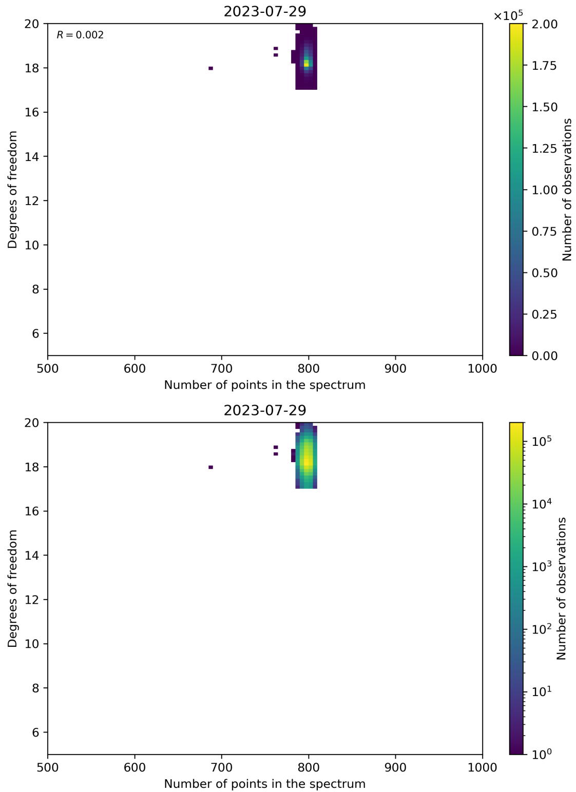
Figure 90: Scatter density plot of “Number of points in the spectrum” against “Degrees of freedom” for 2023-07-29 to 2023-07-30.
