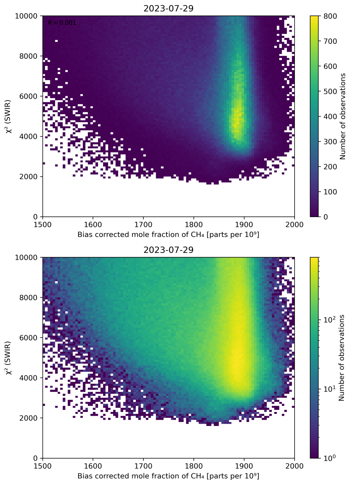
Figure 64: Scatter density plot of “Bias corrected mole fraction of CH 4 ” against “ \chi^2 (SWIR)” for 2023-07-29 to 2023-07-30.
