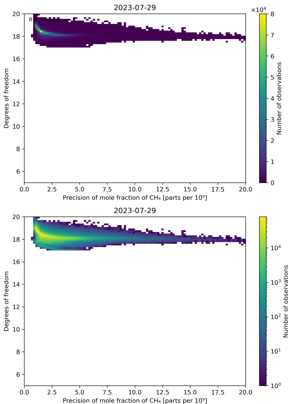
Figure 80: Scatter density plot of “Precision of mole fraction of CH 4 ” against “Degrees of freedom” for 2023-07-29 to 2023-07-30.
