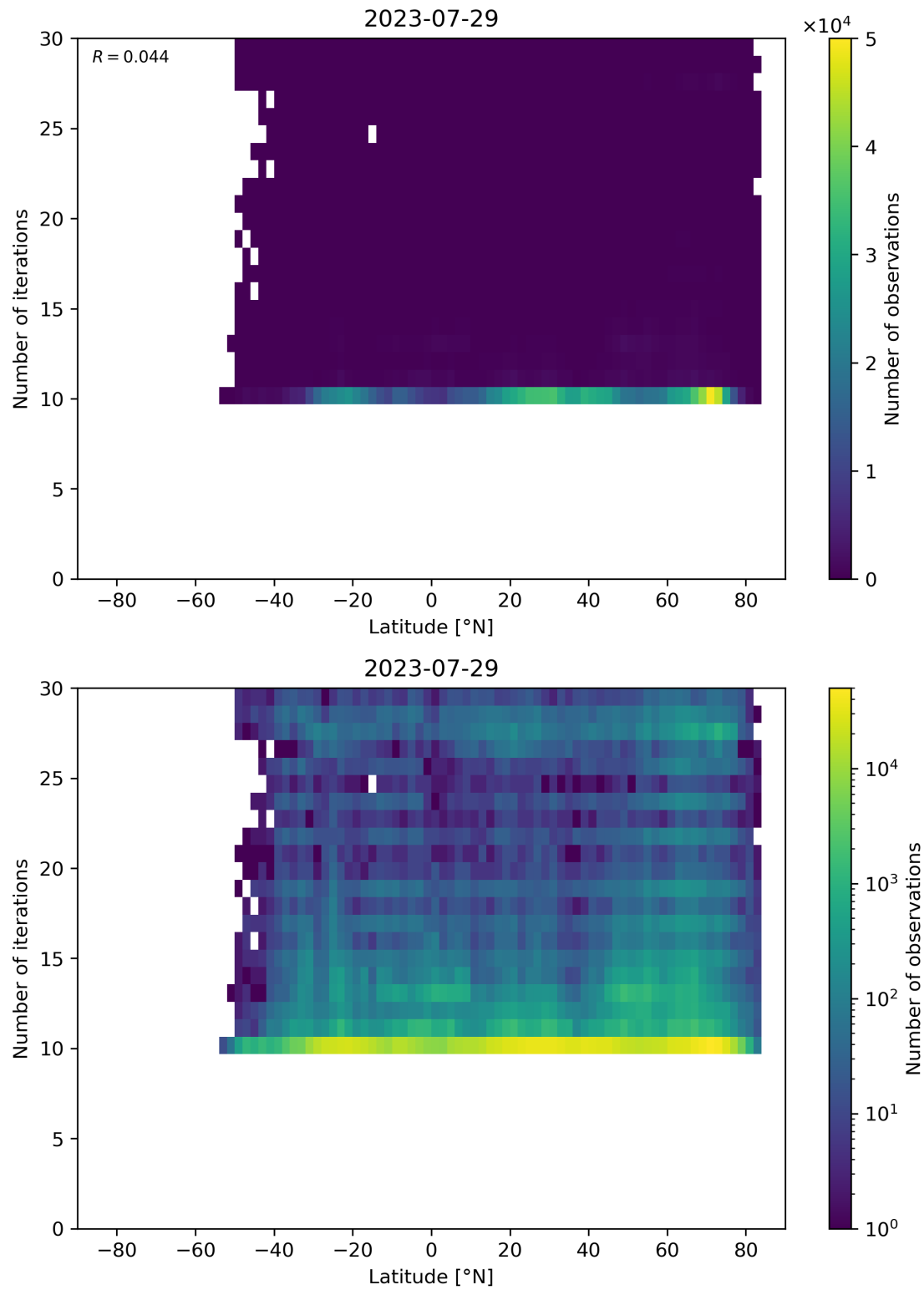
Figure 60: Scatter density plot of “Latitude” against “Number of iterations” for 2023-07-29 to 2023-07-30.
