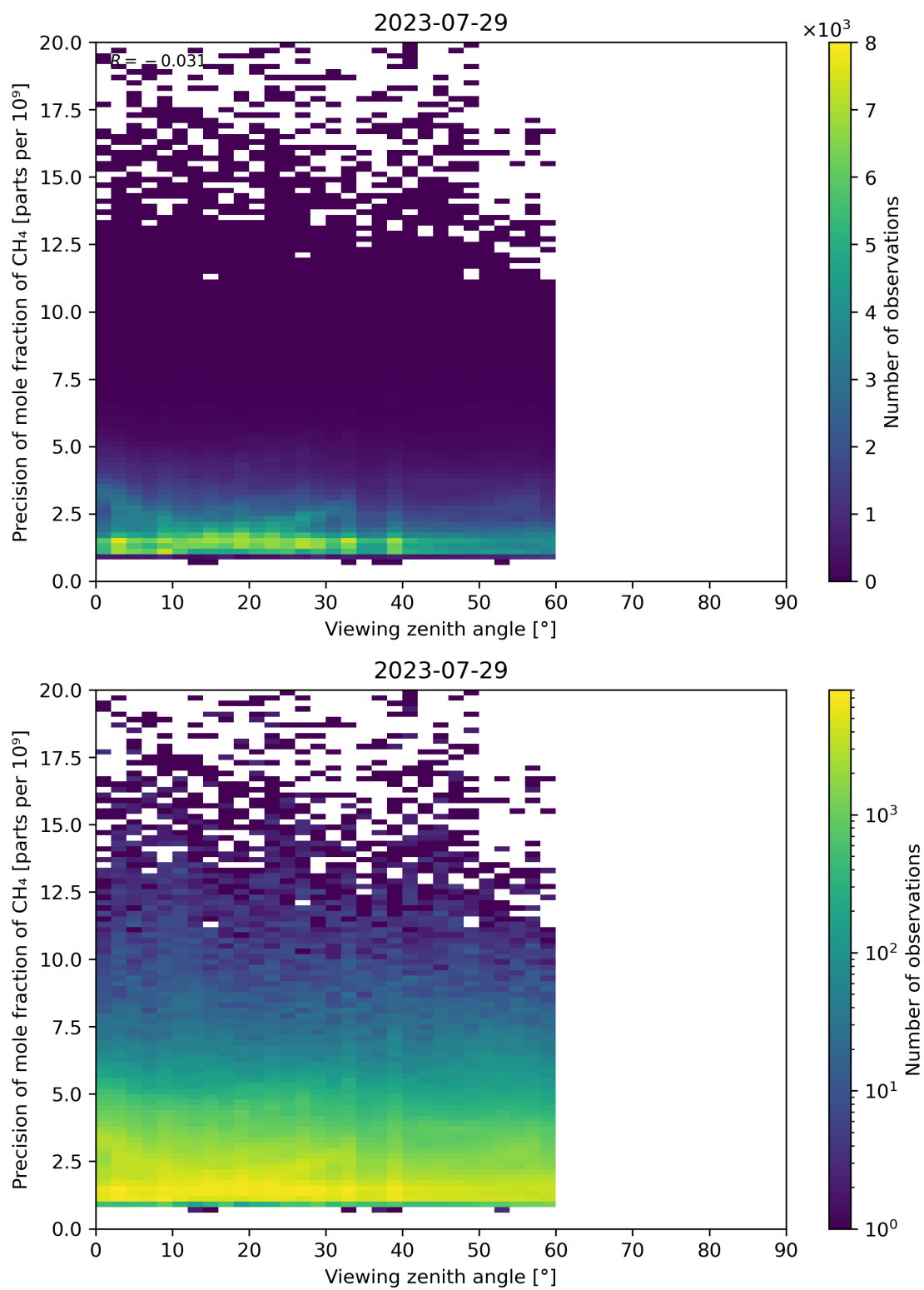
Figure 112: Scatter density plot of “Viewing zenith angle” against “Precision of mole fraction of CH 4 ” for 2023-07-29 to 2023-07-30.
