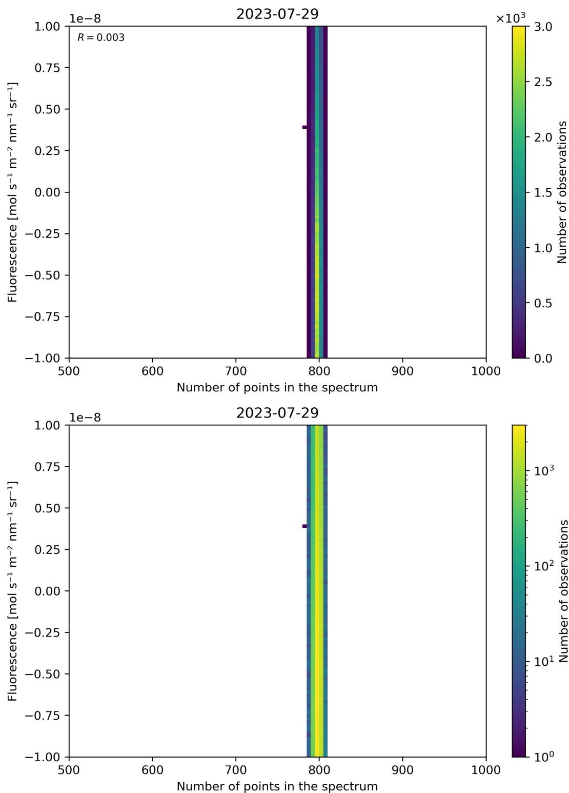
Figure 91: Scatter density plot of “Number of points in the spectrum” against “Fluorescence” for 2023-07-29 to 2023-07-30.
