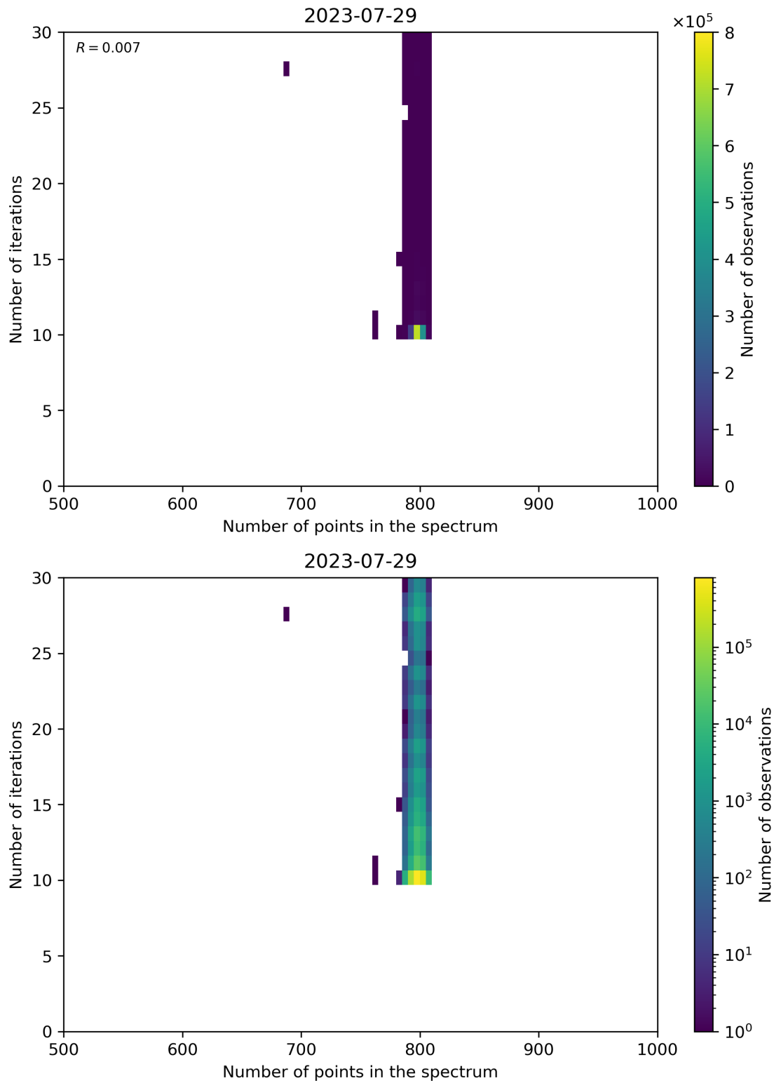
Figure 92: Scatter density plot of “Number of points in the spectrum” against “Number of iterations” for 2023-07-29 to 2023-07-30.
