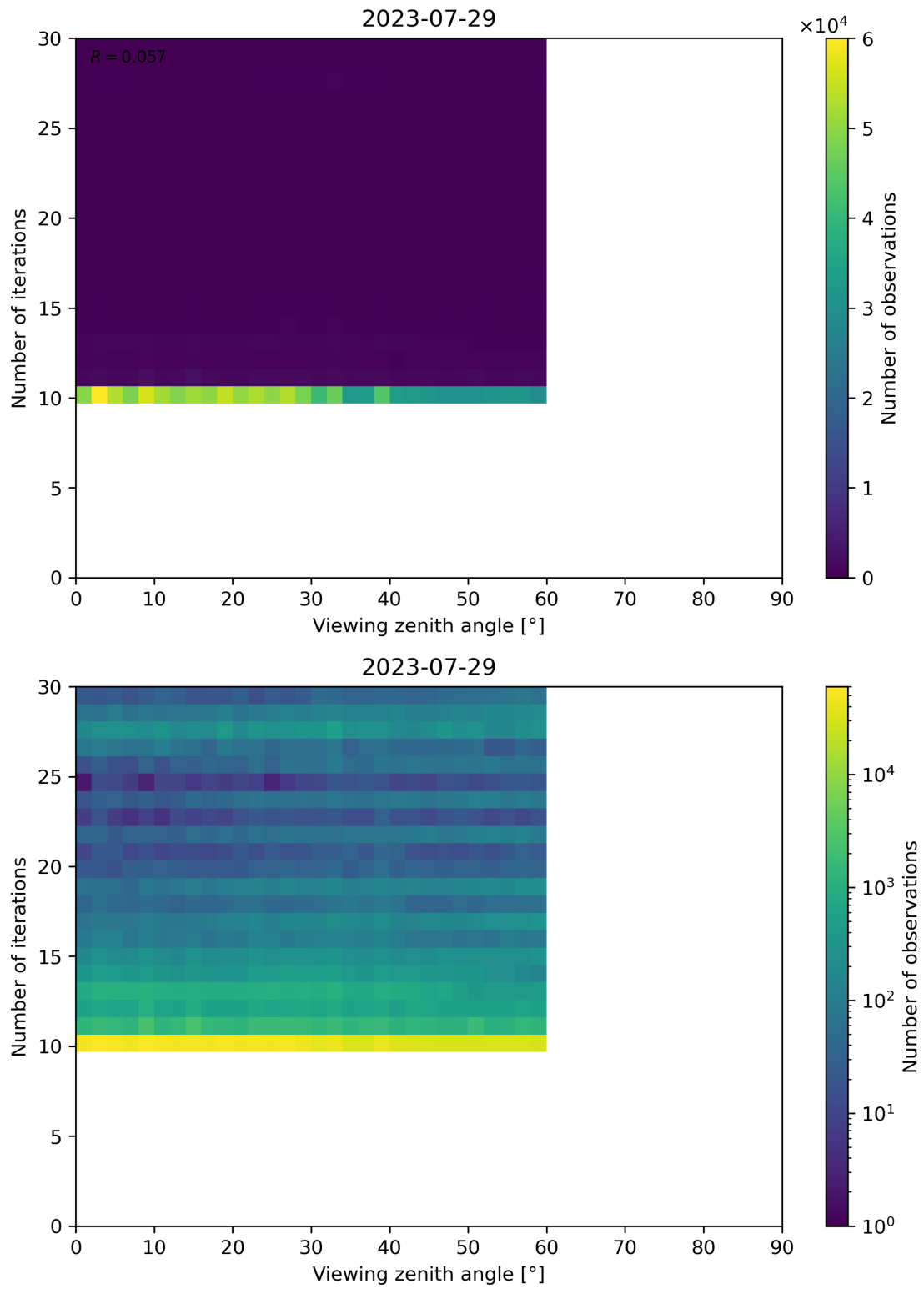
Figure 113: Scatter density plot of “Viewing zenith angle” against “Number of iterations” for 2023-07-29 to 2023-07-30.
