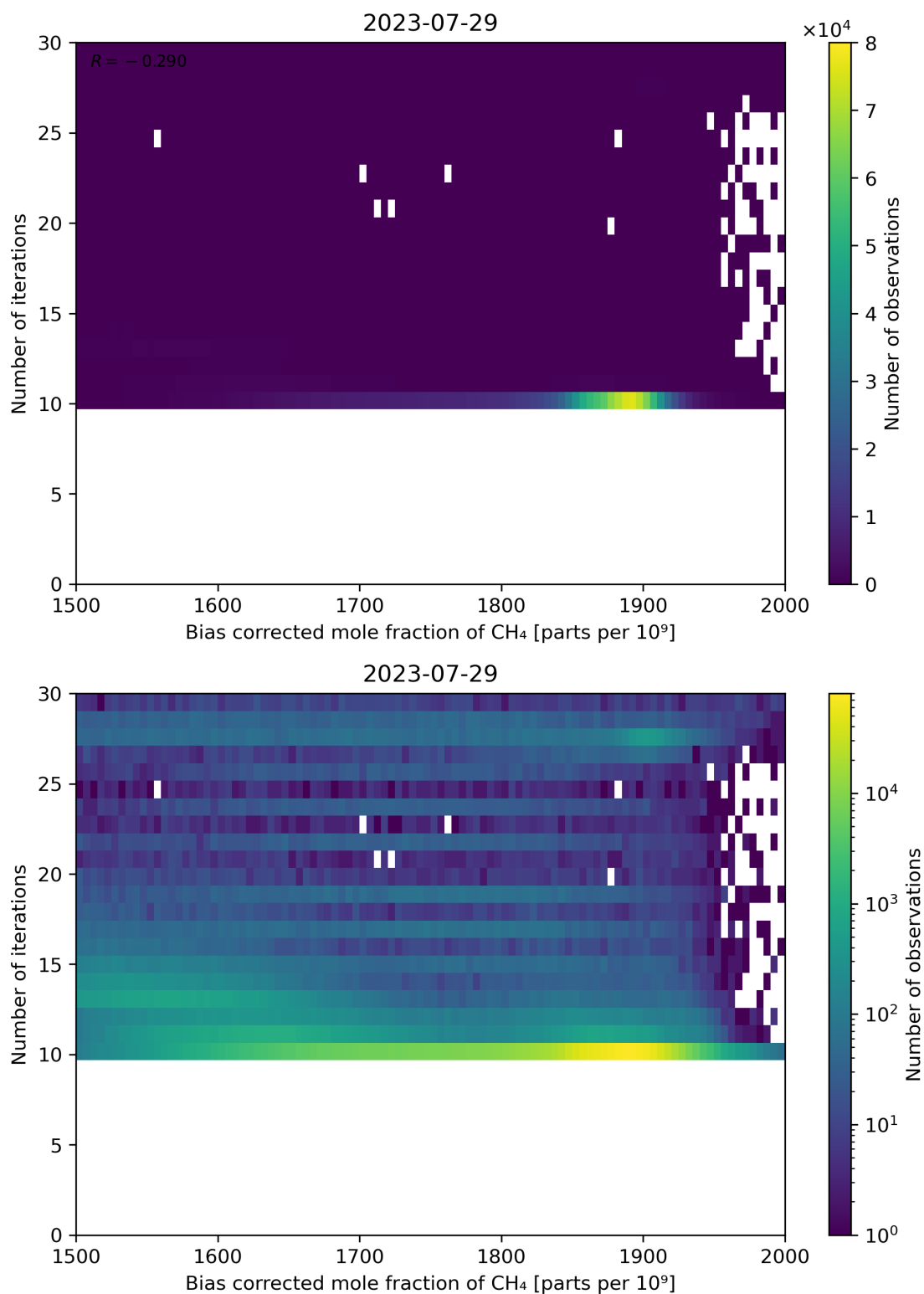
Figure 67: Scatter density plot of “Bias corrected mole fraction of \text{CH}_4 ” against “Number of iterations” for 2023-07-29 to 2023-07-30.
