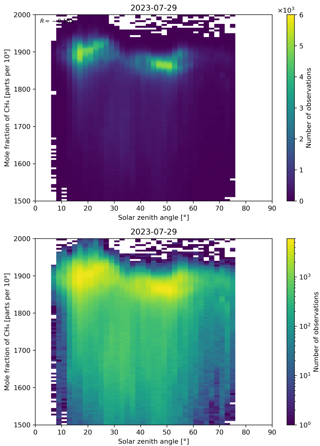
Figure 99: Scatter density plot of “Solar zenith angle” against “Mole fraction of CH 4 ” for 2023-07-29 to 2023-07-30.
