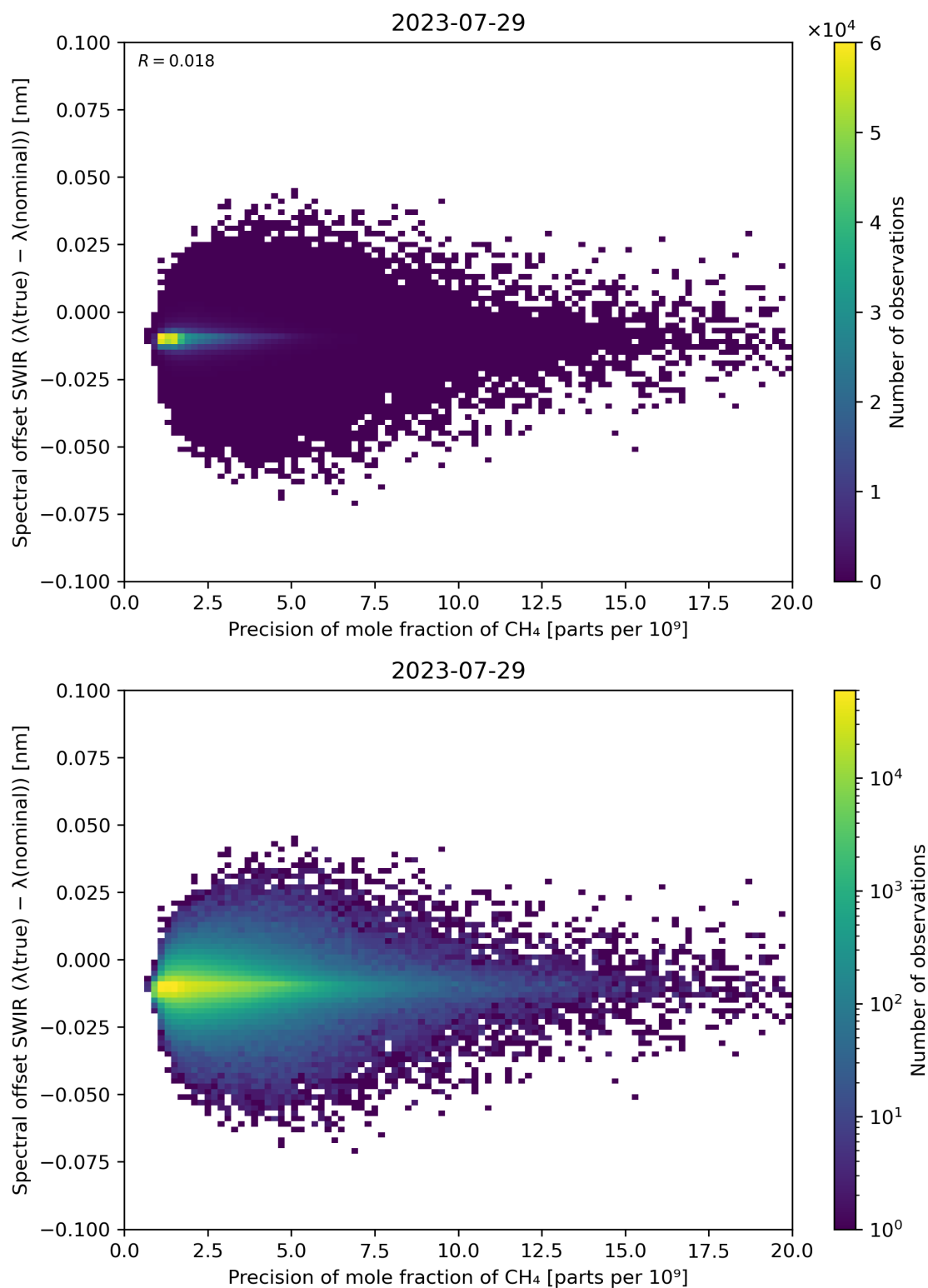
Figure 85: Scatter density plot of “Precision of mole fraction of CH 4 ” against “Spectral offset SWIR ( \lambda(\text{true}) - \lambda(\text{nominal}) )” for 2023-07-29 to 2023-07-30.
