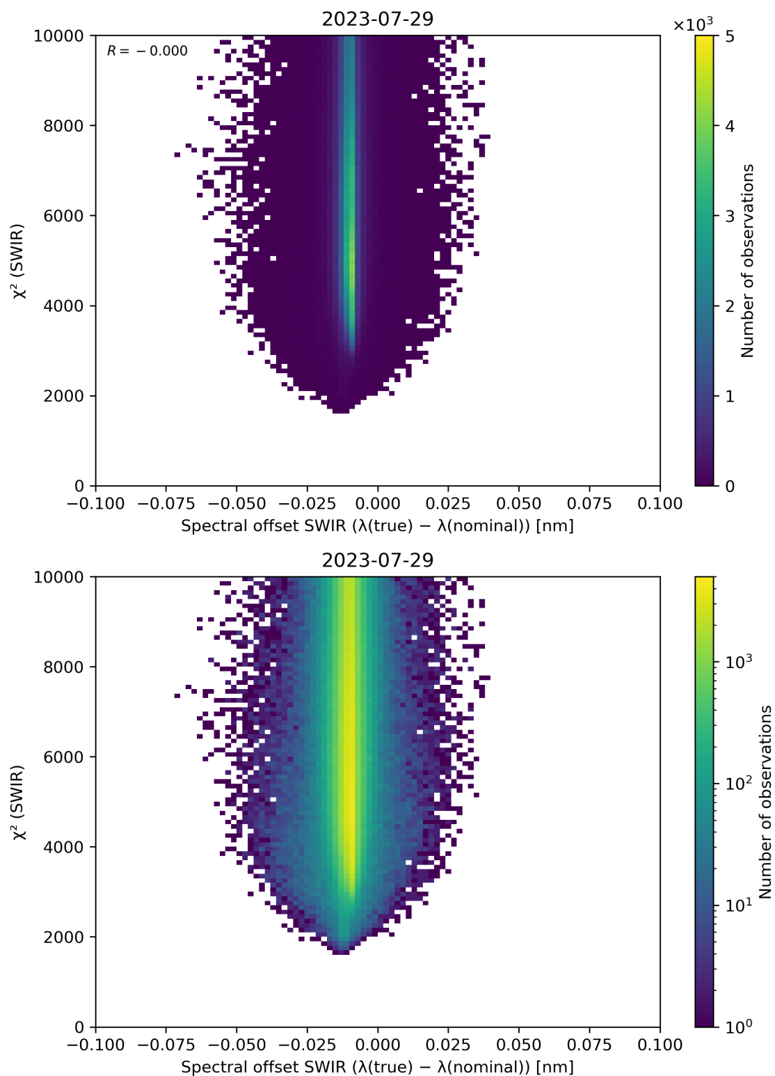
Figure 118: Scatter density plot of “Spectral offset SWIR ( \lambda(\text{true}) - \lambda(\text{nominal}) )” against “ \chi^2 (SWIR)” for 2023-07-29 to 2023-07-30.
