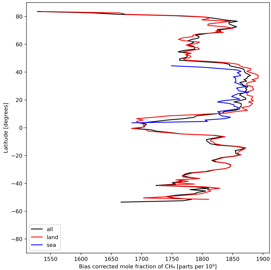
Figure 14: Zonal average of “Bias corrected mole fraction of \text{CH}_4 ” for 2023-07-29 to 2023-07-30.
