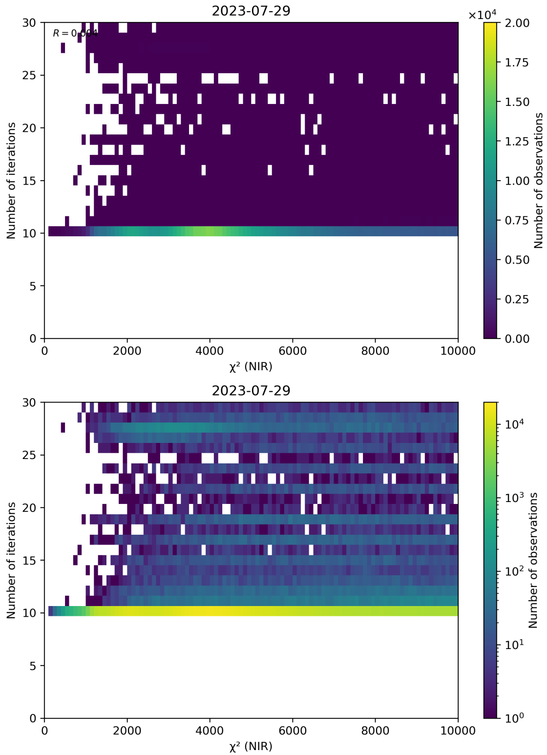
Figure 46: Scatter density plot of “ \chi^2 (NIR)” against “Number of iterations” for 2023-07-29 to 2023-07-30.
