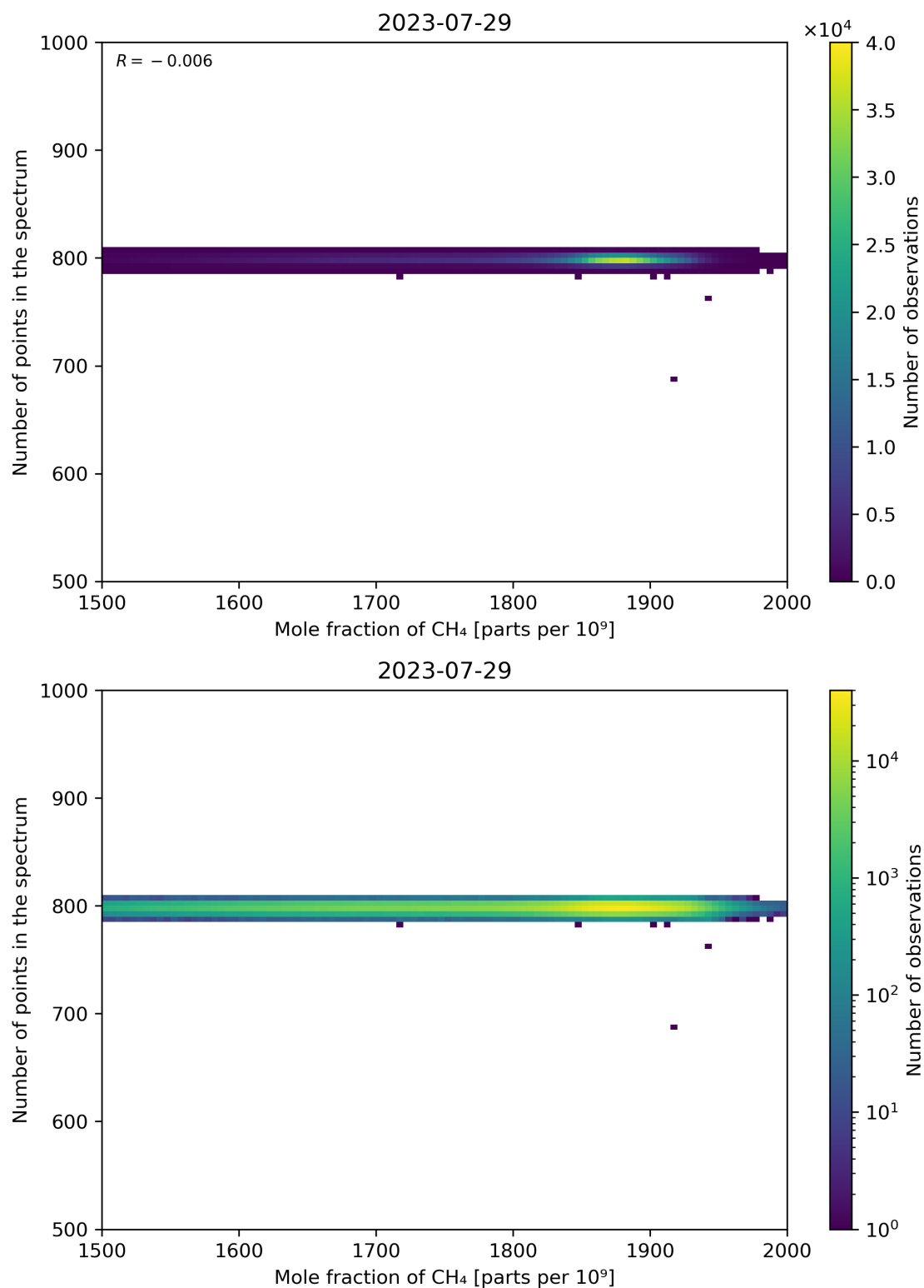
Figure 77: Scatter density plot of “Mole fraction of CH 4 ” against “Number of points in the spectrum” for 2023-07-29 to 2023-07-30.
