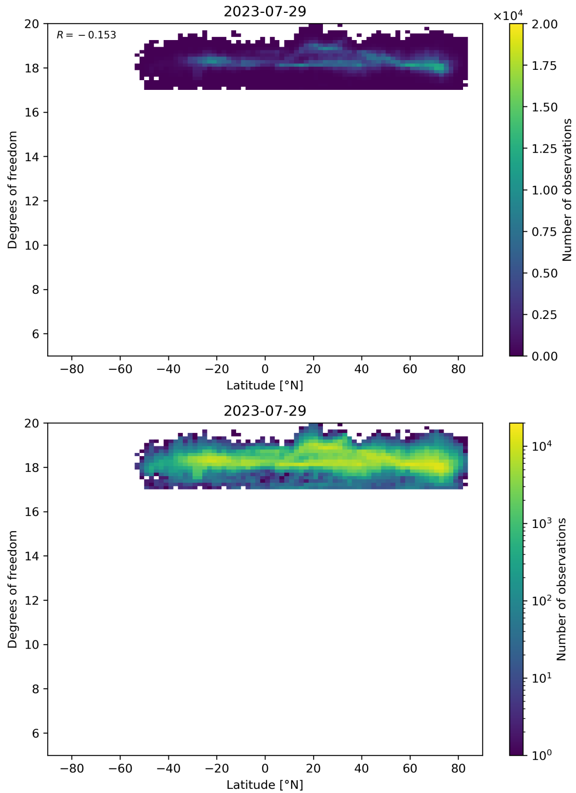
Figure 55: Scatter density plot of “Latitude” against “Degrees of freedom” for 2023-07-29 to 2023-07-30.
