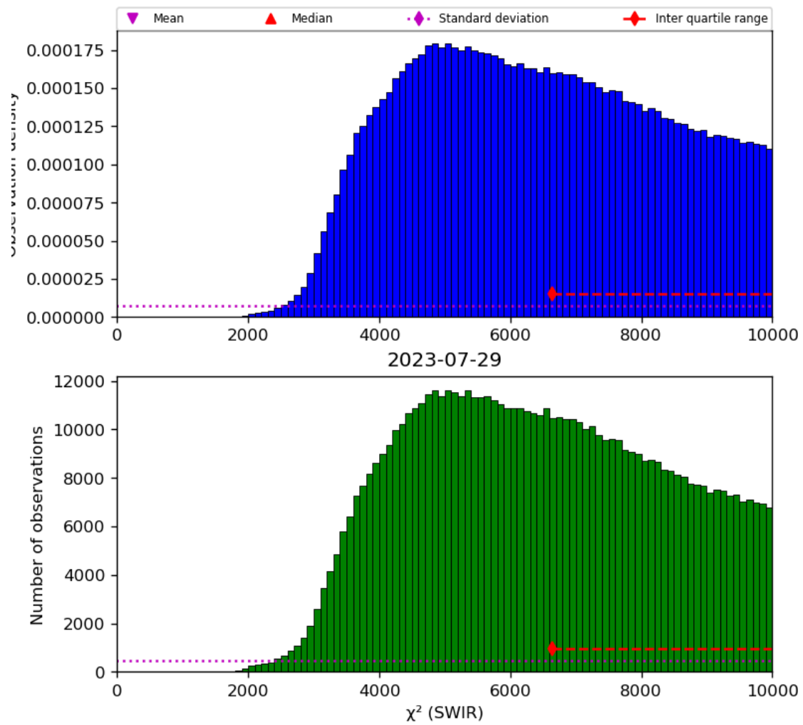
Figure 28: Histogram of “ \chi^2 (SWIR)” for 2023-07-29 to 2023-07-30
