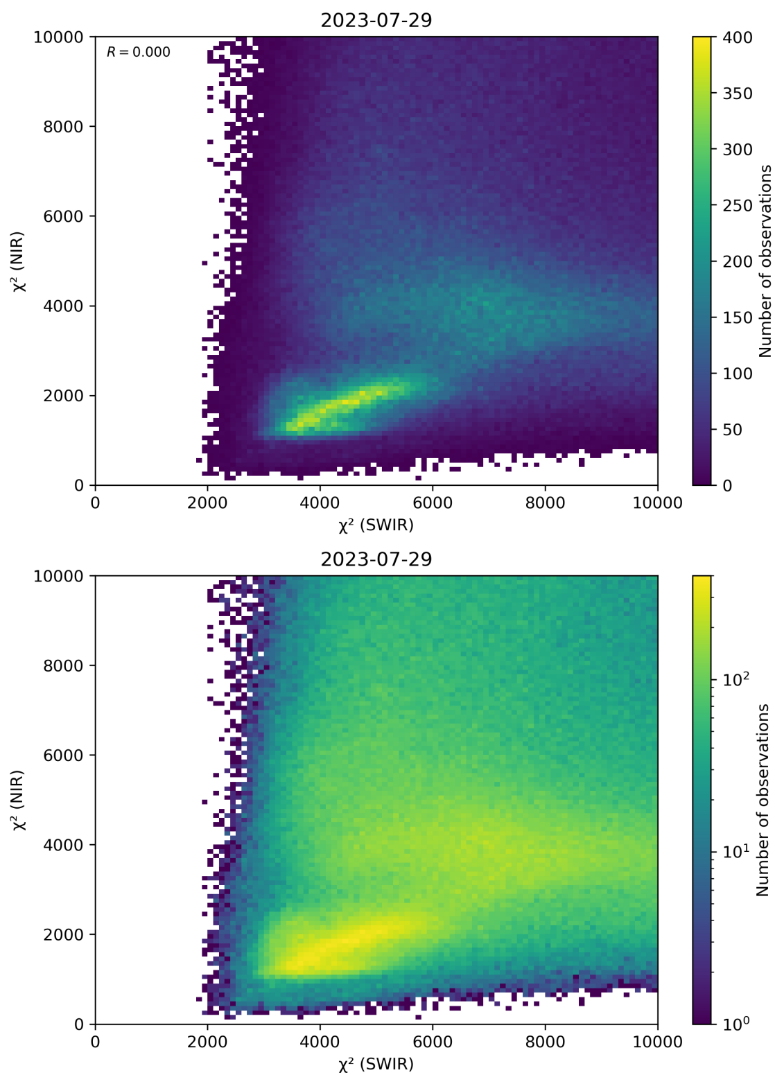
Figure 47: Scatter density plot of “ \chi^2 (SWIR)” against “ \chi^2 (NIR)” for 2023-07-29 to 2023-07-30.
