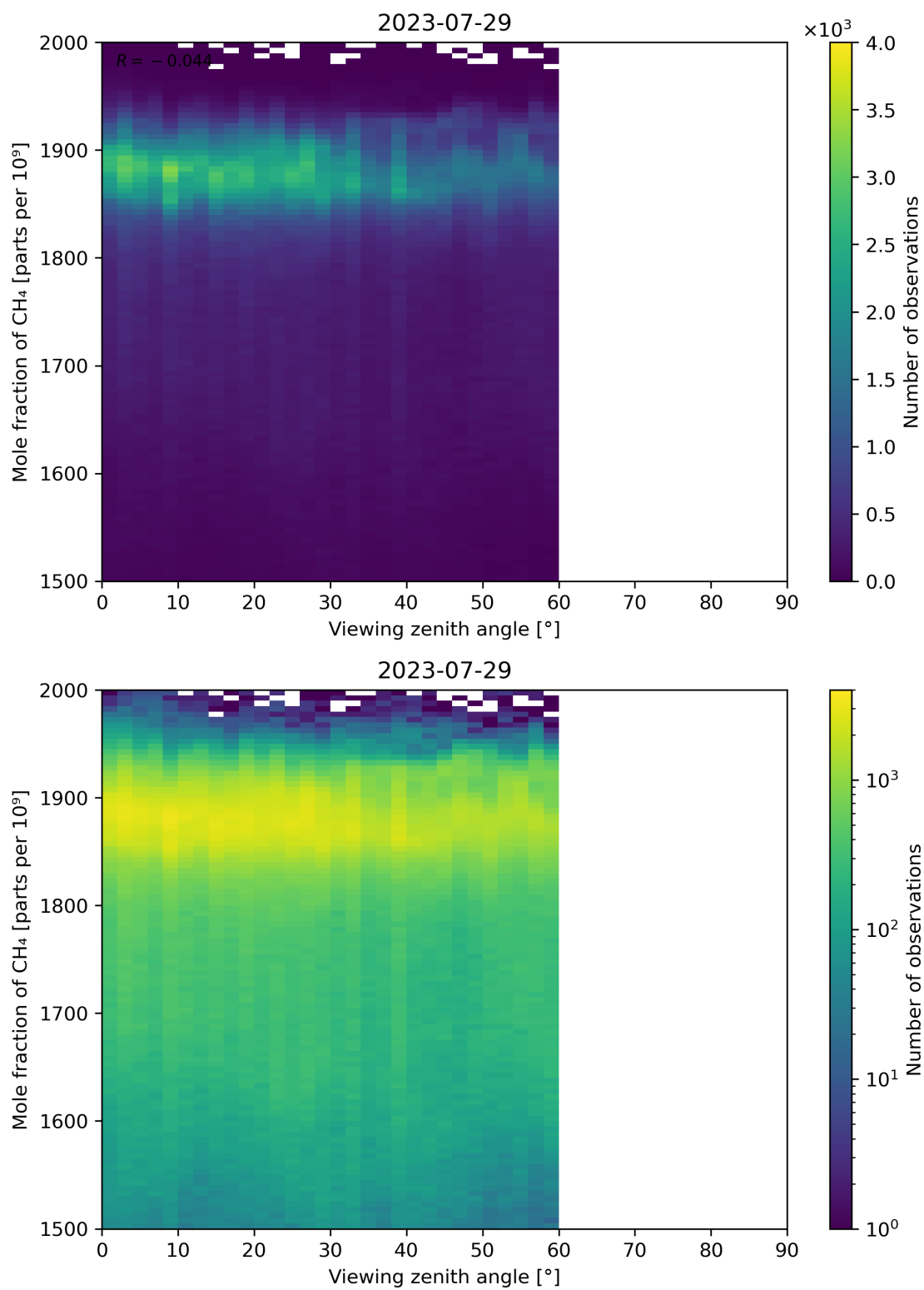
Figure 110: Scatter density plot of “Viewing zenith angle” against “Mole fraction of CH 4 ” for 2023-07-29 to 2023-07-30.
