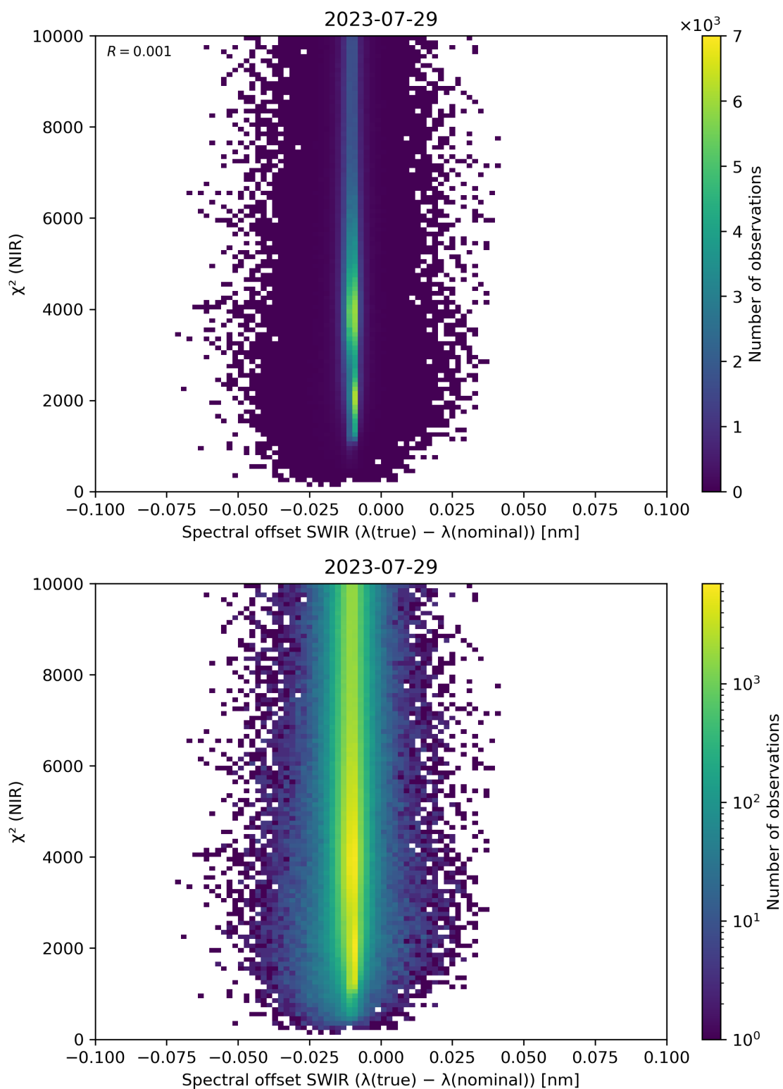
Figure 117: Scatter density plot of “Spectral offset SWIR ( \lambda(\text{true}) - \lambda(\text{nominal}) )” against “ \chi^2 (NIR)” for 2023-07-29 to 2023-07-30.
