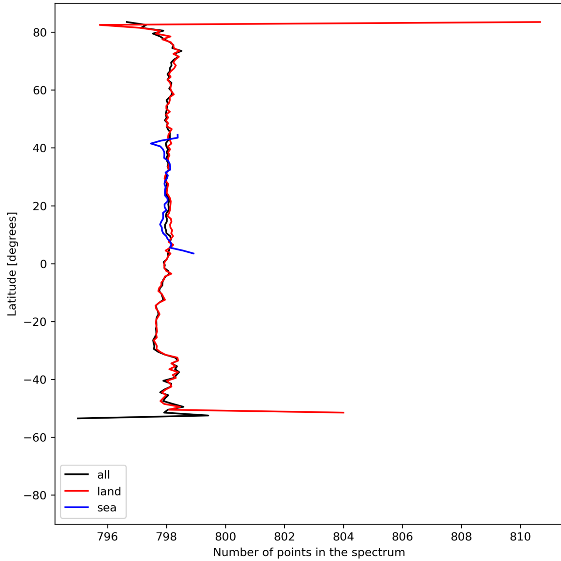
Figure 15: Zonal average of “Number of points in the spectrum” for 2023-07-29 to 2023-07-30.
