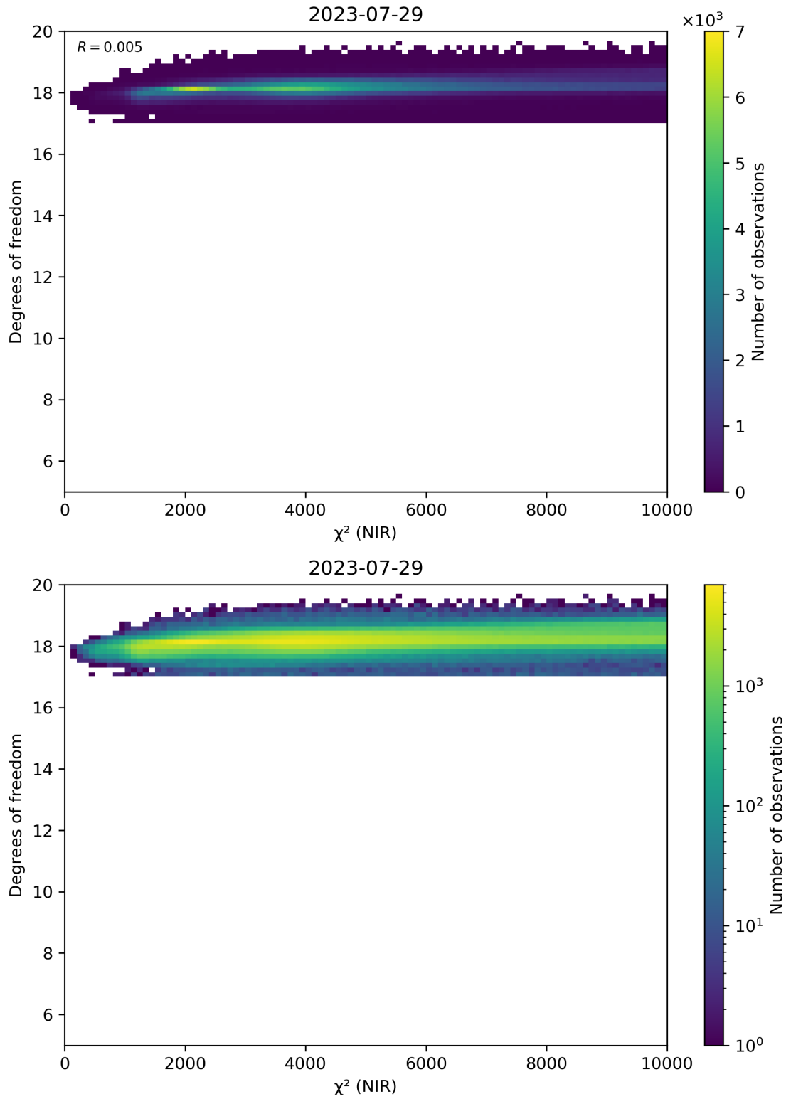
Figure 44: Scatter density plot of “ \chi^2 (NIR)” against “Degrees of freedom” for 2023-07-29 to 2023-07-30.
