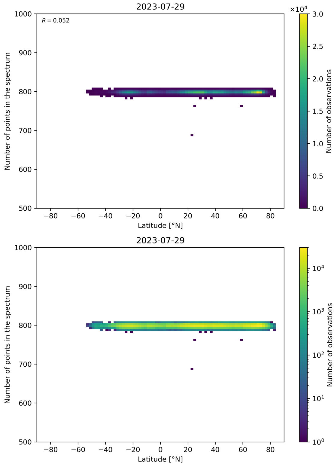
Figure 61: Scatter density plot of “Latitude” against “Number of points in the spectrum” for 2023-07-29 to 2023-07-30.
