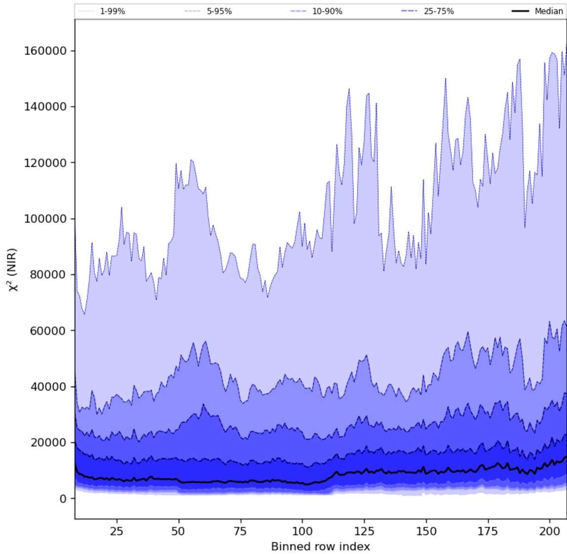
Figure 40: Along track statistics of " \chi^2 (NIR)" for 2023-07-29 to 2023-07-30
