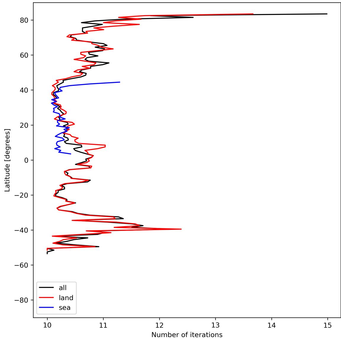
Figure 20: Zonal average of “Number of iterations” for 2023-07-29 to 2023-07-30.
