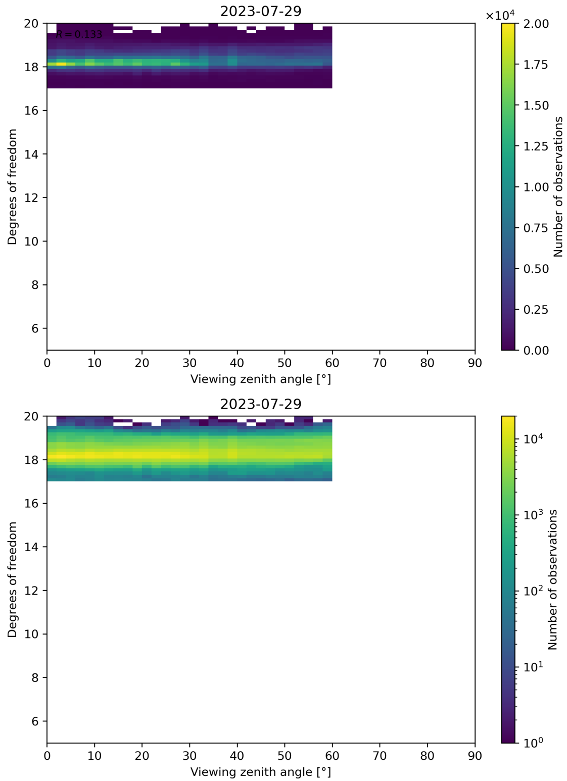
Figure 107: Scatter density plot of “Viewing zenith angle” against “Degrees of freedom” for 2023-07-29 to 2023-07-30.
