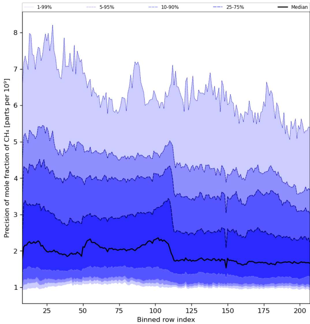
Figure 35: Along track statistics of “Precision of mole fraction of CH 4 ” for 2023-07-29 to 2023-07-30
