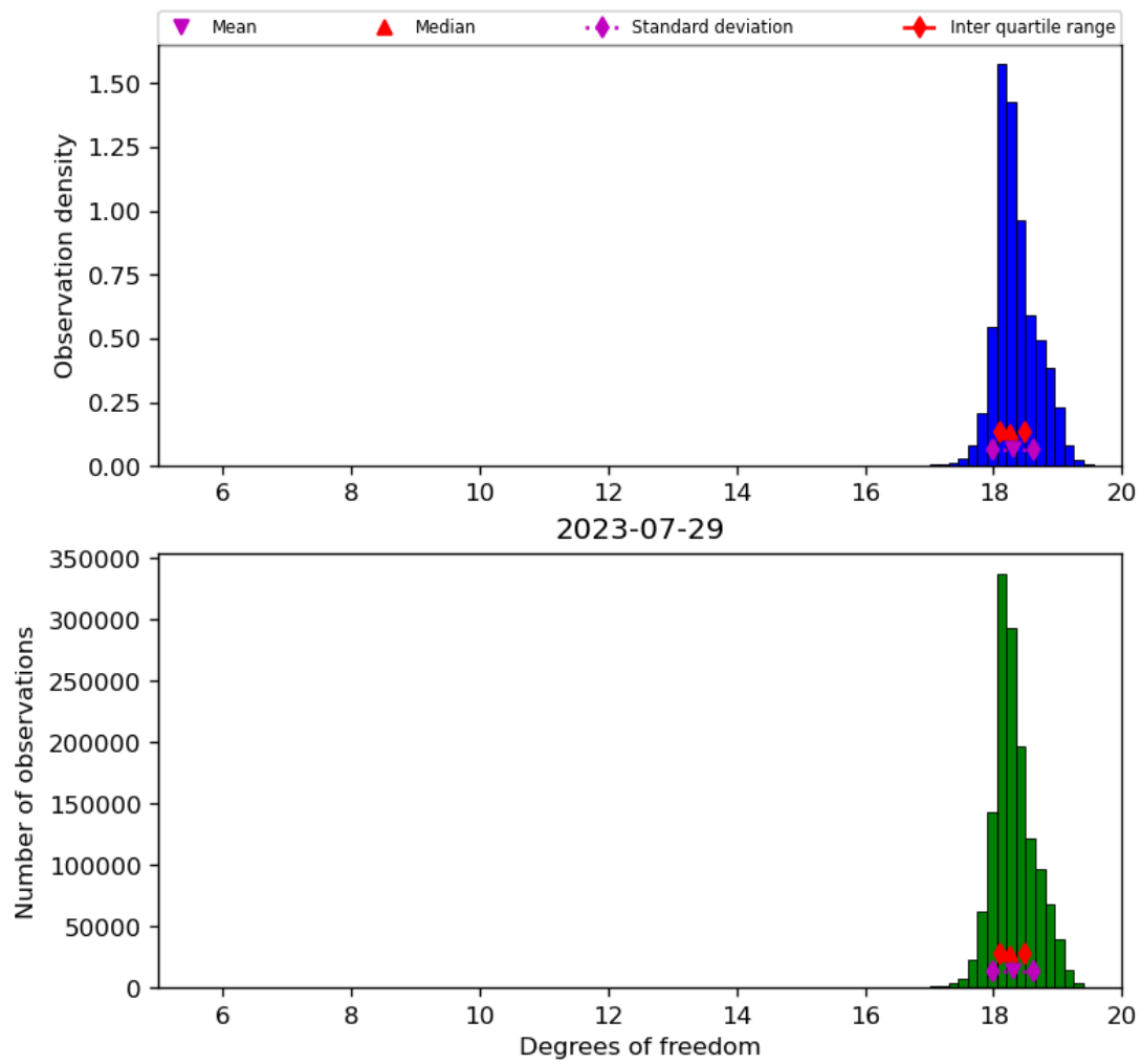
Figure 30: Histogram of “Degrees of freedom” for 2023-07-29 to 2023-07-30
