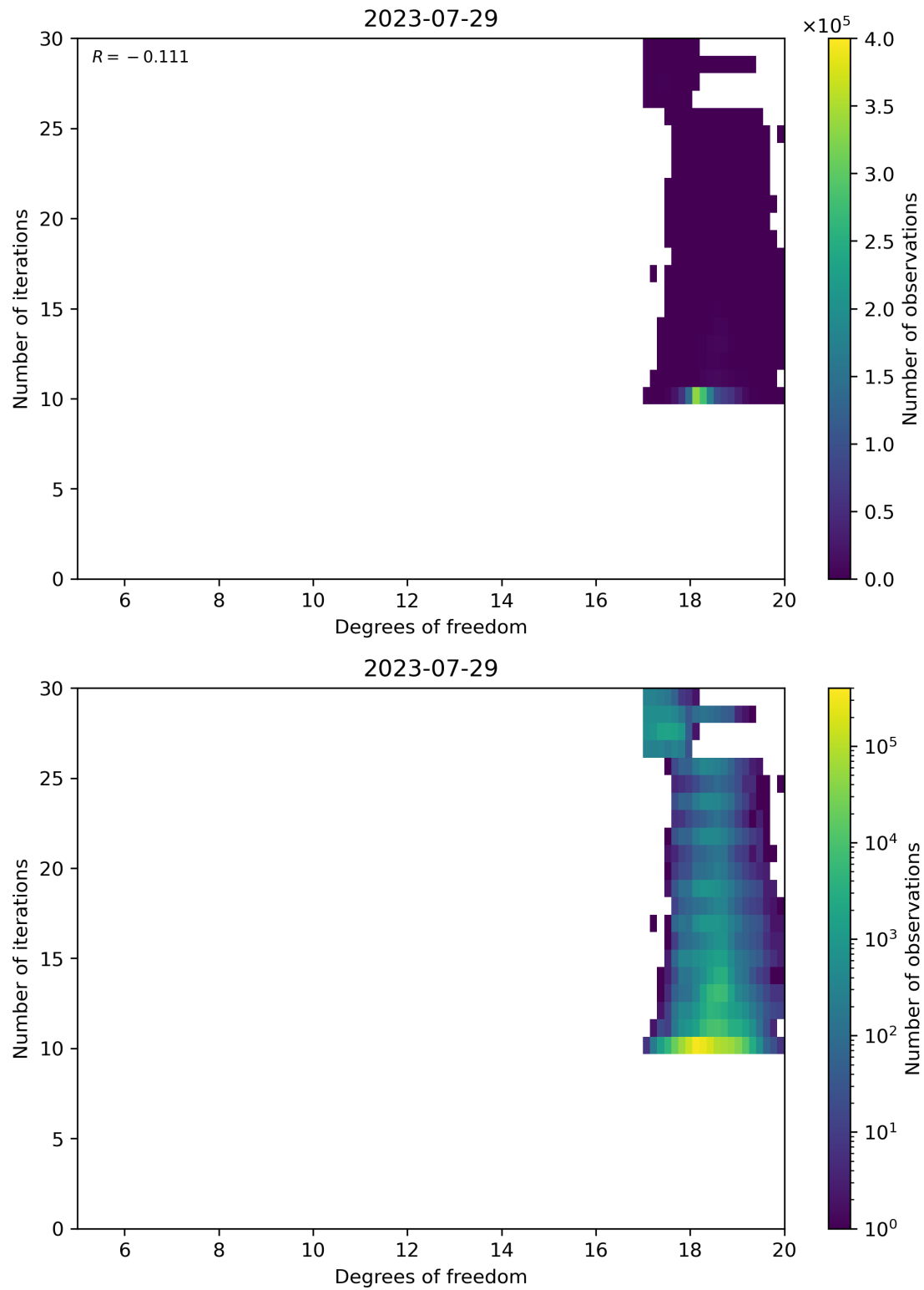
Figure 52: Scatter density plot of “Degrees of freedom” against “Number of iterations” for 2023-07-29 to 2023-07-30.
