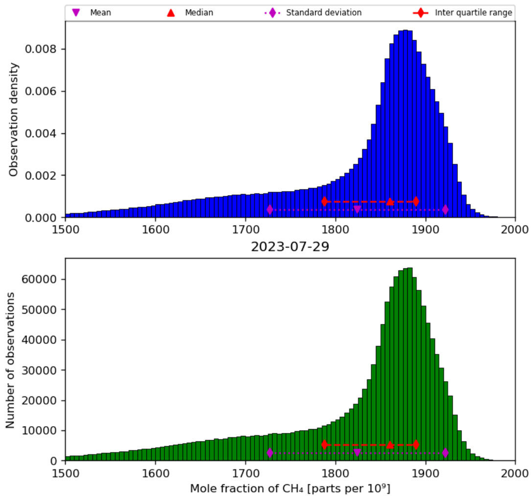
Figure 23: Histogram of “Mole fraction of CH 4 ” for 2023-07-29 to 2023-07-30
