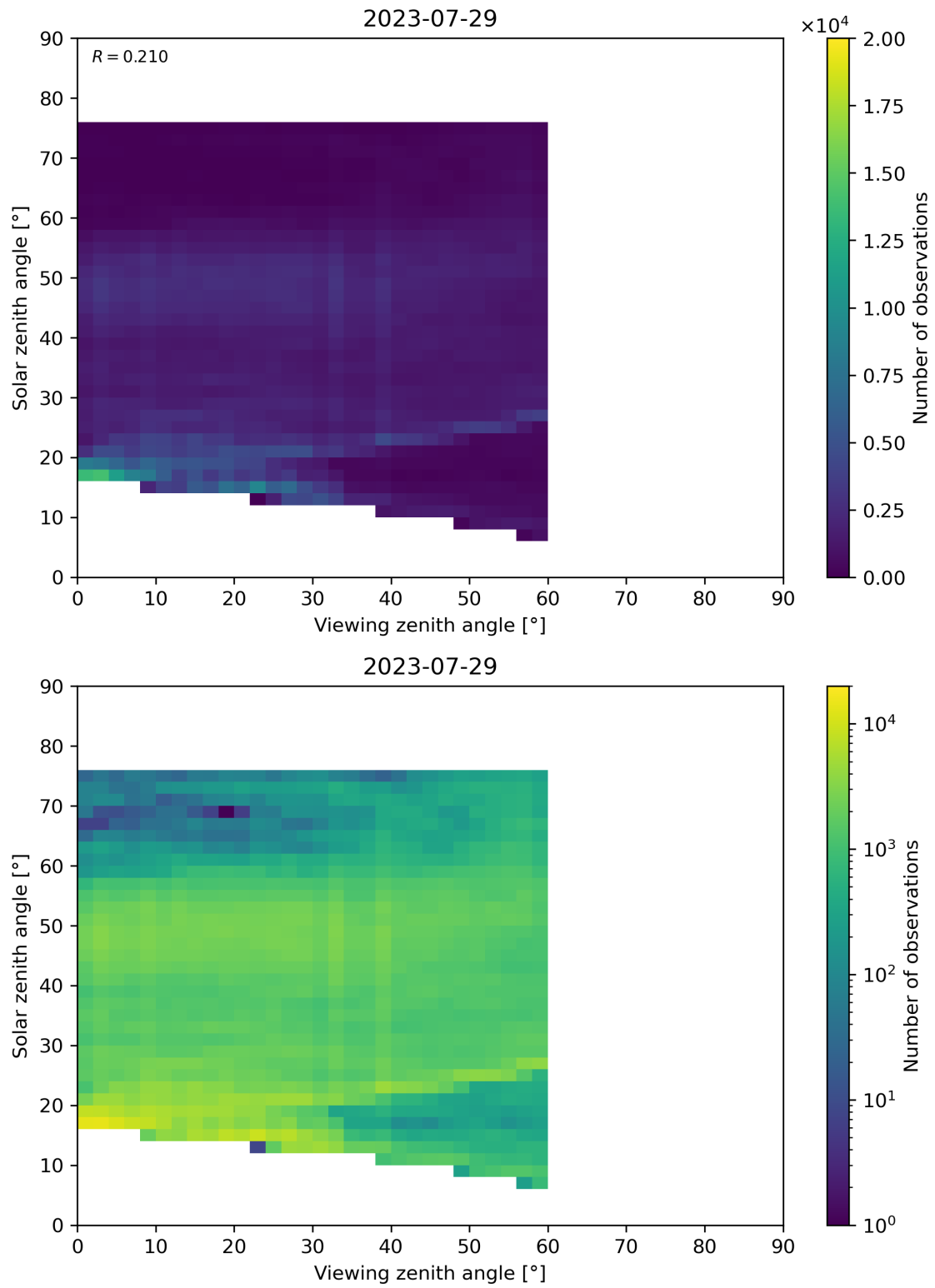
Figure 115: Scatter density plot of “Viewing zenith angle” against “Solar zenith angle” for 2023-07-29 to 2023-07-30.
