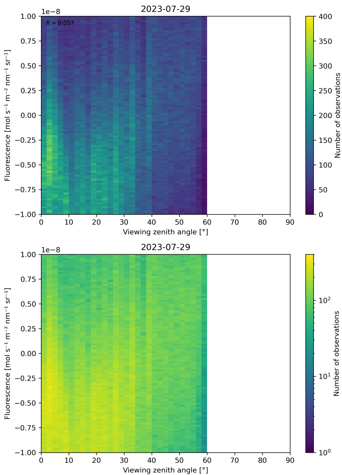
Figure 108: Scatter density plot of “Viewing zenith angle” against “Fluorescence” for 2023-07-29 to 2023-07-30.
