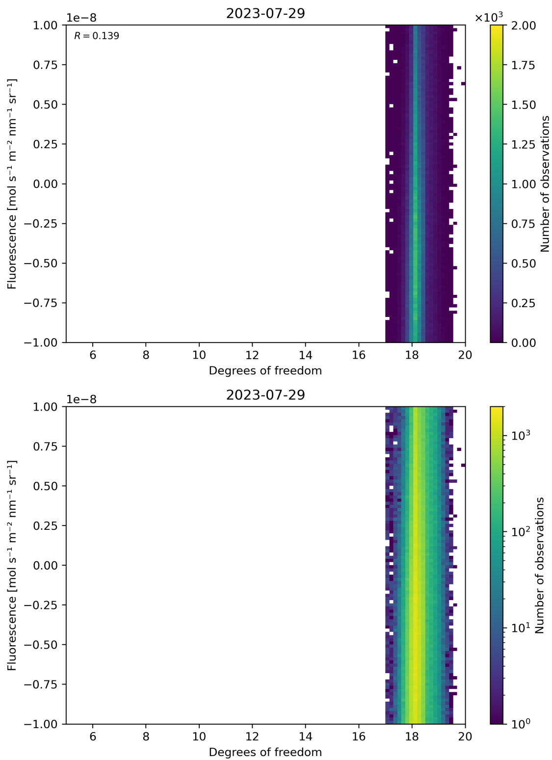
Figure 51: Scatter density plot of “Degrees of freedom” against “Fluorescence” for 2023-07-29 to 2023-07-30.
