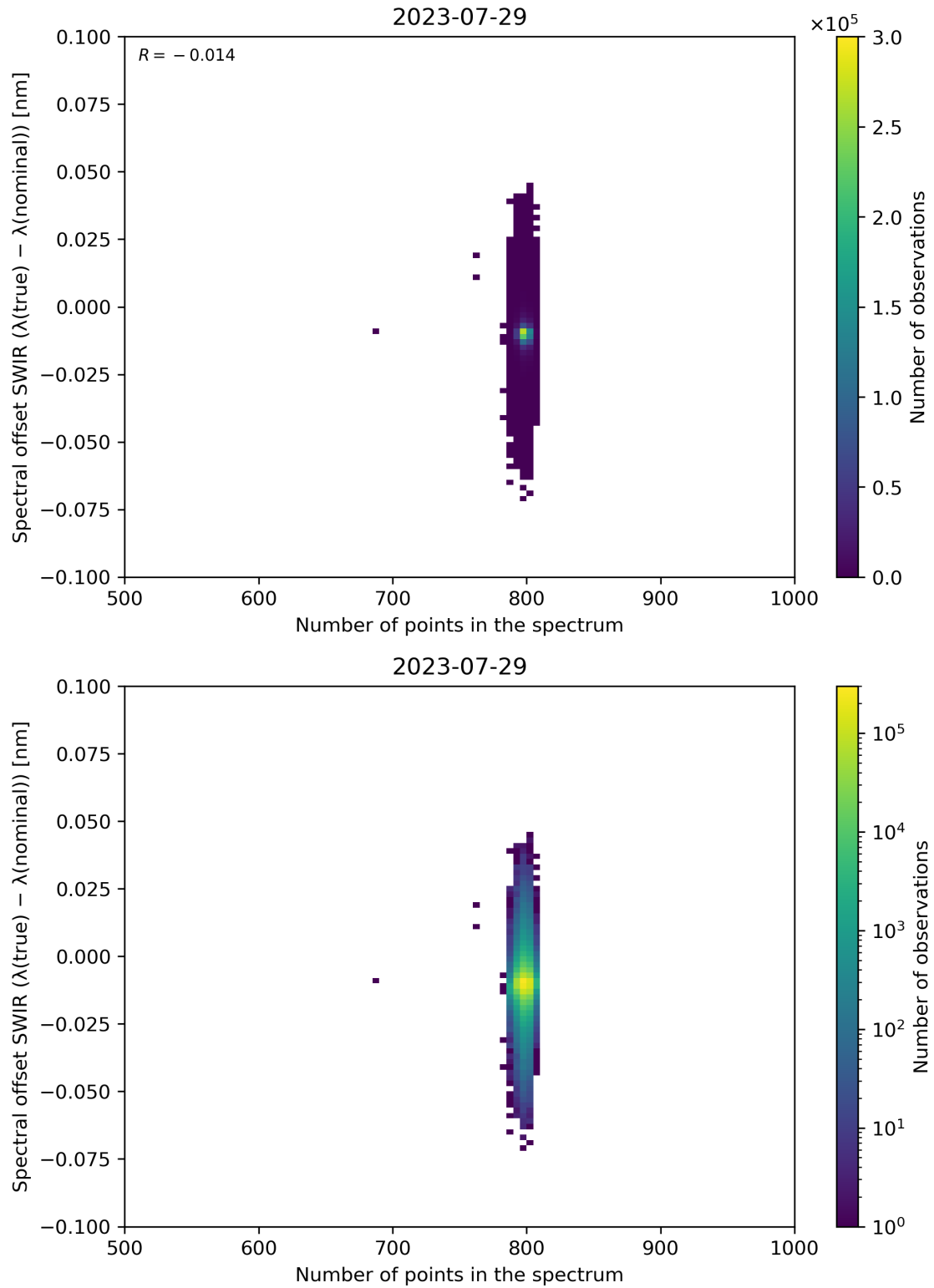
Figure 93: Scatter density plot of “Number of points in the spectrum” against “Spectral offset SWIR ( \lambda(\text{true}) - \lambda(\text{nominal}) )” for 2023-07-29 to 2023-07-30.
