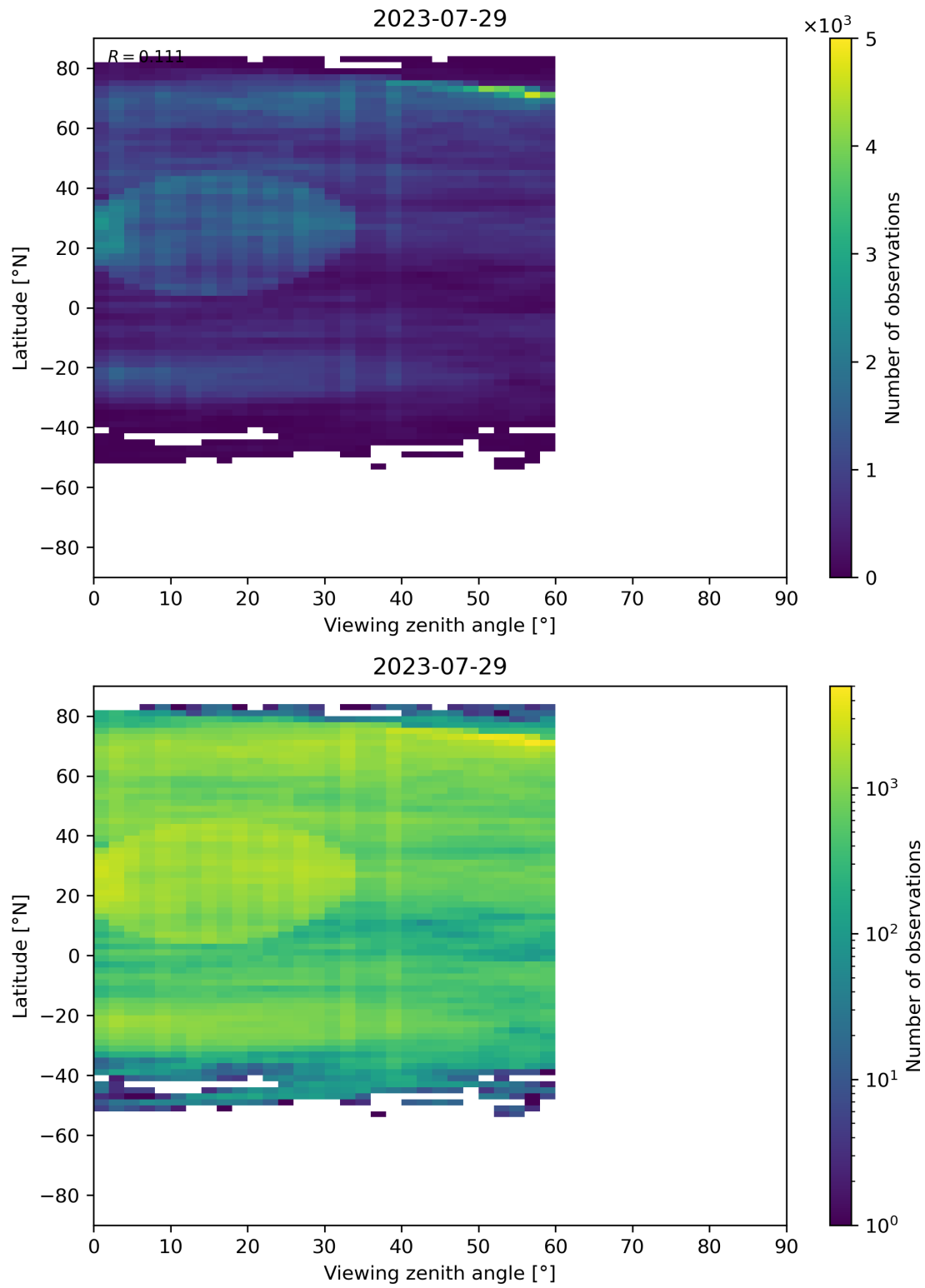
Figure 109: Scatter density plot of “Viewing zenith angle” against “Latitude” for 2023-07-29 to 2023-07-30.
