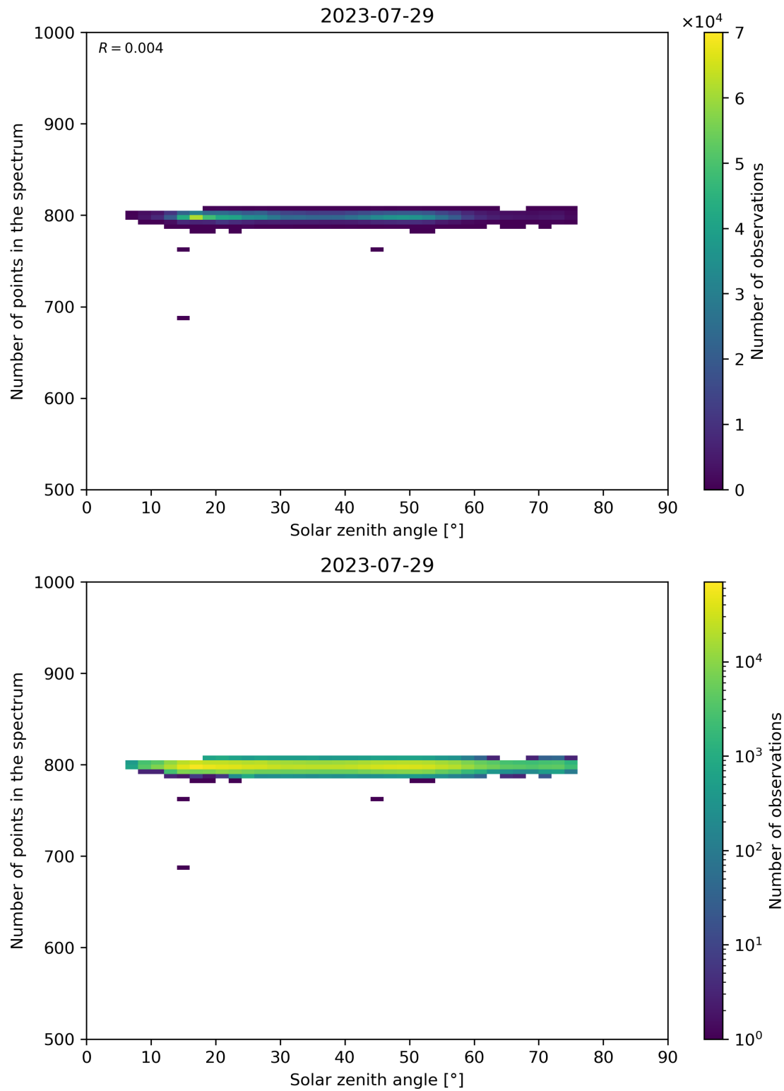
Figure 103: Scatter density plot of “Solar zenith angle” against “Number of points in the spectrum” for 2023-07-29 to 2023-07-30.
