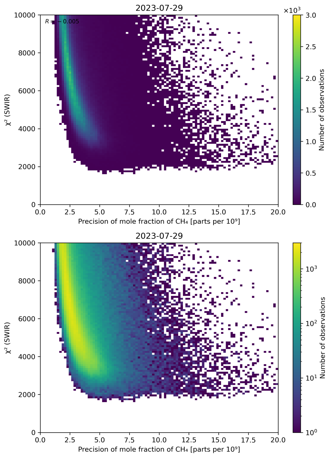
Figure 79: Scatter density plot of “Precision of mole fraction of \text{CH}_4 ” against “ \chi^2 (SWIR)” for 2023-07-29 to 2023-07-30.
