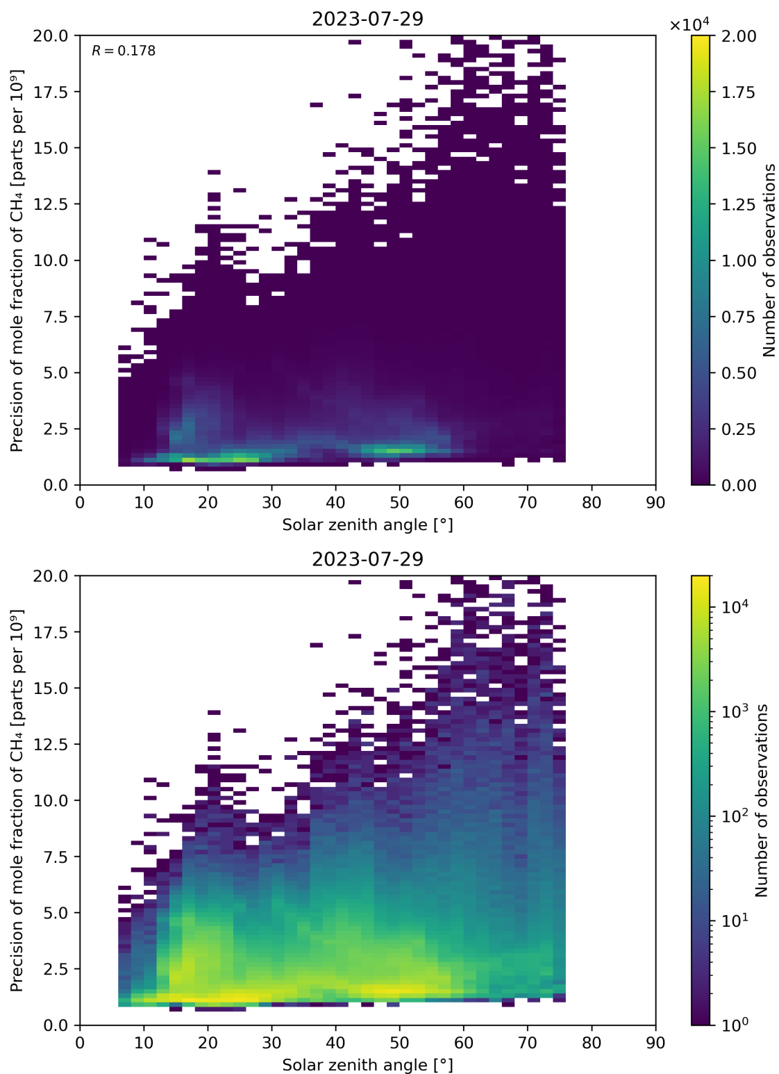
Figure 101: Scatter density plot of “Solar zenith angle” against “Precision of mole fraction of CH 4 ” for 2023-07-29 to 2023-07-30.
