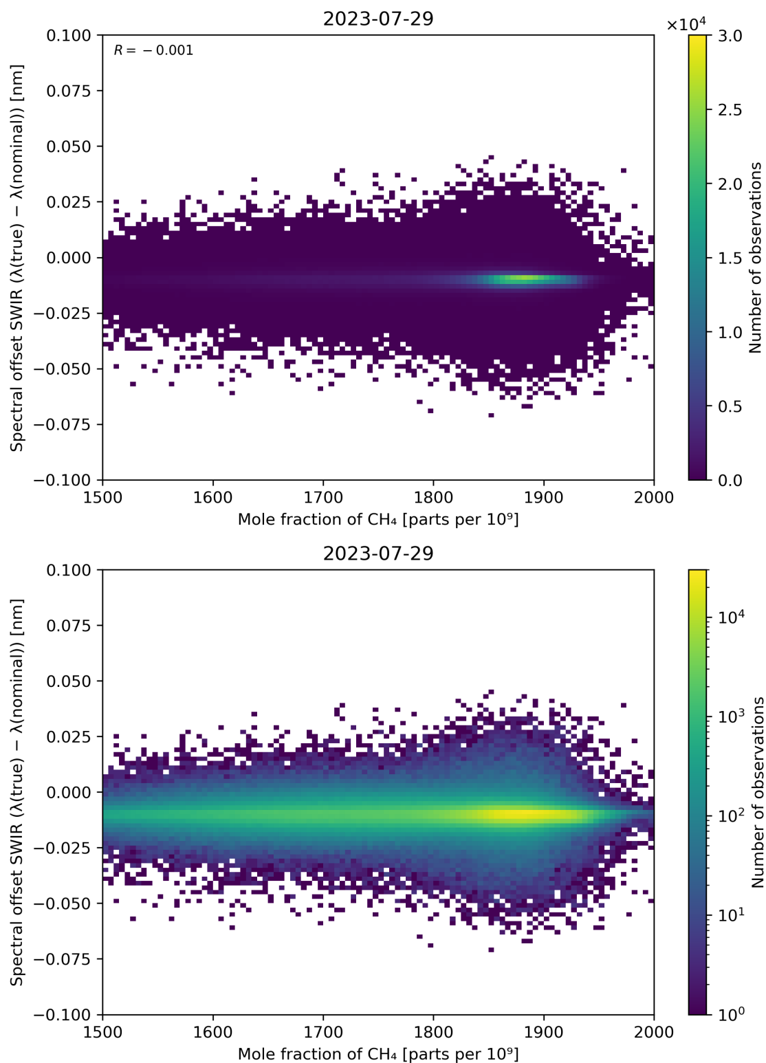
Figure 86: Scatter density plot of “Mole fraction of CH 4 ” against “Spectral offset SWIR ( \lambda(\text{true}) - \lambda(\text{nominal}) )” for 2023-07-29 to 2023-07-30.
