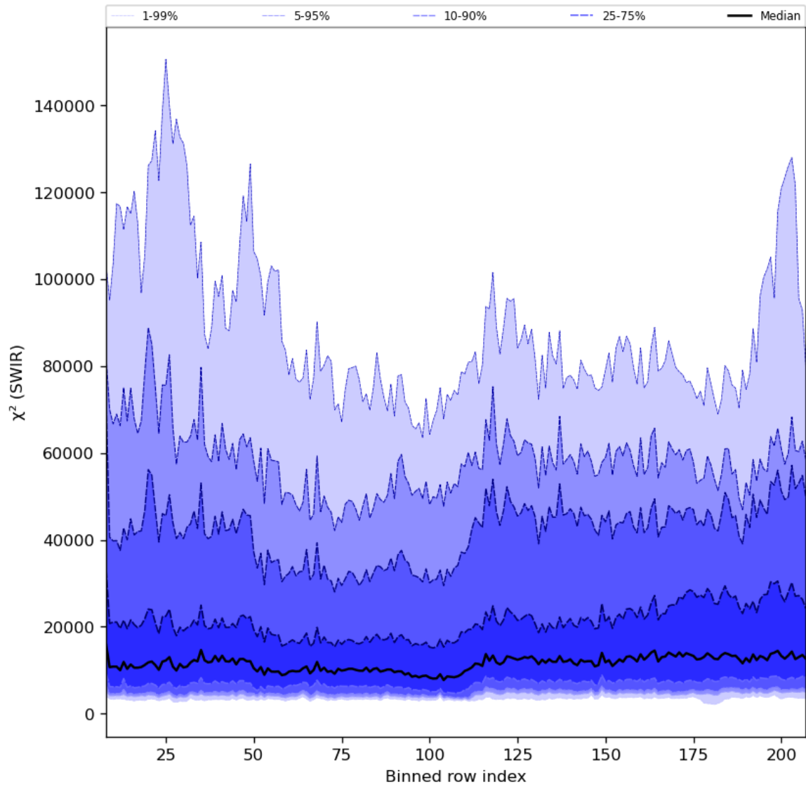
Figure 39: Along track statistics of “ \chi^2 (SWIR)” for 2023-07-29 to 2023-07-30
