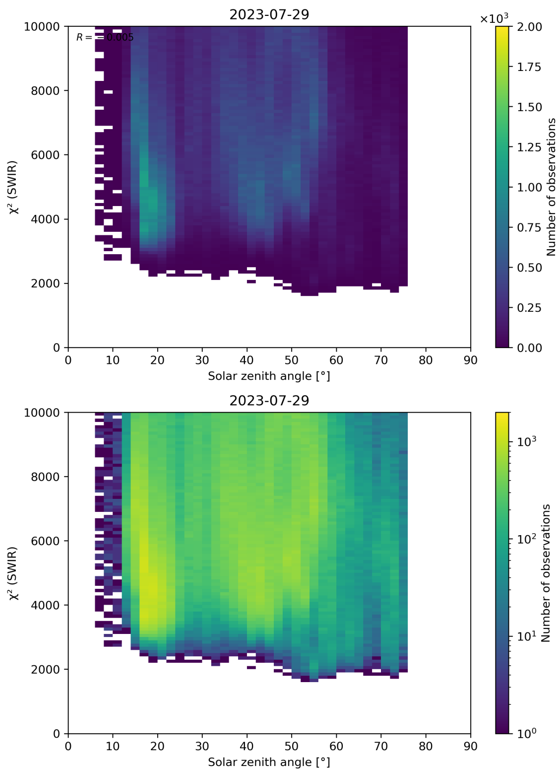
Figure 95: Scatter density plot of “Solar zenith angle” against “ \chi^2 (SWIR)” for 2023-07-29 to 2023-07-30.
