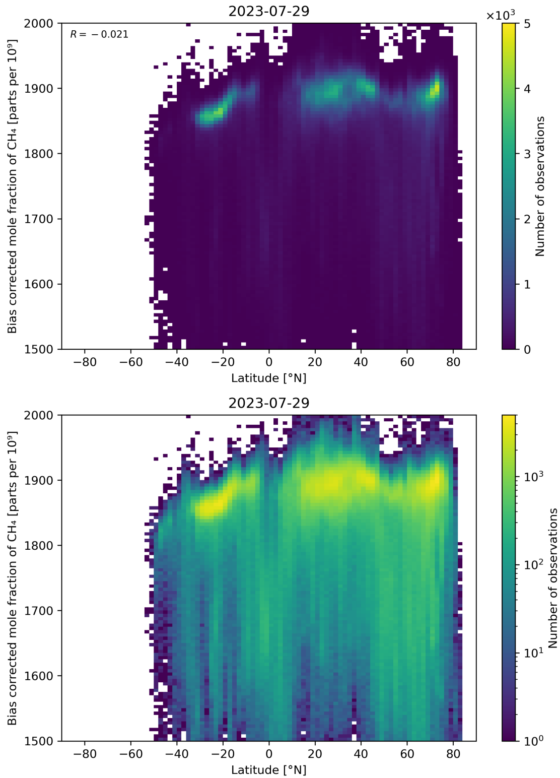
Figure 58: Scatter density plot of “Latitude” against “Bias corrected mole fraction of \text{CH}_4 ” for 2023-07-29 to 2023-07-30.
