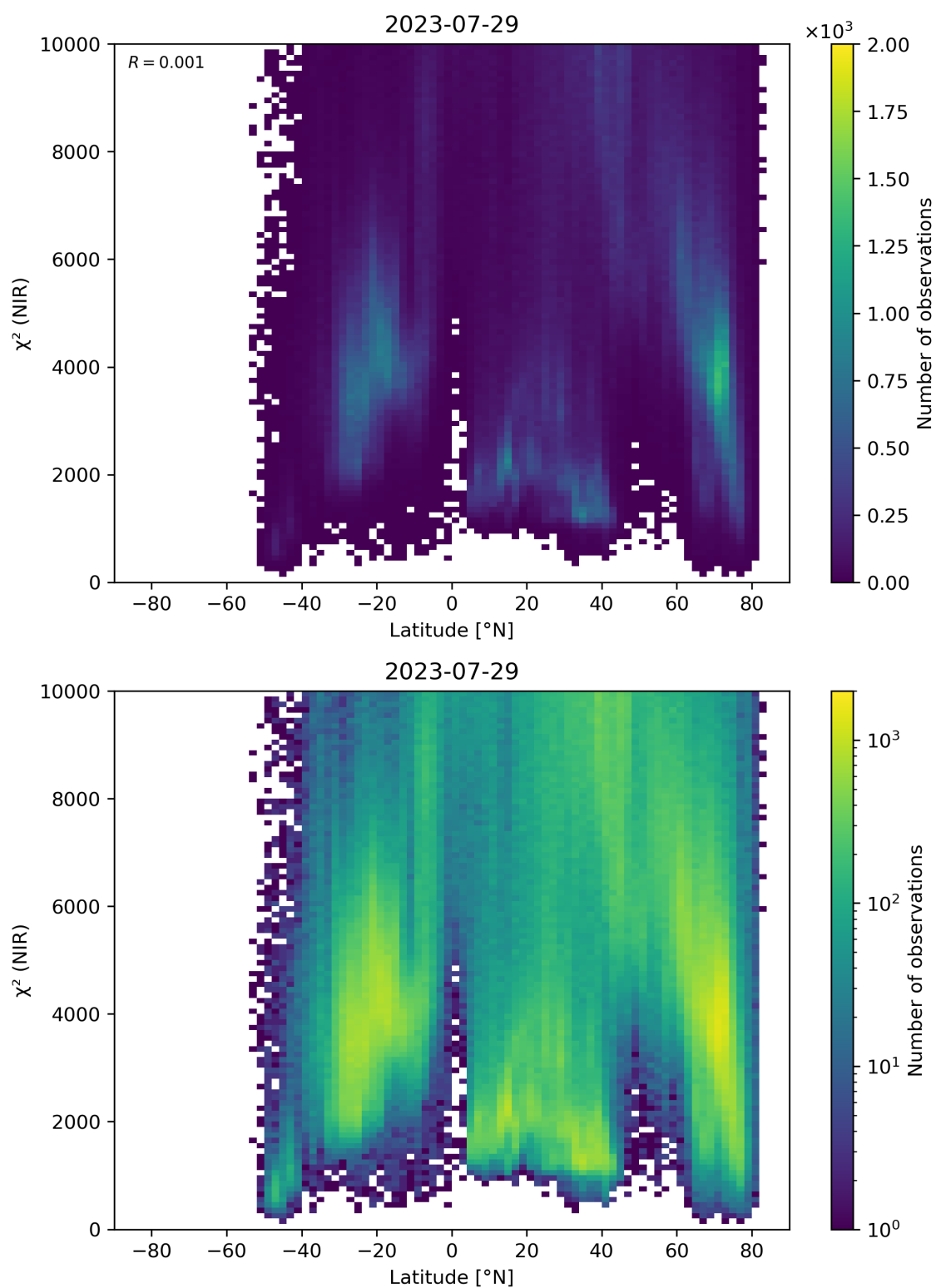
Figure 53: Scatter density plot of “Latitude” against “ \chi^2 (NIR)” for 2023-07-29 to 2023-07-30.
