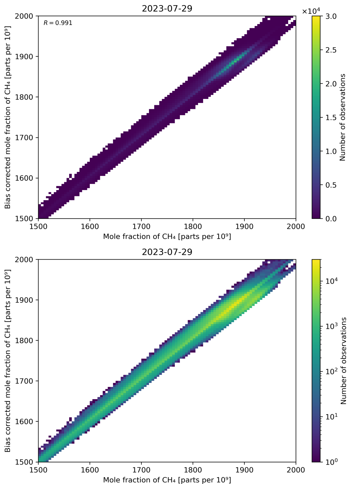
Figure 74: Scatter density plot of “Mole fraction of CH 4 ” against “Bias corrected mole fraction of CH 4 ” for 2023-07-29 to 2023-07-30.
