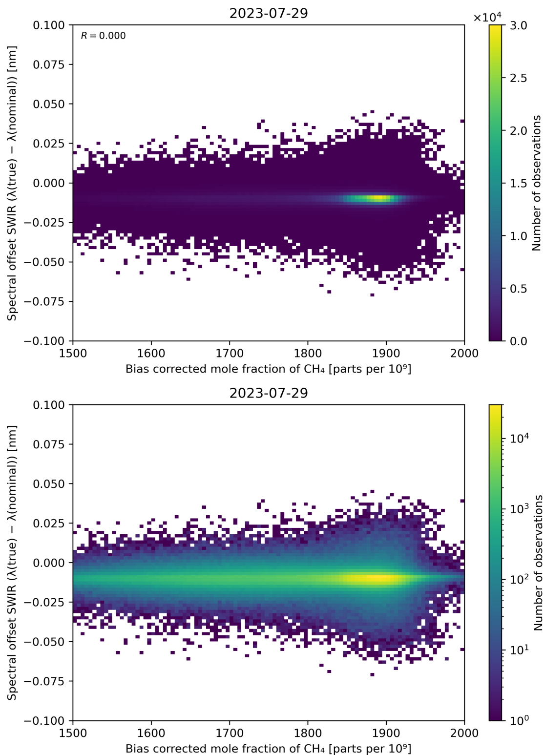
Figure 69: Scatter density plot of “Bias corrected mole fraction of \text{CH}_4 ” against “Spectral offset SWIR ( \lambda(\text{true}) - \lambda(\text{nominal}) )” for 2023-07-29 to 2023-07-30.
