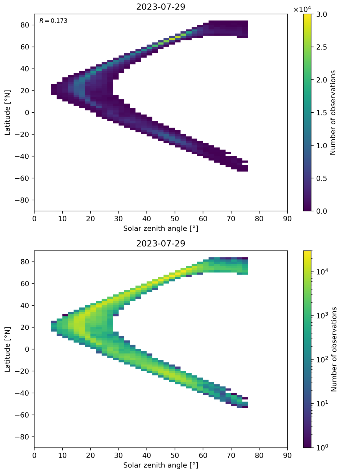
Figure 98: Scatter density plot of “Solar zenith angle” against “Latitude” for 2023-07-29 to 2023-07-30.
