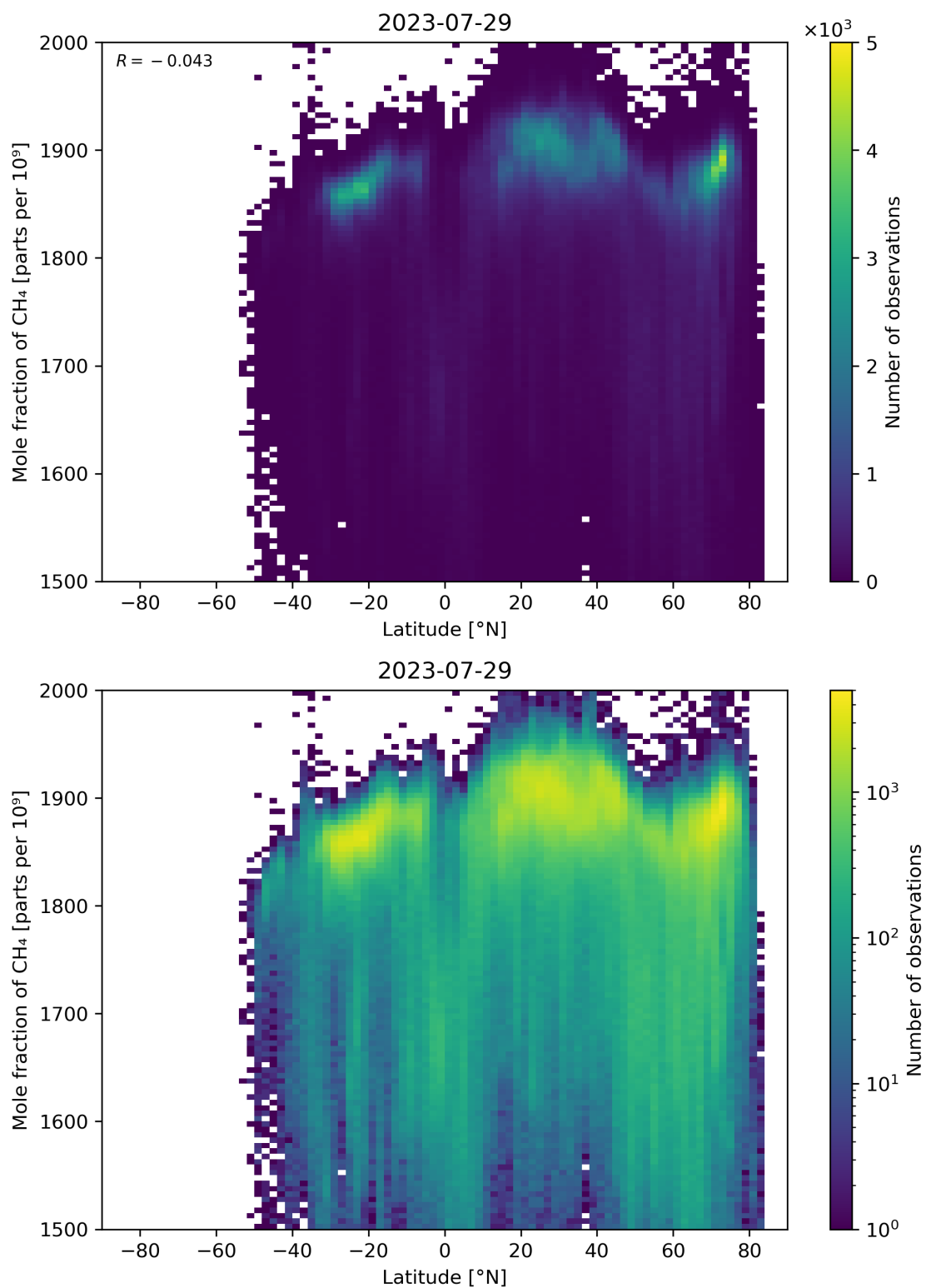
Figure 57: Scatter density plot of “Latitude” against “Mole fraction of CH 4 ” for 2023-07-29 to 2023-07-30.
