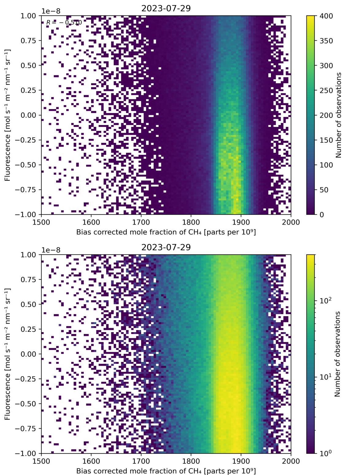
Figure 66: Scatter density plot of “Bias corrected mole fraction of \text{CH}_4 ” against “Fluorescence” for 2023-07-29 to 2023-07-30.
