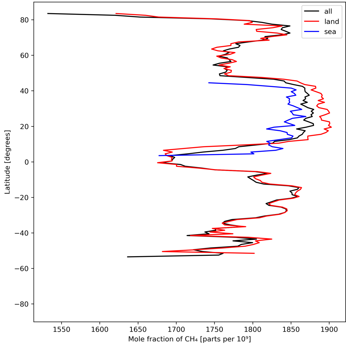
Figure 12: Zonal average of “Mole fraction of CH 4 ” for 2023-07-29 to 2023-07-30.
