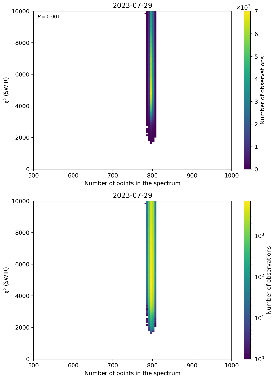
Figure 89: Scatter density plot of “Number of points in the spectrum” against “ \chi^2 (SWIR)” for 2023-07-29 to 2023-07-30.
