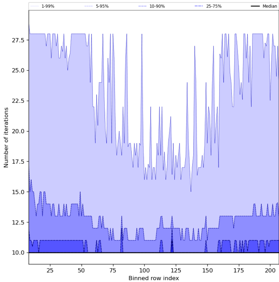
Figure 42: Along track statistics of “Number of iterations” for 2023-07-29 to 2023-07-30
