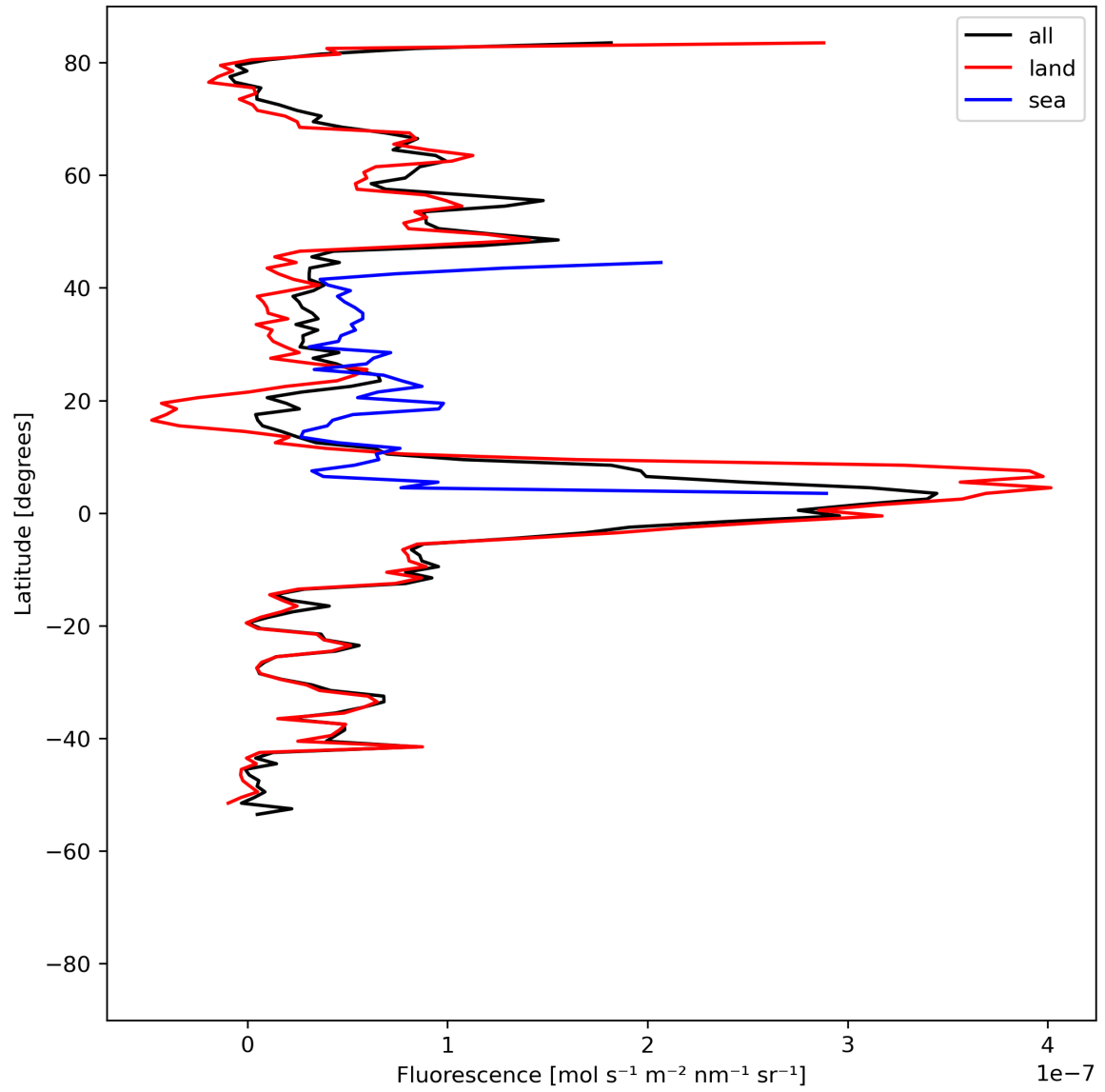
Figure 21: Zonal average of “Fluorescence” for 2023-07-29 to 2023-07-30.
