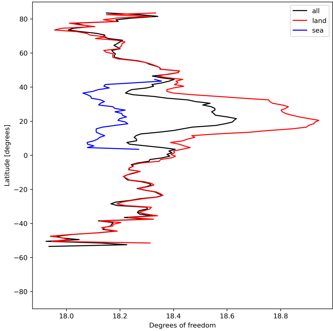
Figure 19: Zonal average of “Degrees of freedom” for 2023-07-29 to 2023-07-30.
