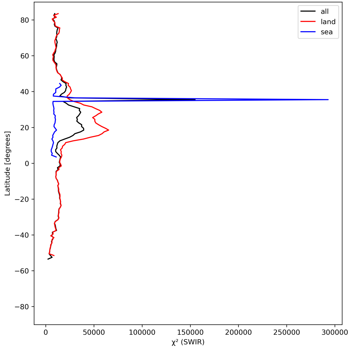
Figure 17: Zonal average of “ \chi^2 (SWIR)” for 2023-07-29 to 2023-07-30.
