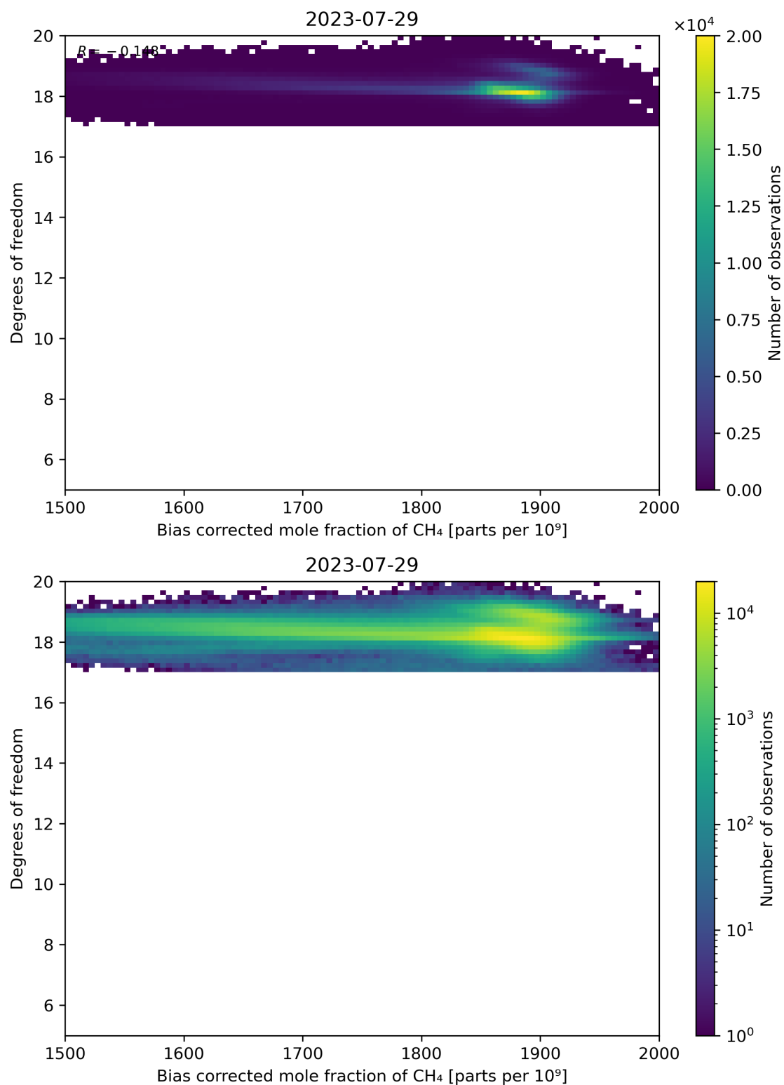
Figure 65: Scatter density plot of “Bias corrected mole fraction of CH 4 ” against “Degrees of freedom” for 2023-07-29 to 2023-07-30.
