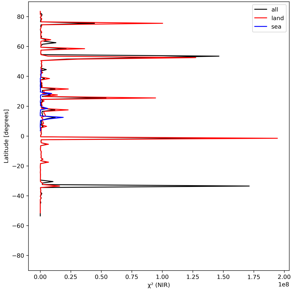
Figure 18: Zonal average of “ \chi^2 (NIR)” for 2023-07-29 to 2023-07-30.
