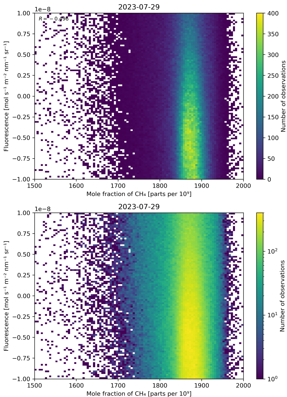
Figure 73: Scatter density plot of “Mole fraction of \text{CH}_4 ” against “Fluorescence” for 2023-07-29 to 2023-07-30.
