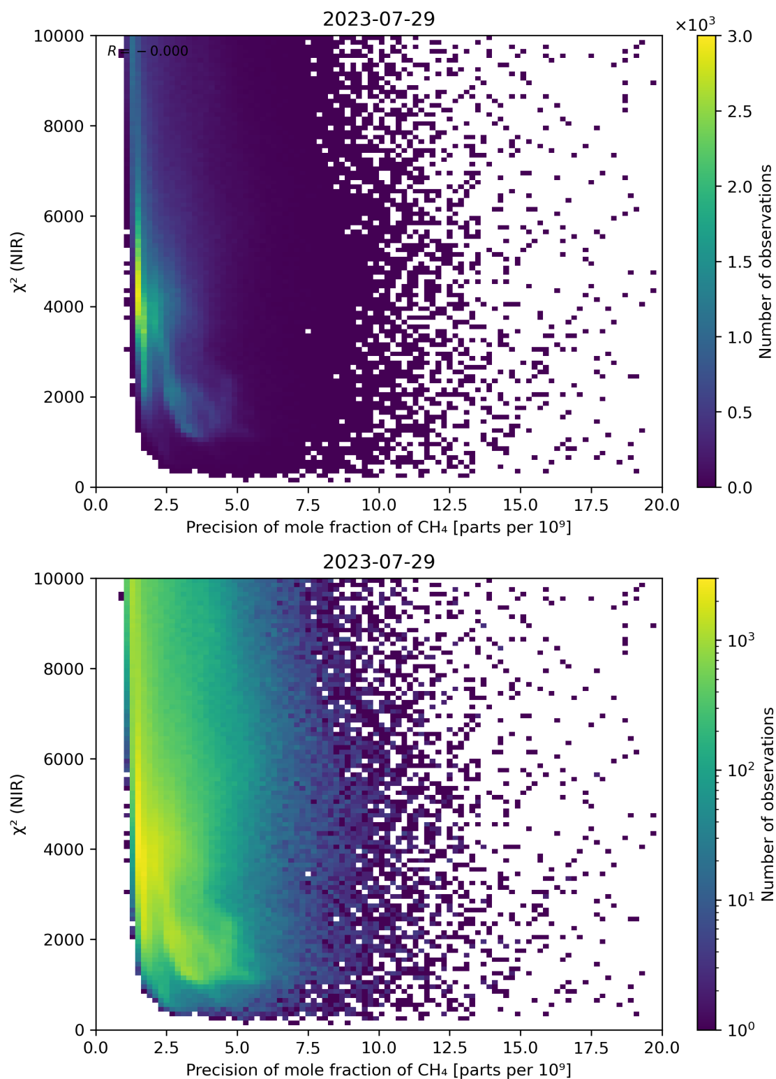
Figure 78: Scatter density plot of “Precision of mole fraction of \text{CH}_4 ” against “ \chi^2 (NIR)” for 2023-07-29 to 2023-07-30.
