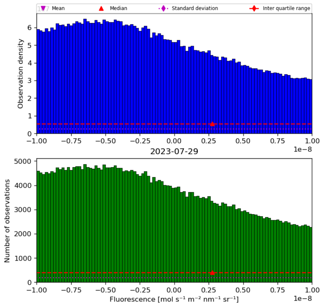
Figure 32: Histogram of “Fluorescence” for 2023-07-29 to 2023-07-30
