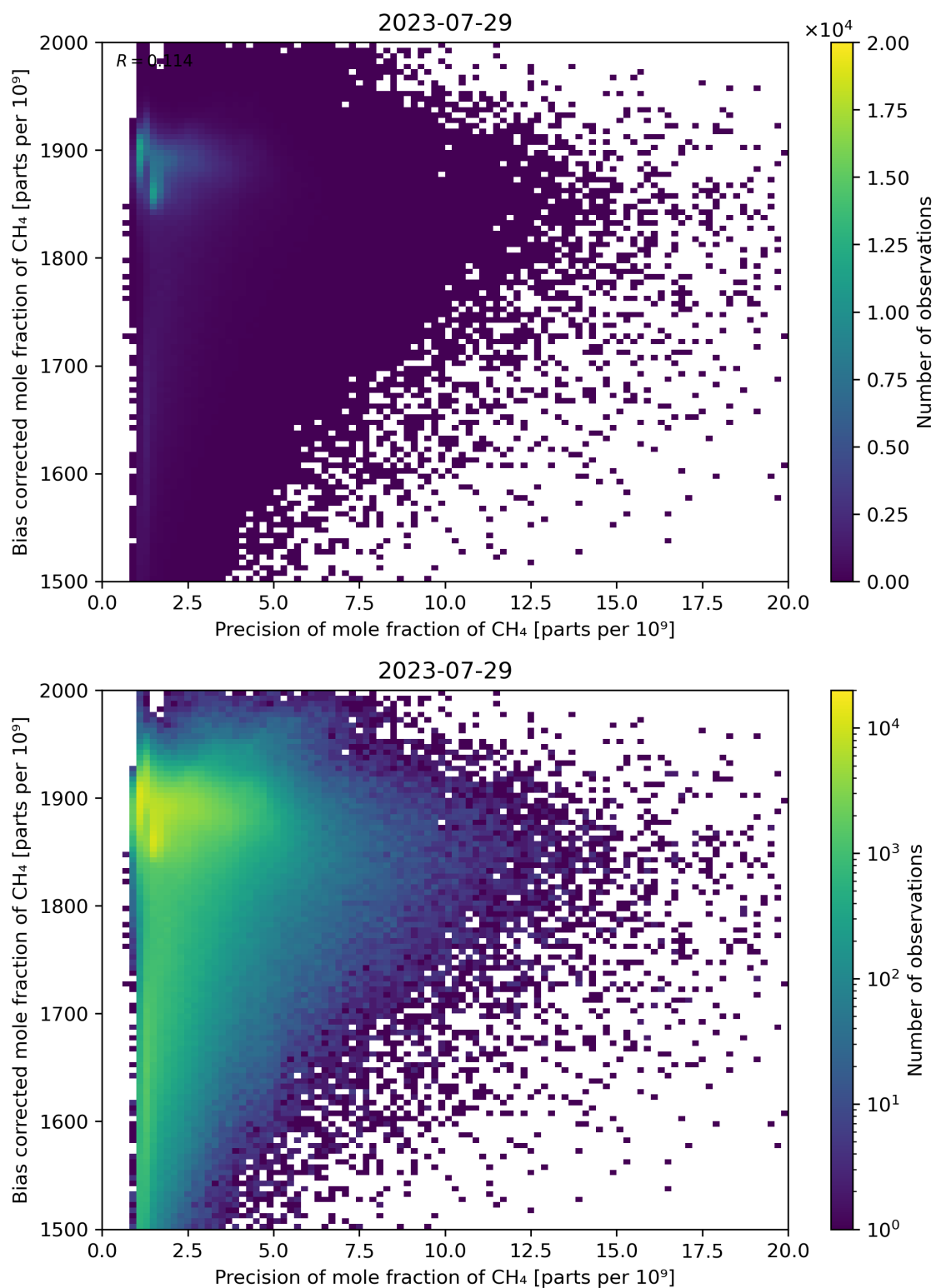
Figure 82: Scatter density plot of “Precision of mole fraction of CH 4 ” against “Bias corrected mole fraction of CH 4 ” for 2023-07-29 to 2023-07-30.
