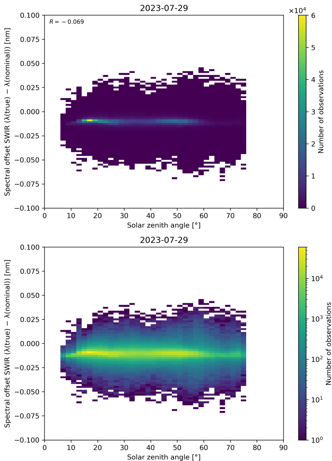
Figure 104: Scatter density plot of “Solar zenith angle” against “Spectral offset SWIR ( \lambda(\text{true}) - \lambda(\text{nominal}) )” for 2023-07-29 to 2023-07-30.
