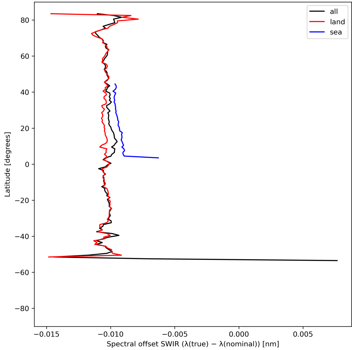
Figure 16: Zonal average of “Spectral offset SWIR ( \lambda(\text{true}) - \lambda(\text{nominal}) )” for 2023-07-29 to 2023-07-30.
