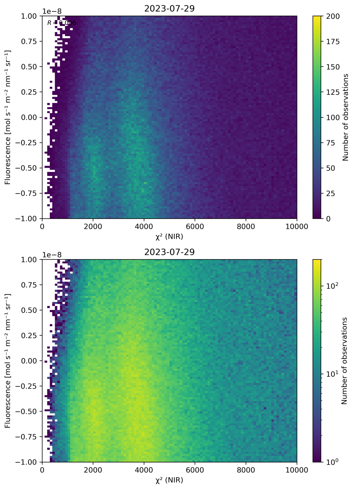
Figure 45: Scatter density plot of “ \chi^2 (NIR)” against “Fluorescence” for 2023-07-29 to 2023-07-30.
