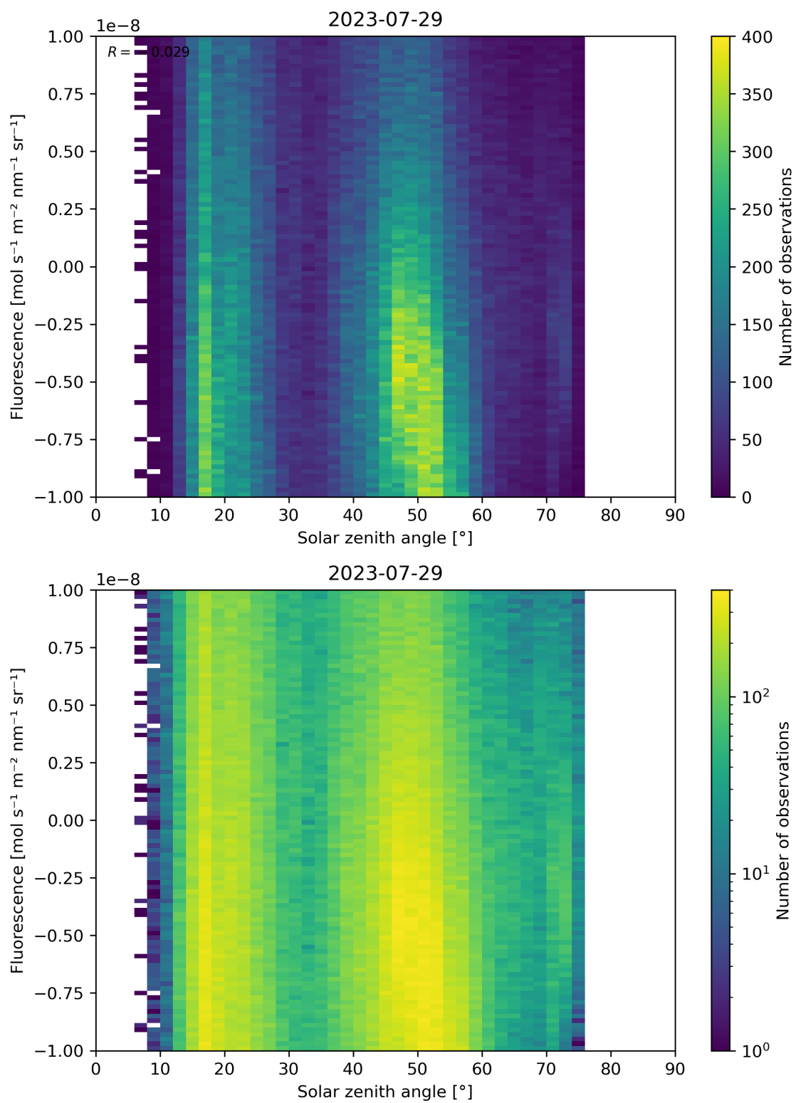
Figure 97: Scatter density plot of “Solar zenith angle” against “Fluorescence” for 2023-07-29 to 2023-07-30.
