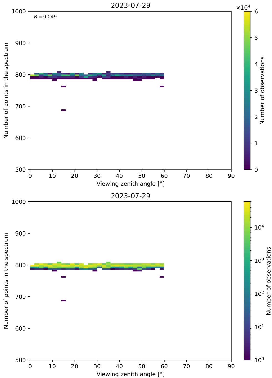
Figure 114: Scatter density plot of “Viewing zenith angle” against “Number of points in the spectrum” for 2023-07-29 to 2023-07-30.
