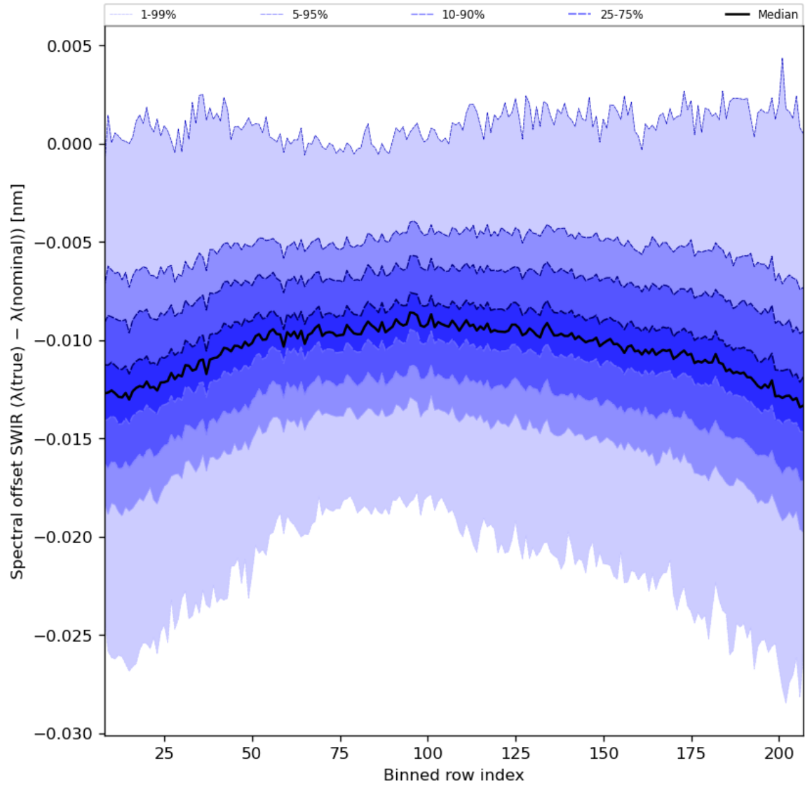
Figure 38: Along track statistics of “Spectral offset SWIR ( \lambda(\text{true}) - \lambda(\text{nominal}) )” for 2023-07-29 to 2023-07-30
