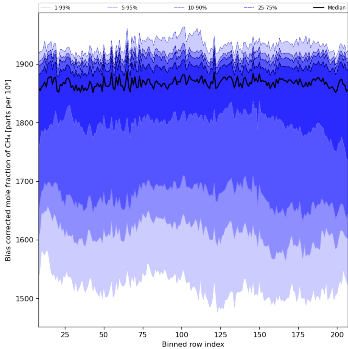
Figure 36: Along track statistics of “Bias corrected mole fraction of CH 4 ” for 2023-07-29 to 2023-07-30
