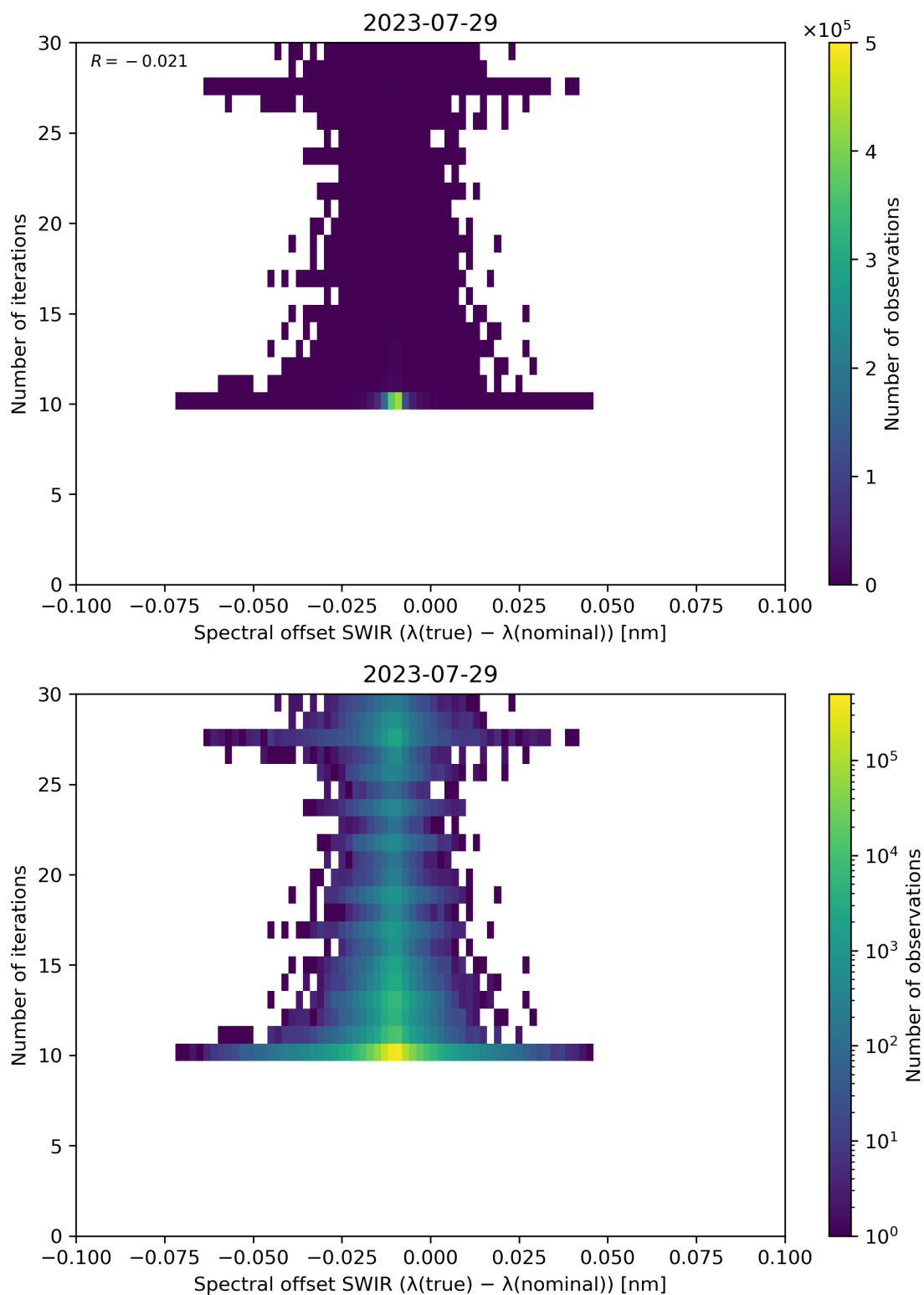
Figure 121: Scatter density plot of “Spectral offset SWIR ( \lambda(\text{true}) - \lambda(\text{nominal}) )” against “Number of iterations” for 2023-07-29 to 2023-07-30.
