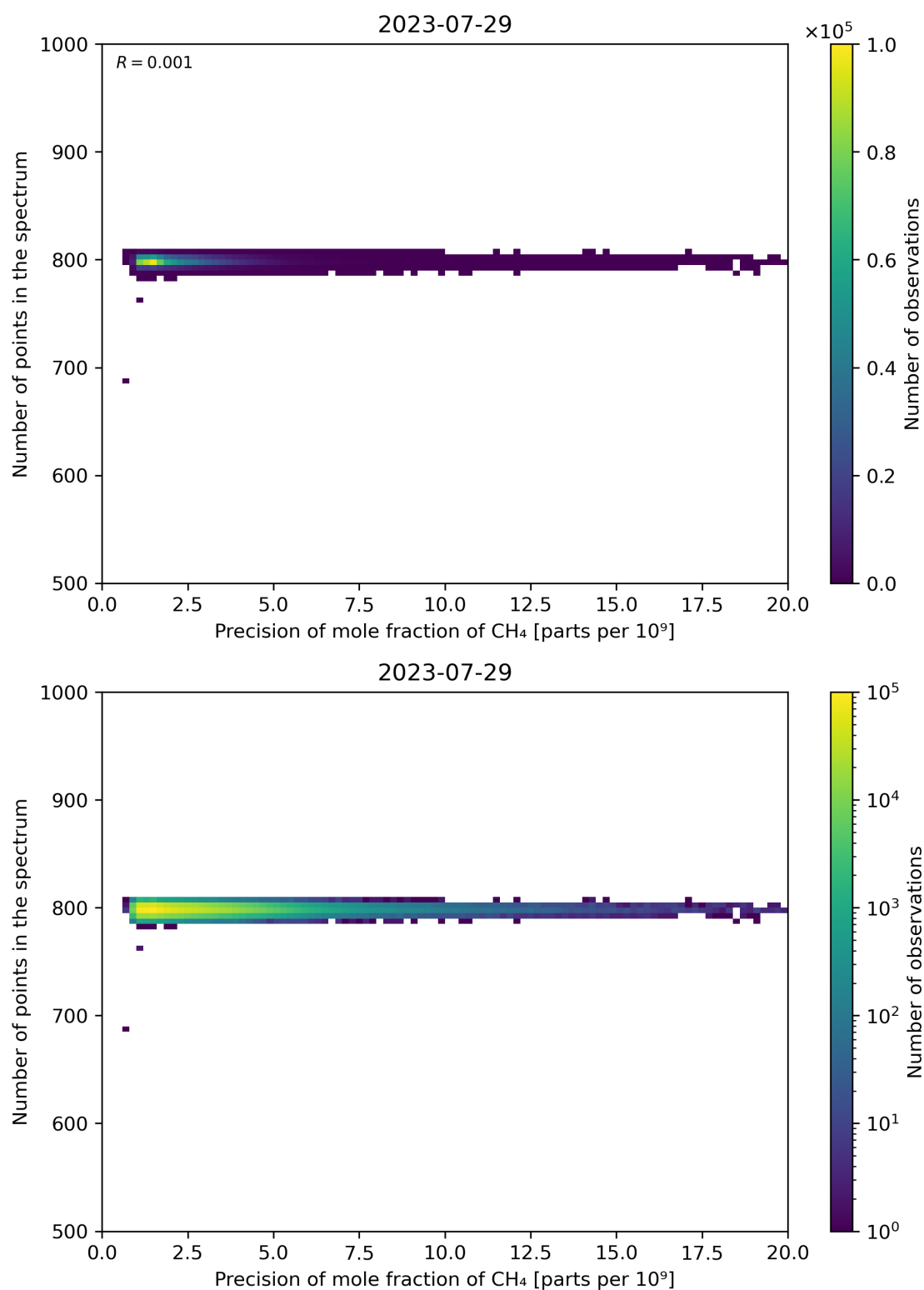
Figure 84: Scatter density plot of “Precision of mole fraction of CH 4 ” against “Number of points in the spectrum” for 2023-07-29 to 2023-07-30.
