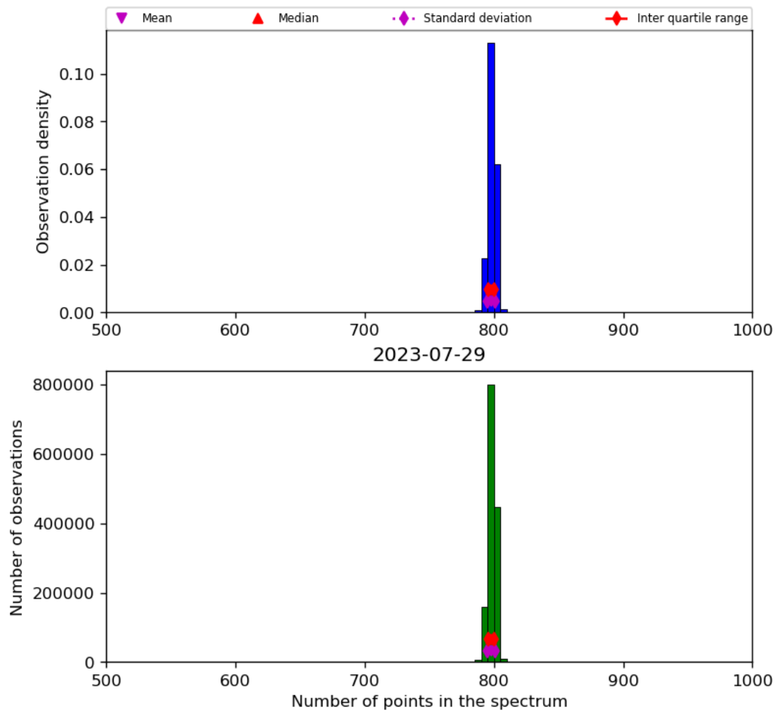
Figure 26: Histogram of “Number of points in the spectrum” for 2023-07-29 to 2023-07-30
