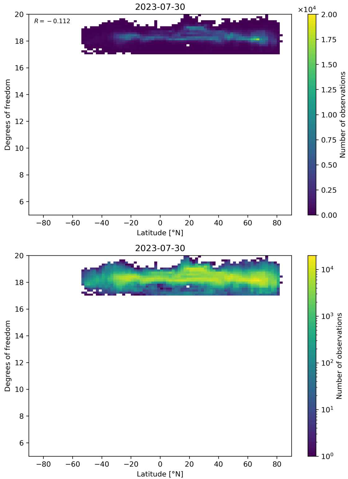
Figure 55: Scatter density plot of “Latitude” against “Degrees of freedom” for 2023-07-29 to 2023-07-31.
