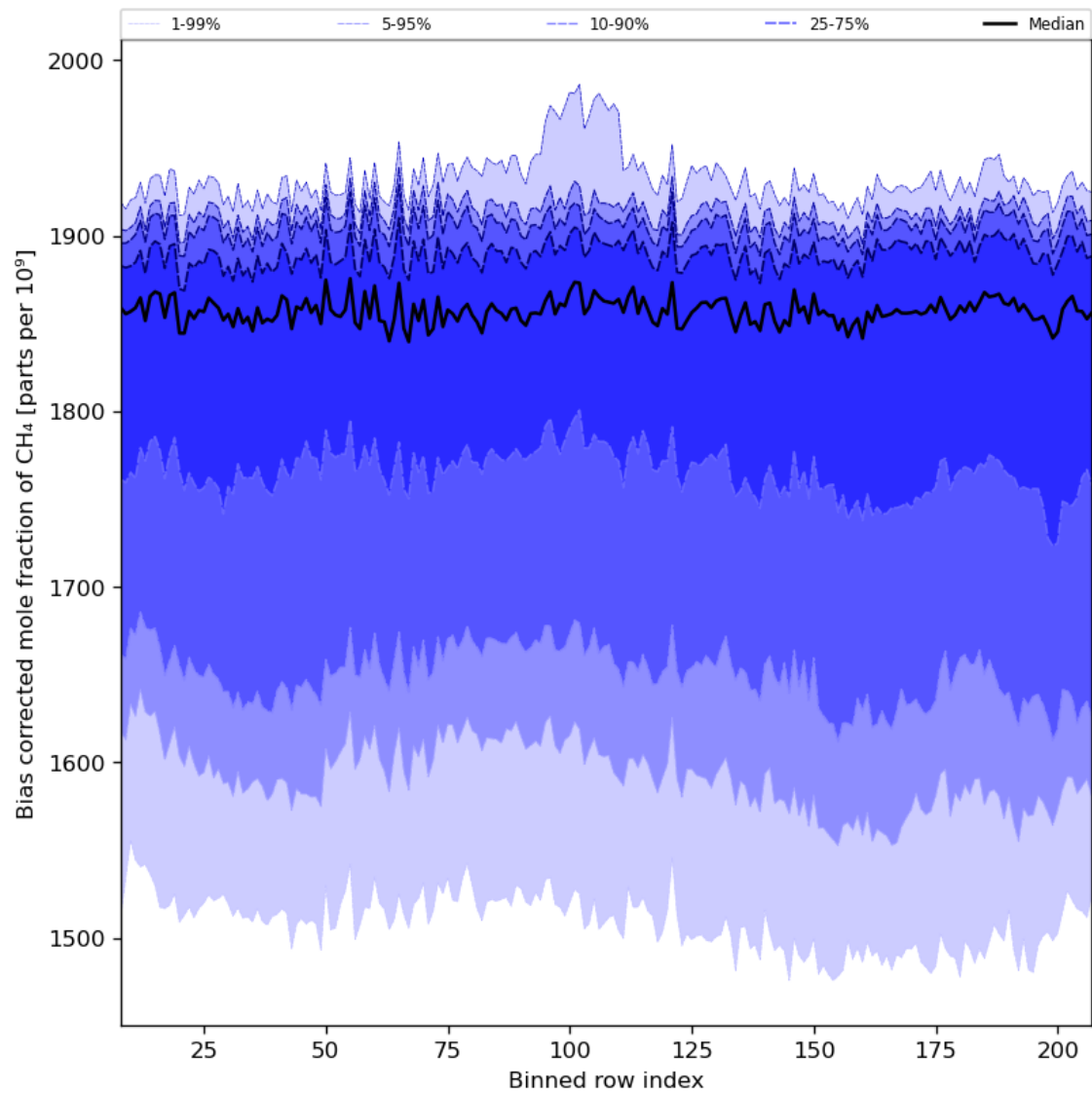
Figure 36: Along track statistics of “Bias corrected mole fraction of CH 4 ” for 2023-07-29 to 2023-07-31
