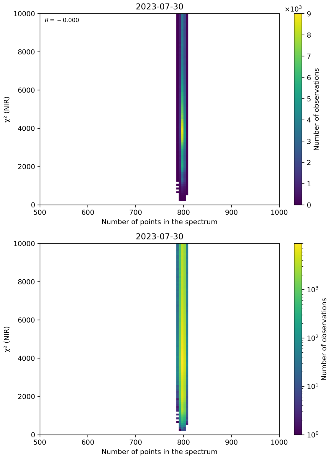
Figure 88: Scatter density plot of “Number of points in the spectrum” against “ \chi^2 (NIR)” for 2023-07-29 to 2023-07-31.
