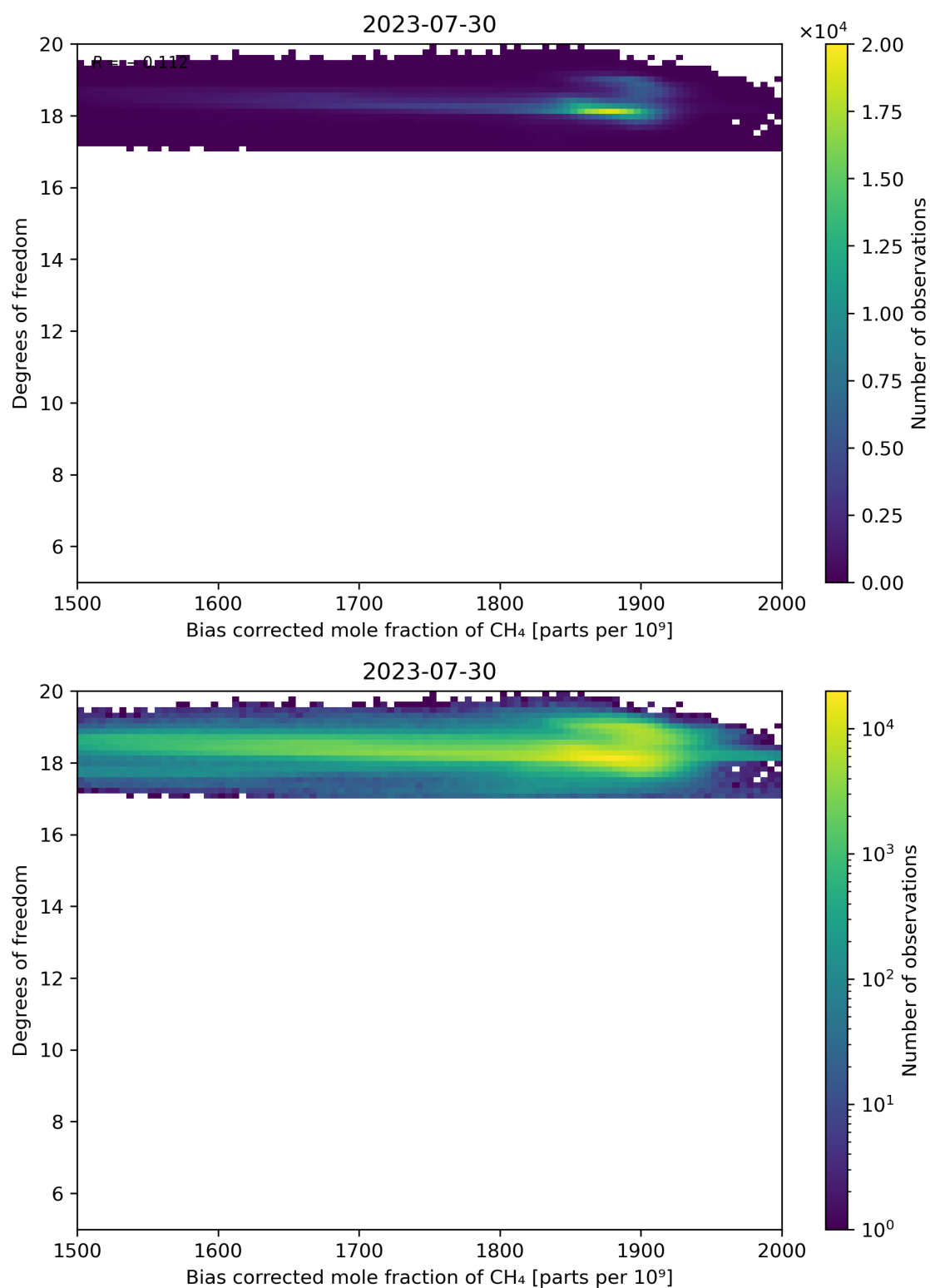
Figure 65: Scatter density plot of “Bias corrected mole fraction of CH 4 ” against “Degrees of freedom” for 2023-07-29 to 2023-07-31.
