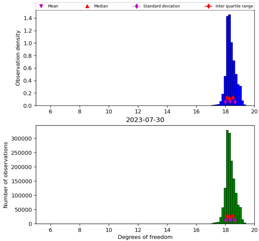
Figure 30: Histogram of “Degrees of freedom” for 2023-07-29 to 2023-07-31
