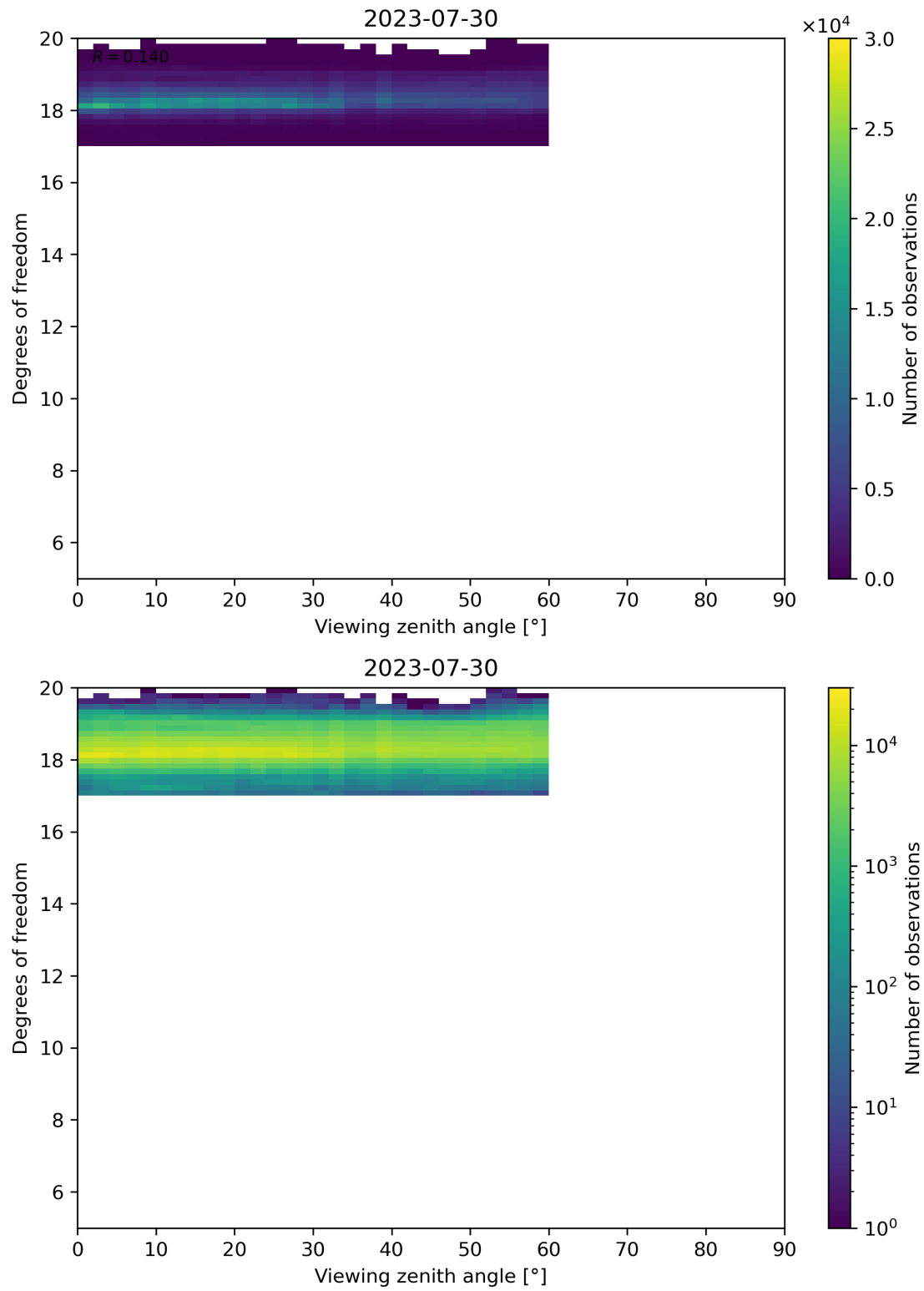
Figure 107: Scatter density plot of “Viewing zenith angle” against “Degrees of freedom” for 2023-07-29 to 2023-07-31.
