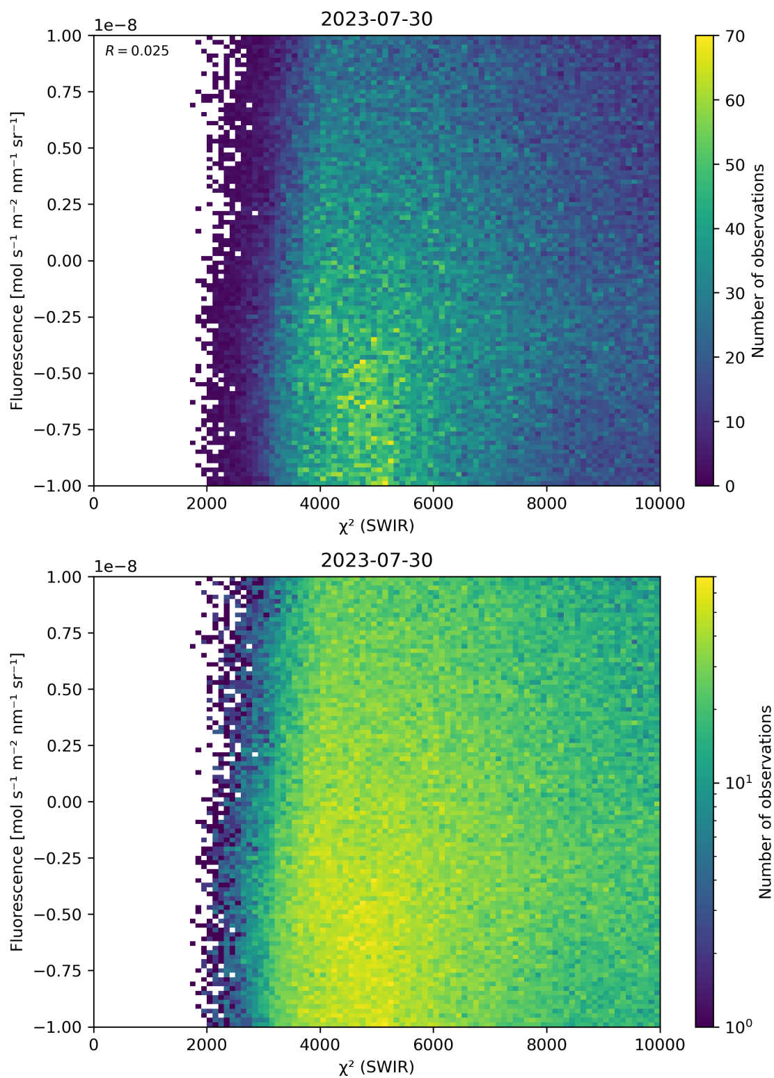
Figure 49: Scatter density plot of “ \chi^2 (SWIR)” against “Fluorescence” for 2023-07-29 to 2023-07-31.
