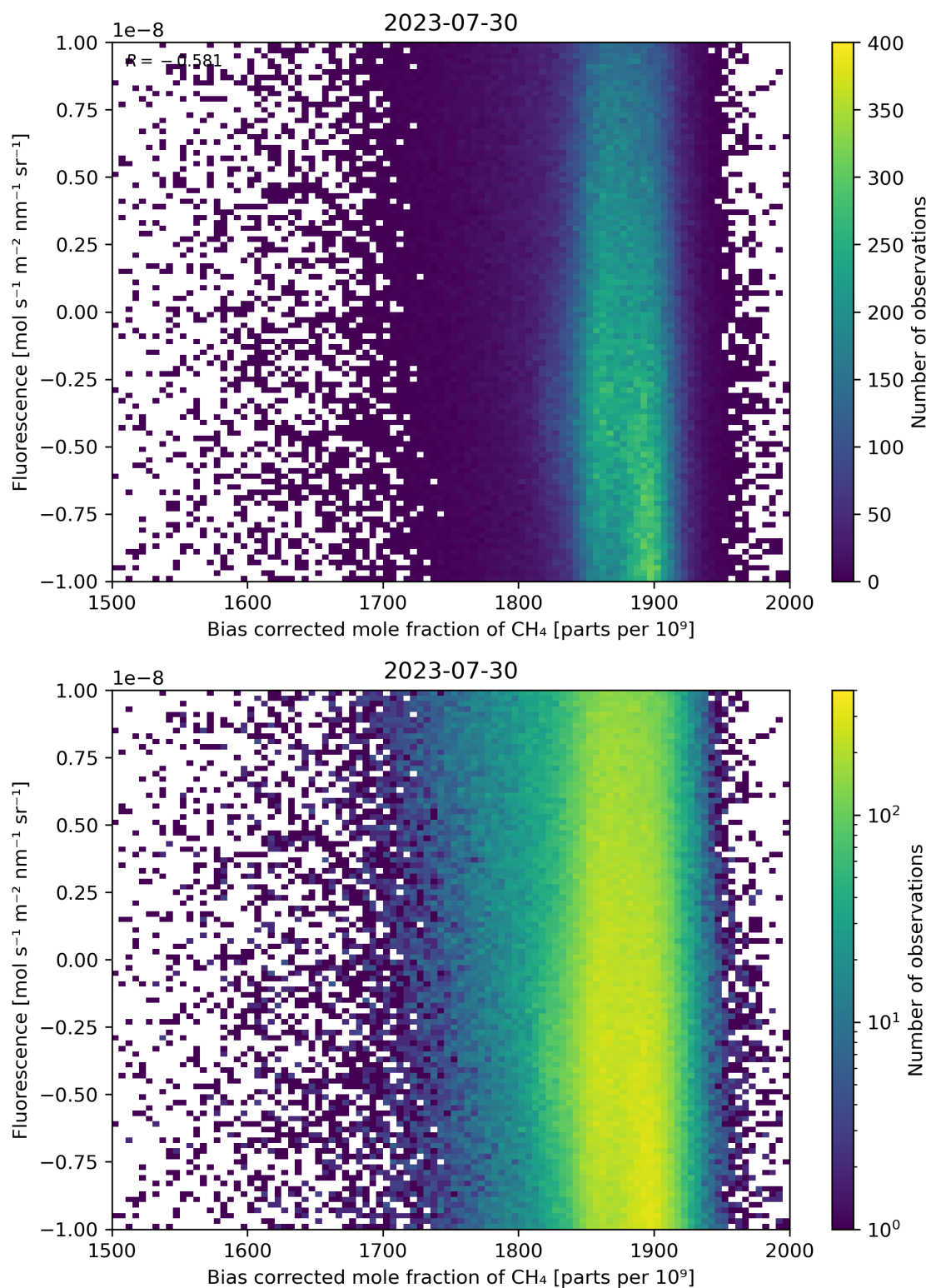
Figure 66: Scatter density plot of “Bias corrected mole fraction of CH 4 ” against “Fluorescence” for 2023-07-29 to 2023-07-31.
