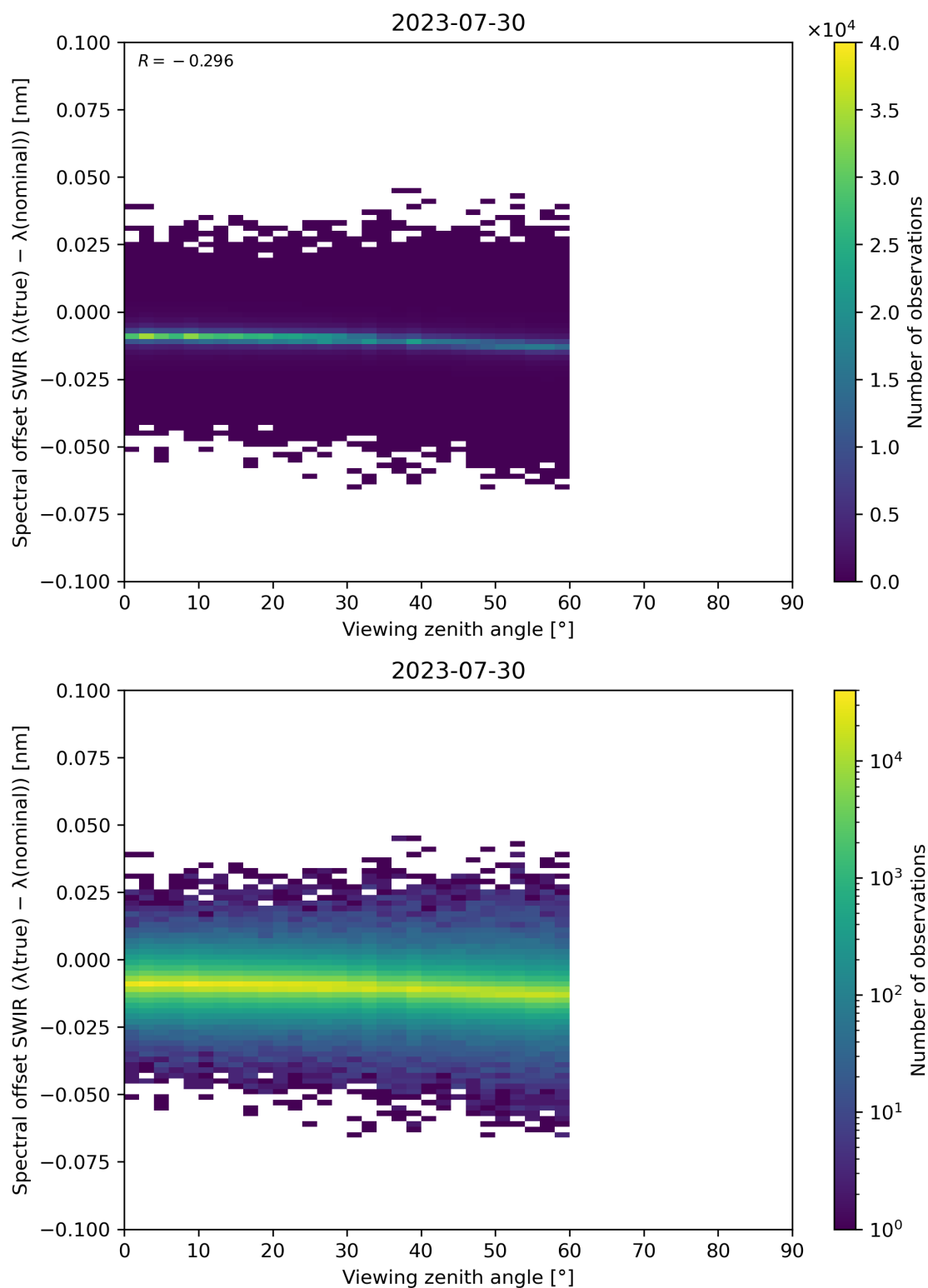
Figure 116: Scatter density plot of “Viewing zenith angle” against “Spectral offset SWIR ( \lambda(\text{true}) - \lambda(\text{nominal}) )” for 2023-07-29 to 2023-07-31.
