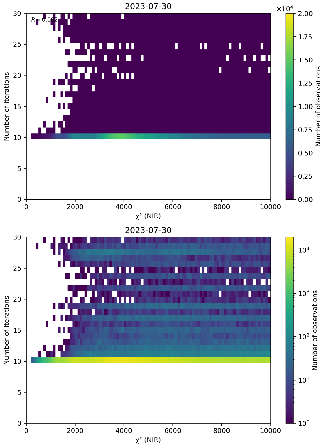
Figure 46: Scatter density plot of “ \chi^2 (NIR)” against “Number of iterations” for 2023-07-29 to 2023-07-31.
