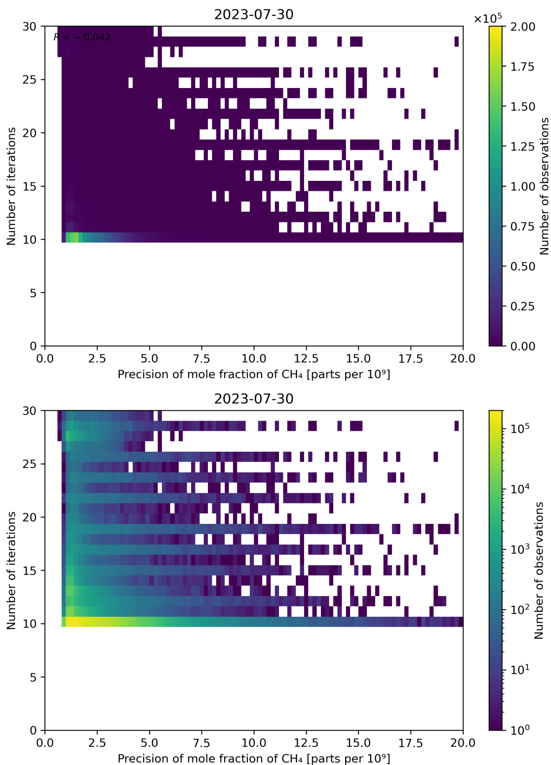
Figure 83: Scatter density plot of “Precision of mole fraction of CH 4 ” against “Number of iterations” for 2023-07-29 to 2023-07-31.
