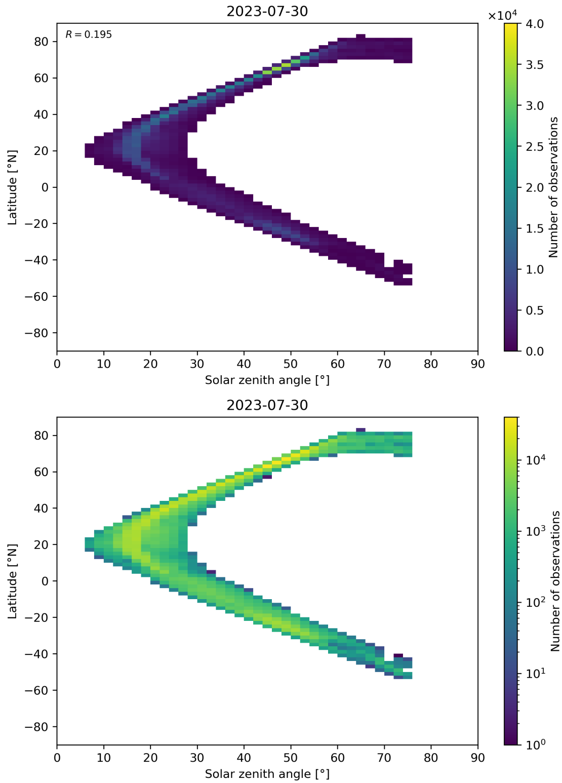
Figure 98: Scatter density plot of “Solar zenith angle” against “Latitude” for 2023-07-29 to 2023-07-31.
