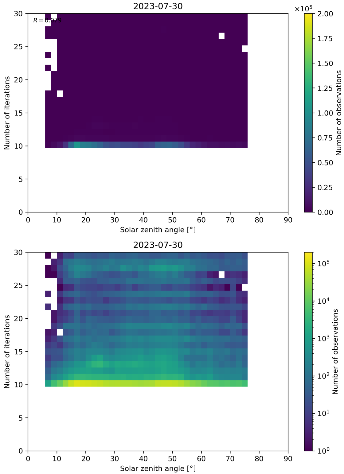
Figure 102: Scatter density plot of “Solar zenith angle” against “Number of iterations” for 2023-07-29 to 2023-07-31.
