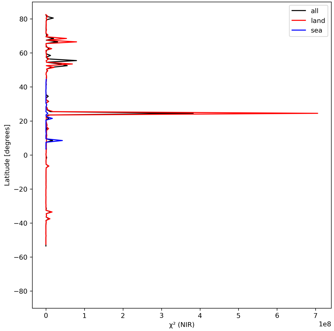
Figure 18: Zonal average of “ \chi^2 (NIR)” for 2023-07-29 to 2023-07-31.
