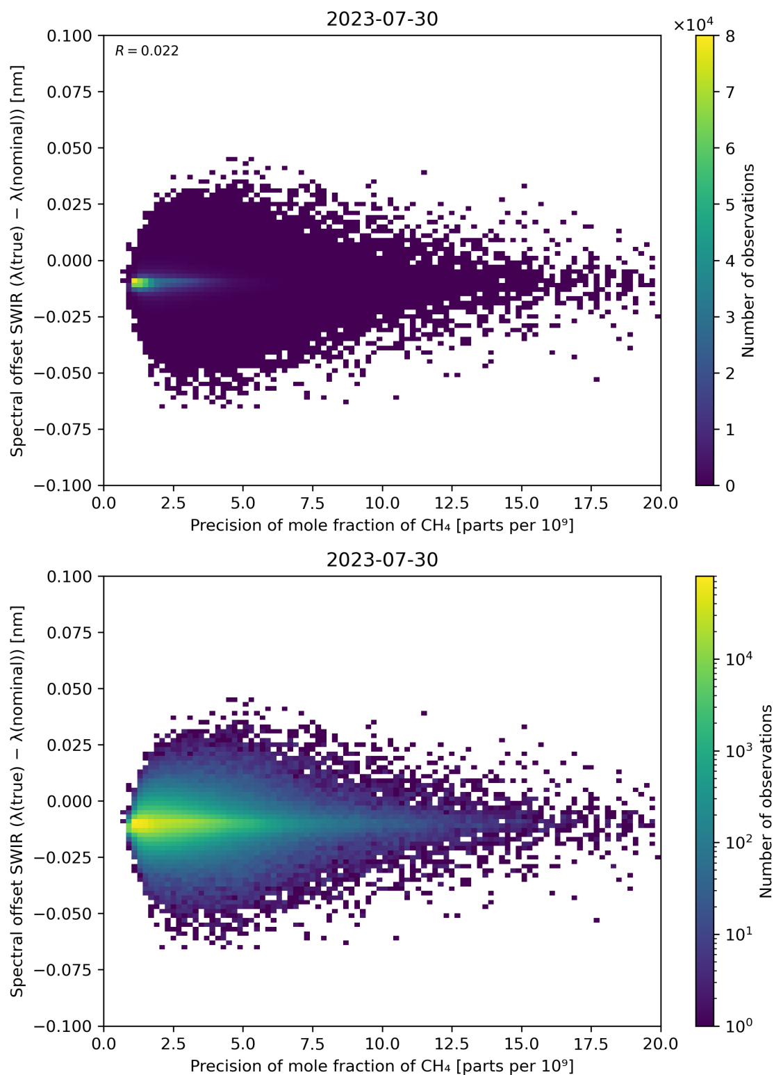
Figure 85: Scatter density plot of “Precision of mole fraction of \text{CH}_4 ” against “Spectral offset SWIR ( \lambda(\text{true}) - \lambda(\text{nominal}) )” for 2023-07-29 to 2023-07-31.
