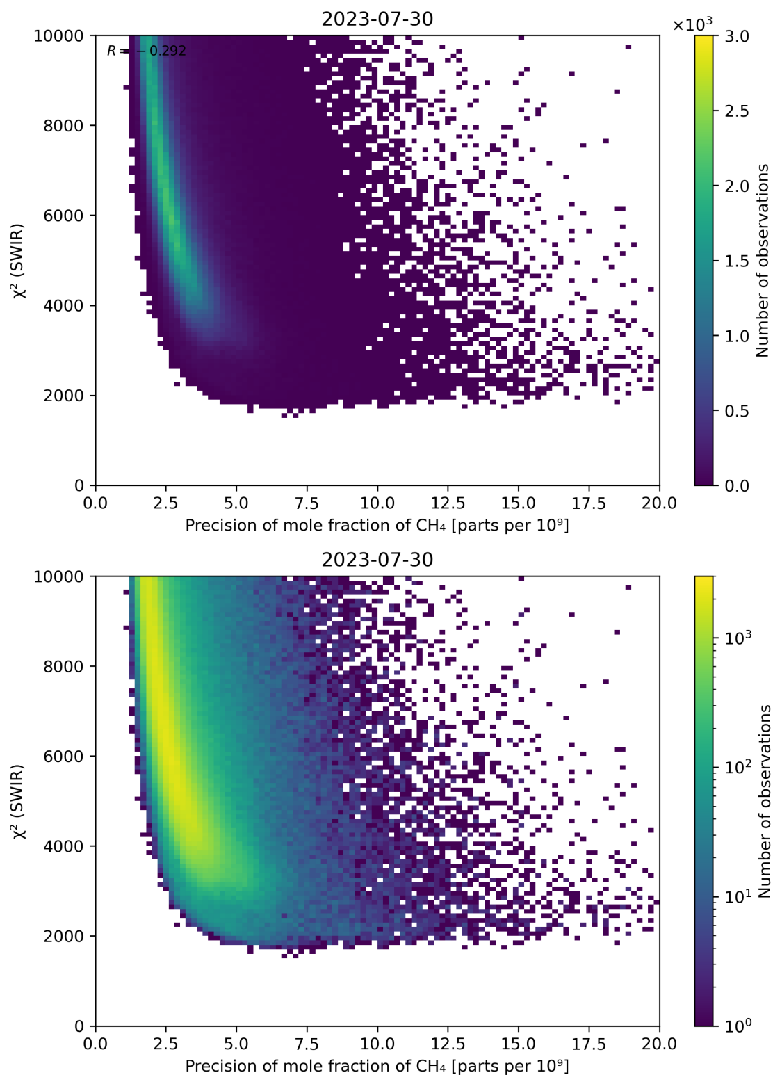
Figure 79: Scatter density plot of “Precision of mole fraction of CH 4 ” against “ \chi^2 (SWIR)” for 2023-07-29 to 2023-07-31.
