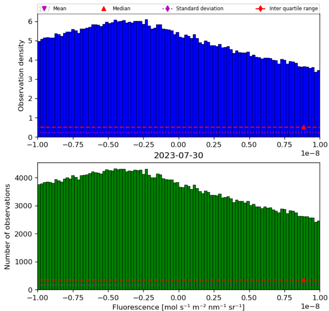
Figure 32: Histogram of “Fluorescence” for 2023-07-29 to 2023-07-31
