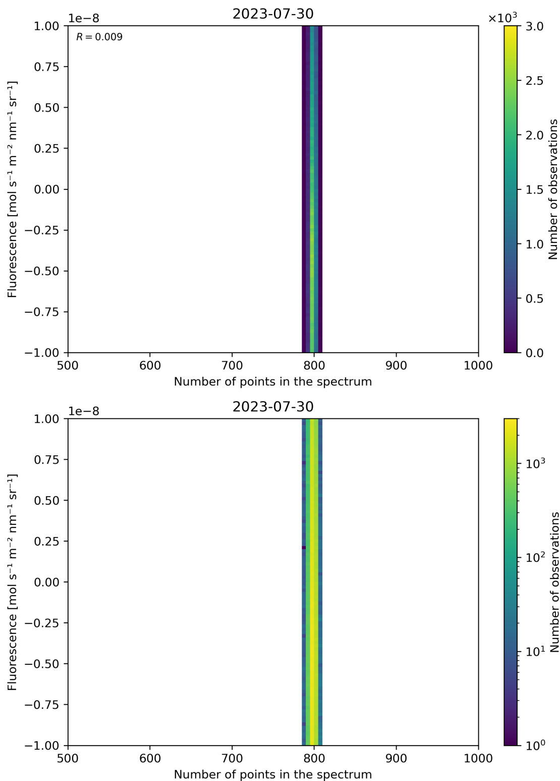
Figure 91: Scatter density plot of “Number of points in the spectrum” against “Fluorescence” for 2023-07-29 to 2023-07-31.
