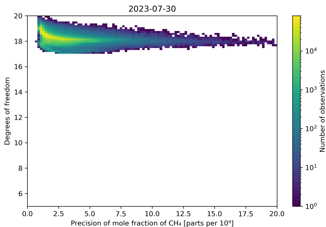
Figure 80: Scatter density plot of “Precision of mole fraction of CH 4 ” against “Degrees of freedom” for 2023-07-29 to 2023-07-31.
