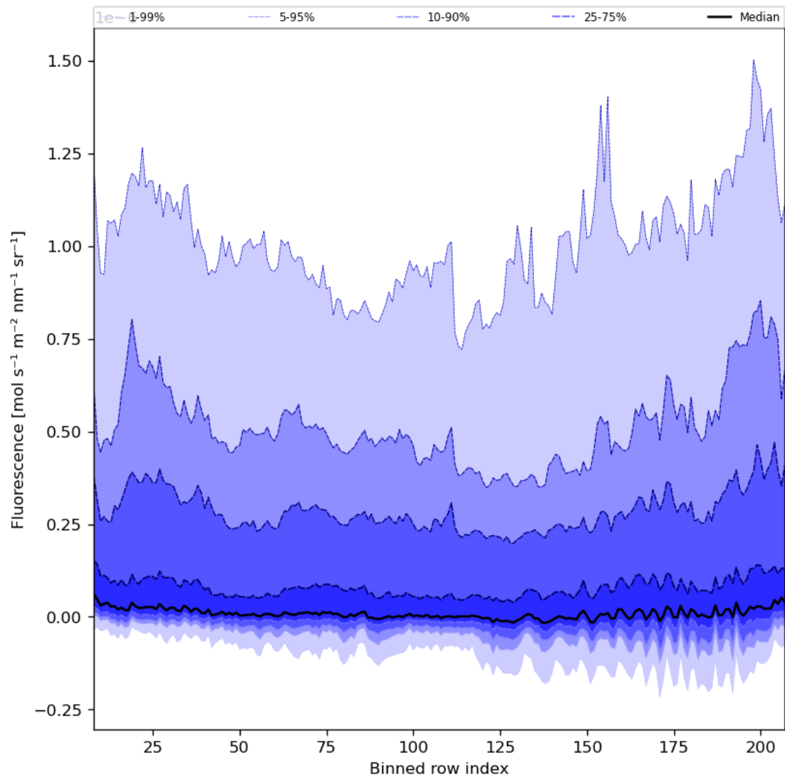
Figure 43: Along track statistics of “Fluorescence” for 2023-07-29 to 2023-07-31
