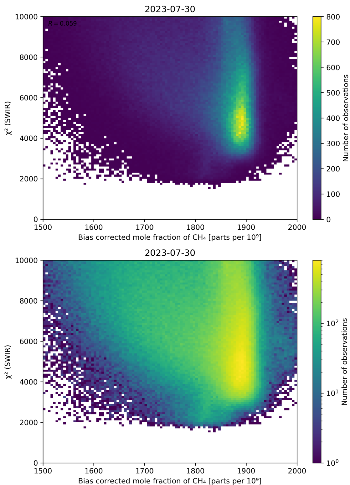
Figure 64: Scatter density plot of “Bias corrected mole fraction of CH 4 ” against “ \chi^2 (SWIR)” for 2023-07-29 to 2023-07-31.
