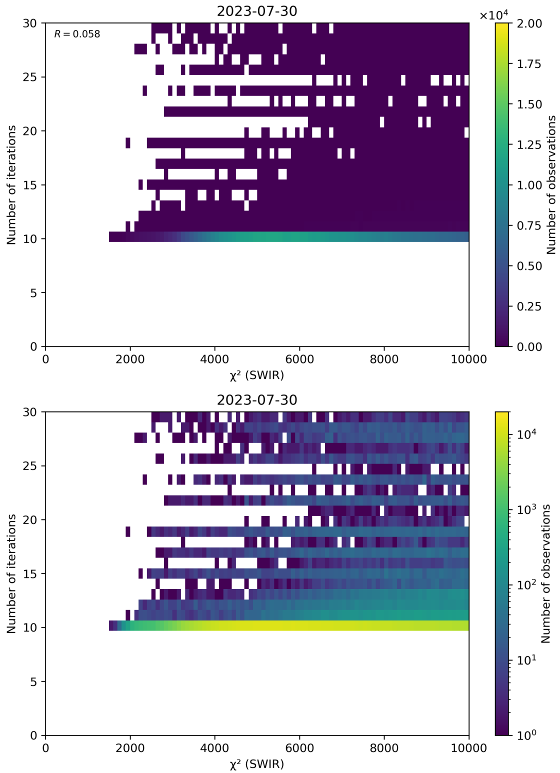
Figure 50: Scatter density plot of “ \chi^2 (SWIR)” against “Number of iterations” for 2023-07-29 to 2023-07-31.
