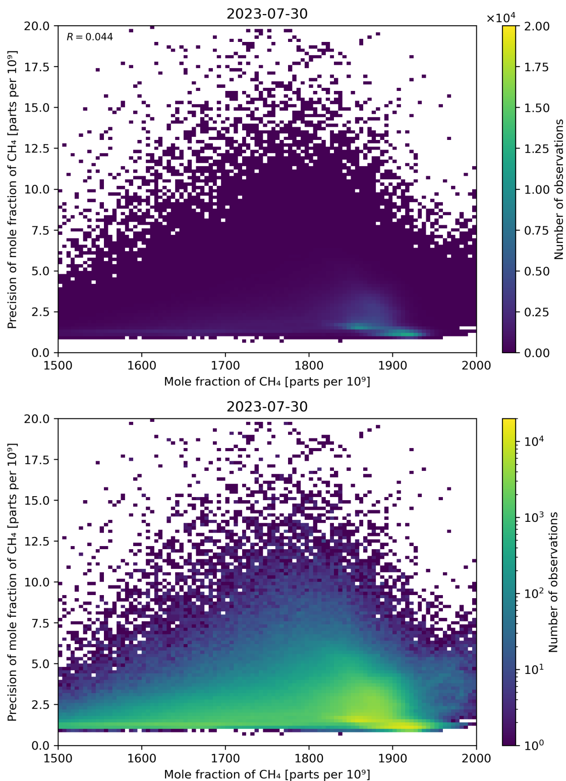
Figure 75: Scatter density plot of “Mole fraction of CH 4 ” against “Precision of mole fraction of CH 4 ” for 2023-07-29 to 2023-07-31.
