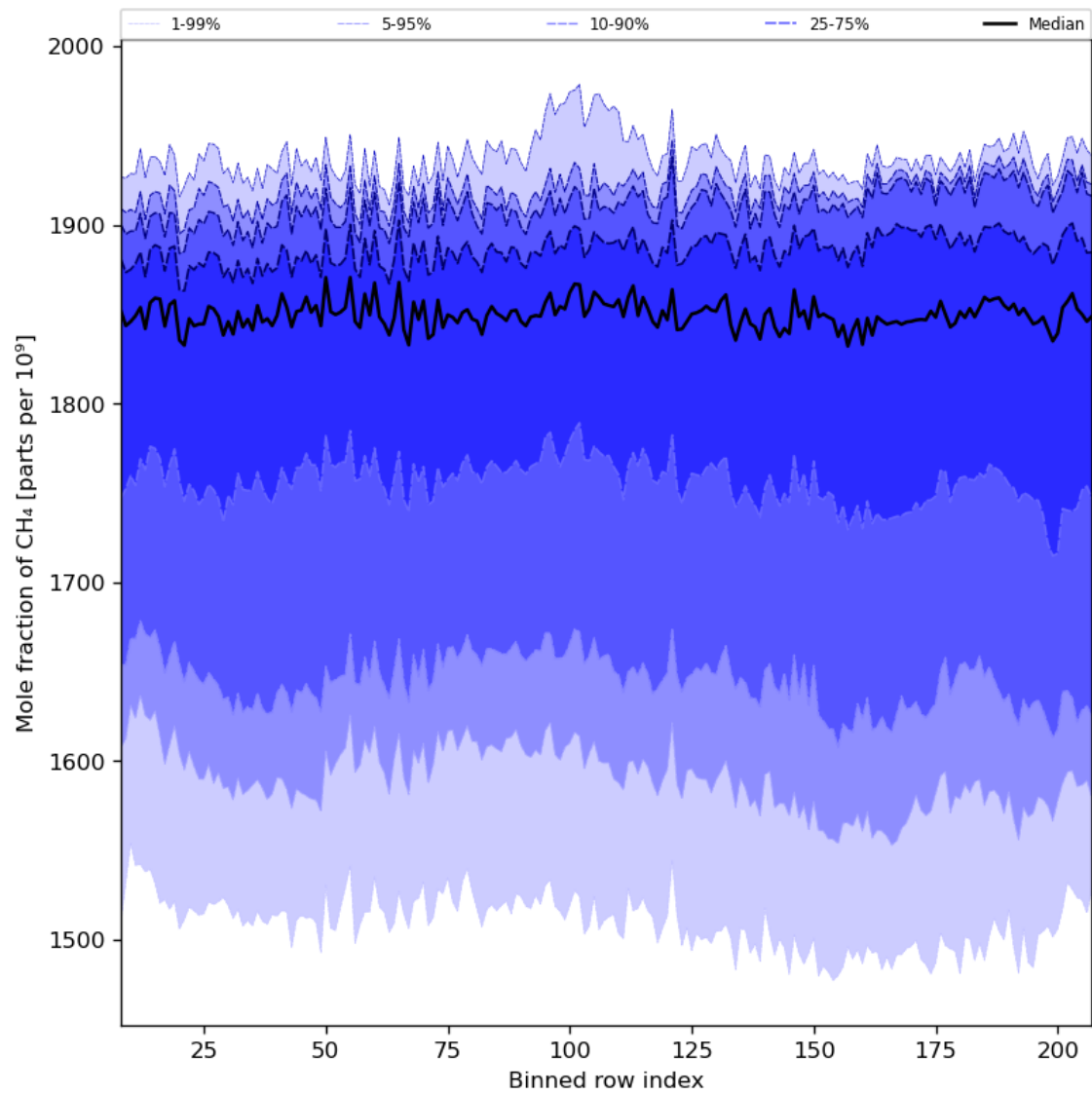
Figure 34: Along track statistics of “Mole fraction of CH 4 ” for 2023-07-29 to 2023-07-31
