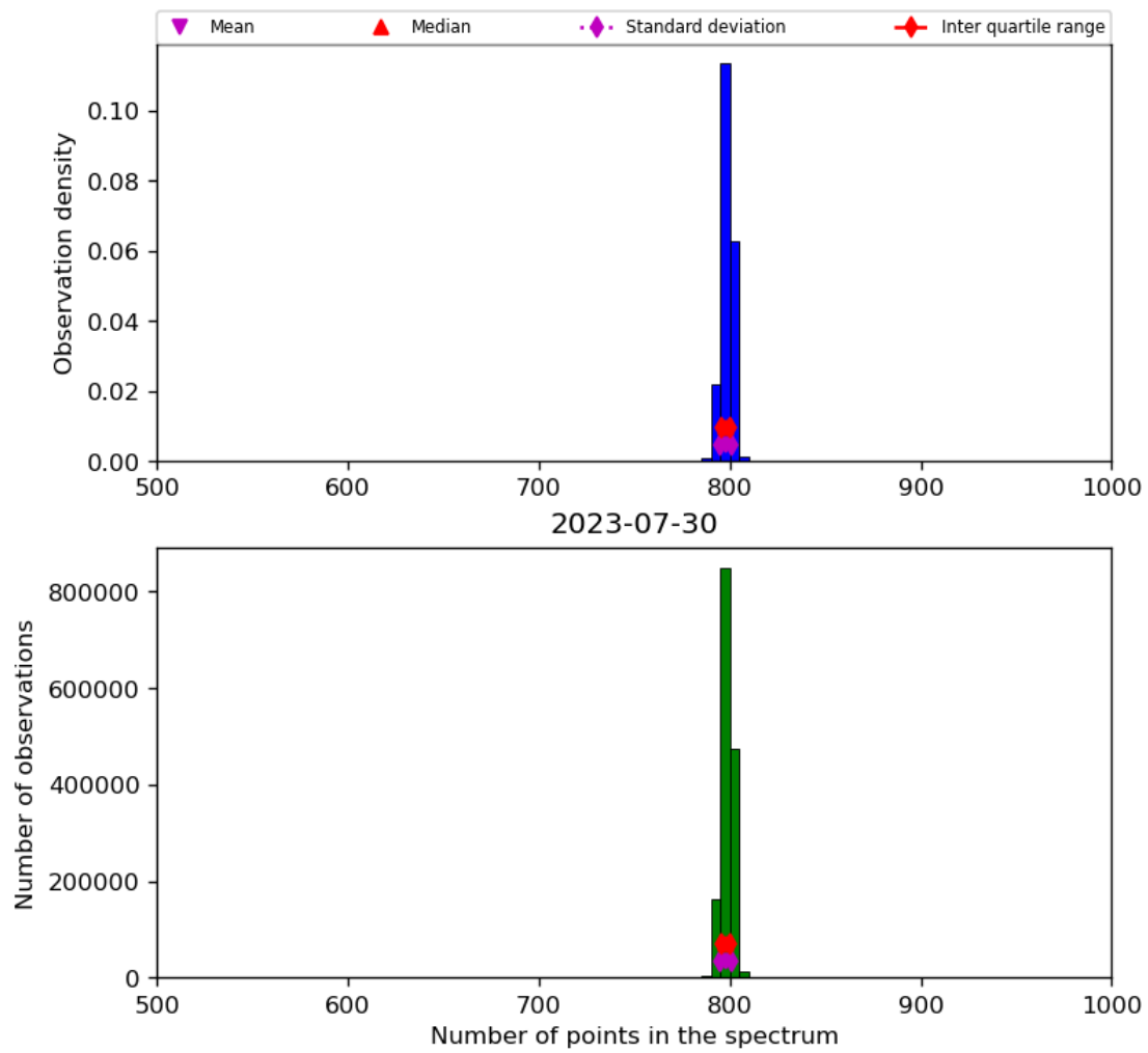
Figure 26: Histogram of “Number of points in the spectrum” for 2023-07-29 to 2023-07-31
