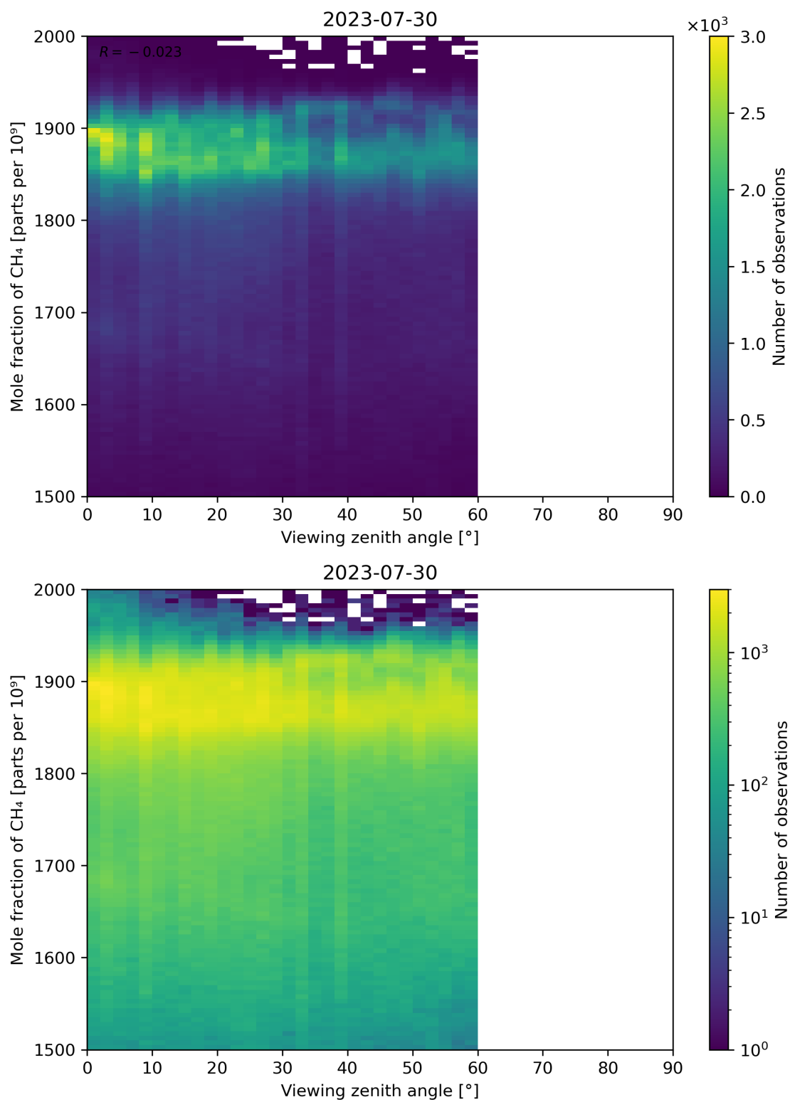
Figure 110: Scatter density plot of “Viewing zenith angle” against “Mole fraction of CH 4 ” for 2023-07-29 to 2023-07-31.
