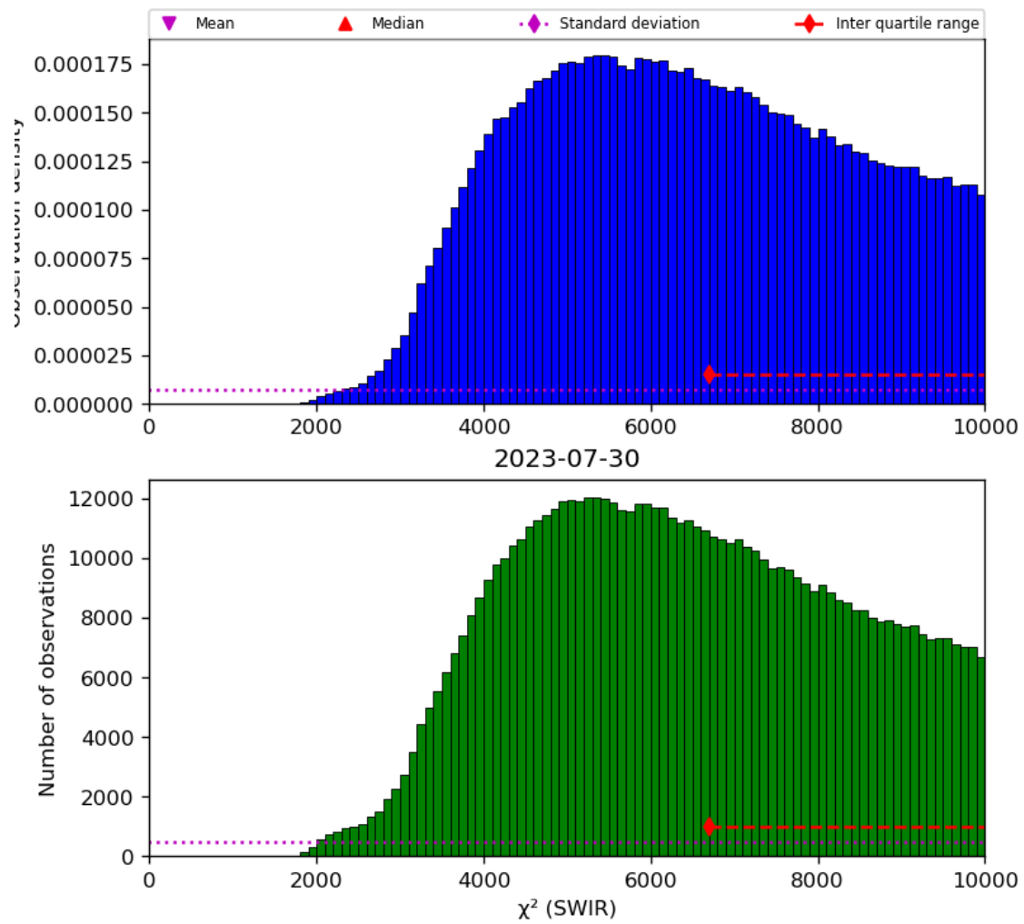
Figure 28: Histogram of “ \chi^2 (SWIR)” for 2023-07-29 to 2023-07-31
