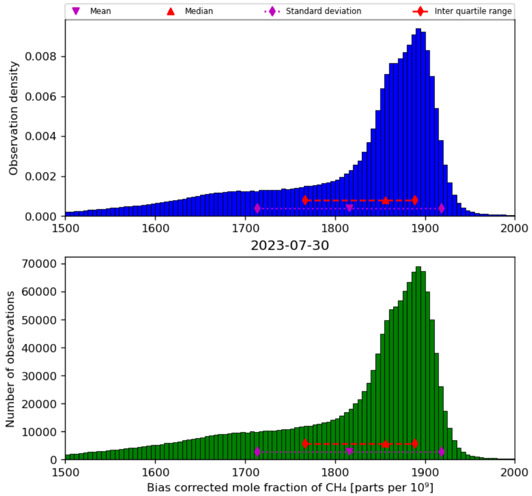
Figure 25: Histogram of “Bias corrected mole fraction of CH 4 ” for 2023-07-29 to 2023-07-31
