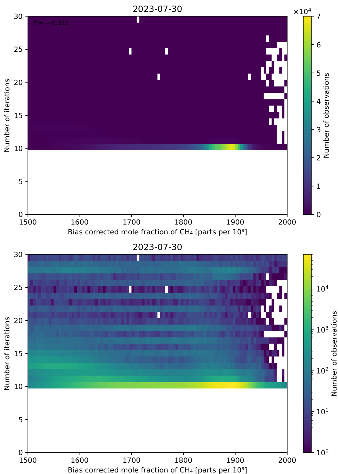
Figure 67: Scatter density plot of “Bias corrected mole fraction of CH 4 ” against “Number of iterations” for 2023-07-29 to 2023-07-31.
