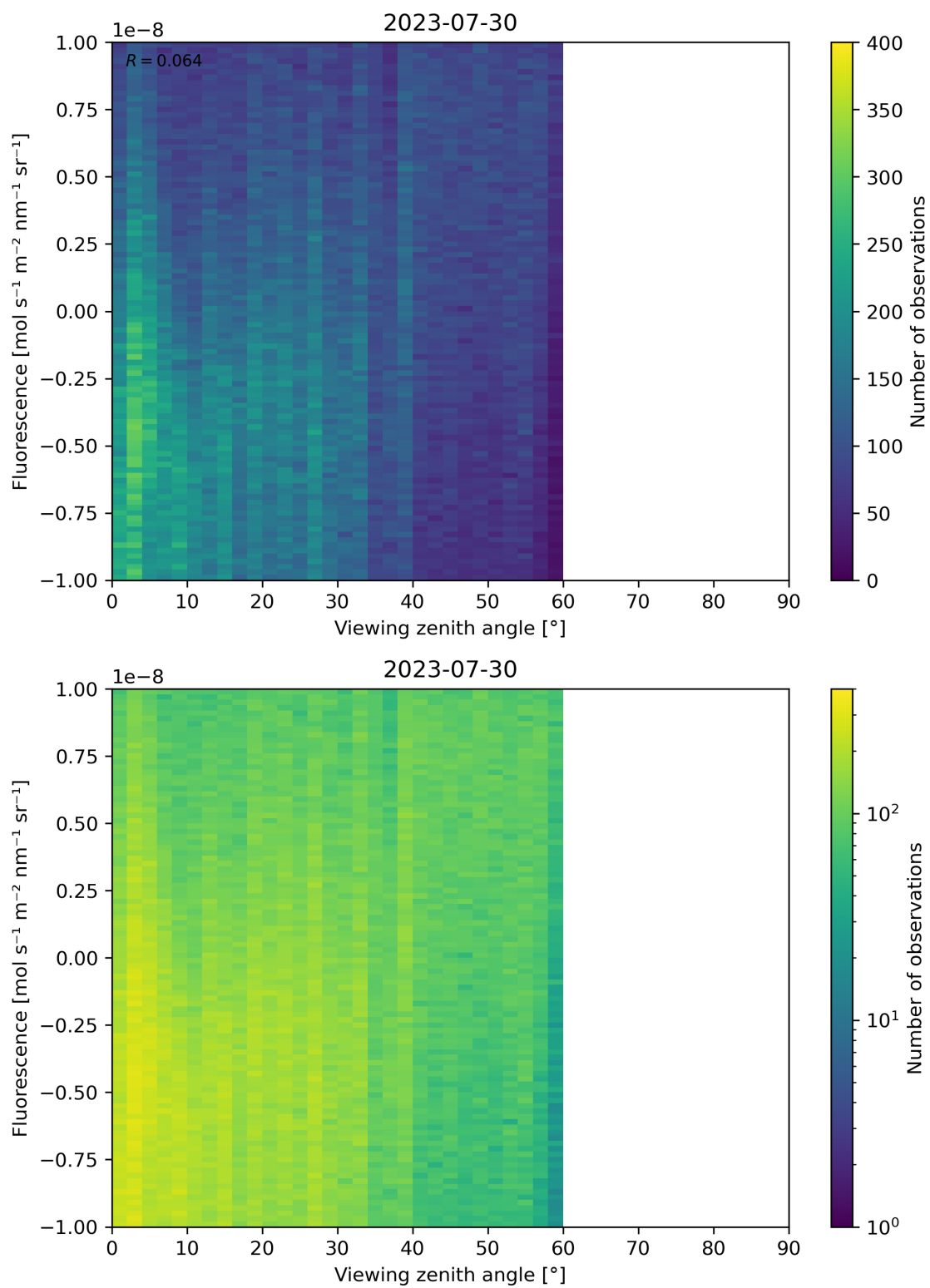
Figure 108: Scatter density plot of “Viewing zenith angle” against “Fluorescence” for 2023-07-29 to 2023-07-31.
