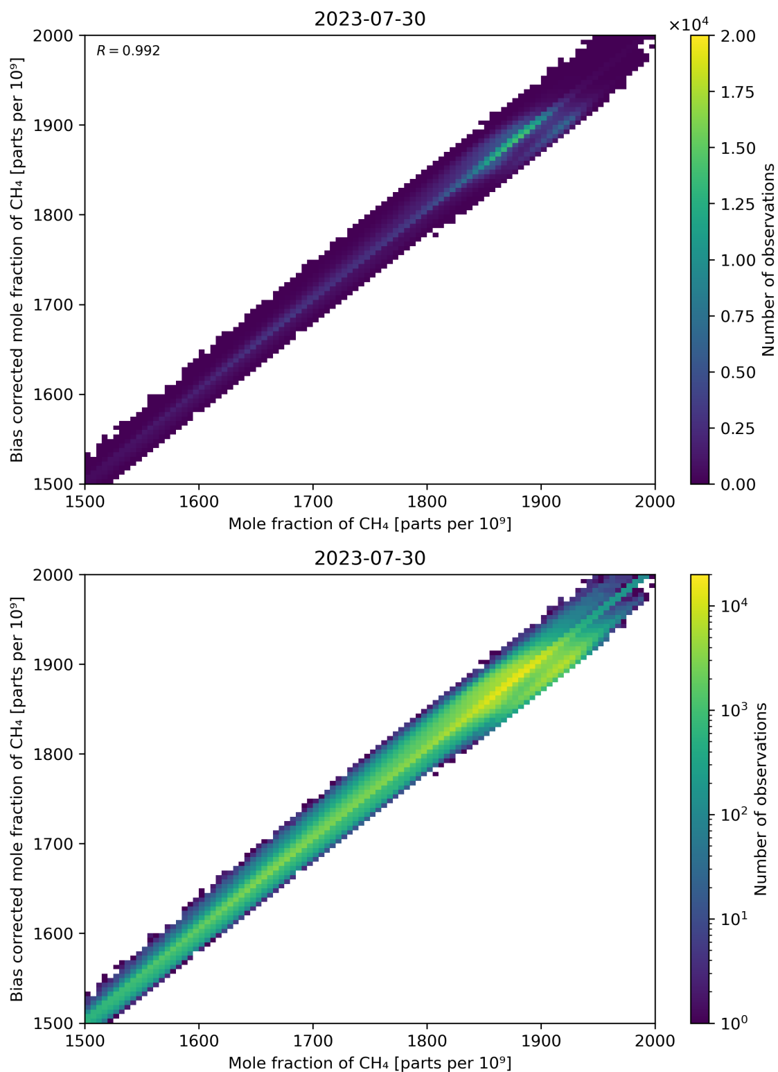
Figure 74: Scatter density plot of “Mole fraction of CH 4 ” against “Bias corrected mole fraction of CH 4 ” for 2023-07-29 to 2023-07-31.
