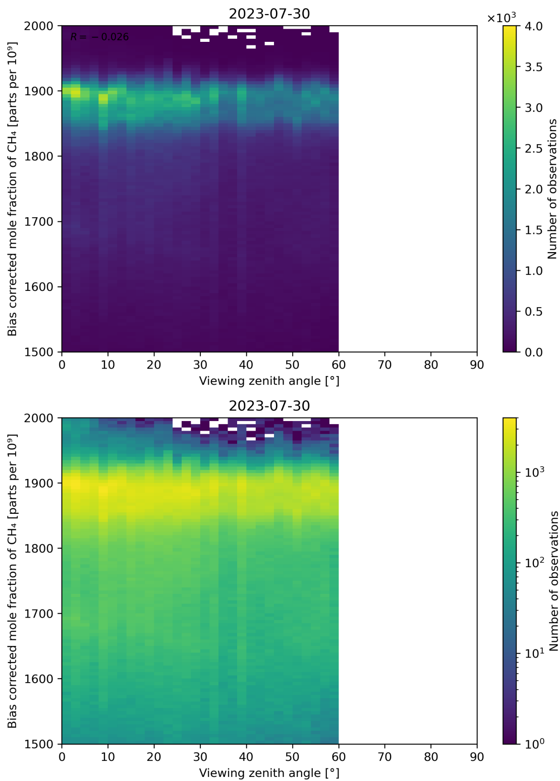
Figure 111: Scatter density plot of “Viewing zenith angle” against “Bias corrected mole fraction of CH 4 ” for 2023-07-29 to 2023-07-31.
