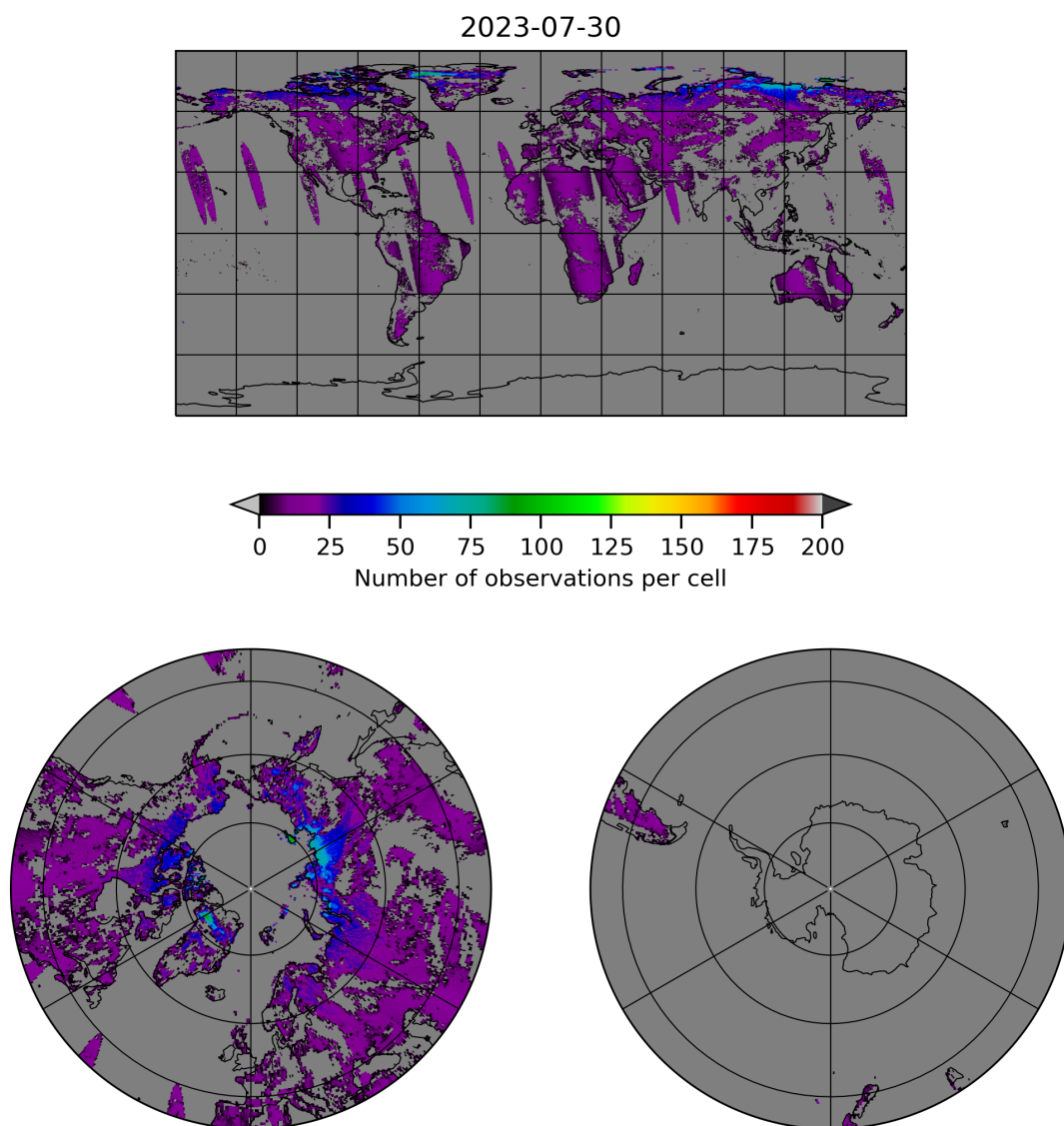
Figure 10: Map of the number of observations for 2023-07-29 to 2023-07-31
