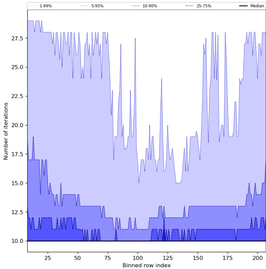
Figure 42: Along track statistics of “Number of iterations” for 2023-07-29 to 2023-07-31
