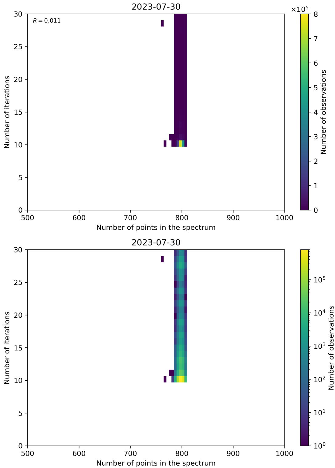
Figure 92: Scatter density plot of “Number of points in the spectrum” against “Number of iterations” for 2023-07-29 to 2023-07-31.
