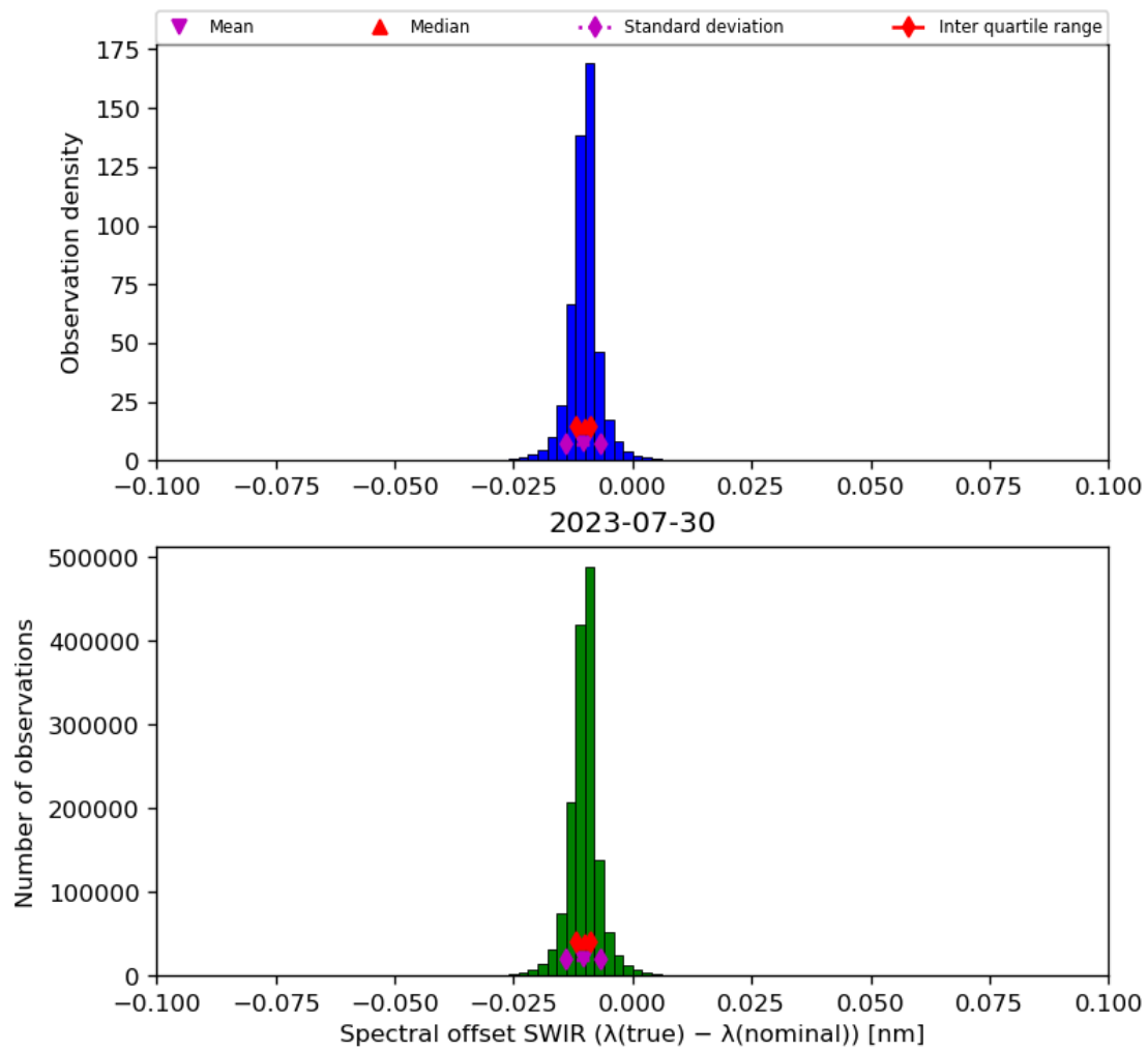
Figure 27: Histogram of “Spectral offset SWIR ( \lambda(\text{true}) - \lambda(\text{nominal}) )” for 2023-07-29 to 2023-07-31
