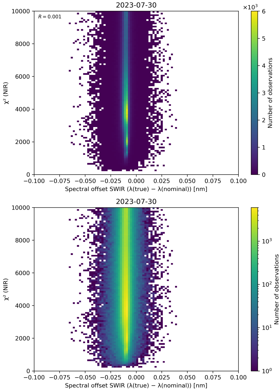
Figure 117: Scatter density plot of “Spectral offset SWIR ( \lambda(\text{true}) - \lambda(\text{nominal}) )” against “ \chi^2 (NIR)” for 2023-07-29 to 2023-07-31.
