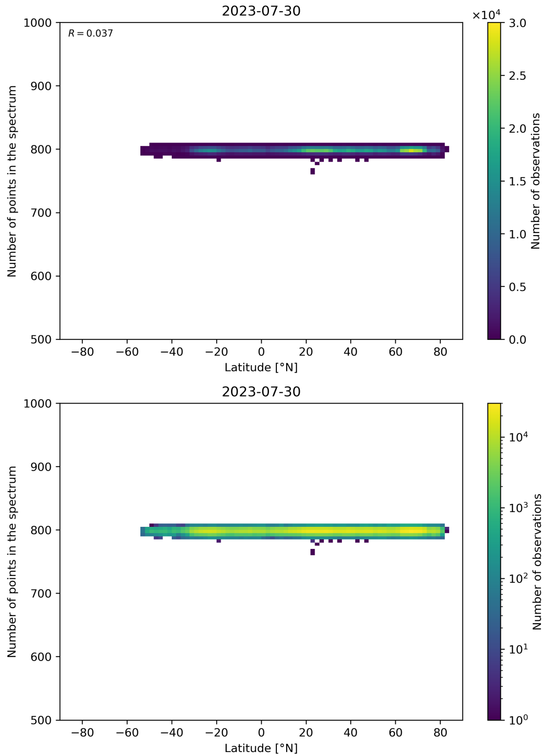
Figure 61: Scatter density plot of “Latitude” against “Number of points in the spectrum” for 2023-07-29 to 2023-07-31.
