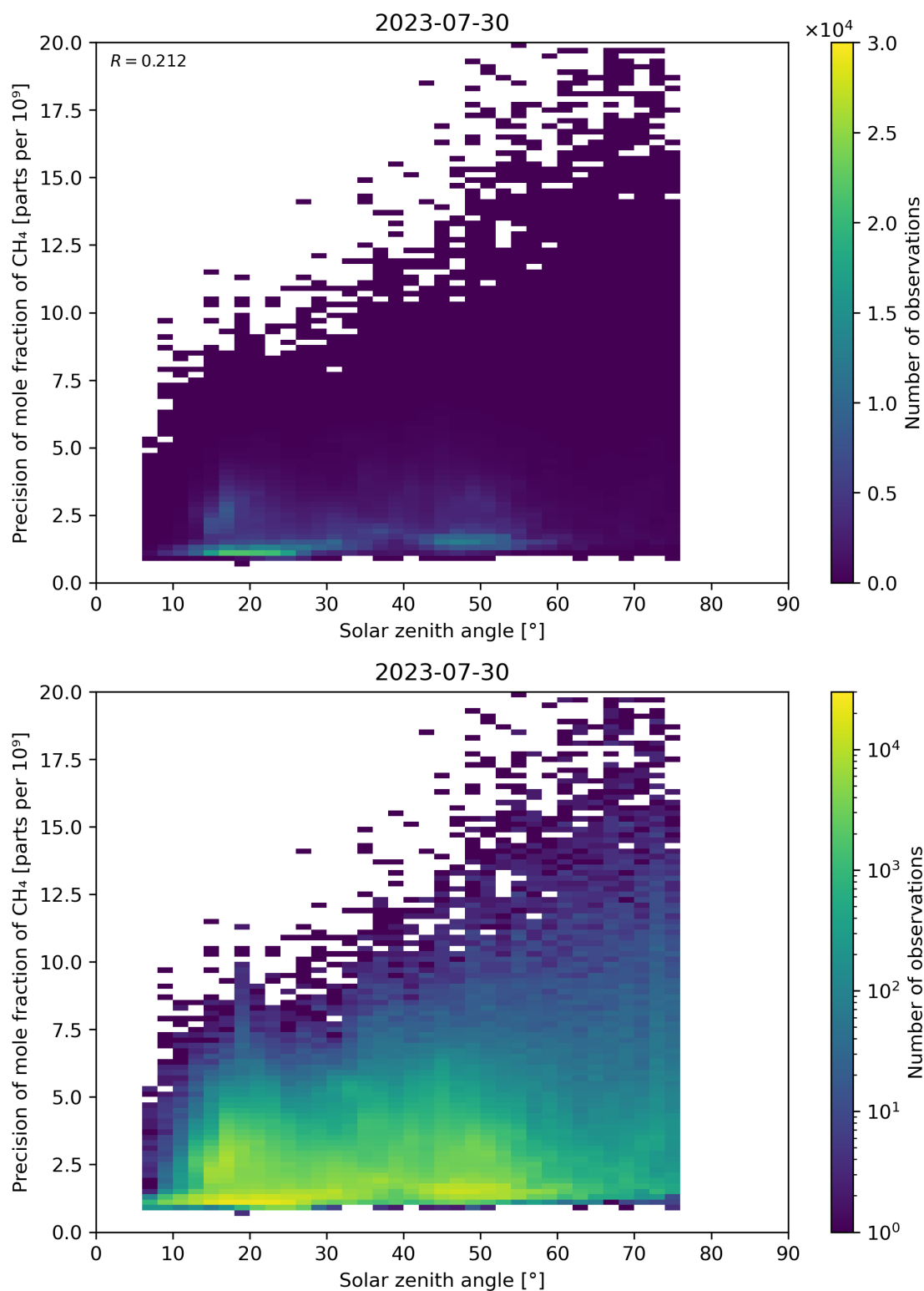
Figure 101: Scatter density plot of “Solar zenith angle” against “Precision of mole fraction of \text{CH}_4 ” for 2023-07-29 to 2023-07-31.
