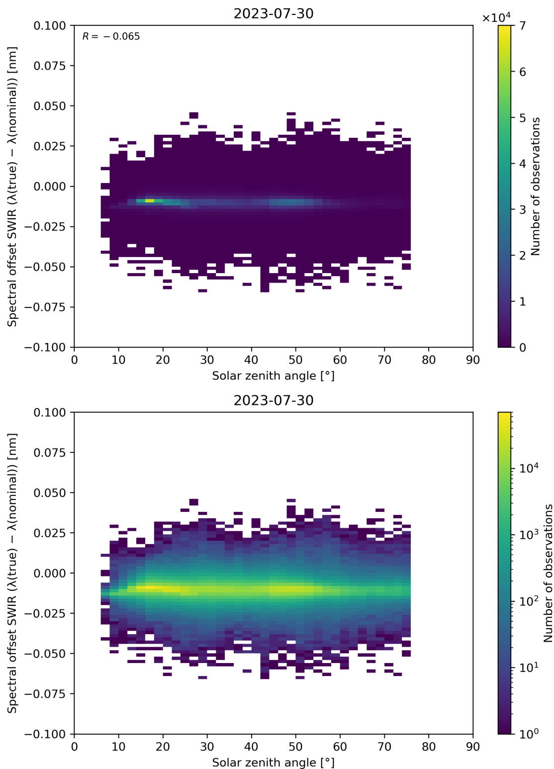
Figure 104: Scatter density plot of “Solar zenith angle” against “Spectral offset SWIR ( \lambda(\text{true}) - \lambda(\text{nominal}) )” for 2023-07-29 to 2023-07-31.
