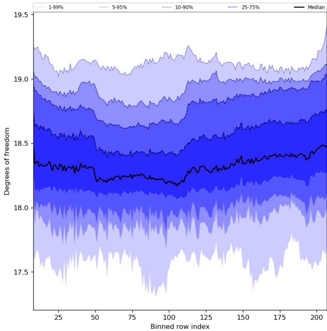
Figure 41: Along track statistics of “Degrees of freedom” for 2023-07-29 to 2023-07-31
