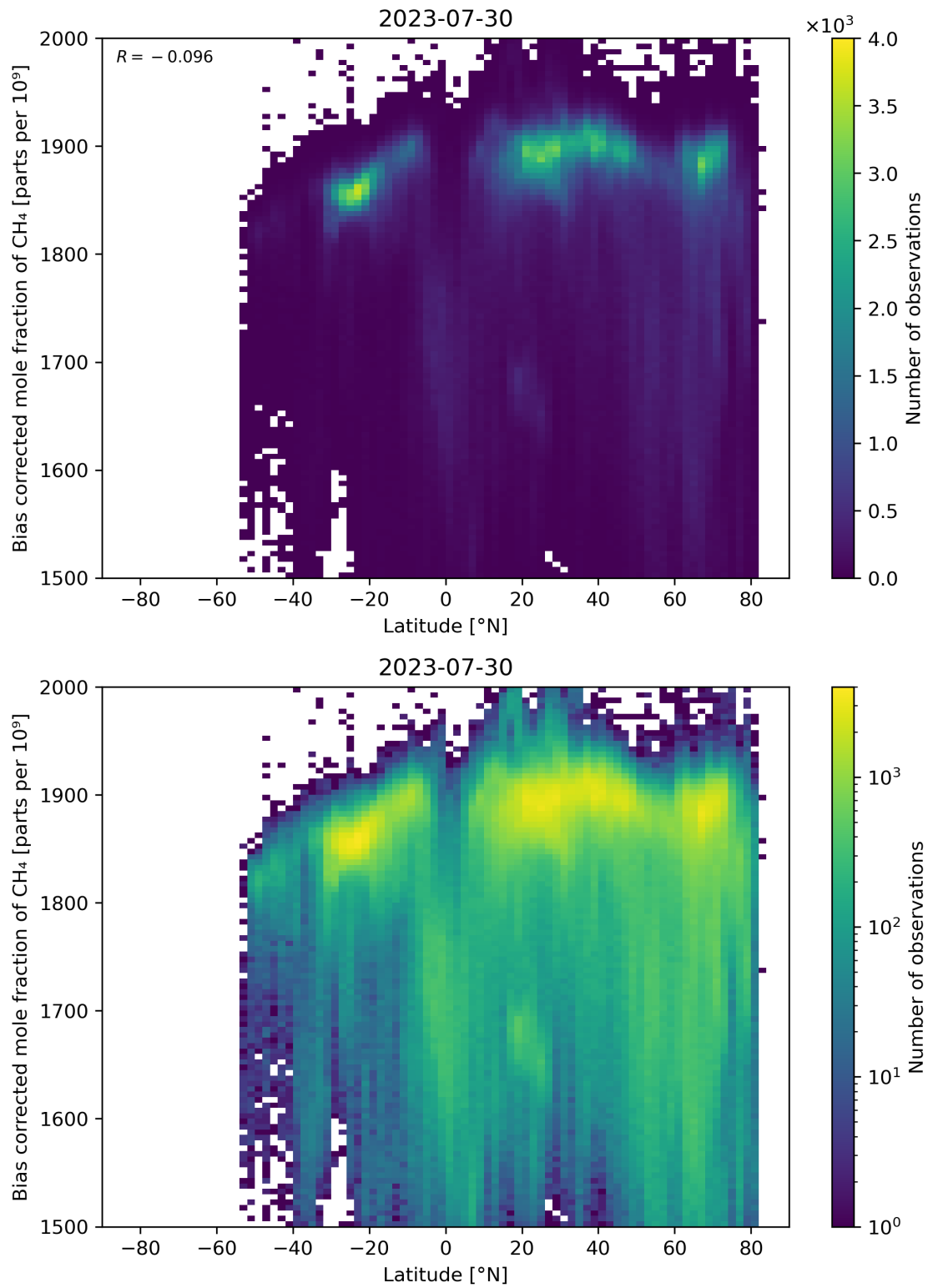
Figure 58: Scatter density plot of “Latitude” against “Bias corrected mole fraction of \text{CH}_4 ” for 2023-07-29 to 2023-07-31.
