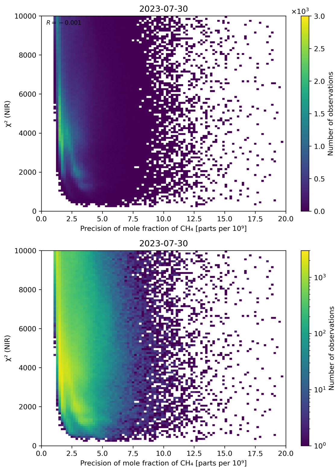
Figure 78: Scatter density plot of “Precision of mole fraction of CH 4 ” against “ \chi^2 (NIR)” for 2023-07-29 to 2023-07-31.
