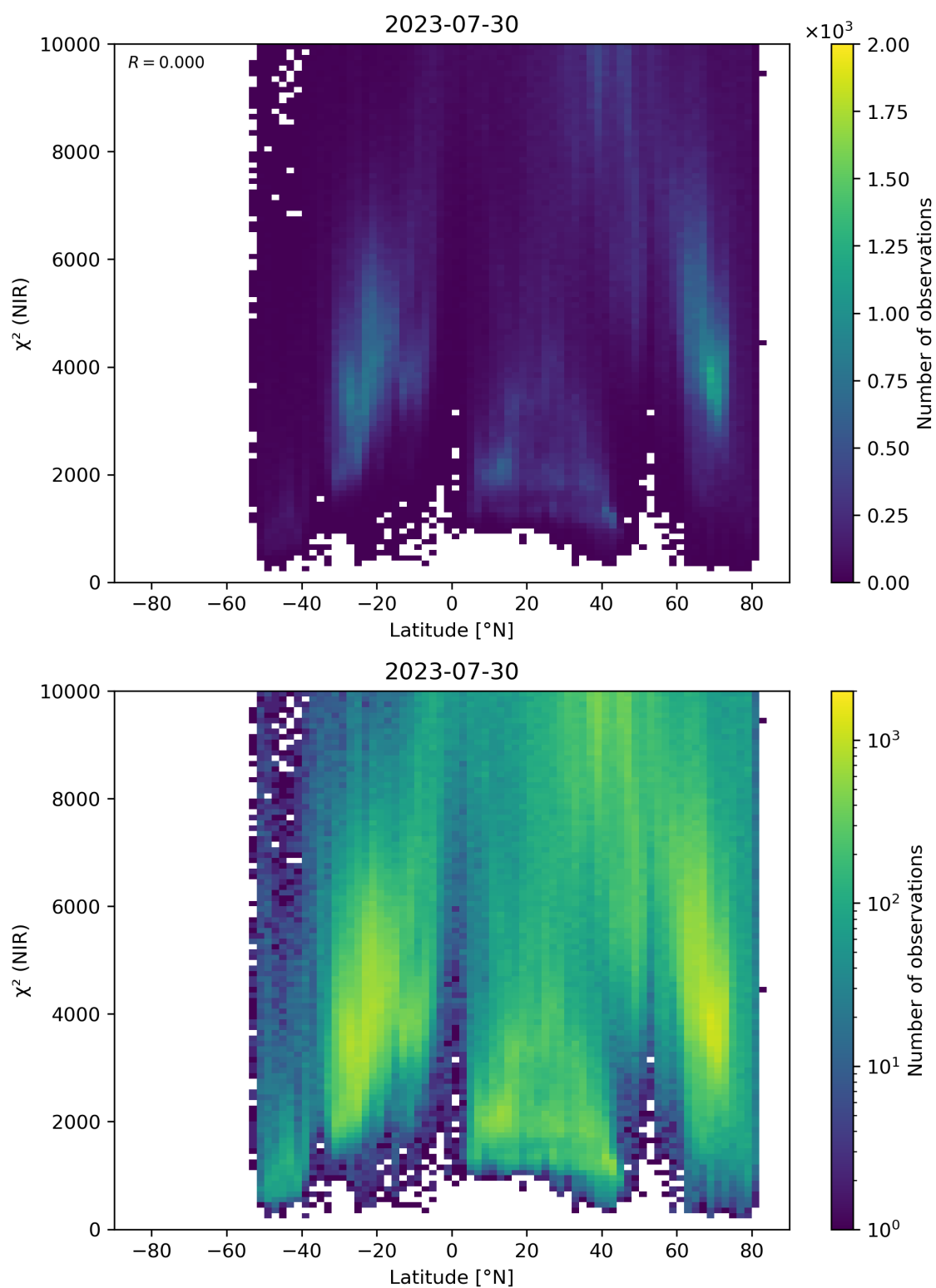
Figure 53: Scatter density plot of “Latitude” against “ \chi^2 (NIR)” for 2023-07-29 to 2023-07-31.
