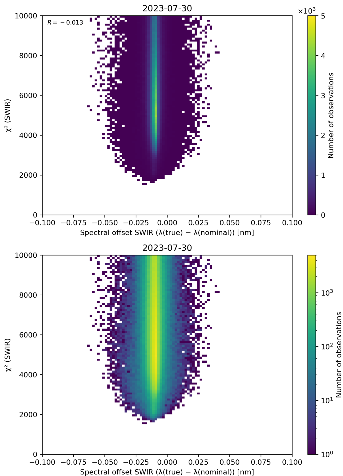
Figure 118: Scatter density plot of “Spectral offset SWIR ( \lambda(\text{true}) - \lambda(\text{nominal}) )” against “ \chi^2 (SWIR)” for 2023-07-29 to 2023-07-31.
