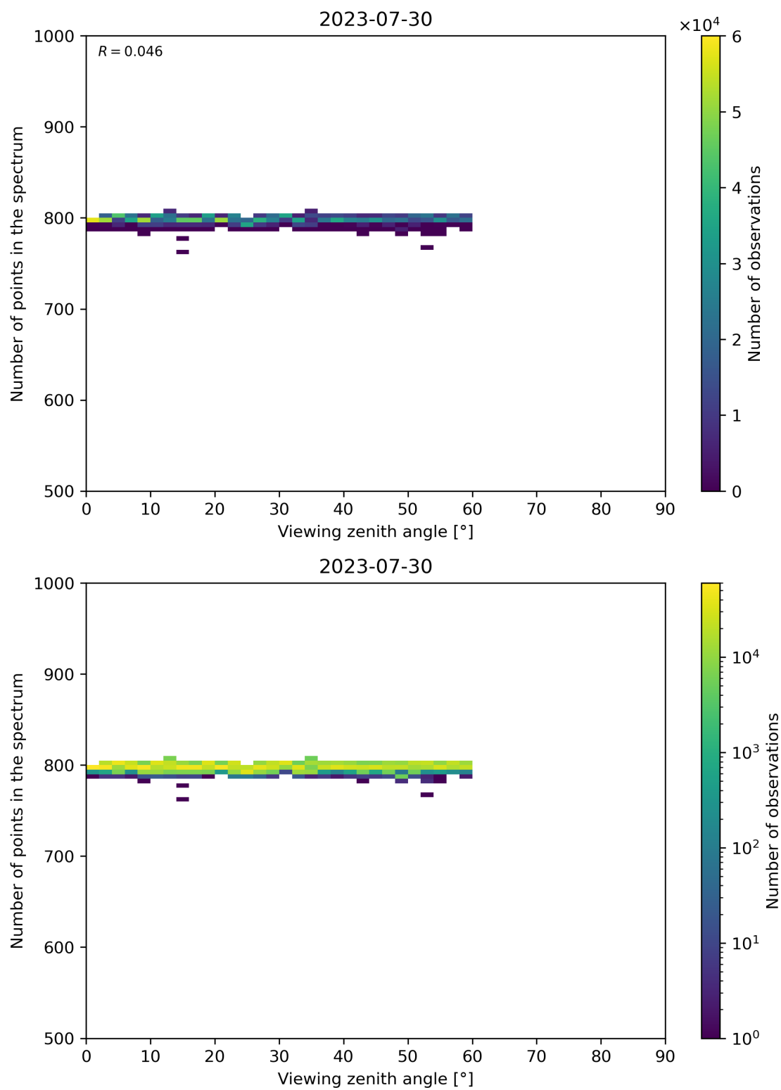
Figure 114: Scatter density plot of “Viewing zenith angle” against “Number of points in the spectrum” for 2023-07-29 to 2023-07-31.
