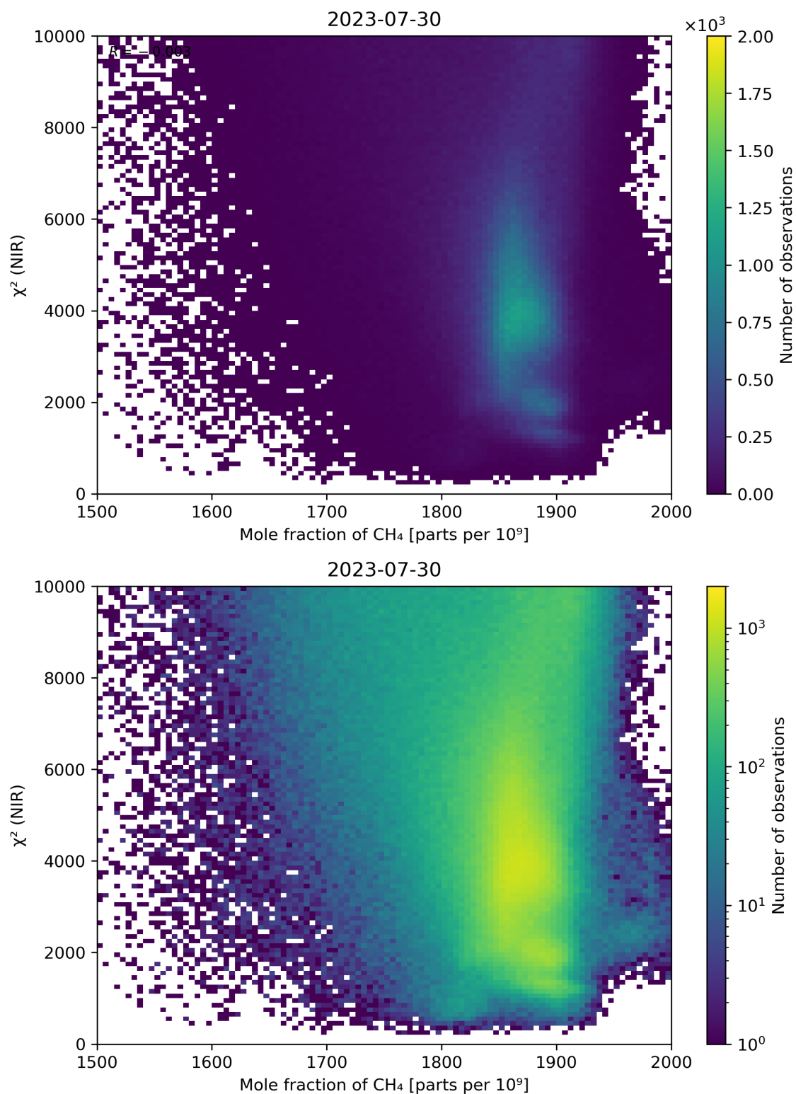
Figure 70: Scatter density plot of “Mole fraction of \text{CH}_4 ” against “ \chi^2 (NIR)” for 2023-07-29 to 2023-07-31.
