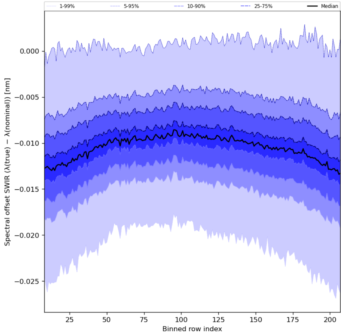
Figure 38: Along track statistics of “Spectral offset SWIR ( \lambda(\text{true}) - \lambda(\text{nominal}) )” for 2023-07-29 to 2023-07-31
