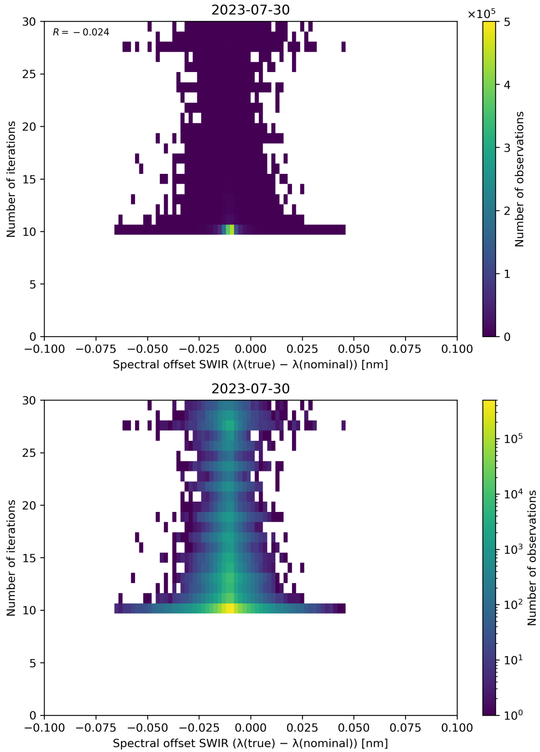
Figure 121: Scatter density plot of “Spectral offset SWIR ( \lambda(\text{true}) - \lambda(\text{nominal}) )” against “Number of iterations” for 2023-07-29 to 2023-07-31.
