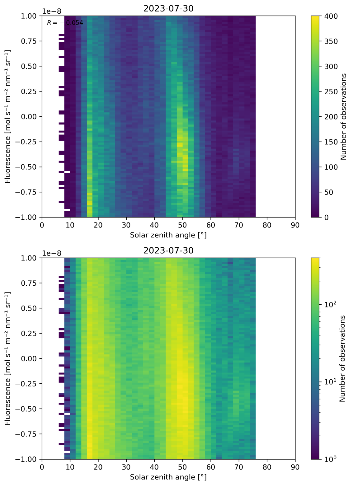
Figure 97: Scatter density plot of “Solar zenith angle” against “Fluorescence” for 2023-07-29 to 2023-07-31.
