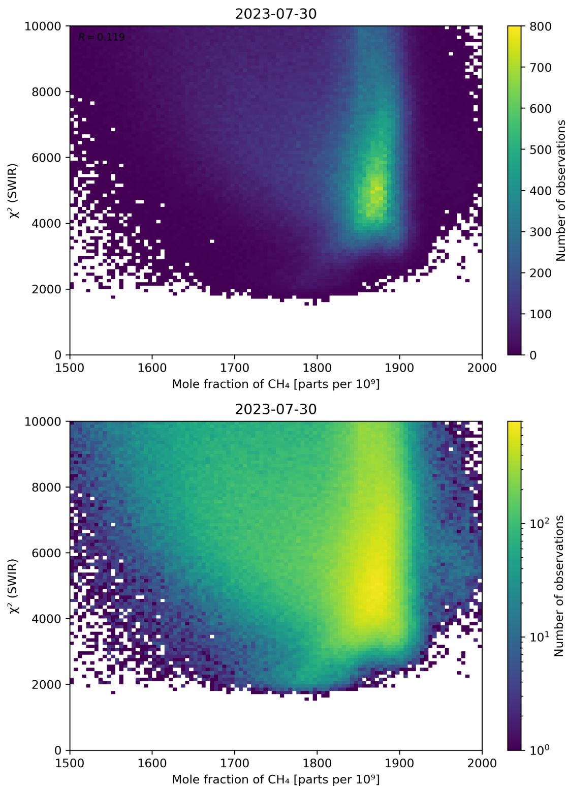
Figure 71: Scatter density plot of “Mole fraction of CH 4 ” against “ \chi^2 (SWIR)” for 2023-07-29 to 2023-07-31.
