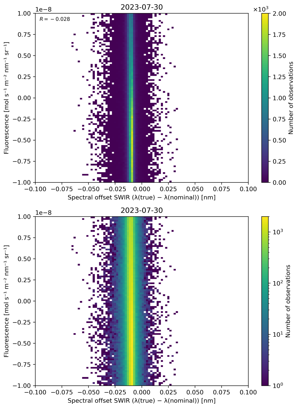
Figure 120: Scatter density plot of “Spectral offset SWIR ( \lambda(\text{true}) - \lambda(\text{nominal}) )” against “Fluorescence” for 2023-07-29 to 2023-07-31.
