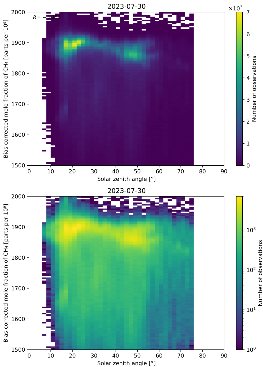
Figure 100: Scatter density plot of “Solar zenith angle” against “Bias corrected mole fraction of CH 4 ” for 2023-07-29 to 2023-07-31.
