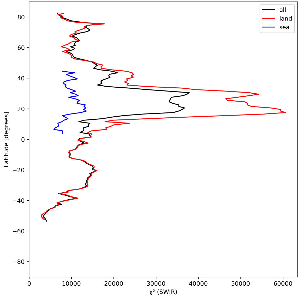
Figure 17: Zonal average of “ \chi^2 (SWIR)” for 2023-07-29 to 2023-07-31.
