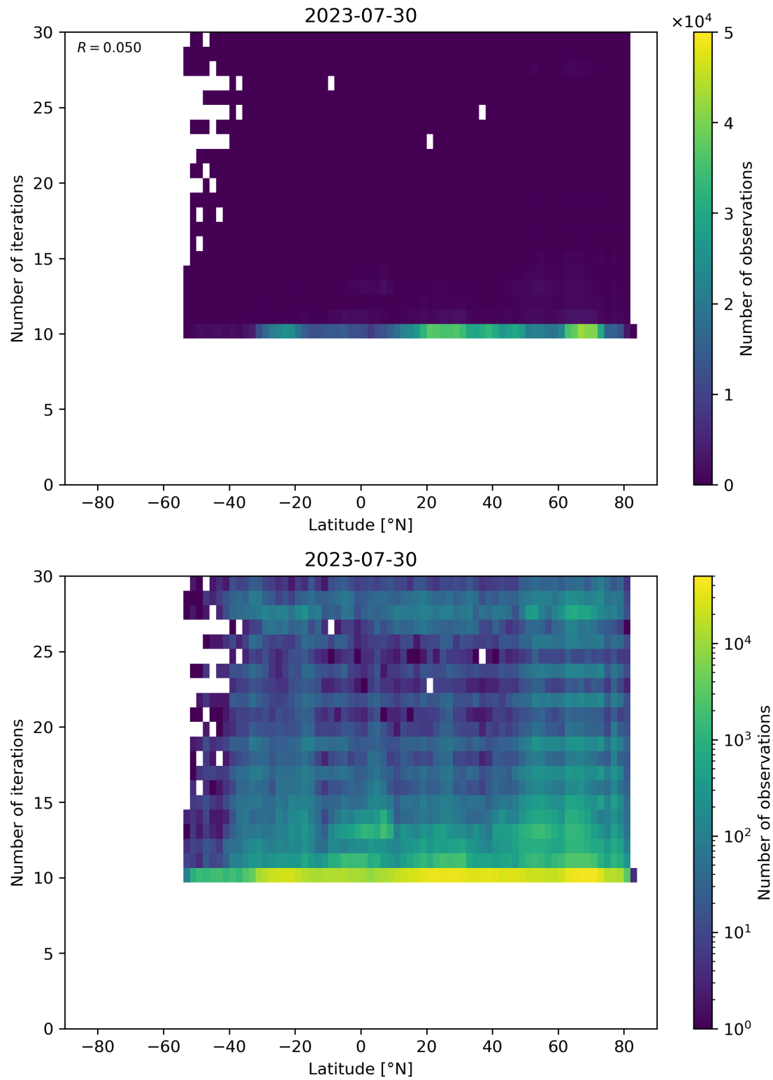
Figure 60: Scatter density plot of “Latitude” against “Number of iterations” for 2023-07-29 to 2023-07-31.
