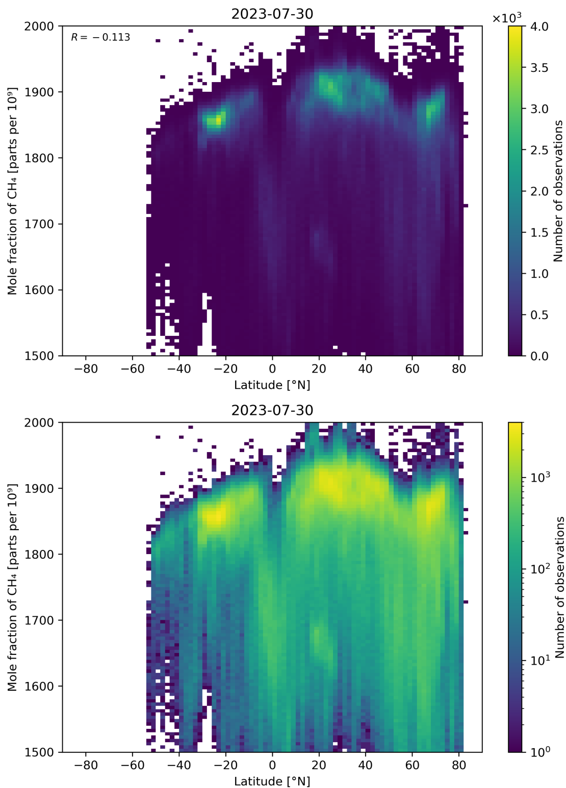
Figure 57: Scatter density plot of “Latitude” against “Mole fraction of CH 4 ” for 2023-07-29 to 2023-07-31.
