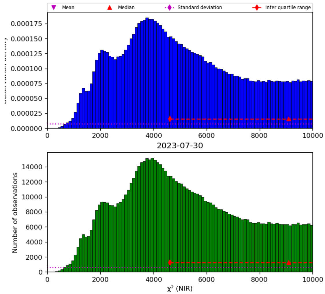
Figure 29: Histogram of “ \chi^2 (NIR)” for 2023-07-29 to 2023-07-31
