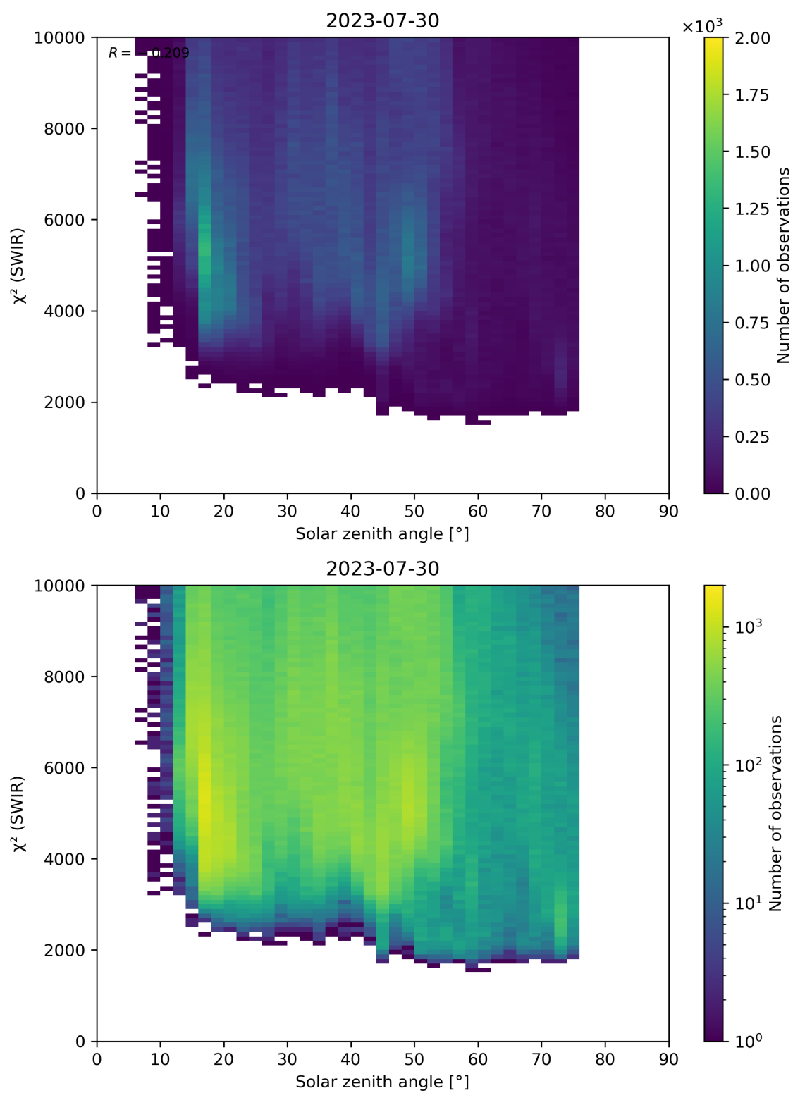
Figure 95: Scatter density plot of “Solar zenith angle” against “ \chi^2 (SWIR)” for 2023-07-29 to 2023-07-31.
