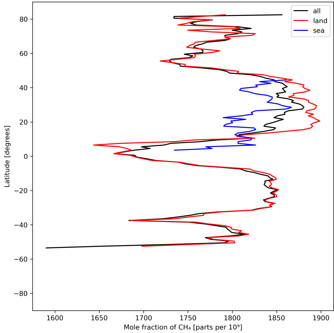
Figure 12: Zonal average of “Mole fraction of CH 4 ” for 2023-07-29 to 2023-07-31.
