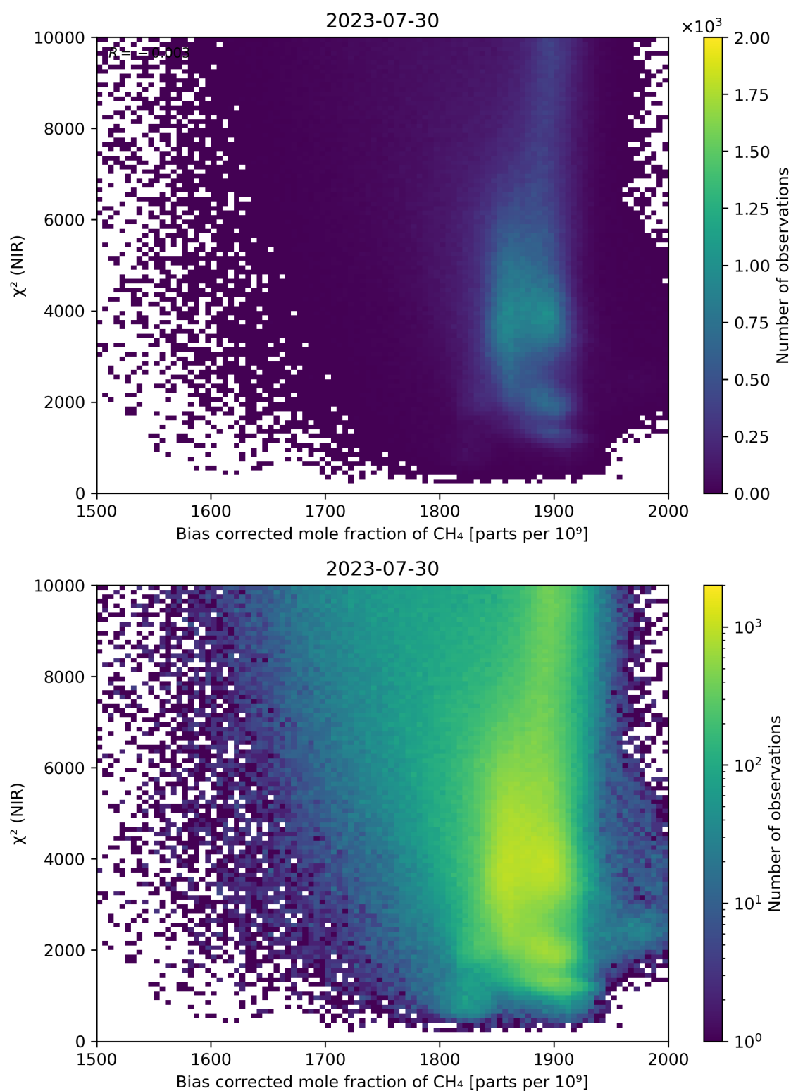
Figure 63: Scatter density plot of “Bias corrected mole fraction of CH 4 ” against “ \chi^2 (NIR)” for 2023-07-29 to 2023-07-31.
