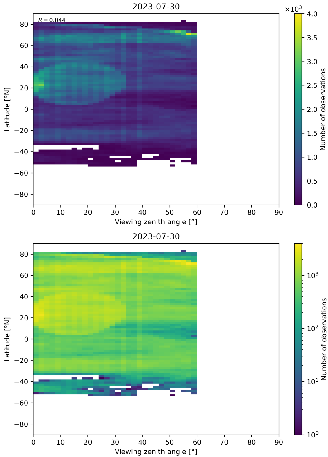
Figure 109: Scatter density plot of “Viewing zenith angle” against “Latitude” for 2023-07-29 to 2023-07-31.
