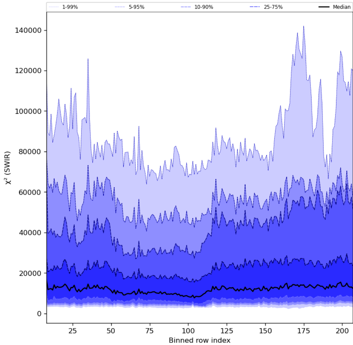
Figure 39: Along track statistics of “ \chi^2 (SWIR)” for 2023-07-29 to 2023-07-31
