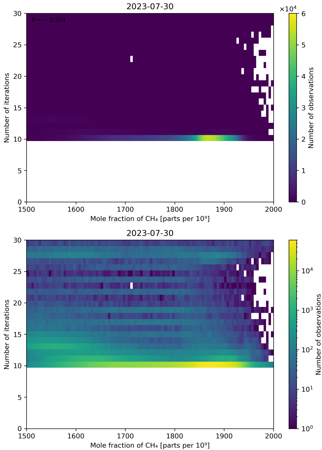
Figure 76: Scatter density plot of “Mole fraction of CH 4 ” against “Number of iterations” for 2023-07-29 to 2023-07-31.
