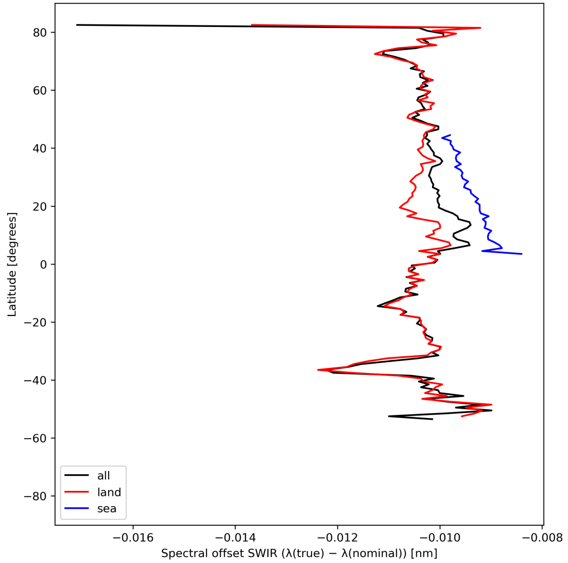
Figure 16: Zonal average of “Spectral offset SWIR ( \lambda(\text{true}) - \lambda(\text{nominal}) )” for 2023-07-29 to 2023-07-31.
