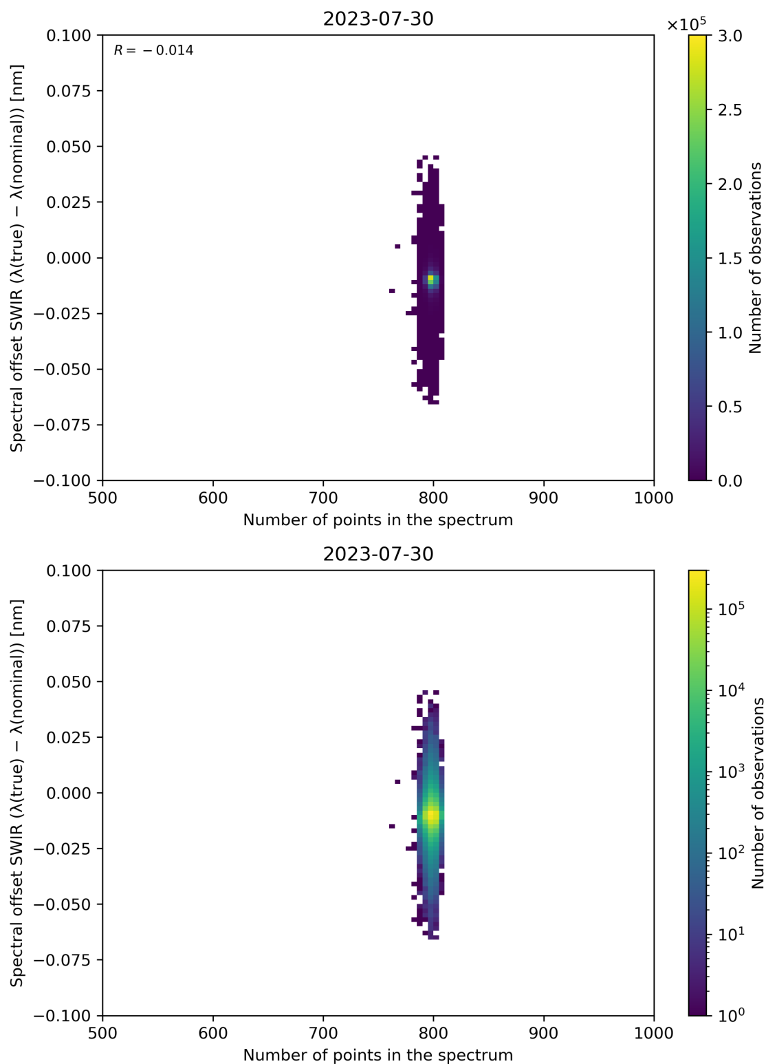
Figure 93: Scatter density plot of “Number of points in the spectrum” against “Spectral offset SWIR ( \lambda(\text{true}) - \lambda(\text{nominal}) )” for 2023-07-29 to 2023-07-31.
