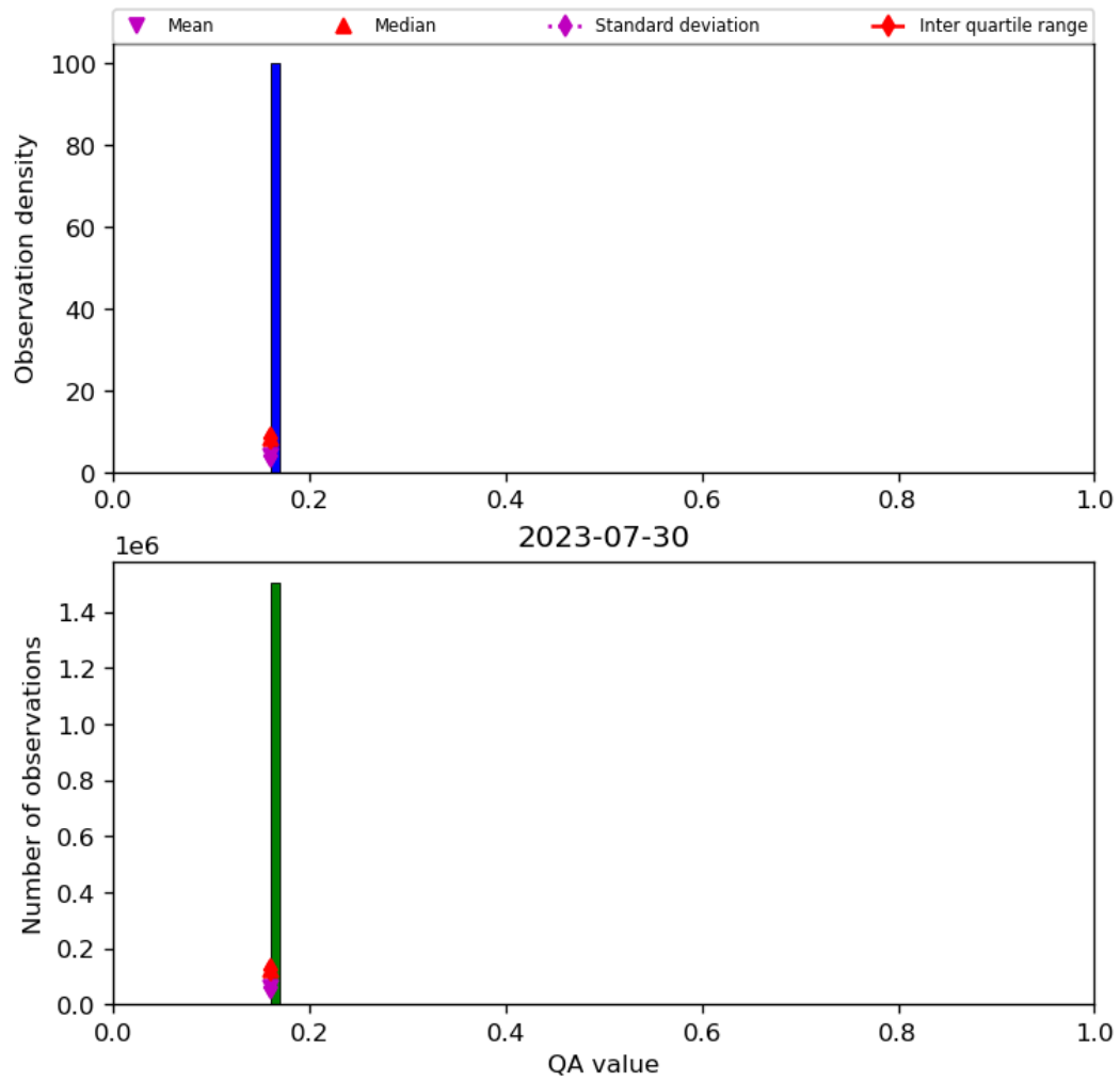
Figure 22: Histogram of “QA value” for 2023-07-29 to 2023-07-31
