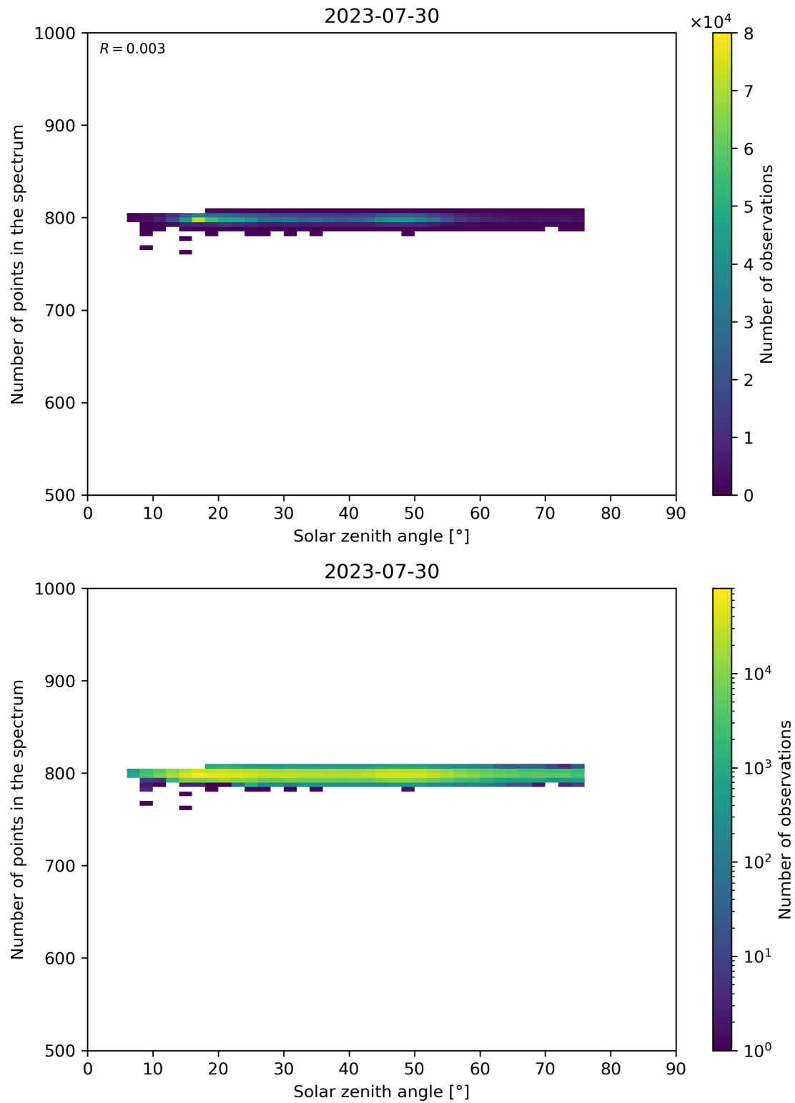
Figure 103: Scatter density plot of “Solar zenith angle” against “Number of points in the spectrum” for 2023-07-29 to 2023-07-31.
