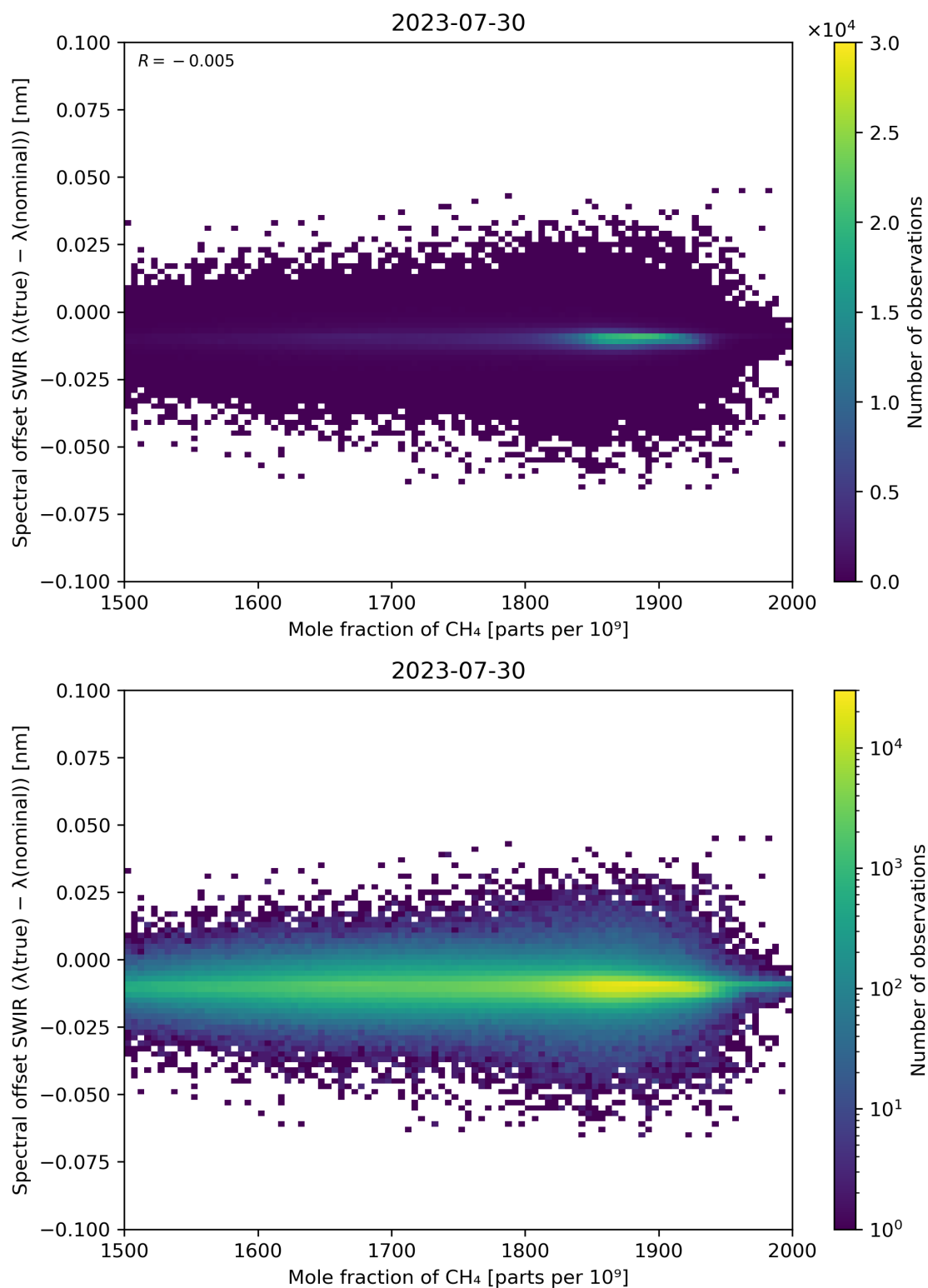
Figure 86: Scatter density plot of “Mole fraction of CH 4 ” against “Spectral offset SWIR ( \lambda(\text{true}) - \lambda(\text{nominal}) )” for 2023-07-29 to 2023-07-31.
