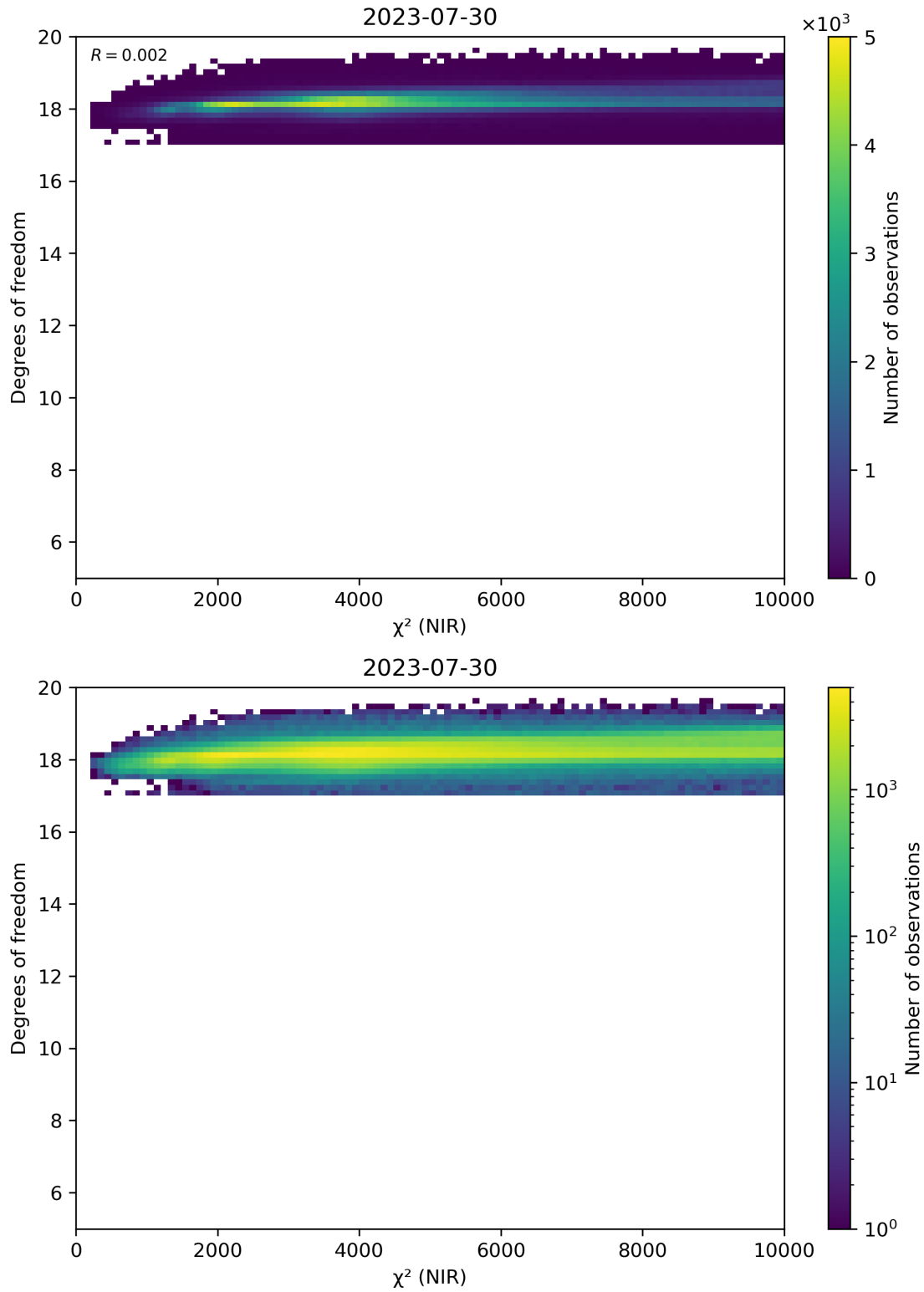
Figure 44: Scatter density plot of “ \chi^2 (NIR)” against “Degrees of freedom” for 2023-07-29 to 2023-07-31.
