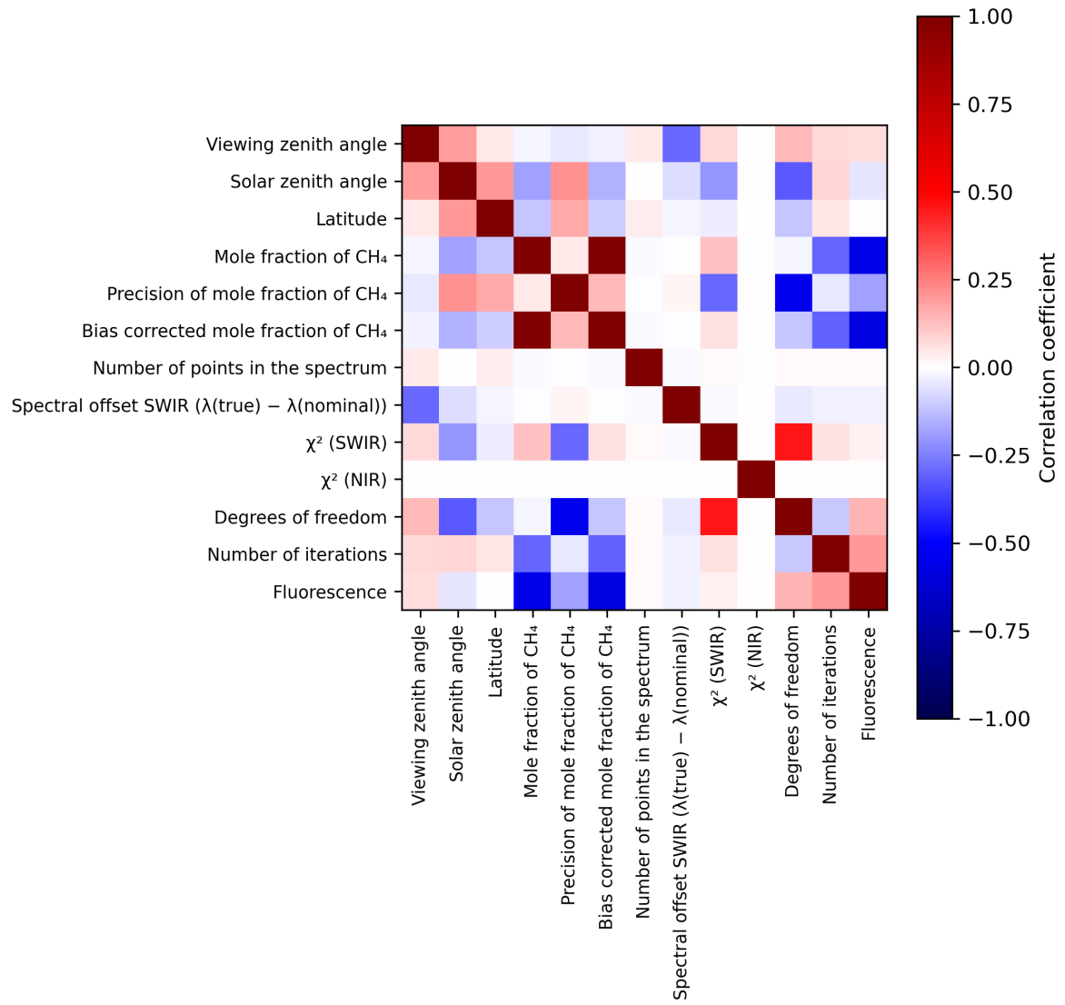
Figure 2: Map of correlation matrix for 2023-07-29 to 2023-07-31.
