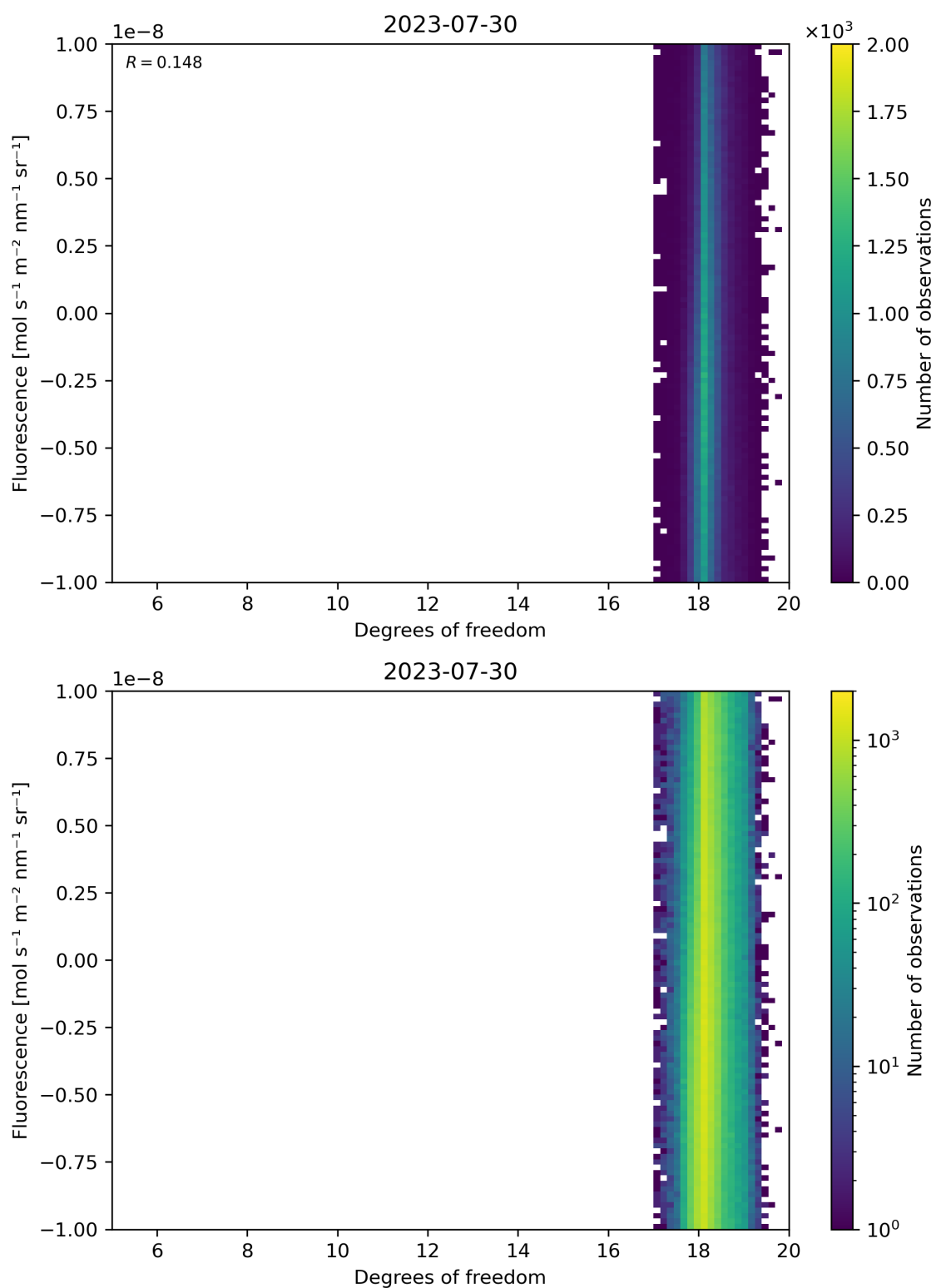
Figure 51: Scatter density plot of “Degrees of freedom” against “Fluorescence” for 2023-07-29 to 2023-07-31.
