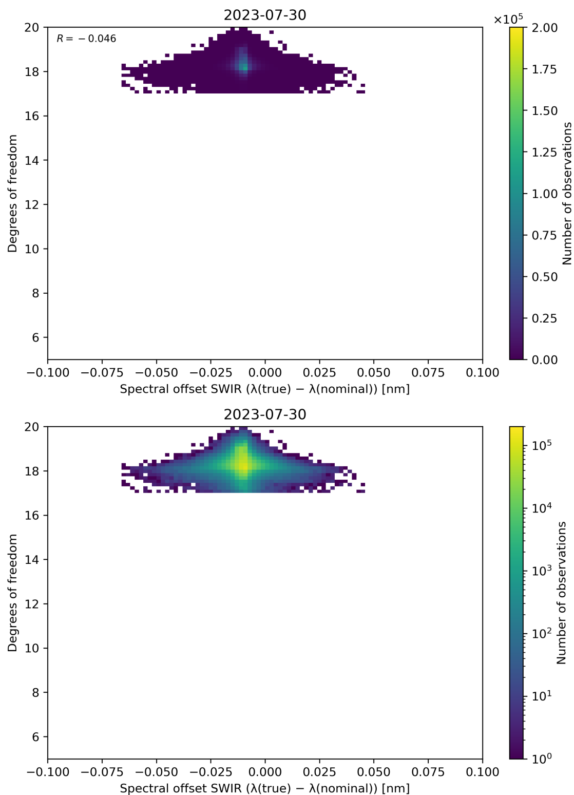
Figure 119: Scatter density plot of “Spectral offset SWIR ( \lambda(\text{true}) - \lambda(\text{nominal}) )” against “Degrees of freedom” for 2023-07-29 to 2023-07-31.
