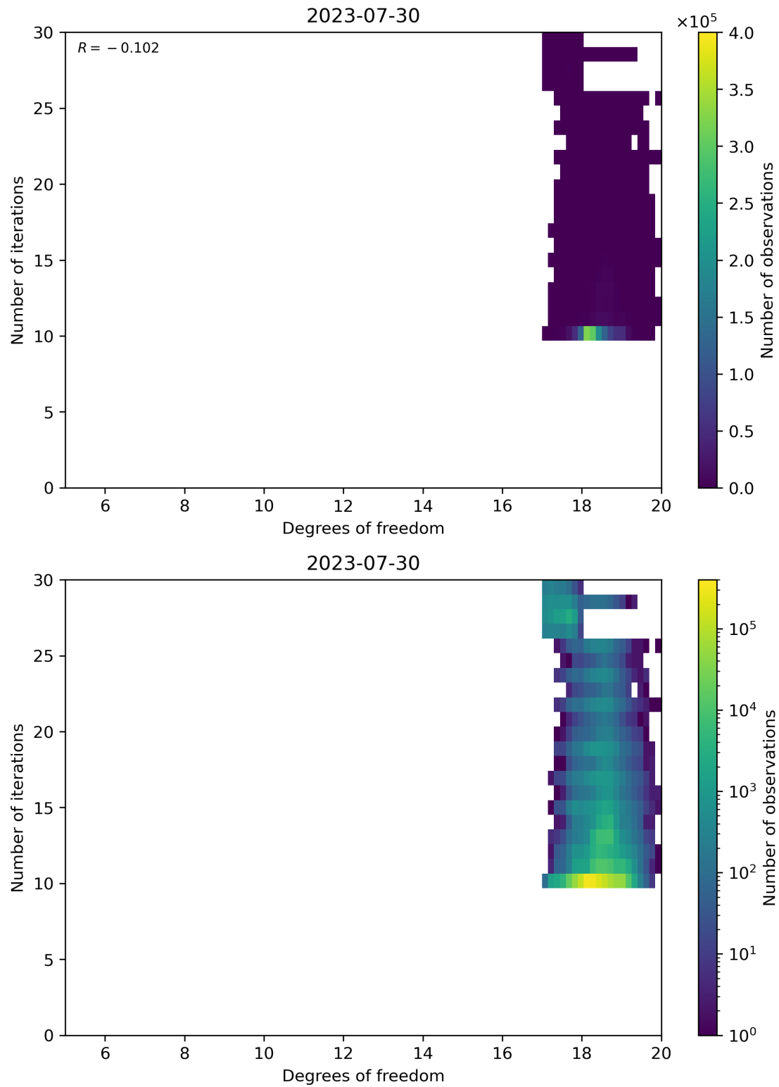
Figure 52: Scatter density plot of “Degrees of freedom” against “Number of iterations” for 2023-07-29 to 2023-07-31.
