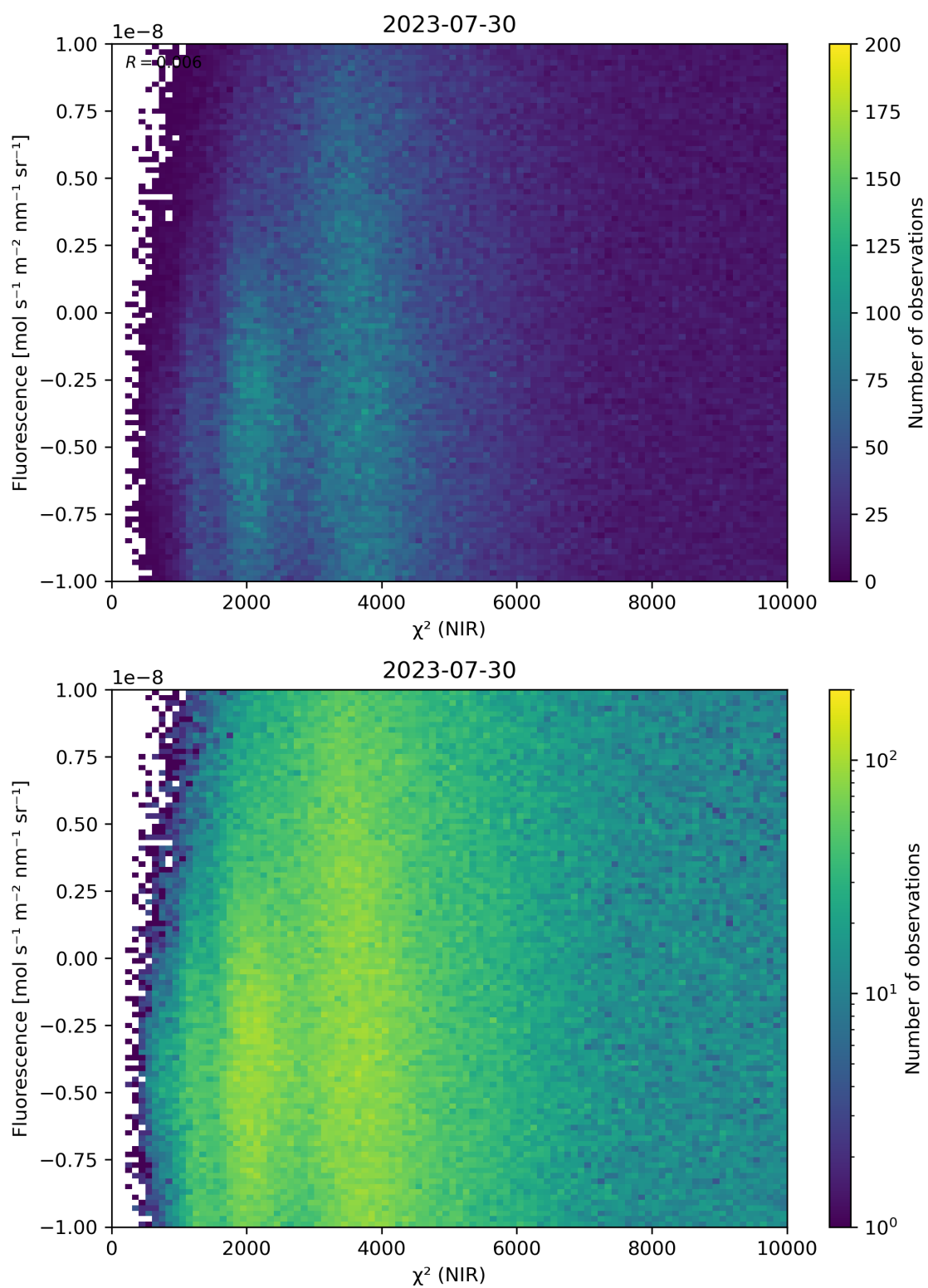
Figure 45: Scatter density plot of “ \chi^2 (NIR)” against “Fluorescence” for 2023-07-29 to 2023-07-31.
