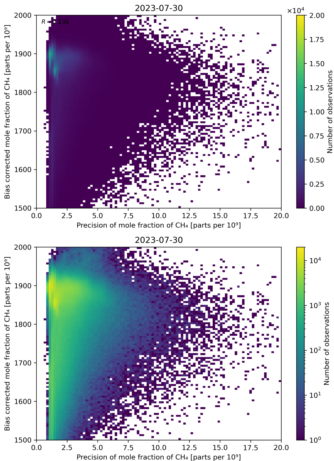
Figure 82: Scatter density plot of “Precision of mole fraction of CH 4 ” against “Bias corrected mole fraction of CH 4 ” for 2023-07-29 to 2023-07-31.
