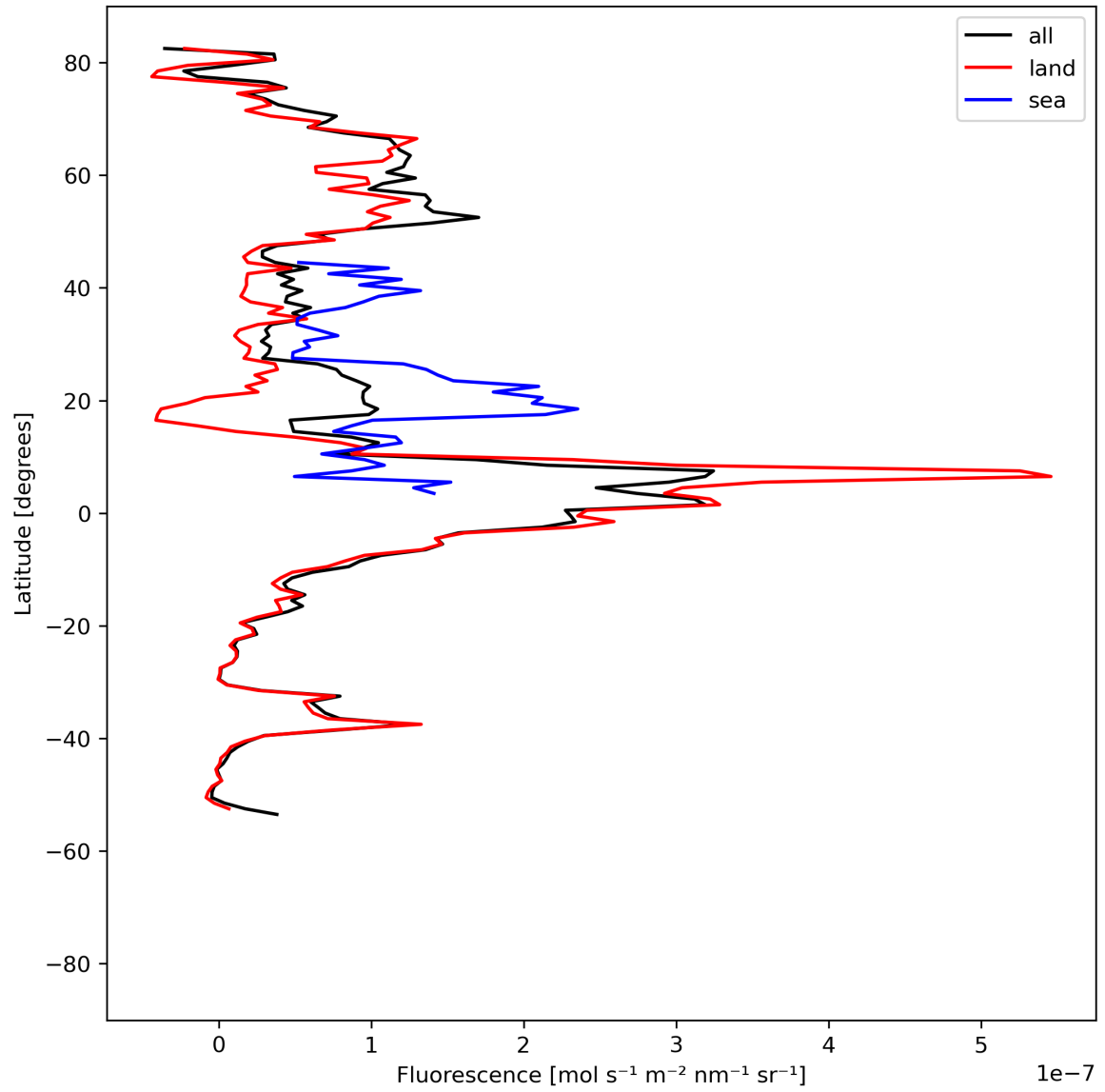
Figure 21: Zonal average of “Fluorescence” for 2023-07-29 to 2023-07-31.
