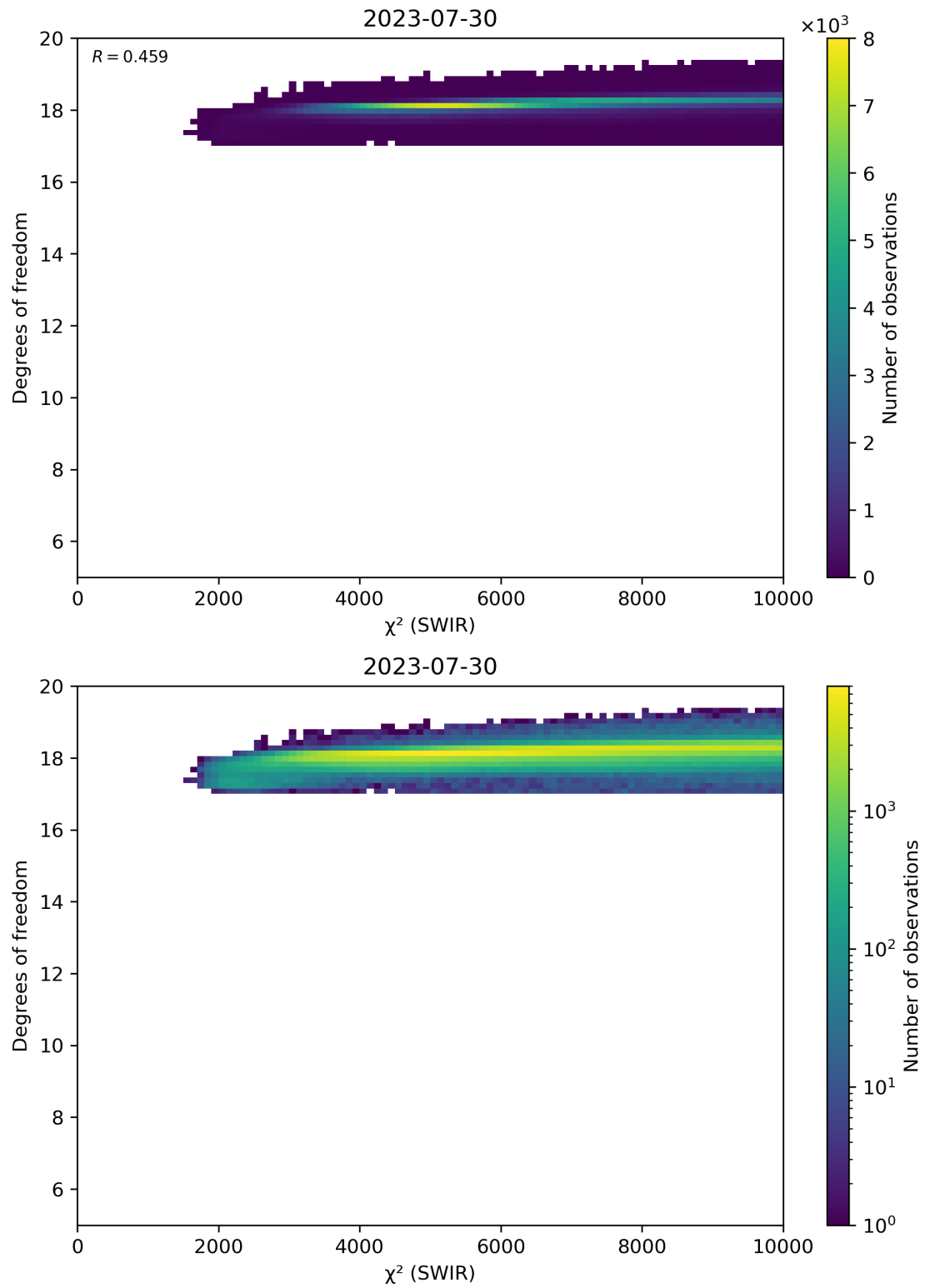
Figure 48: Scatter density plot of “ \chi^2 (SWIR)” against “Degrees of freedom” for 2023-07-29 to 2023-07-31.
