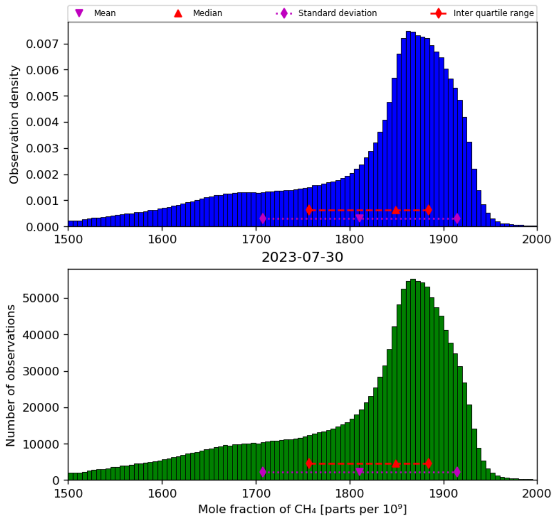
Figure 23: Histogram of “Mole fraction of CH 4 ” for 2023-07-29 to 2023-07-31
