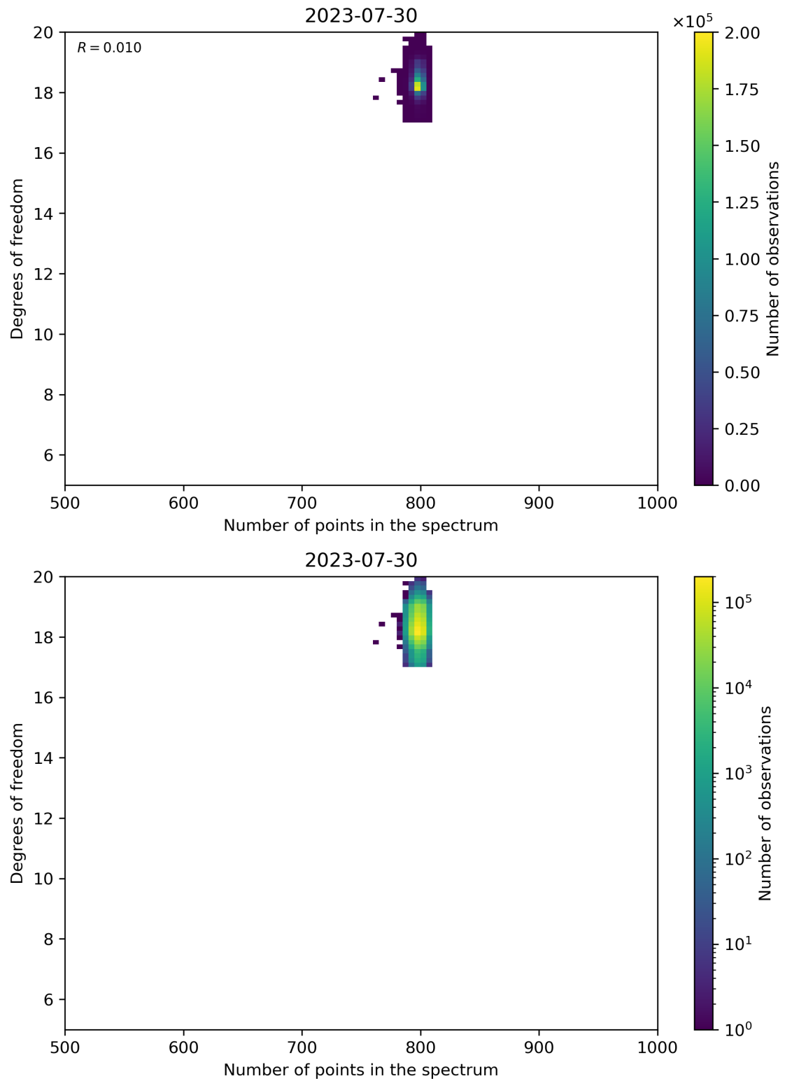
Figure 90: Scatter density plot of “Number of points in the spectrum” against “Degrees of freedom” for 2023-07-29 to 2023-07-31.
