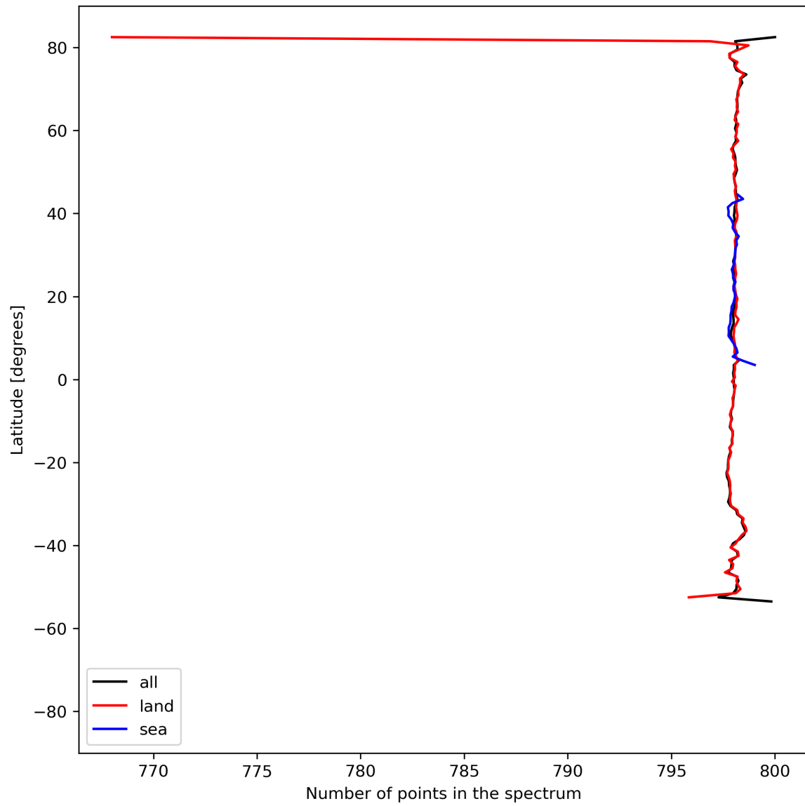
Figure 15: Zonal average of “Number of points in the spectrum” for 2023-07-29 to 2023-07-31.
