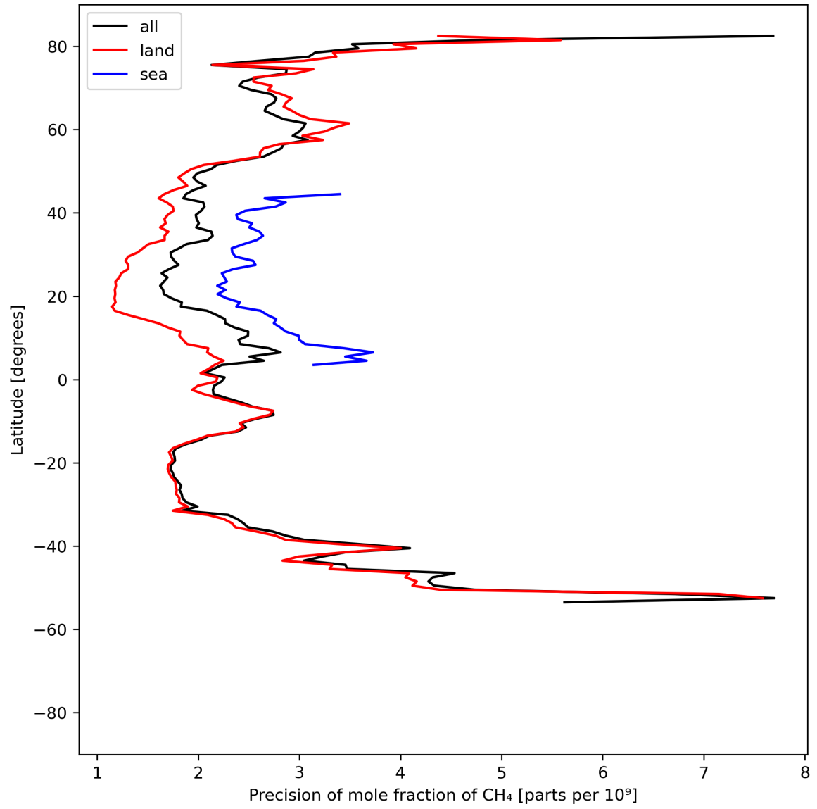
Figure 13: Zonal average of “Precision of mole fraction of CH 4 ” for 2023-07-29 to 2023-07-31.
