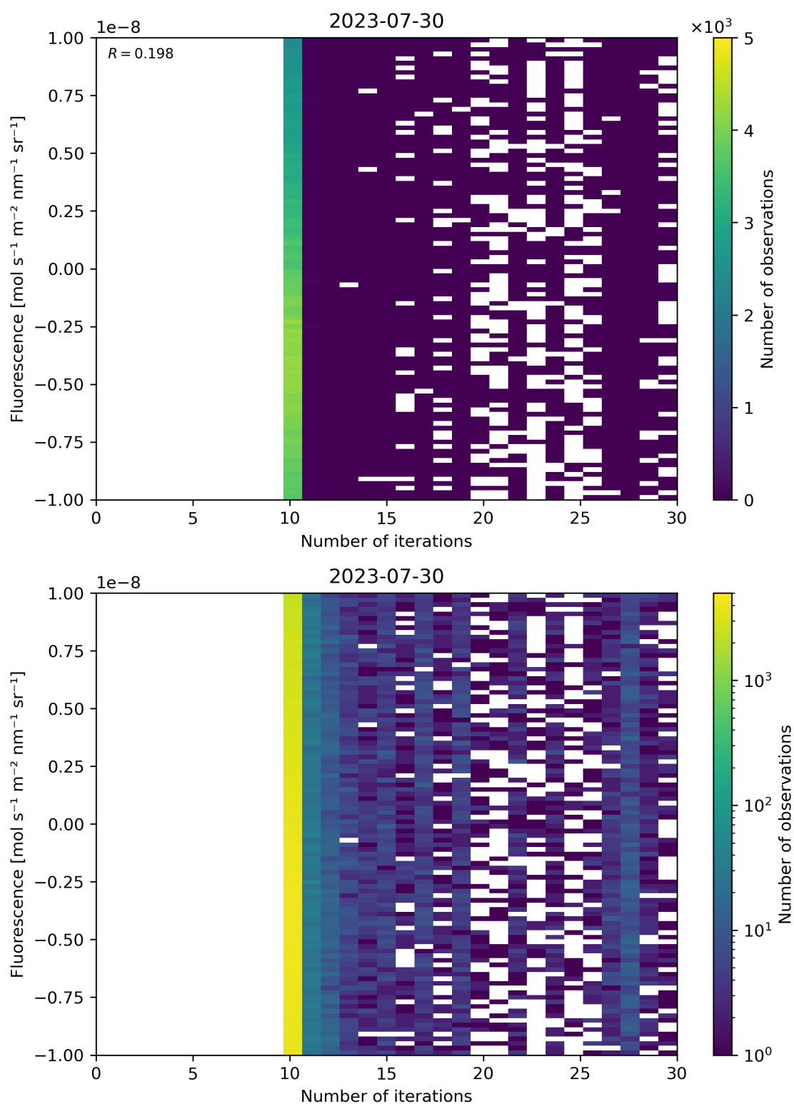
Figure 87: Scatter density plot of “Number of iterations” against “Fluorescence” for 2023-07-29 to 2023-07-31.
