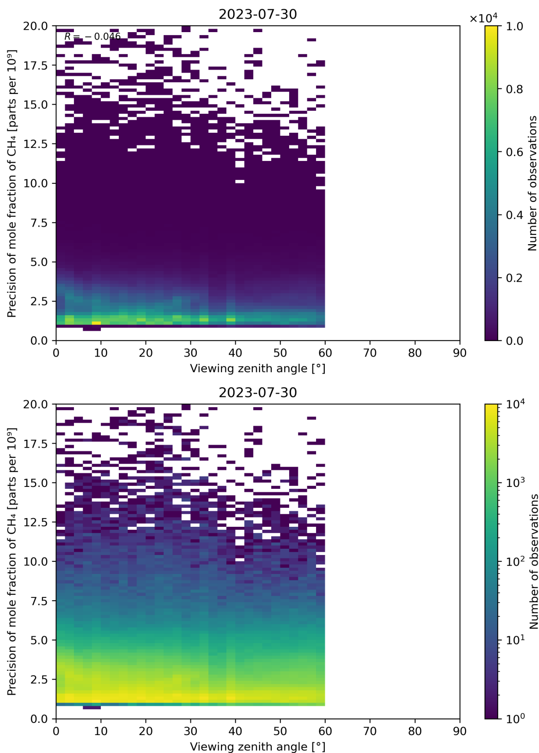
Figure 112: Scatter density plot of “Viewing zenith angle” against “Precision of mole fraction of \text{CH}_4 ” for 2023-07-29 to 2023-07-31.
