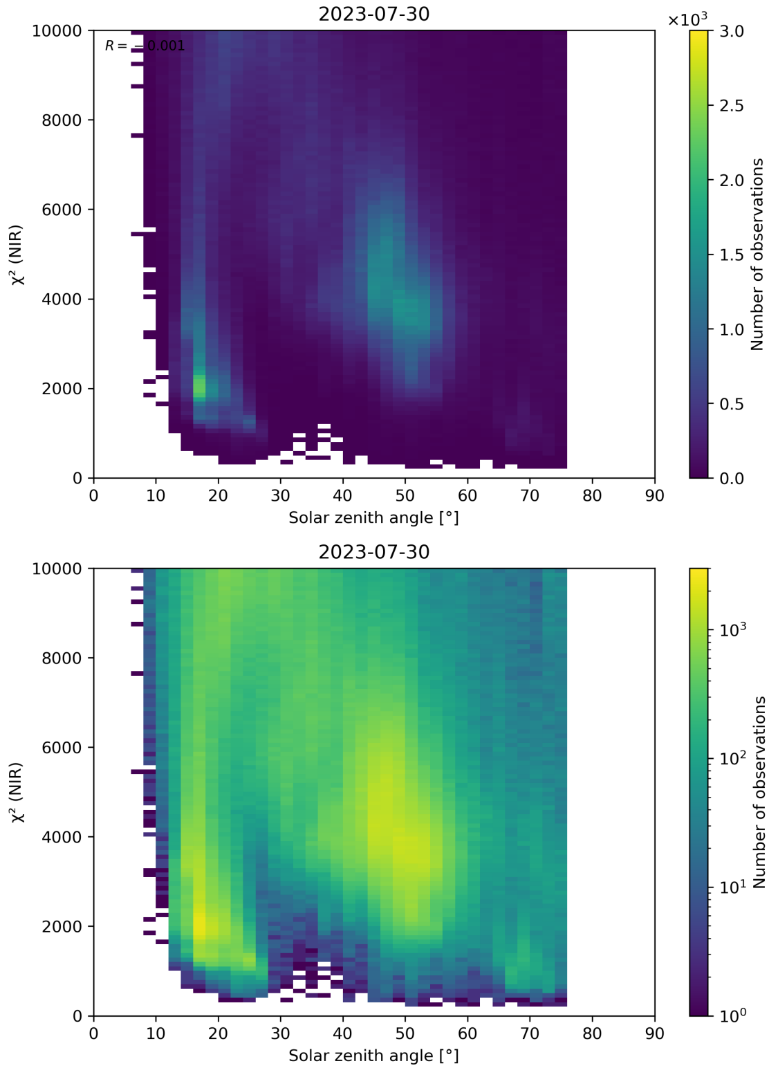
Figure 94: Scatter density plot of “Solar zenith angle” against “ \chi^2 (NIR)” for 2023-07-29 to 2023-07-31.
