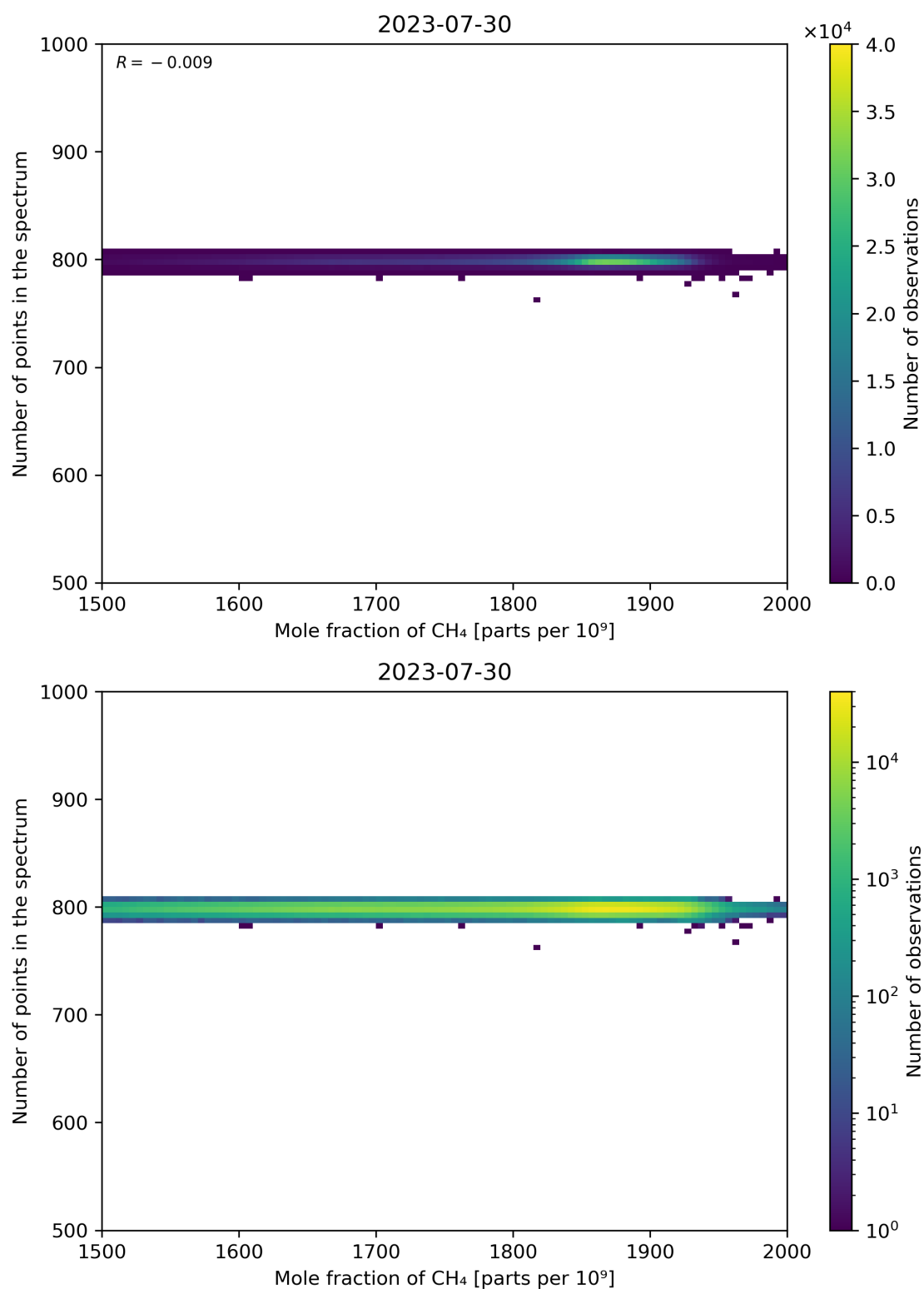
Figure 77: Scatter density plot of “Mole fraction of CH 4 ” against “Number of points in the spectrum” for 2023-07-29 to 2023-07-31.
