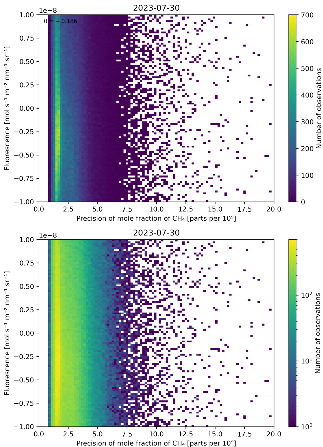
Figure 81: Scatter density plot of “Precision of mole fraction of \text{CH}_4 ” against “Fluorescence” for 2023-07-29 to 2023-07-31.
