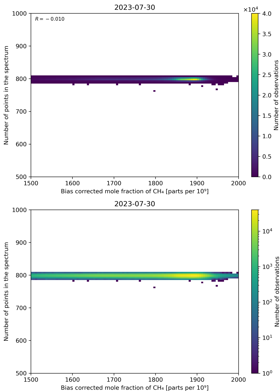
Figure 68: Scatter density plot of “Bias corrected mole fraction of CH 4 ” against “Number of points in the spectrum” for 2023-07-29 to 2023-07-31.
