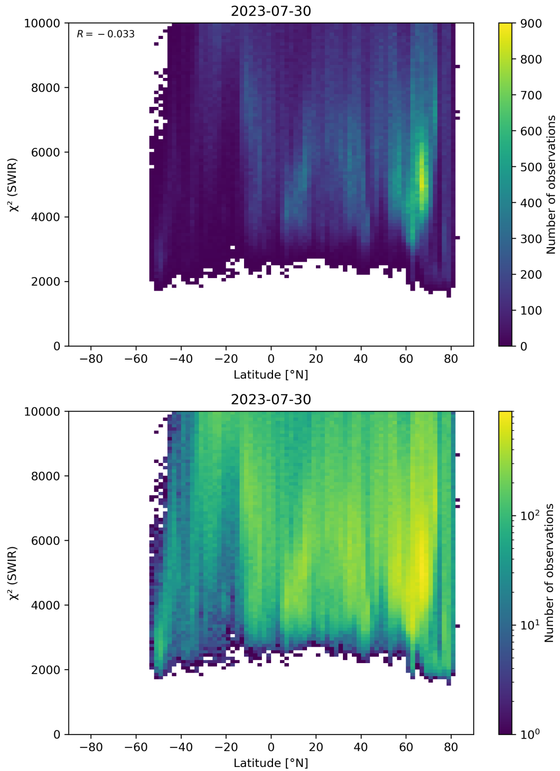
Figure 54: Scatter density plot of “Latitude” against “ \chi^2 (SWIR)” for 2023-07-29 to 2023-07-31.
