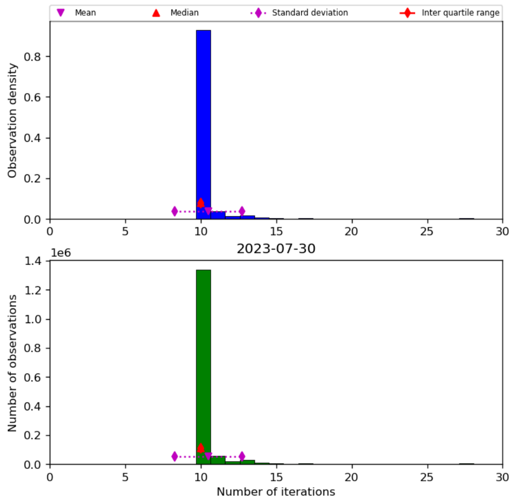
Figure 31: Histogram of “Number of iterations” for 2023-07-29 to 2023-07-31
