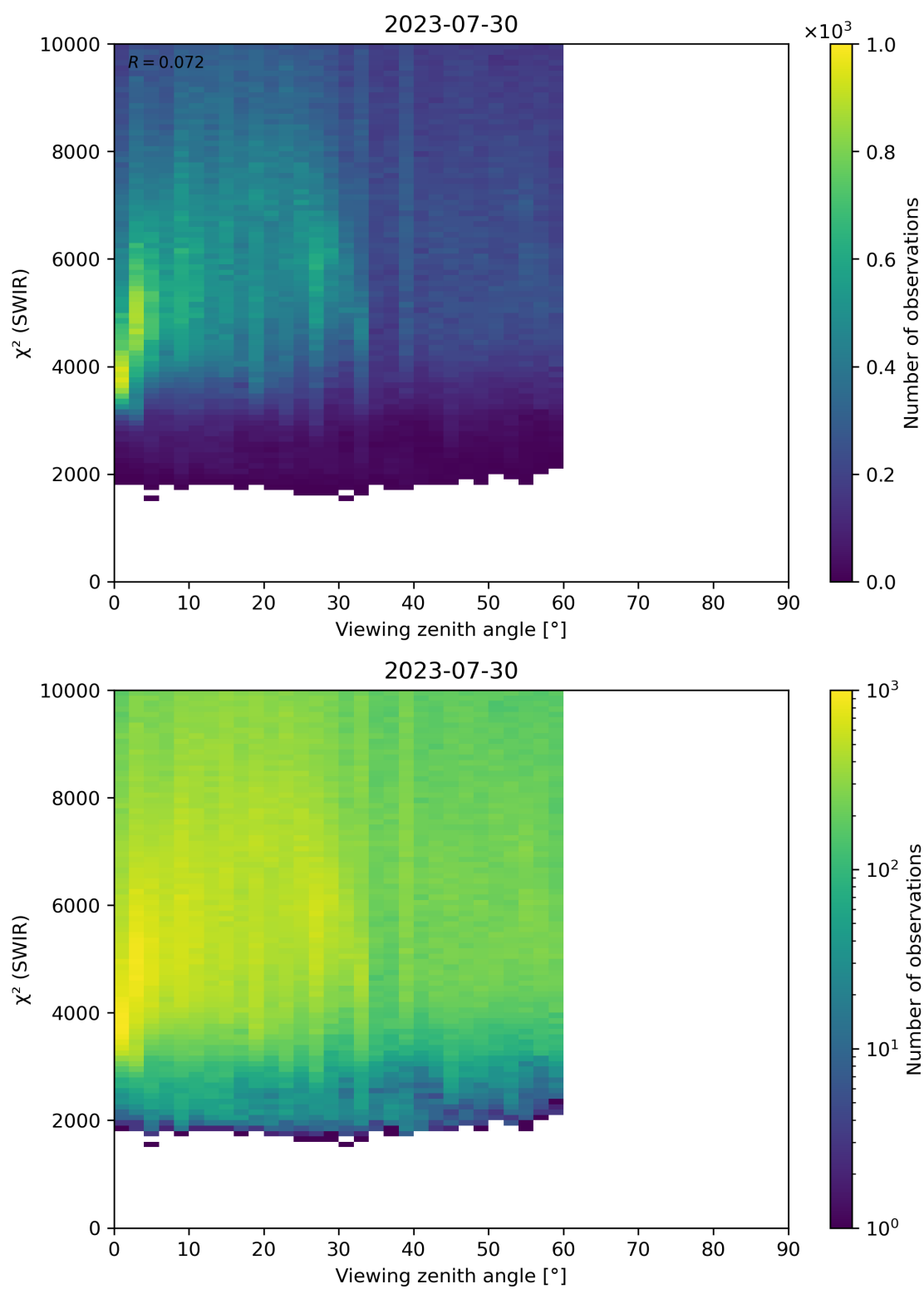
Figure 106: Scatter density plot of “Viewing zenith angle” against “ \chi^2 (SWIR)” for 2023-07-29 to 2023-07-31.
