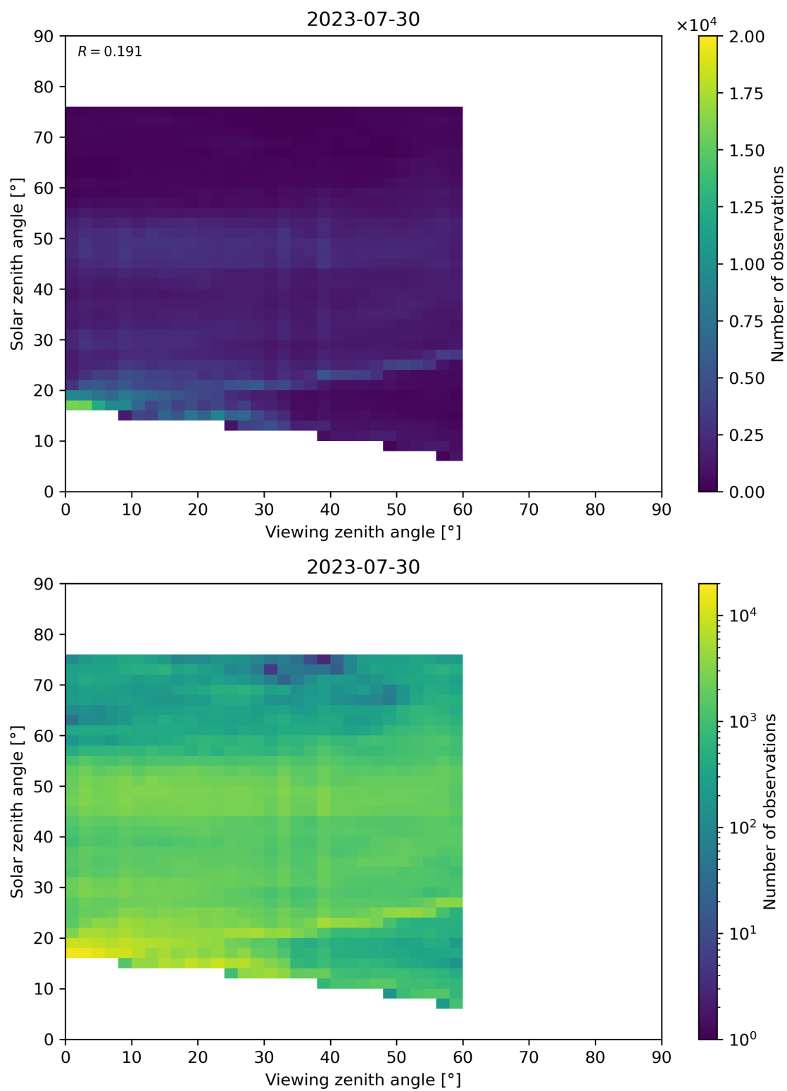
Figure 115: Scatter density plot of “Viewing zenith angle” against “Solar zenith angle” for 2023-07-29 to 2023-07-31.
