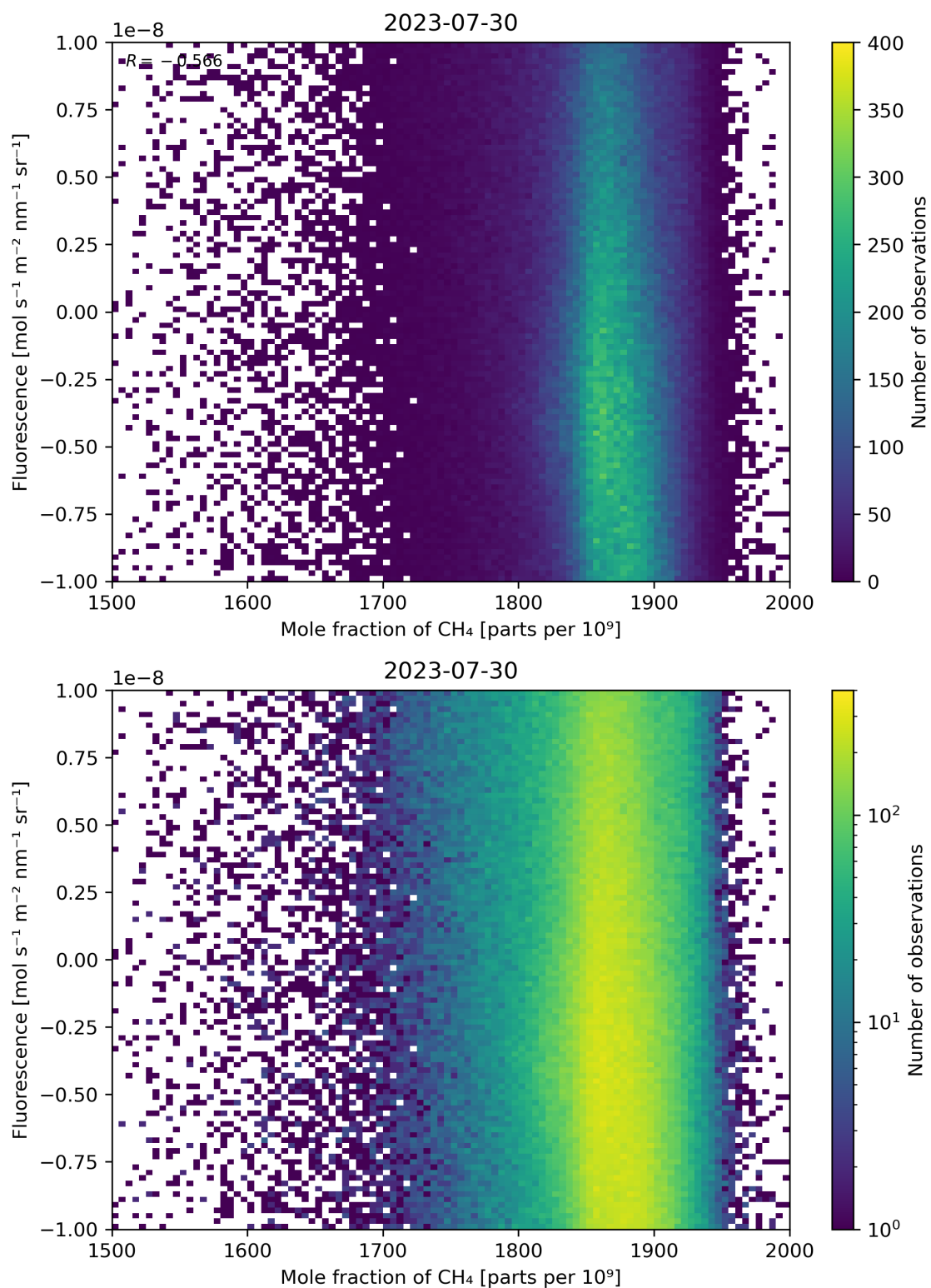
Figure 73: Scatter density plot of “Mole fraction of \text{CH}_4 ” against “Fluorescence” for 2023-07-29 to 2023-07-31.
