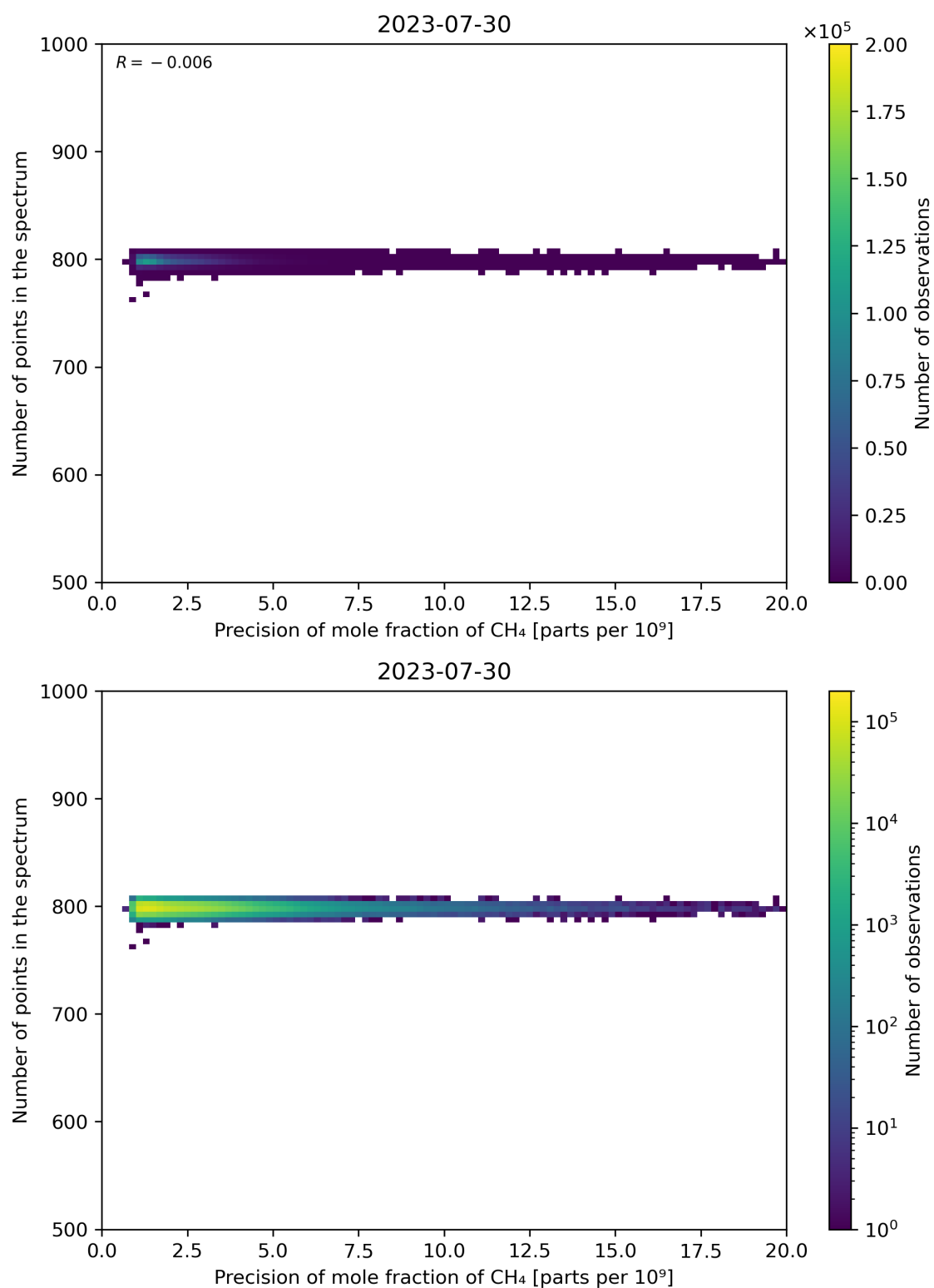
Figure 84: Scatter density plot of “Precision of mole fraction of CH 4 ” against “Number of points in the spectrum” for 2023-07-29 to 2023-07-31.
