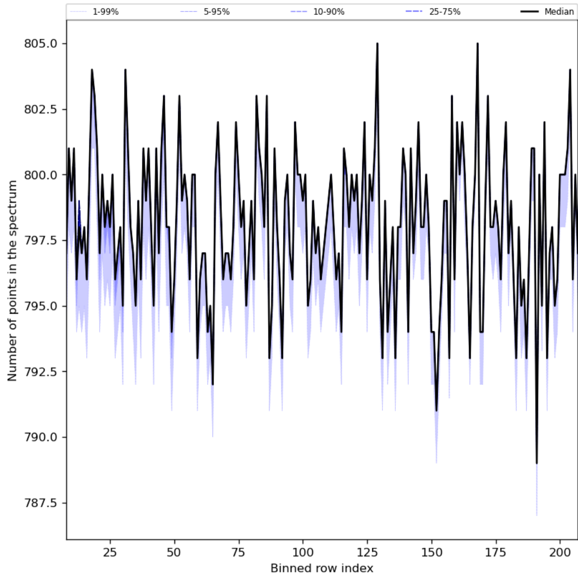
Figure 37: Along track statistics of “Number of points in the spectrum” for 2023-07-29 to 2023-07-31
