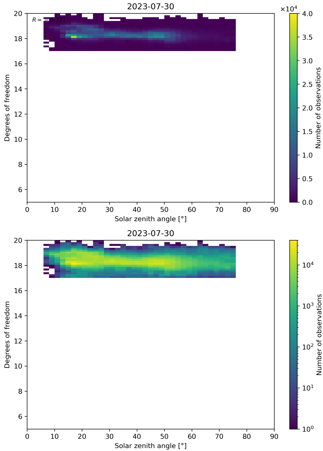
Figure 96: Scatter density plot of “Solar zenith angle” against “Degrees of freedom” for 2023-07-29 to 2023-07-31.
