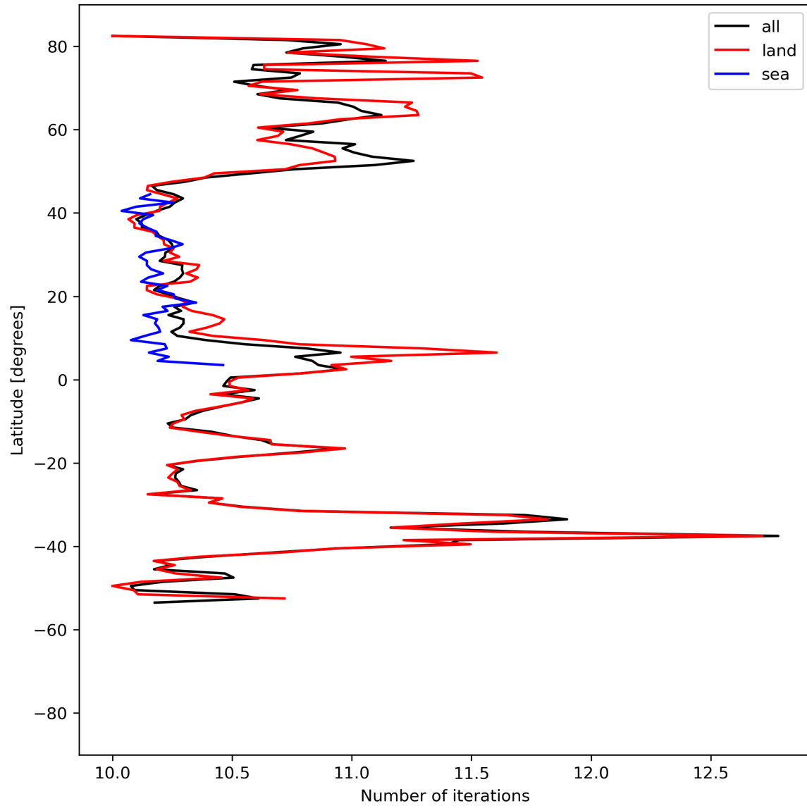
Figure 20: Zonal average of “Number of iterations” for 2023-07-29 to 2023-07-31.
