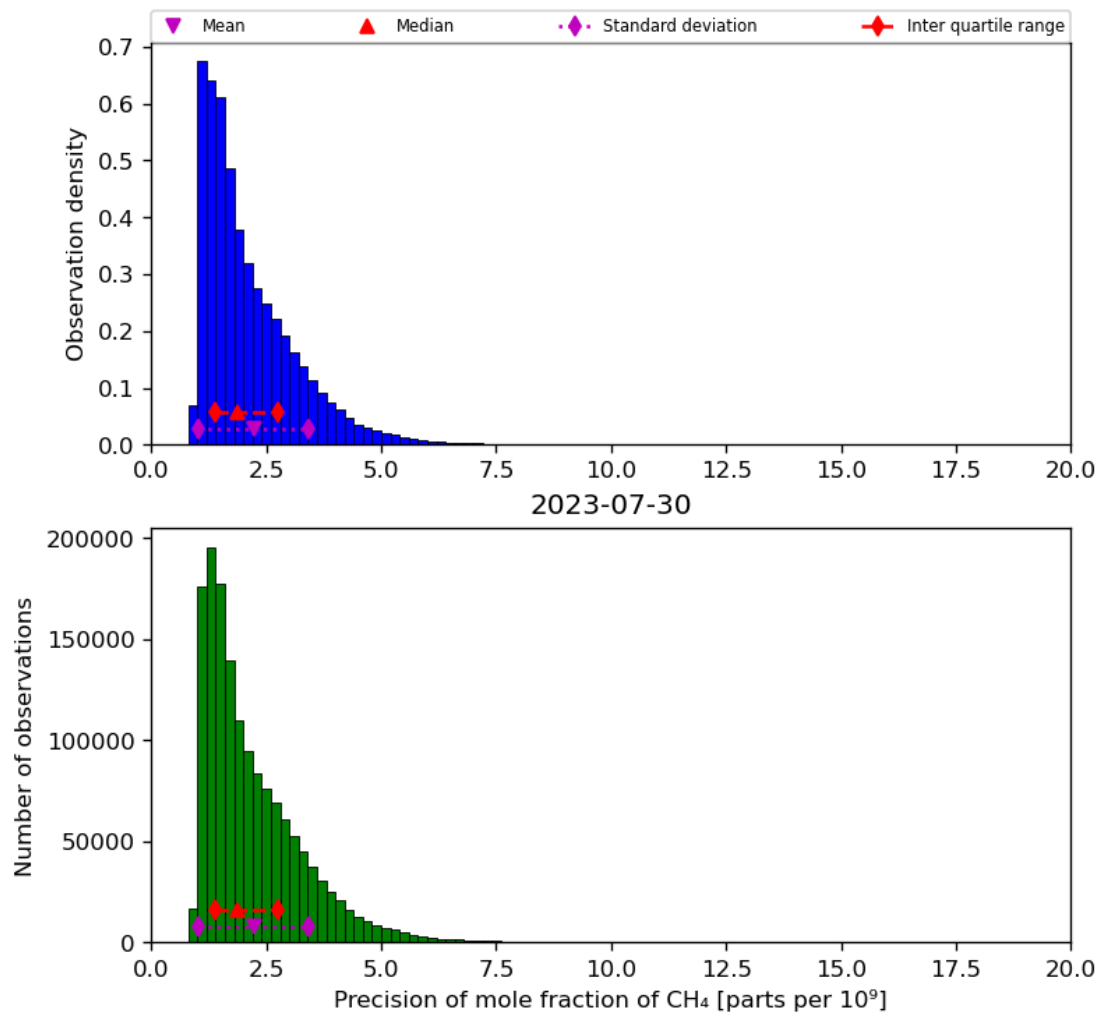
Figure 24: Histogram of “Precision of mole fraction of CH 4 ” for 2023-07-29 to 2023-07-31
