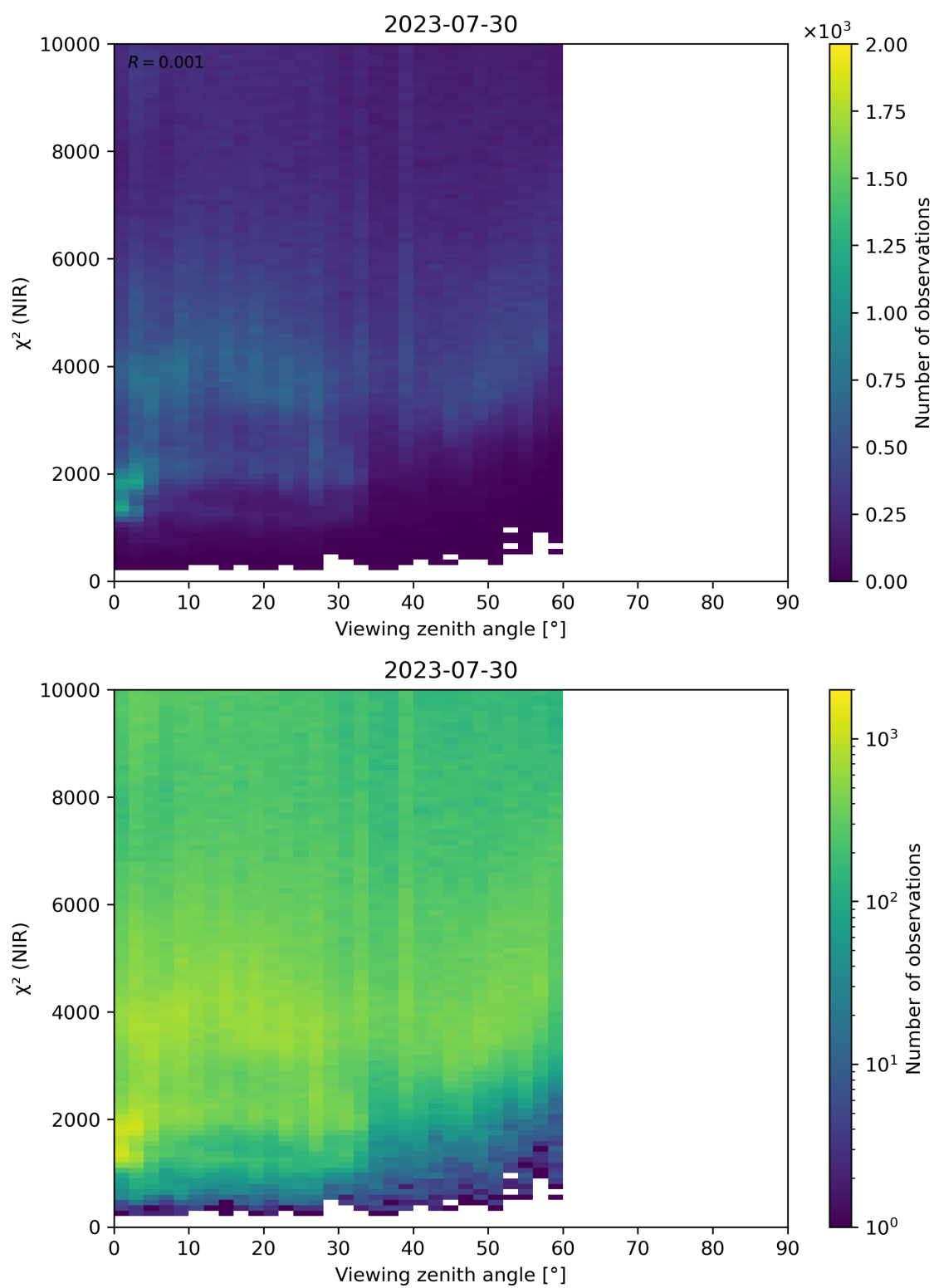
Figure 105: Scatter density plot of “Viewing zenith angle” against “ \chi^2 (NIR)” for 2023-07-29 to 2023-07-31.
