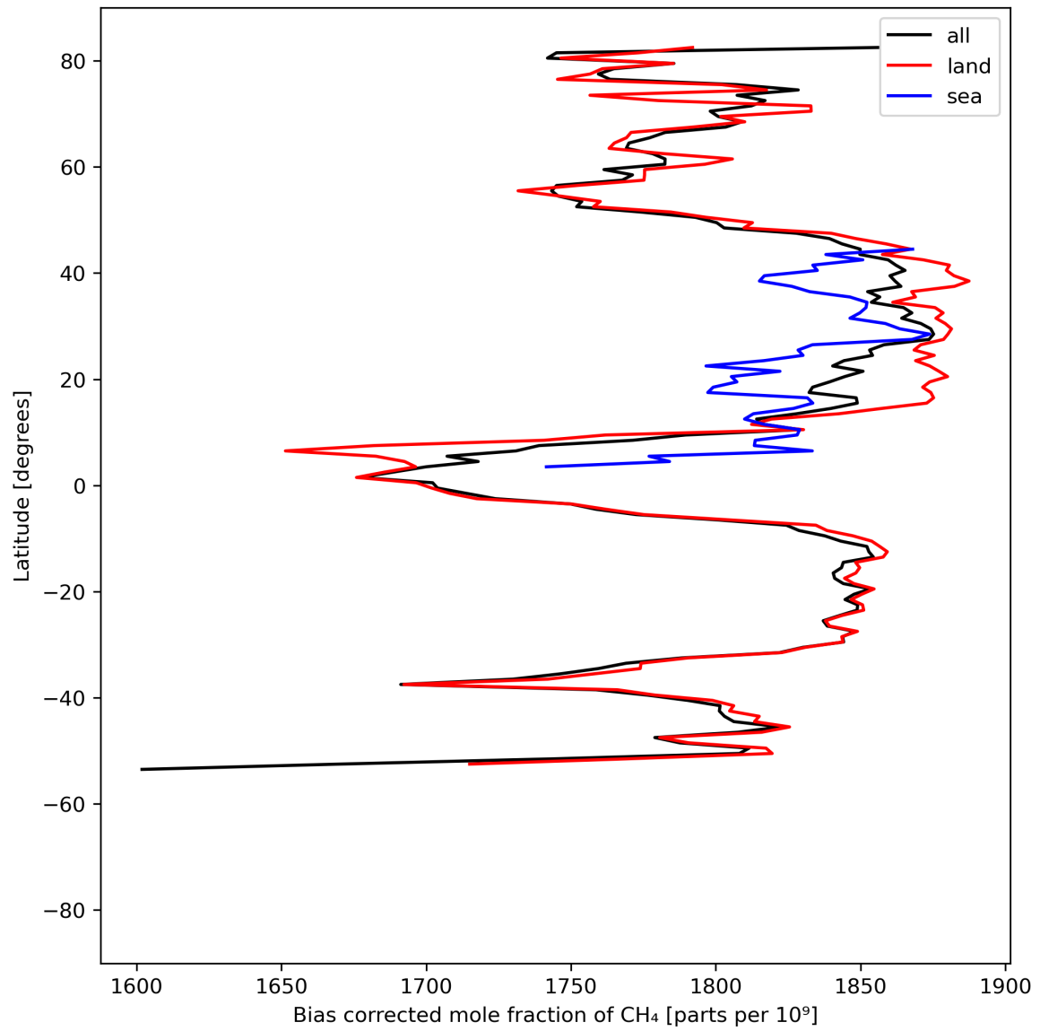
Figure 14: Zonal average of “Bias corrected mole fraction of \text{CH}_4 ” for 2023-07-29 to 2023-07-31.
