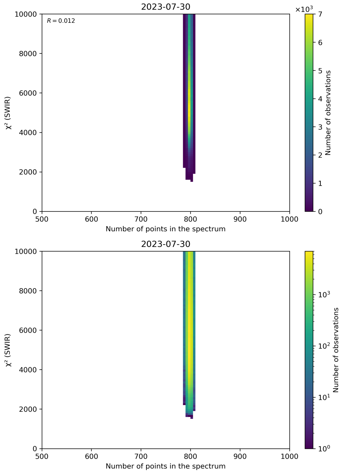
Figure 89: Scatter density plot of “Number of points in the spectrum” against “ \chi^2 (SWIR)” for 2023-07-29 to 2023-07-31.
