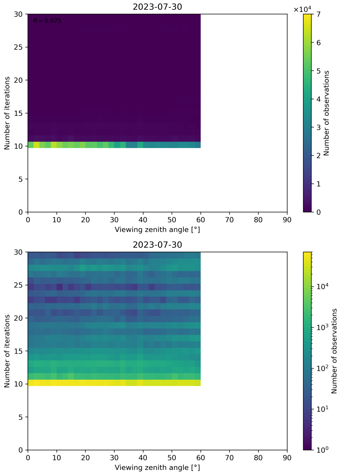
Figure 113: Scatter density plot of “Viewing zenith angle” against “Number of iterations” for 2023-07-29 to 2023-07-31.
