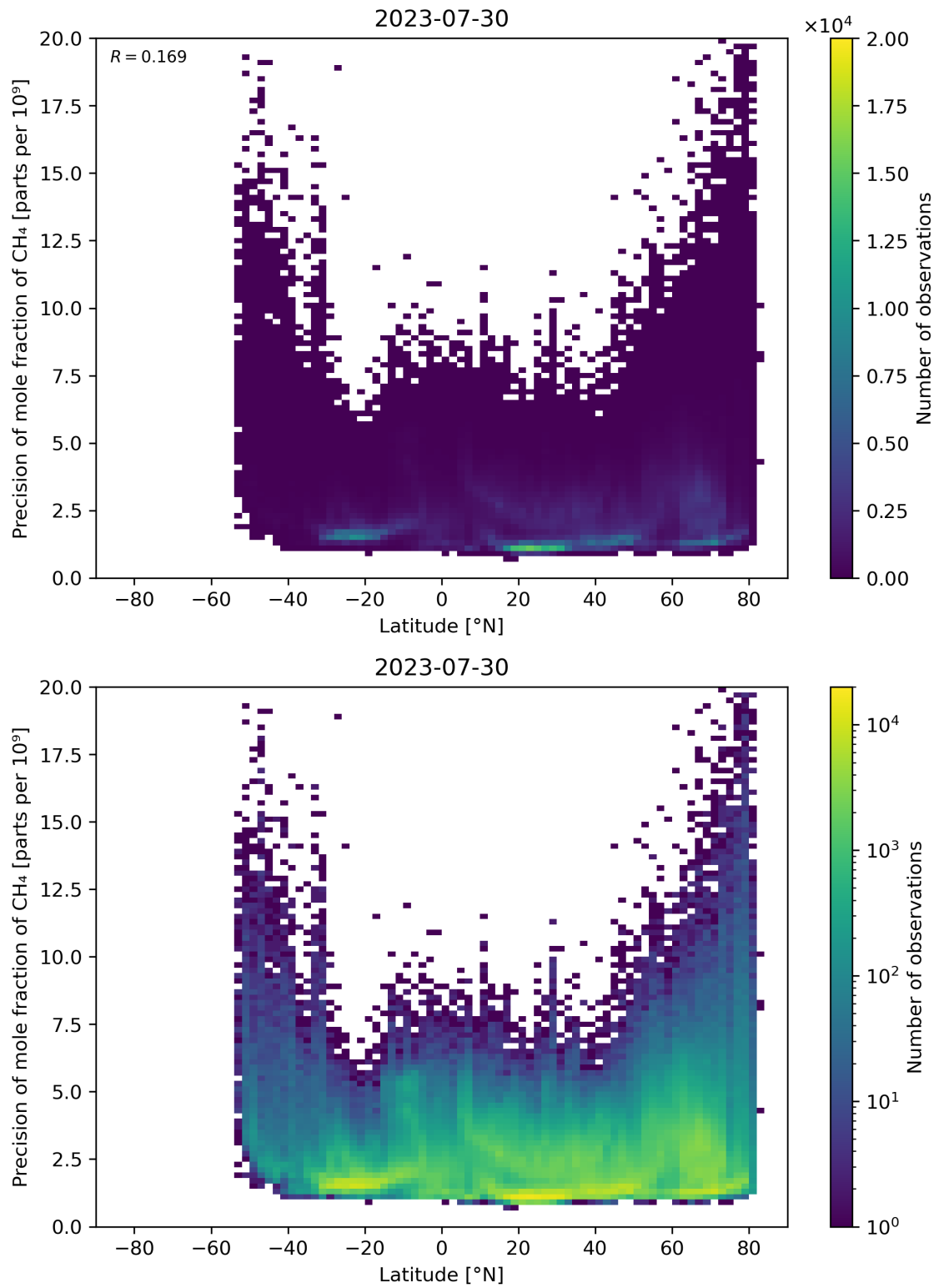
Figure 59: Scatter density plot of “Latitude” against “Precision of mole fraction of \text{CH}_4 ” for 2023-07-29 to 2023-07-31.
