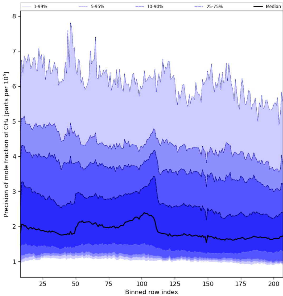
Figure 35: Along track statistics of “Precision of mole fraction of CH 4 ” for 2023-07-29 to 2023-07-31
