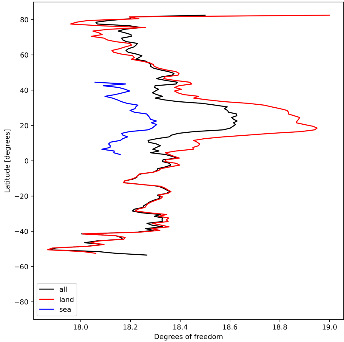
Figure 19: Zonal average of “Degrees of freedom” for 2023-07-29 to 2023-07-31.
