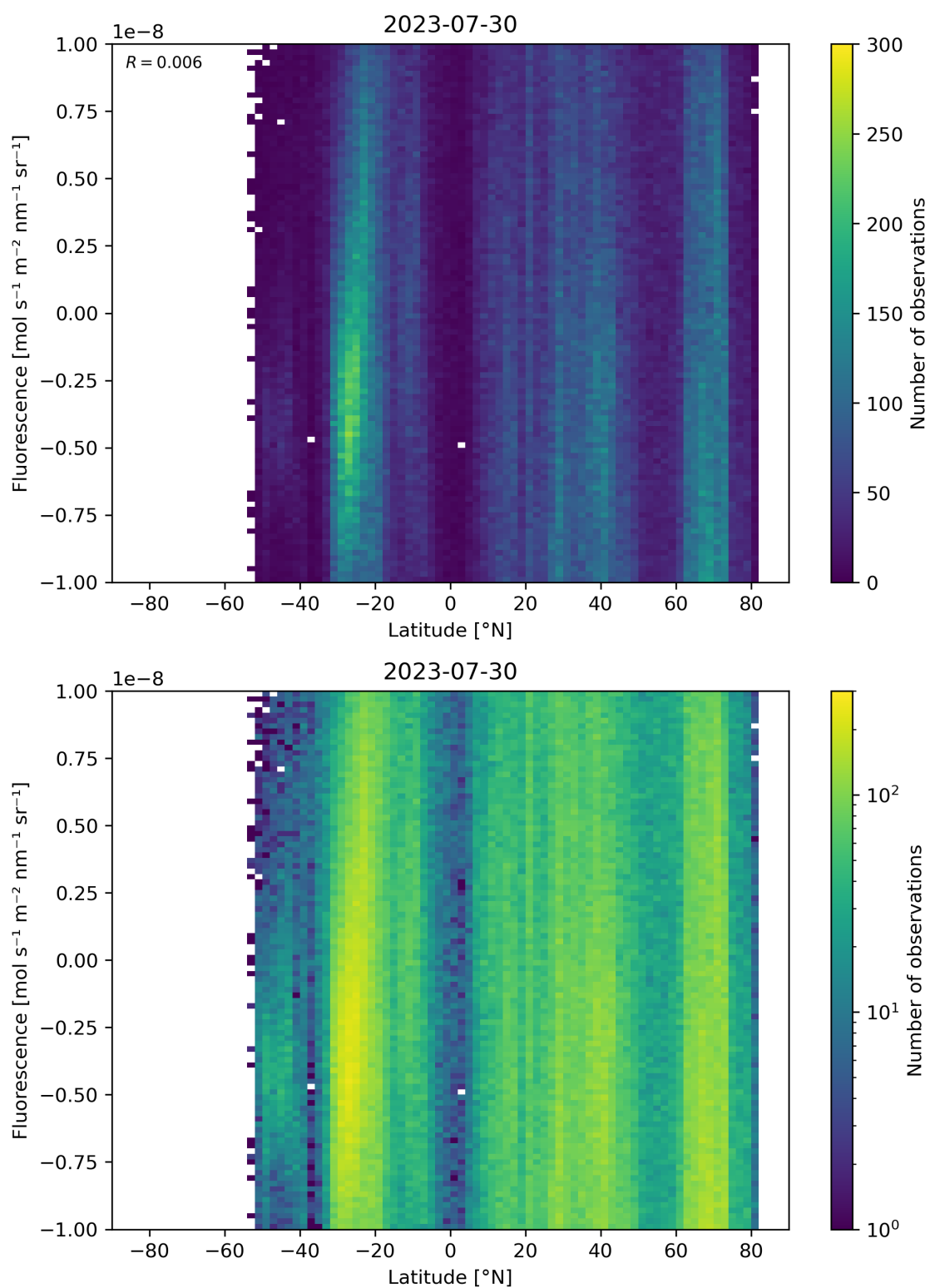
Figure 56: Scatter density plot of “Latitude” against “Fluorescence” for 2023-07-29 to 2023-07-31.
