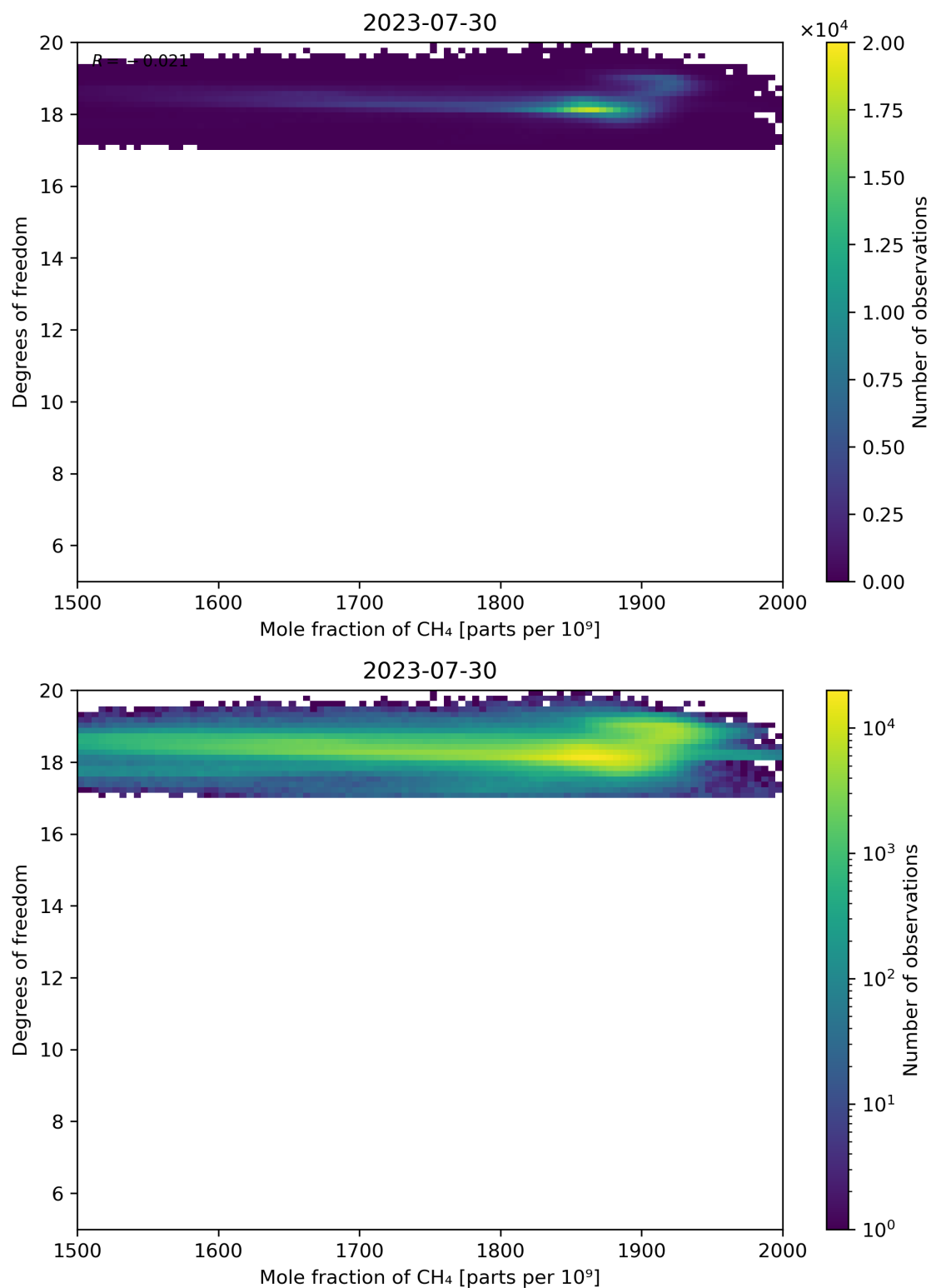
Figure 72: Scatter density plot of “Mole fraction of CH 4 ” against “Degrees of freedom” for 2023-07-29 to 2023-07-31.
