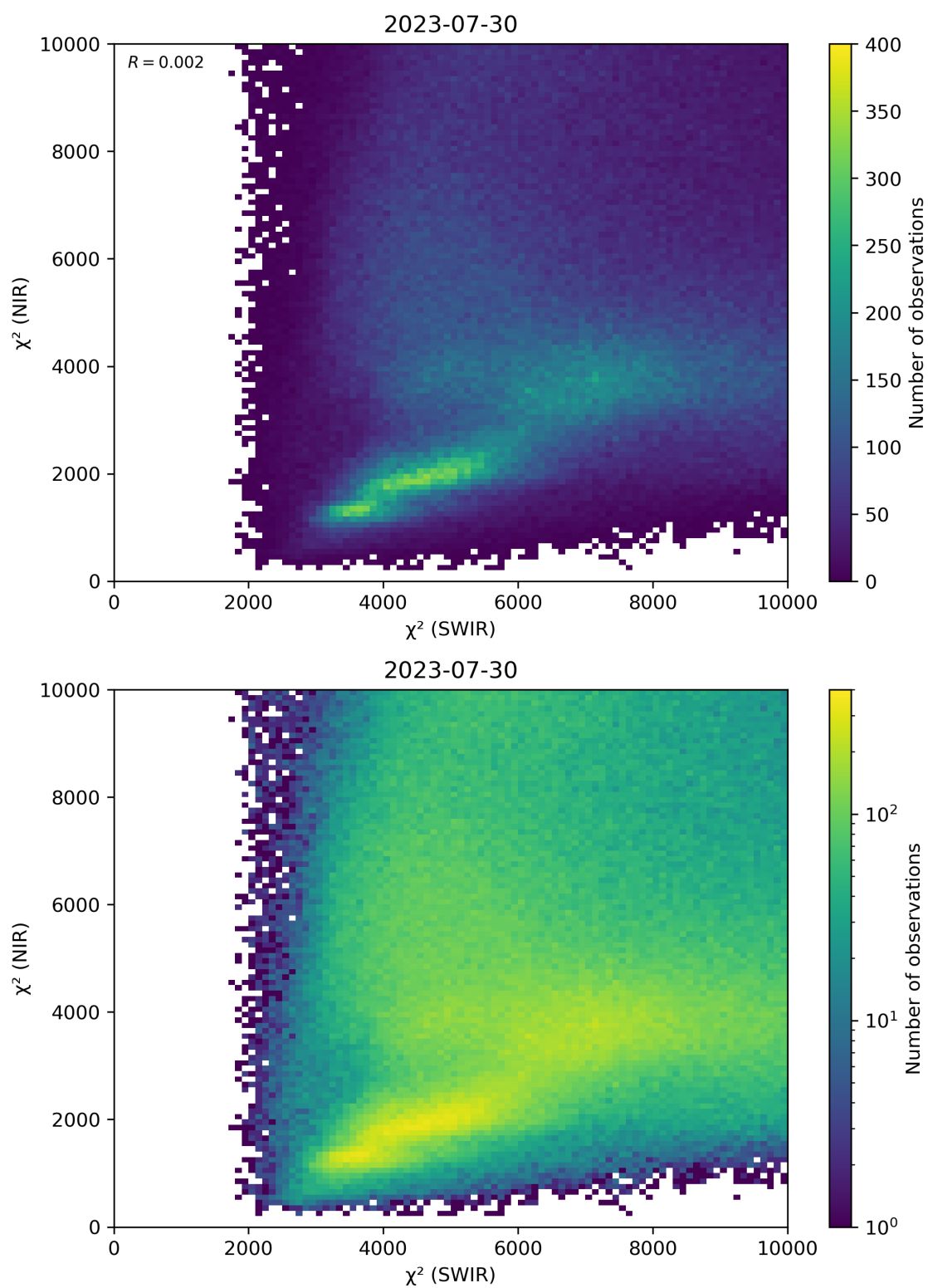
Figure 47: Scatter density plot of “ \chi^2 (SWIR)” against “ \chi^2 (NIR)” for 2023-07-29 to 2023-07-31.
