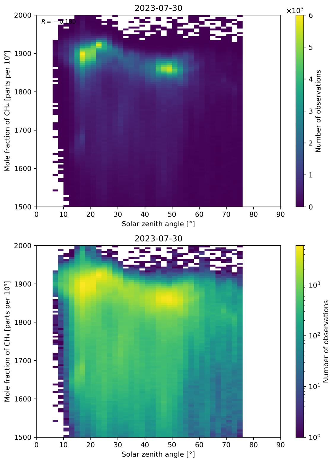
Figure 99: Scatter density plot of “Solar zenith angle” against “Mole fraction of \text{CH}_4 ” for 2023-07-29 to 2023-07-31.
