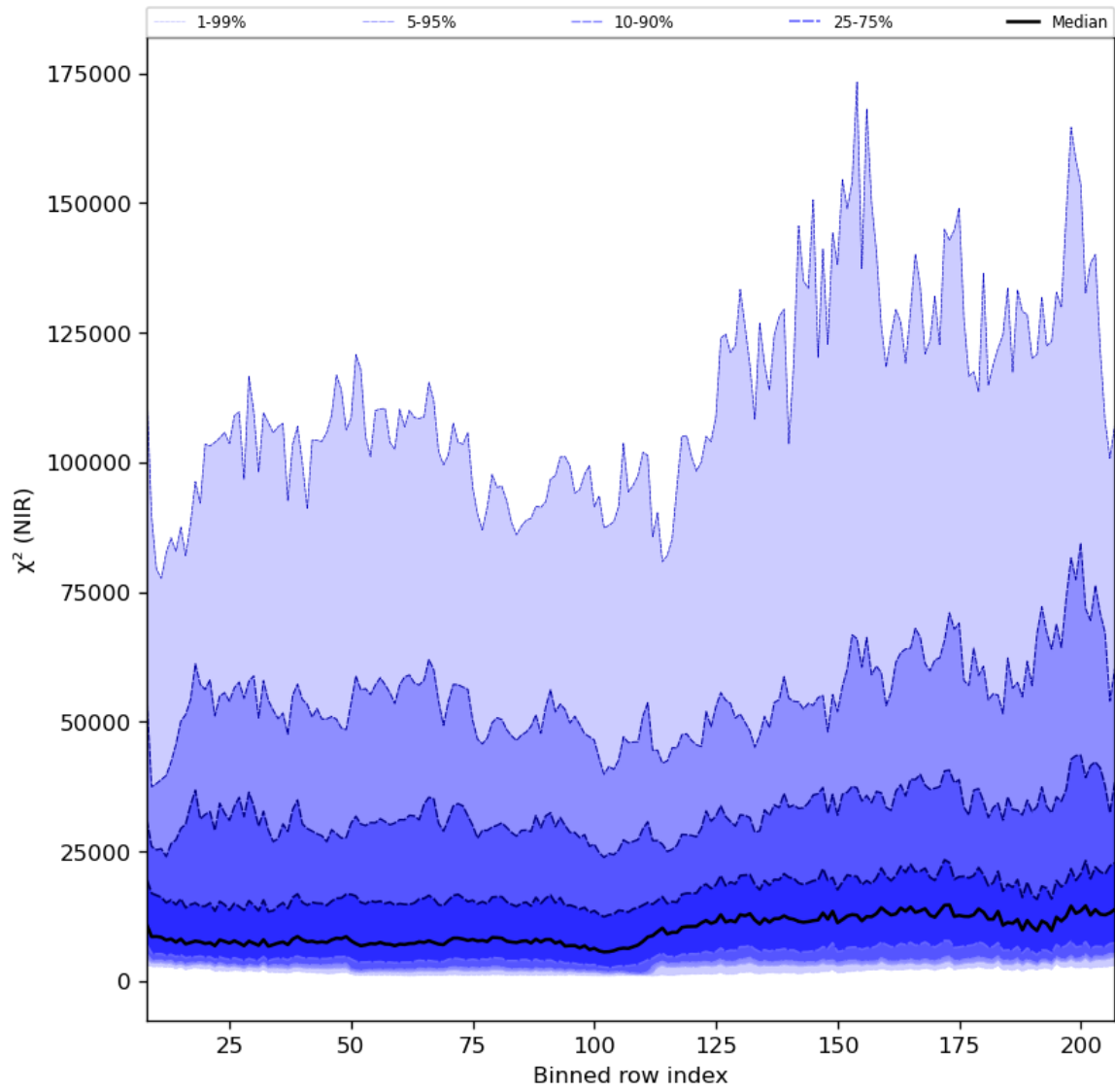
Figure 40: Along track statistics of " \chi^2 (NIR)" for 2023-07-29 to 2023-07-31
