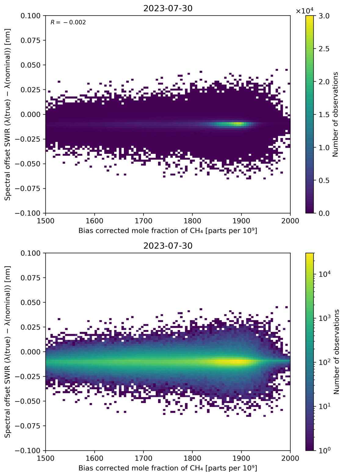
Figure 69: Scatter density plot of “Bias corrected mole fraction of \text{CH}_4 ” against “Spectral offset SWIR ( \lambda(\text{true}) - \lambda(\text{nominal}) )” for 2023-07-29 to 2023-07-31.
