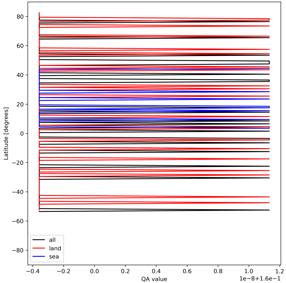
Figure 11: Zonal average of “QA value” for 2023-07-29 to 2023-07-31.
