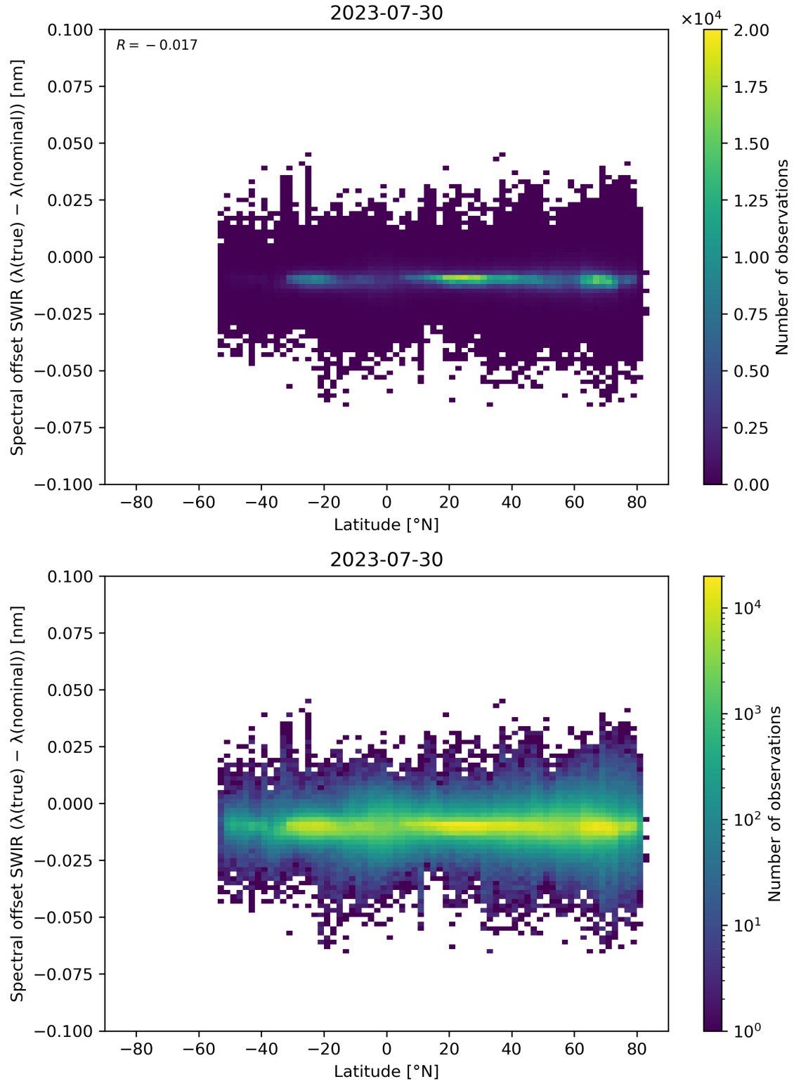
Figure 62: Scatter density plot of “Latitude” against “Spectral offset SWIR ( \lambda(\text{true}) - \lambda(\text{nominal}) )” for 2023-07-29 to 2023-07-31.
